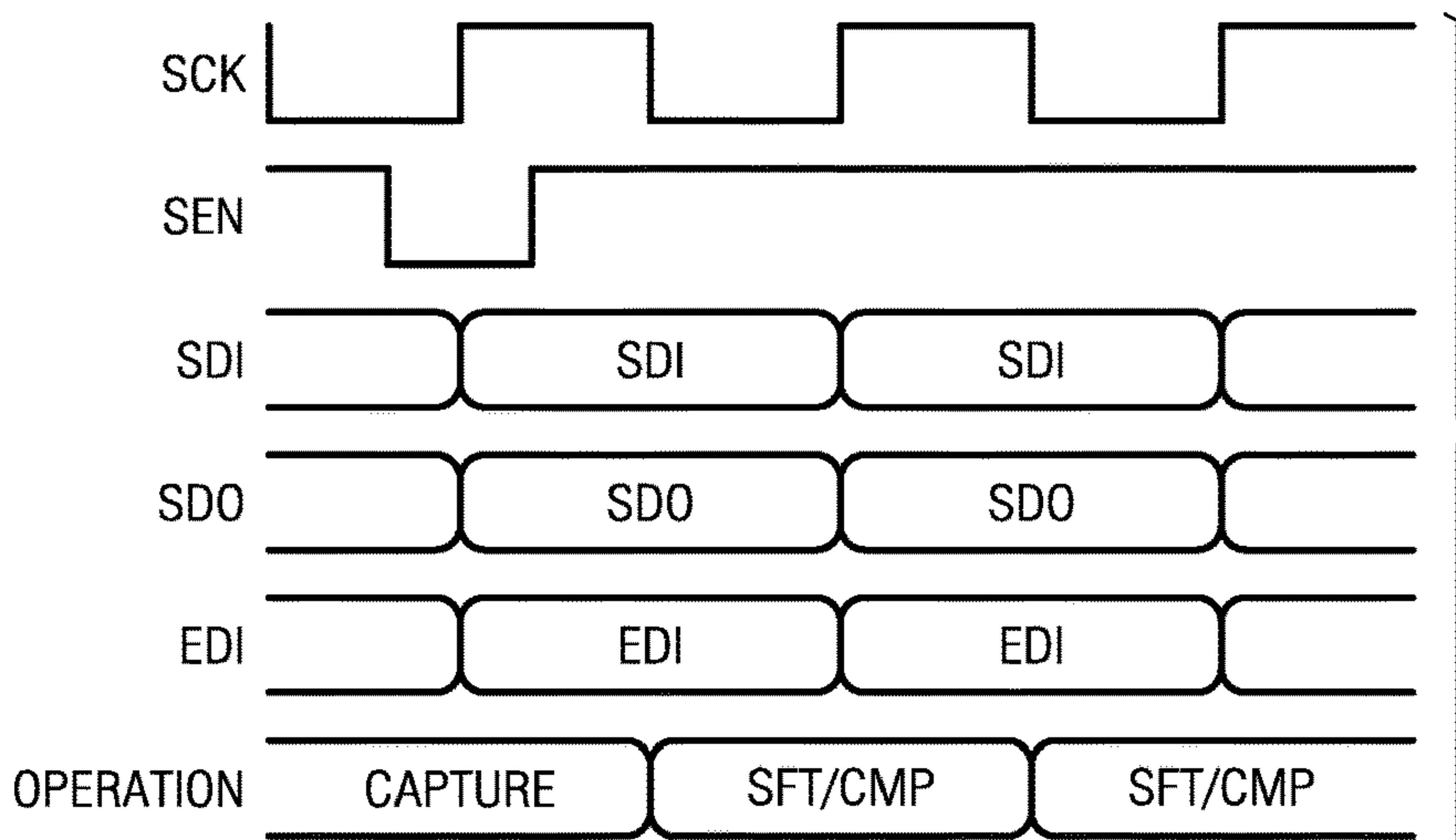
FIG. 4C (PRIOR ART)
