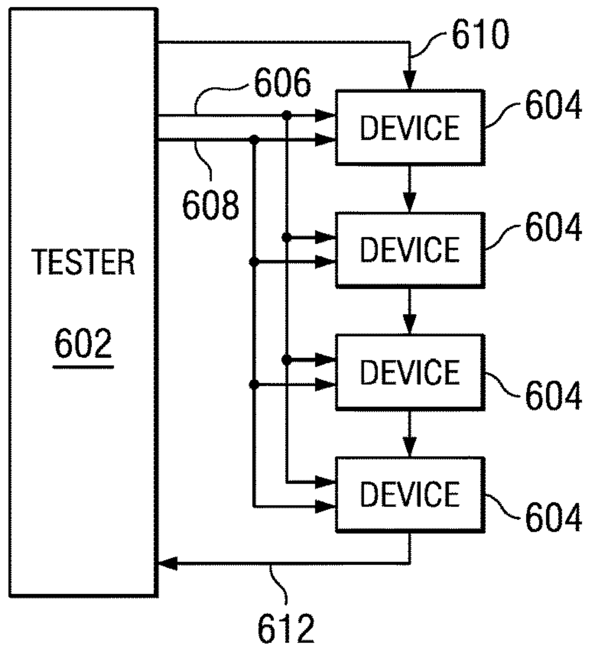
FIG. 6 (PRIOR ART)
