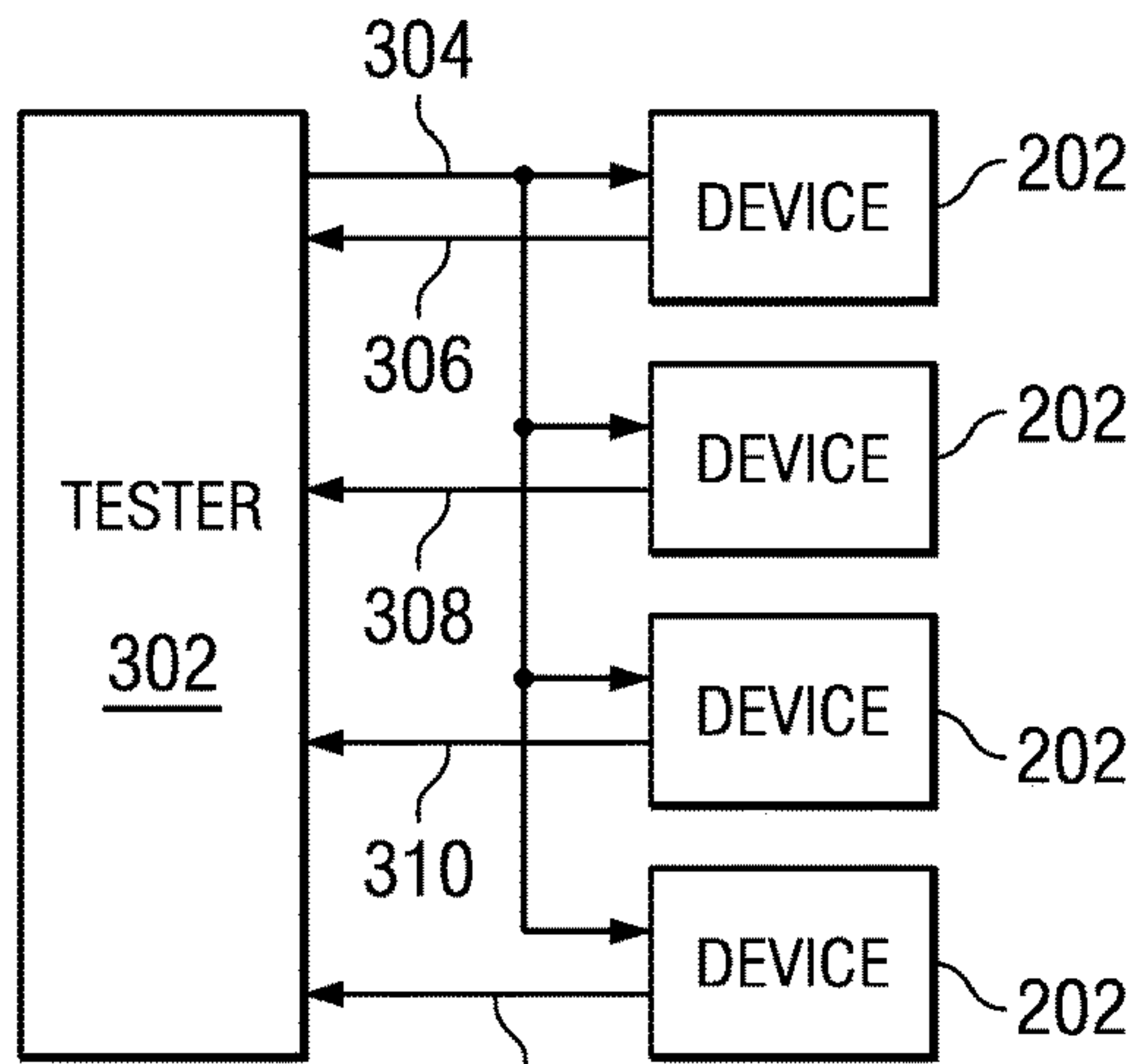
FIG. 3 (PRIOR ART)
