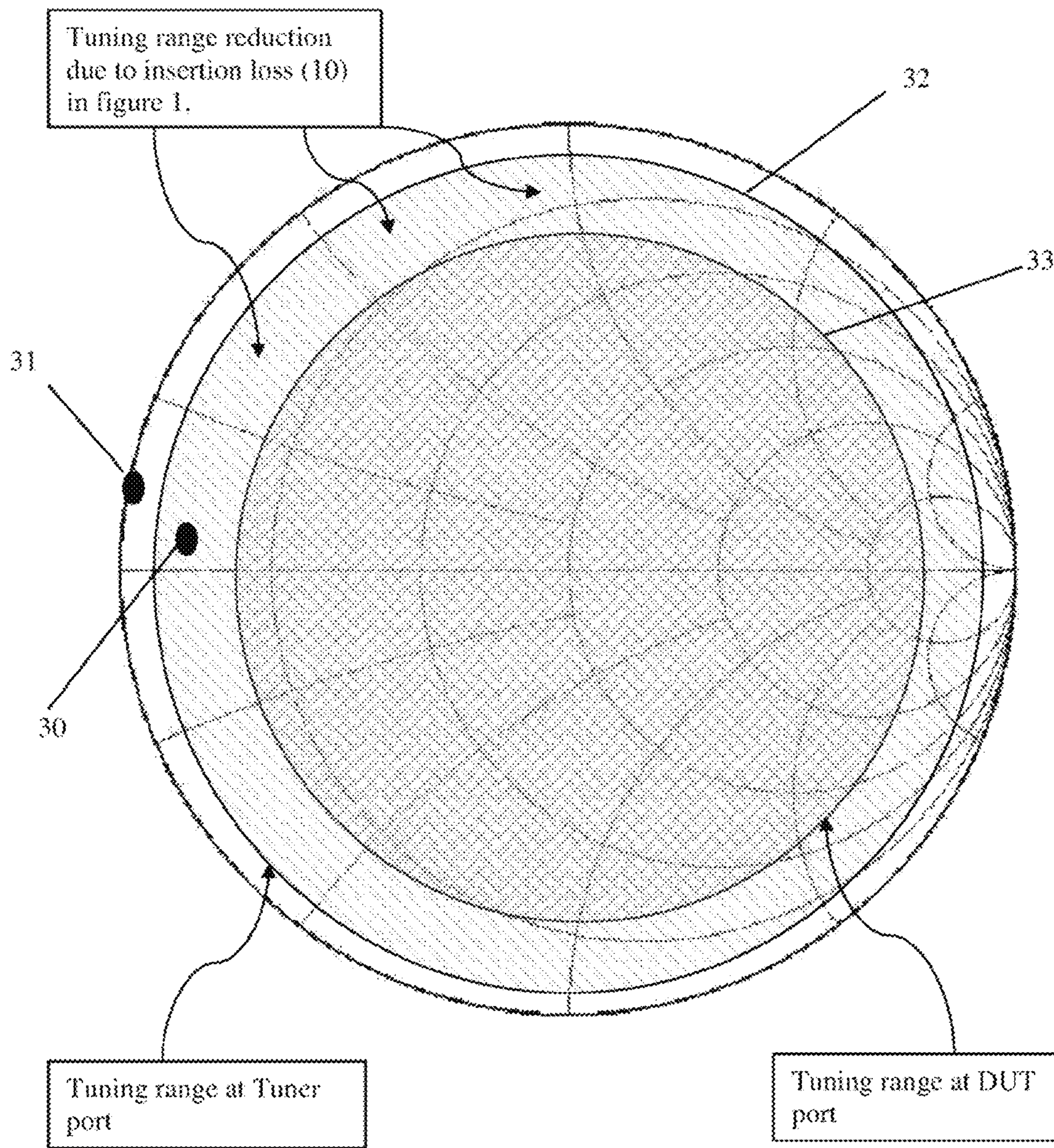
FIG. 3: Prior art
