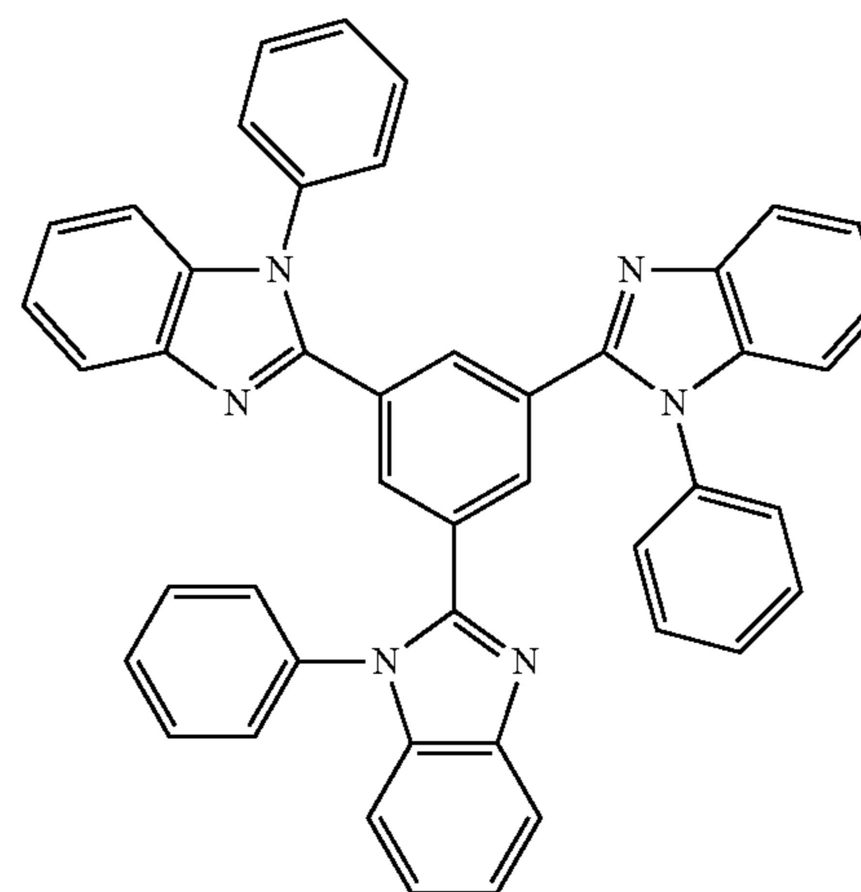
TPBI 2,2',2''-(1,3,5-benzenetriyl)tris (1-phenyl-1H-benzimidazole)
