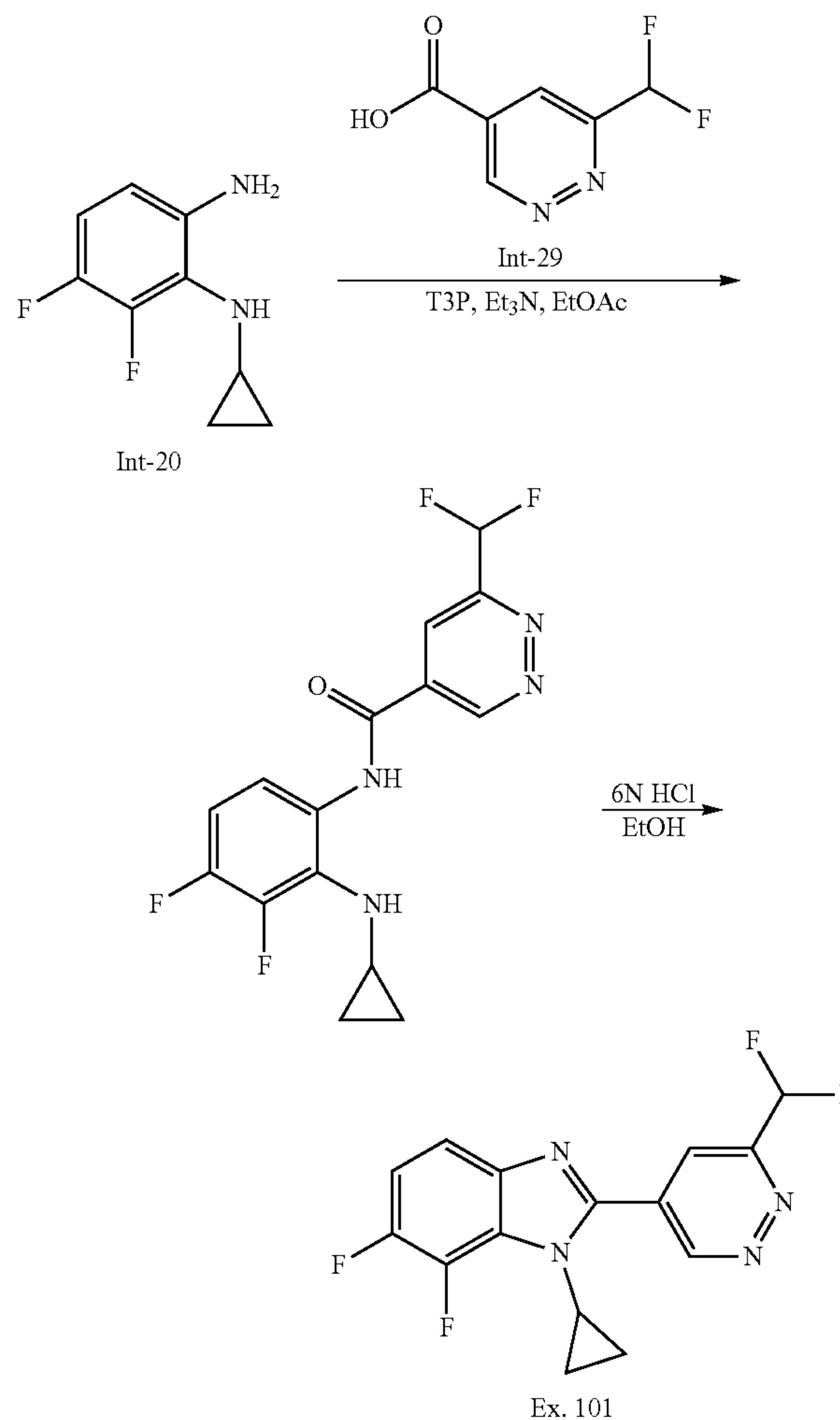
N-(2-(Cyclopropylamino)-3,4-difluorophenyl)-6-(difluoromethyl)pyridazine-4-carboxamide
