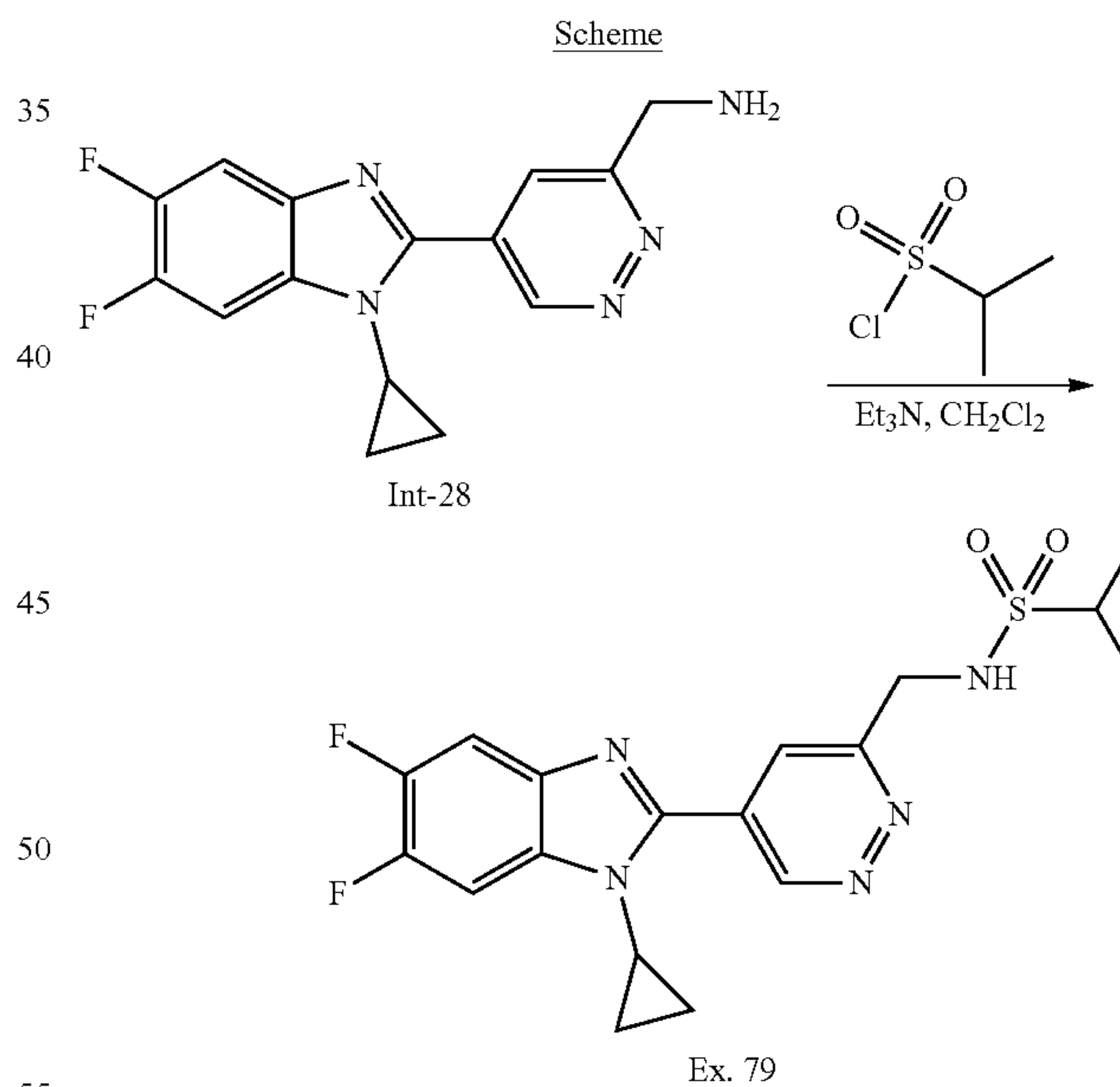
N-((5-(1-Cyclopropyl-5,6-difluoro-1H-benzo[d]imidazol-2-yl)pyridazin-3-yl)methyl)propane-2-sulfonamide (Ex. 79)
