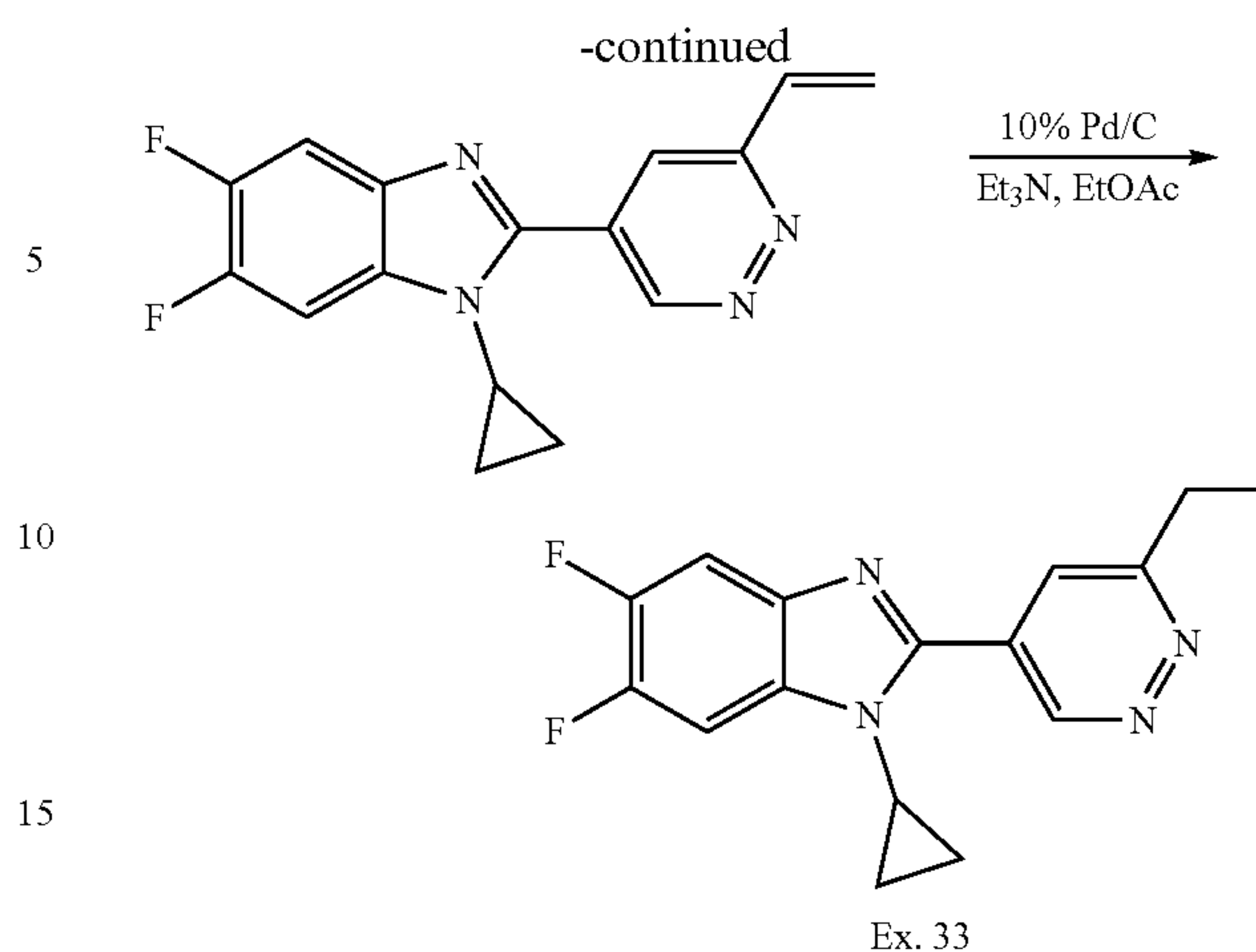
1-Cyclopropyl-5,6-difluoro-2-(6-vinylpyridazin-4-yl)-1H-benzo[d]imidazole
