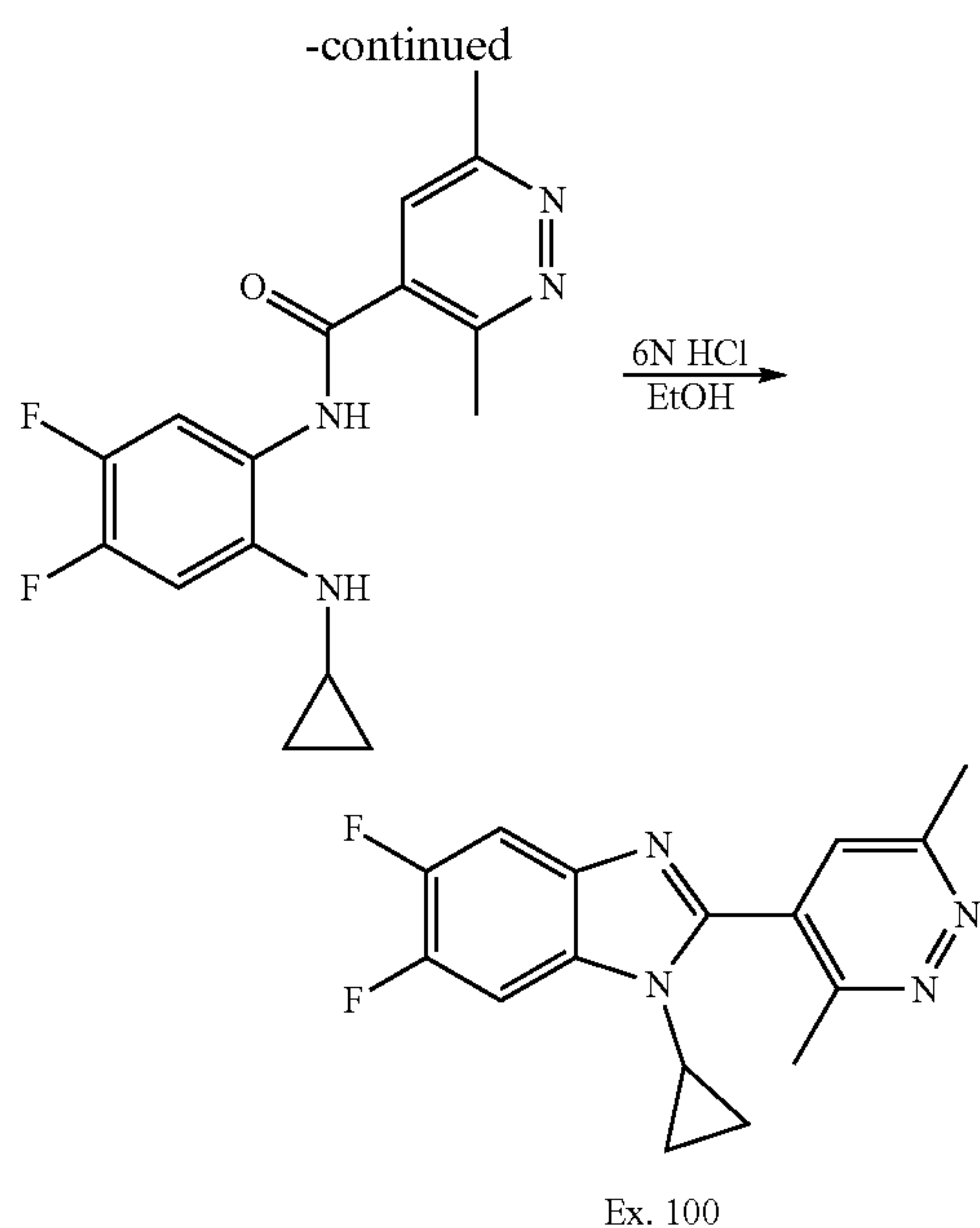
N-(2-(Cyclopropylamino)-4,5-difluorophenyl)-3,6-dimethylpyridazine-4-carboxamide
