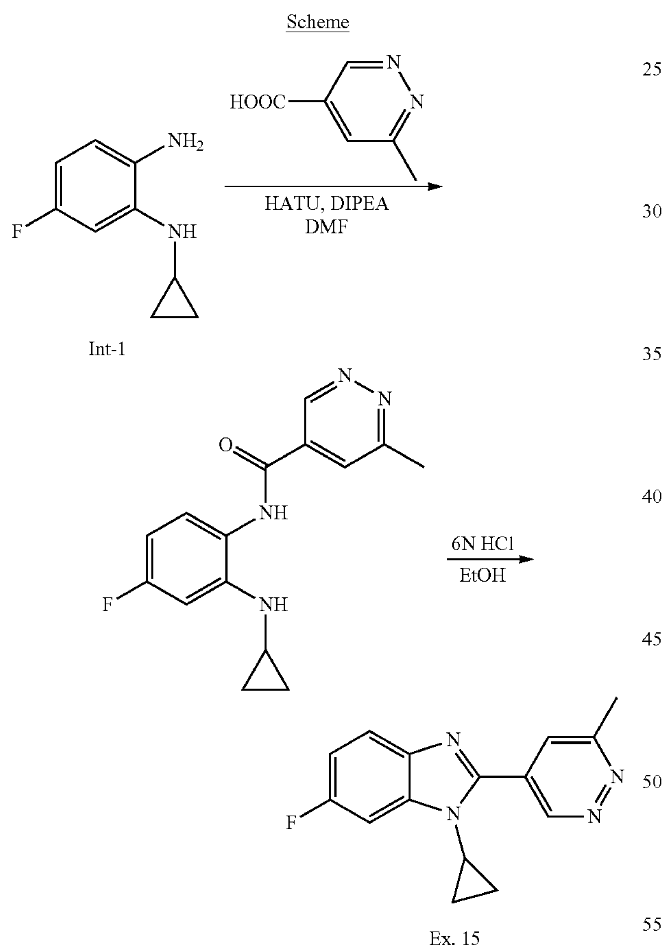
N-(2-(Cyclopropylamino)-4-fluorophenyl)-6-methylpyridazine-4-carboxamide
