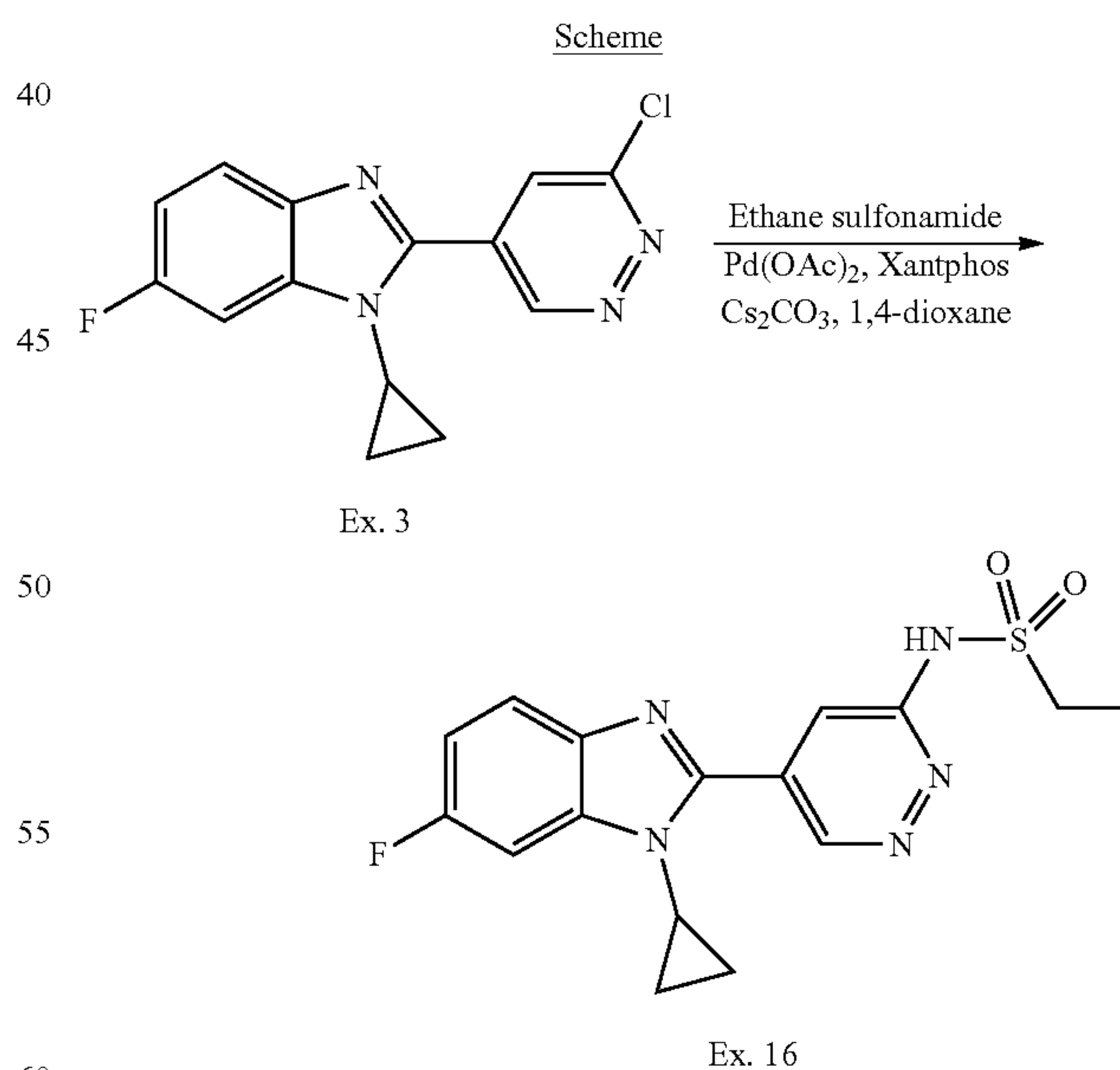
N-(5-(1-Cyclopropyl-6-fluoro-1H-benzo[d]imidazol-2-yl)pyridazin-3-yl)ethanesulfonamide (Ex. 16)
