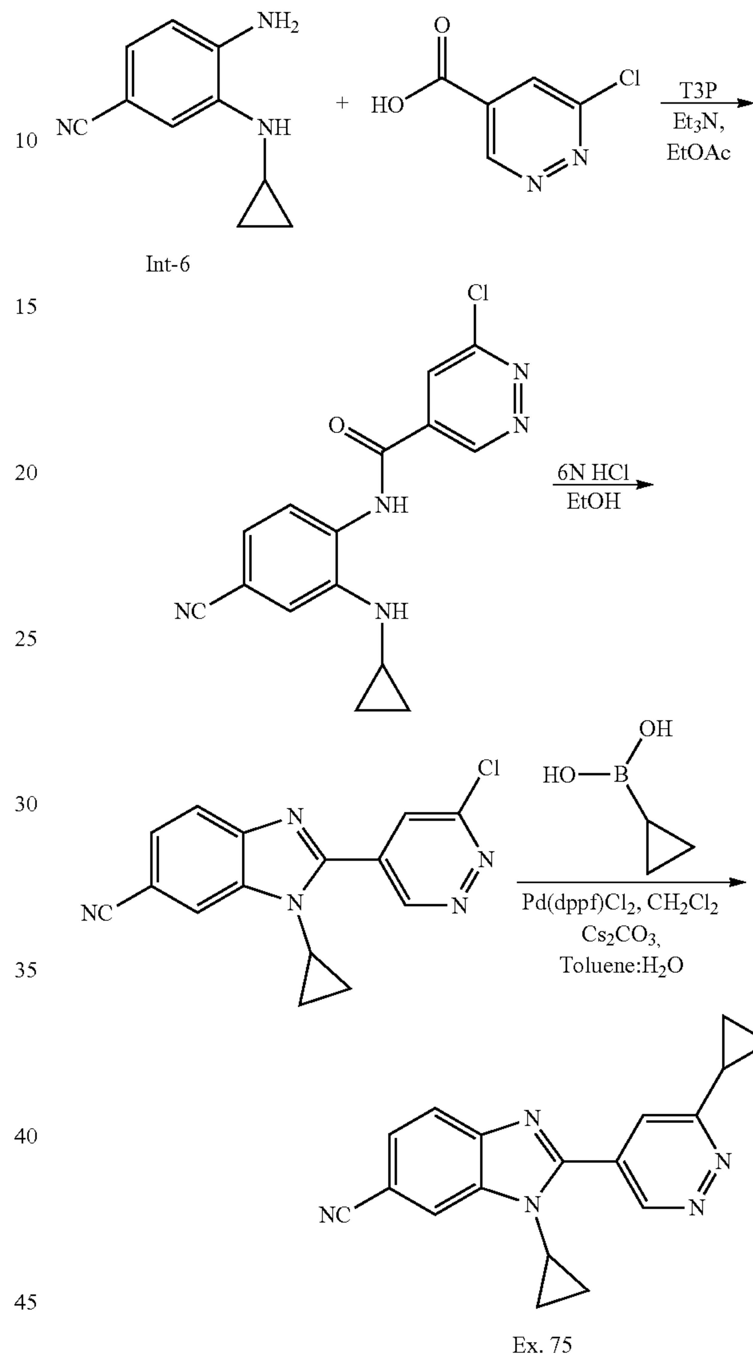
6-Chloro-N-(4-cyano-2-(cyclopropylamino)phenyl)pyridazine-4-carboxamide
