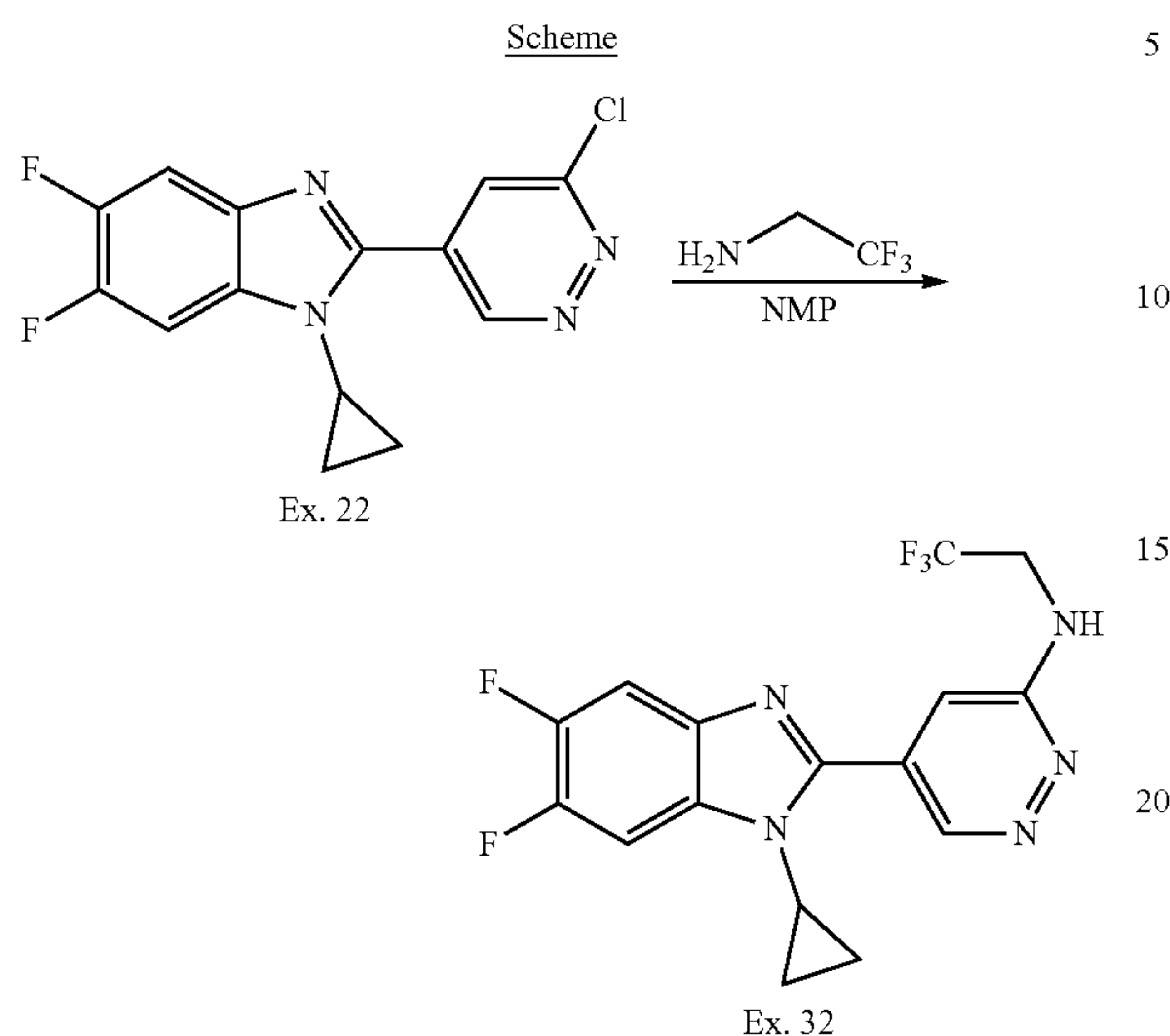
5-(1-Cyclopropyl-5,6-difluoro-1H-benzo[d]imidazol-2-yl)-N-(2,2,2-trifluoroethyl)pyridazin-3-amine (Ex. 32)
