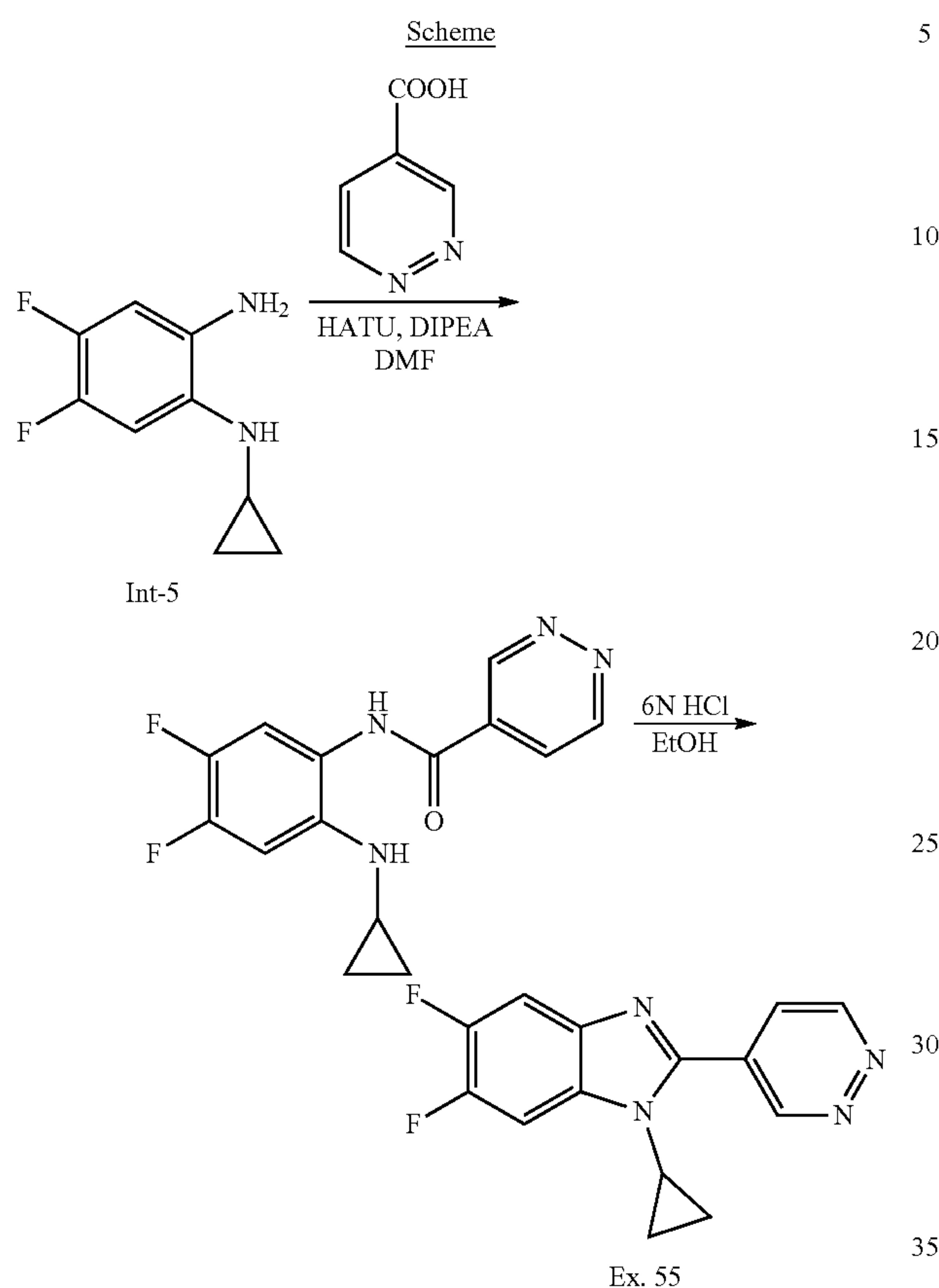
N-(2-(Cyclopropylamino)-4,5-difluorophenyl) pyridazine-4-carboxamide
