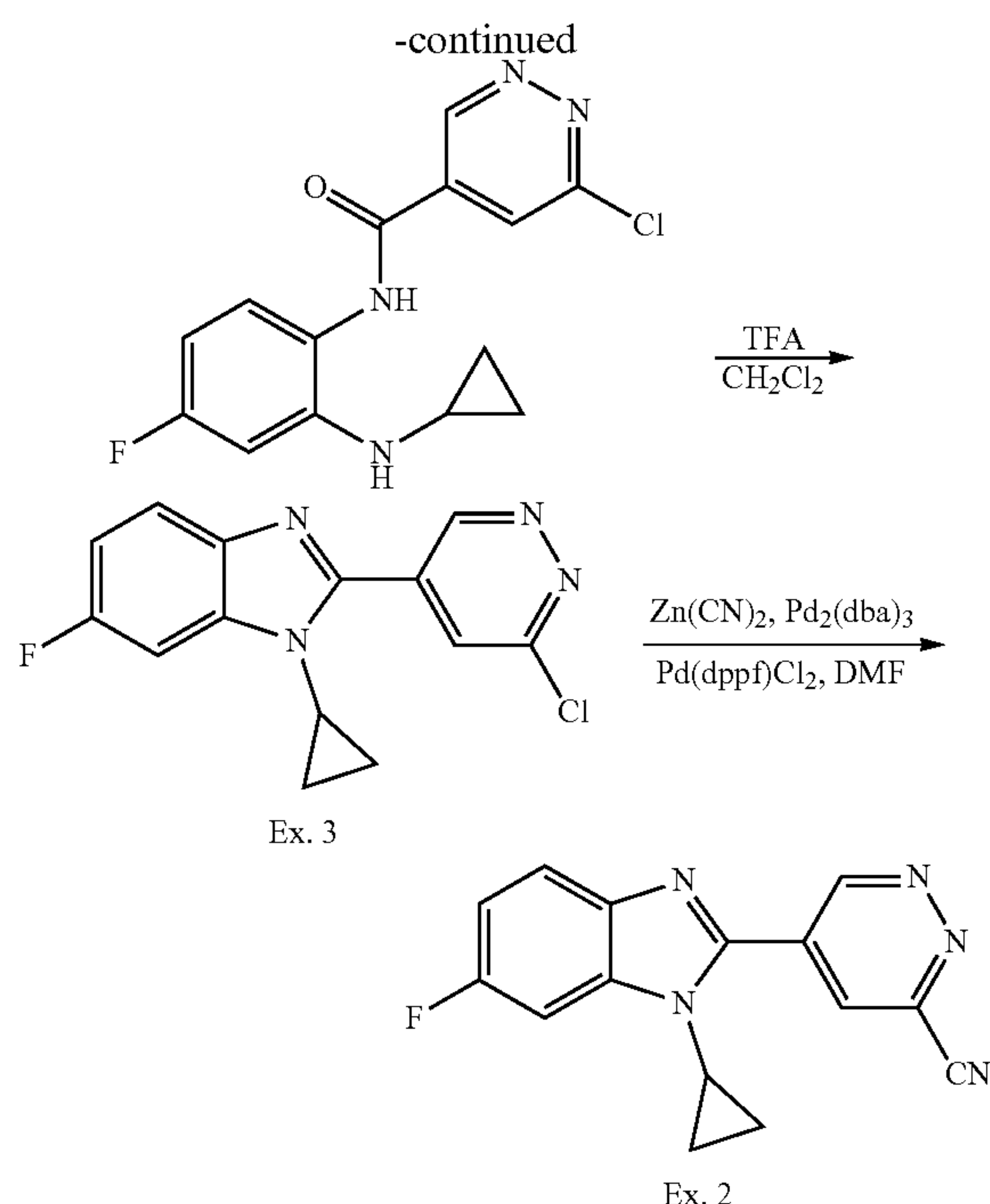
6-Chloro-N-(2-(cyclopropylamino)-4-fluorophenyl) pyridazine-4-carboxamide
