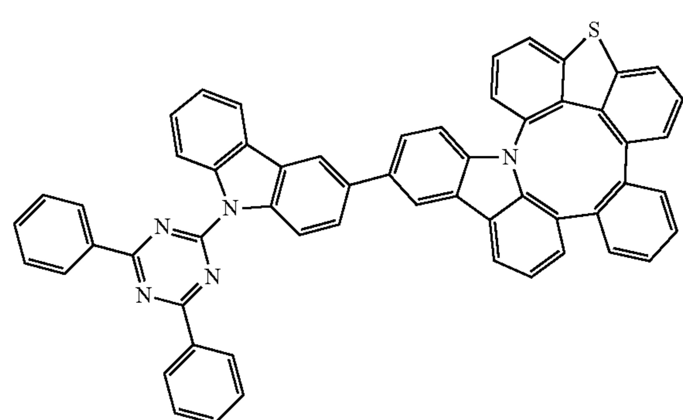
Compound 104
