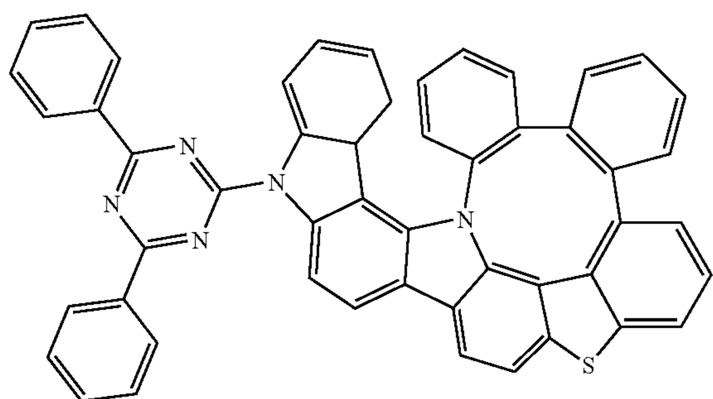
Compound 334
