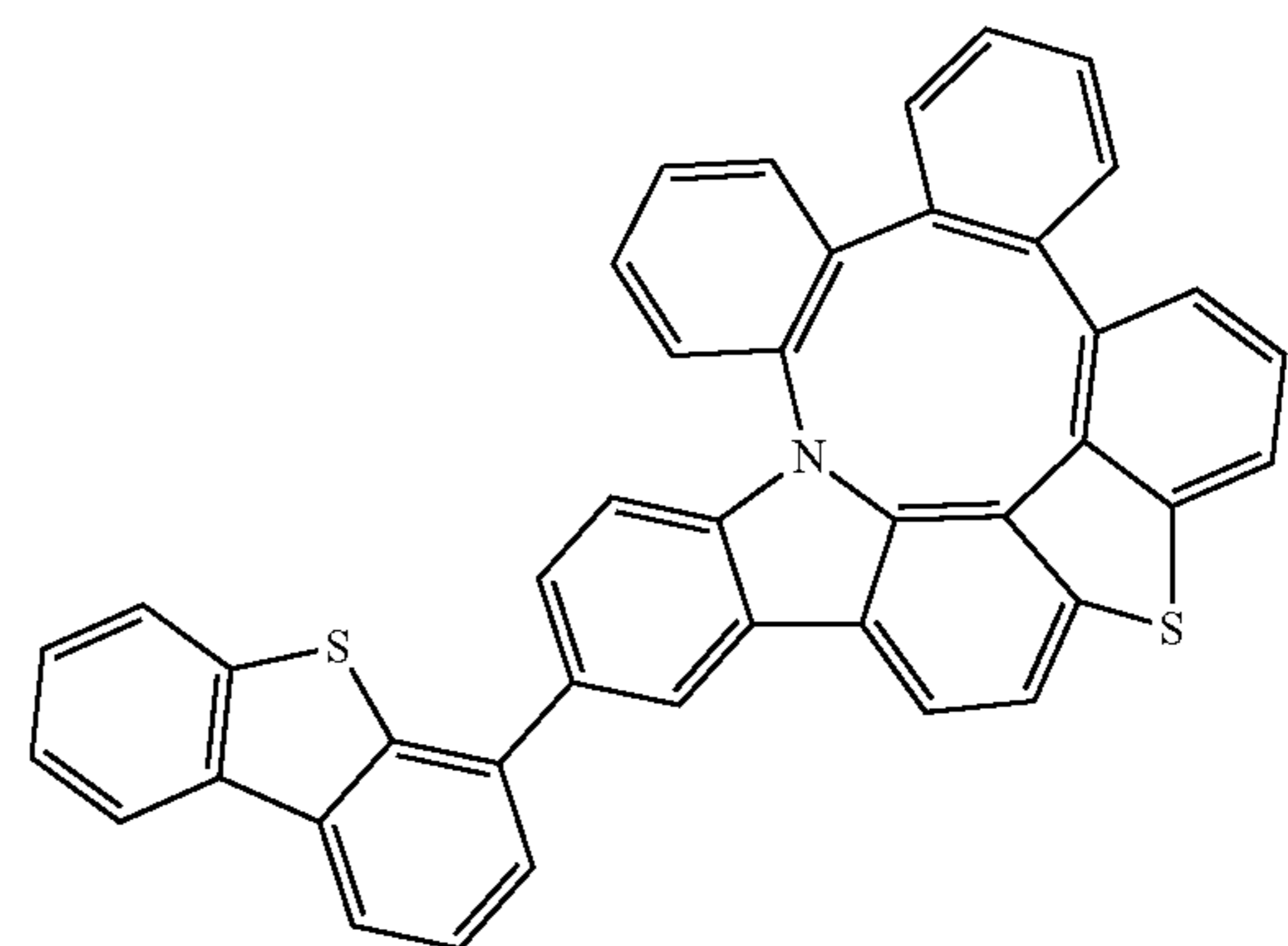
Compound 262
