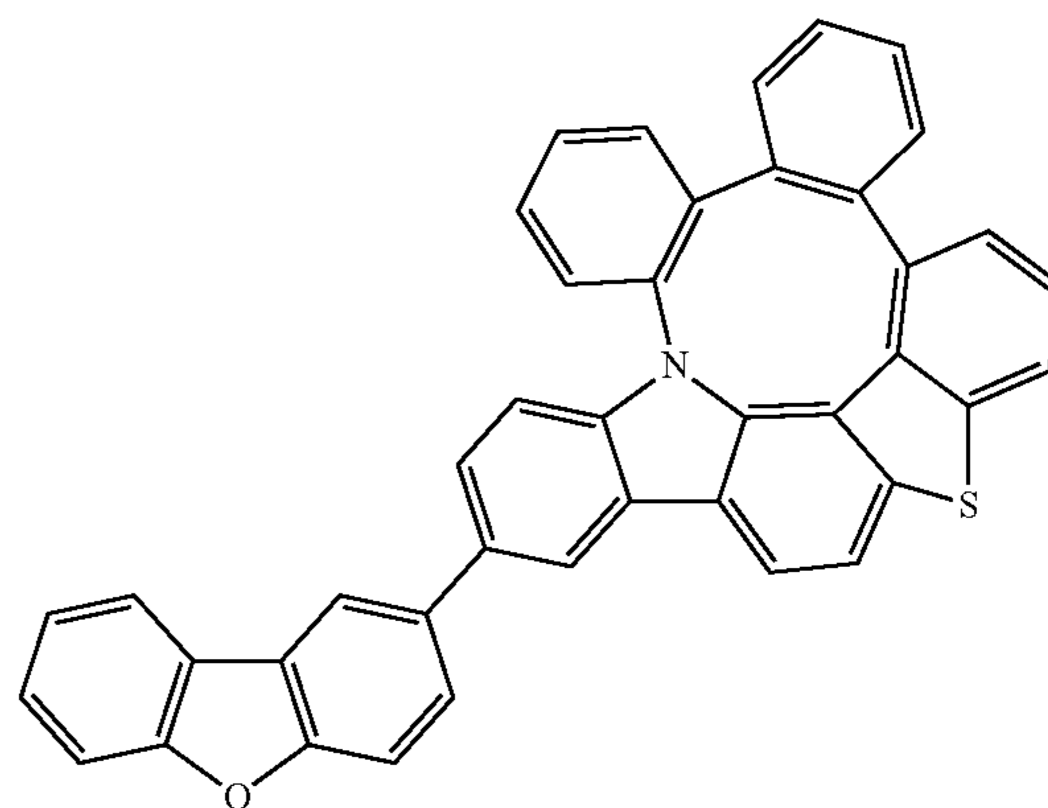
Compound 261
