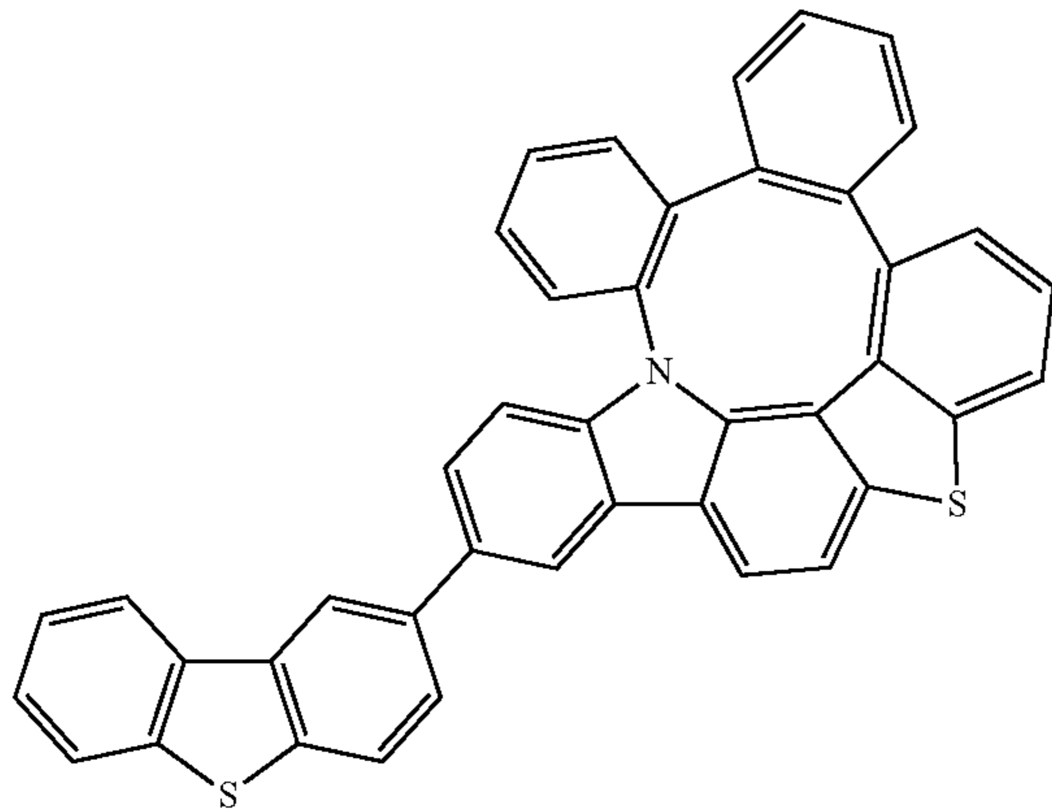
Compound 264
