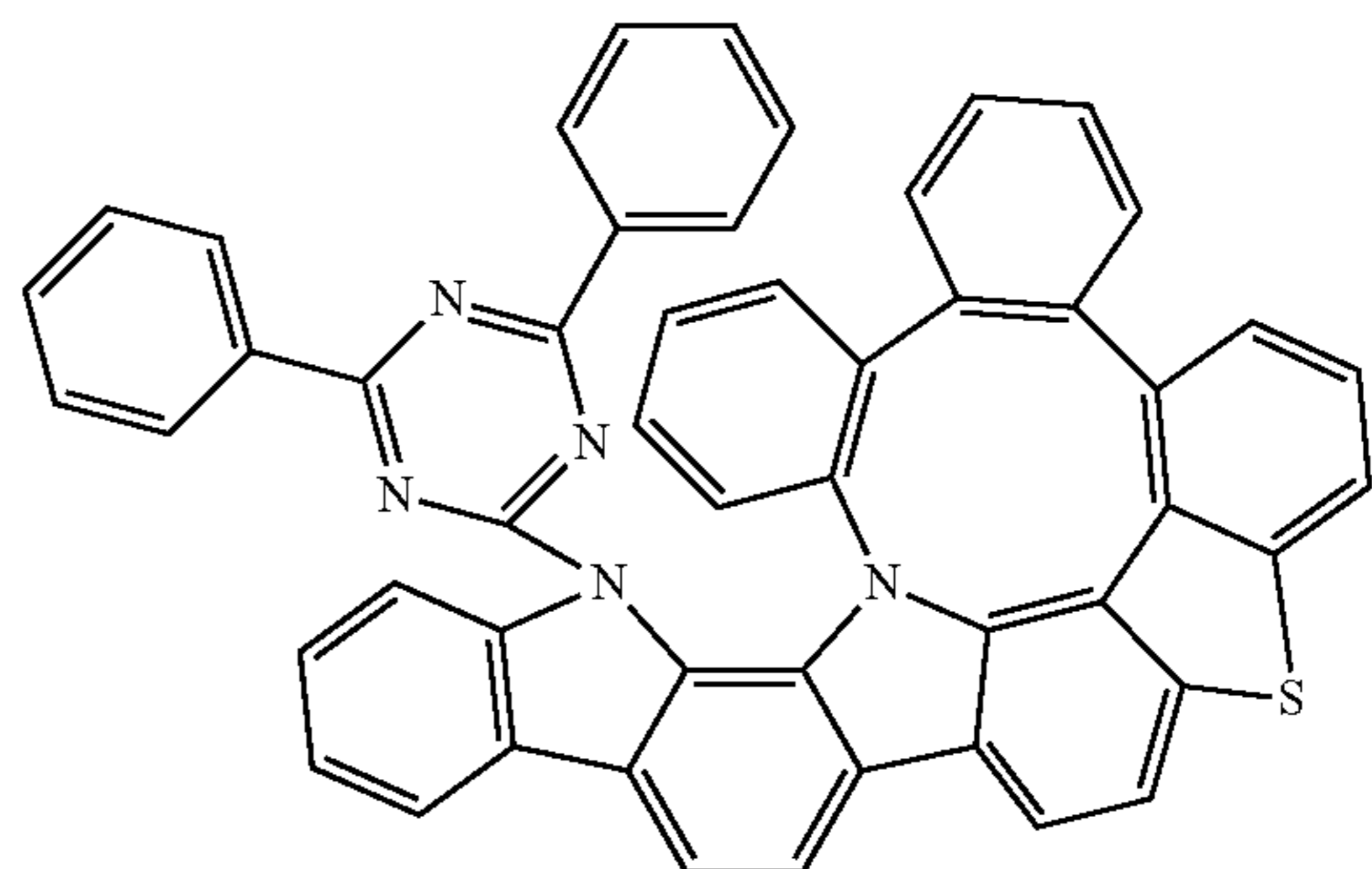
Compound 335
