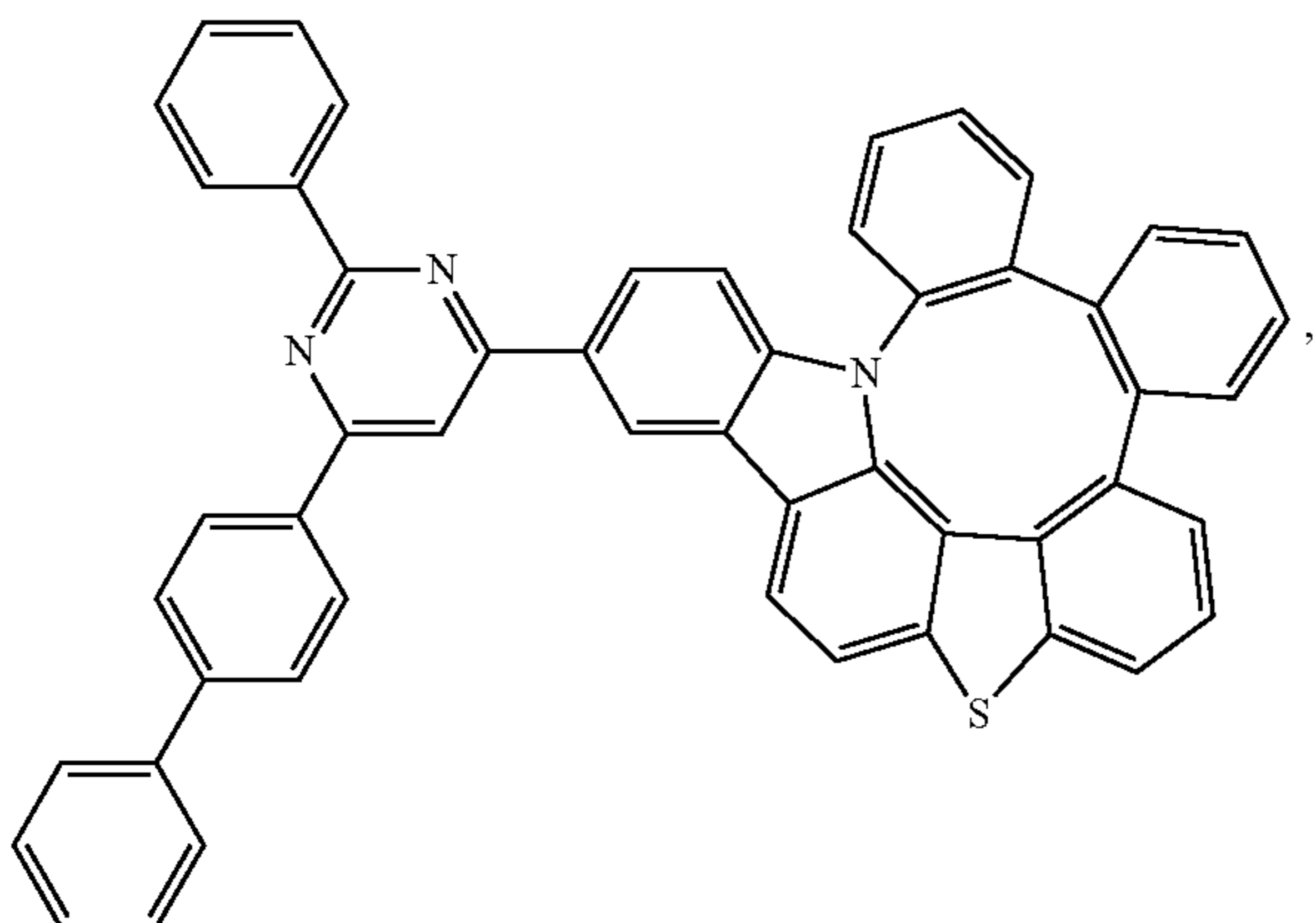
Compound 283
