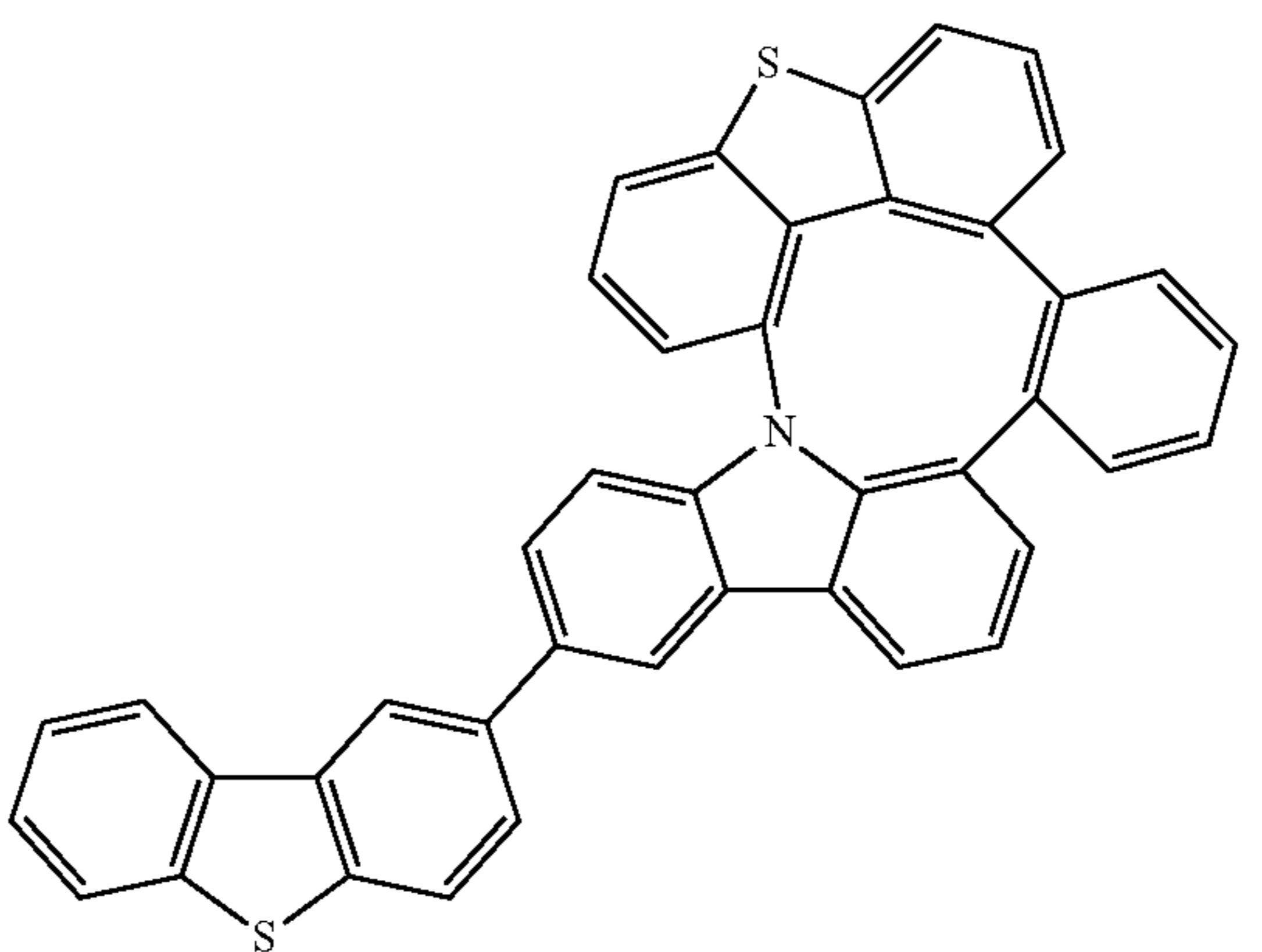
Compound 93
