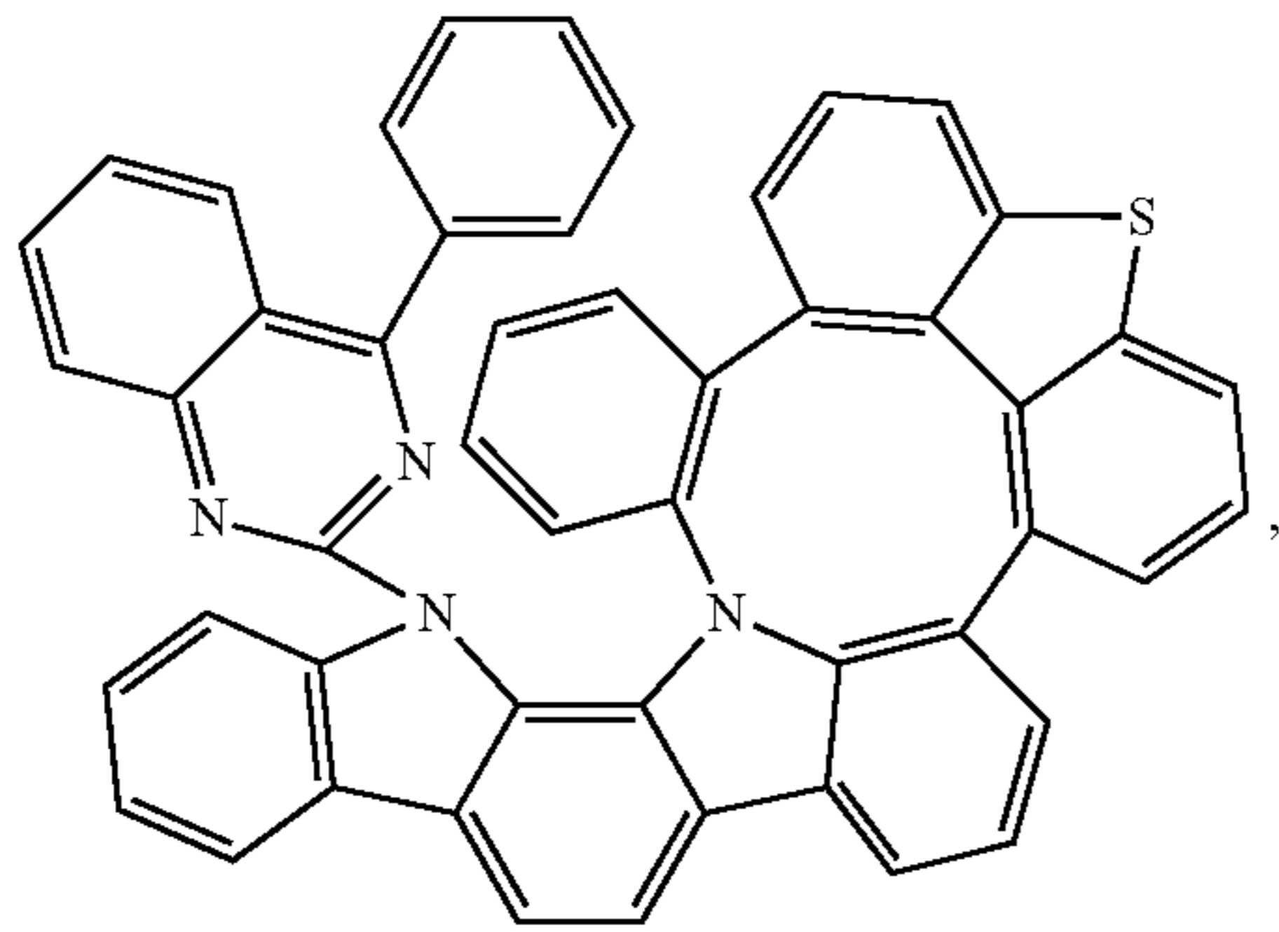
Compound 255
