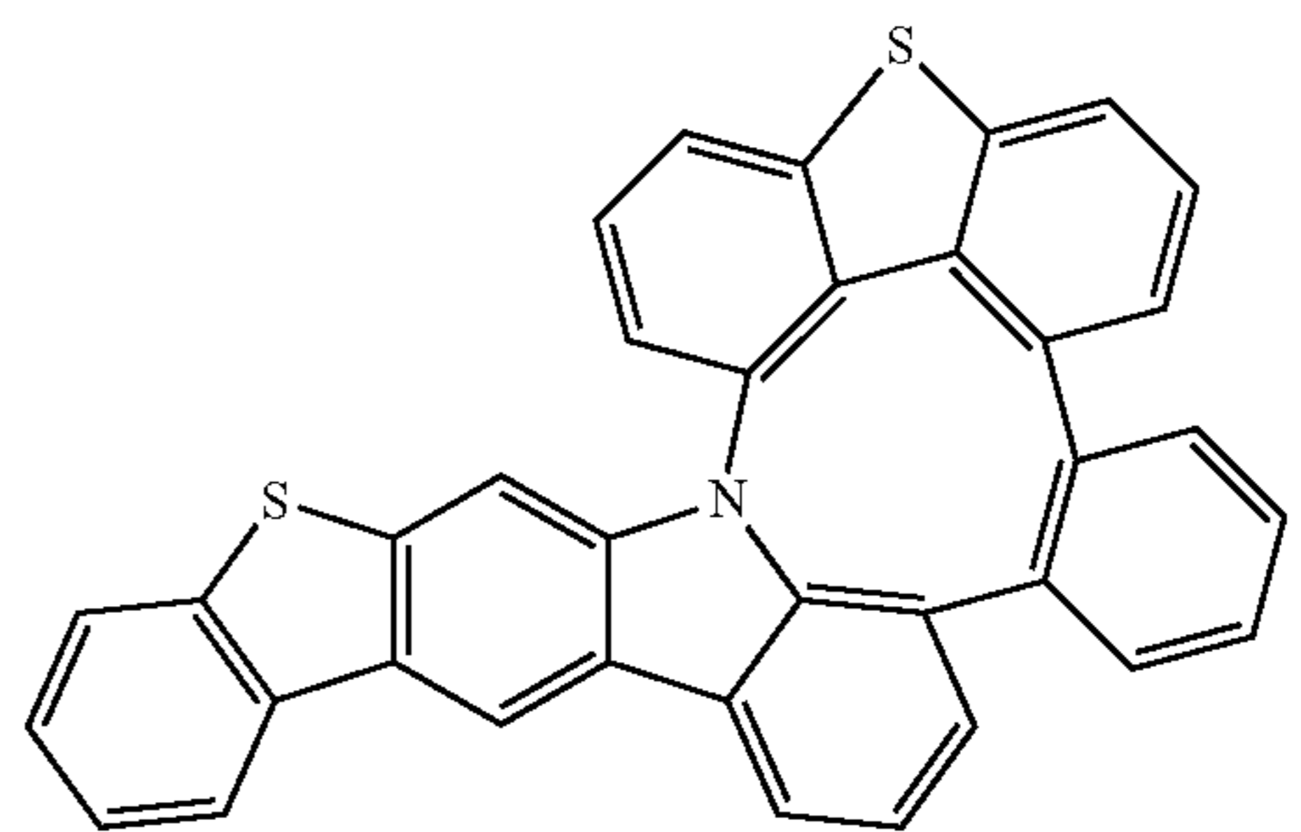
Compound 150
