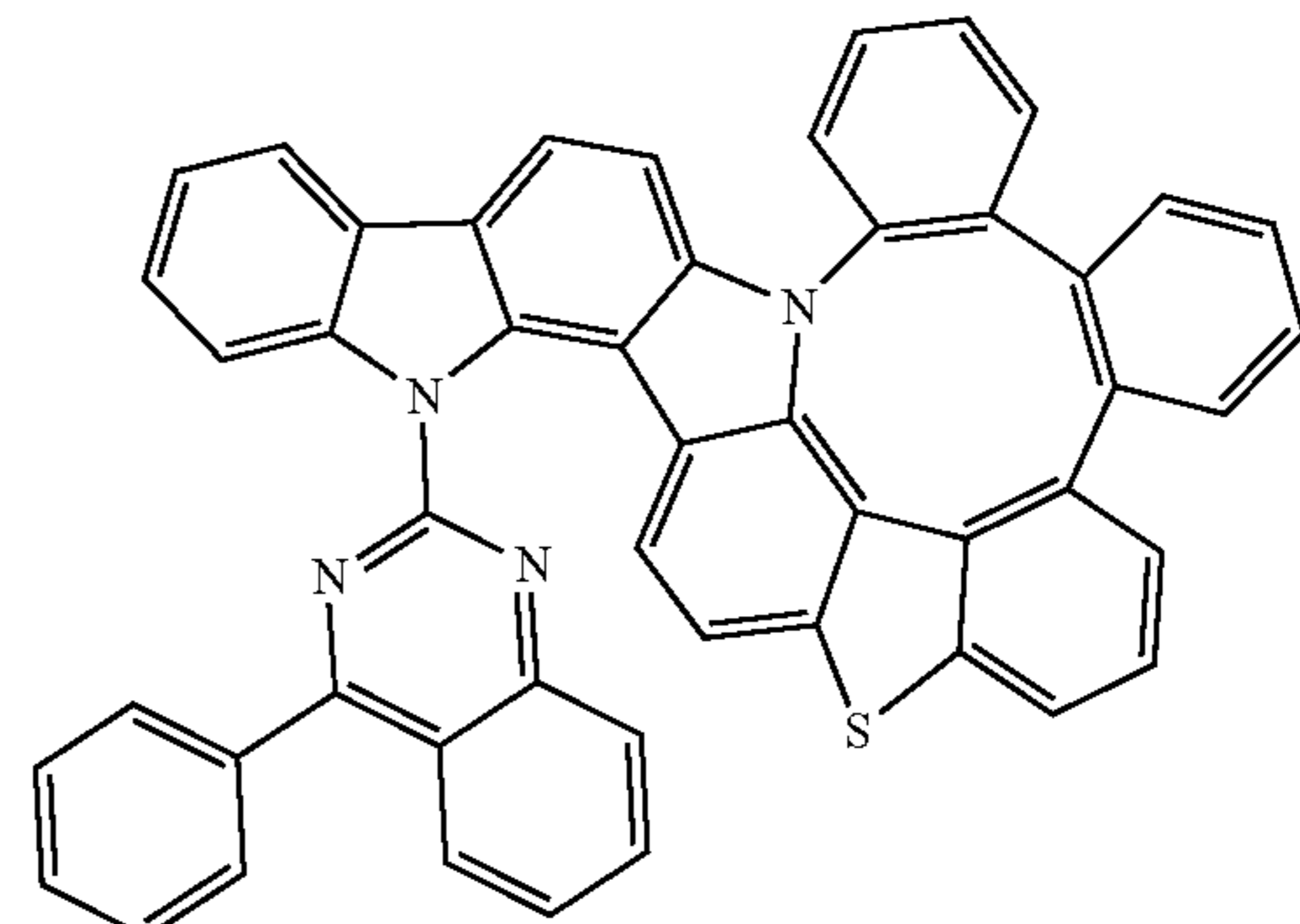
Compound 336
