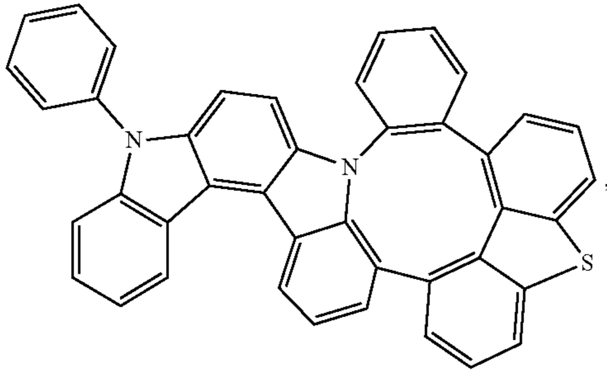
Compound 221
