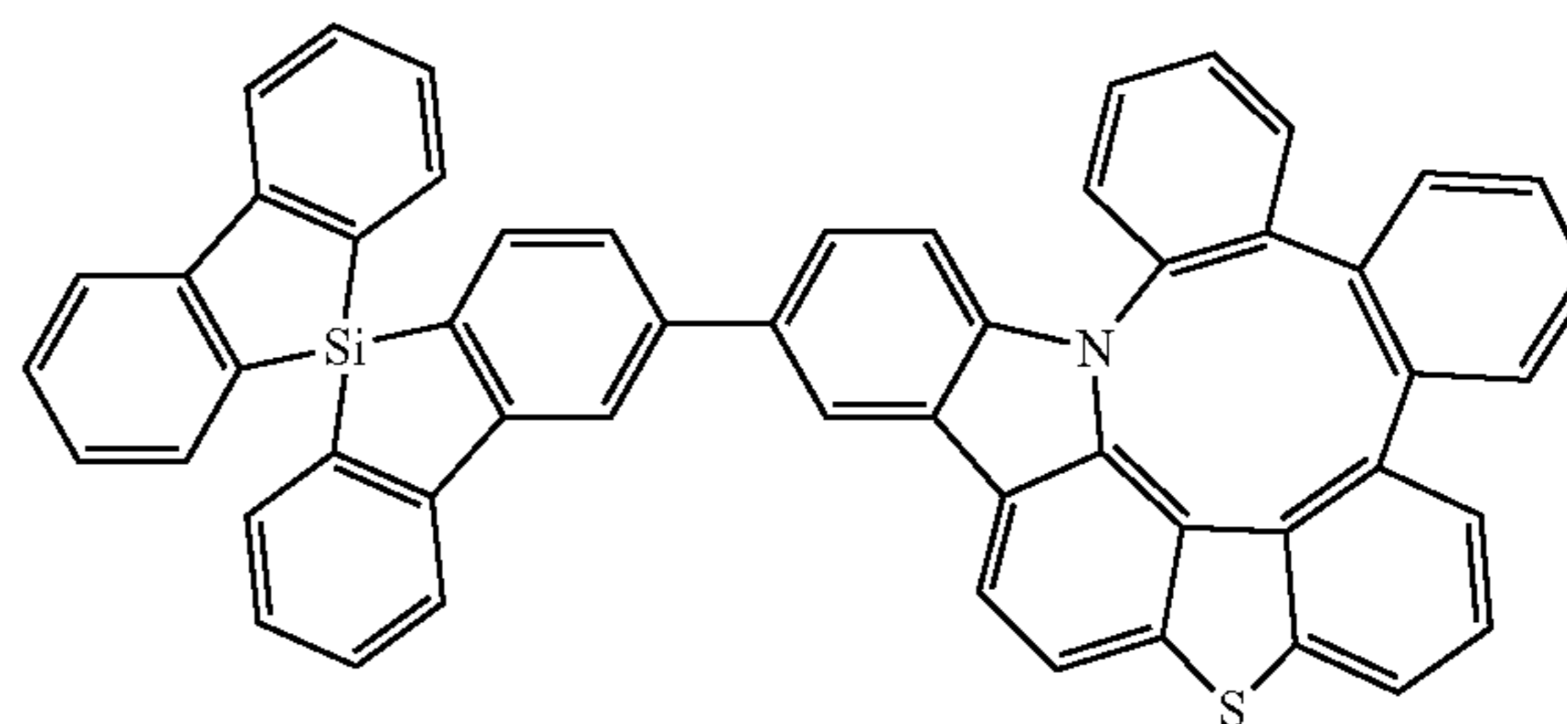
Compound 363
