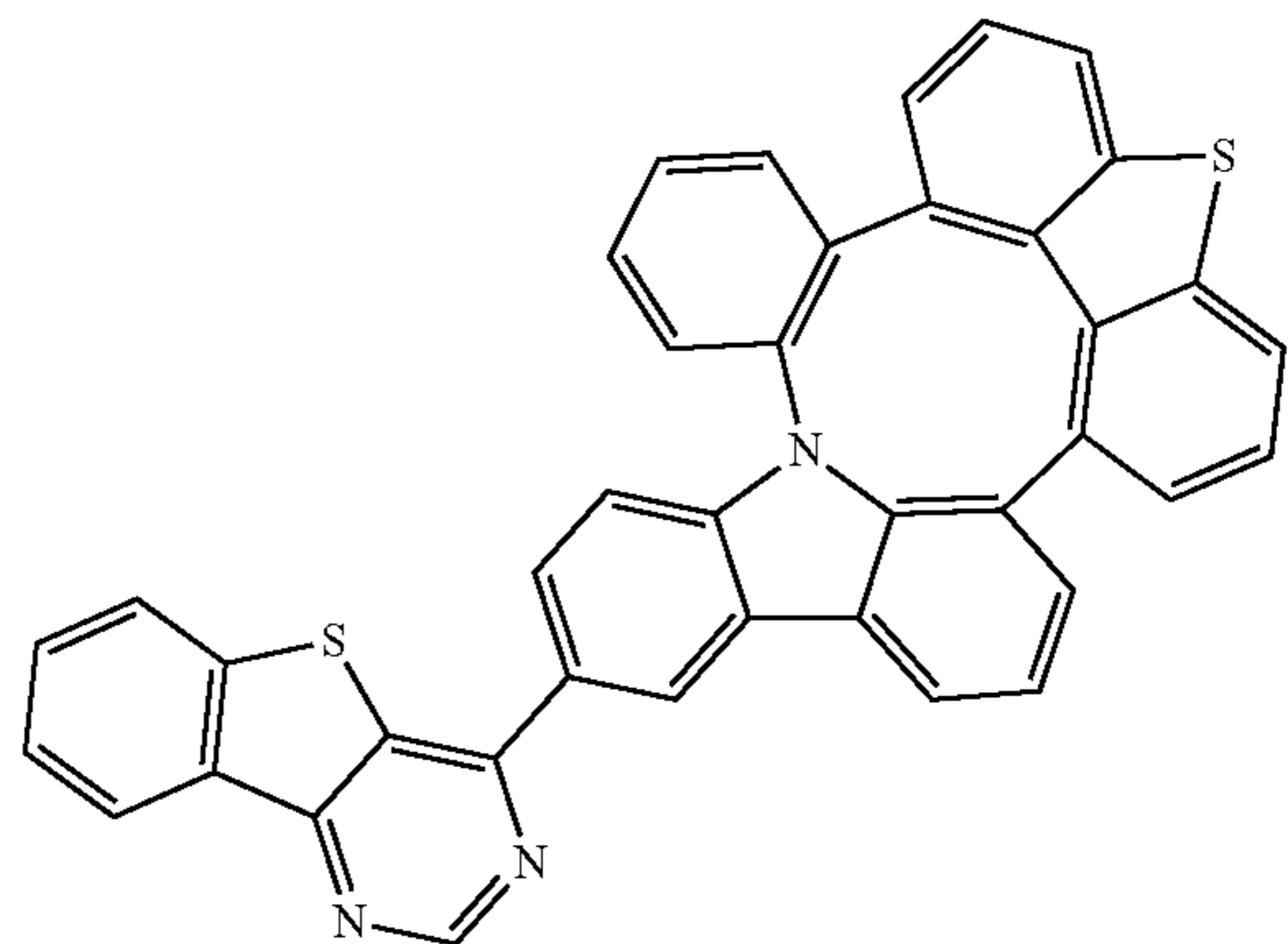
Compound 203
