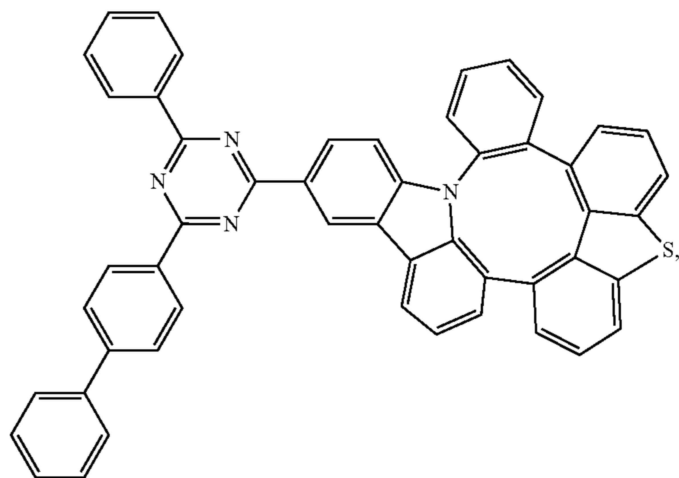
Compound 196
