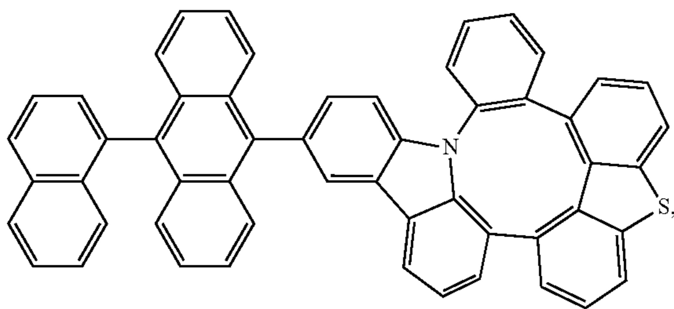
Compound 207
