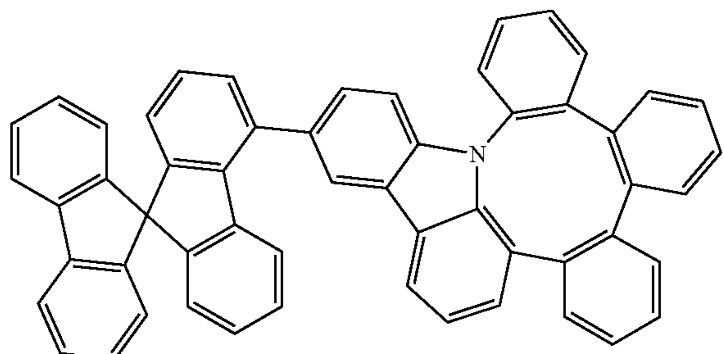
Compound 24
