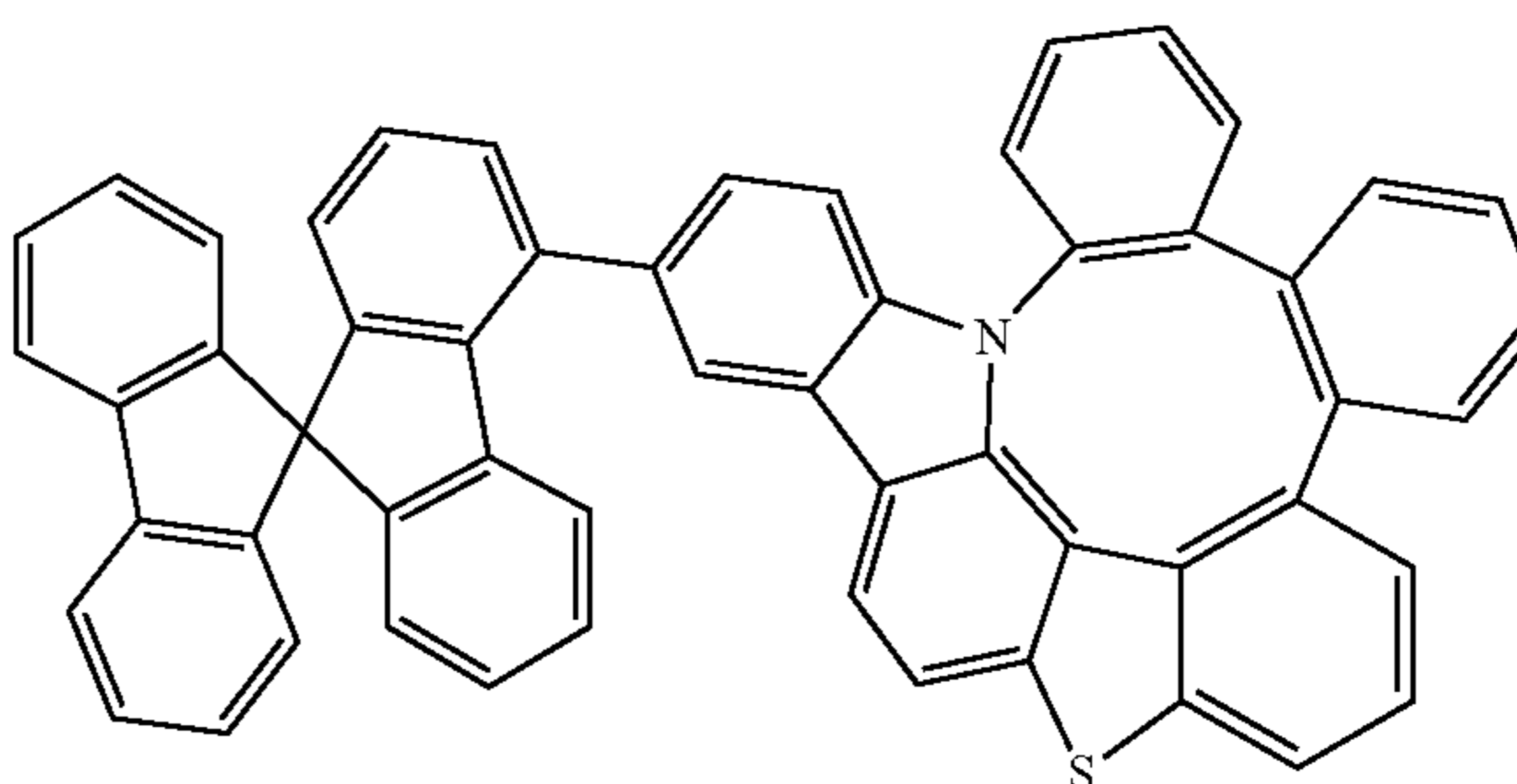
Compound 279
