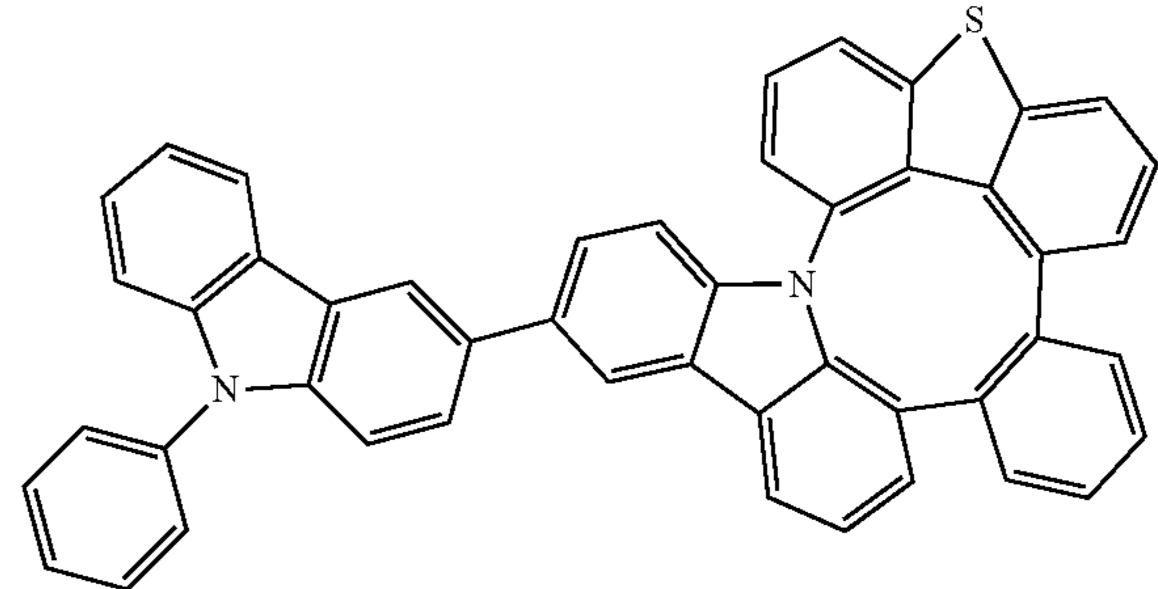
Compound 101
