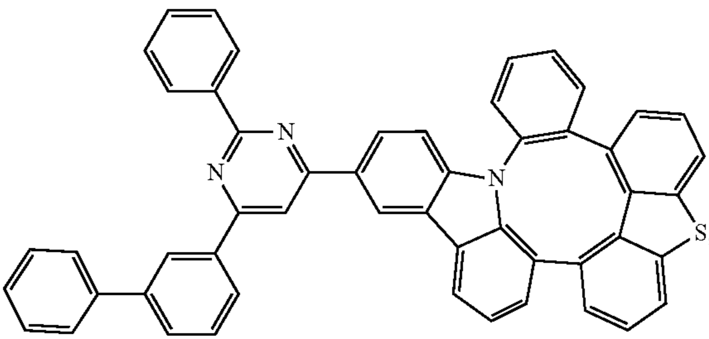
Compound 199
