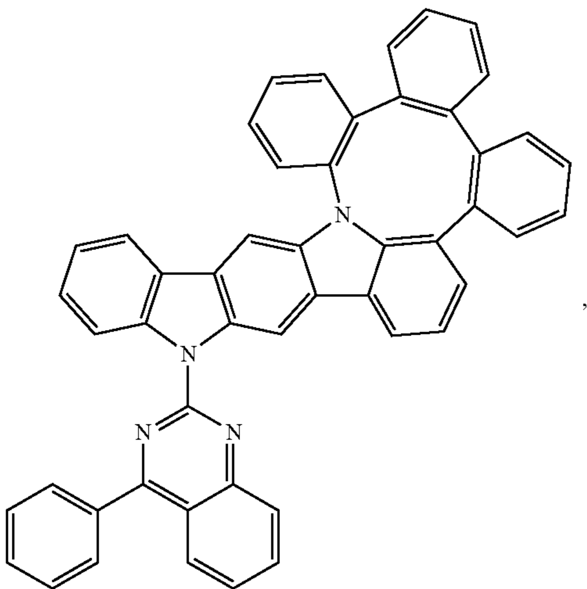
Compound 84
