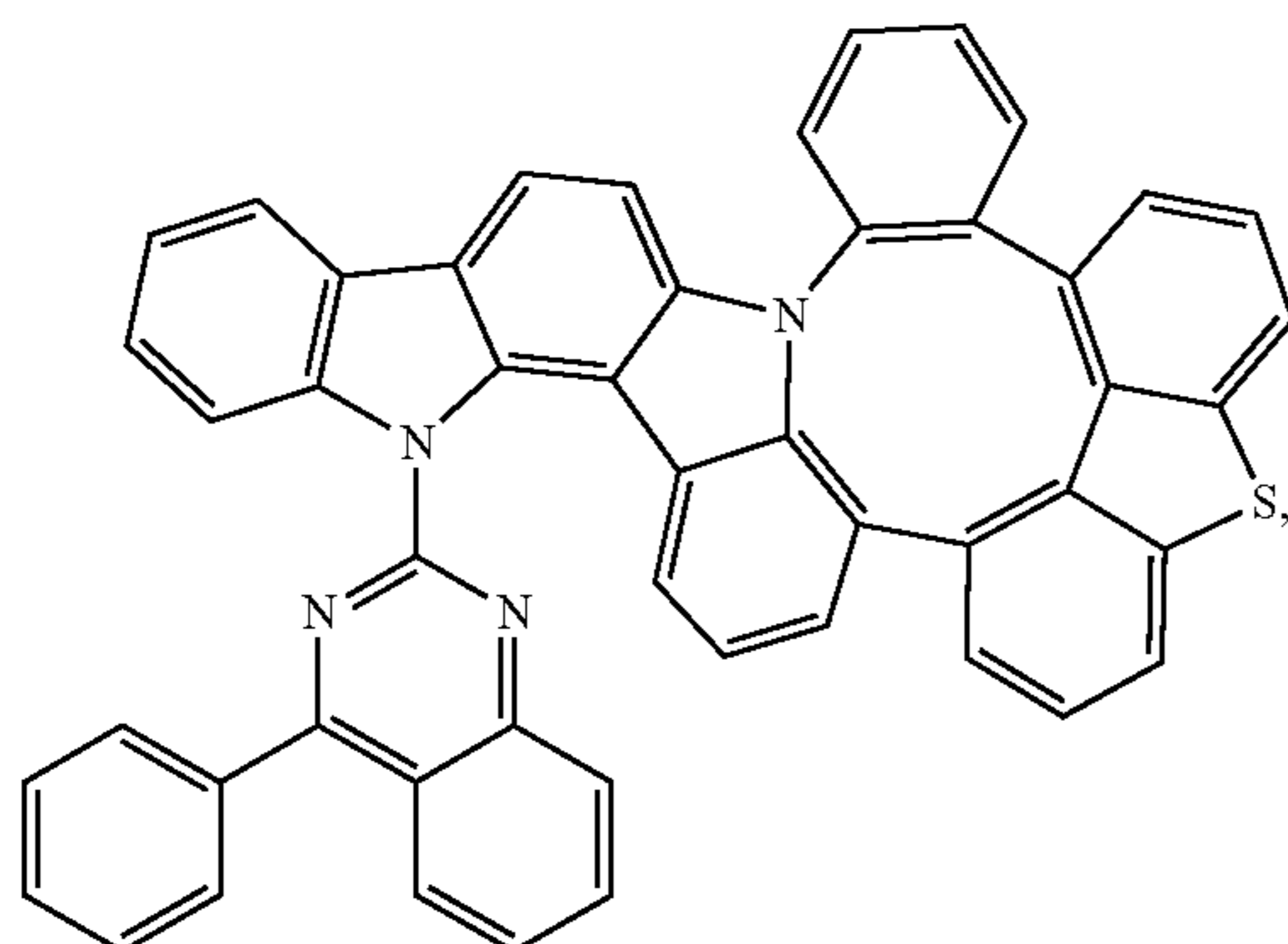
Compound 250
