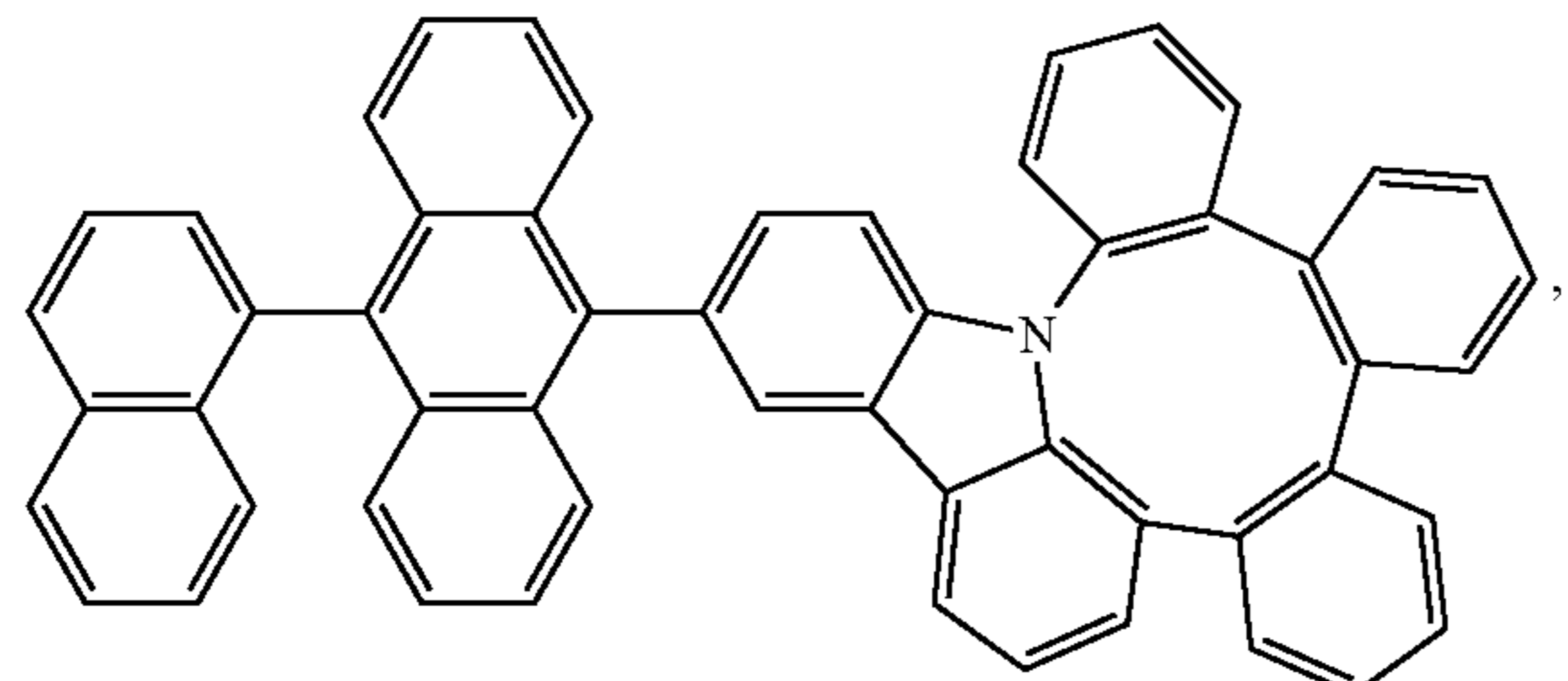
Compound 38
