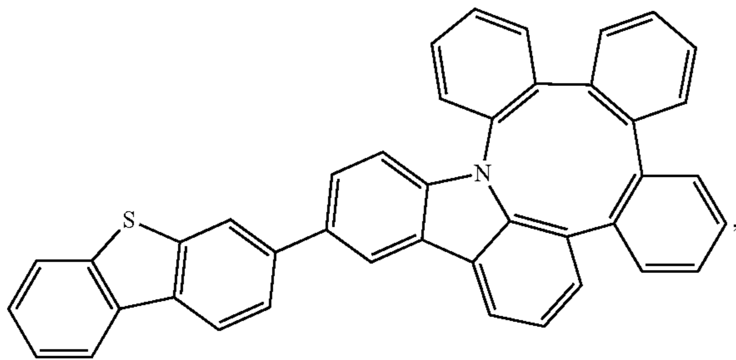
Compound 10
