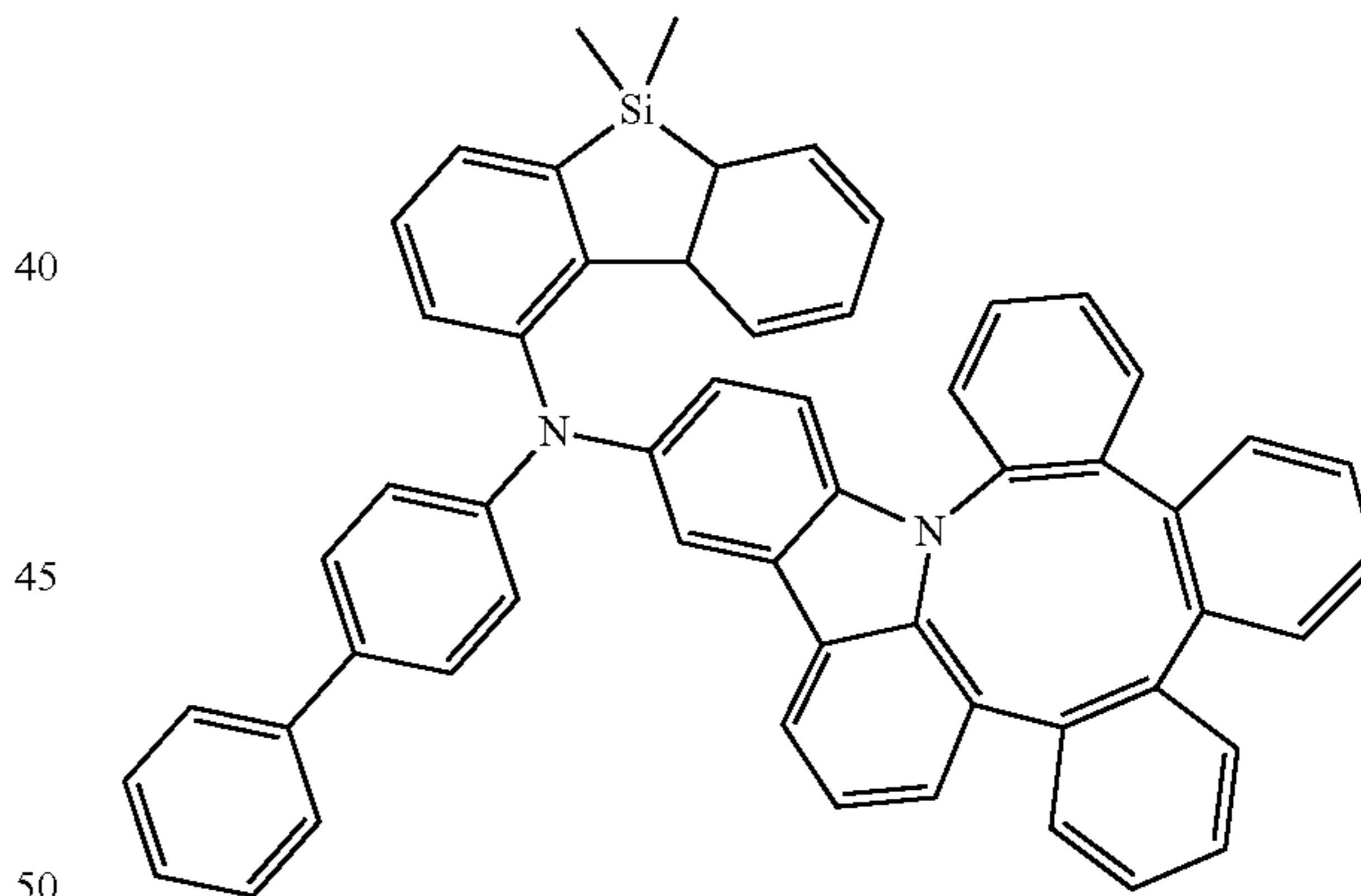
Compound 347
