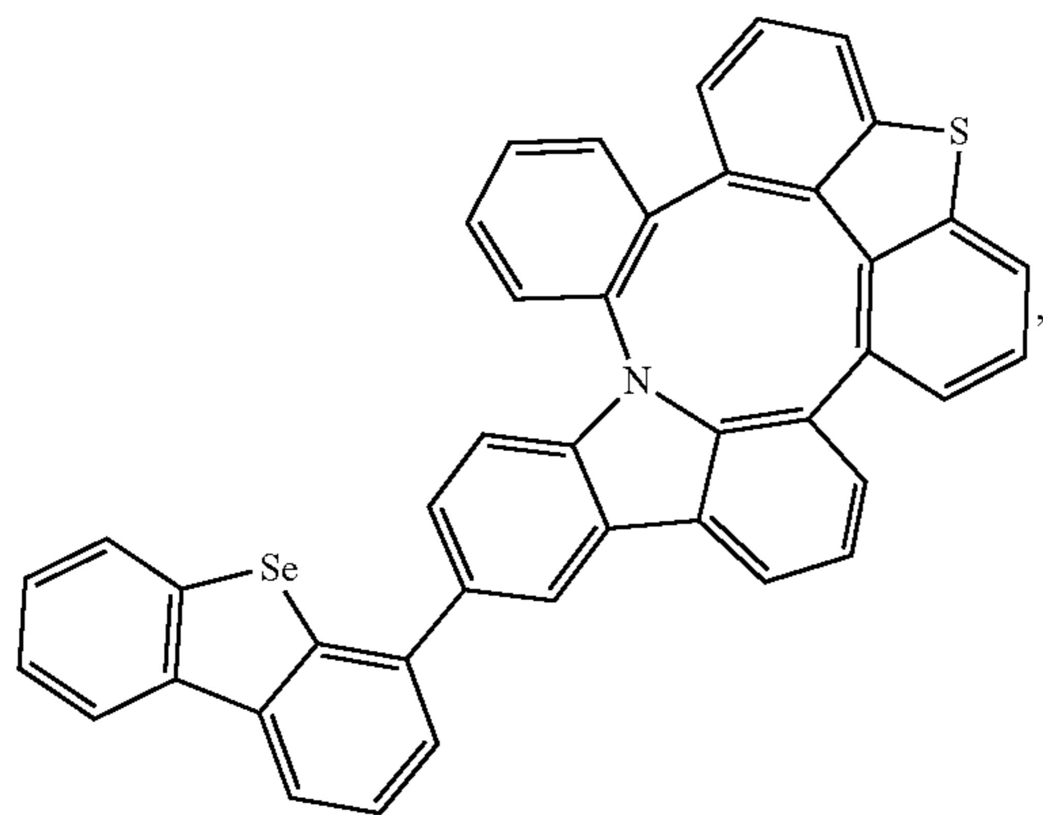
Compound 181
