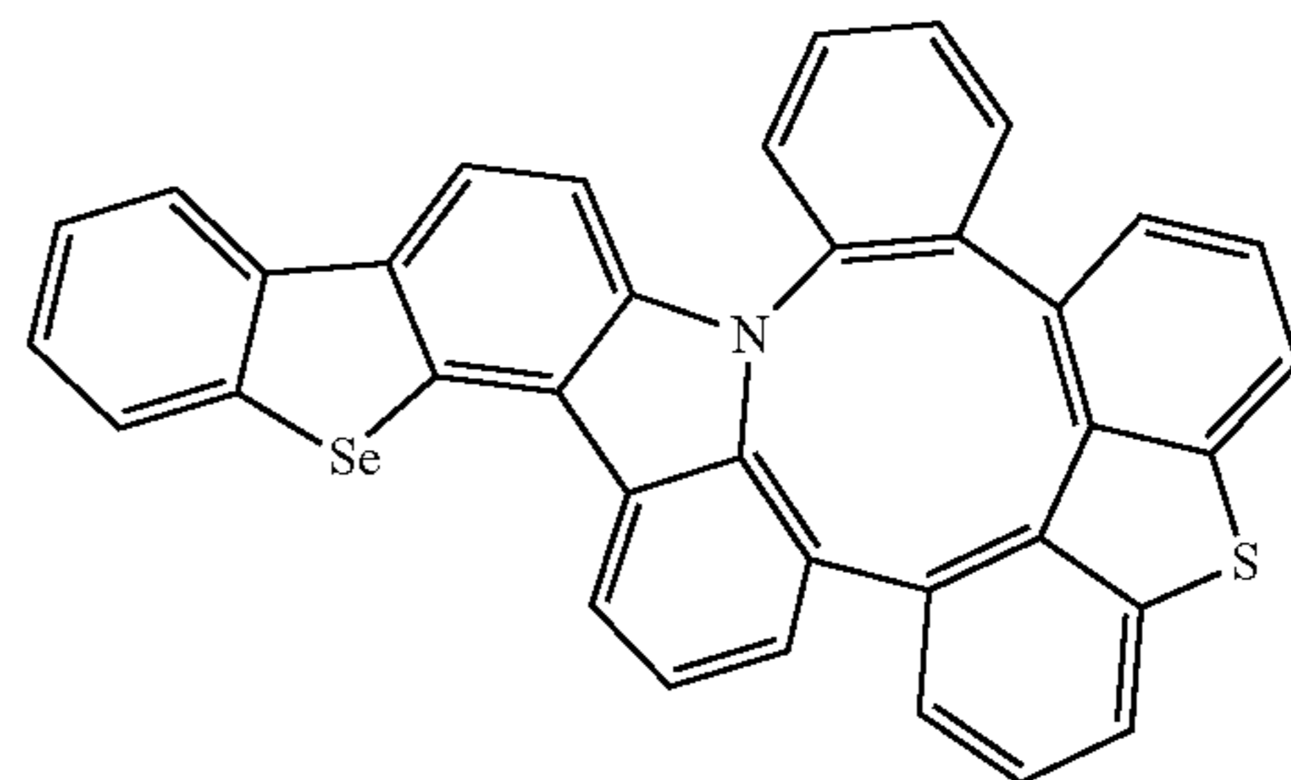
Compound 238
