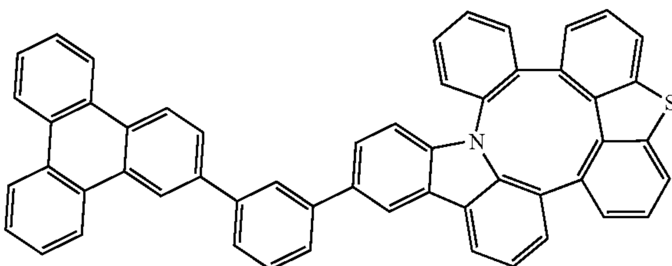
Compound 205
