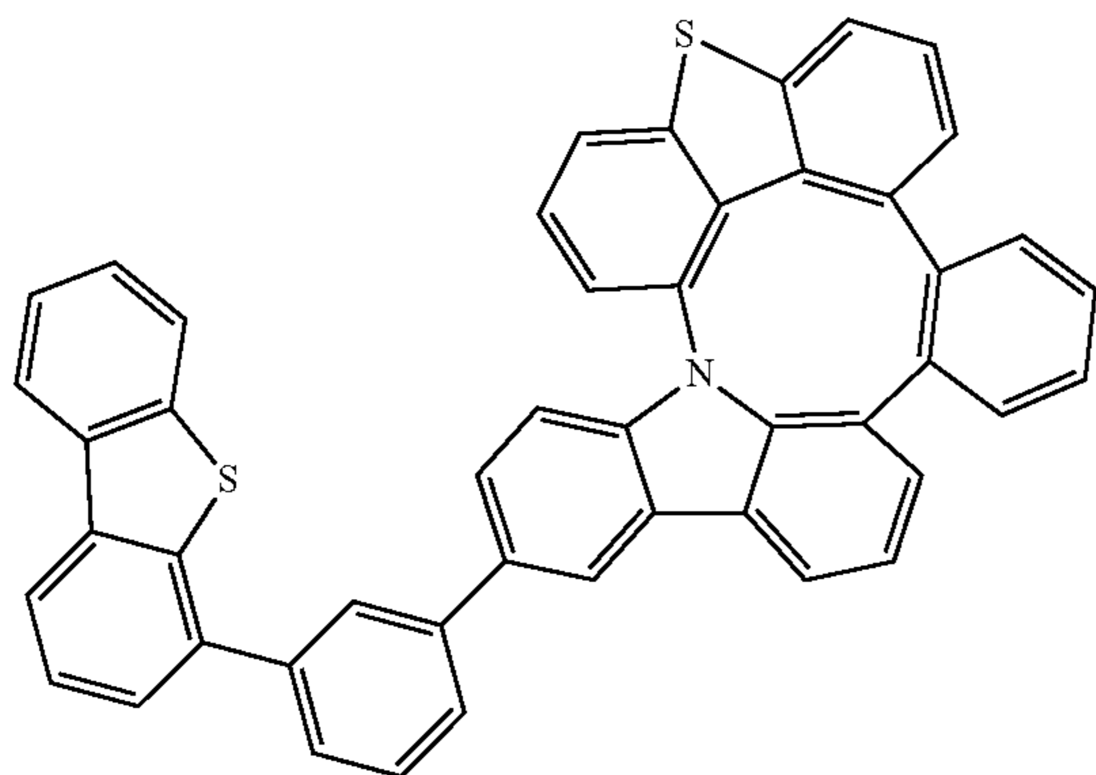
Compound 100
