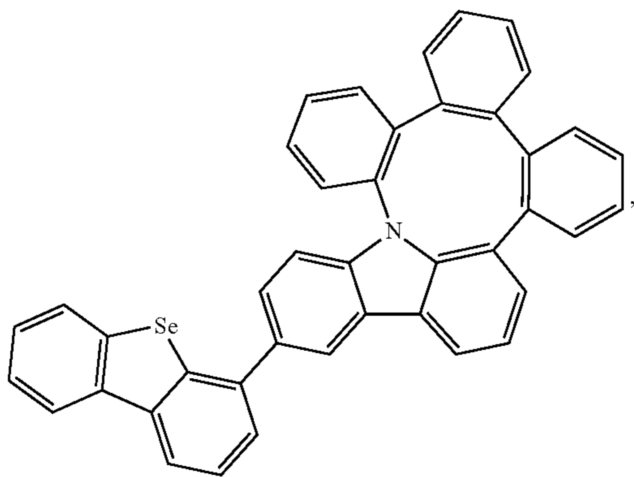
Compound 10
