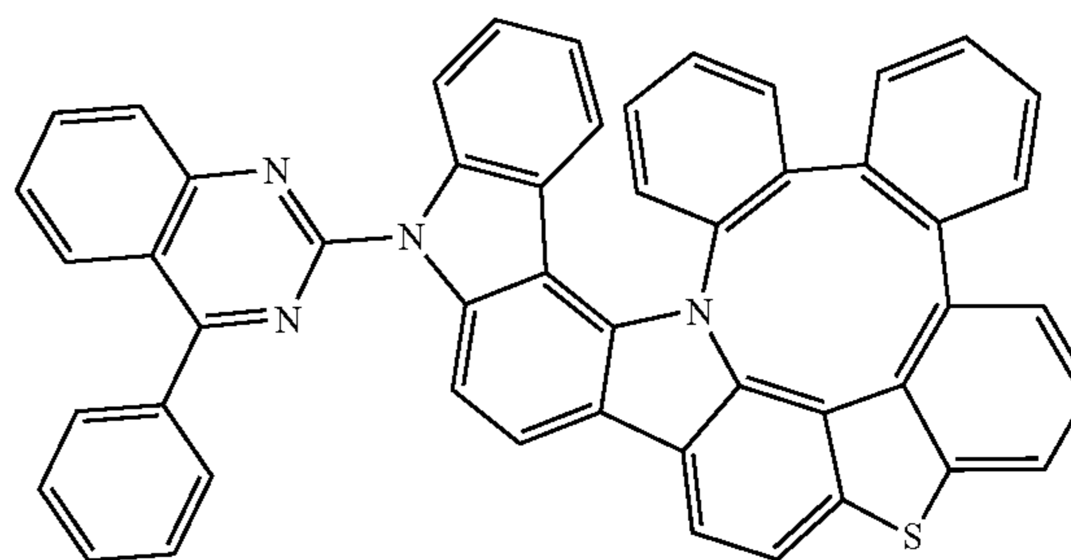
Compound 339
