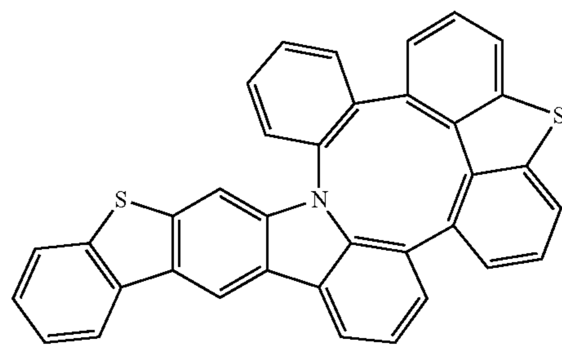
Compound 235
