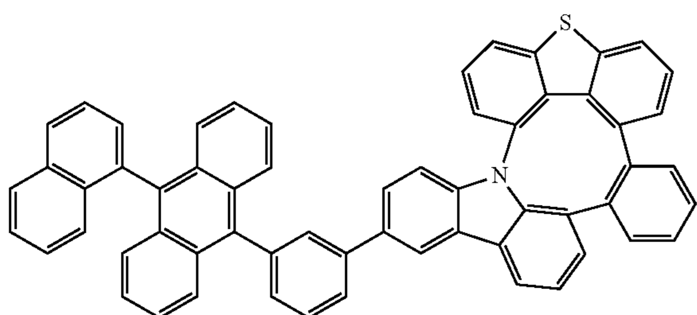
Compound 124
