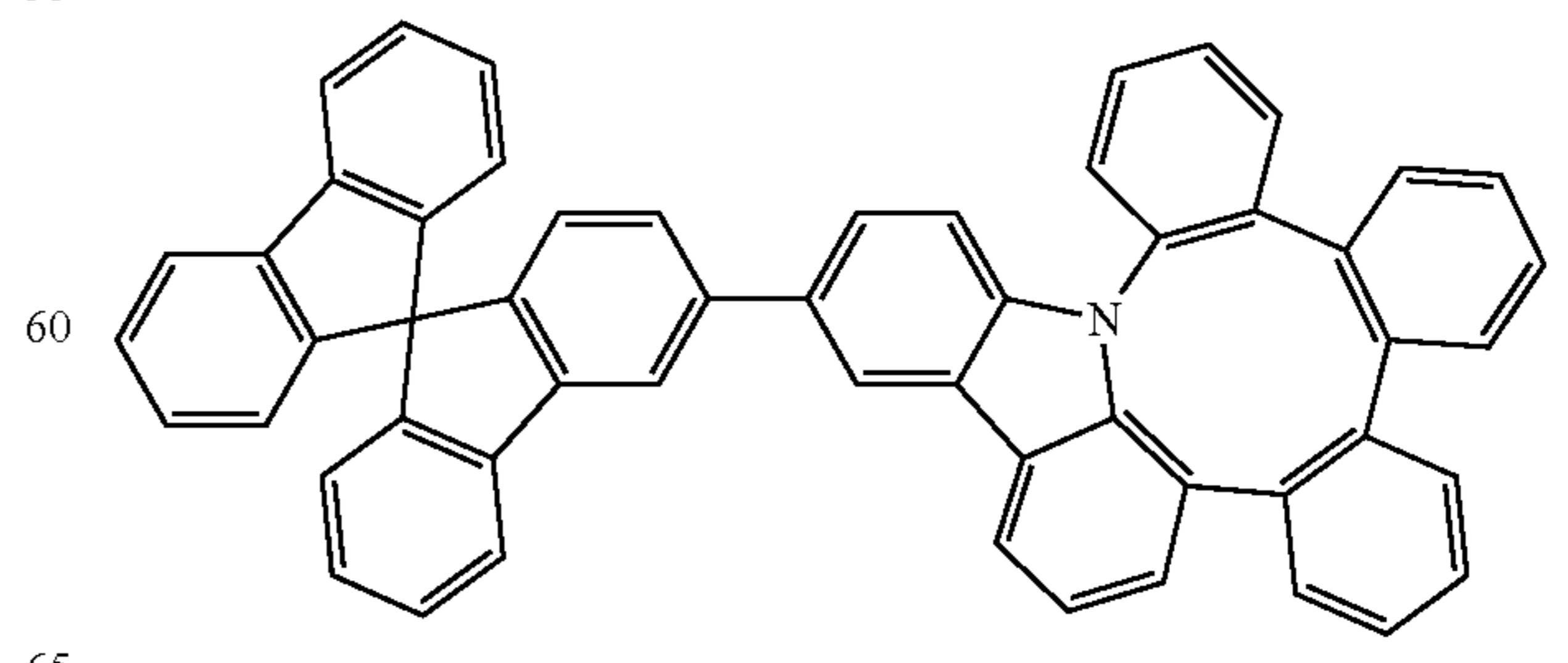
Compound 22
