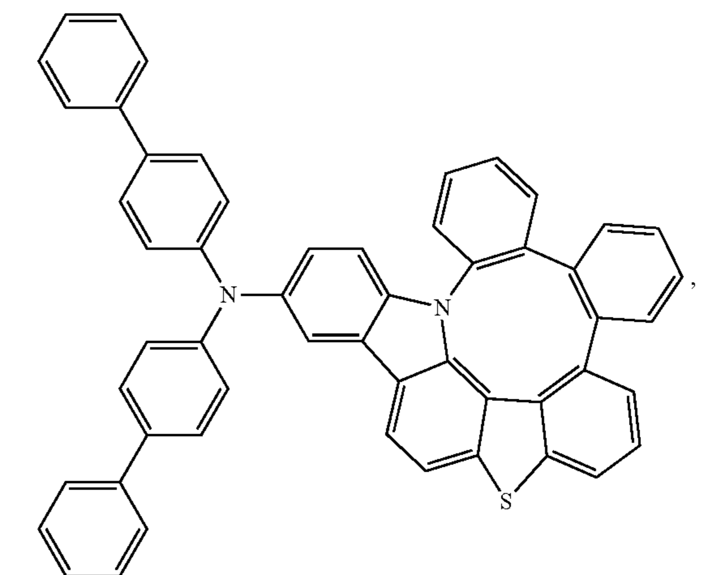
Compound 296
