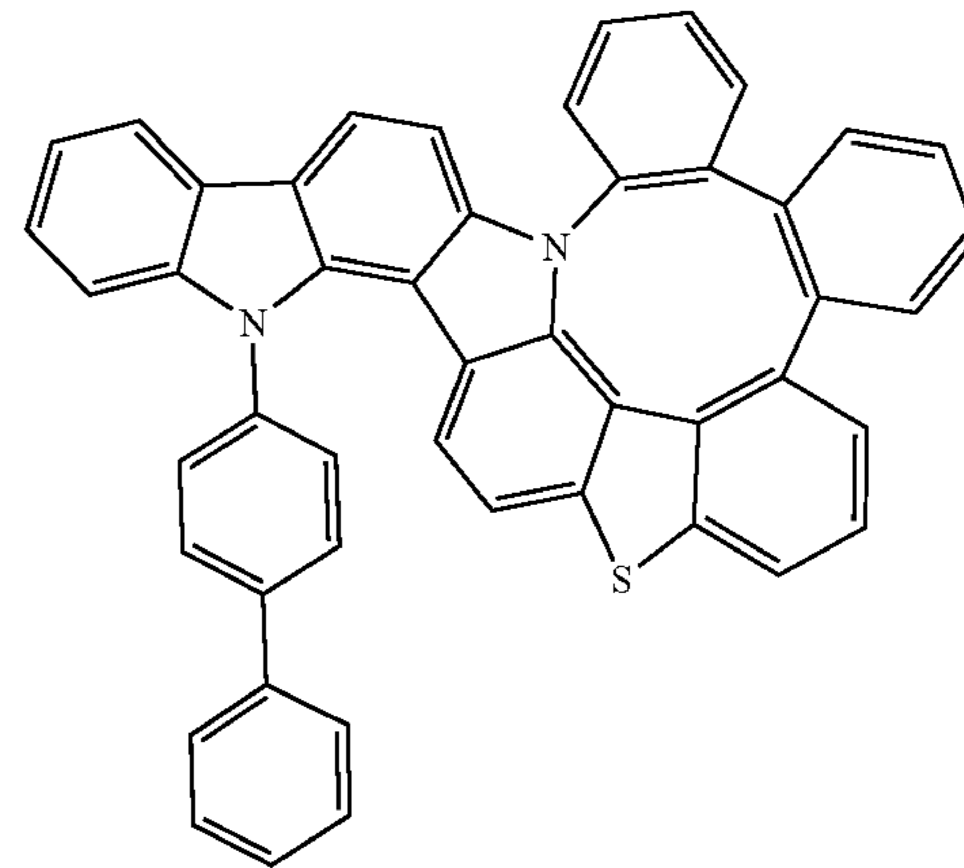
Compound 312
