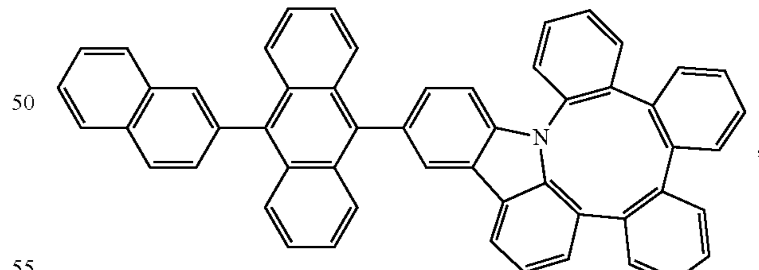
Compound 39
