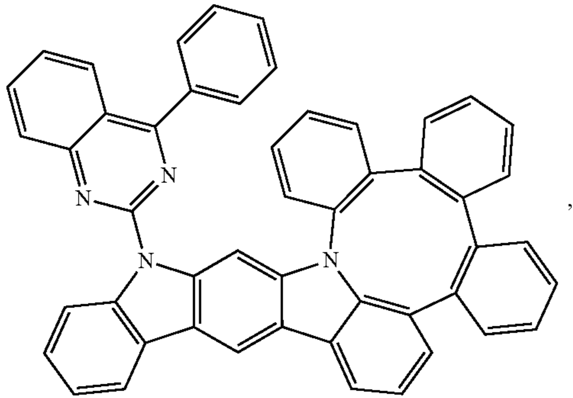
Compound 83
