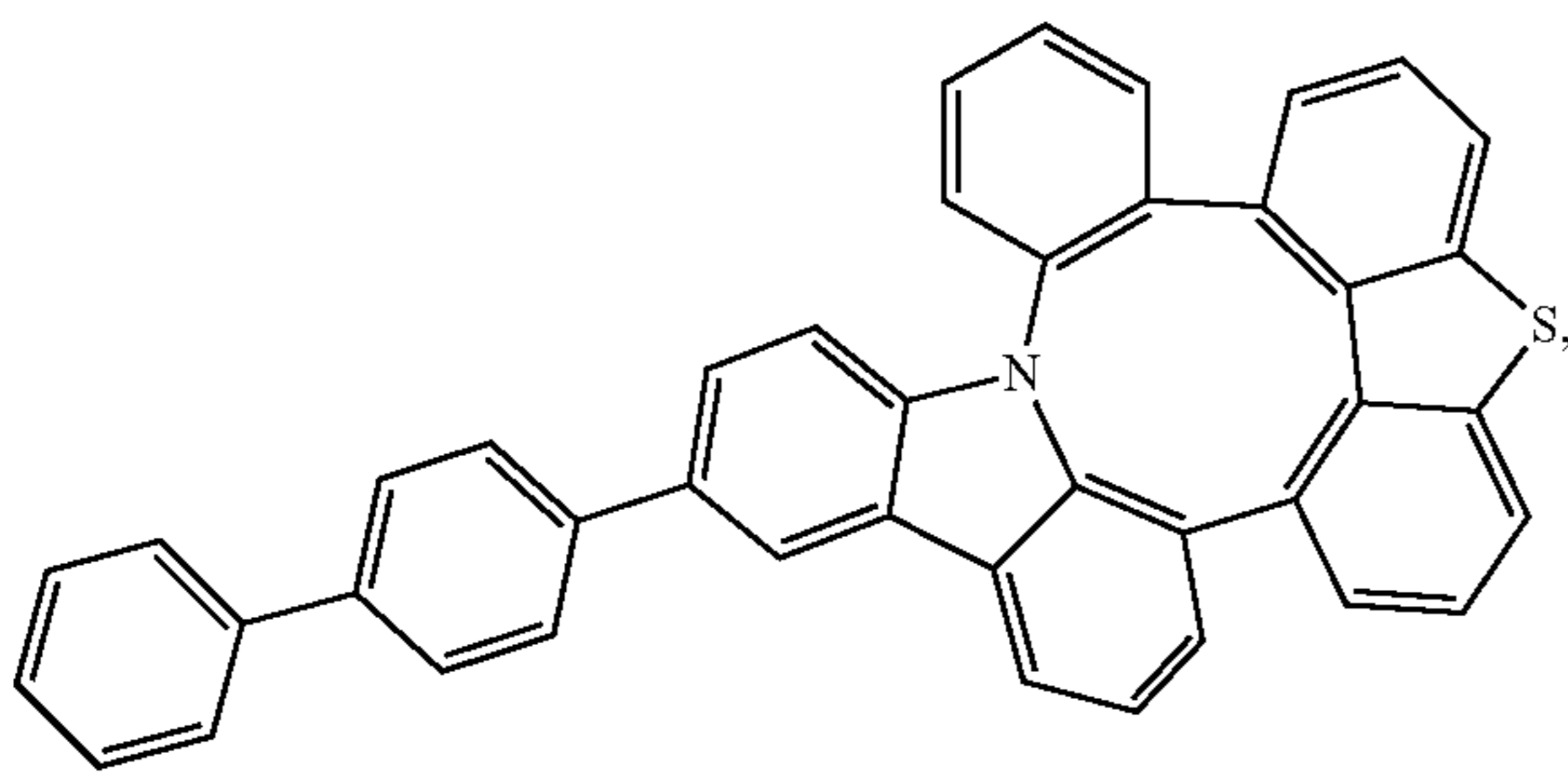
Compound 172
