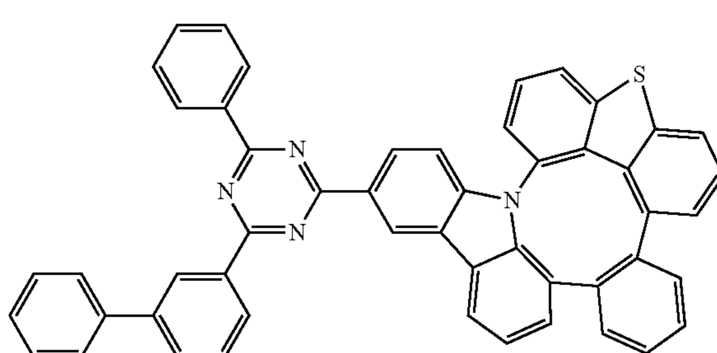
Compound 112
