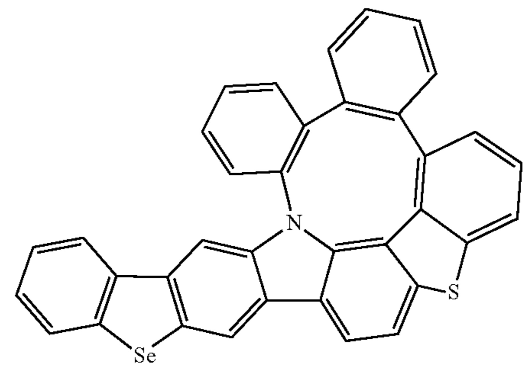
Compound 327
