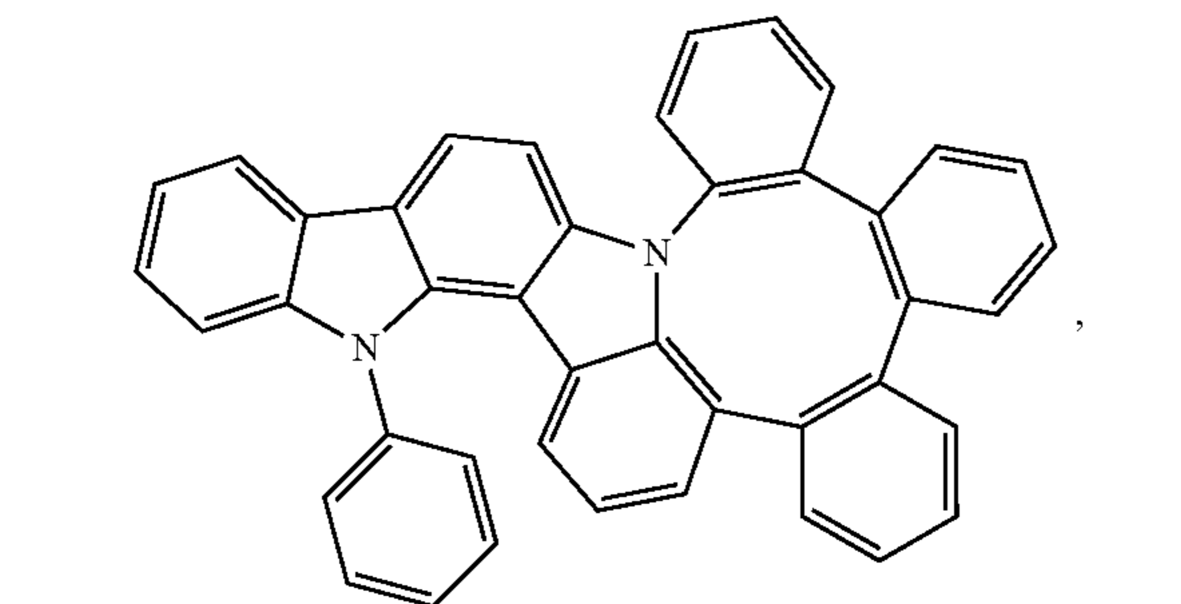
Compound 50
