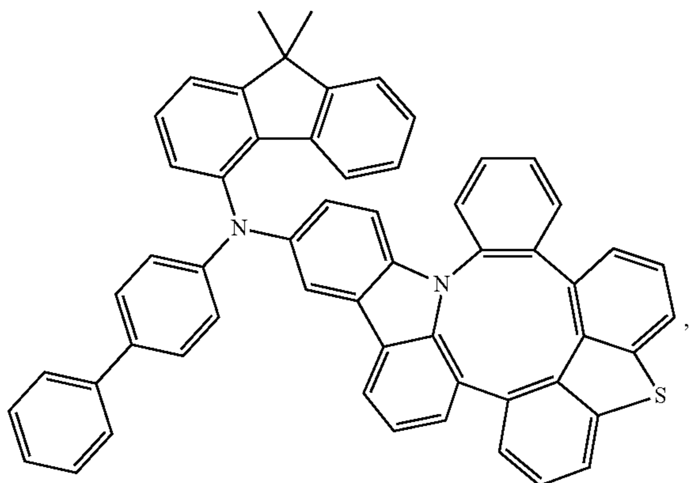
Compound 214
