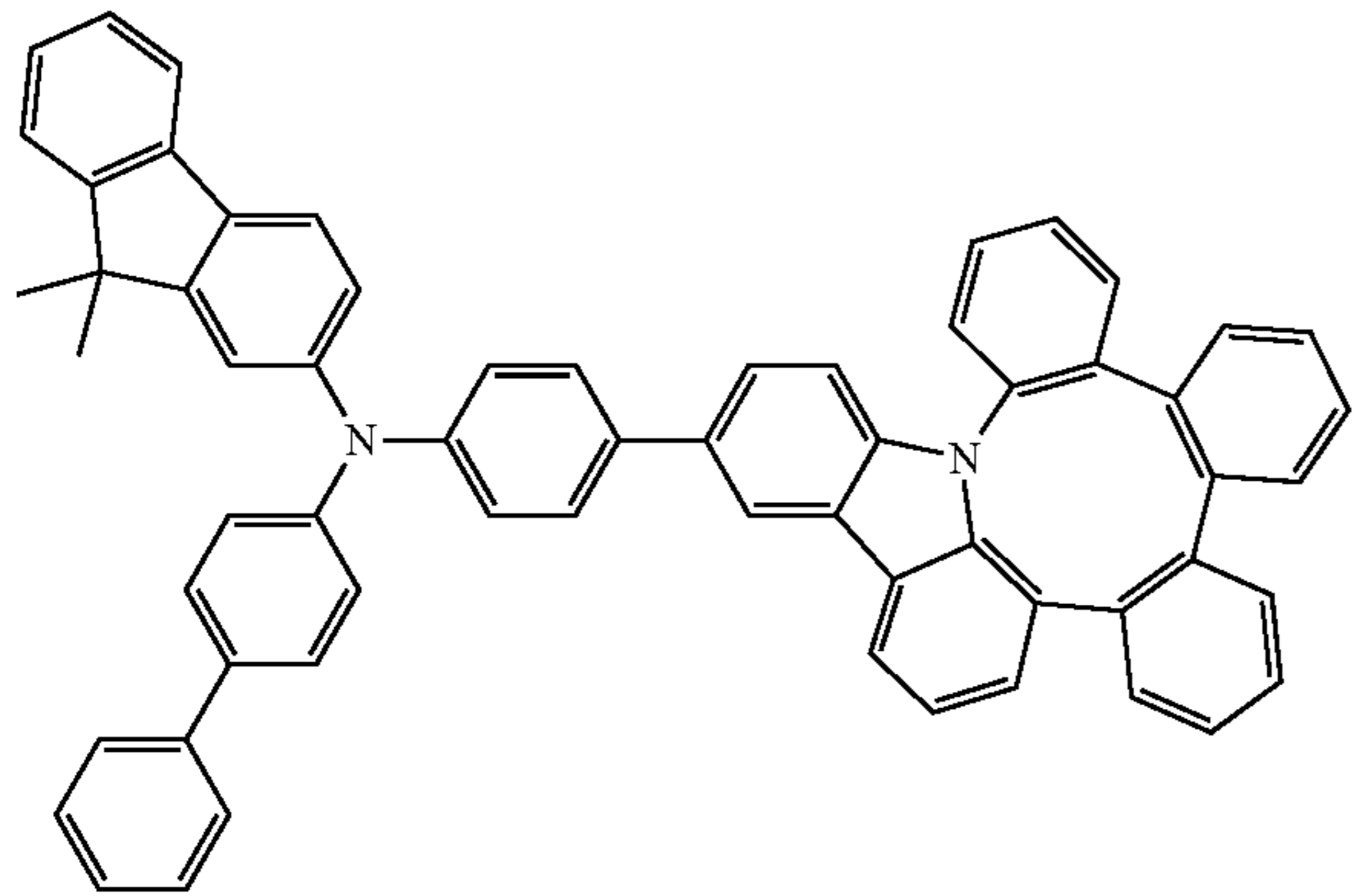
Compound 47
