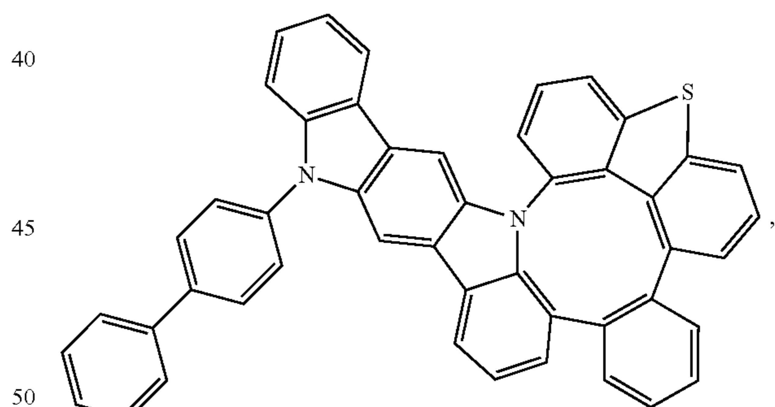
Compound 145
