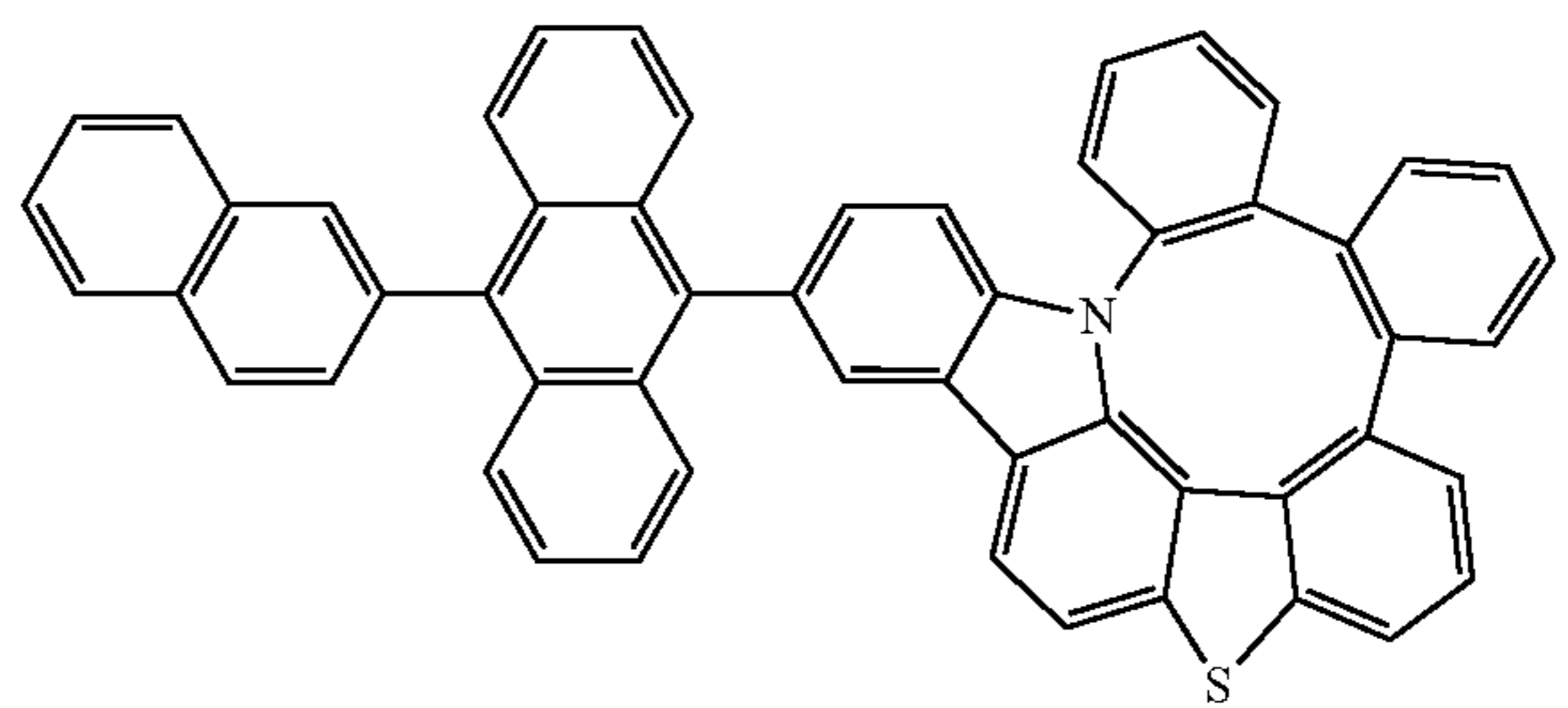
Compound 293
