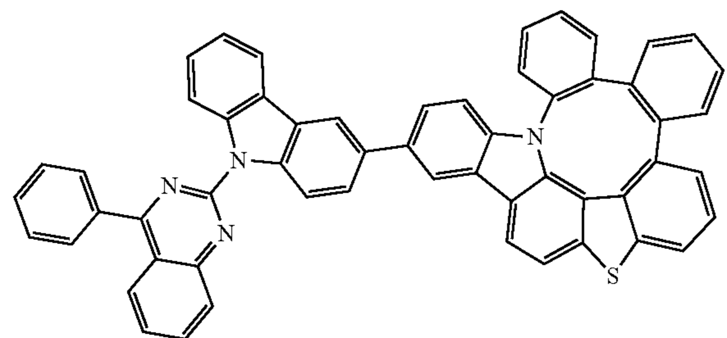
Compound 275
