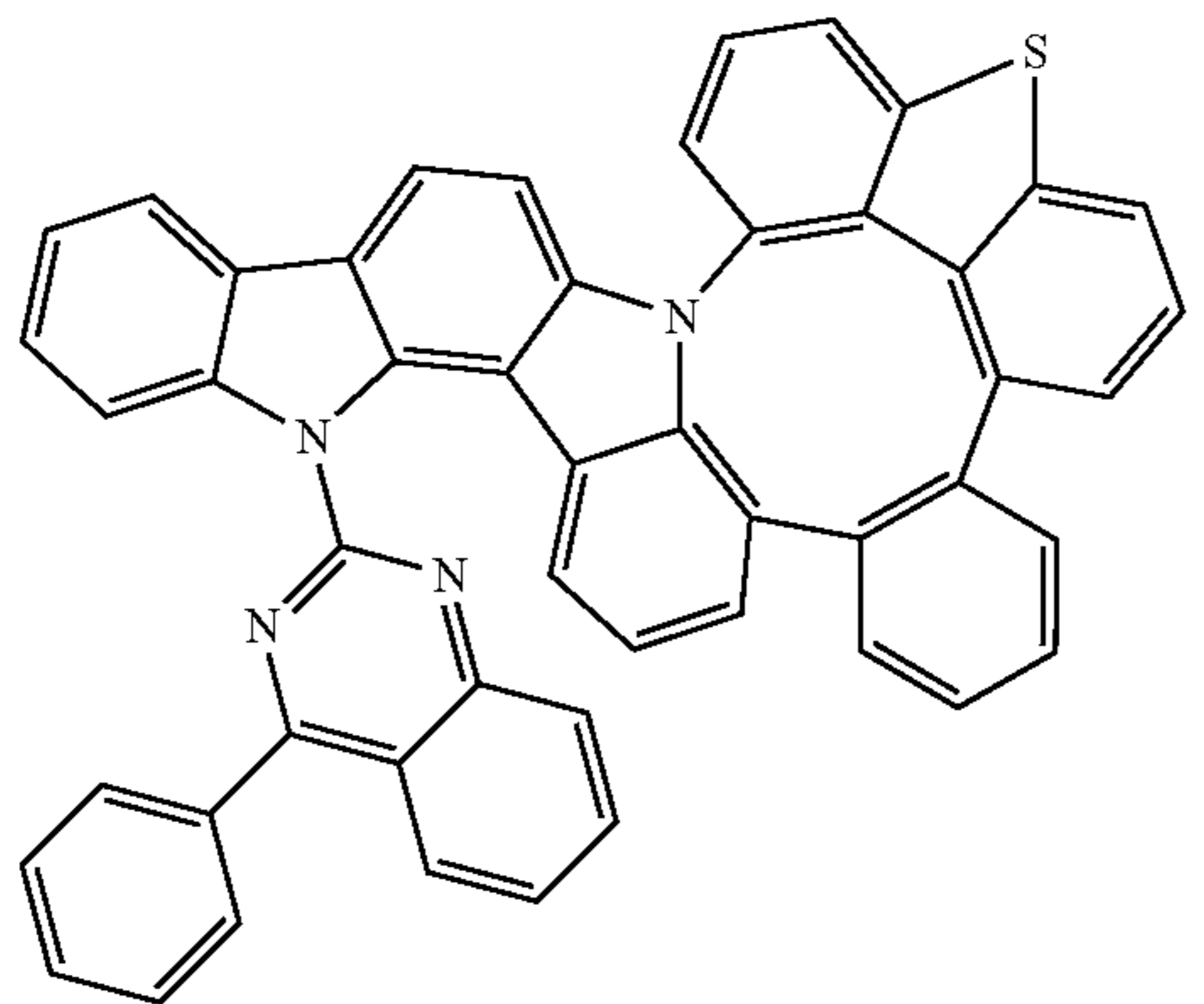
Compound 165
