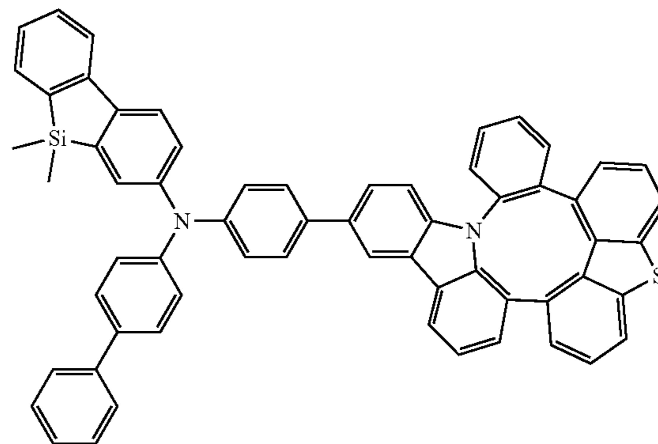
Compound 361
