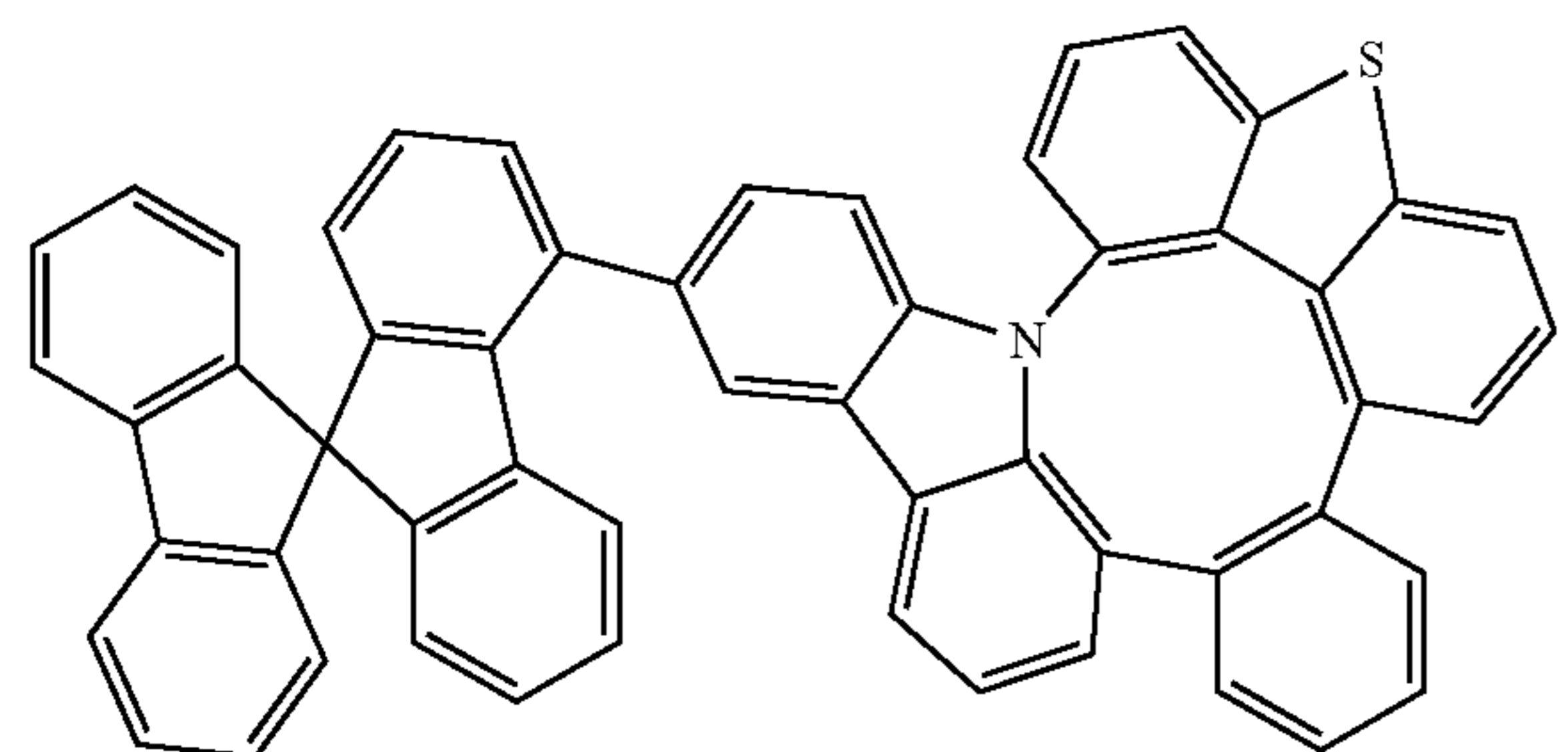
Compound 109
