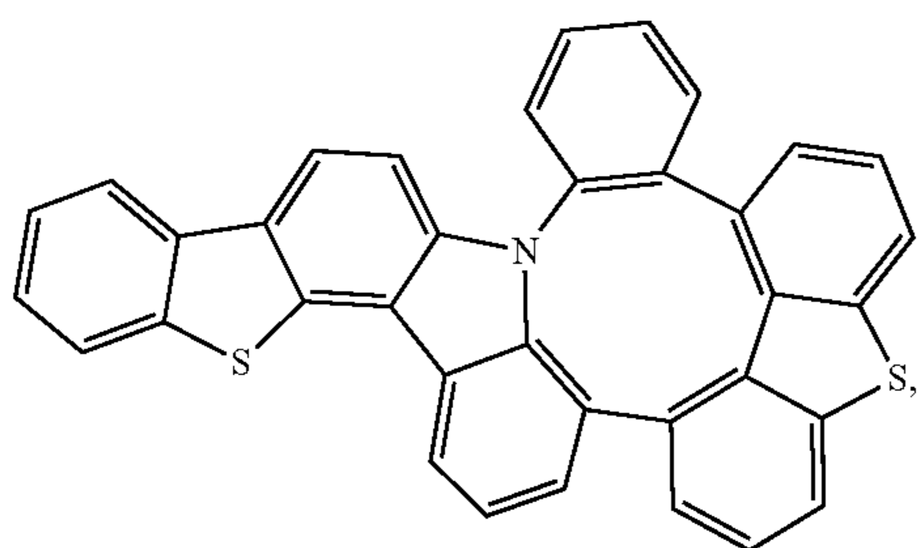
Compound 232
