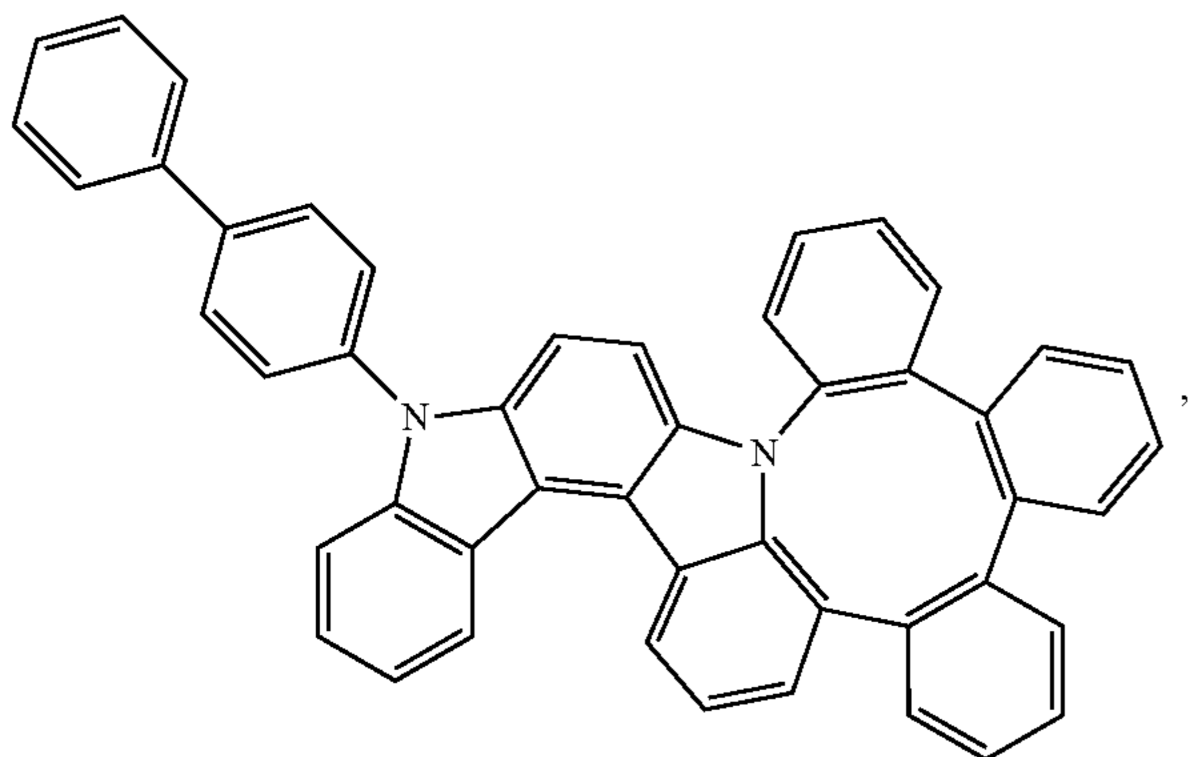
Compound 58
