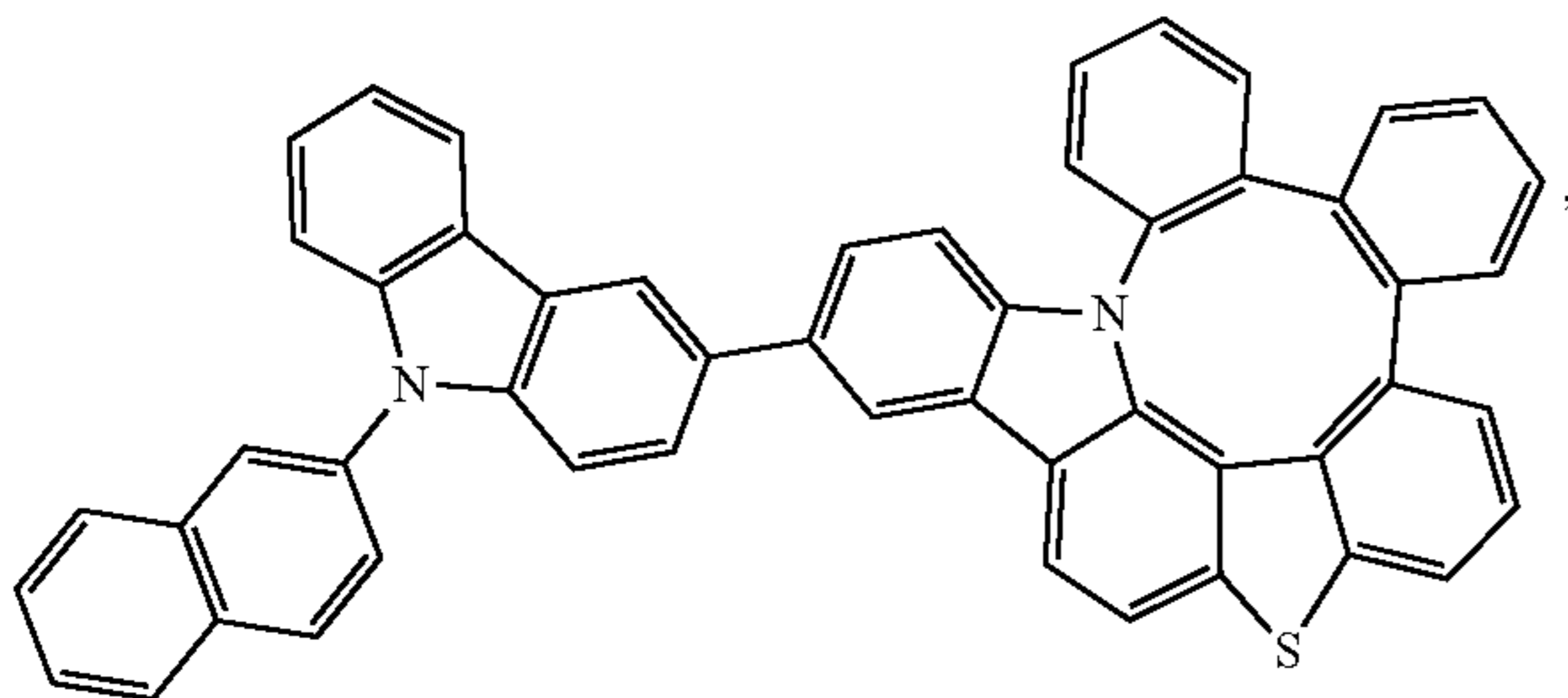
Compound 273
