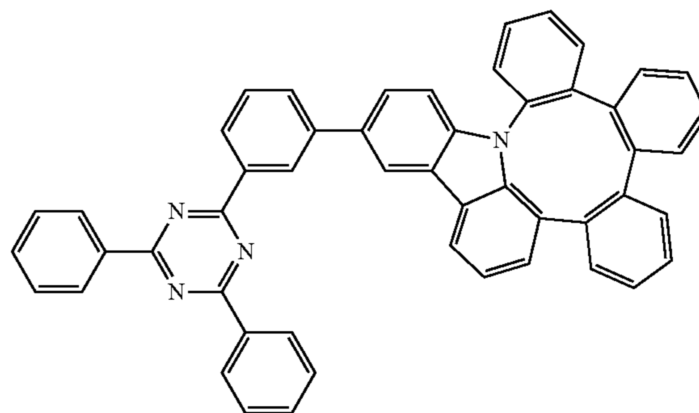
Compound 30
