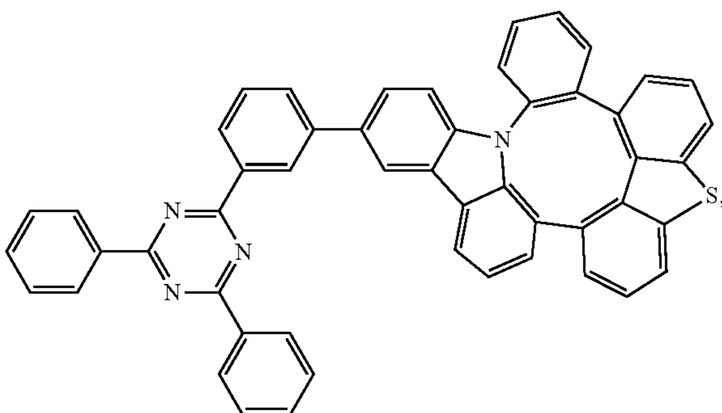
Compound 200
