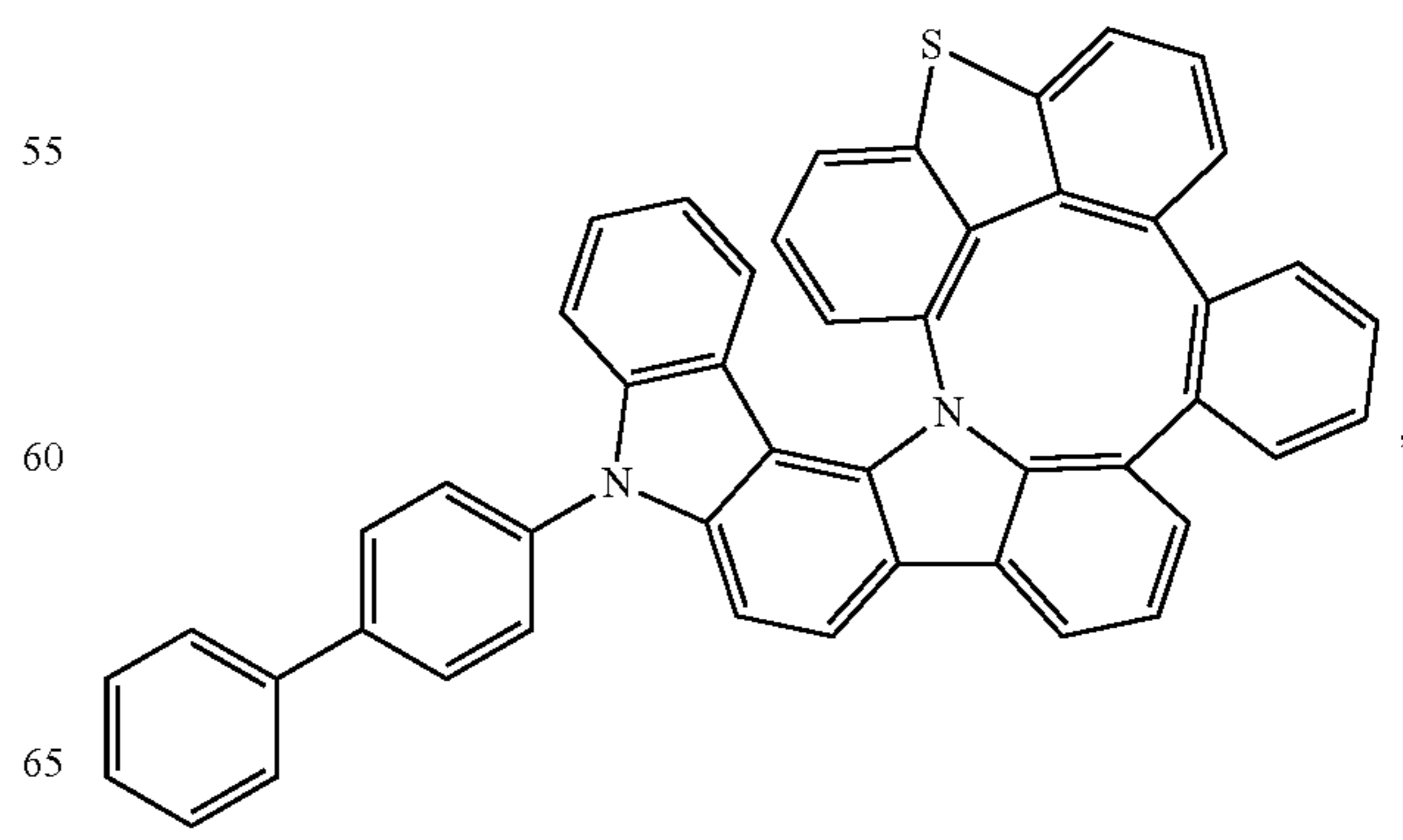
Compound 145
