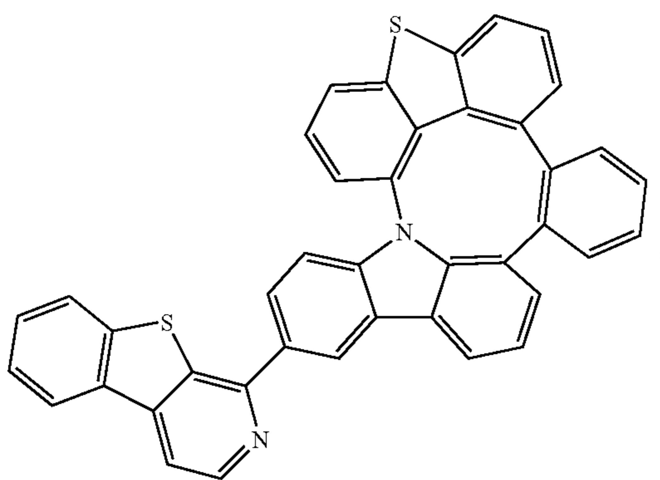
Compound 117
