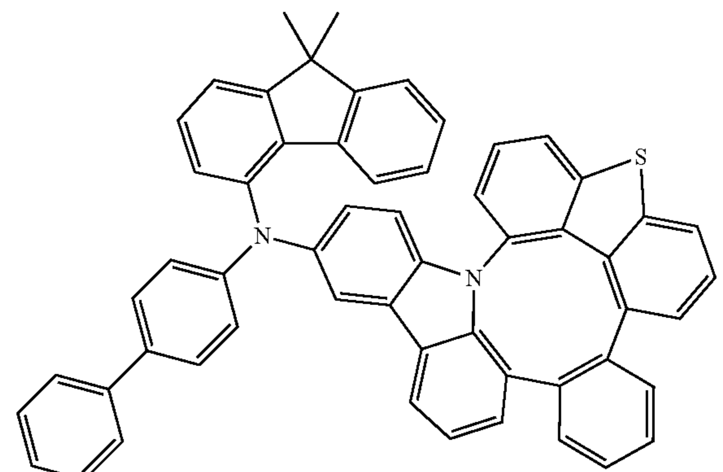
Compound 129
