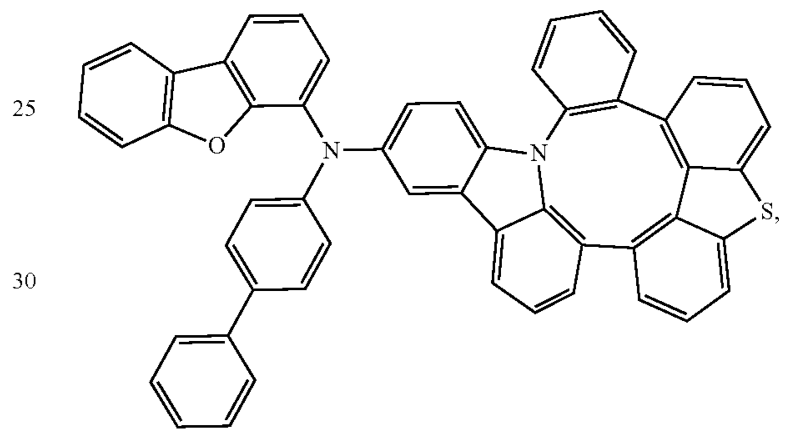
Compound 218
