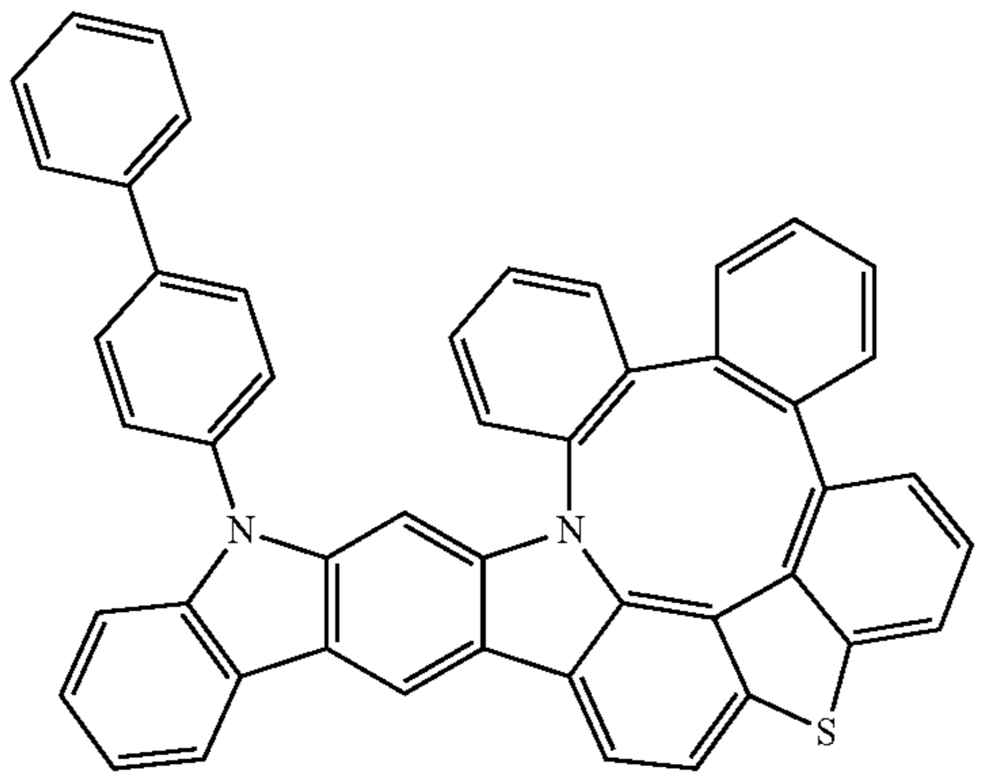
Compound 314
