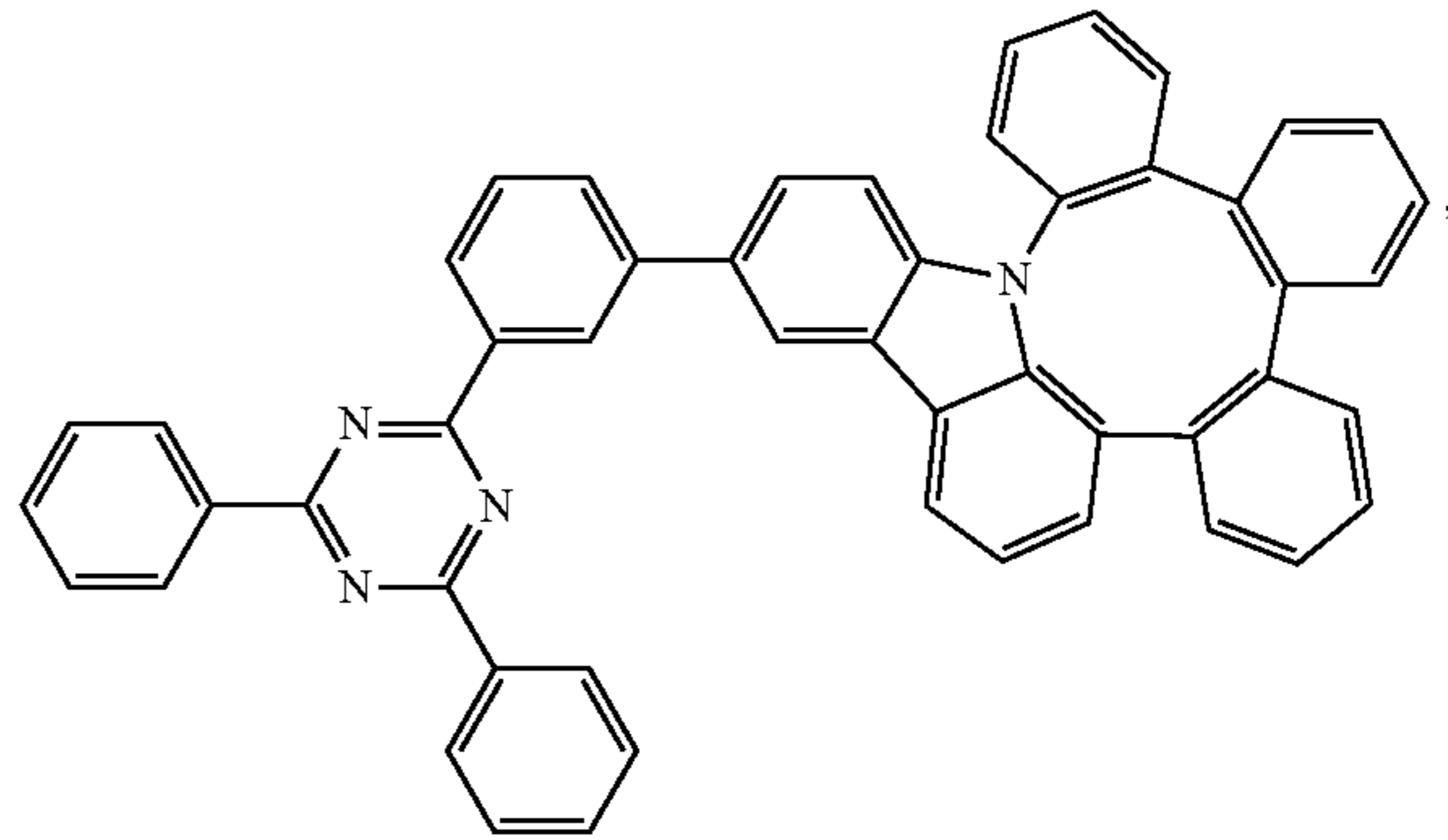
Compound 30
