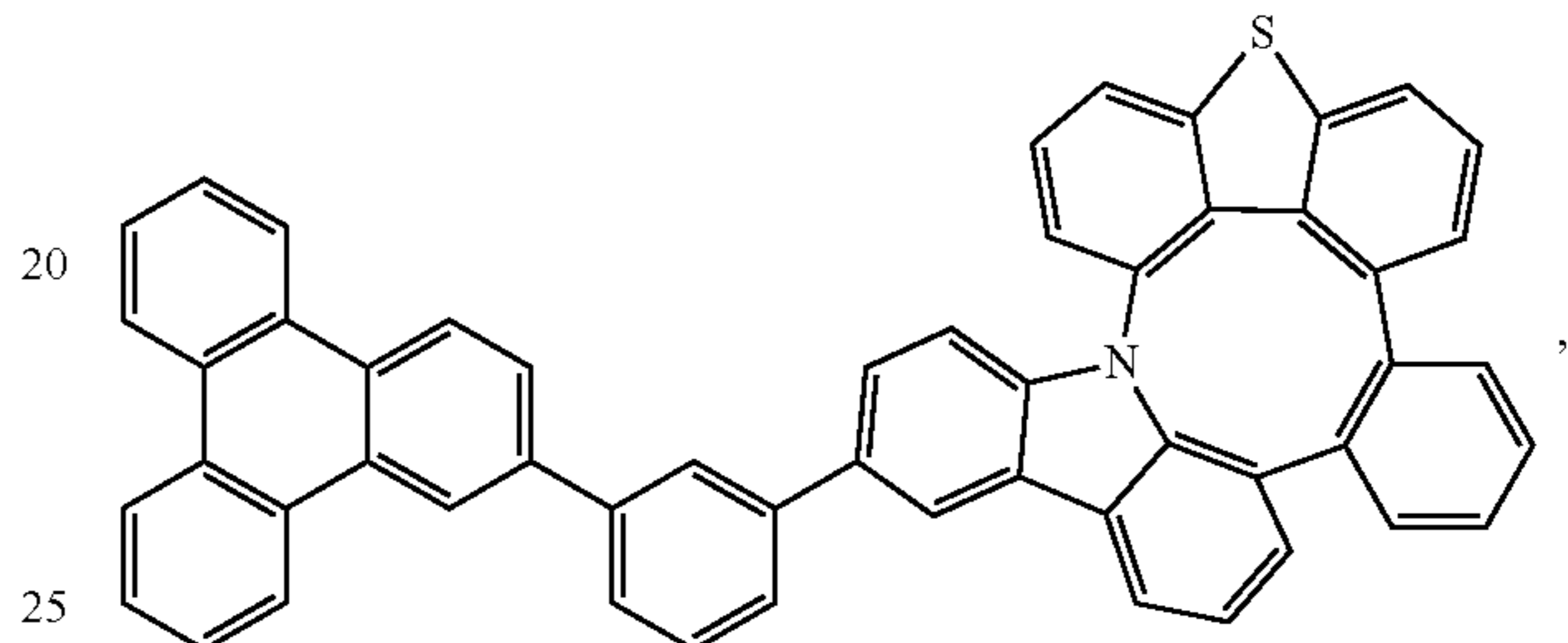
Compound 120
