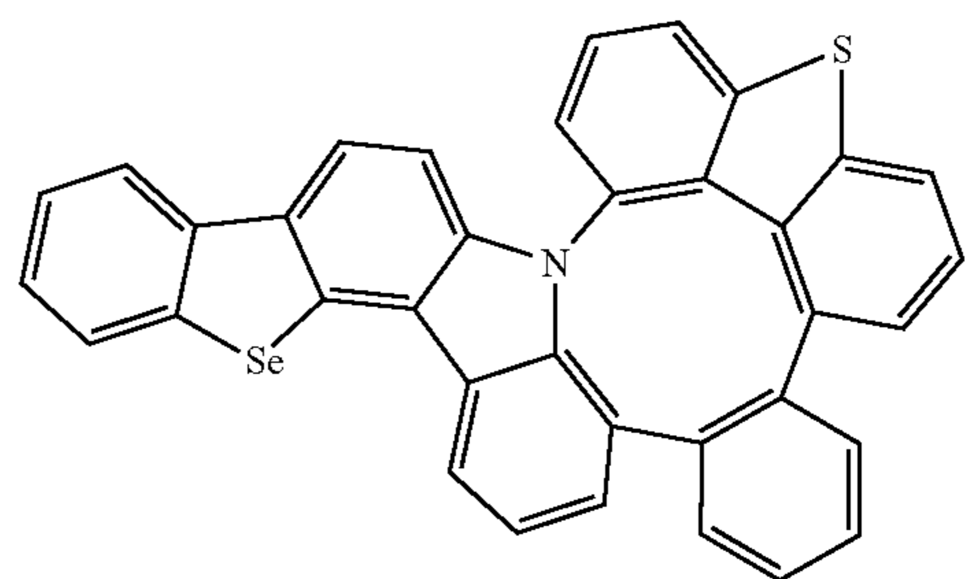
Compound 154
