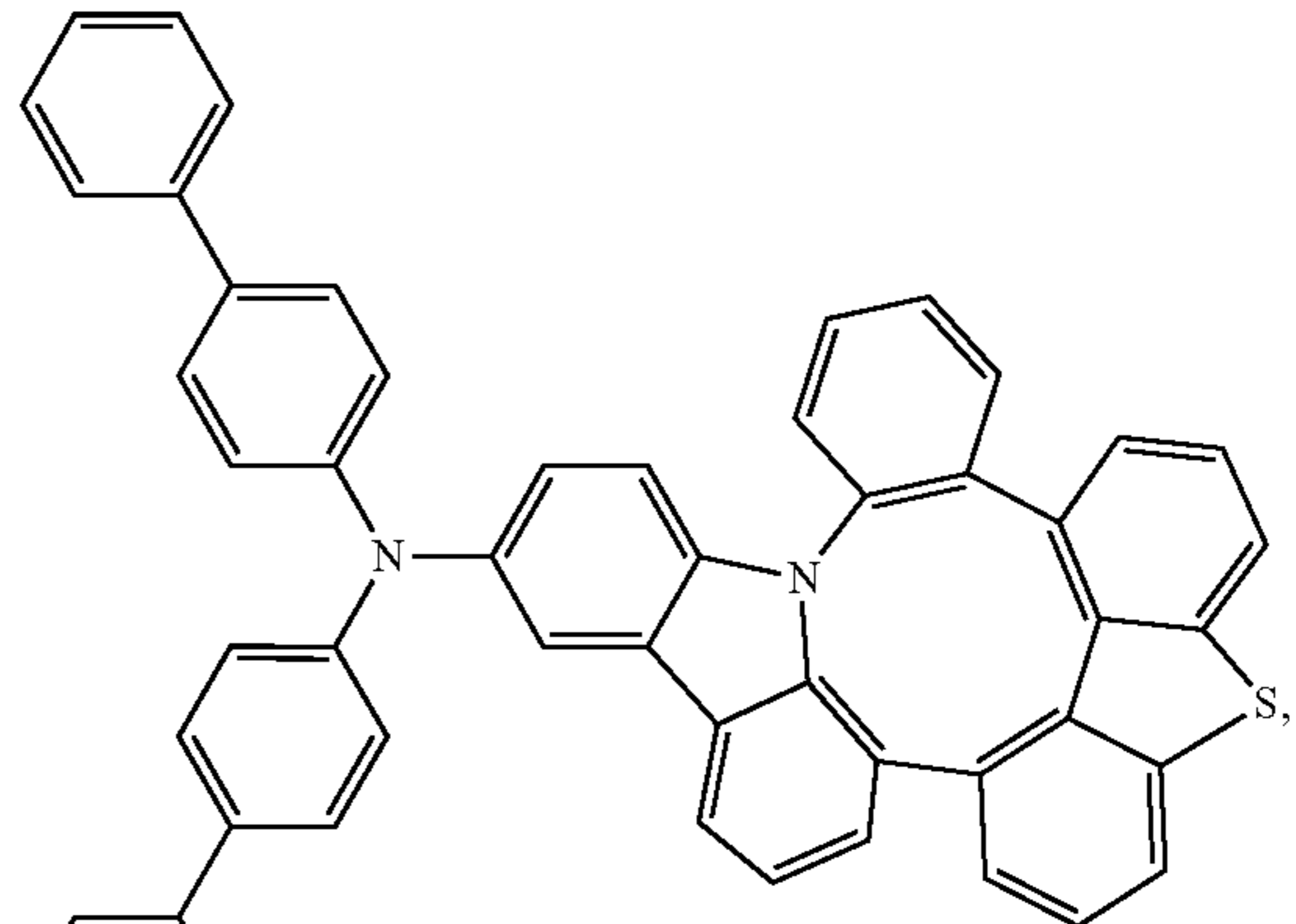
Compound 211
