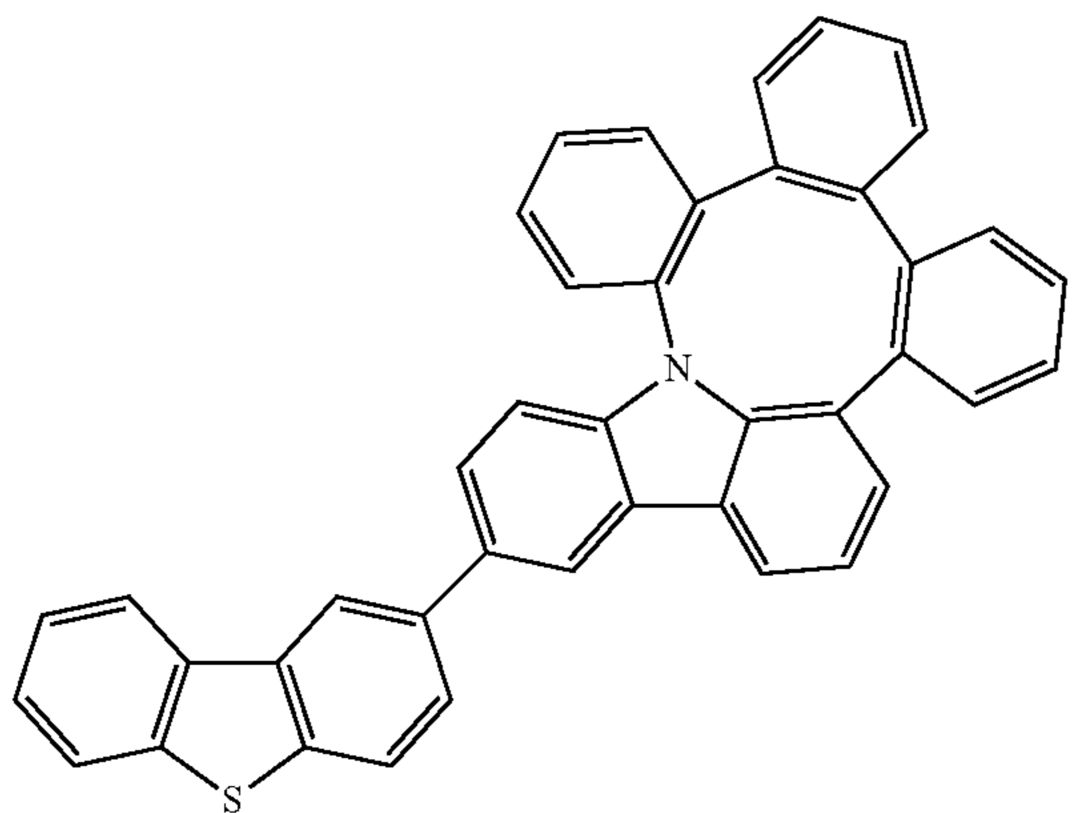
Compound 8
