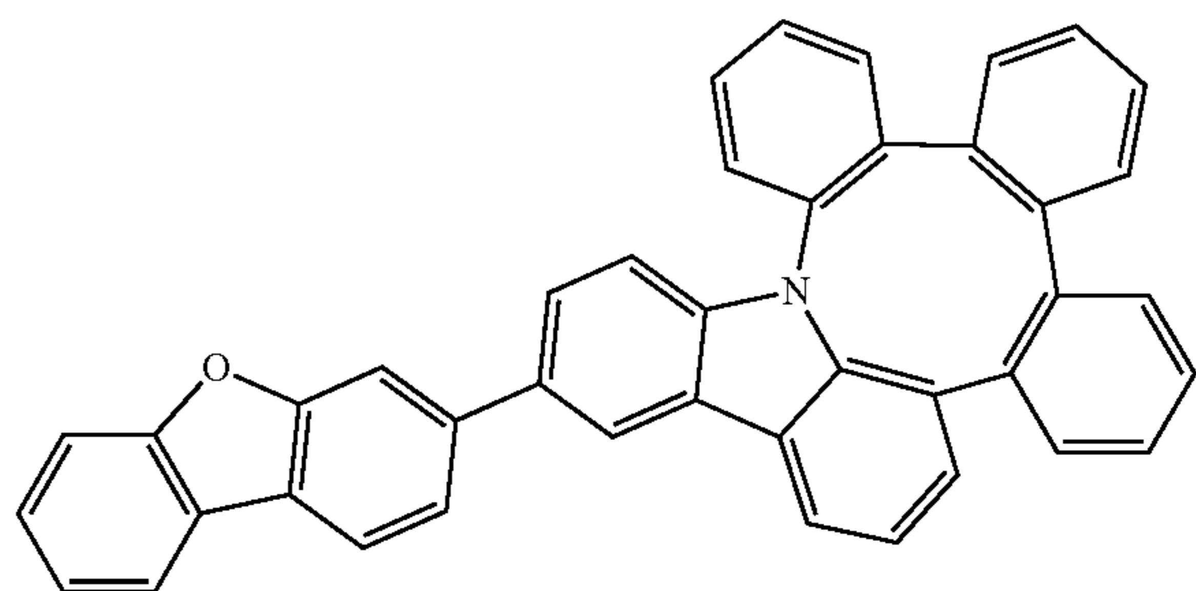
Compound 7
