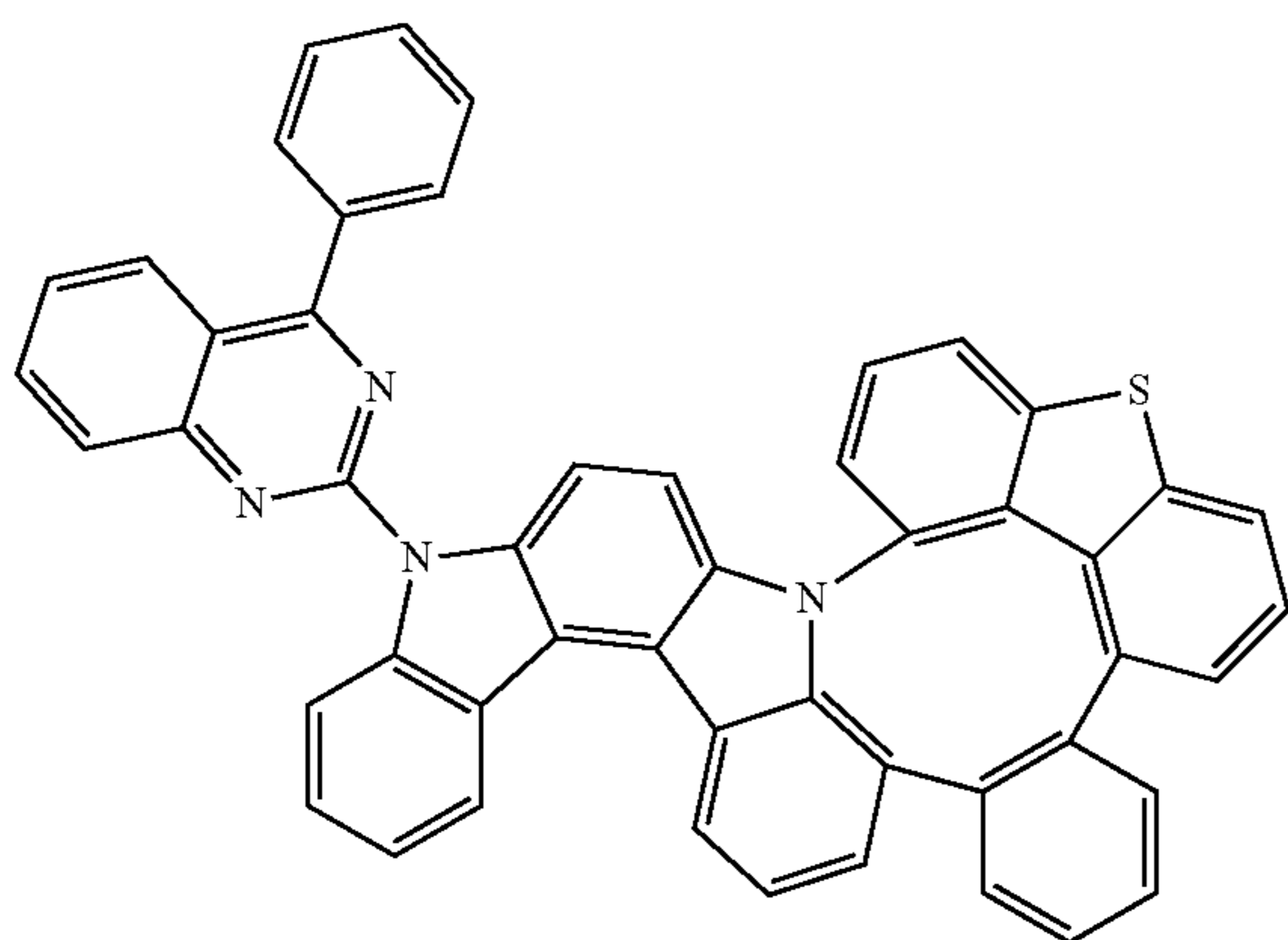
Compound 166
