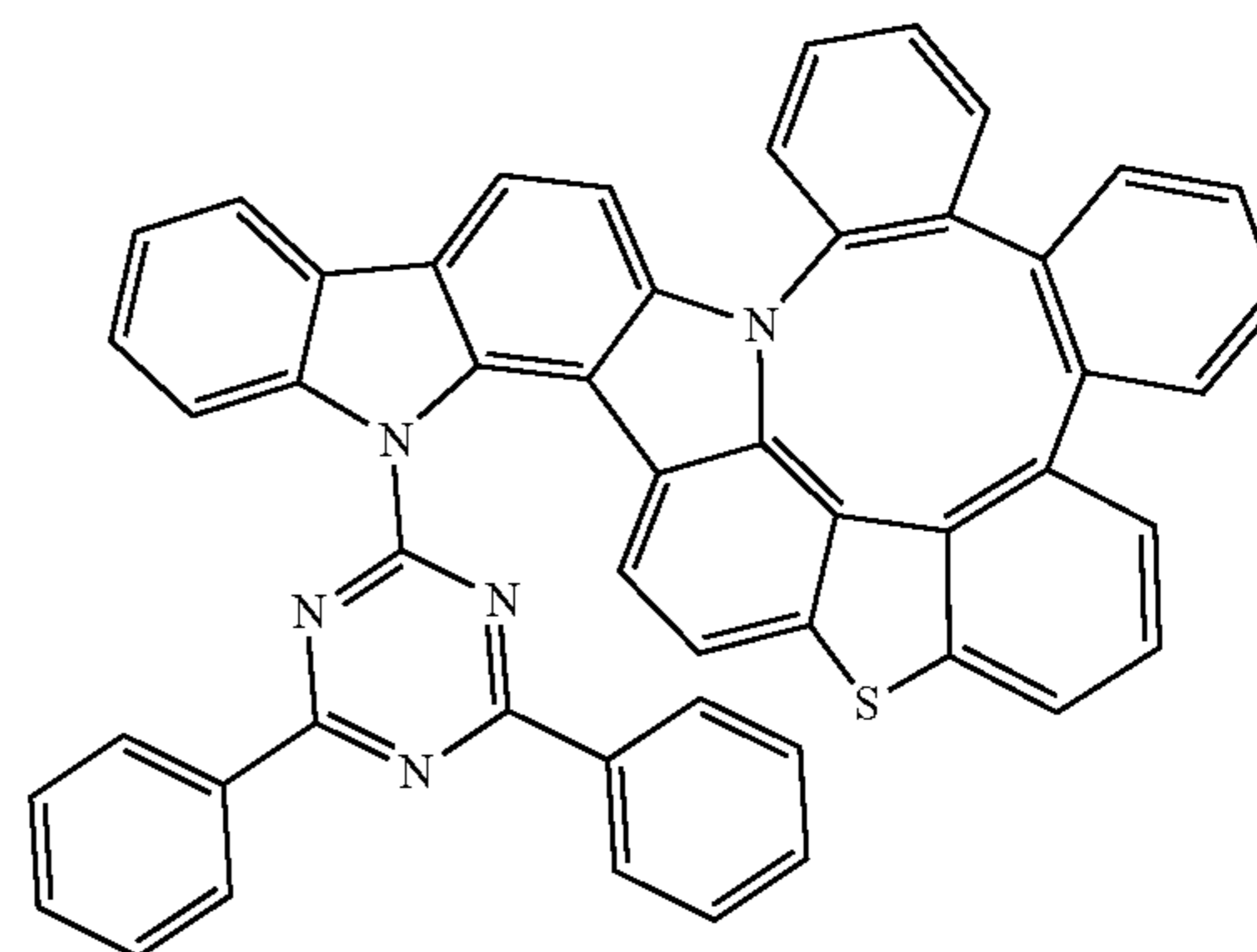
Compound 330
