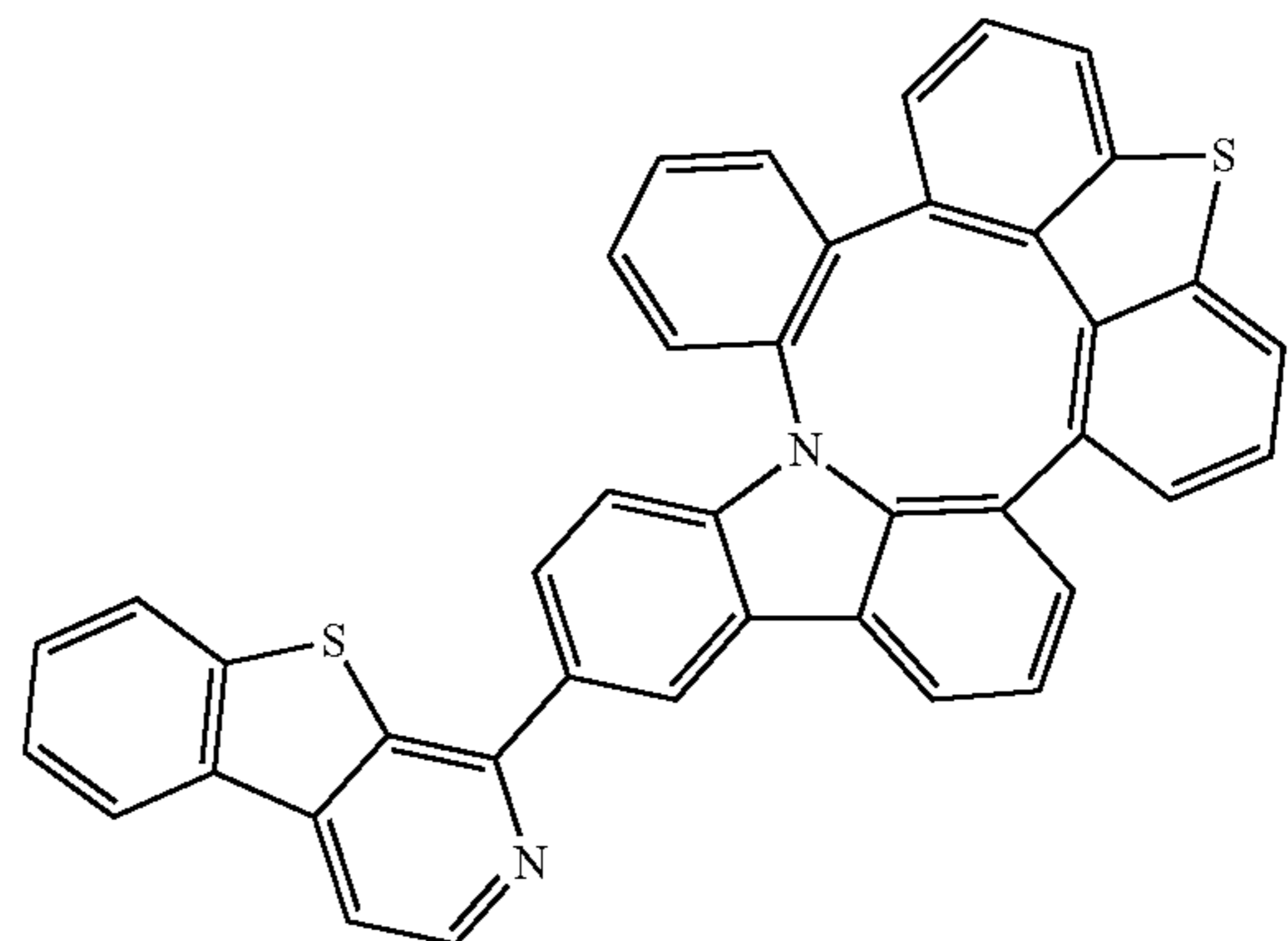
Compound 202
