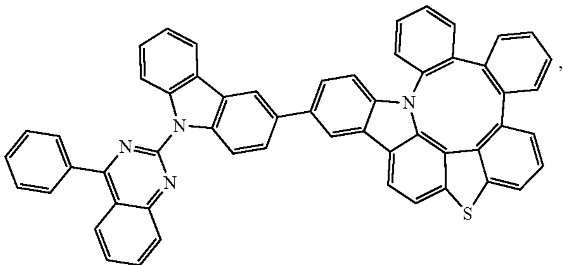
Compound 275
