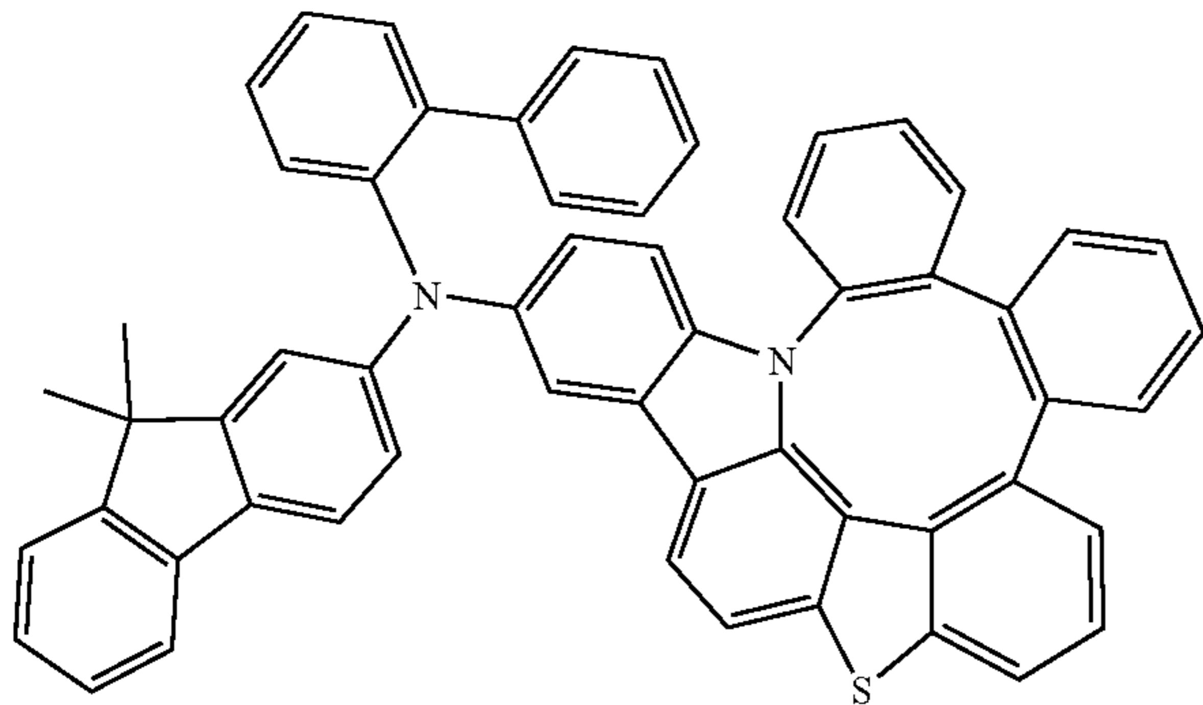
Compound 299
