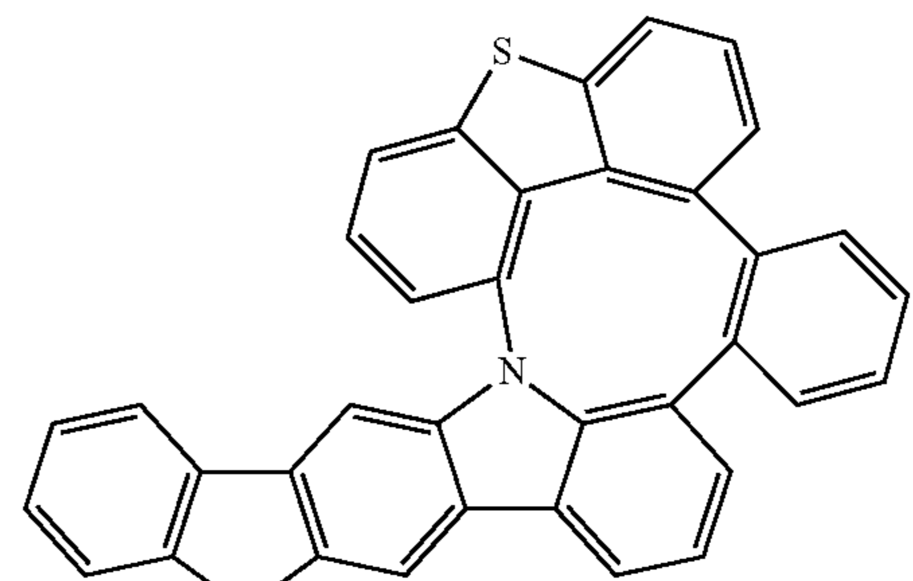
Compound 168
