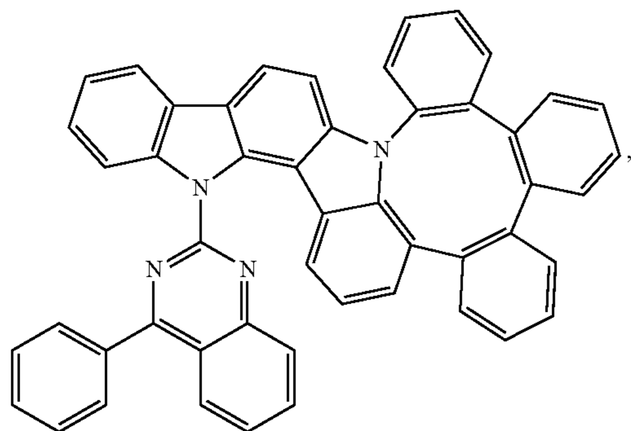
Compound 80
