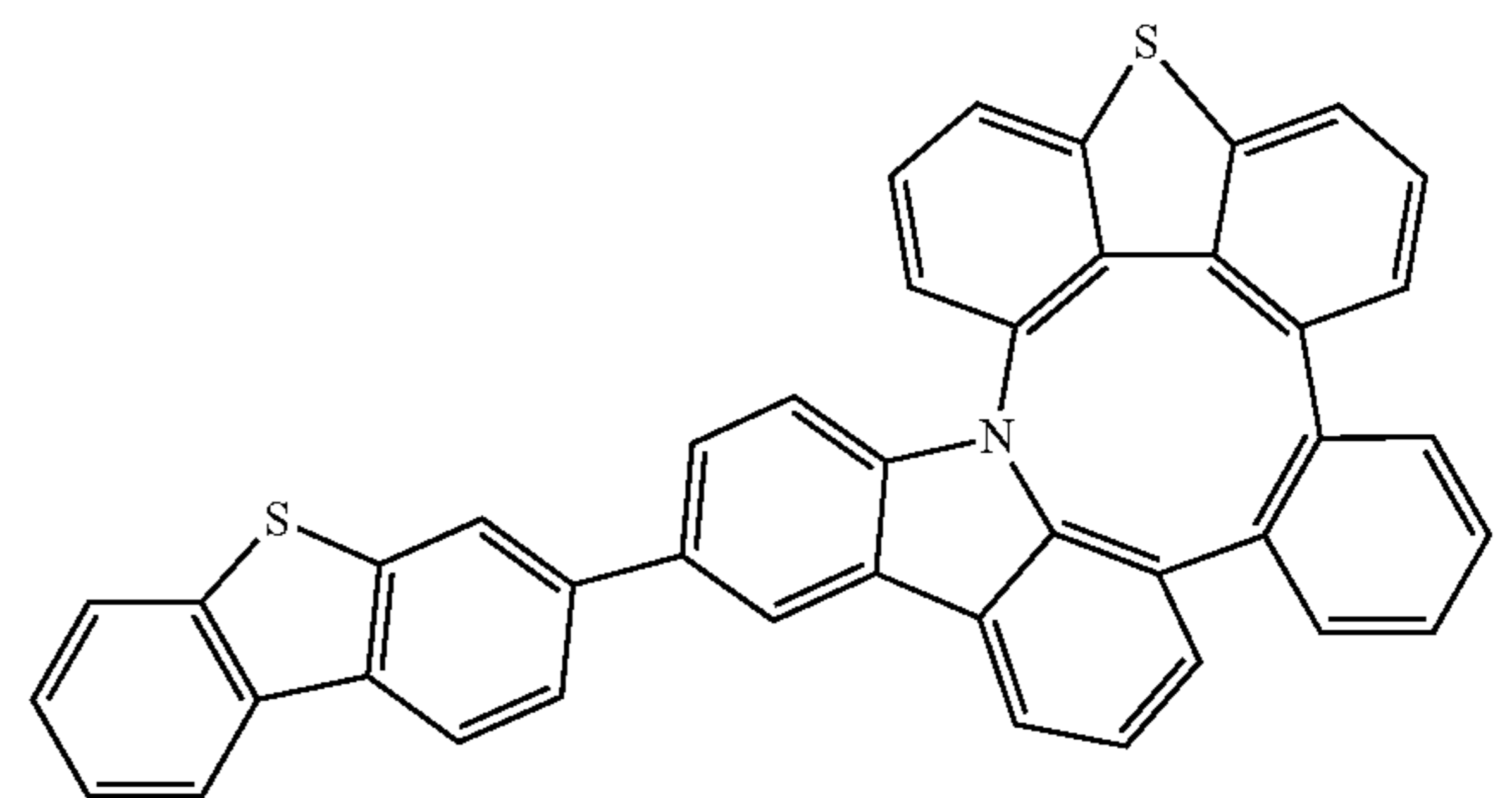
Compound 95
