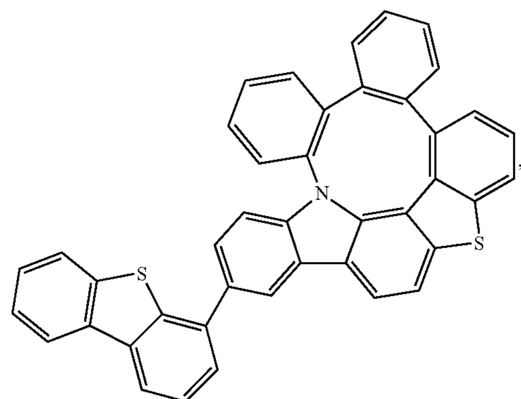
Compound 262
