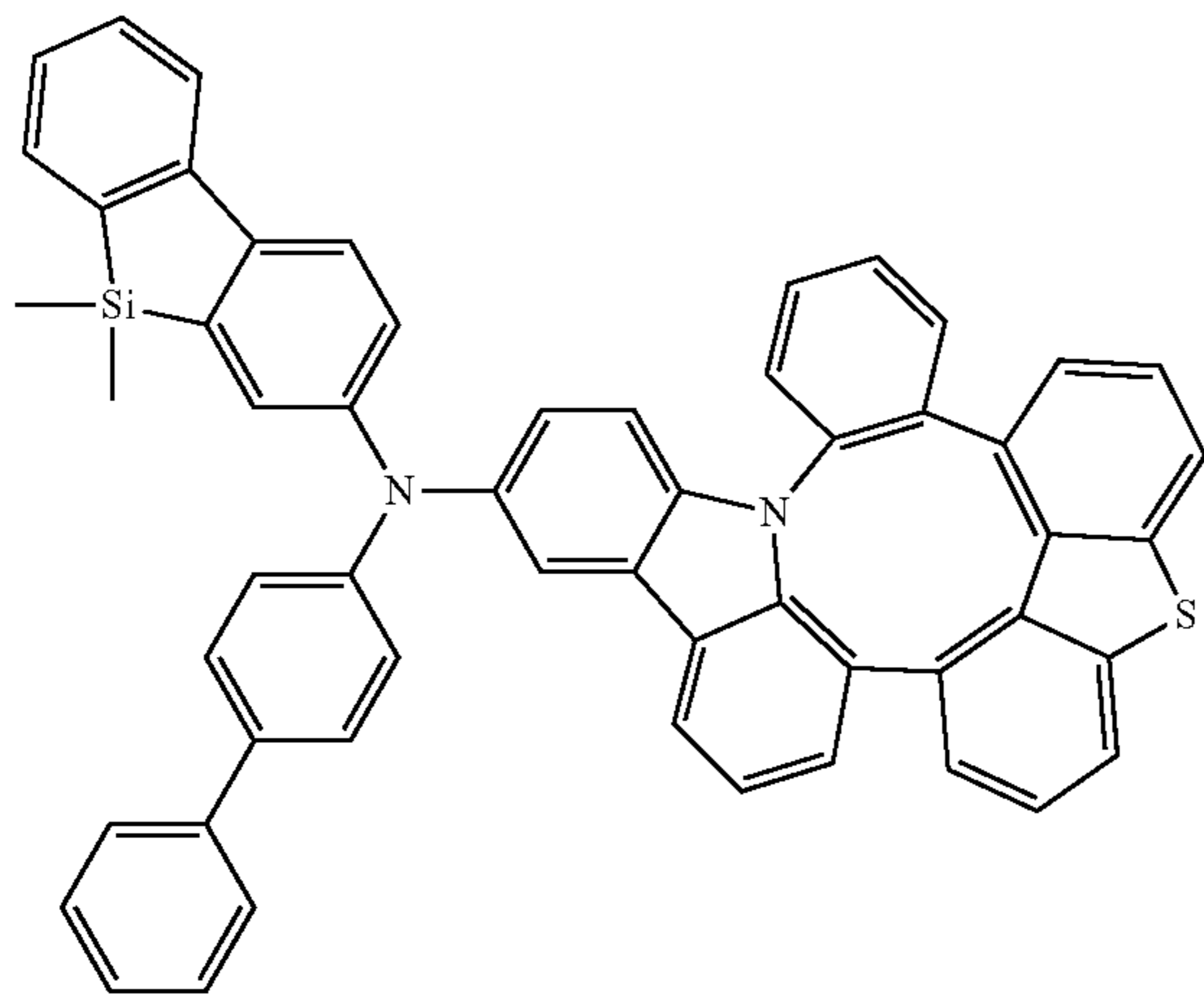
Compound 358
