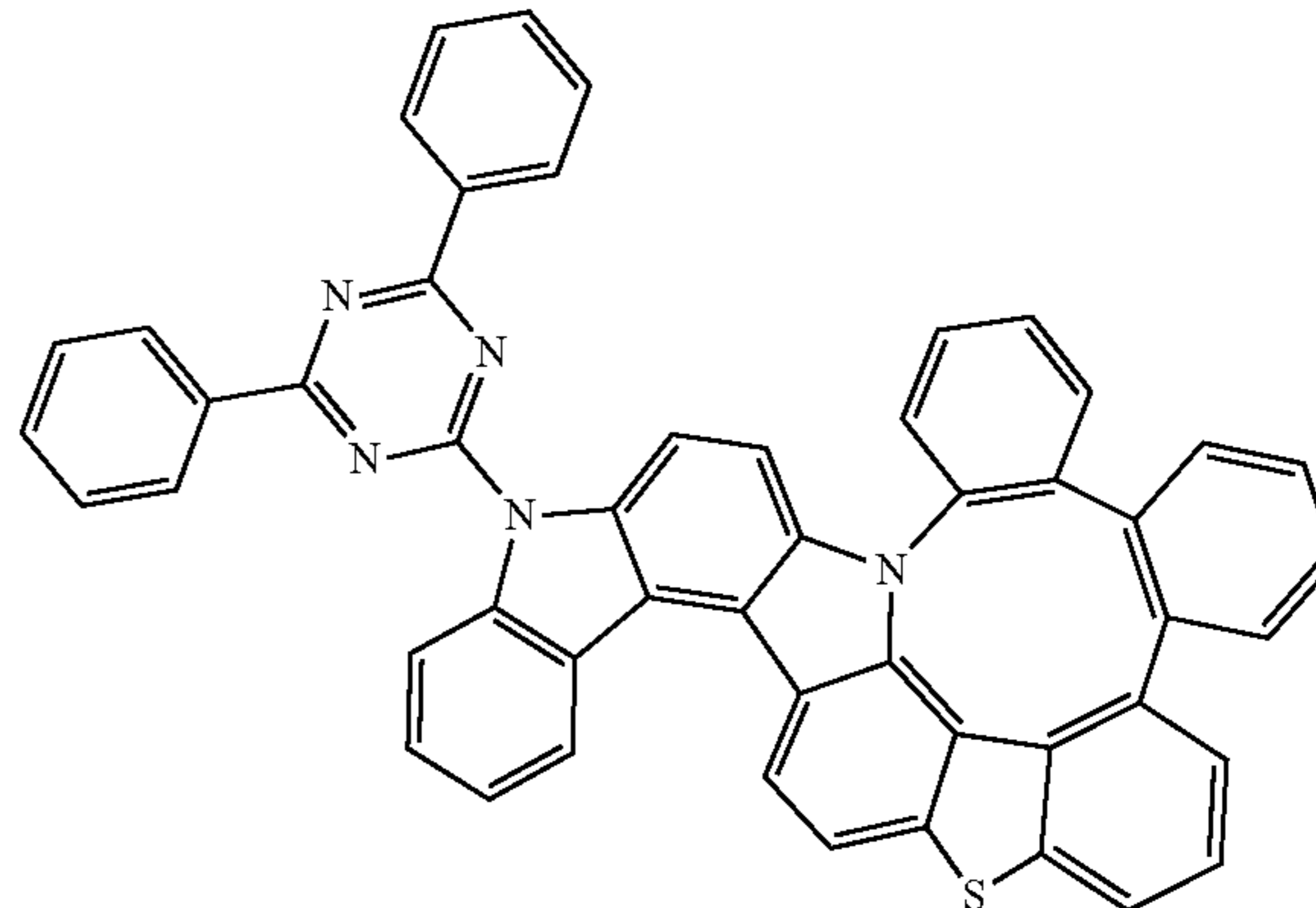
Compound 330
