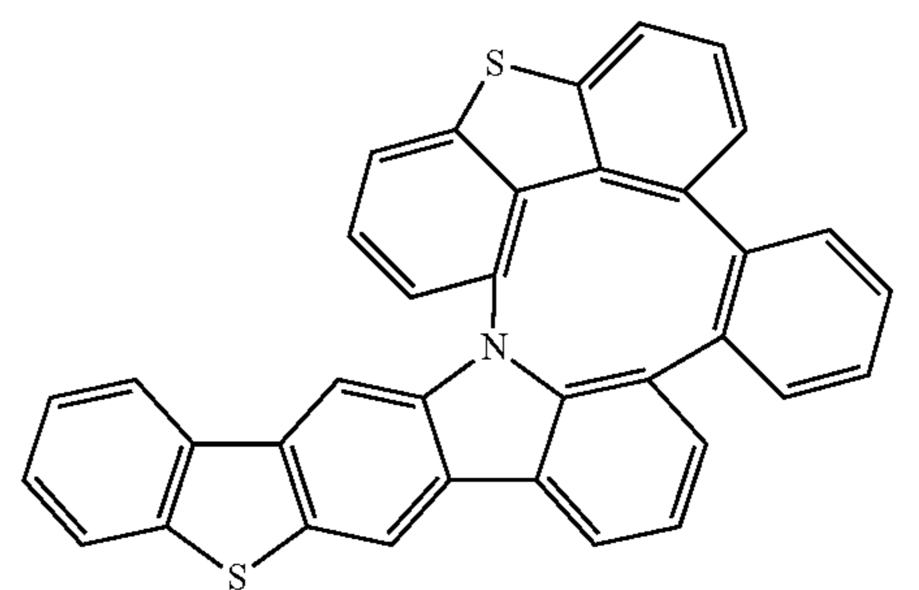
Compound 151
