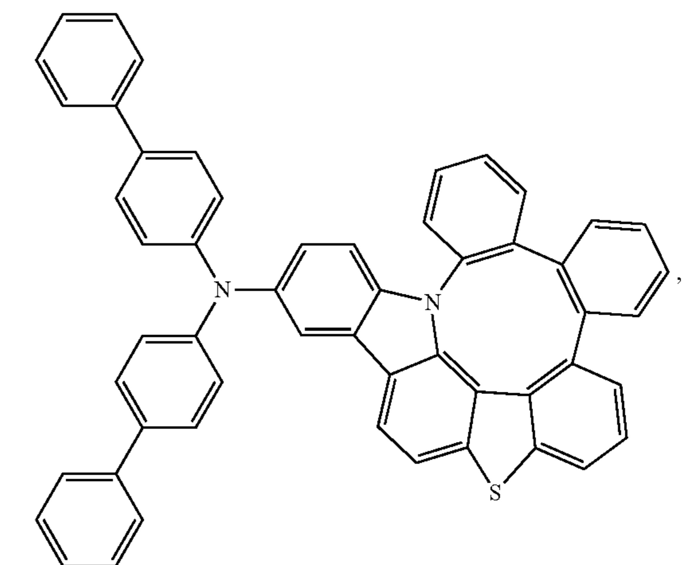
Compound 296
