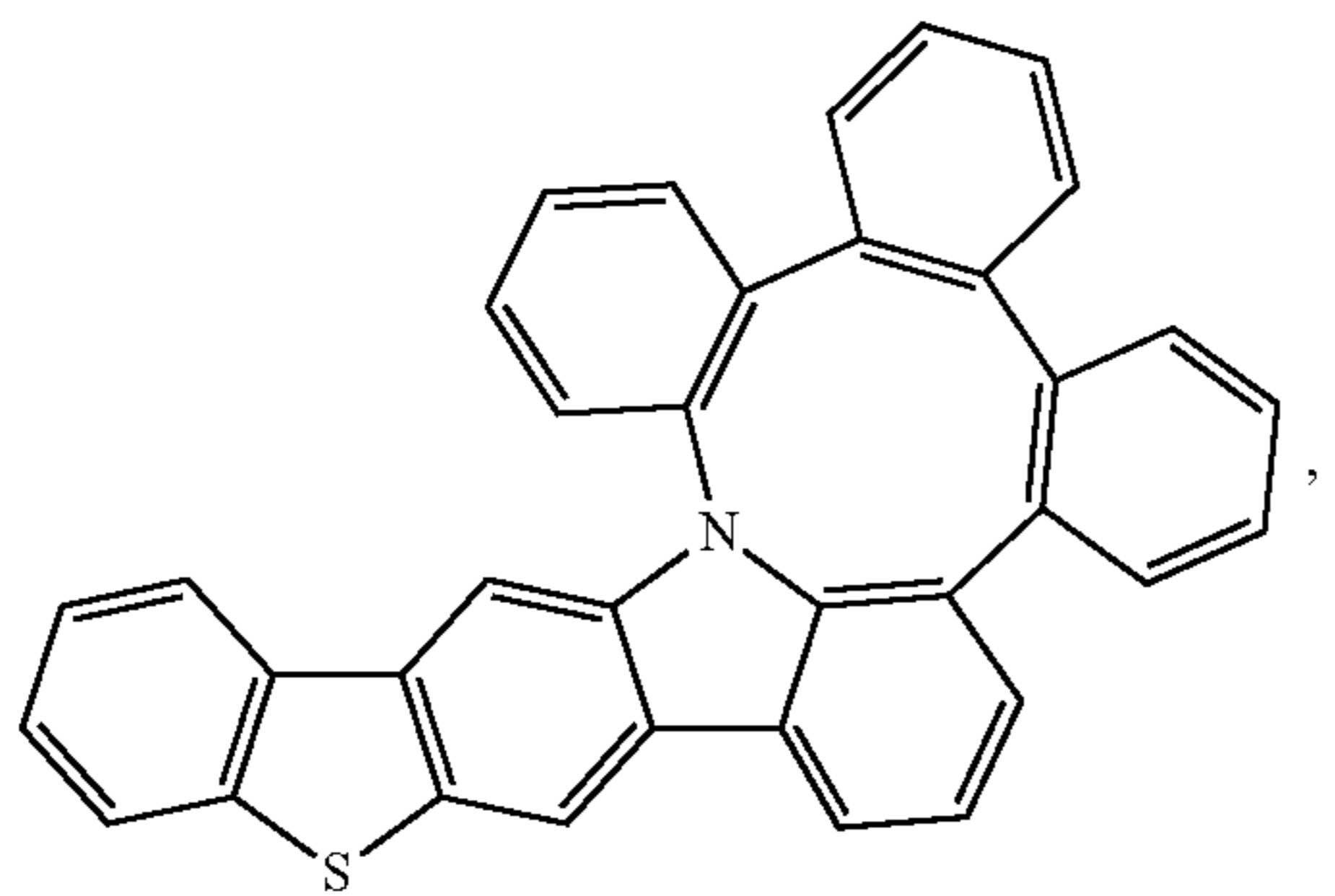
Compound 67
