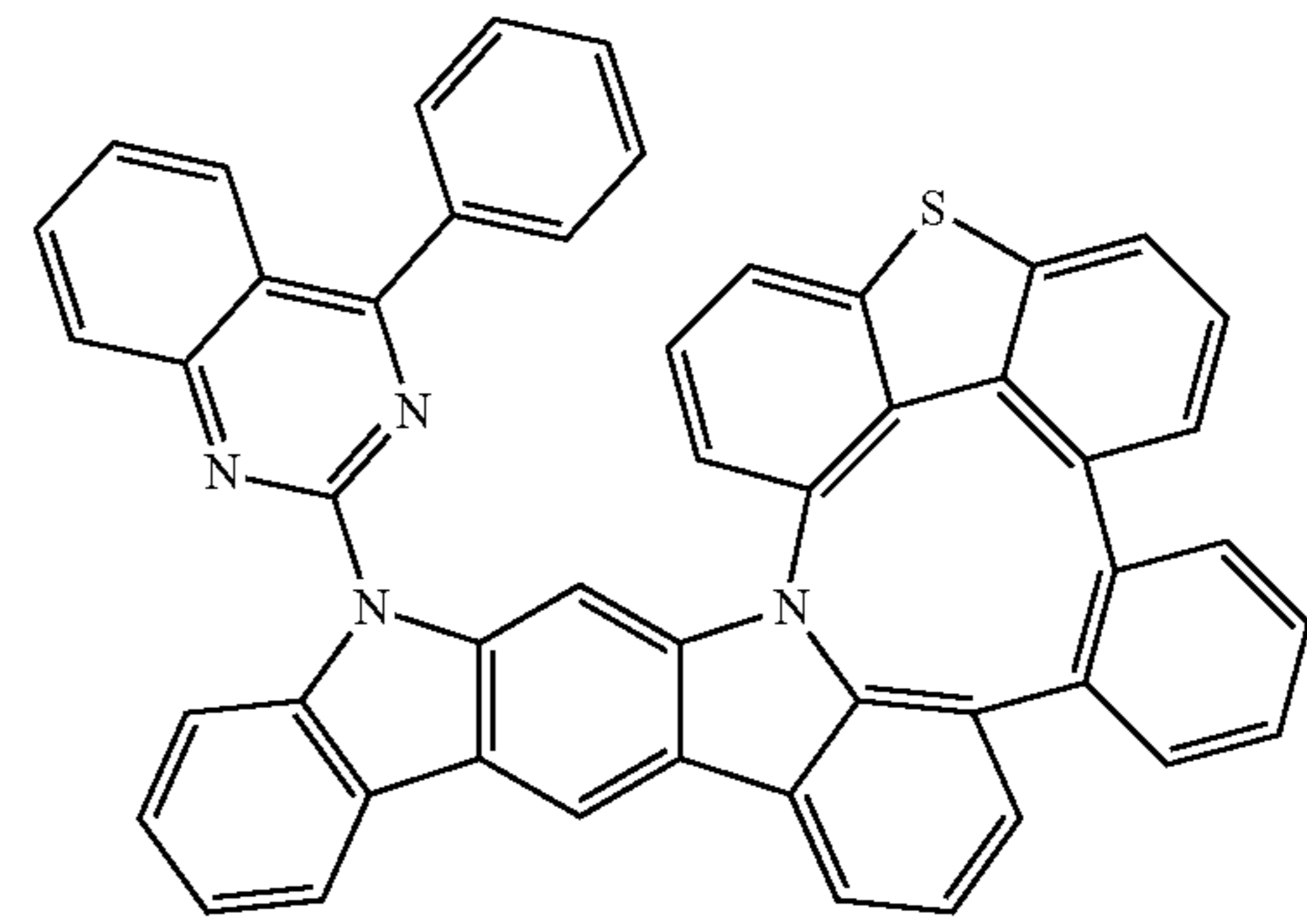
Compound 168
