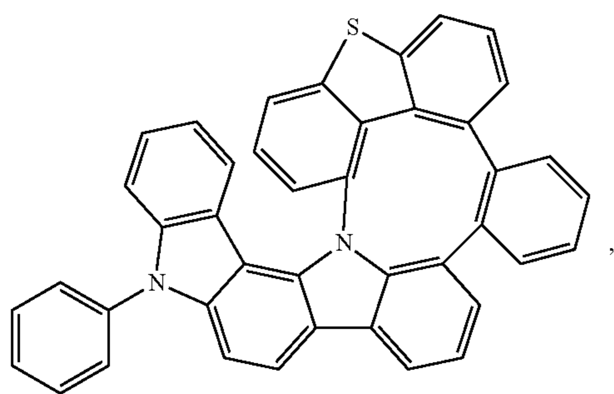
Compound 139
