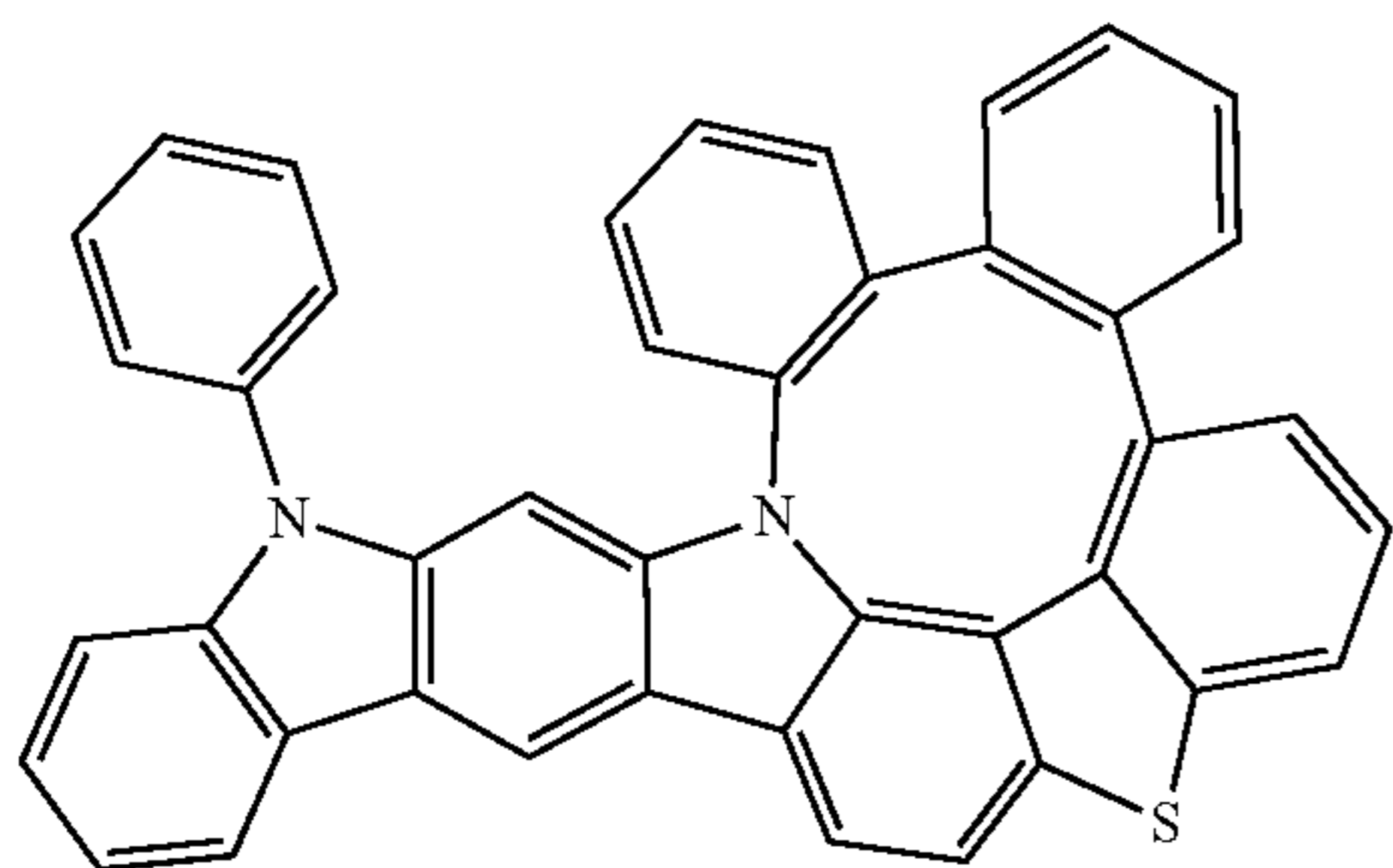
Compound 307
