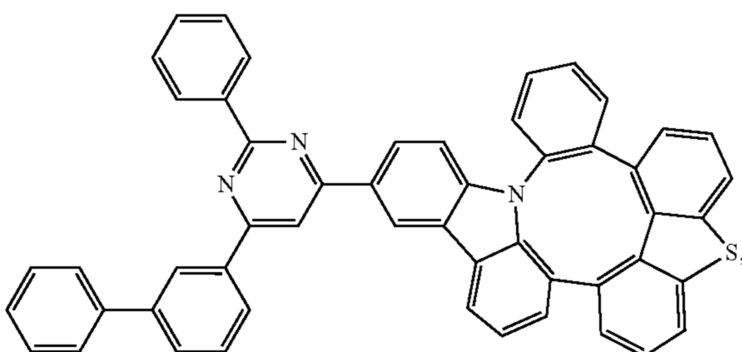
Compound 200
