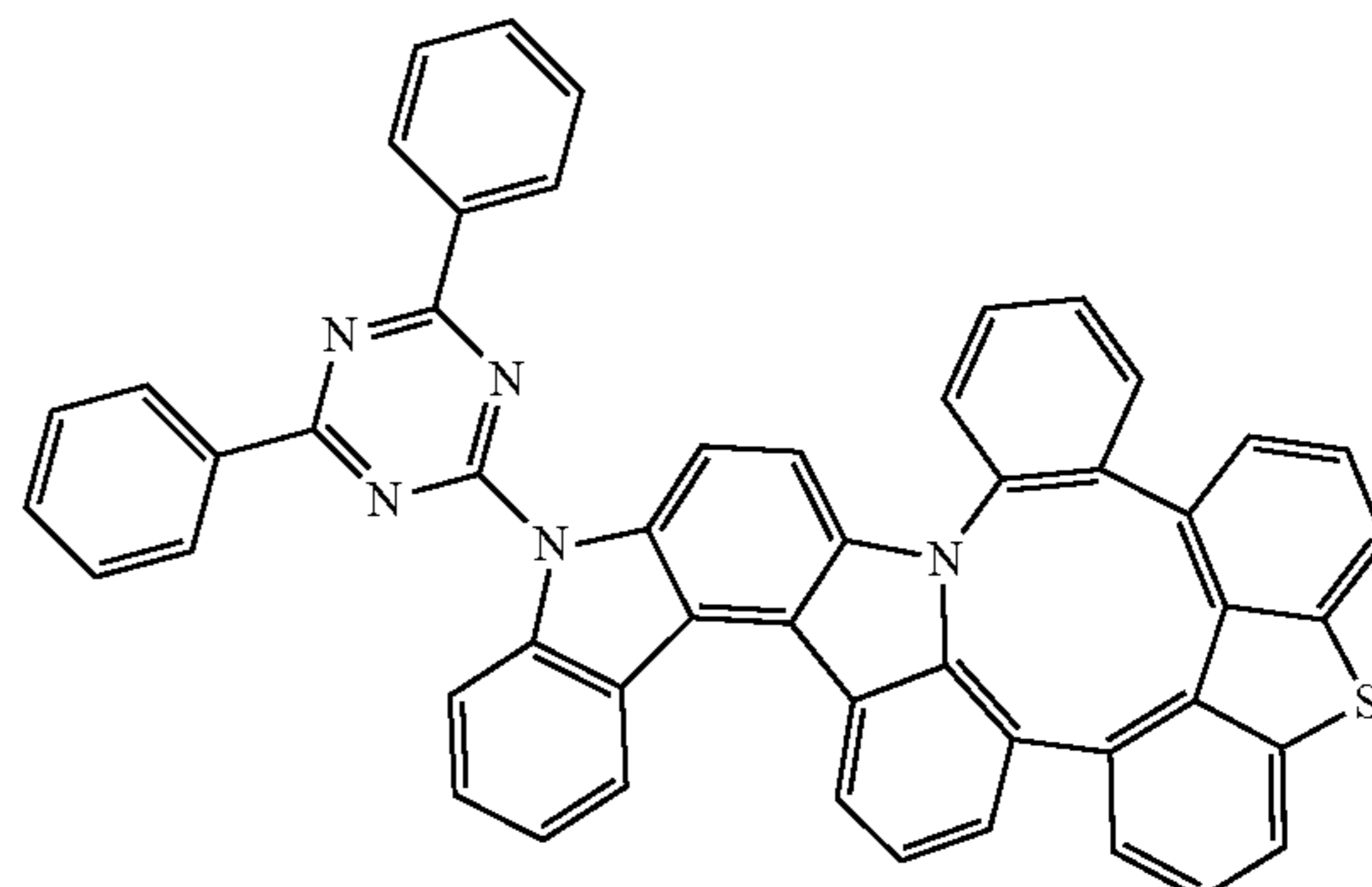
Compound 246
