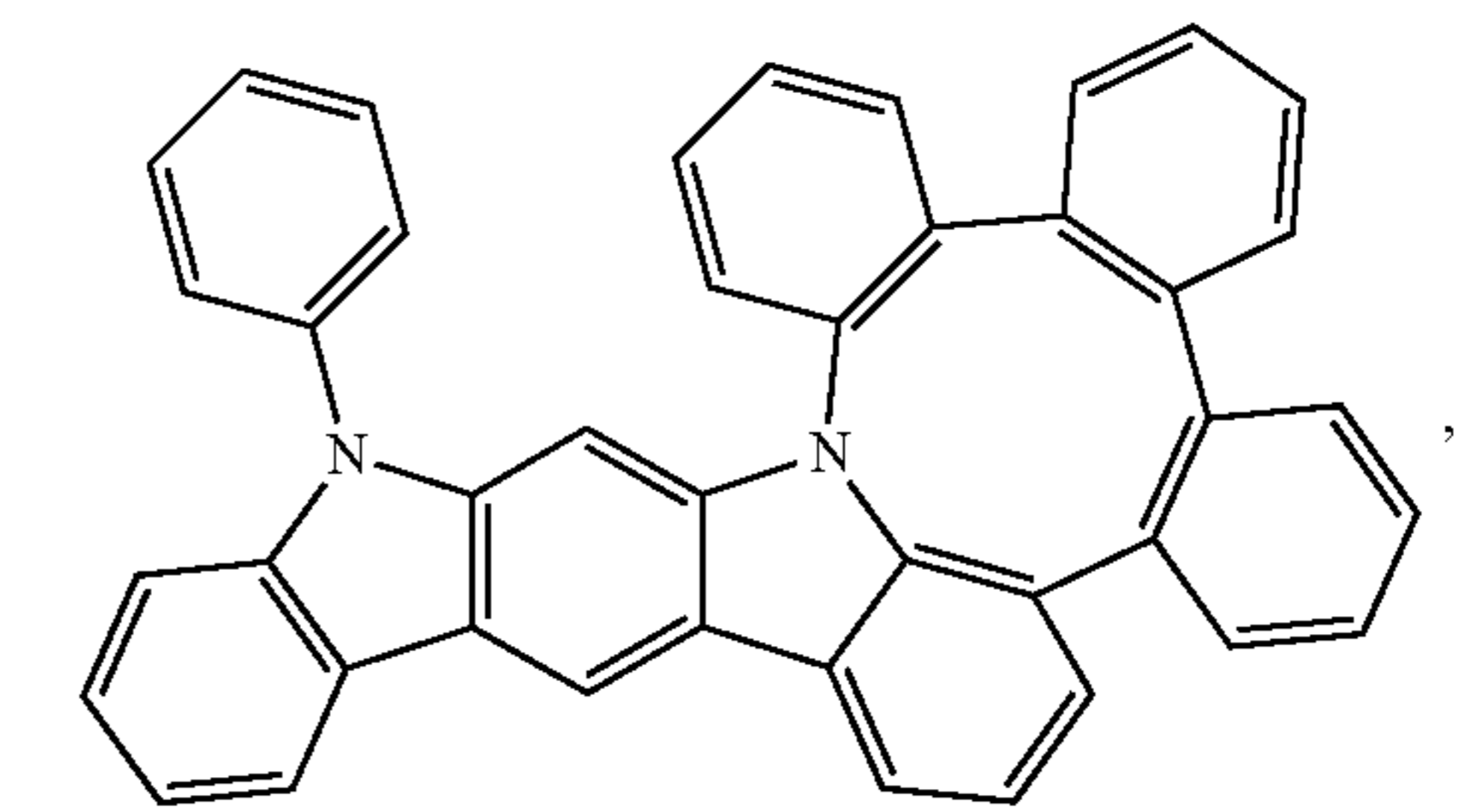
Compound 52
