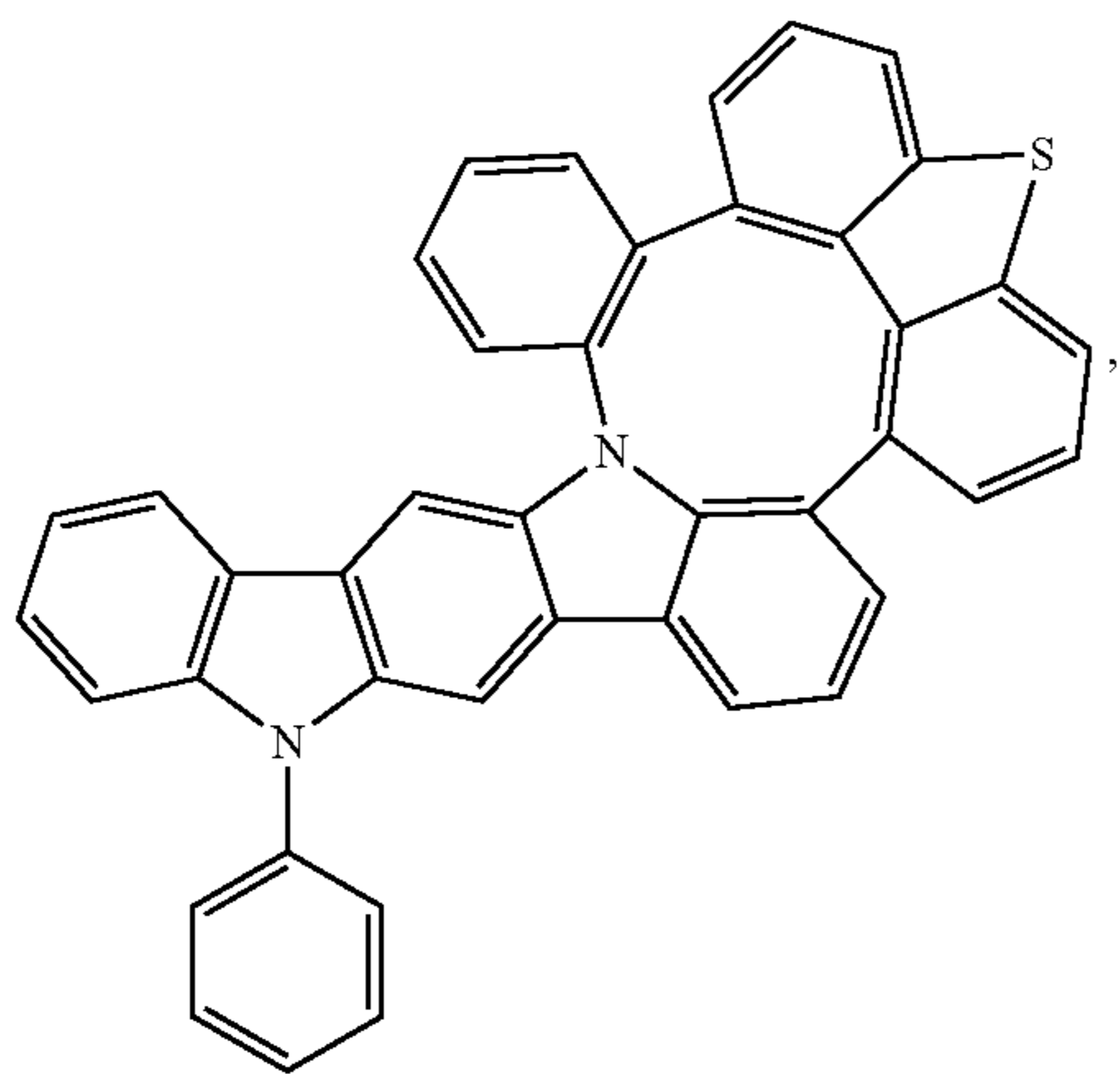
Compound 223
