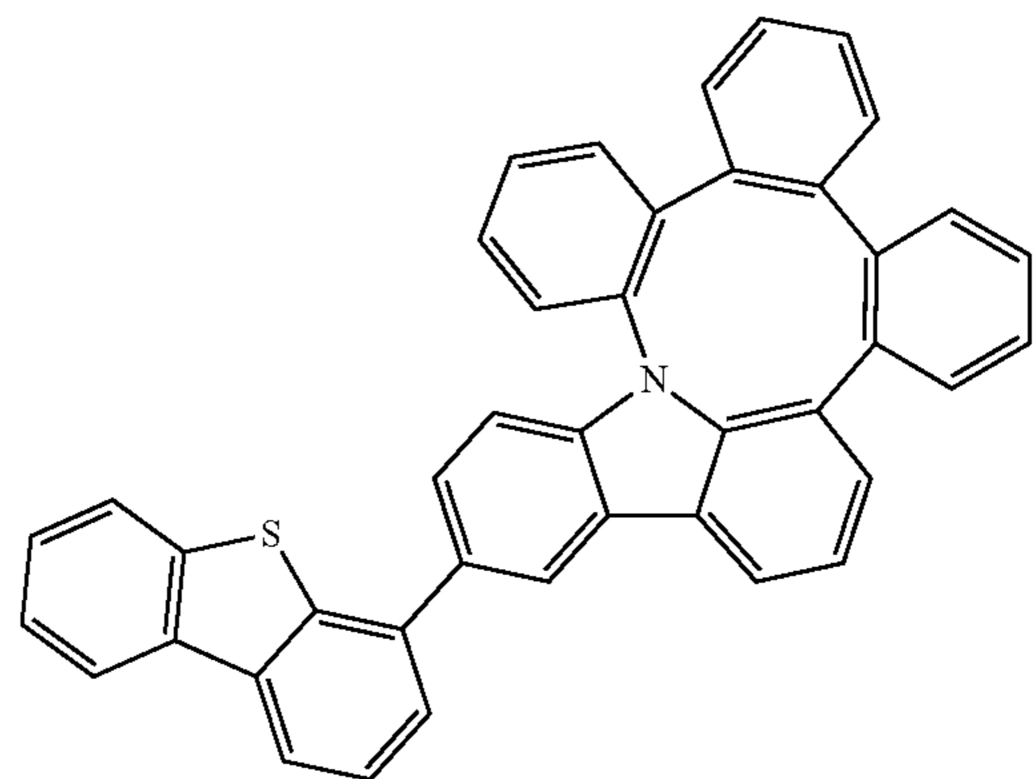
Compound 7
