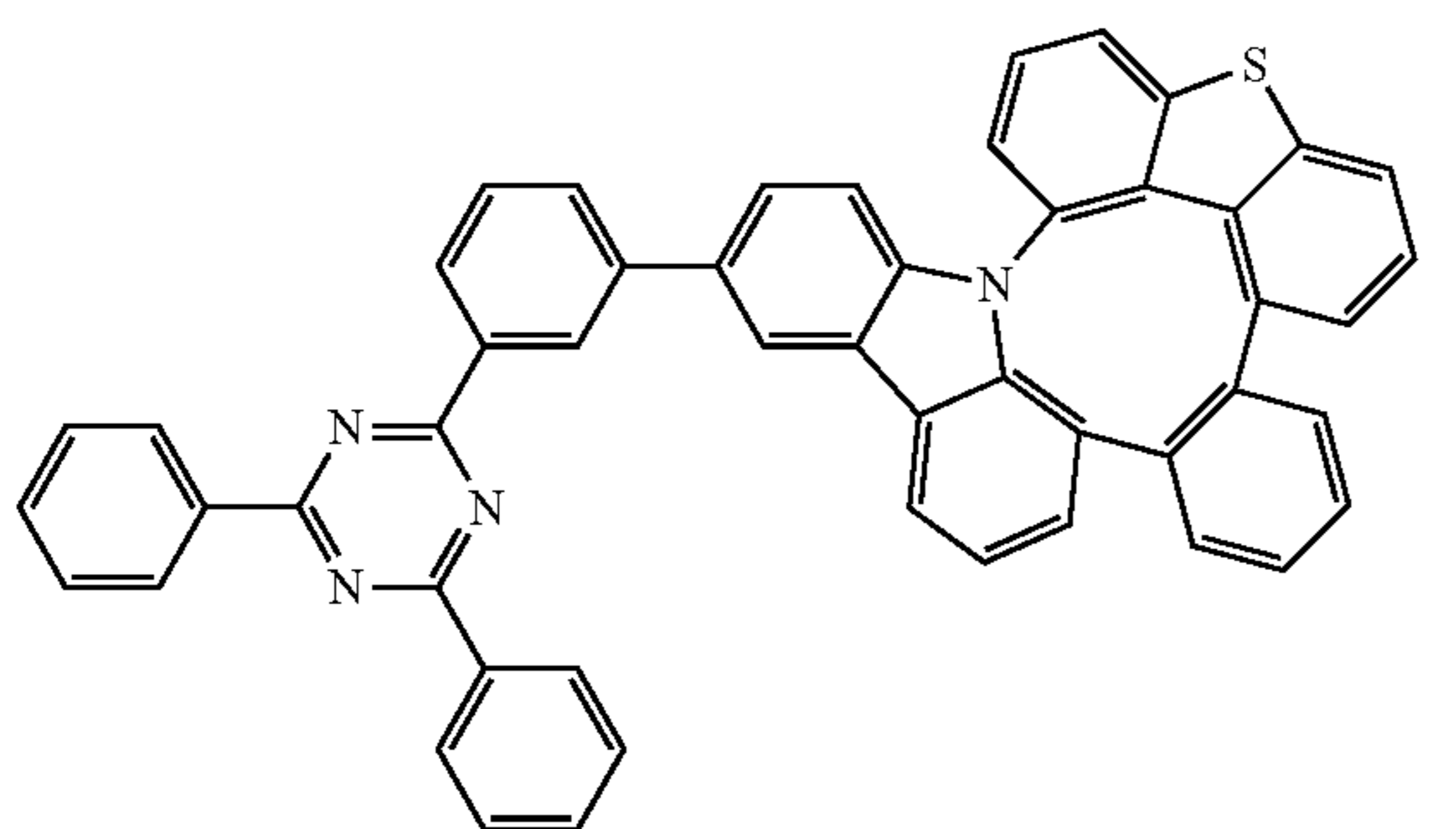
Compound 115
