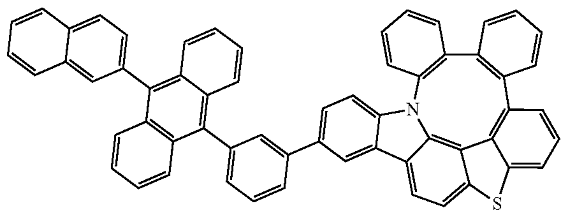
Compound 295
