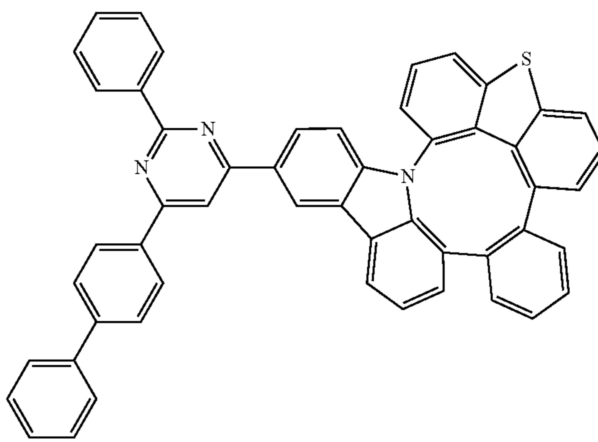
Compound 113
