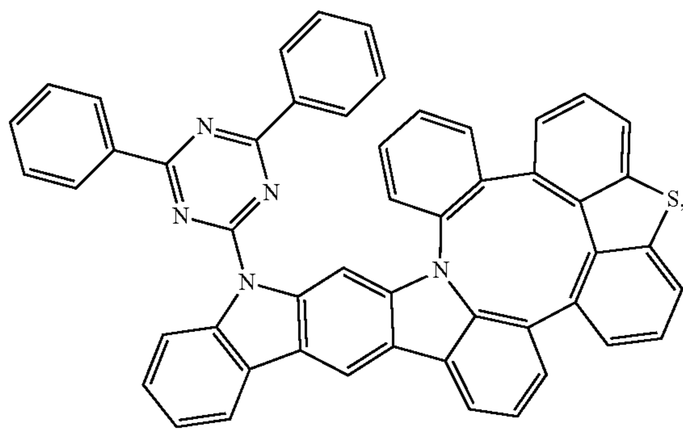
Compound 246
