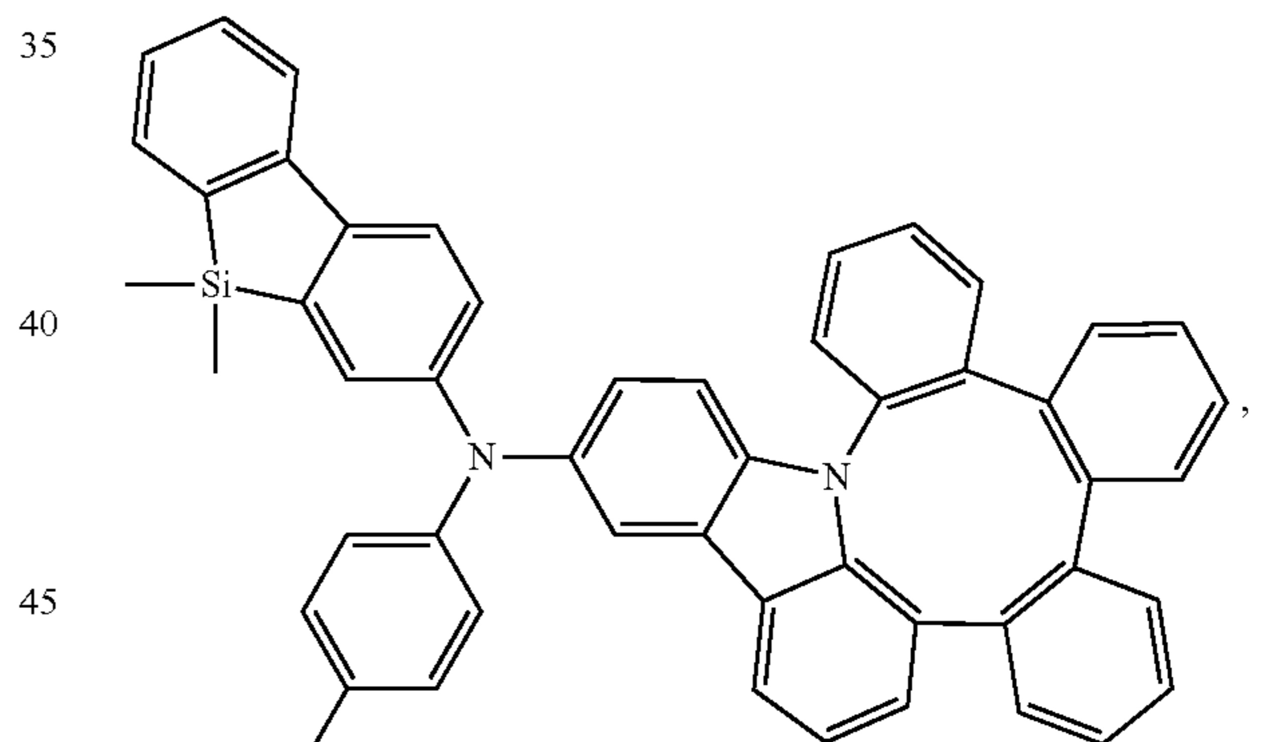
Compound 344
