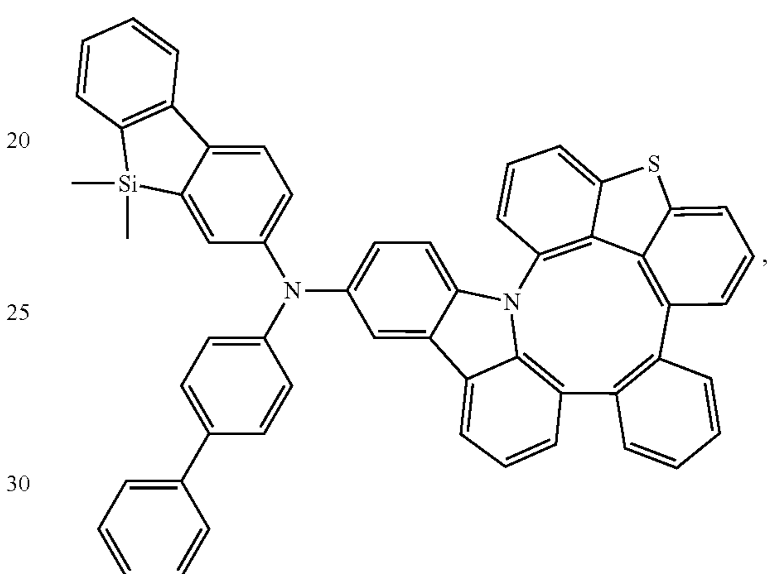
Compound 352
