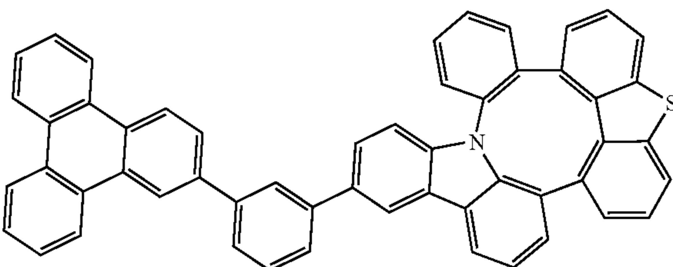
Compound 205
