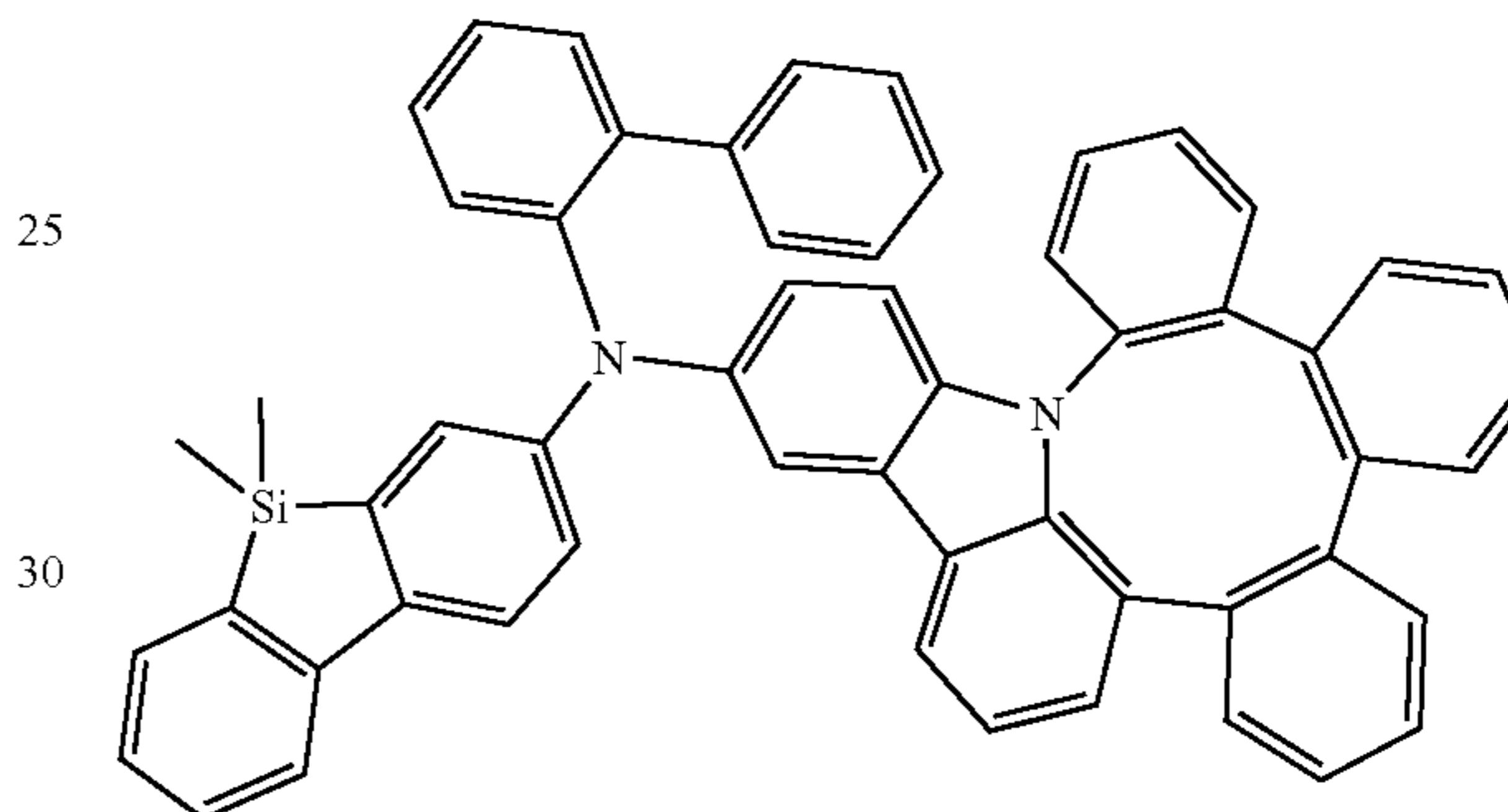
Compound 346
