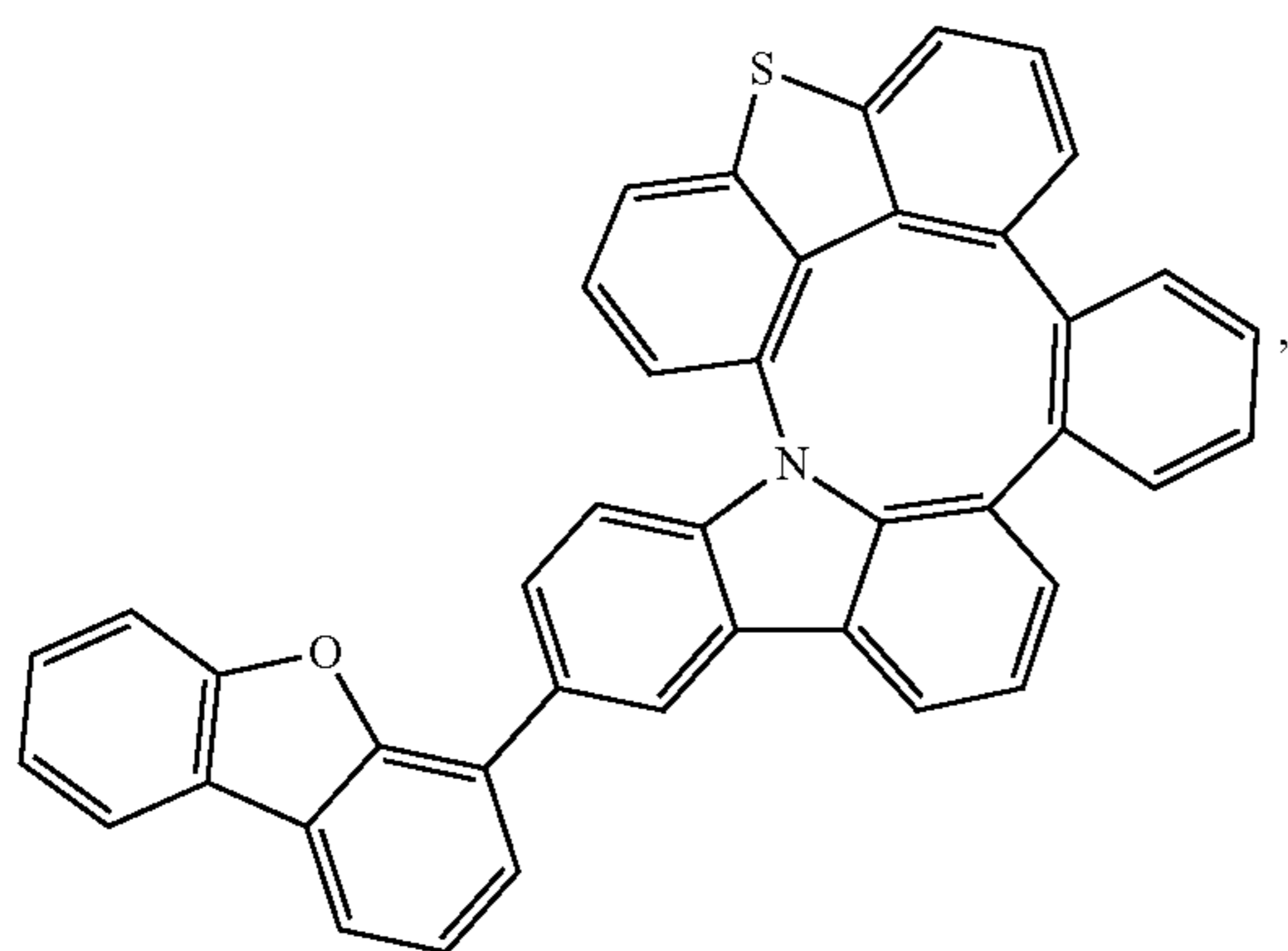
Compound 89
