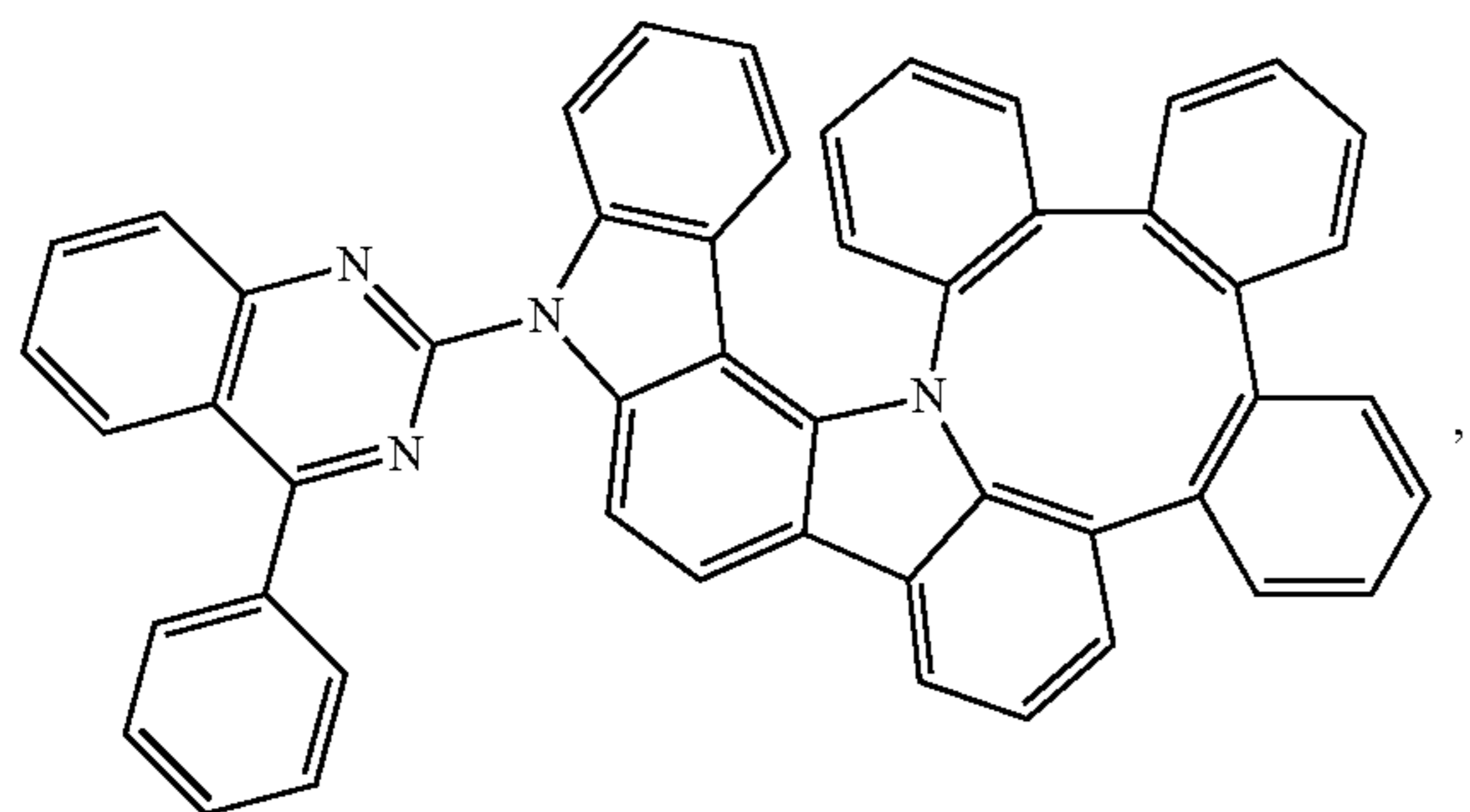
Compound 84
