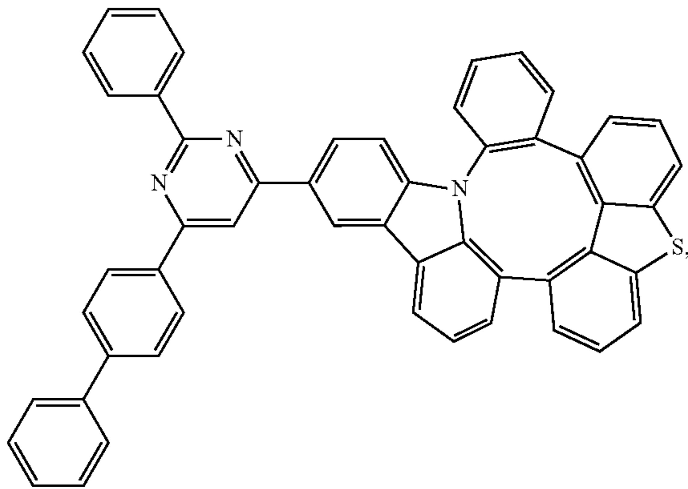
Compound 198
