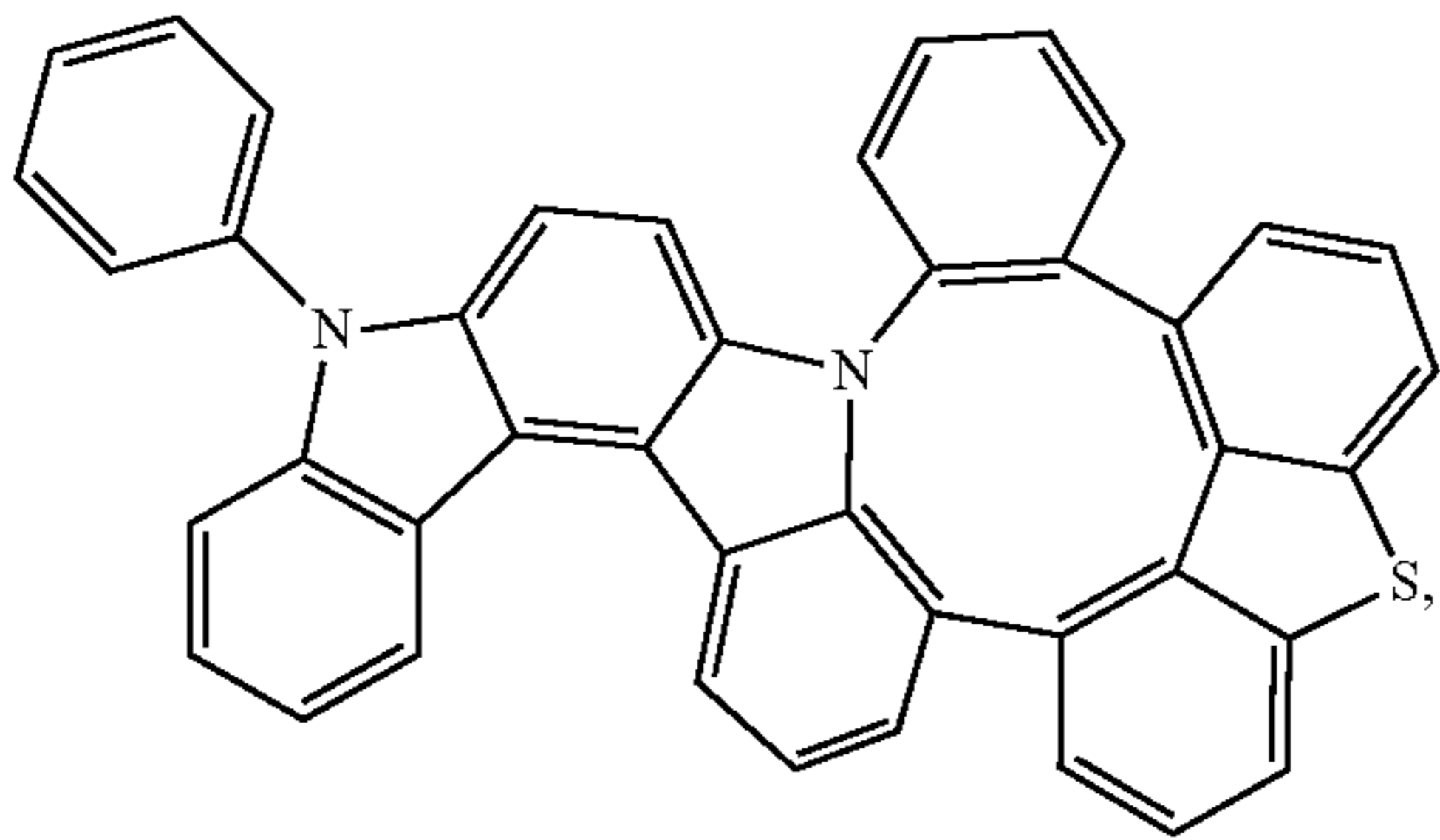
Compound 221
