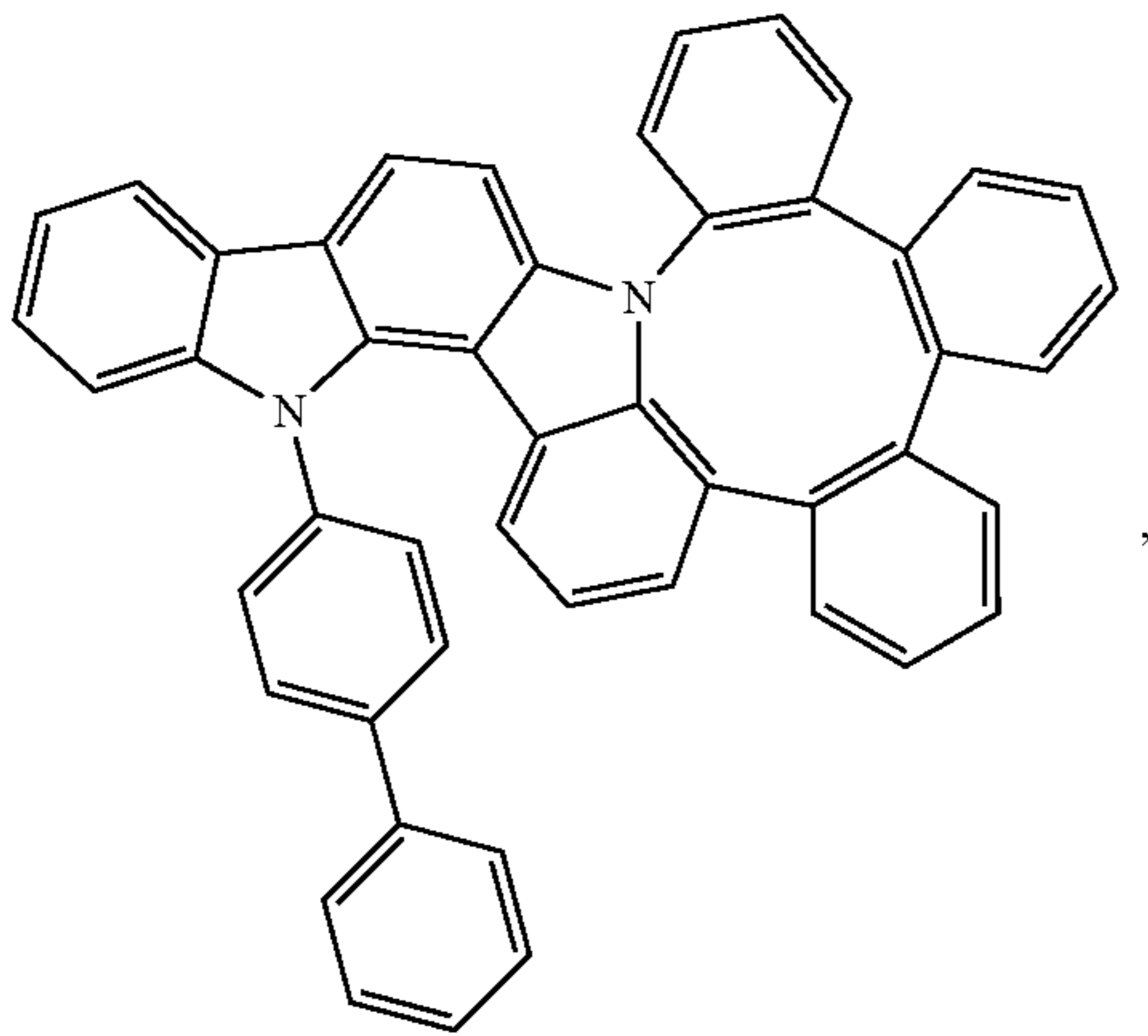
Compound 57
