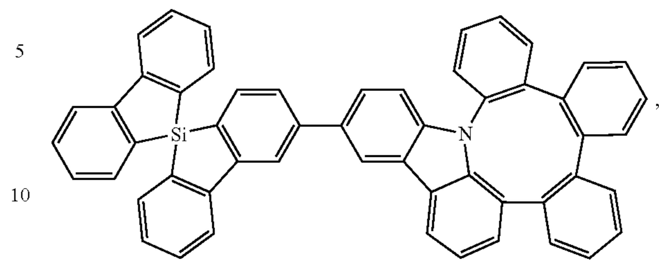
Compound 342
