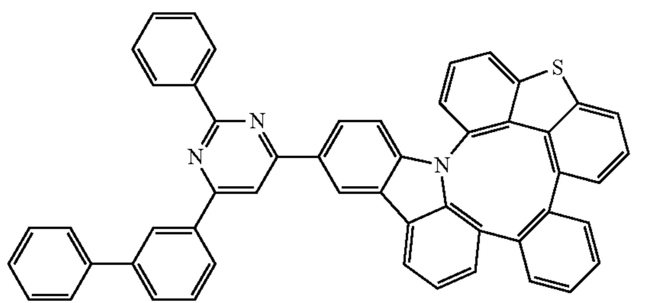
Compound 114
