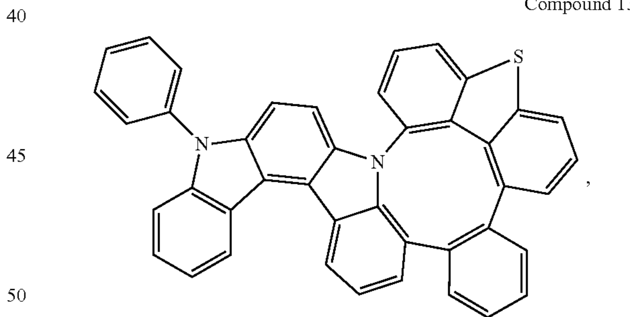
Compound 136
