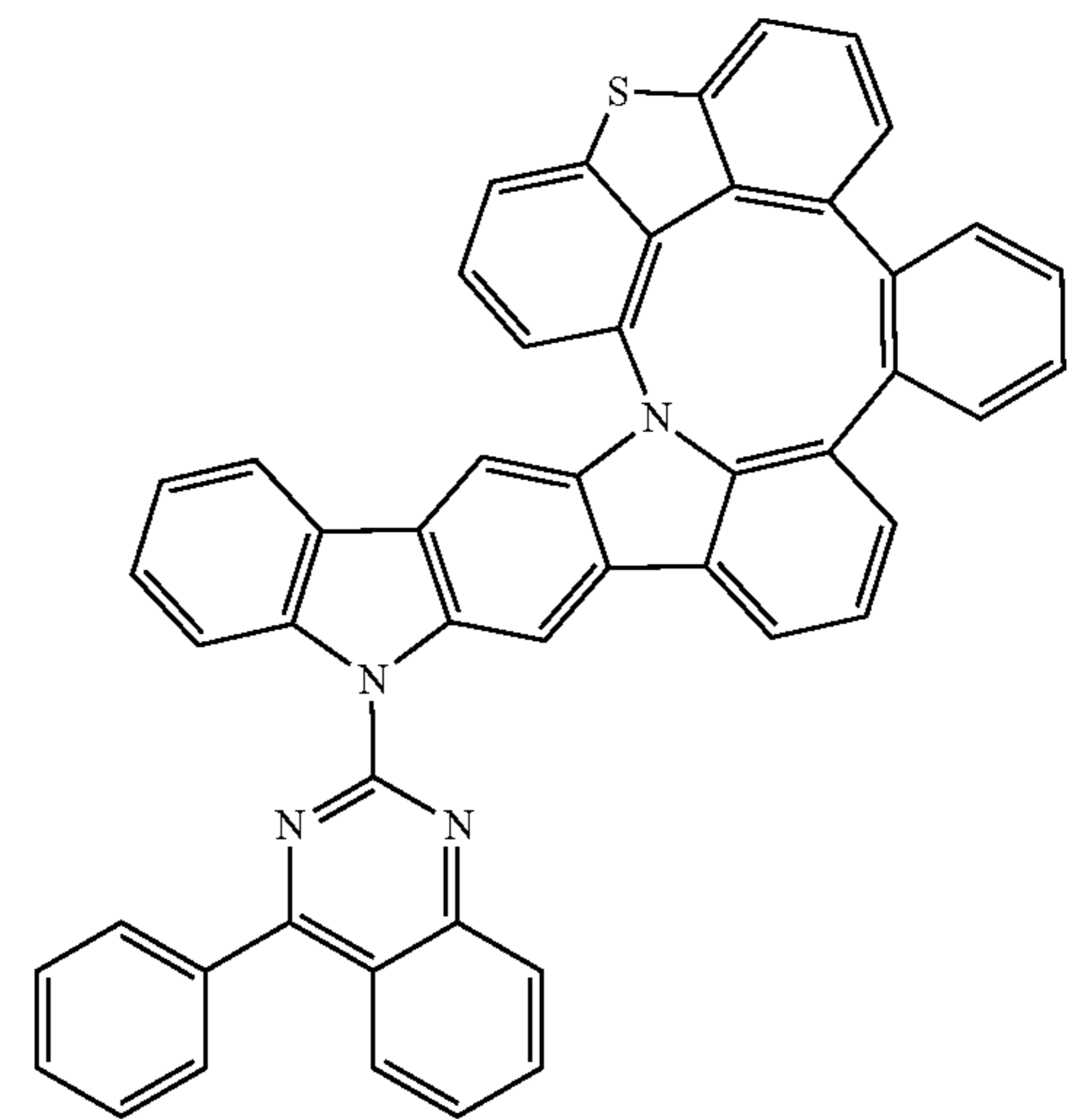
Compound 169
