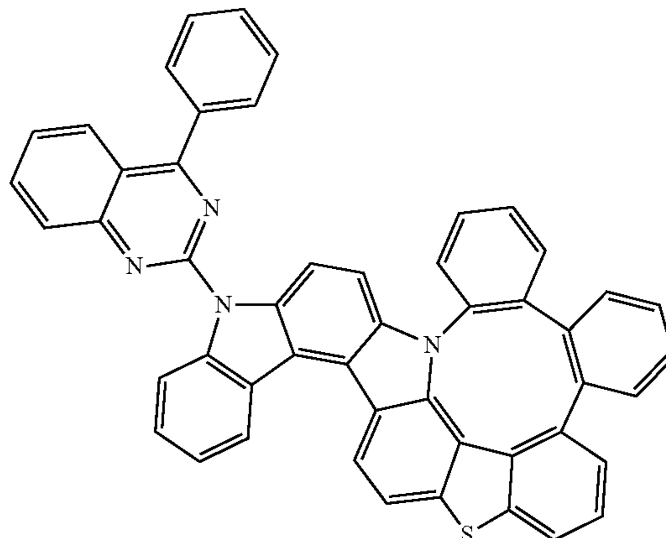
Compound 336
