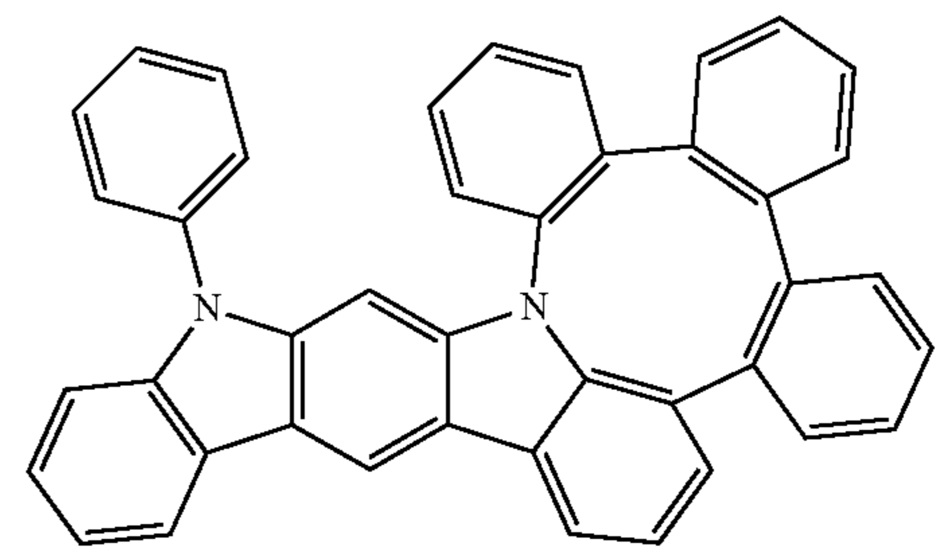
Compound 52
