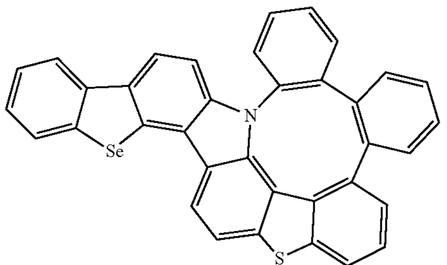
Compound 325
