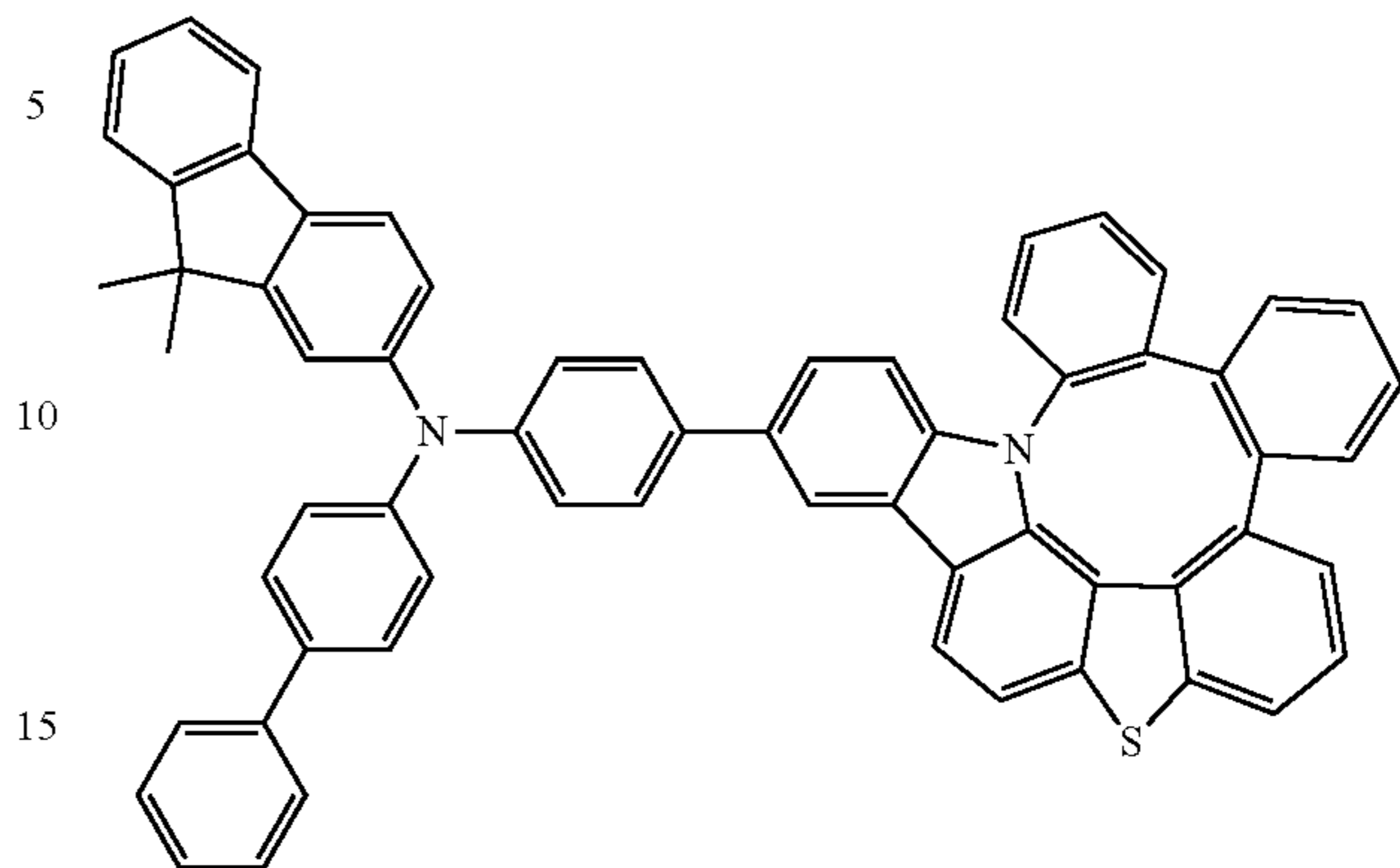
Compound 303
