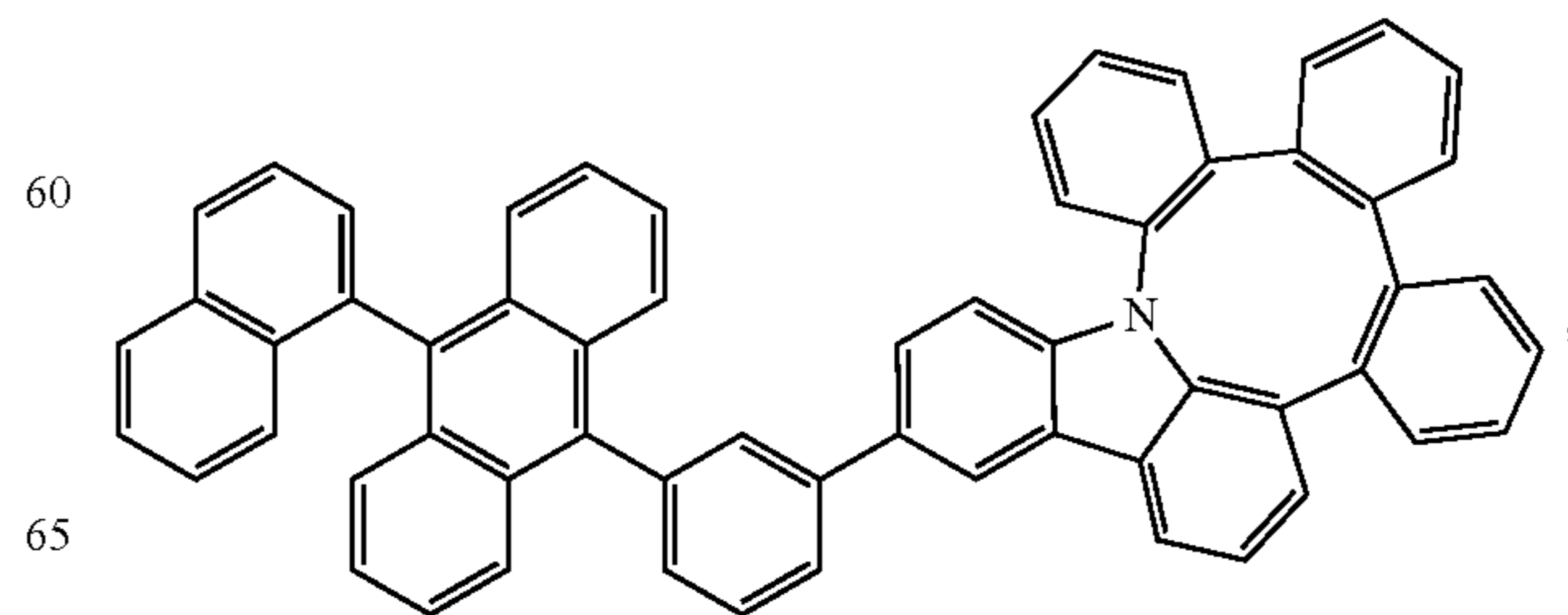
Compound 39
