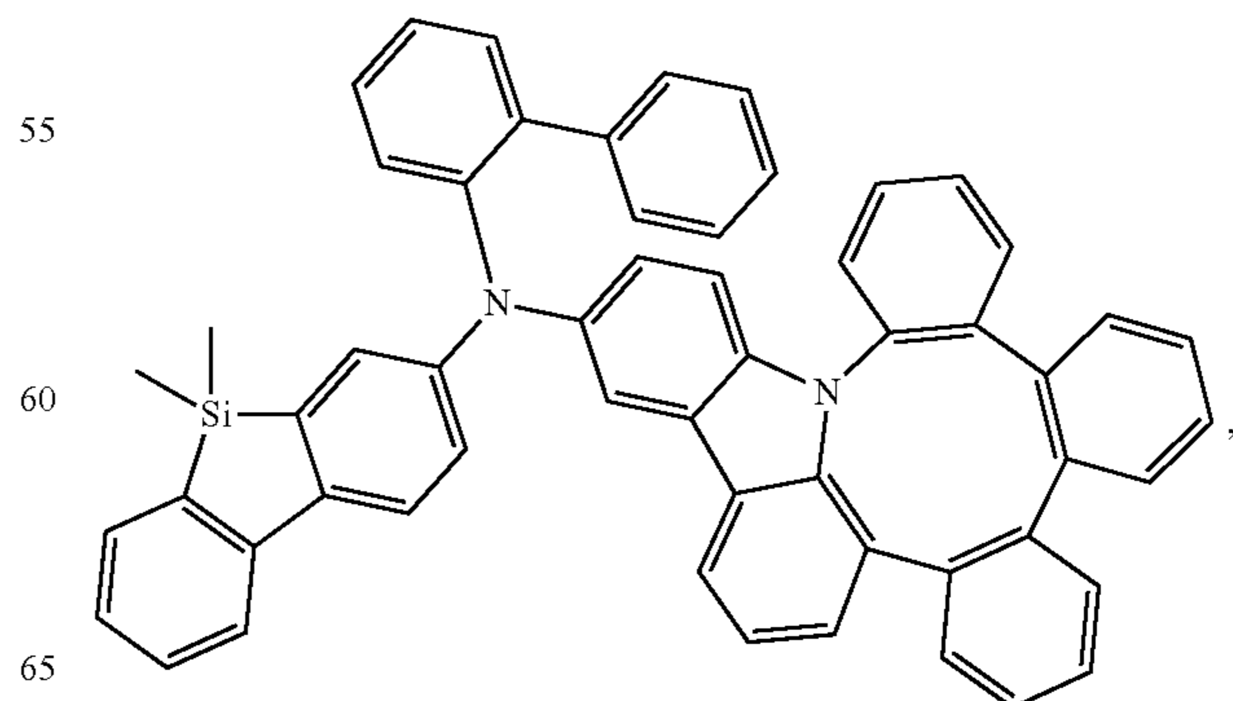
Compound 345
