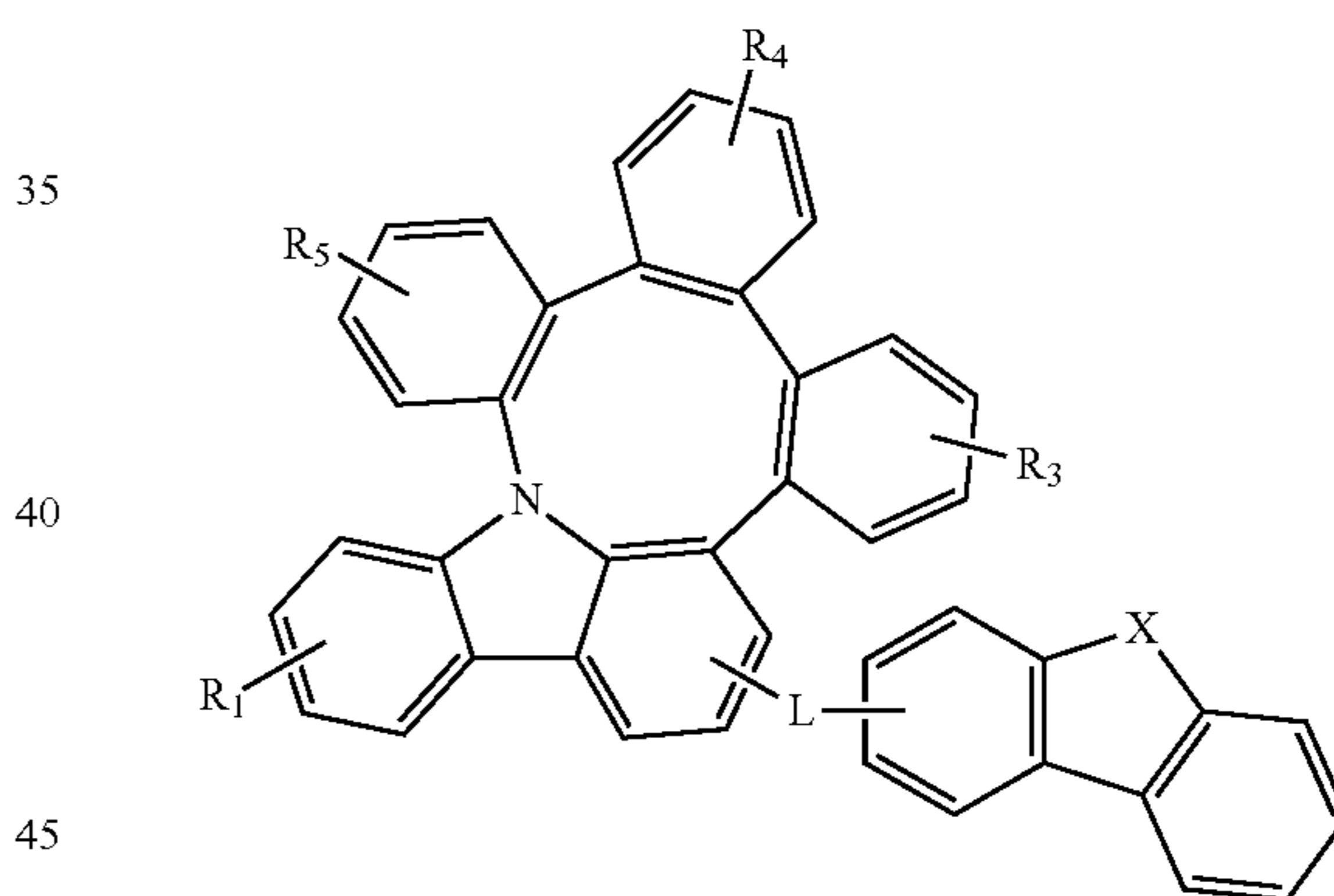
Formula 6
