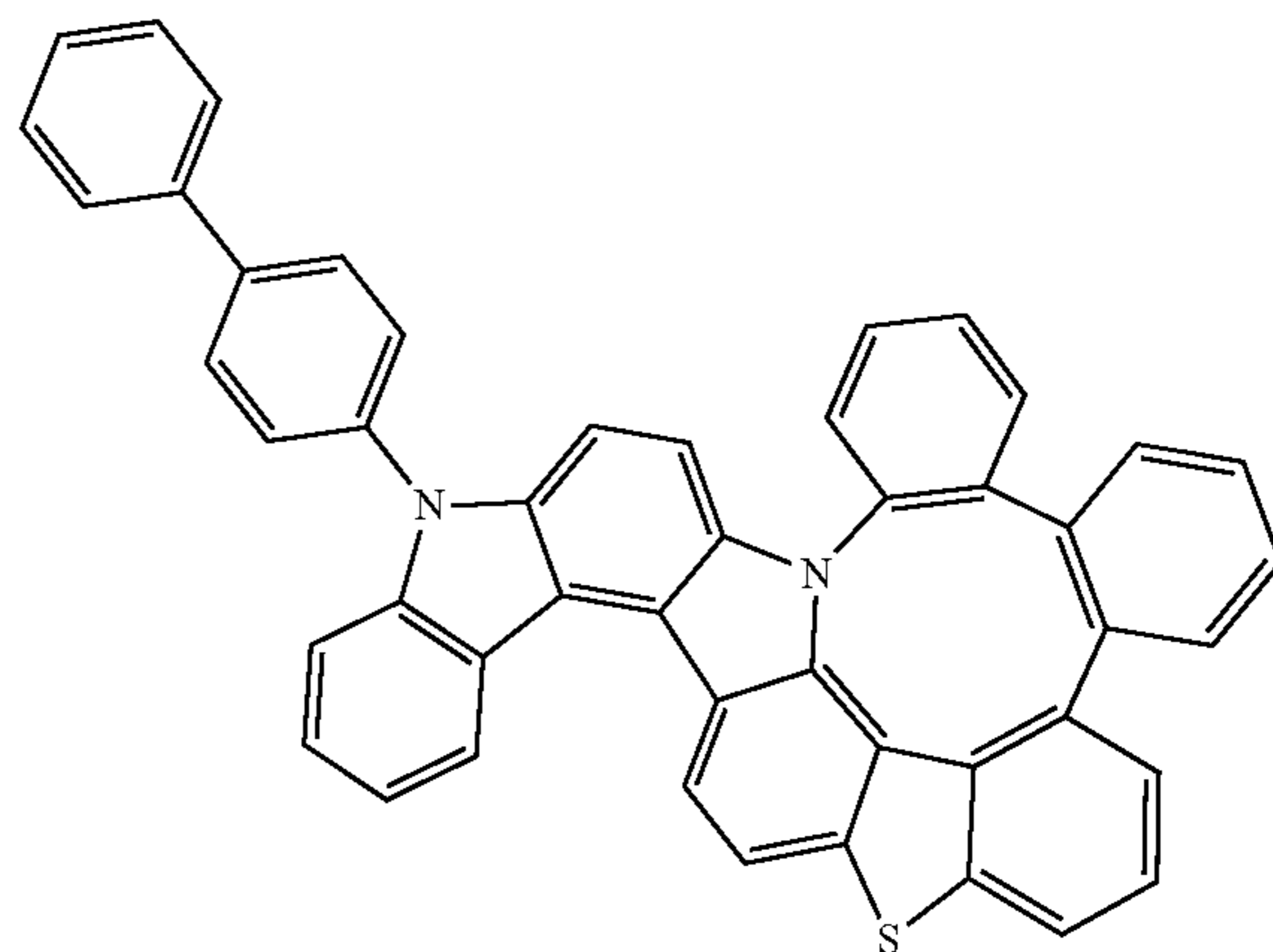
Compound 313
