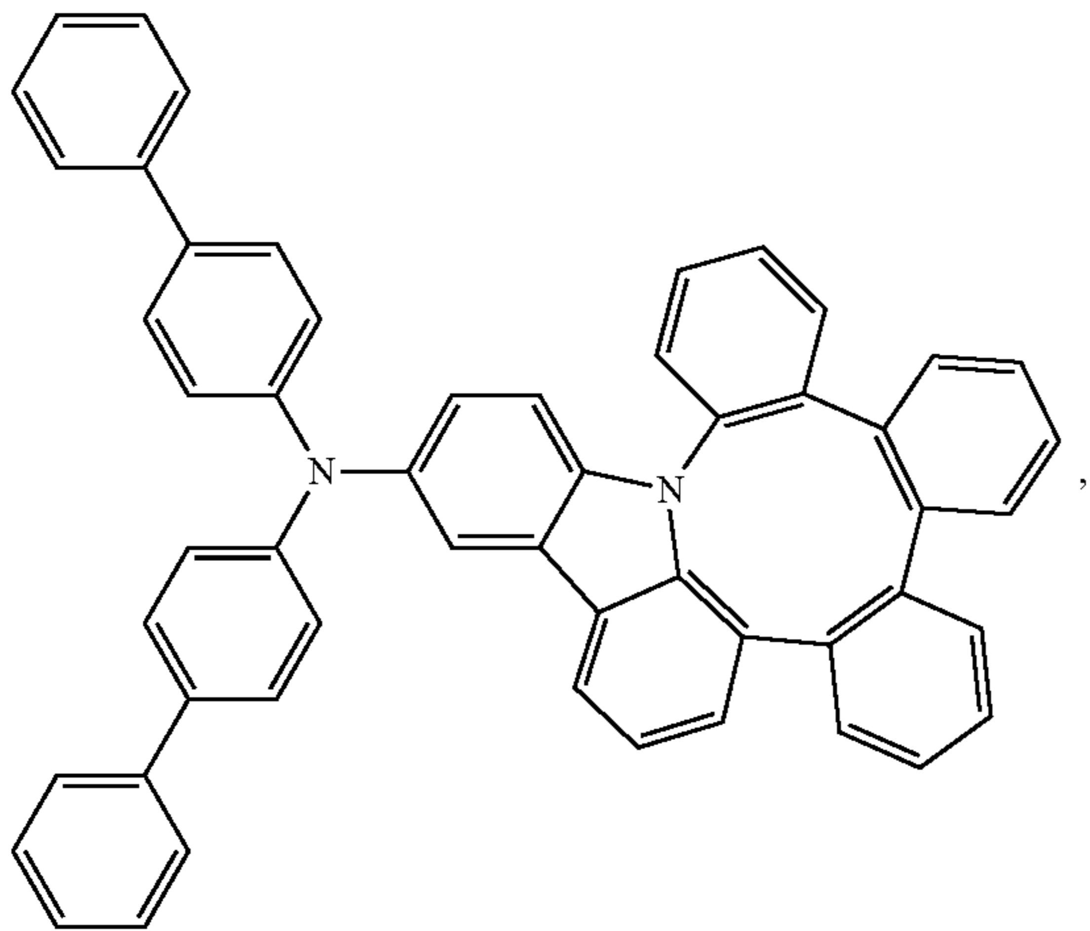
Compound 42
