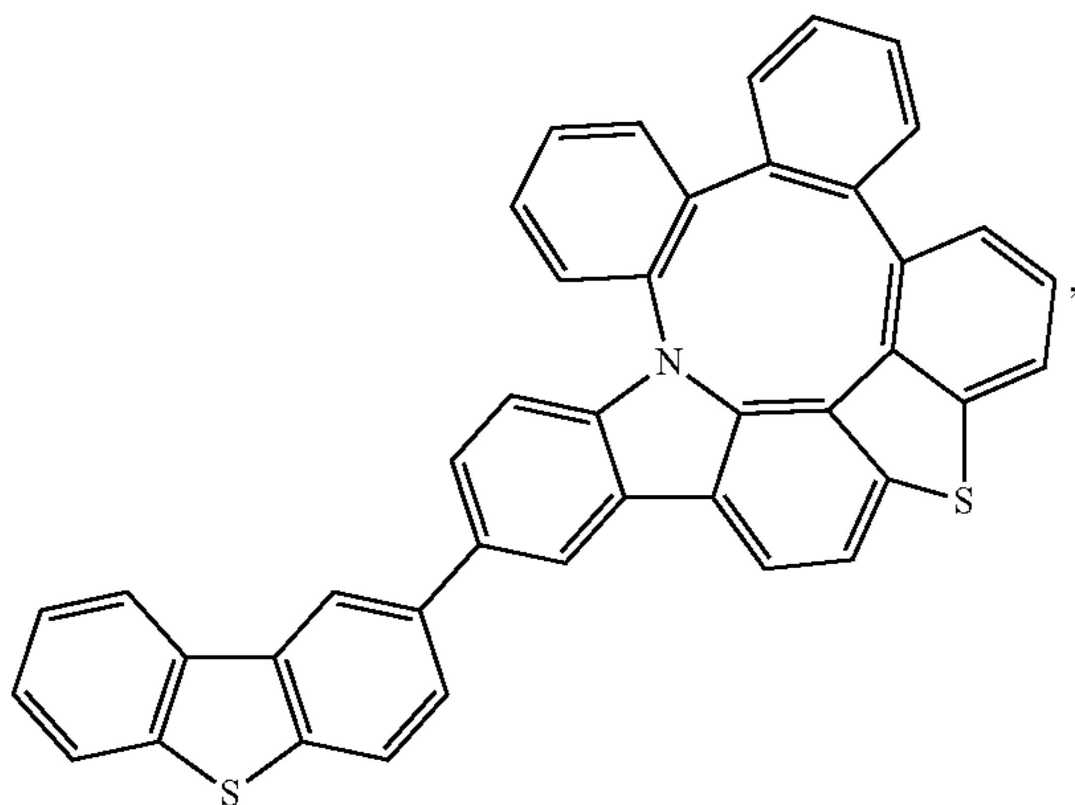
Compound 263
