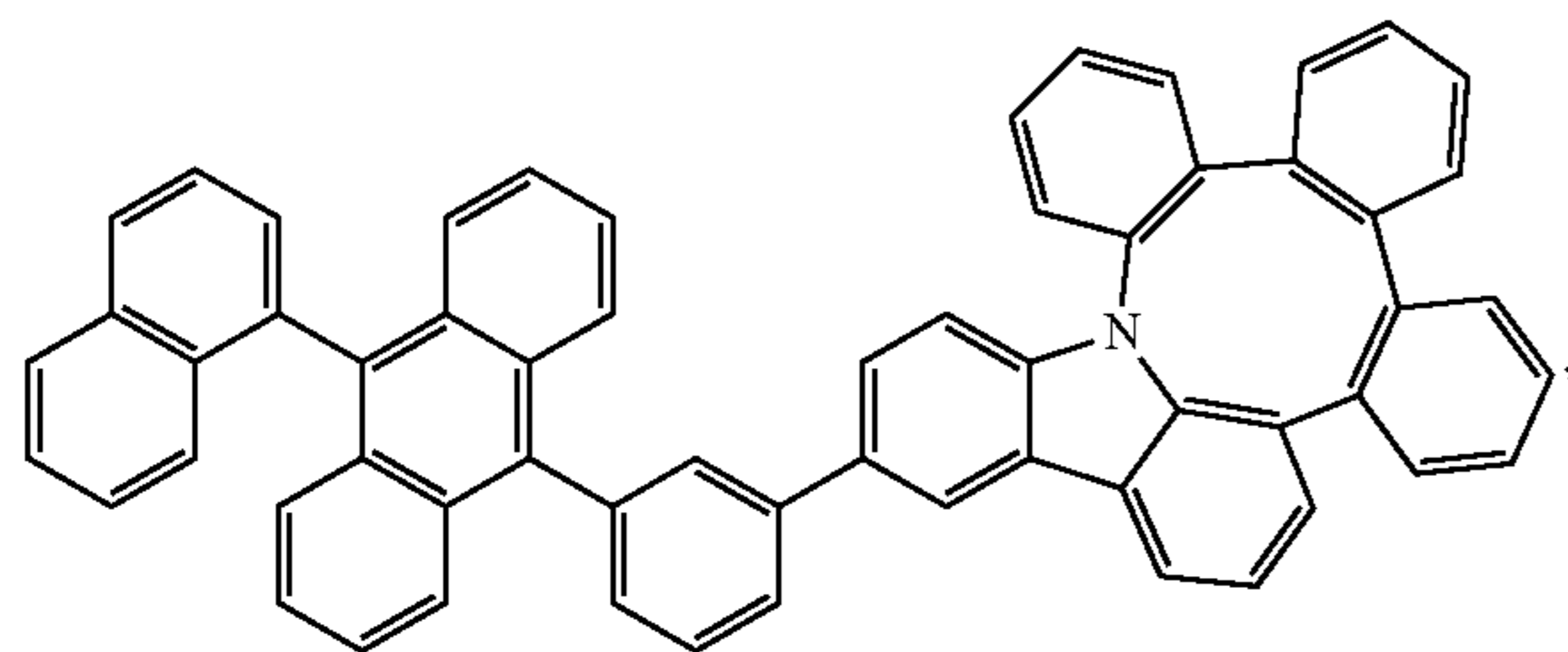
Compound 39
