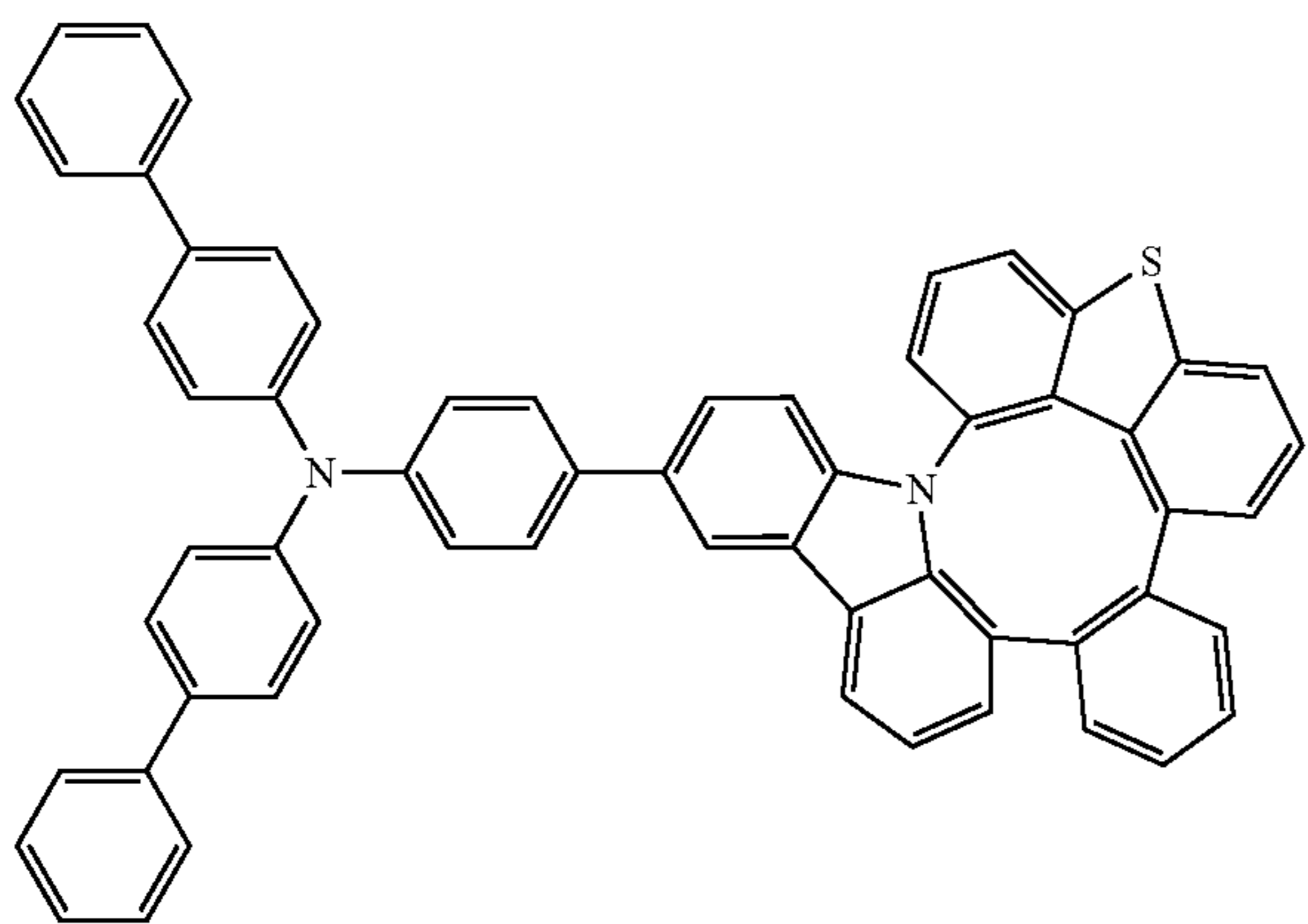
Compound 132
