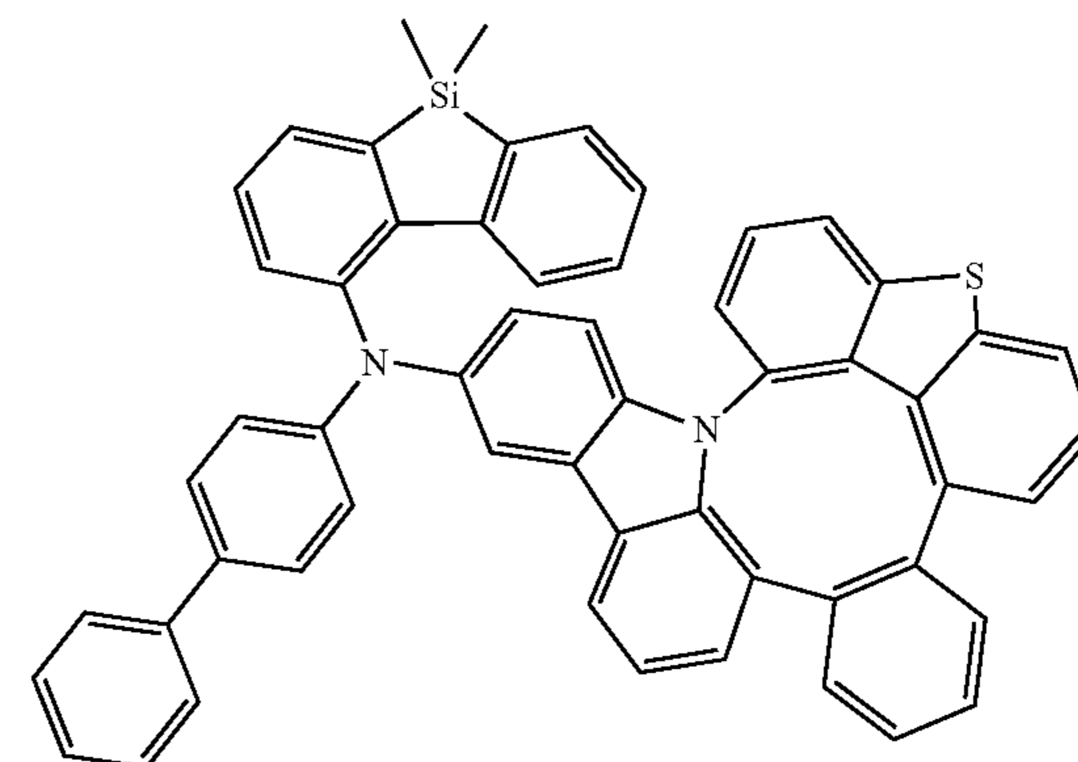
Compound 353
