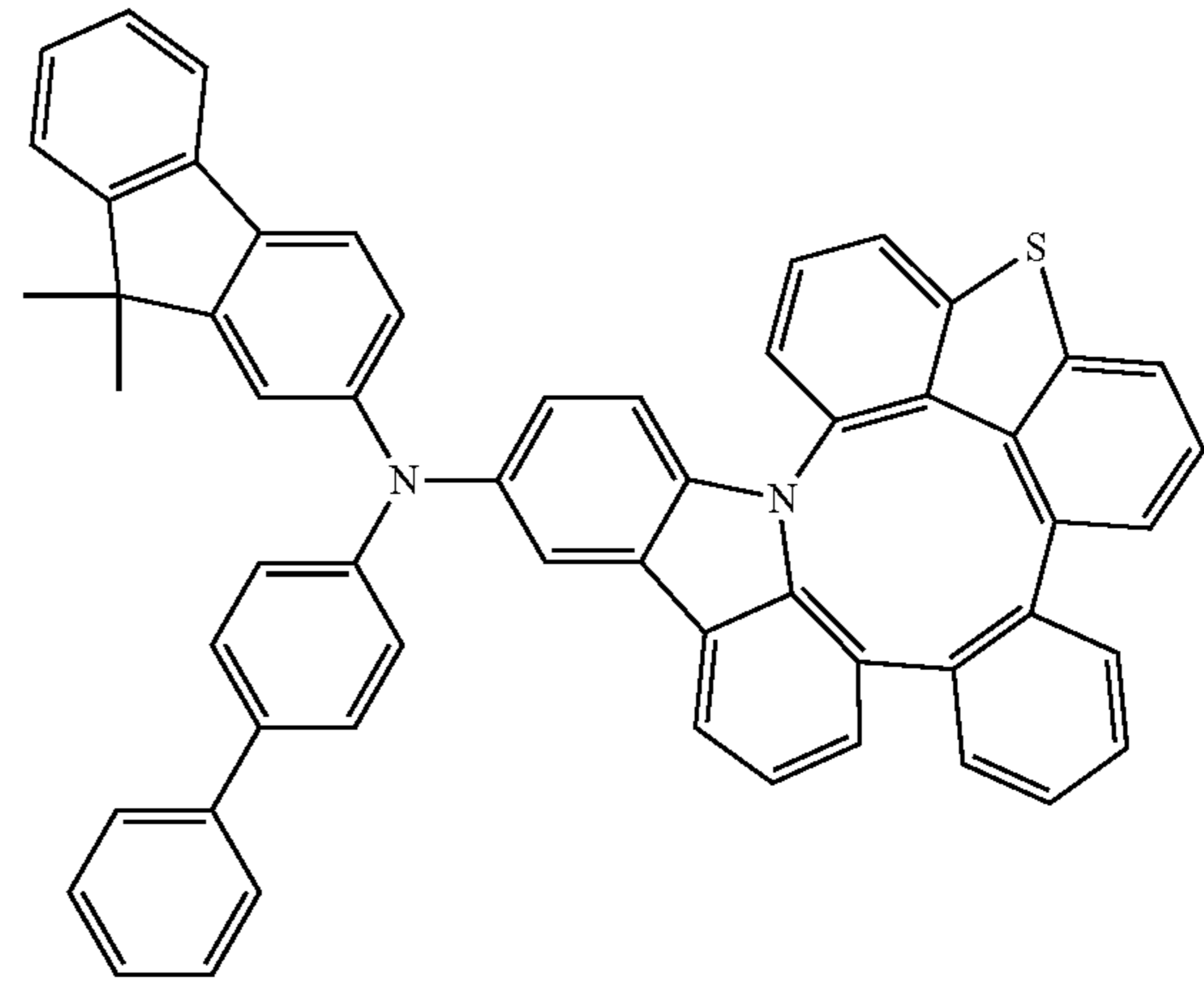
Compound 127
