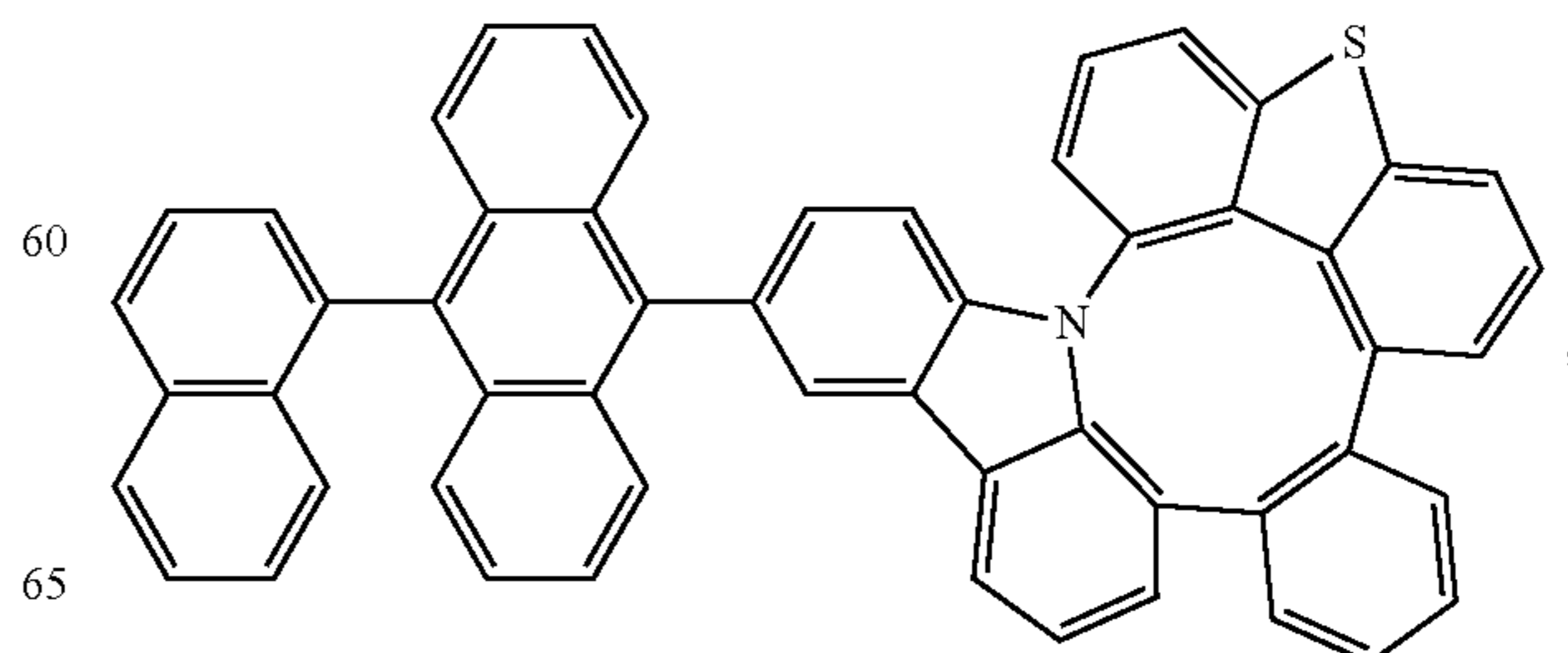
Compound 122
