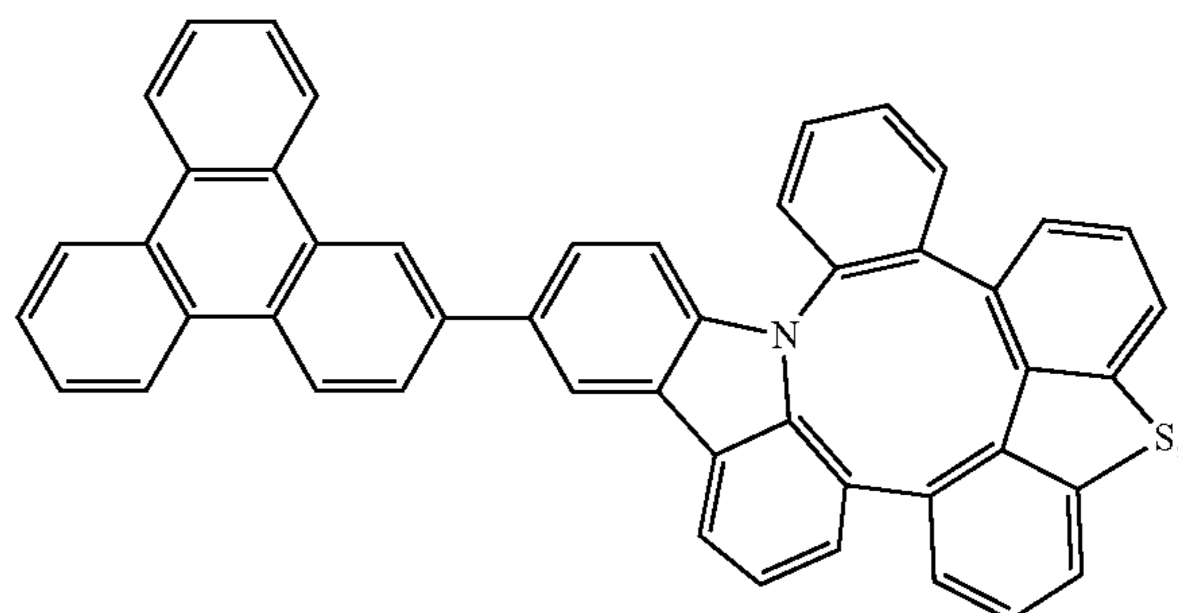
Compound 204
