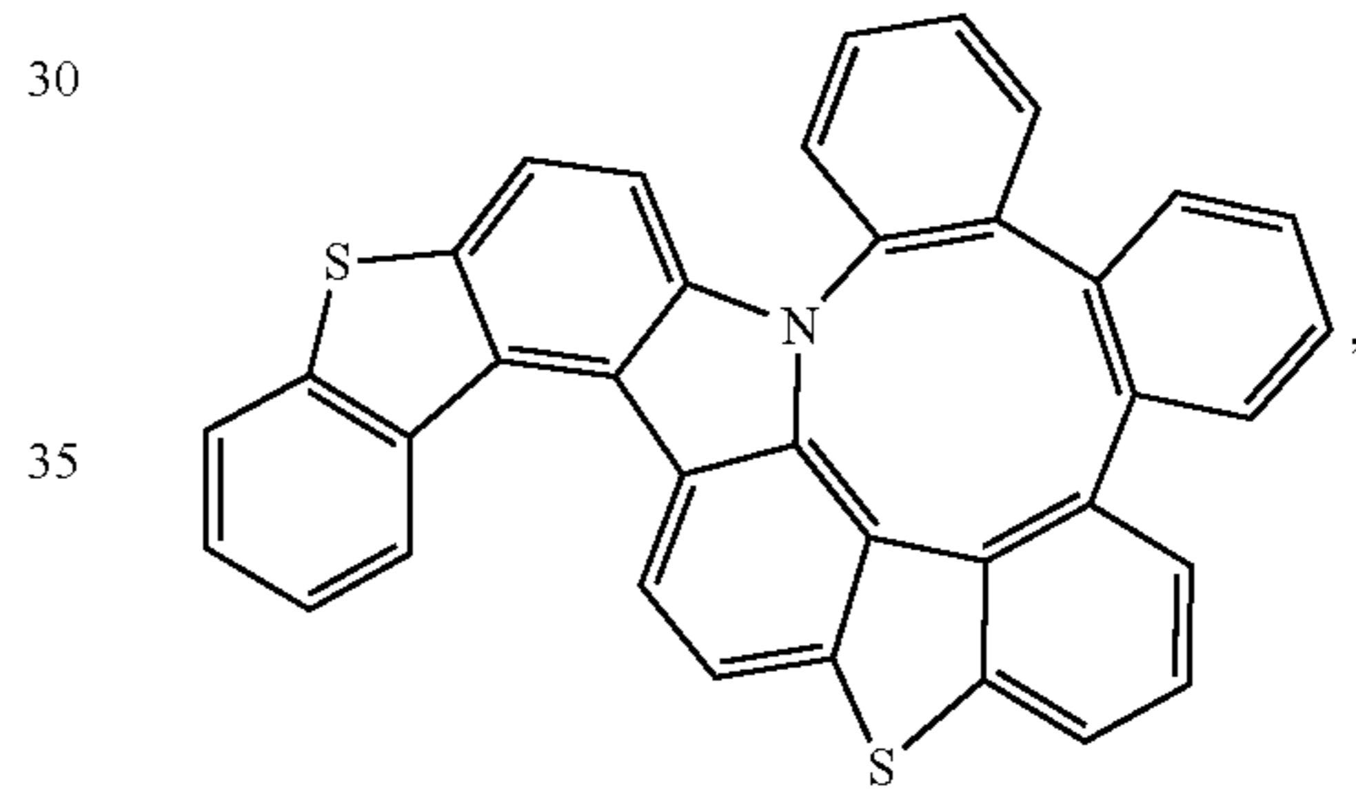
Compound 314
