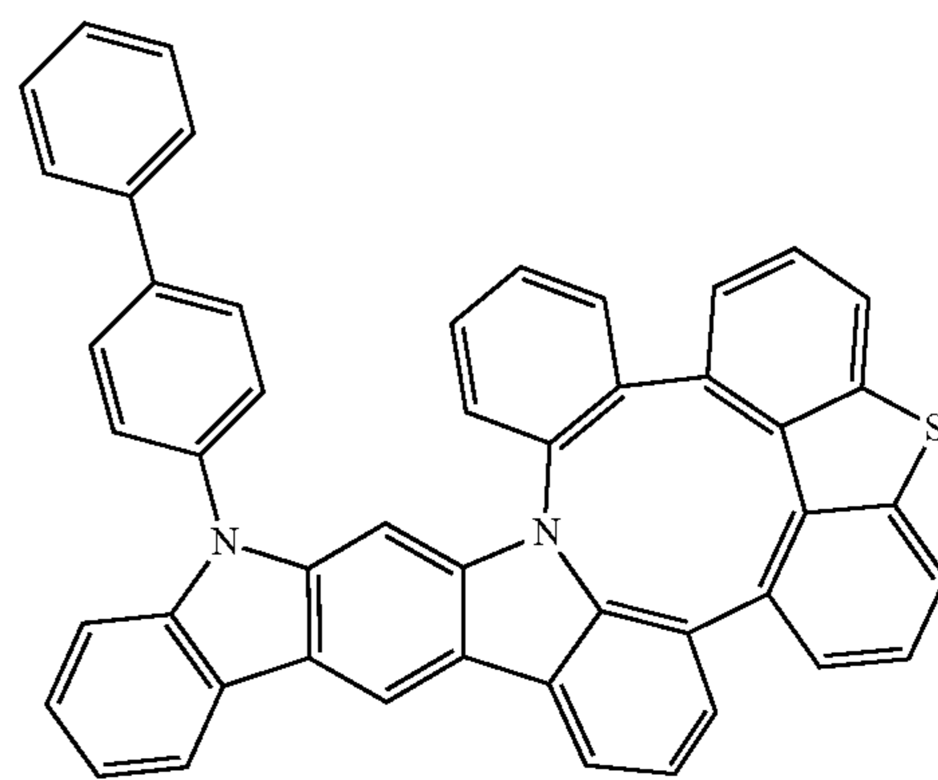
Compound 228
