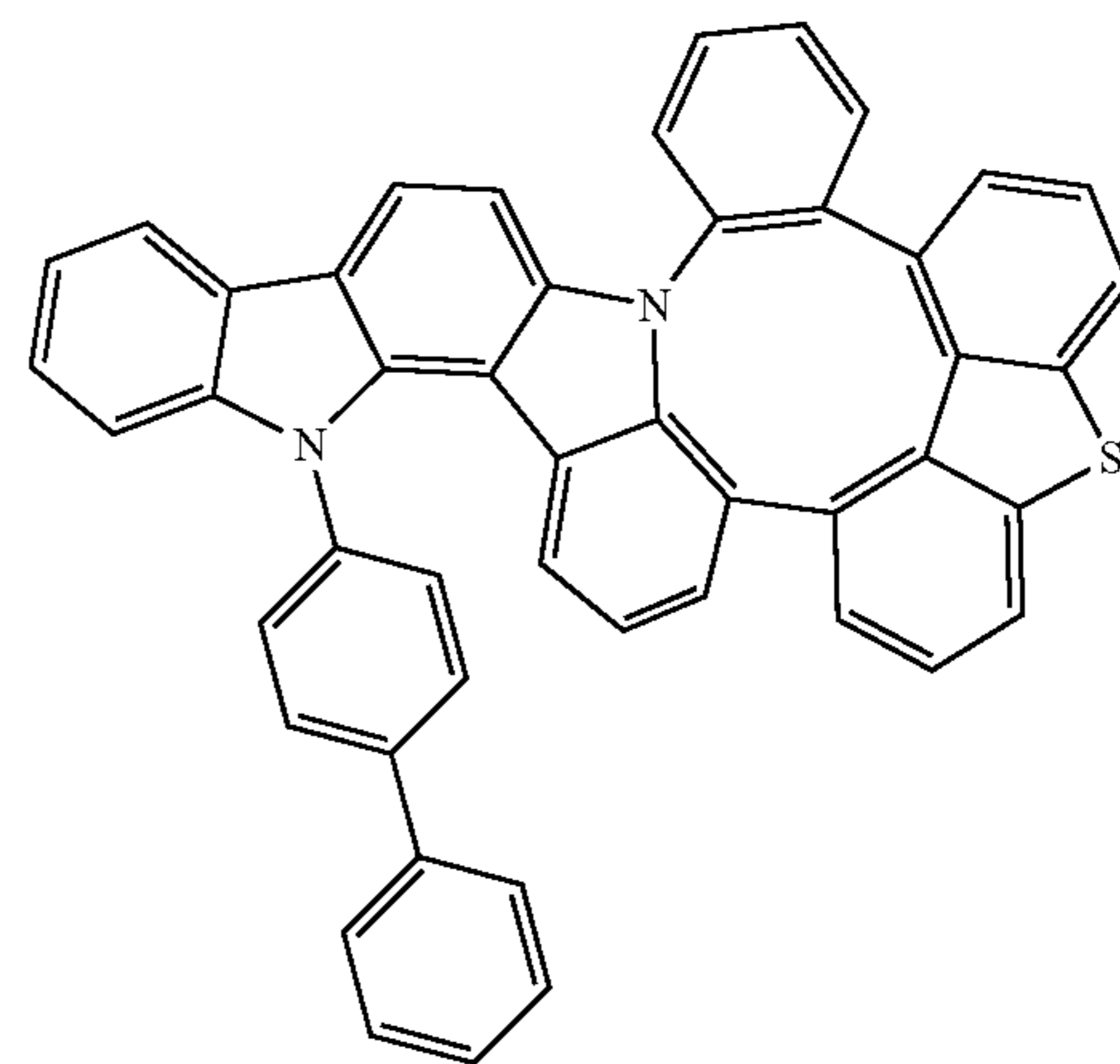
Compound 227
