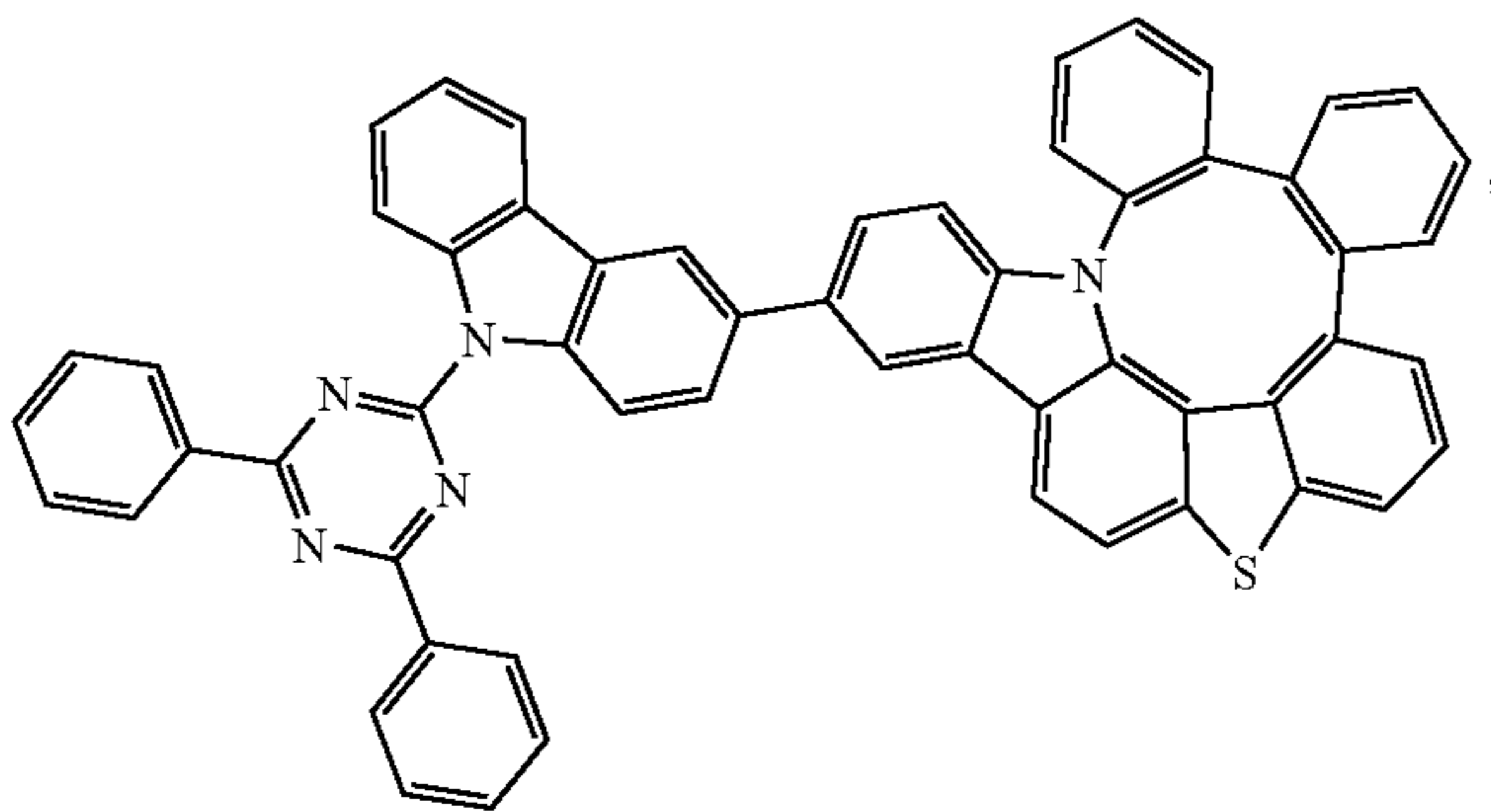
Compound 274
