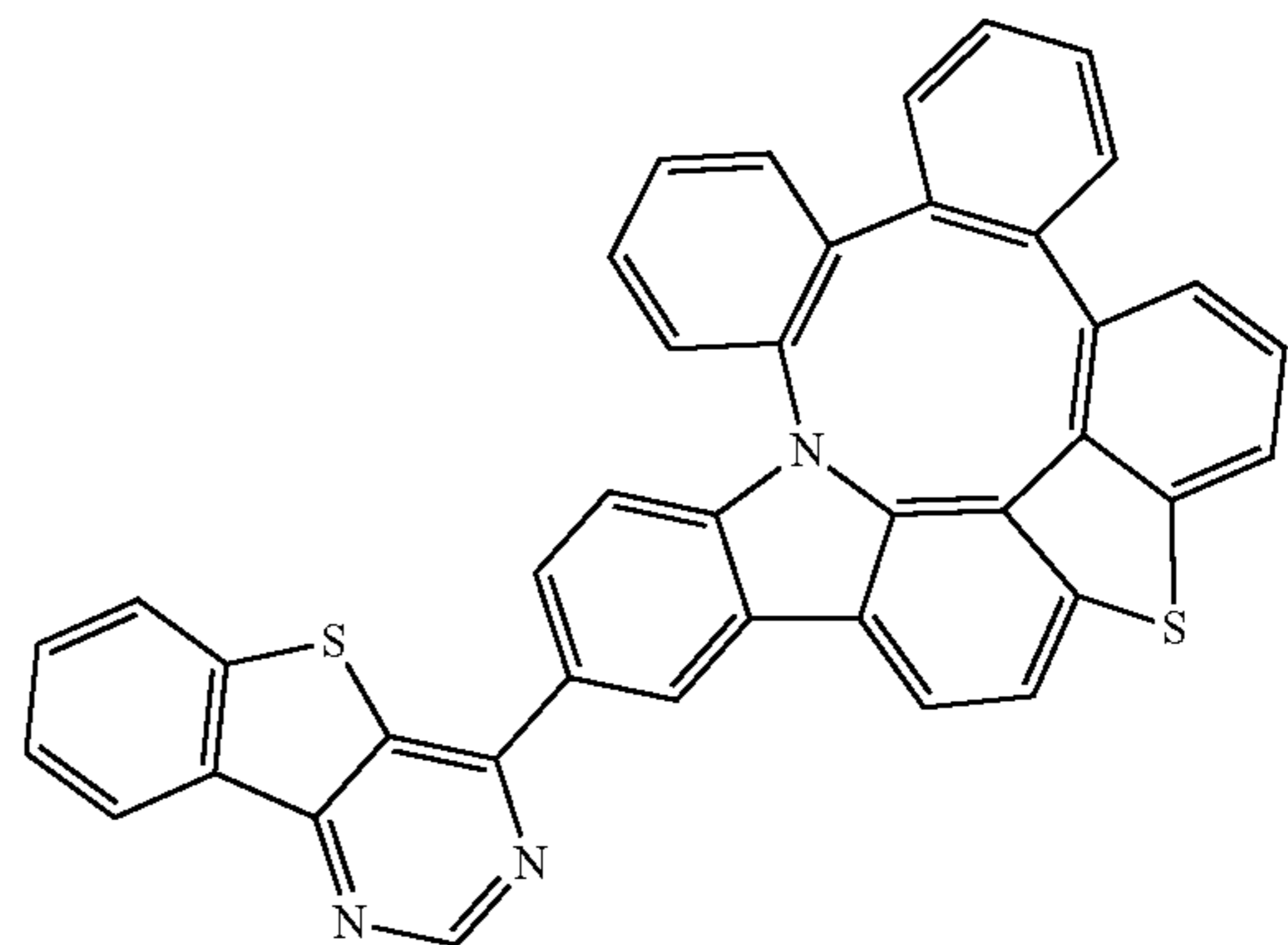
Compound 287
