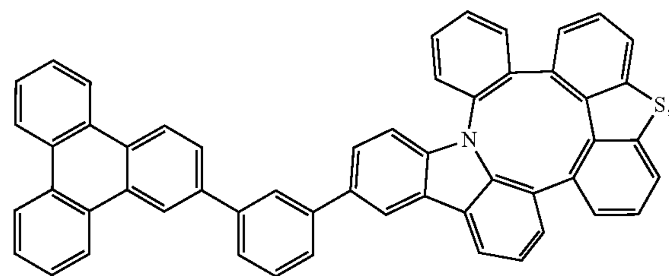
Compound 205
