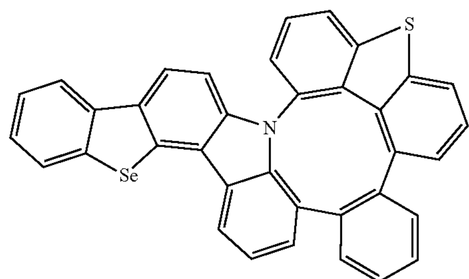
Compound 154
