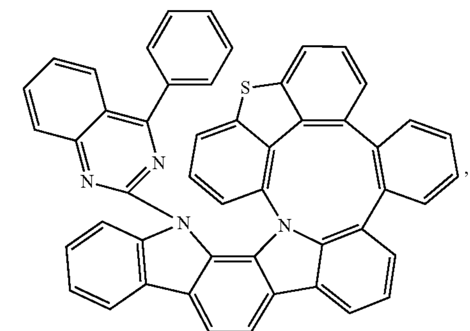
Compound 170
