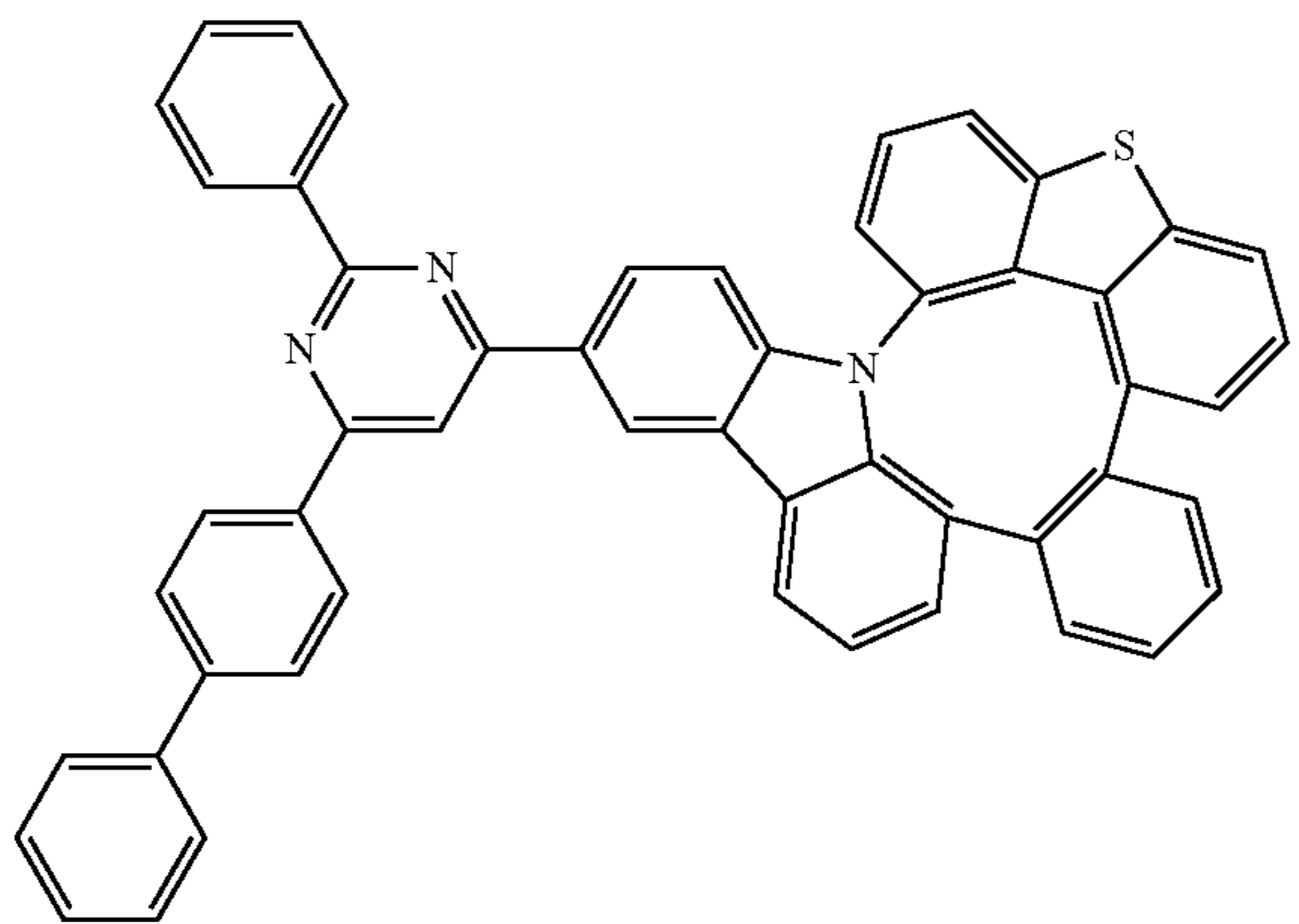
Compound 113
