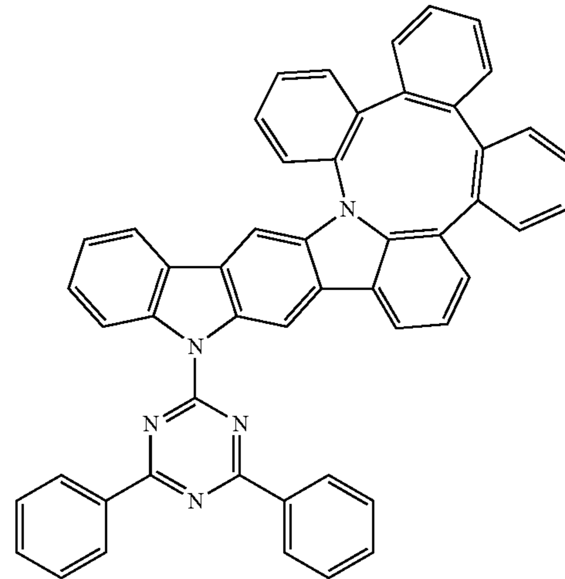
Compound 78
