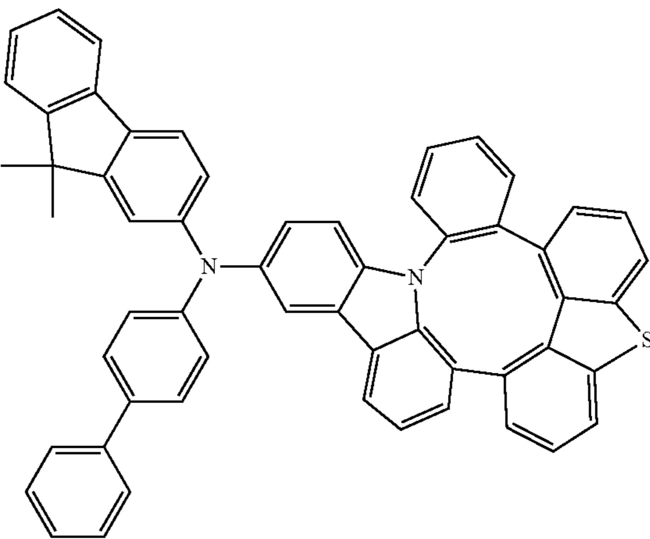
Compound 212
