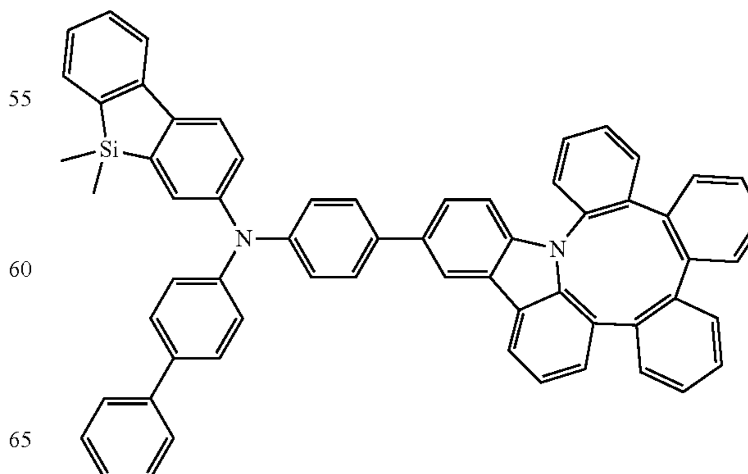
Compound 347
