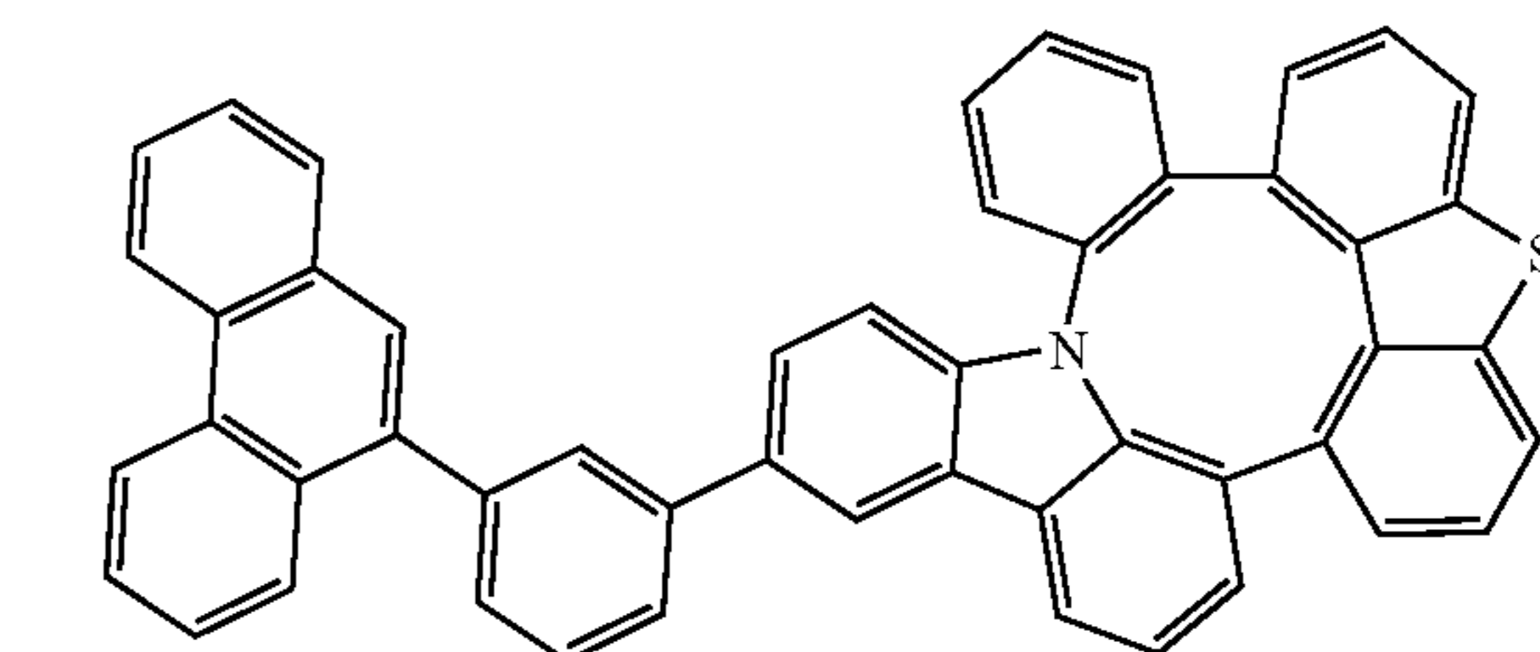
Compound 205
