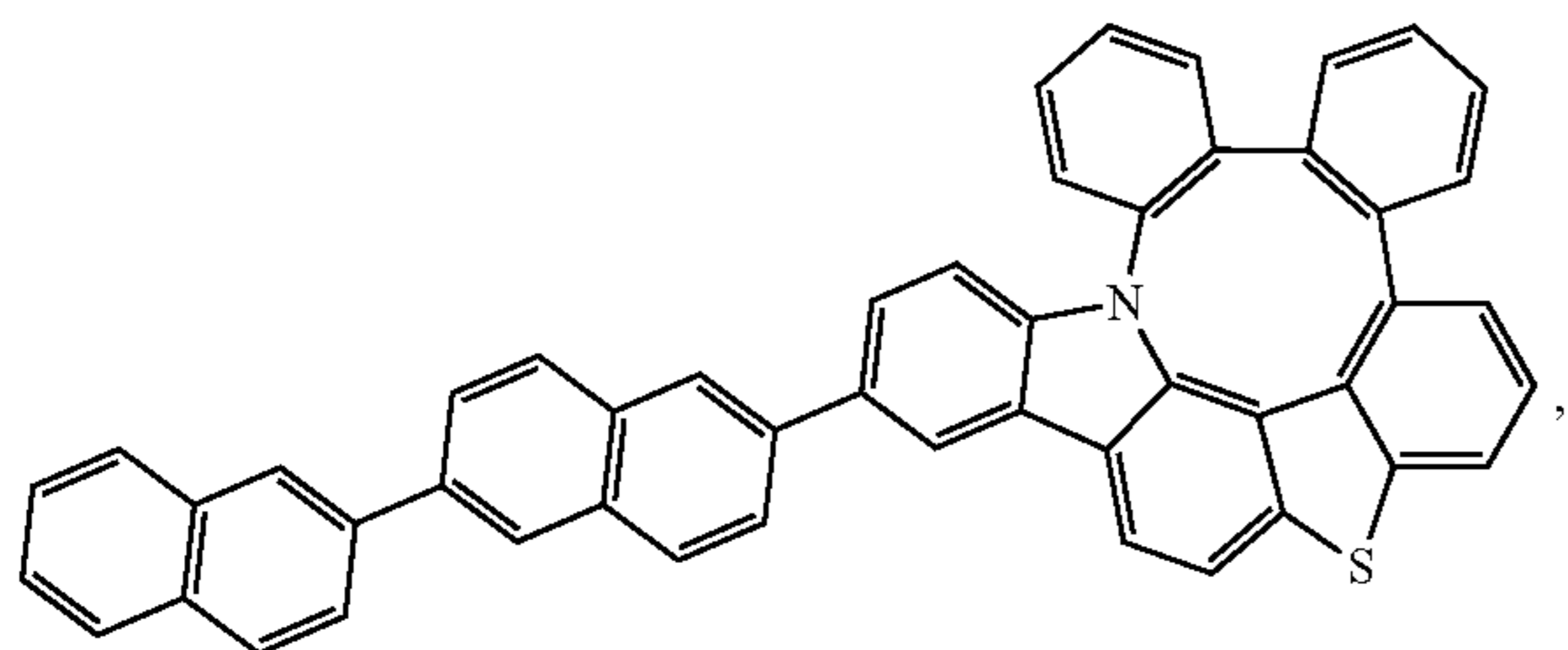
Compound 292
