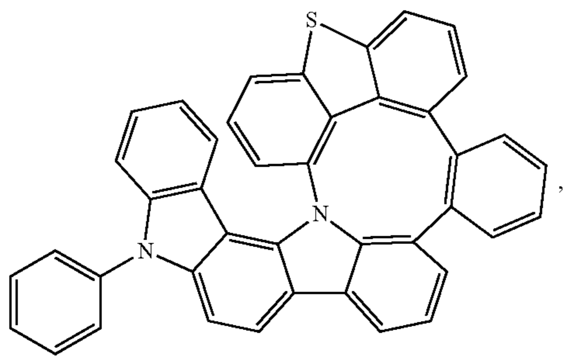
Compound 139
