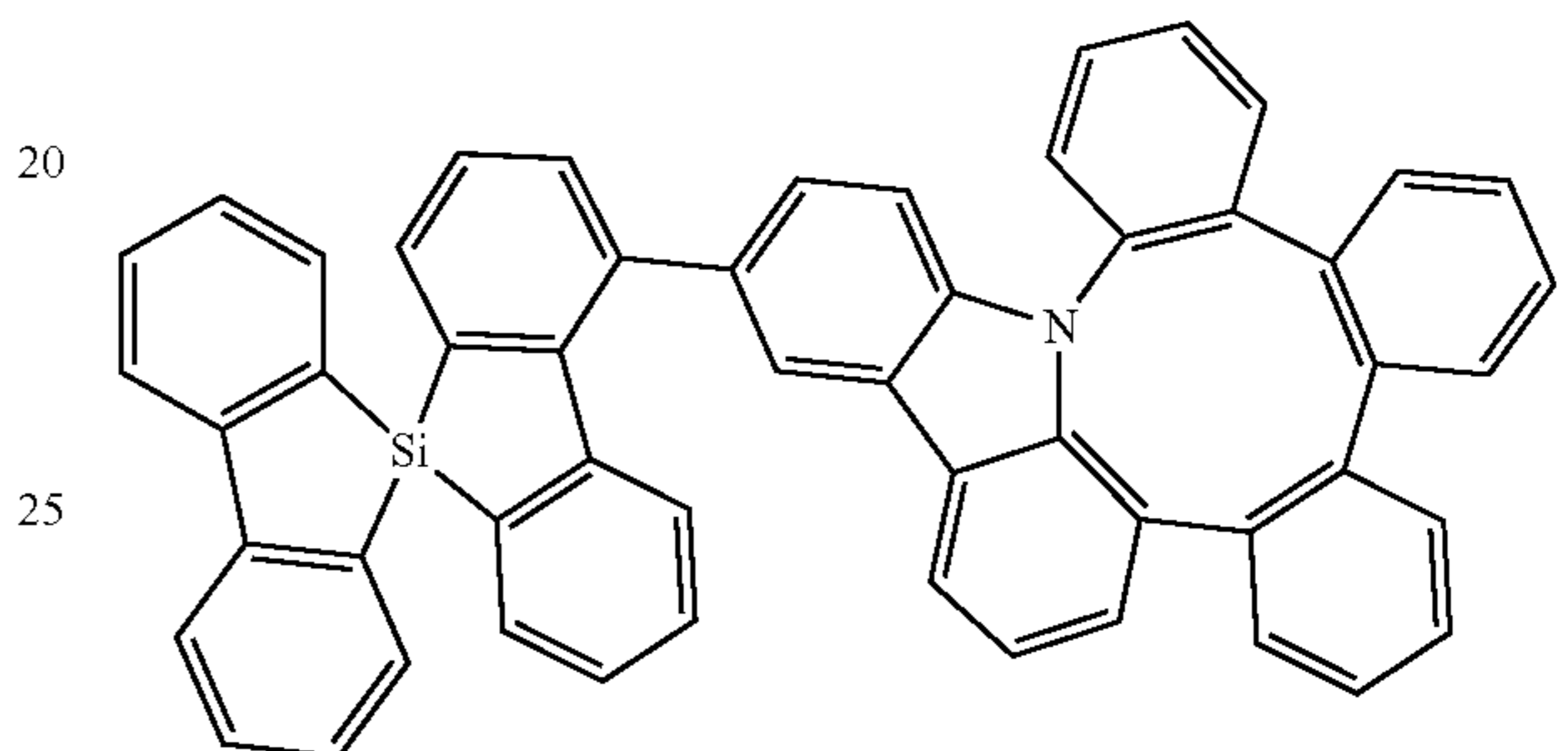
Compound 343
