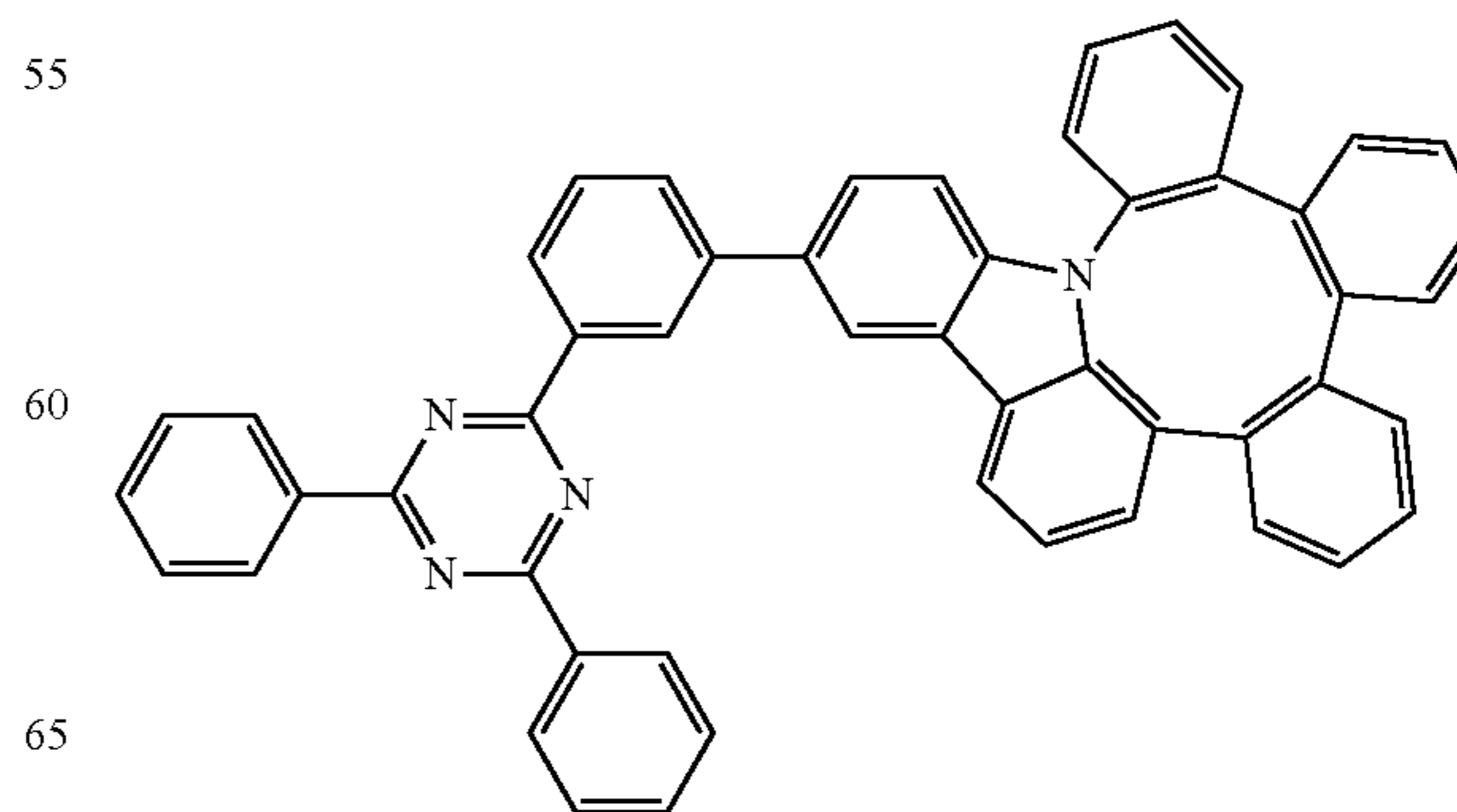
Compound 30
