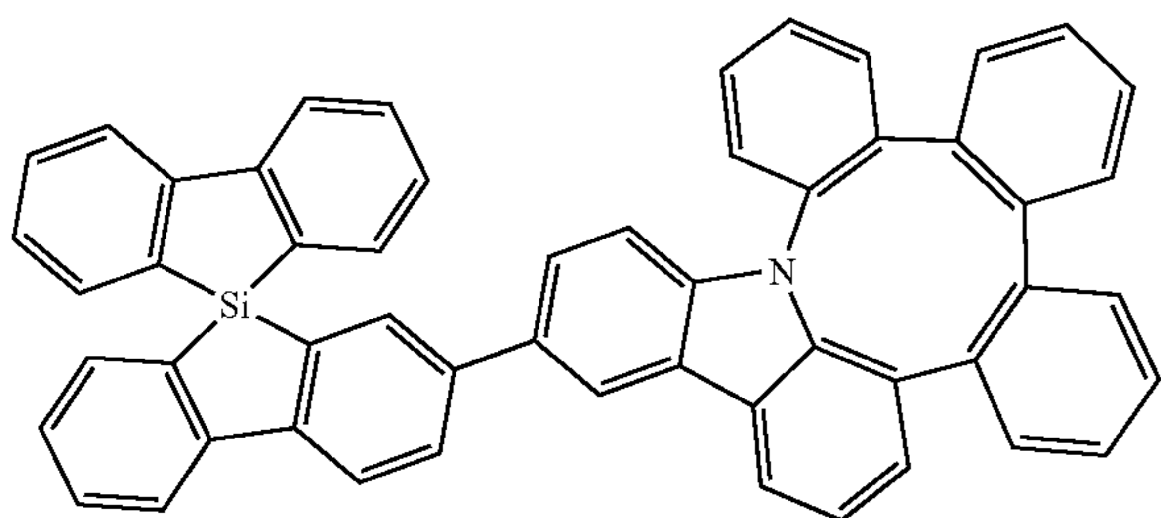
Compound 341
