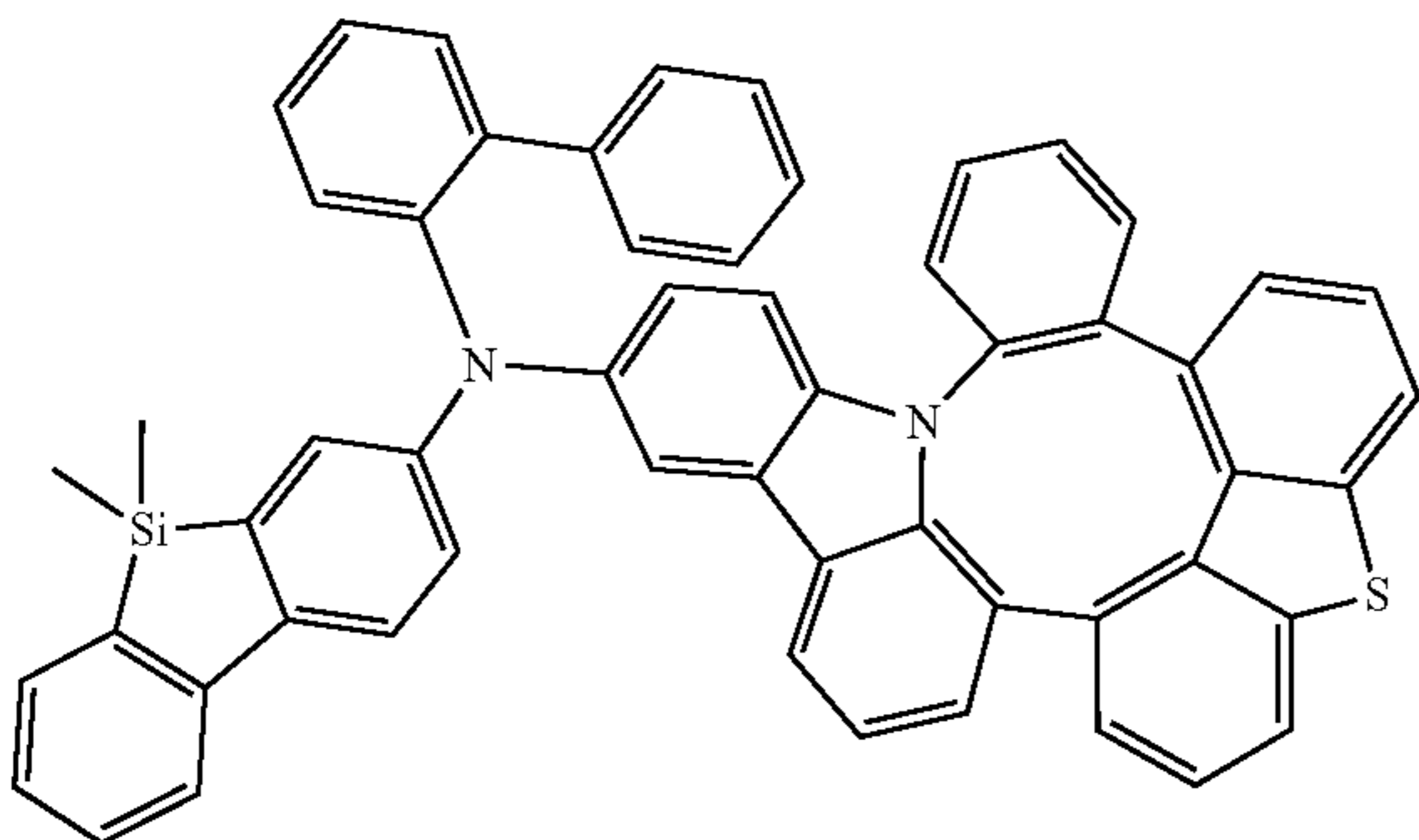
Compound 359
