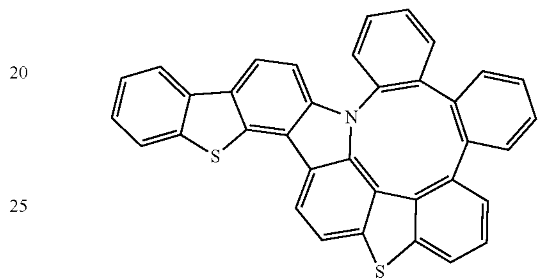
Compound 318
