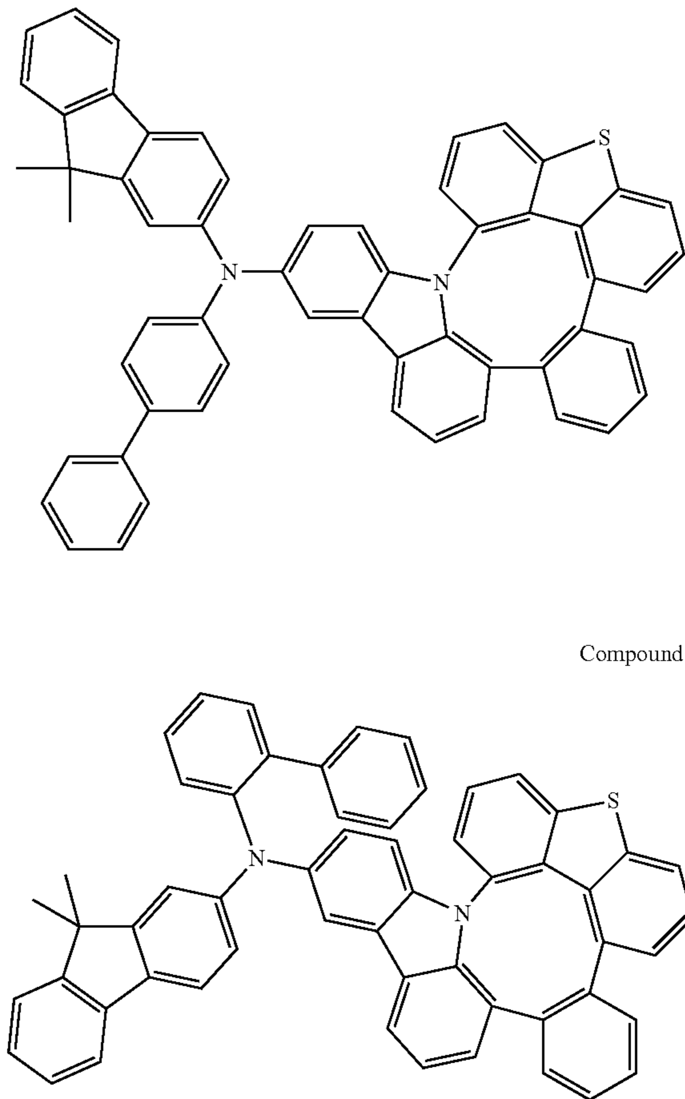
Compound 127
