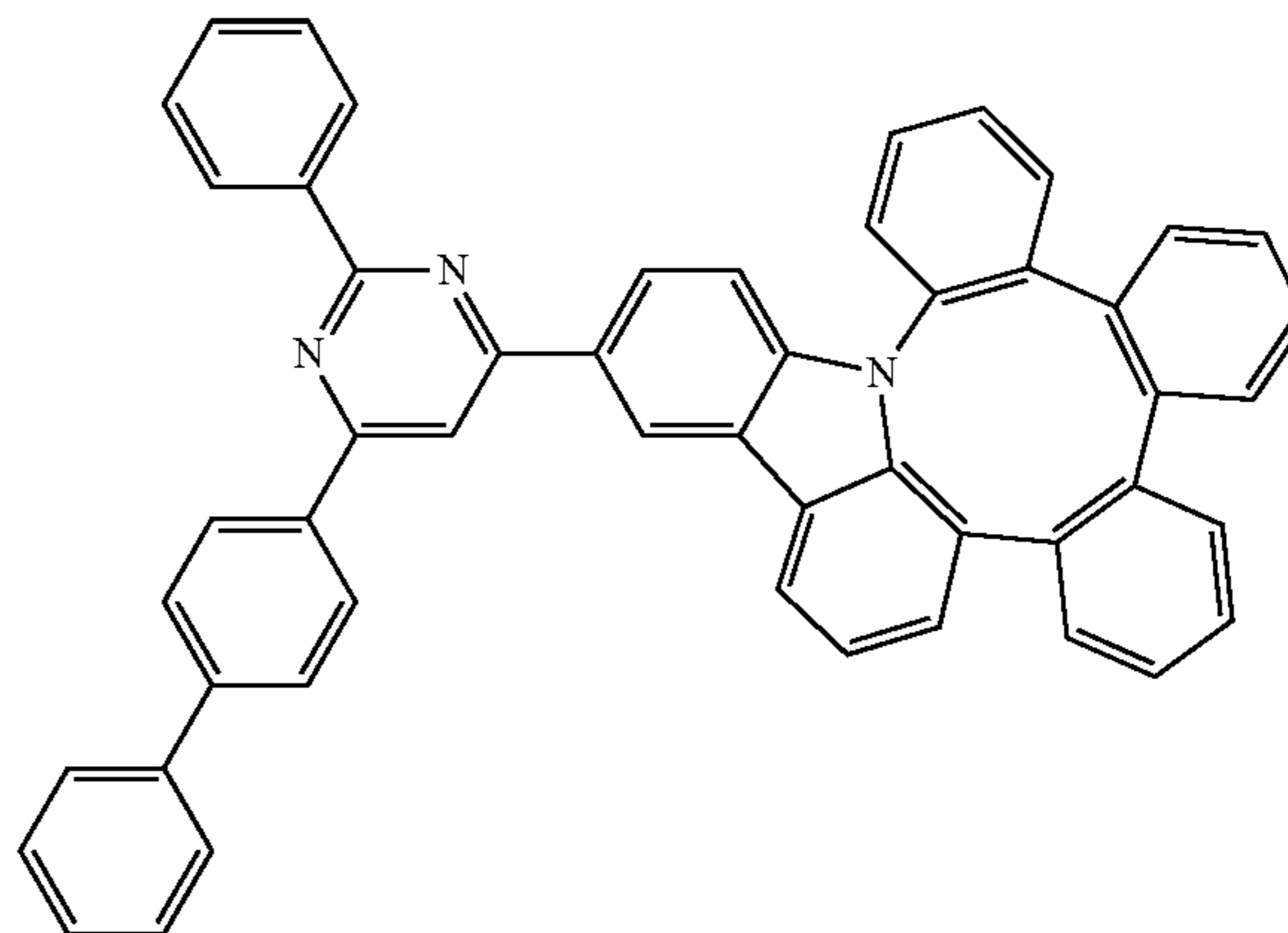
Compound 28
