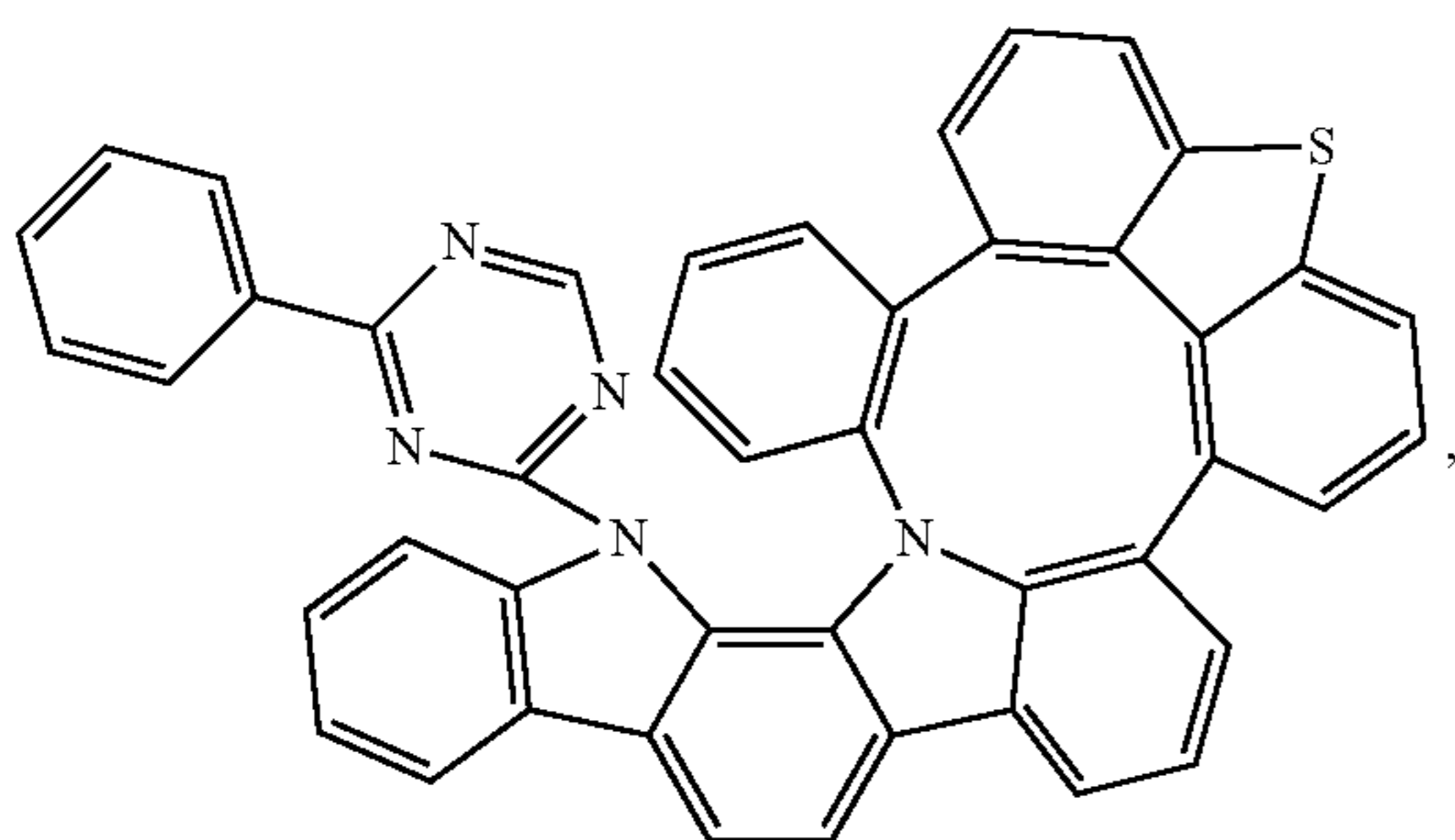
Compound 250
