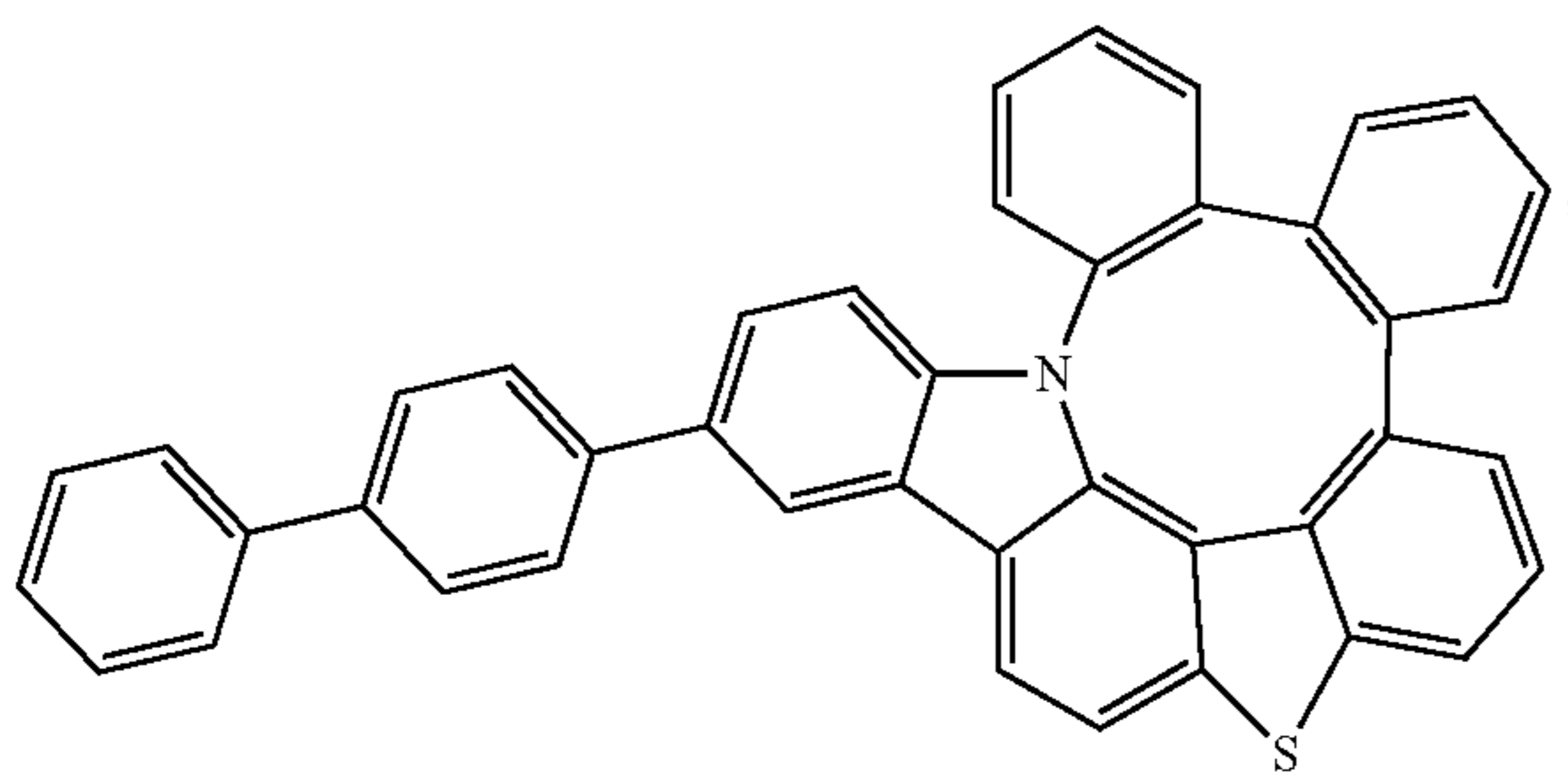
Compound 258
