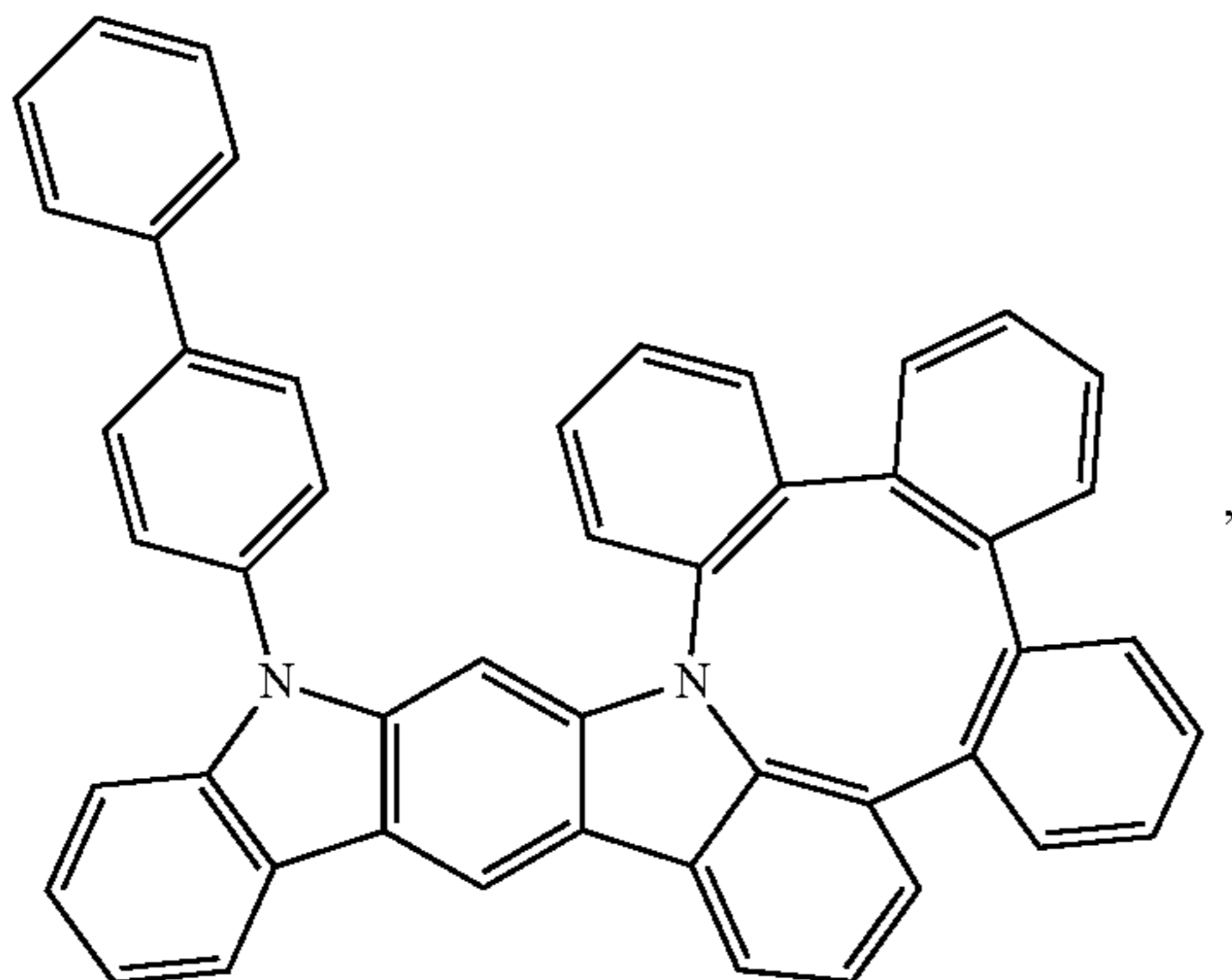
Compound 58
