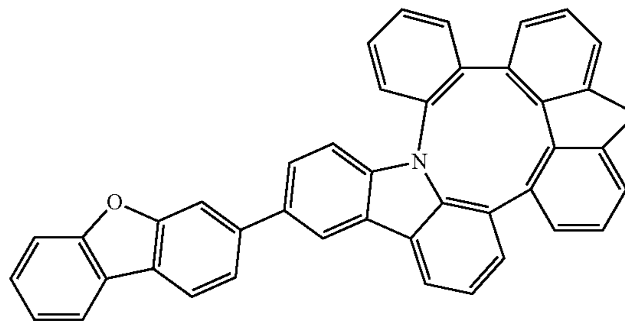
Compound 177
