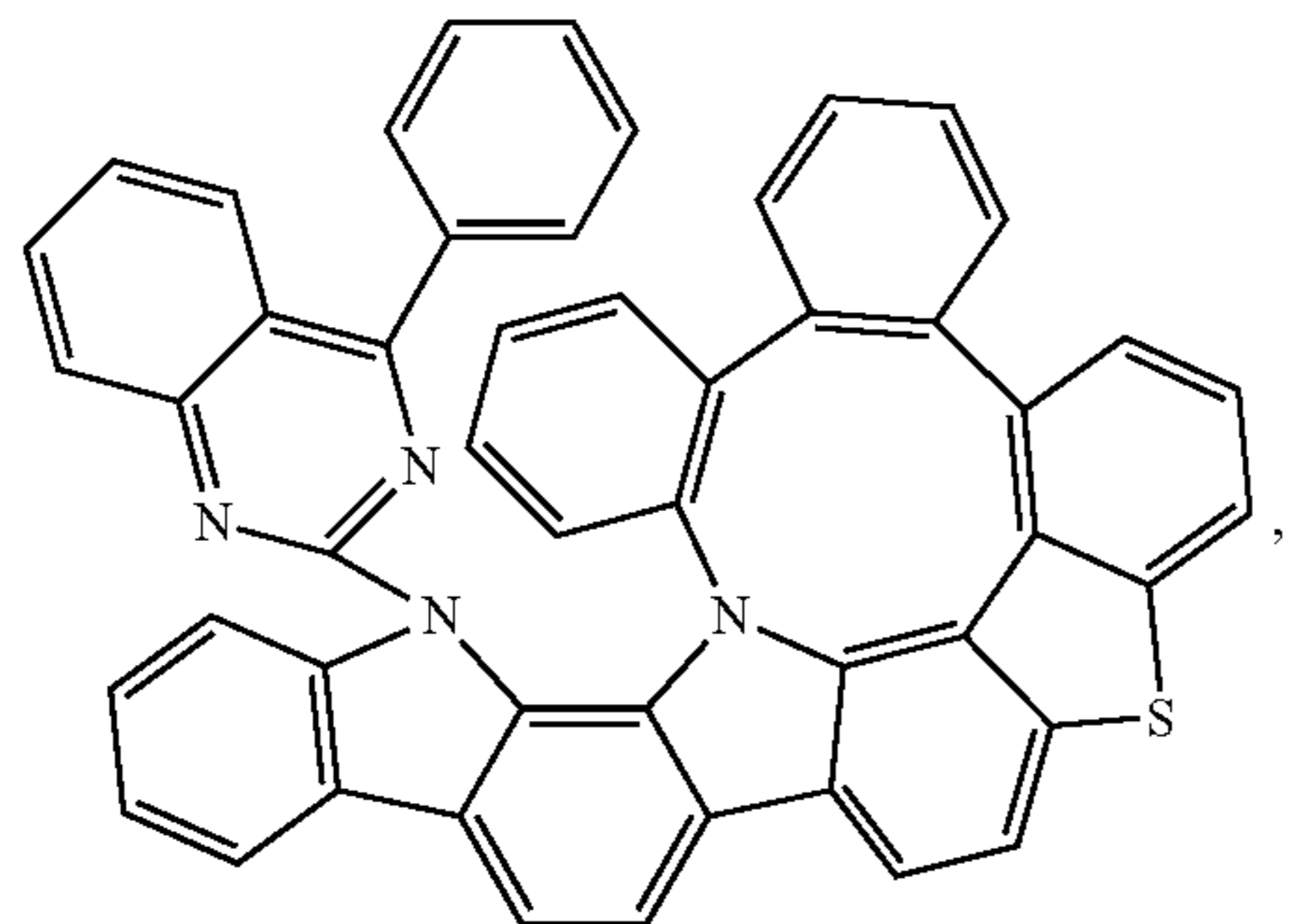
Compound 341
