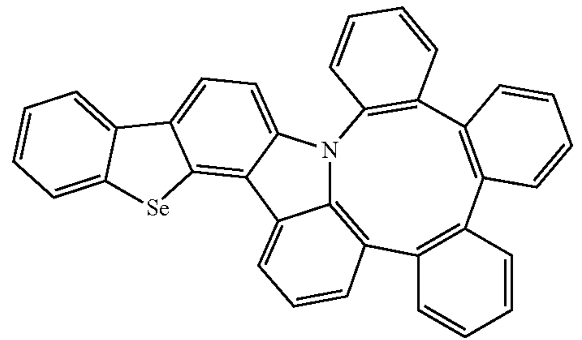
Compound 68
