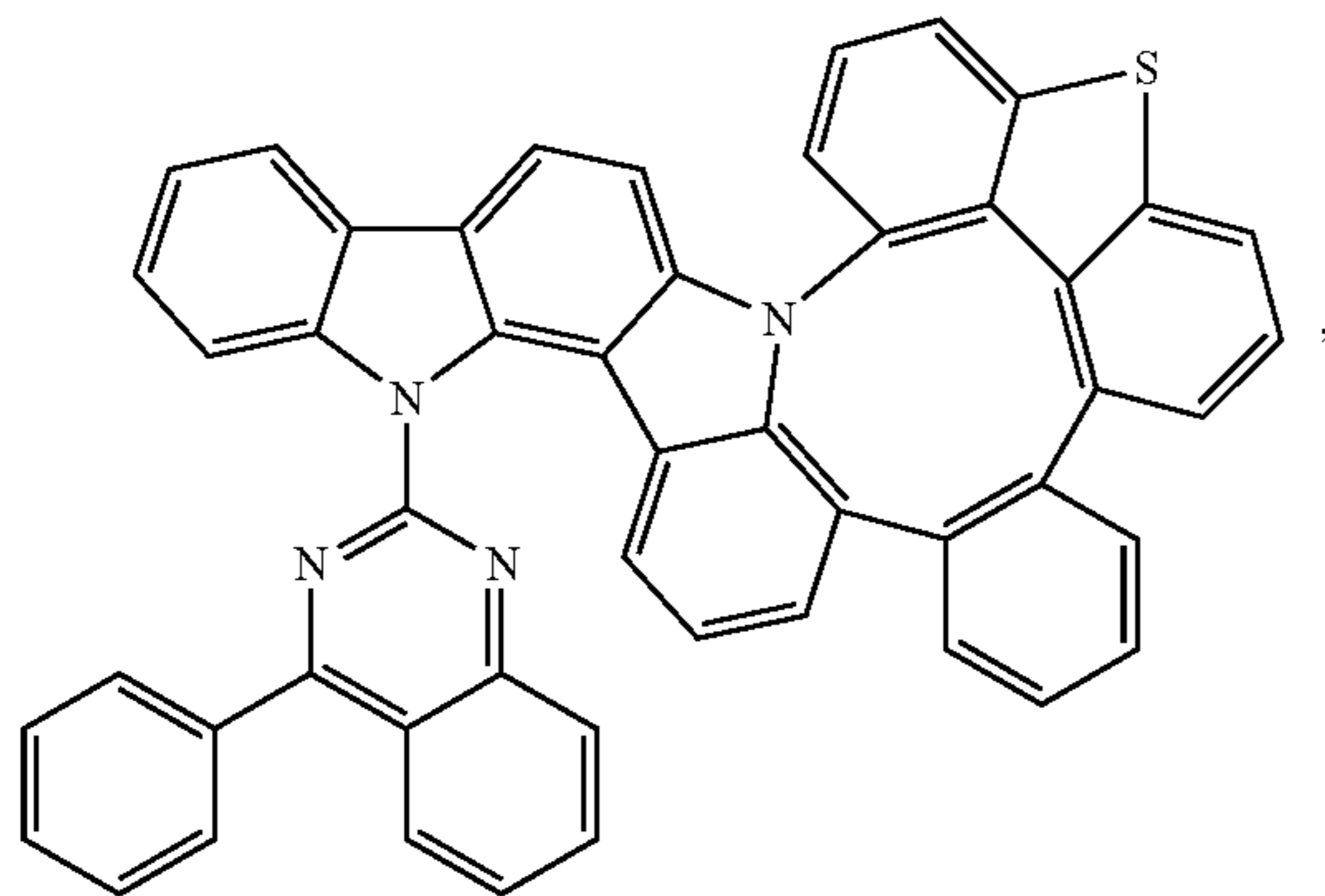
Compound 165
