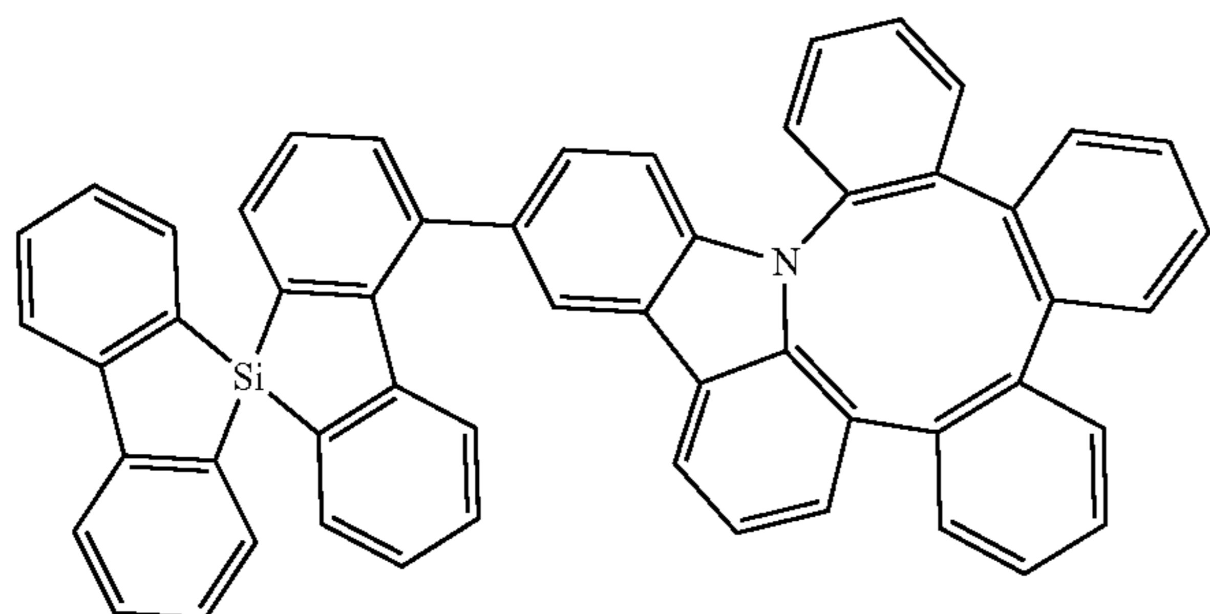
Compound 343
