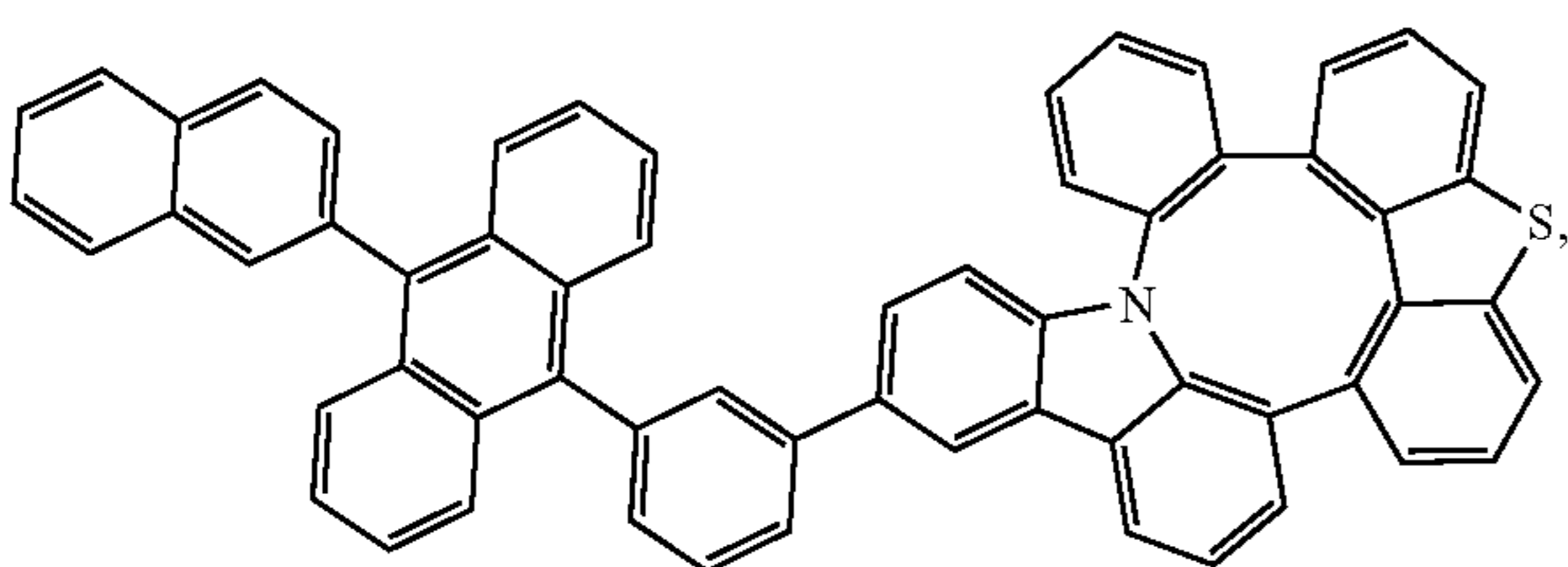
Compound 210
