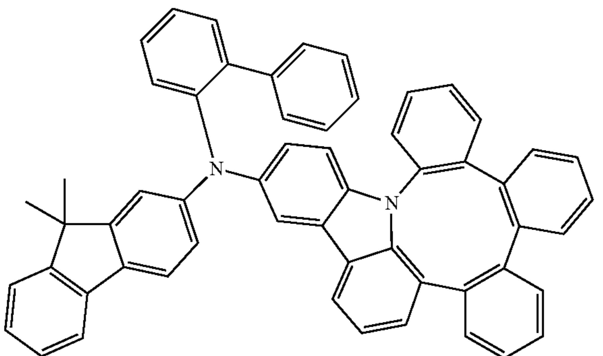
Compound 43
