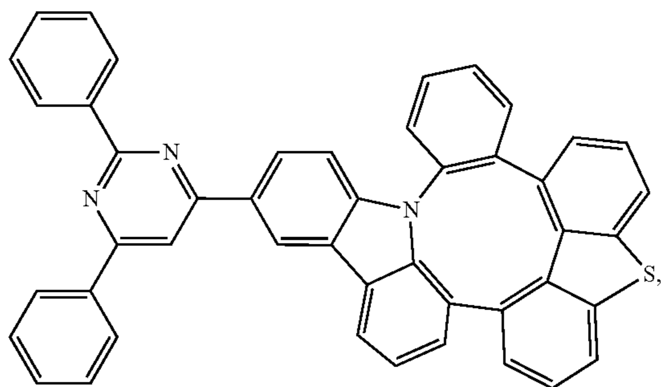
Compound 197
