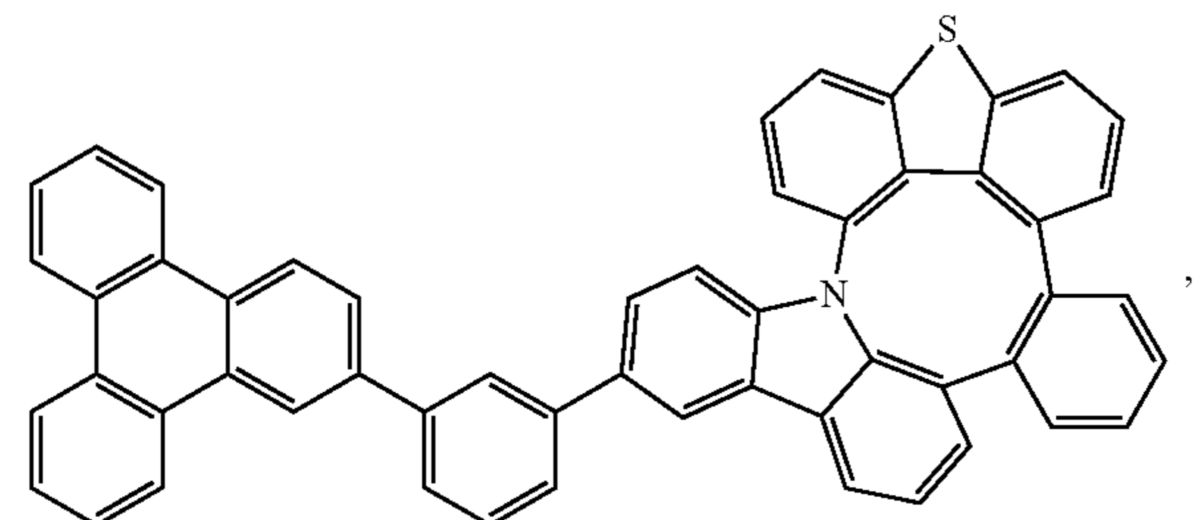
Compound 120
