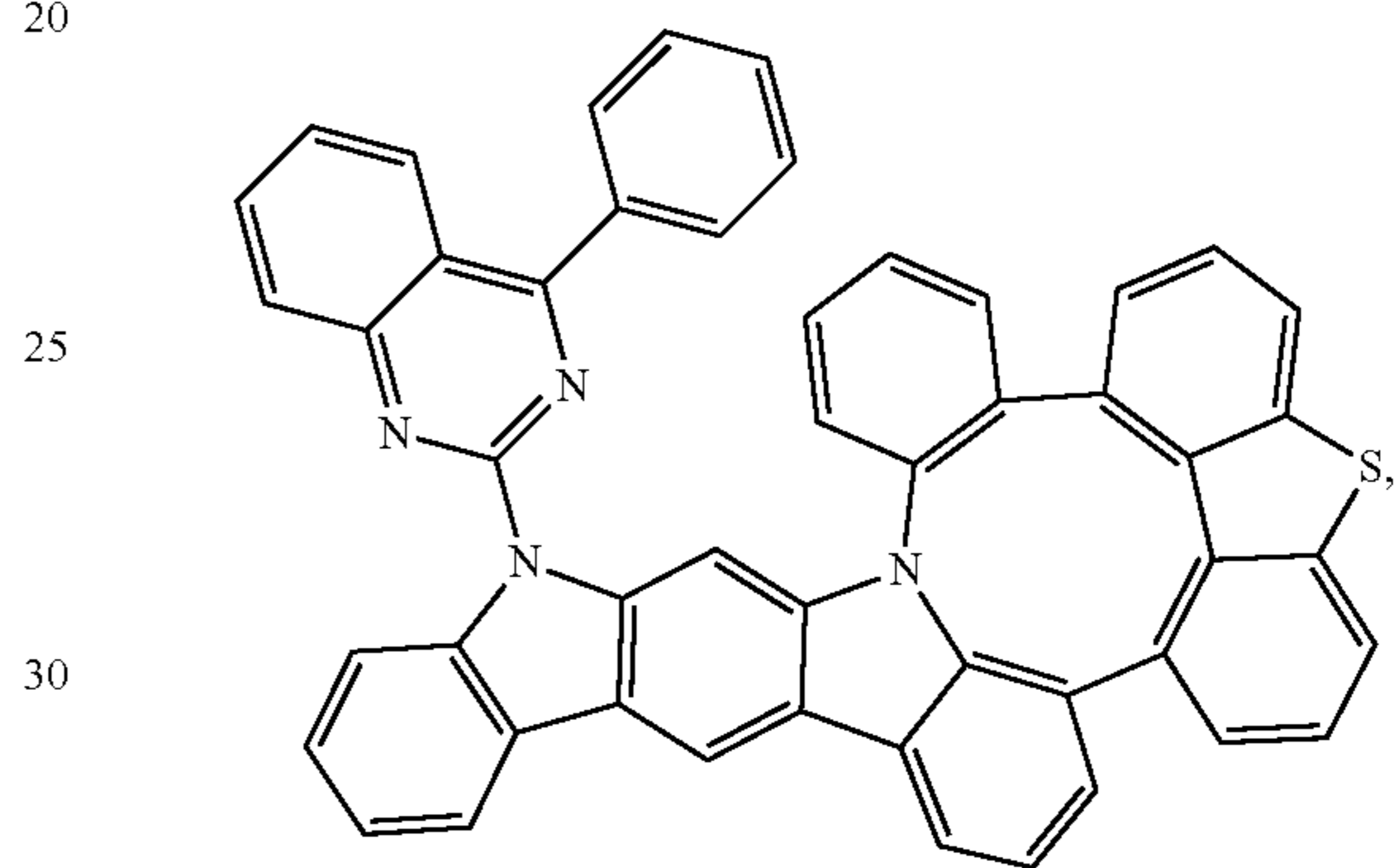
Compound 253
