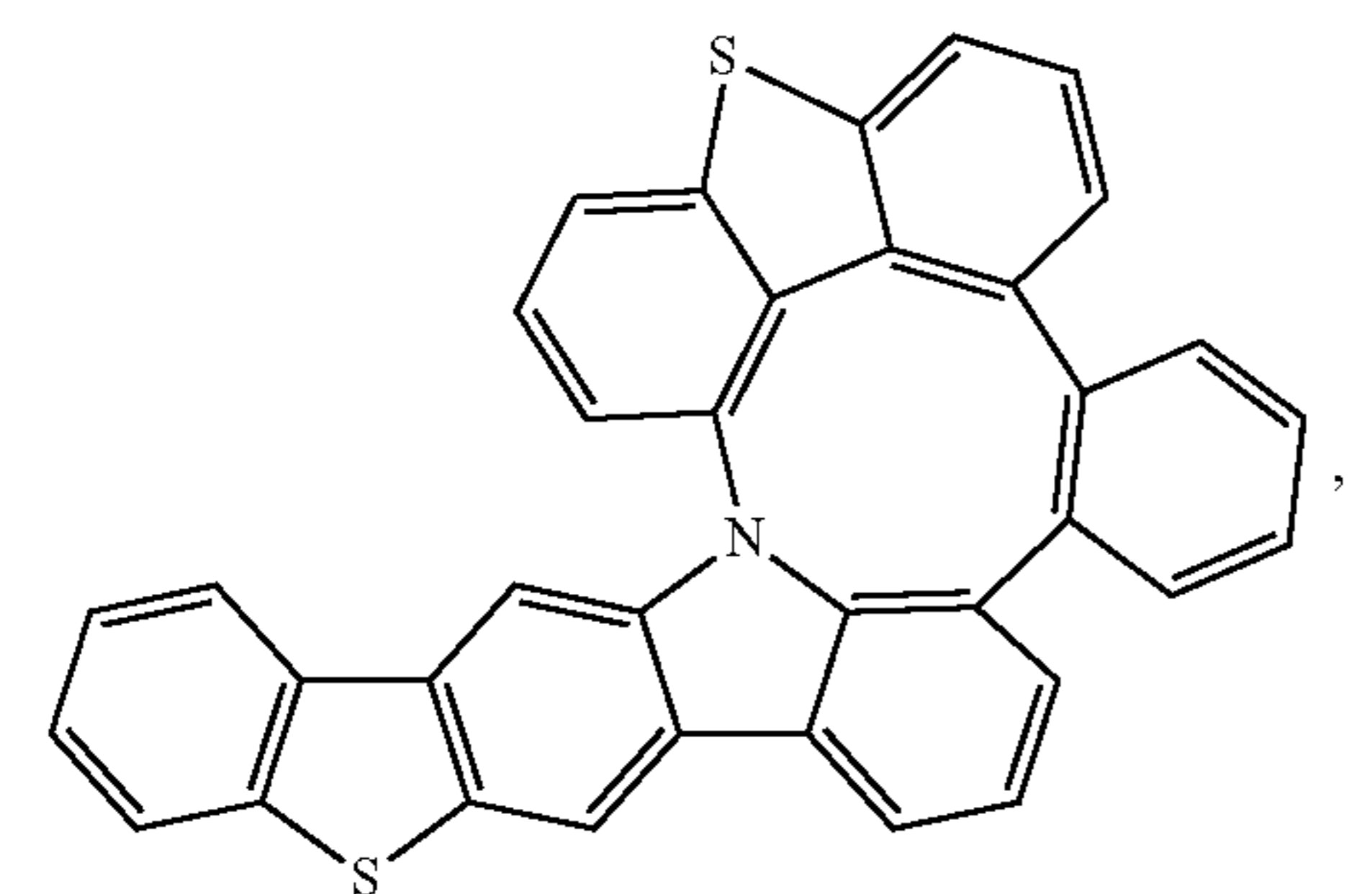
Compound 150
