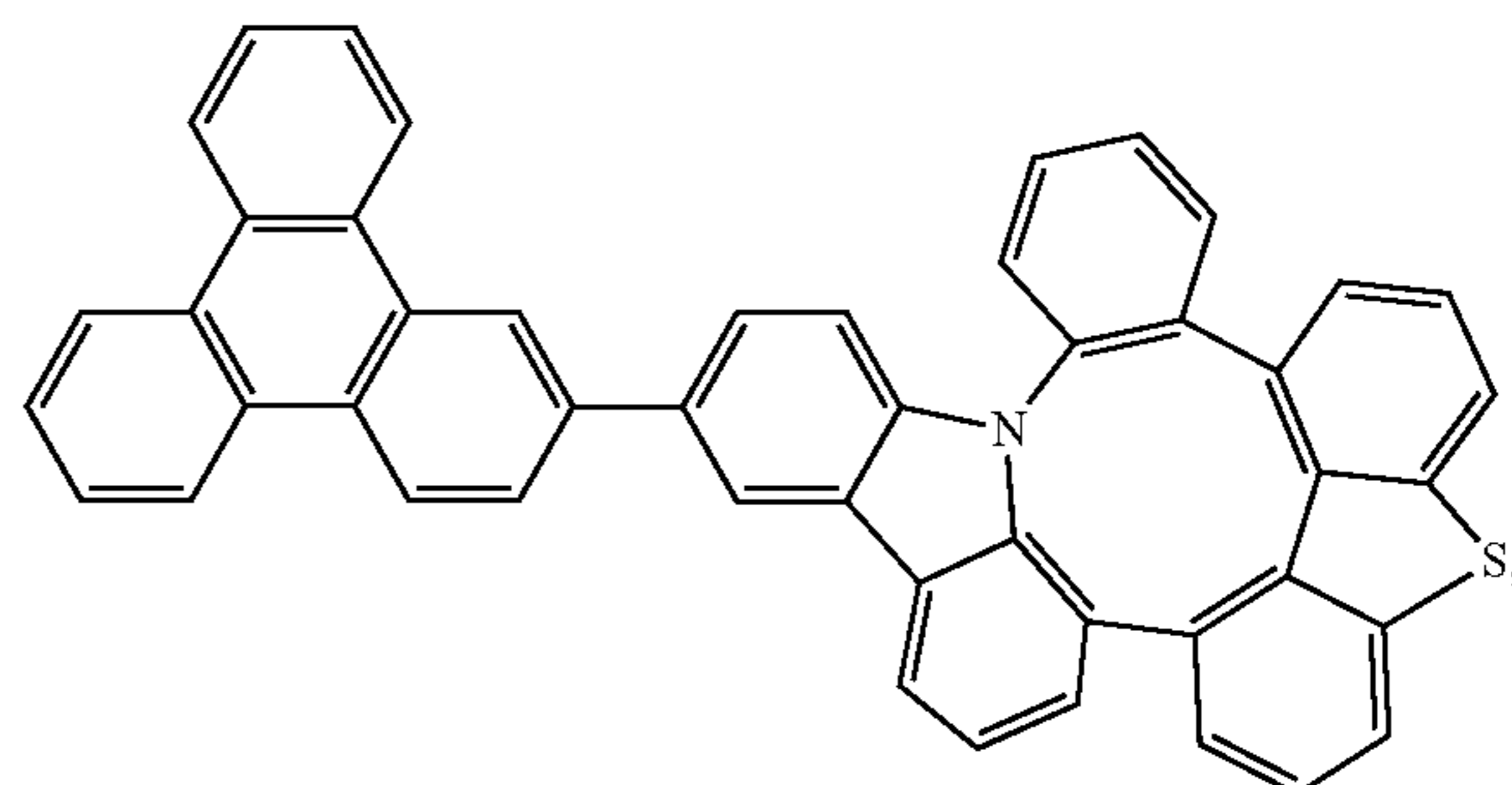
Compound 204
