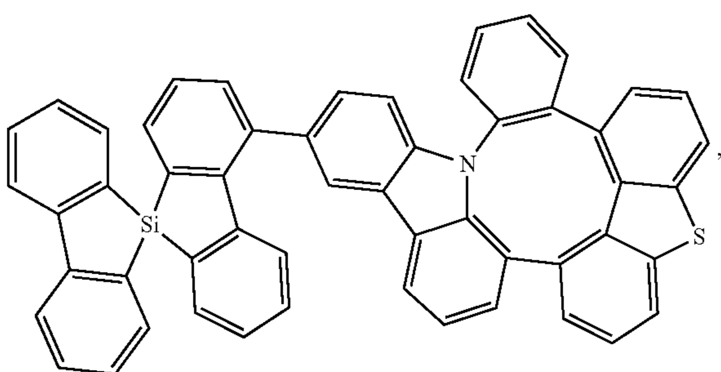
Compound 357
