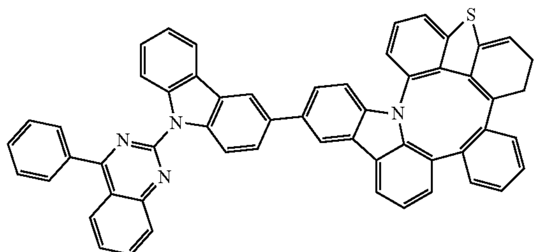
Compound 105
