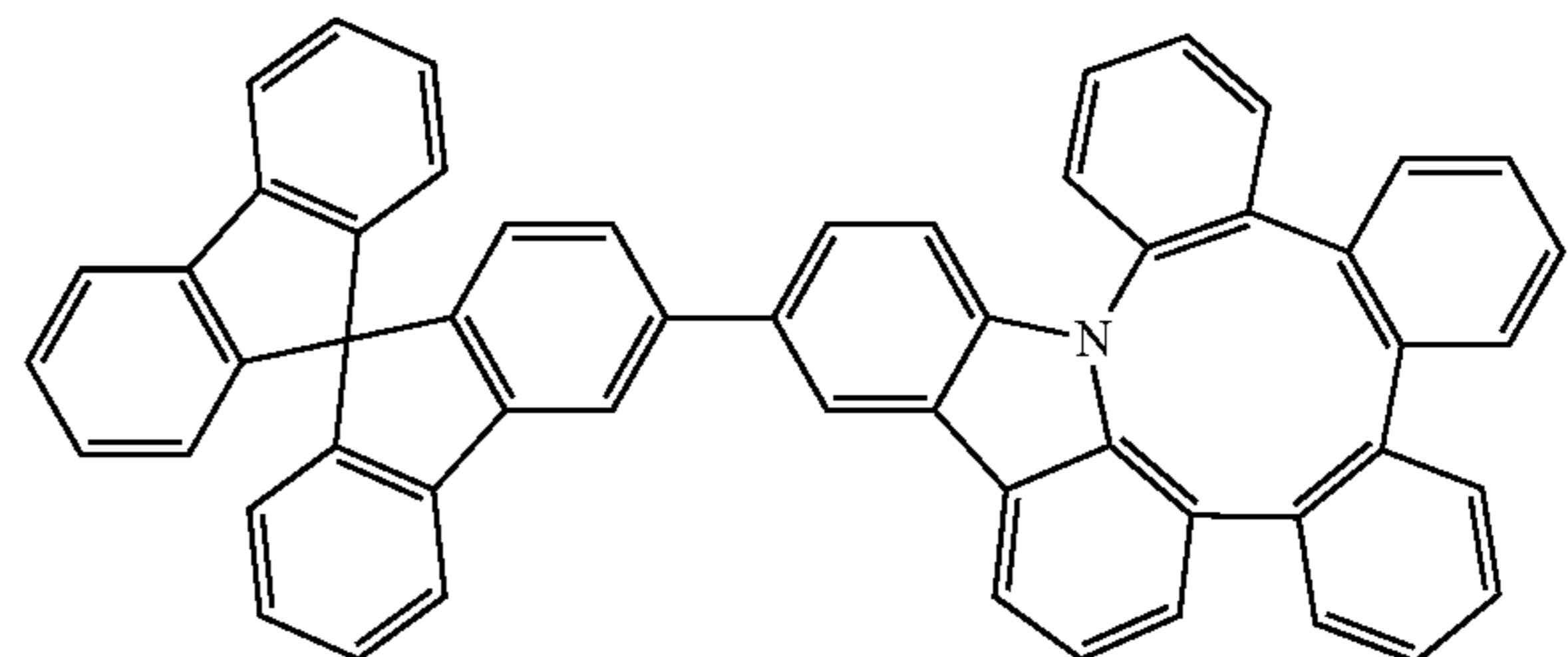
Compound 23
