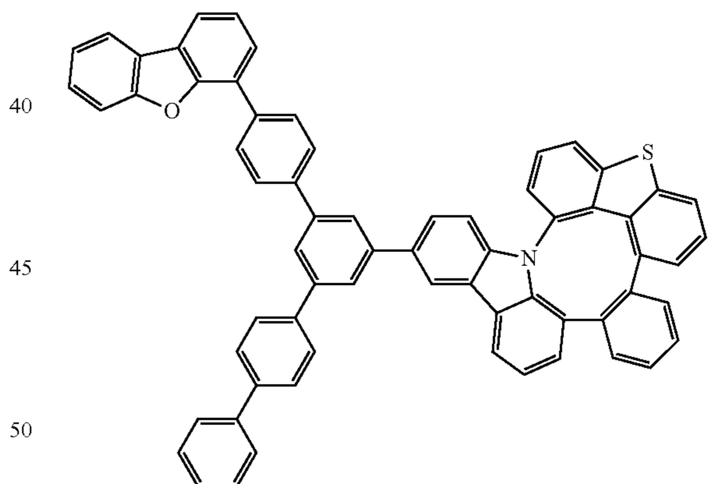
Compound 135
