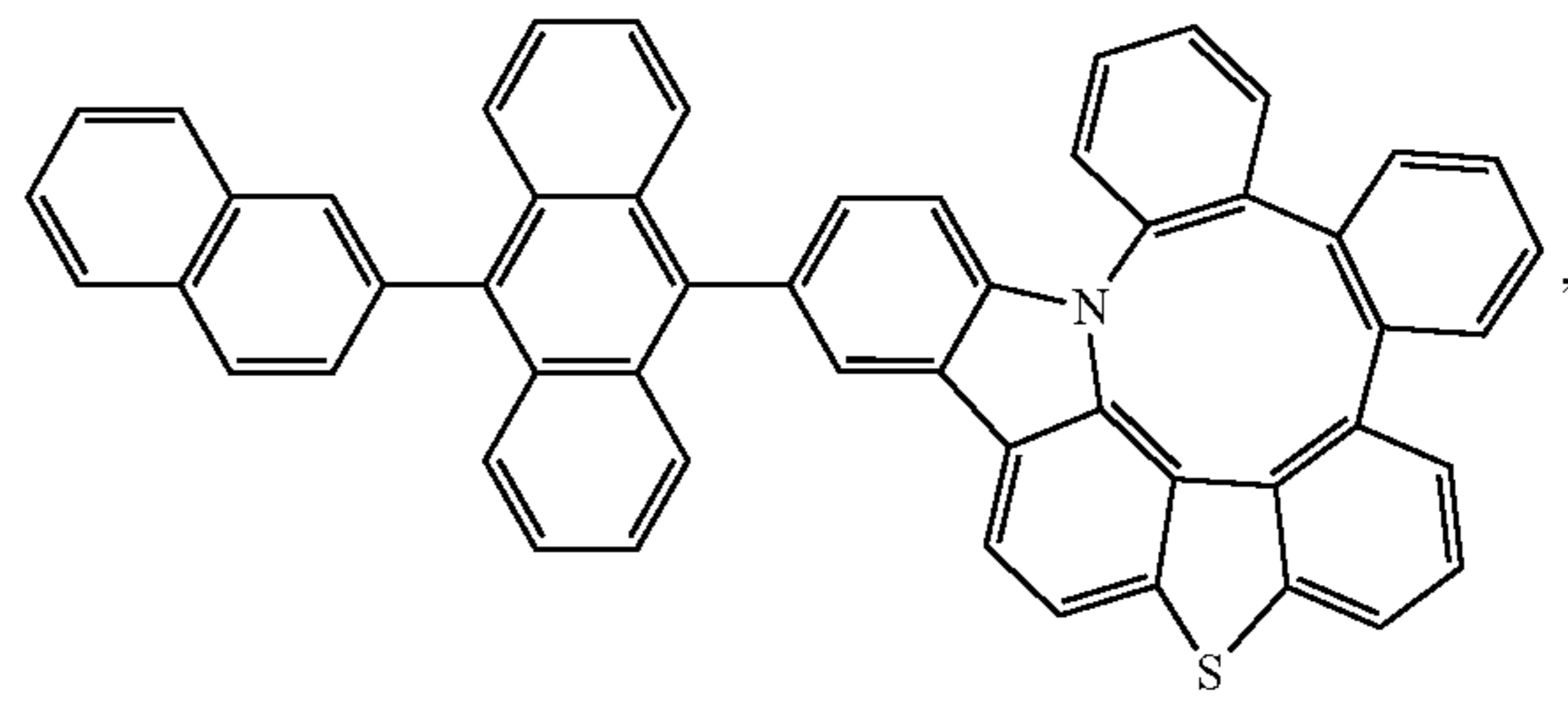
Compound 293
