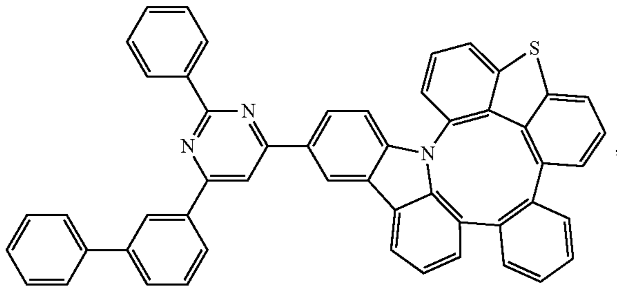
Compound 114
