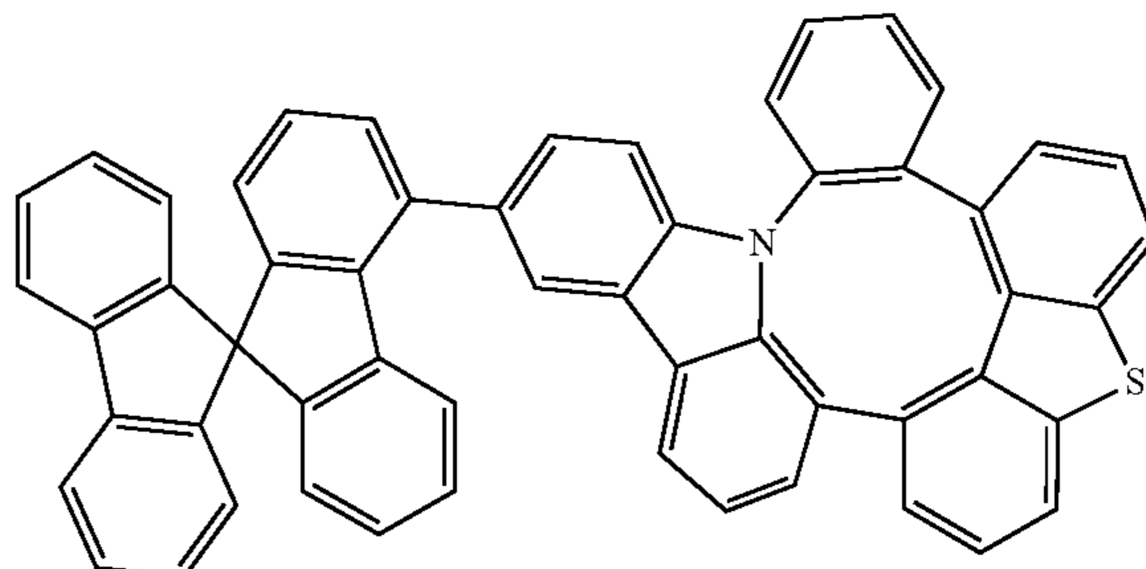
Compound 194
