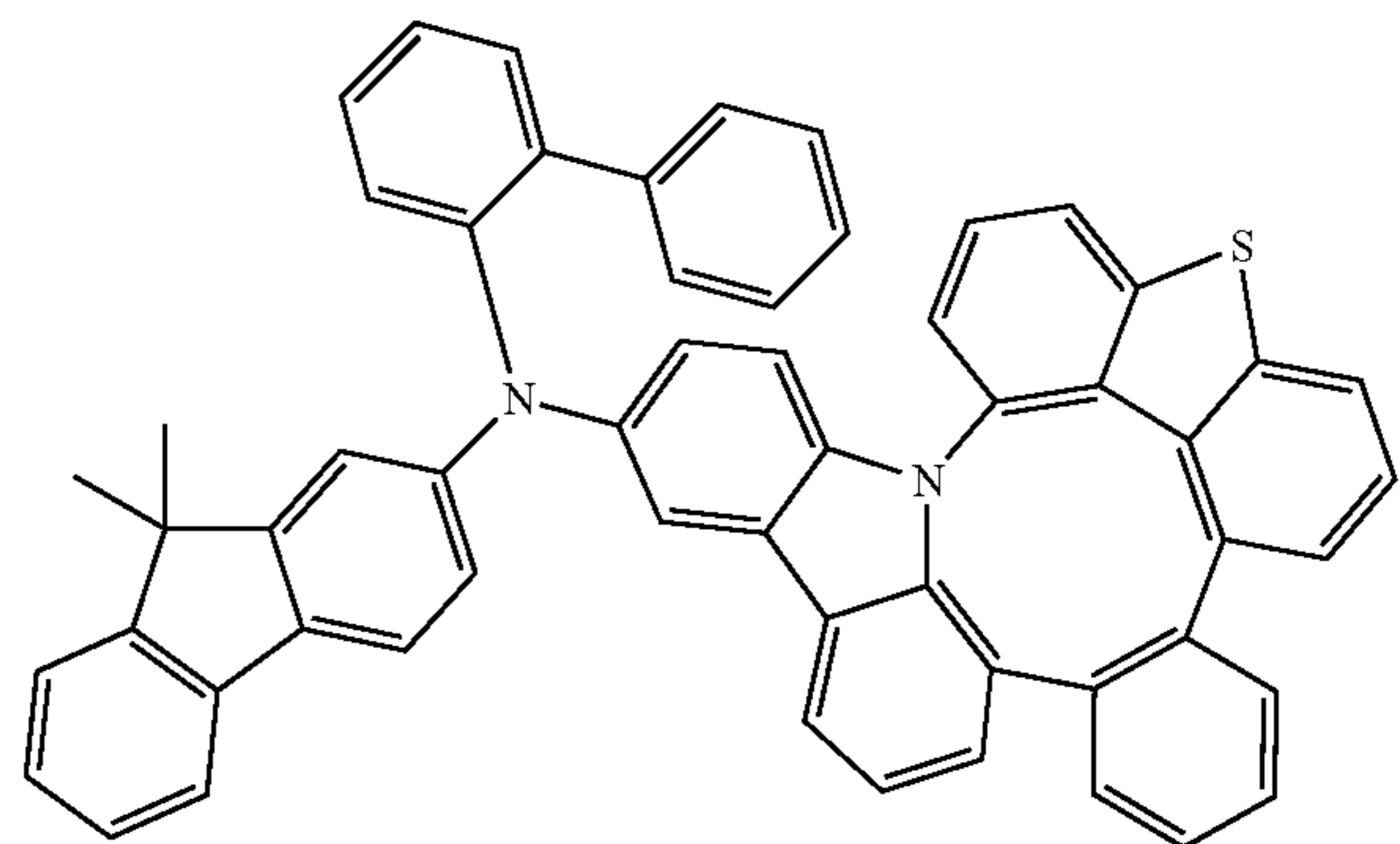
Compound 128
