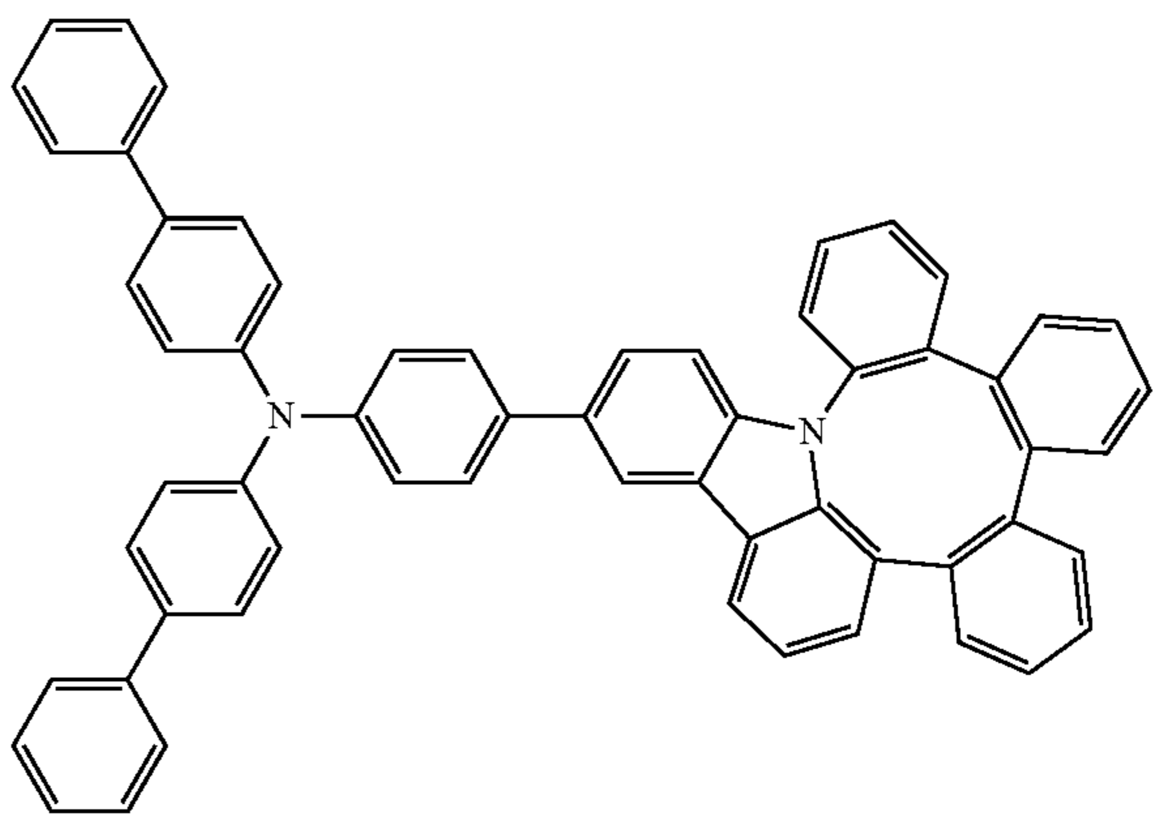
Compound 46
