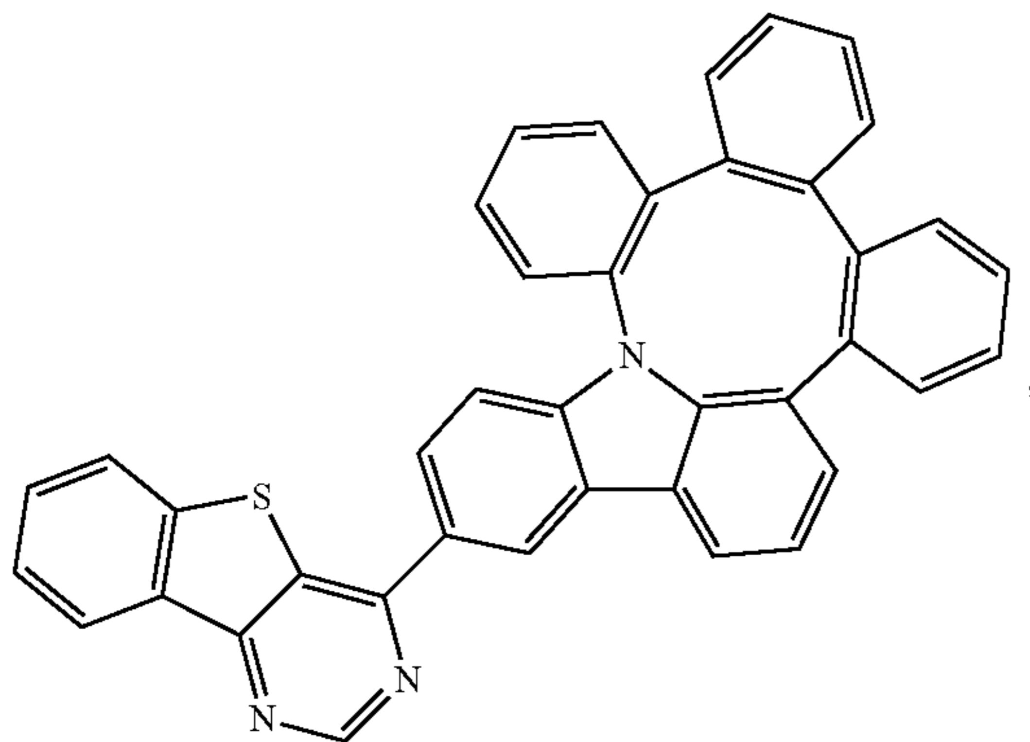
Compound 32
