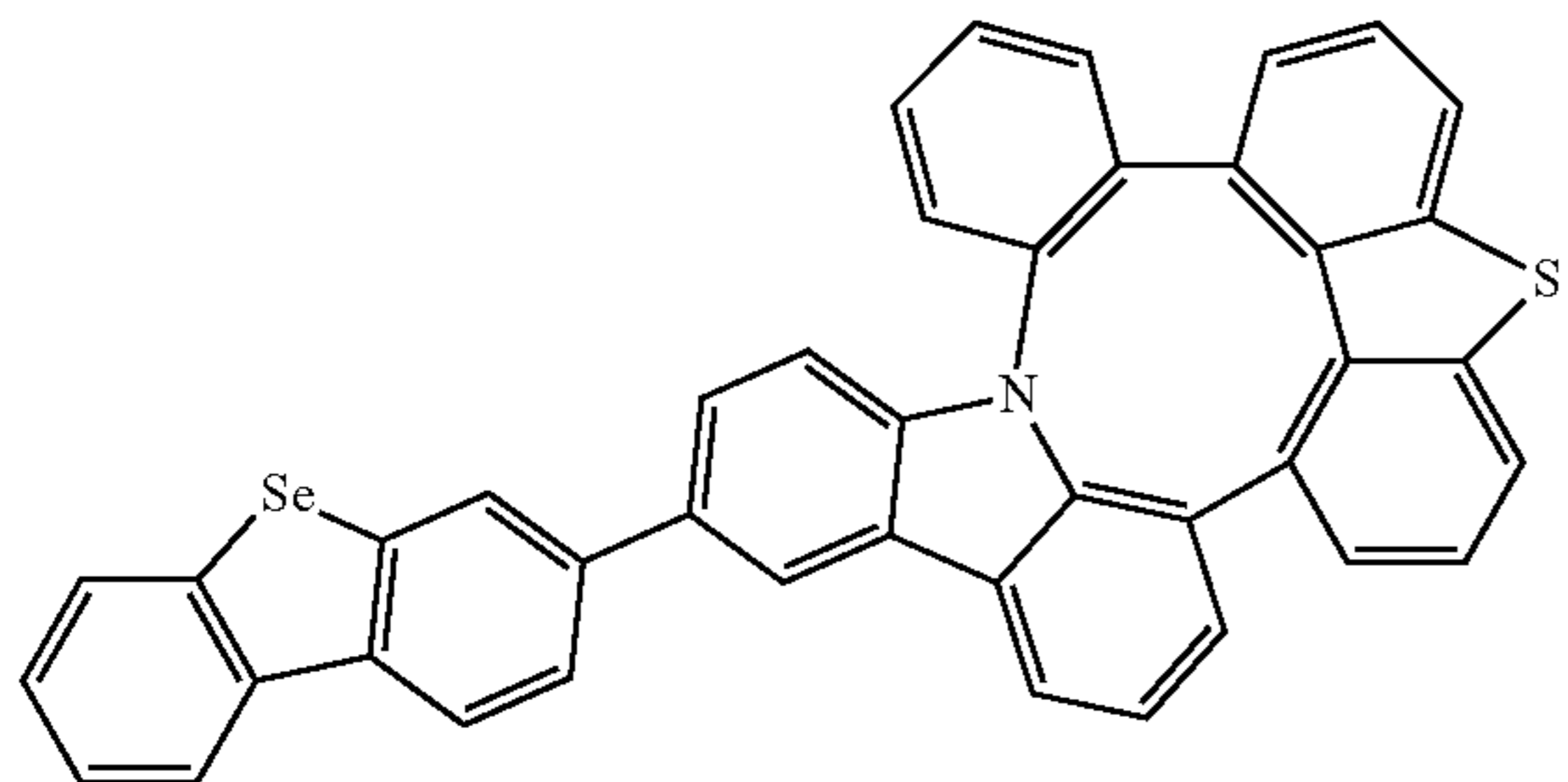
Compound 182
