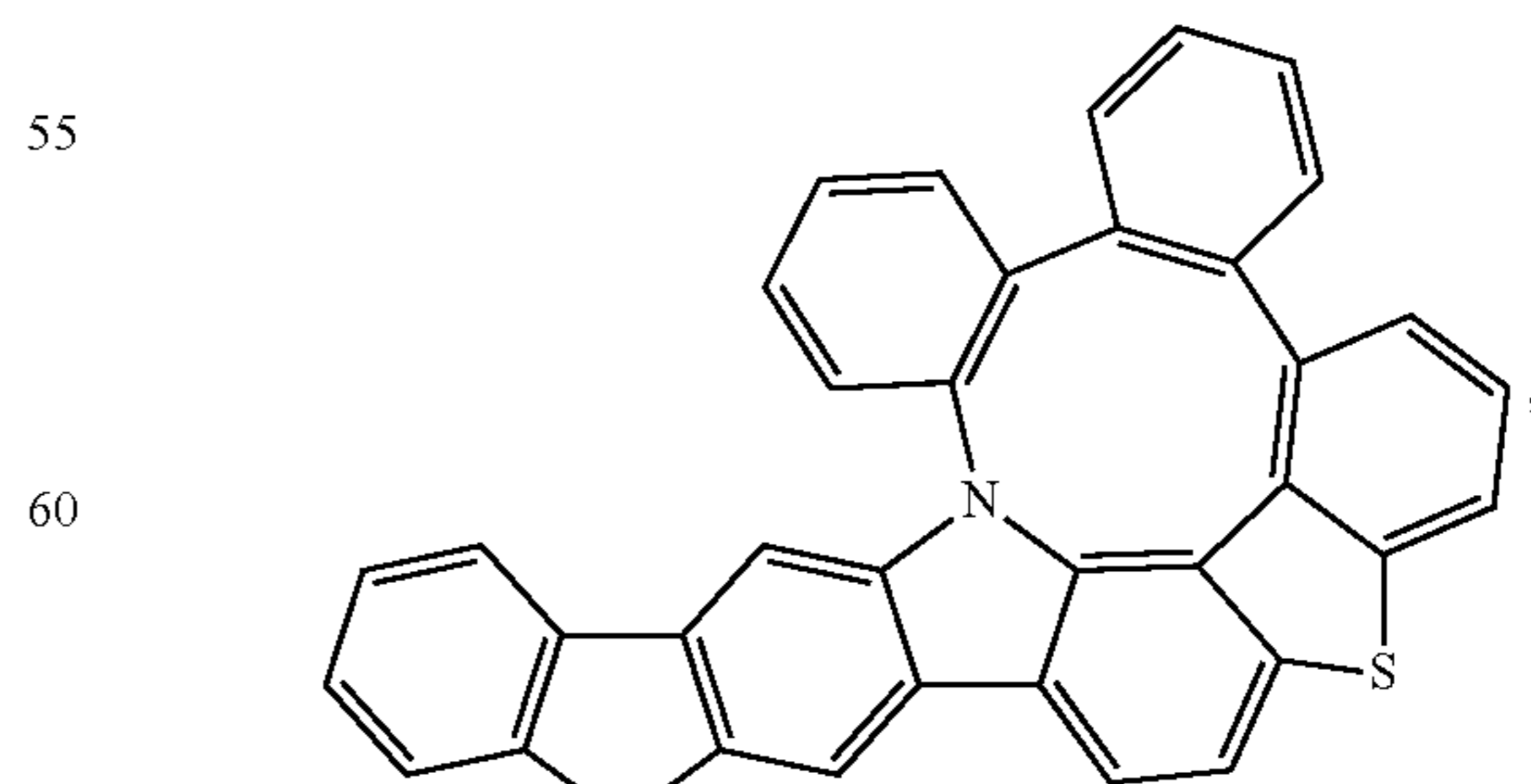
Compound 320
