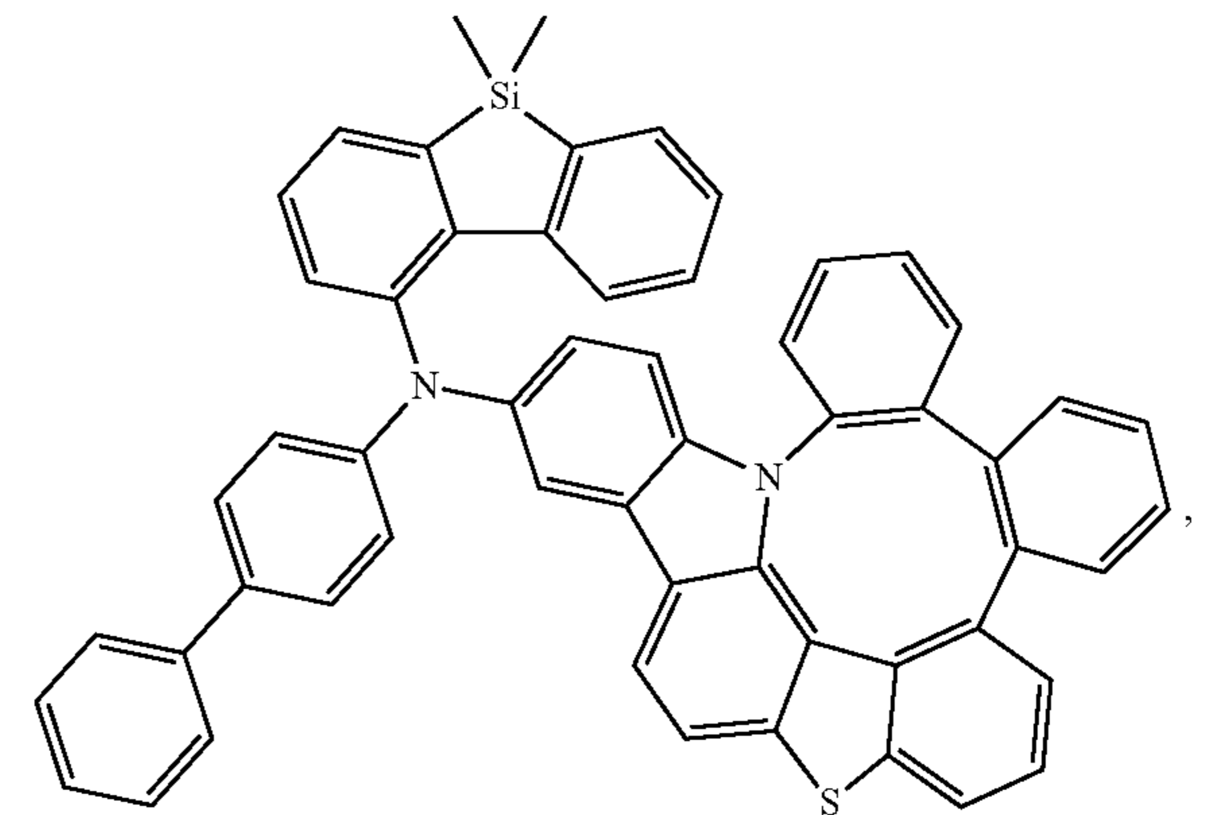
Compound 367
