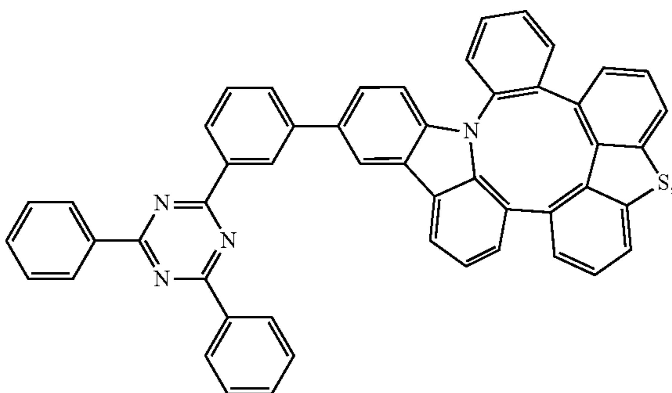
Compound 200
