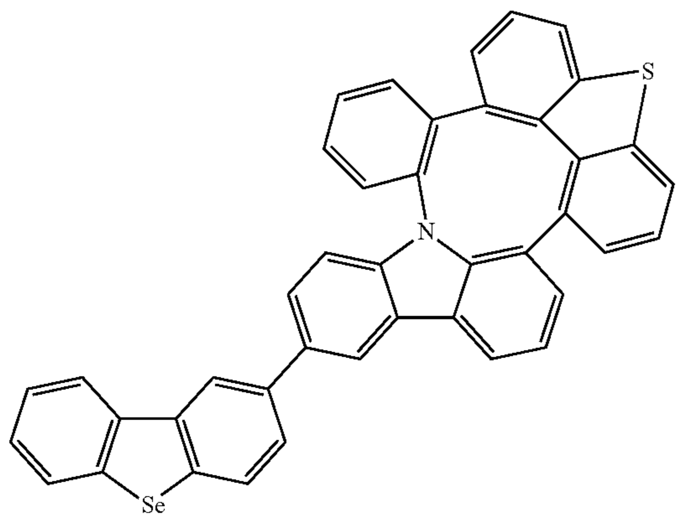
Compound 182
