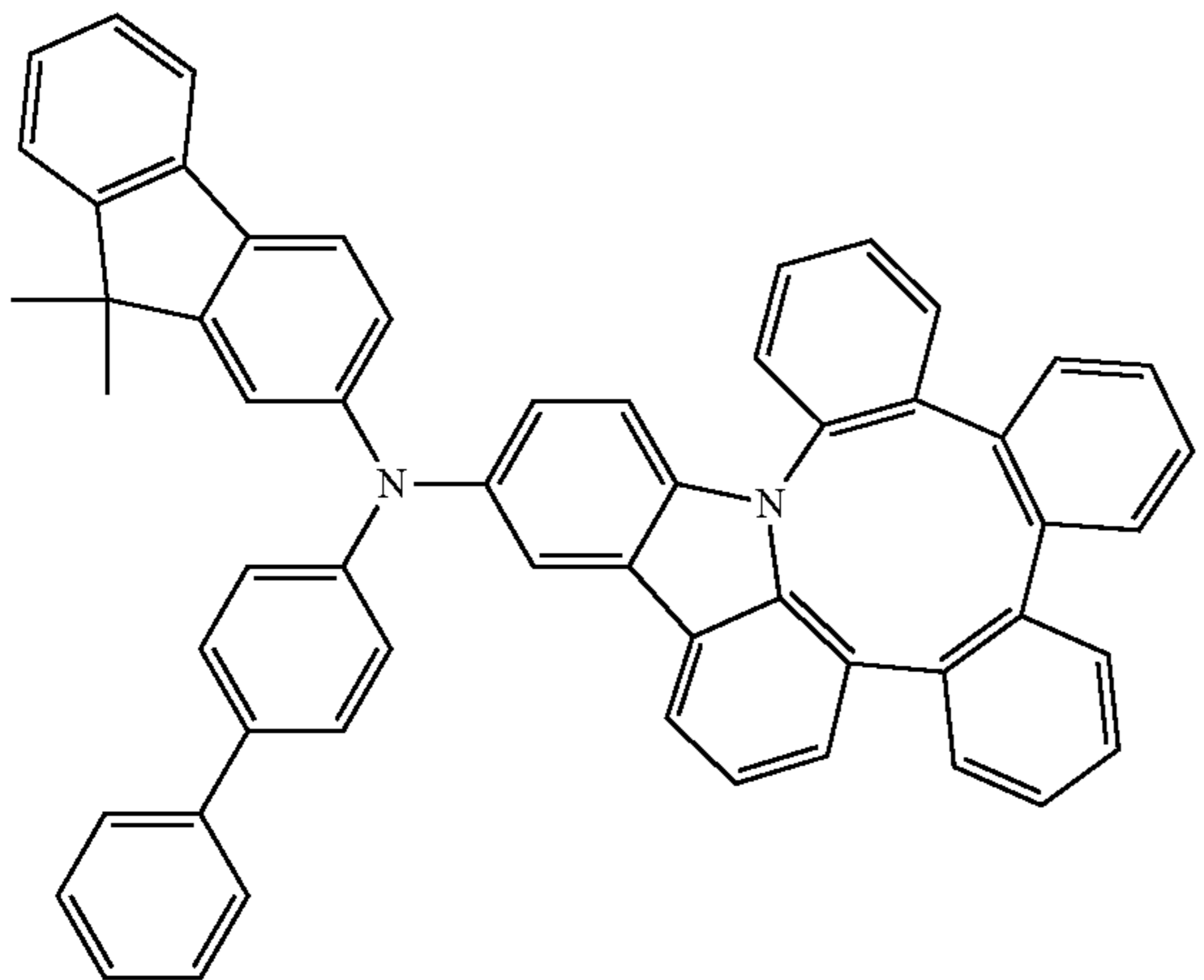
Compound 43
