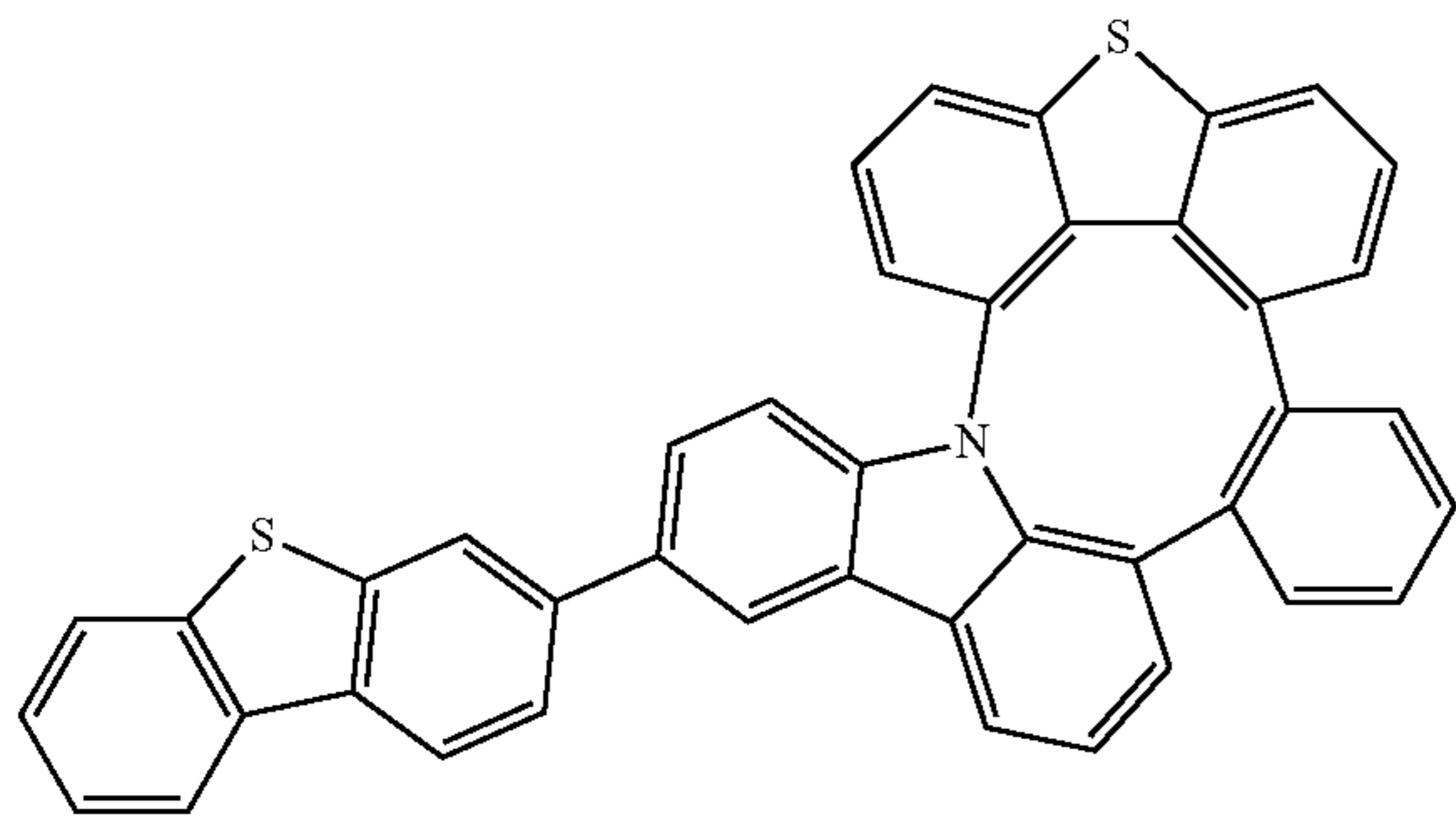
Compound 95
