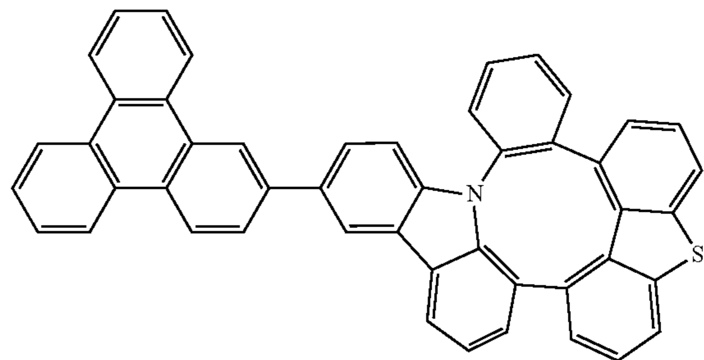
Compound 204
