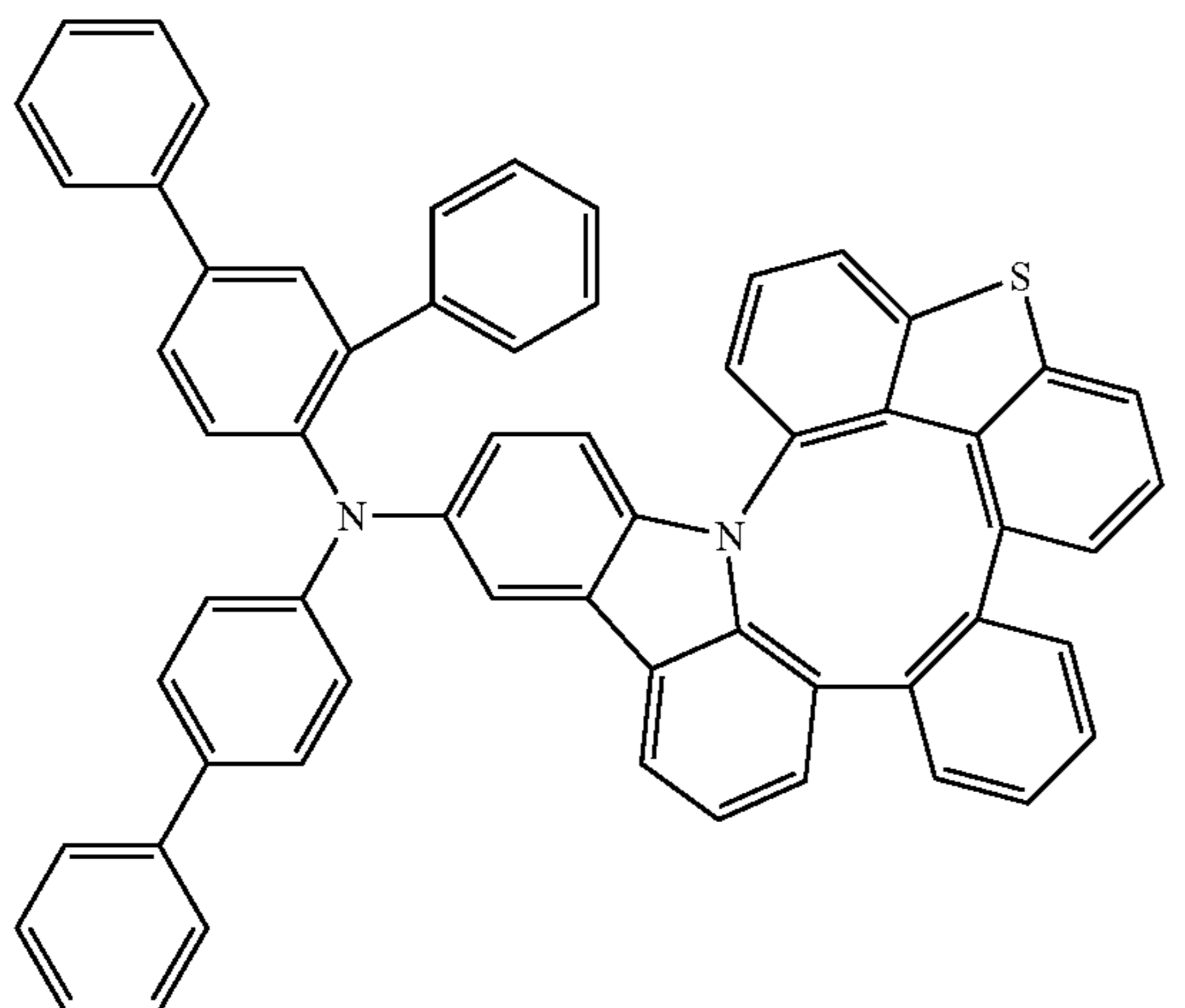
Compound 130
