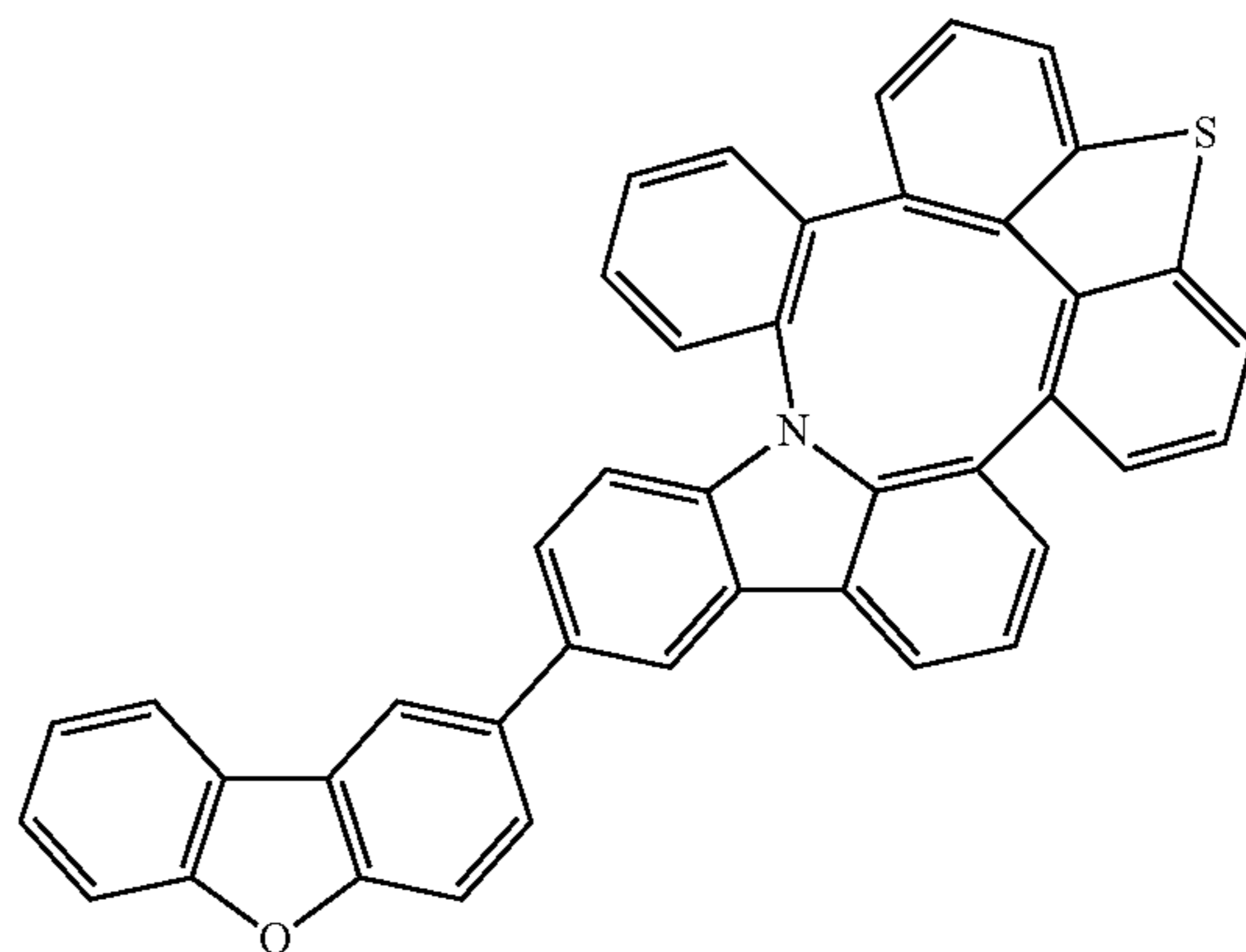
Compound 175
