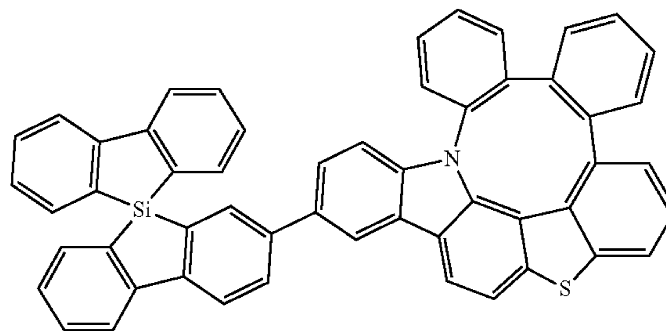
Compound 362
