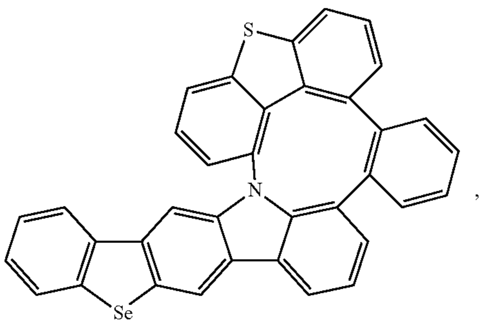
Compound 157
