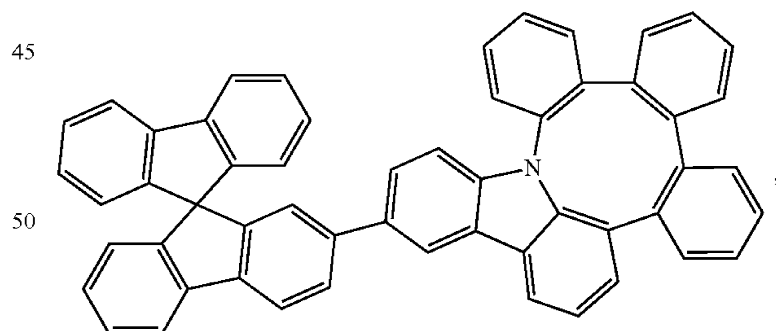
Compound 22
