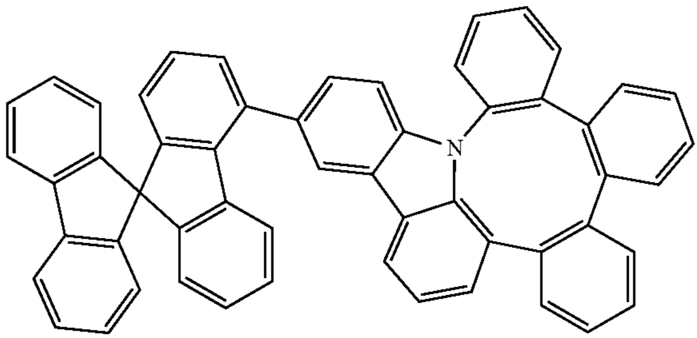
Compound 23
