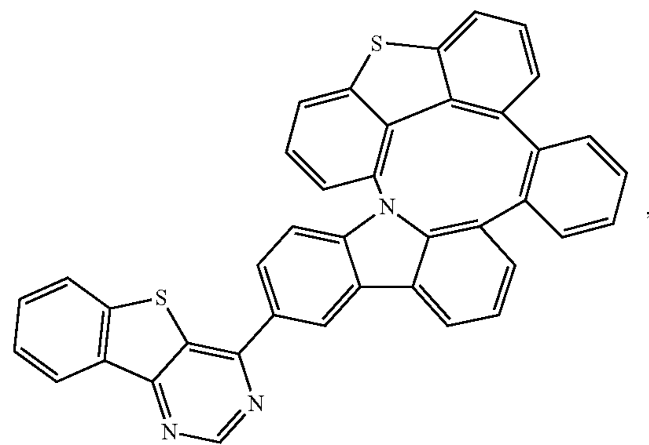
Compound 117
