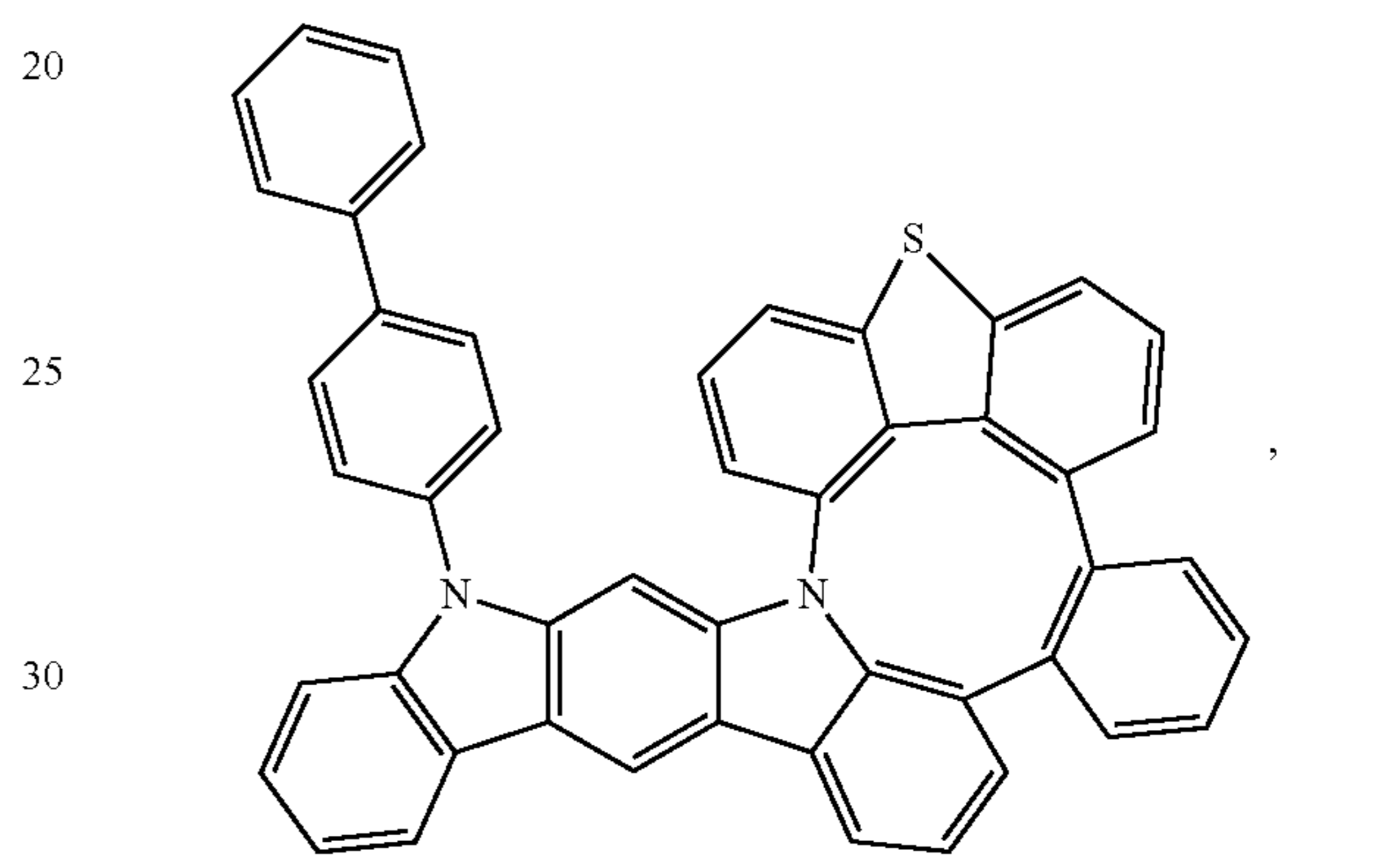
Compound 143
