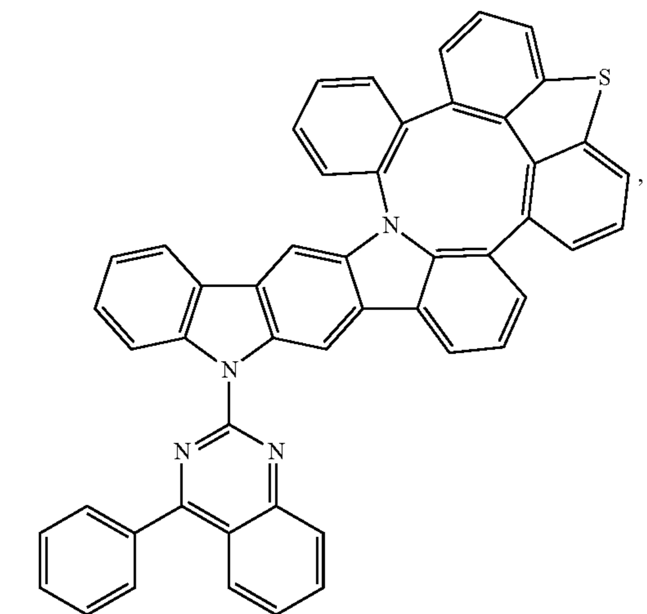
Compound 254
