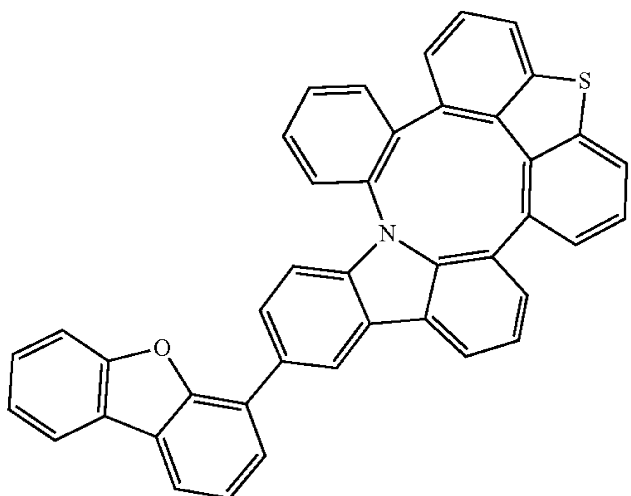
Compound 174
