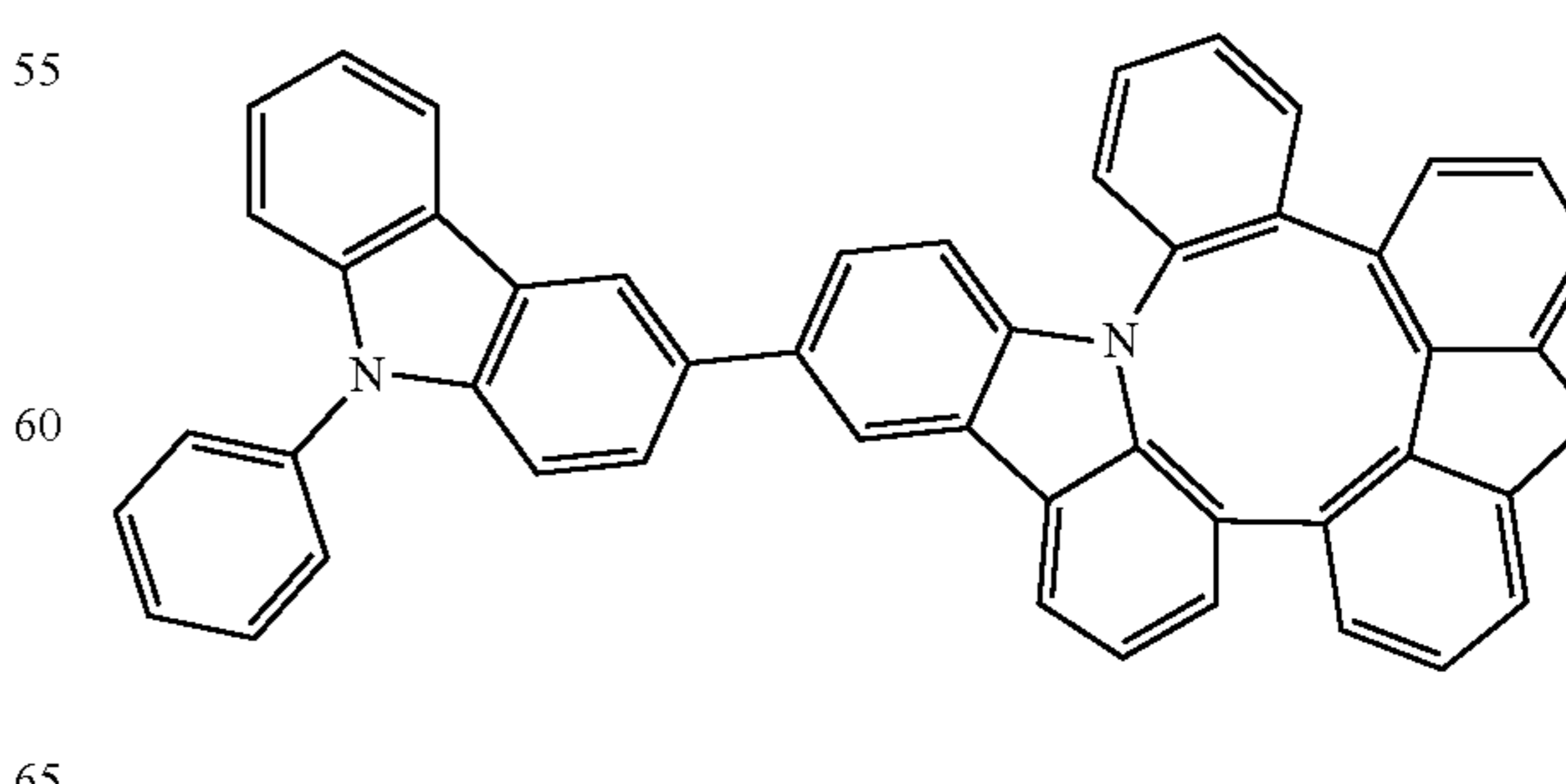
Compound 186
