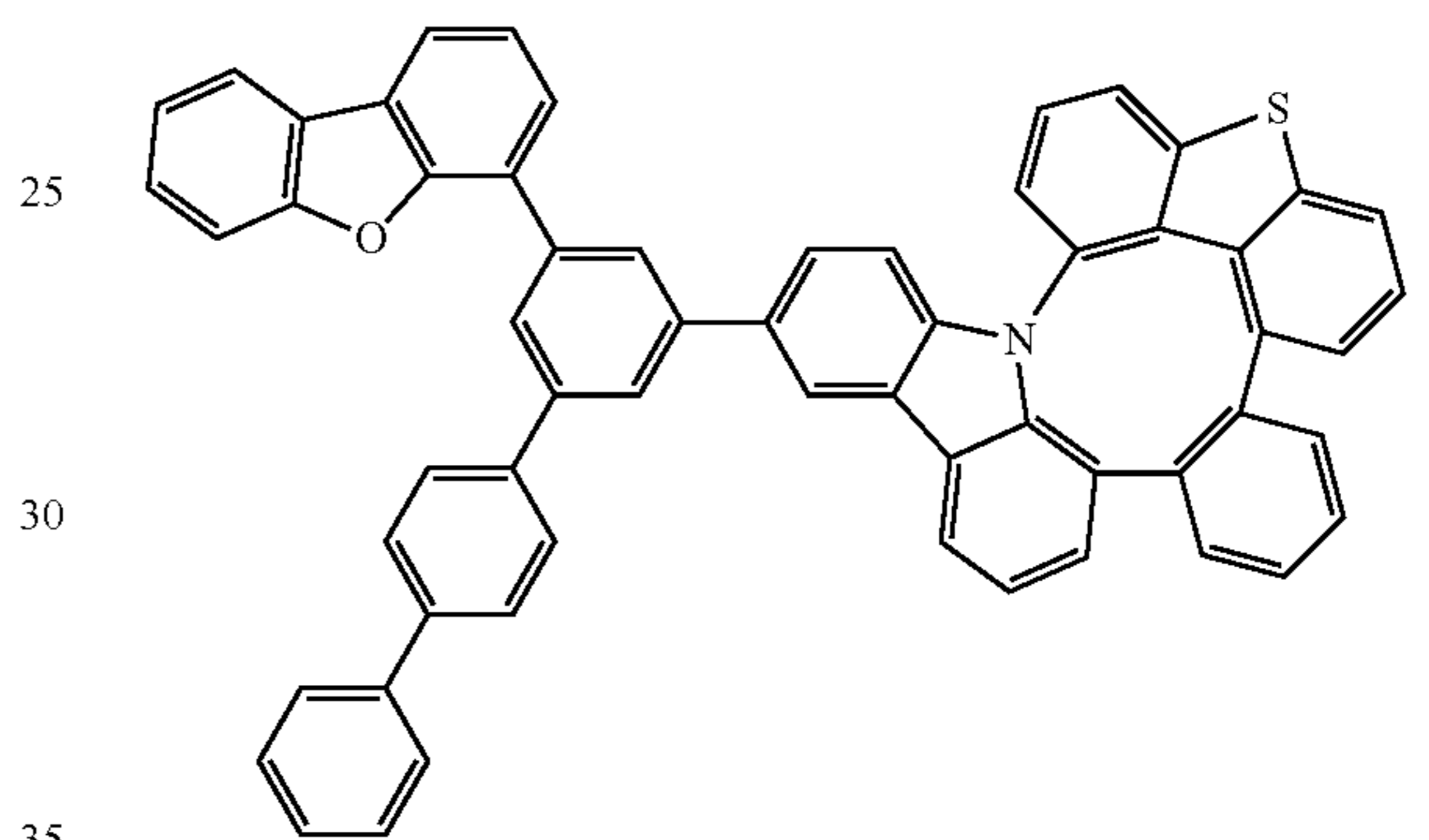
Compound 134
