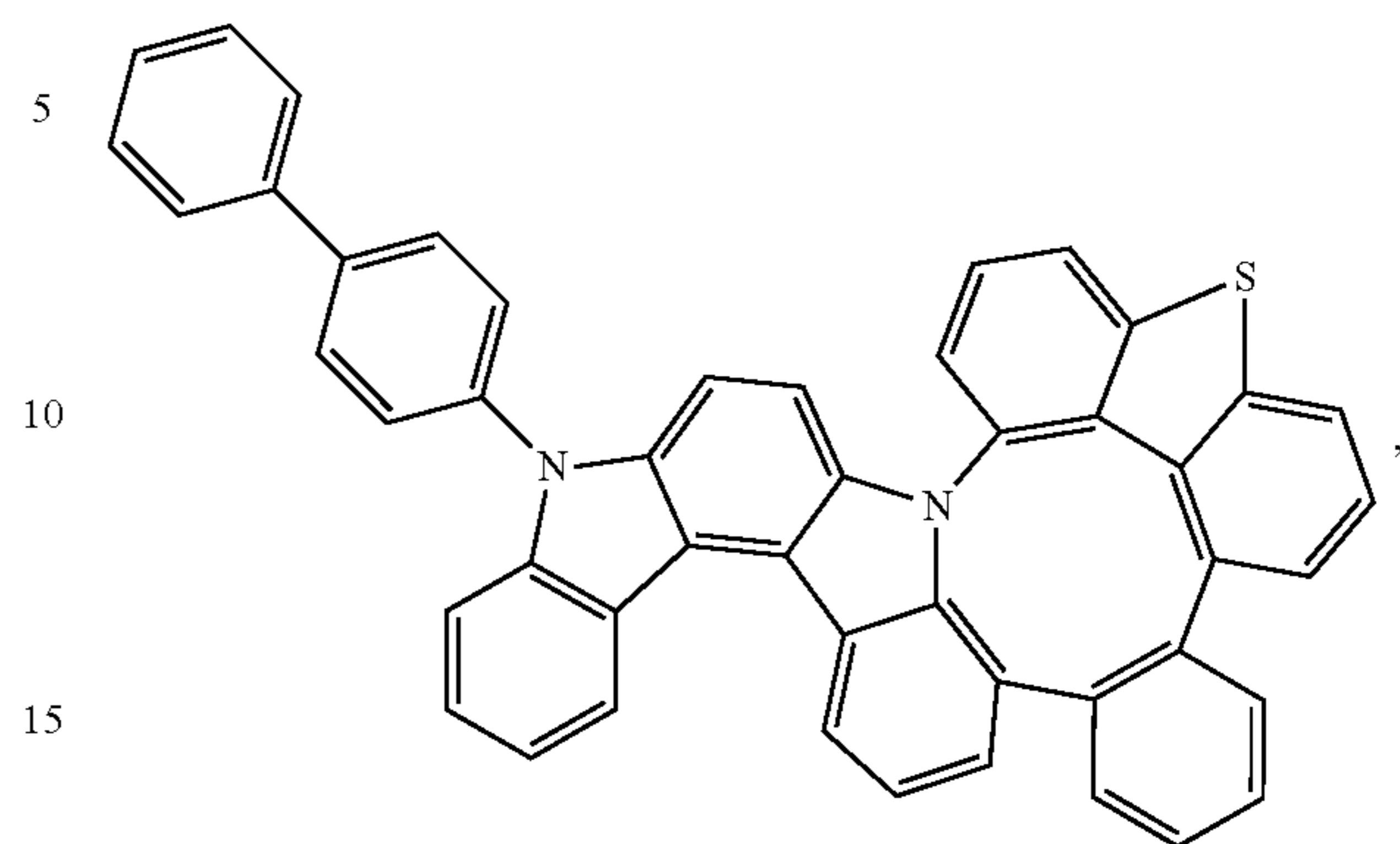
Compound 143
