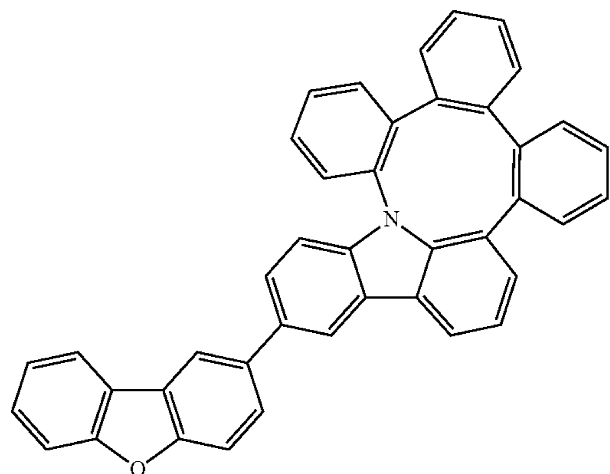
Compound 6
