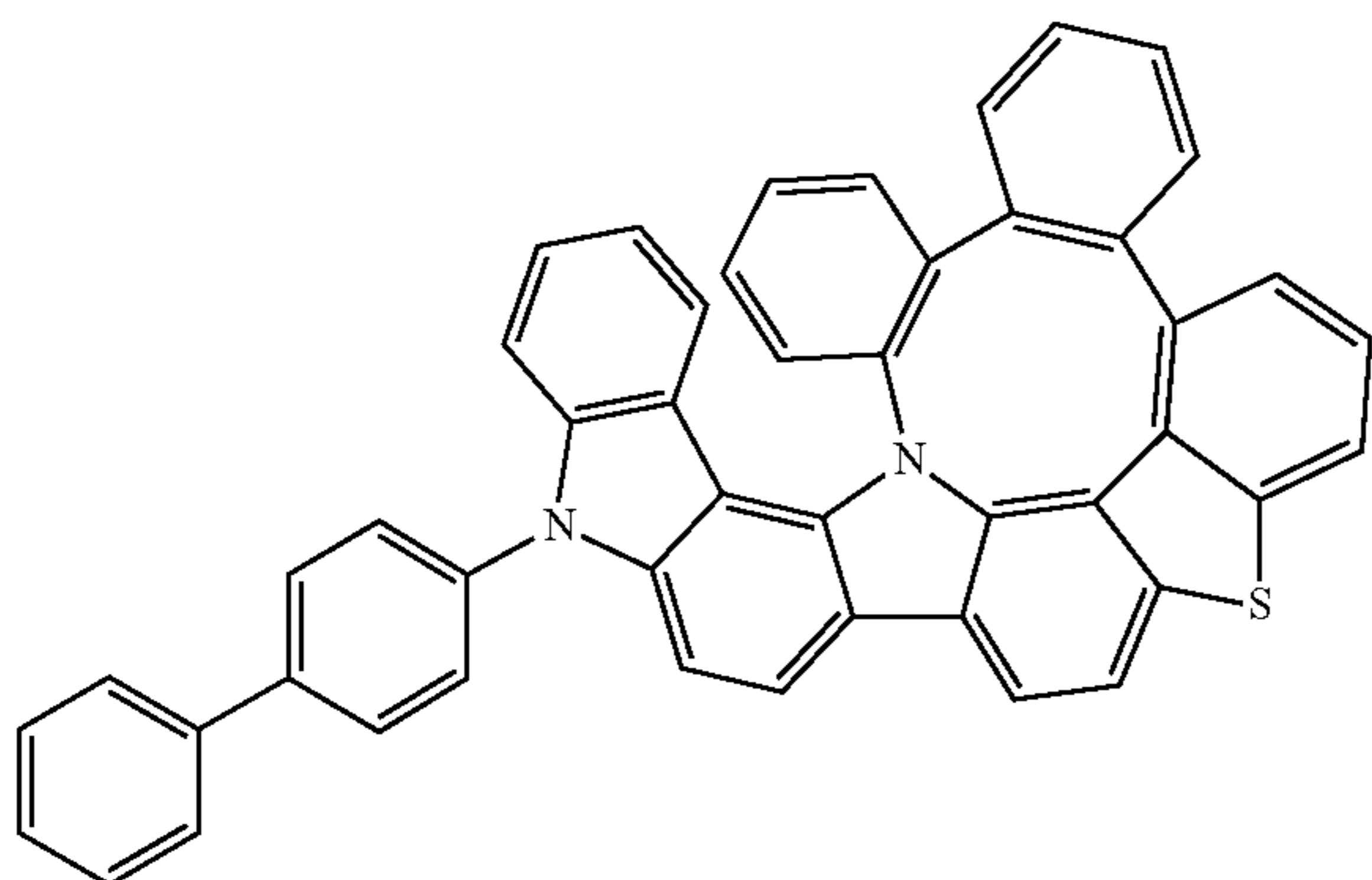
Compound 315
