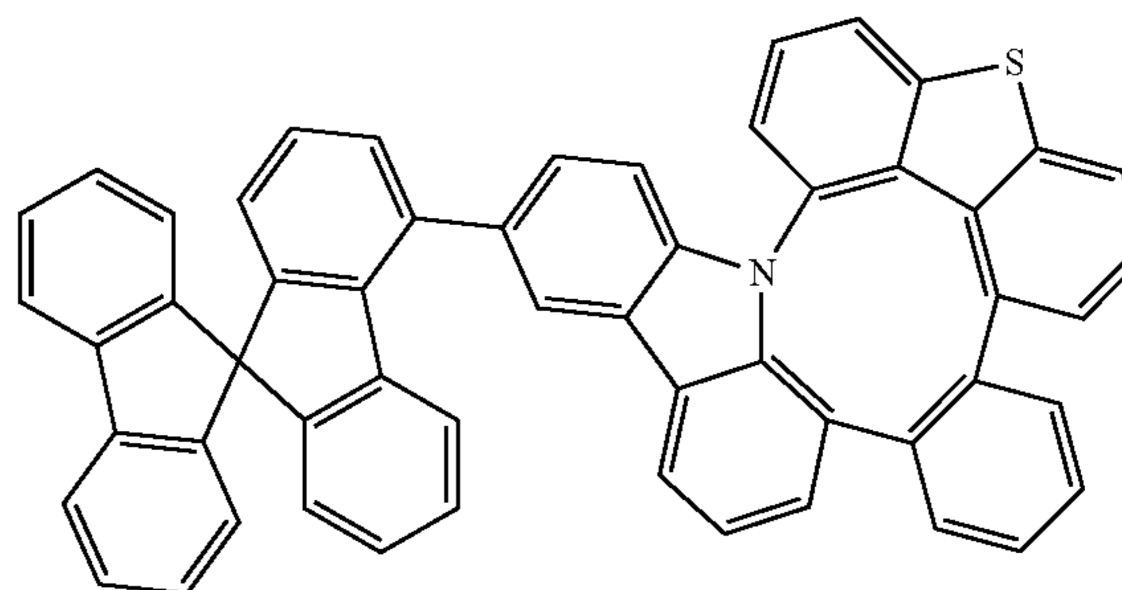
Compound 109
