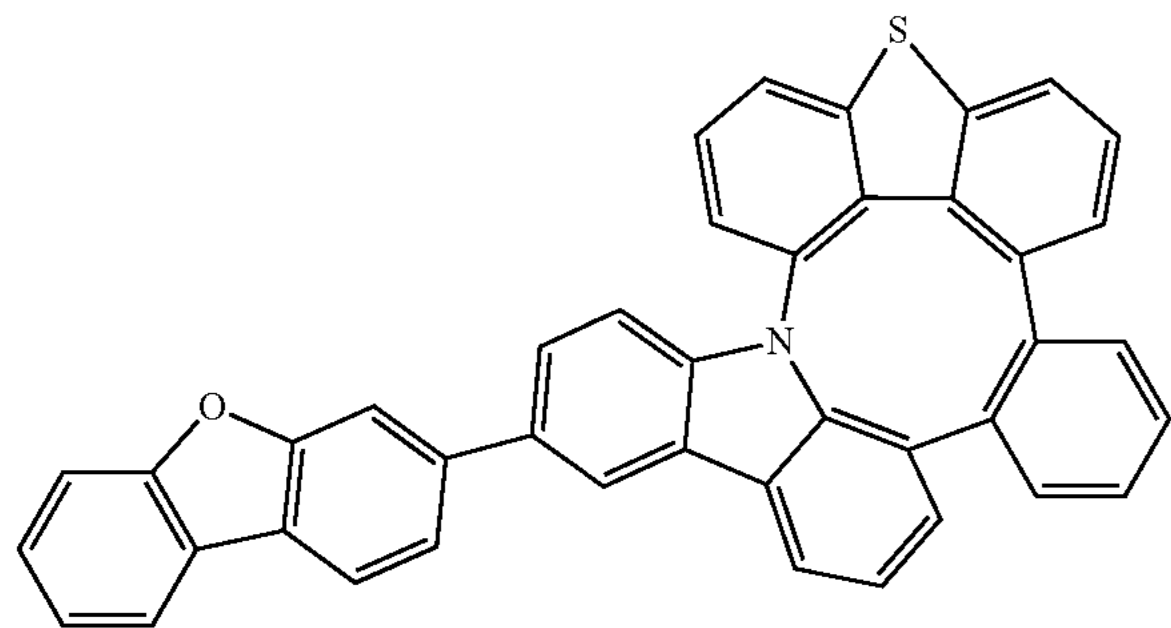
Compound 92
