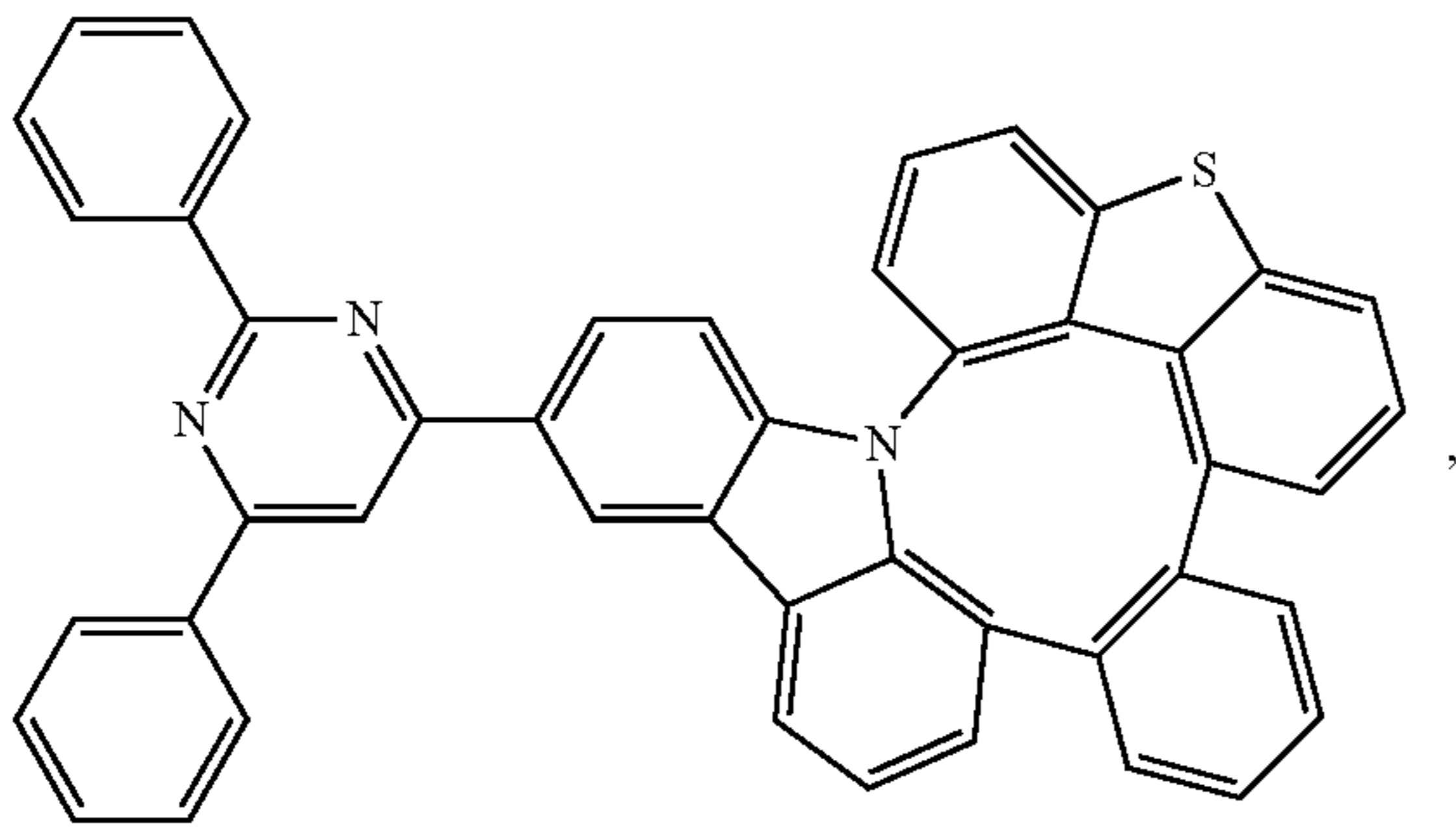
Compound 112
