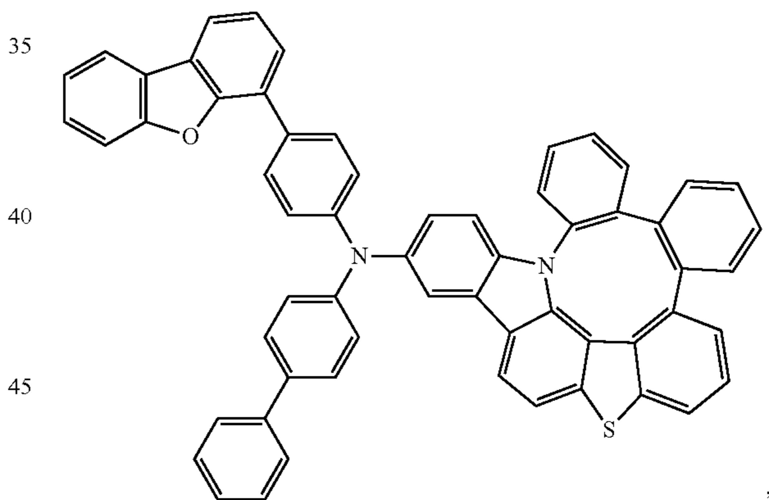
Compound 304
