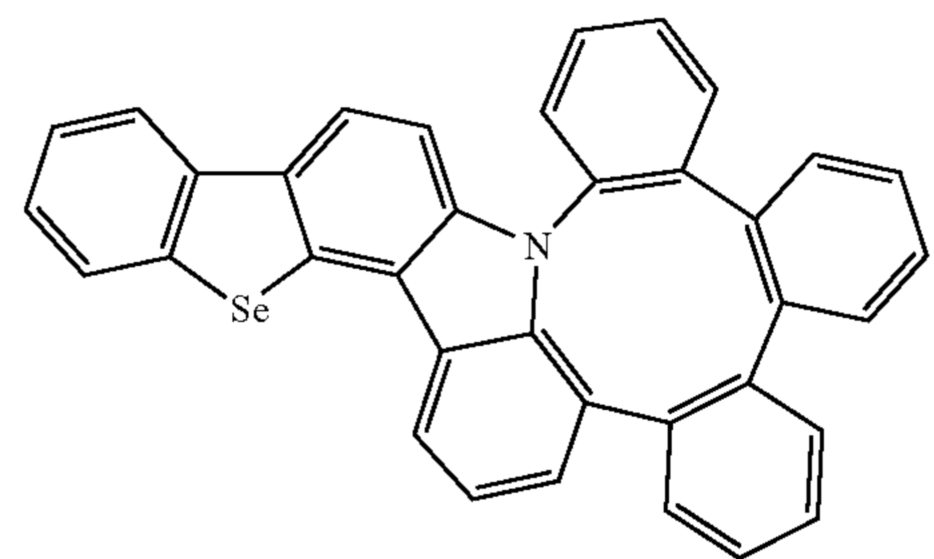
Compound 68
