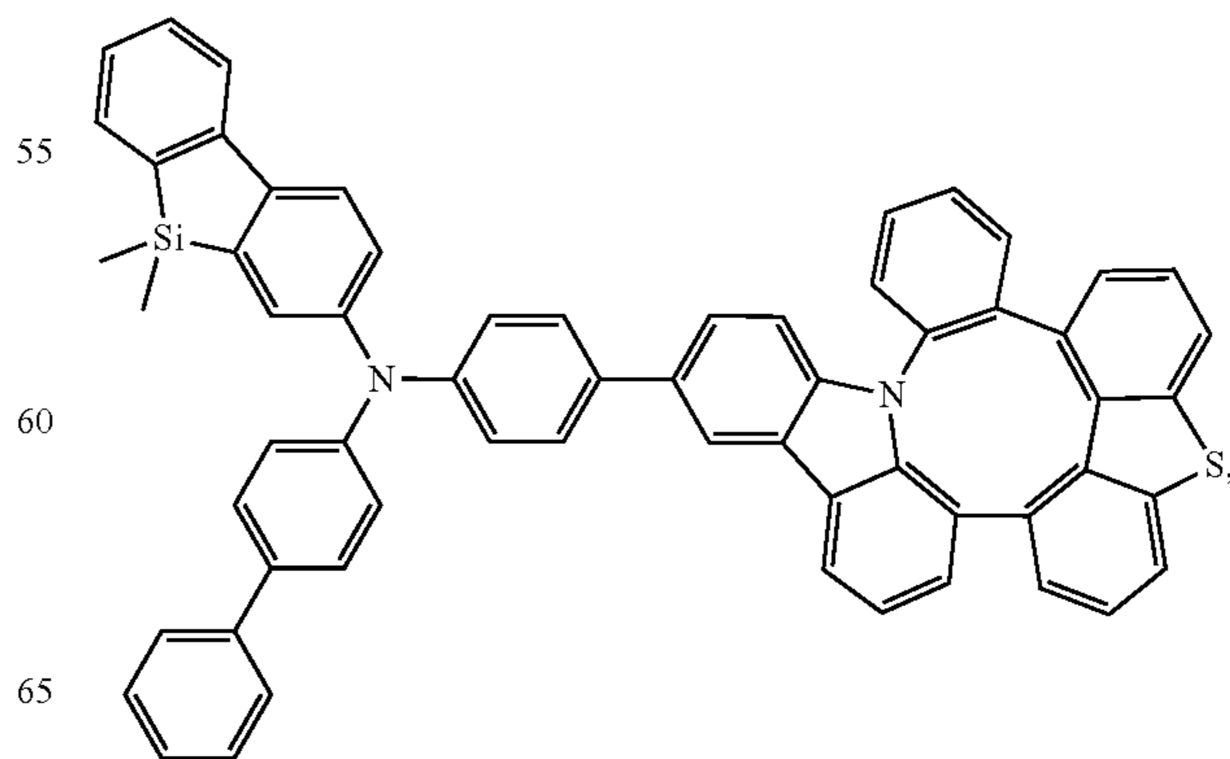
Compound 361
