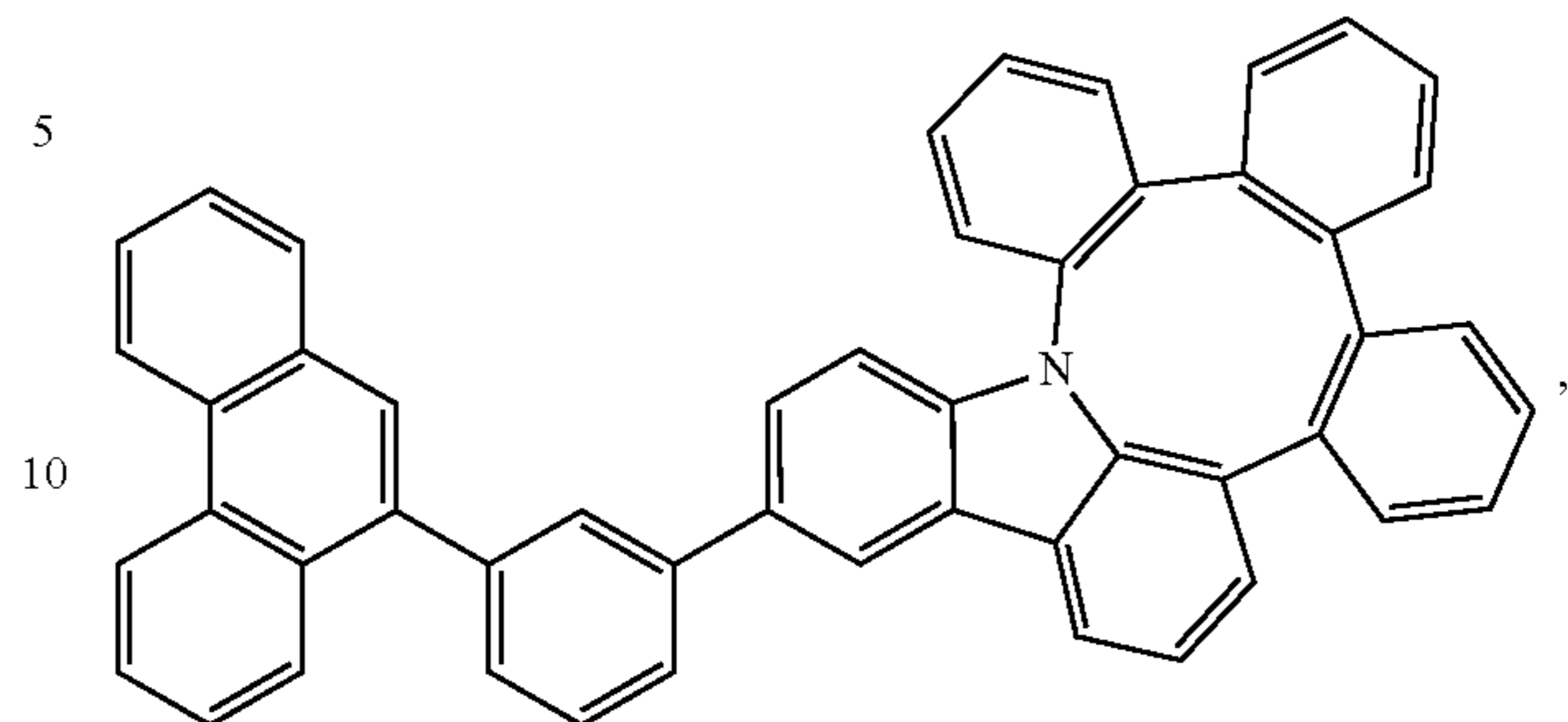
Compound 35
