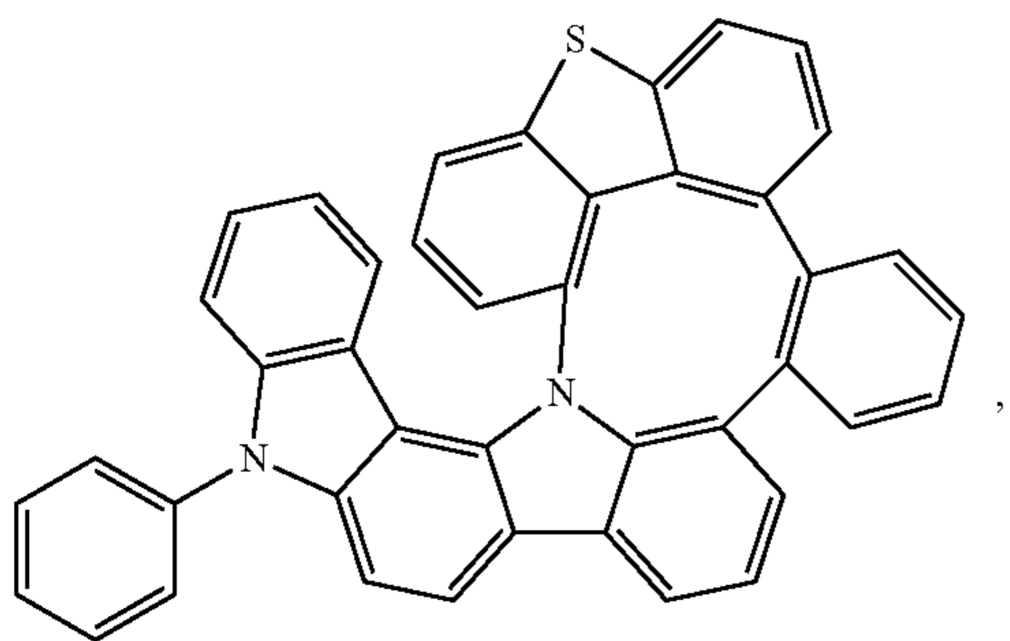
Compound 139
