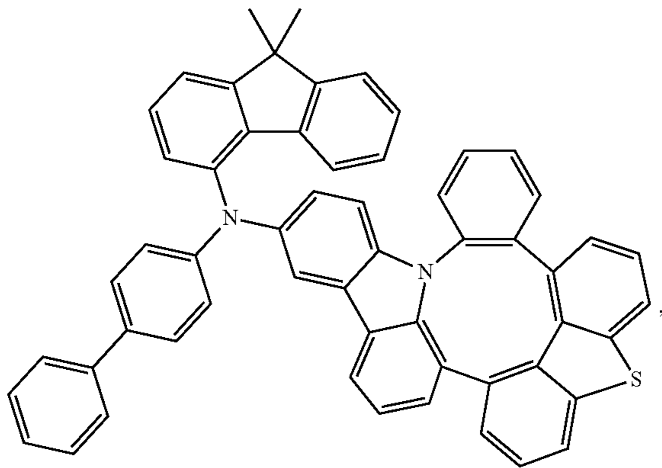
Compound 214
