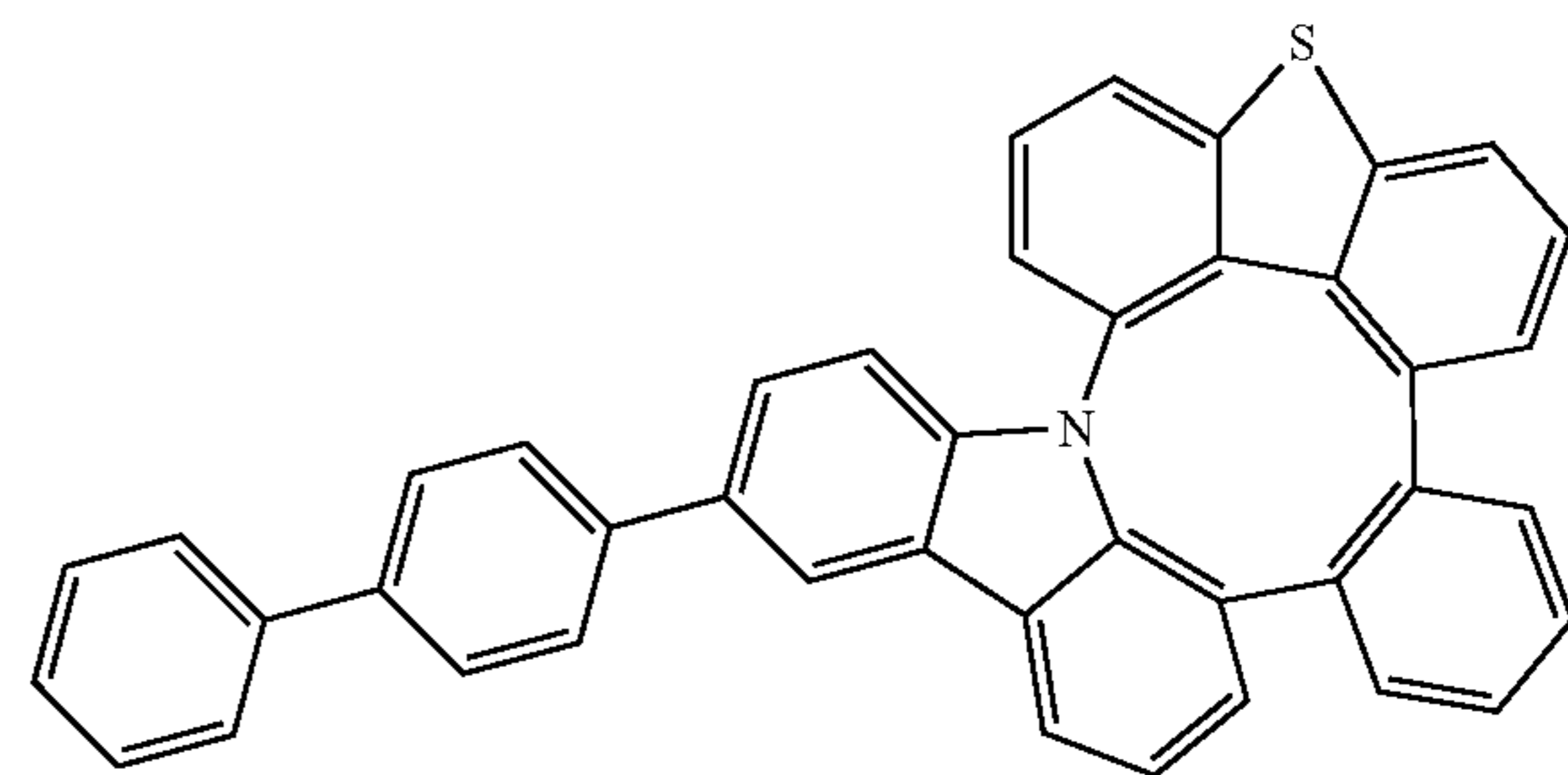
Compound 87
