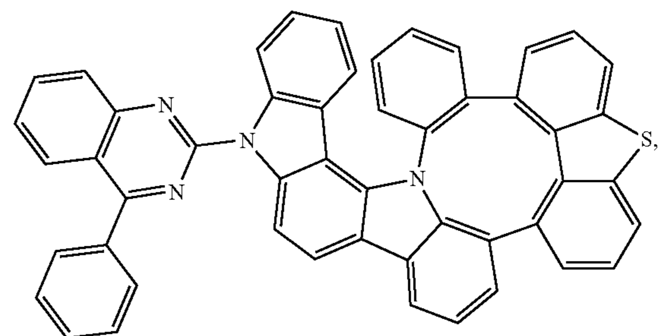
Compound 254
