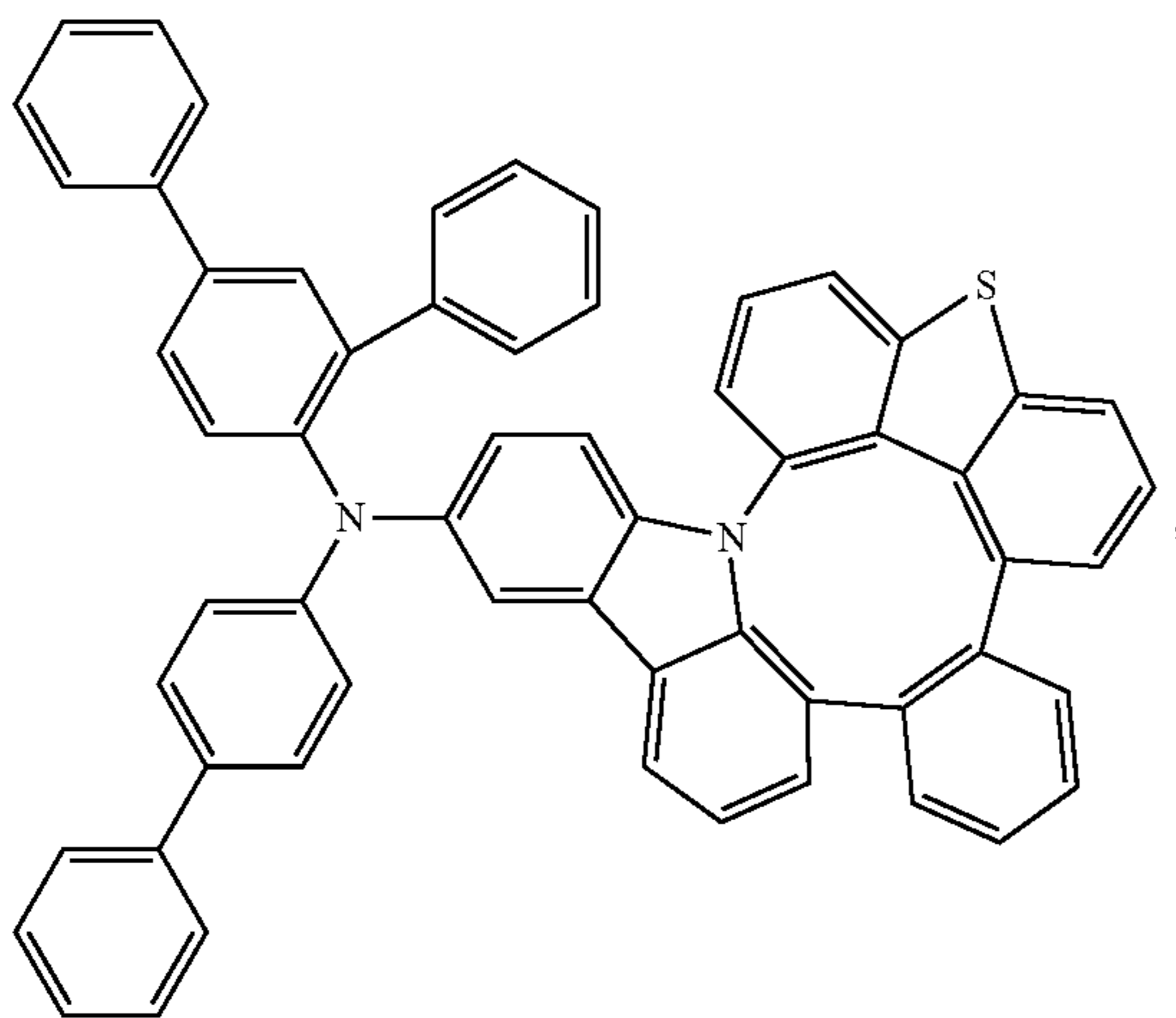
Compound 131
