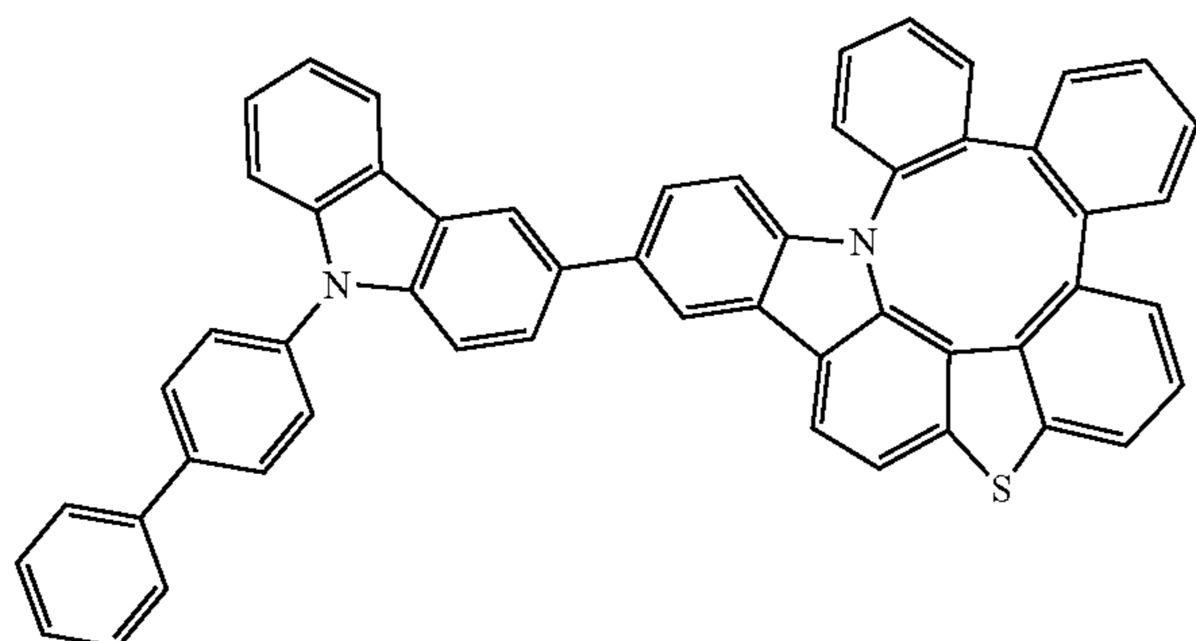
Compound 274
