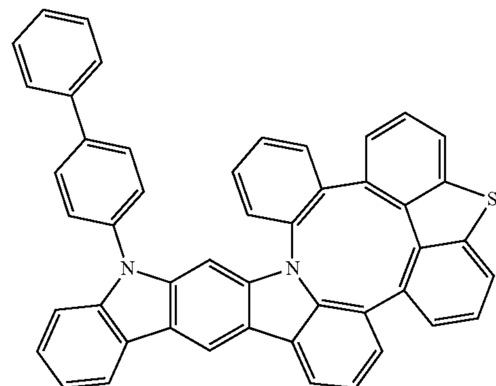
Compound 228
