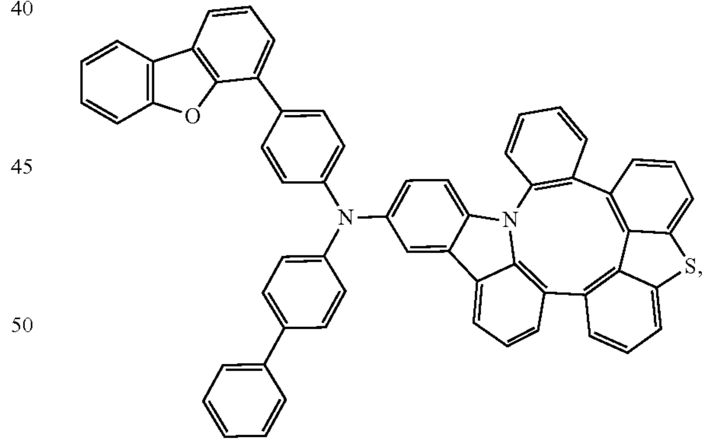
Compound 220
