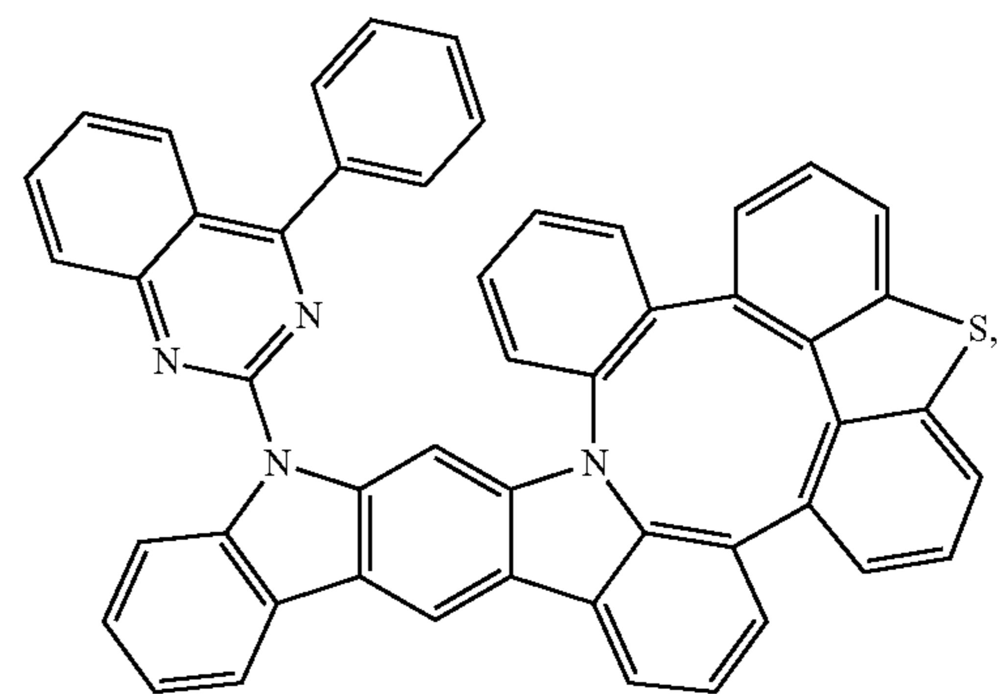
Compound 253
