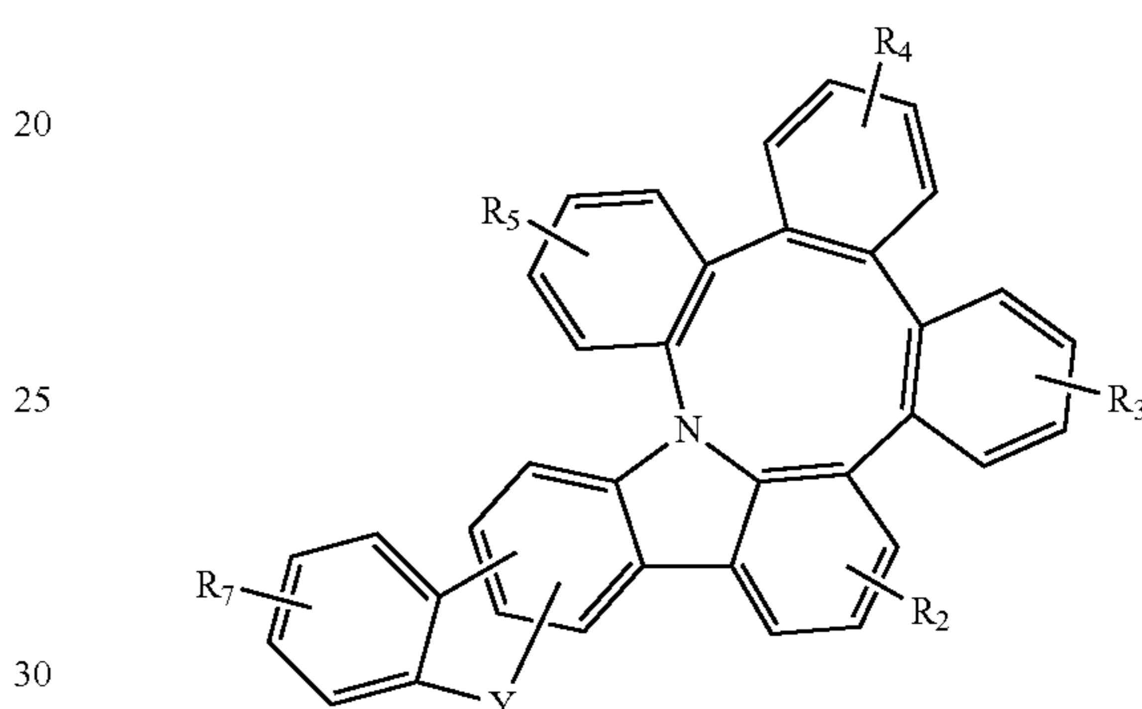
Formula 5
