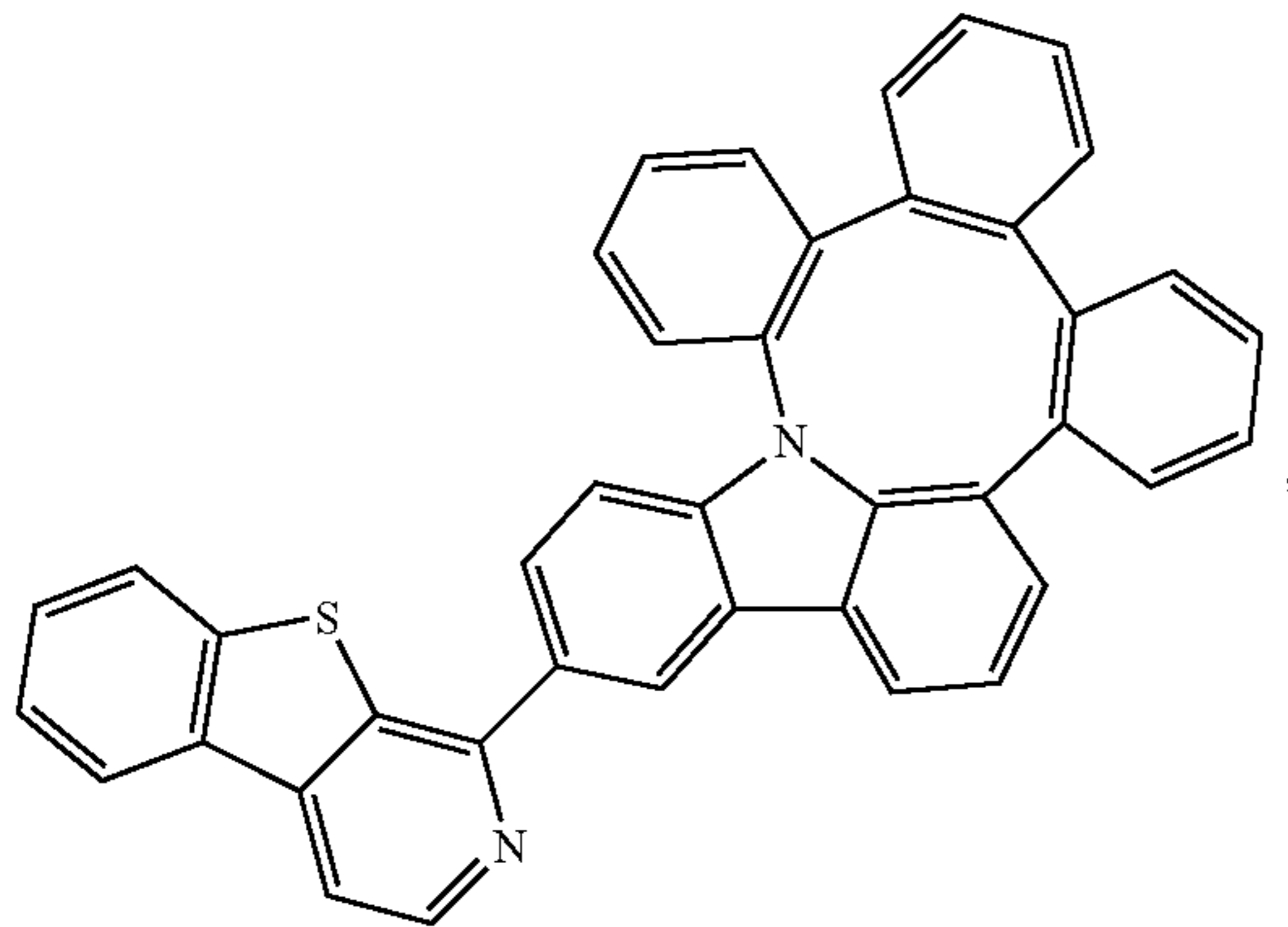
Compound 32
