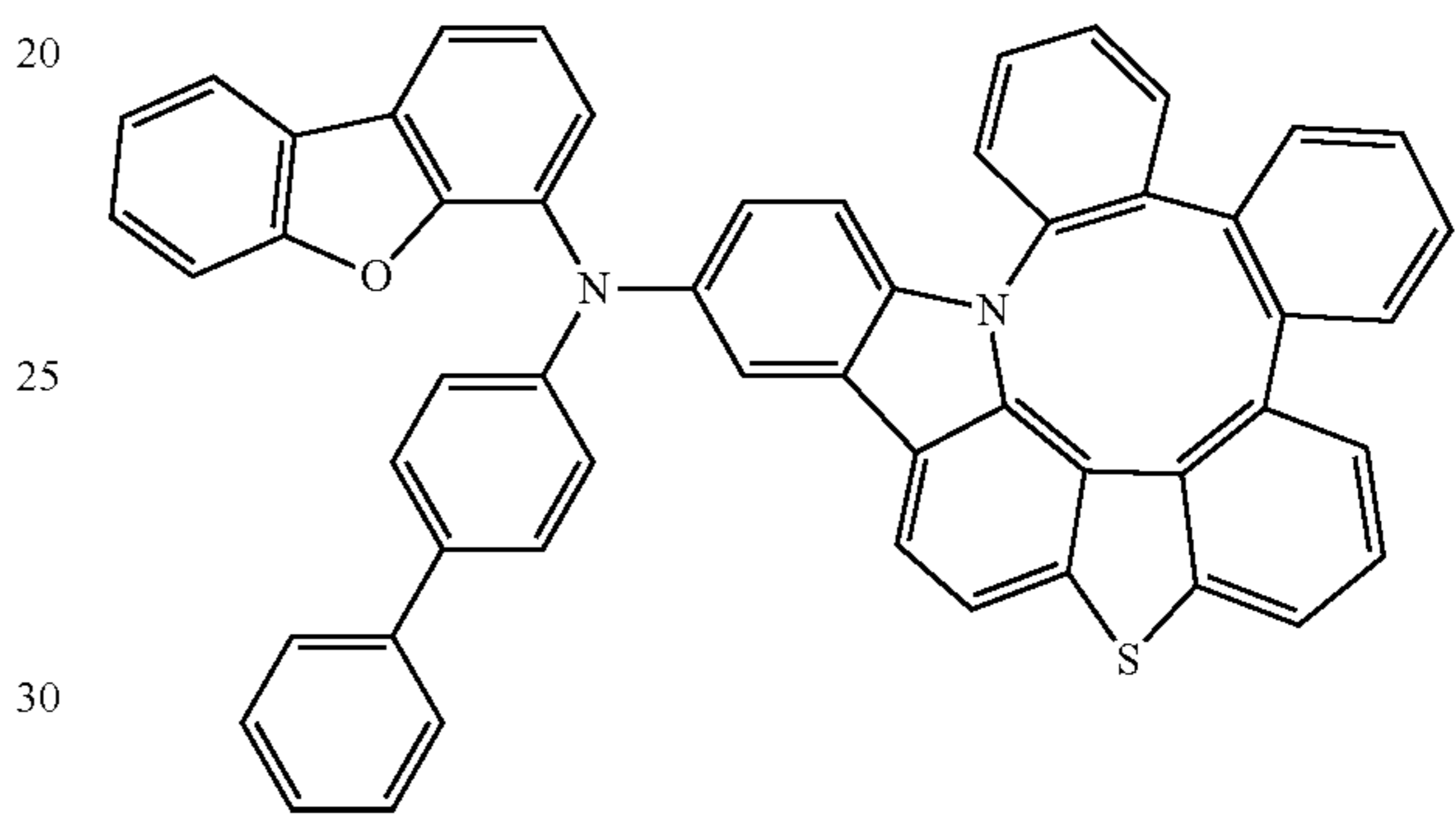
Compound 304
