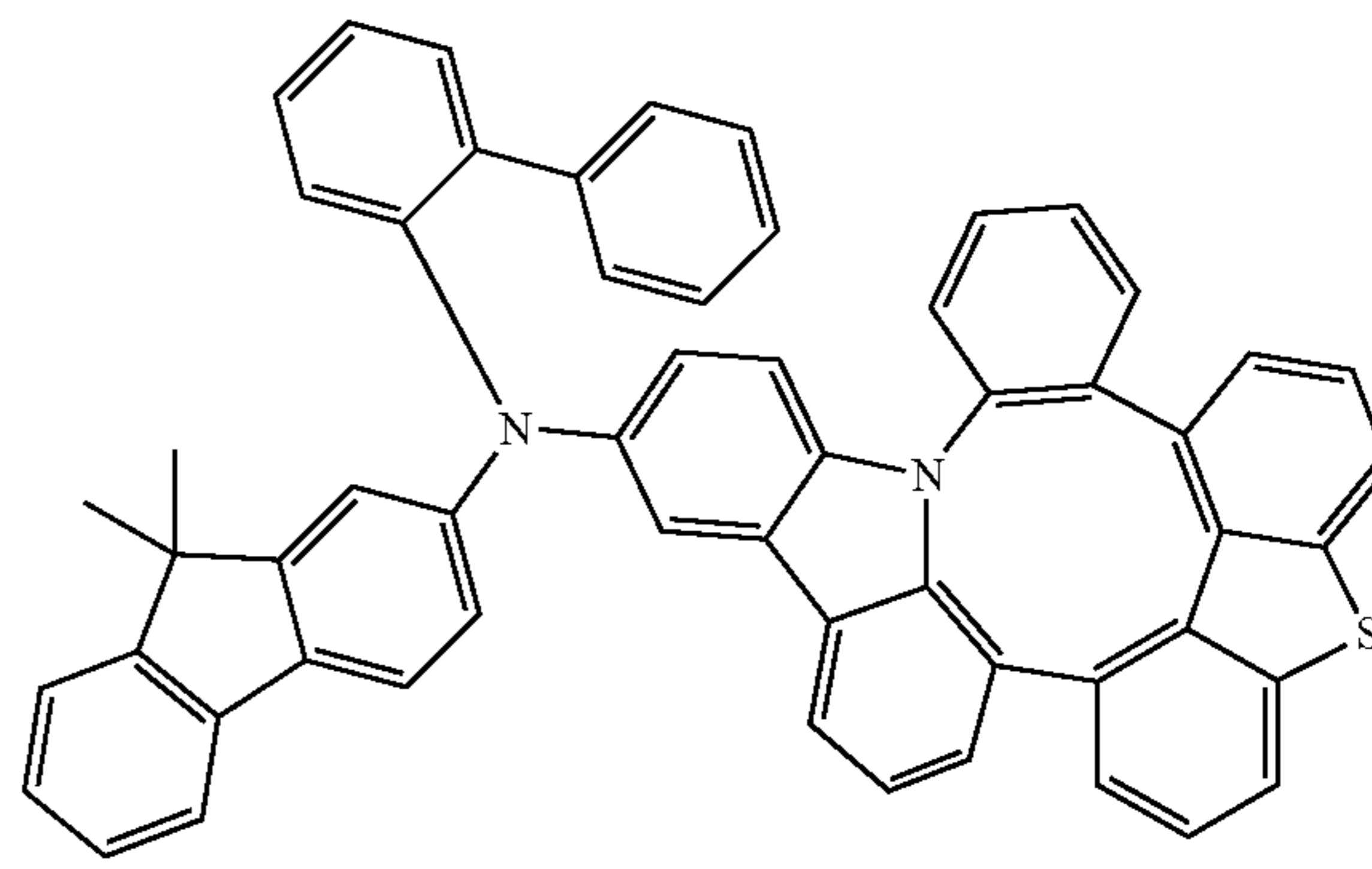
Compound 213
