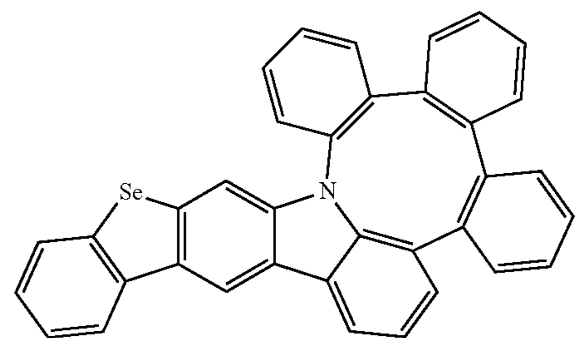
Compound 71
