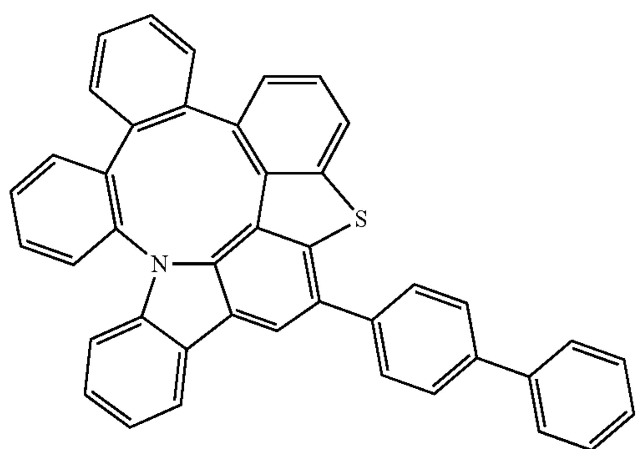
Compound 258
