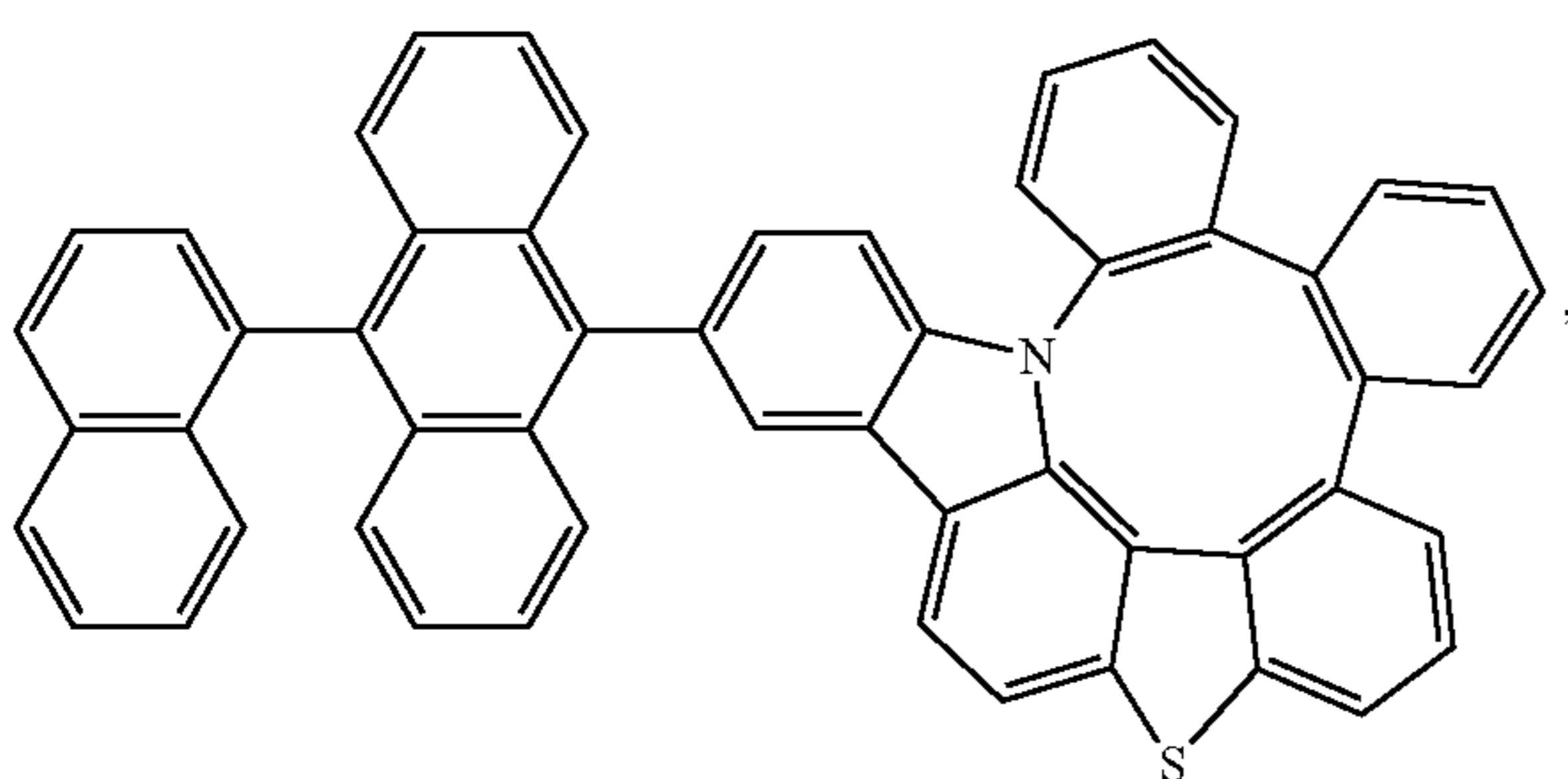
Compound 292
