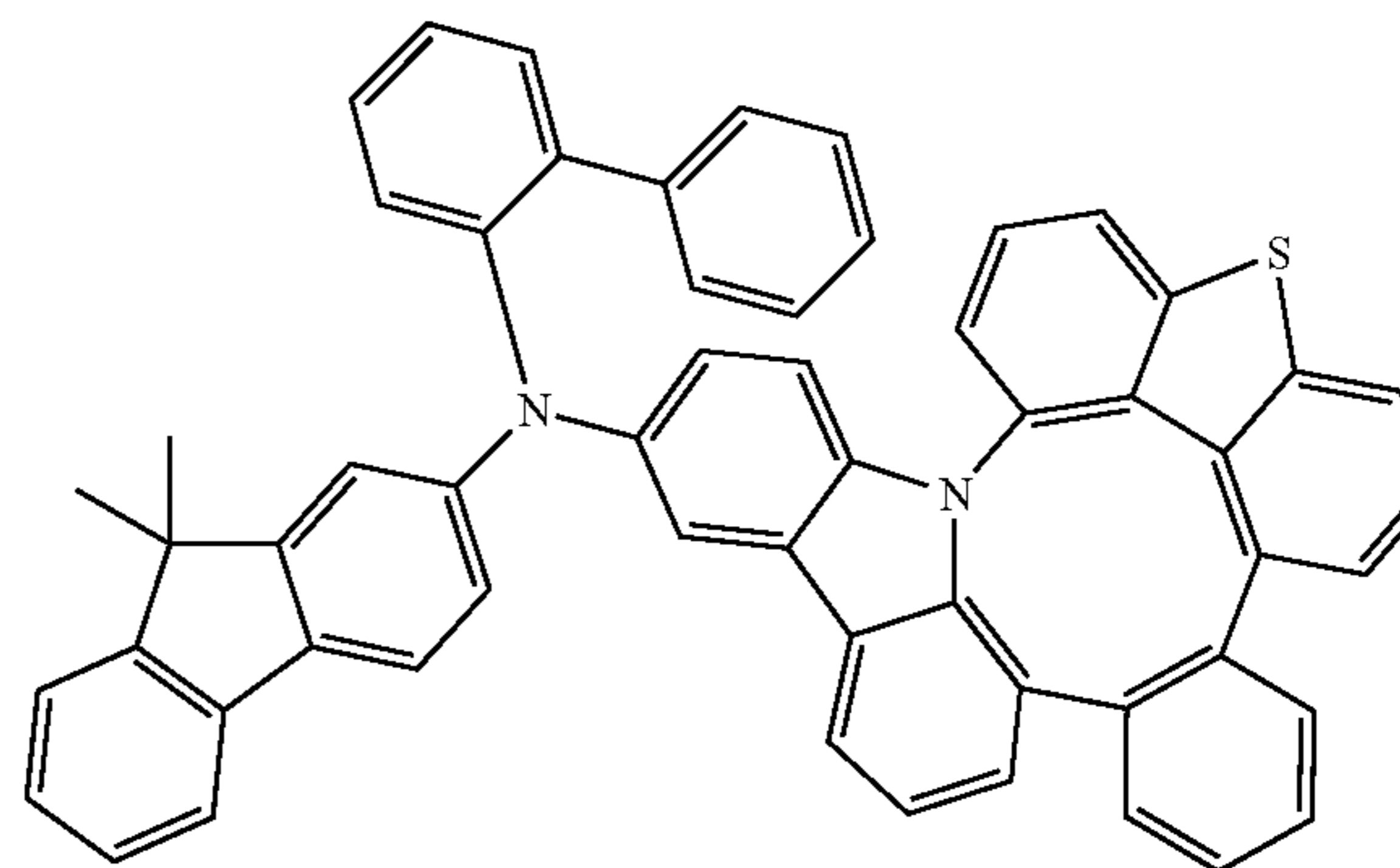
Compound 128
