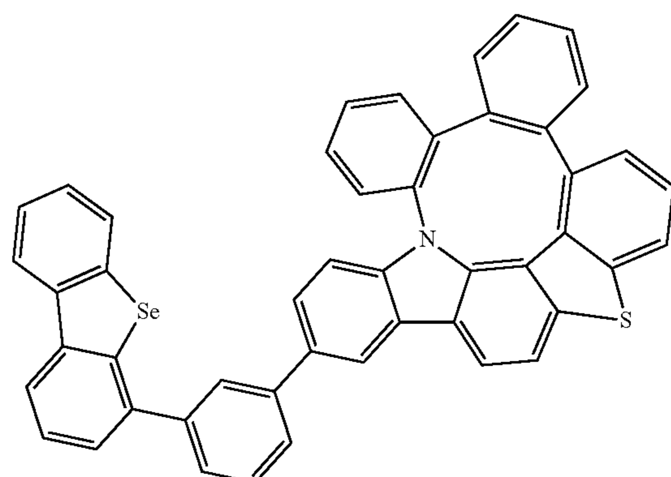
Compound 270
