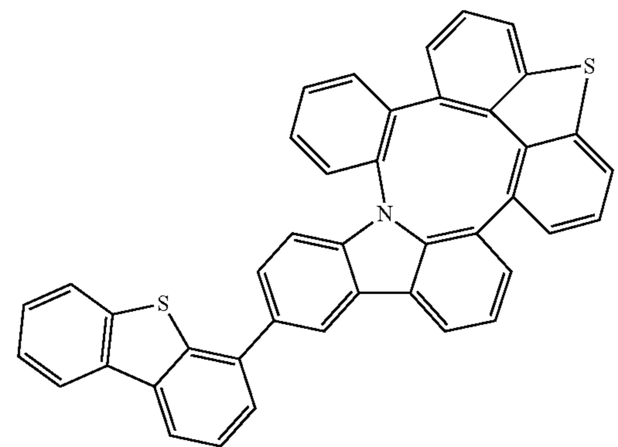
Compound 178
