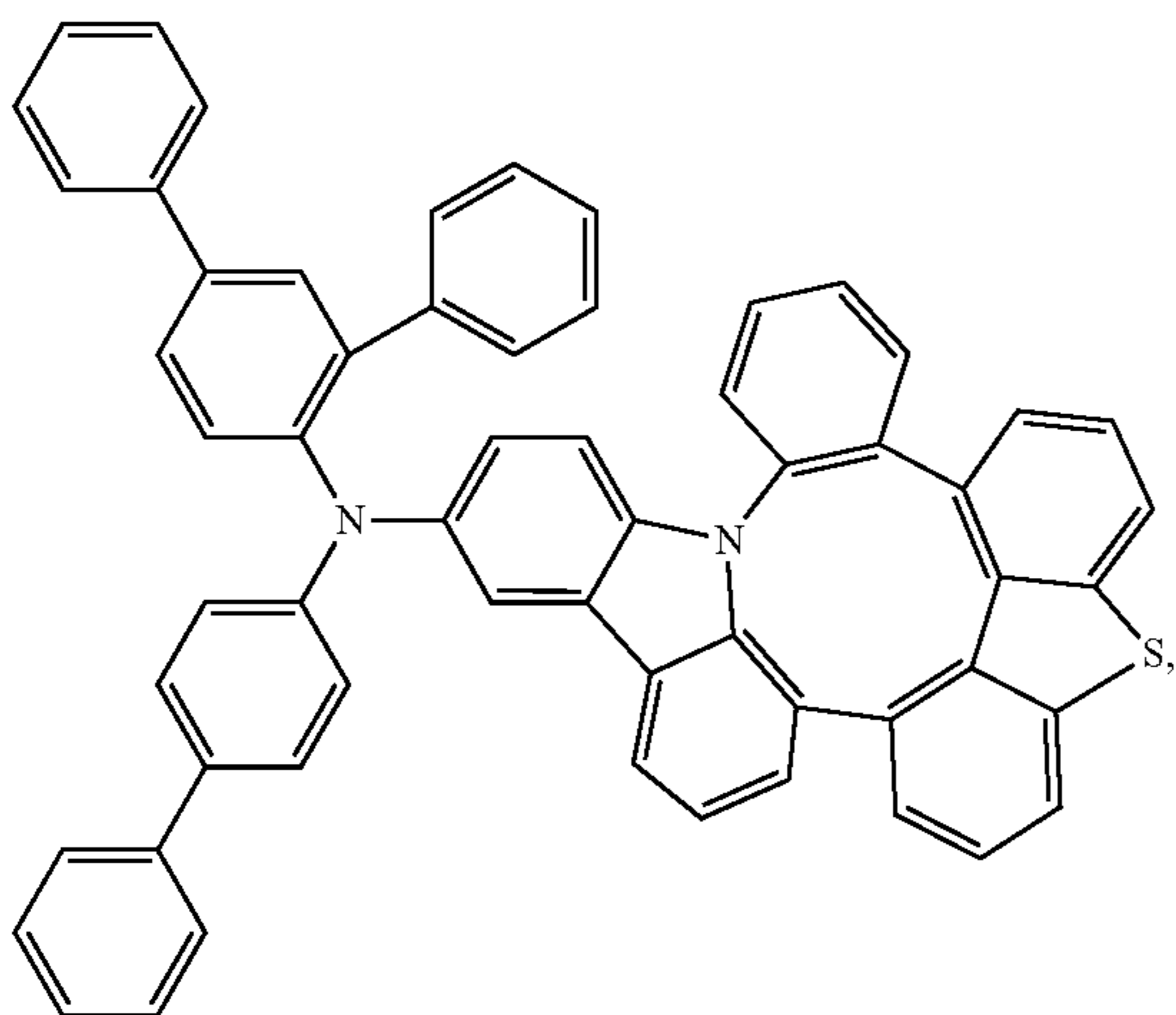
Compound 215
