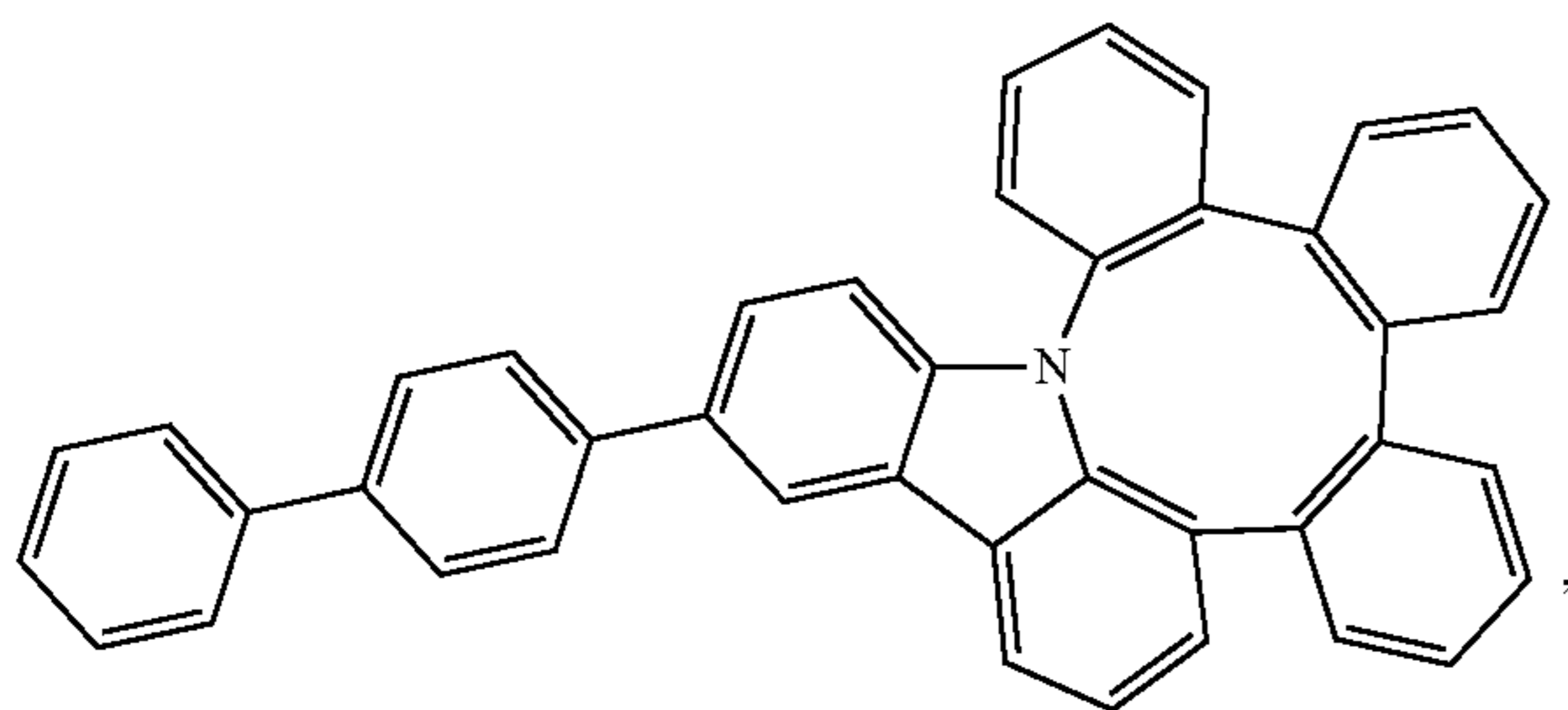
Compound 2
