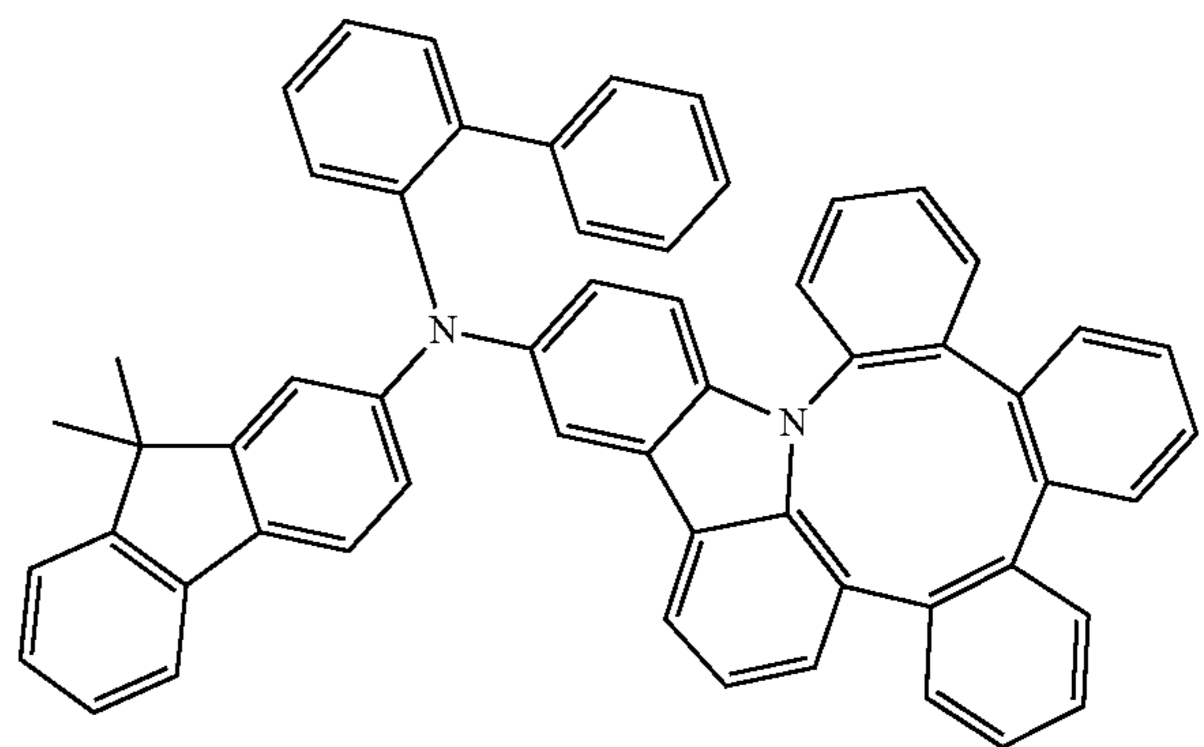
Compound 43
