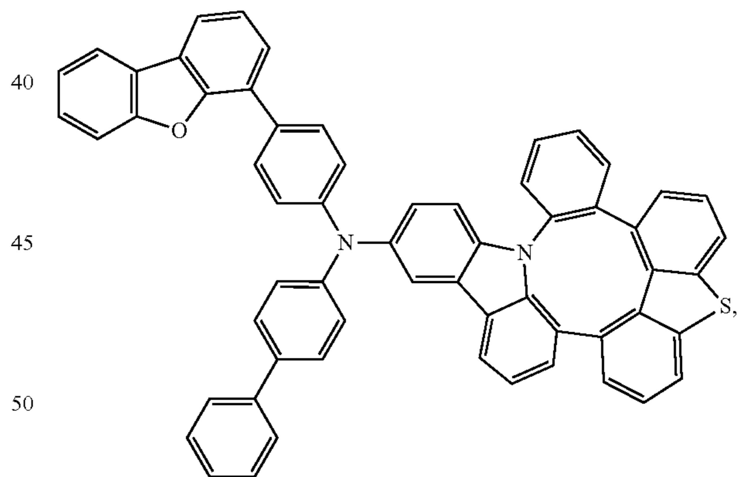
Compound 220
