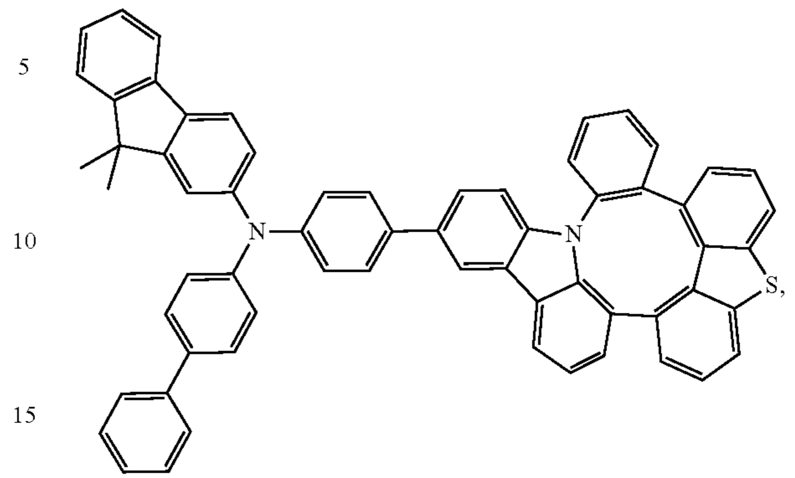
Compound 217
