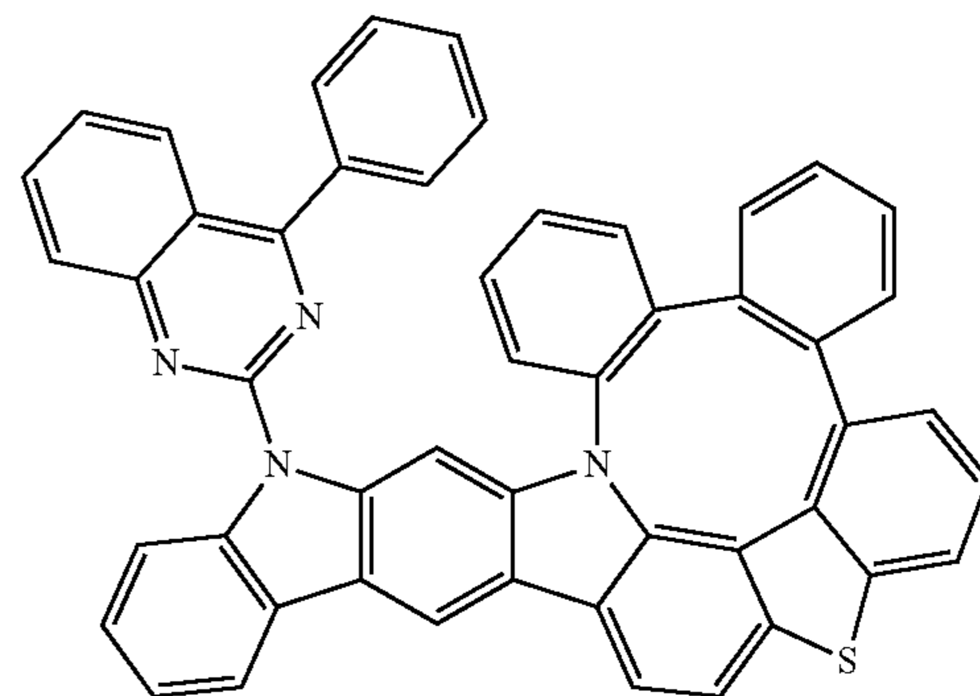
Compound 337
