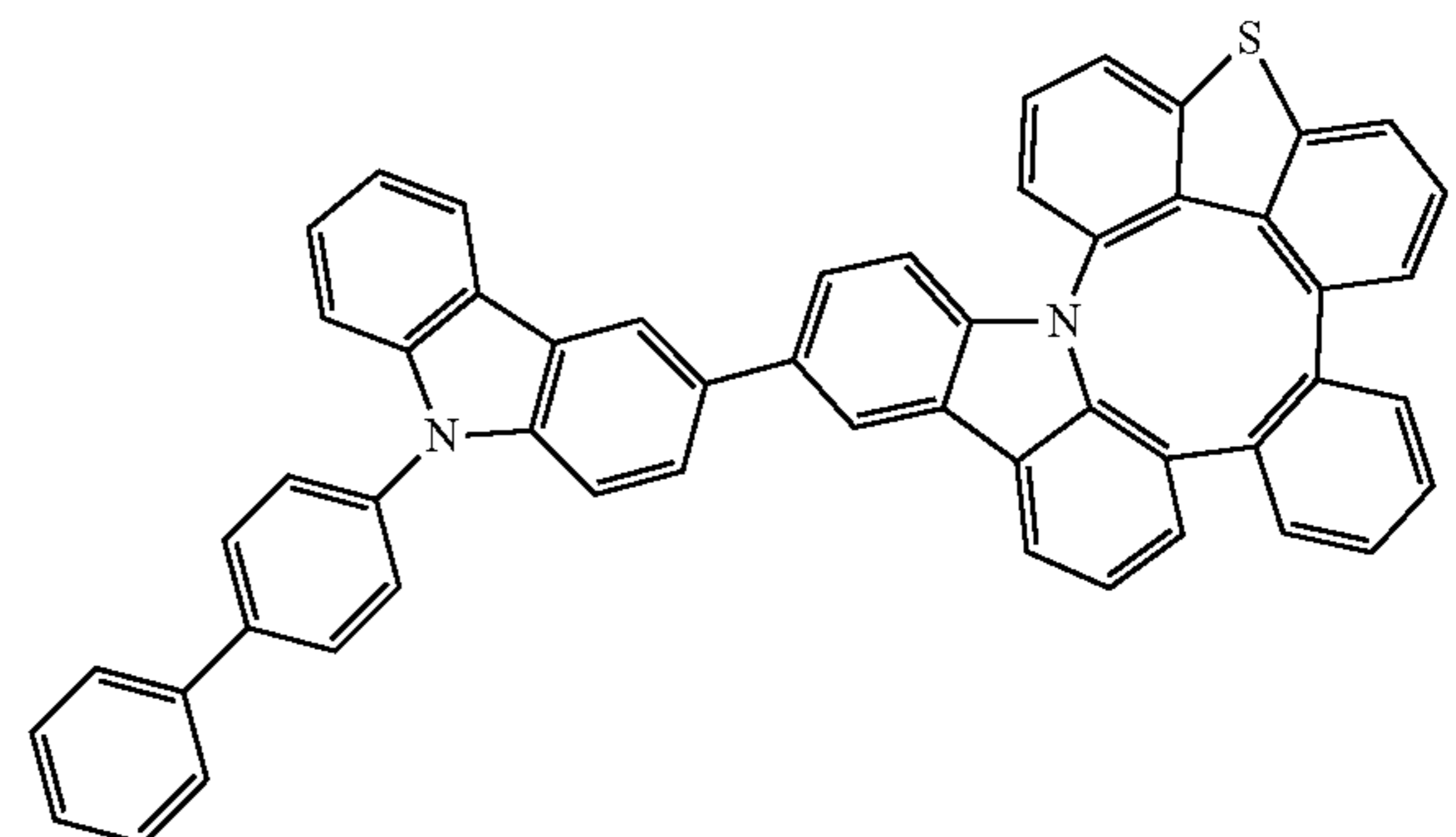
Compound 103
