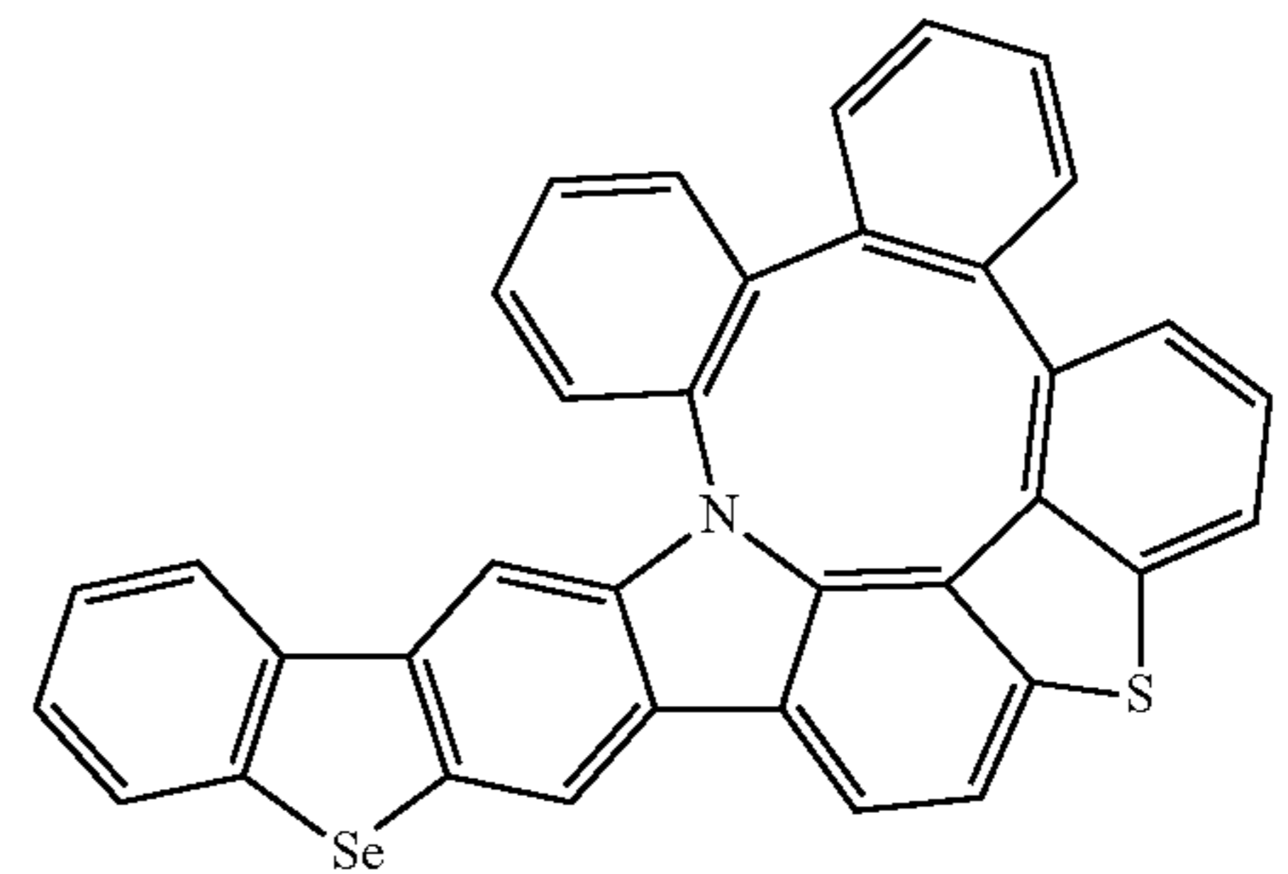
Compound 327
