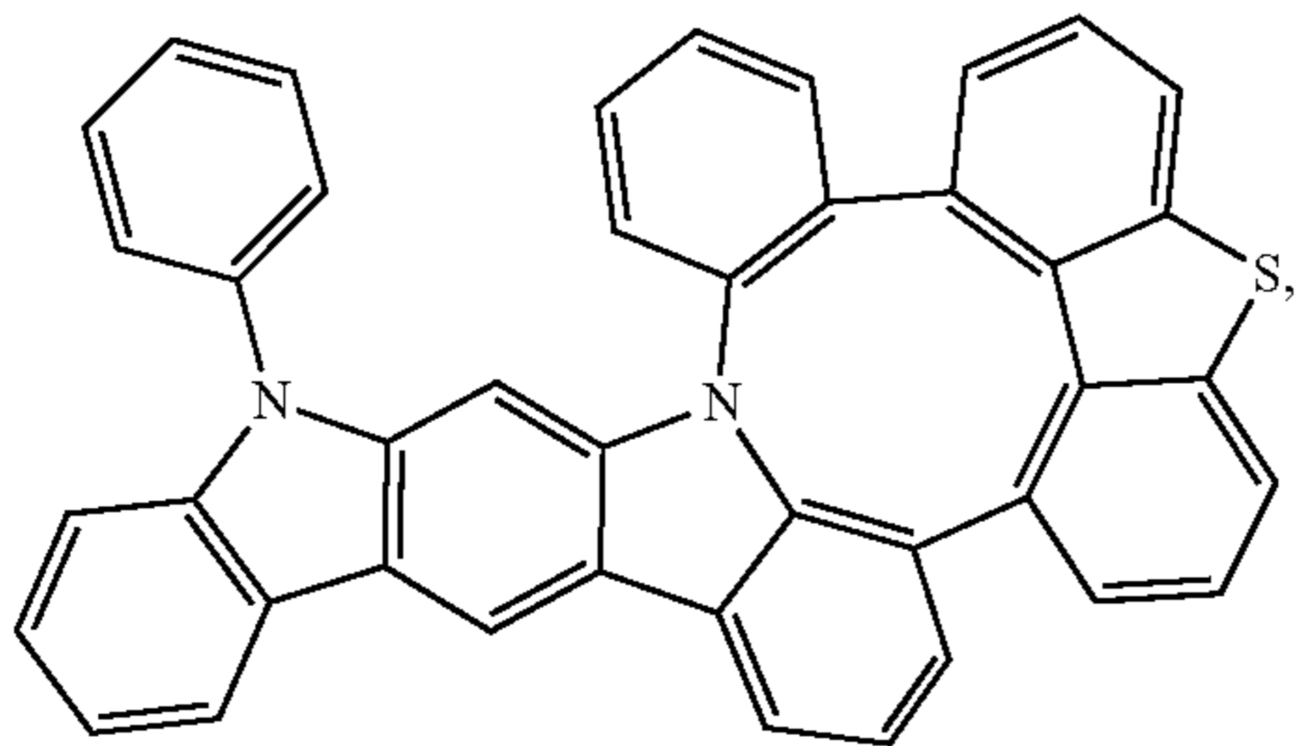
Compound 222
