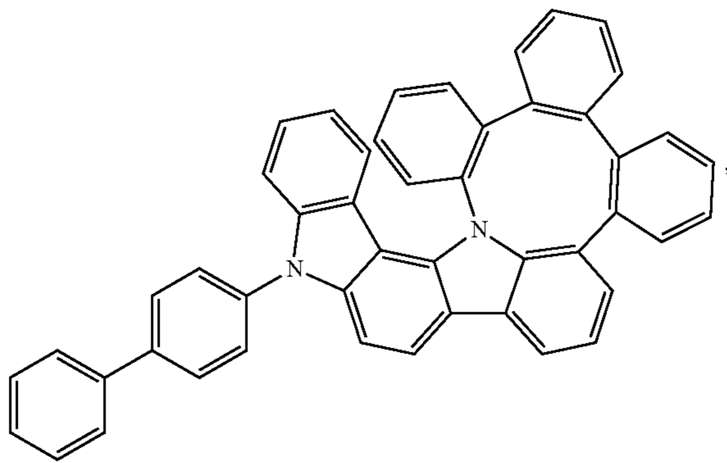
Compound 61
