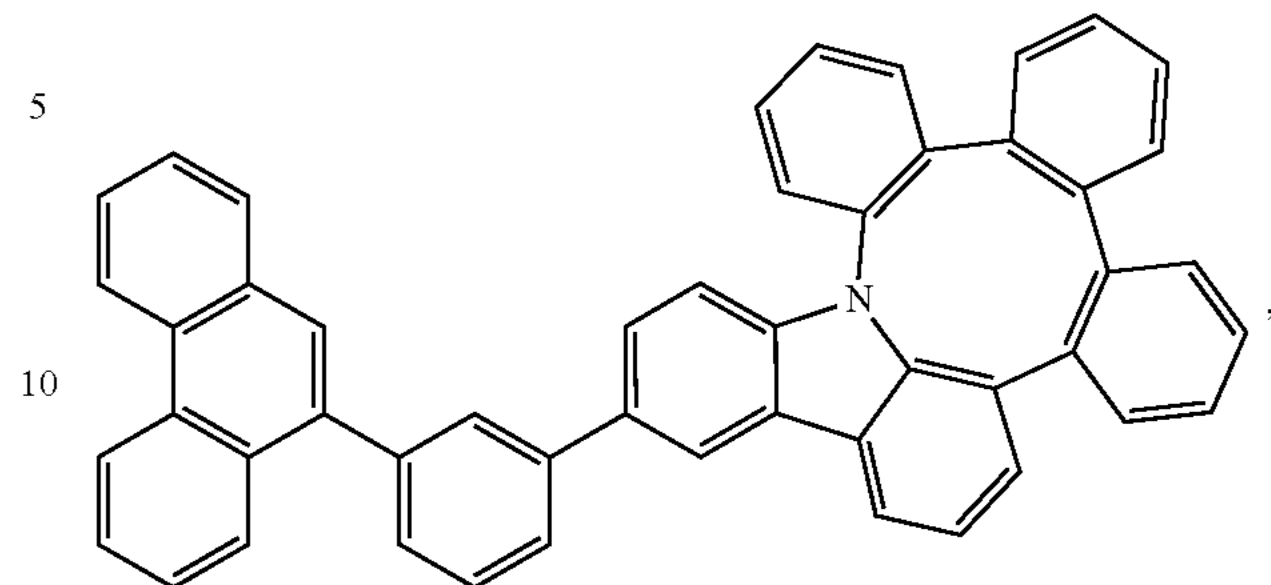
Compound 35
