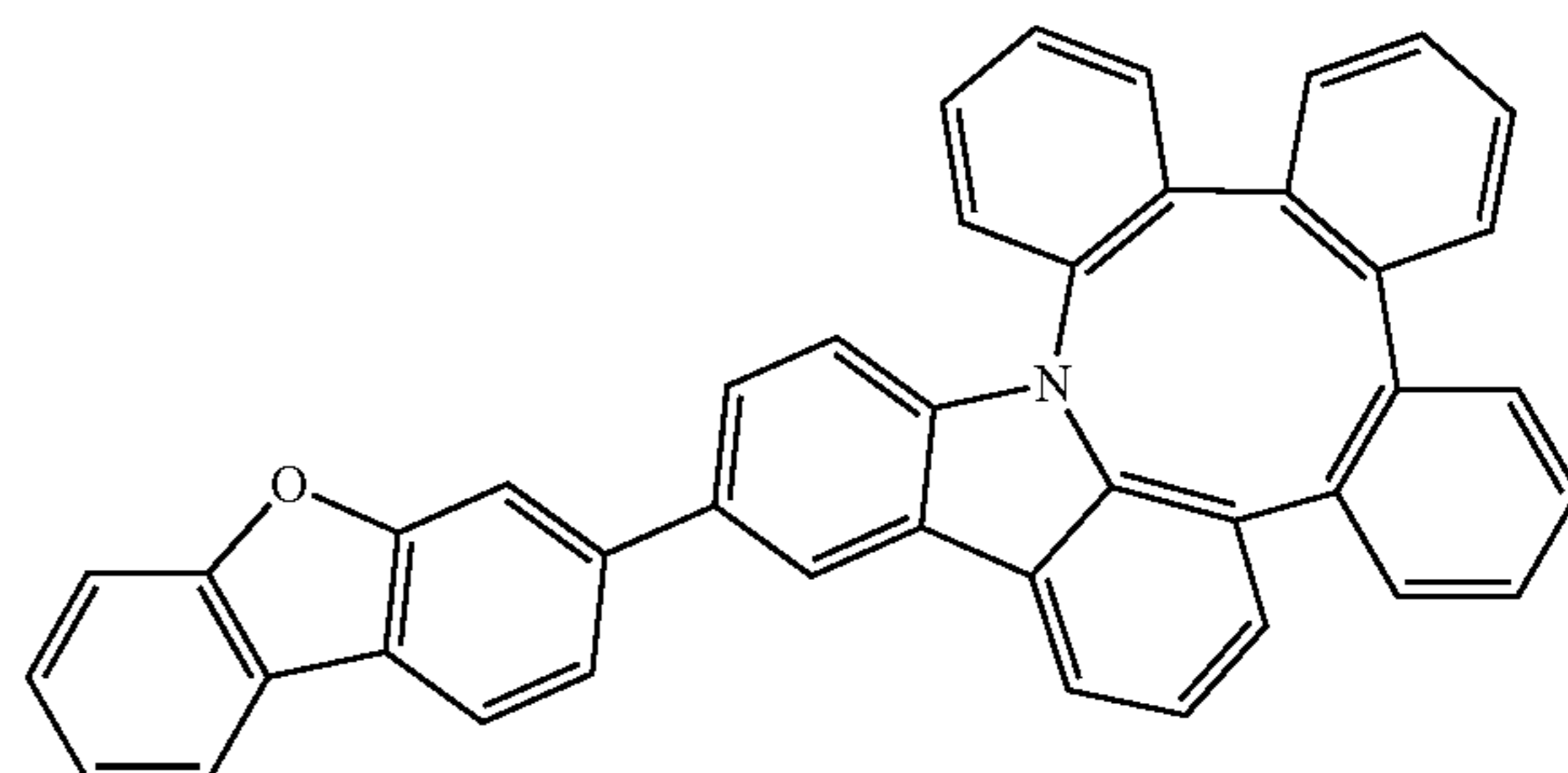
Compound 7
