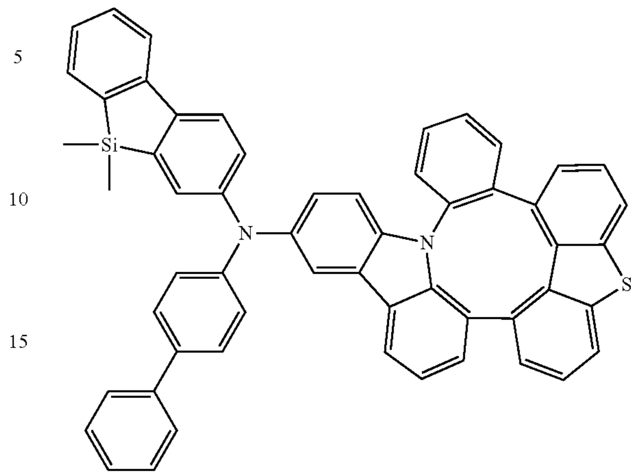
Compound 359
