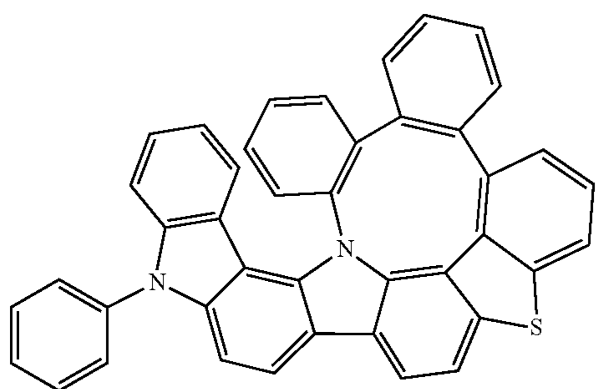
Compound 309
