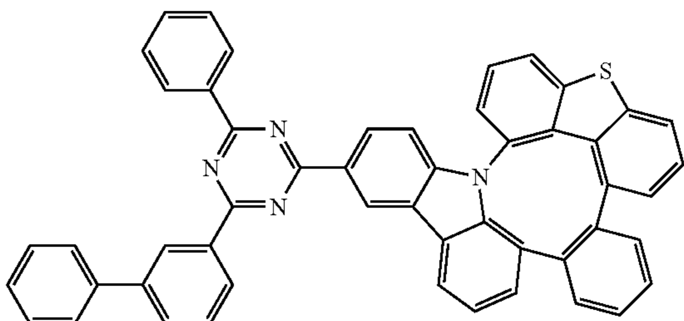
Compound 111
