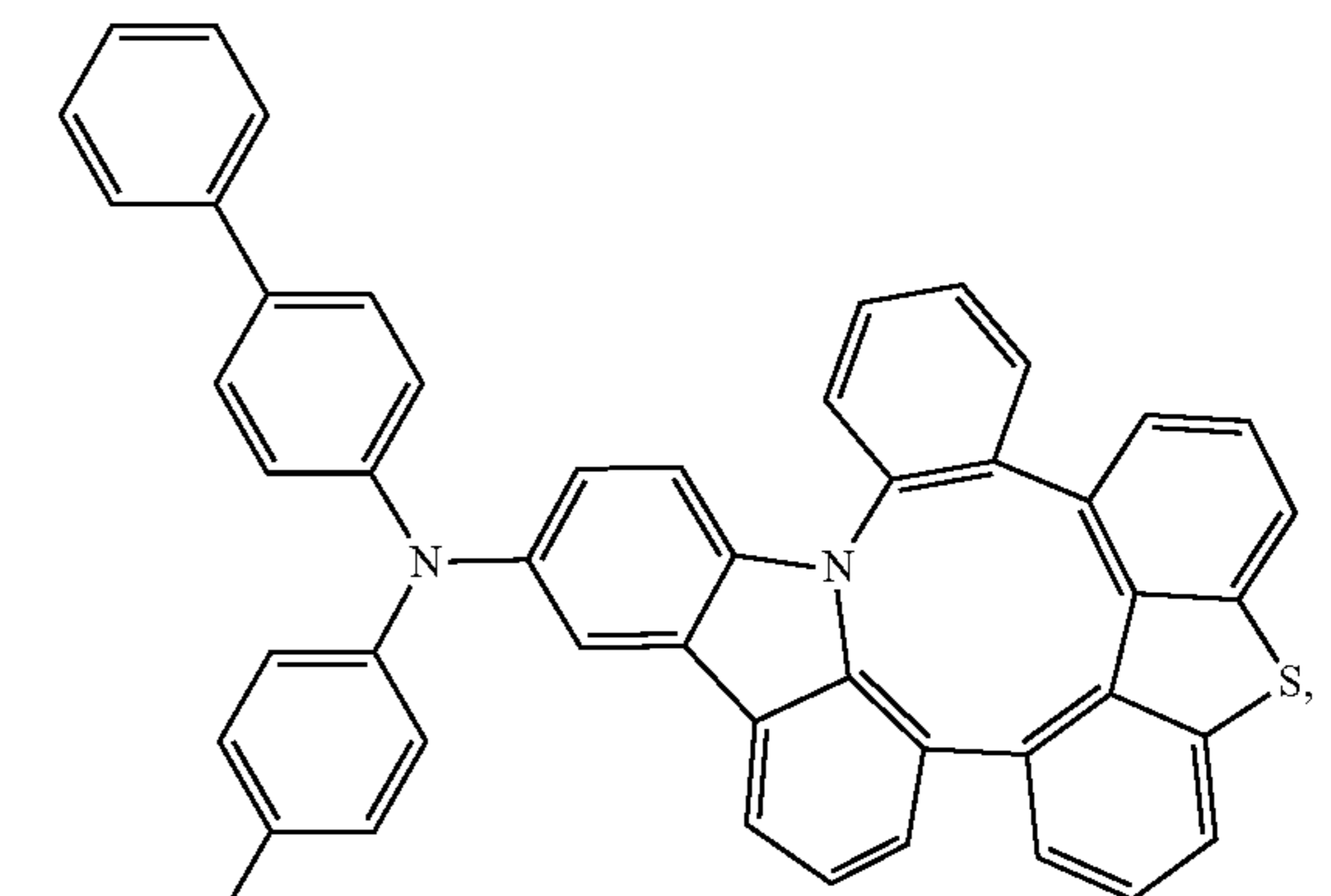
Compound 211
