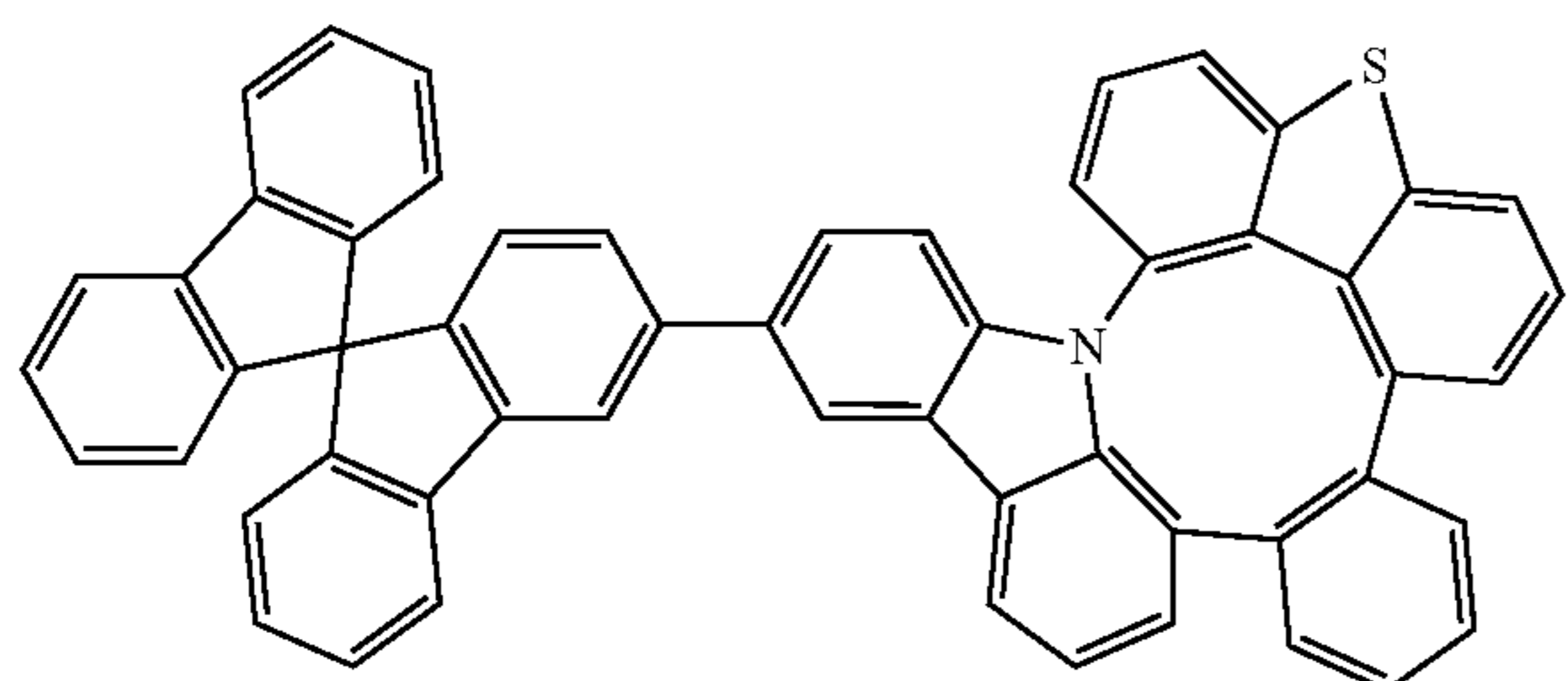
Compound 108
