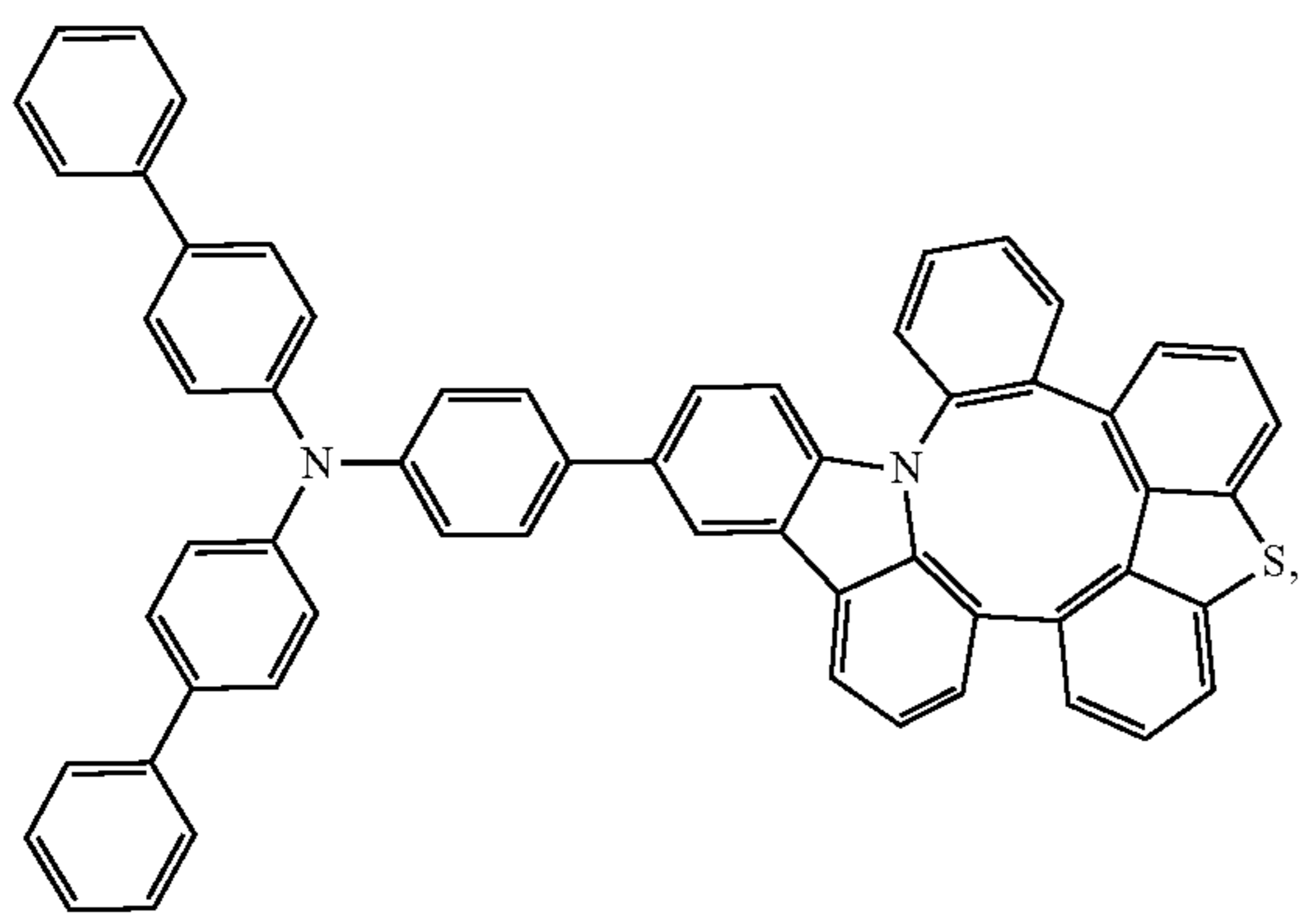
Compound 216
