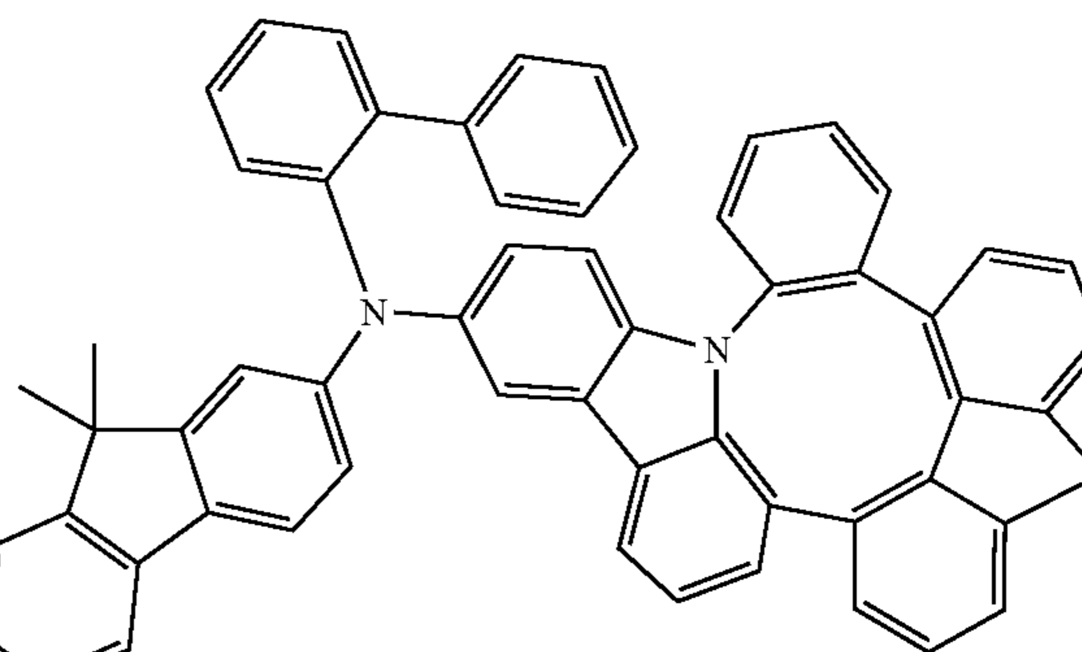
Compound 213
