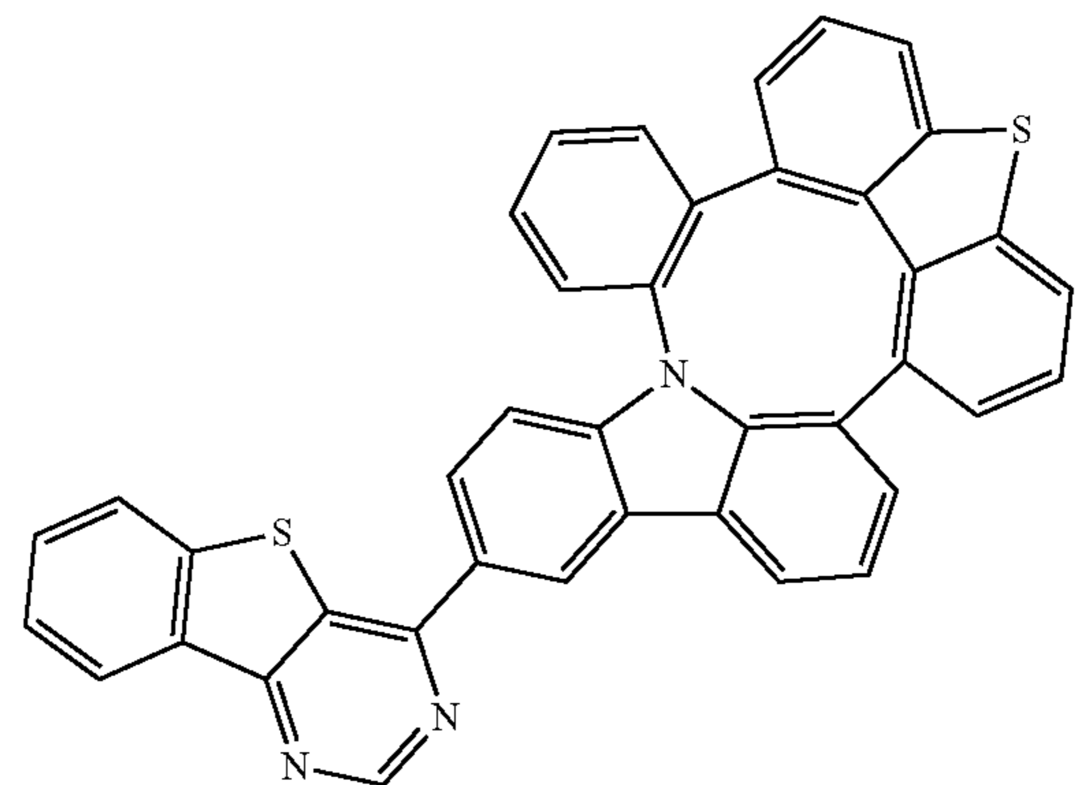
Compound 203
