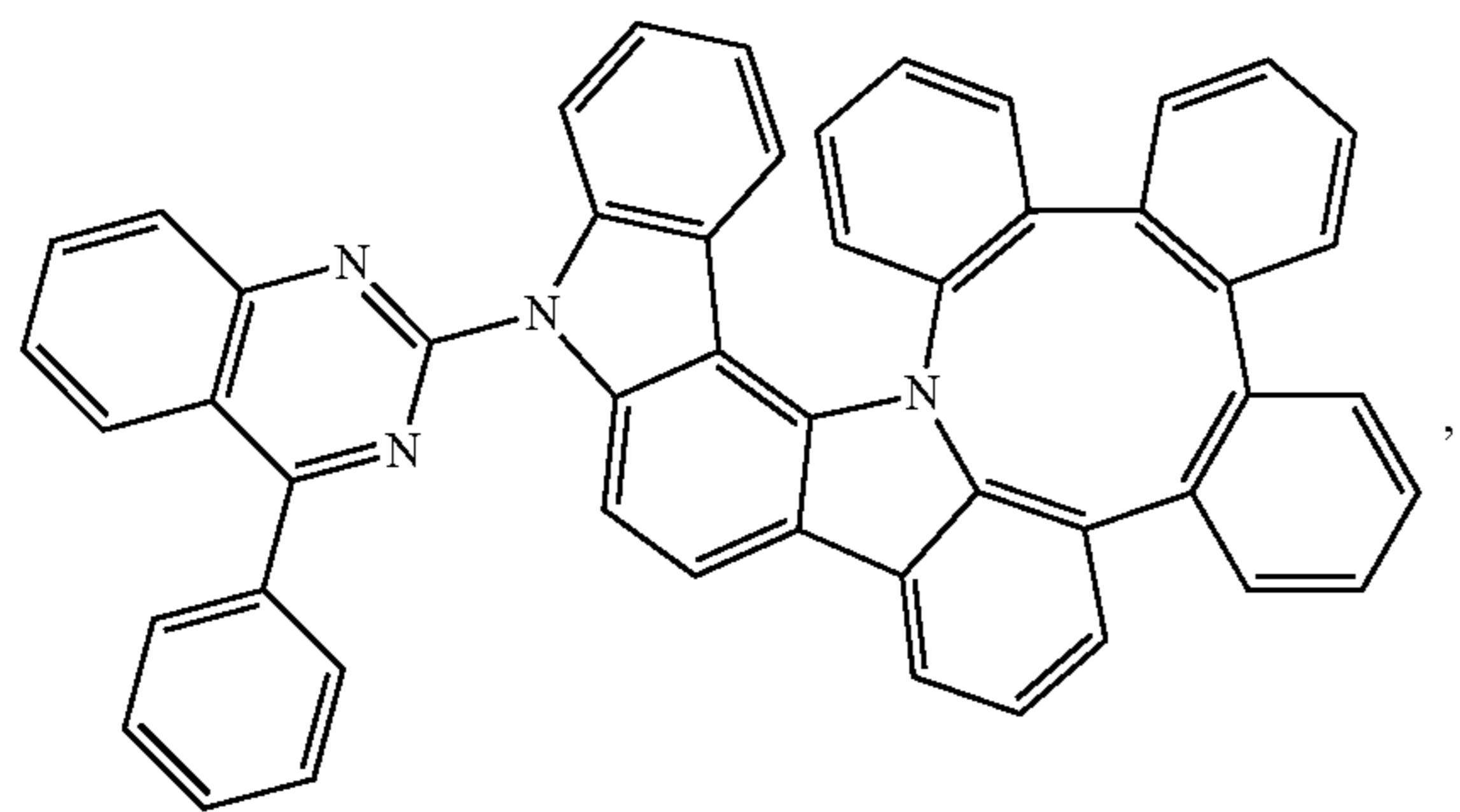
Compound 84
