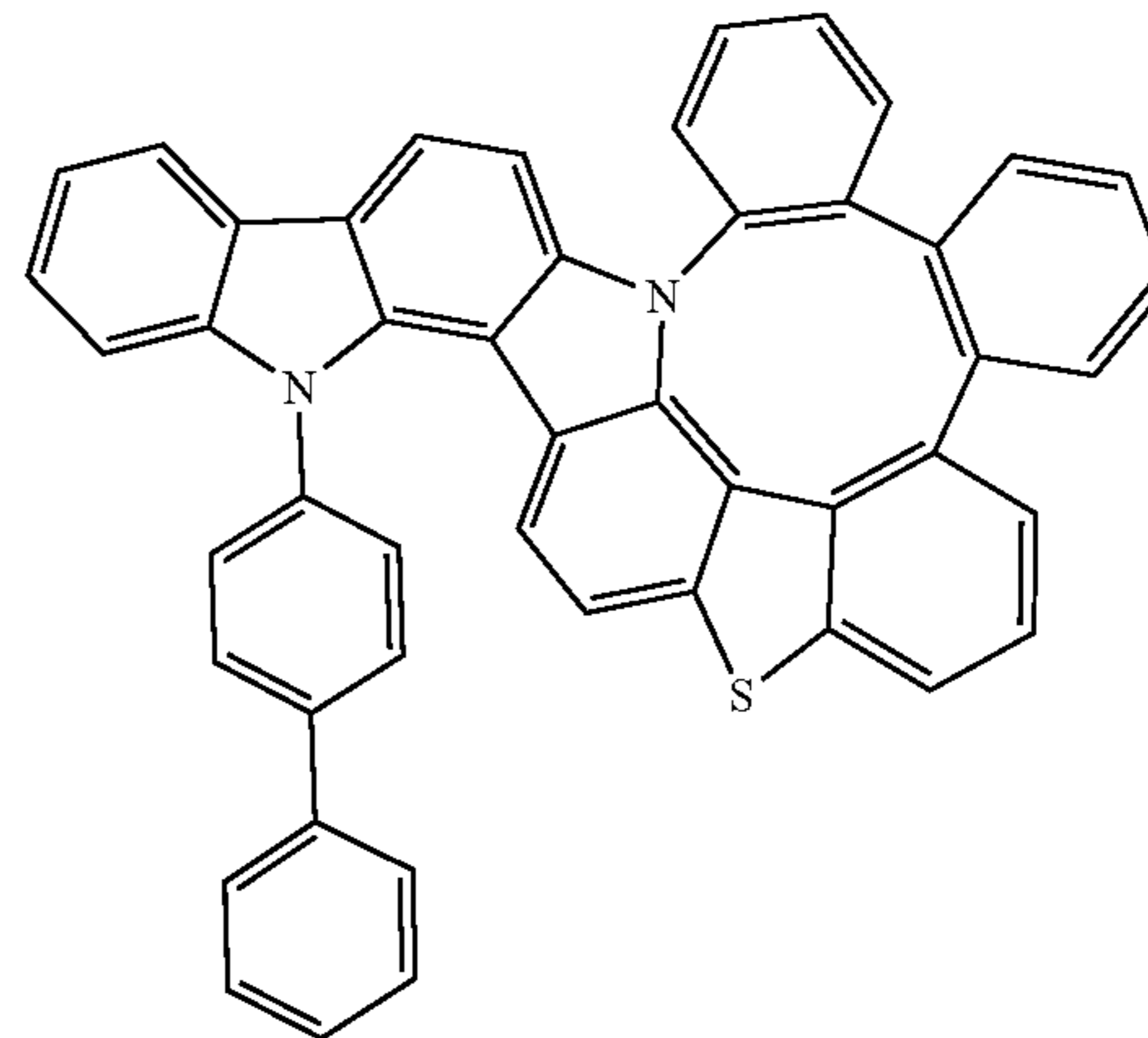
Compound 312
