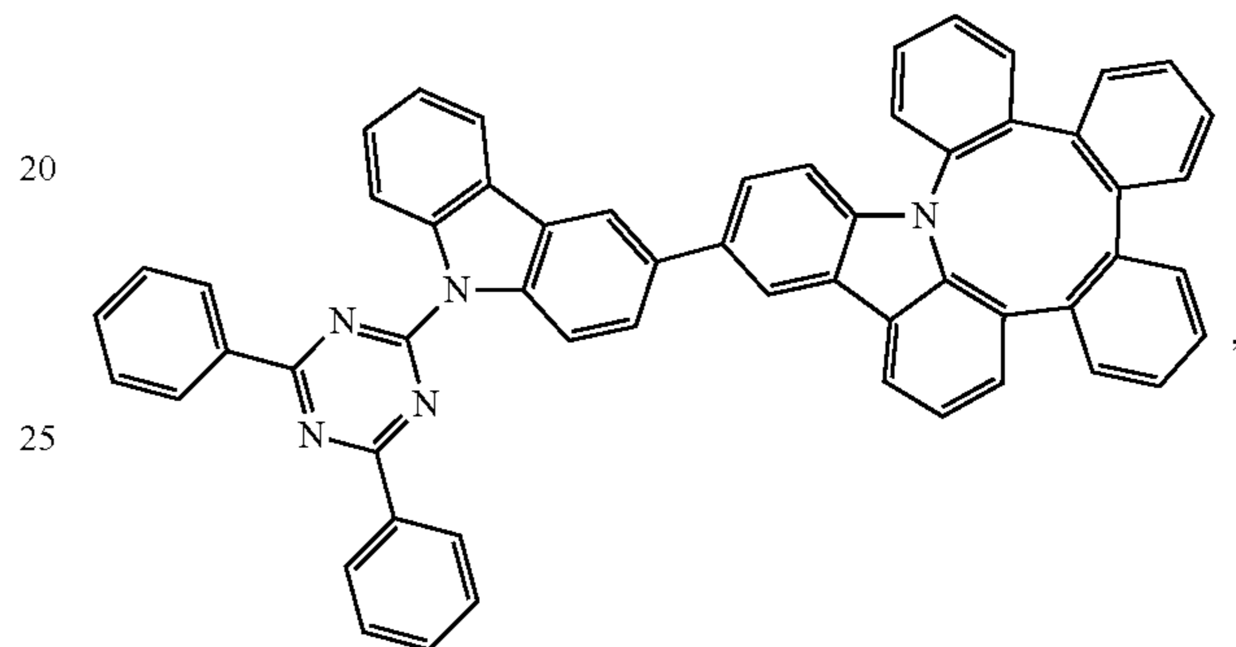
Compound 20
