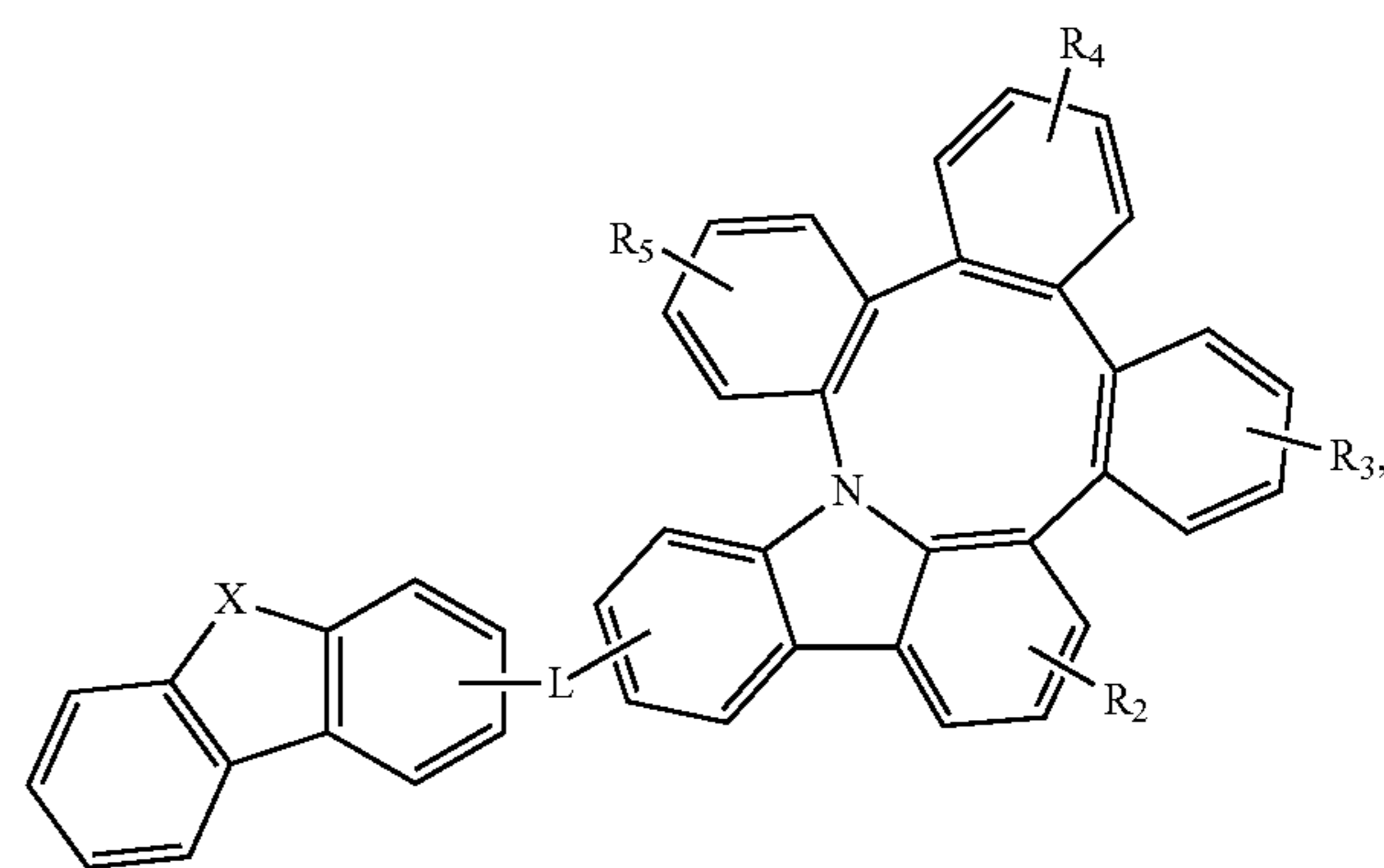
Formula 3
