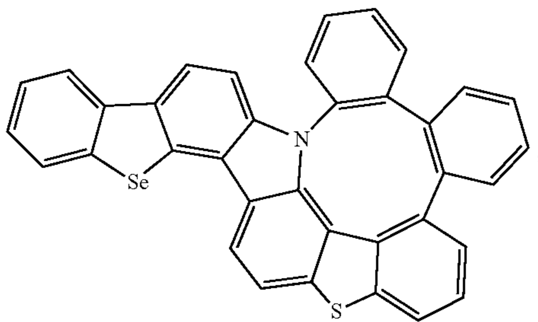
Compound 325
