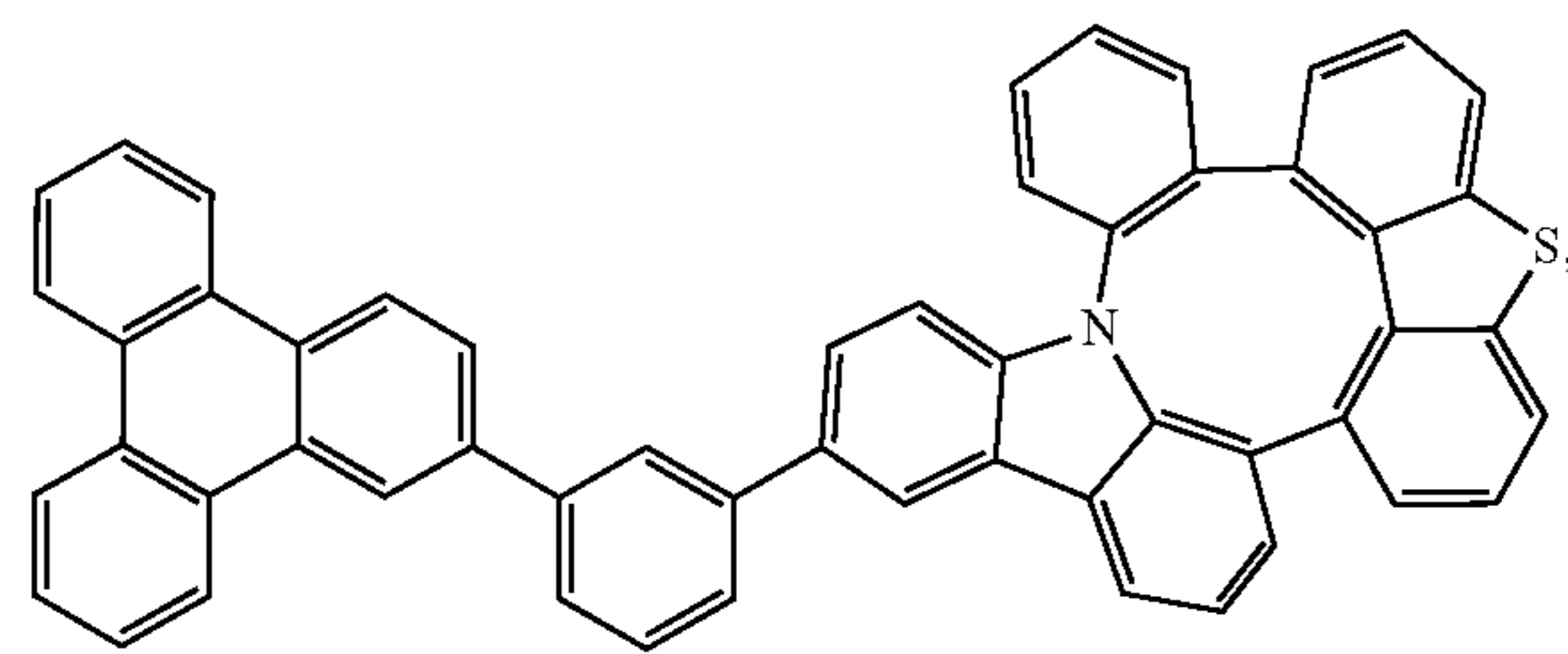
Compound 205
