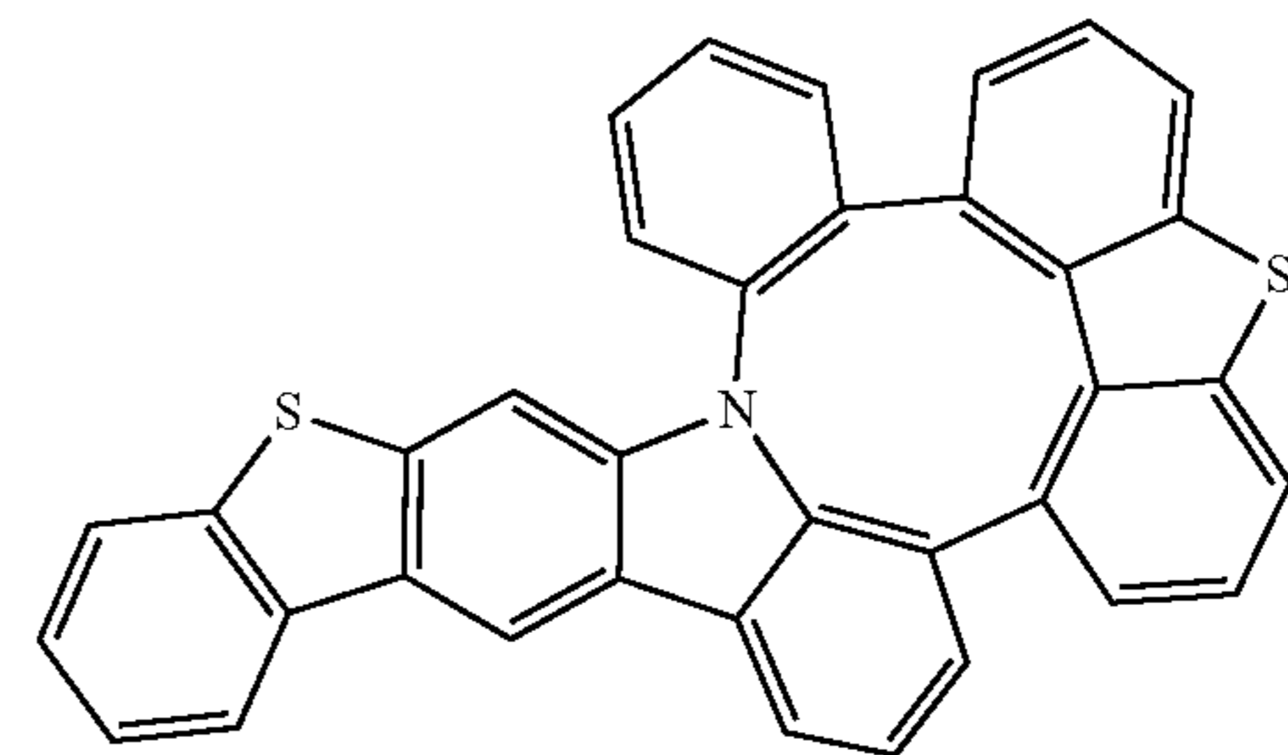
Compound 234
