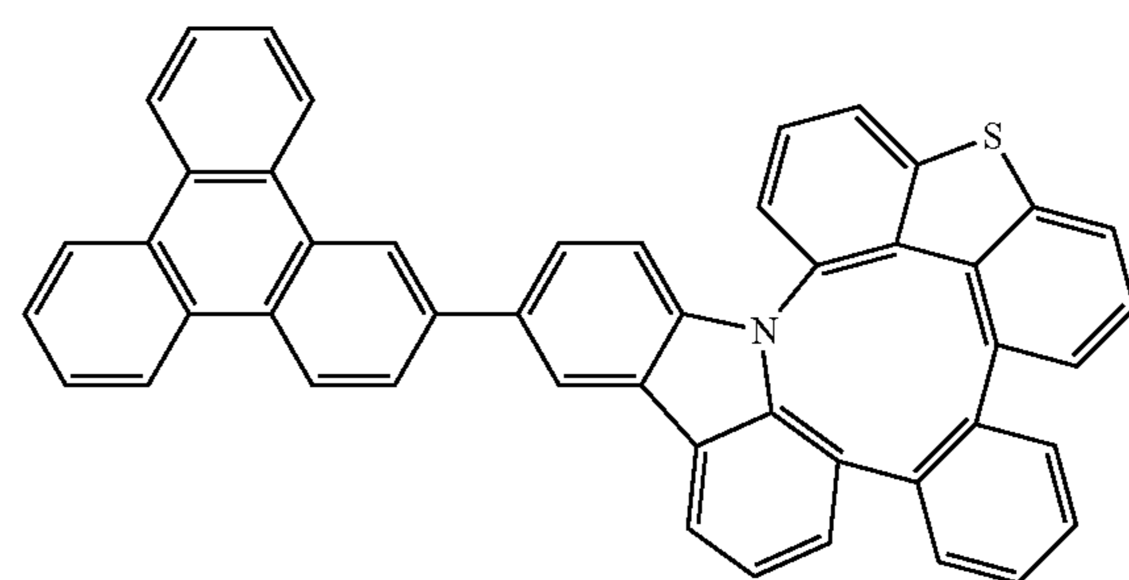
Compound 118
