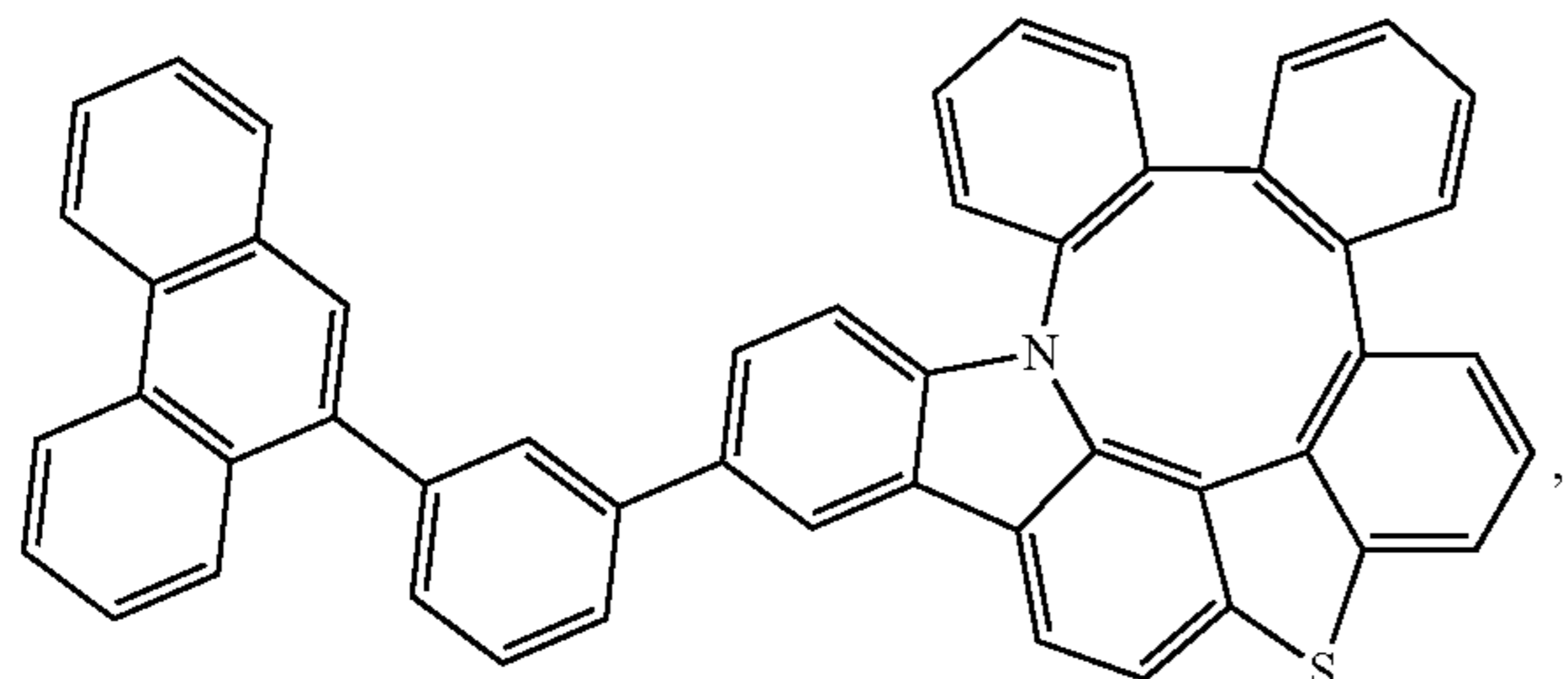
Compound 291
