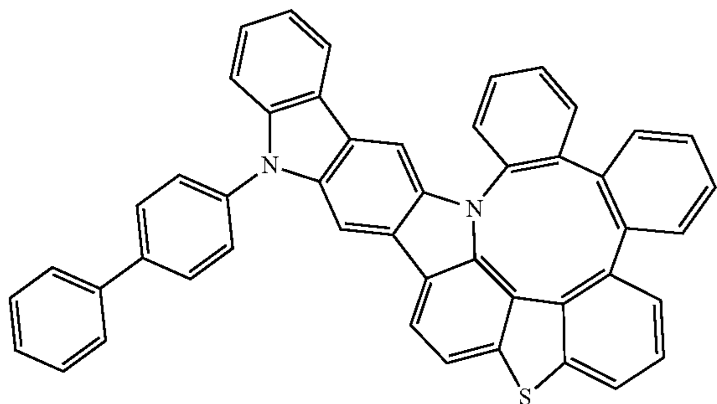
Compound 314
