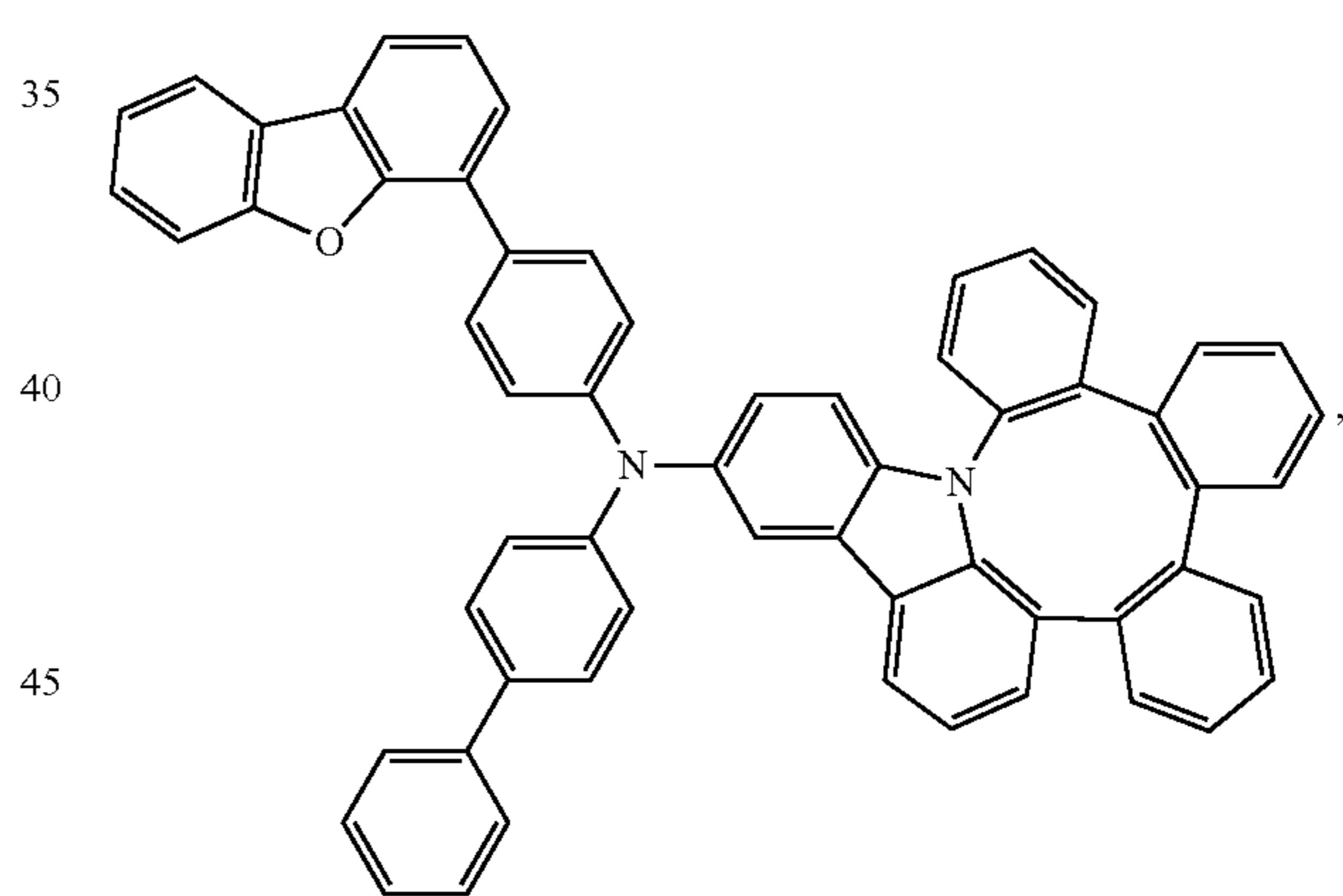
Compound 49
