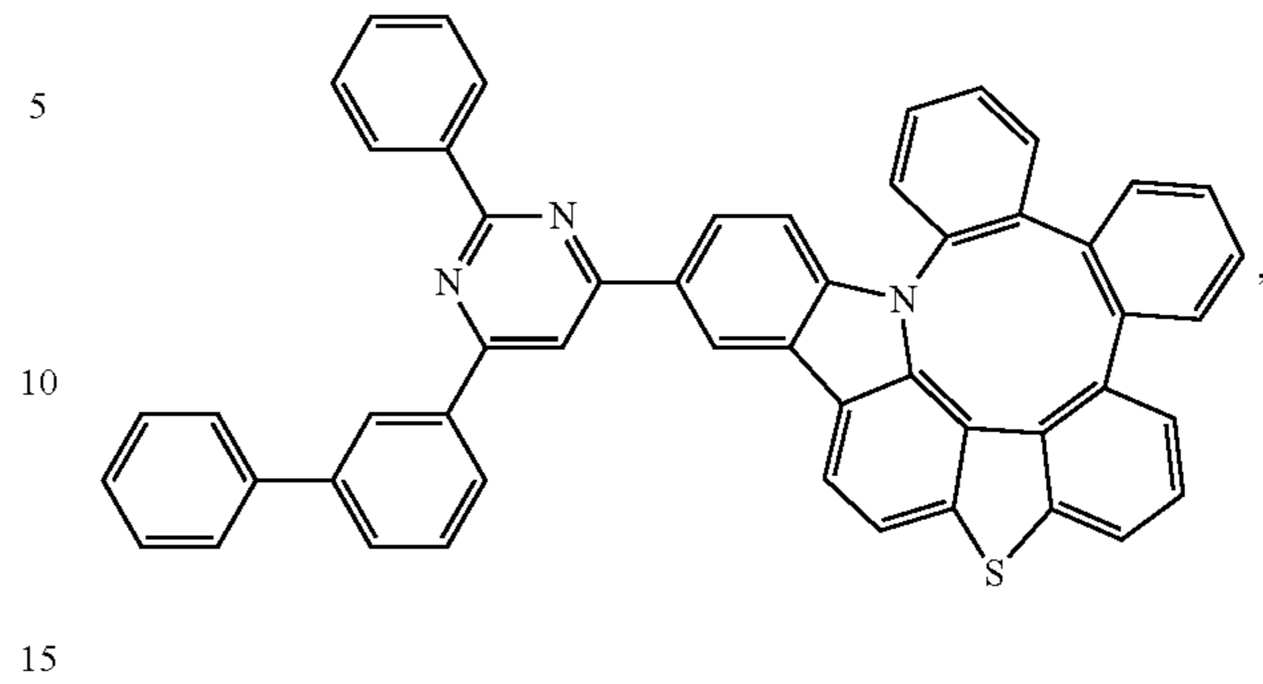
Compound 284
