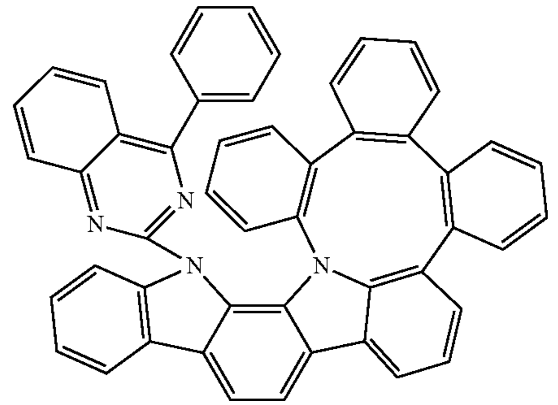
Compound 85
