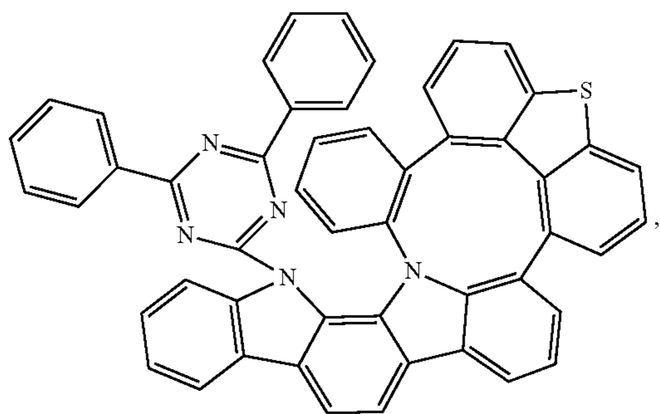
Compound 250
