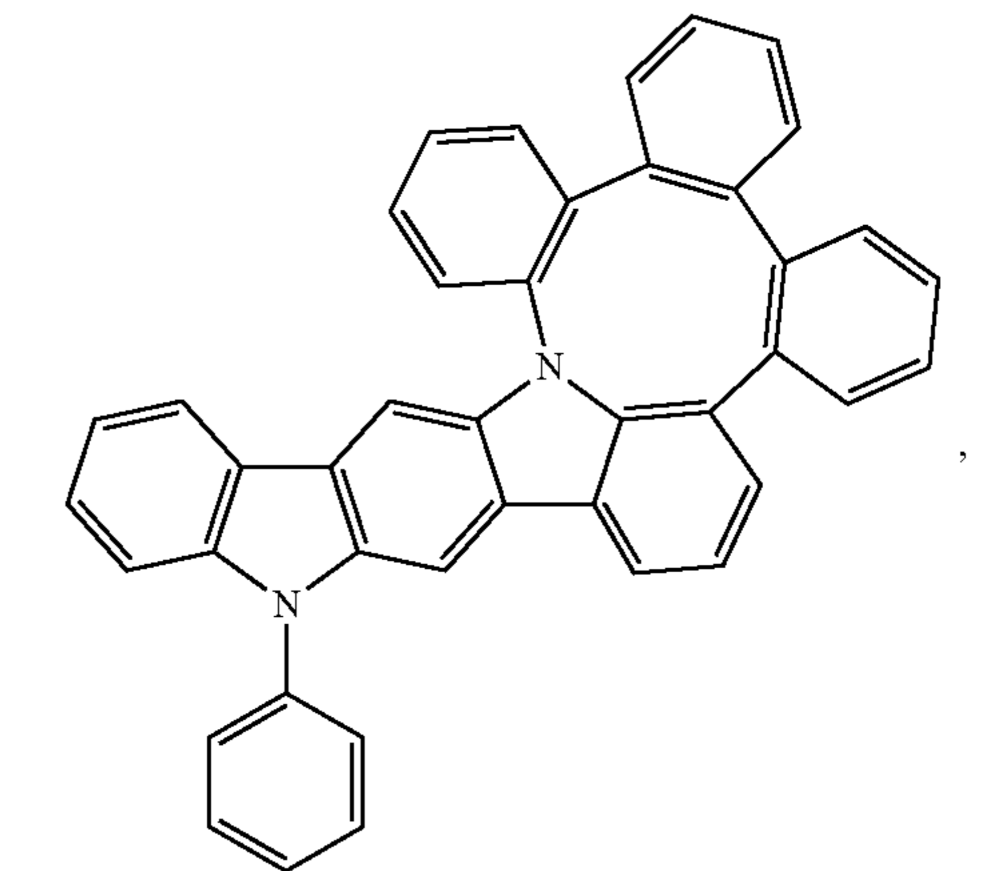
Compound 53
