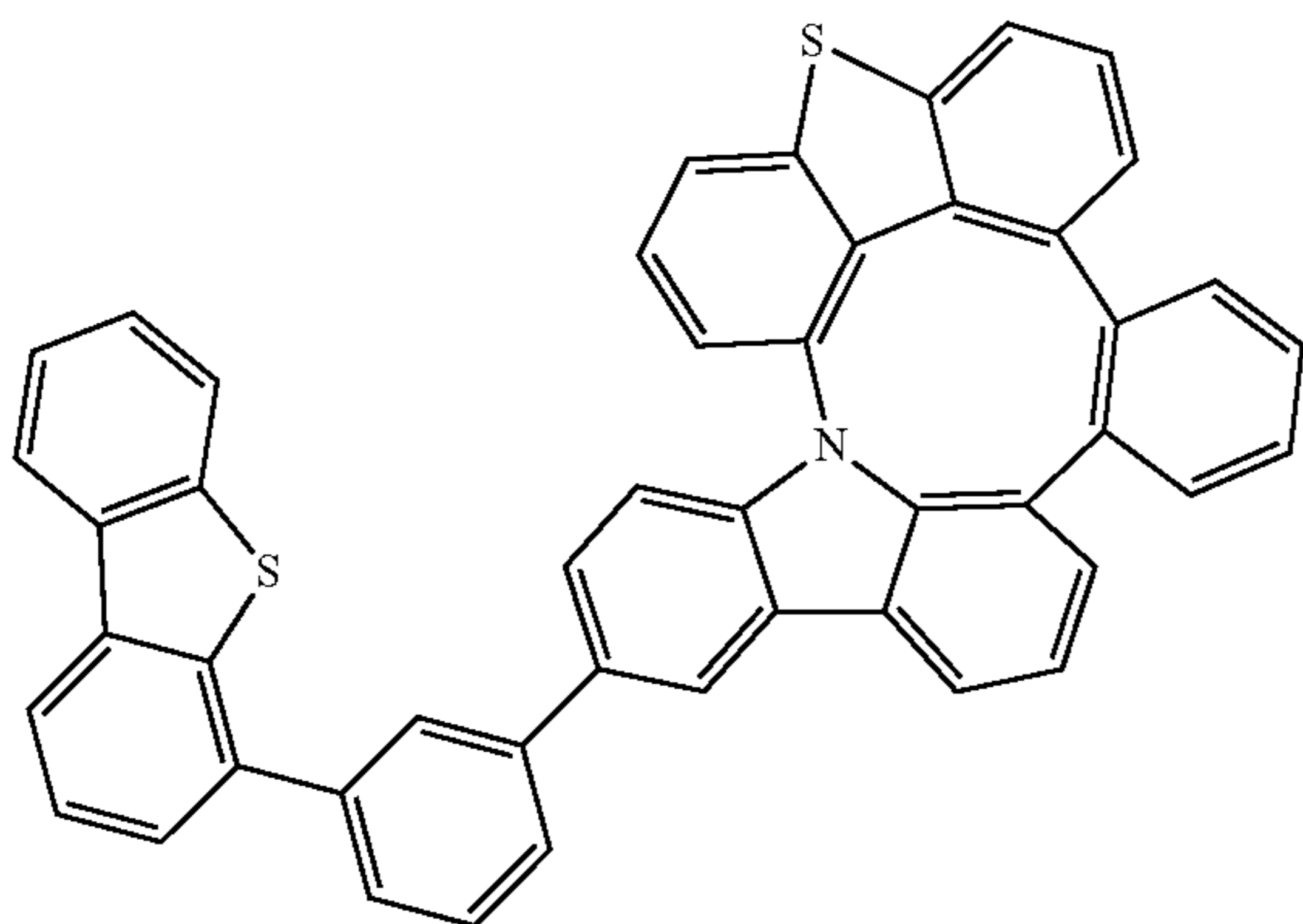
Compound 100
