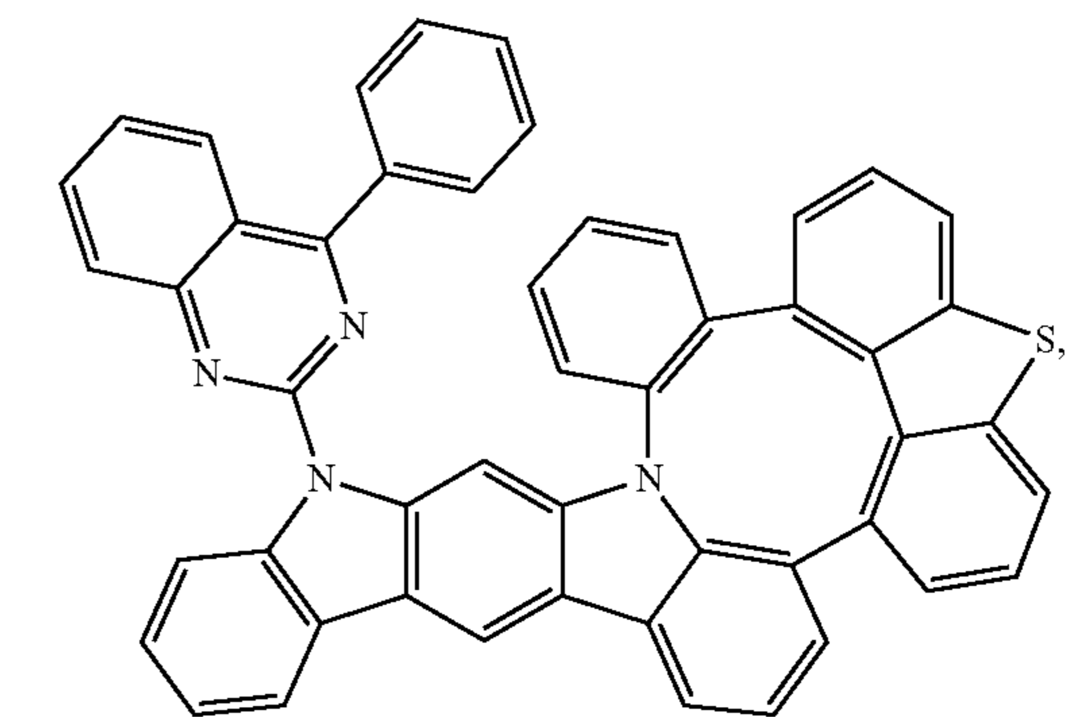
Compound 253
