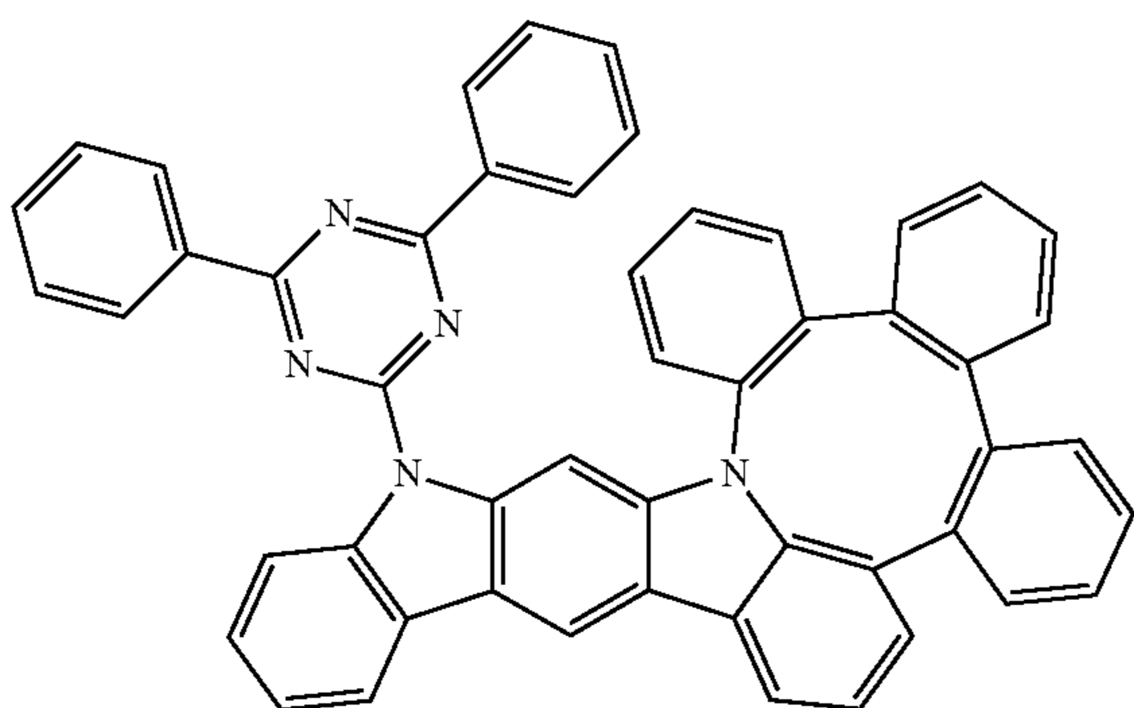
Compound 76
