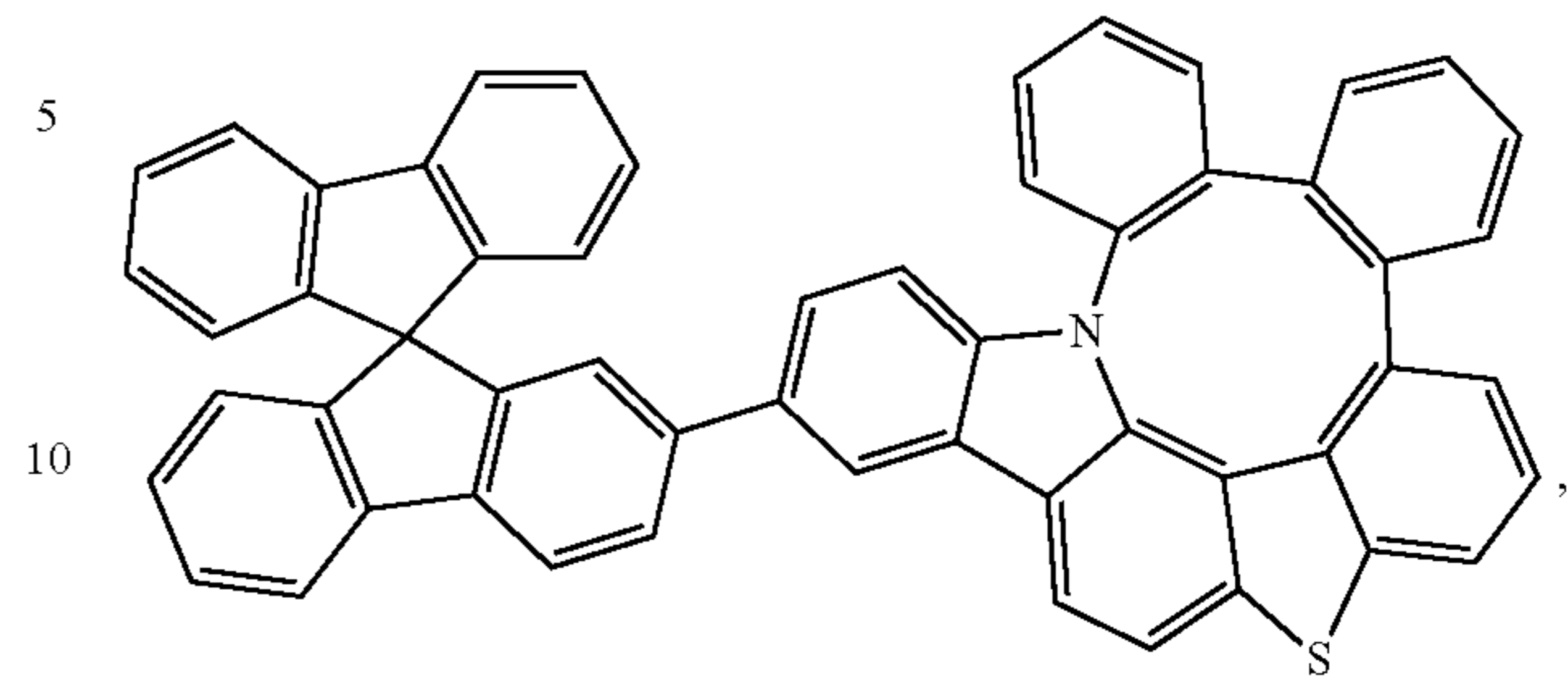
Compound 277
