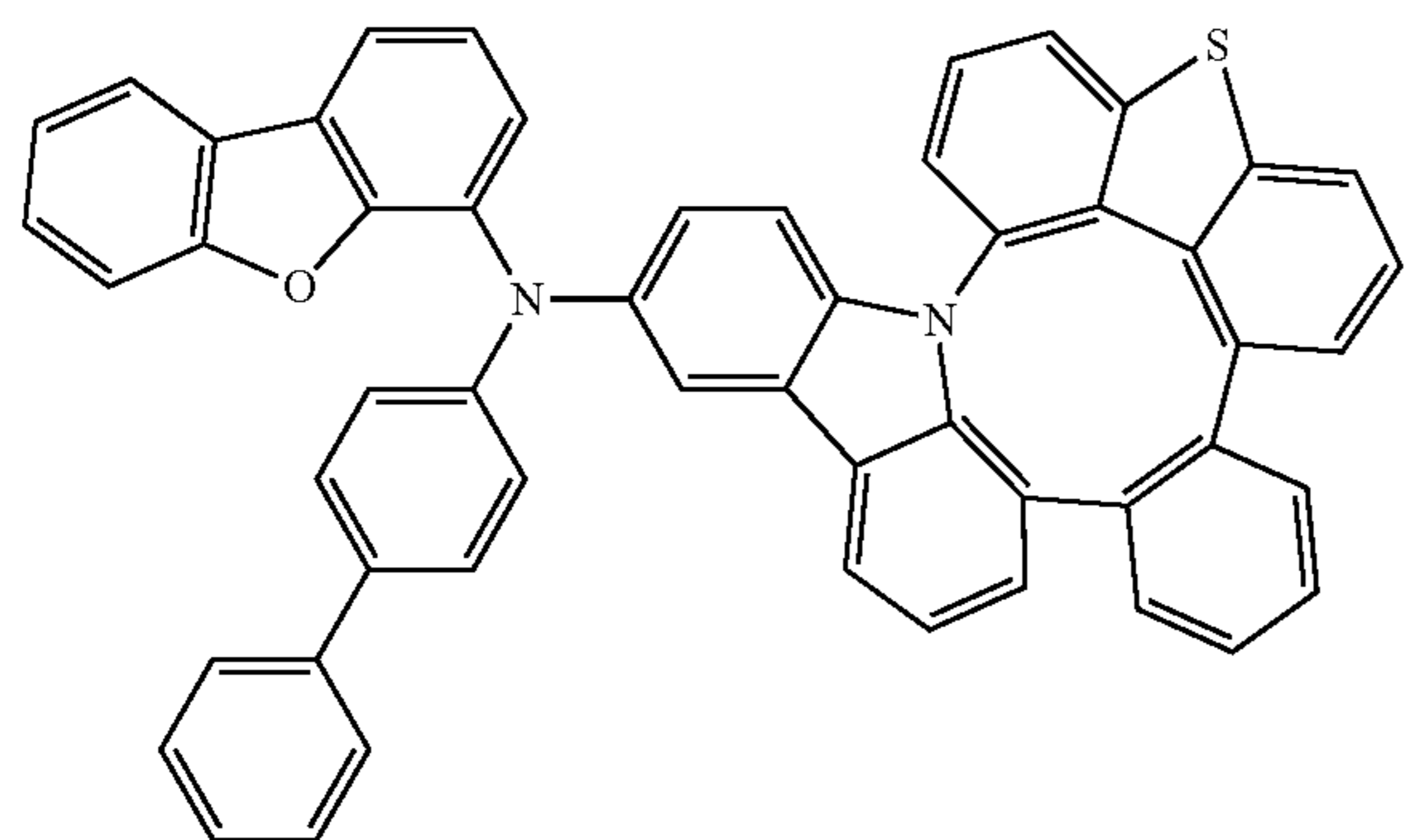
Compound 133
