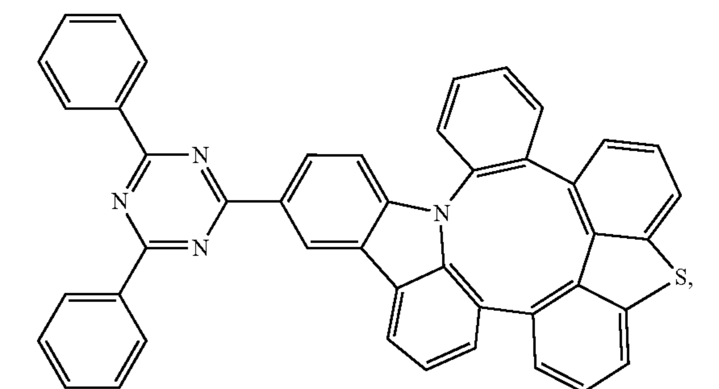
Compound 195
