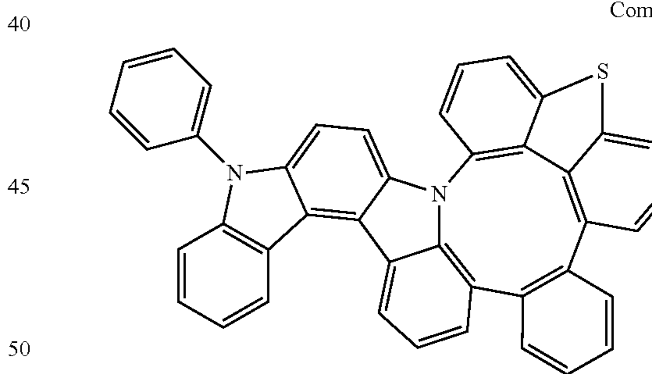
Compound 136
