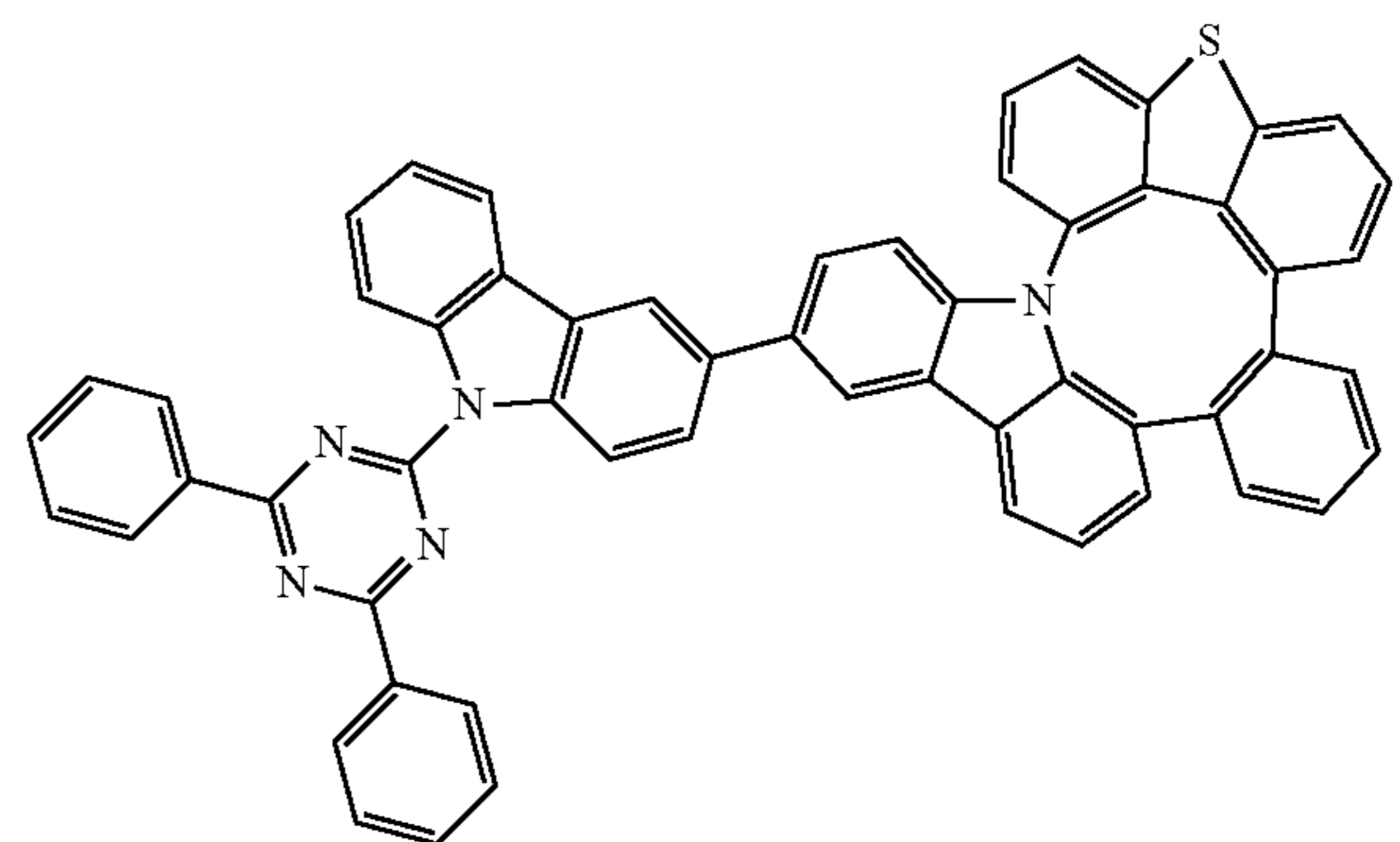
Compound 104
