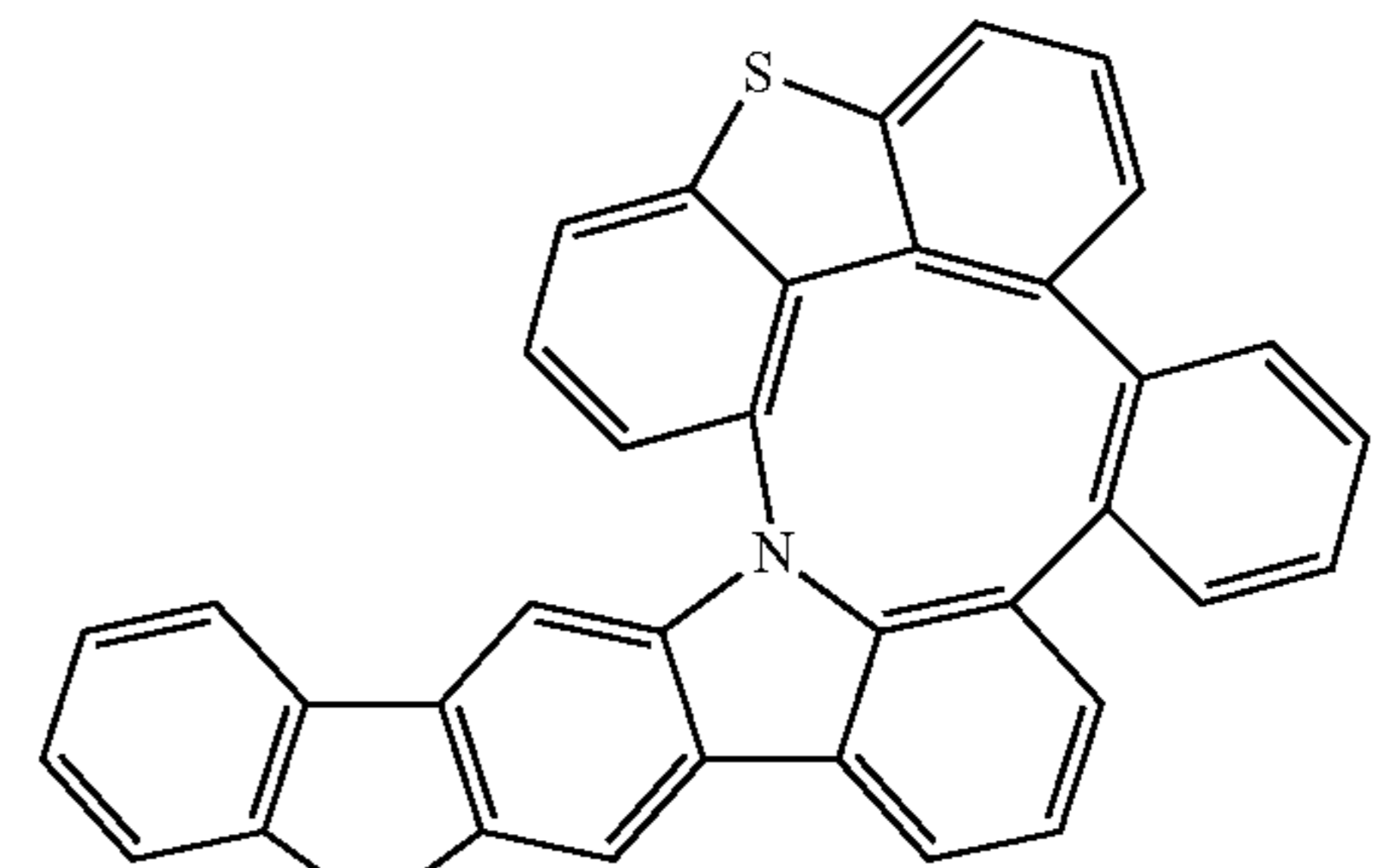
Compound 168
