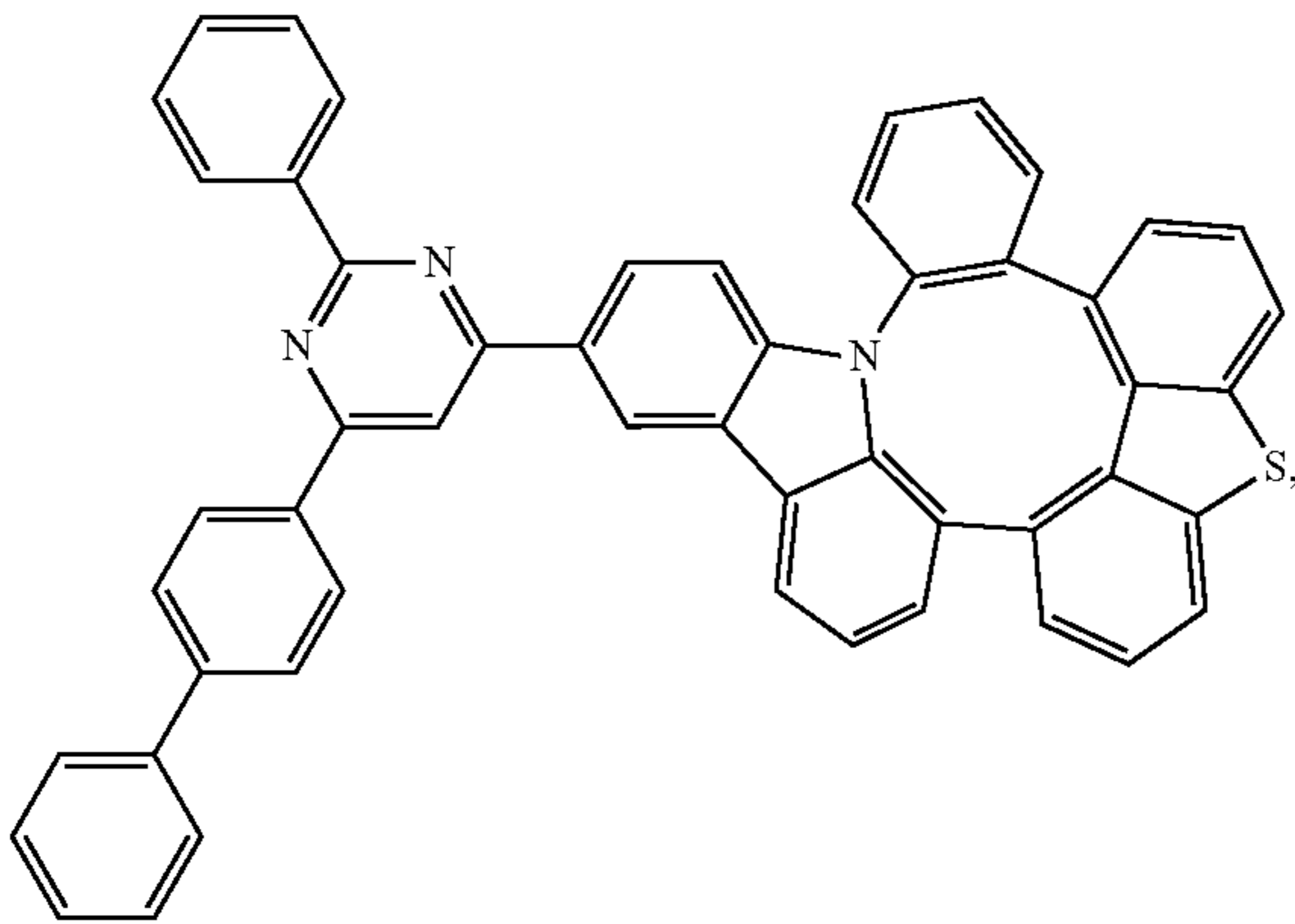
Compound 198
