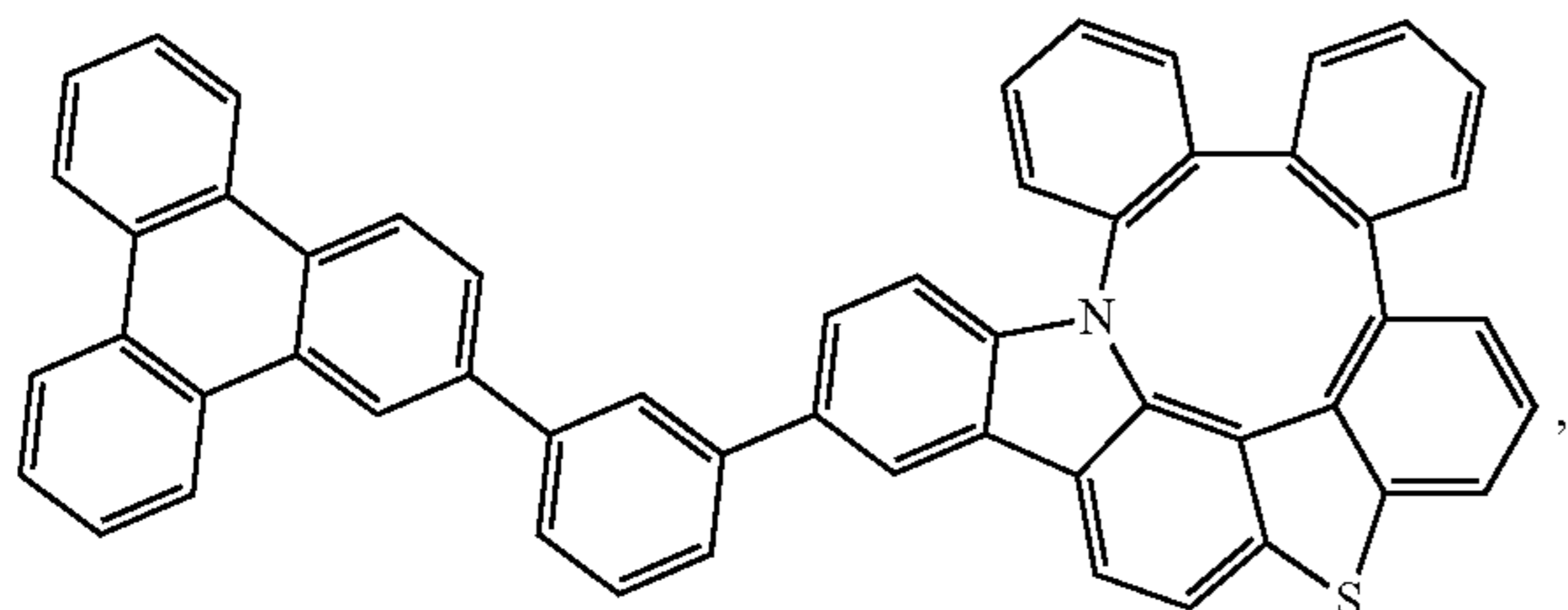
Compound 289
