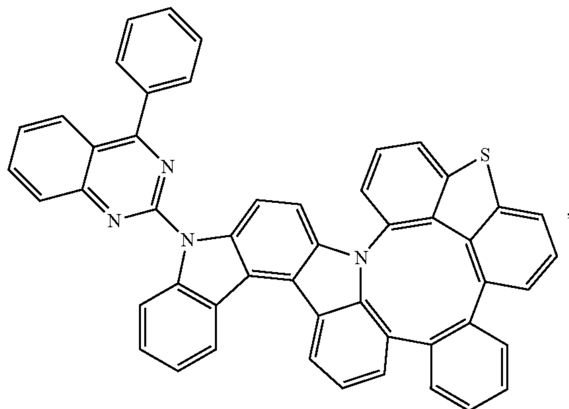
Compound 166
