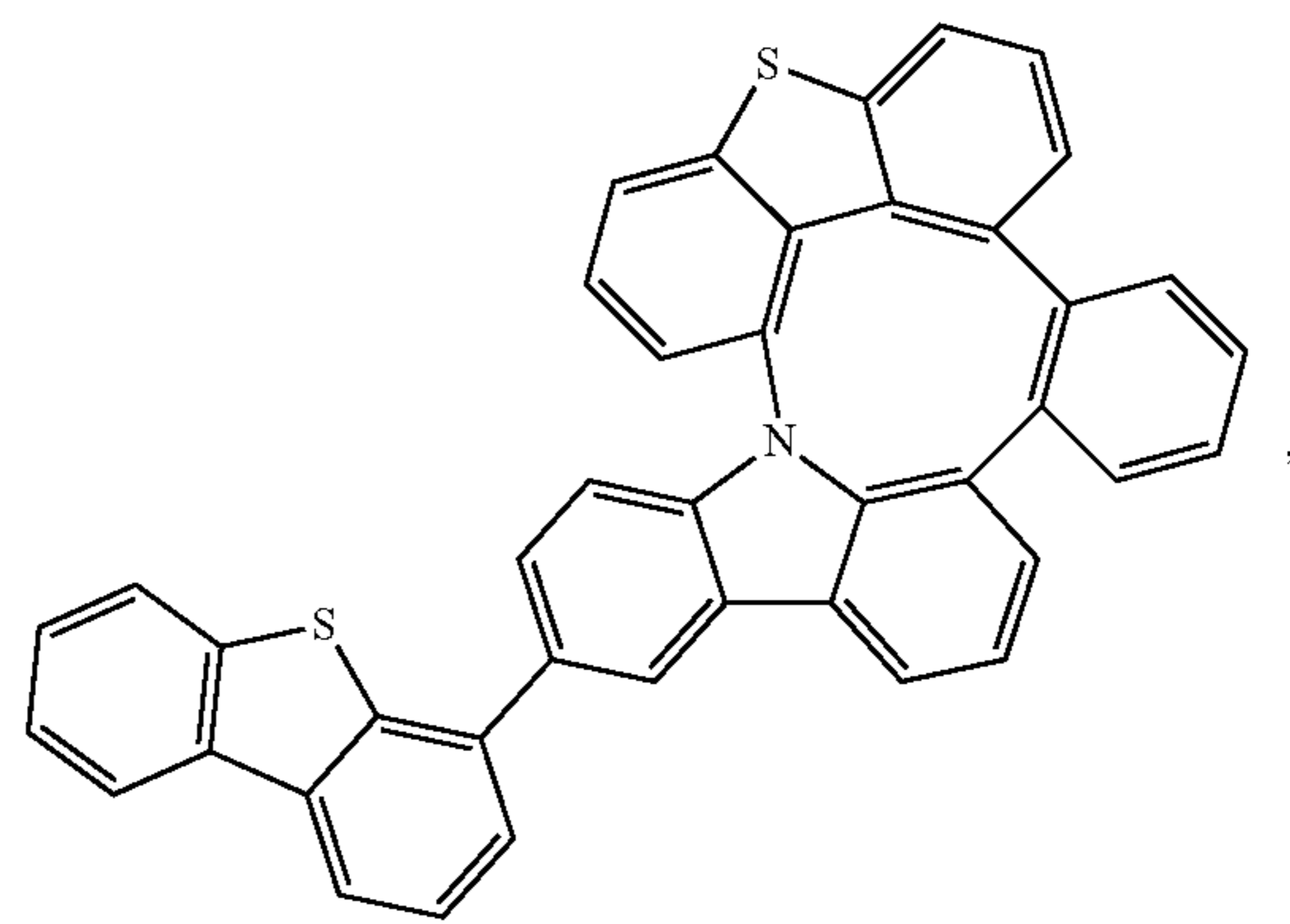
Compound 93
