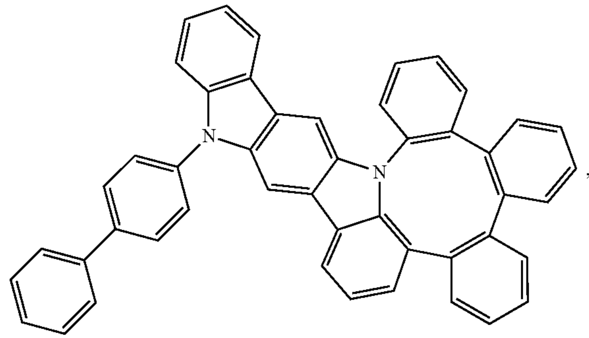
Compound 59
