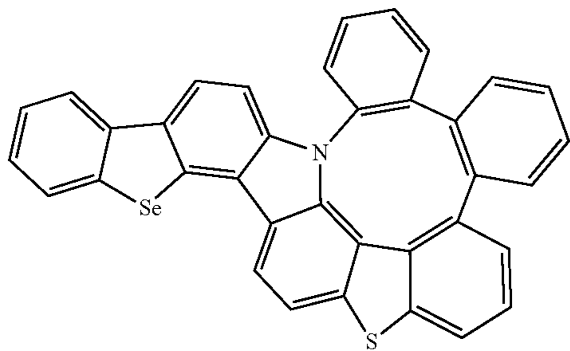
Compound 324
