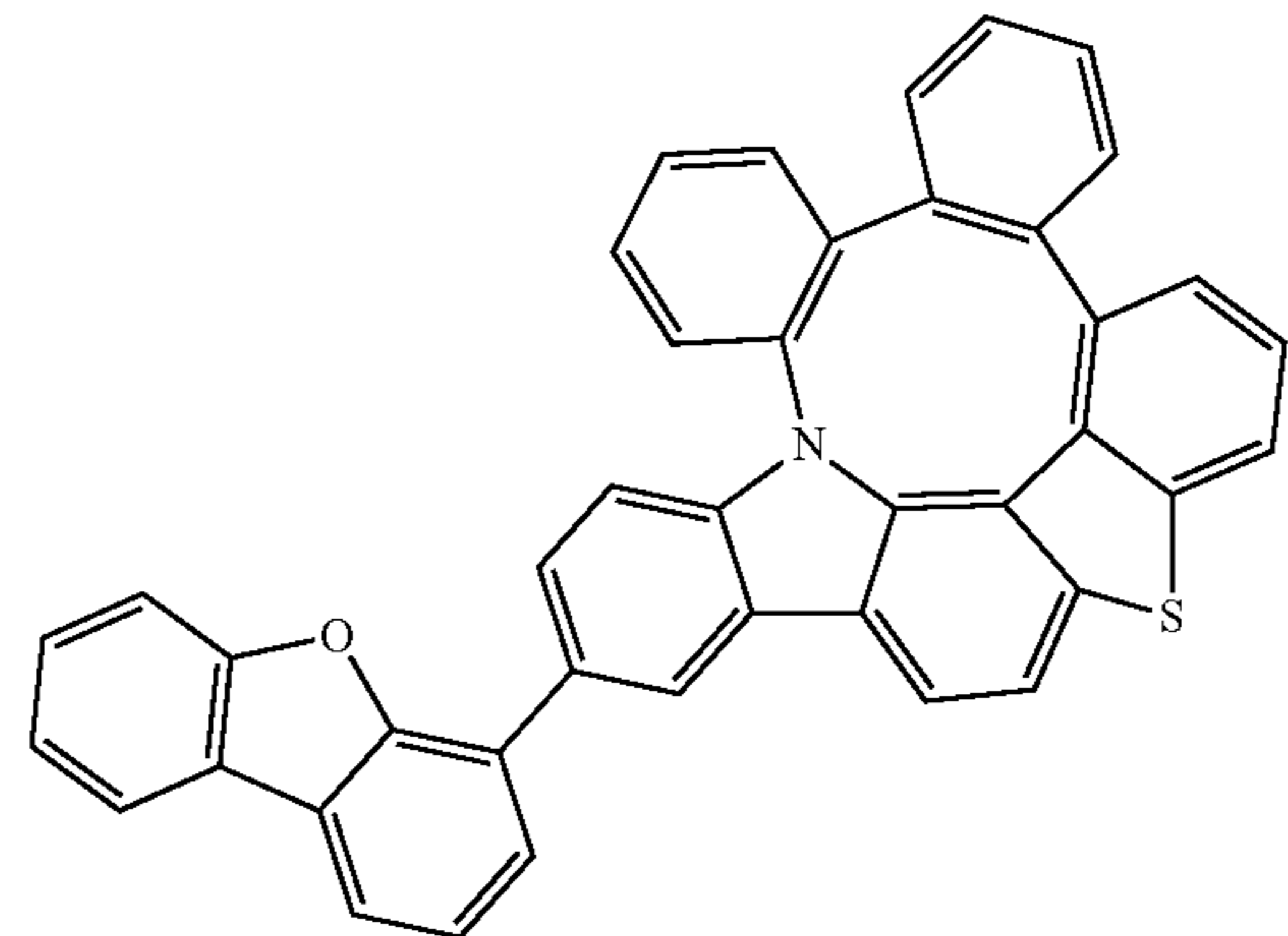
Compound 259
