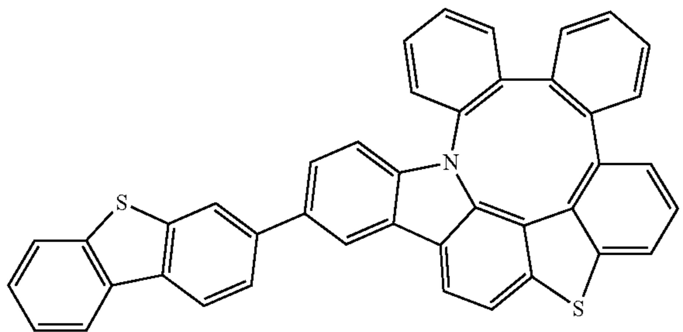
Compound 265
