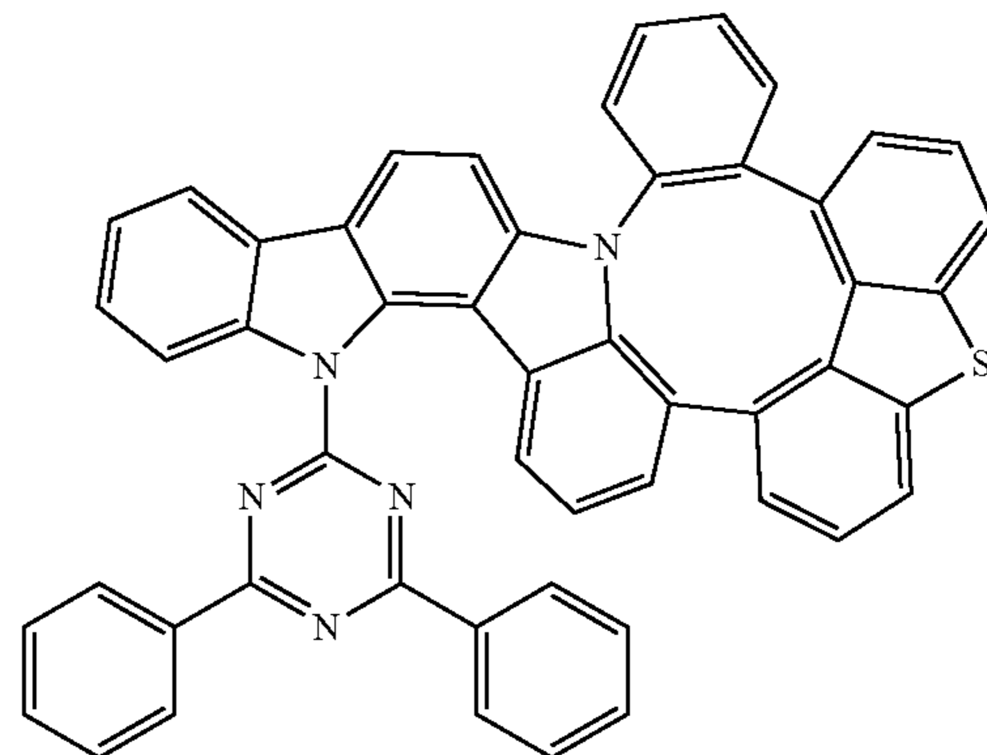
Compound 244
