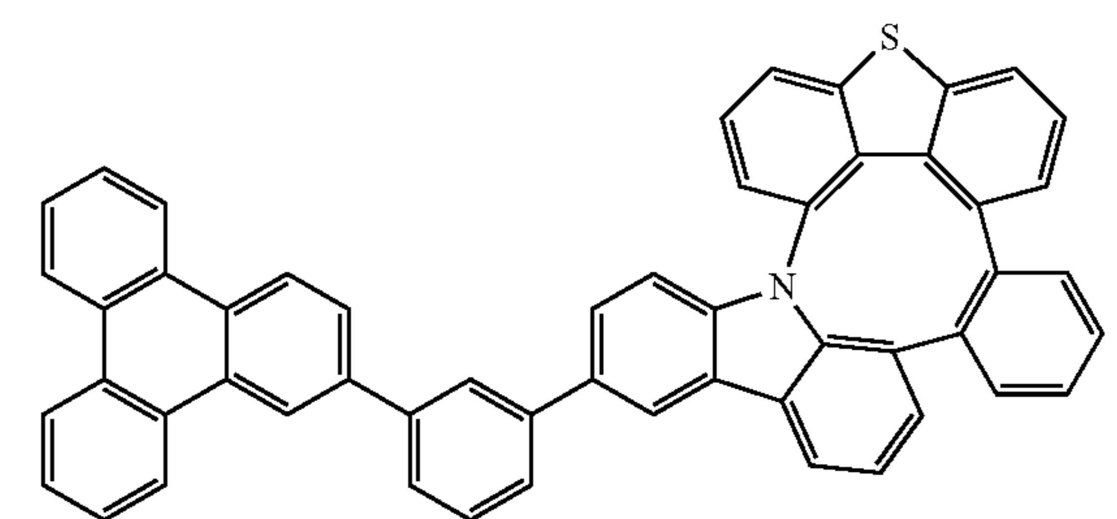
Compound 119
