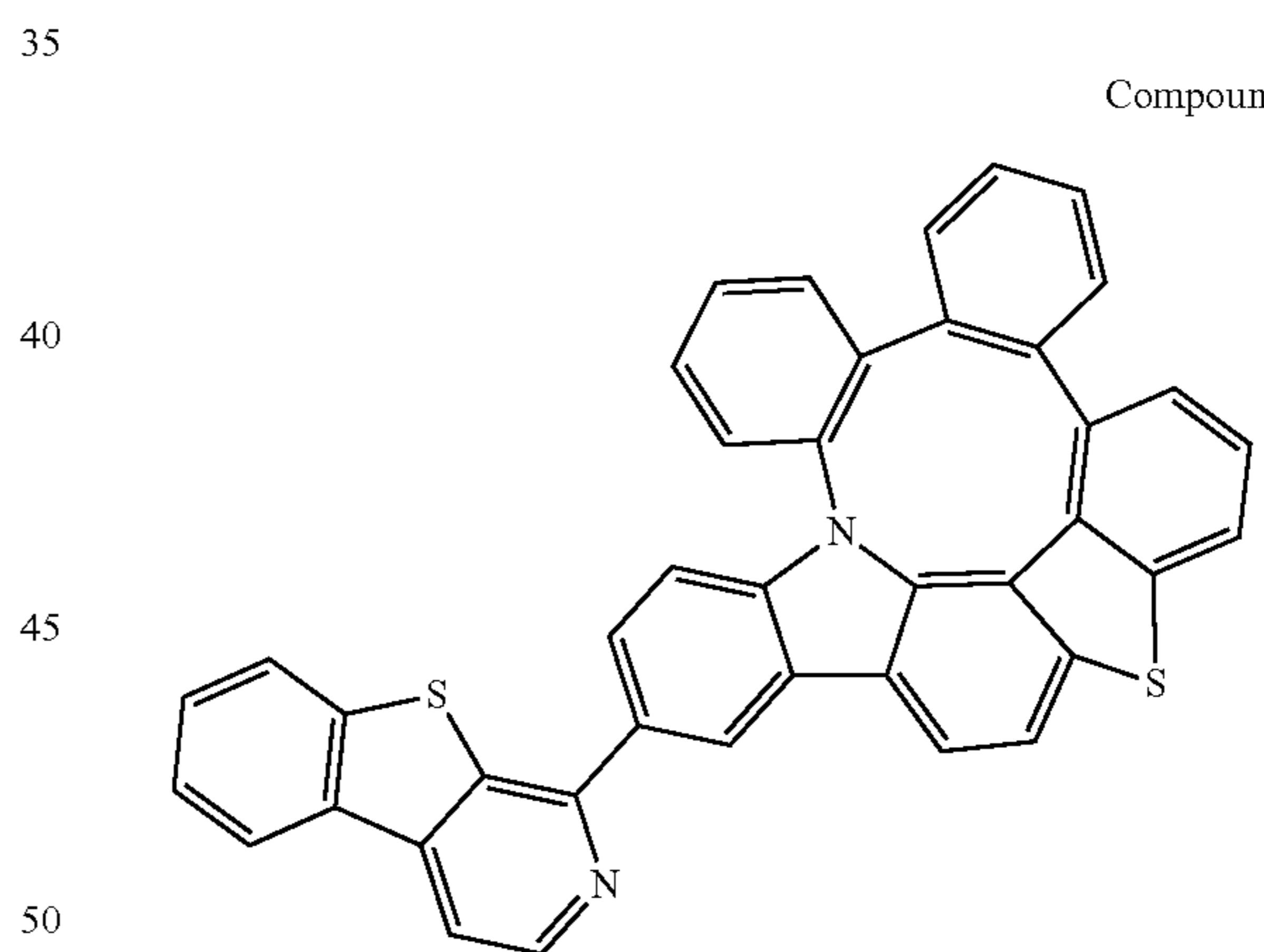
Compound 287
