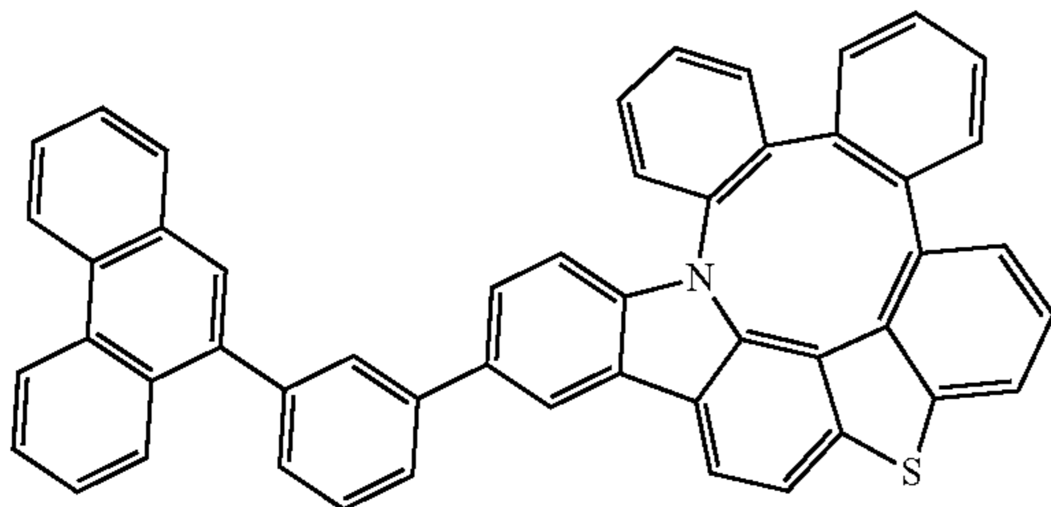
Compound 290
