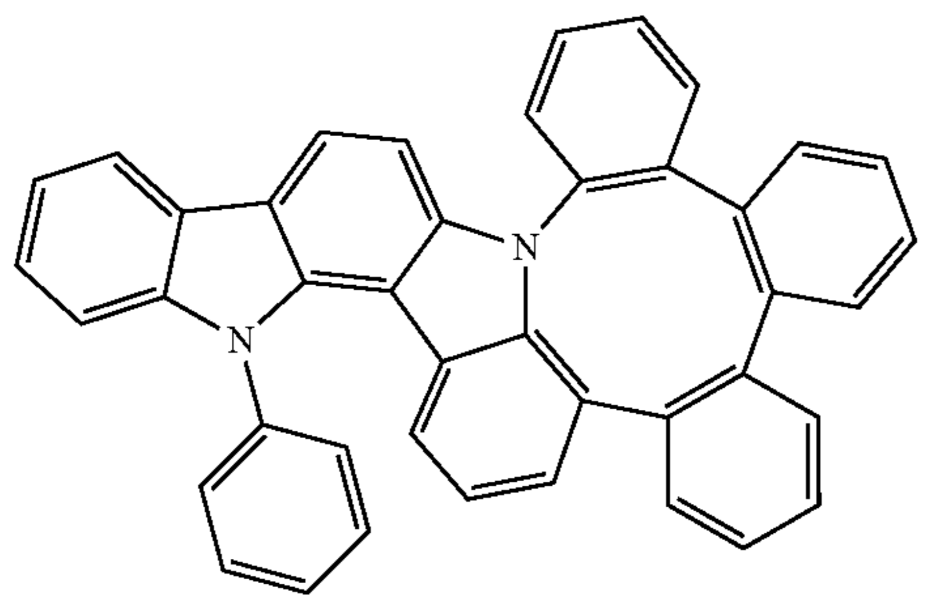
Compound 50
