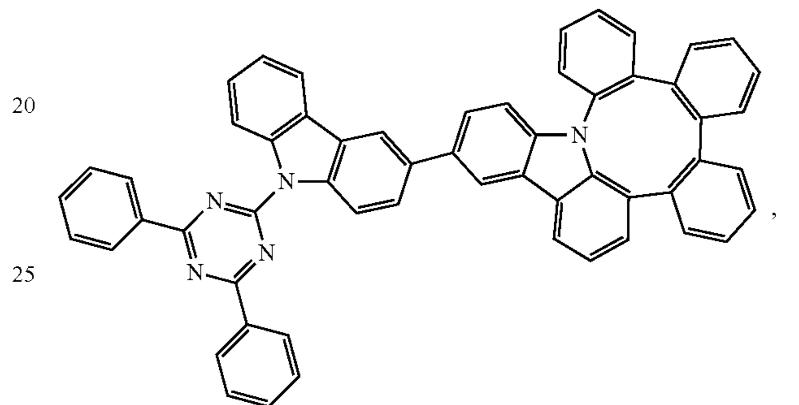
Compound 20
