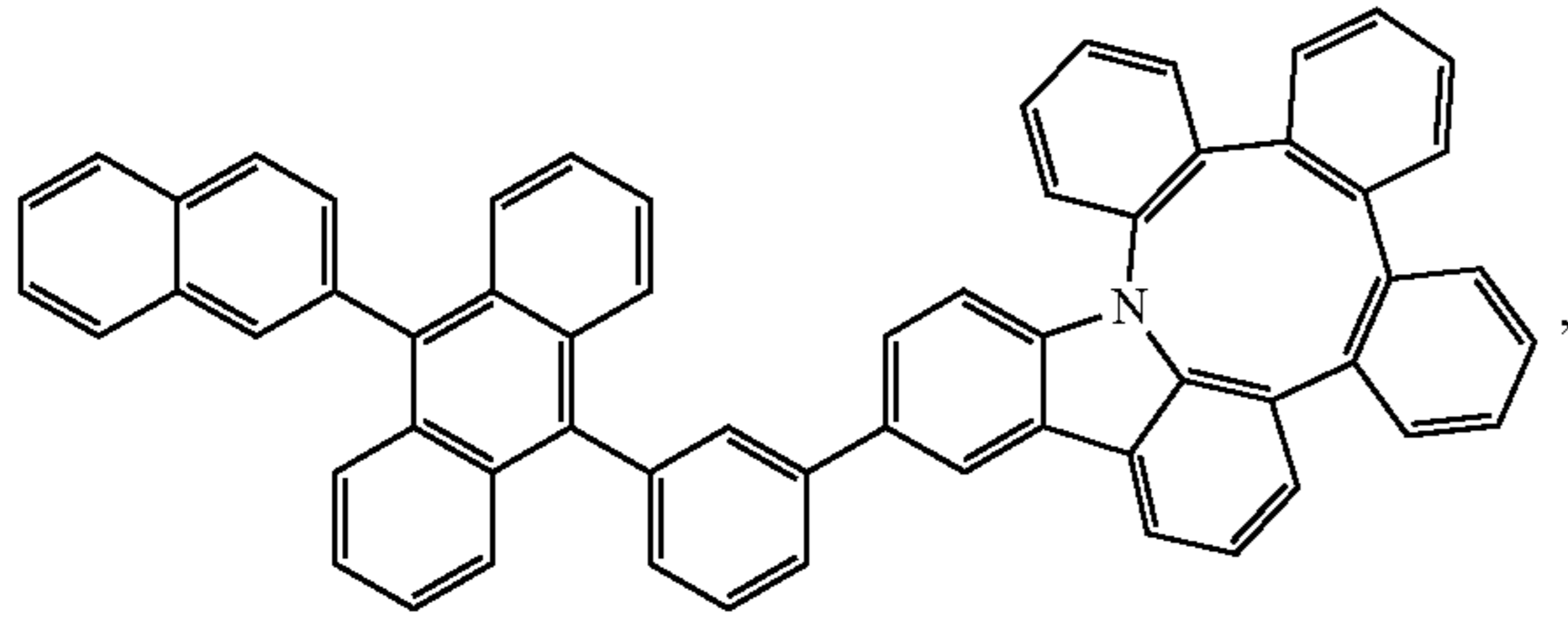
Compound 41
