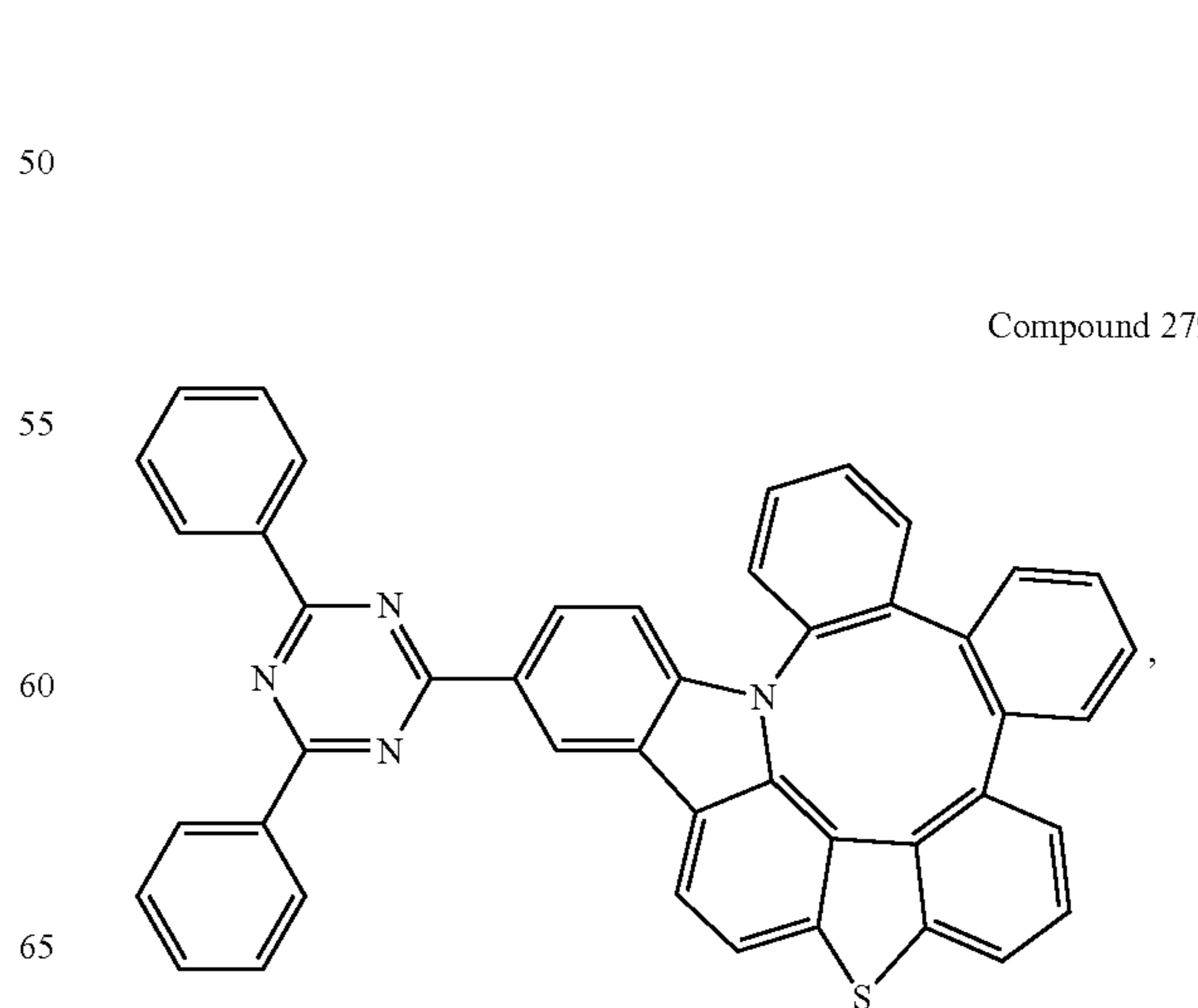
Compound 279
