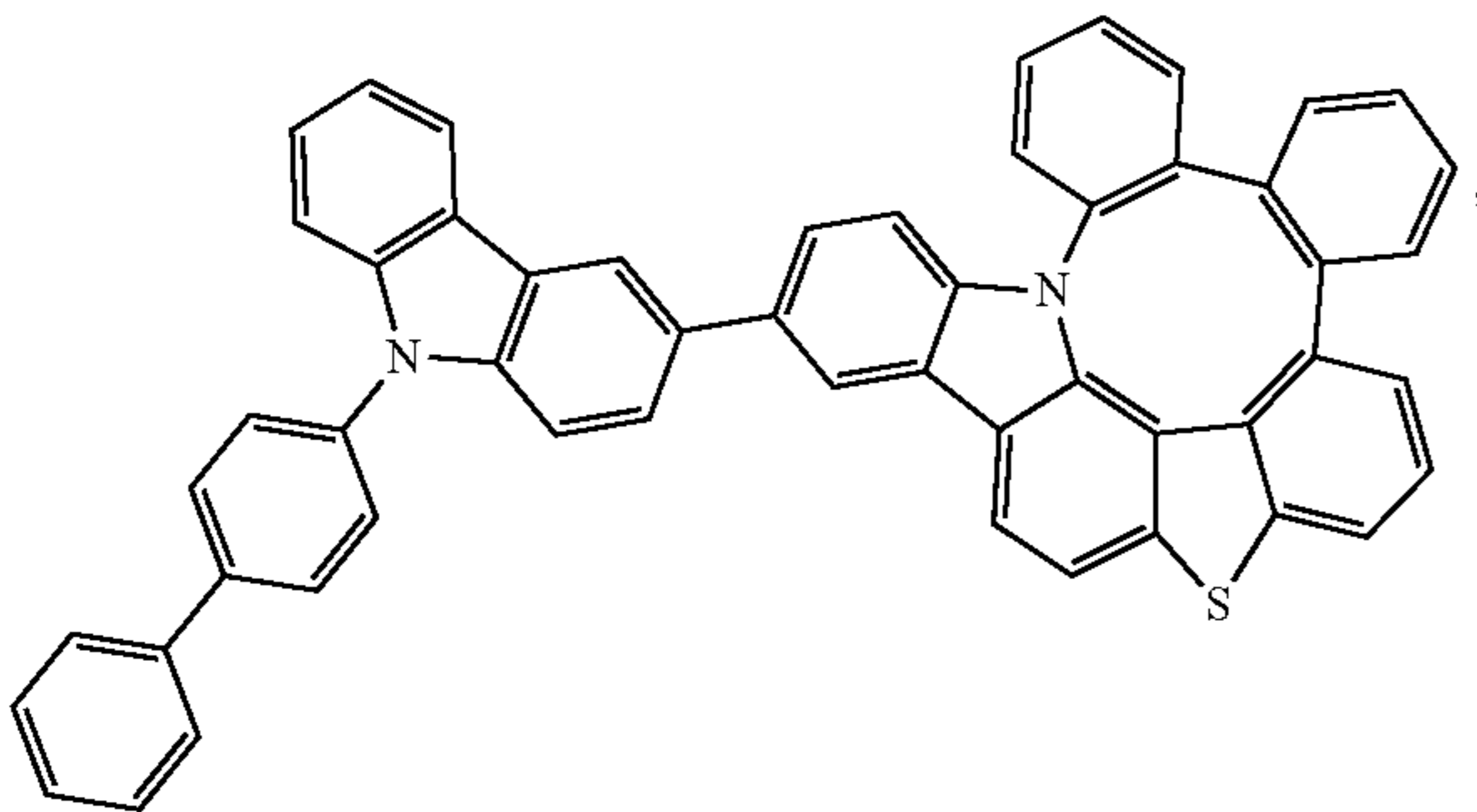
Compound 274
