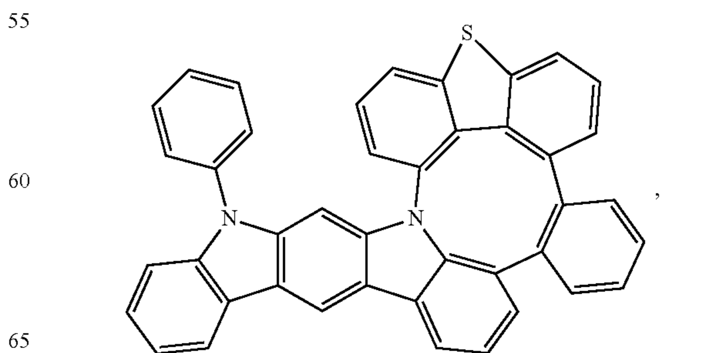
Compound 137
