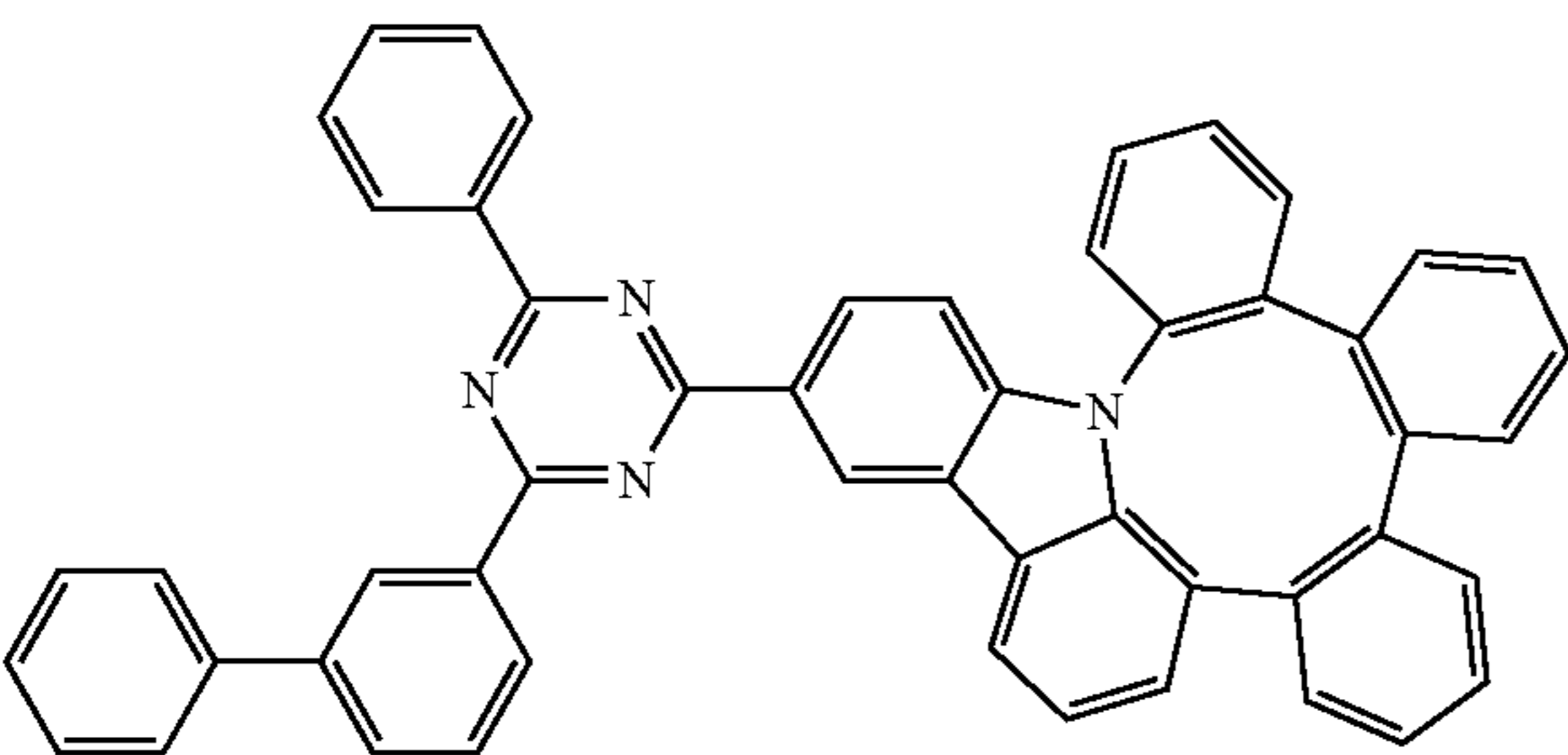
Compound 26
