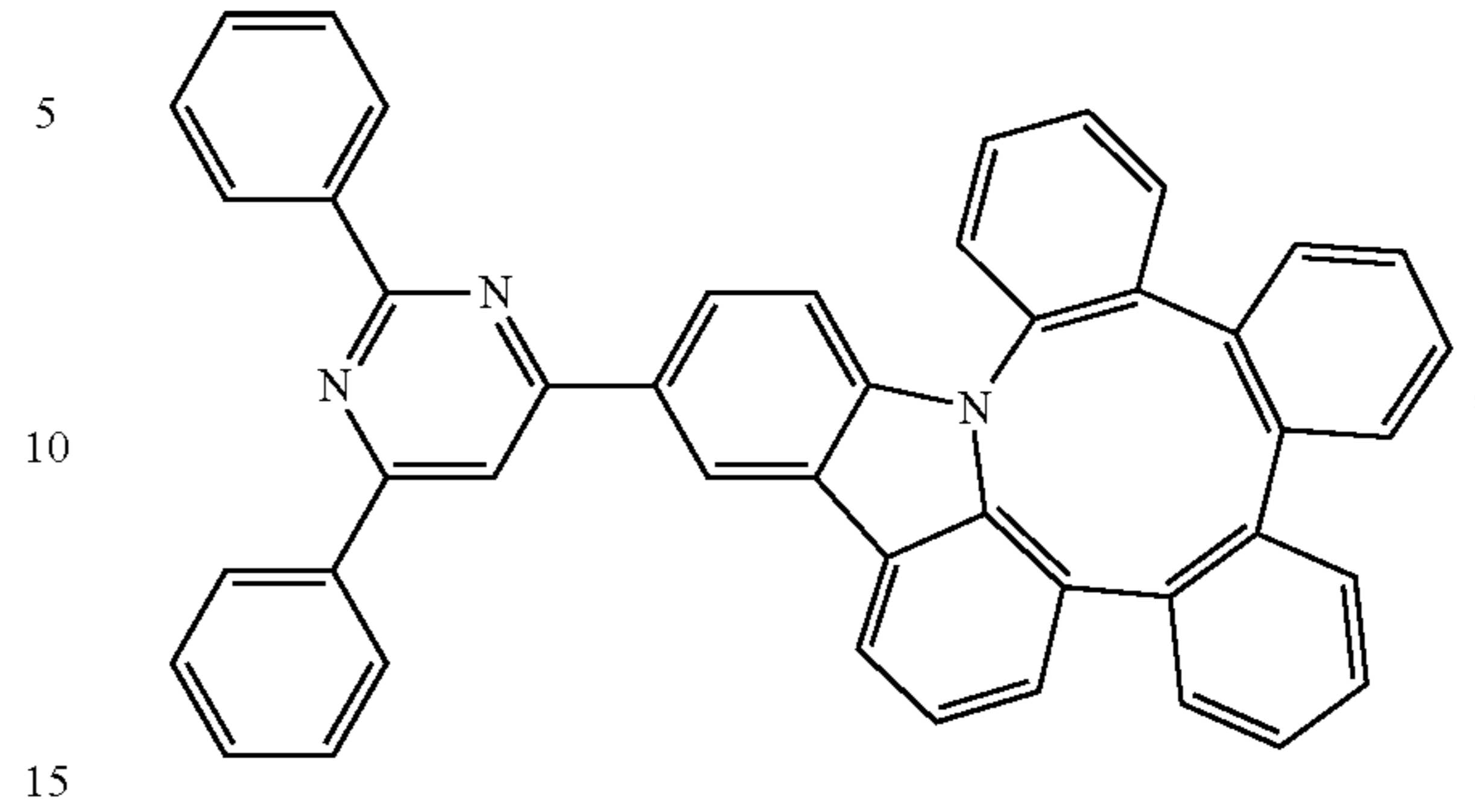
Compound 27
