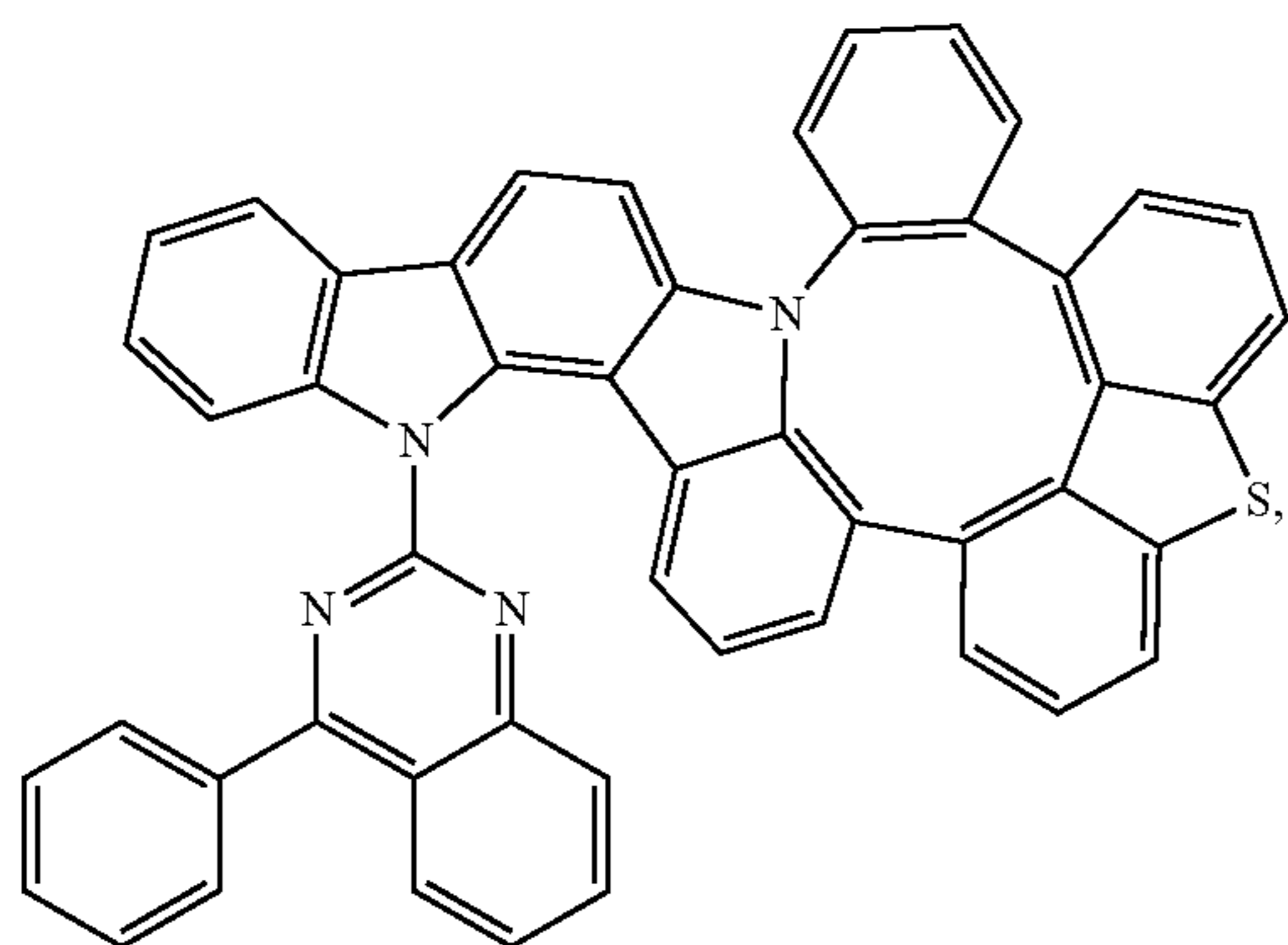
Compound 250
