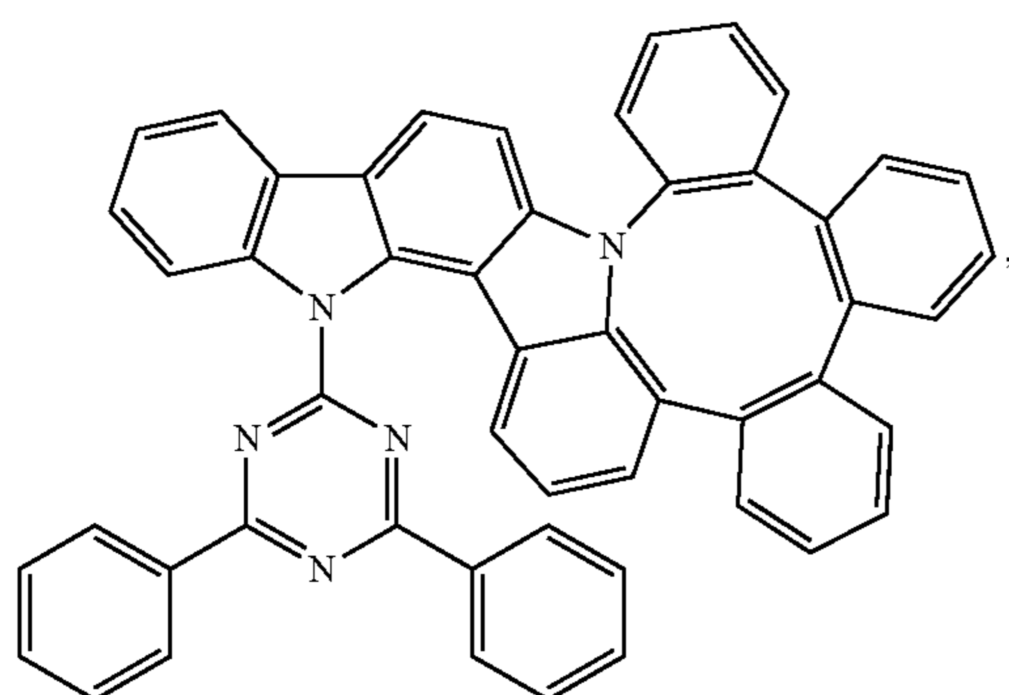
Compound 74
