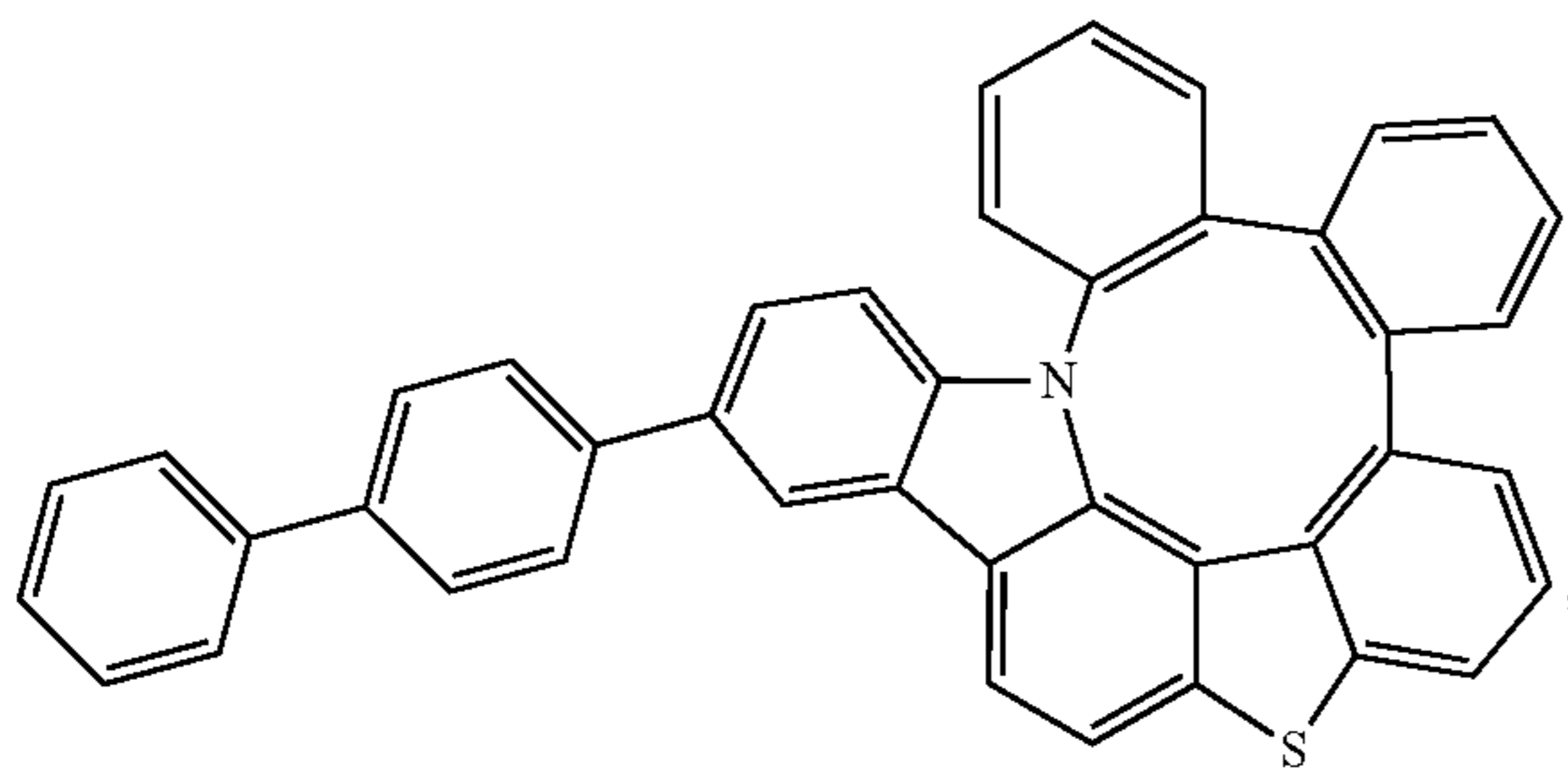
Compound 258
