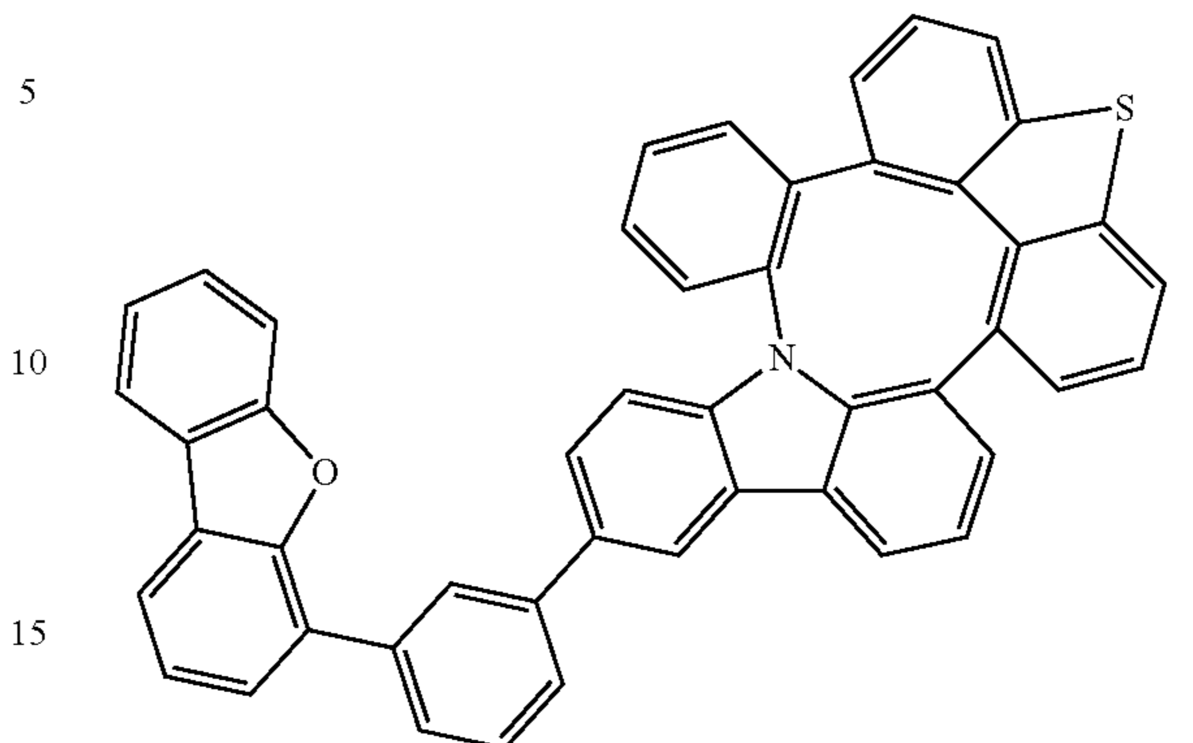
Compound 184
