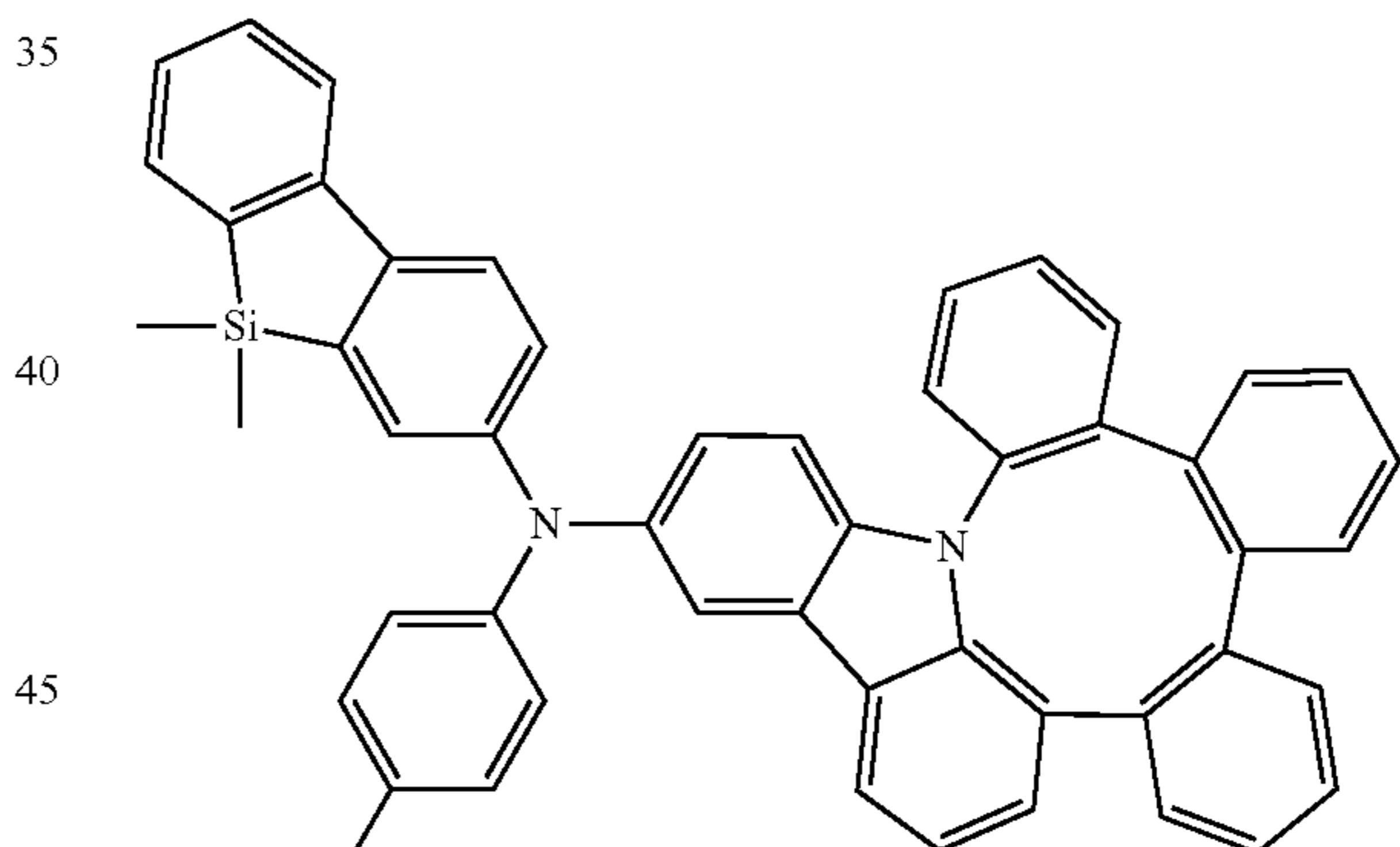
Compound 344
