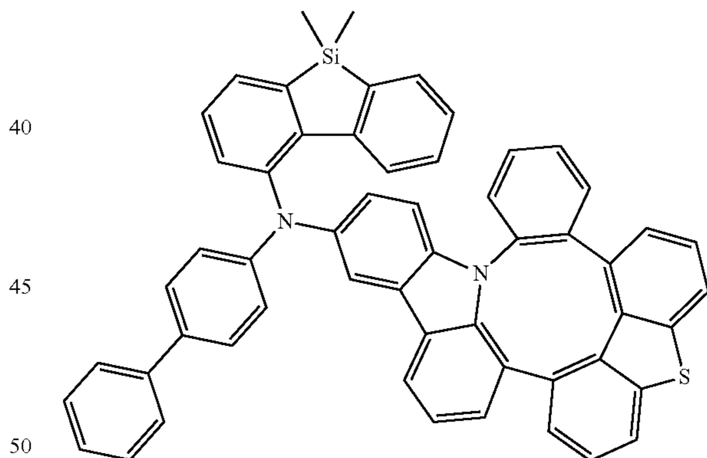
Compound 361
