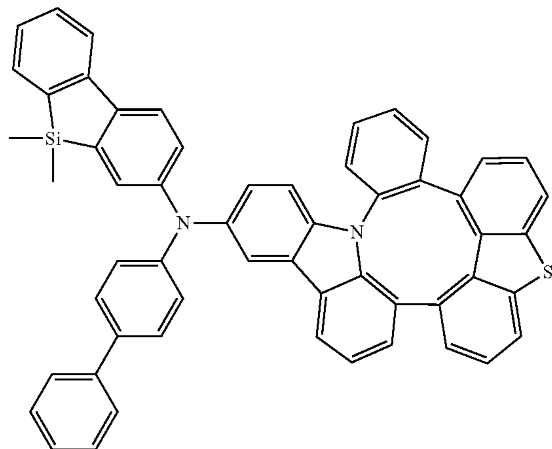
Compound 359
