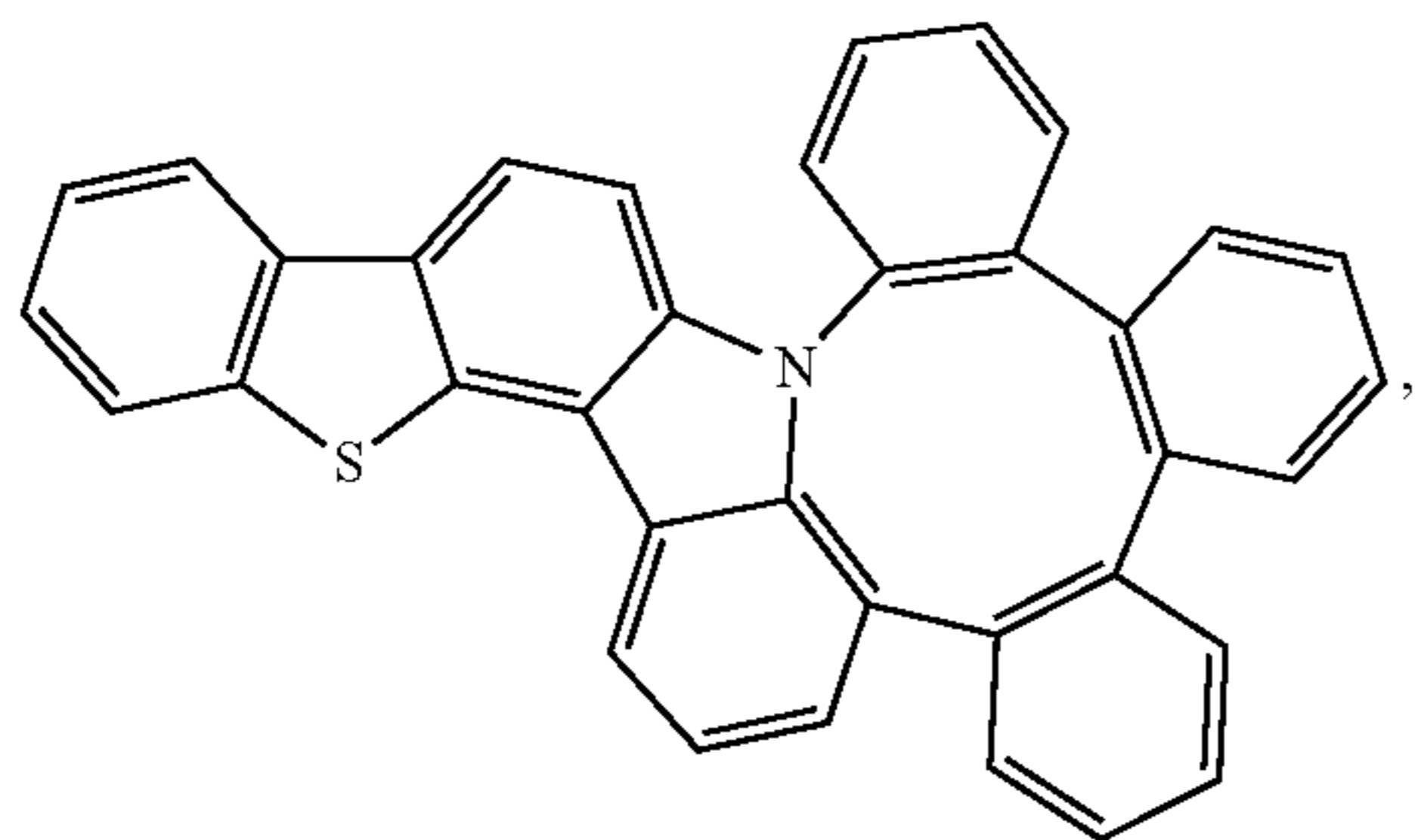
Compound 63
