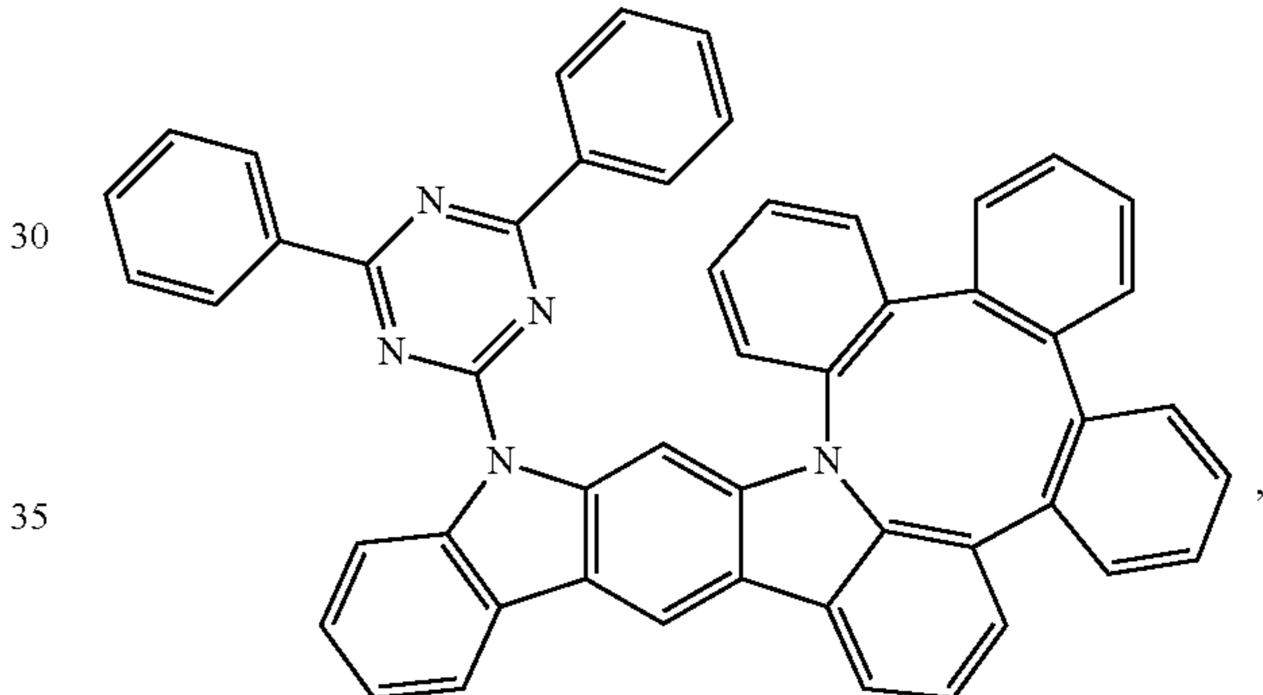
Compound 76
