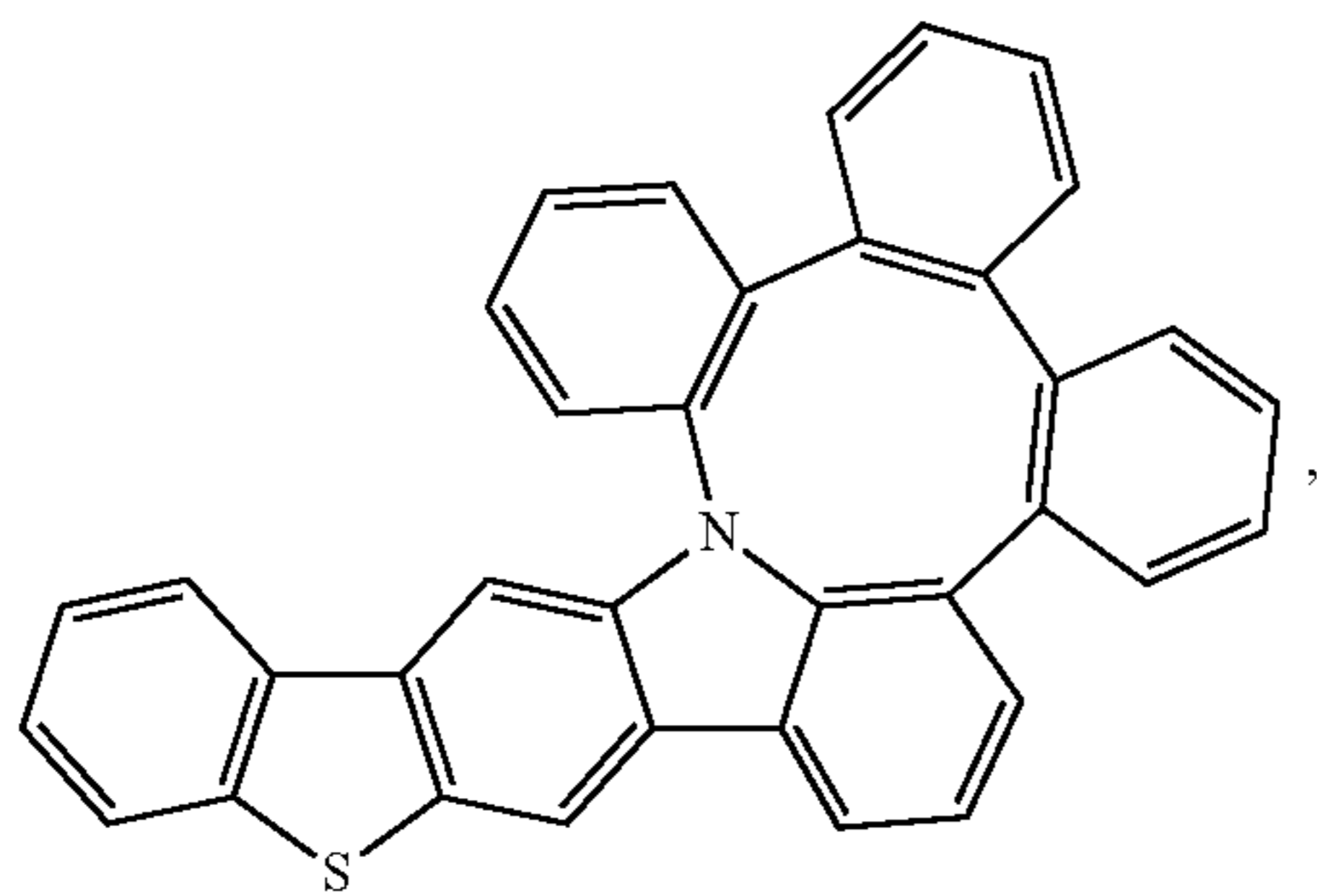
Compound 66
