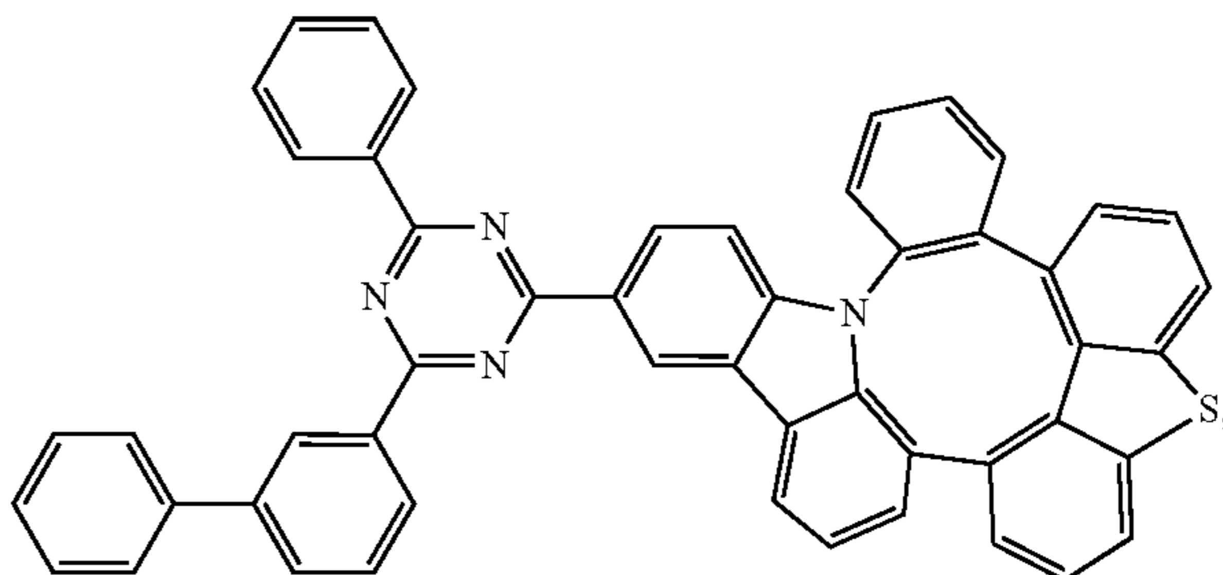
Compound 196
