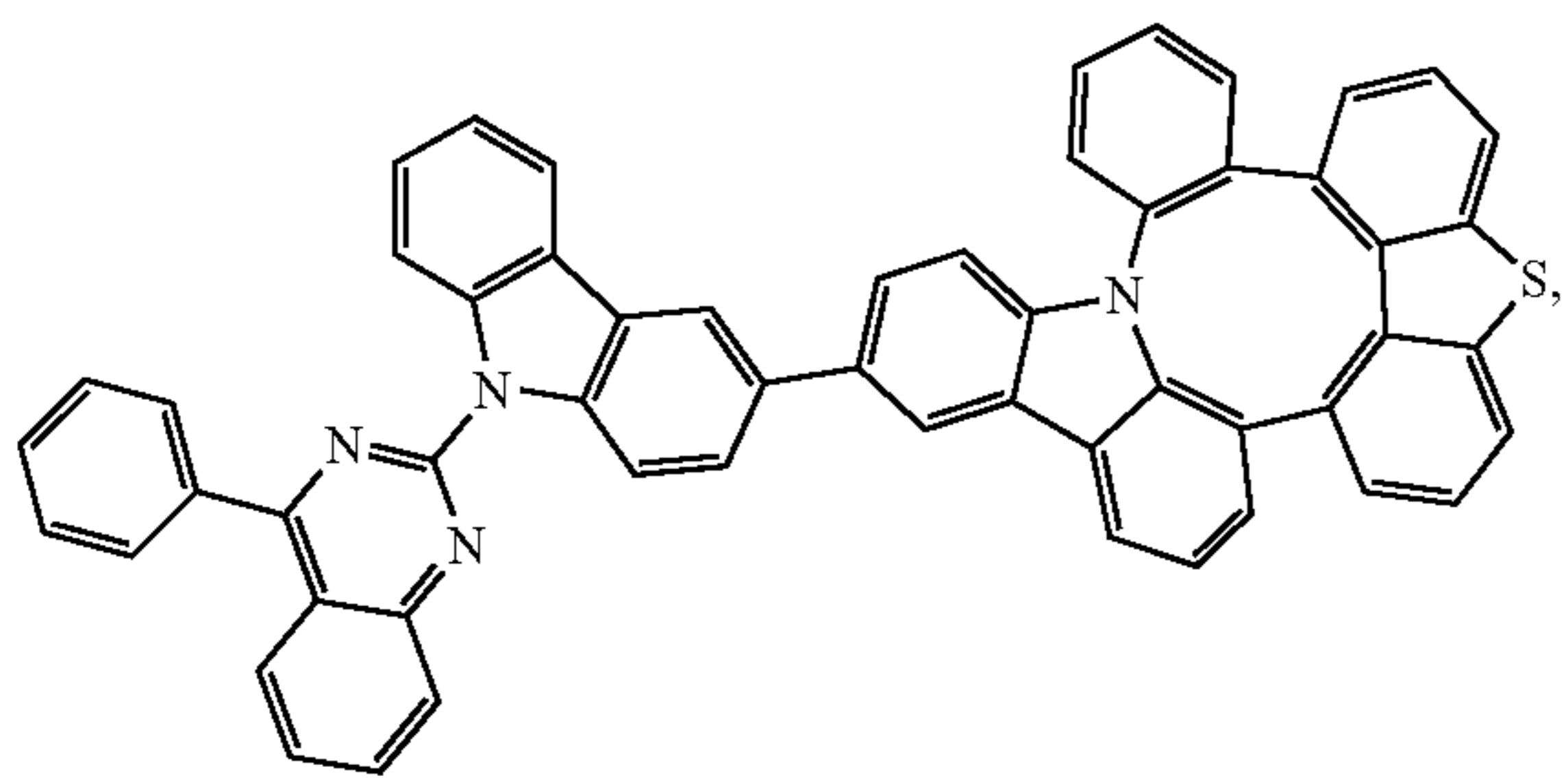
Compound 190
