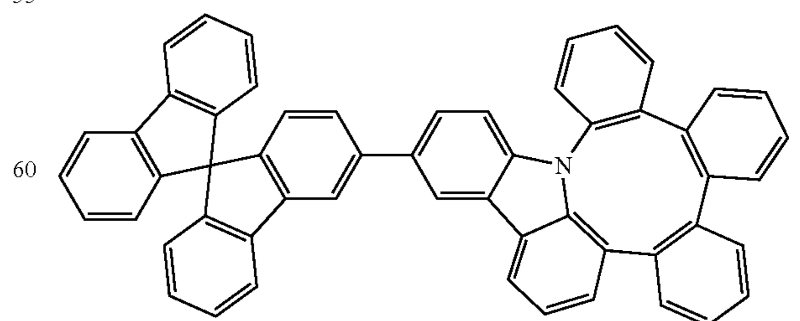
Compound 22
