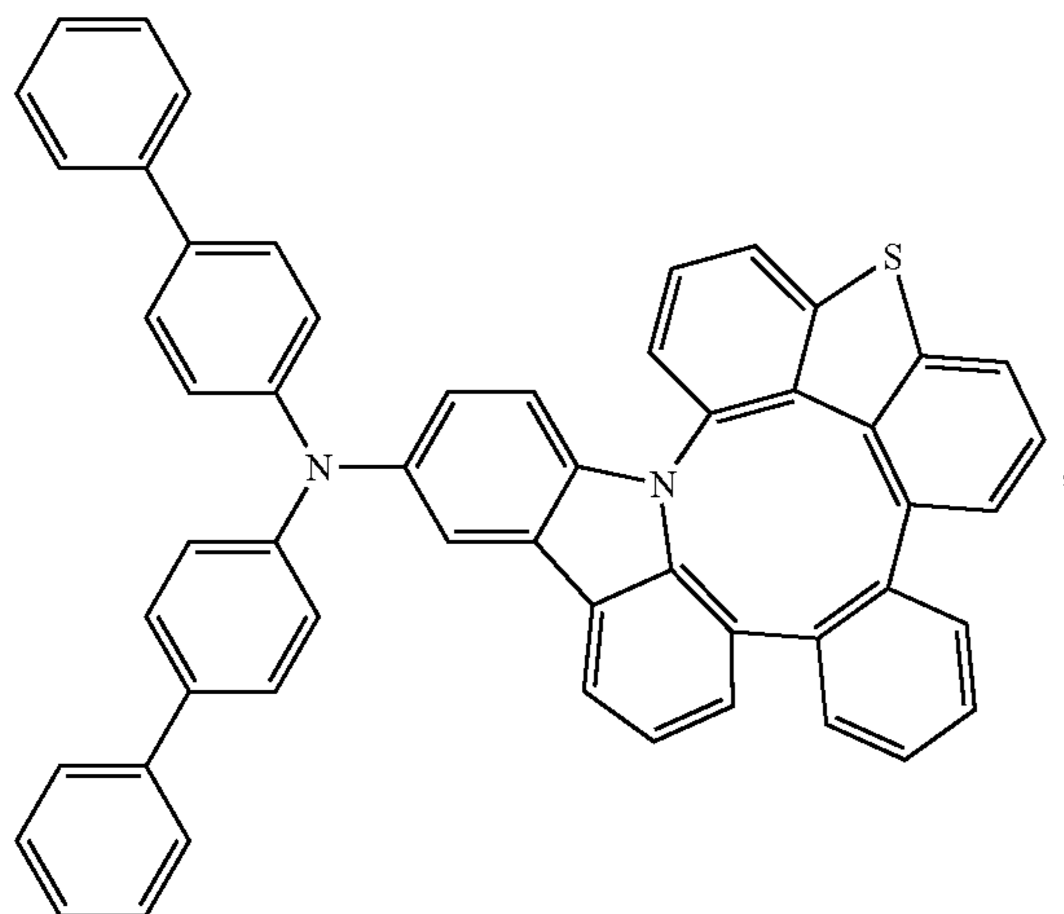
Compound 126
