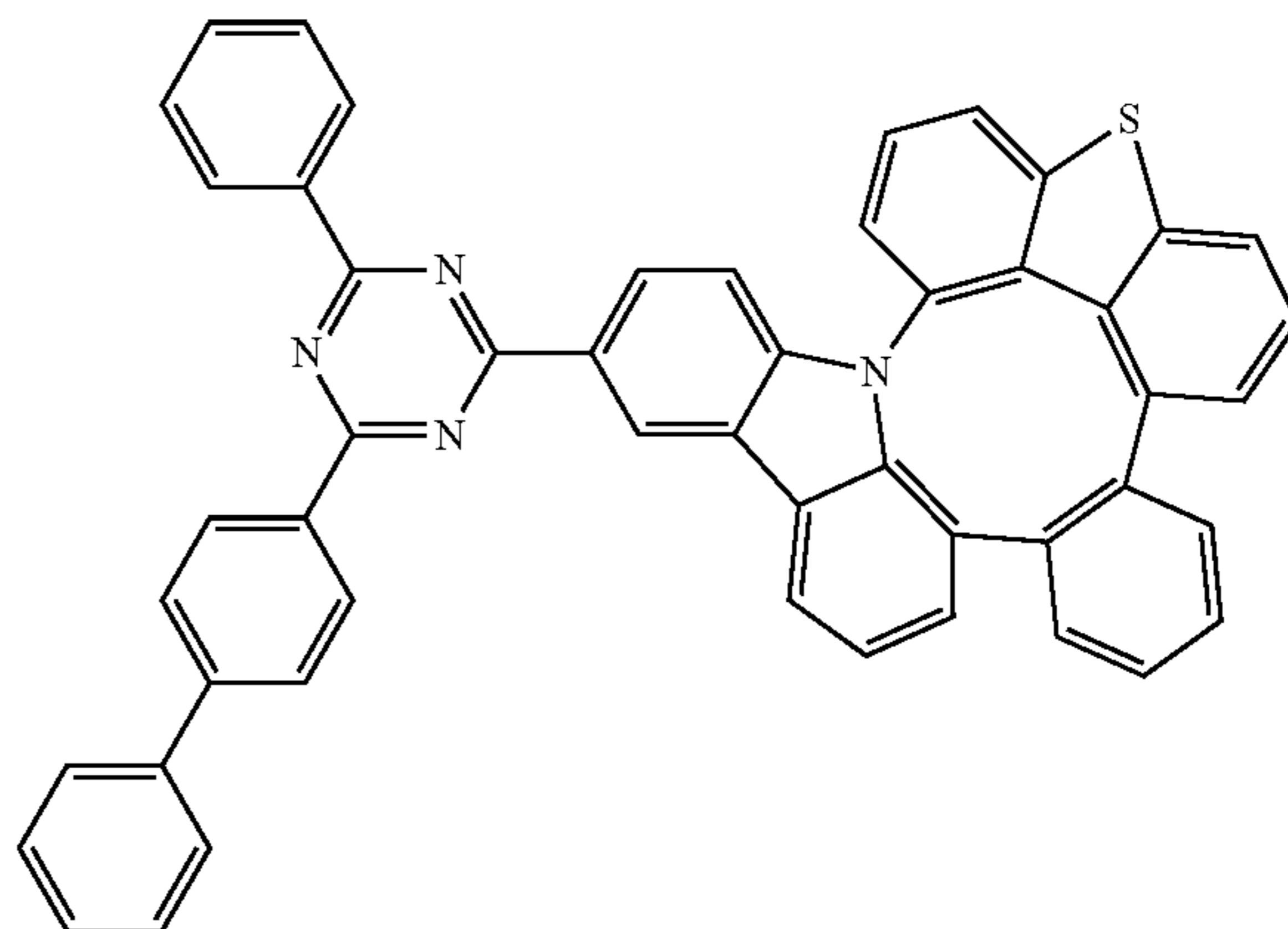
Compound 110
