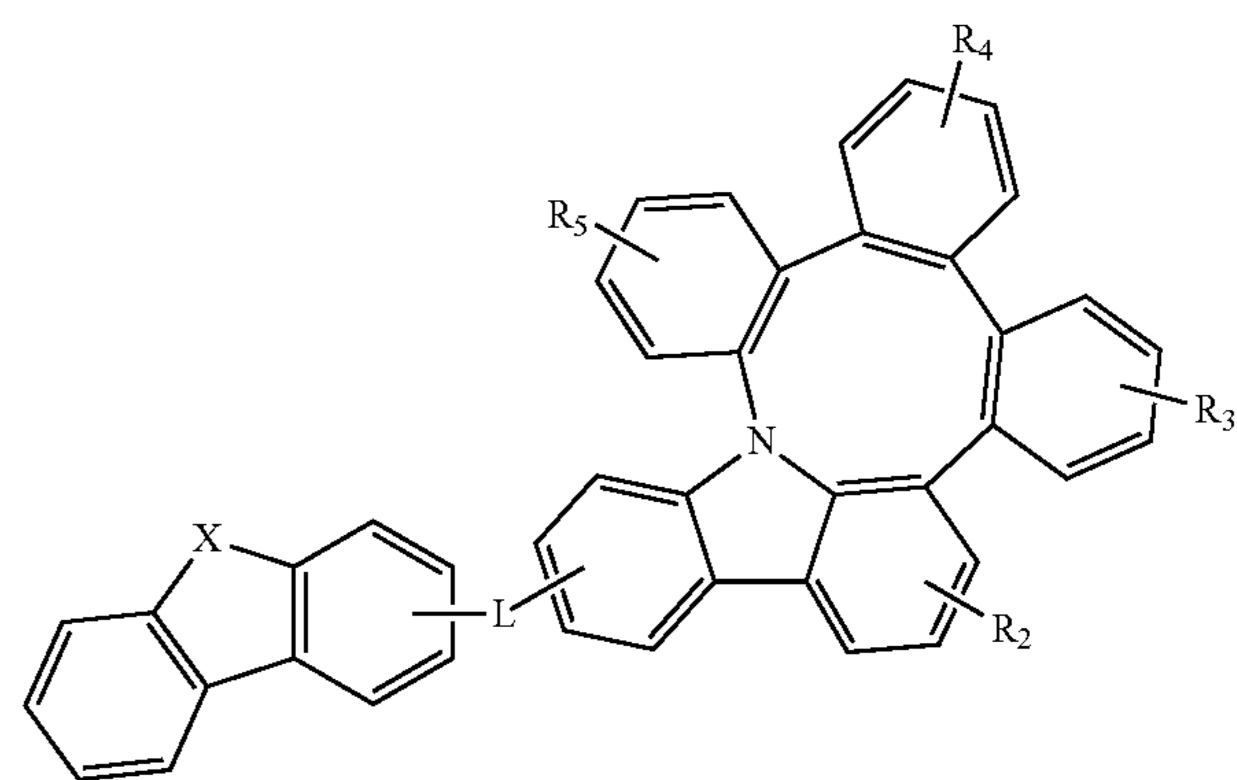
Formula 3
