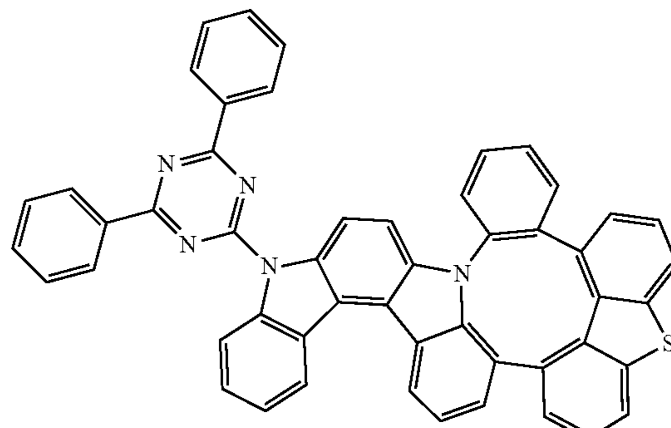
Compound 246
