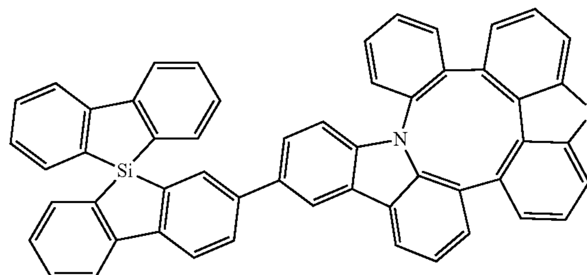
Compound 355
