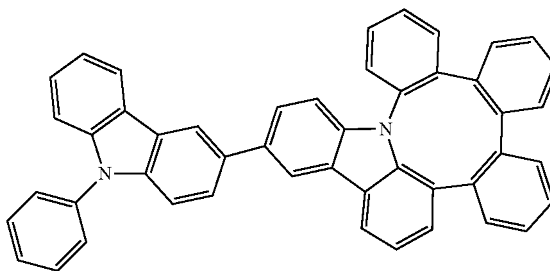
Compound 16
