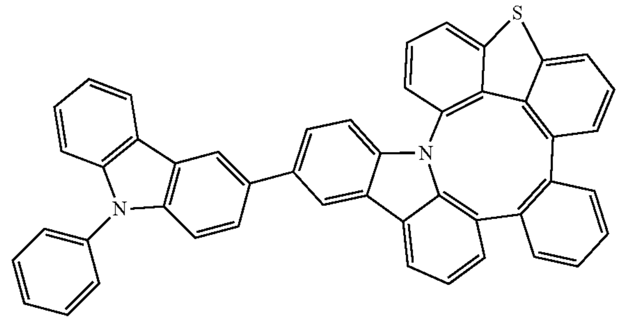
Compound 101
