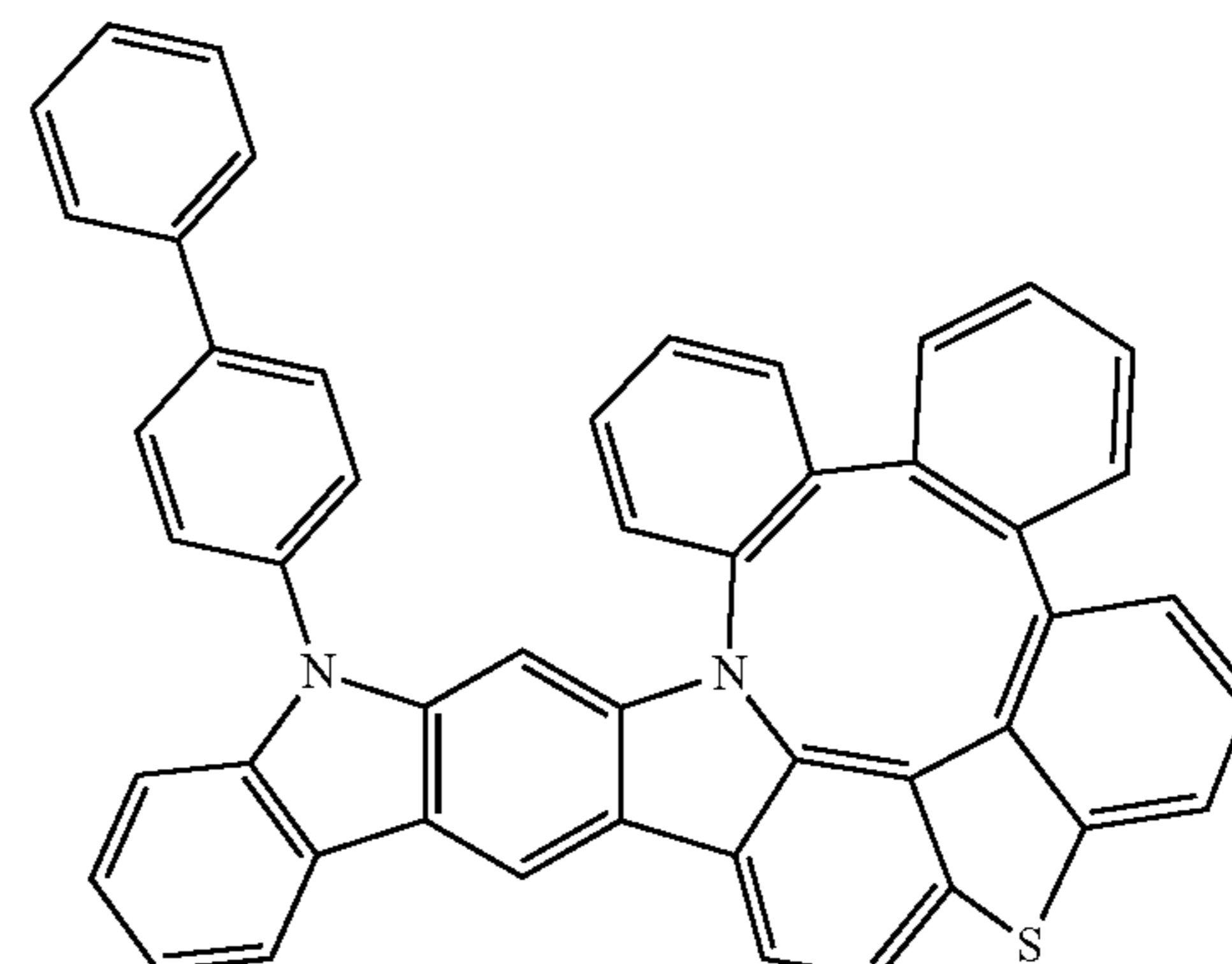
Compound 313
