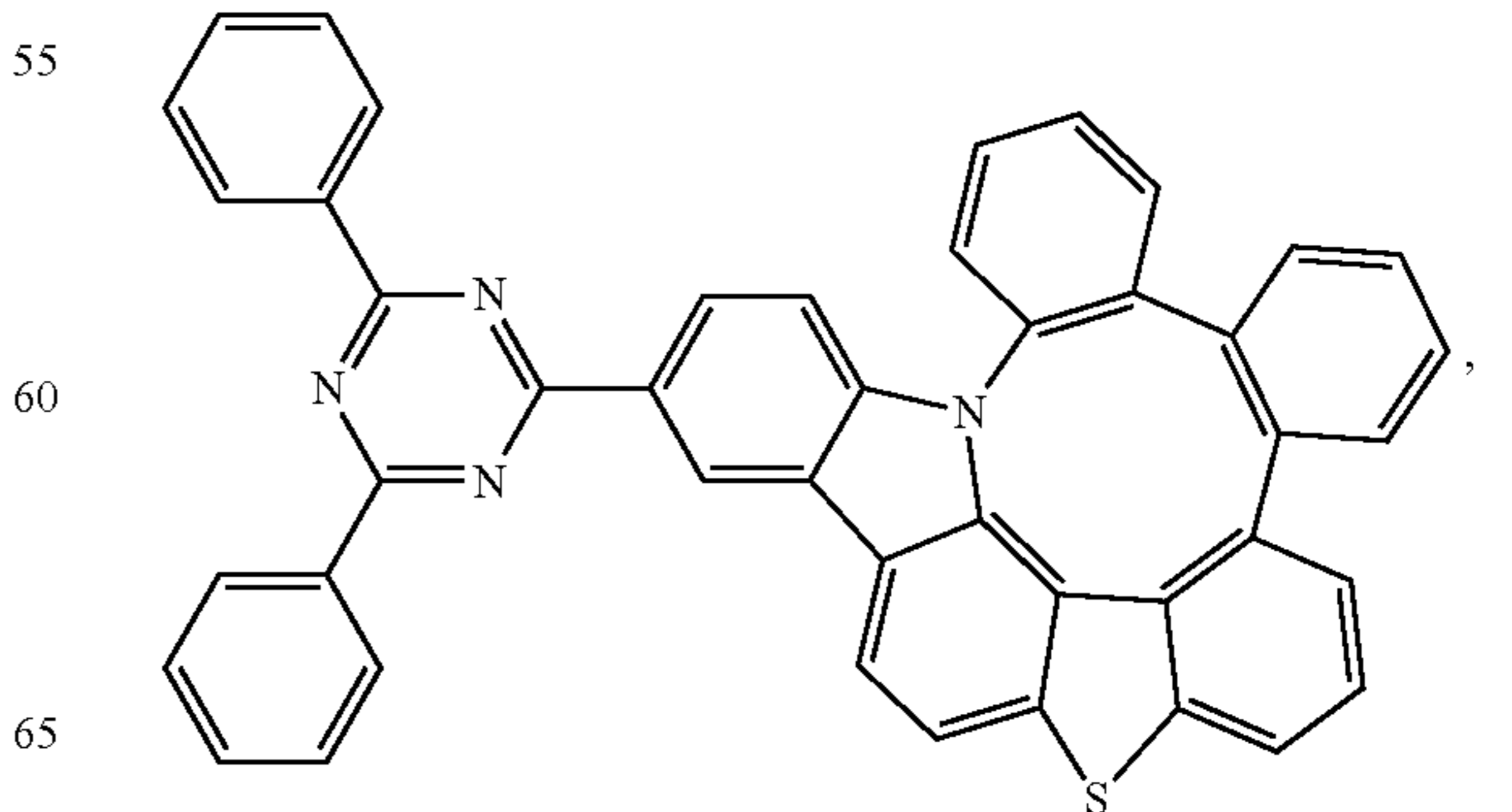
Compound 279
