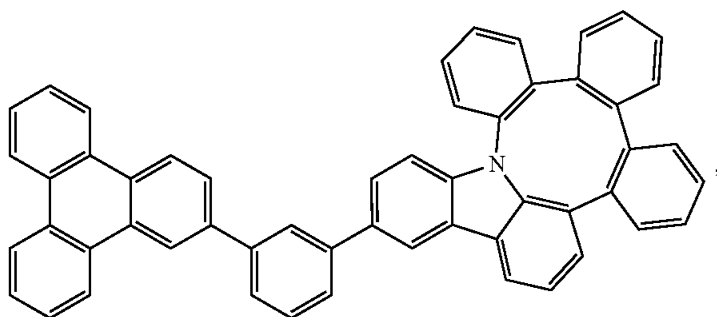
Compound 34
