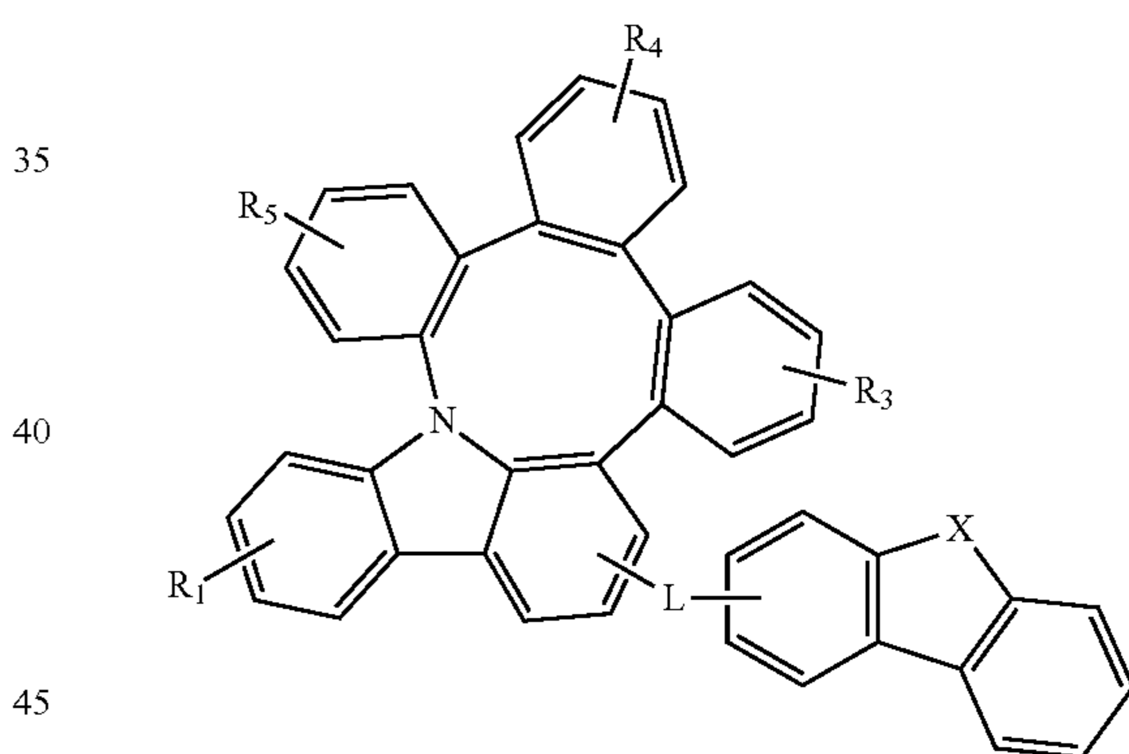
Formula 6
