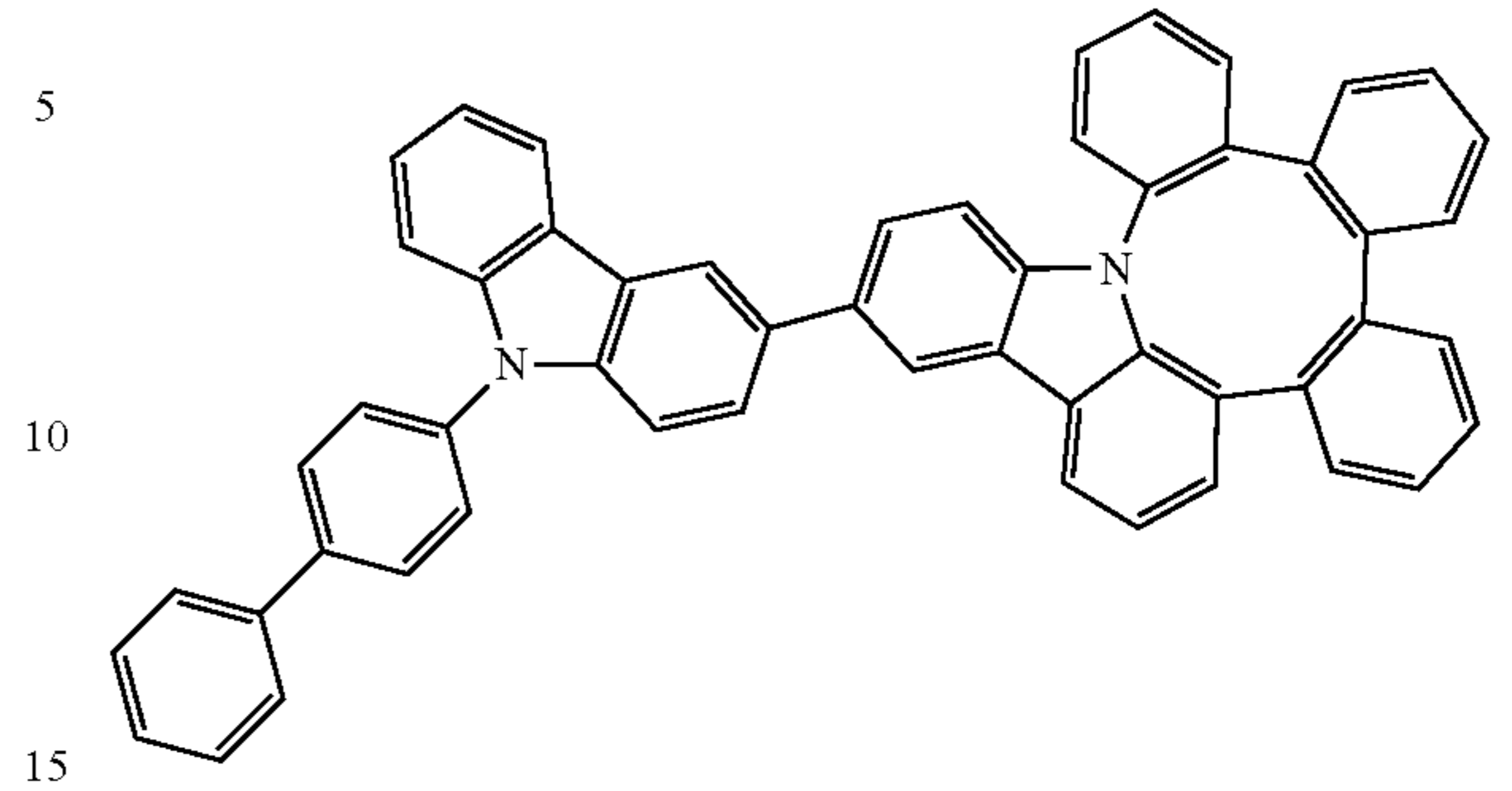
Compound 19
