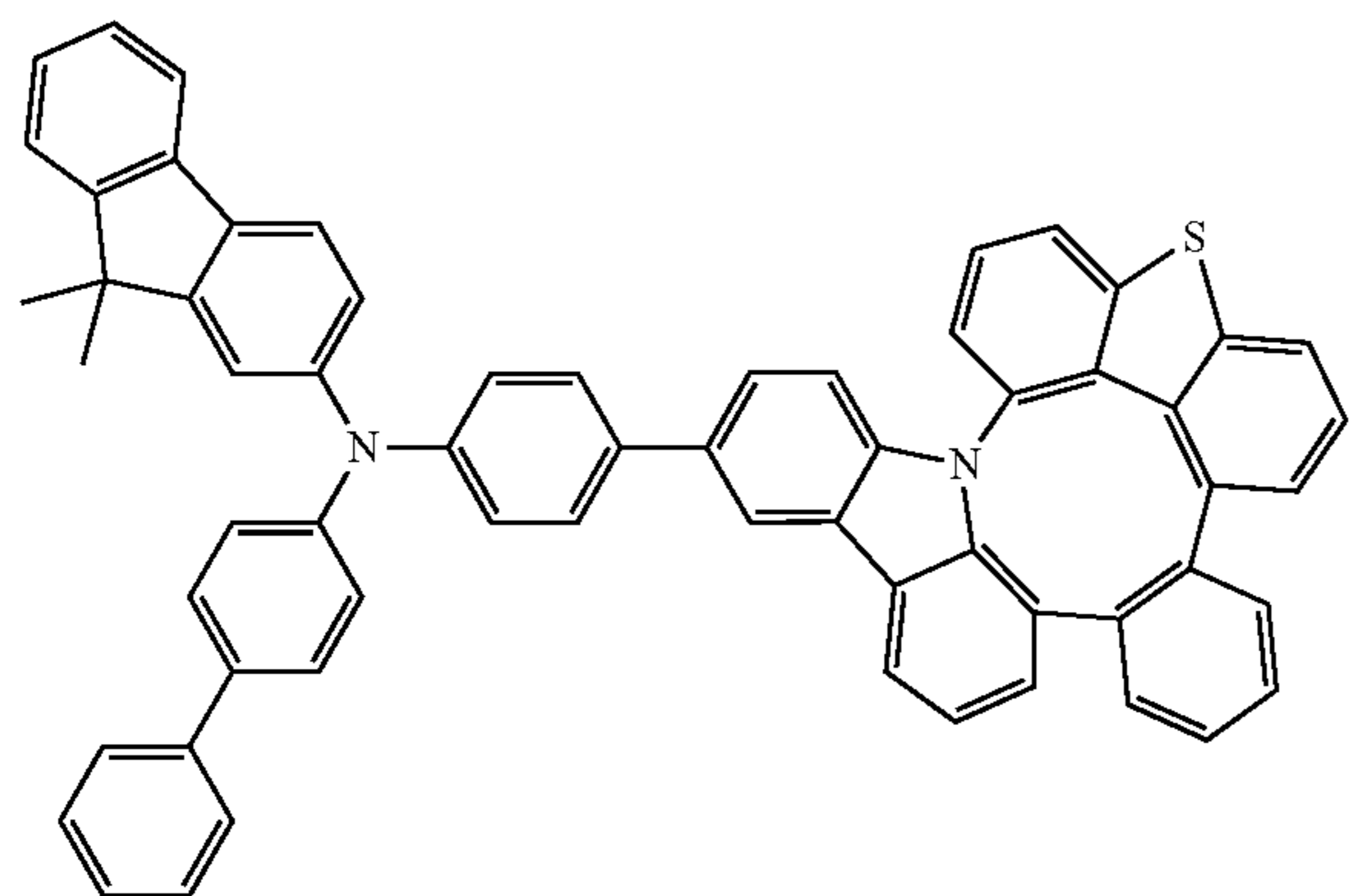
Compound 133
