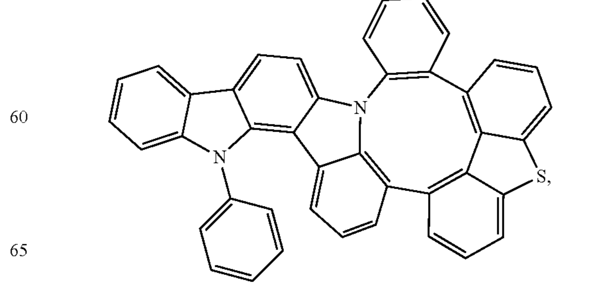
Compound 220
