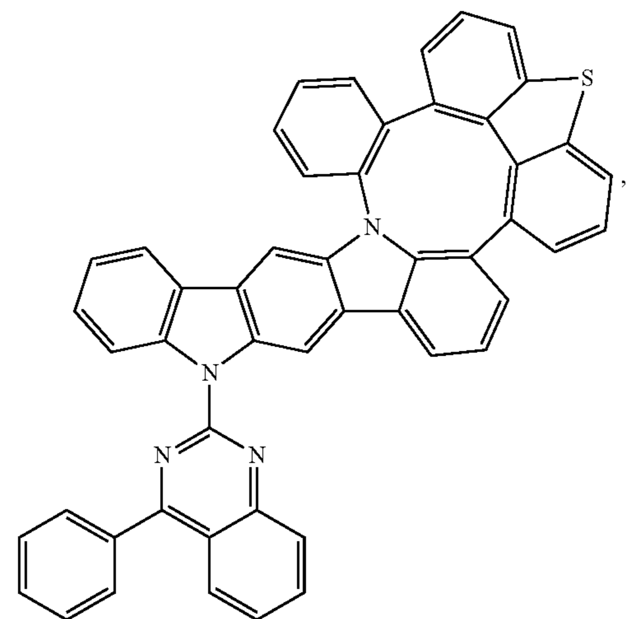
Compound 254
