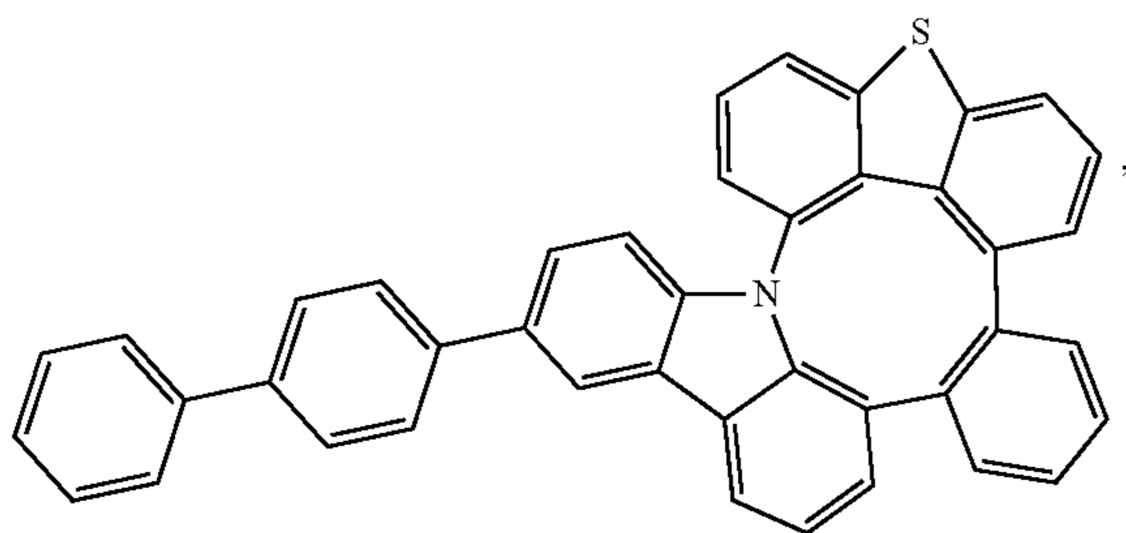
Compound 87
