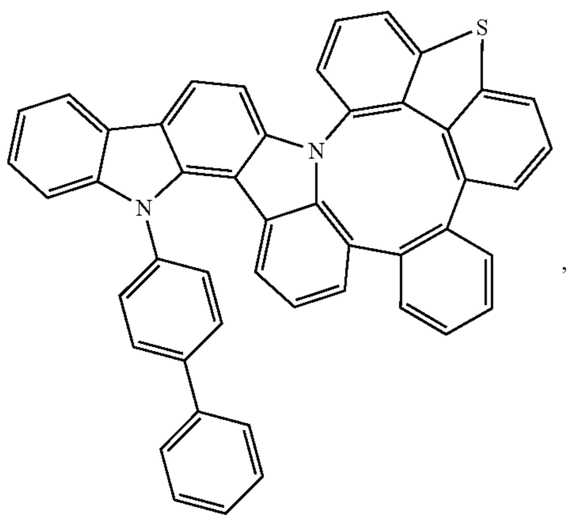
Compound 141
