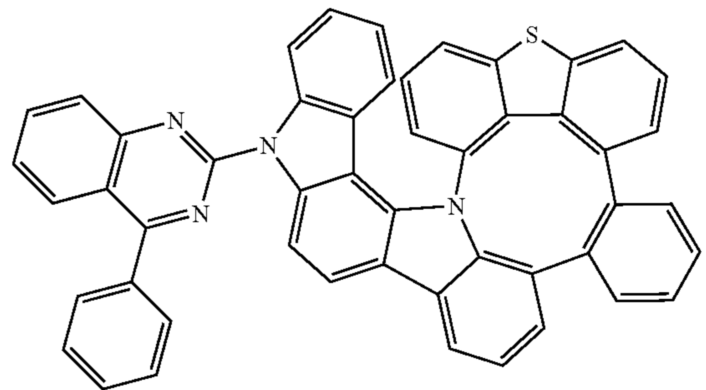
Compound 170
