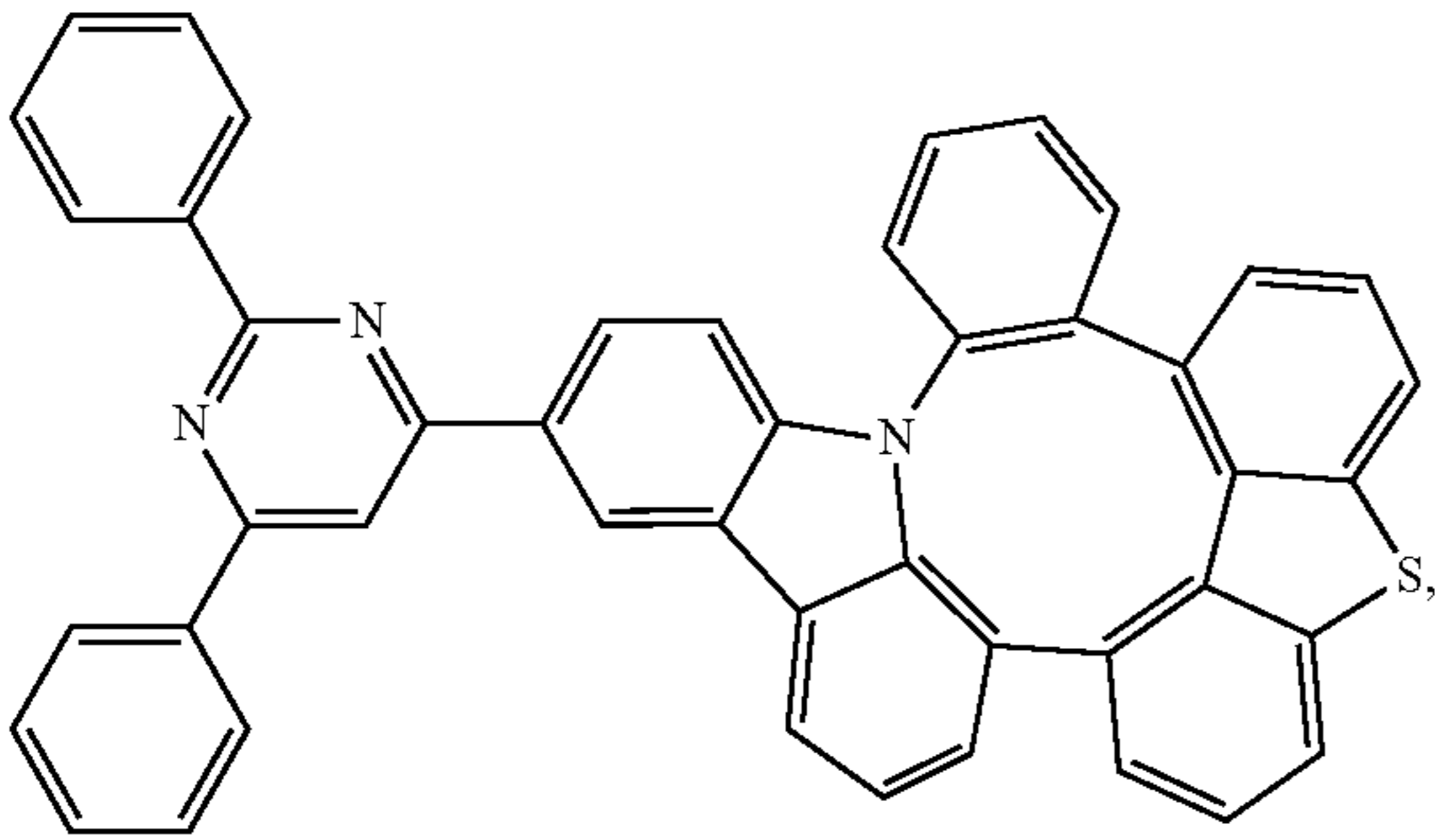
Compound 197
