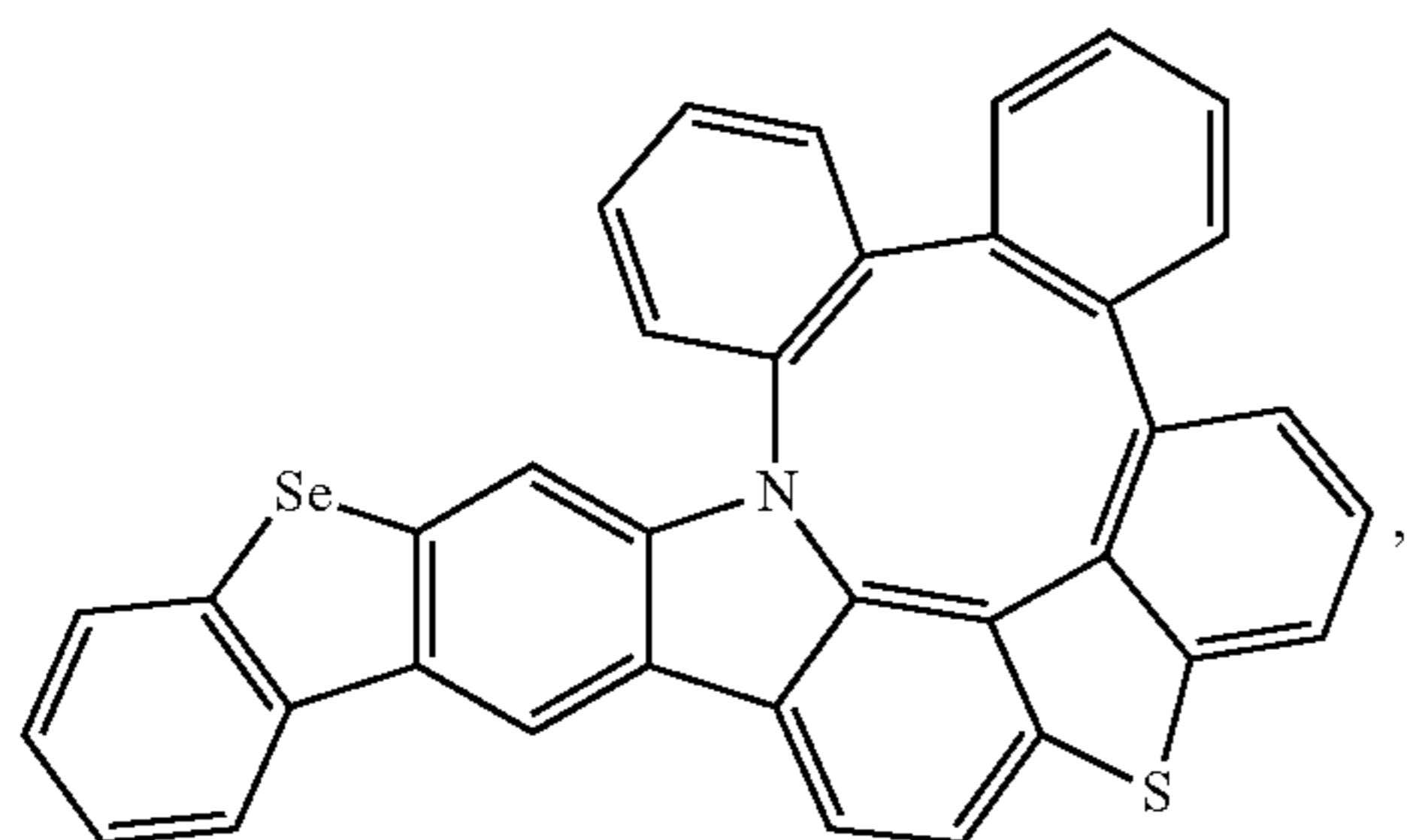
Compound 326
