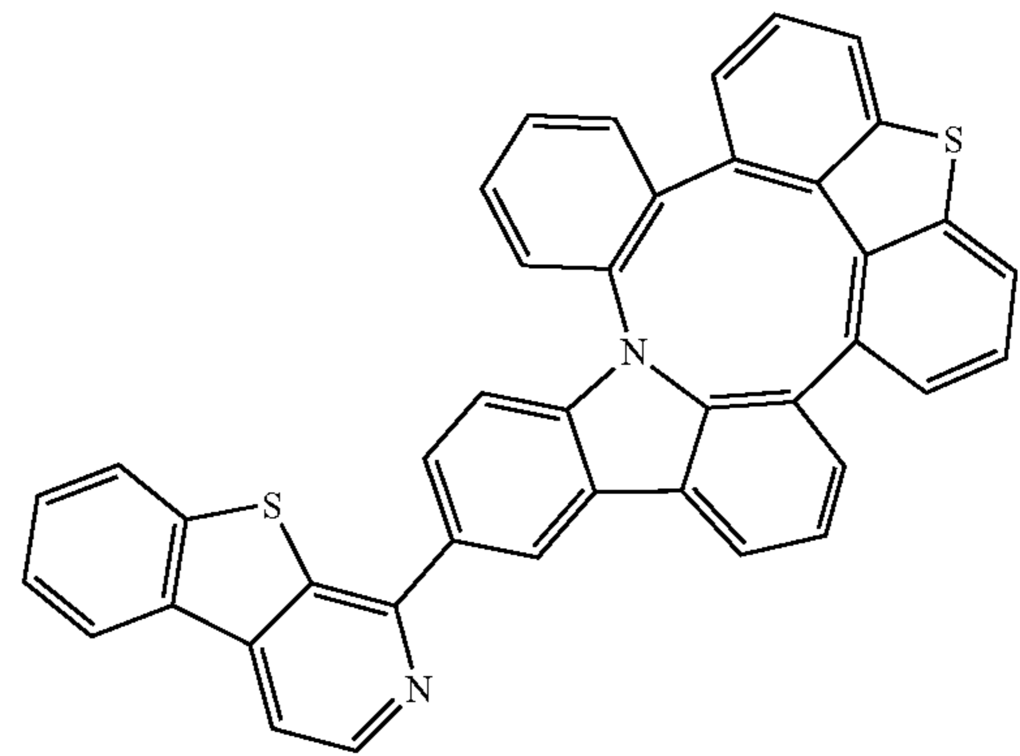
Compound 202
