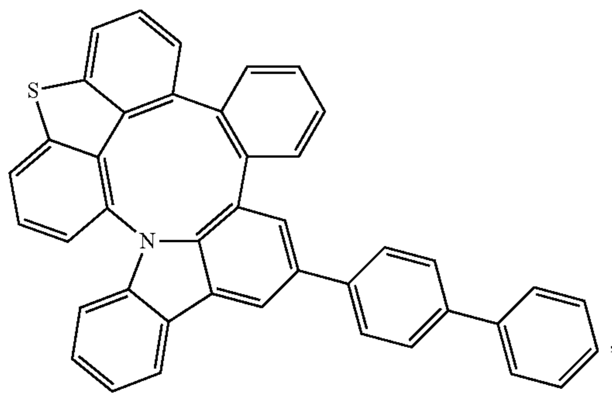
Compound 88
