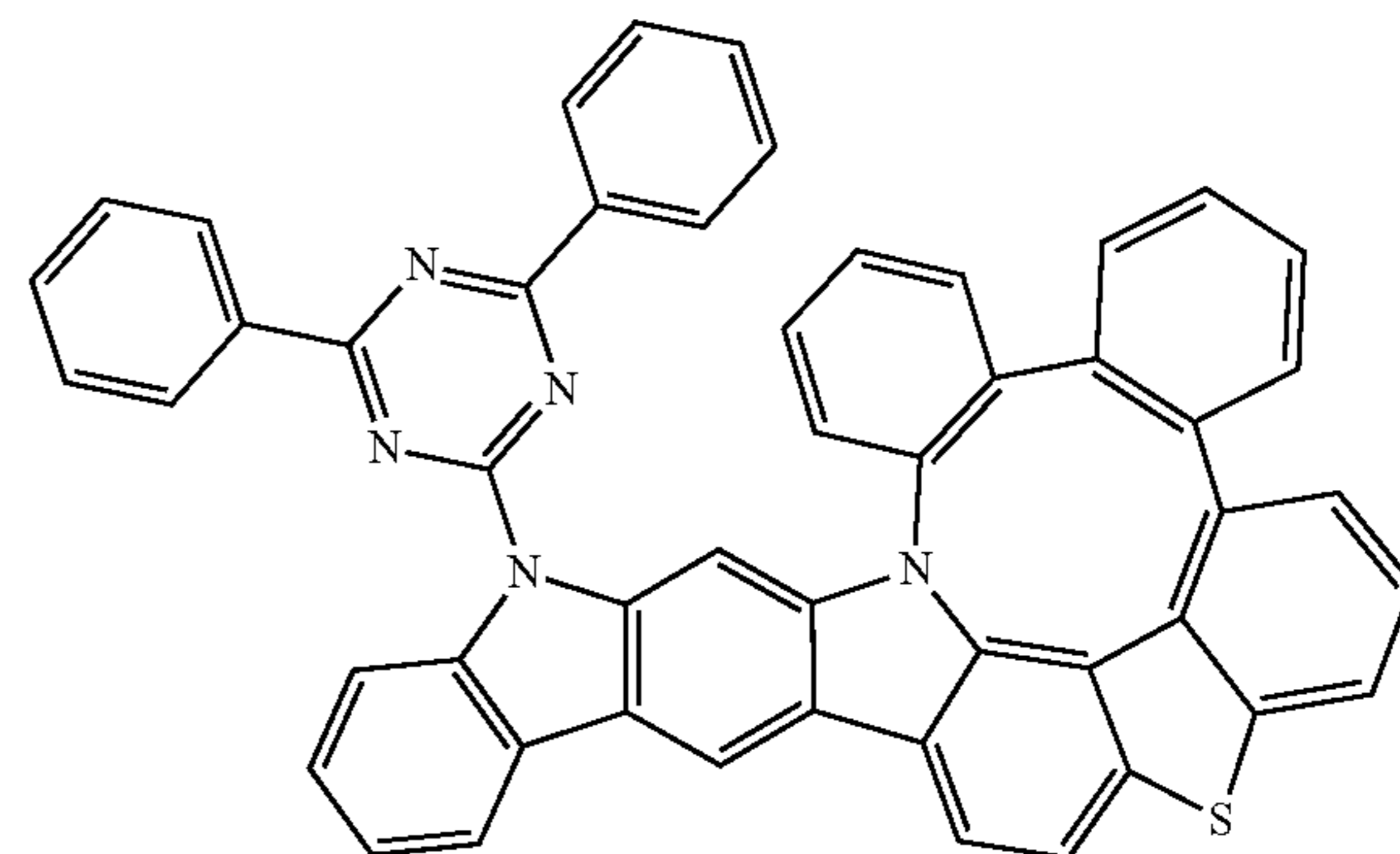
Compound 331
