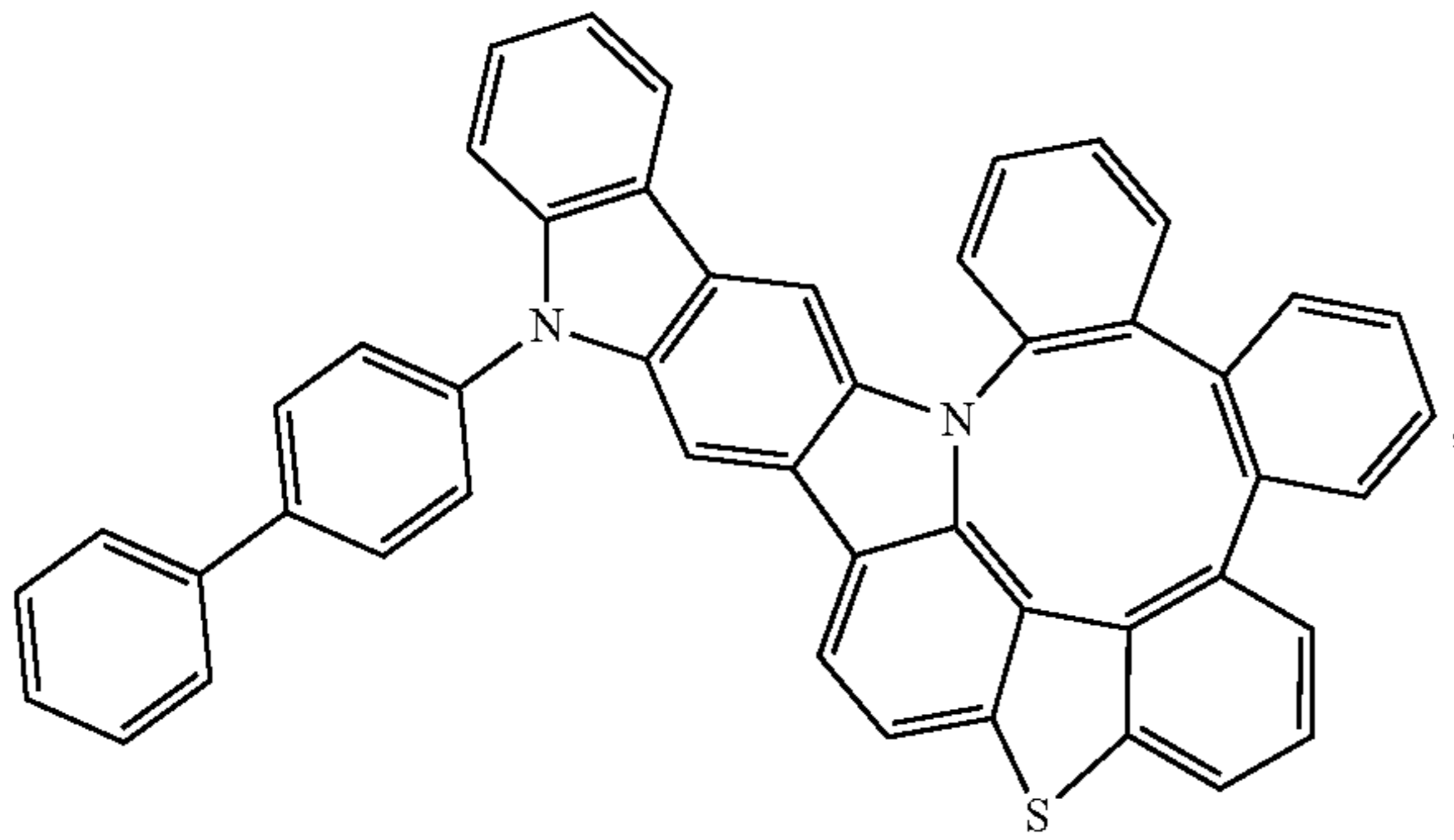
Compound 314
