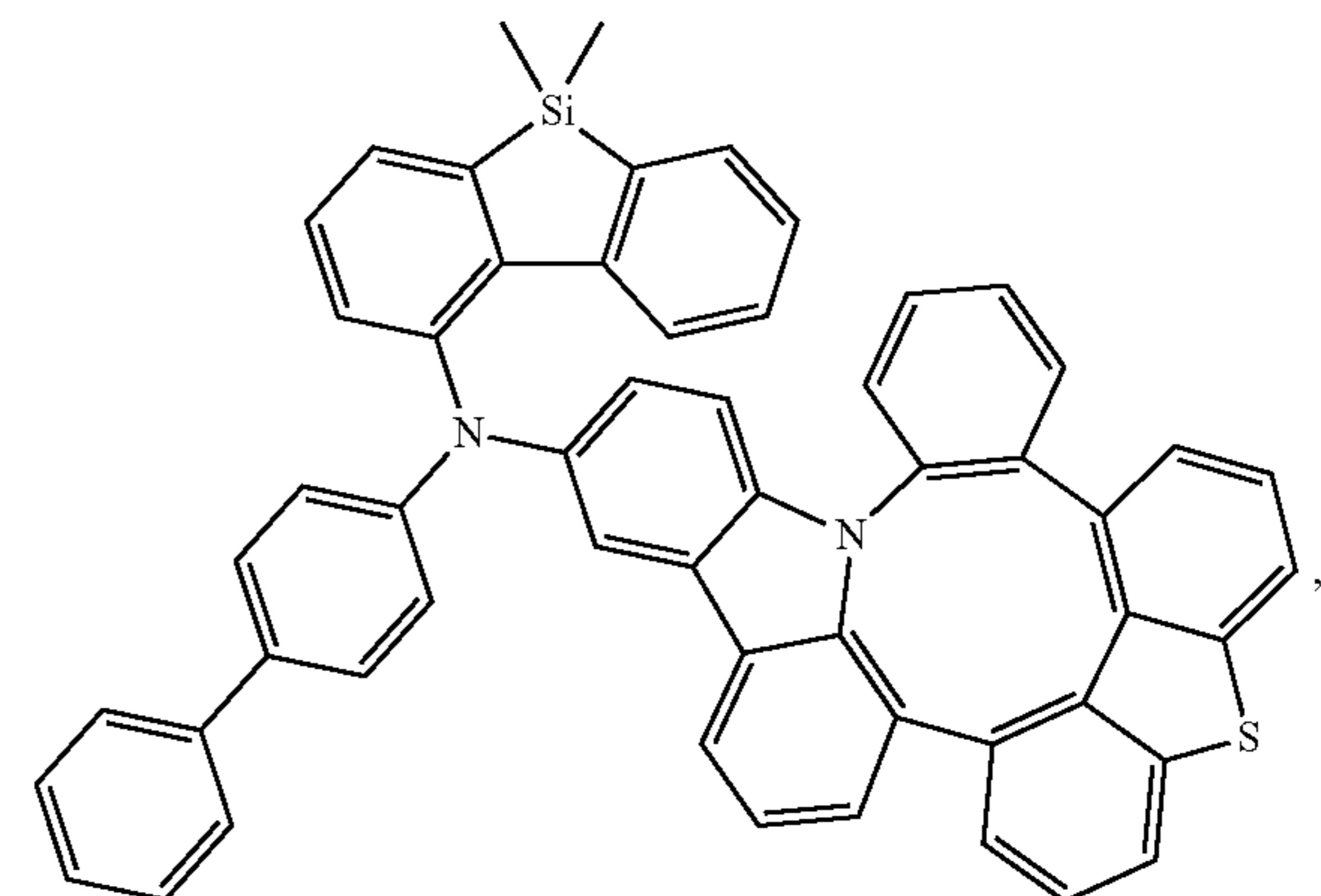
Compound 361
