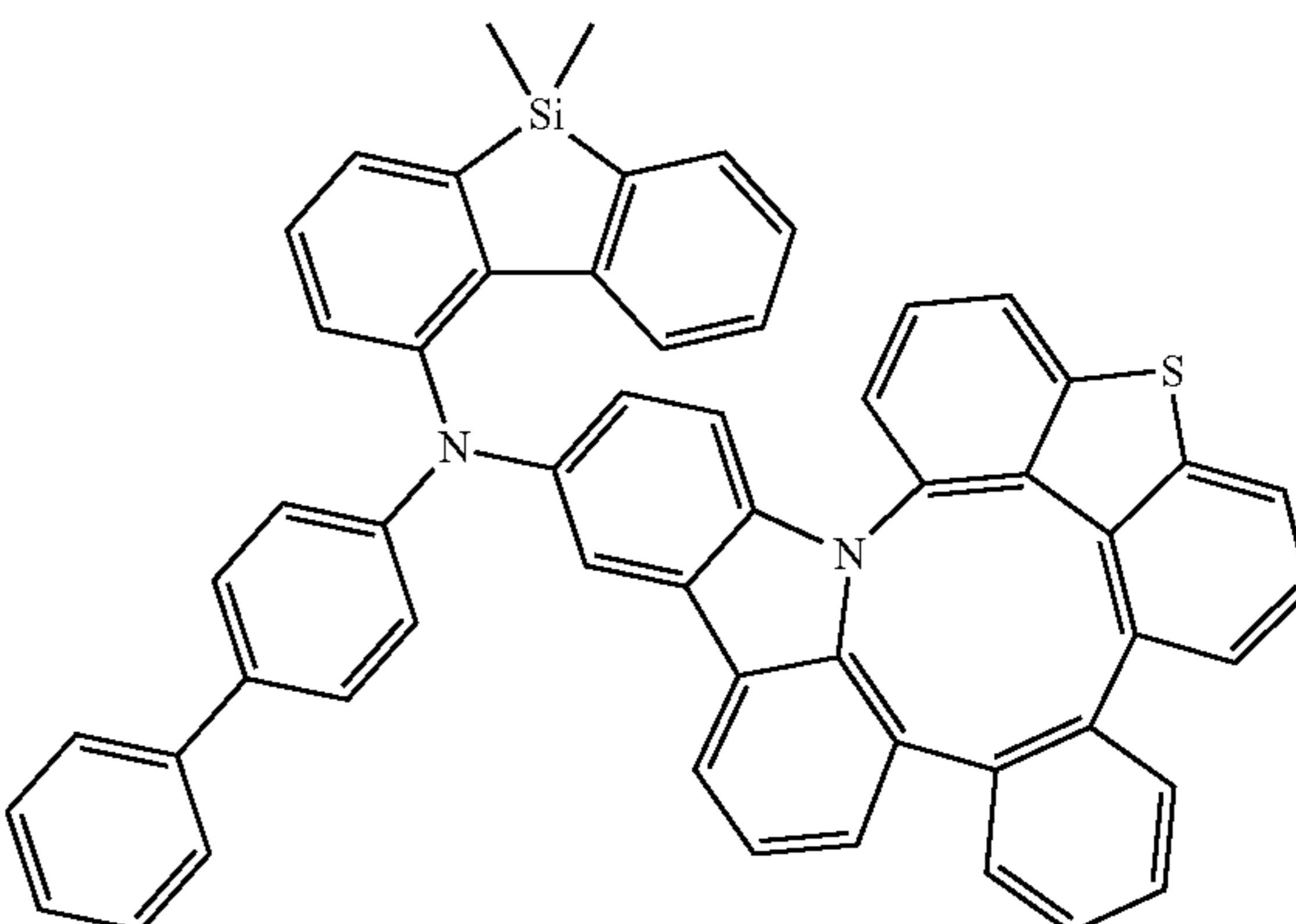
Compound 353
