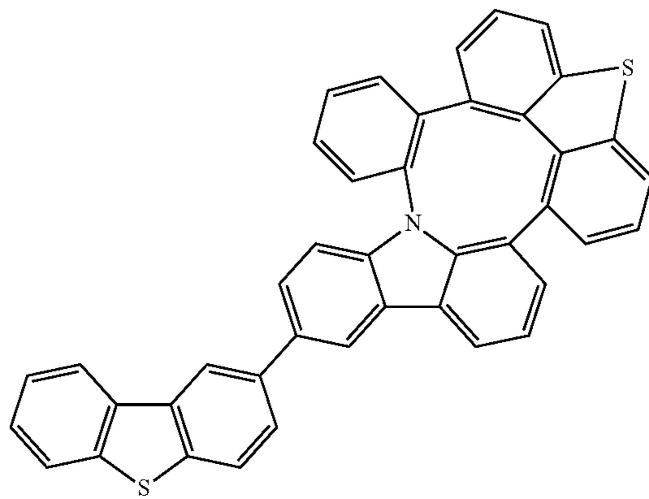
Compound 178
