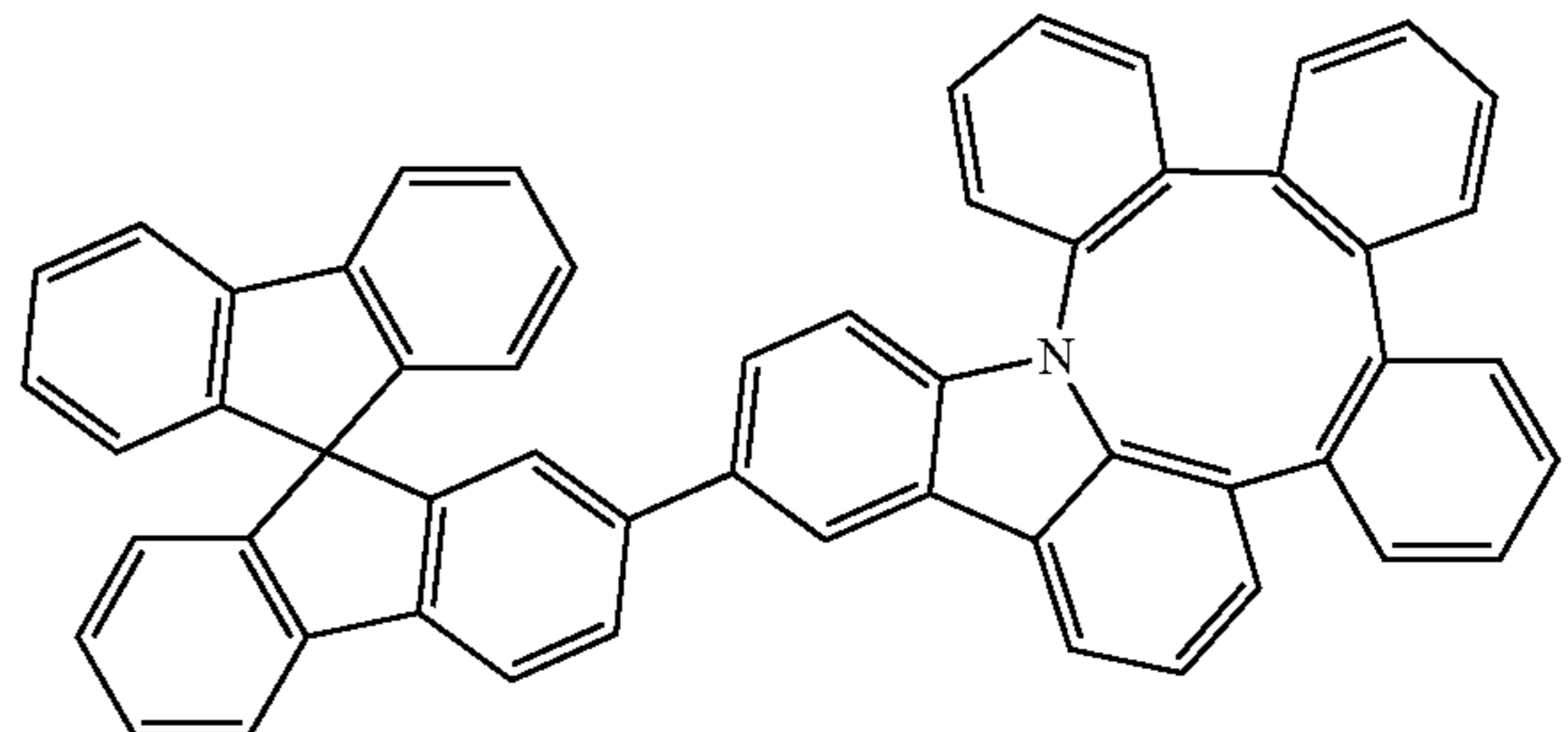
Compound 22
