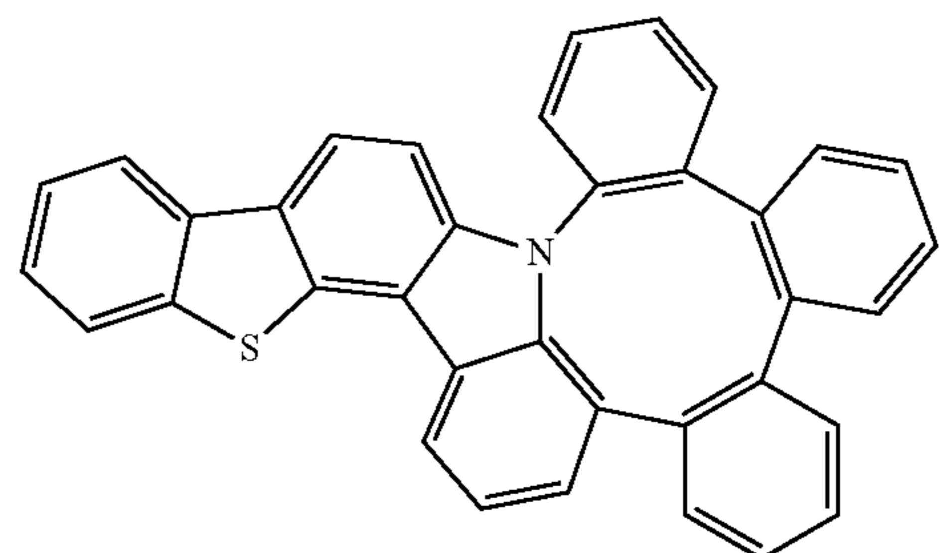
Compound 62
