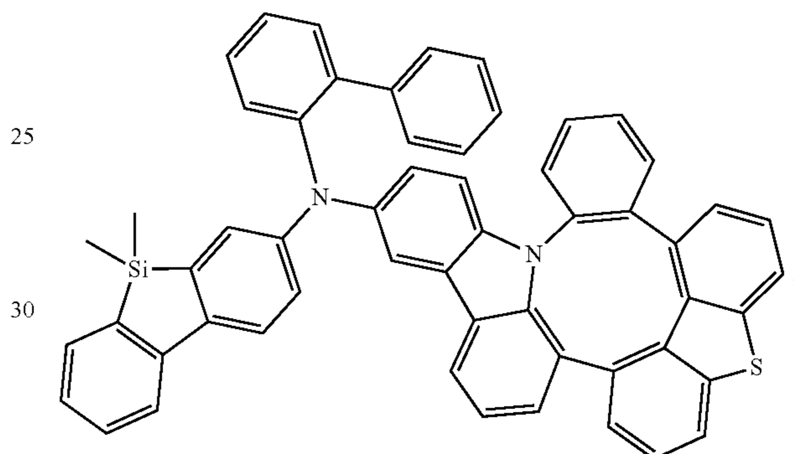
Compound 360
