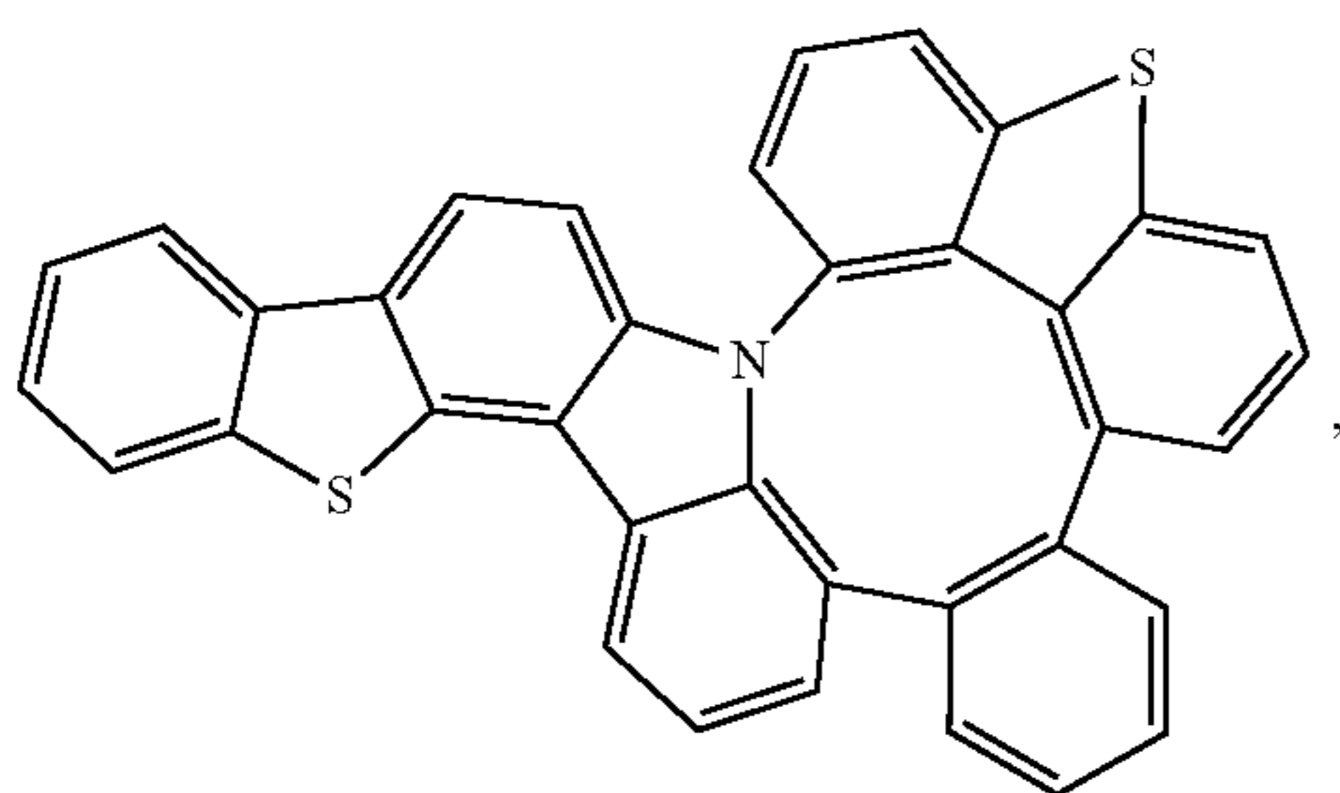
Compound 148
