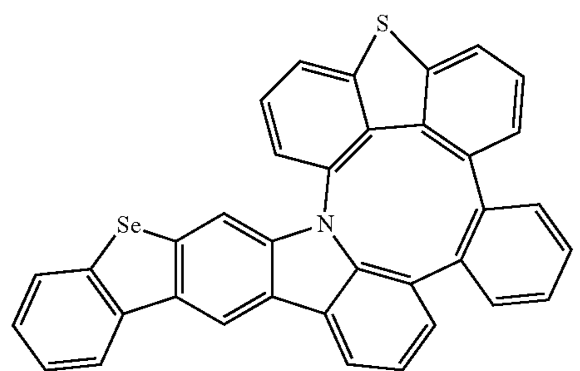
Compound 155
