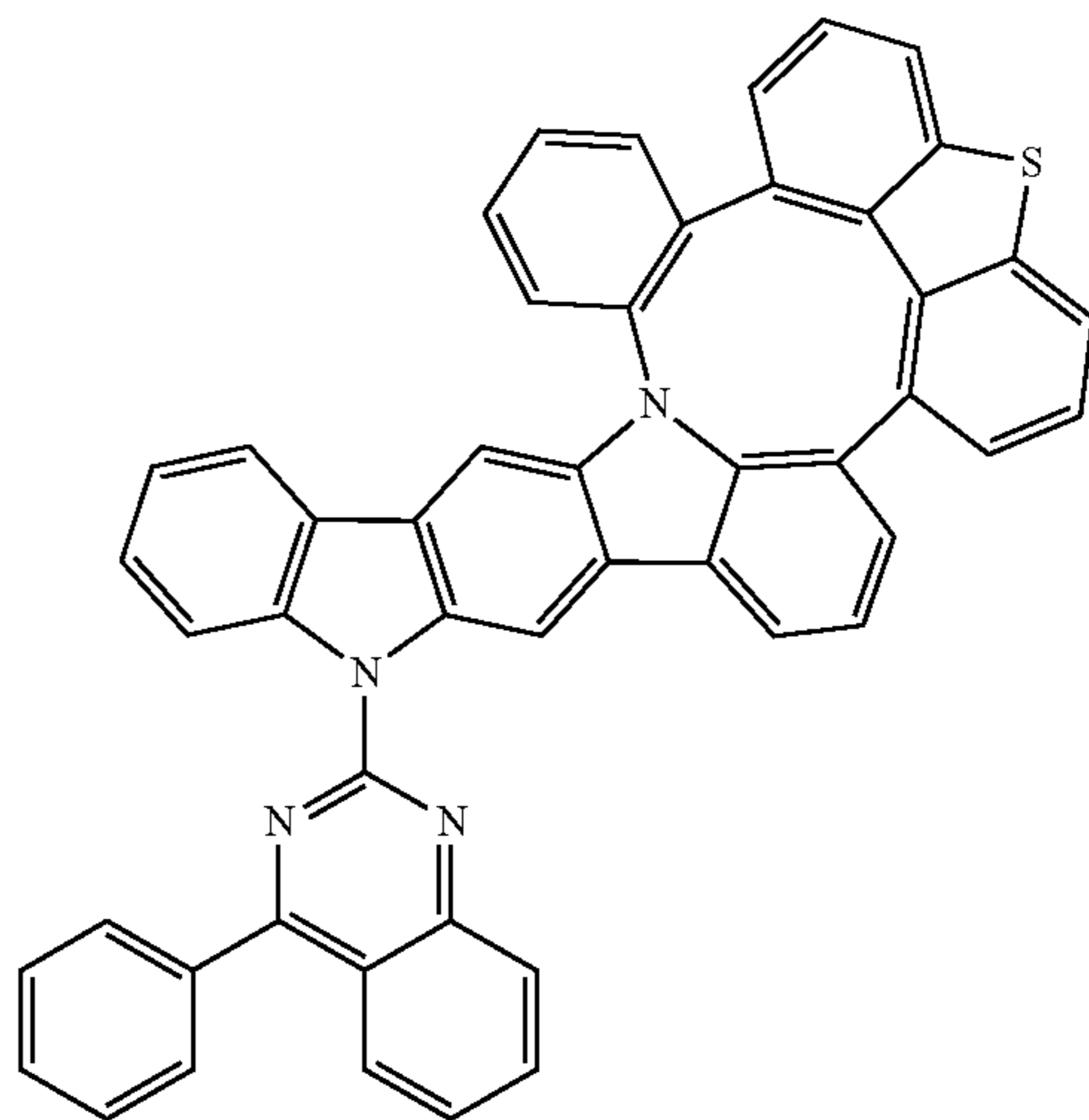
Compound 254
