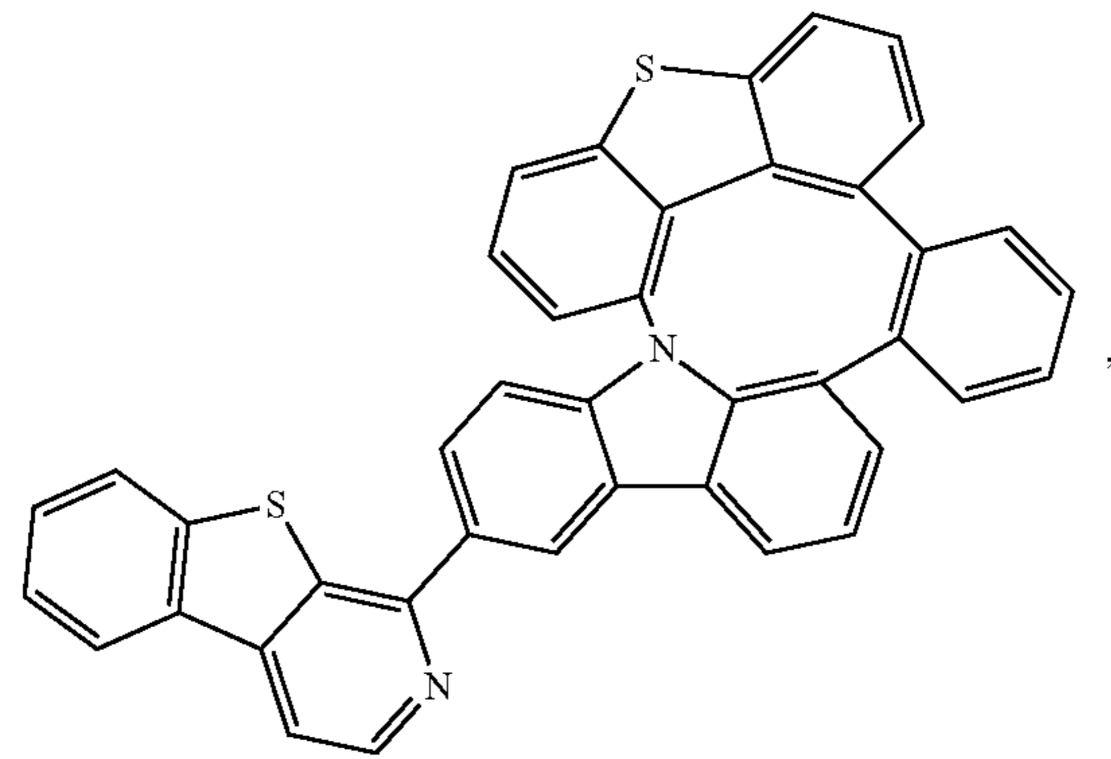
Compound 116
