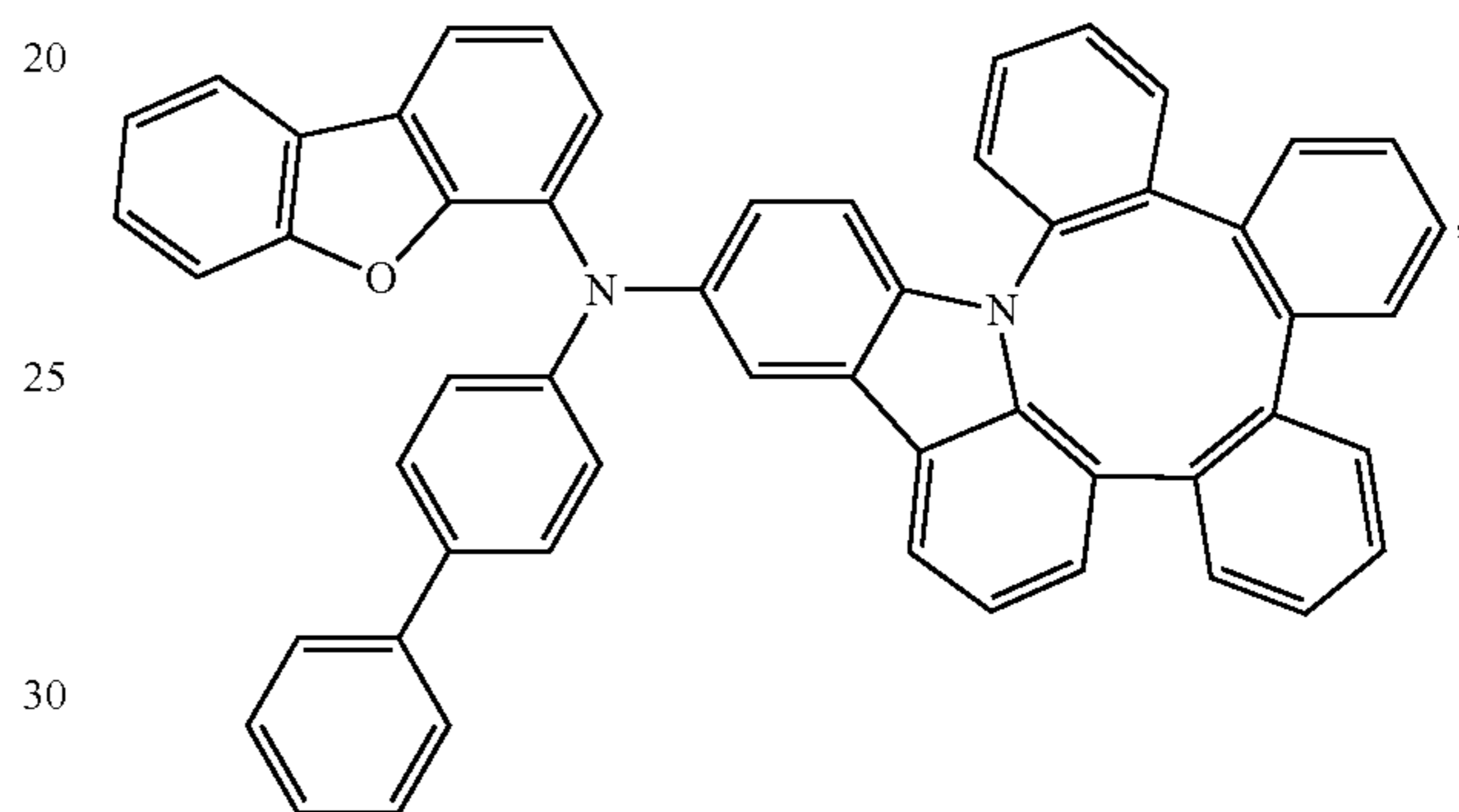
Compound 49
