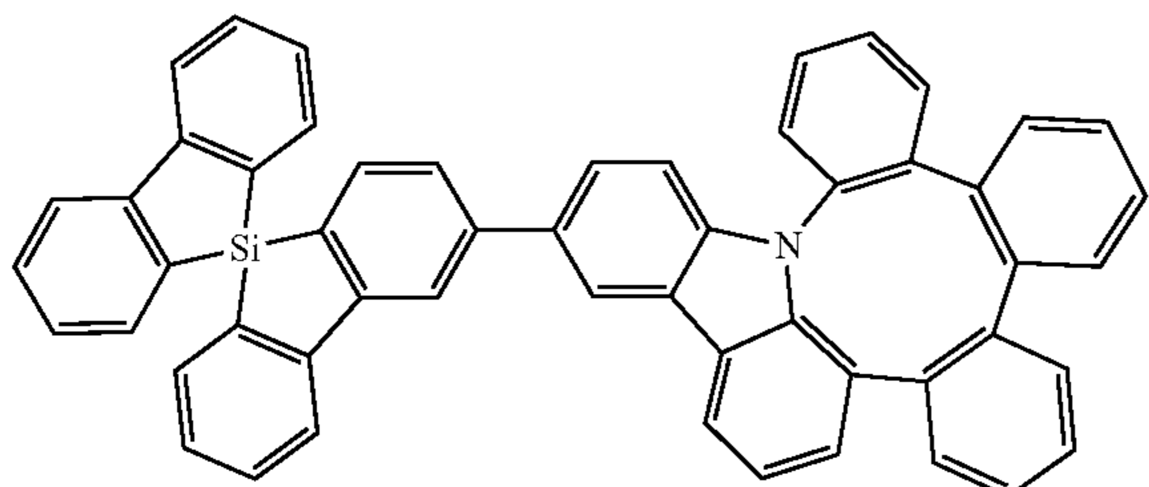
Compound 342
