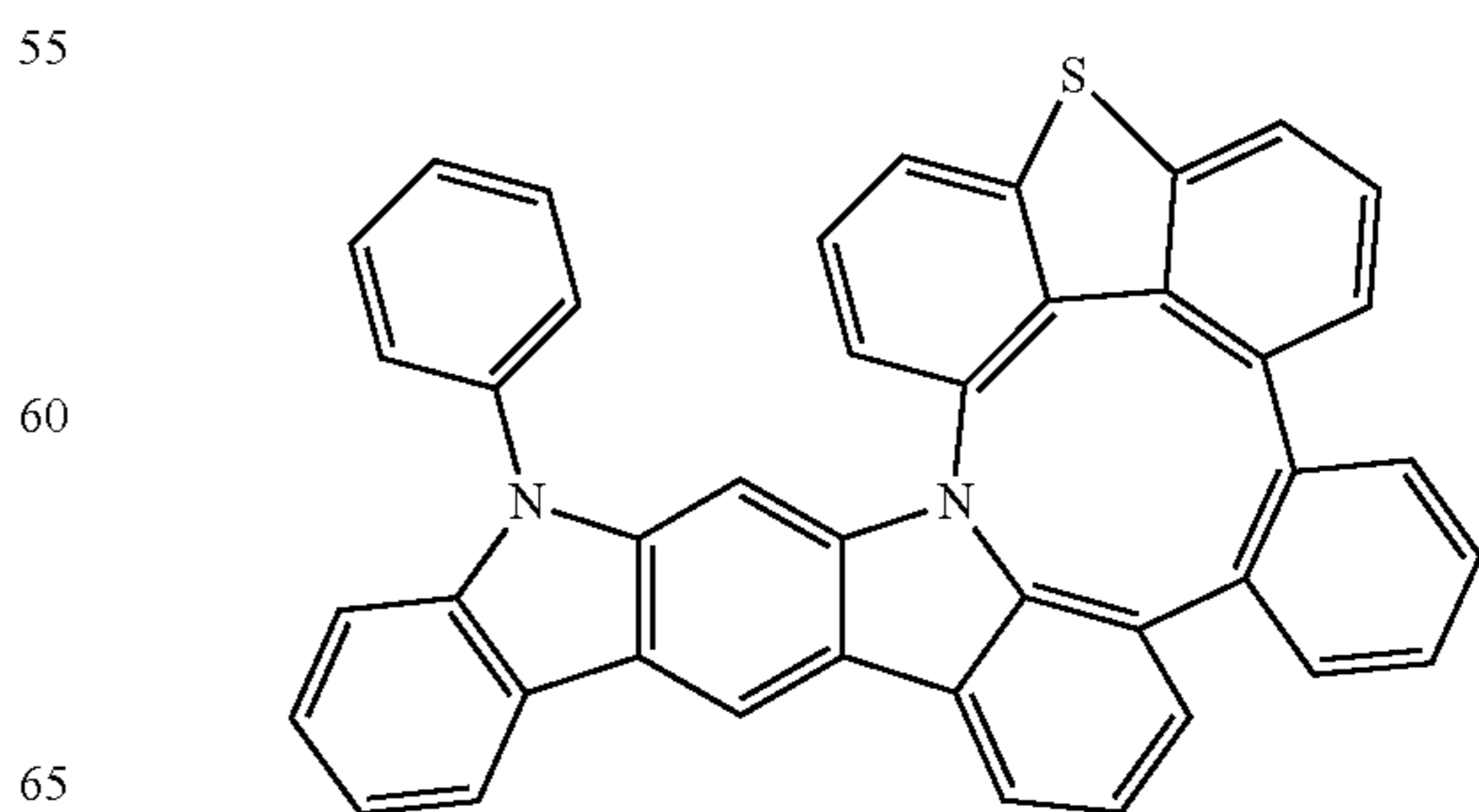
Compound 137
