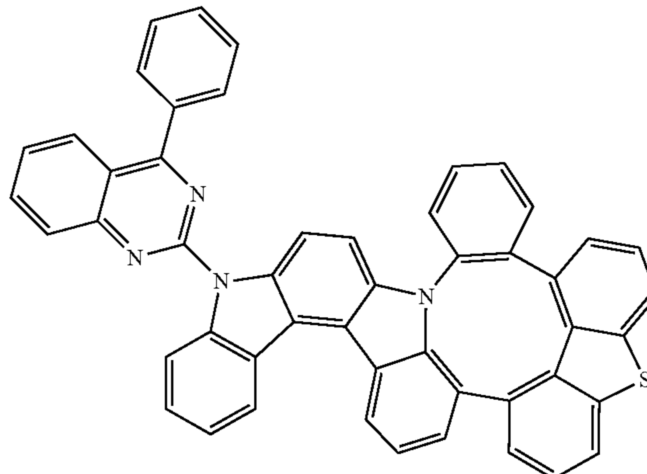
Compound 252
