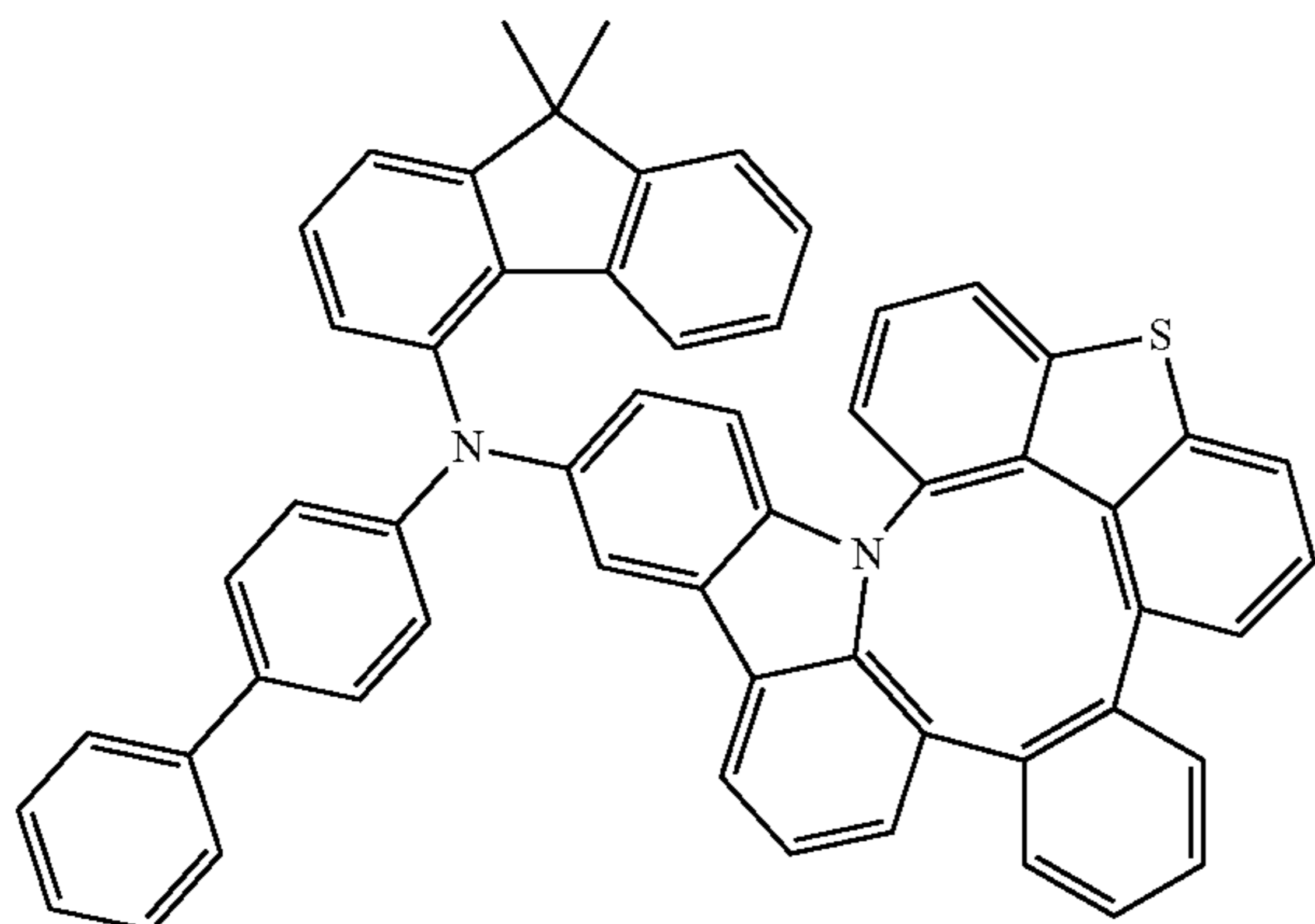
Compound 129
