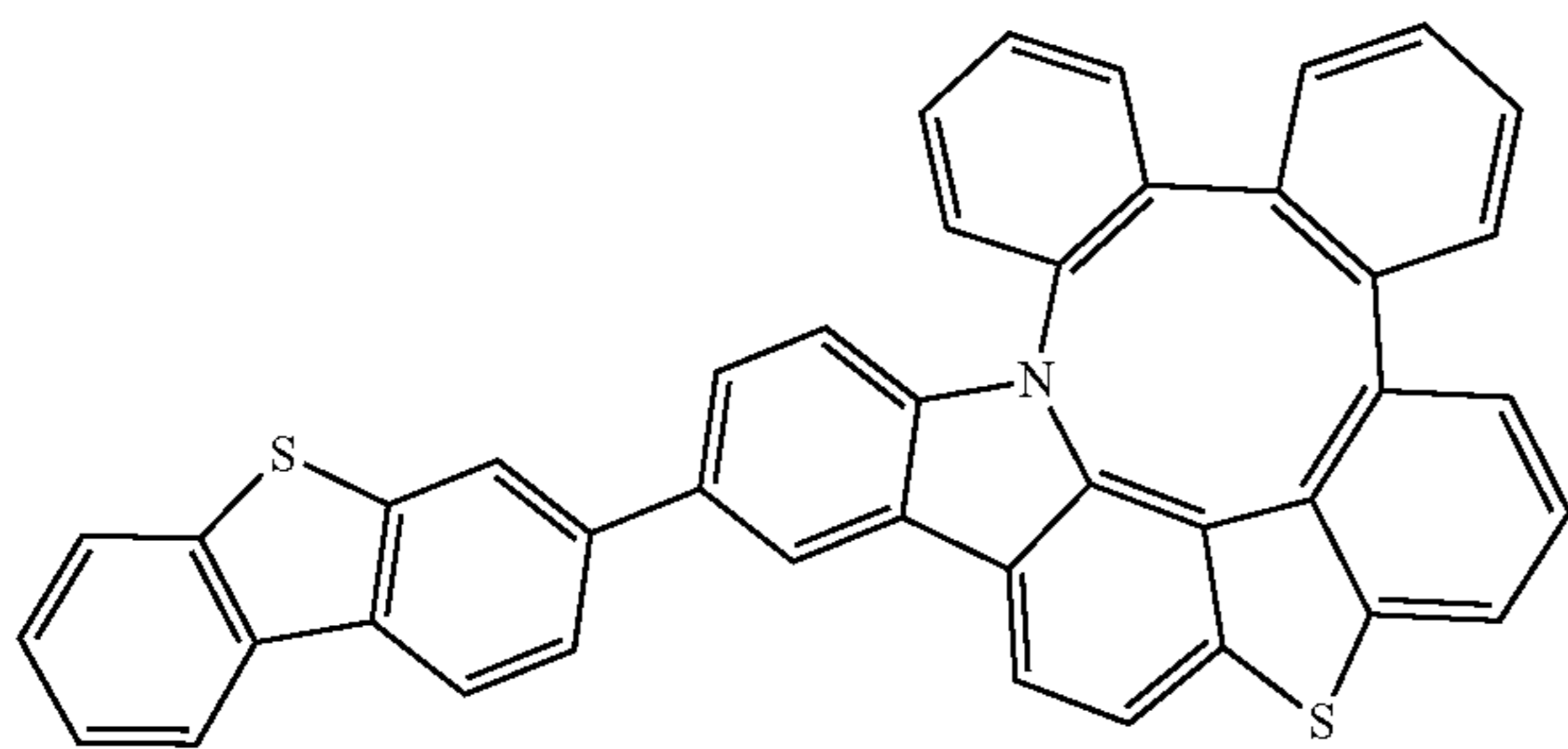
Compound 265
