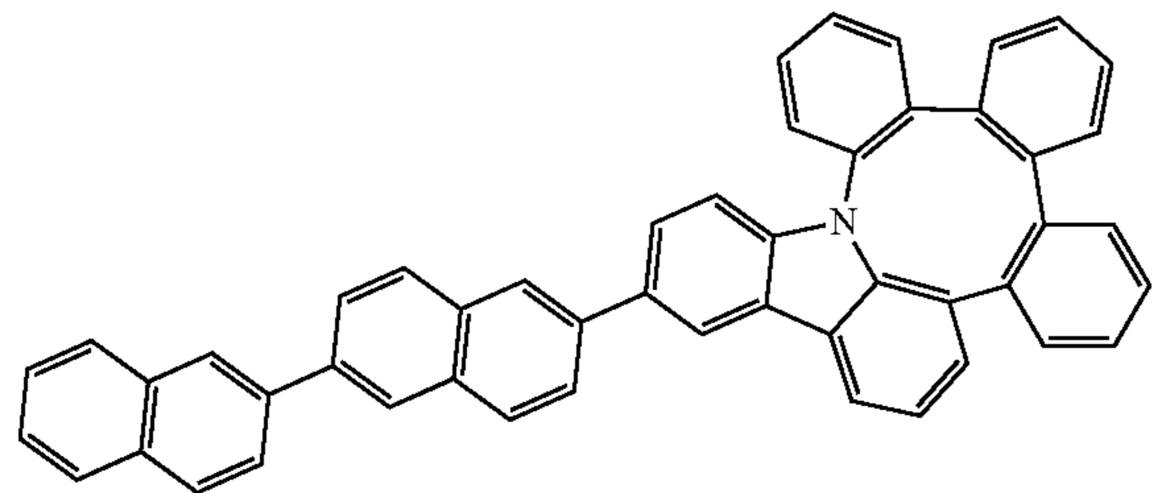
Compound 37
