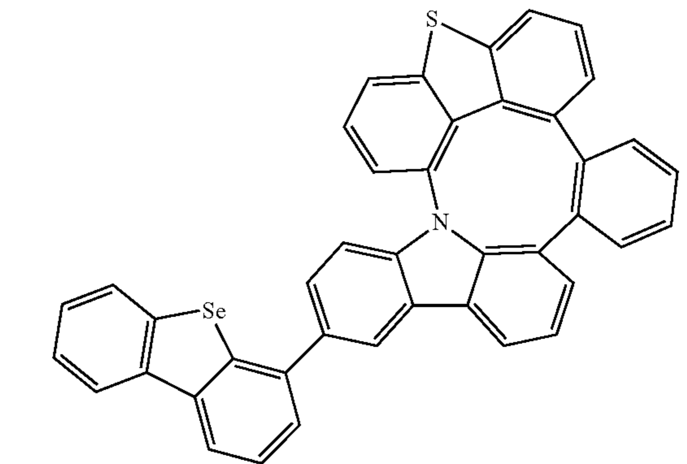
Compound 95
