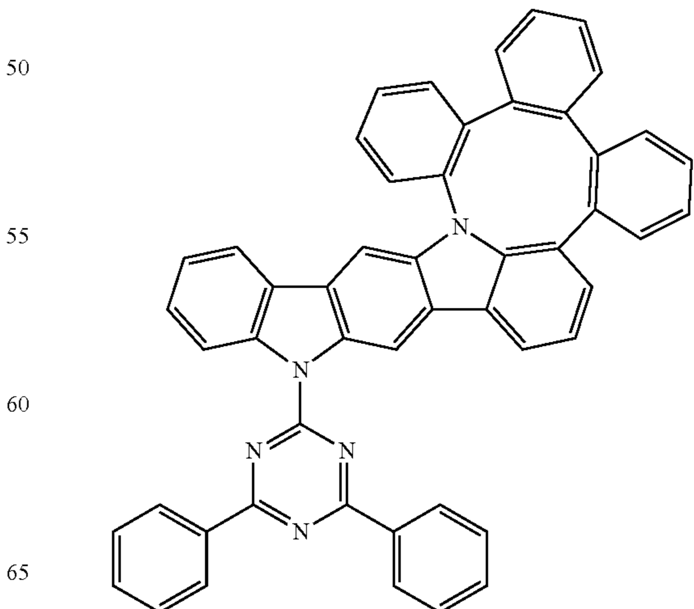
Compound 77
