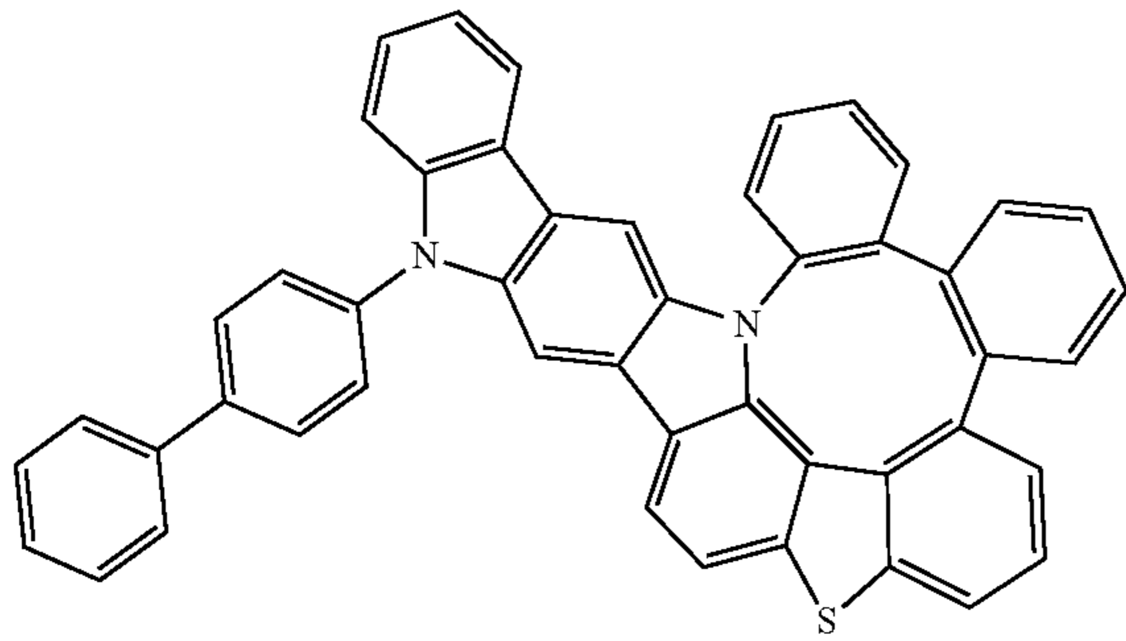
Compound 314
