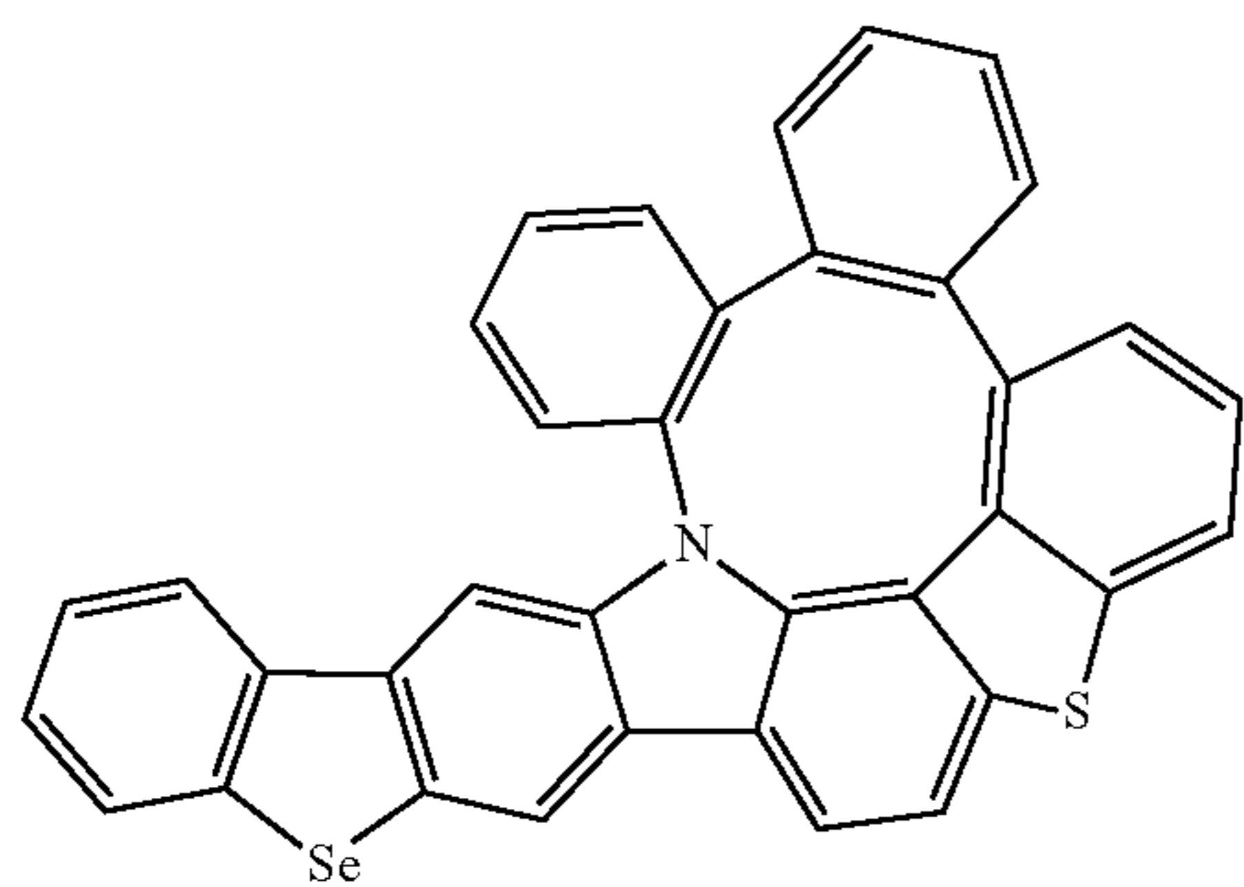
Compound 327
