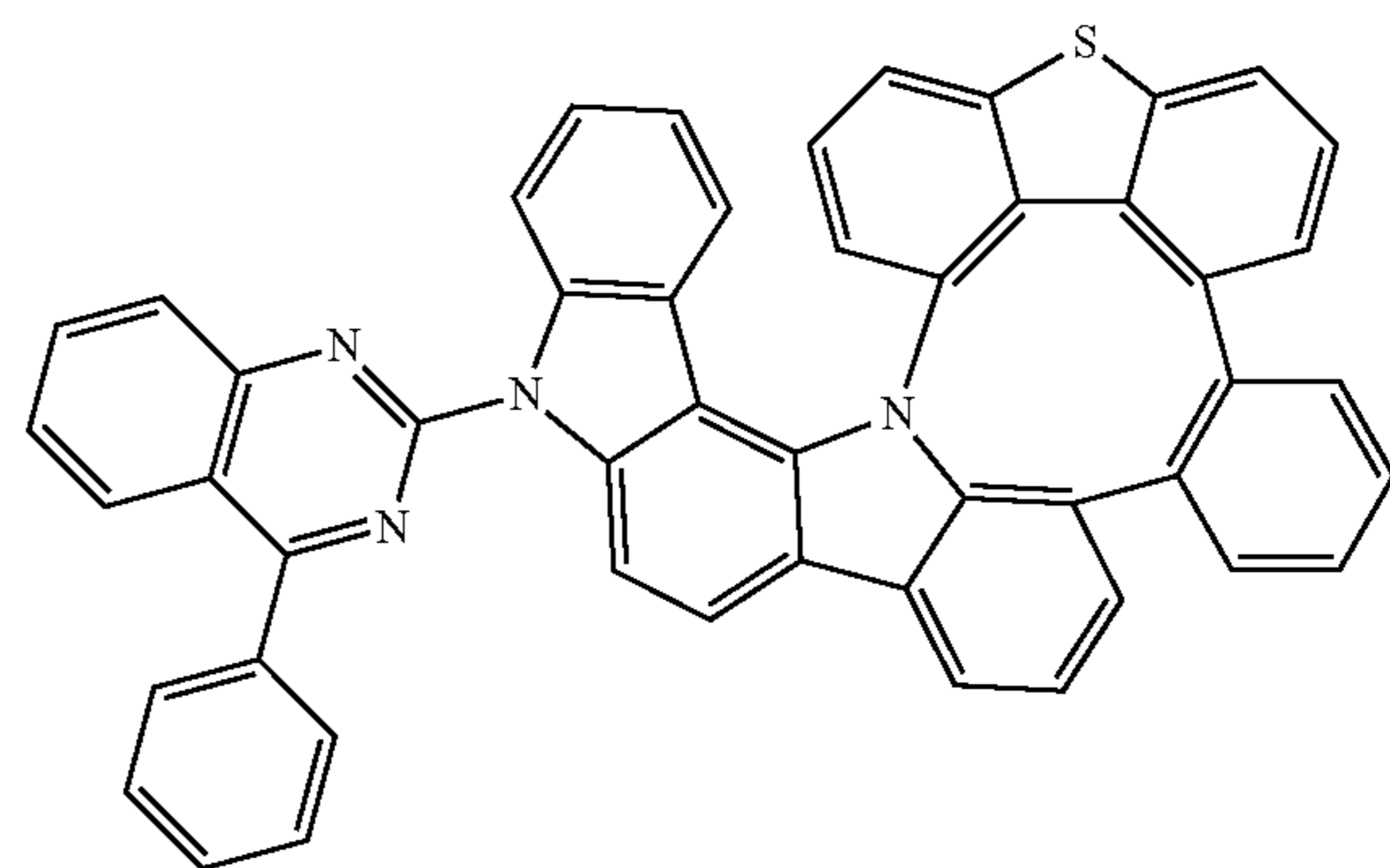
Compound 170
