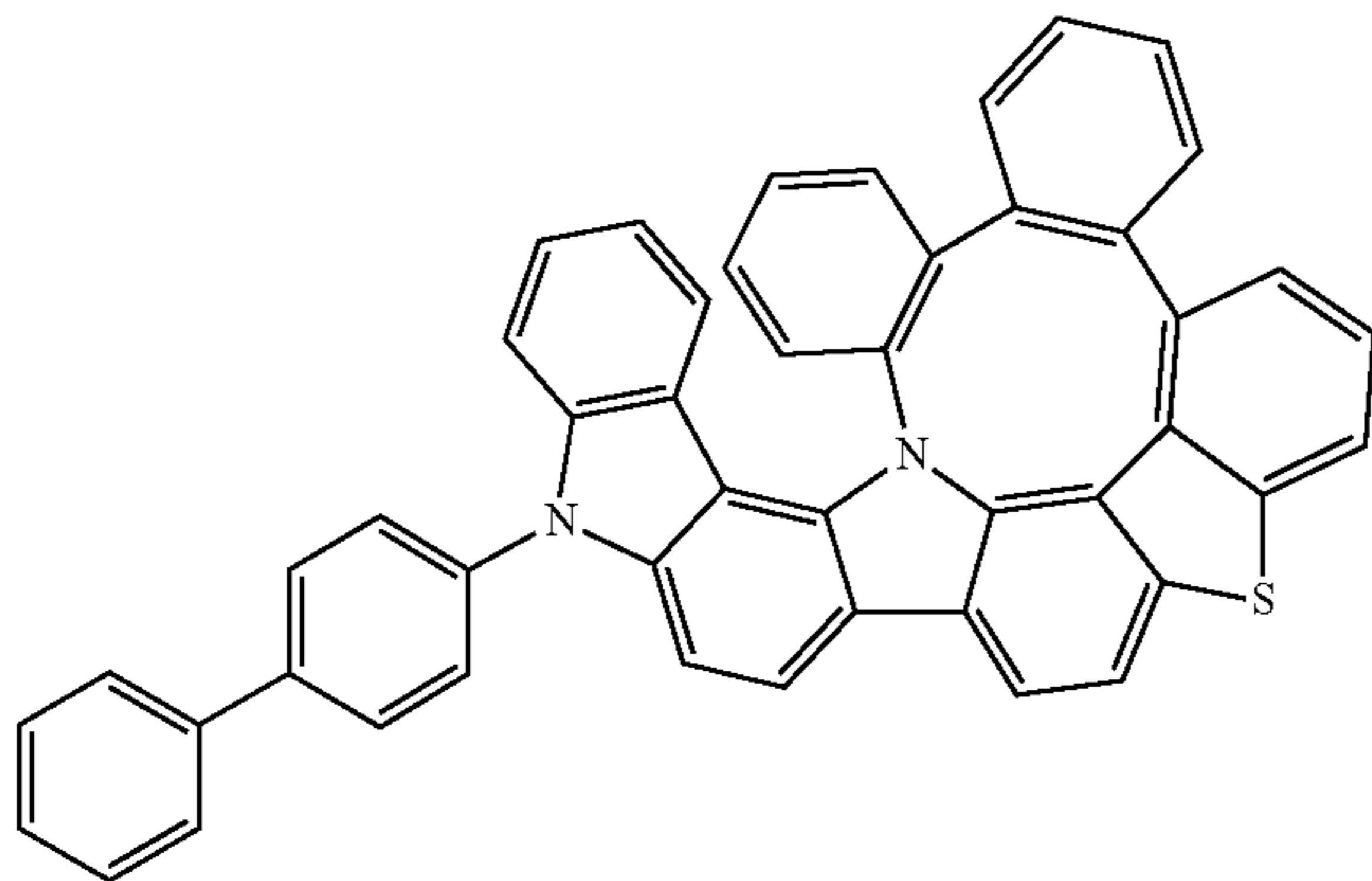
Compound 315
