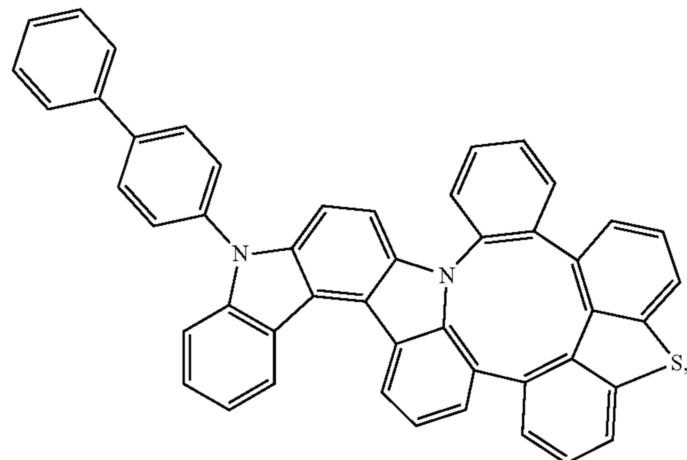
Compound 228
