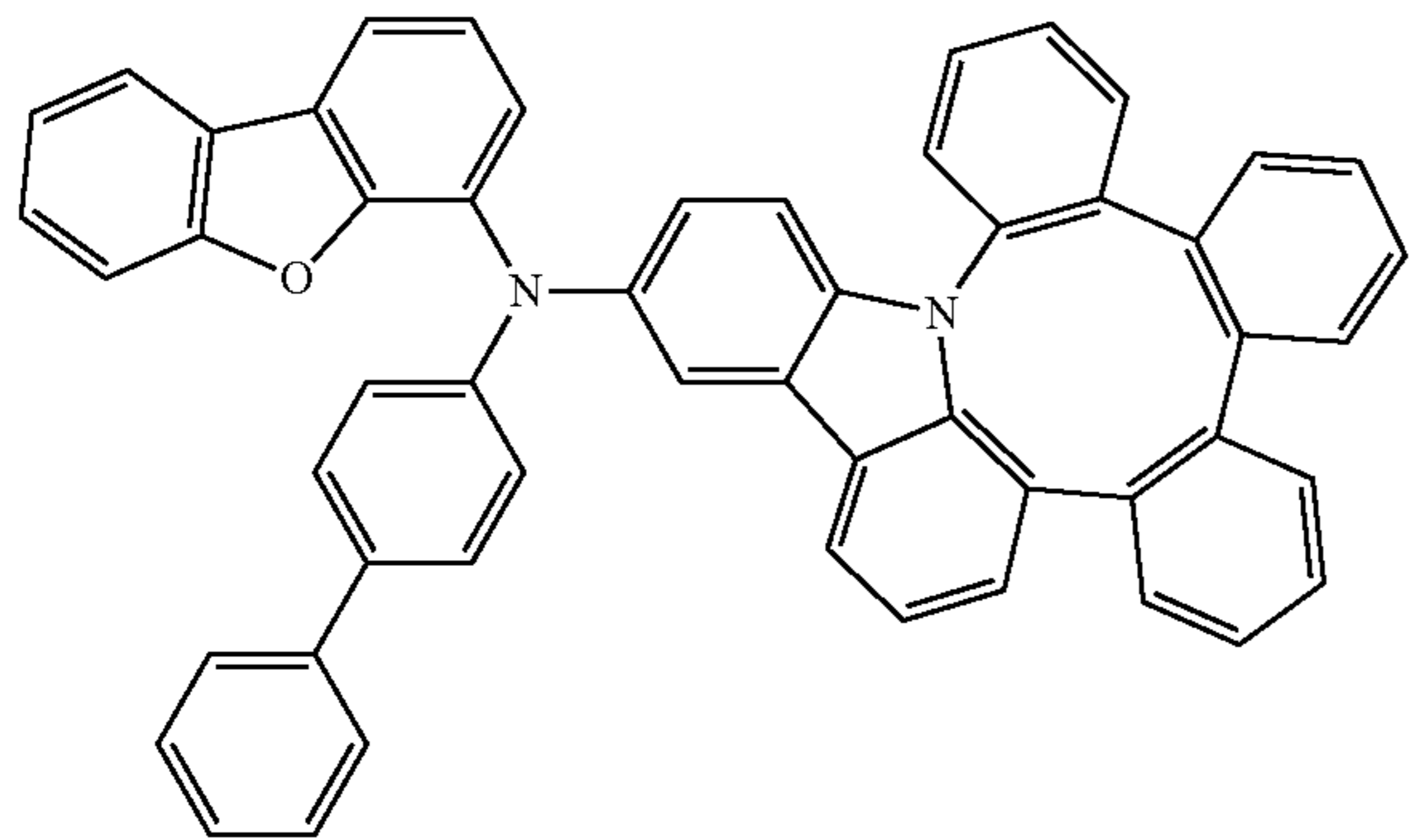
Compound 48
