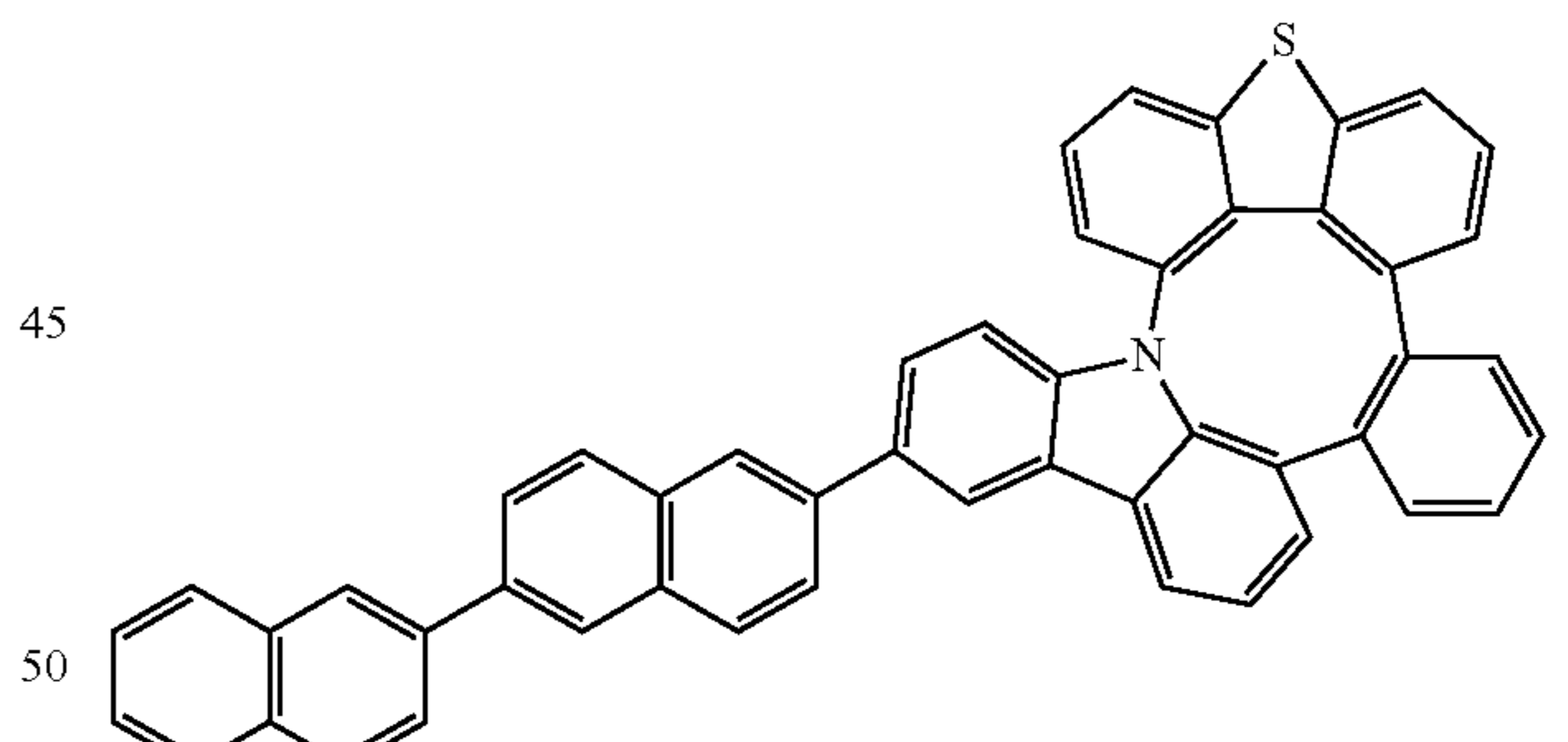
Compound 121
