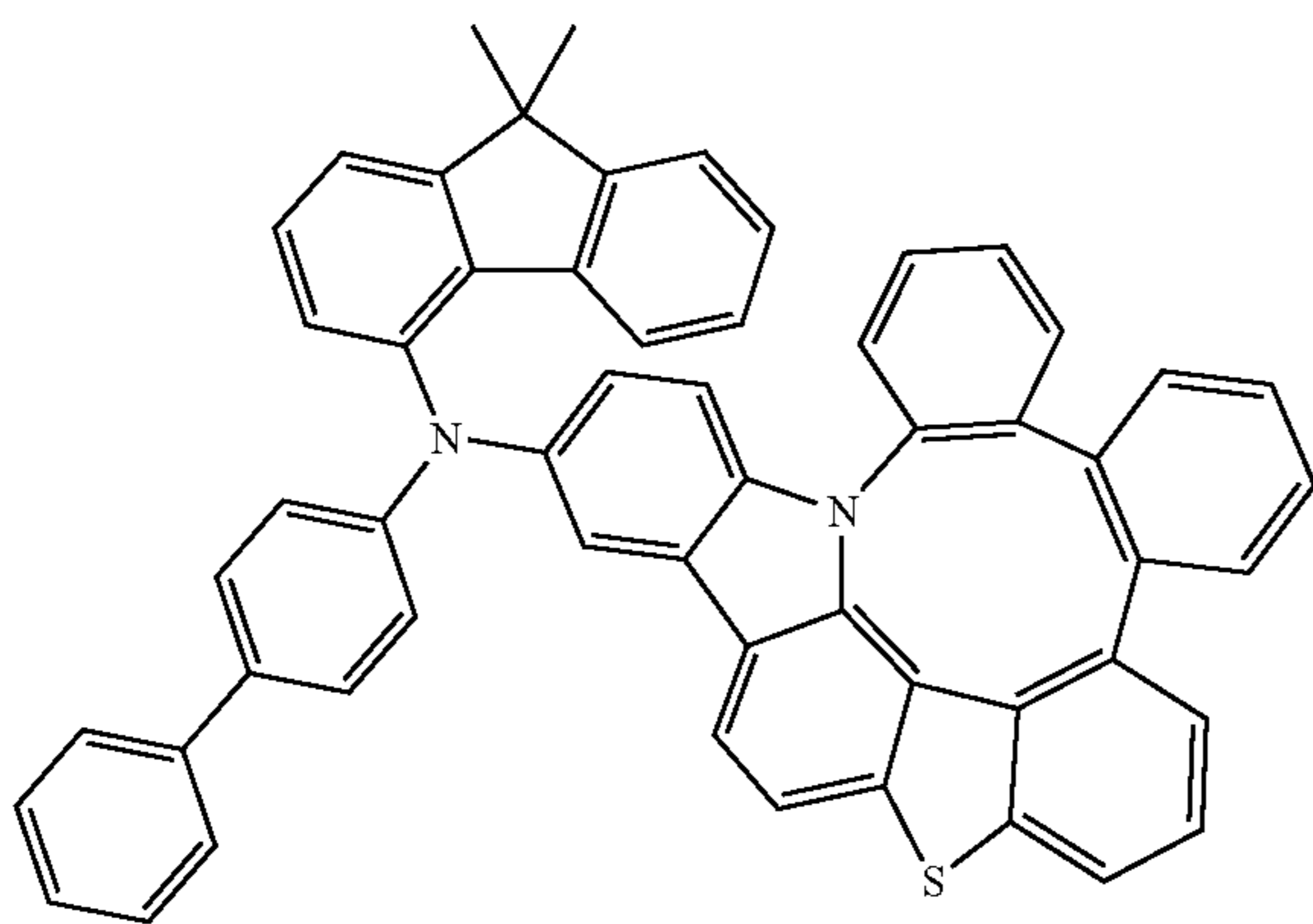
Compound 300
