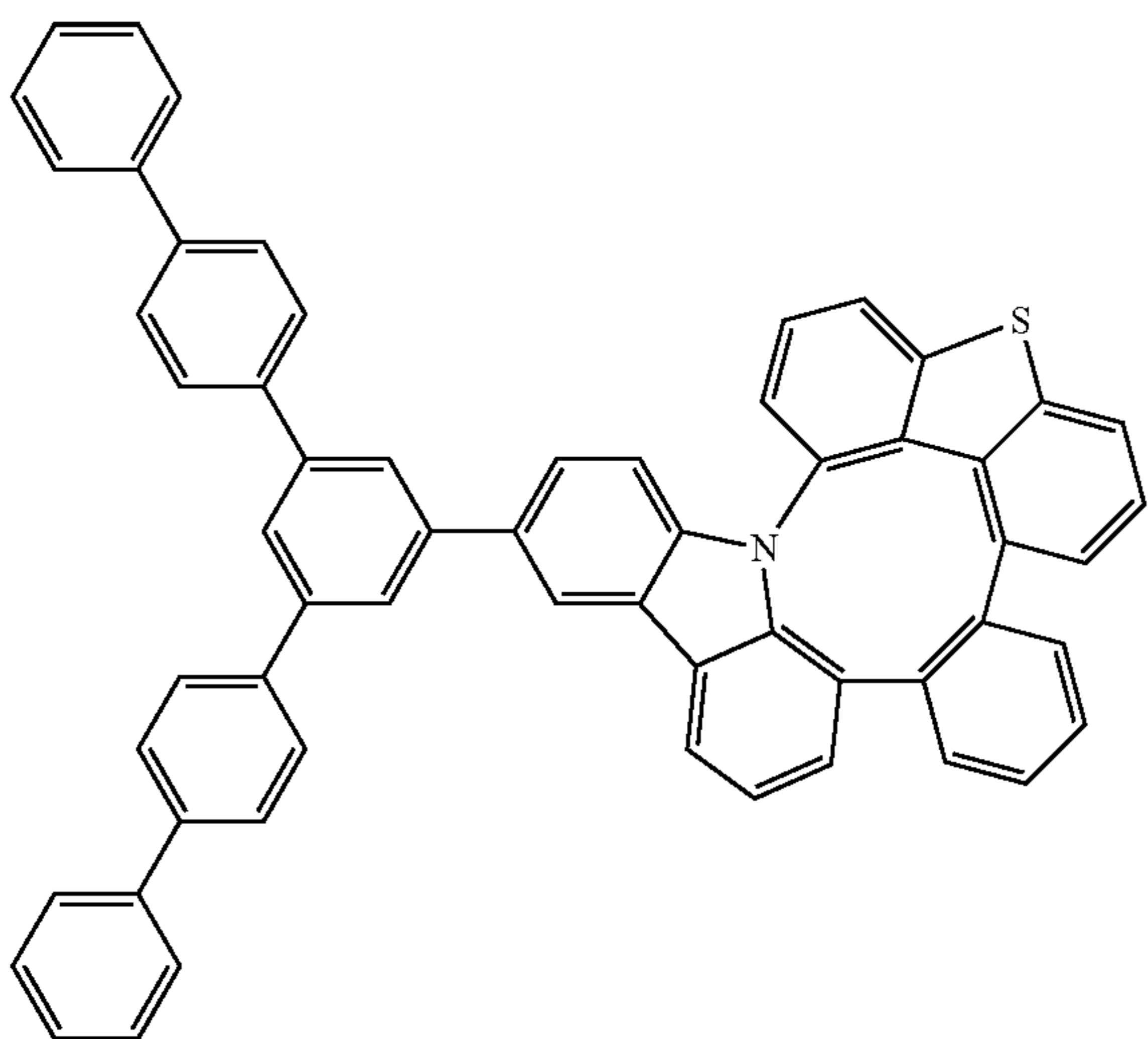
Compound 131
