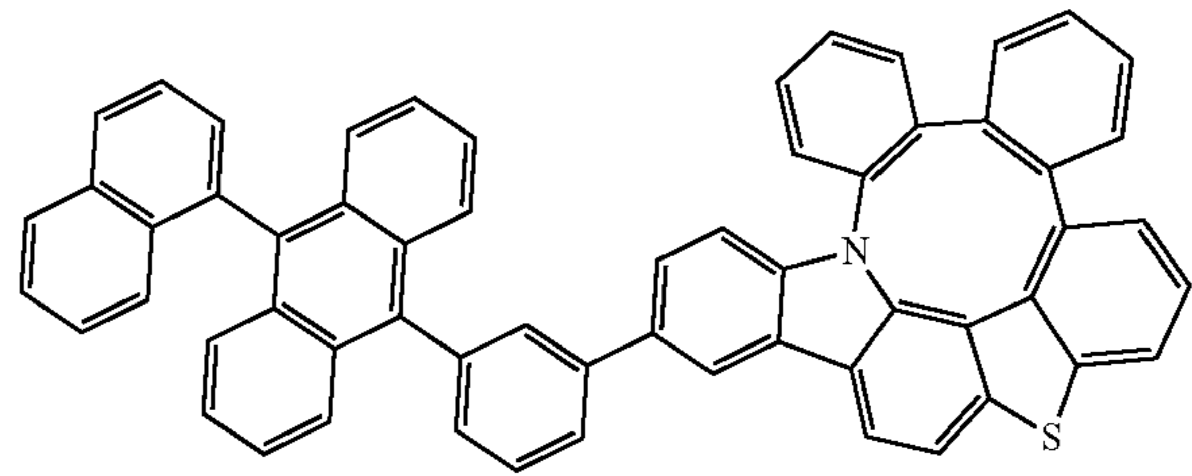
Compound 294
