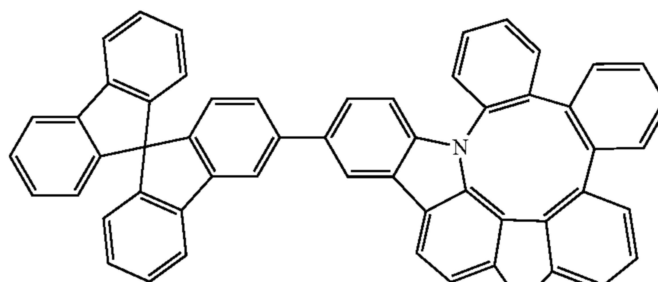
Compound 278
