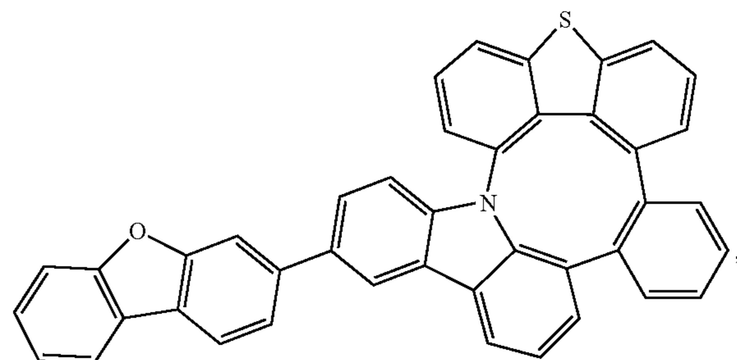
Compound 91
