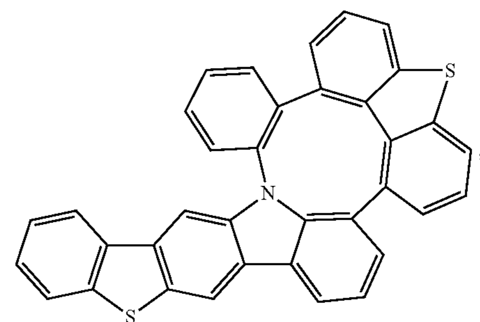
Compound 236
