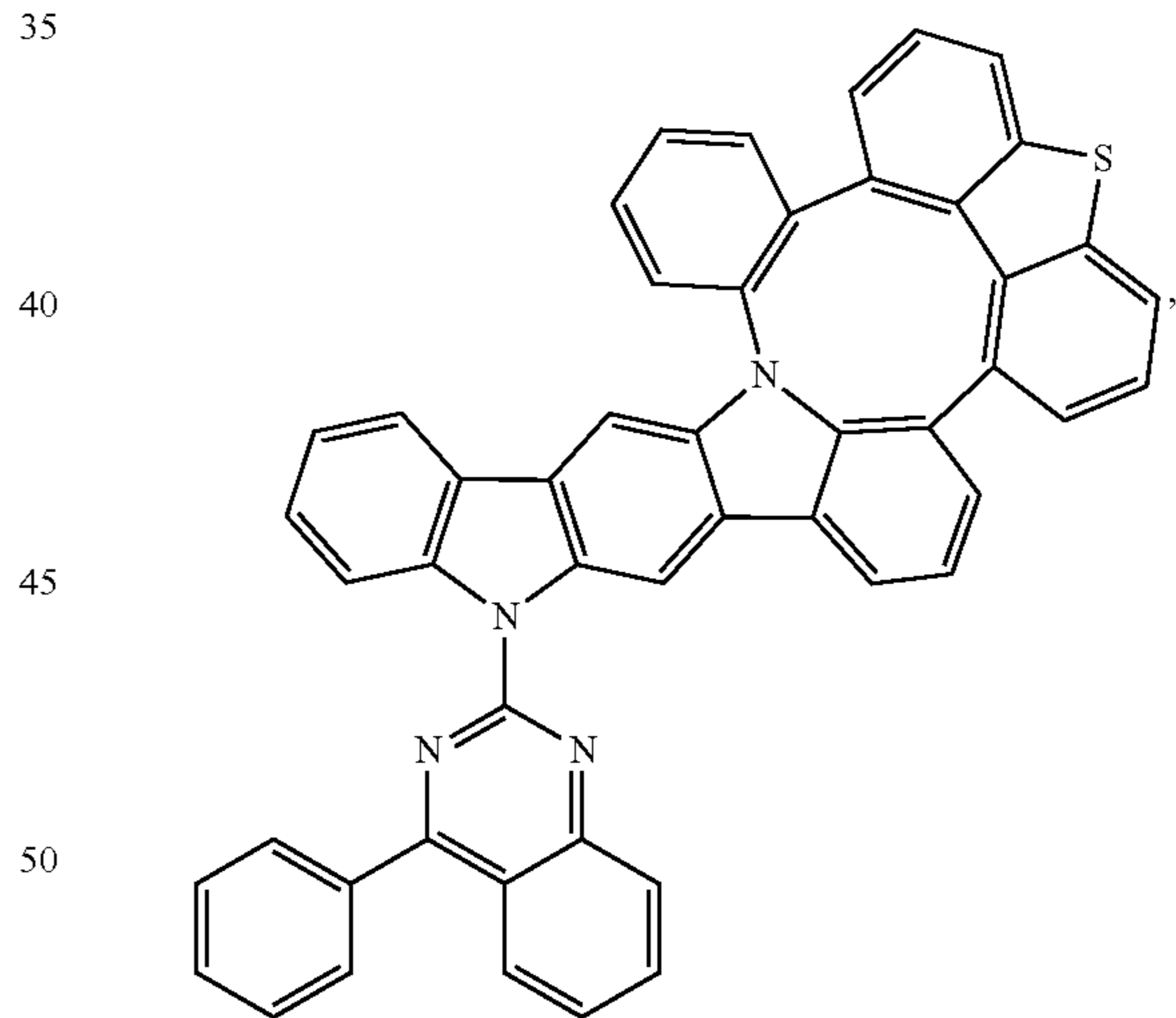
Compound 254
