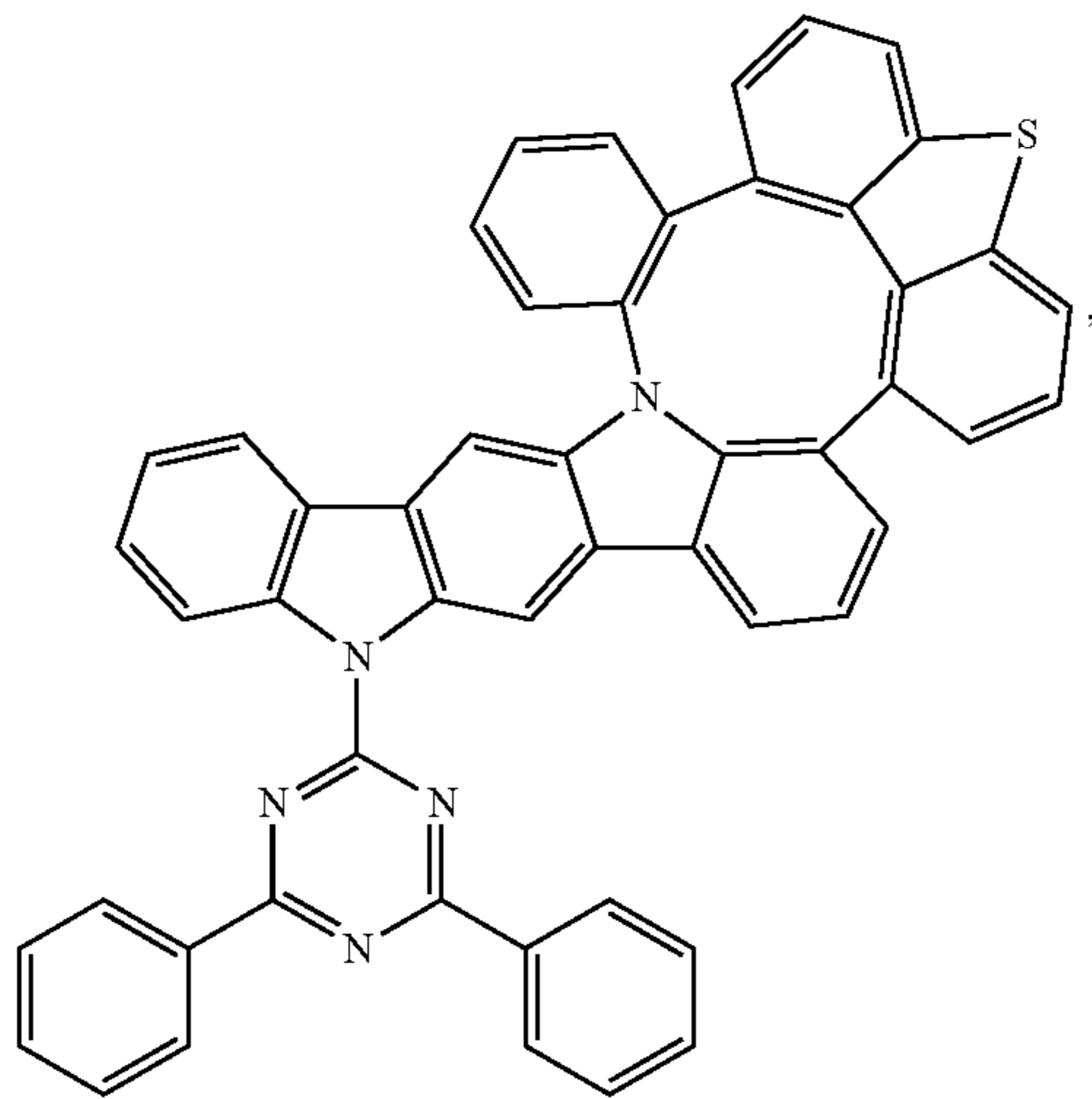
Compound 247
