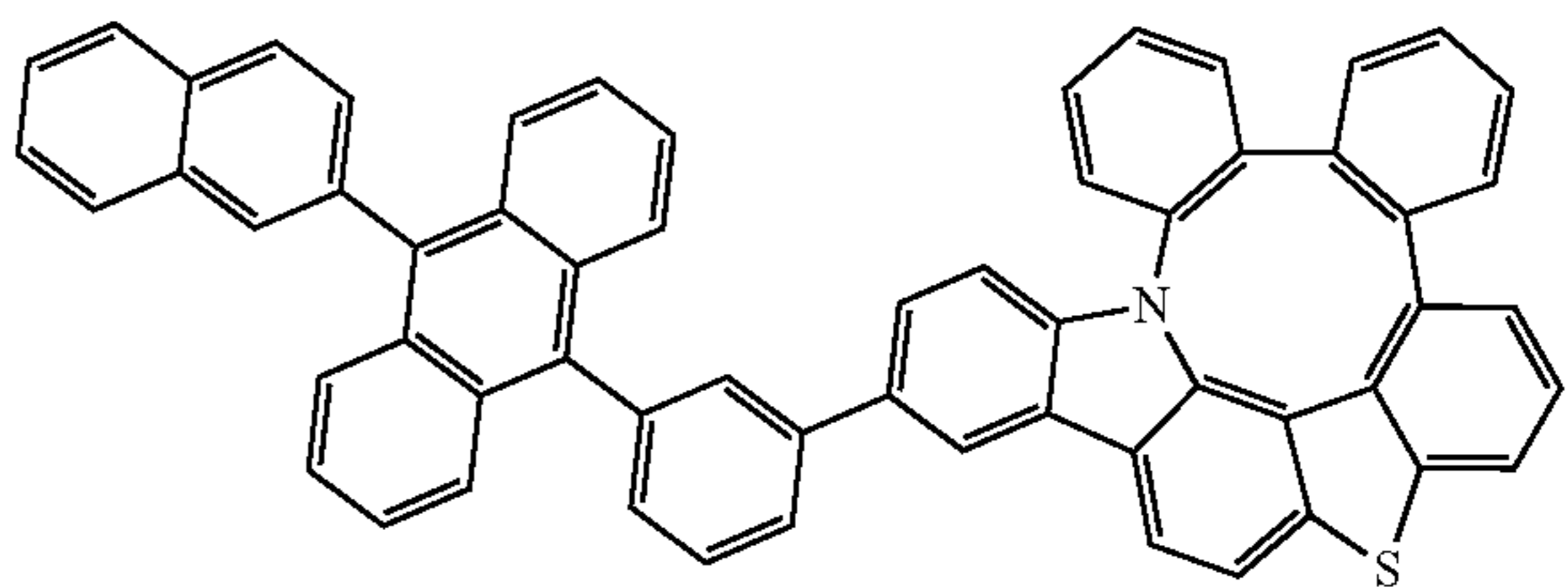
Compound 295
