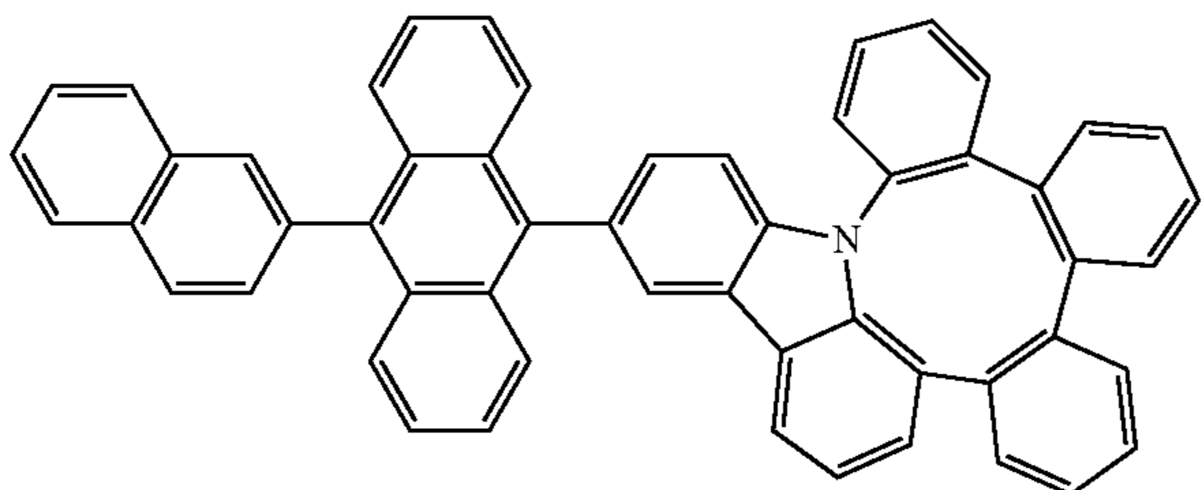
Compound 39
