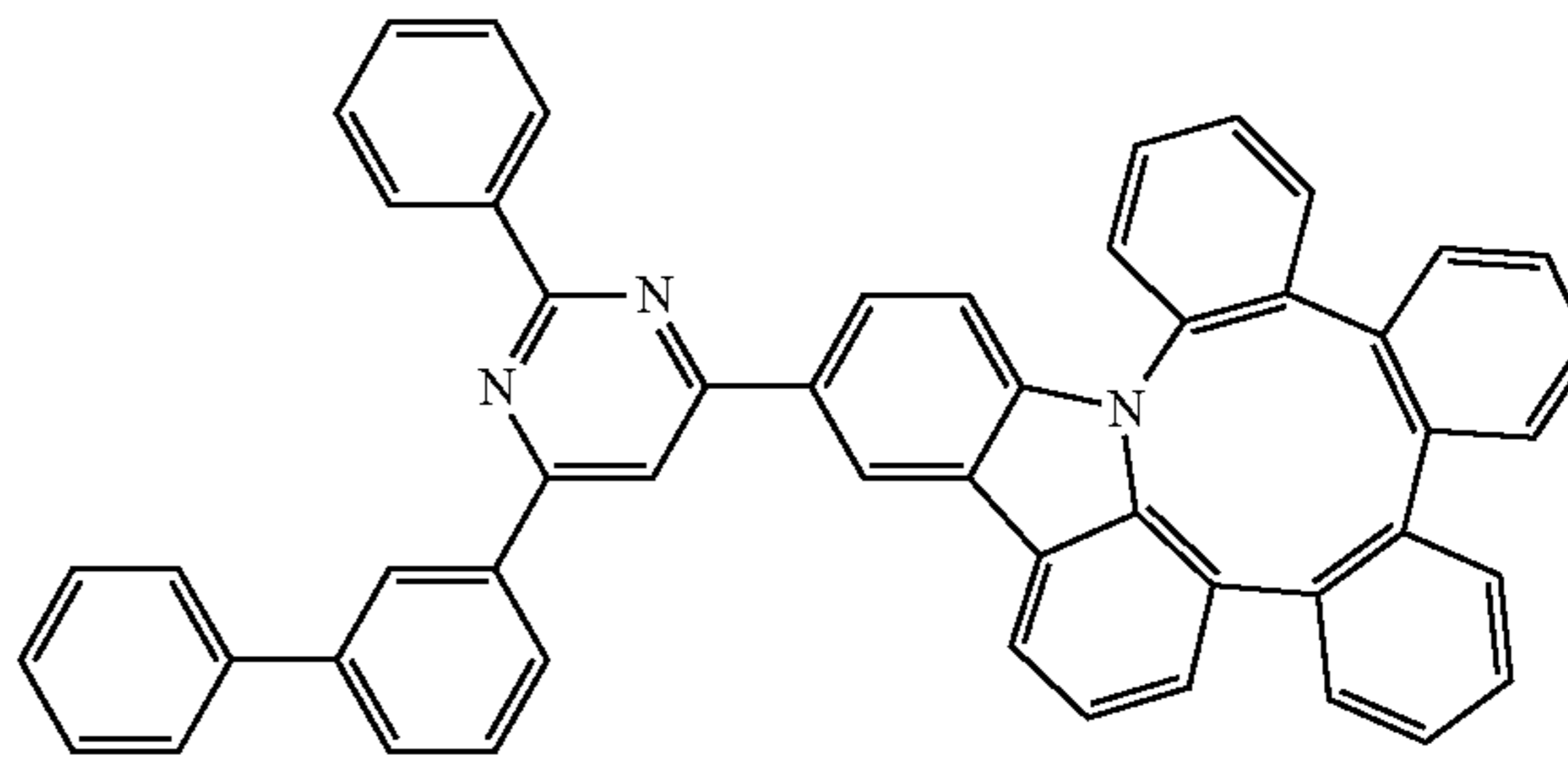
Compound 29
