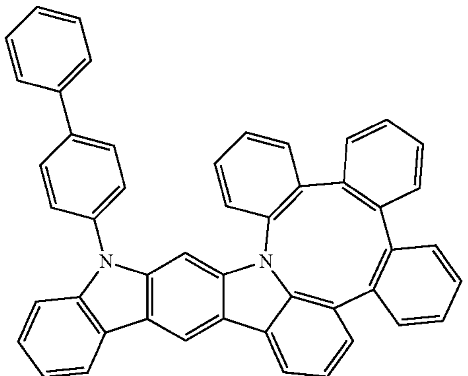
Compound 58
