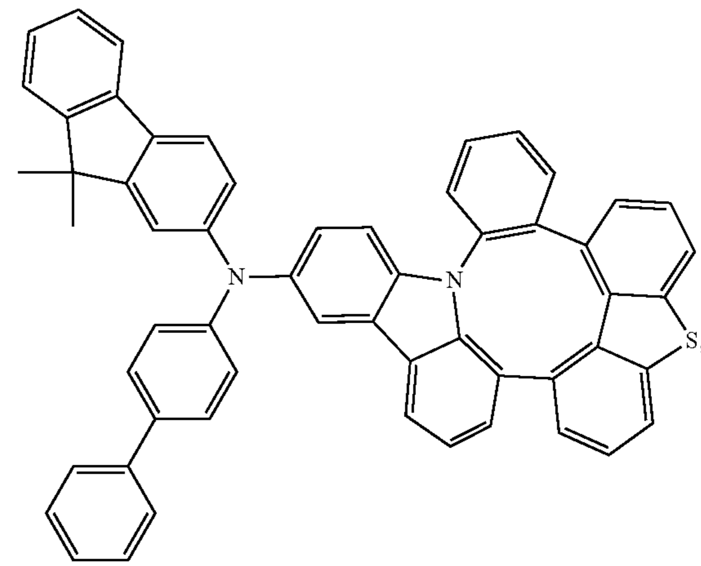
Compound 212
