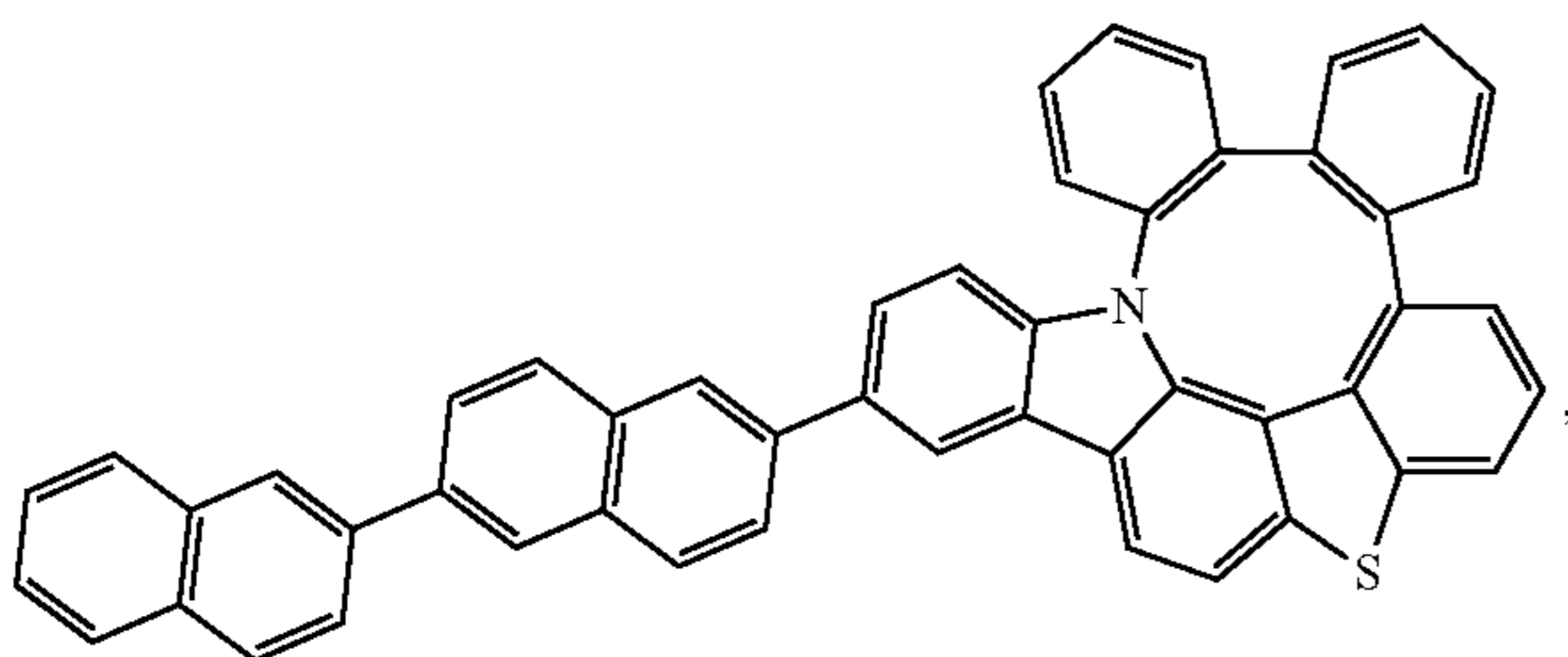
Compound 292
