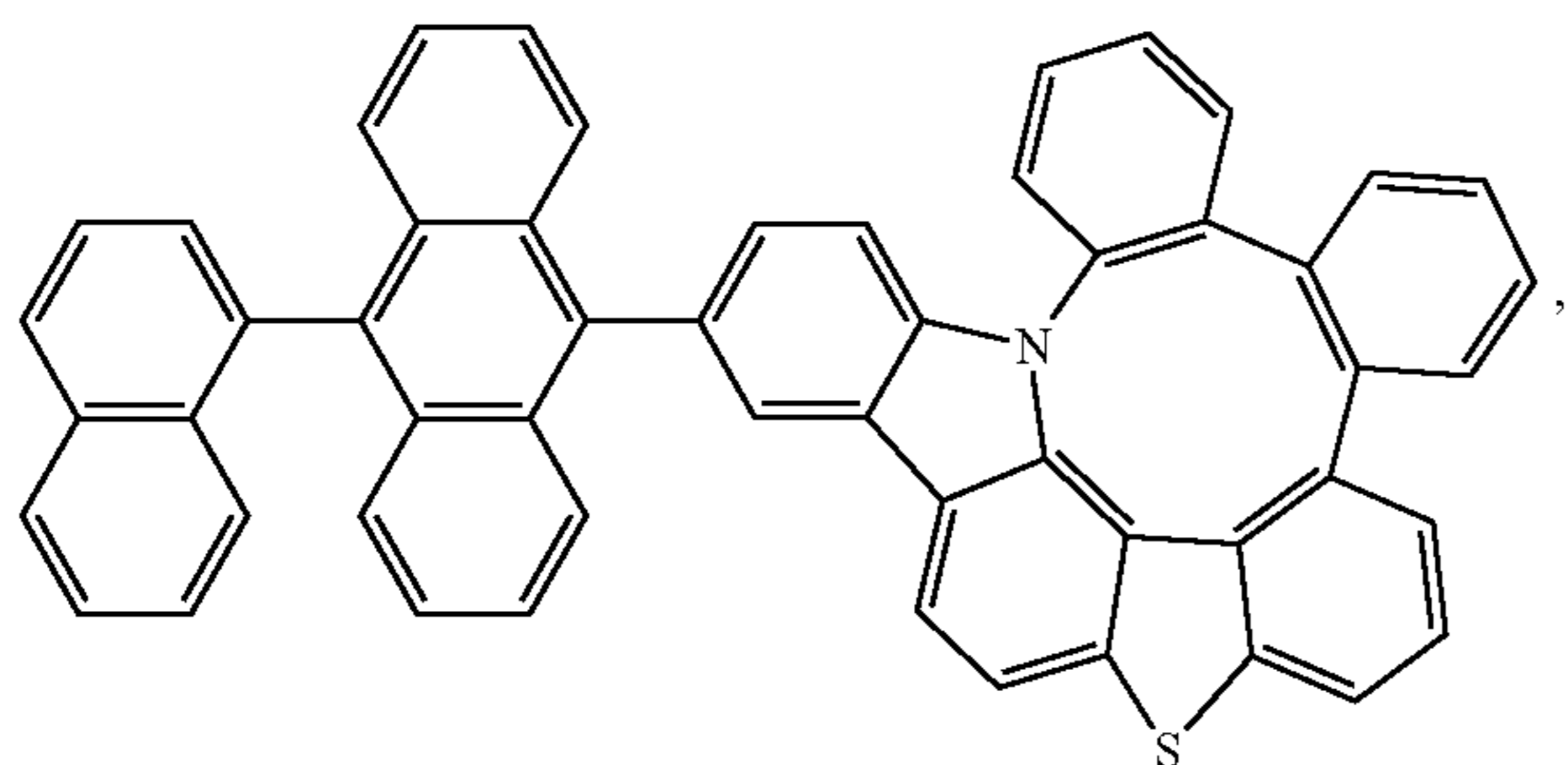
Compound 292
