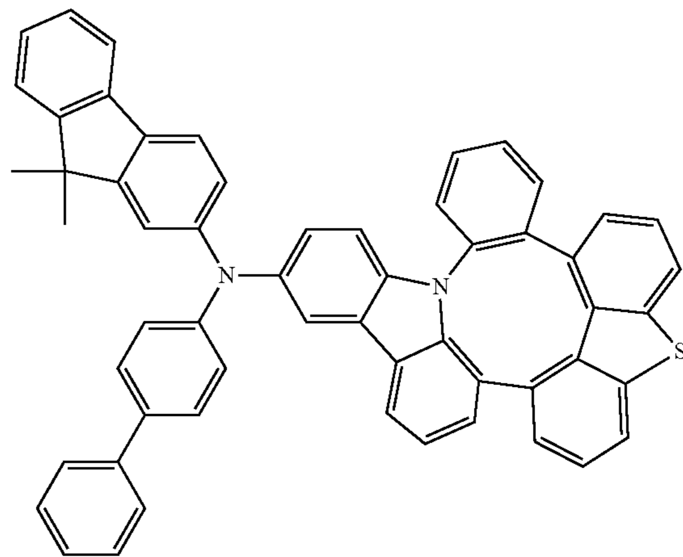
Compound 212
