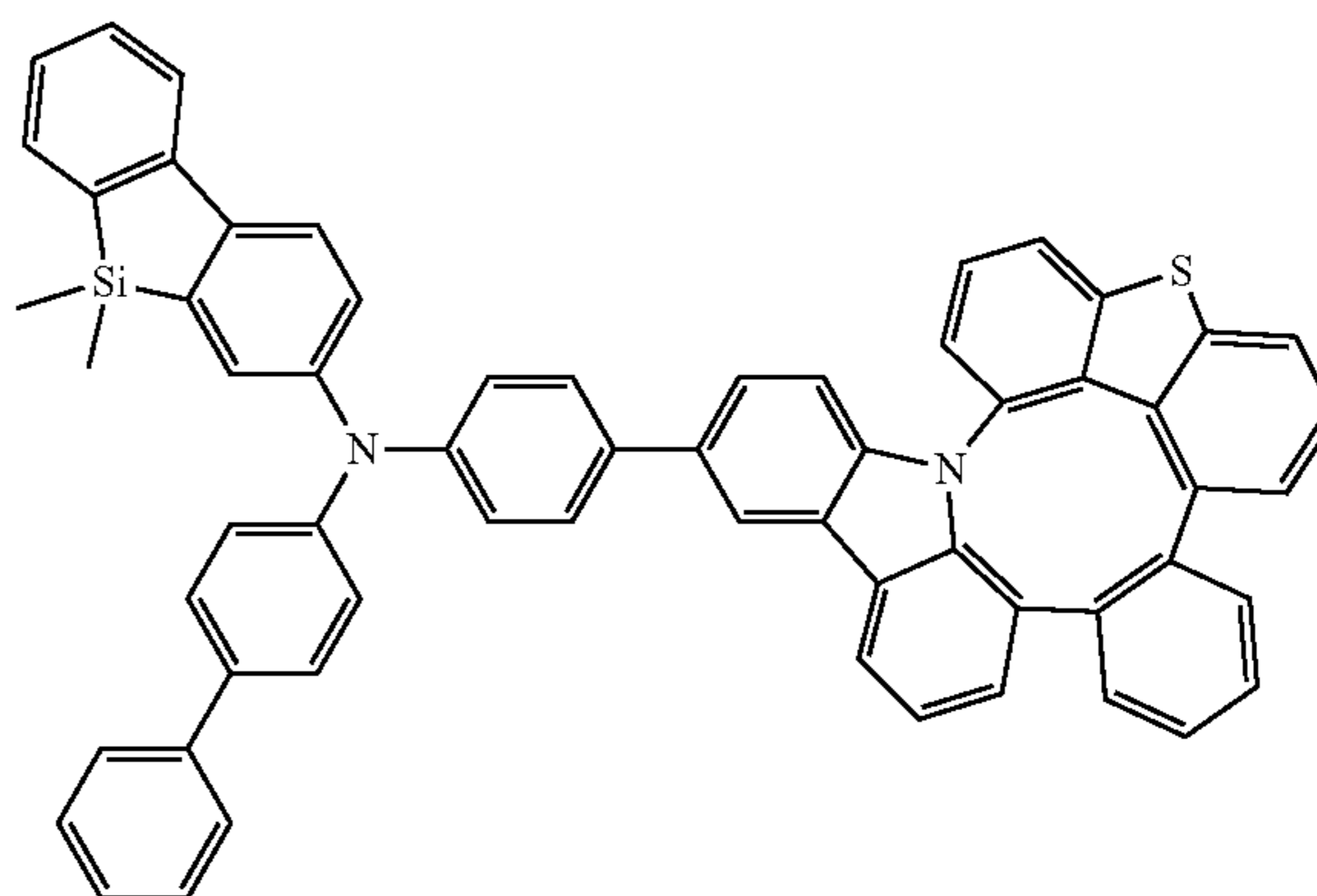
Compound 355
