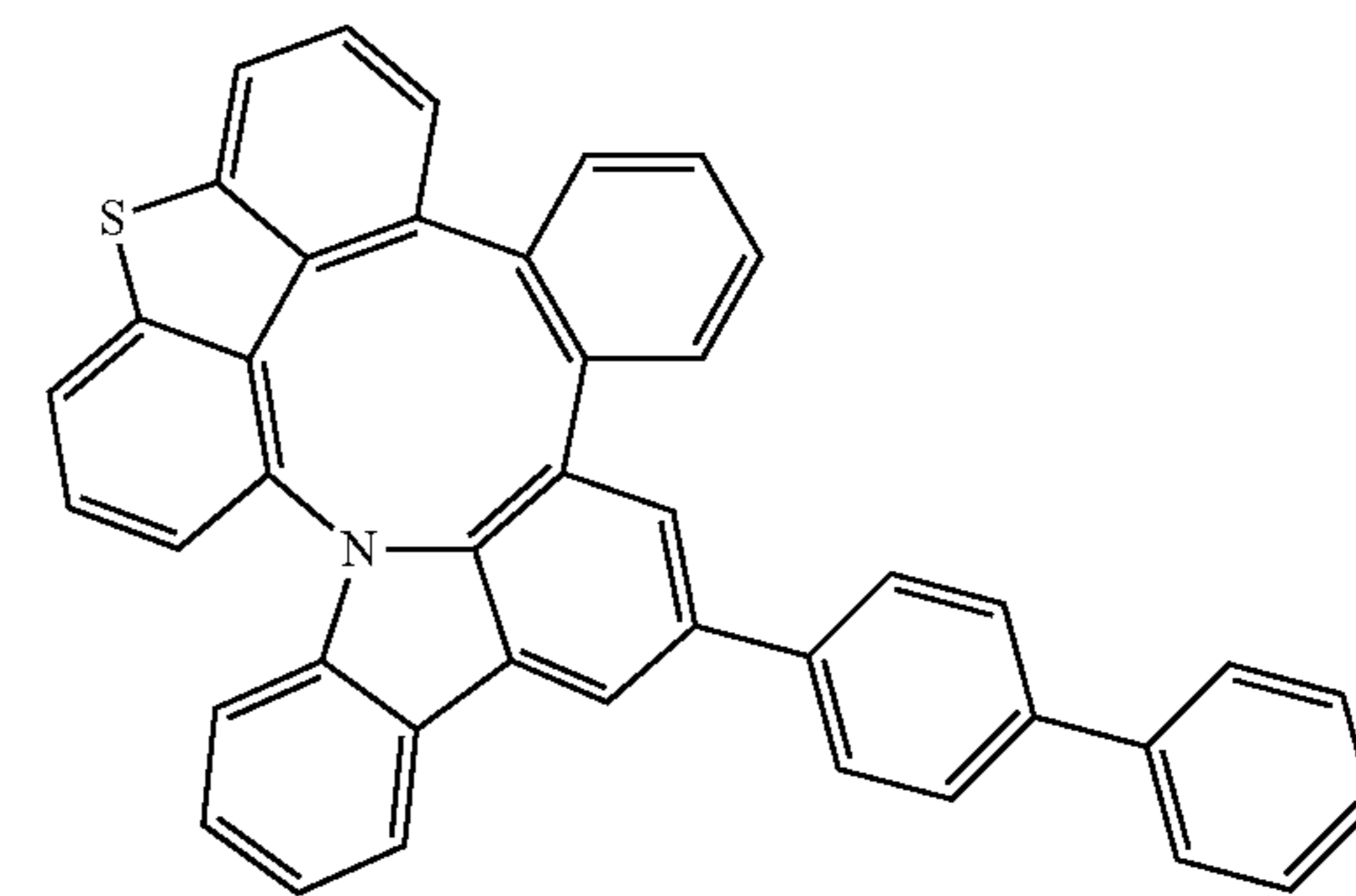
Compound 88
