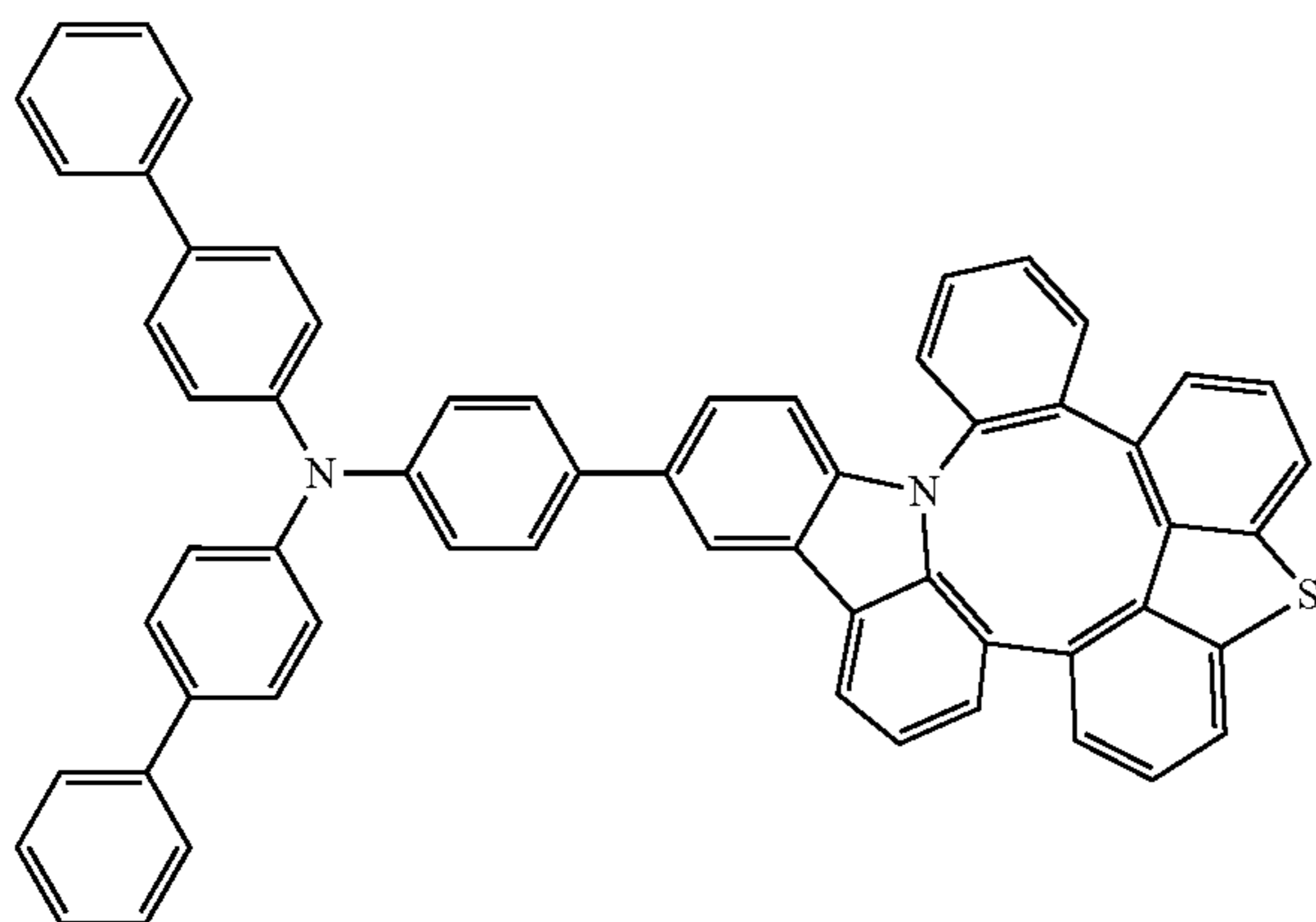
Compound 216
