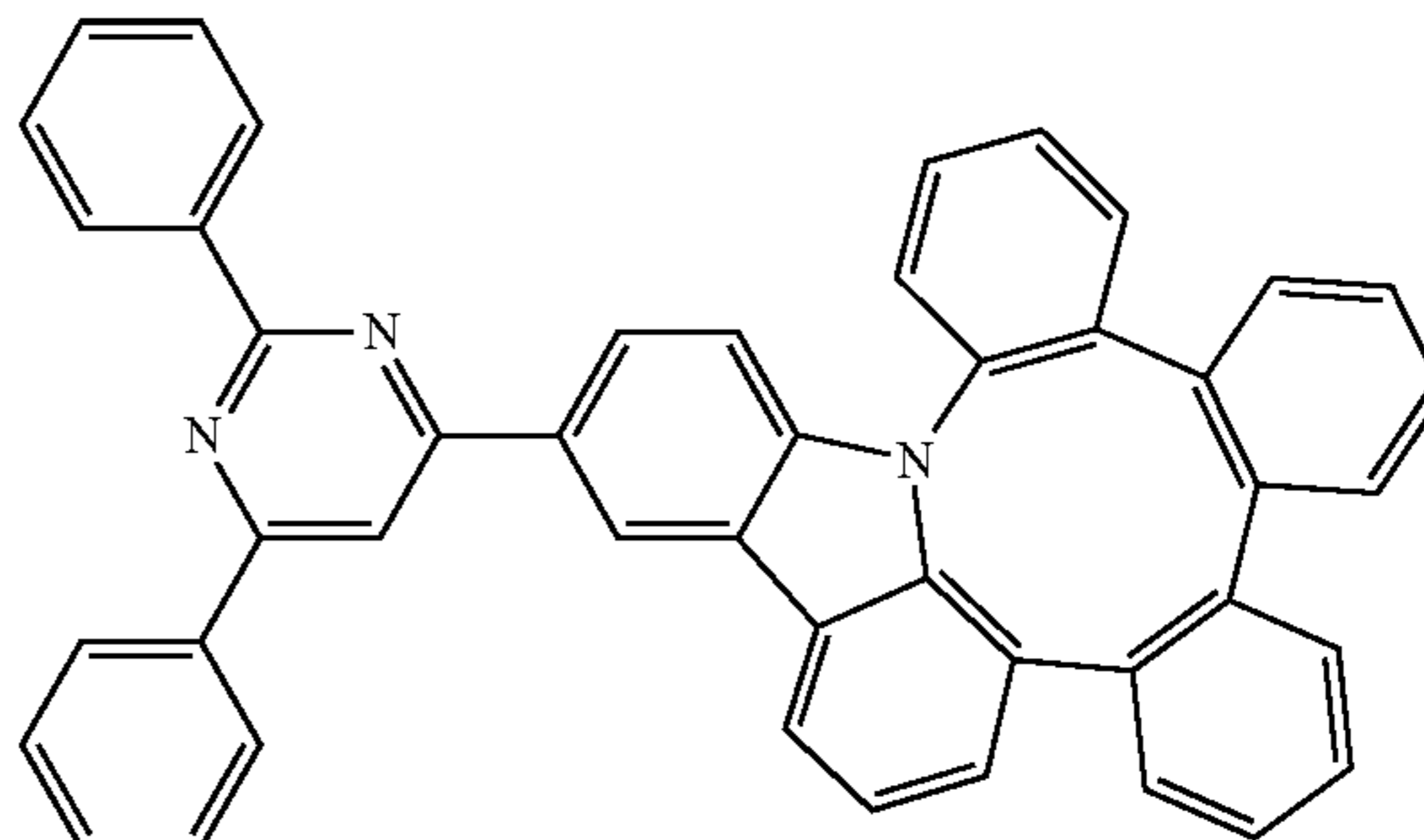
Compound 27
