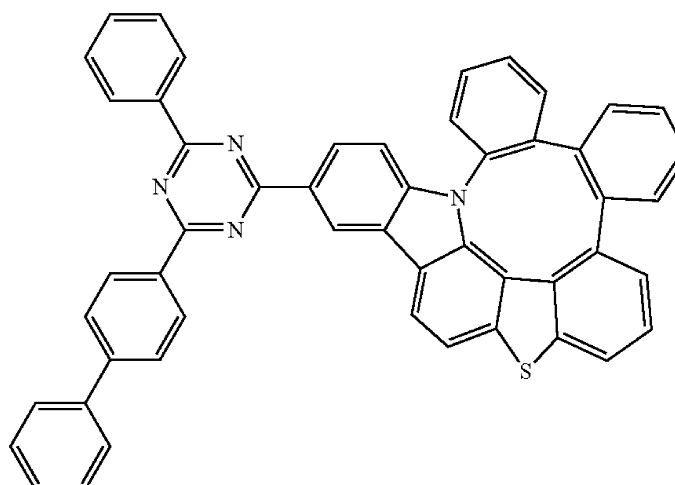
Compound 280
