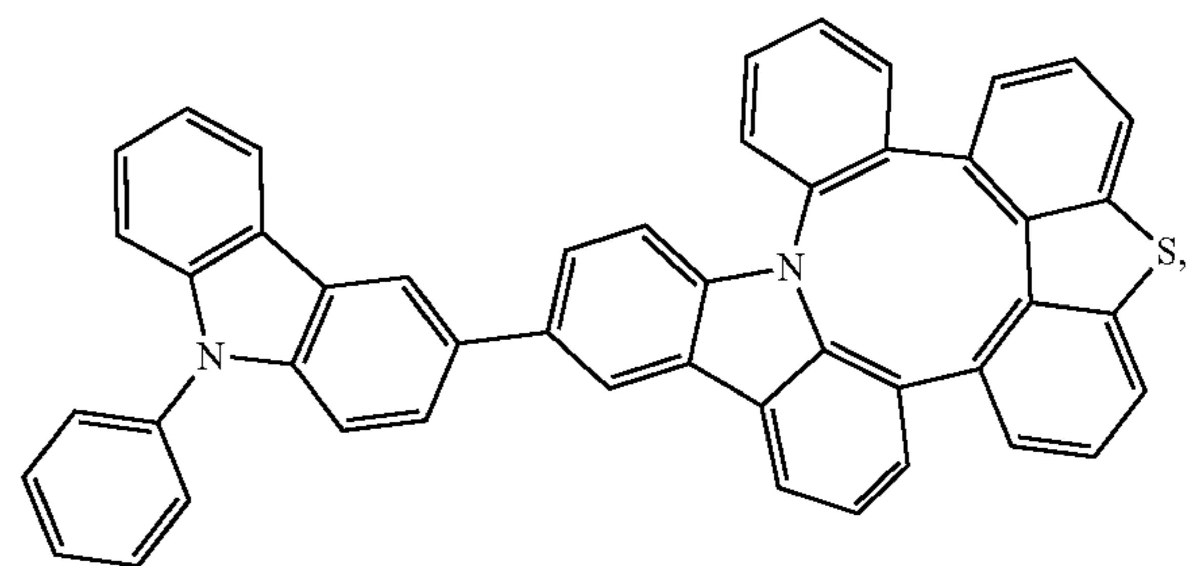
Compound 186
