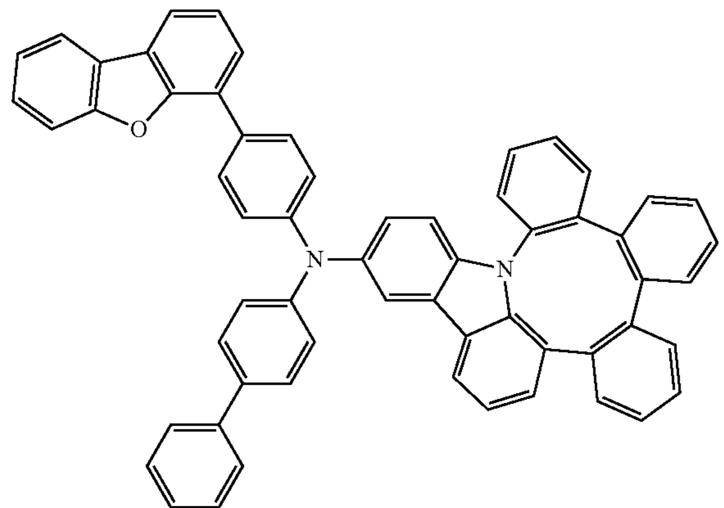
Compound 50
