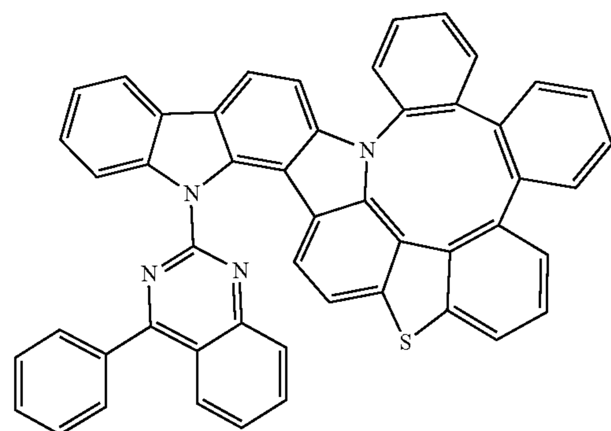
Compound 335
