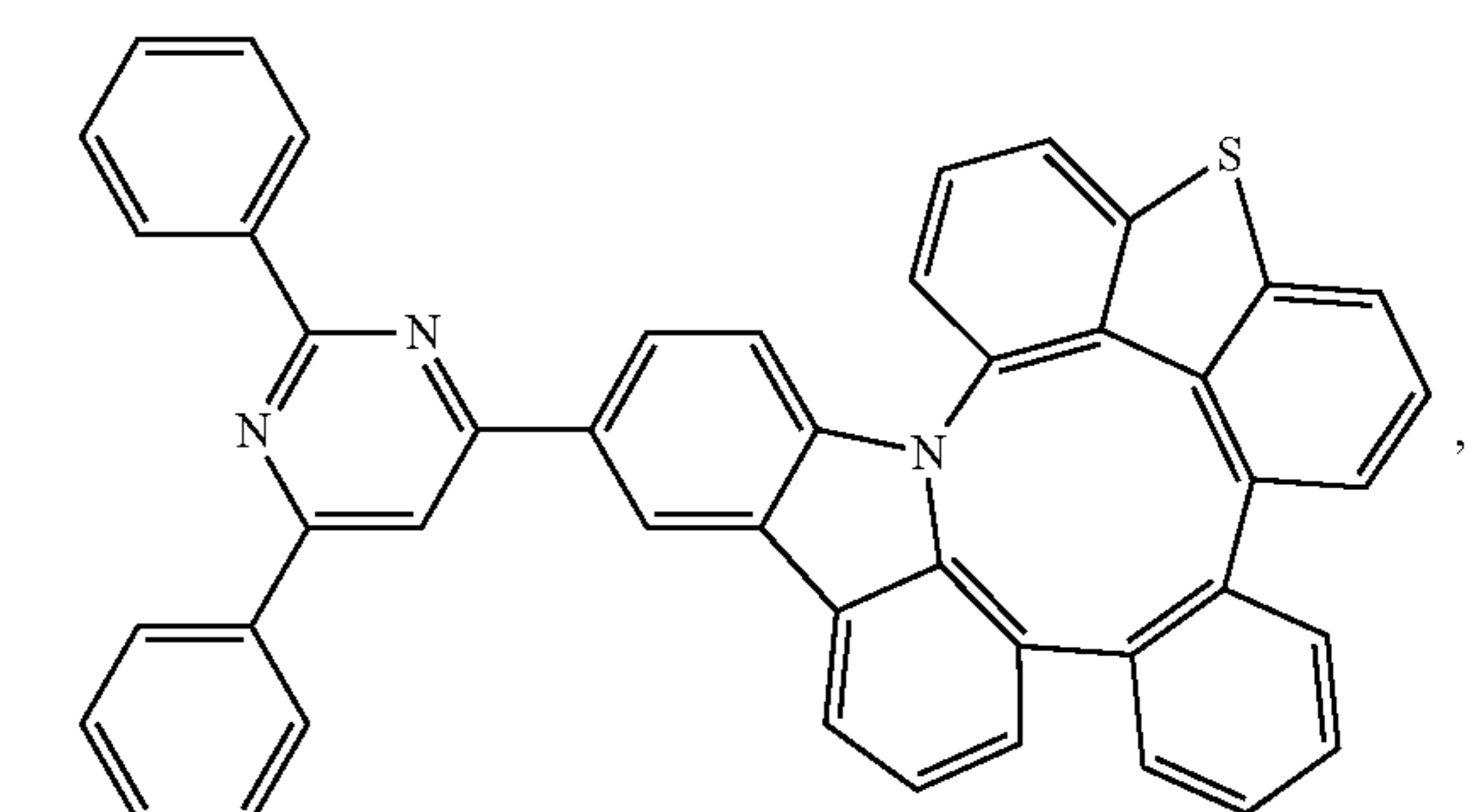
Compound 113
