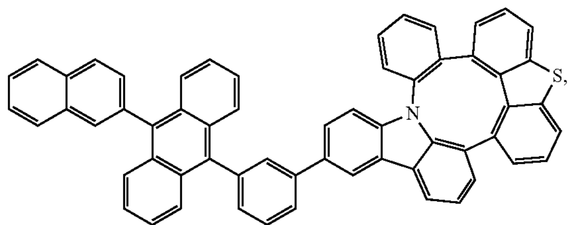
Compound 210
