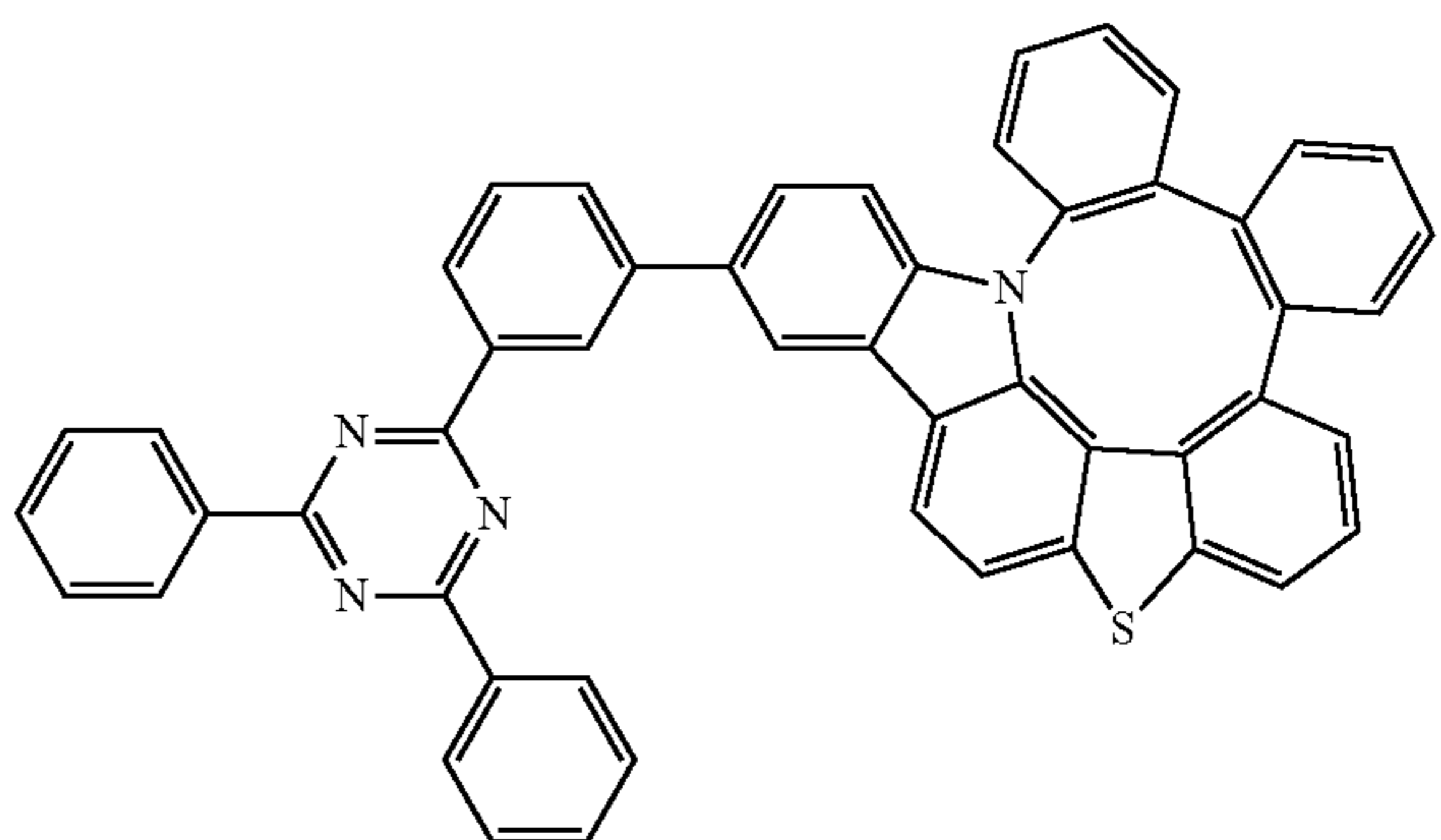
Compound 285
