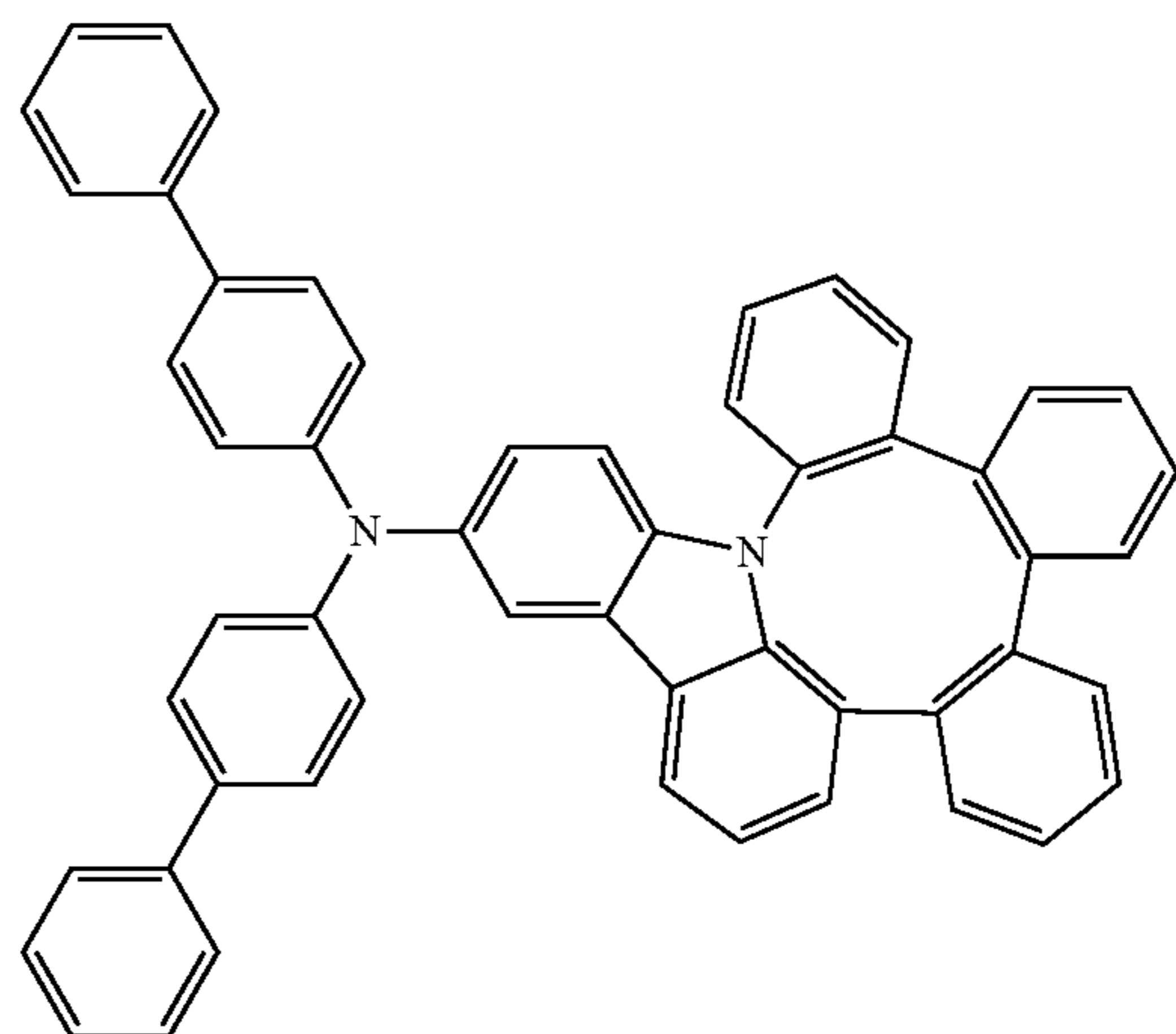
Compound 42
