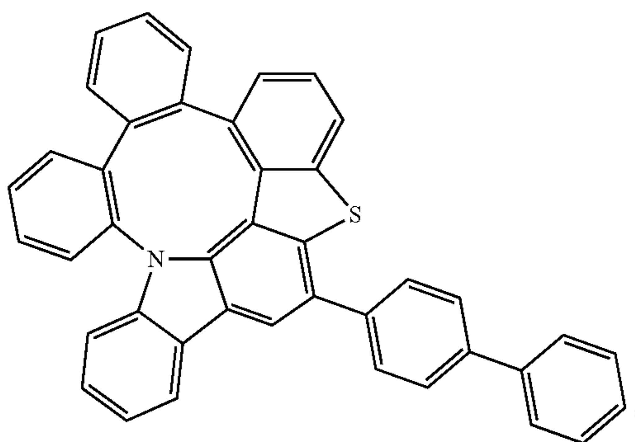
Compound 258
