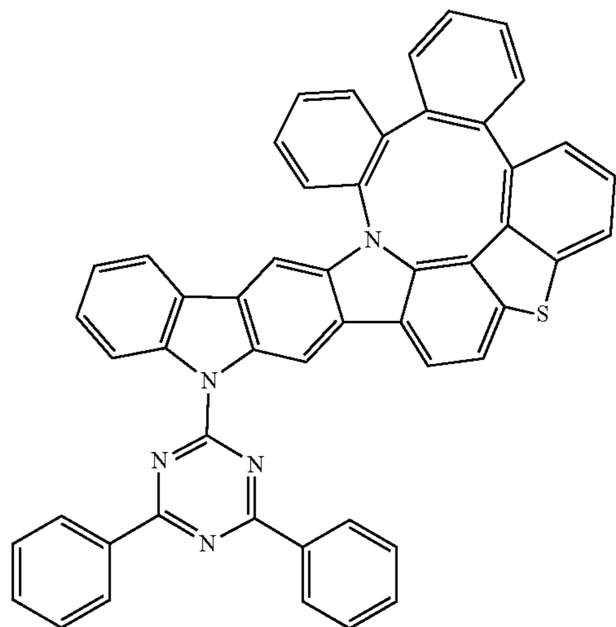
Compound 333
