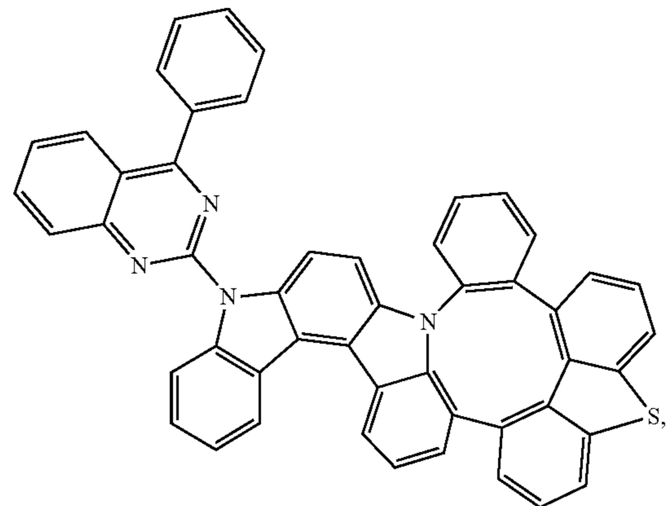
Compound 252
