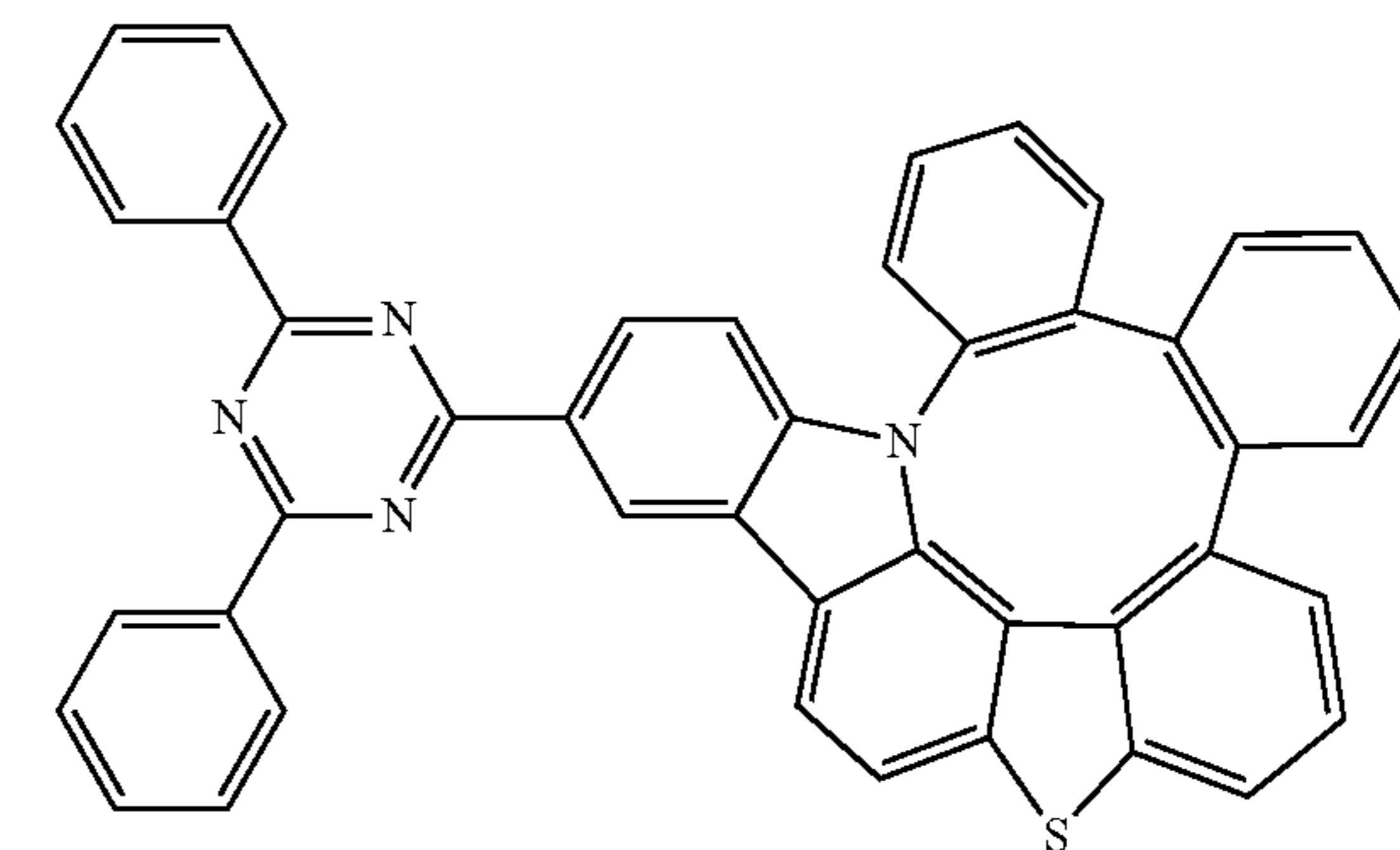
Compound 280
