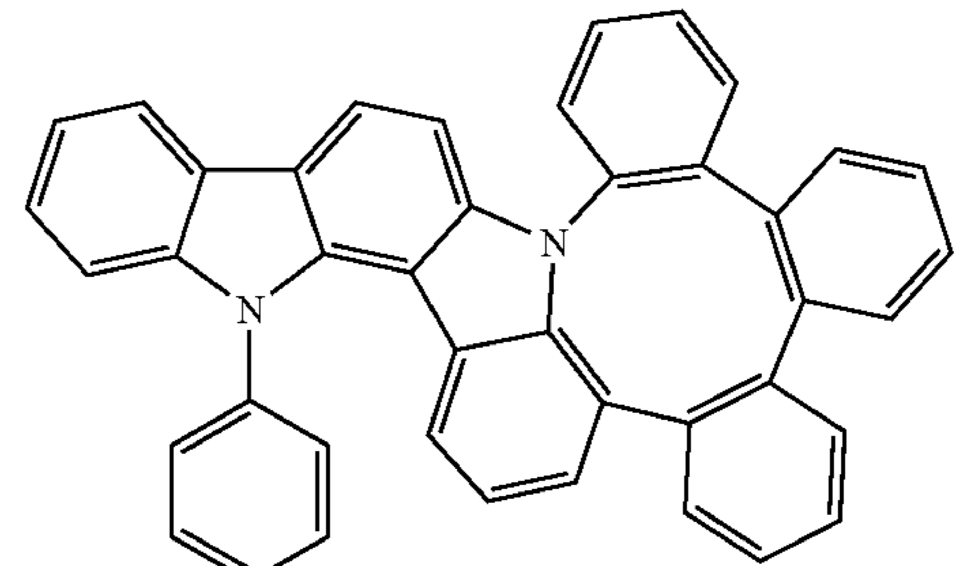
Compound 56
