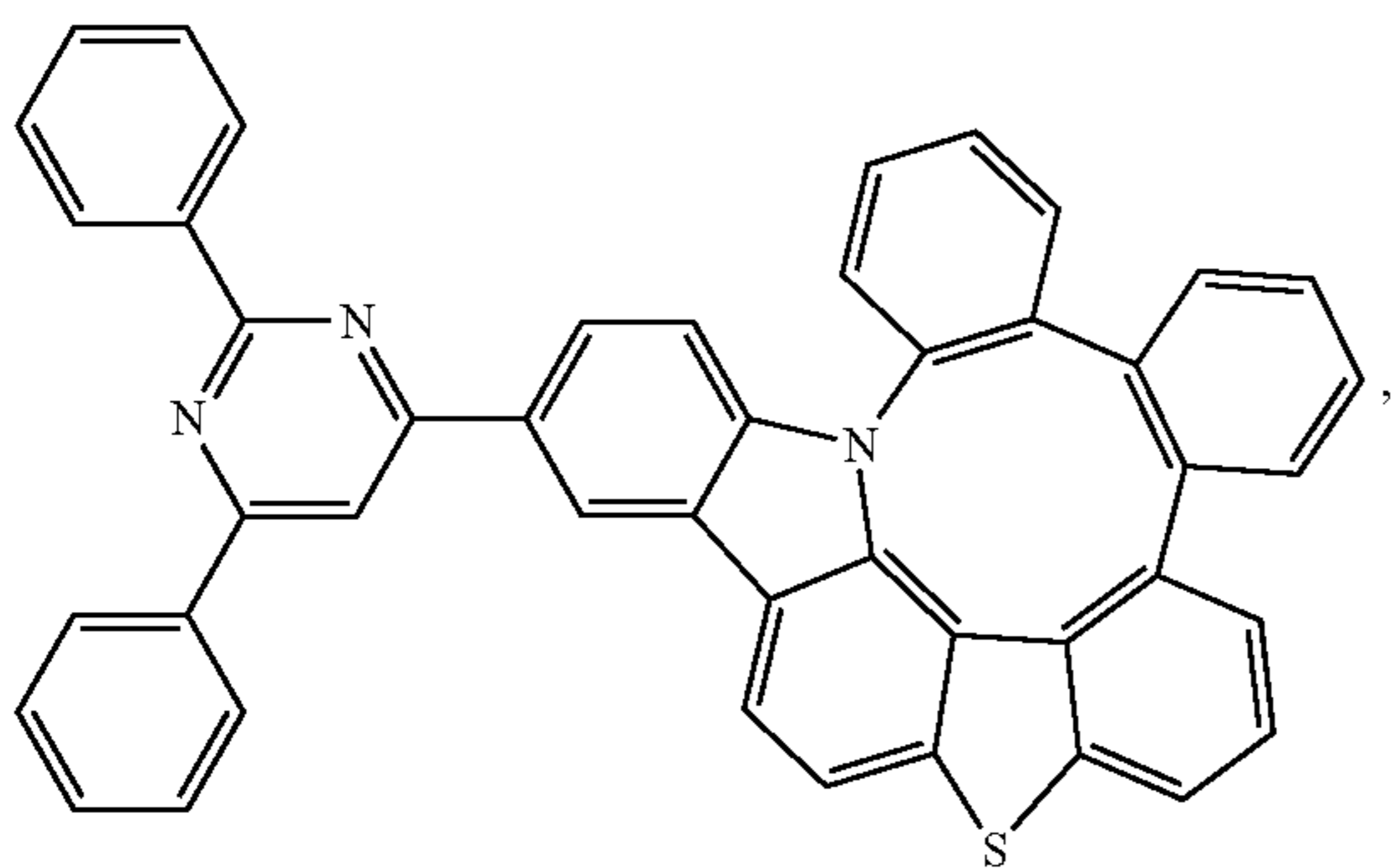
Compound 282
