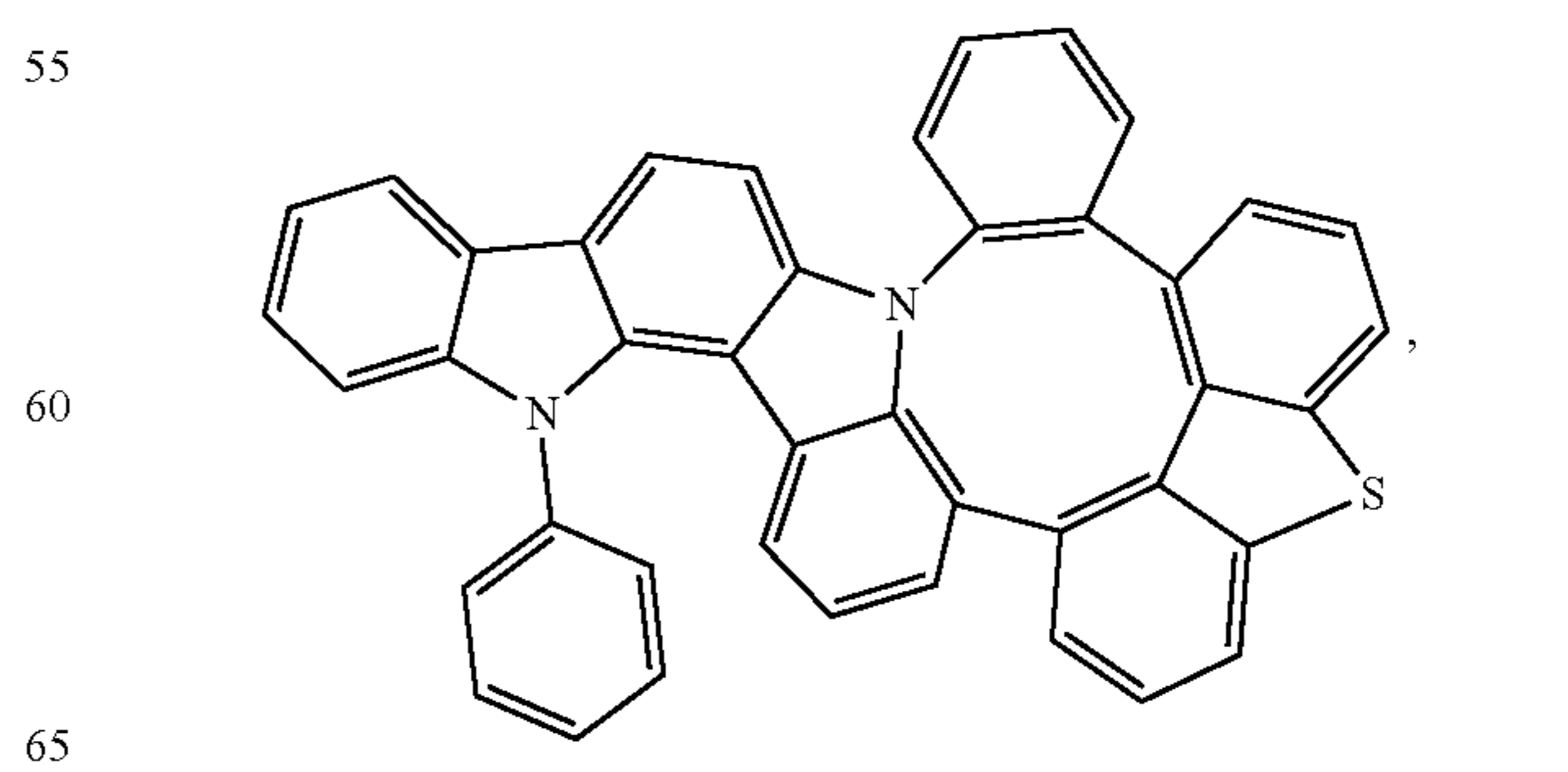
Compound 220
