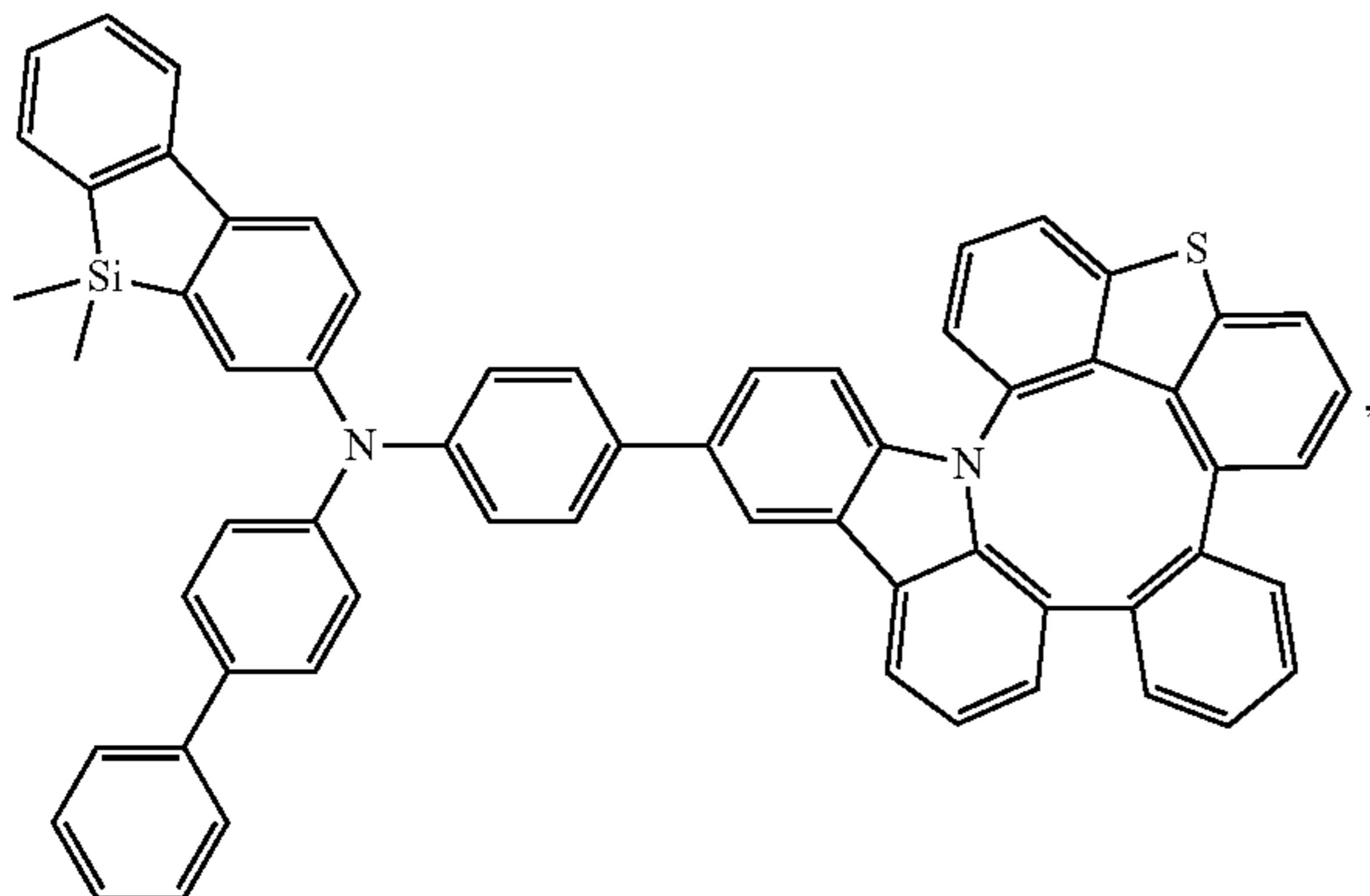
Compound 354
