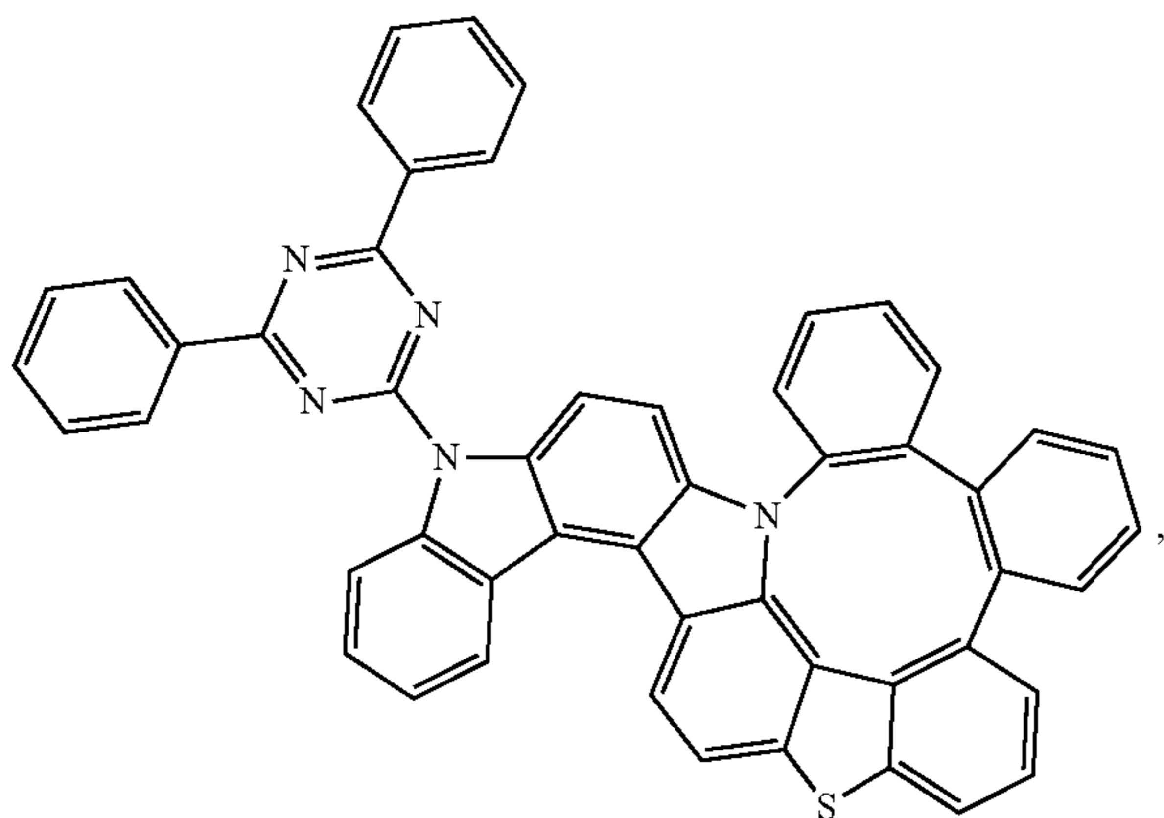
Compound 331
