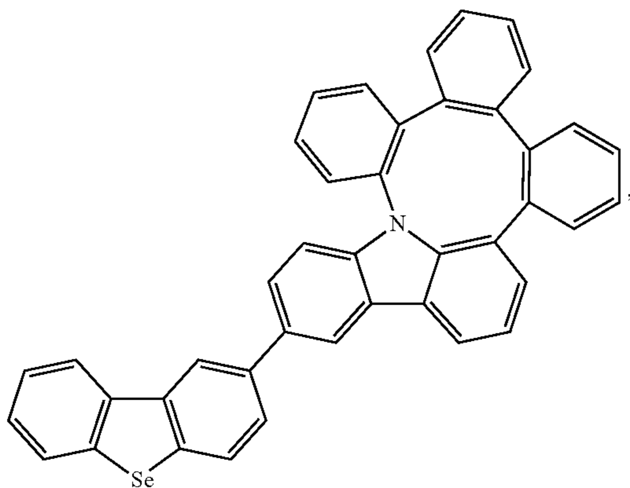
Compound 11
