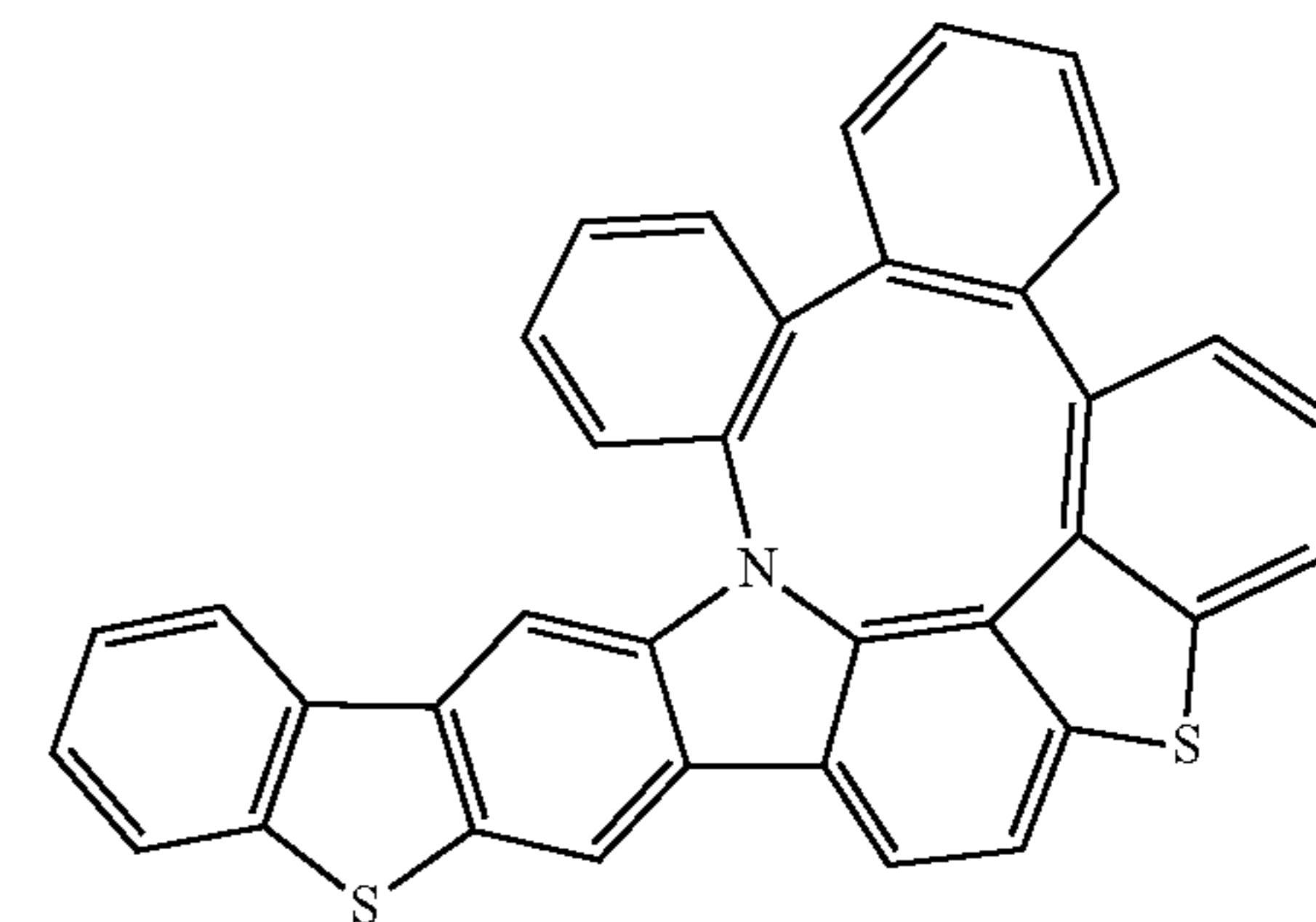
Compound 321
