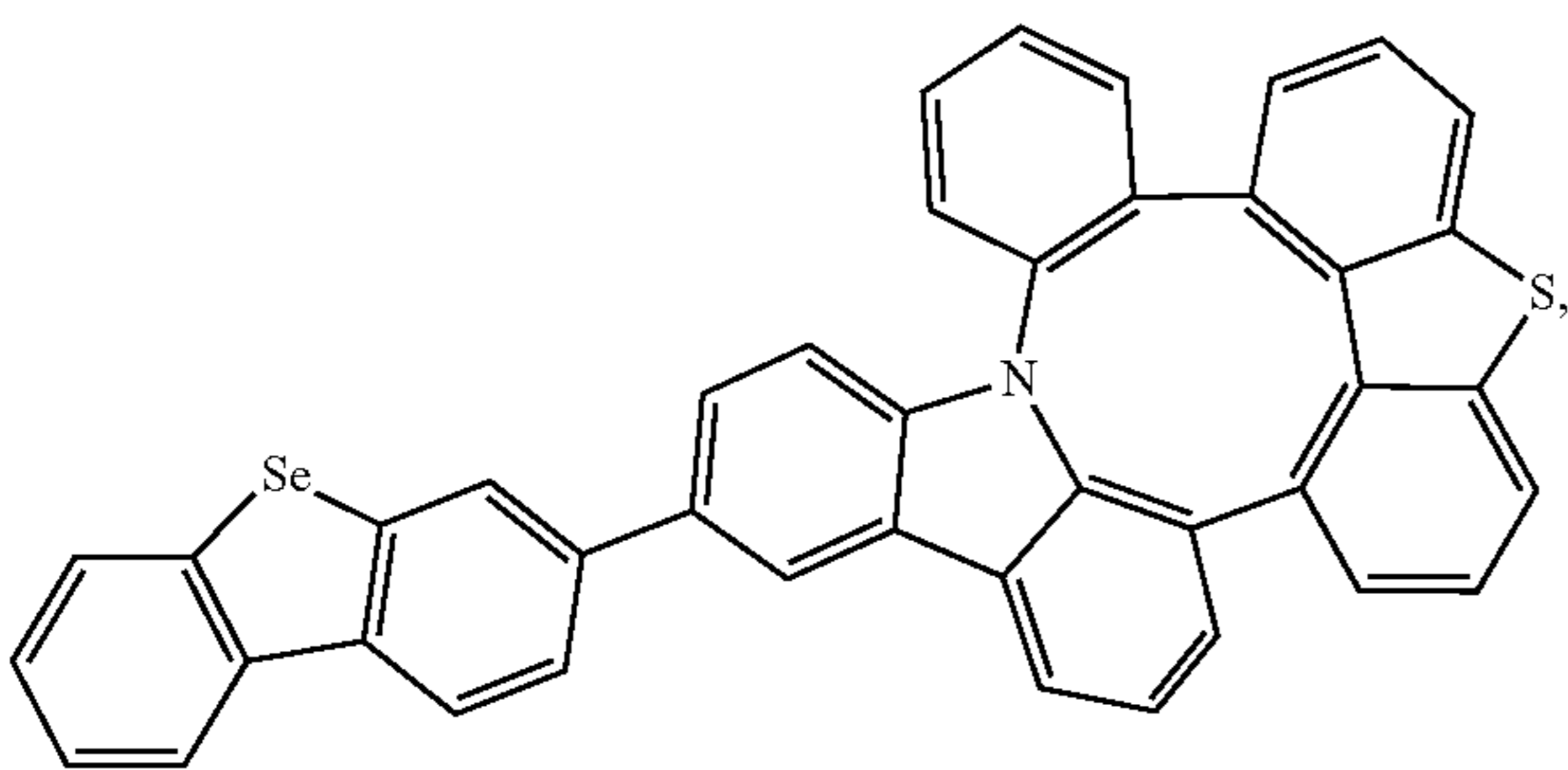
Compound 182
