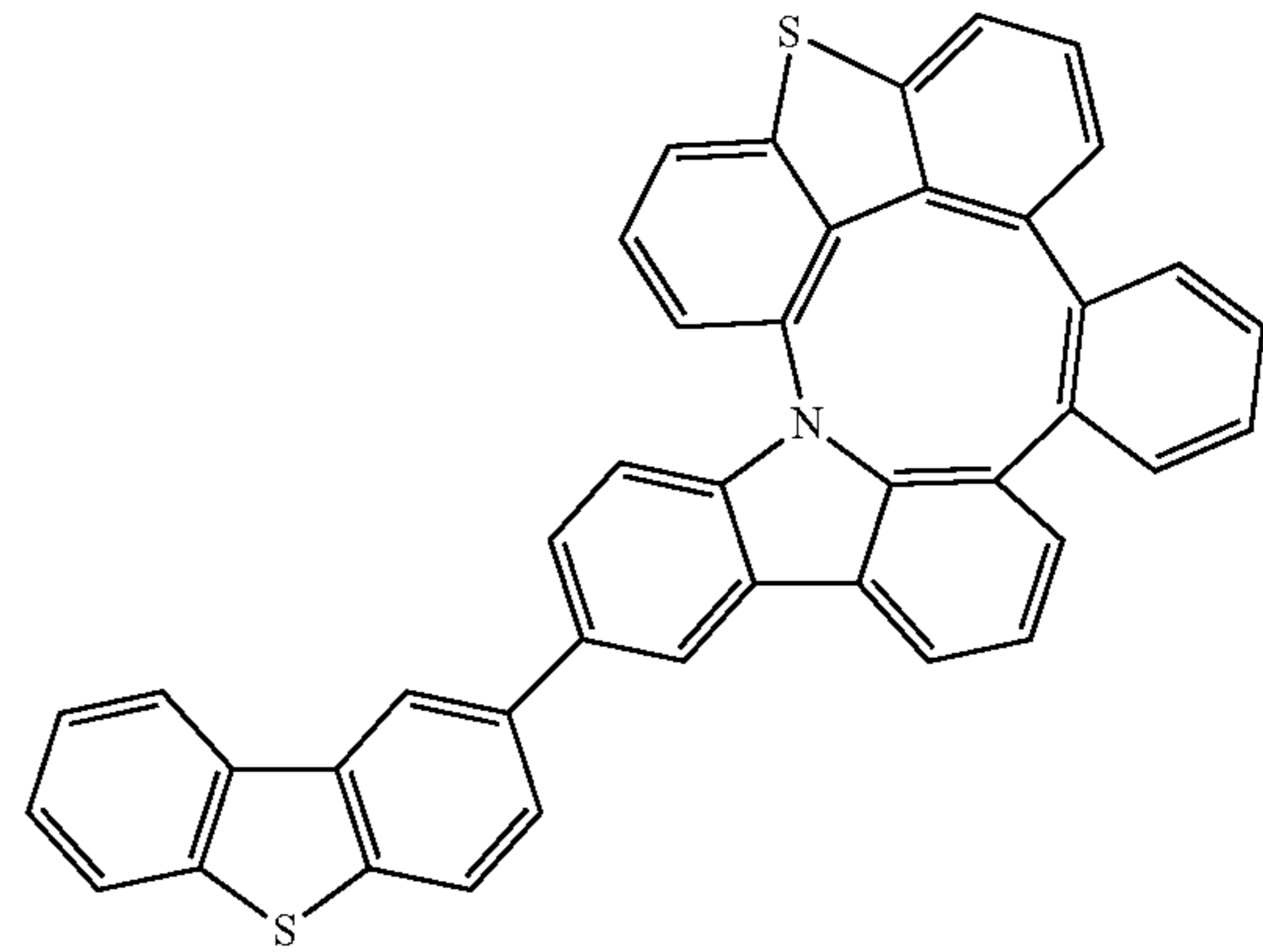
Compound 94
