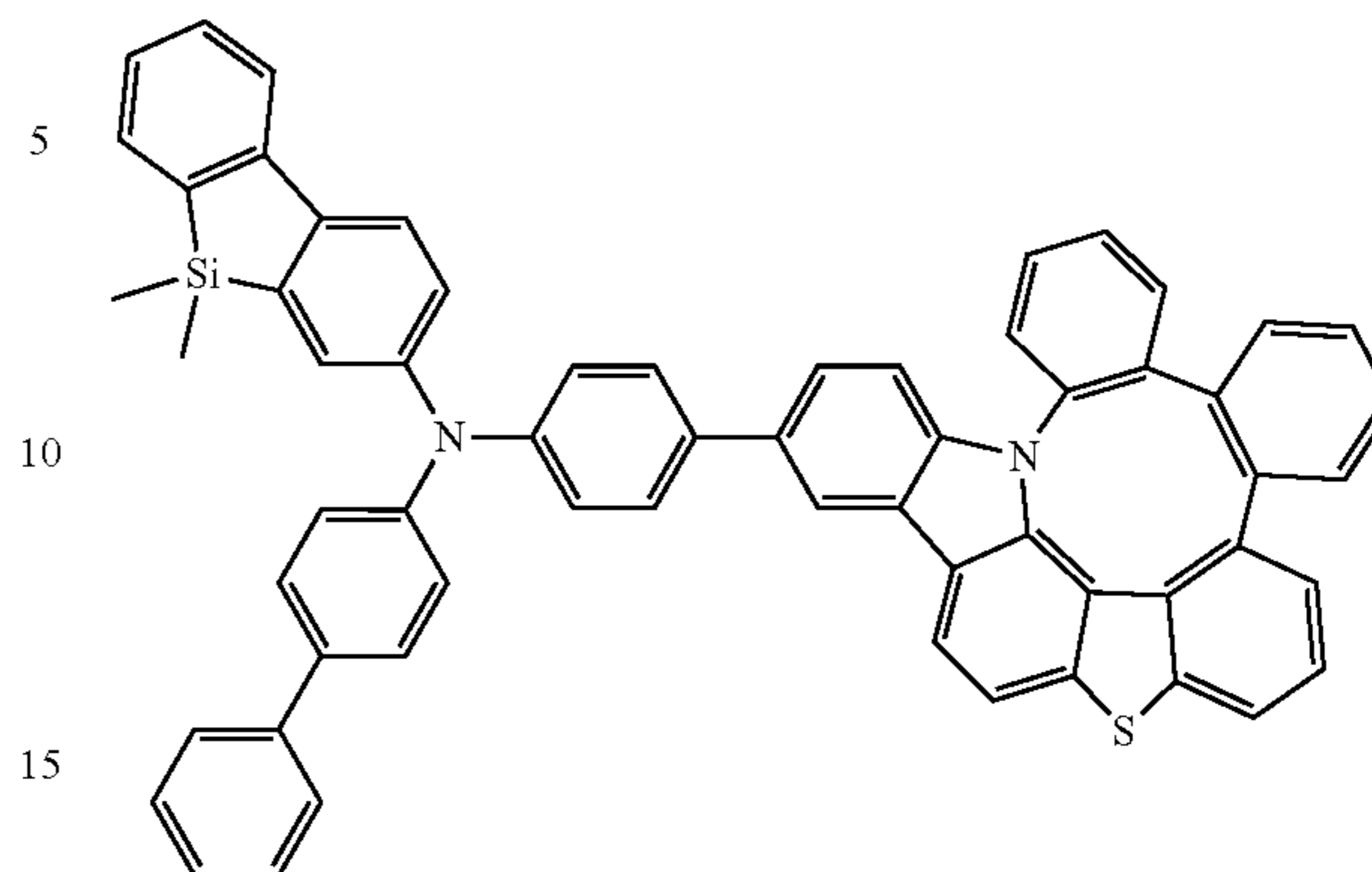
Compound 365
