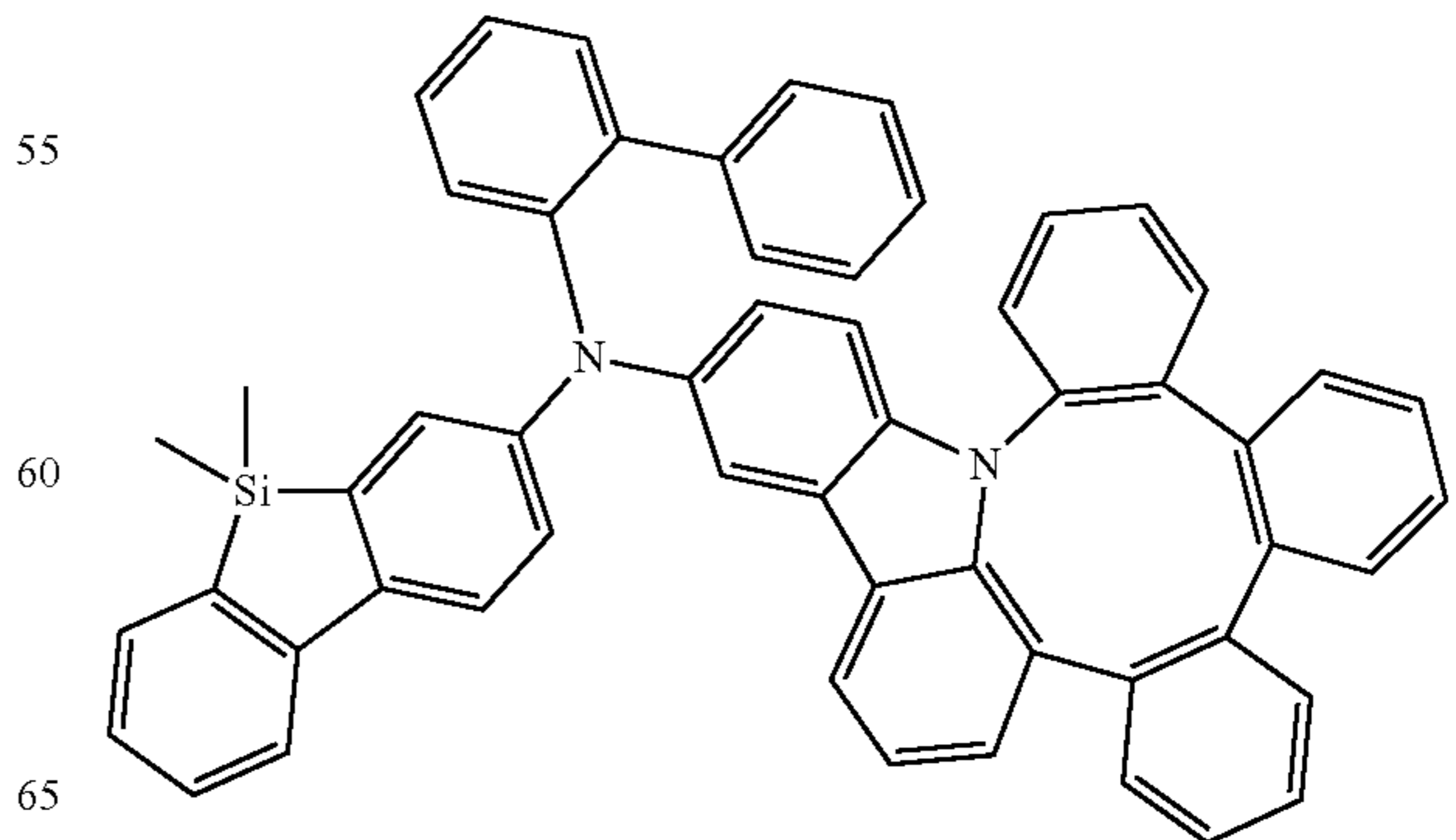
Compound 345
