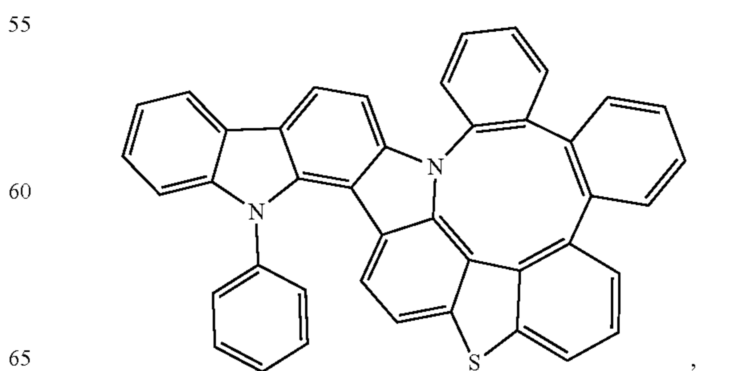
Compound 305
