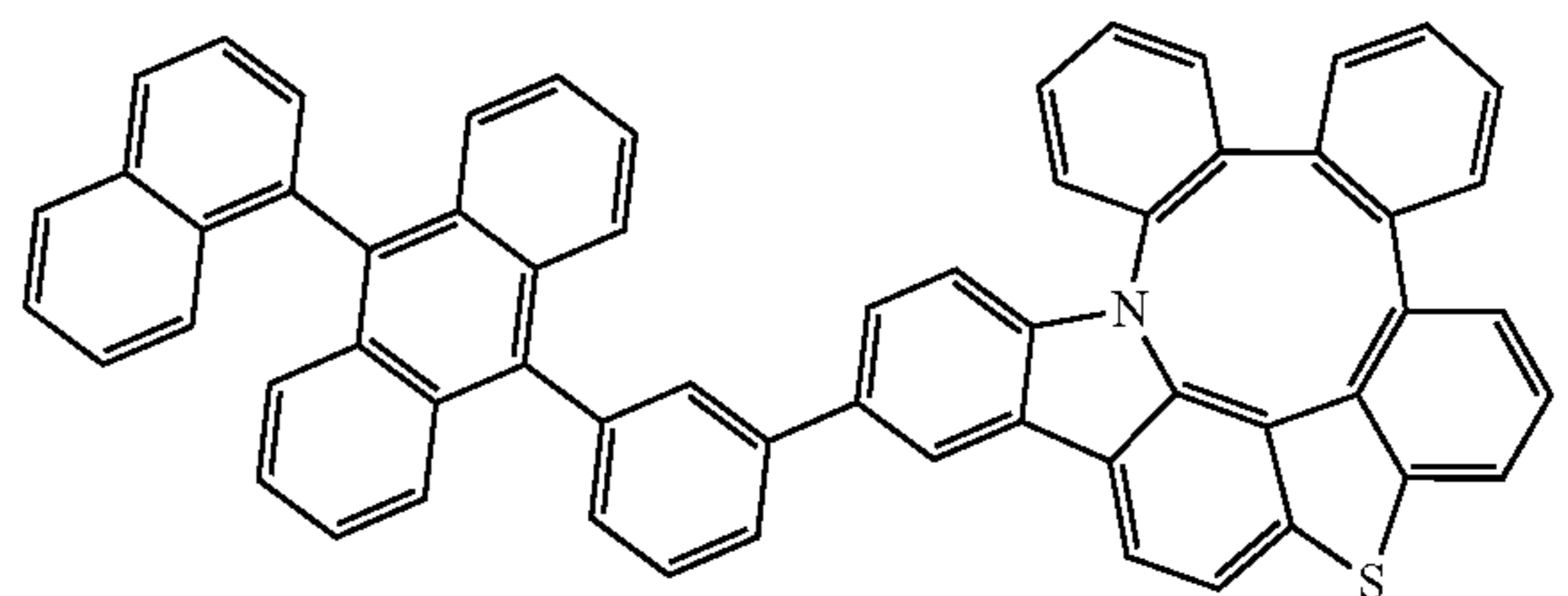
Compound 294
