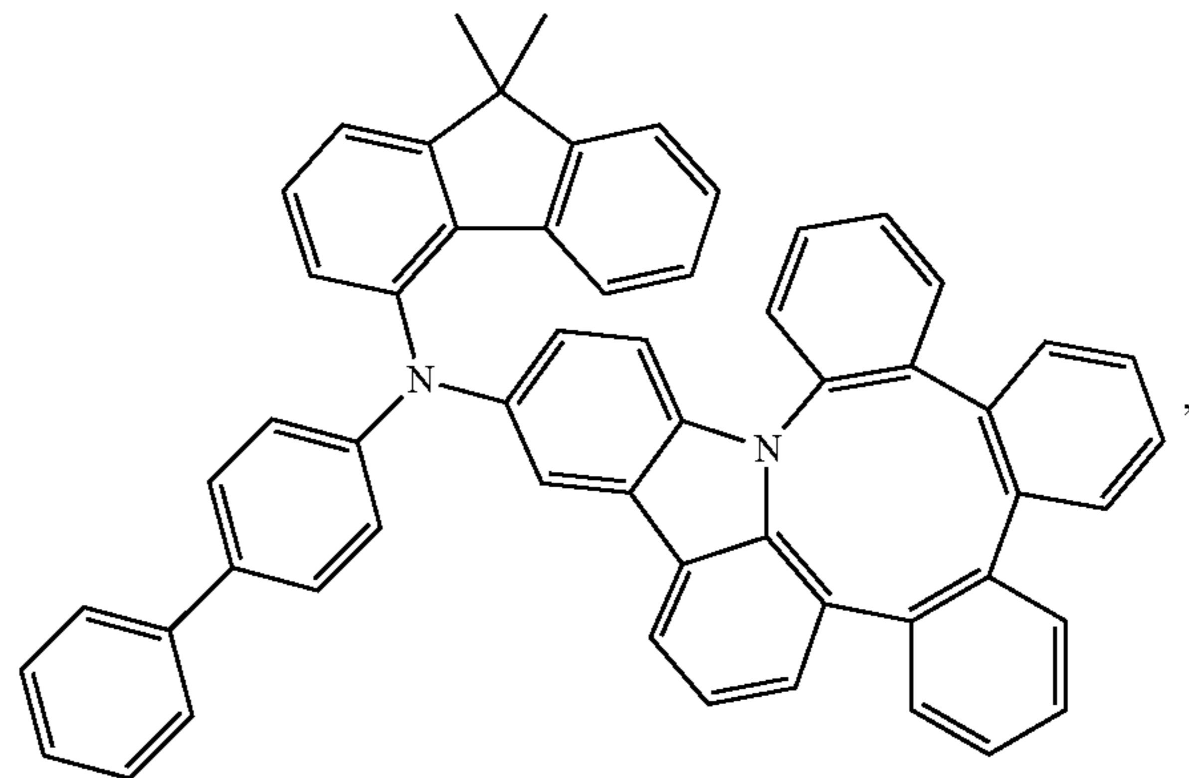
Compound 44
