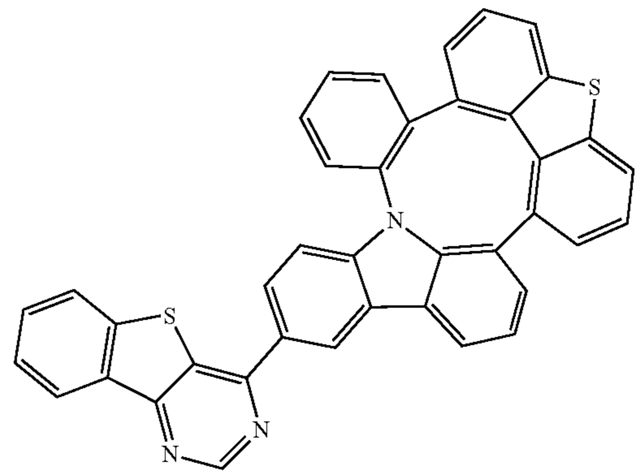
Compound 203
