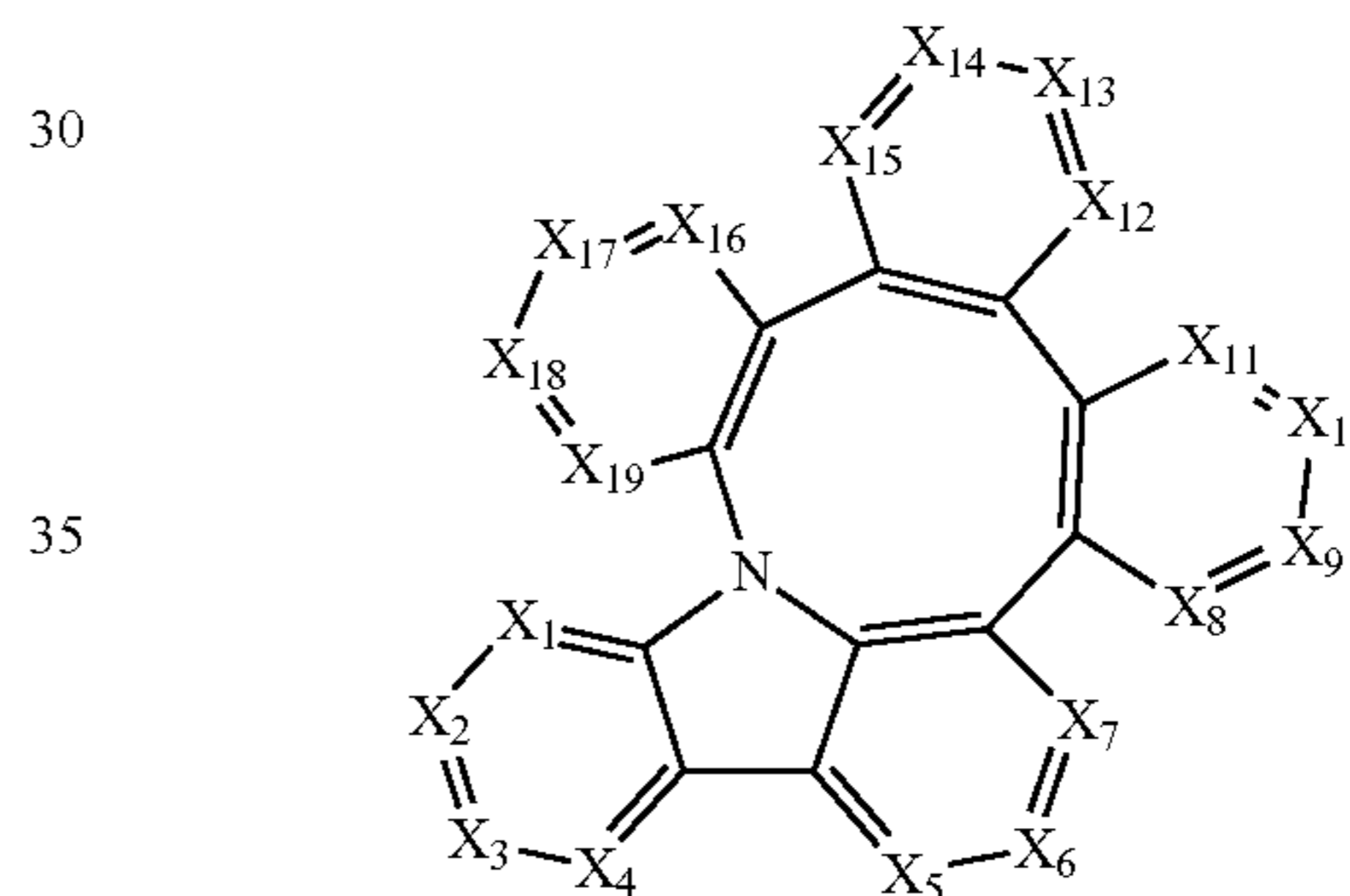
Compound 366
