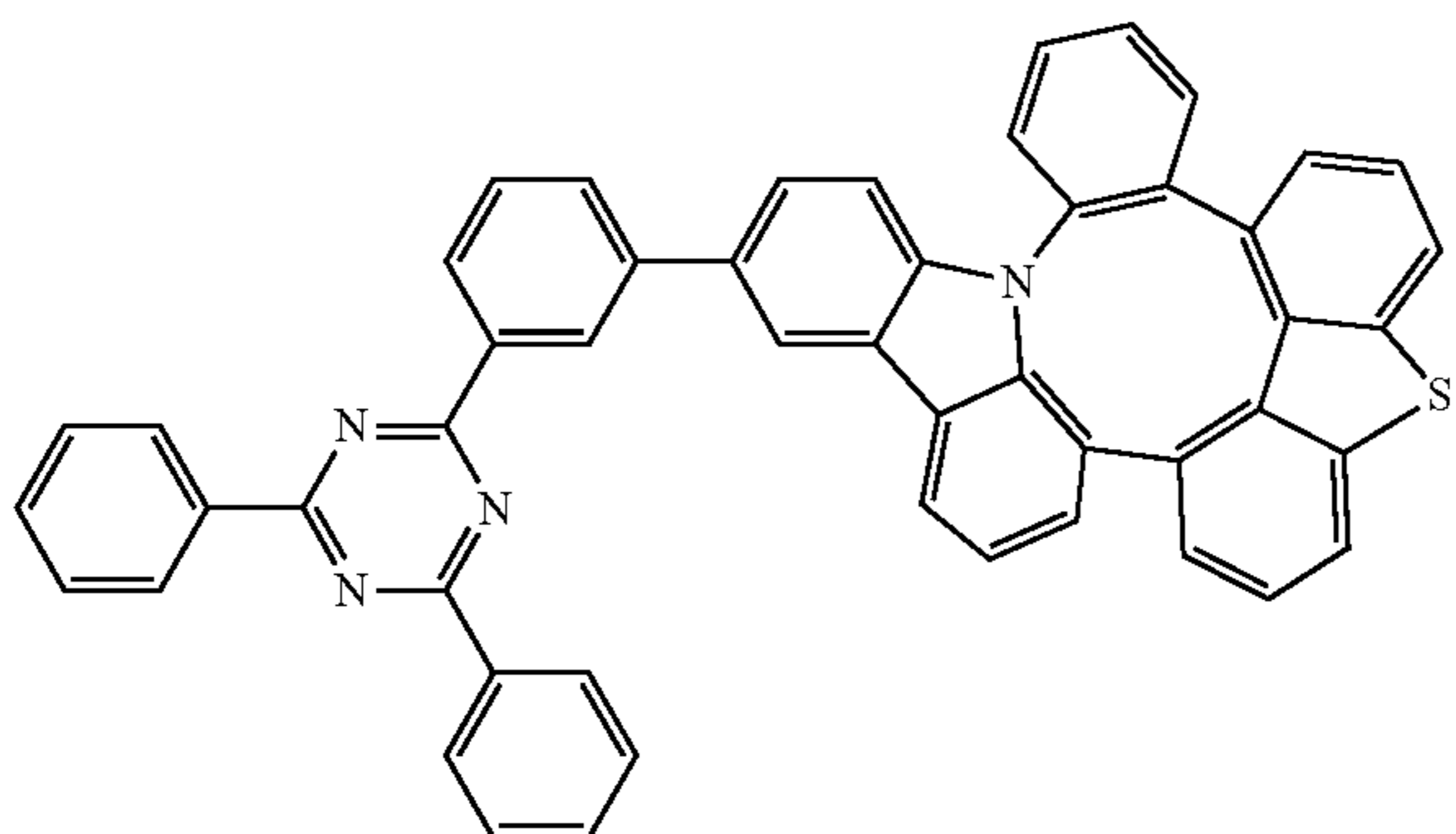
Compound 200
