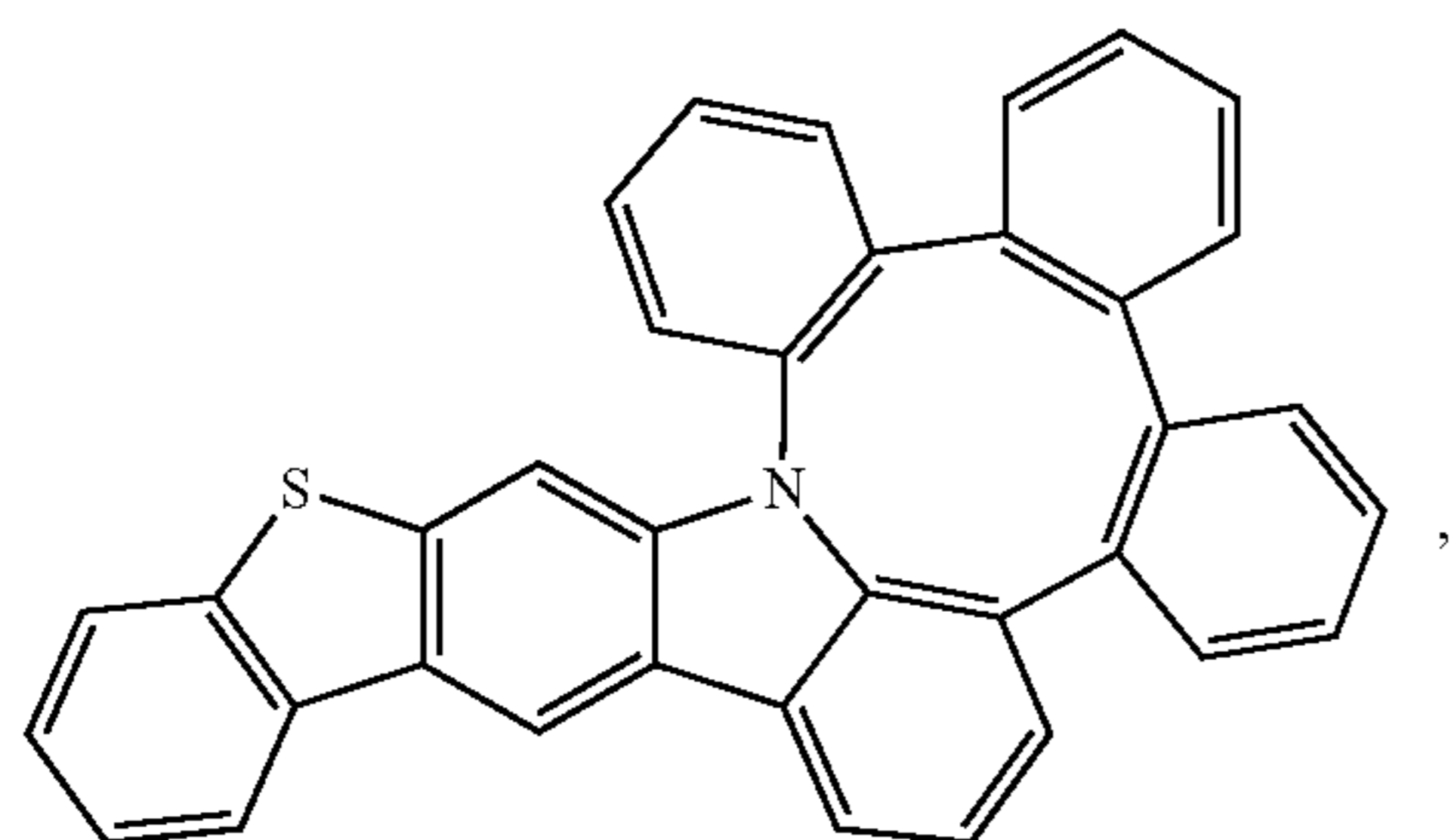
Compound 64
