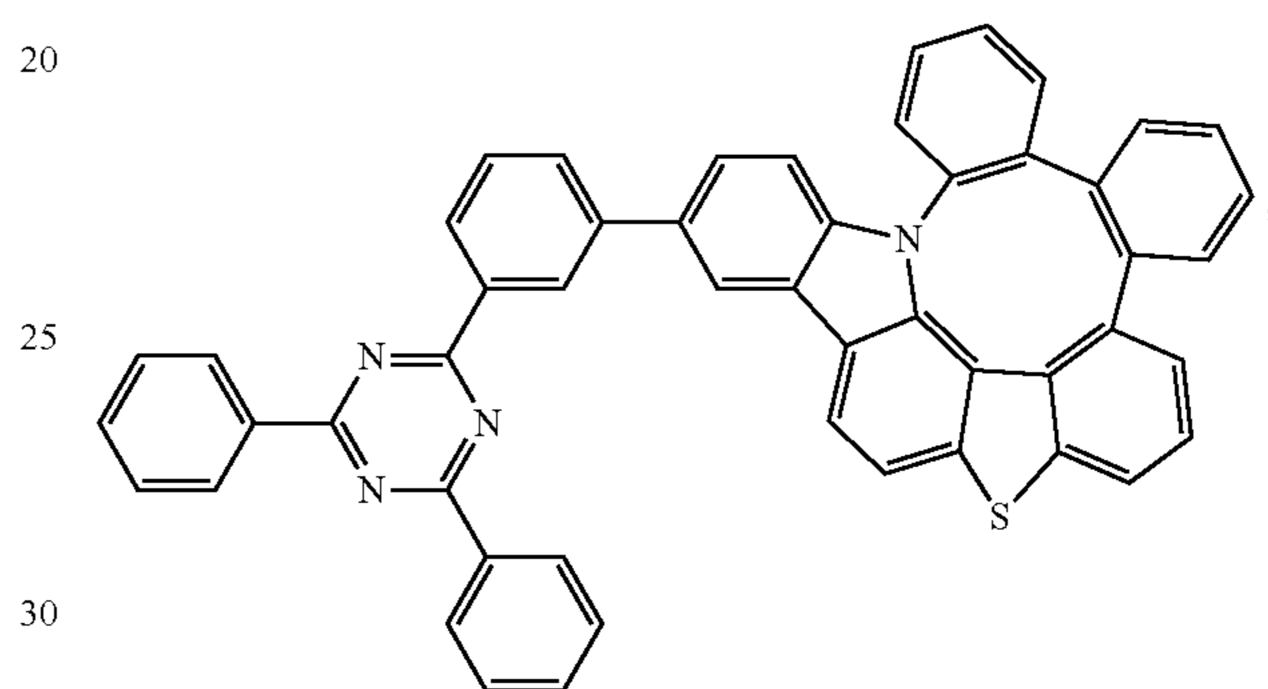
Compound 285
