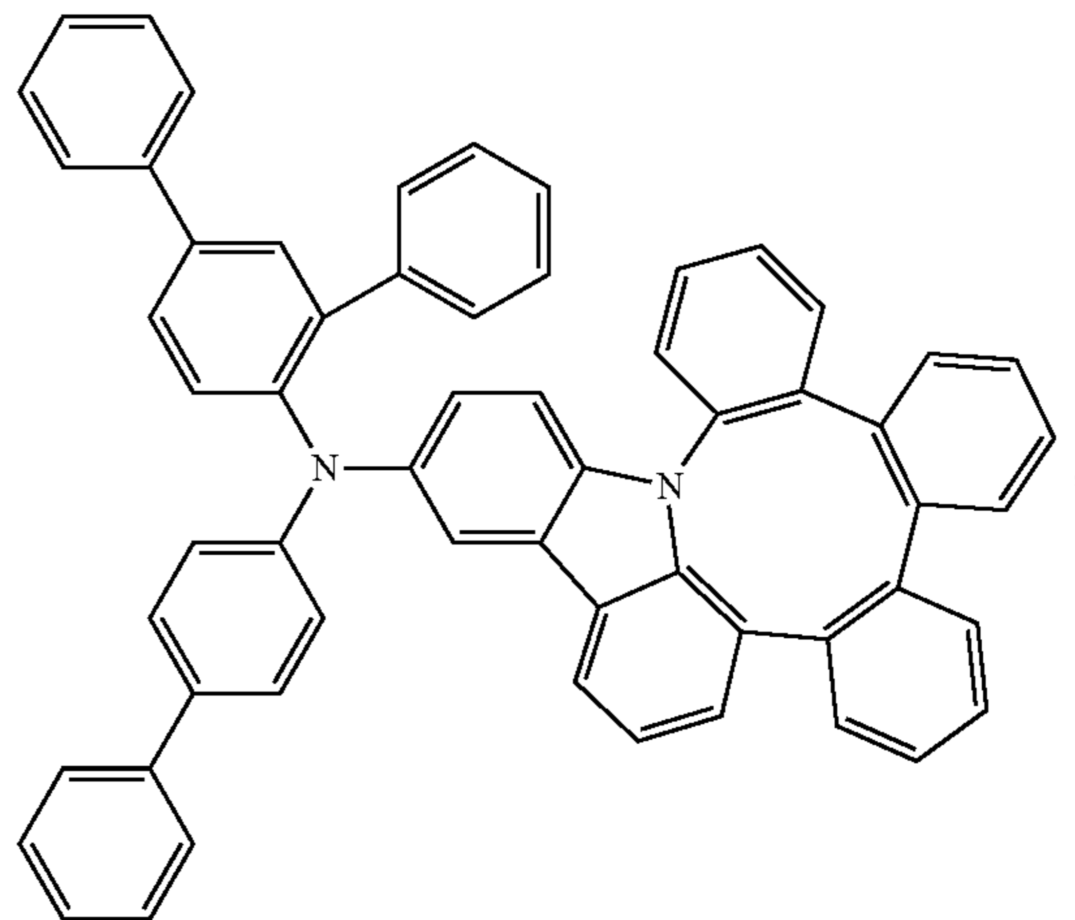
Compound 45
