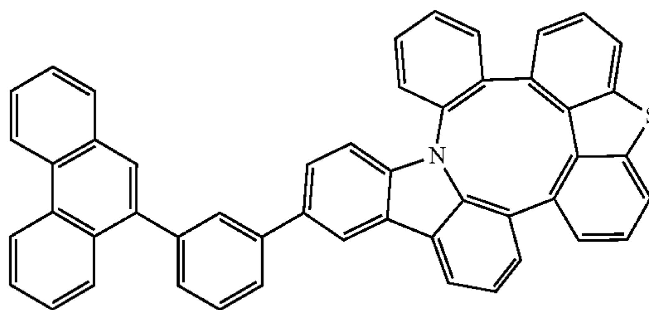
Compound 205
