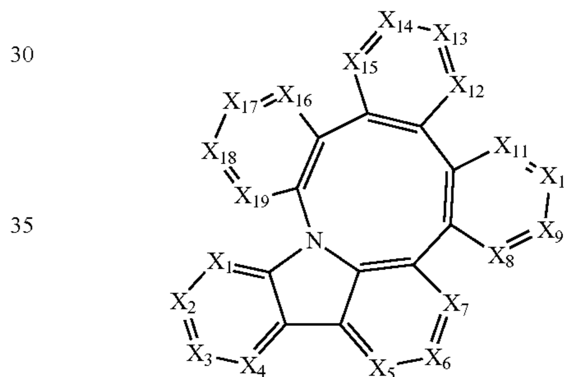
Compound 366
