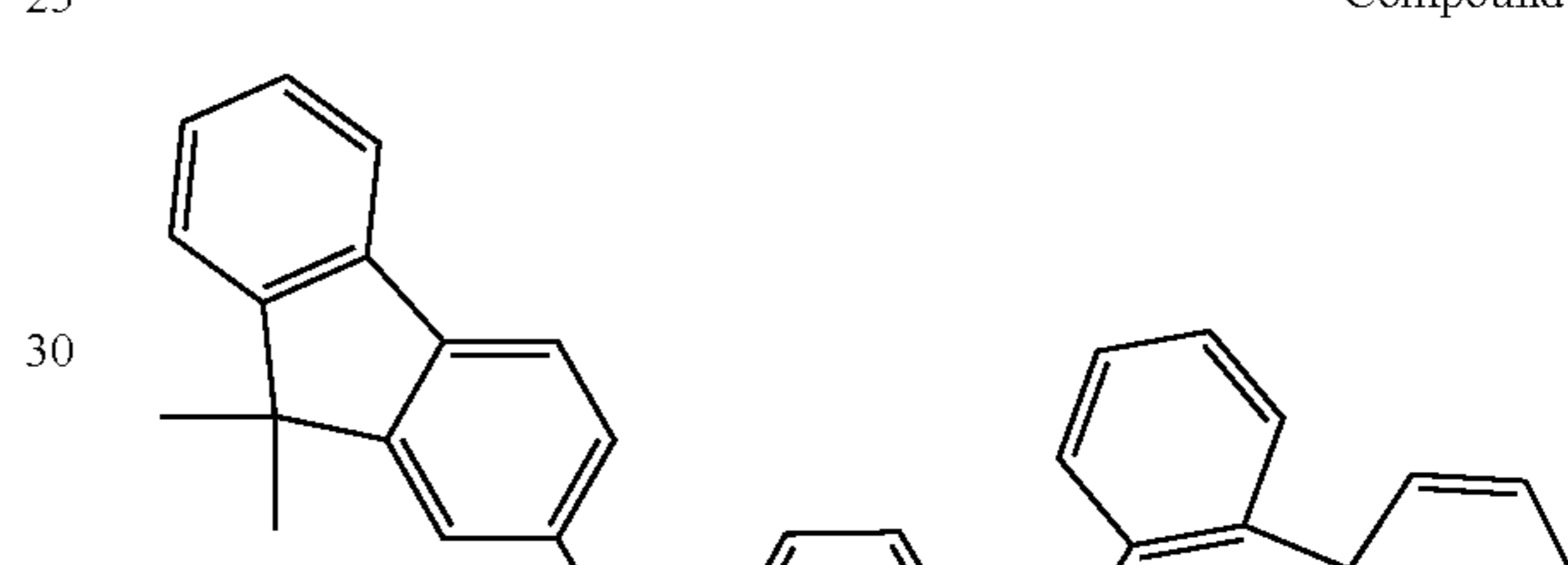
Compound 208
