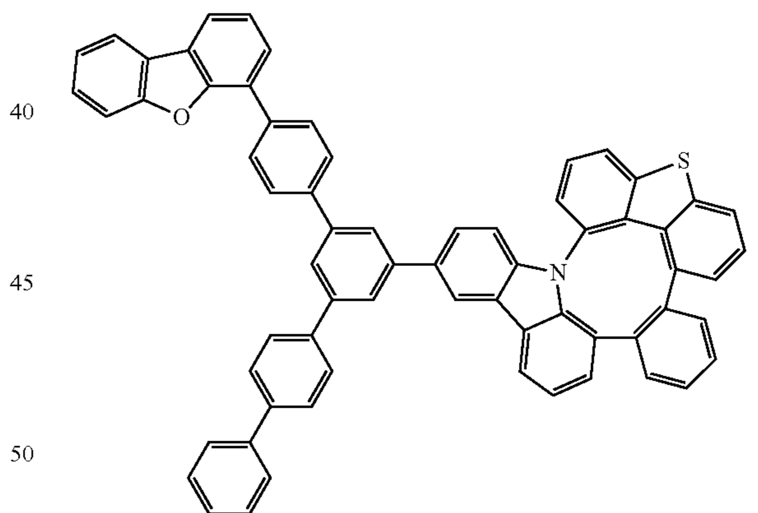
Compound 135
