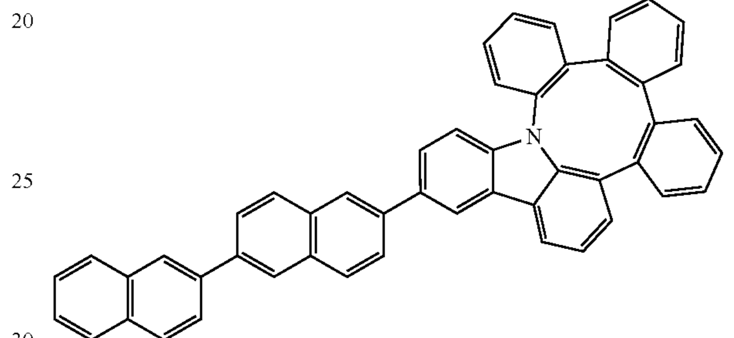
Compound 36
