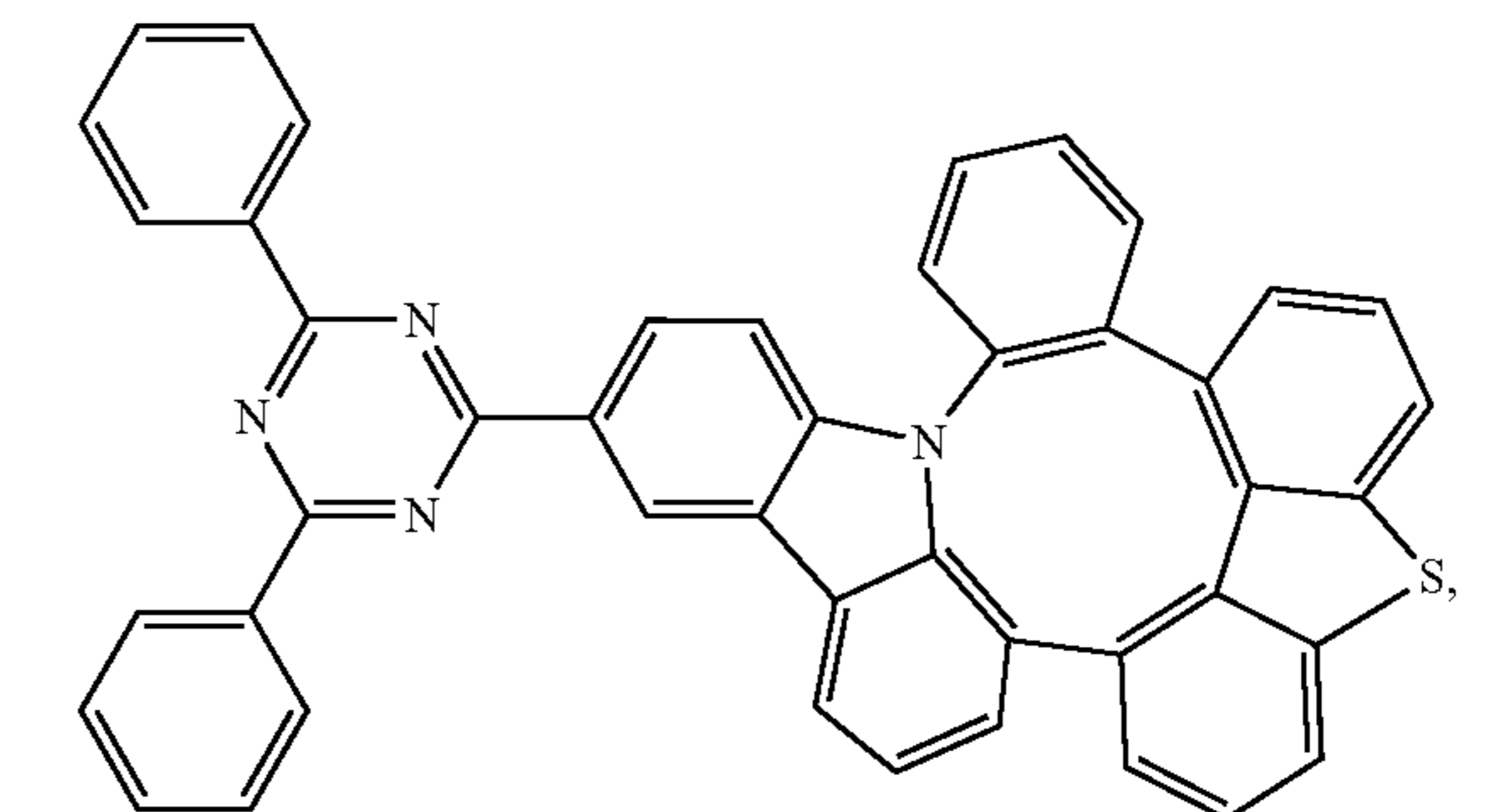
Compound 195
