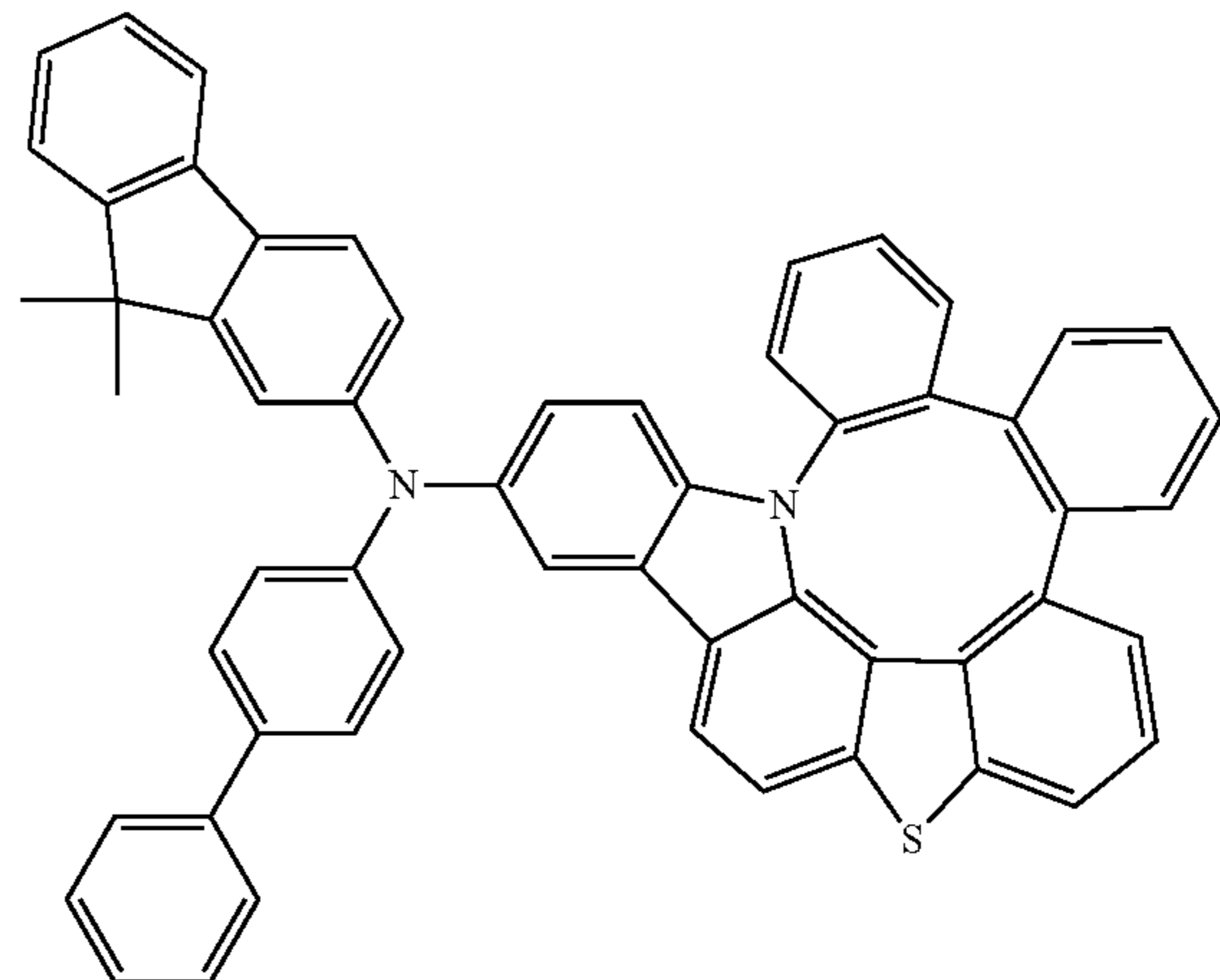
Compound 297
