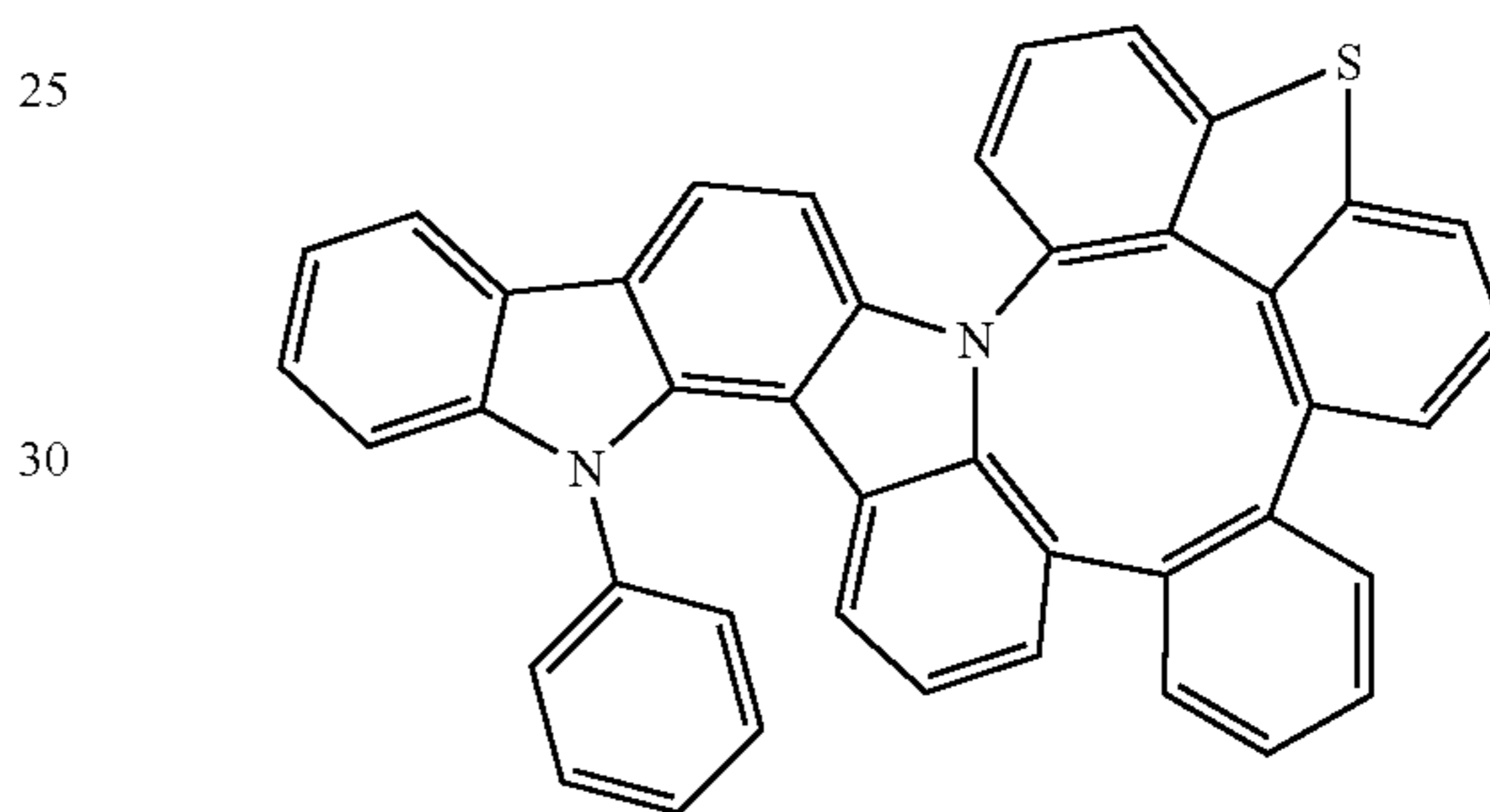
Compound 135
