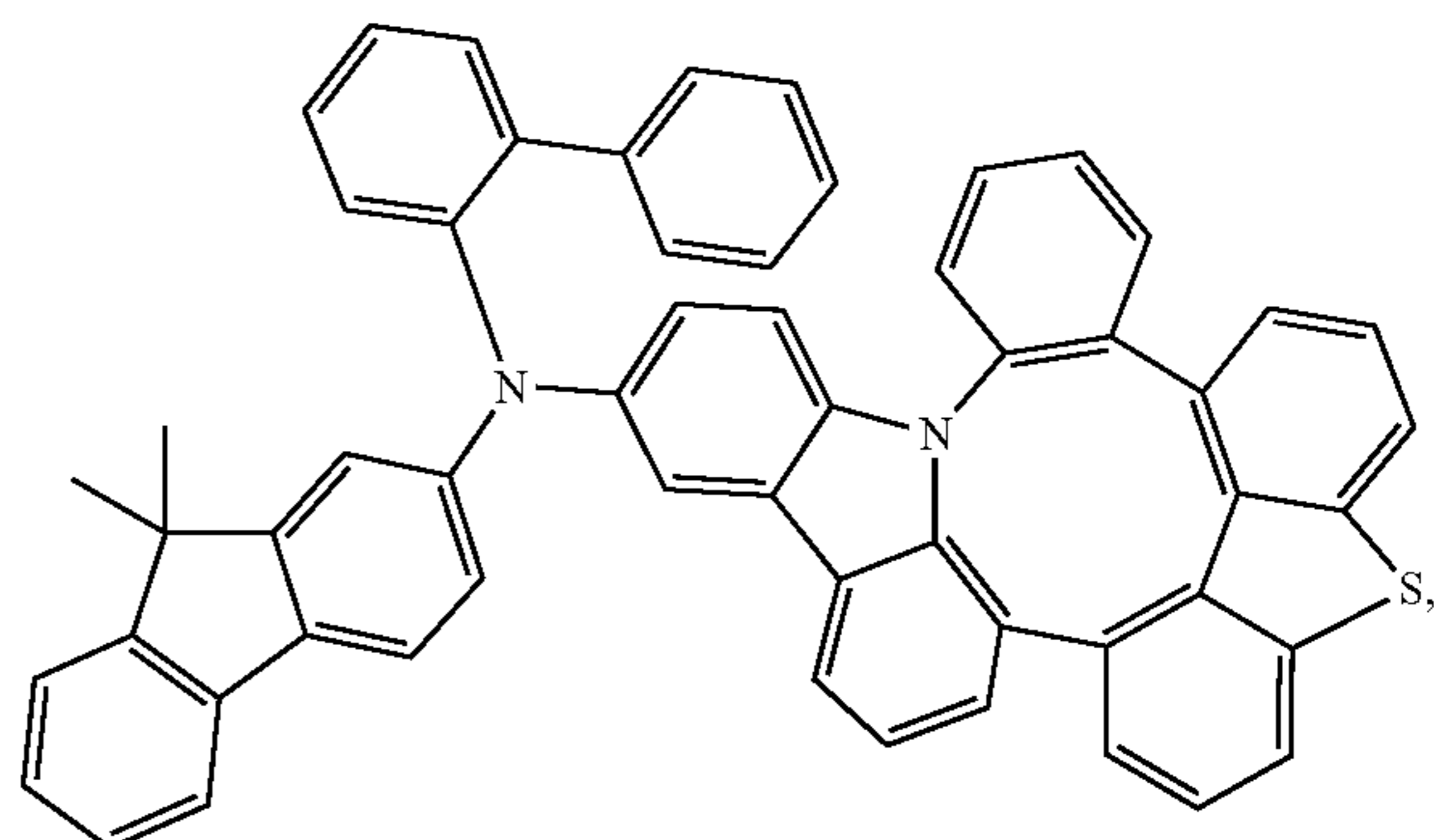
Compound 213
