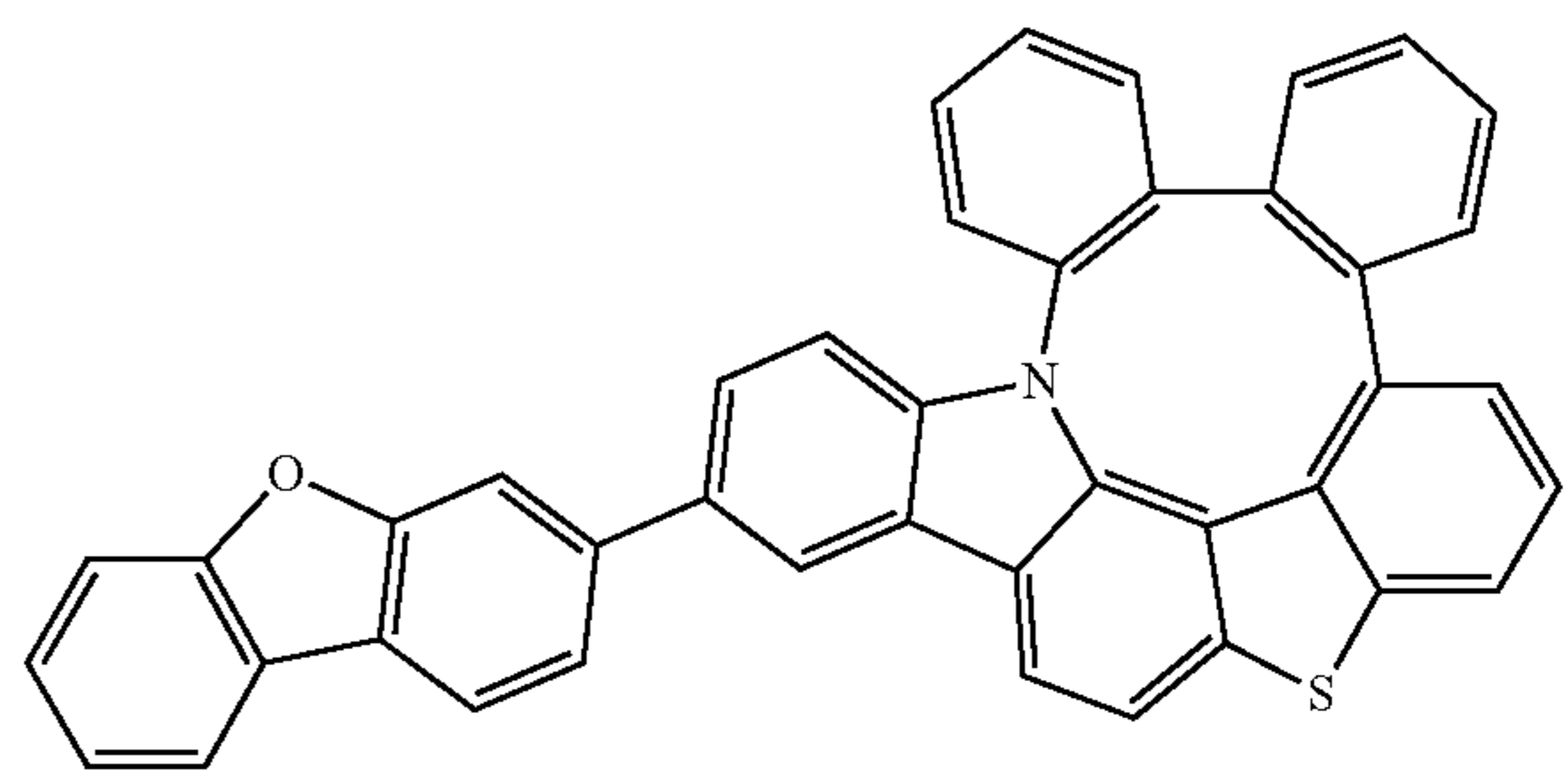
Compound 262
