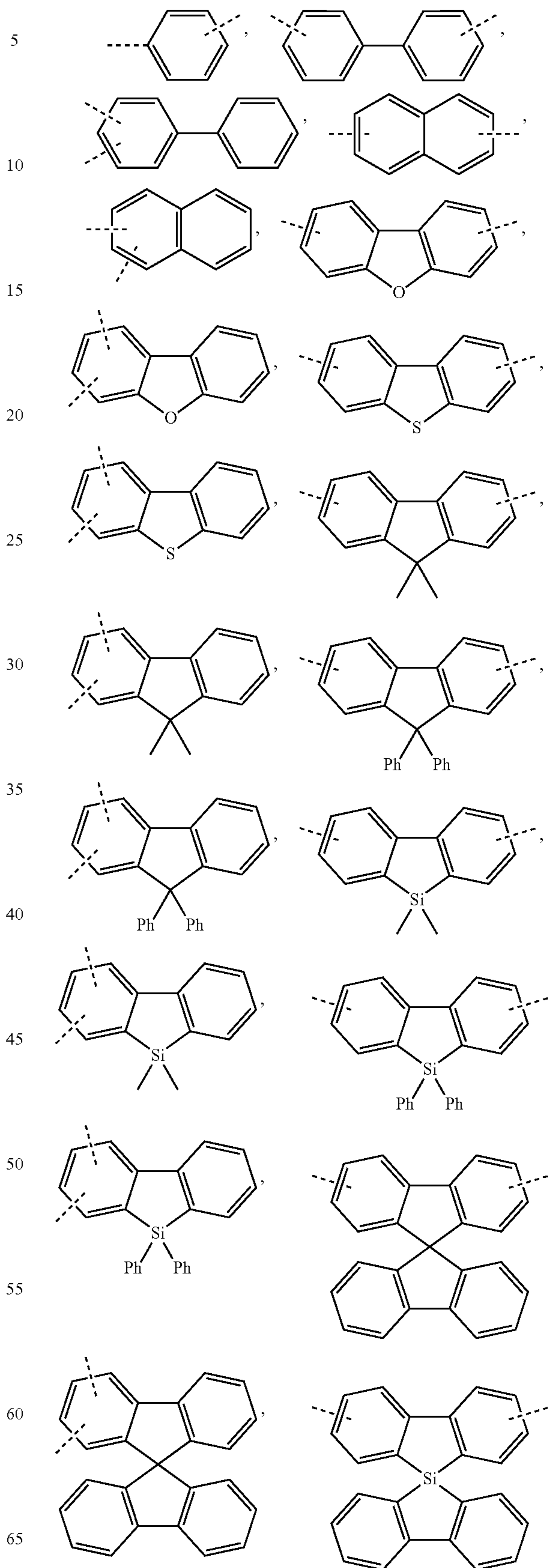
Formula 6
