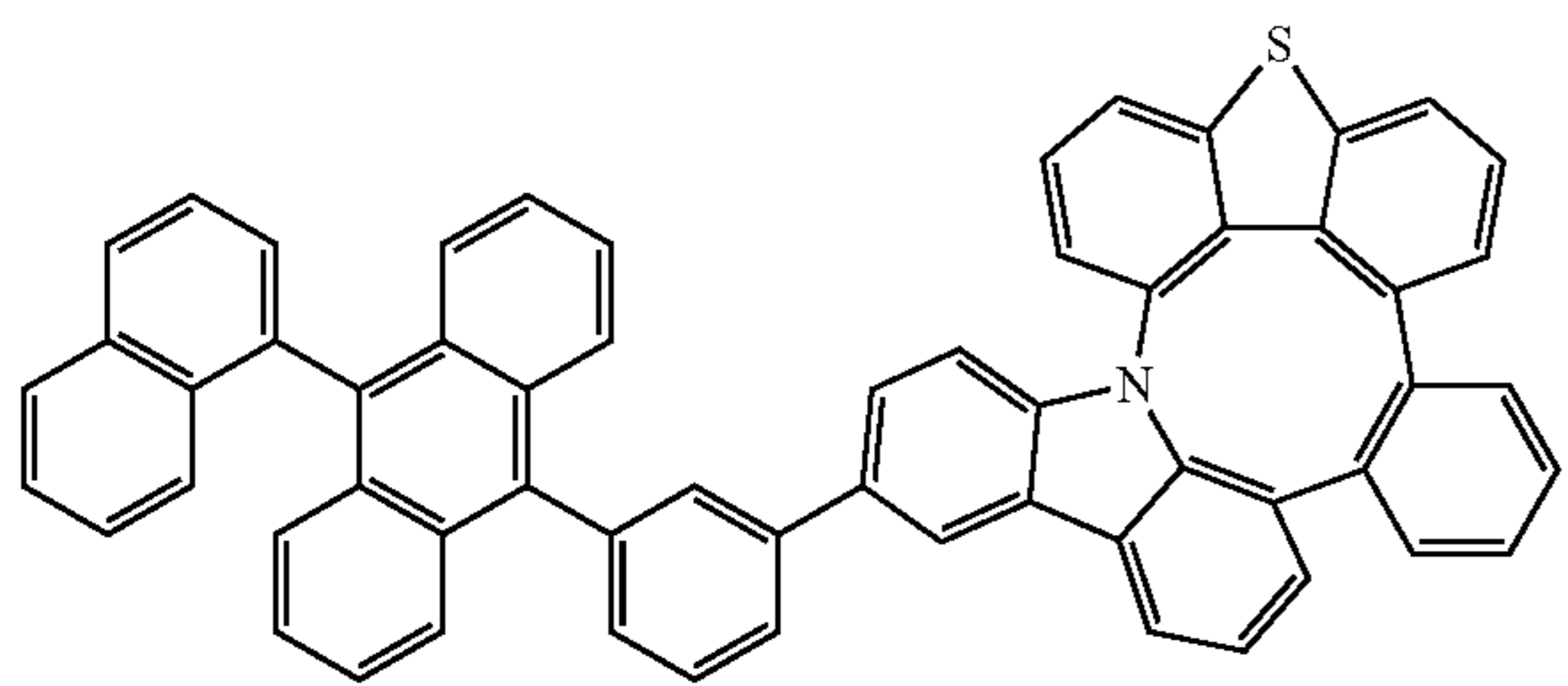
Compound 124
