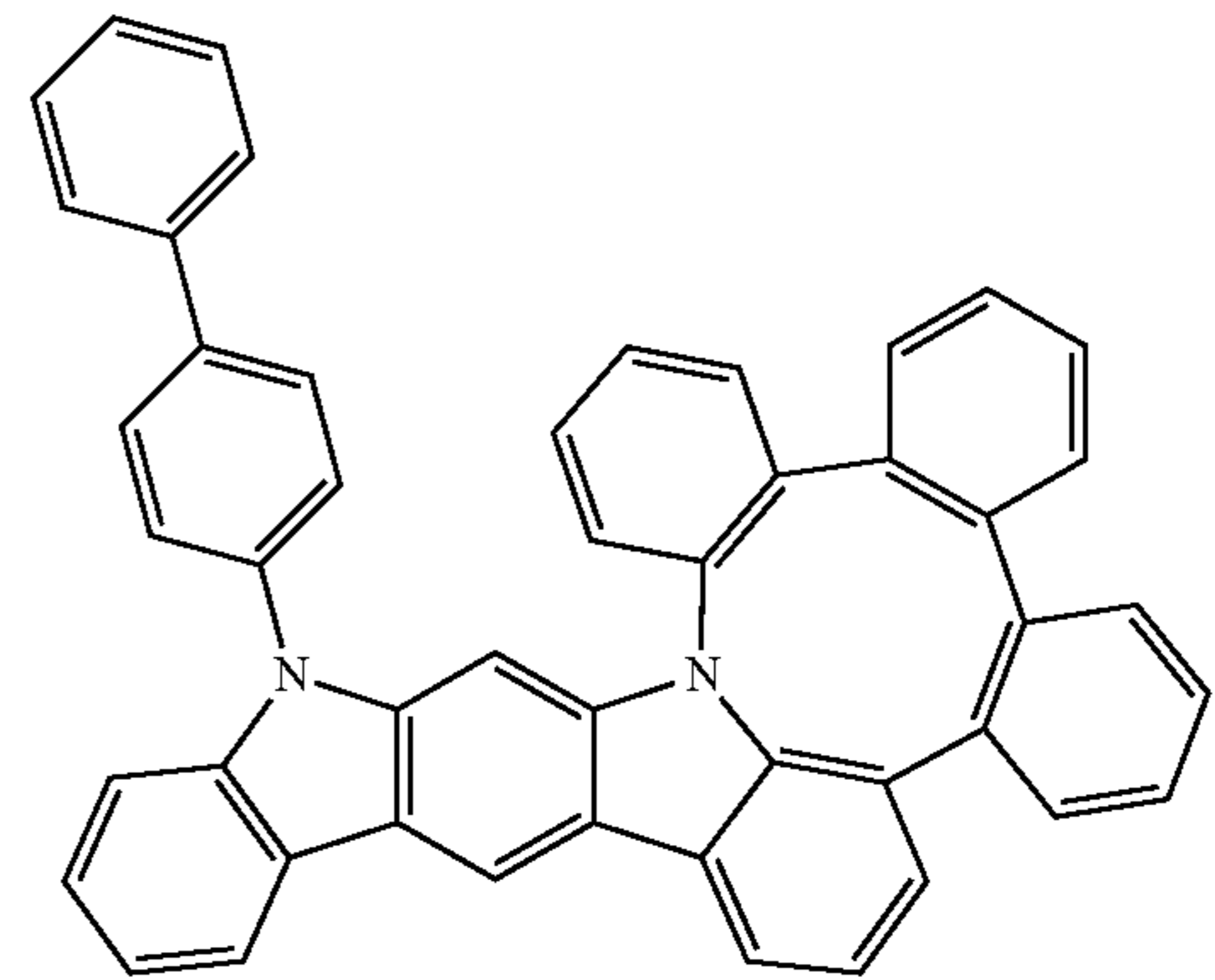
Compound 59
