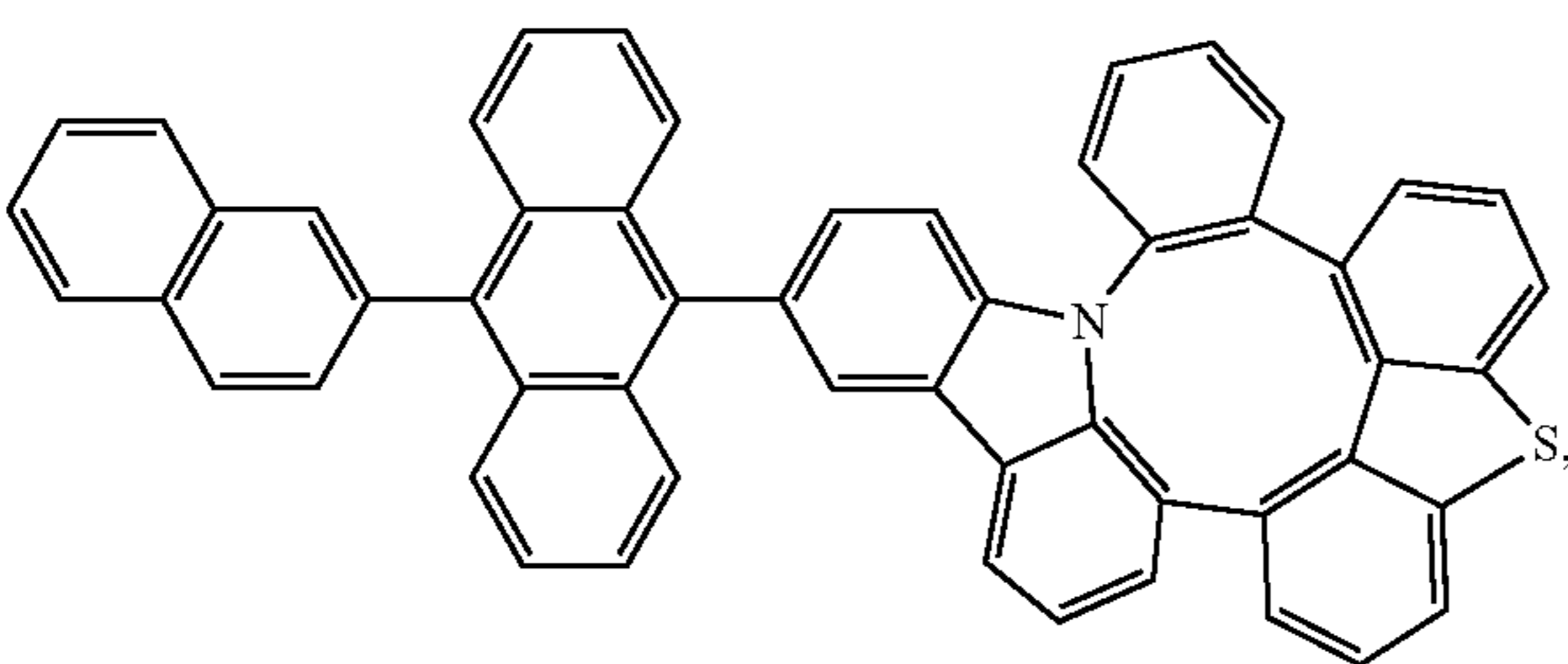
Compound 208
