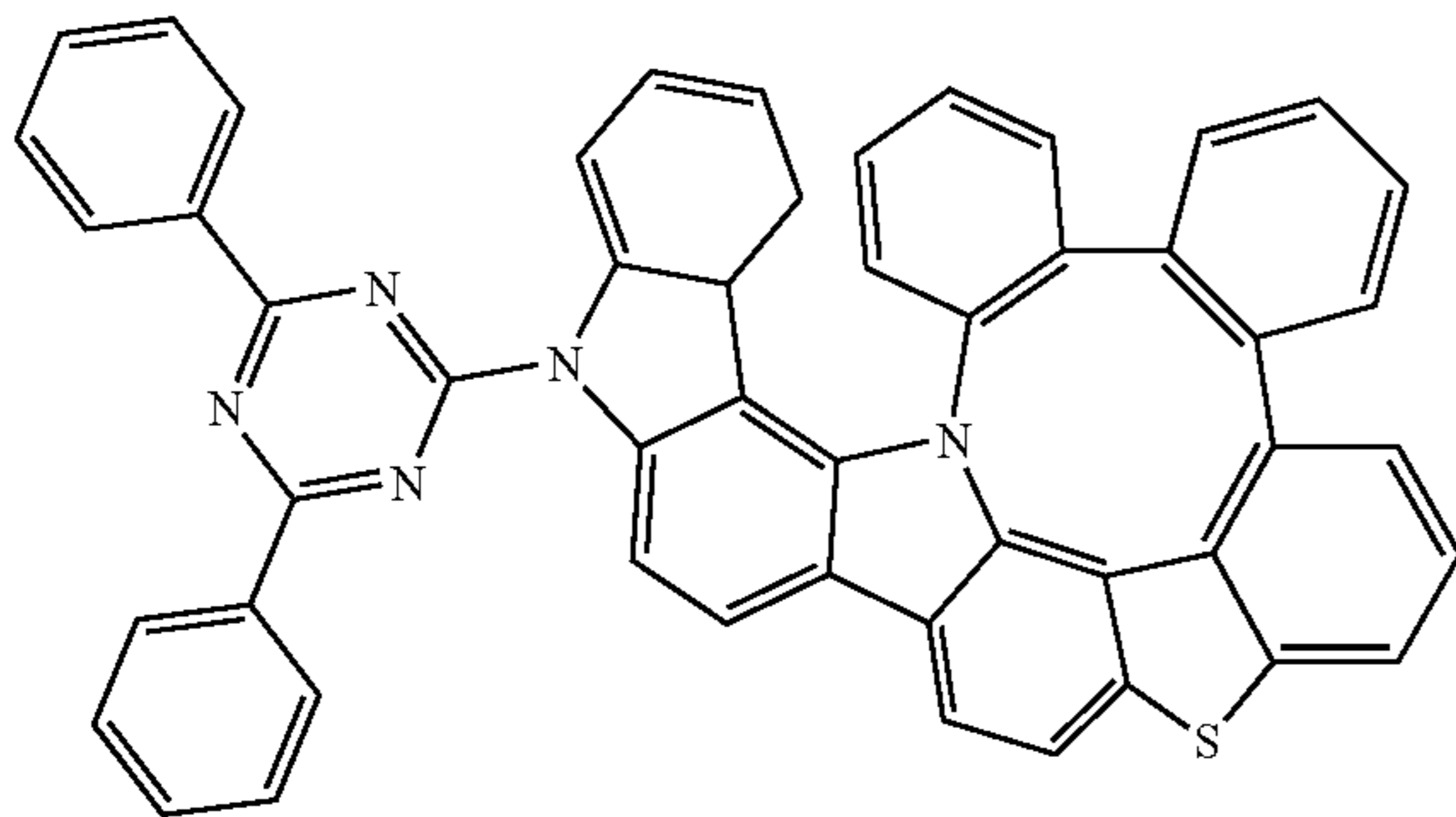
Compound 334
