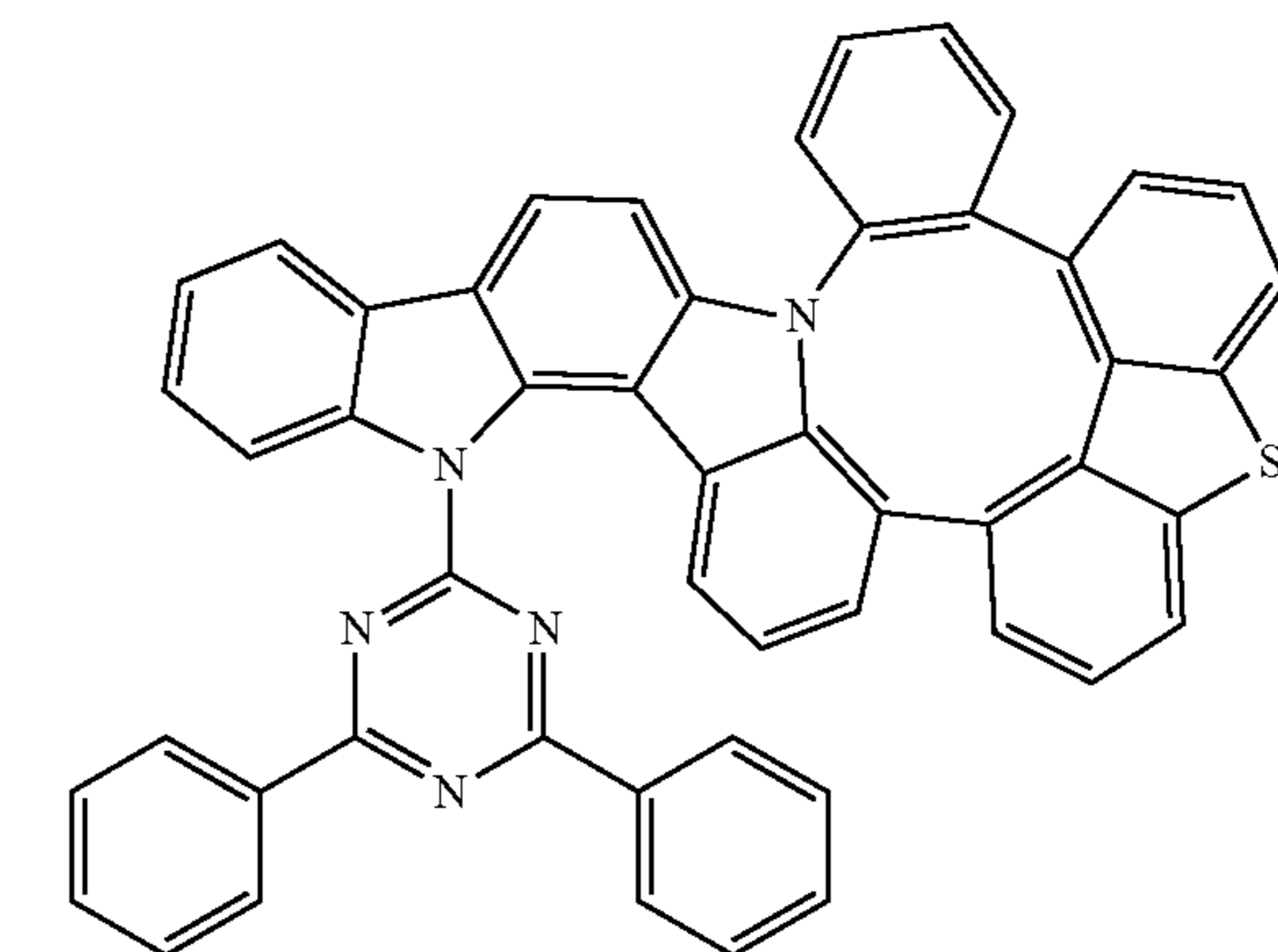
Compound 244
