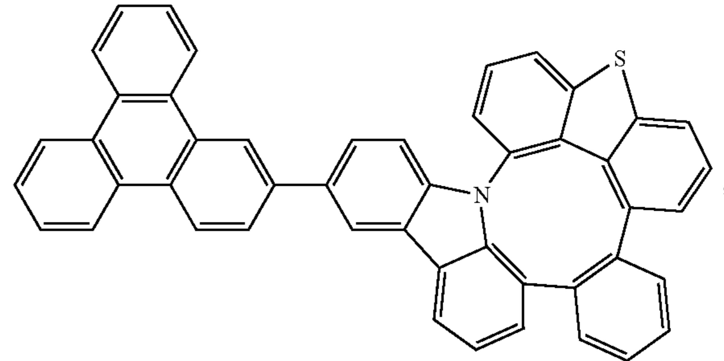
Compound 119
