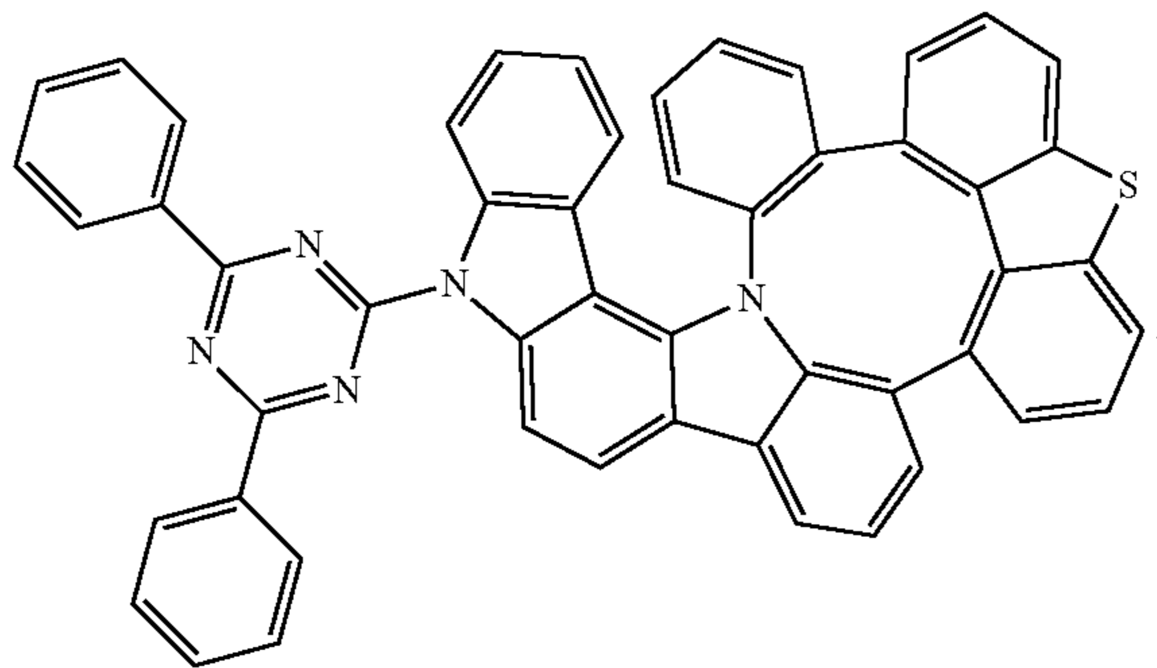
Compound 249
