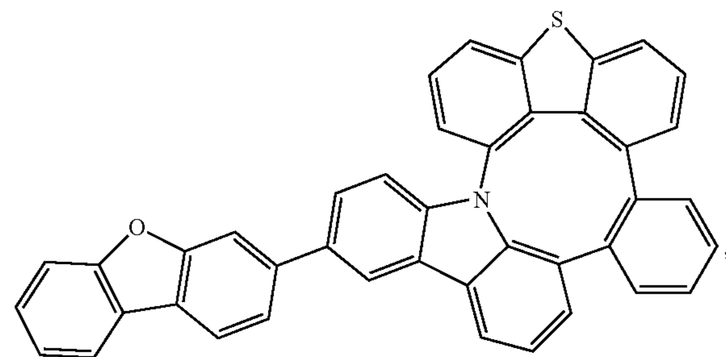
Compound 91
