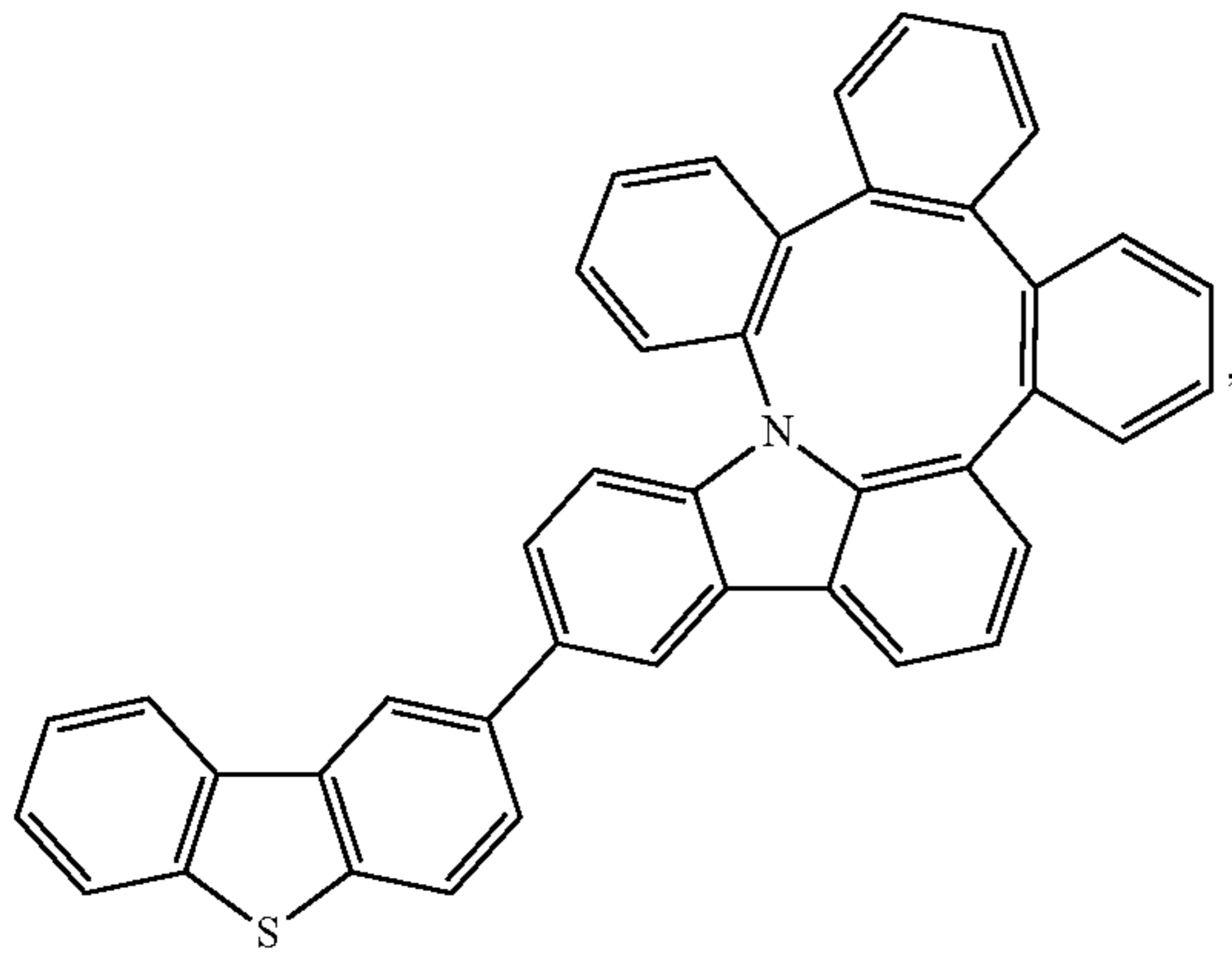
Compound 9
