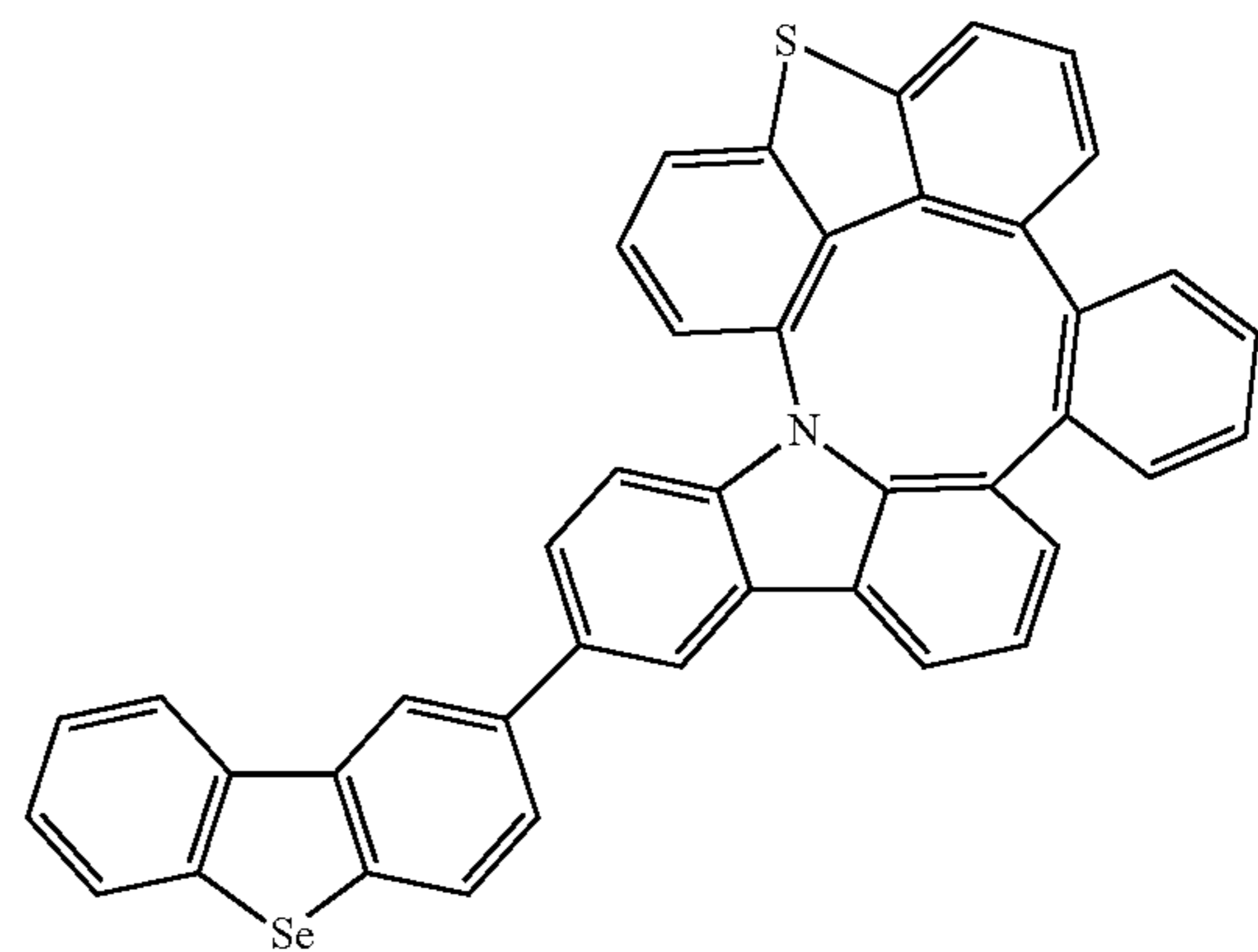
Compound 96
