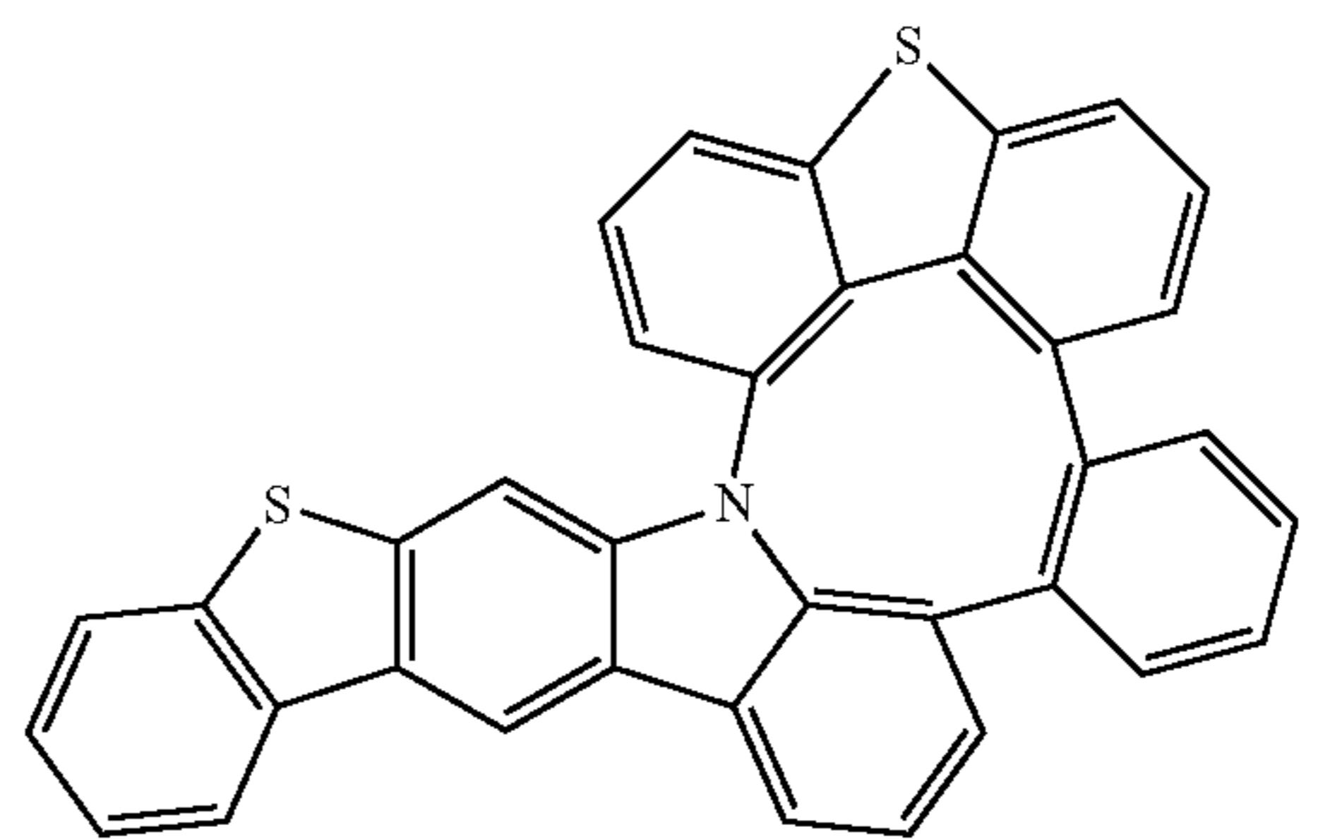
Compound 150
