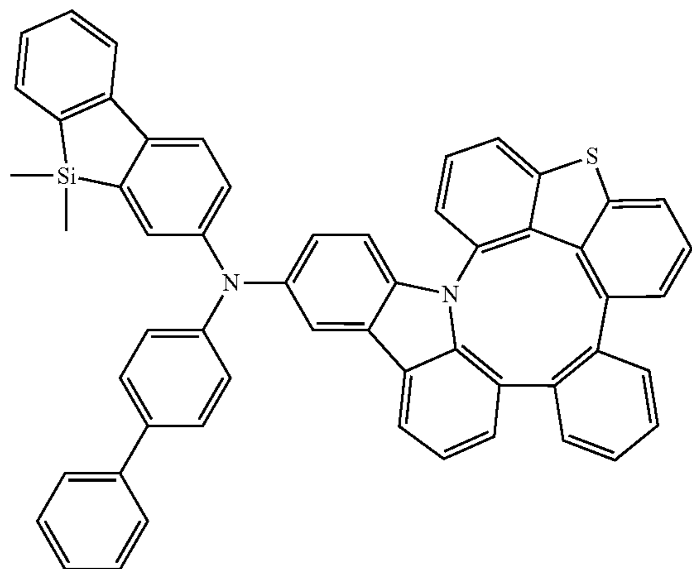
Compound 352
