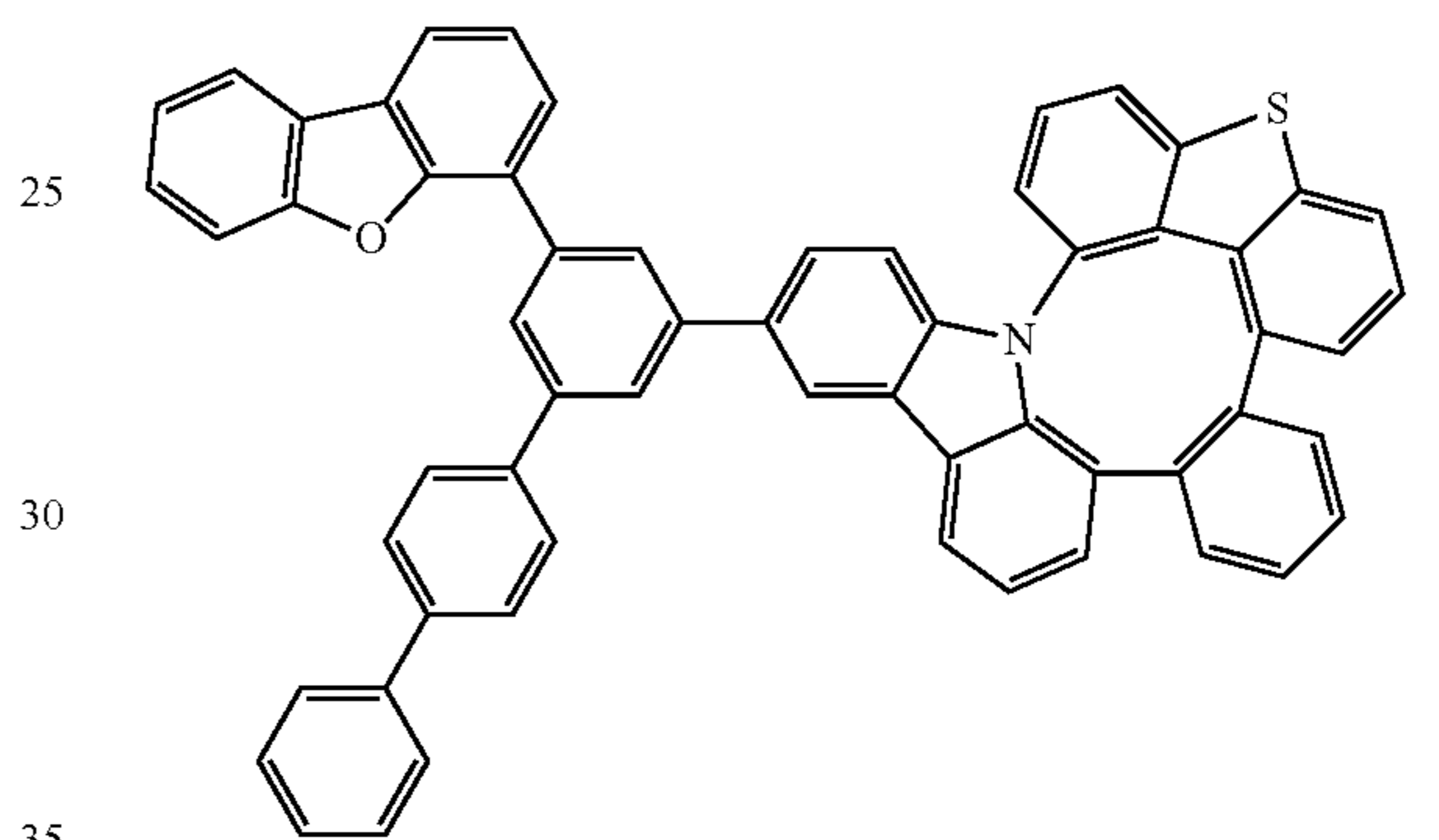
Compound 134
