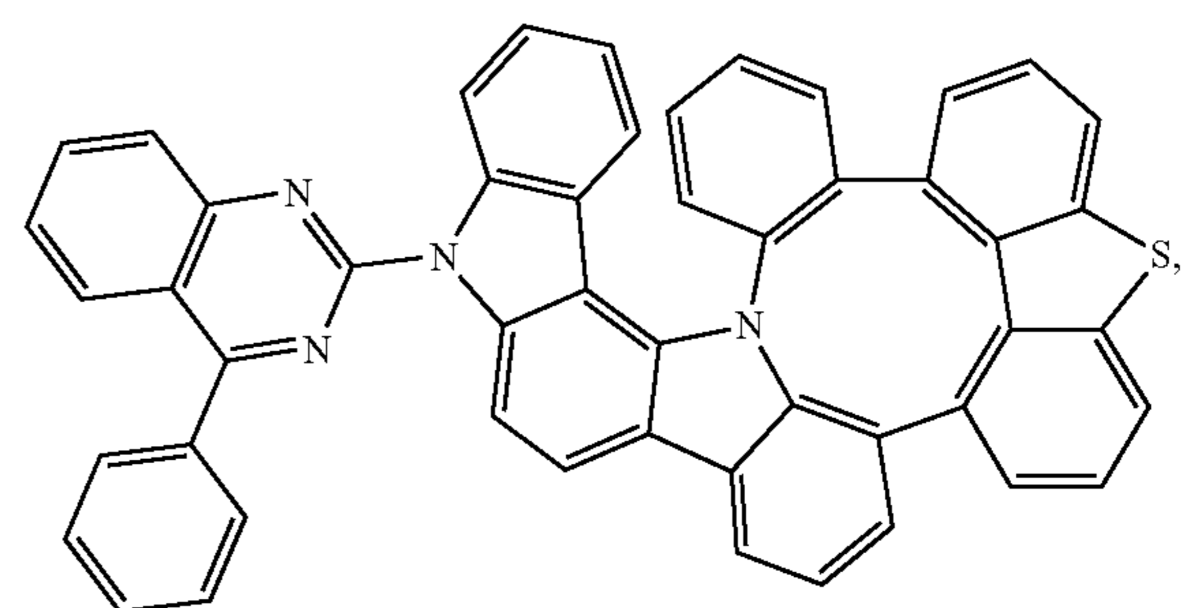
Compound 254
