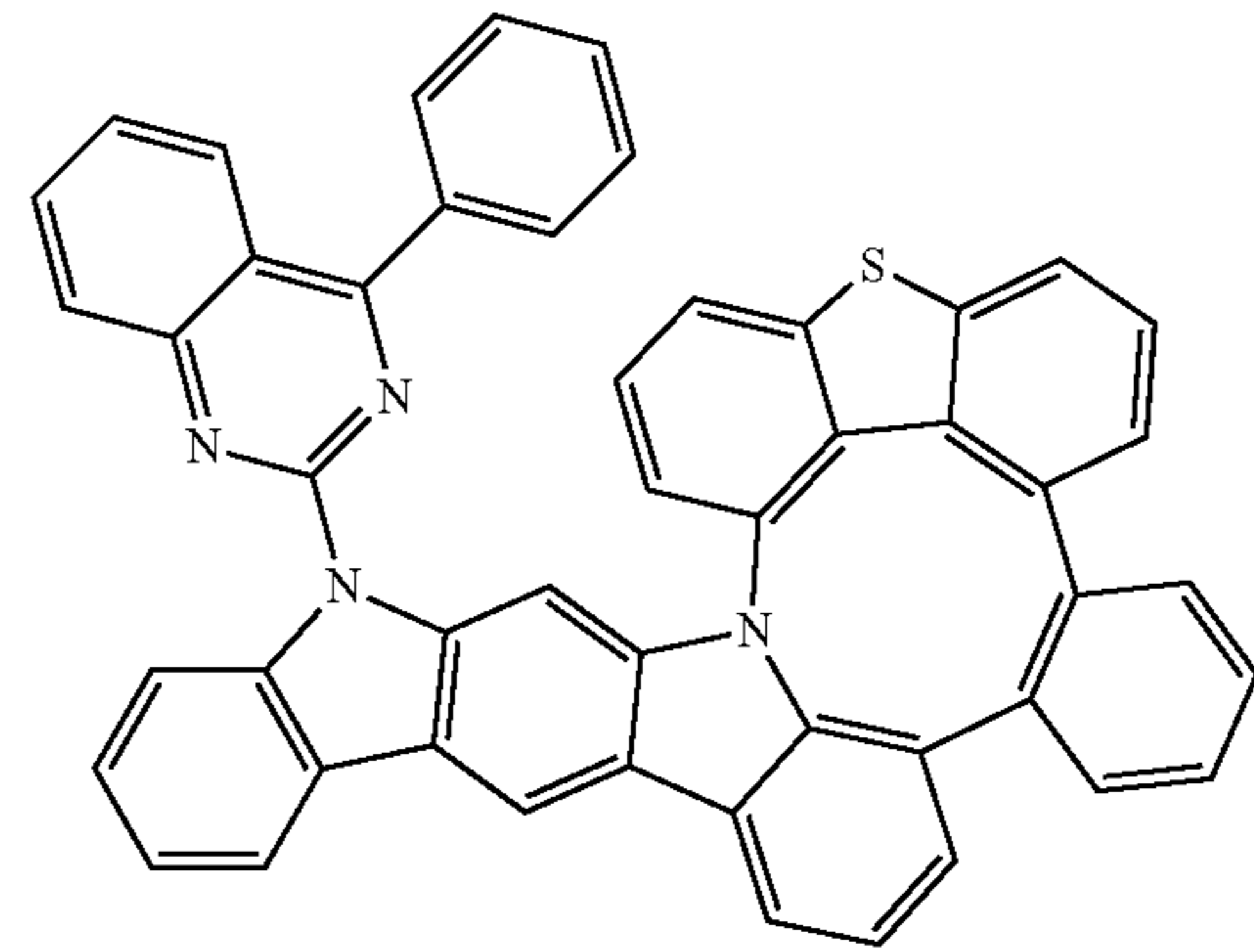
Compound 168
