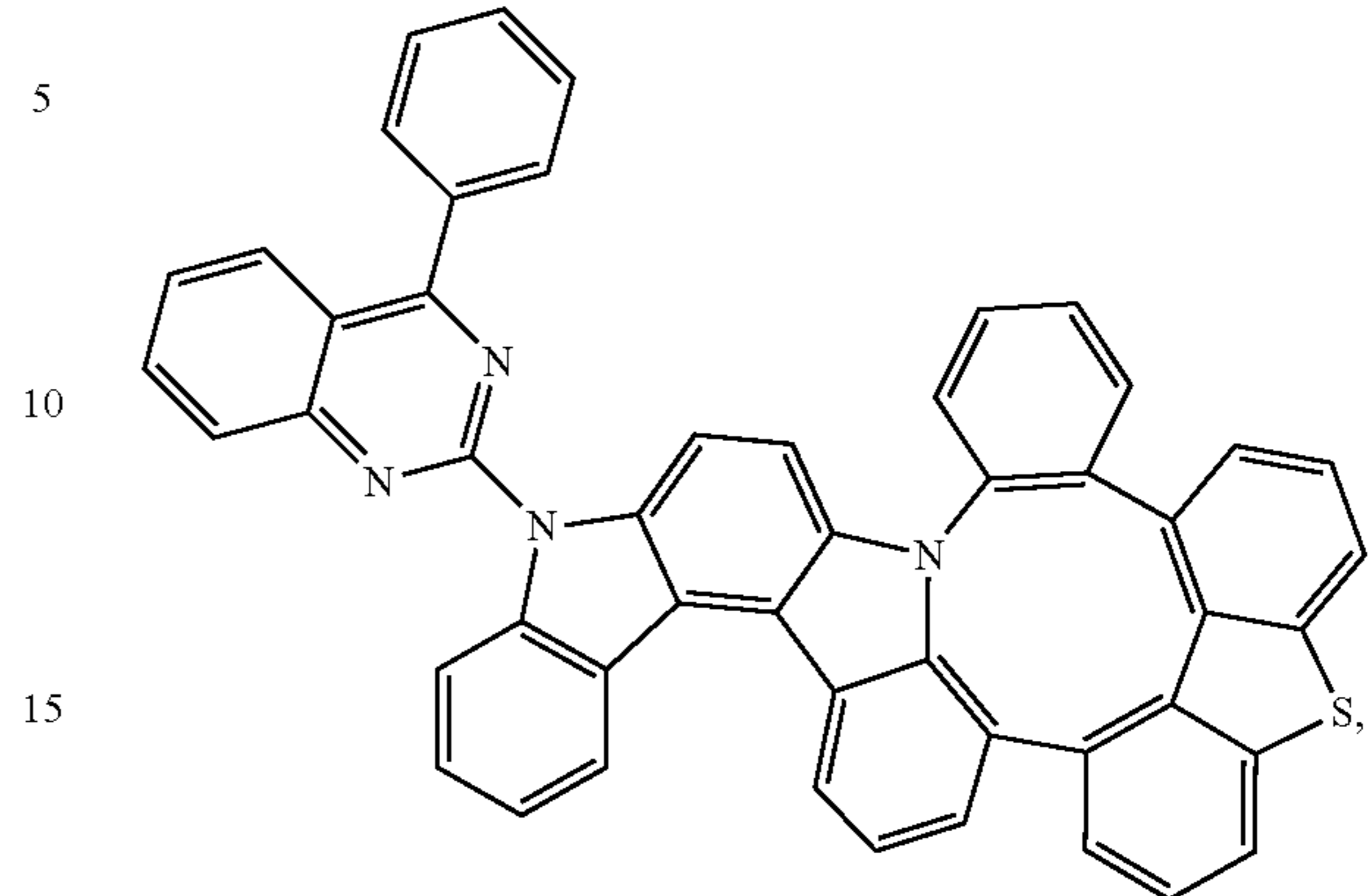
Compound 252
