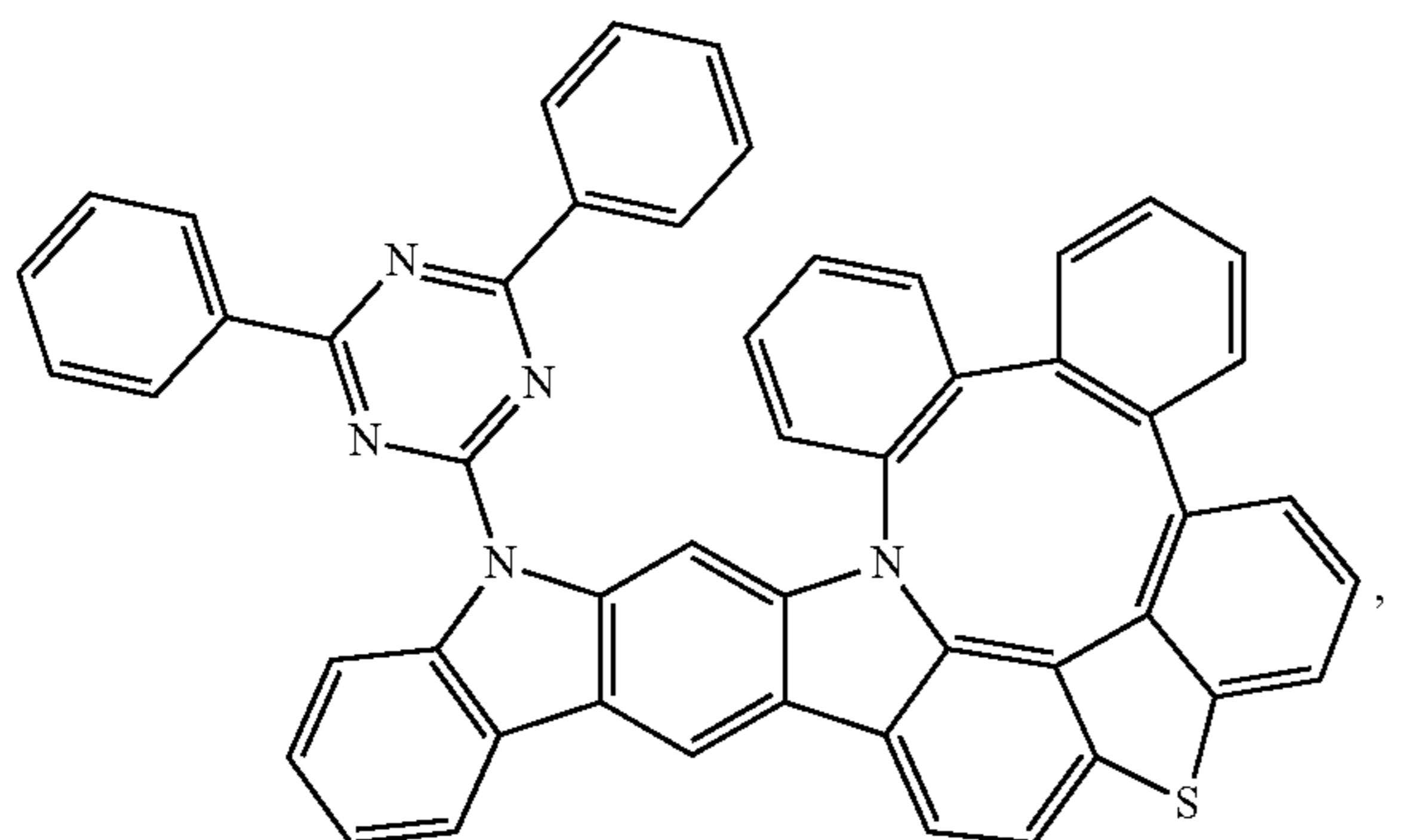
Compound 332
