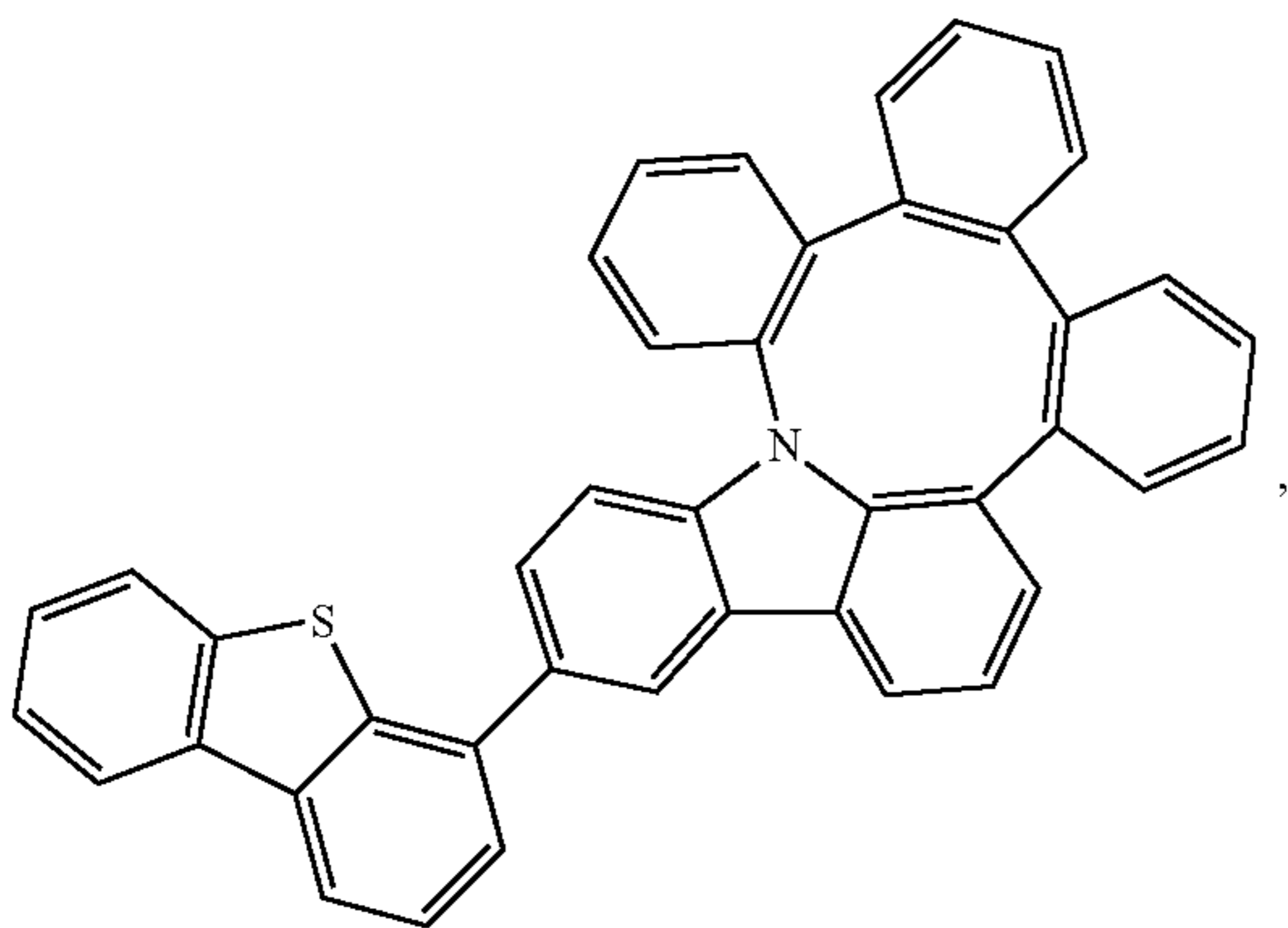
Compound 7
