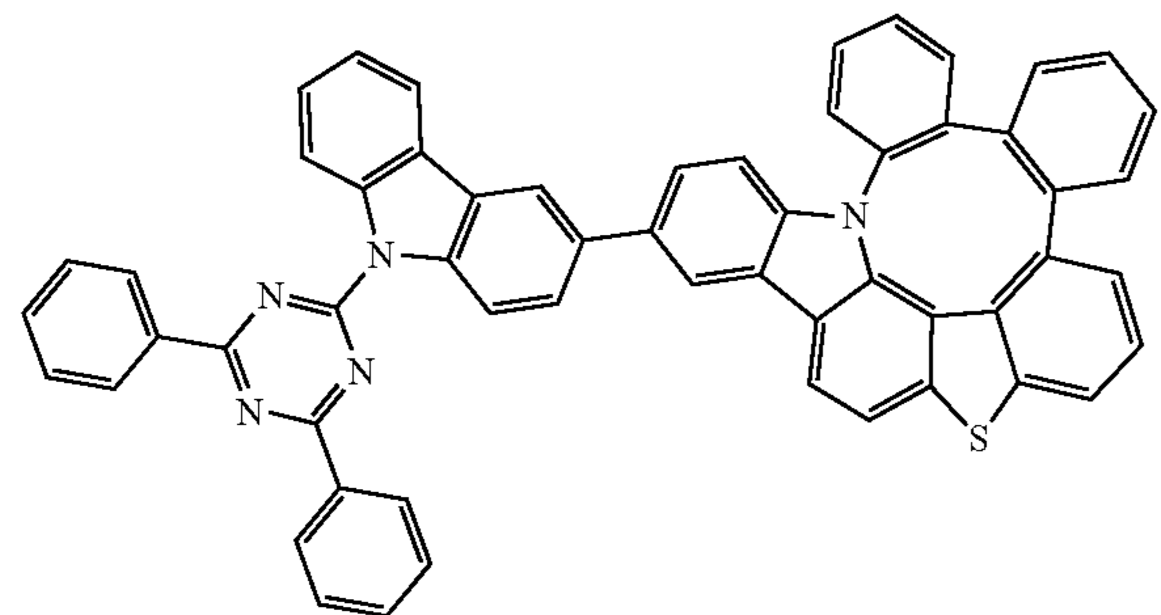
Compound 274
