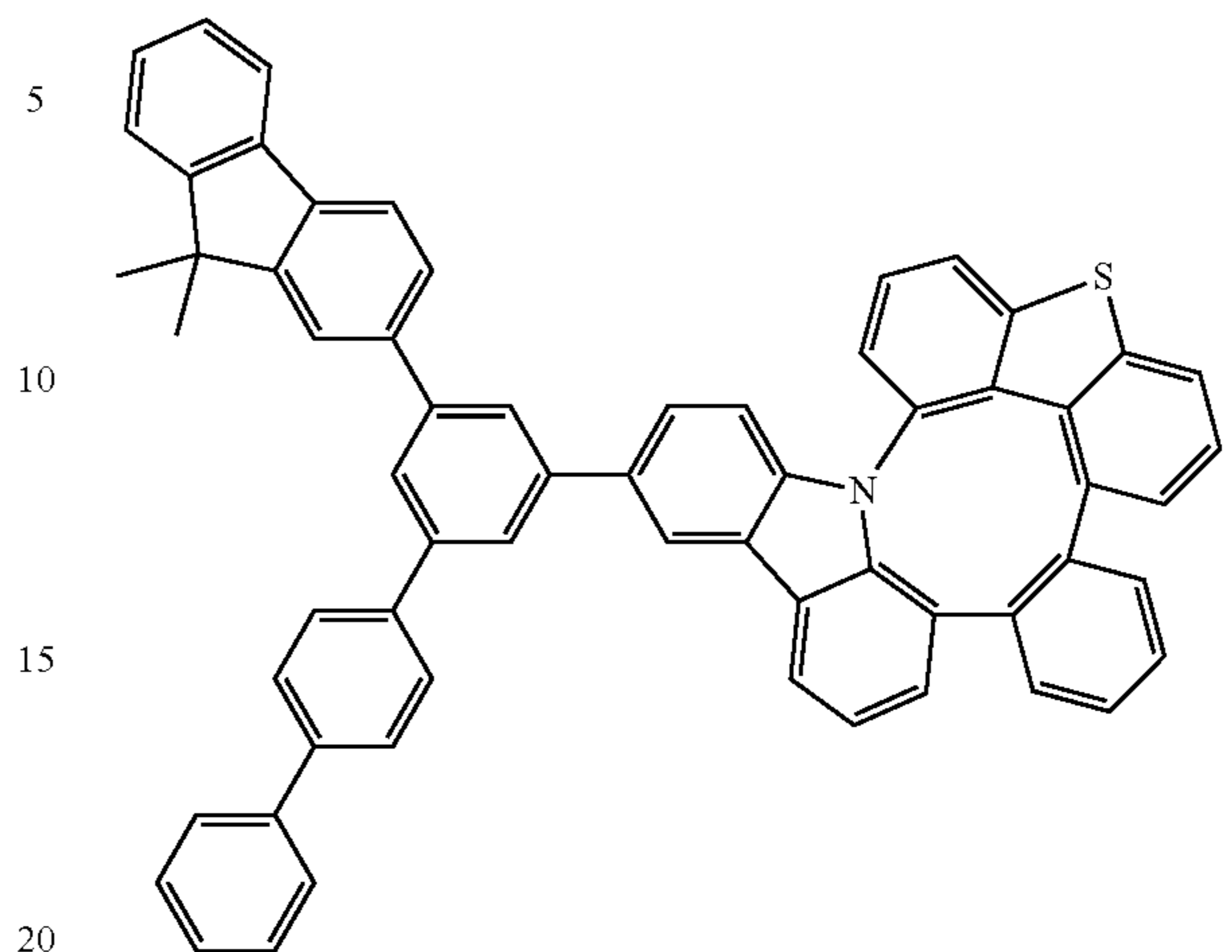
Compound 133
