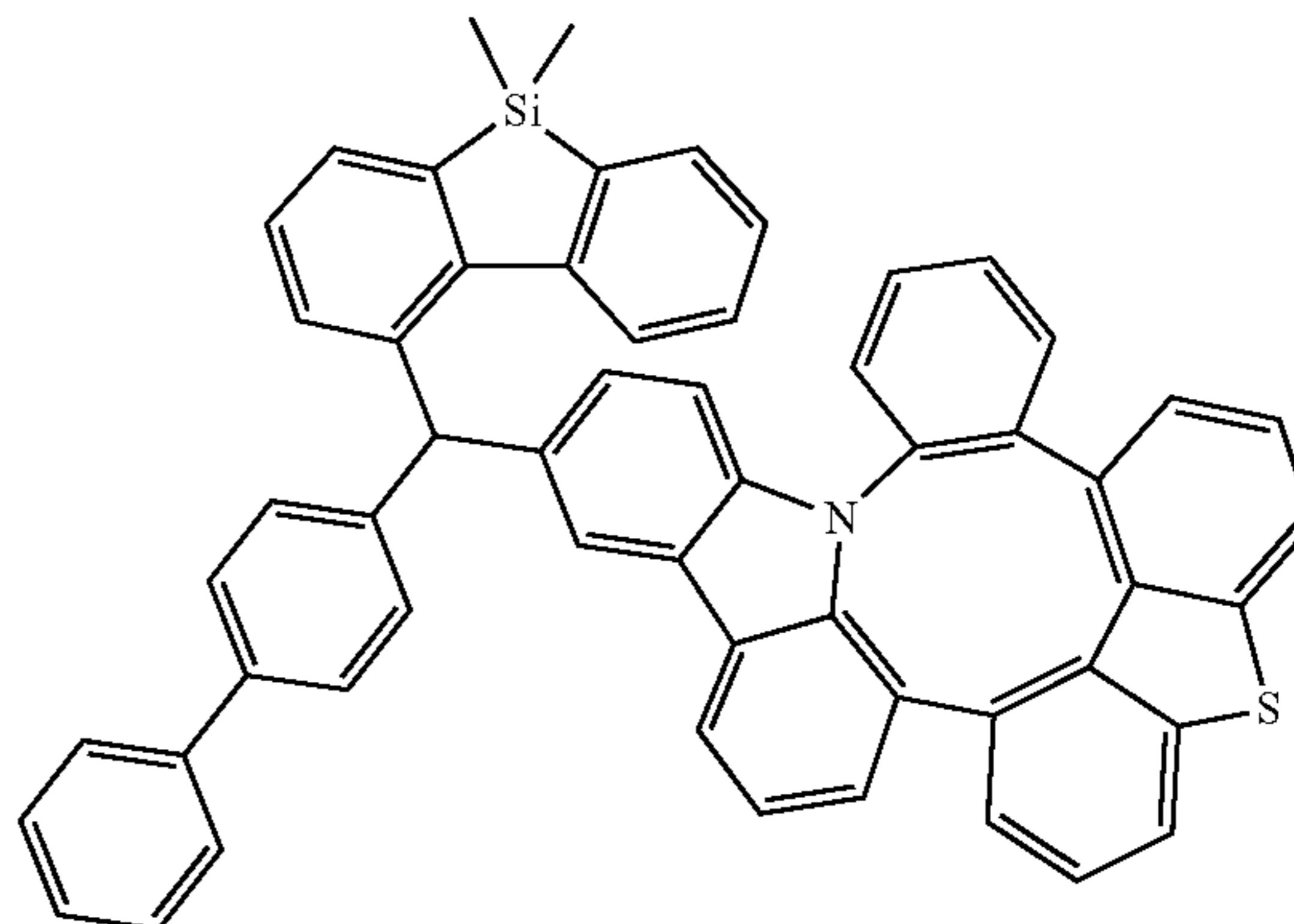
Compound 360
