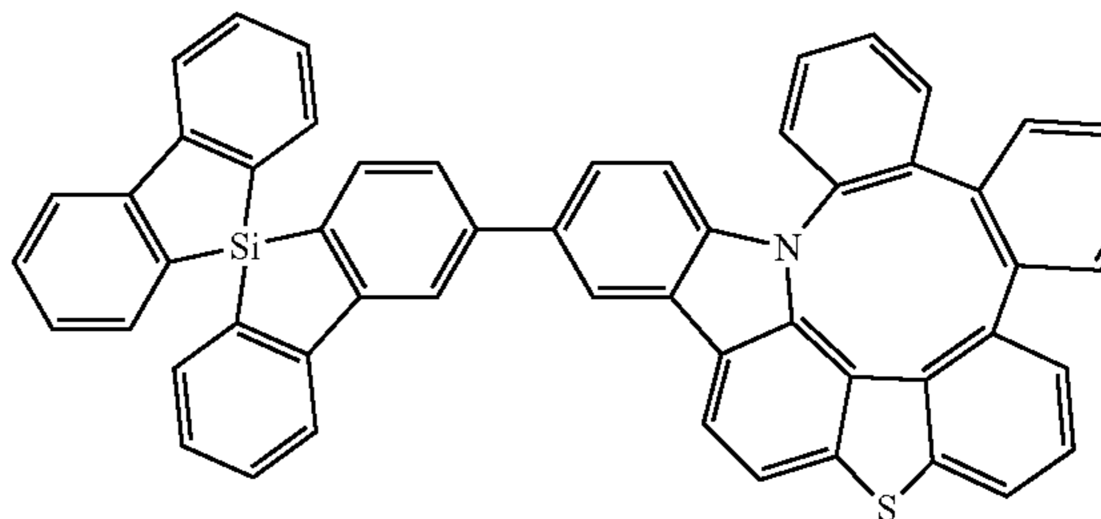
Compound 363
