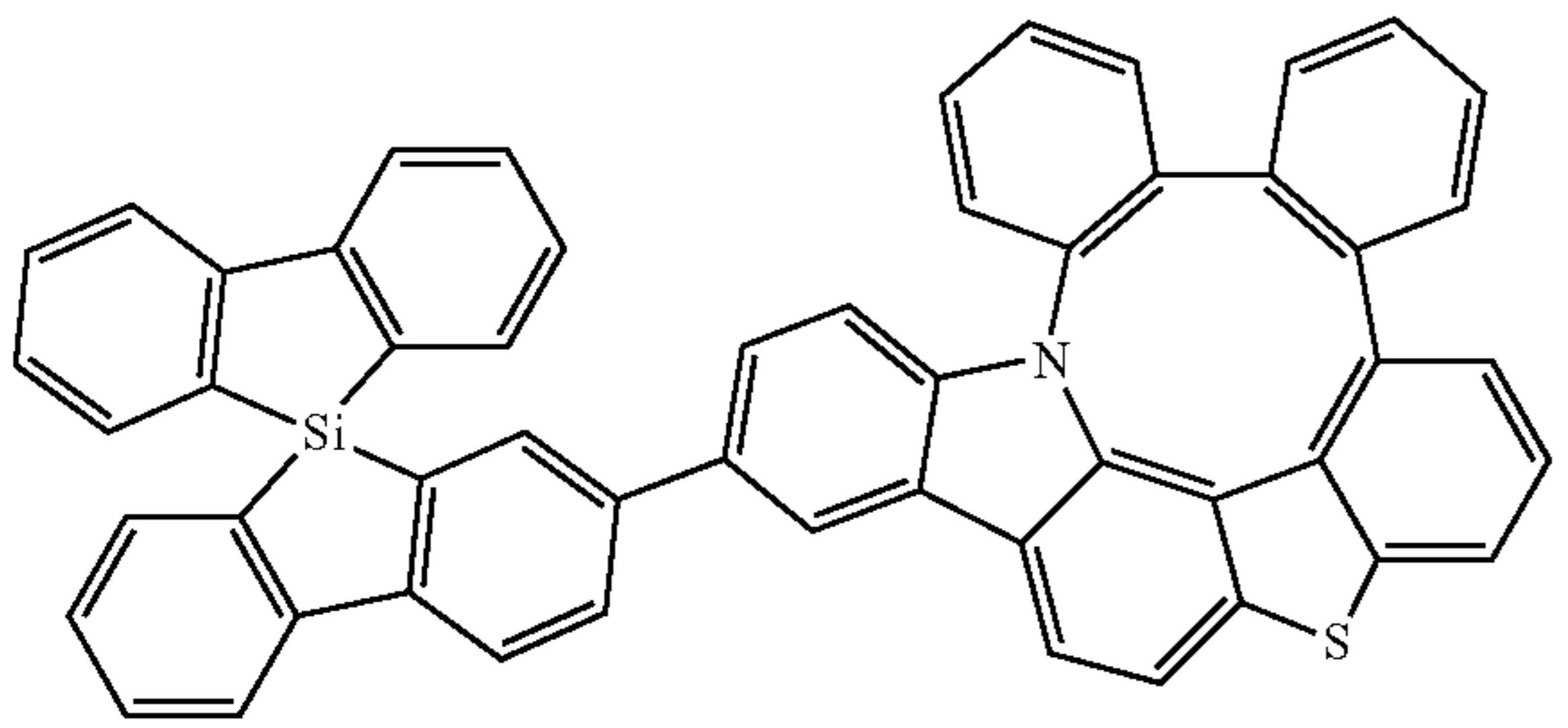
Compound 362
