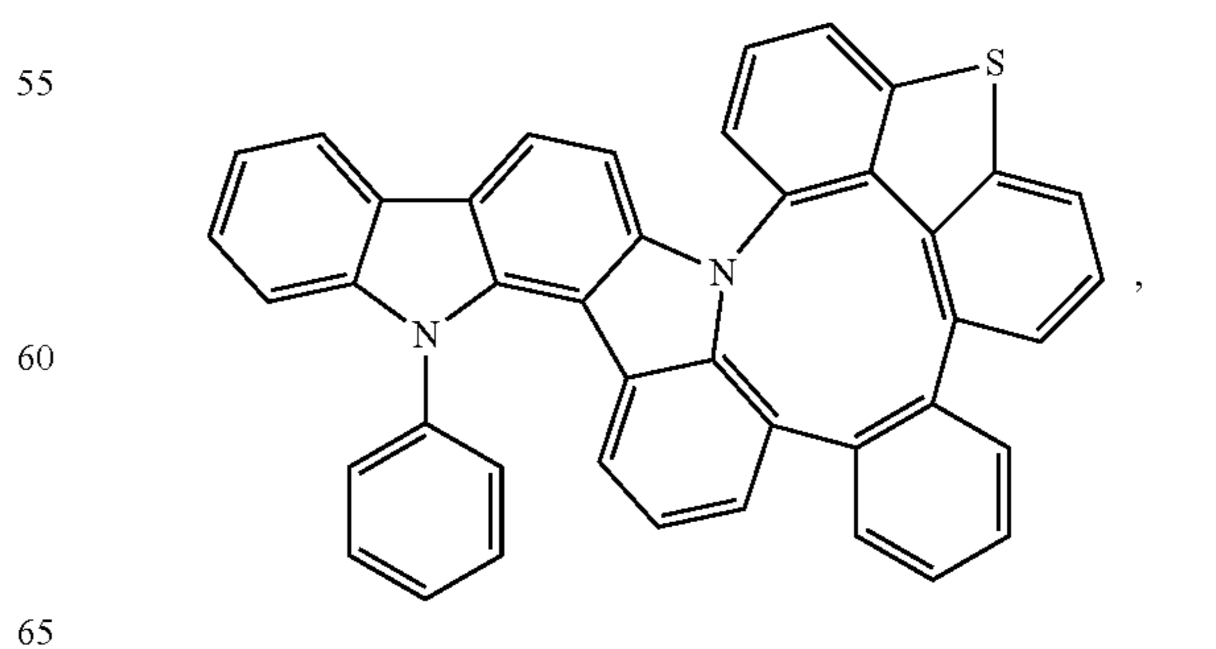
Compound 135
