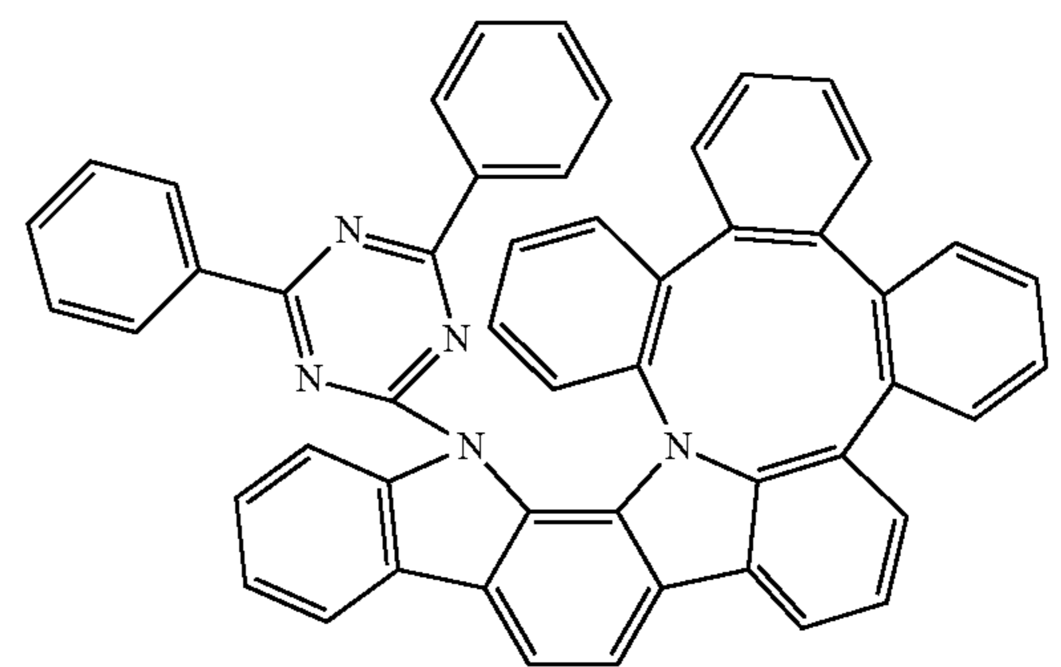
Compound 80
