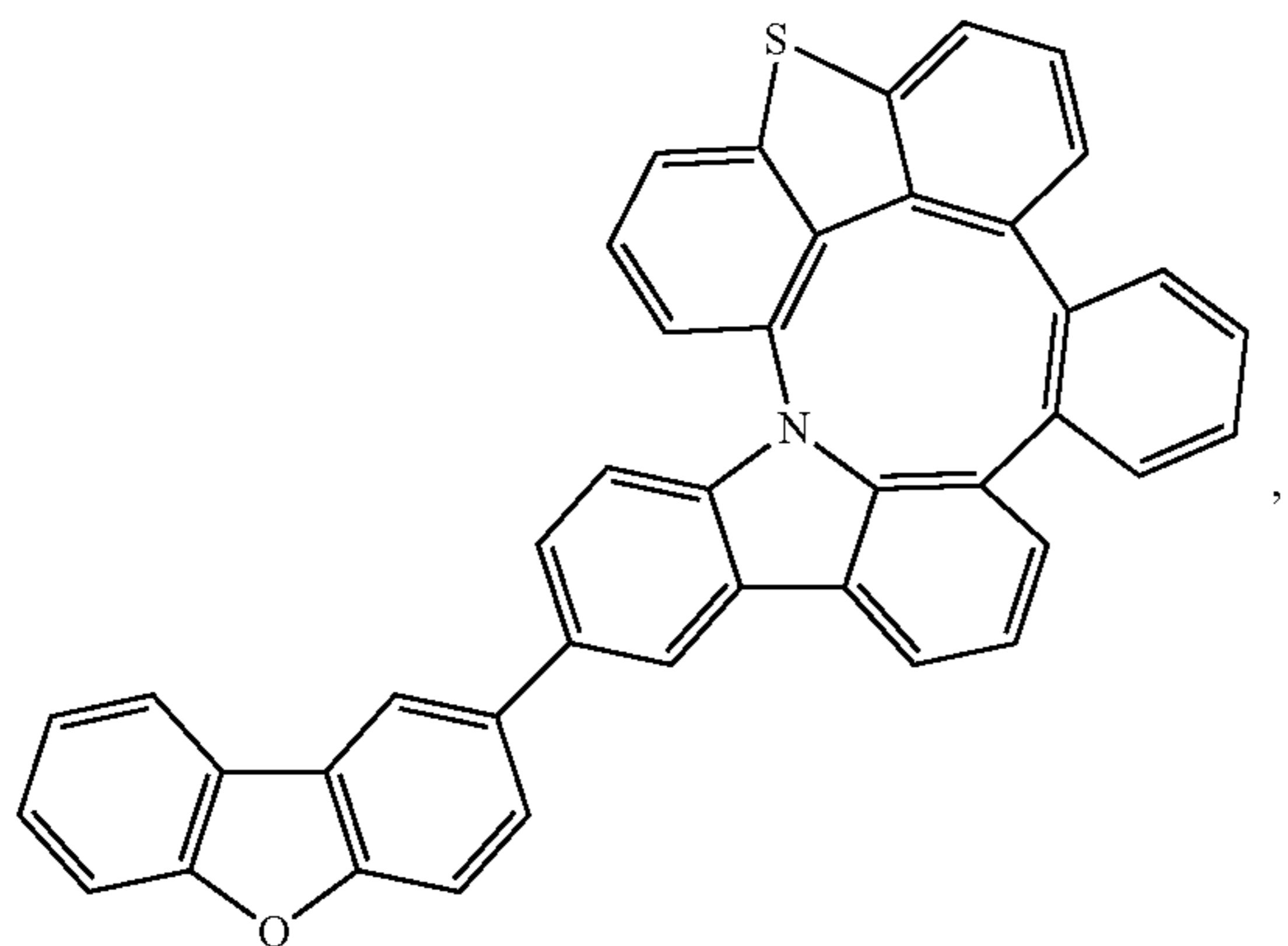
Compound 91
