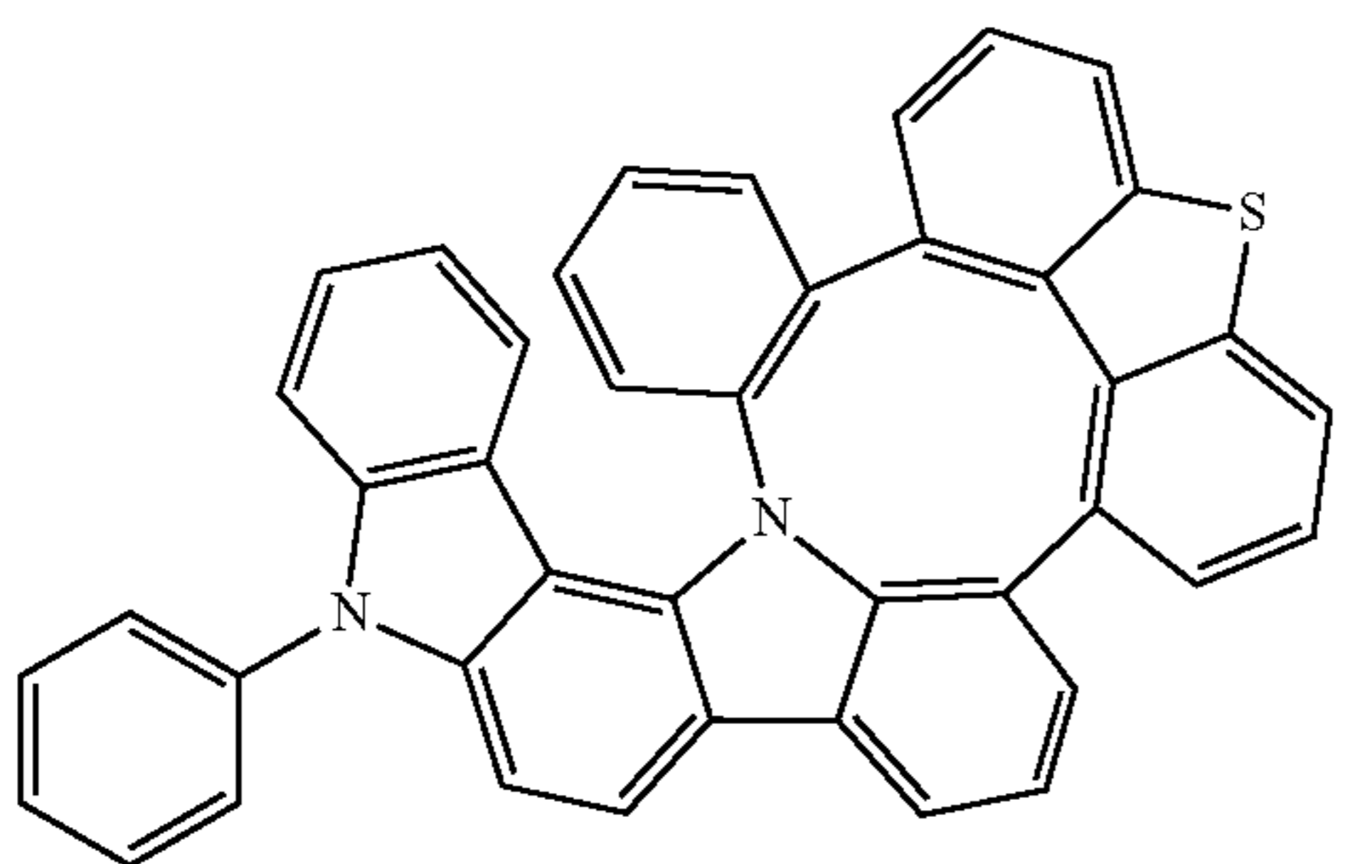
Compound 224
