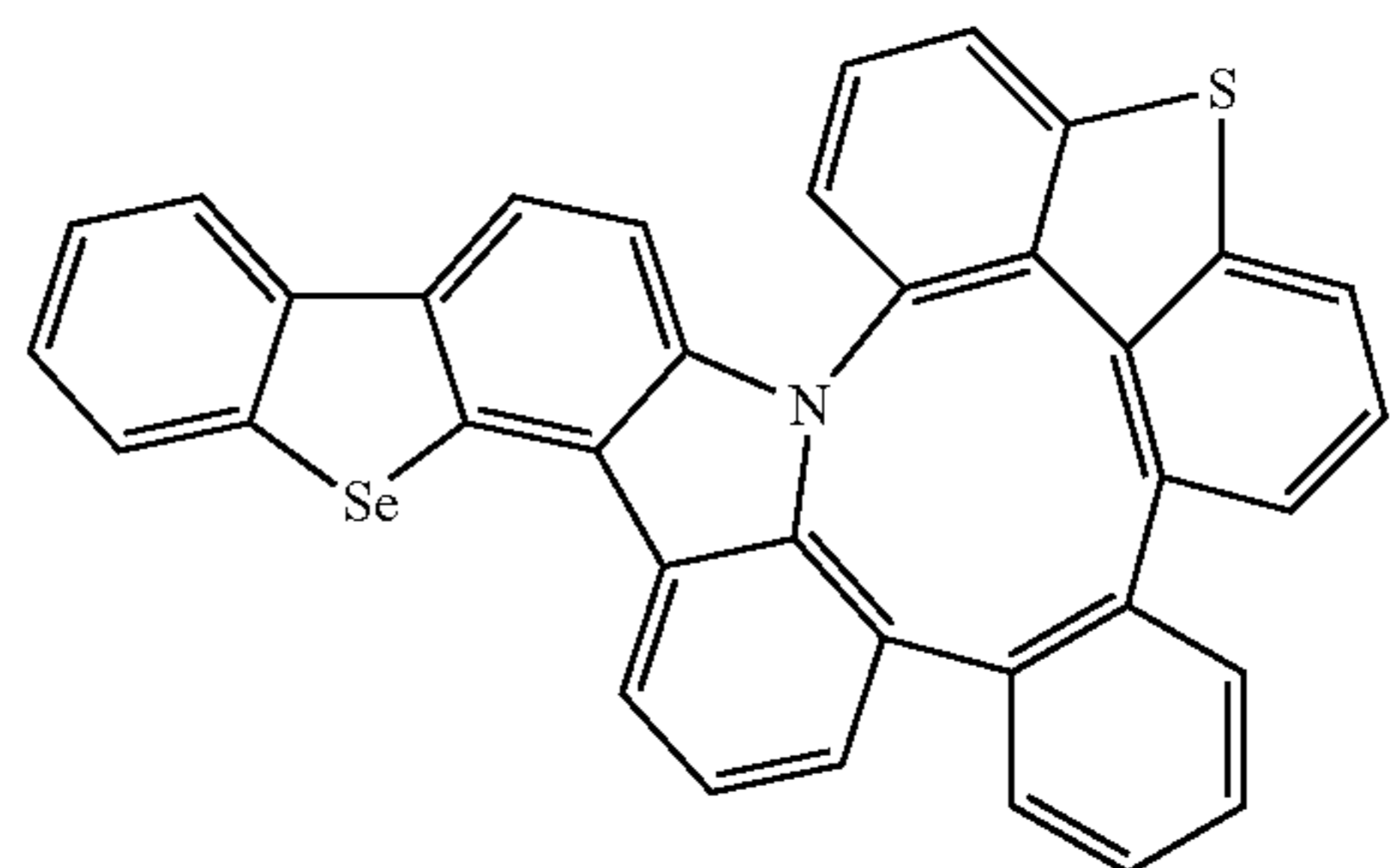
Compound 153
