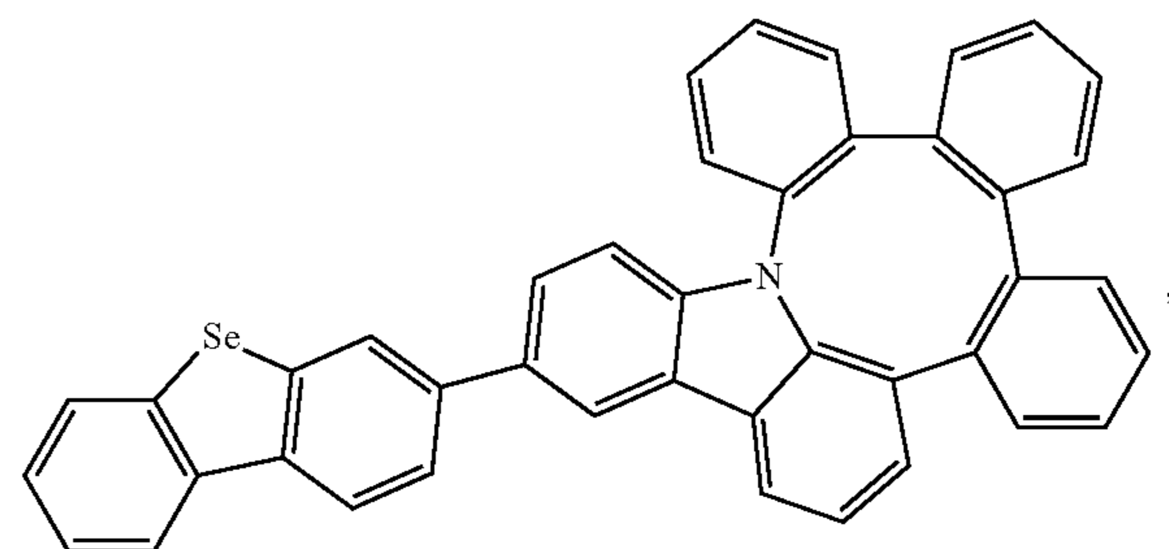
Compound 12
