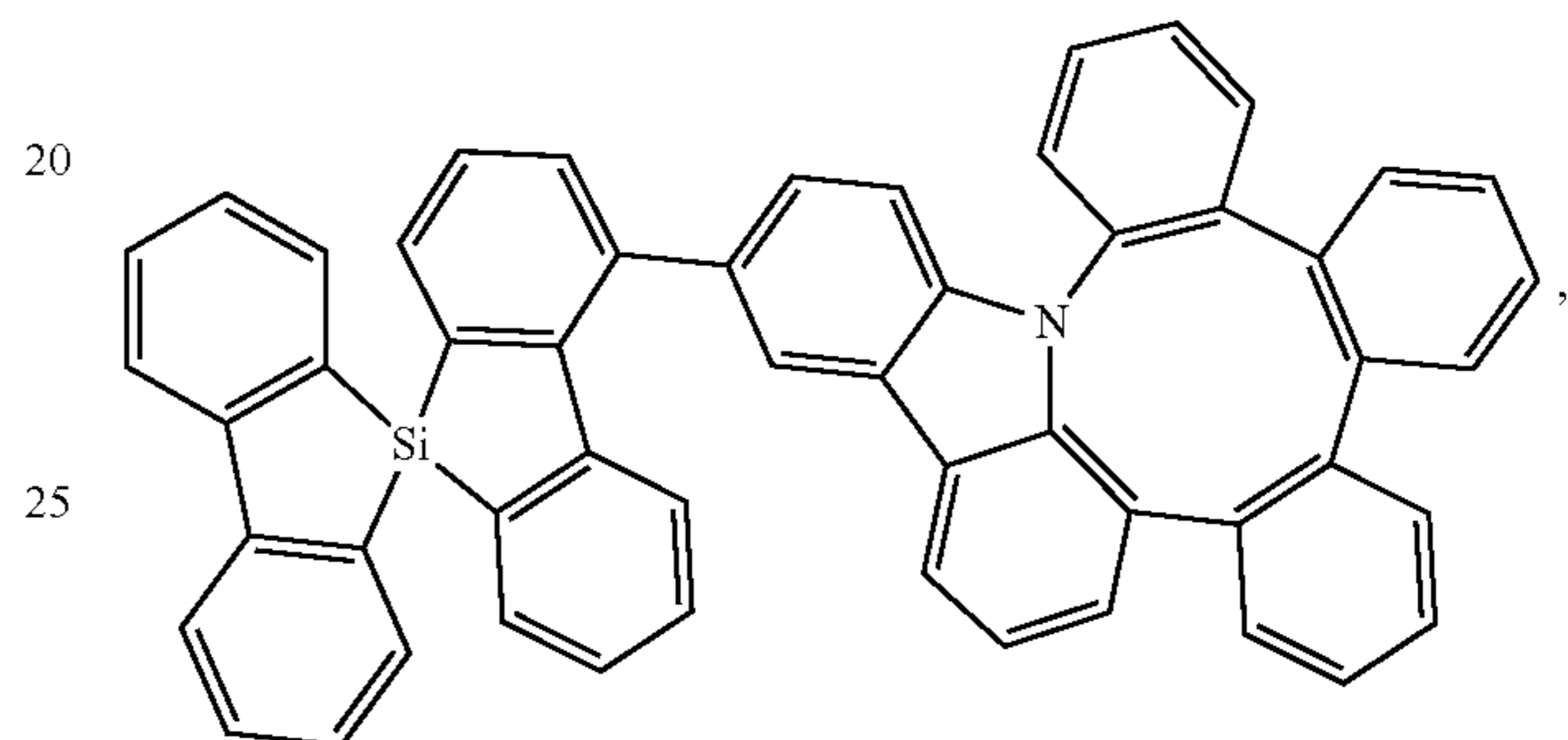
Compound 343
