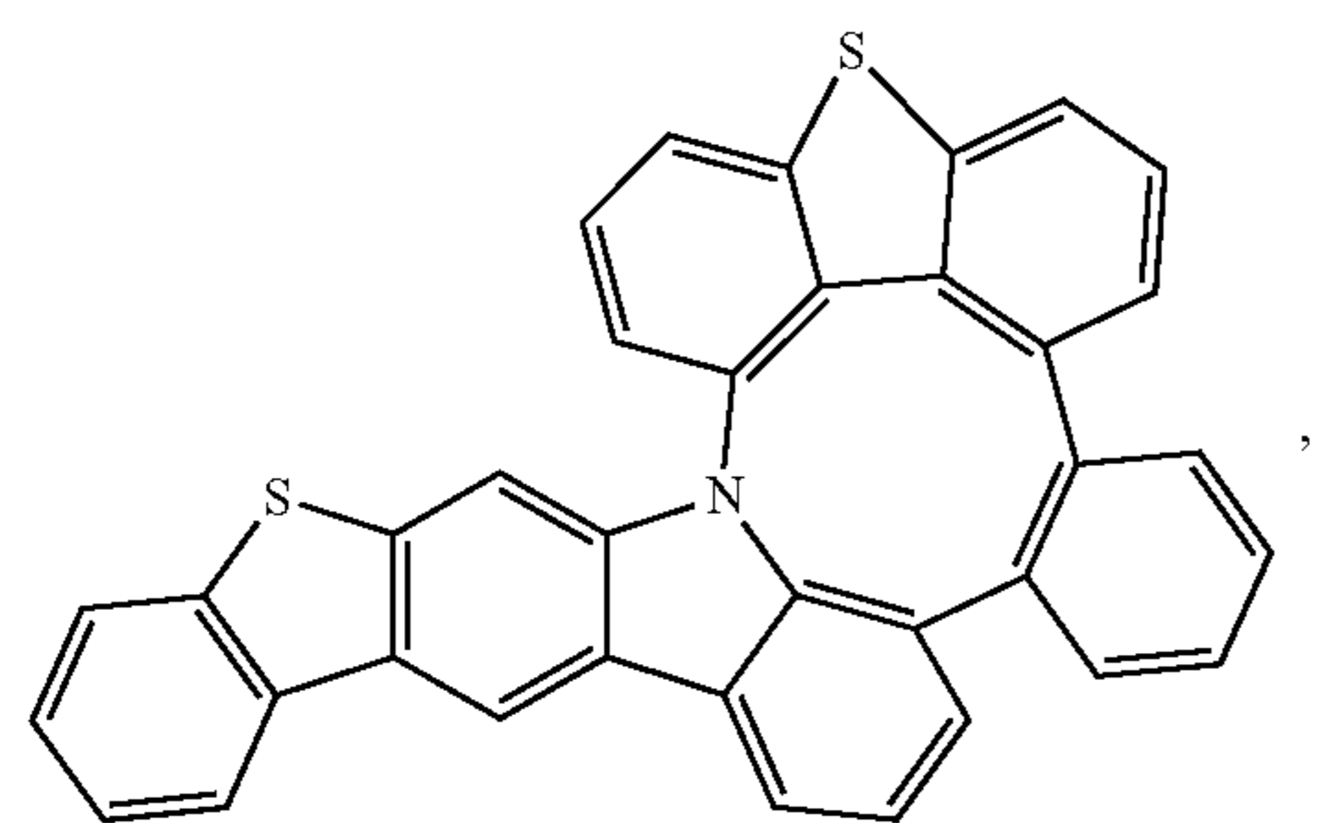
Compound 150
