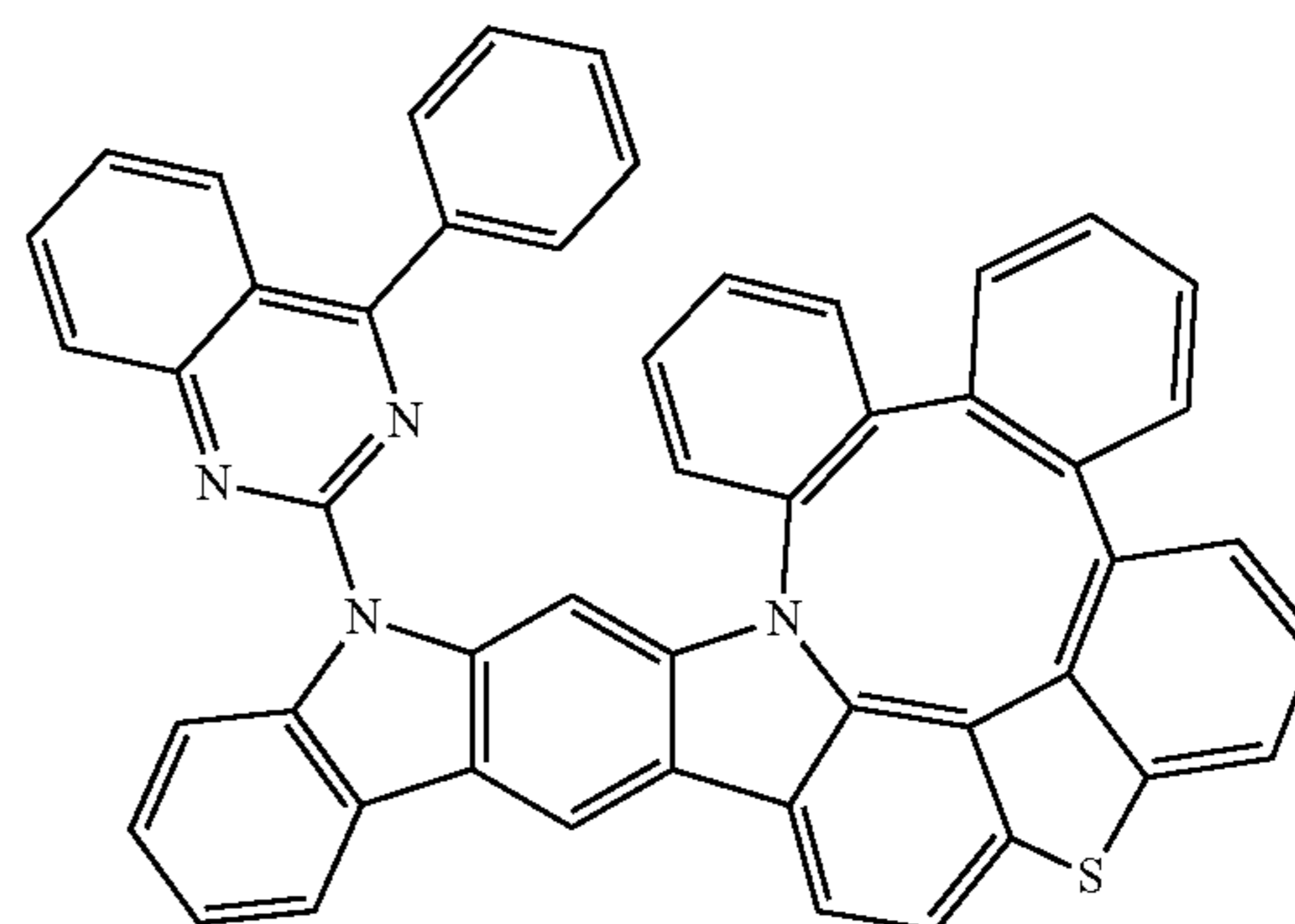
Compound 338
