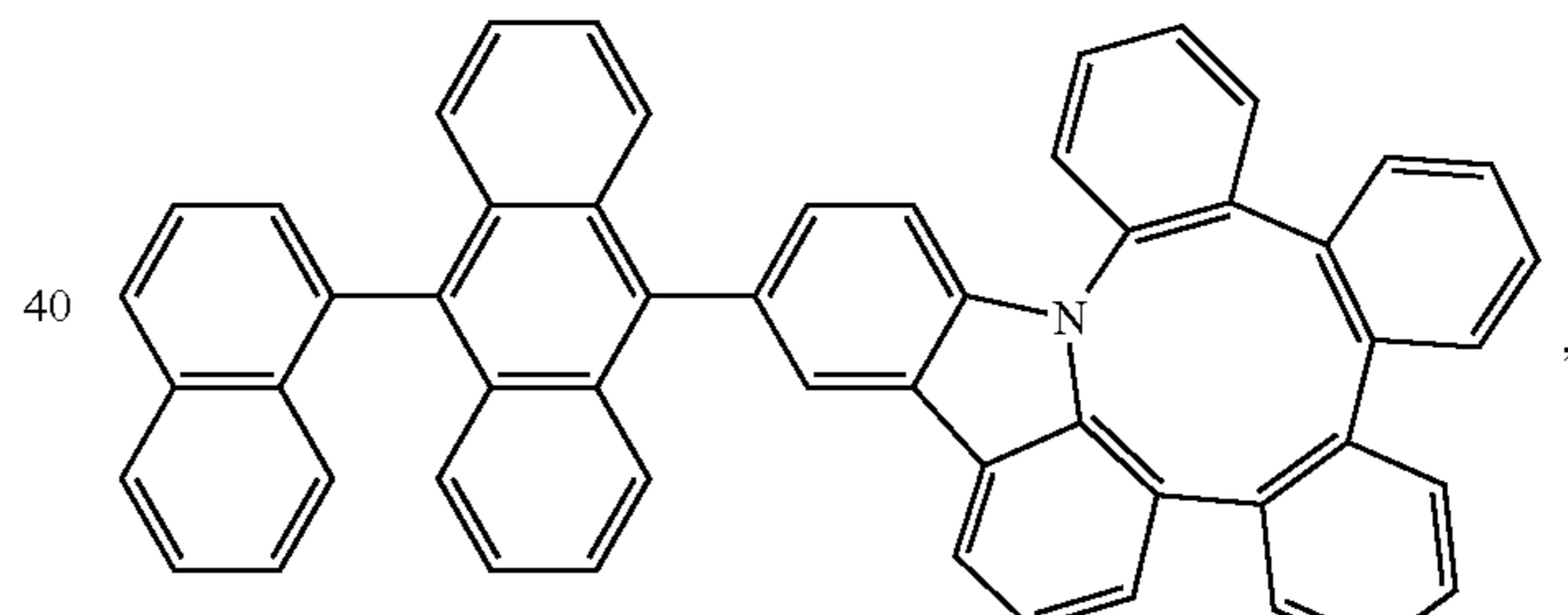
Compound 38
