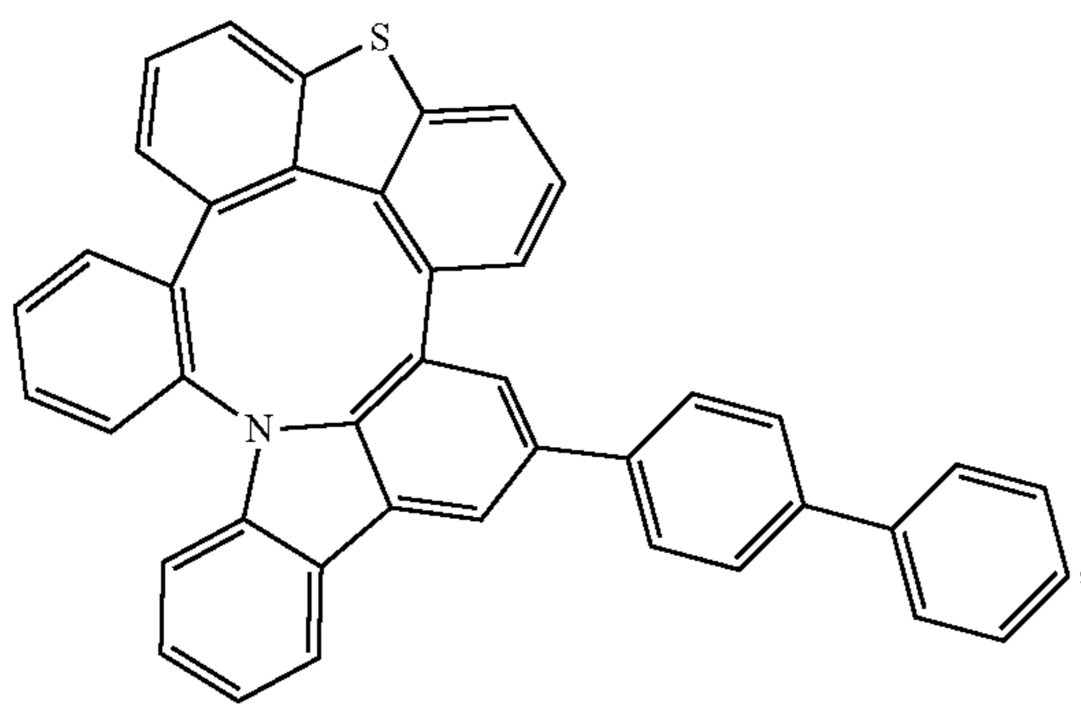
Compound 173
