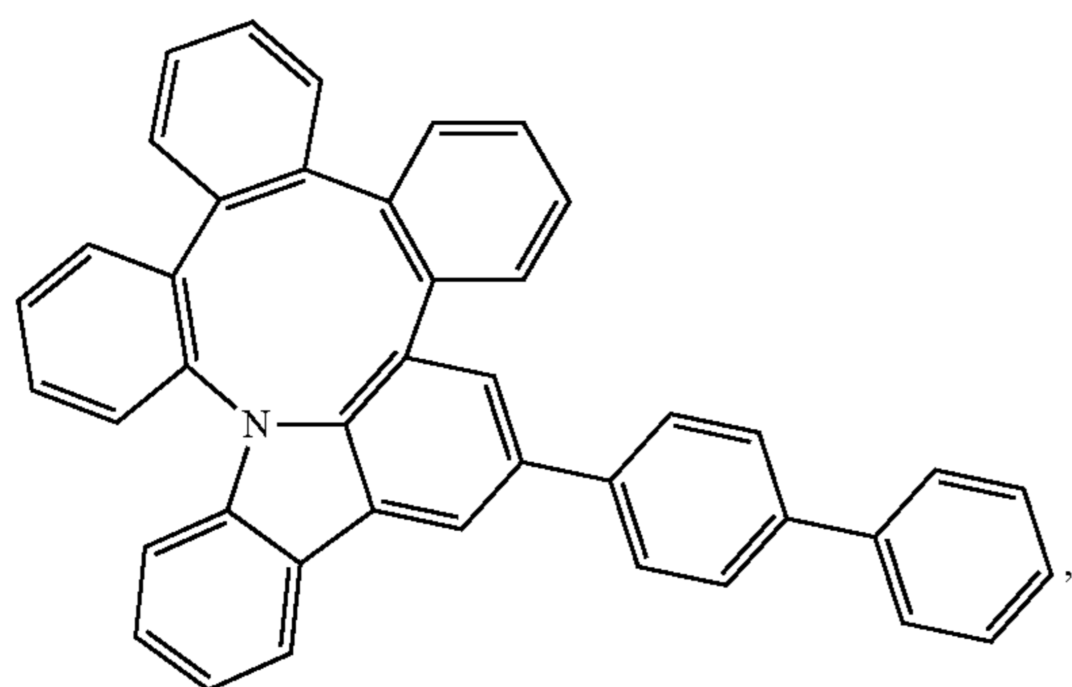
Compound 3
