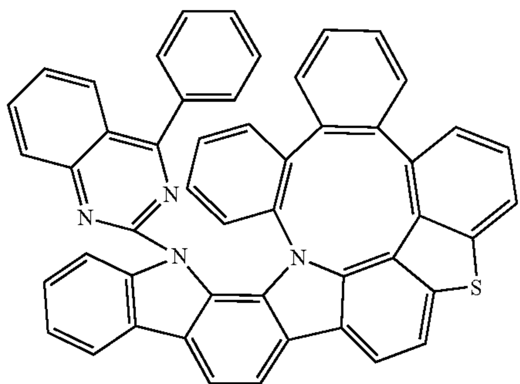
Compound 340
