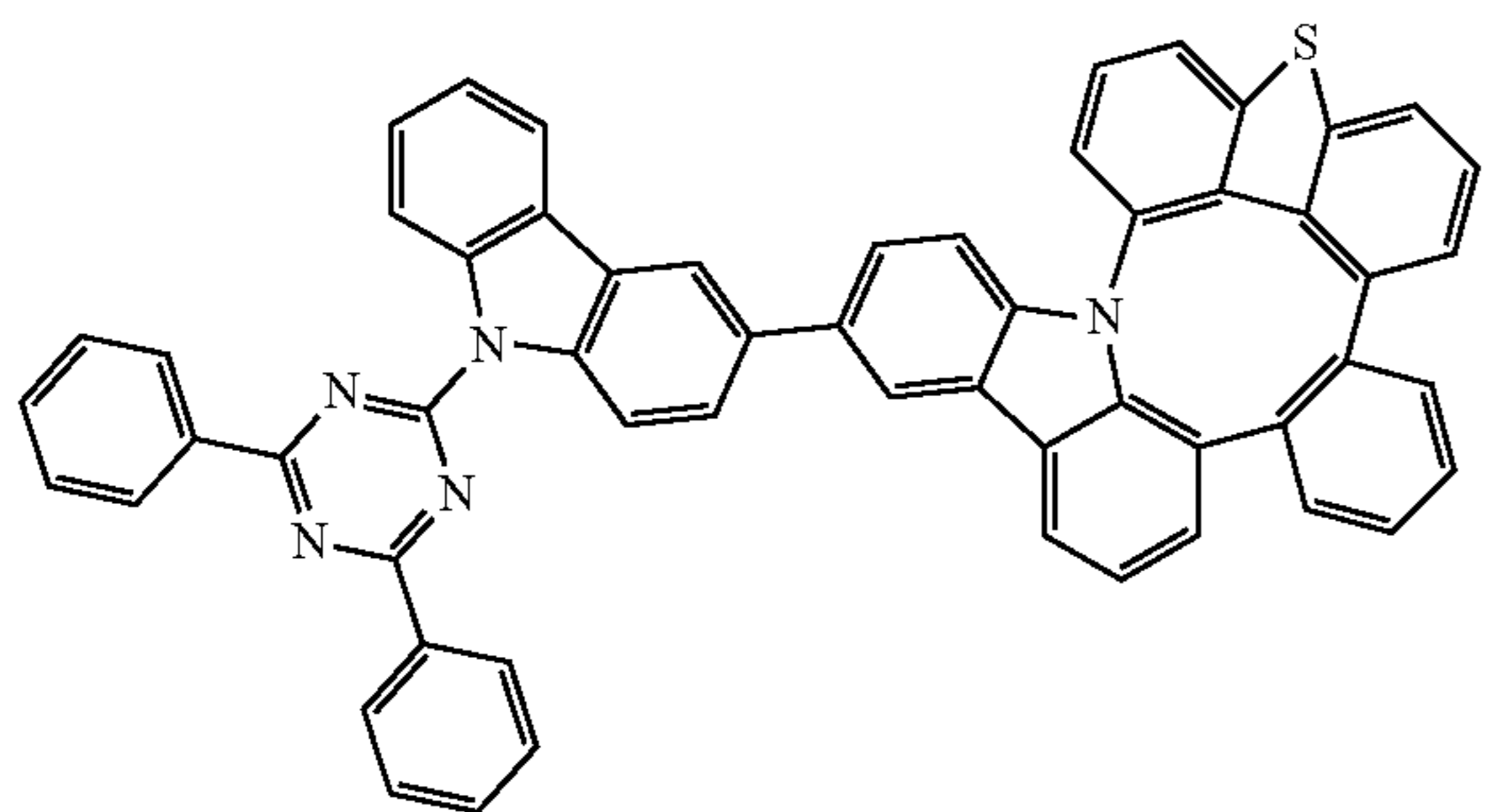
Compound 105
