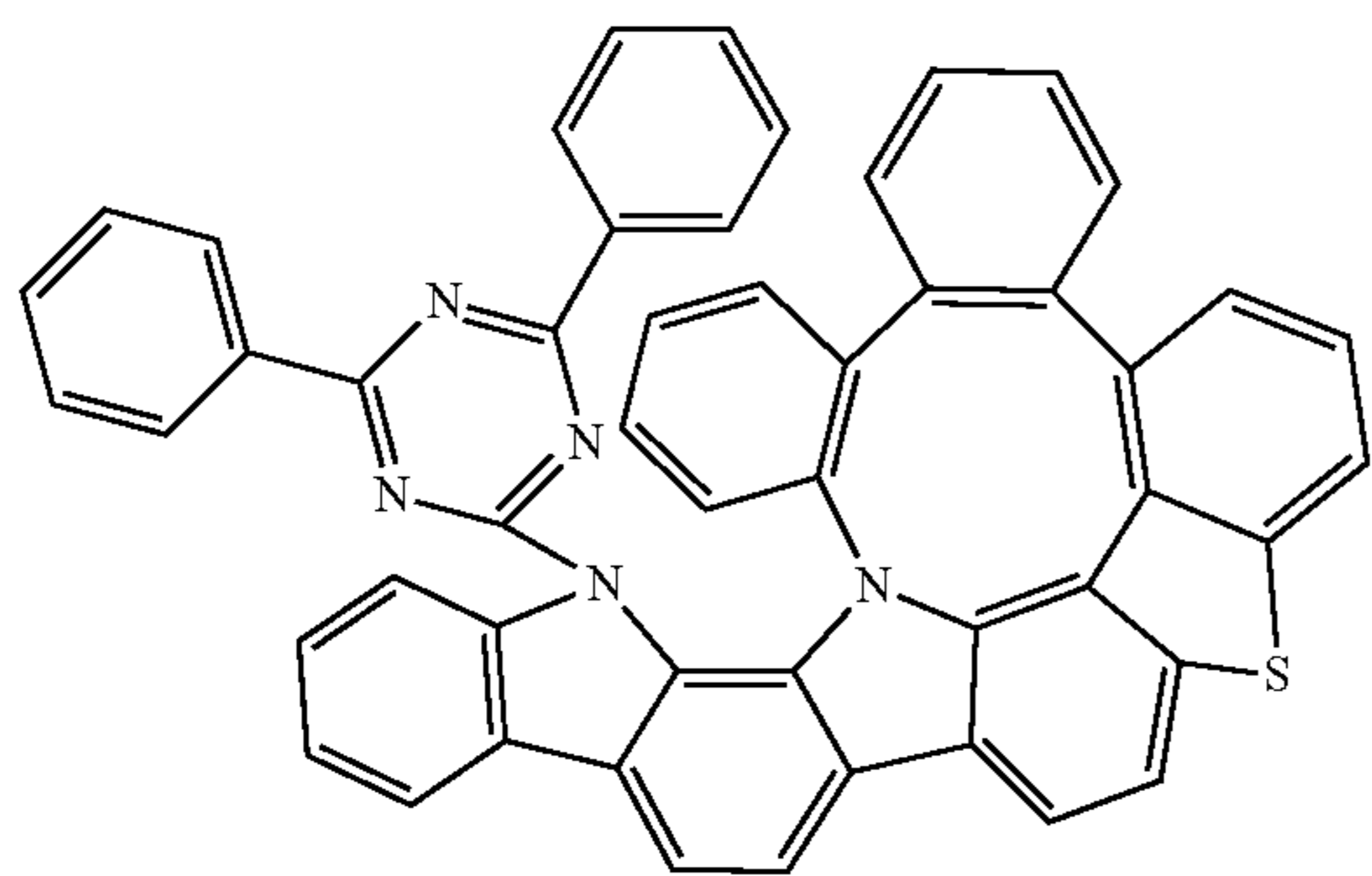
Compound 335
