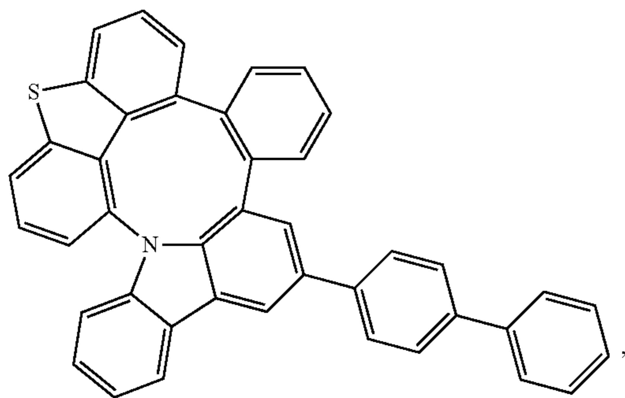
Compound 88
