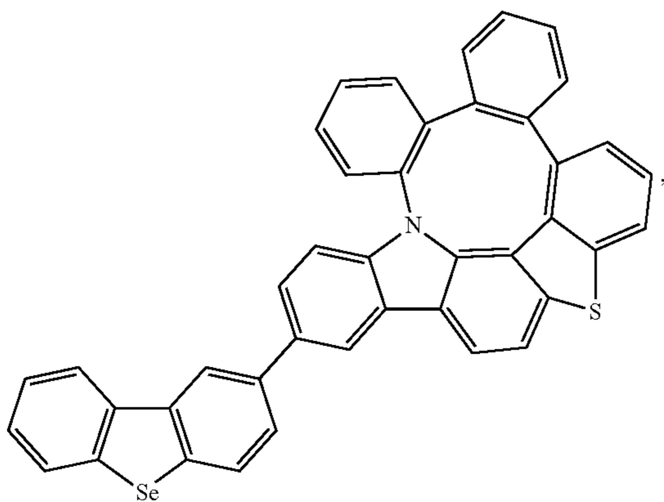
Compound 266
