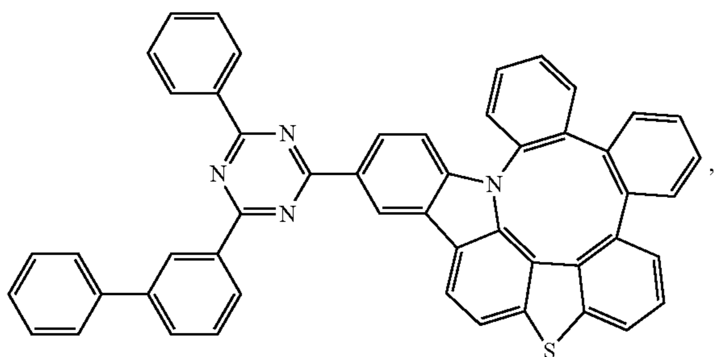
Compound 282
