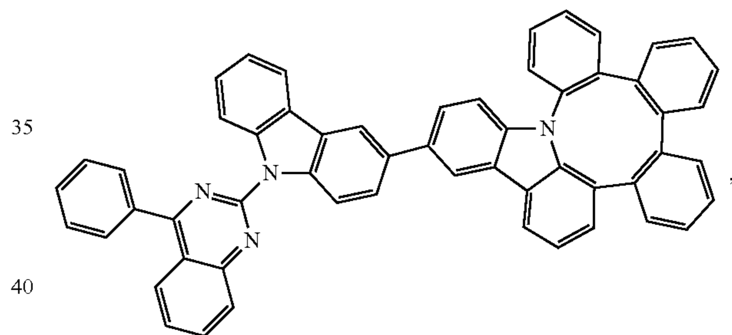
Compound 21
