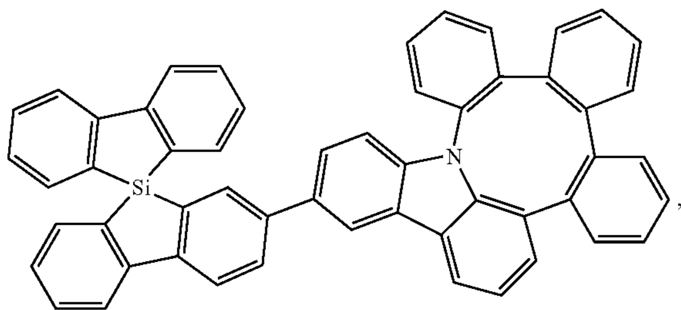
Compound 341
