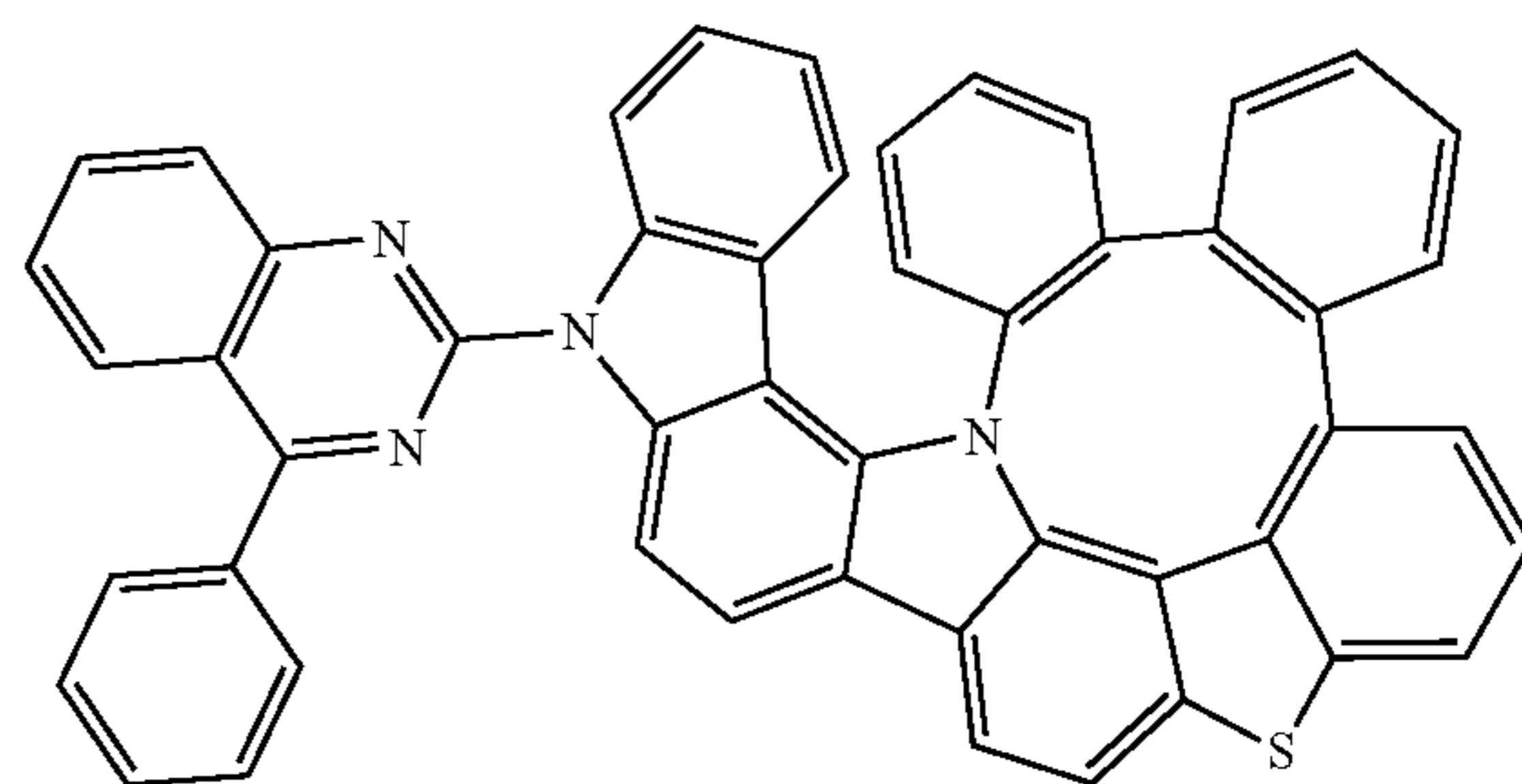
Compound 339
