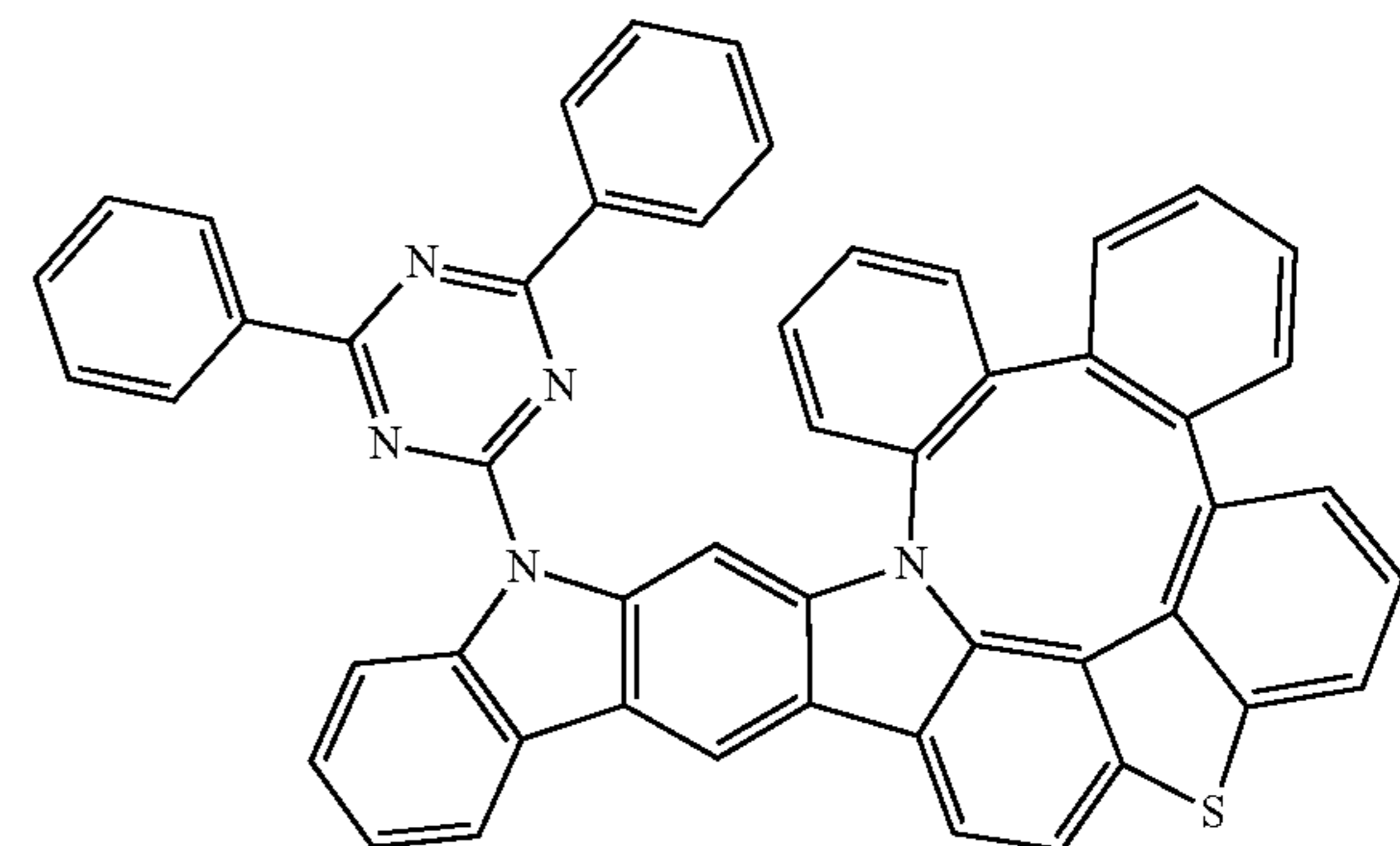
Compound 331
