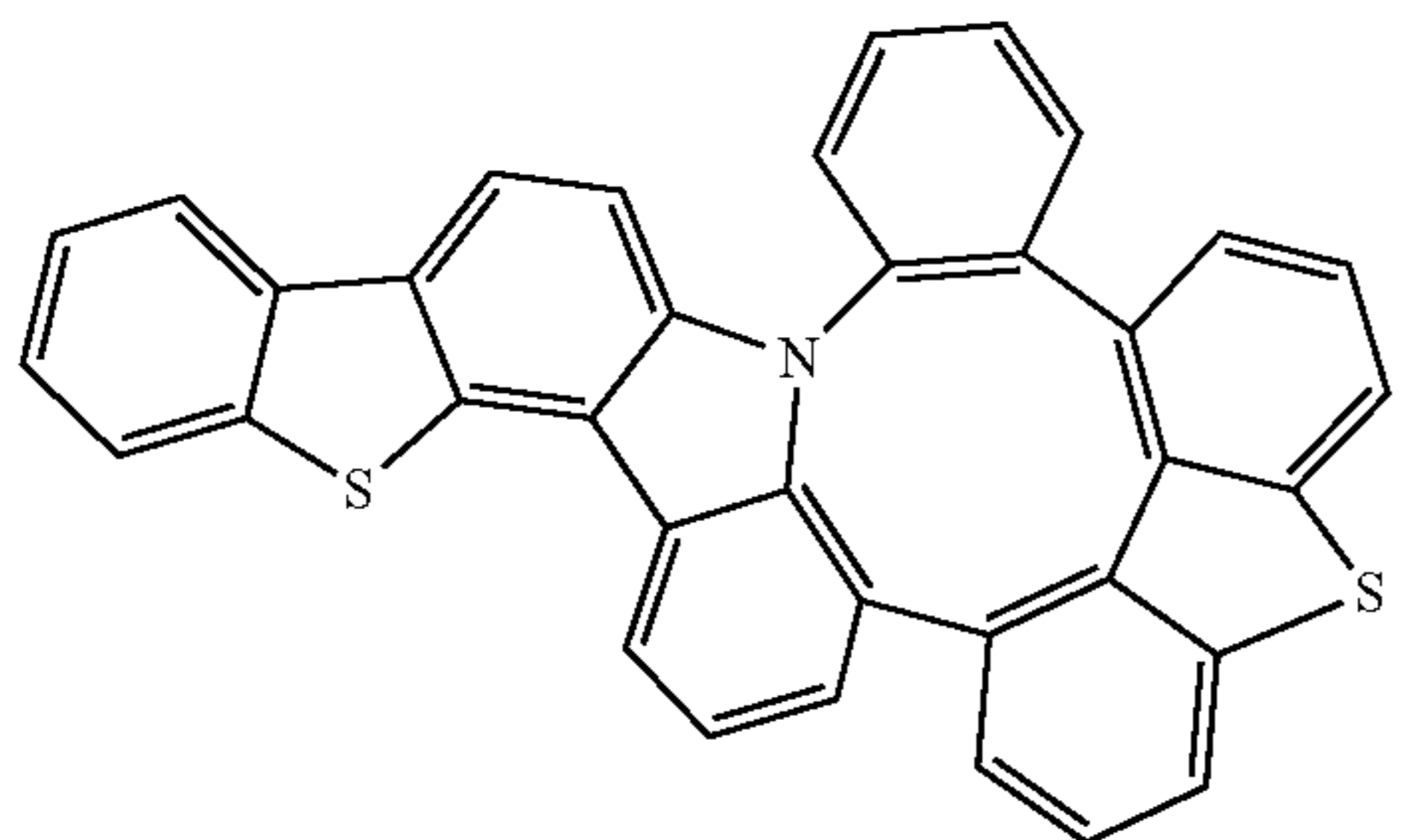
Compound 233
