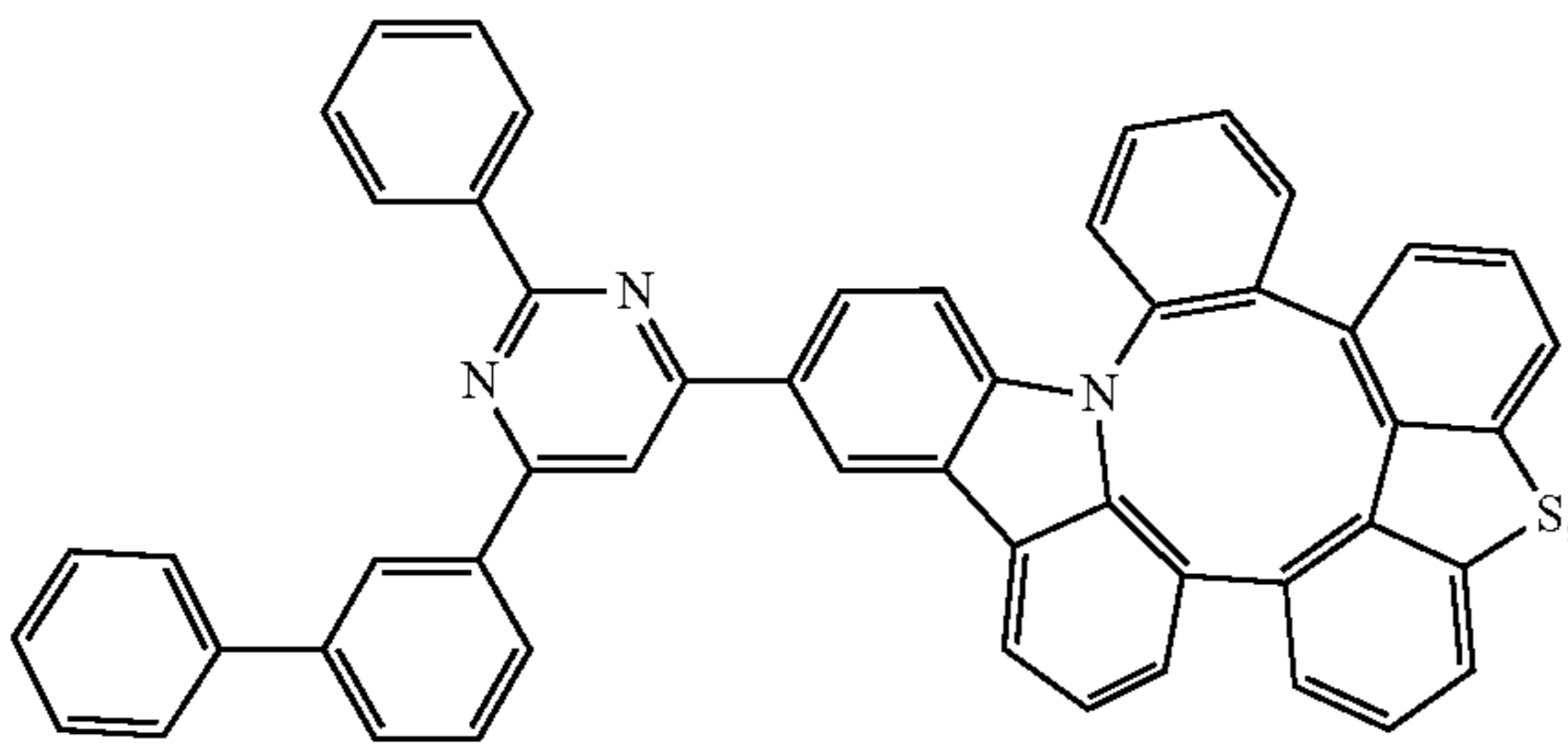
Compound 199
