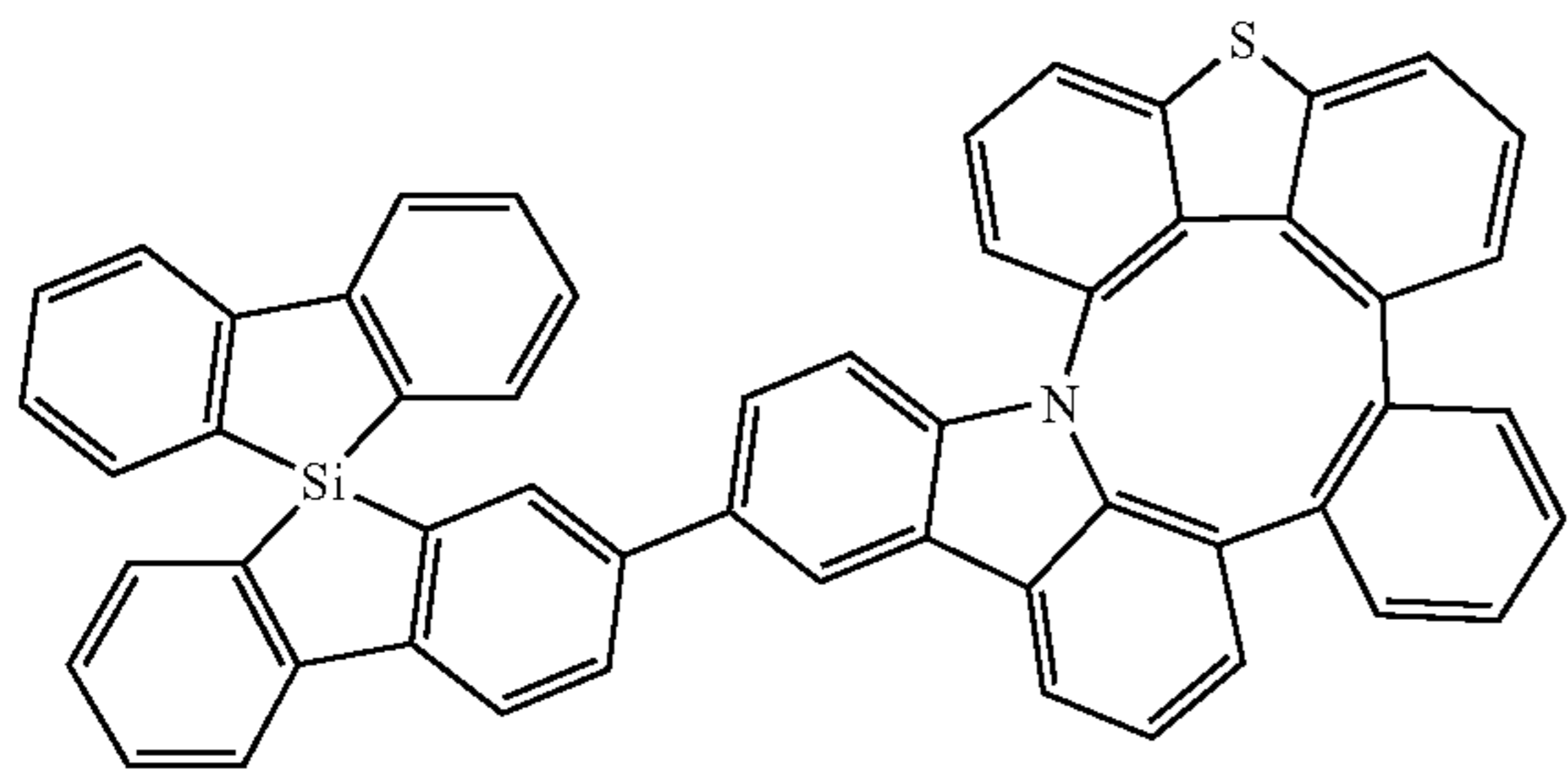
Compound 348
