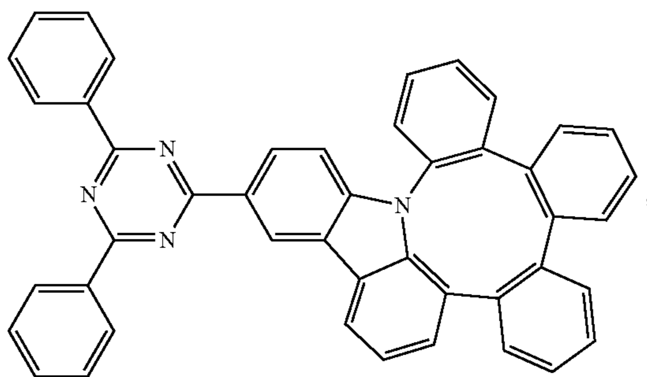
Compound 24
