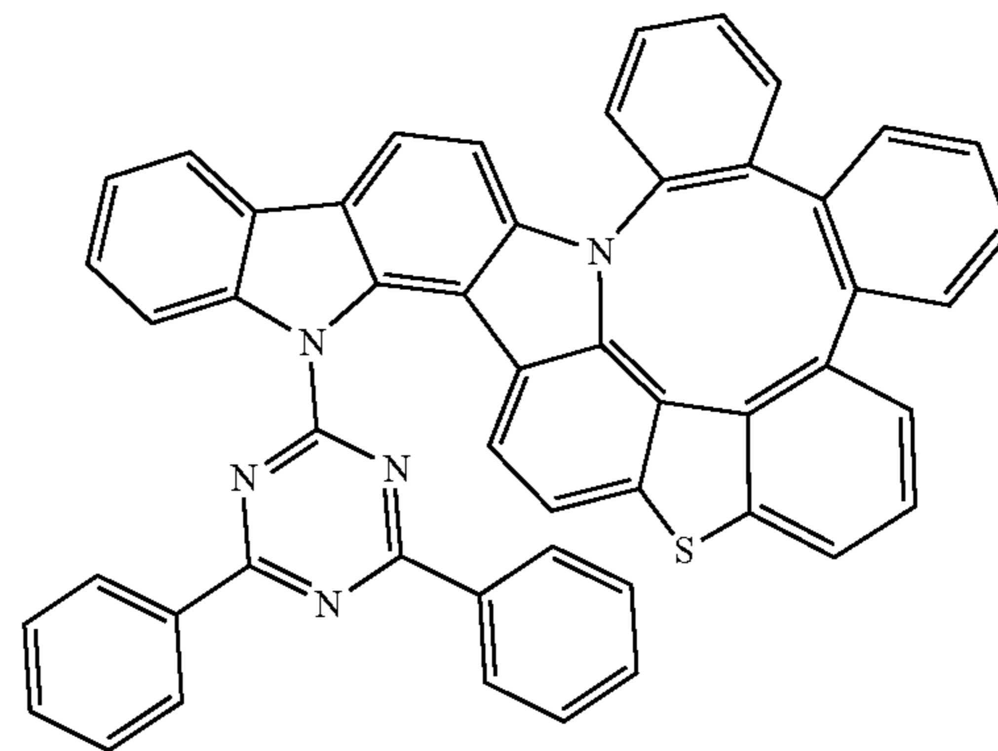
Compound 330
