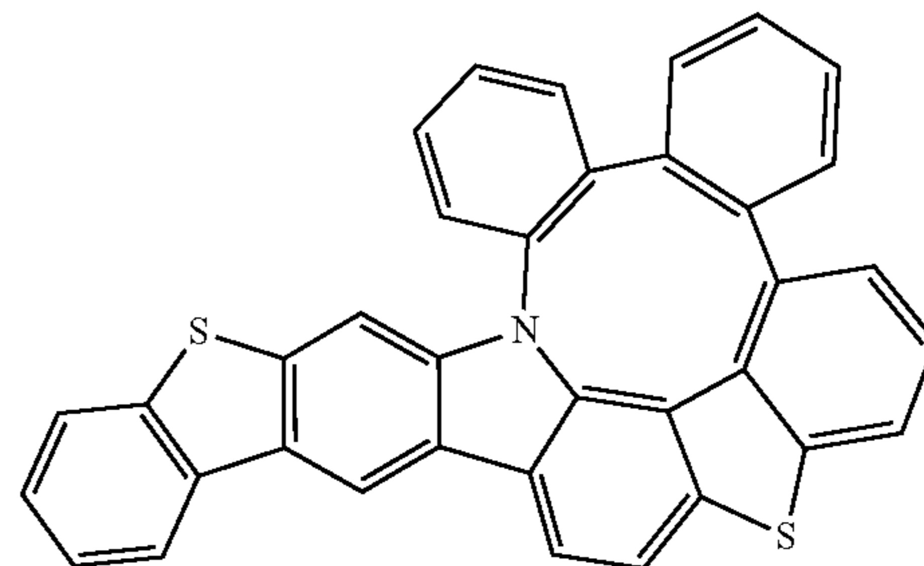
Compound 320
