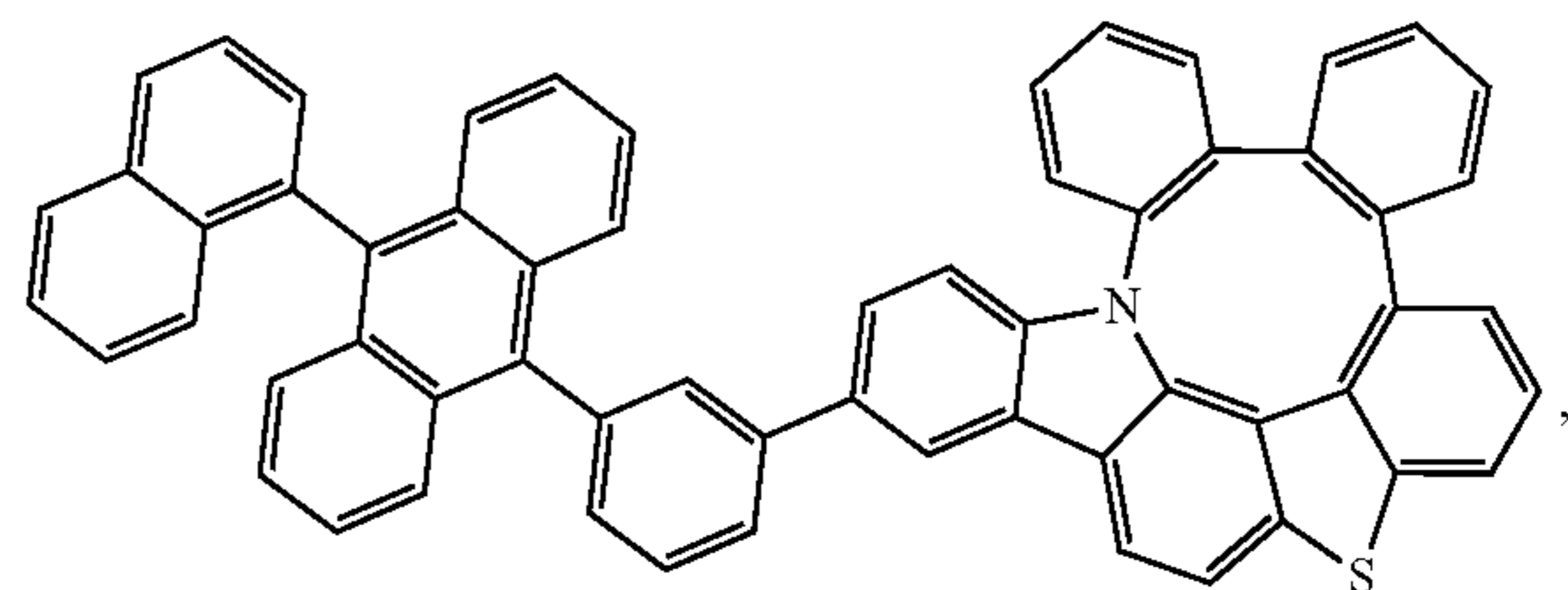
Compound 294
