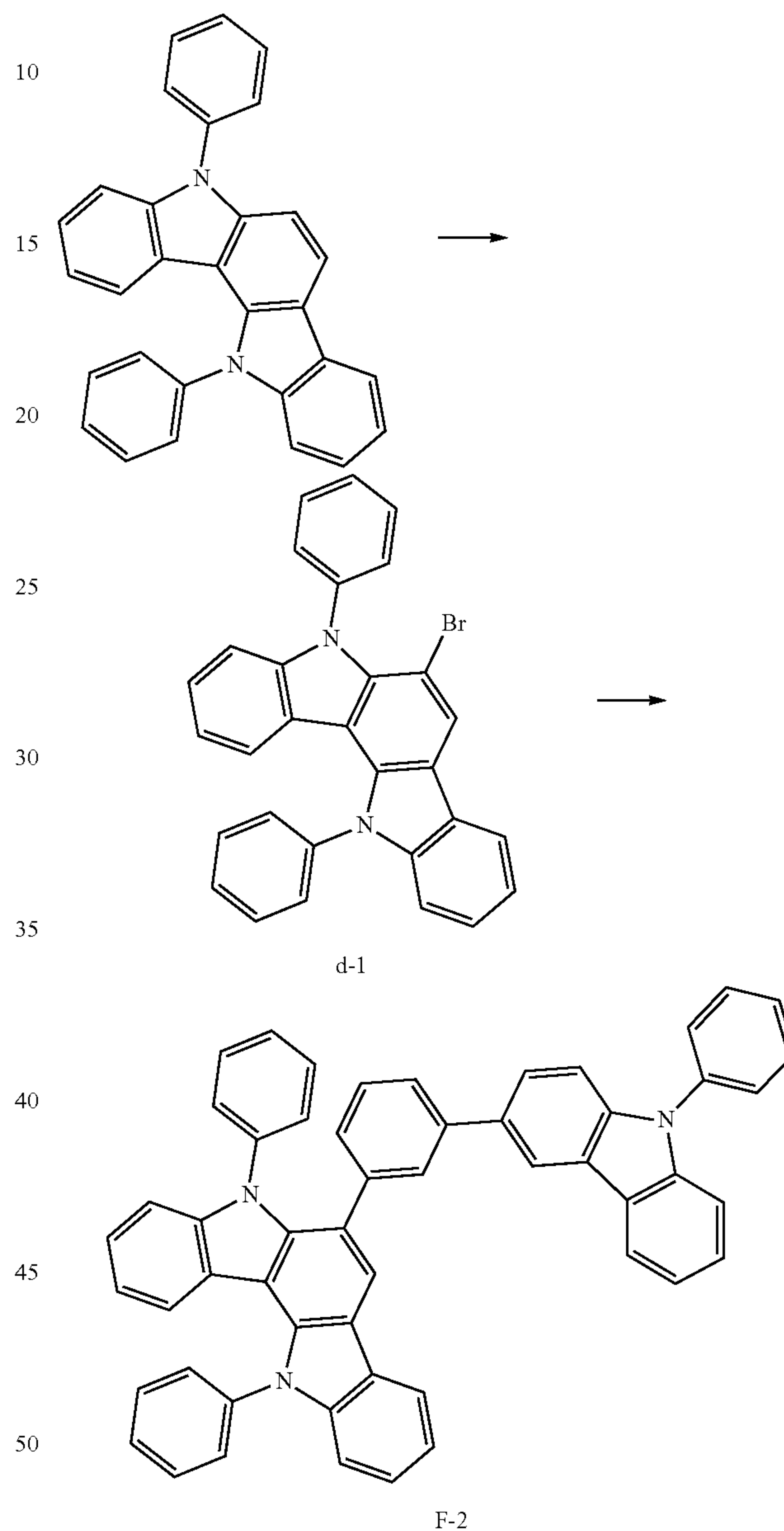
[Reaction Scheme 4]
