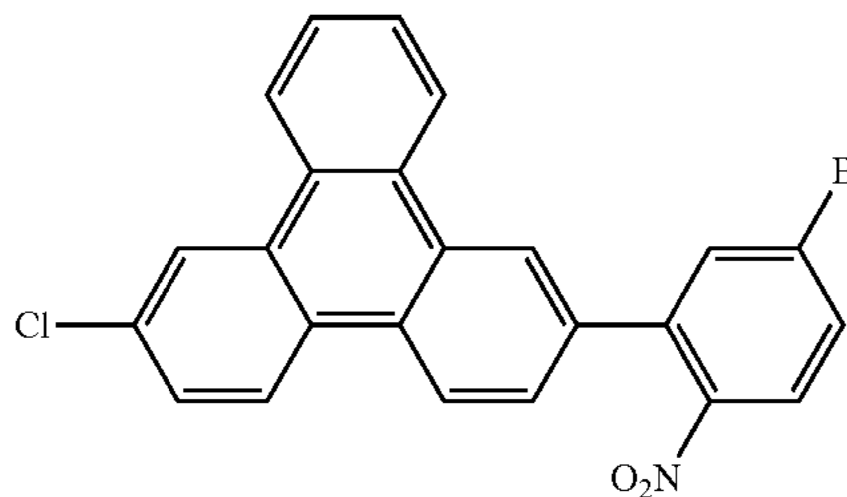
Intermediate 1-1
