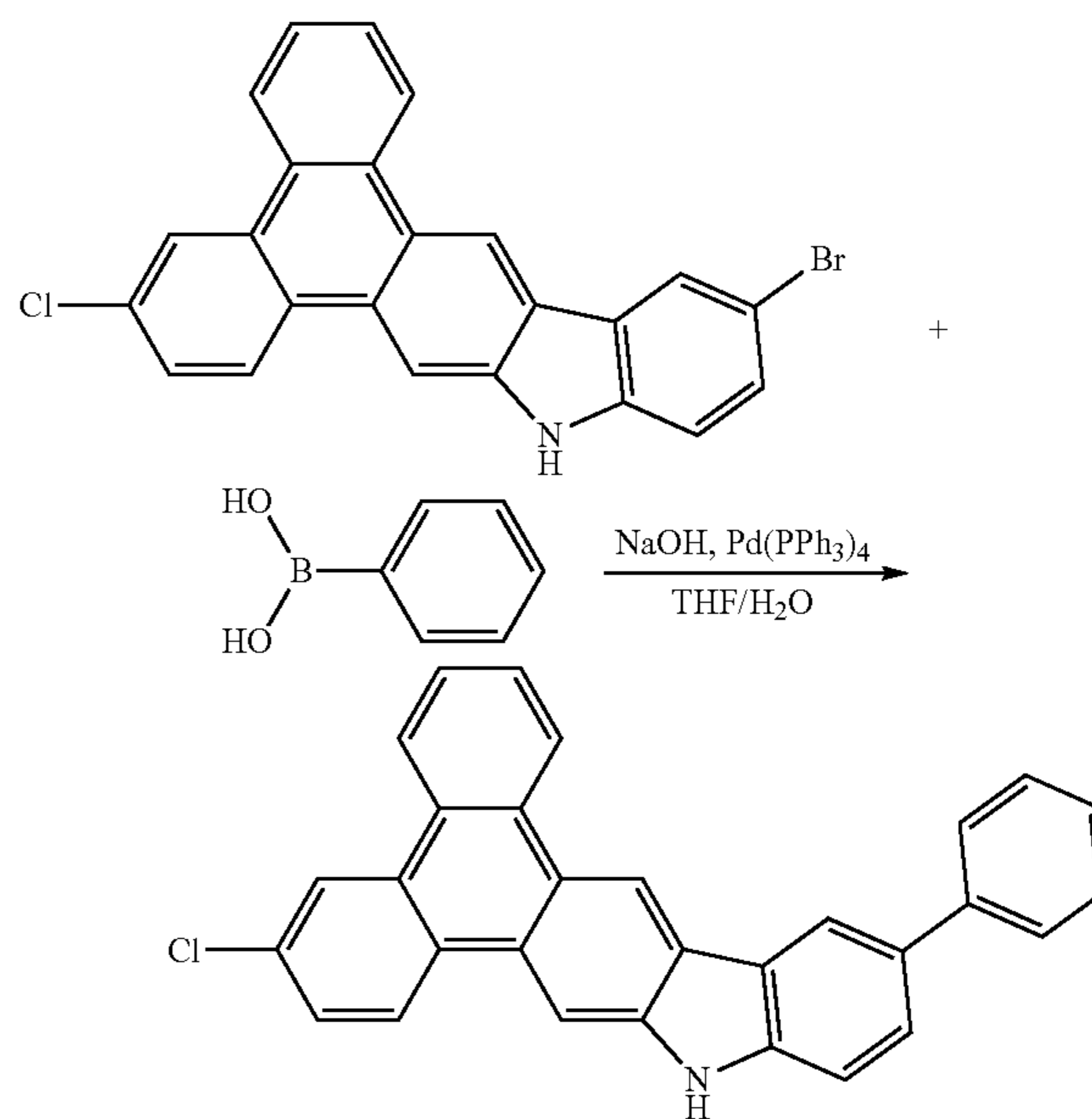
Intermediate 1-3
