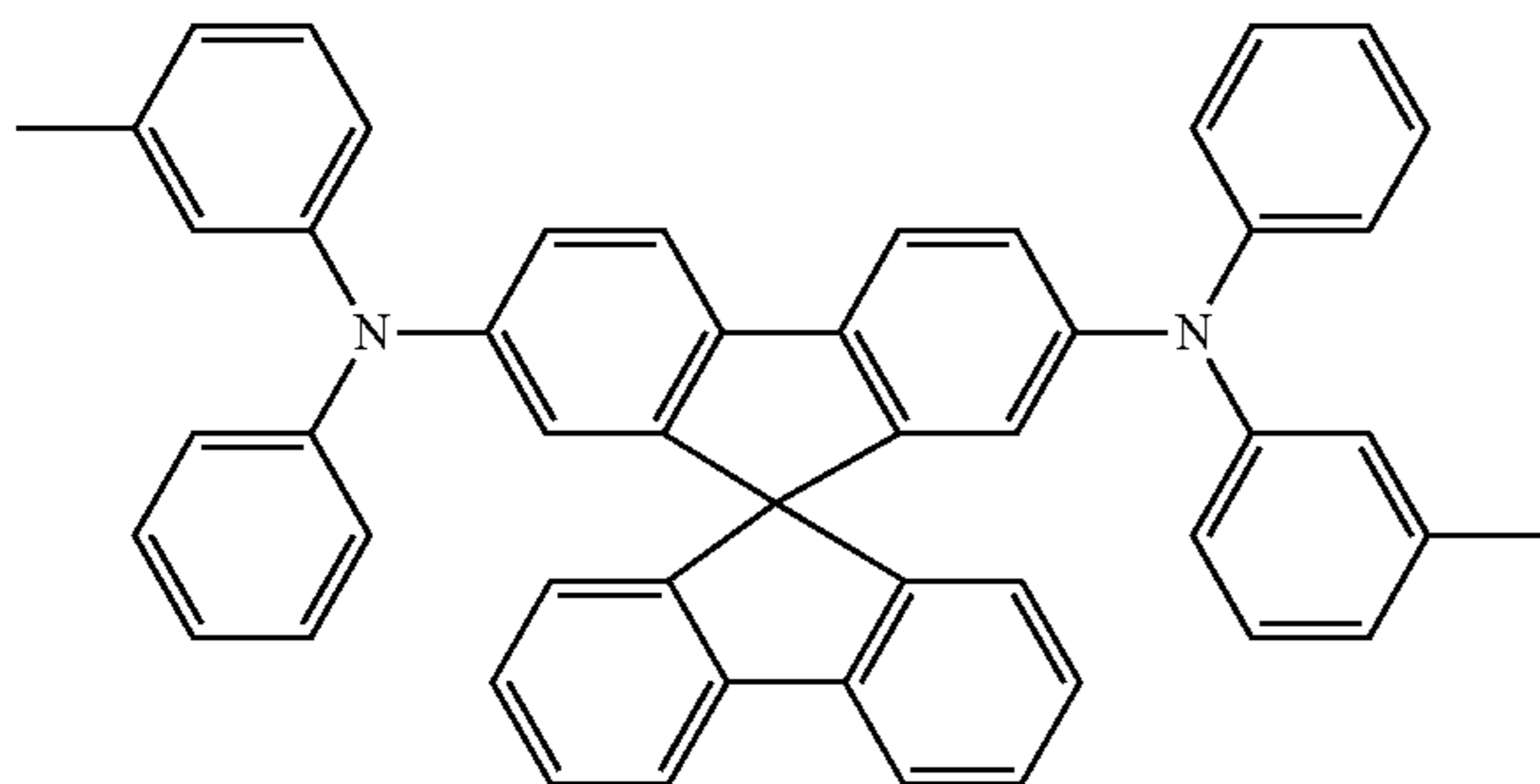
Spiro-TPD
