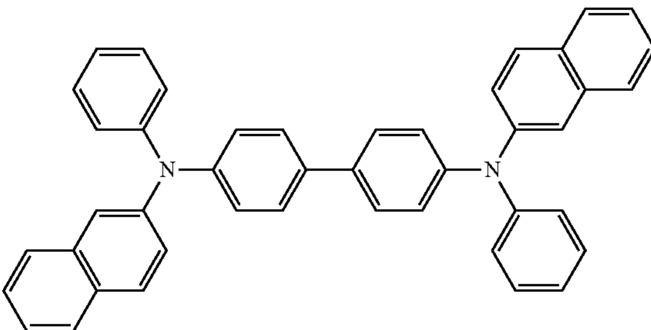
\beta -NPB
