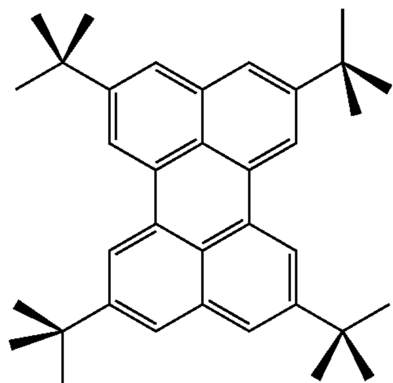
TBPc
