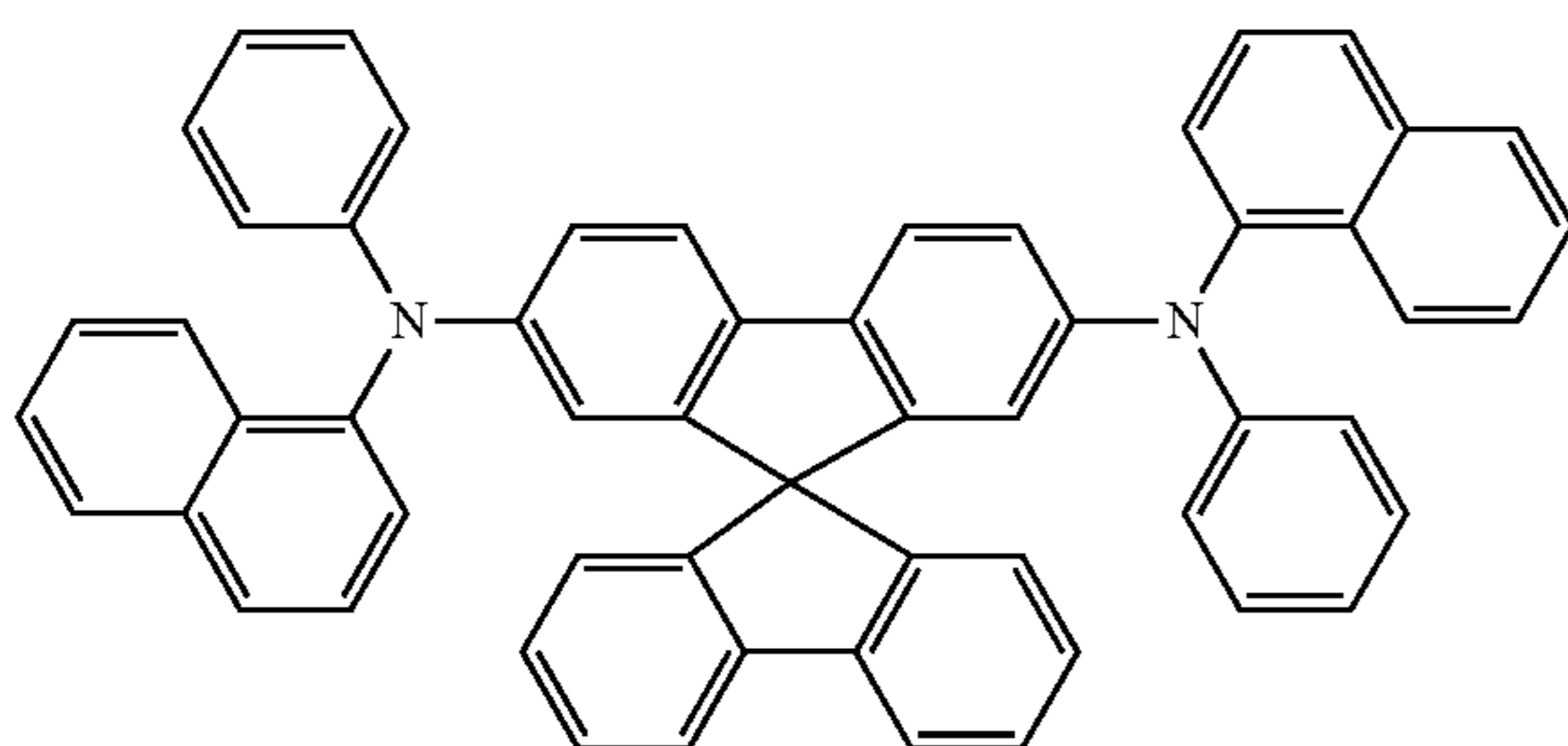
Spiro-NPB
