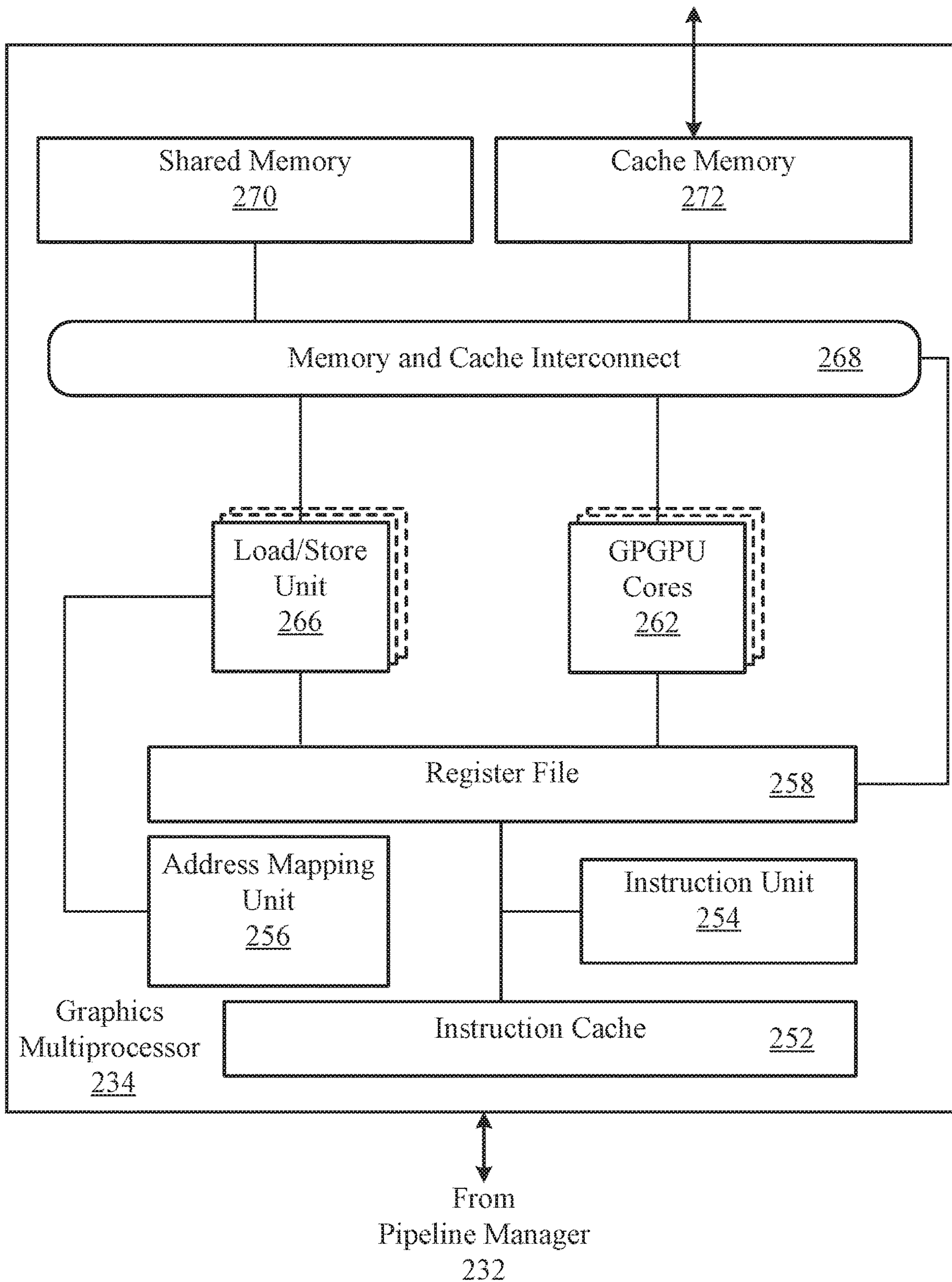
FIG. 2D
