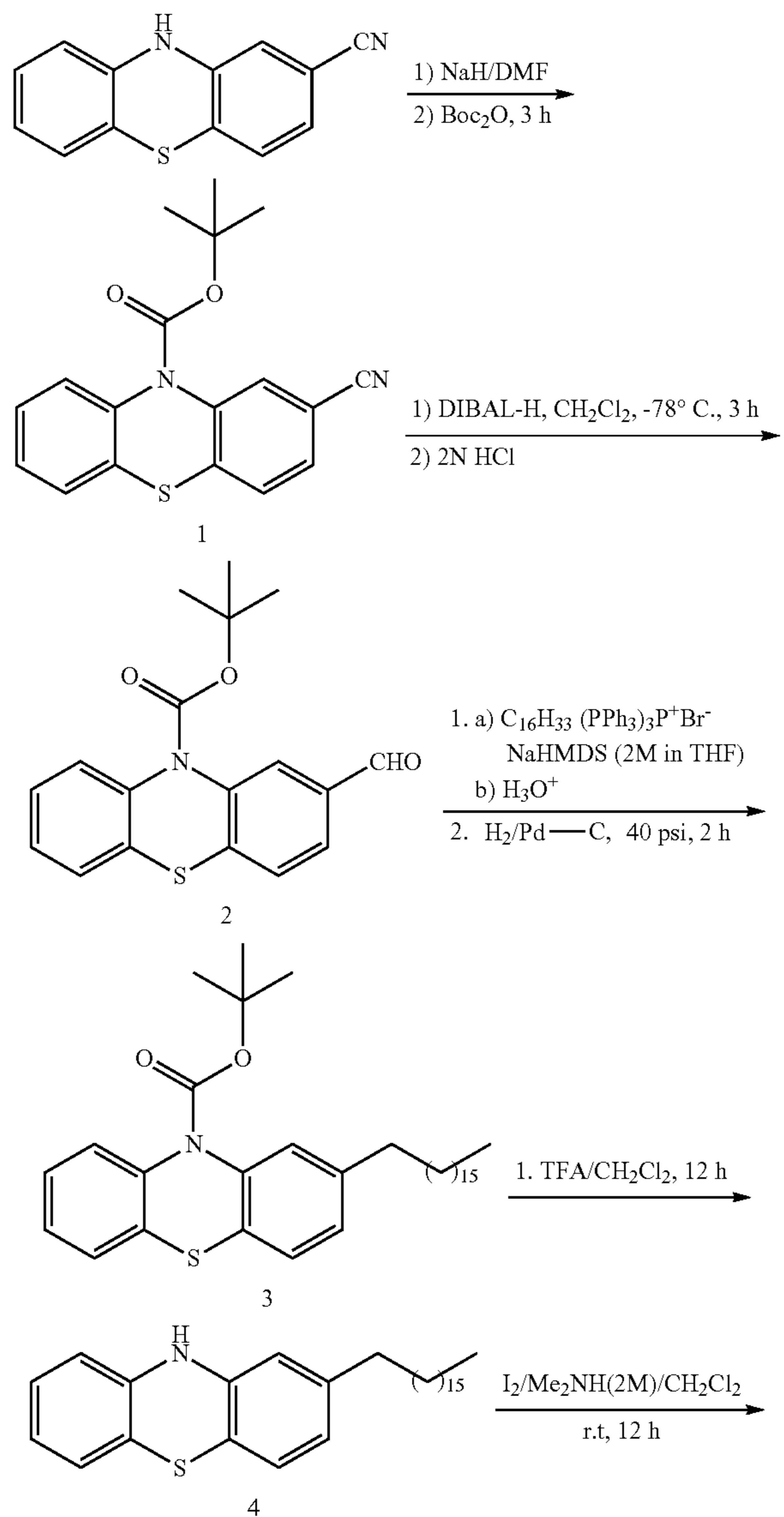
Scheme 1
