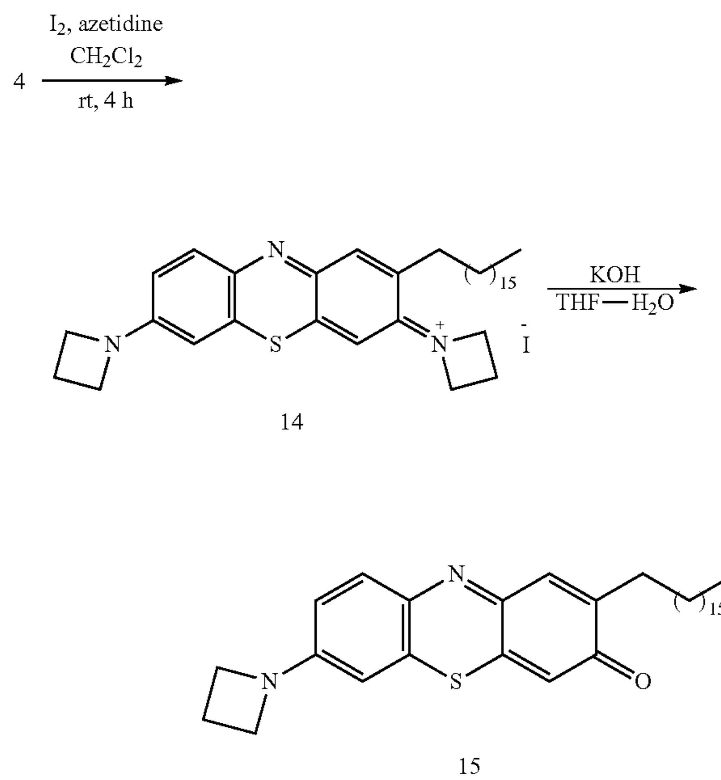
Scheme 6
