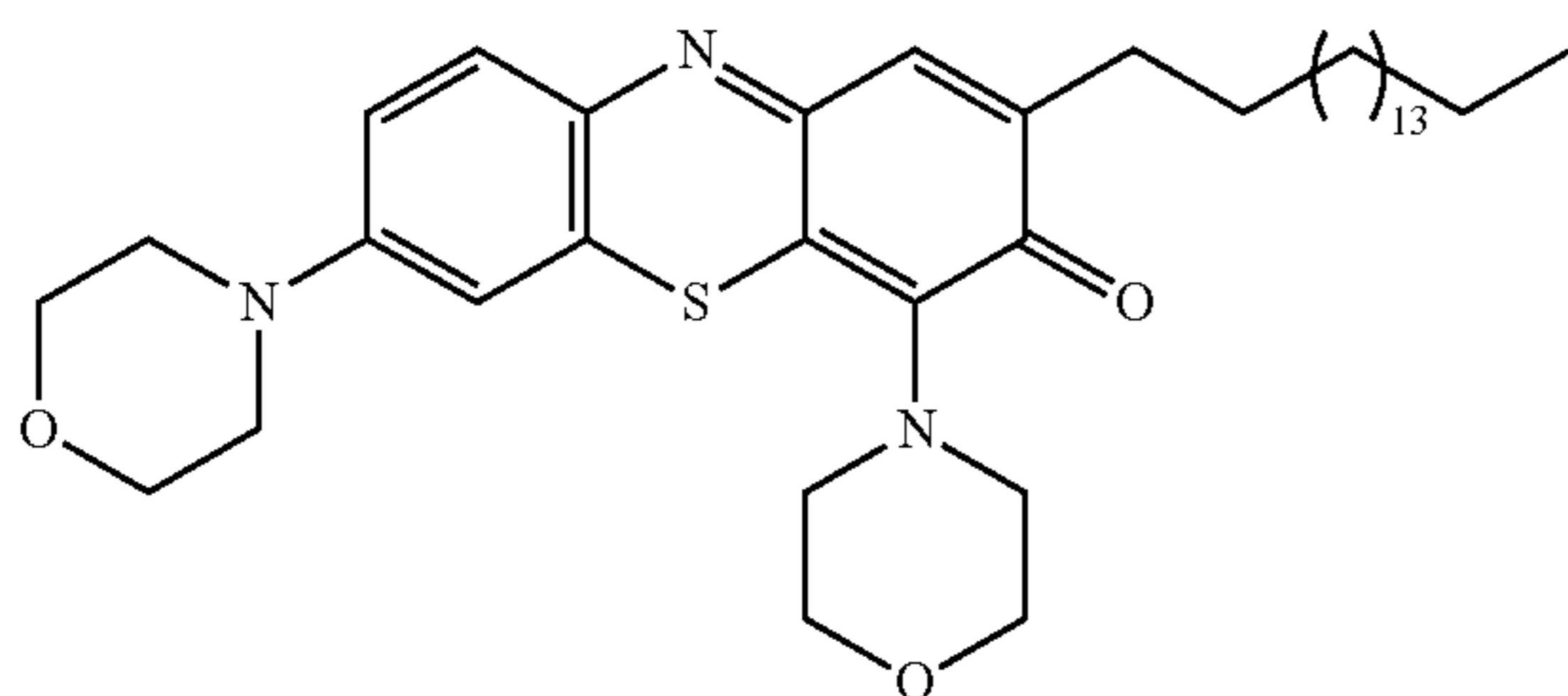
4,7-bis(morpholino)-2-heptadecyl-3H-phenothiazin-3-one (13)
