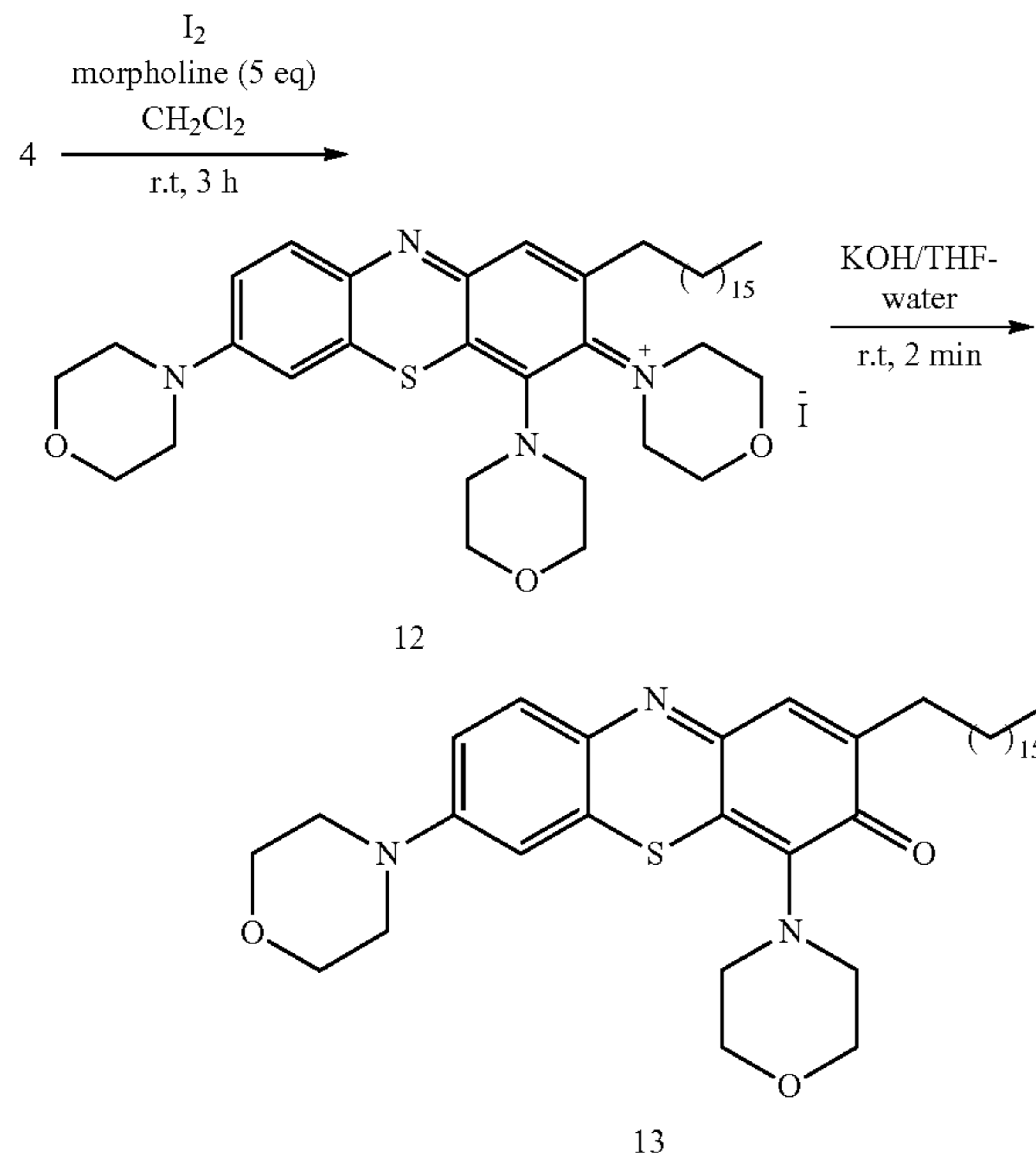
Scheme 5
