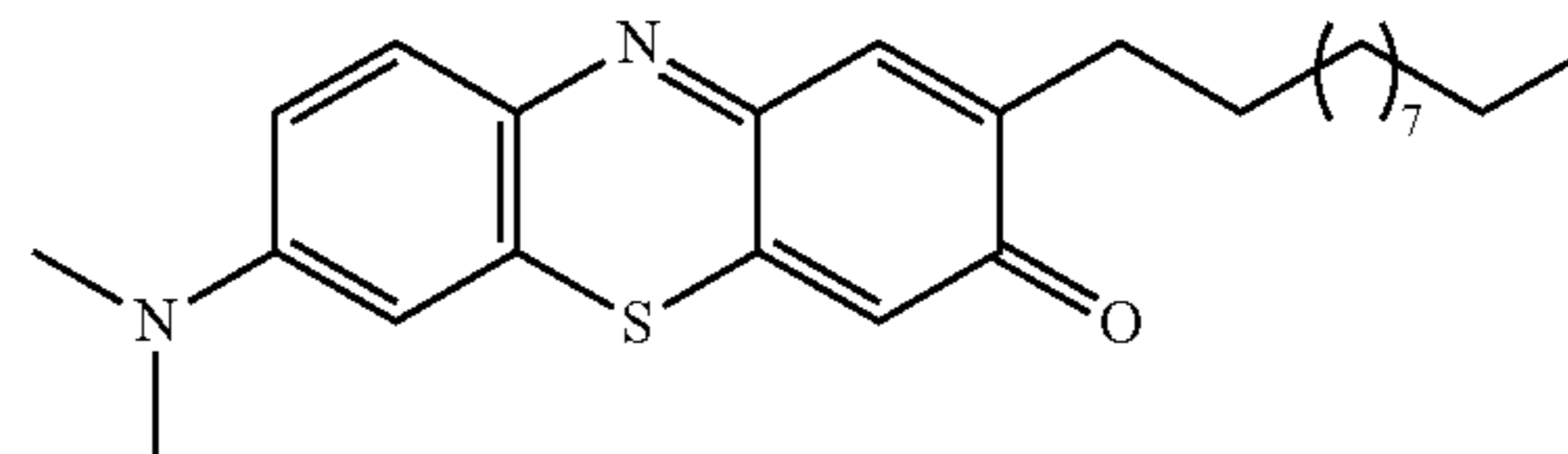
7-(dimethylamino)-2-undecyl-3H-phenothiazin-3-one (23)
