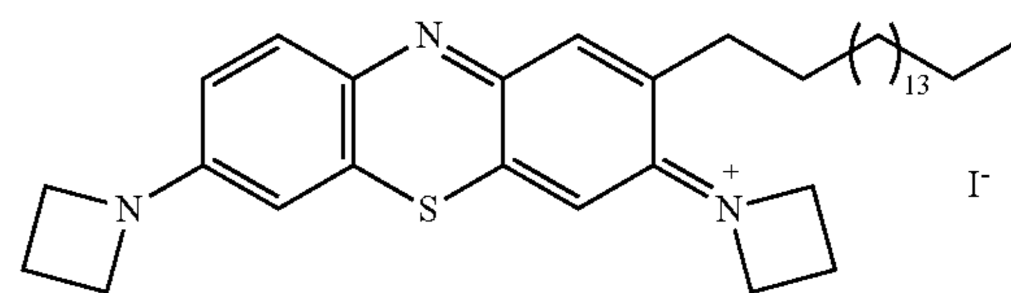
N-(7-(azetidino)-2-heptadecyl-3H-phenothiazin-3-ylidene)-N-azetidinium iodide (14)
