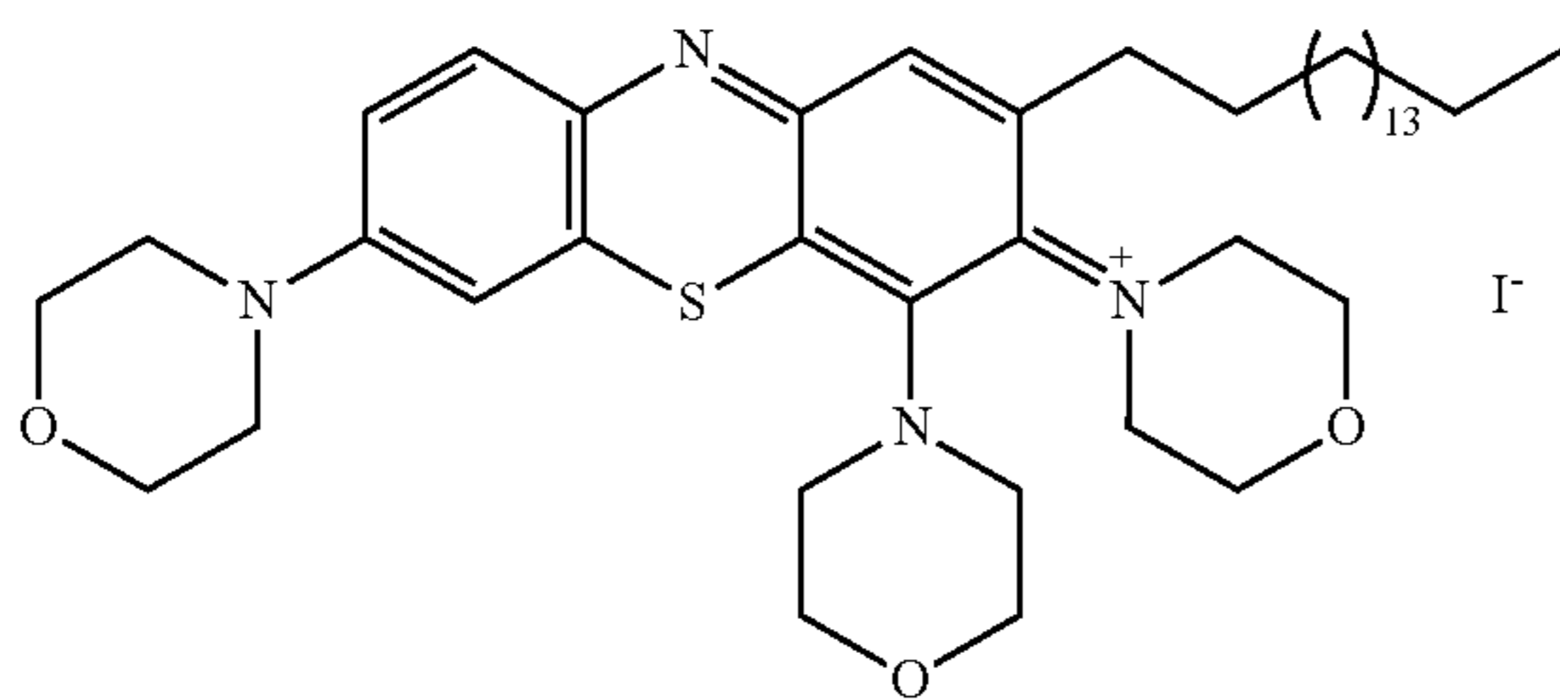
N-(4,7-bis(morpholino)-2-heptadecyl-3H-phenothiazin-3-ylidene)-N-morpholinium iodide (12)
