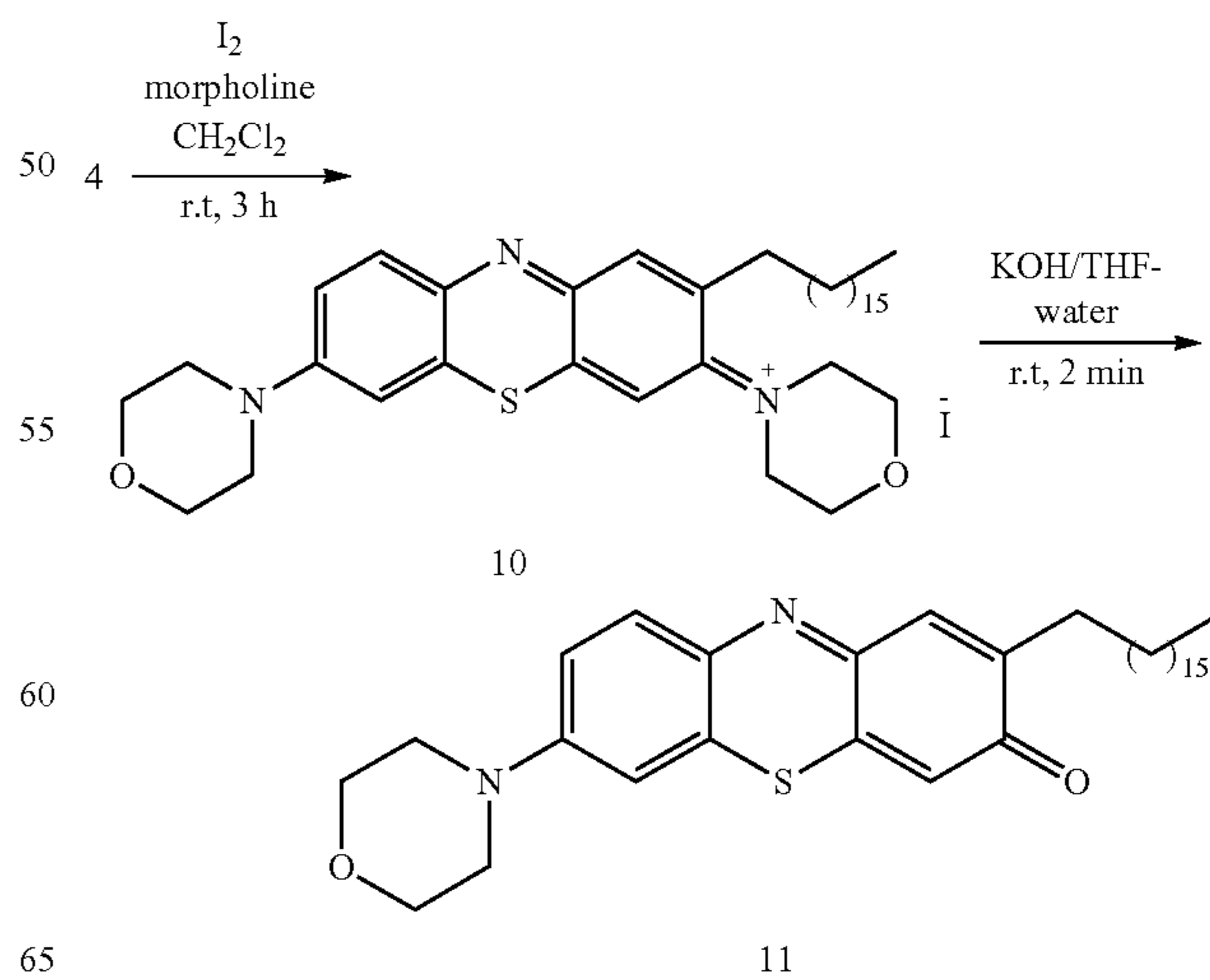
Scheme 4
