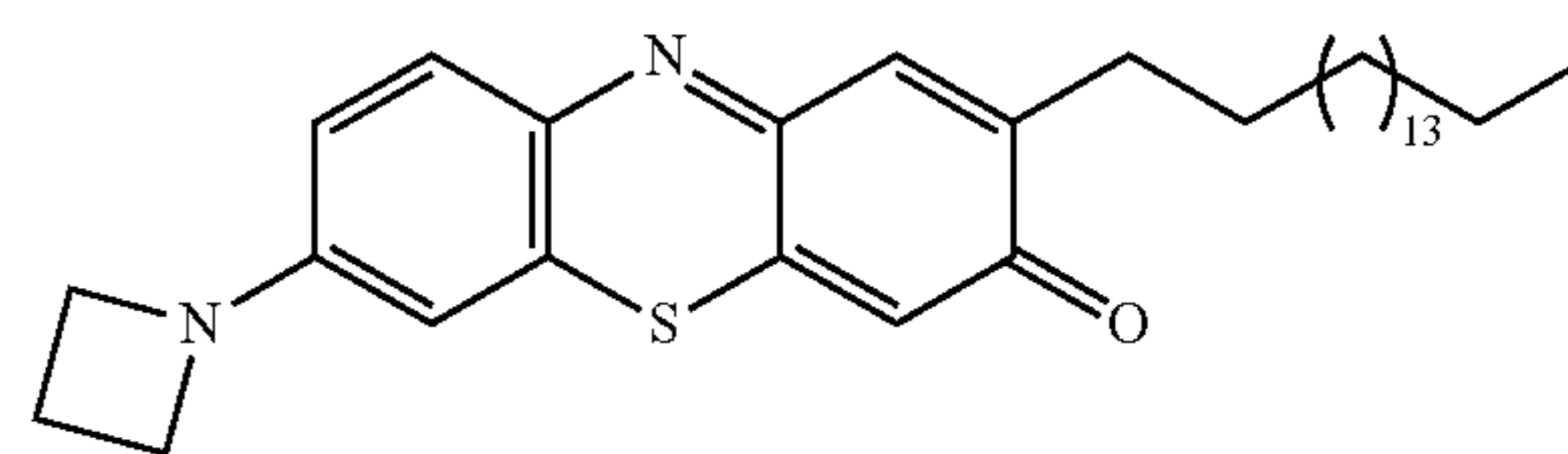
7-(azetidino)-2-heptadecyl-3H-phenothiazin-3-one (15)
