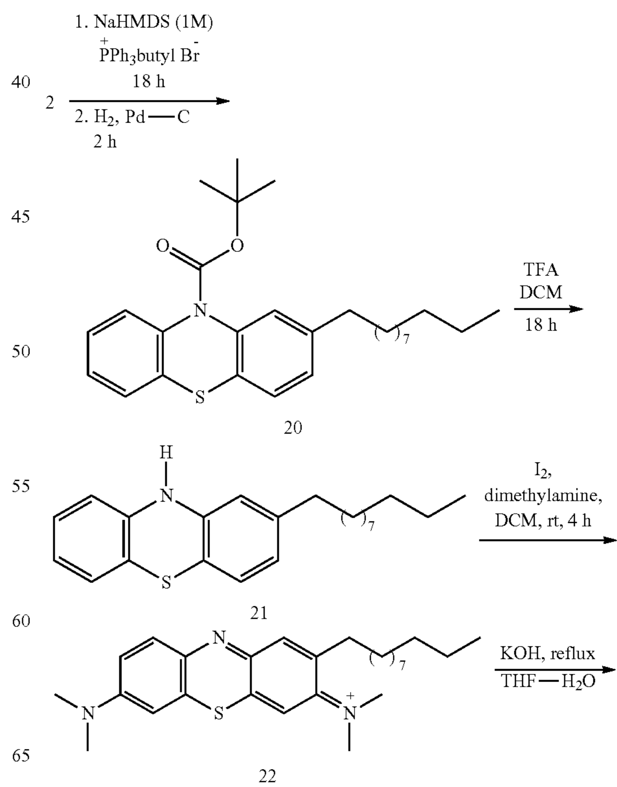
Scheme 8
