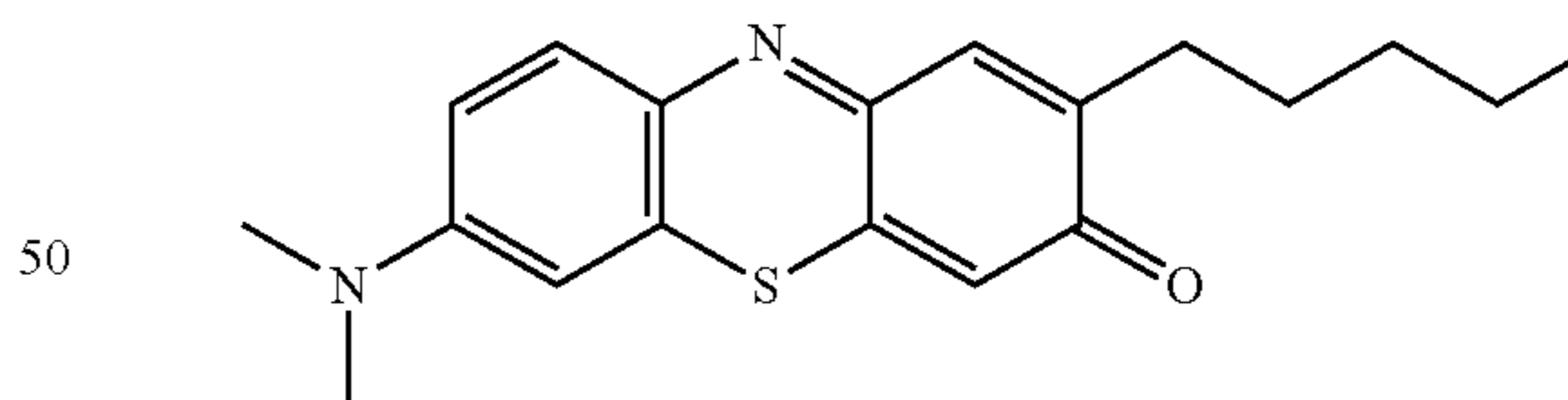
7-(dimethylamino)-2-pentyl-3H-phenothiazin-3-one (19)
