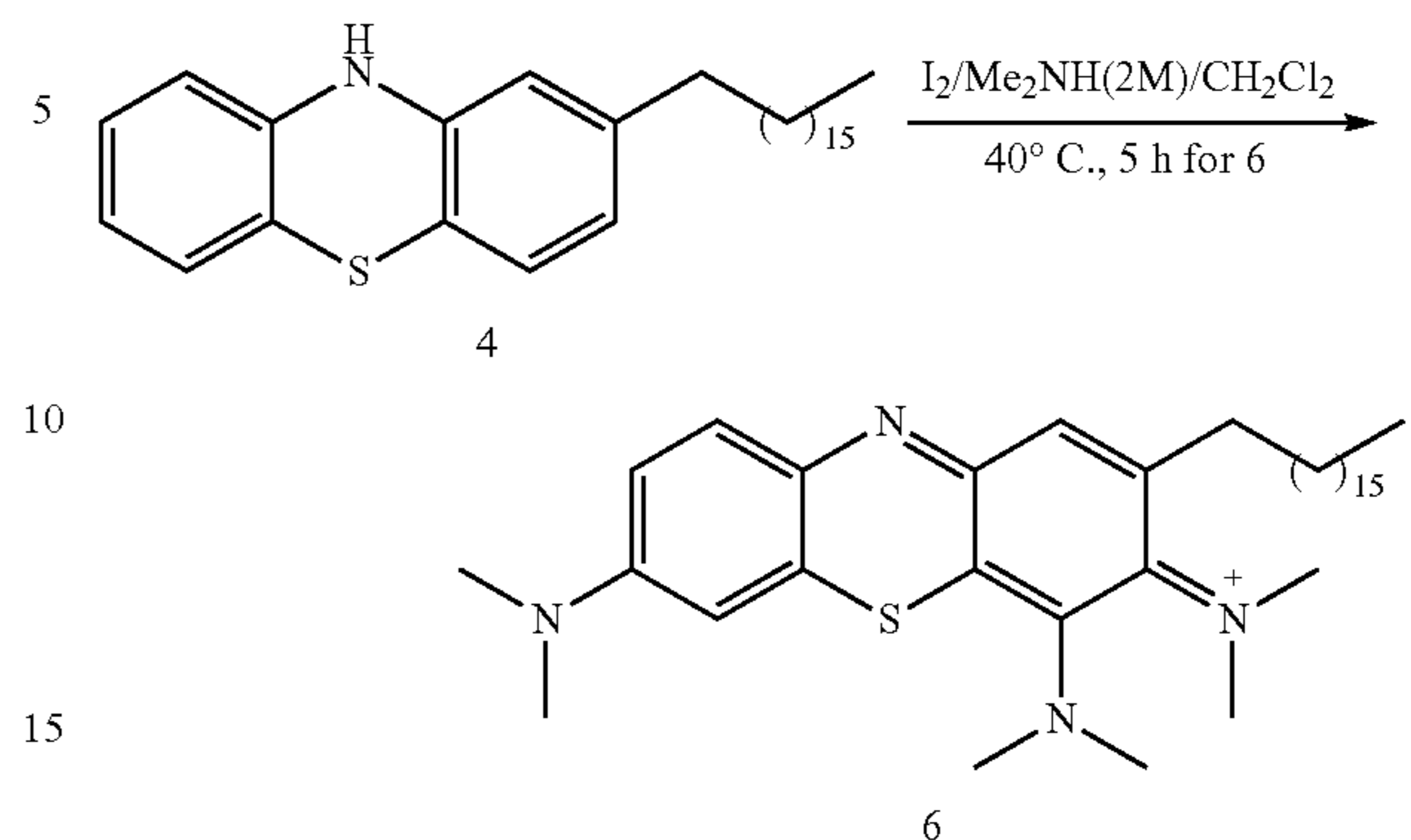
Scheme 2
