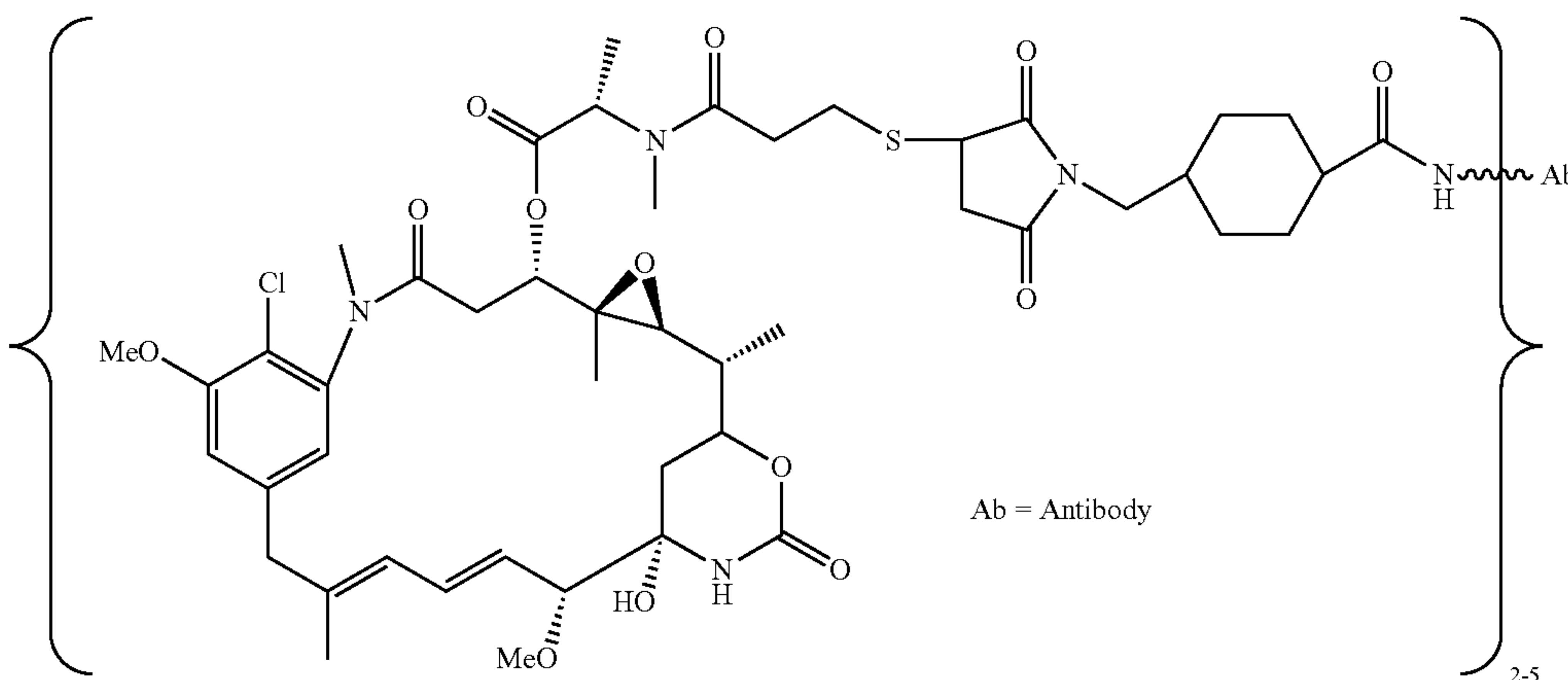
Ab-SMCC-DM1
