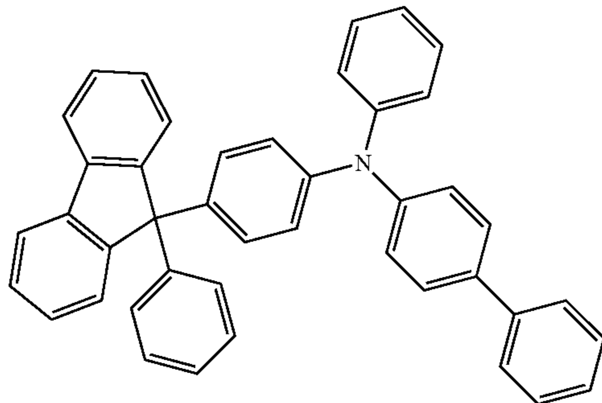
BPAFLP
