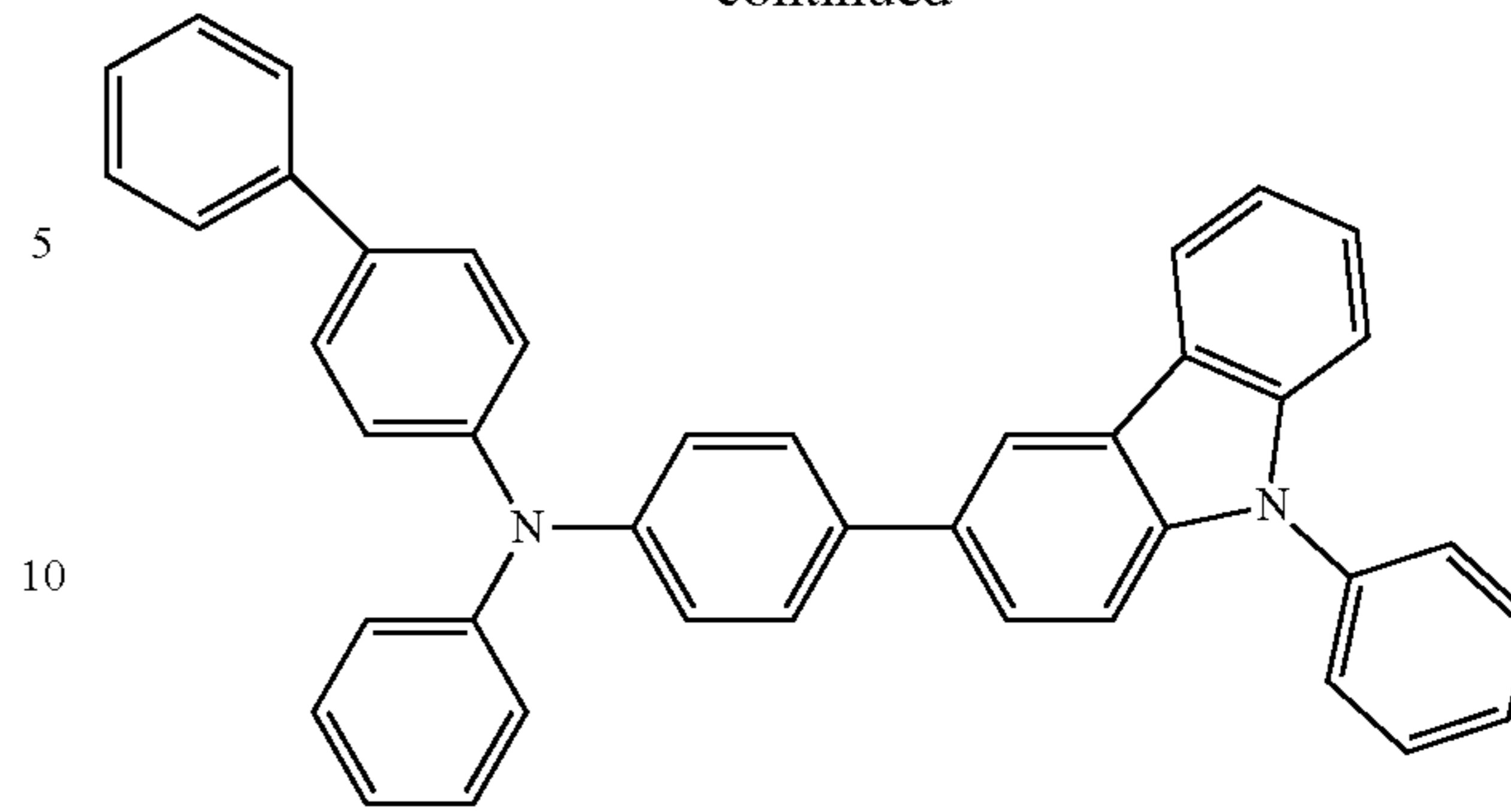
PCBA1BP
