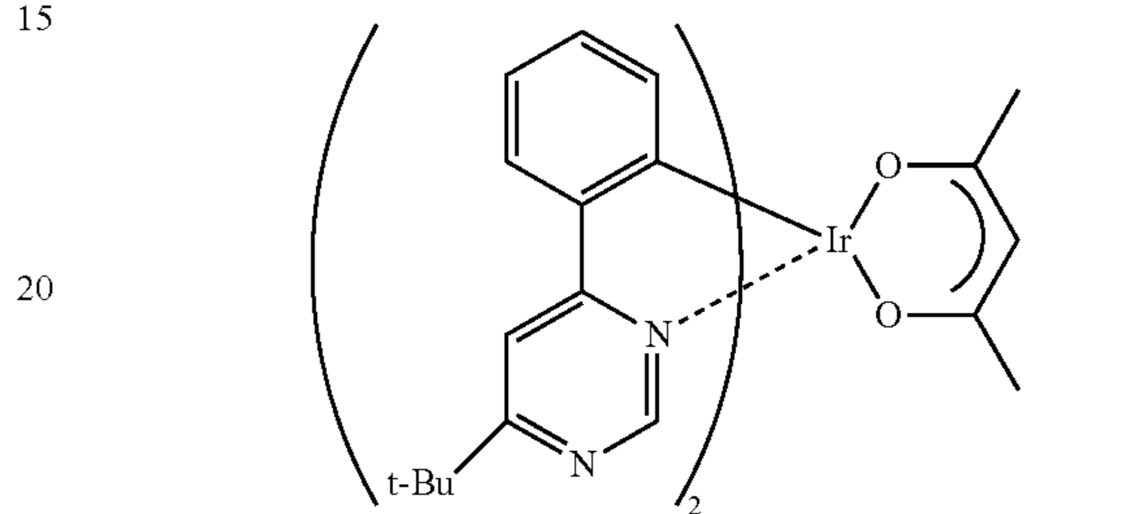
Ir(tBuppm) 2 (acac)
