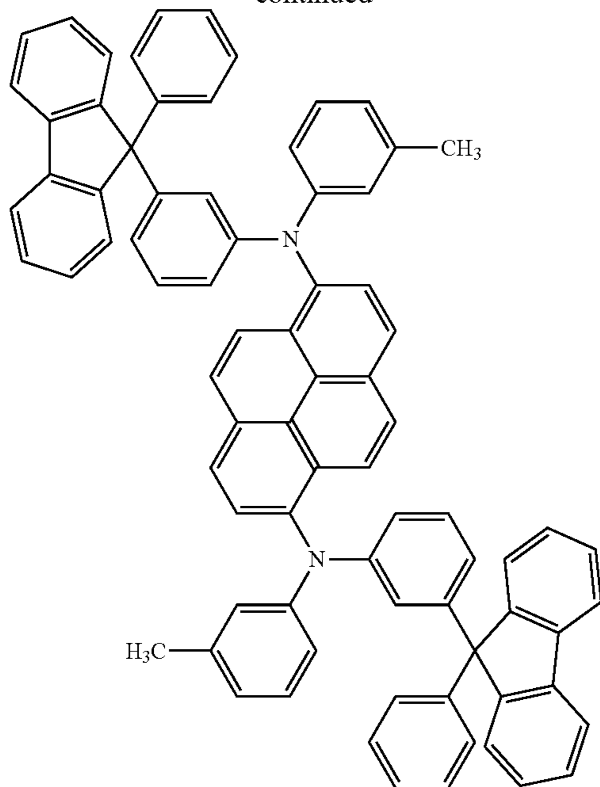
1,6mMemFLPAPm
