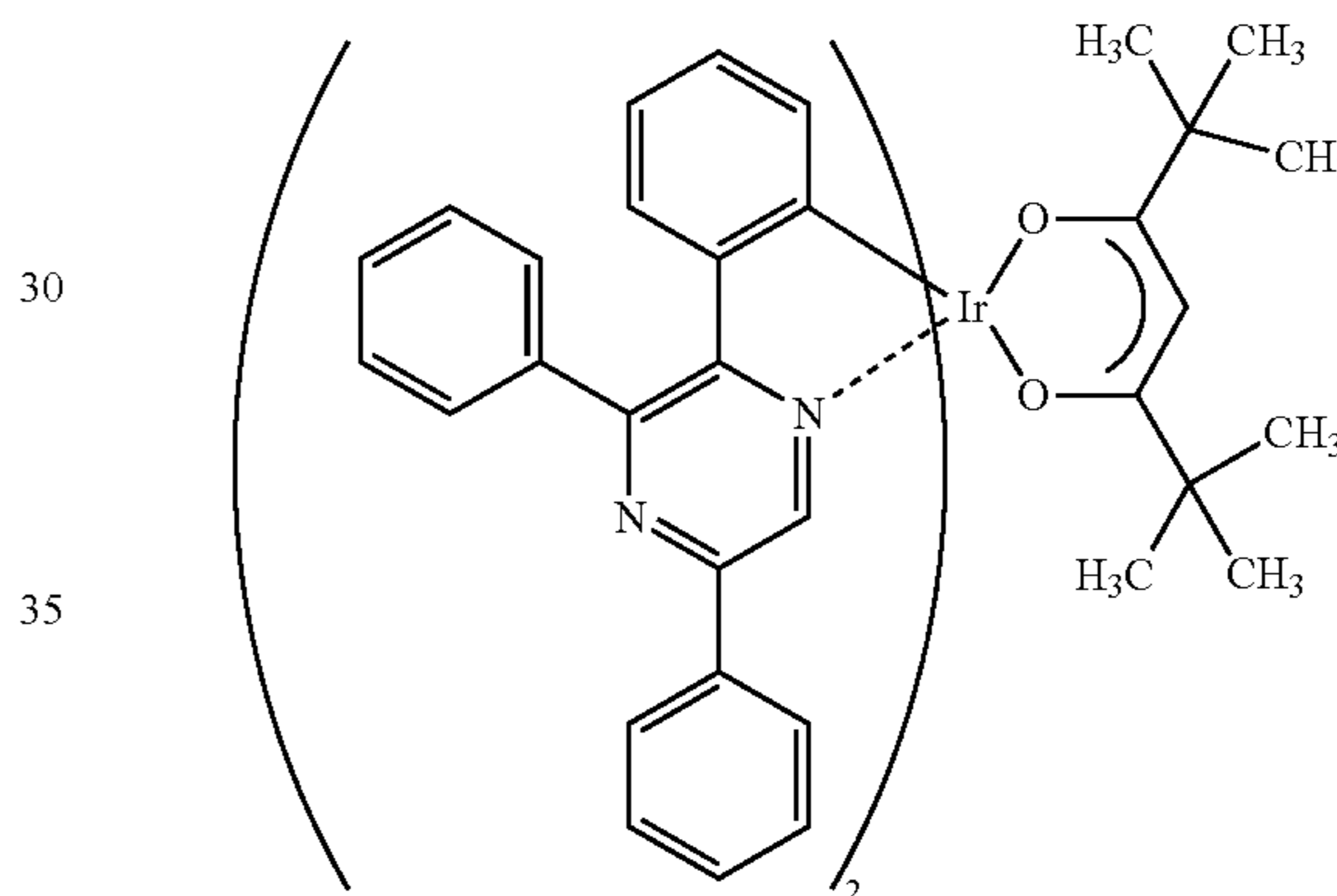
Ir(tppr) 2 (dpm)
