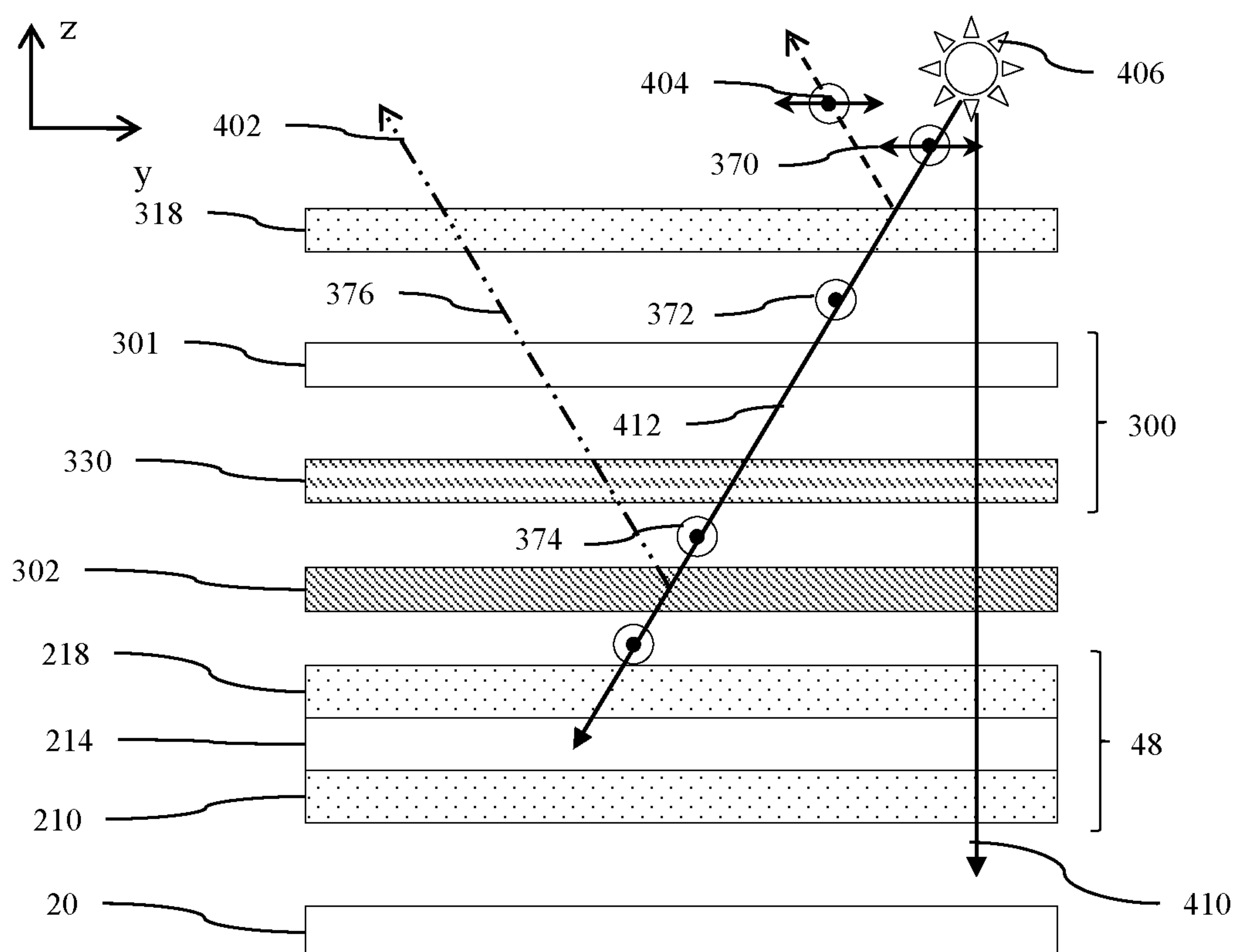
FIG. 17A Reflectivity
