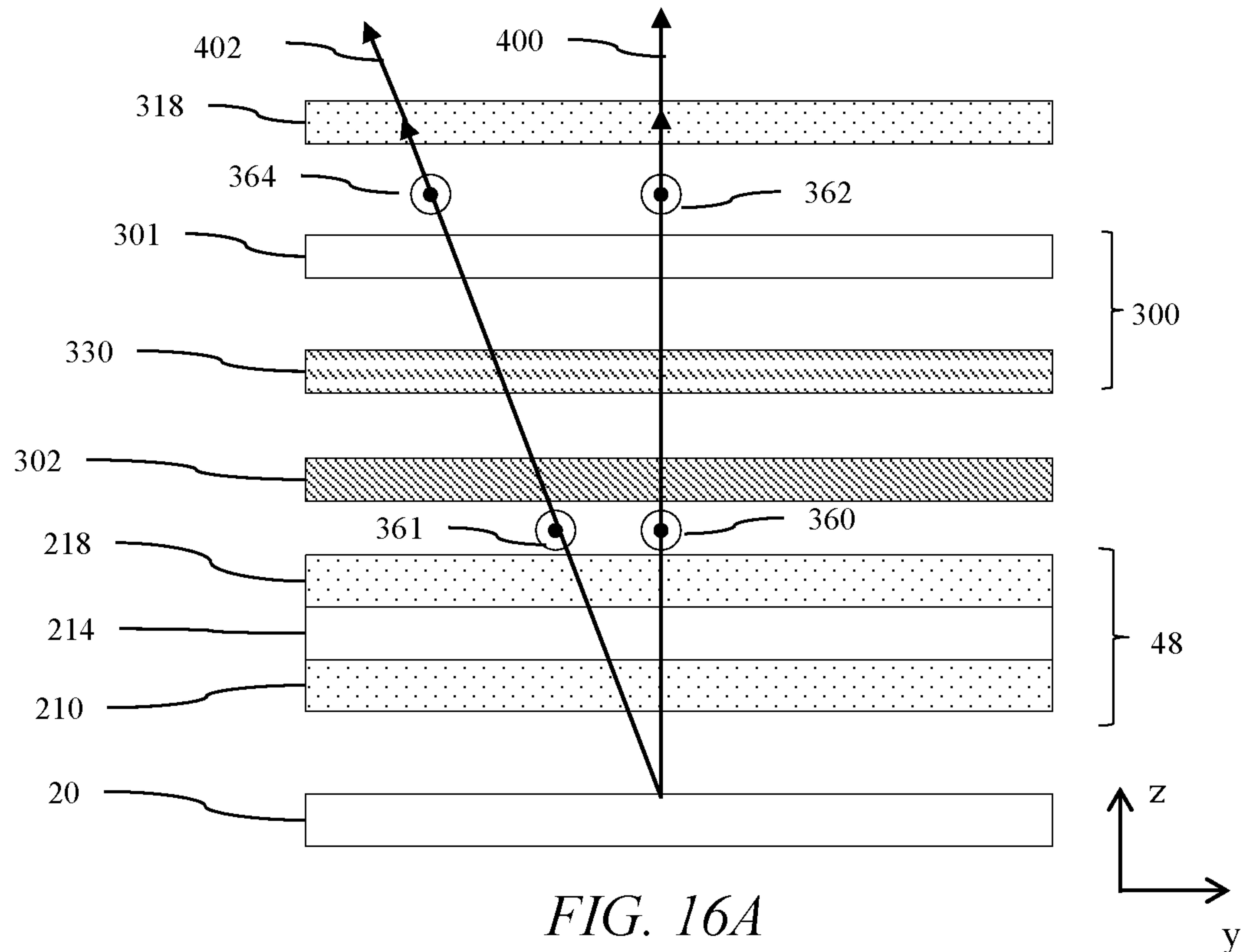
Transmission
