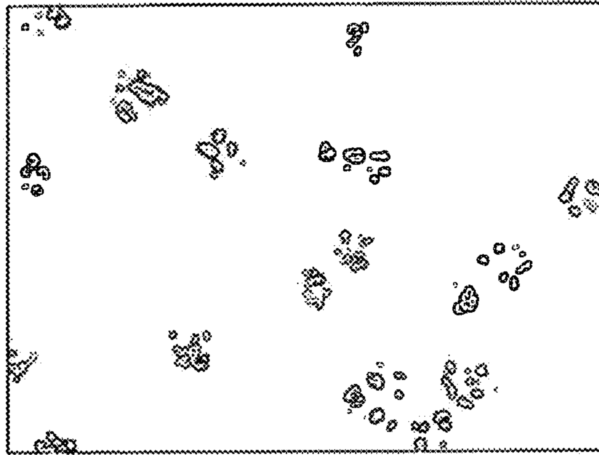
HeLa (30-50 copies)
