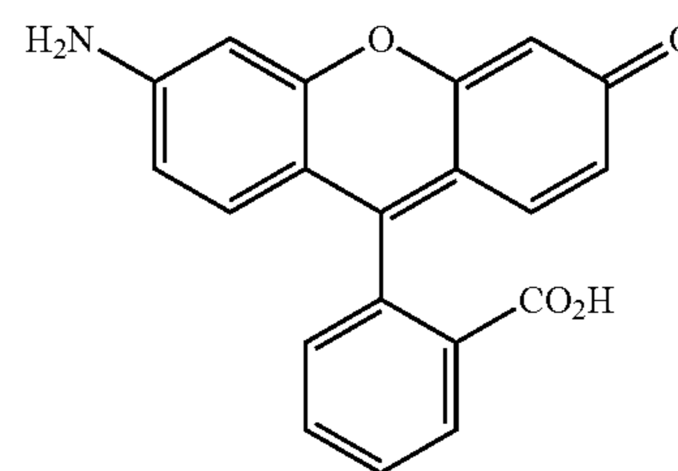
Rhodol
