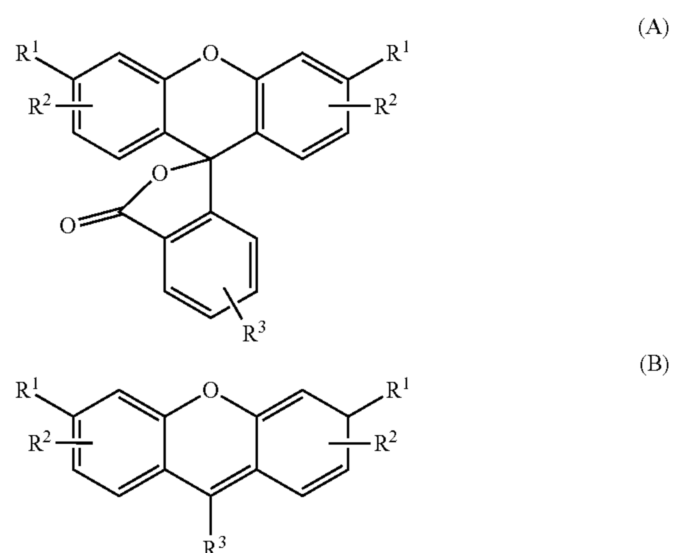
Scheme I
