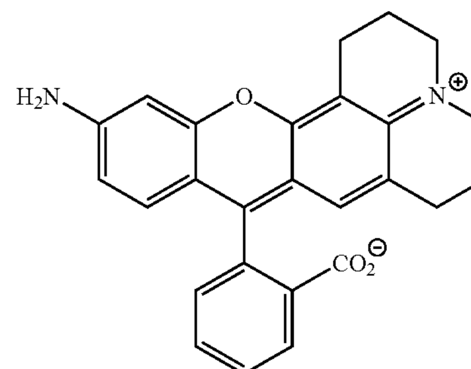
Scheme III
