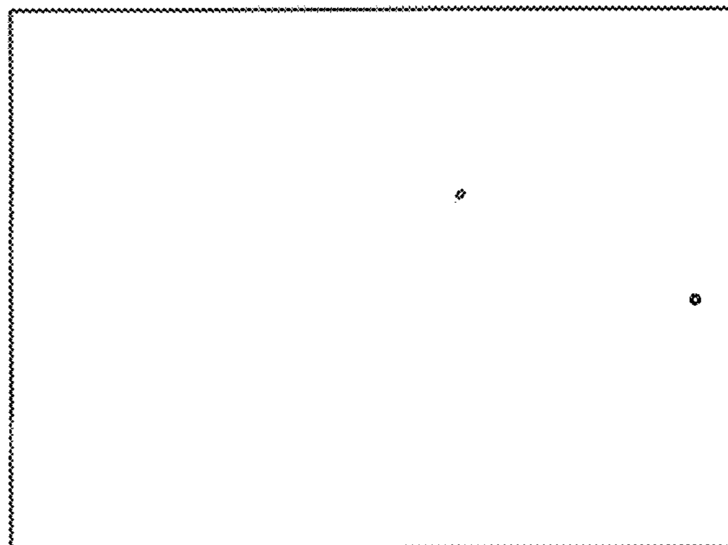
SK-N-SH (0 copies)
