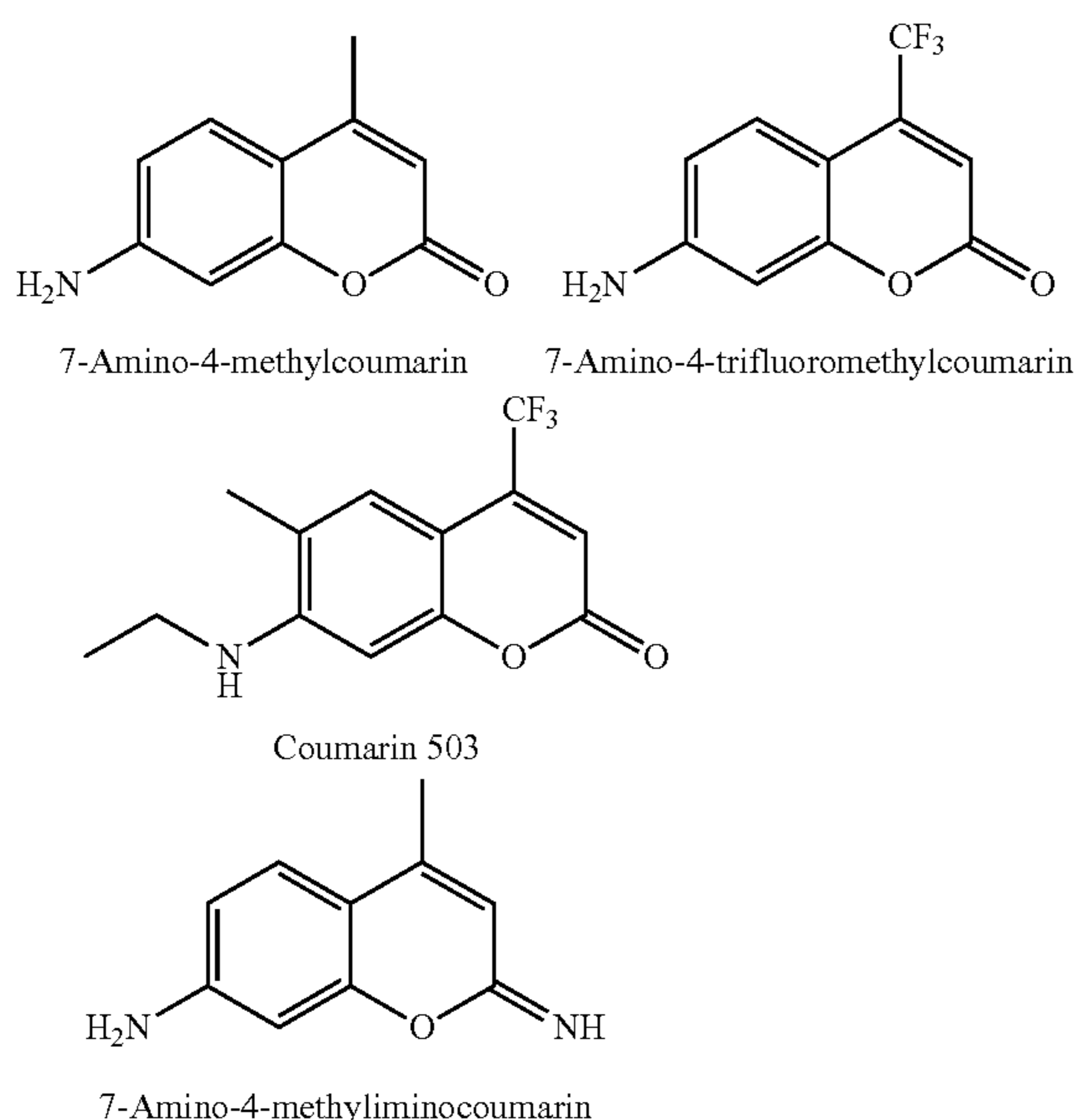
Scheme V
