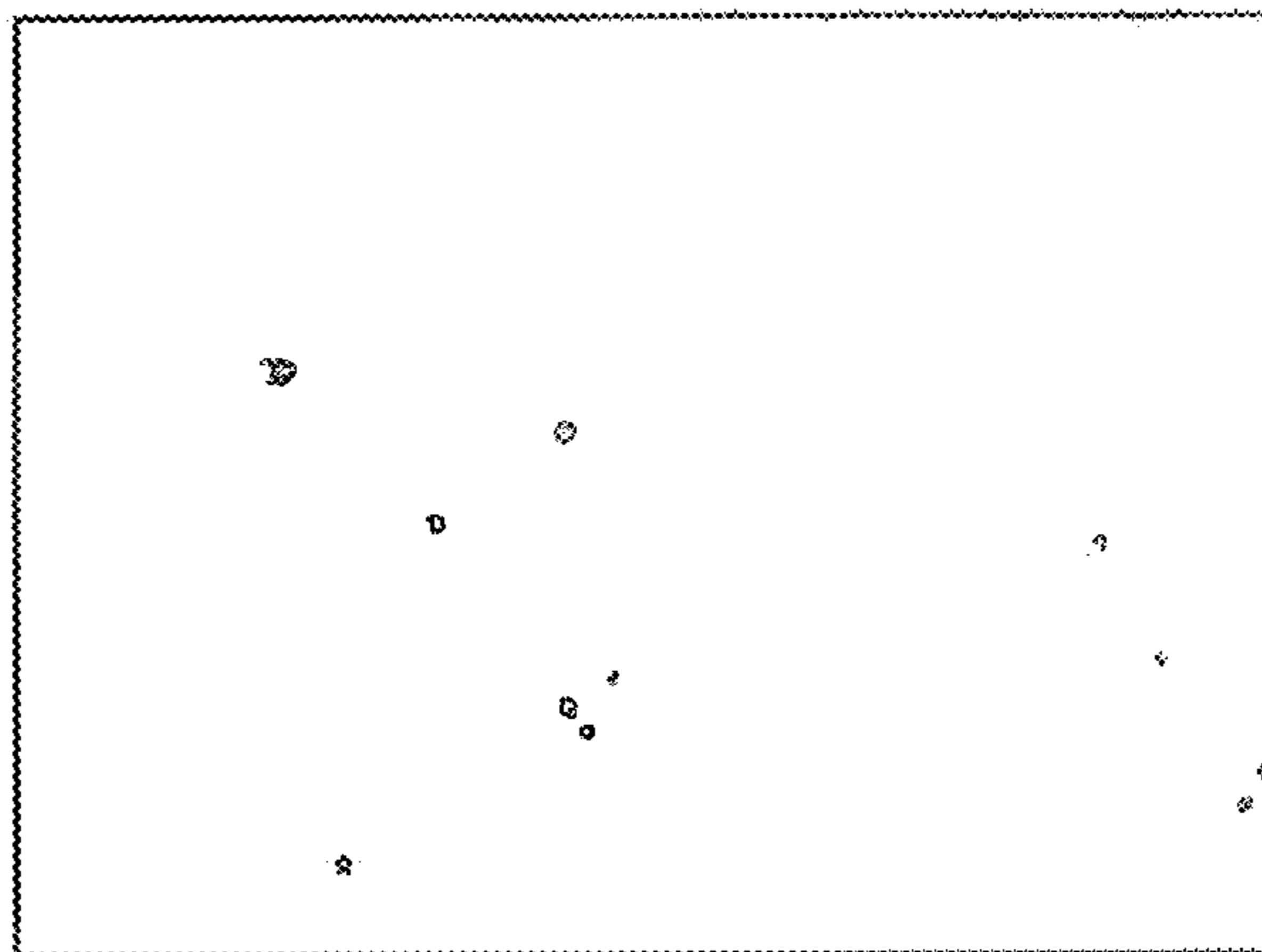
SiHa (1-5 copies)
