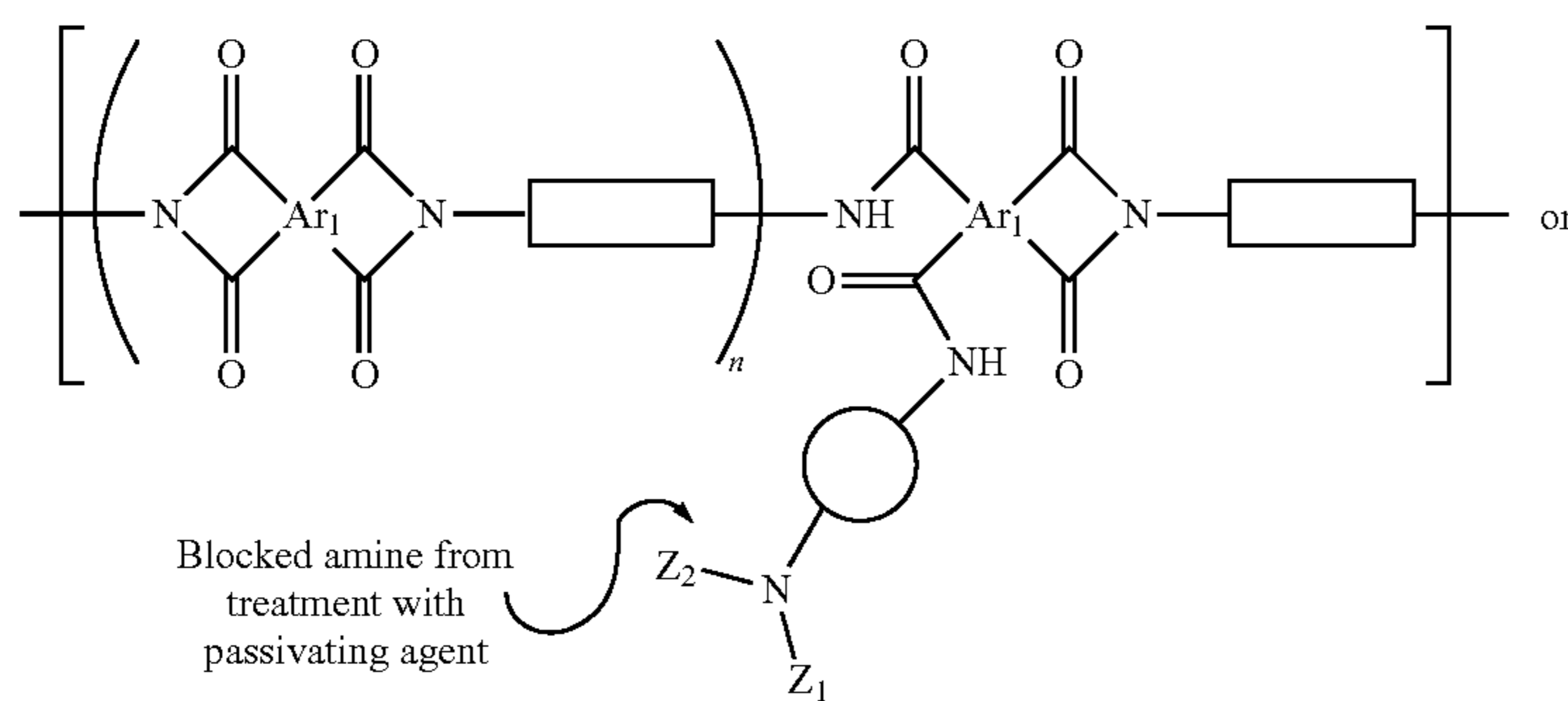
Inventive membrane
