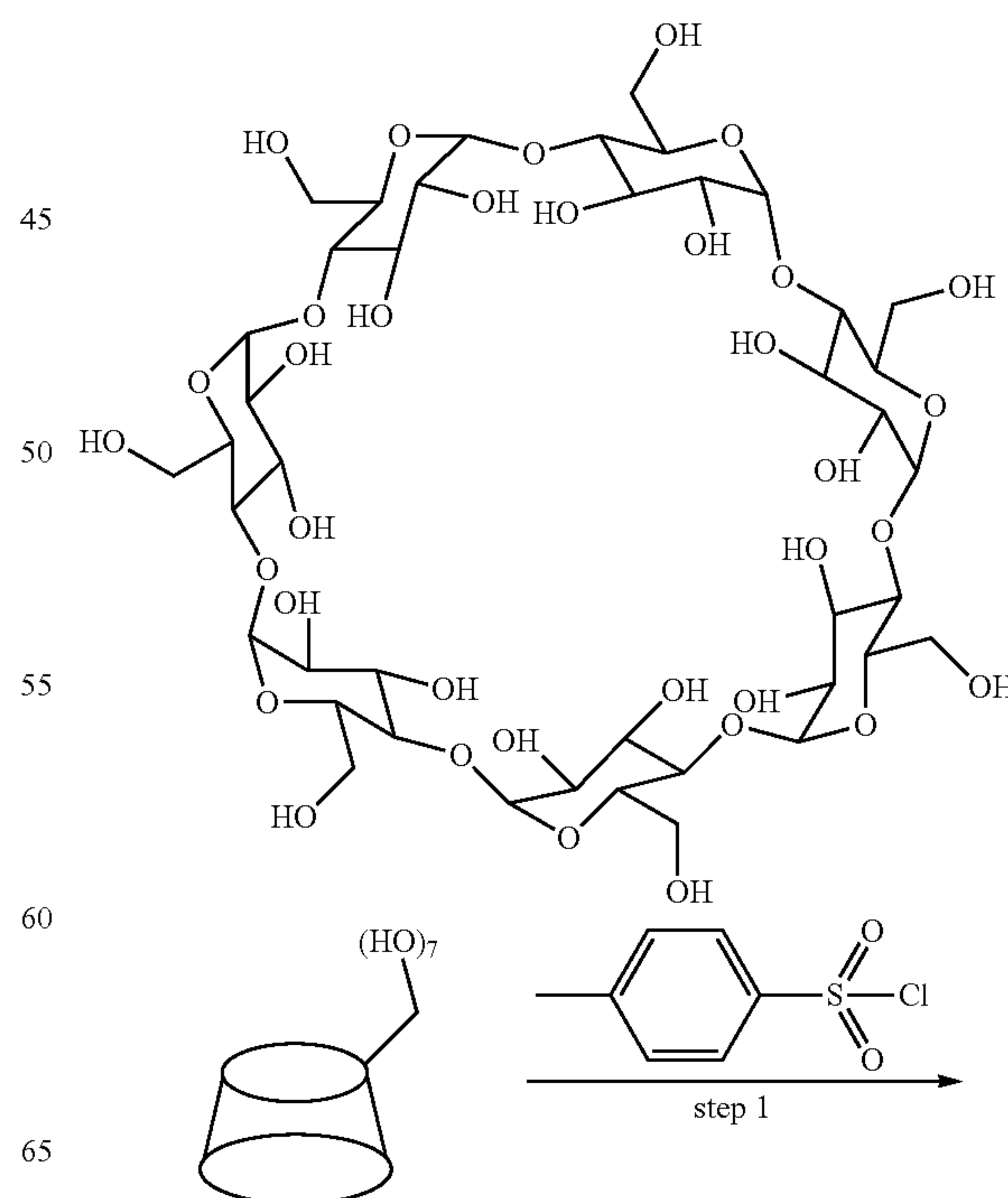
Scheme S1. Synthesis route of secondary amine-modified mono-substituted CD derivatives.
