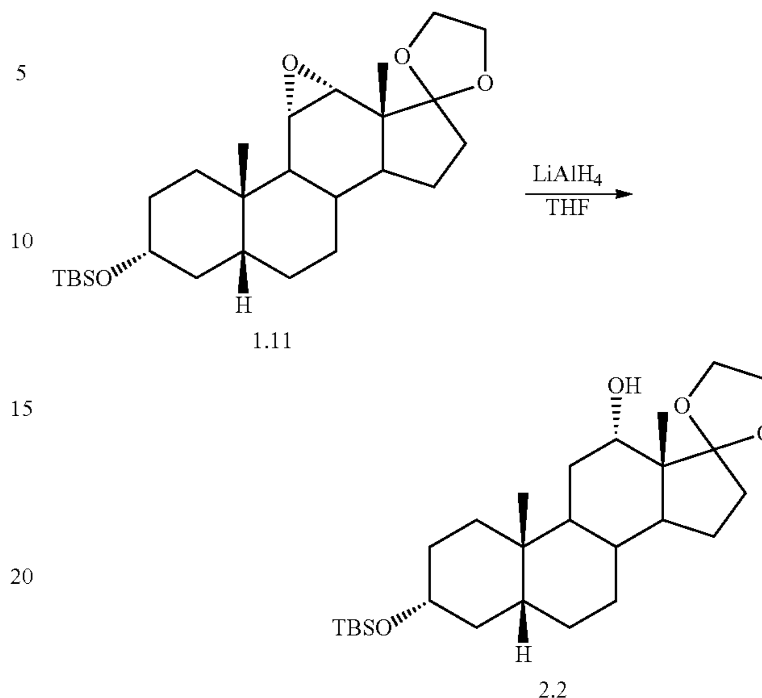
Scheme 3. Stereoselective Reduction of C 11 -C 12 epoxide.
