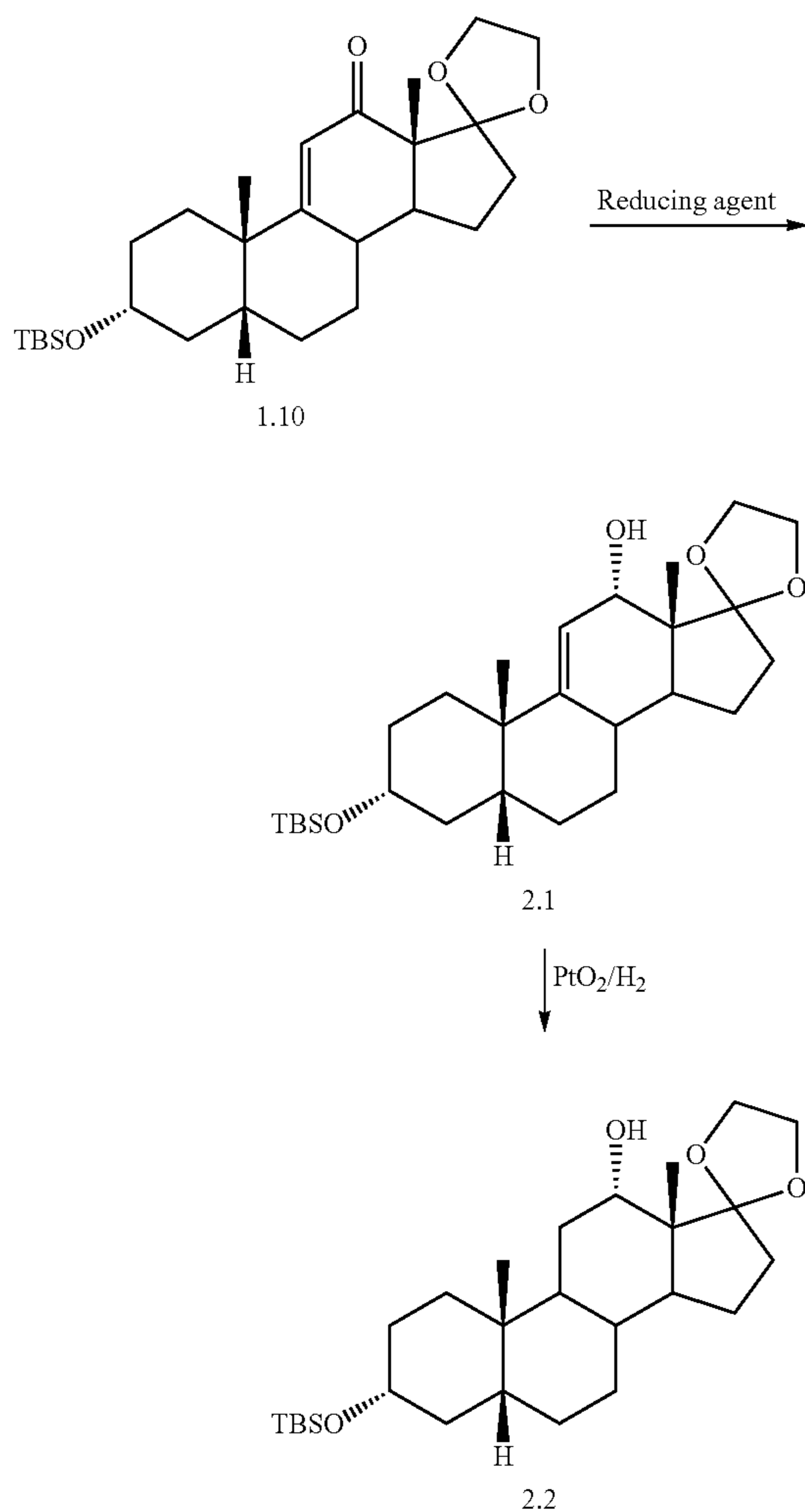
Scheme 2. Introduction of C 12 a hydroxyl group using the allylic oxidation route
