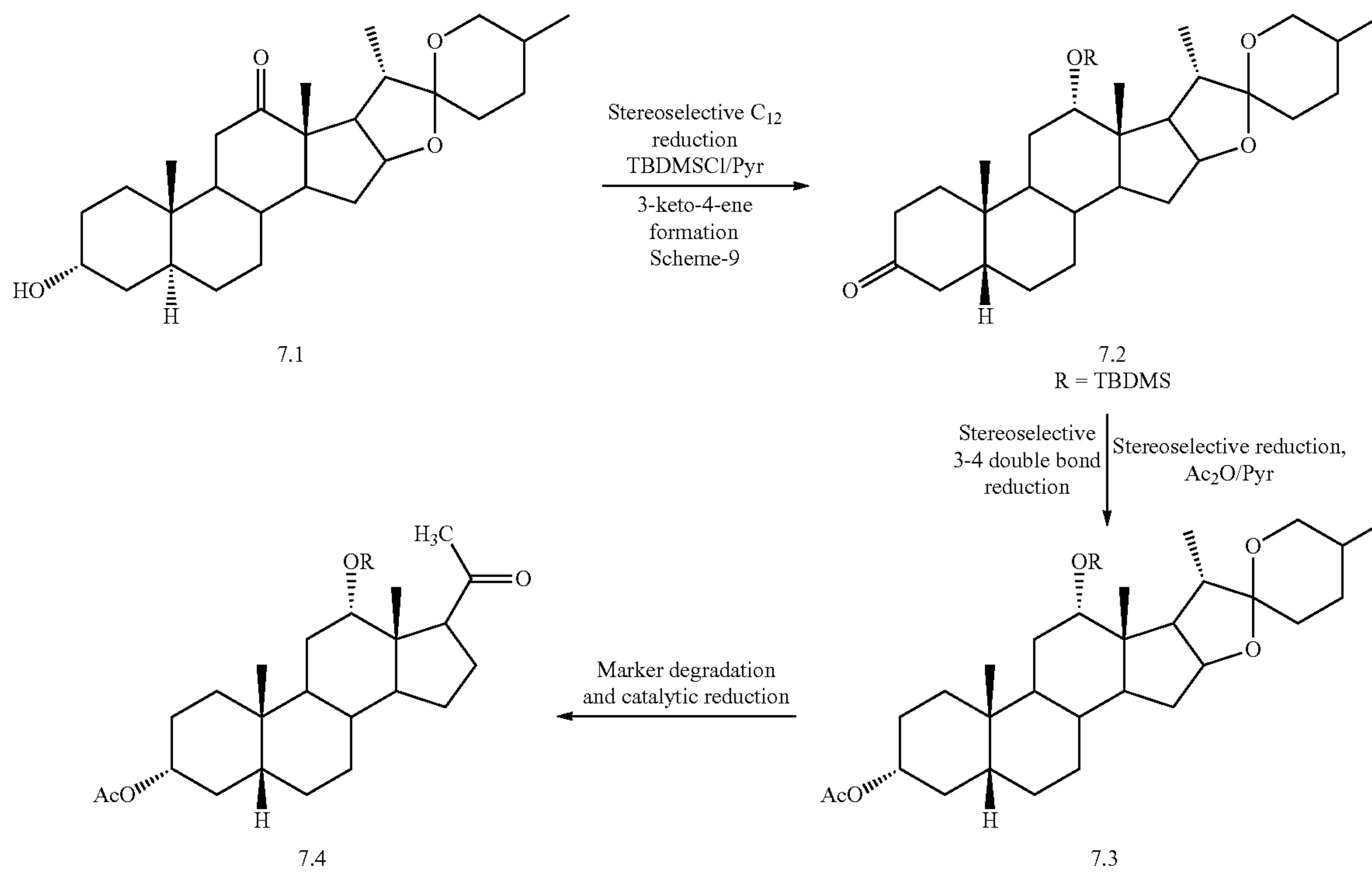
Scheme 8. Side-chain introduction
