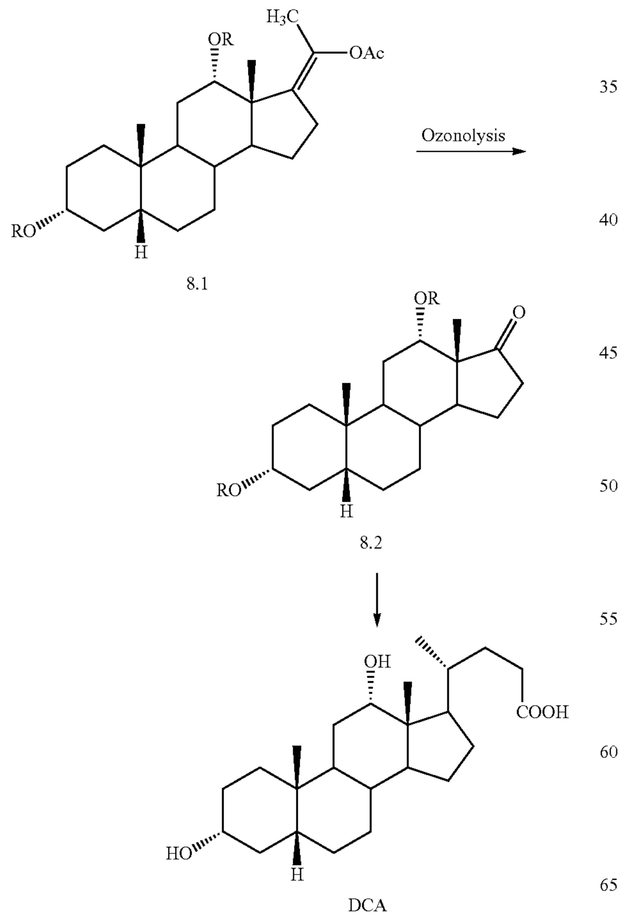
Scheme 8. Side-chain introduction
