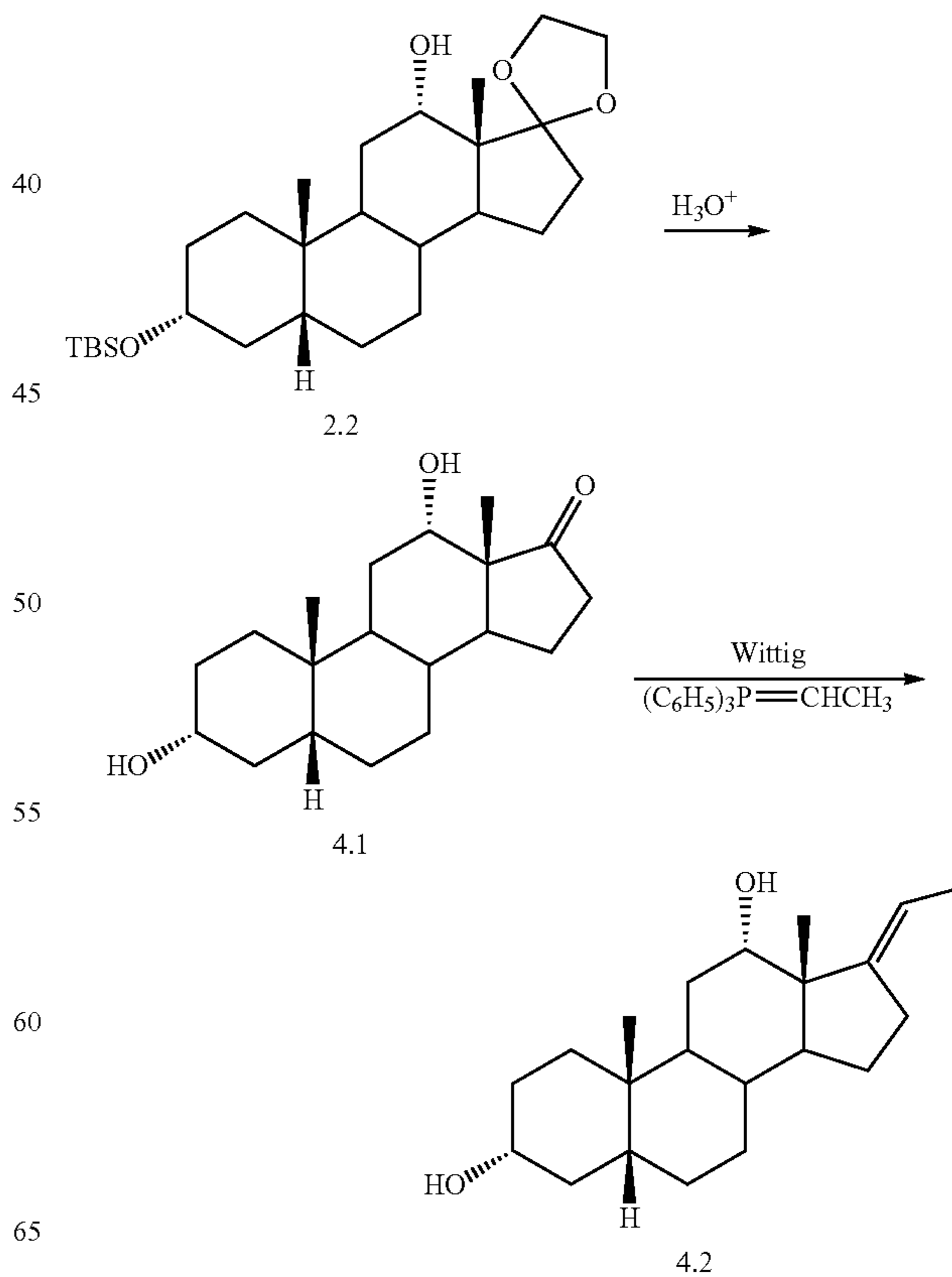
Scheme 4. Deprotection and Wittig Reaction
