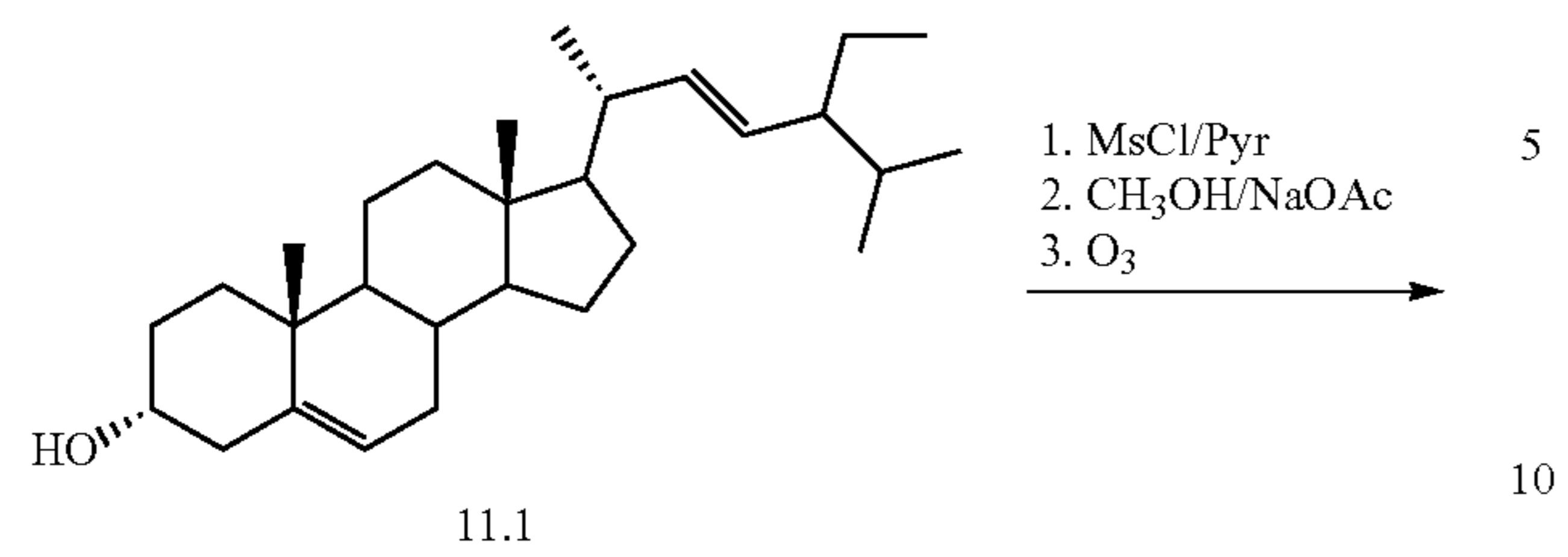
Scheme 11. Ozonolysis of i-steroid and side chain reduction
