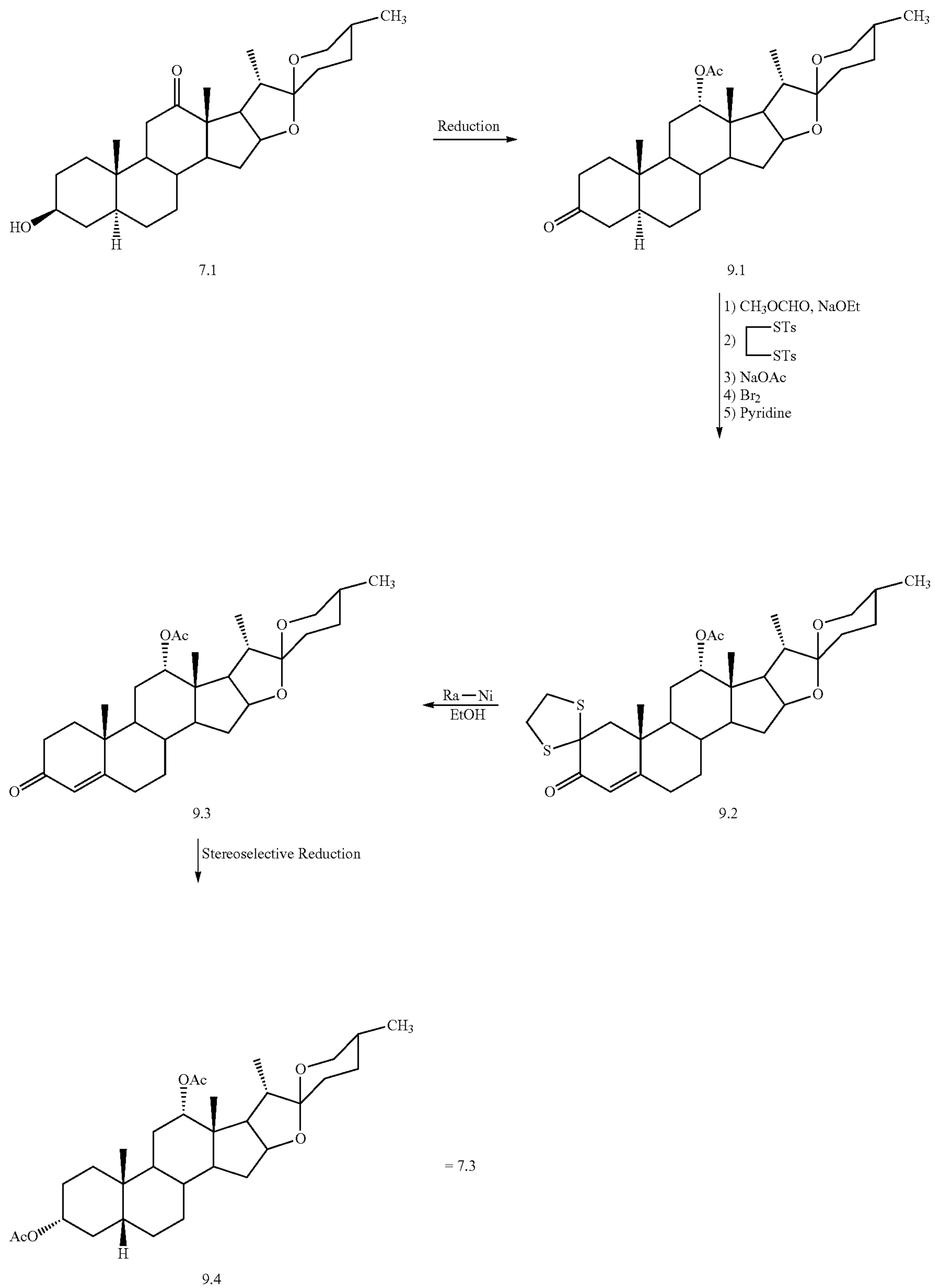
Scheme 9. Dithioethane route to 3-keto-4-ene
