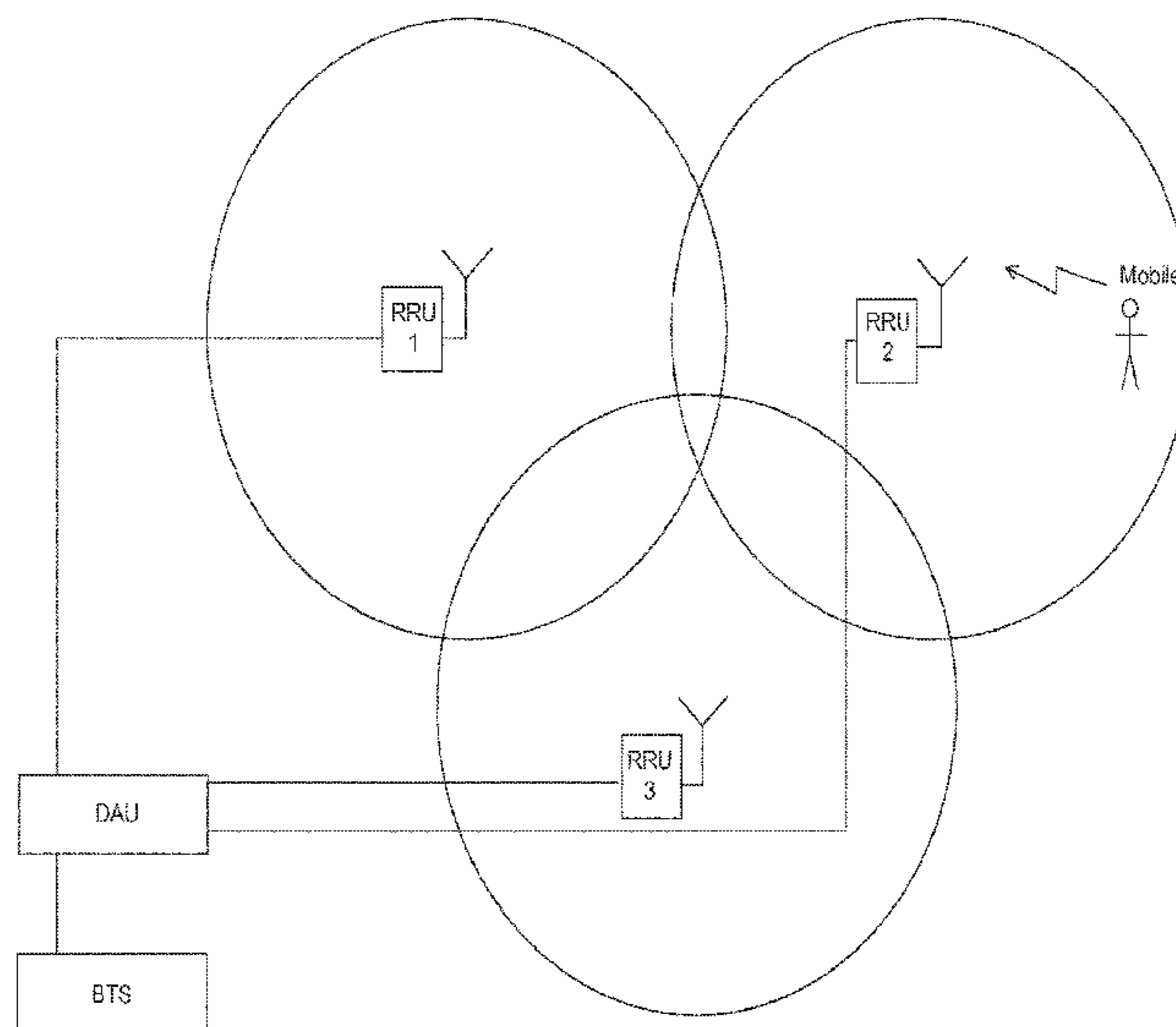
Indoor Localization System of GSM and LTE
