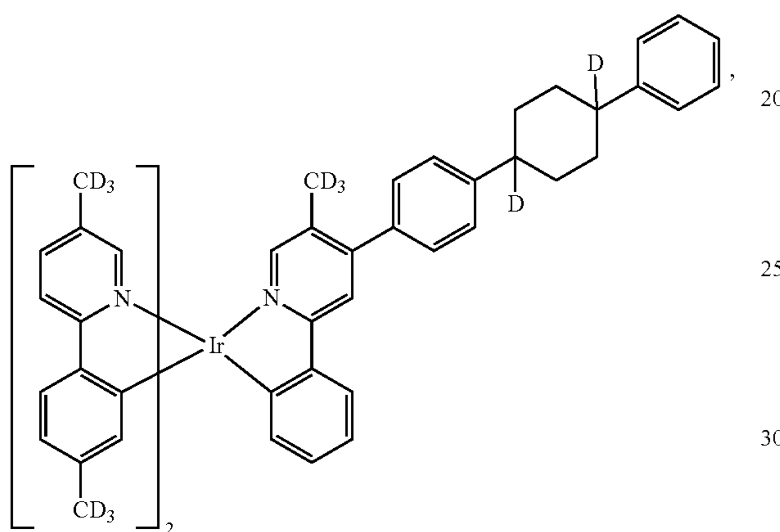
Compound 60
