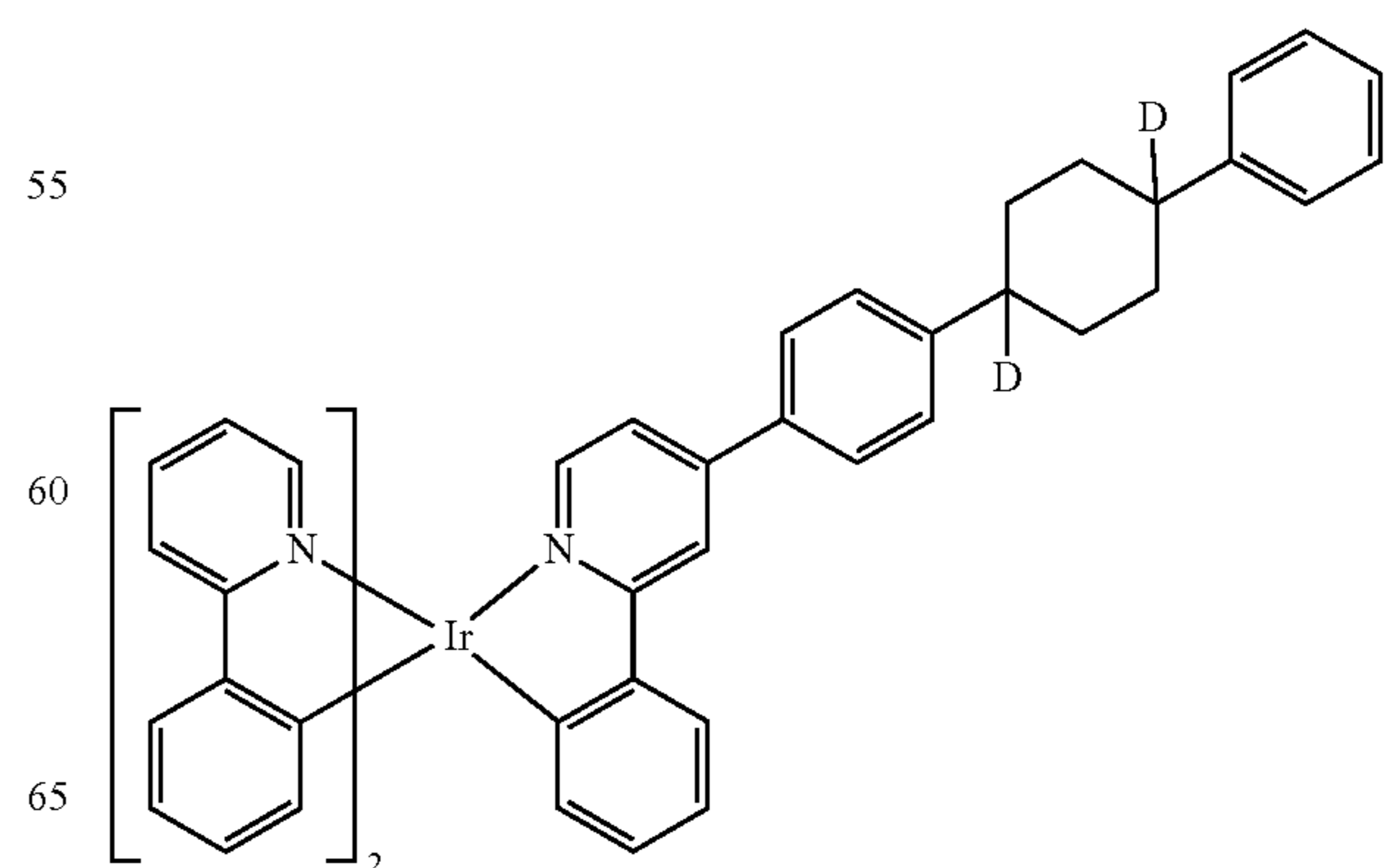
Compound 49
