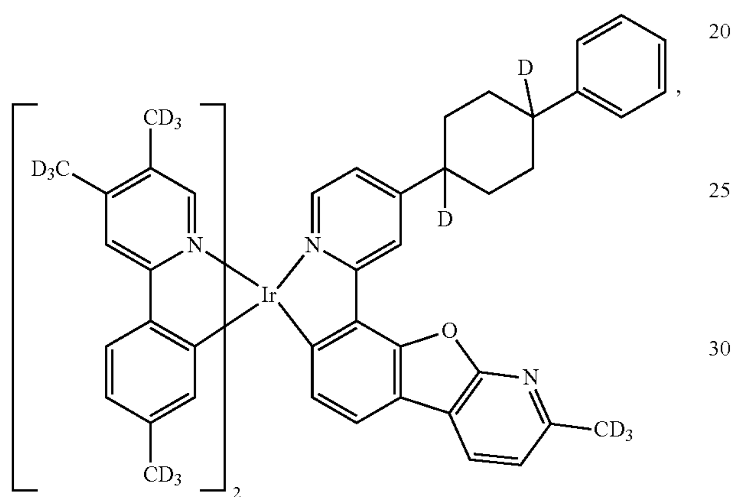
Compound 37
