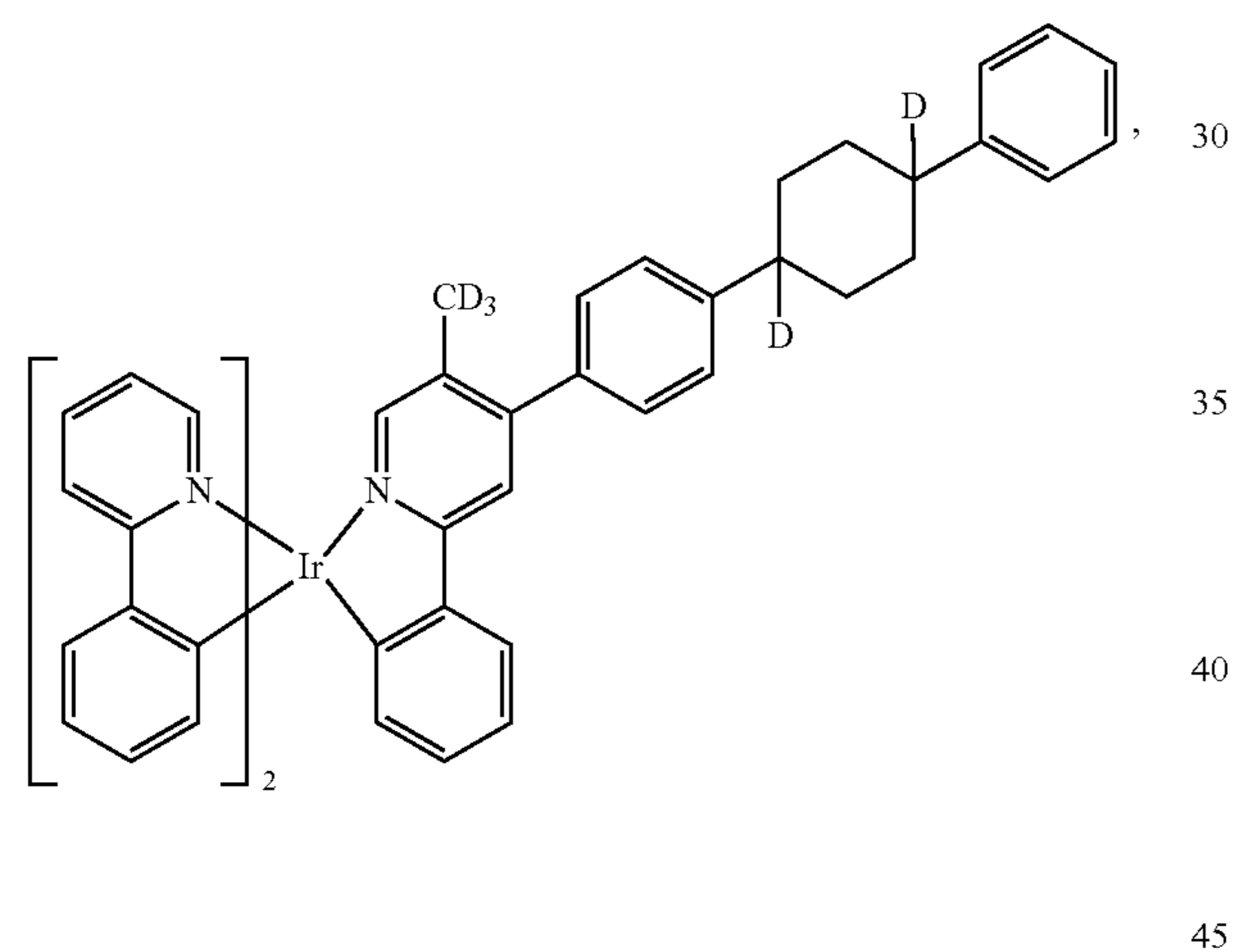
Compound 55
