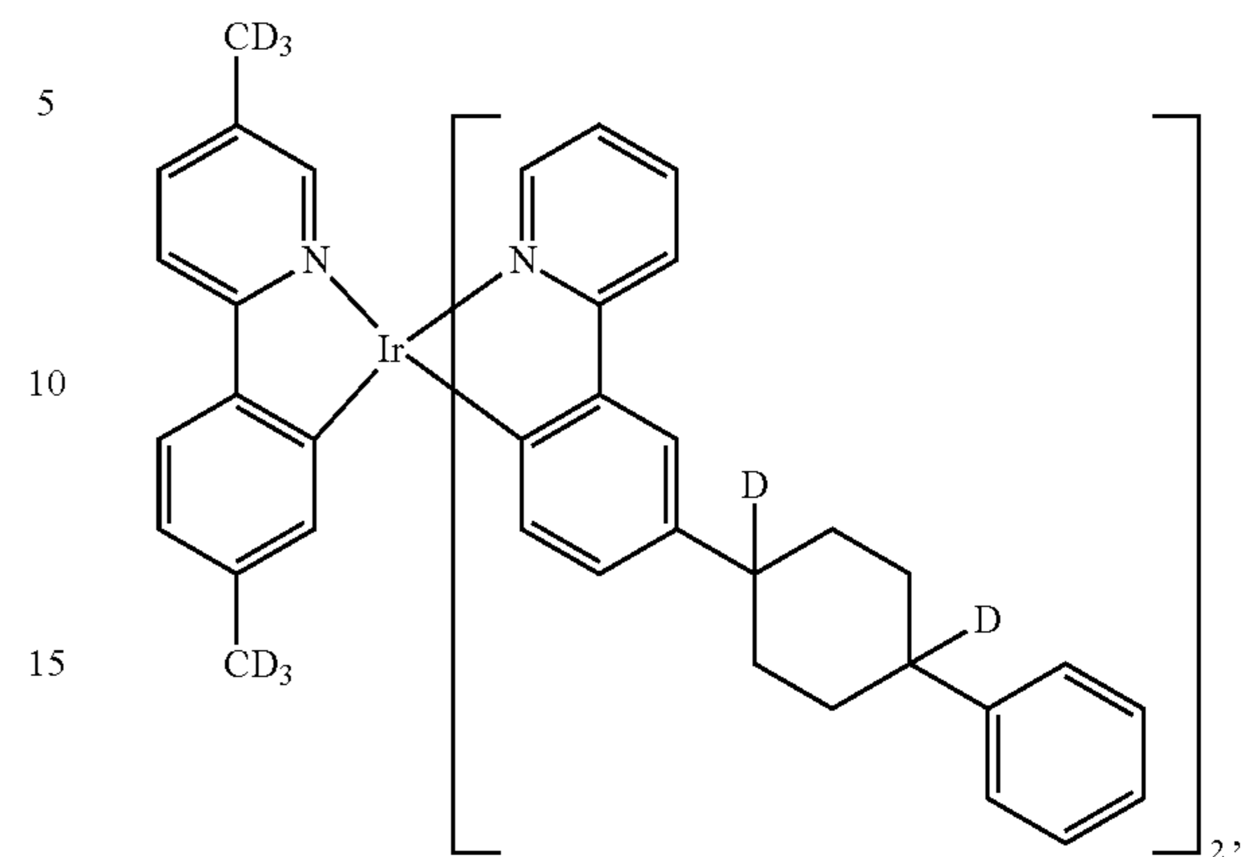
Compound 77
