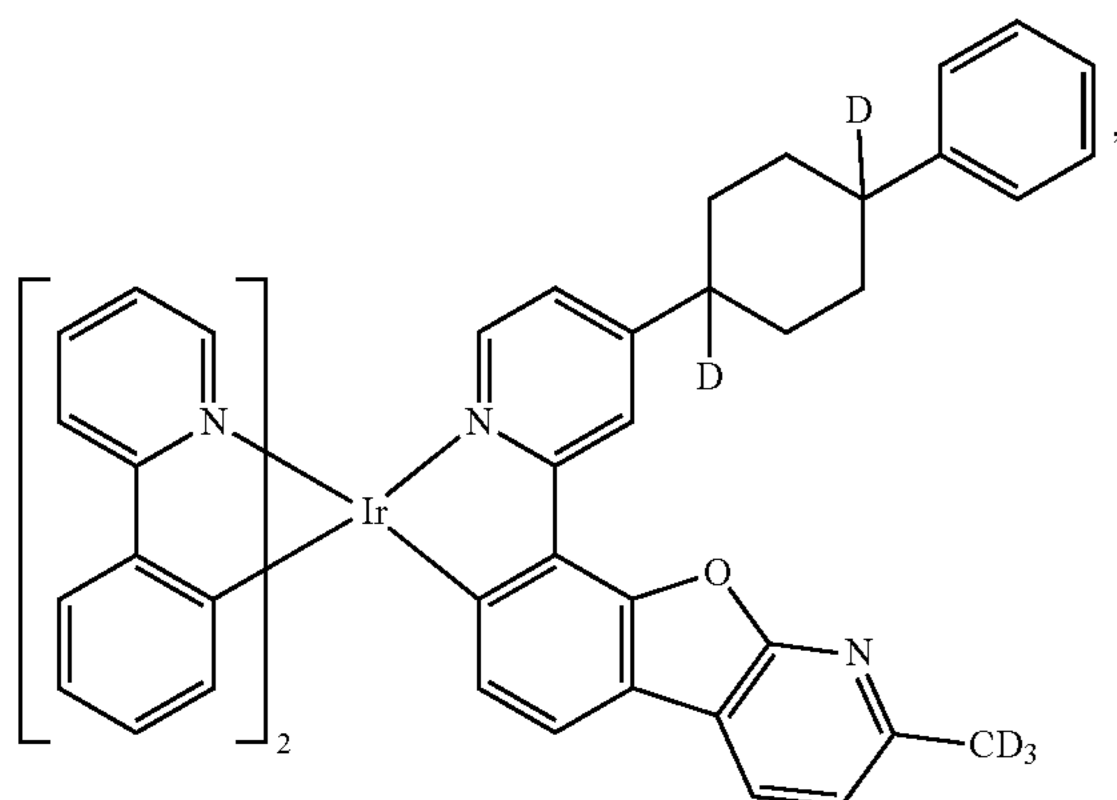
Compound 31
