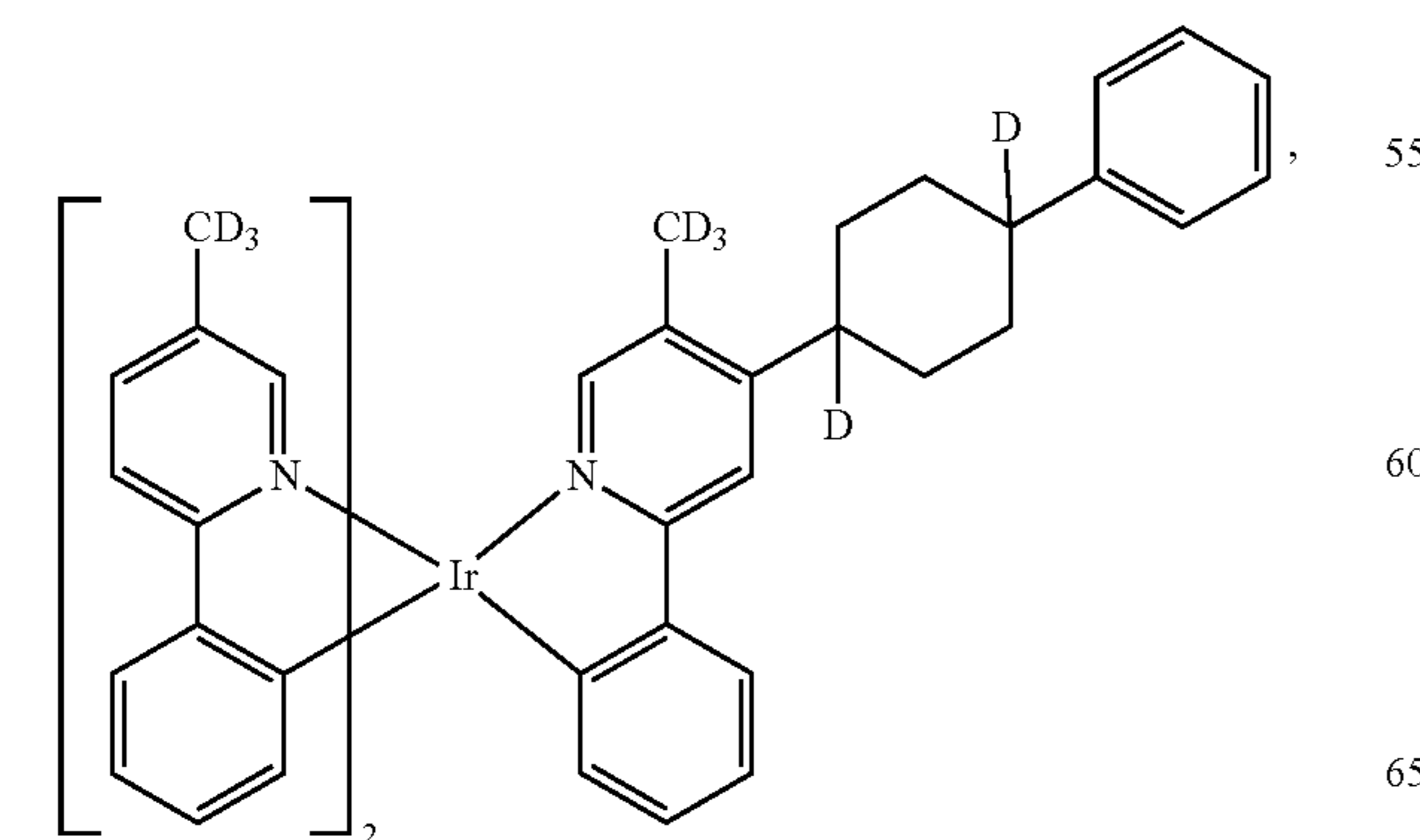
Compound 38
