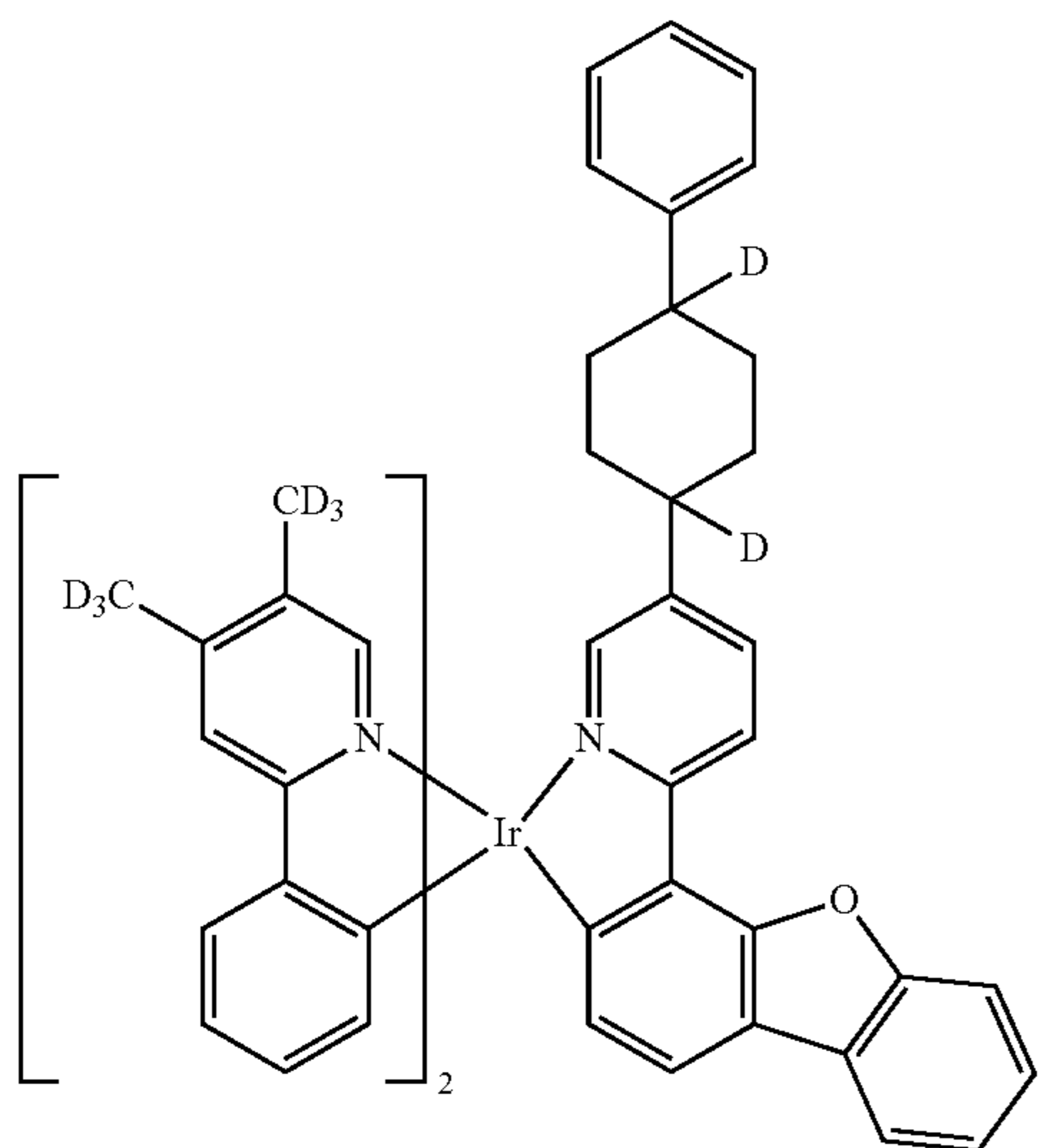
Compound 17
