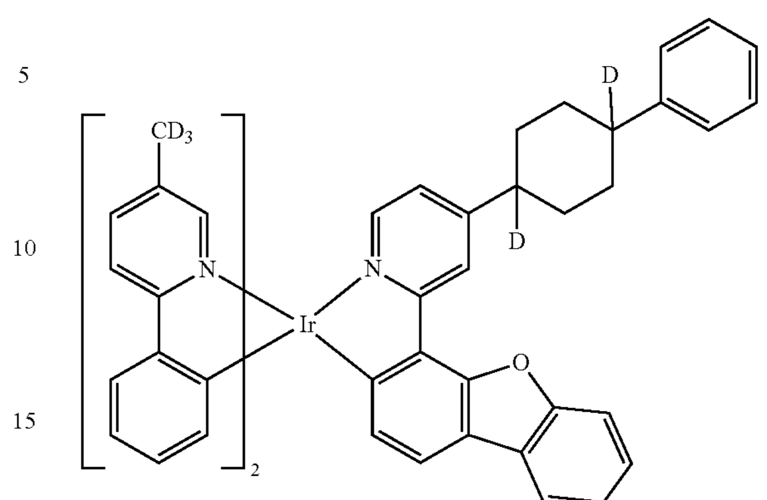
Compound 20
