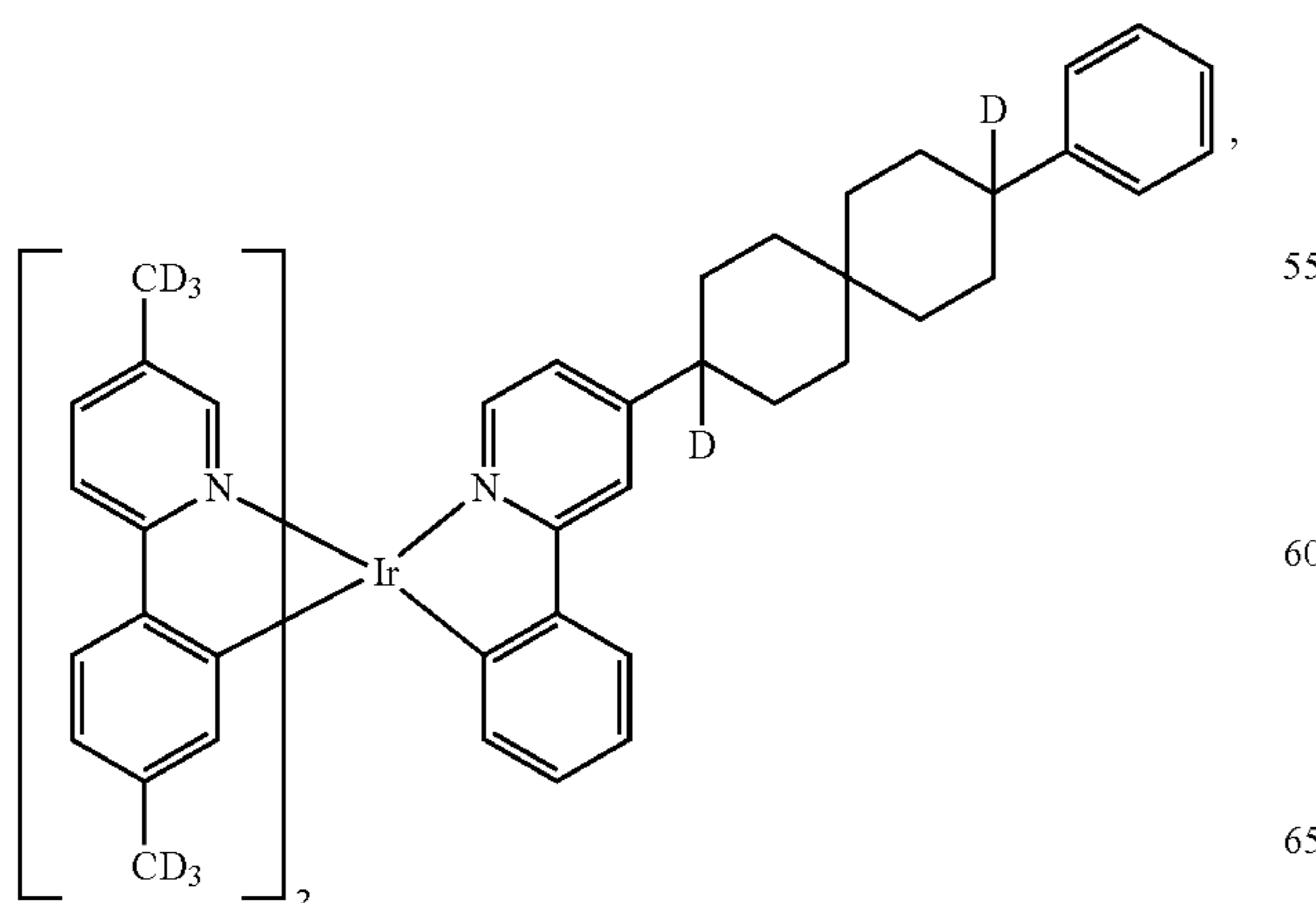
Compound 61
