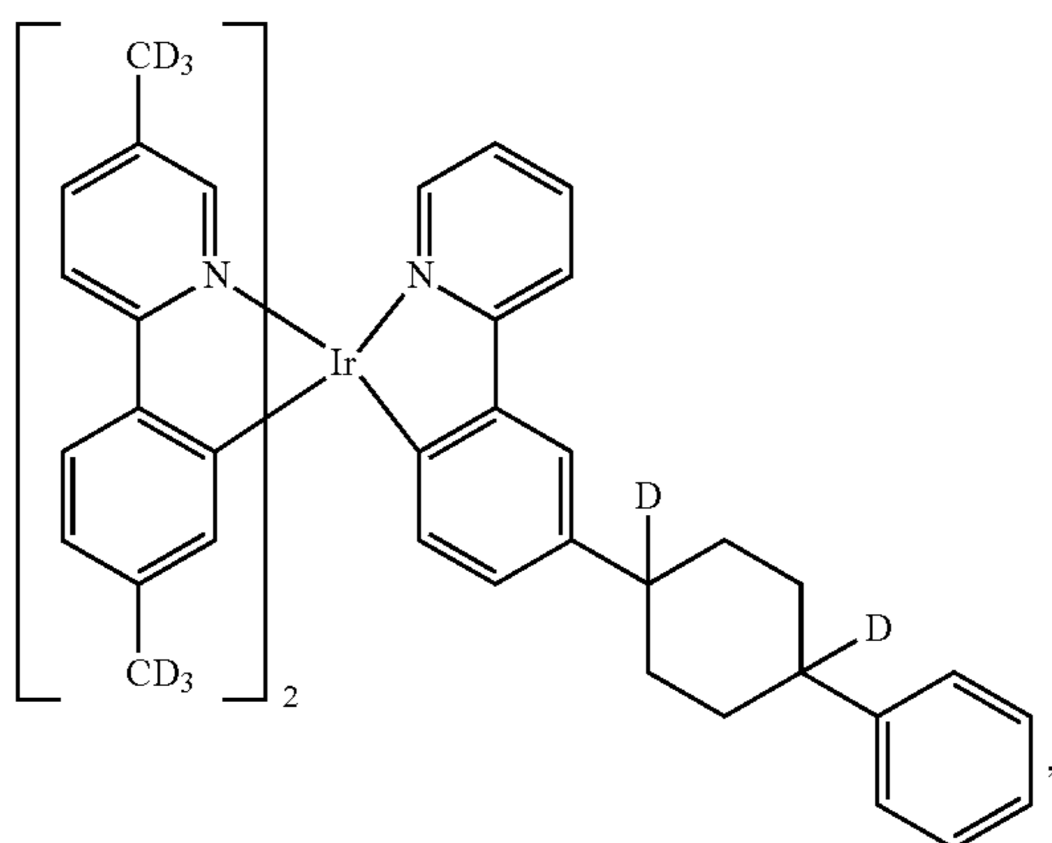
Compound 74
