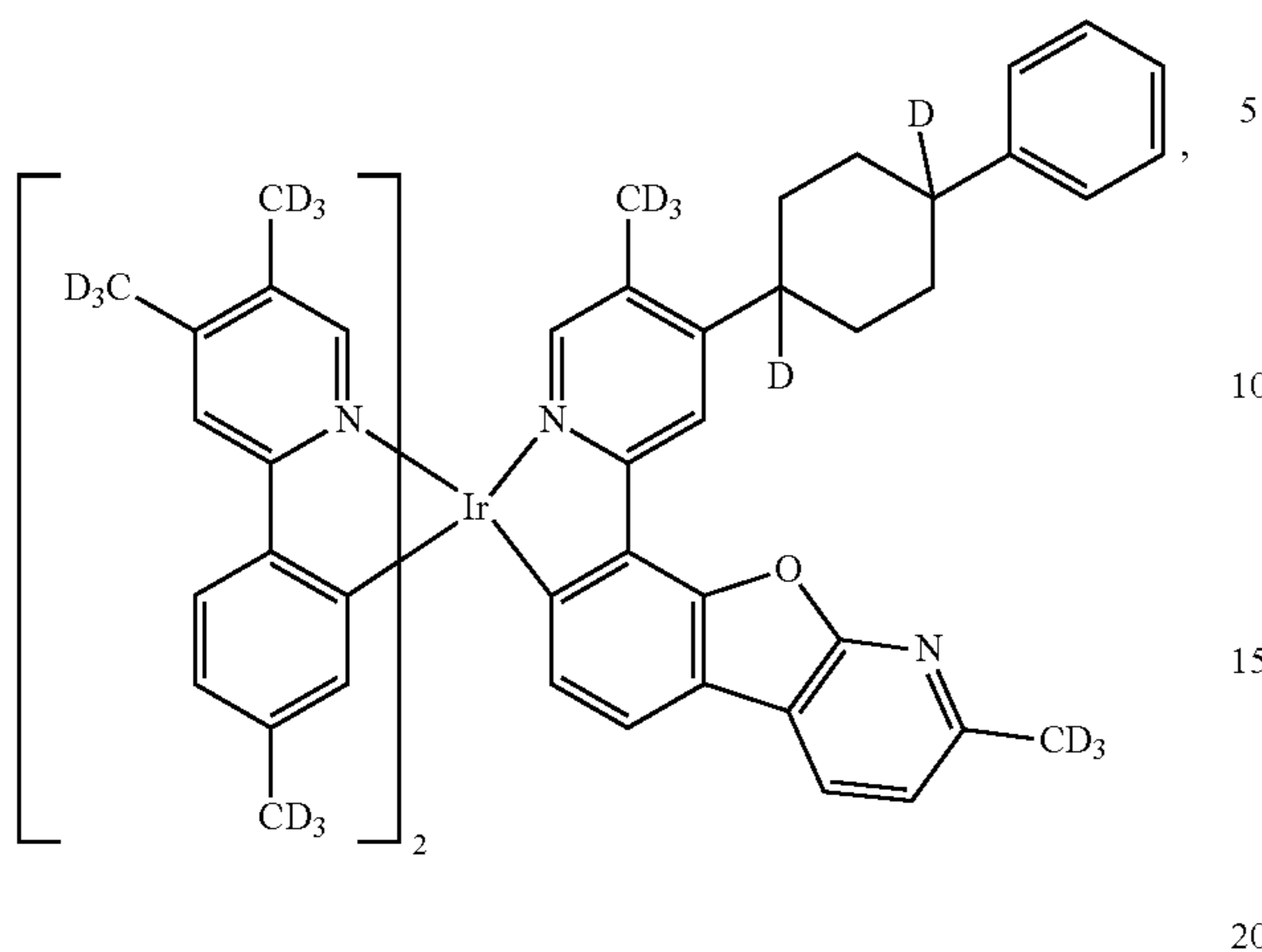
Compound 48
