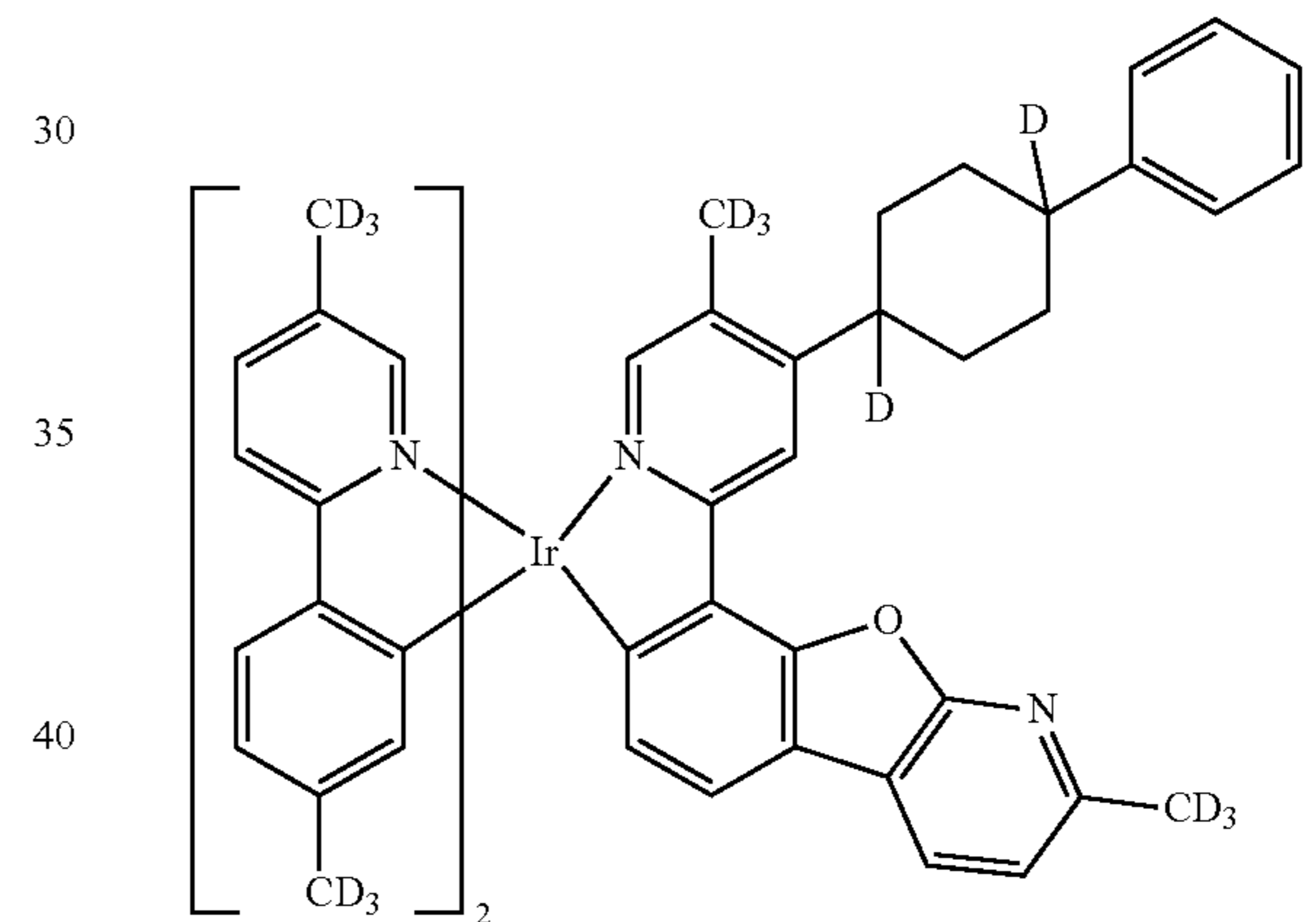
Compound 46
