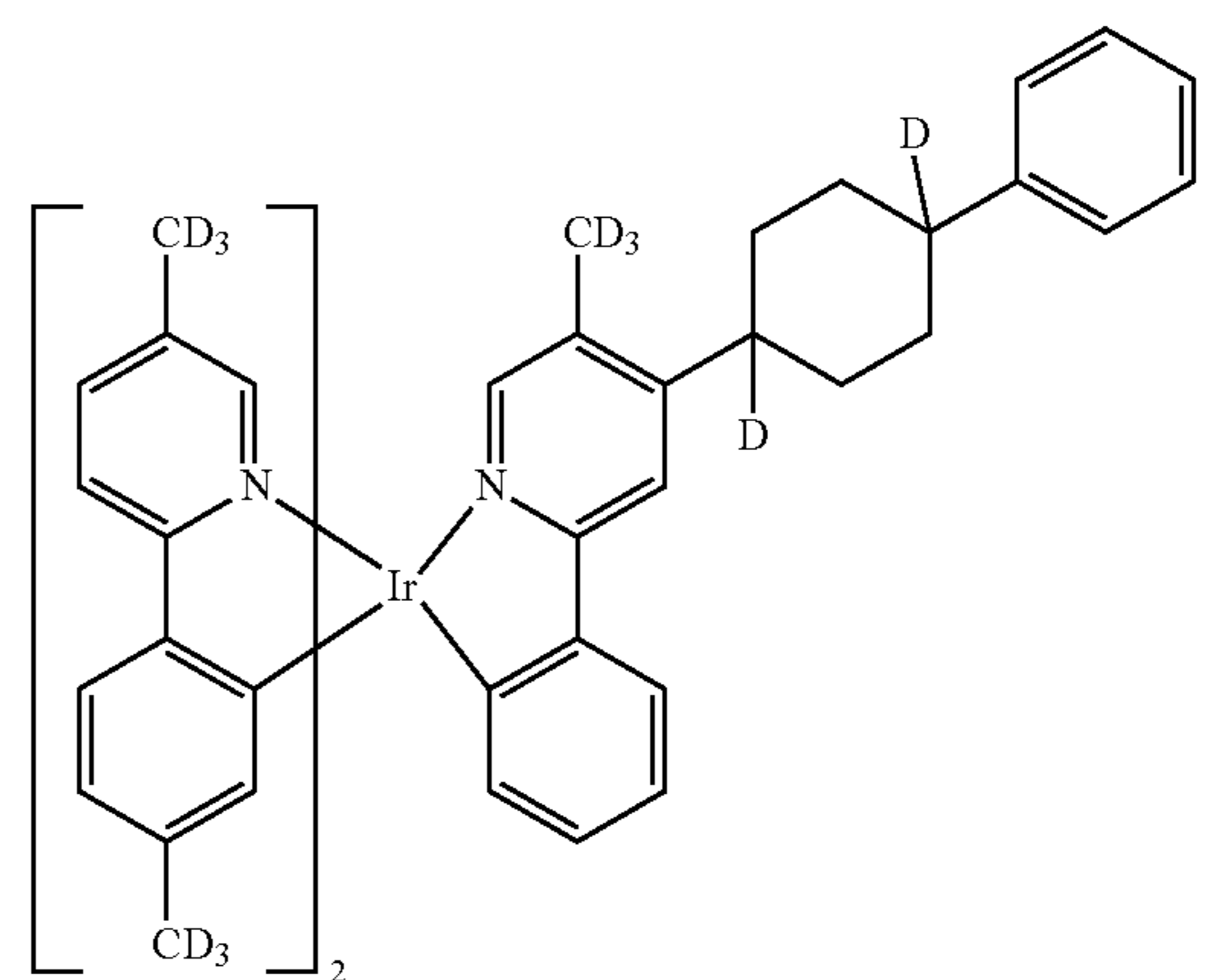
Compound 40
