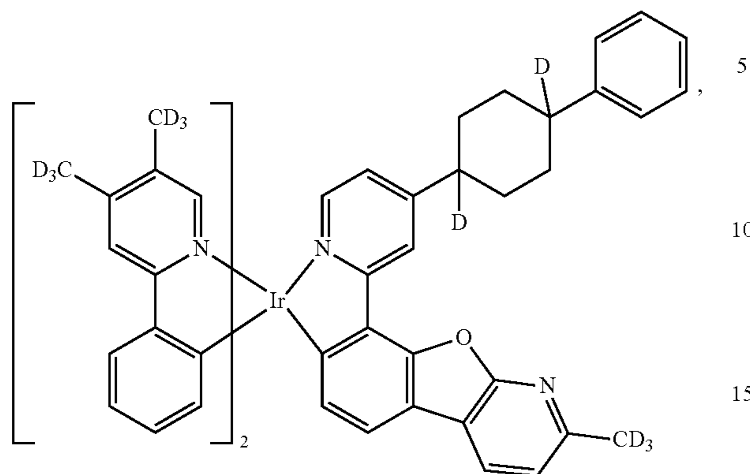
Compound 36
