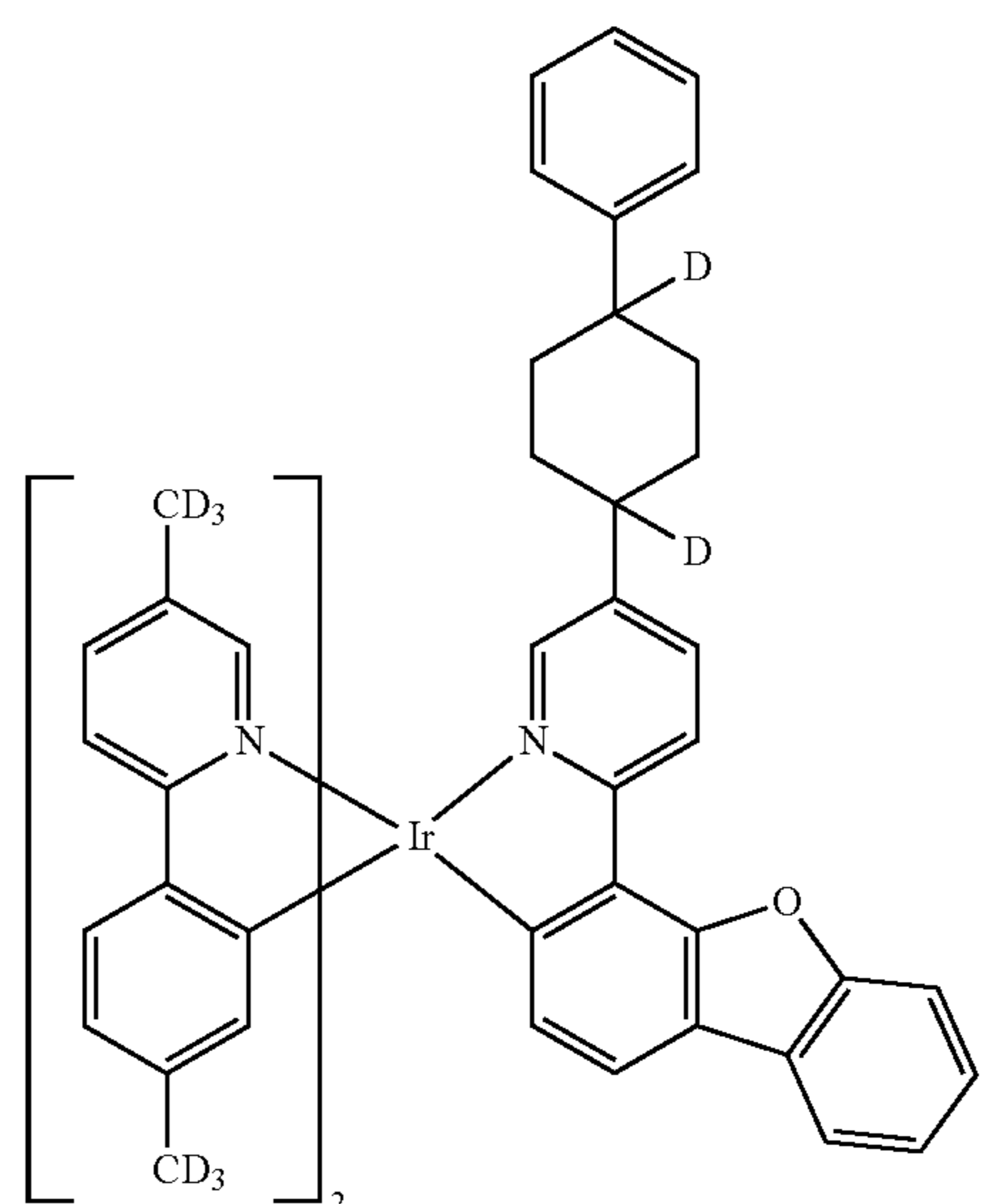
Compound 16
