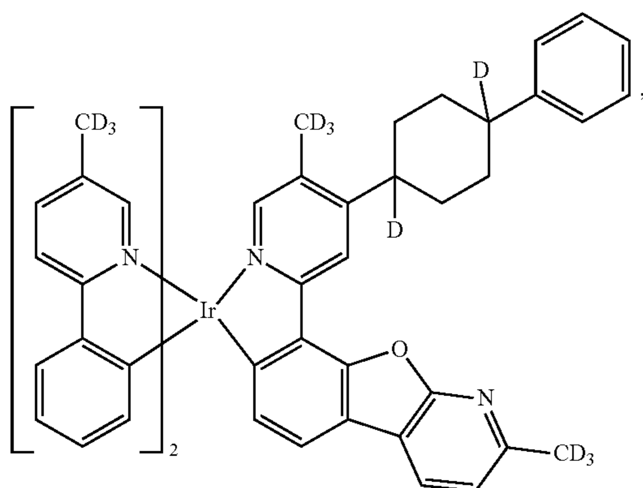
Compound 44
