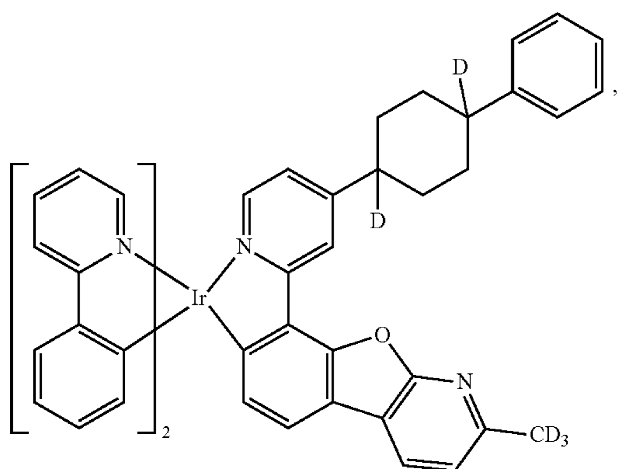
Compound 31
