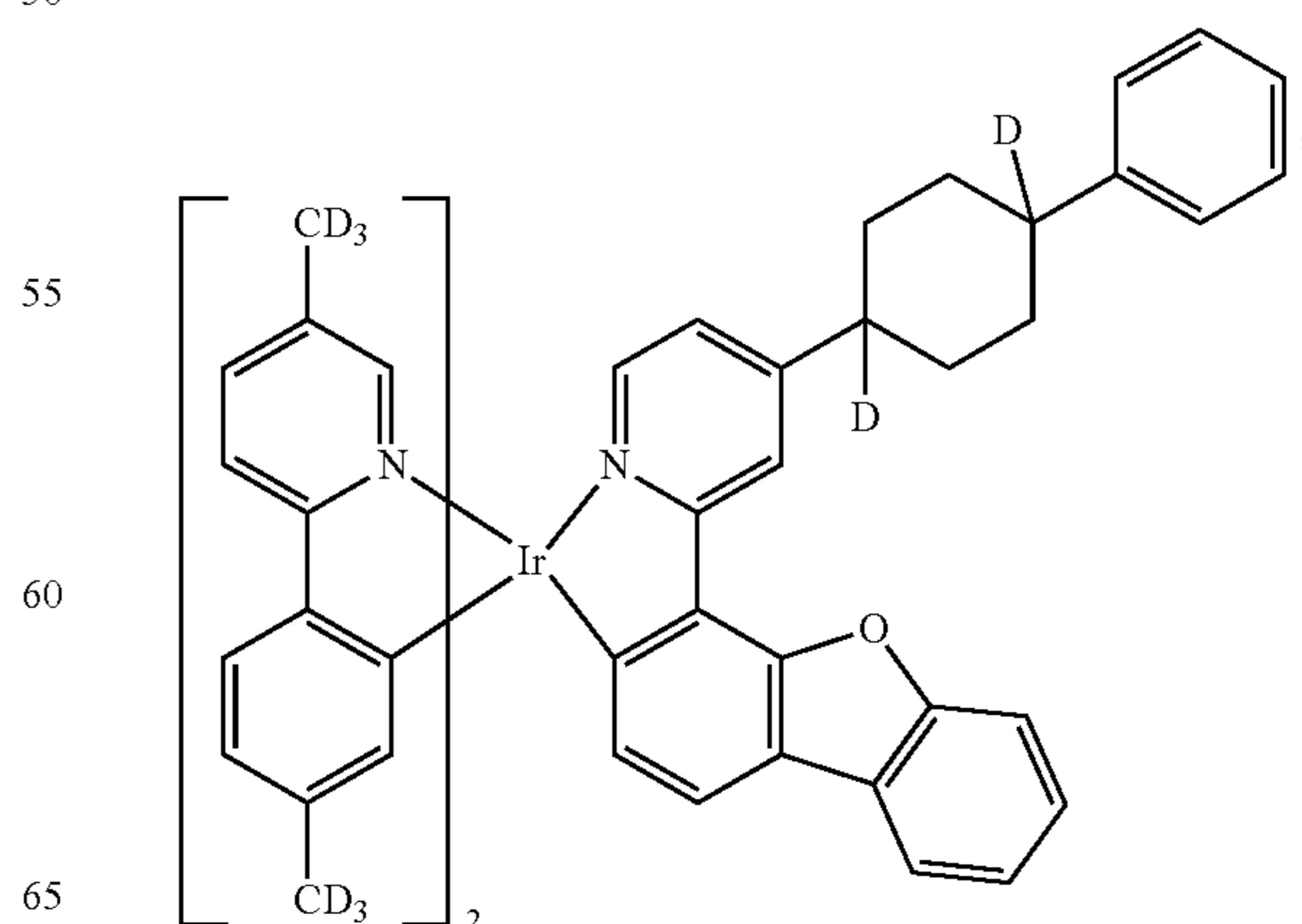
Compound 22
