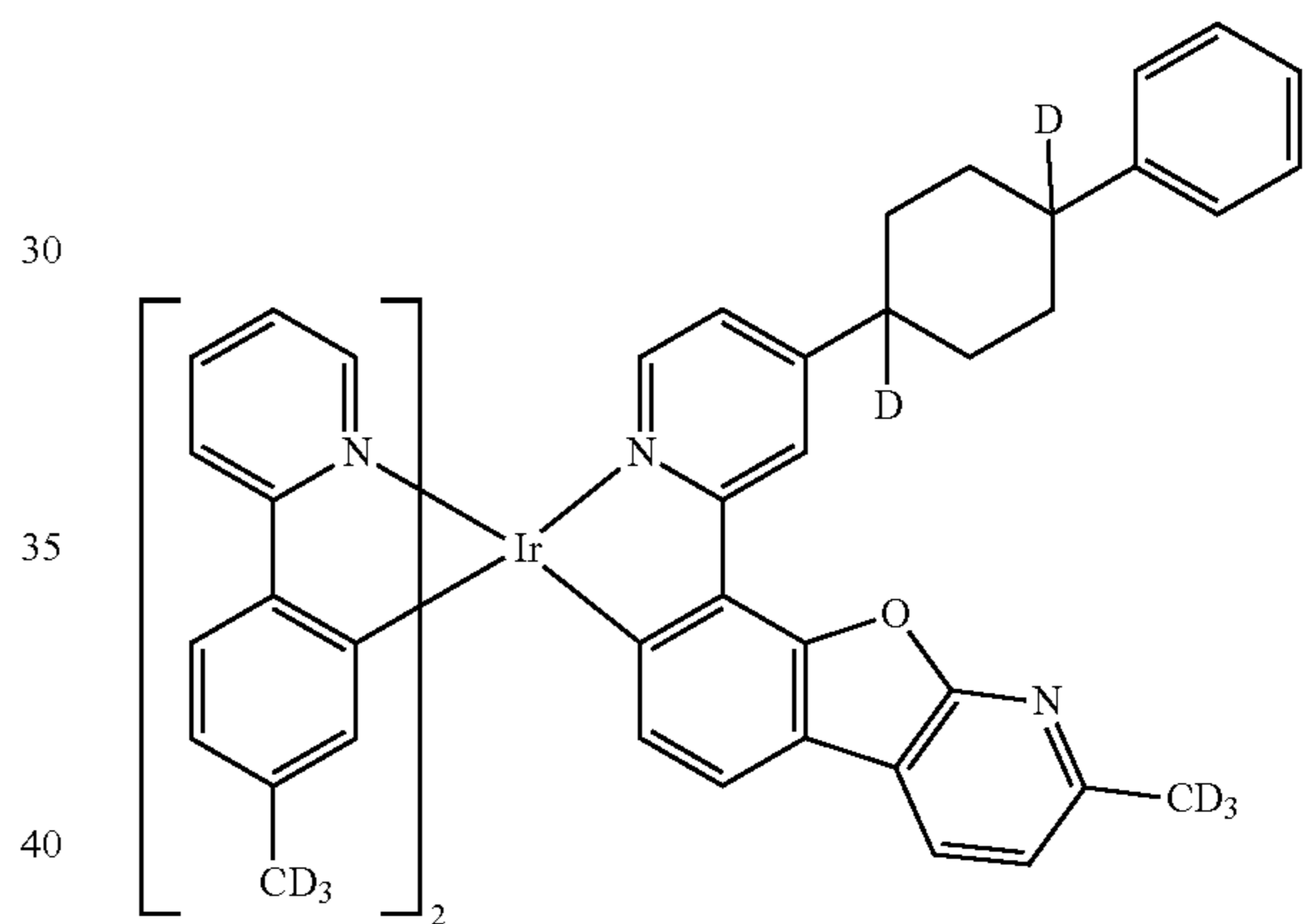
Compound 33
