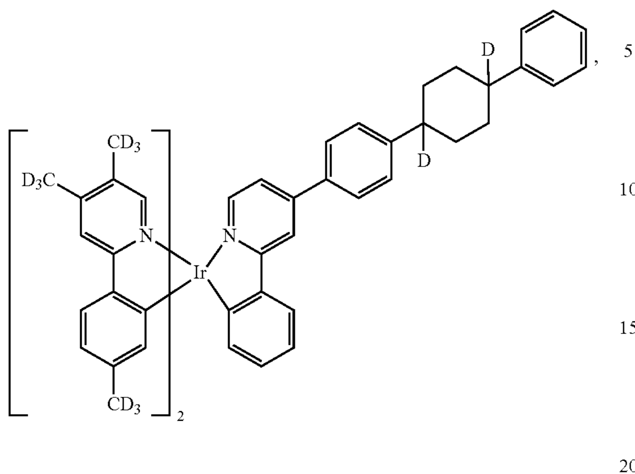
Compound 54
