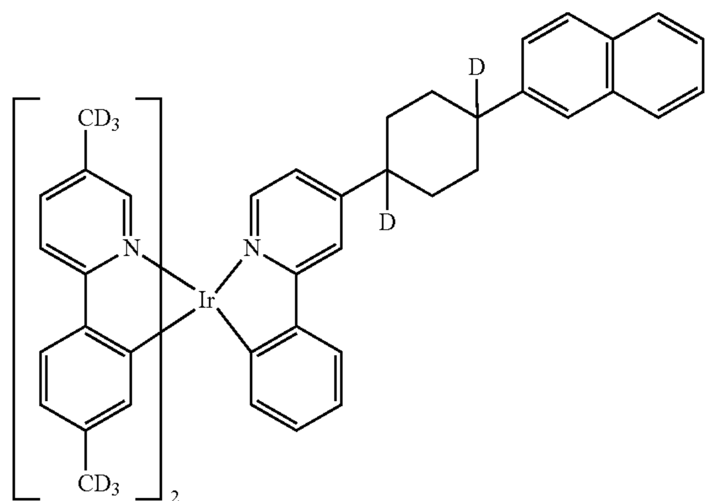
Compound 65
