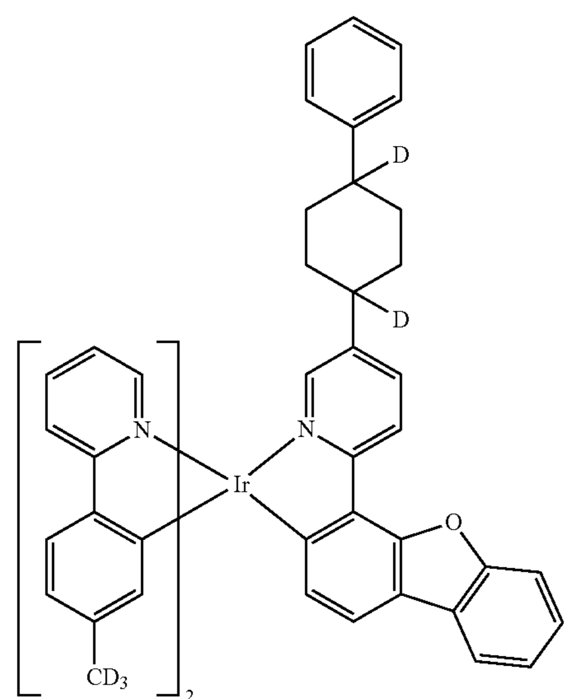
Compound 16
