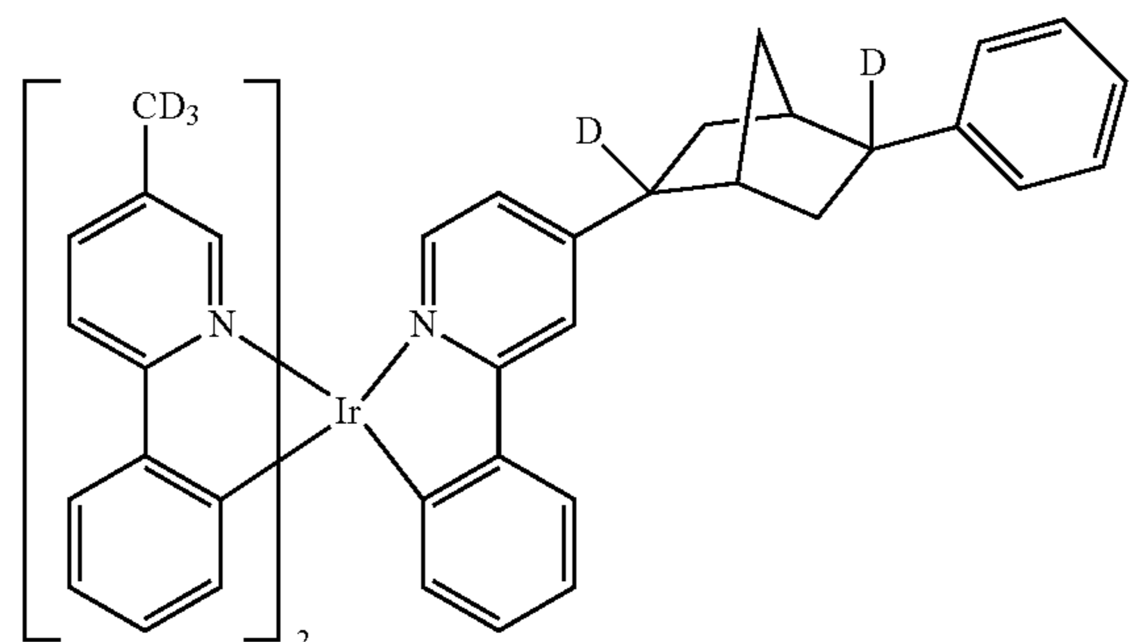
Compound 63
