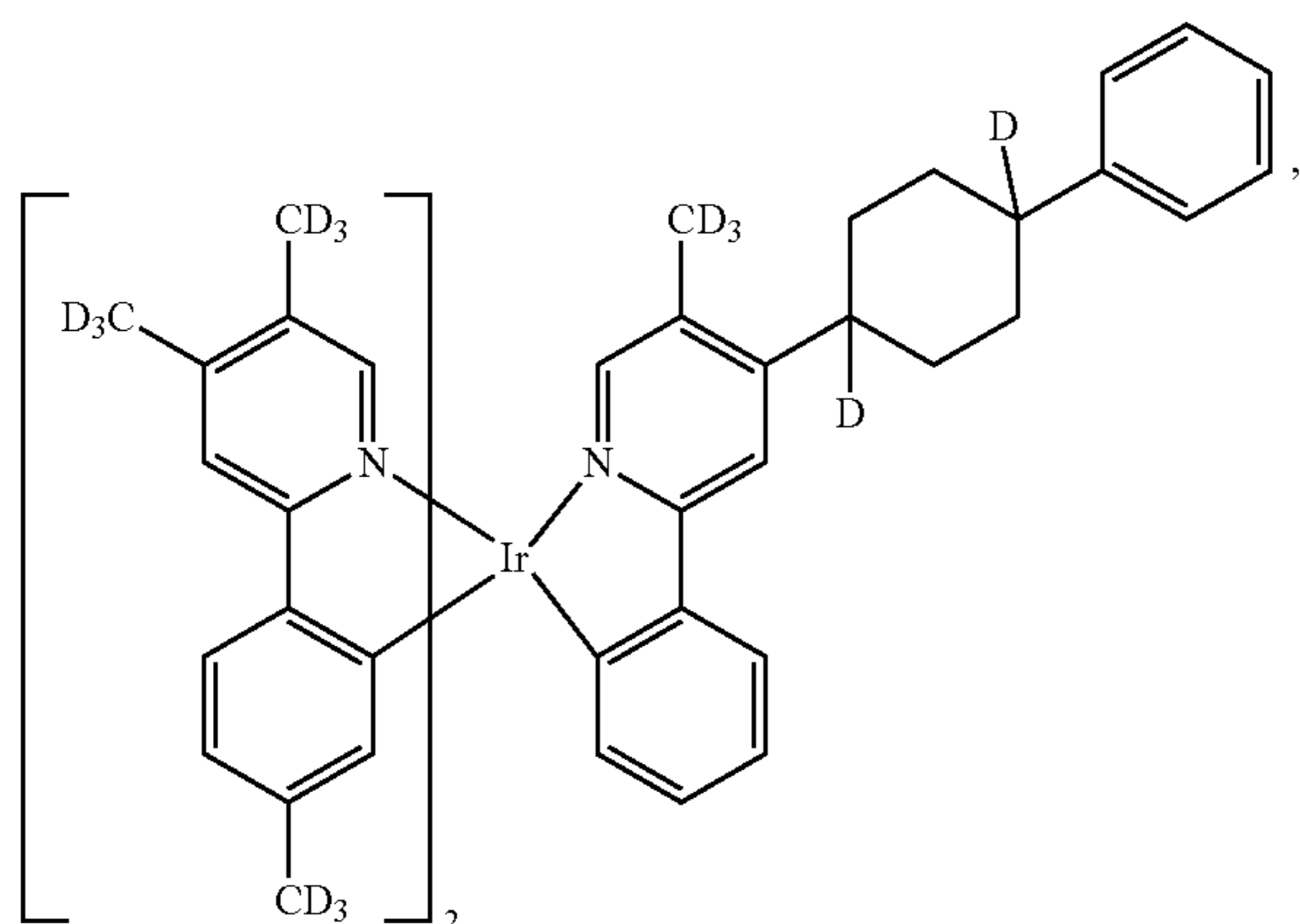
Compound 42
