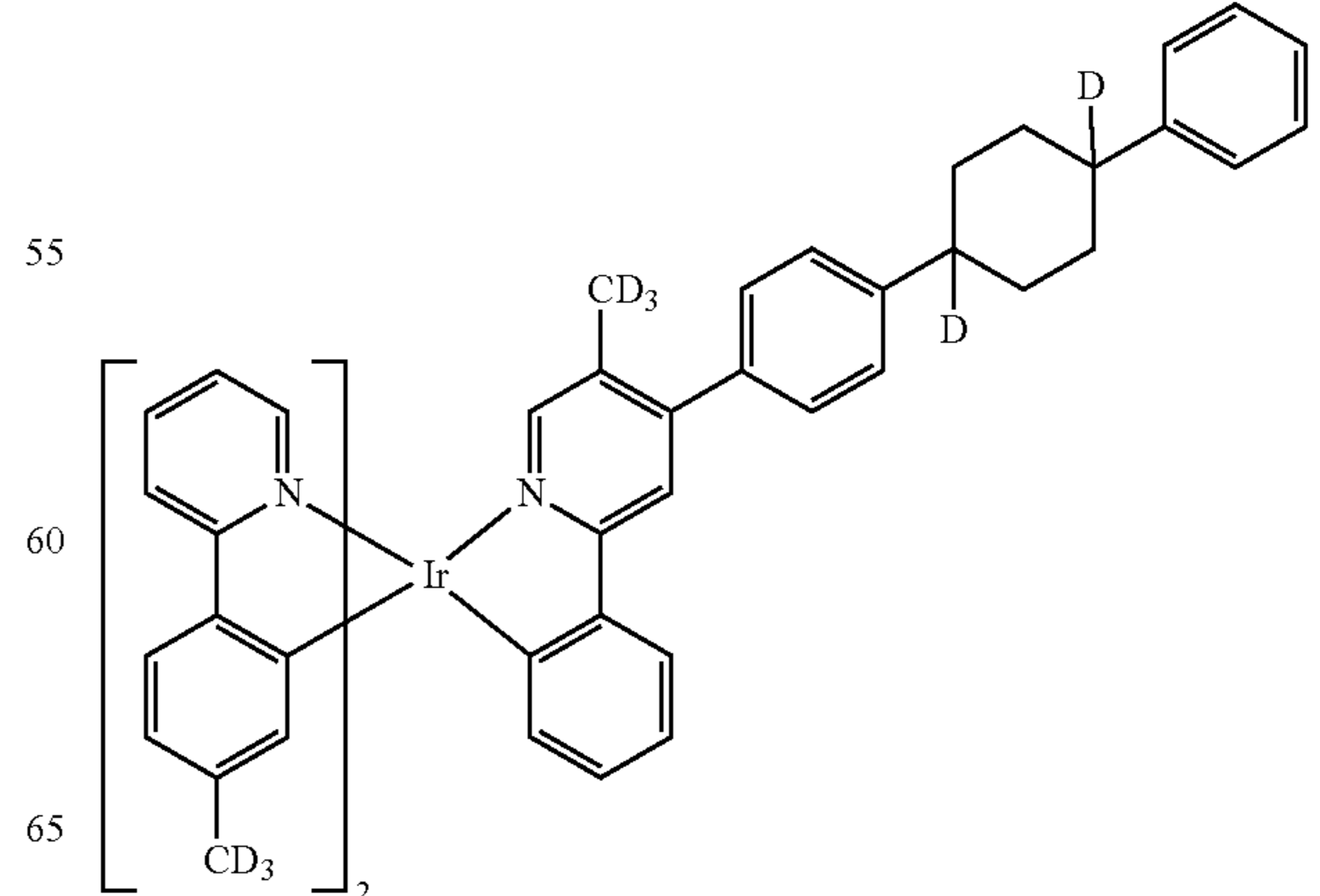
Compound 57
