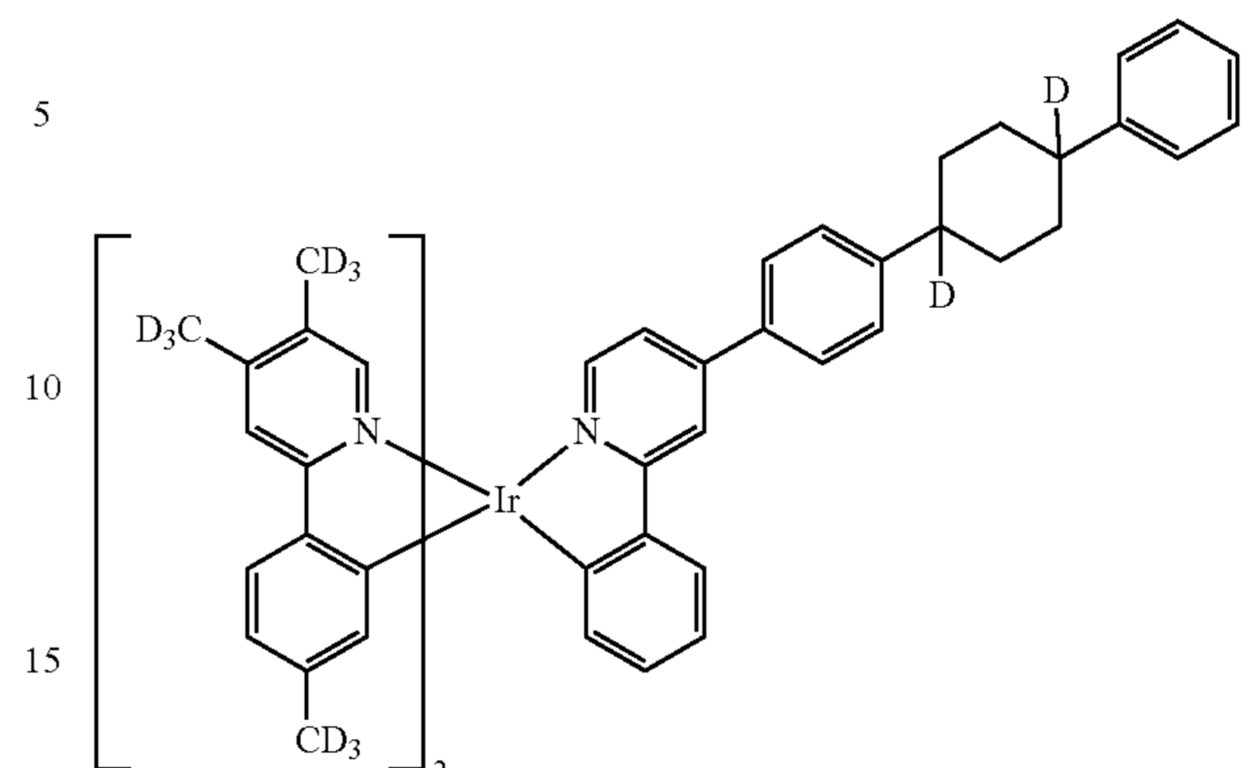
Compound 55
