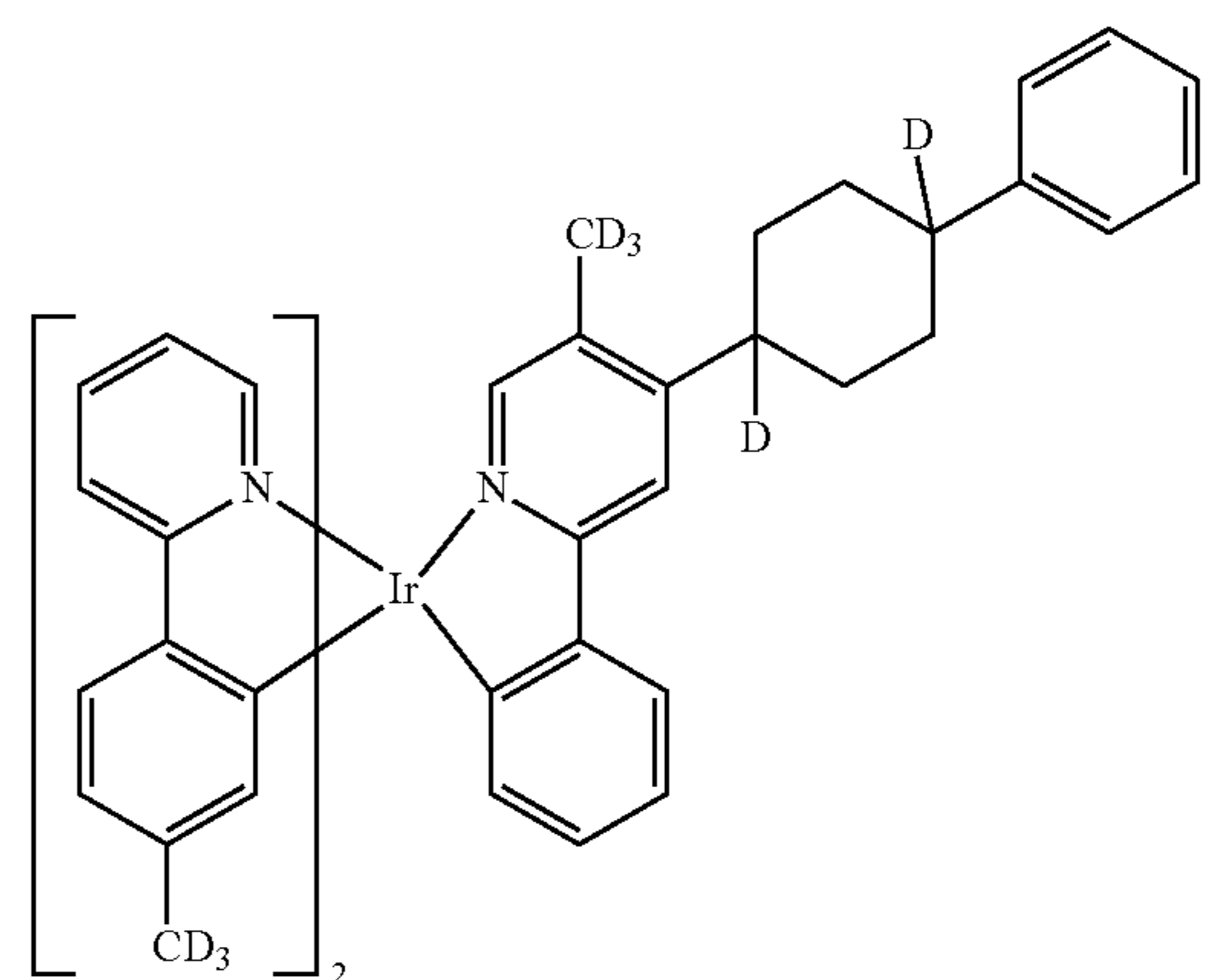
Compound 39
