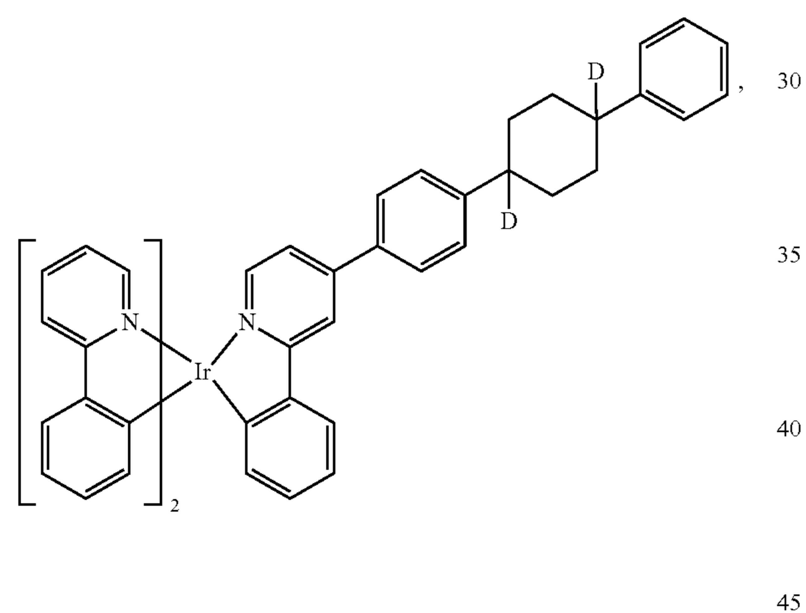
Compound 49
