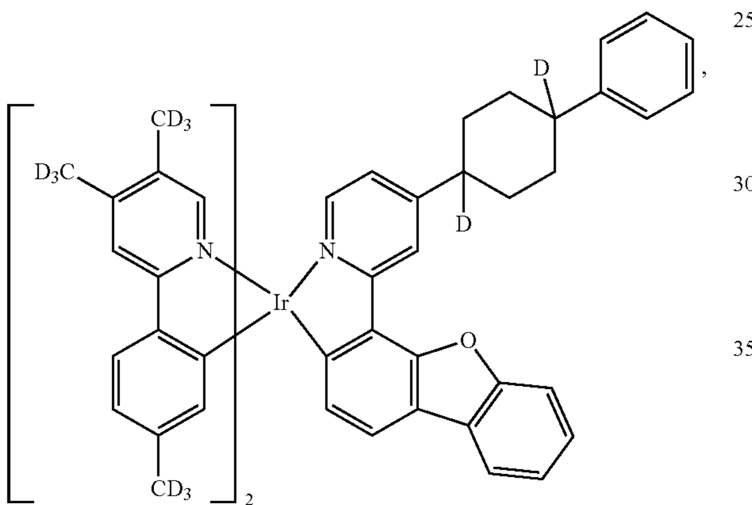
Compound 24
