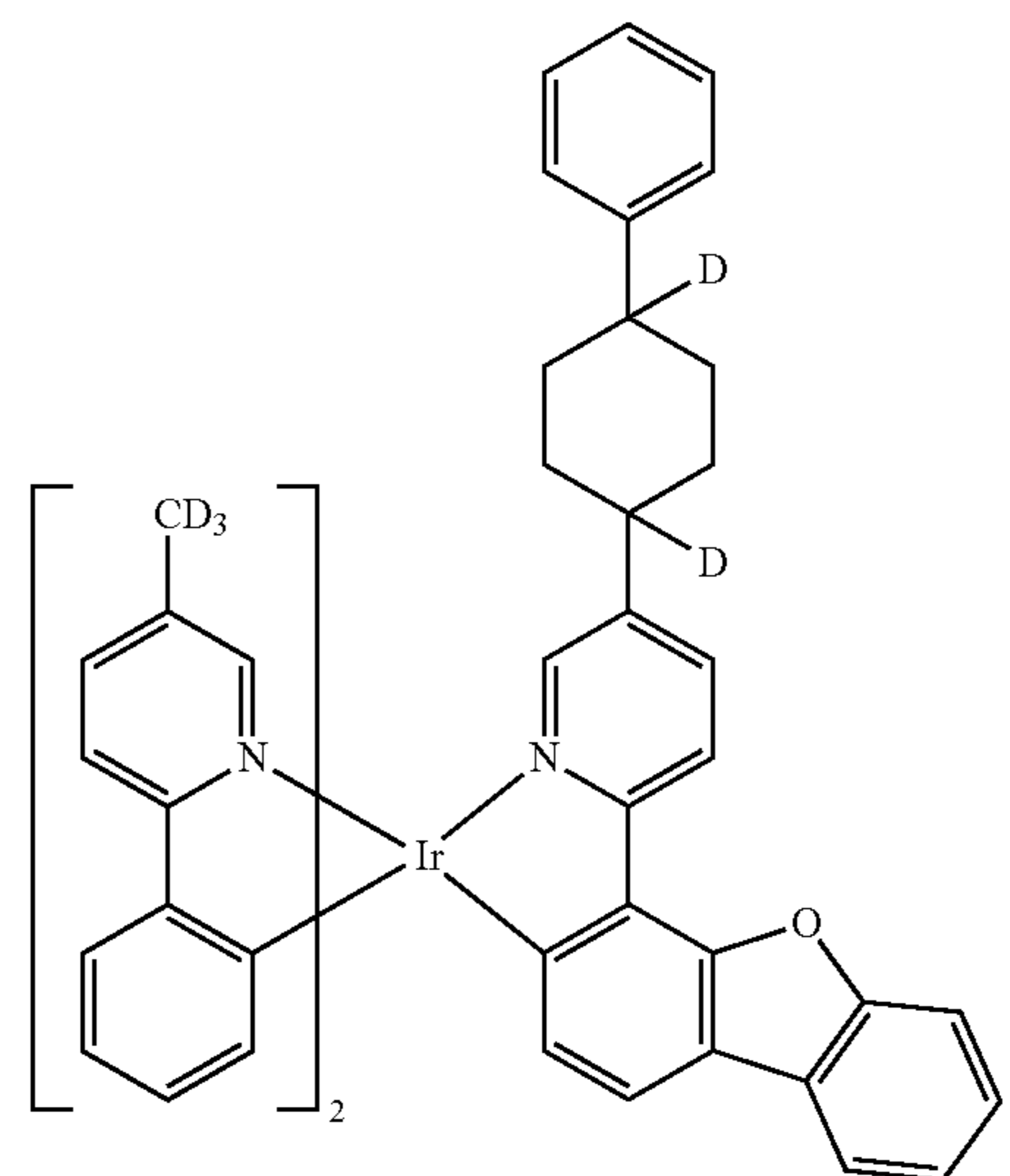
Compound 15
