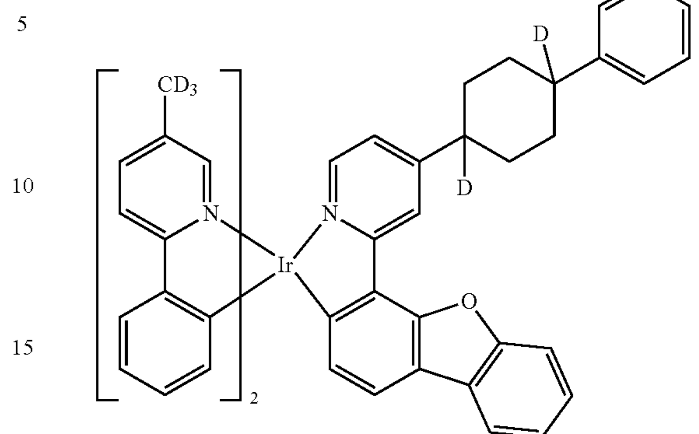
Compound 20
