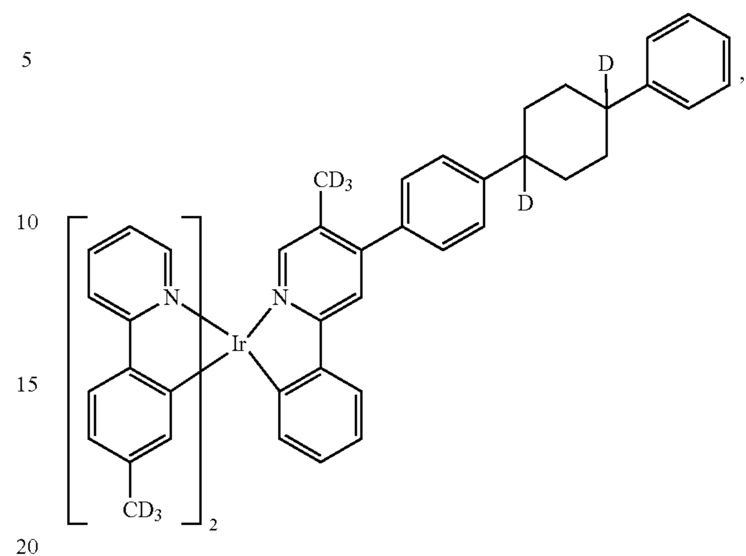
Compound 57
