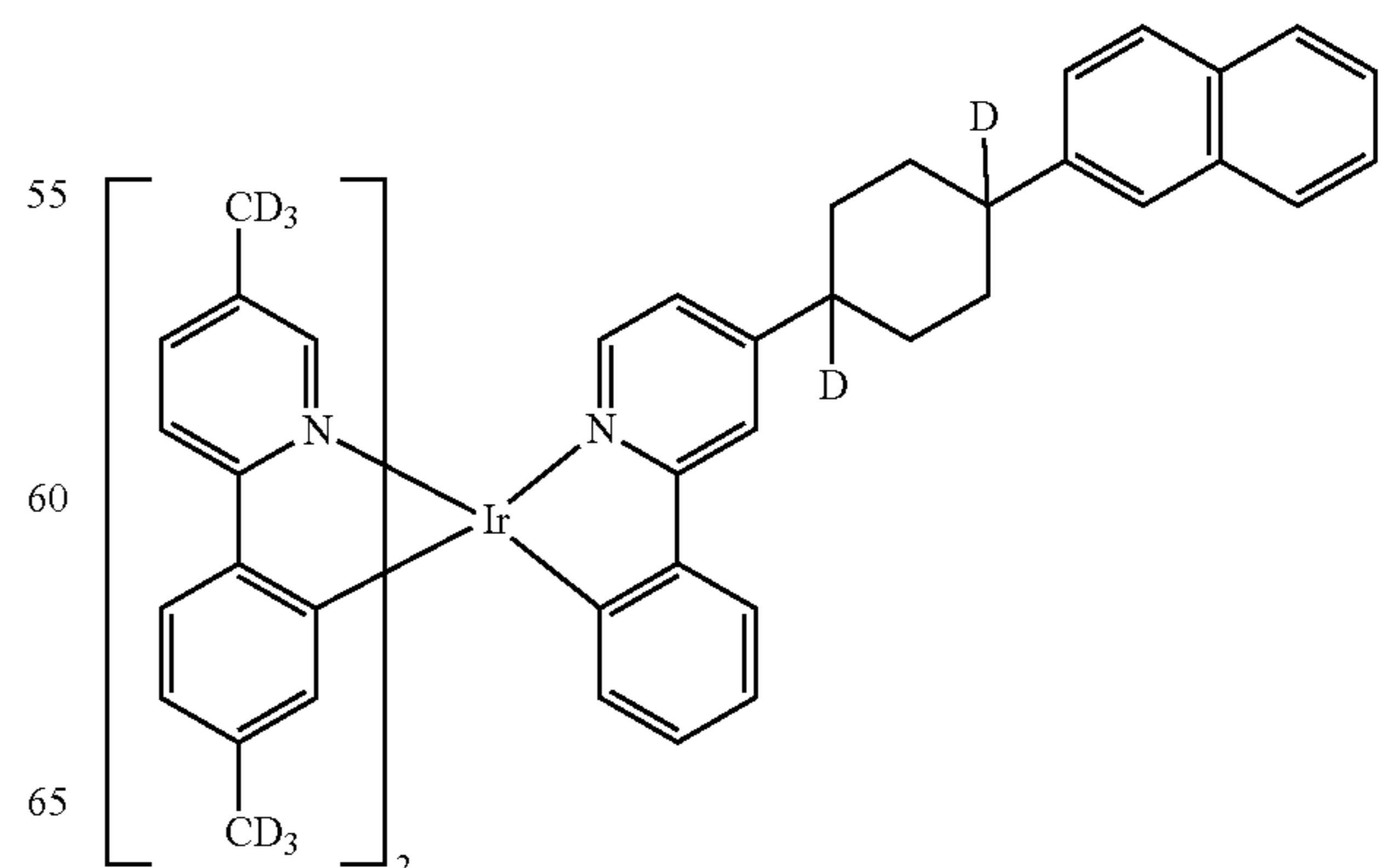
Compound 65
