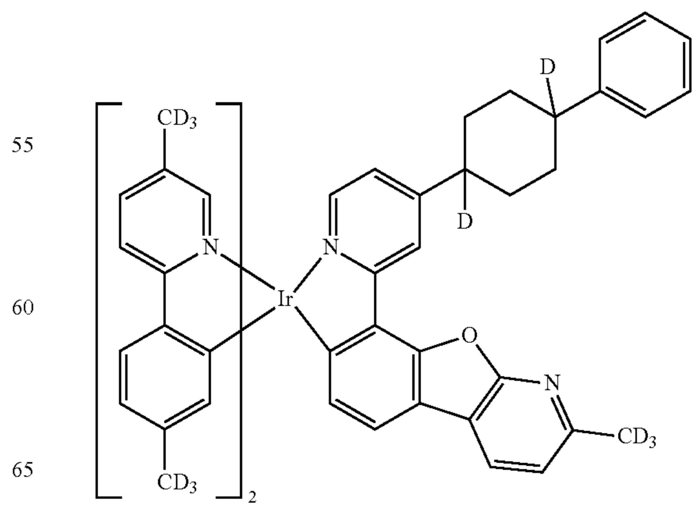
Compound 34
