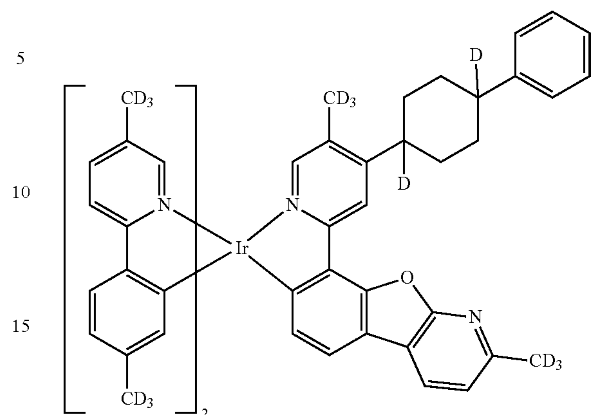
Compound 47
