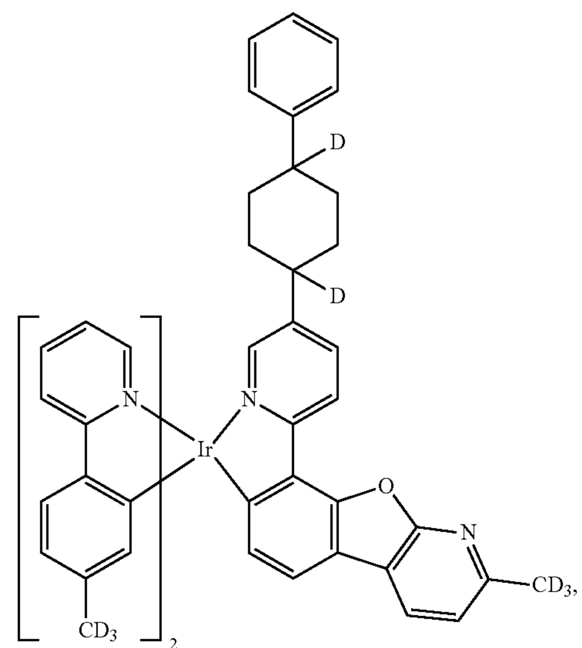
Compound 28
