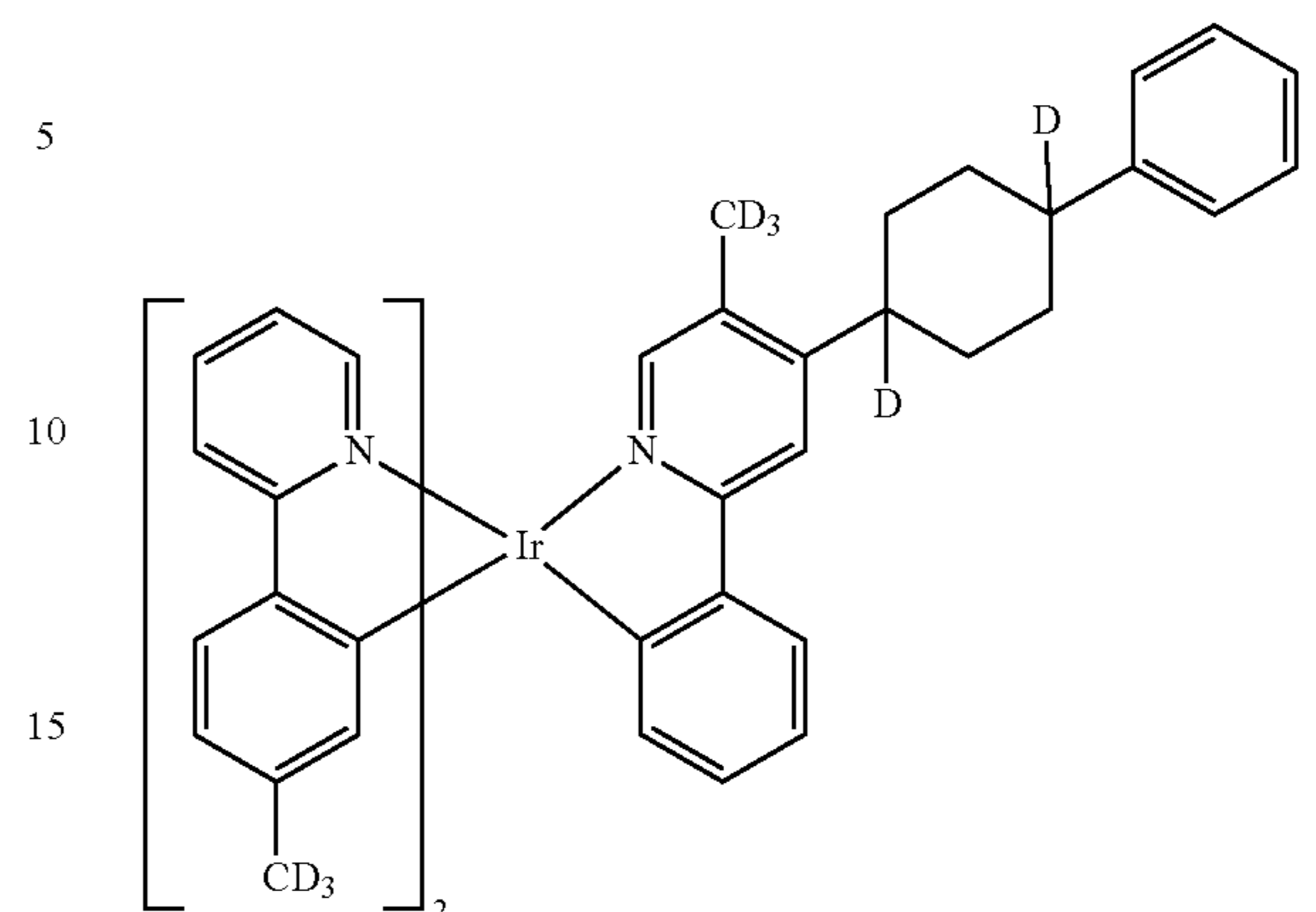
Compound 40
