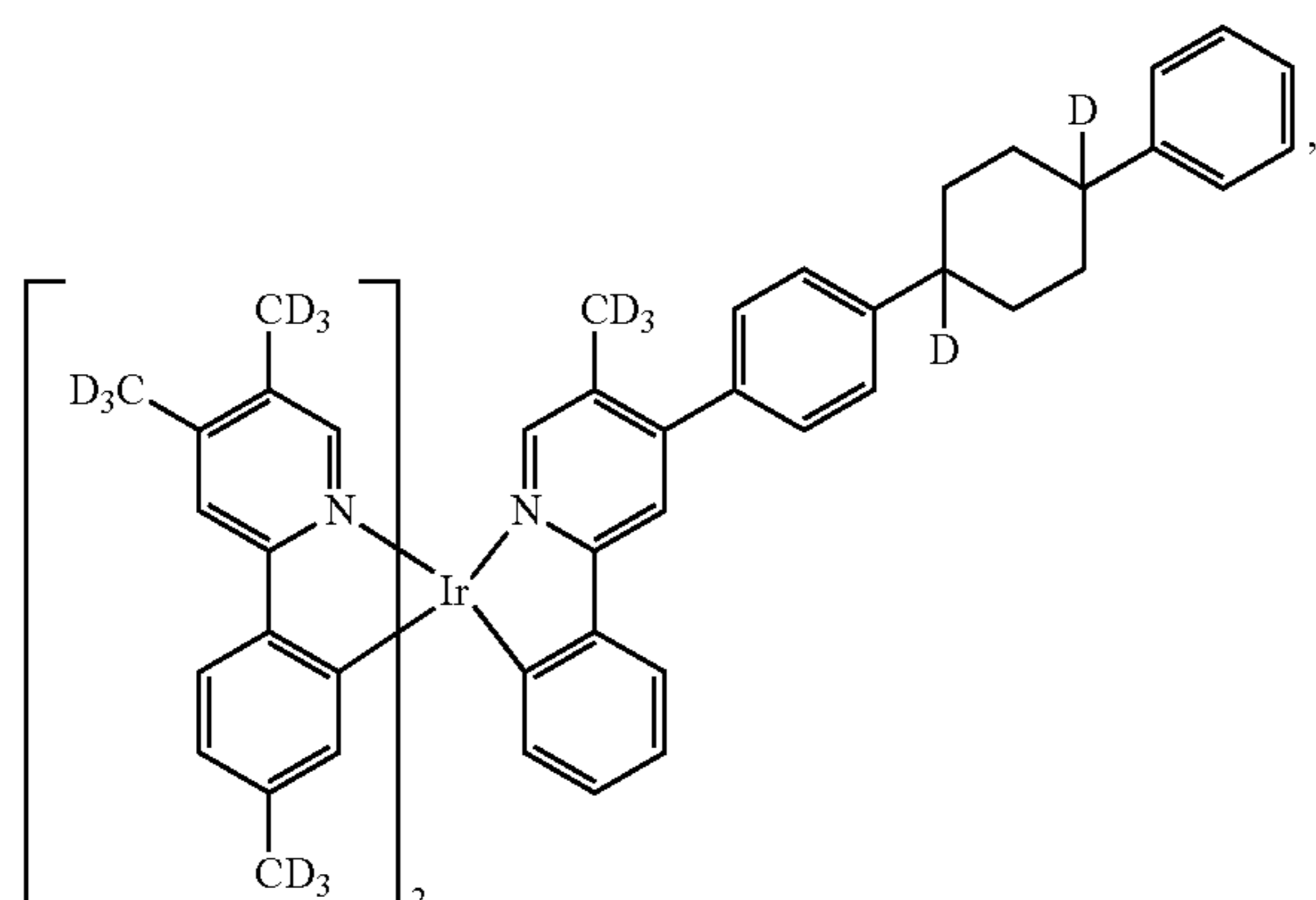
Compound 60
