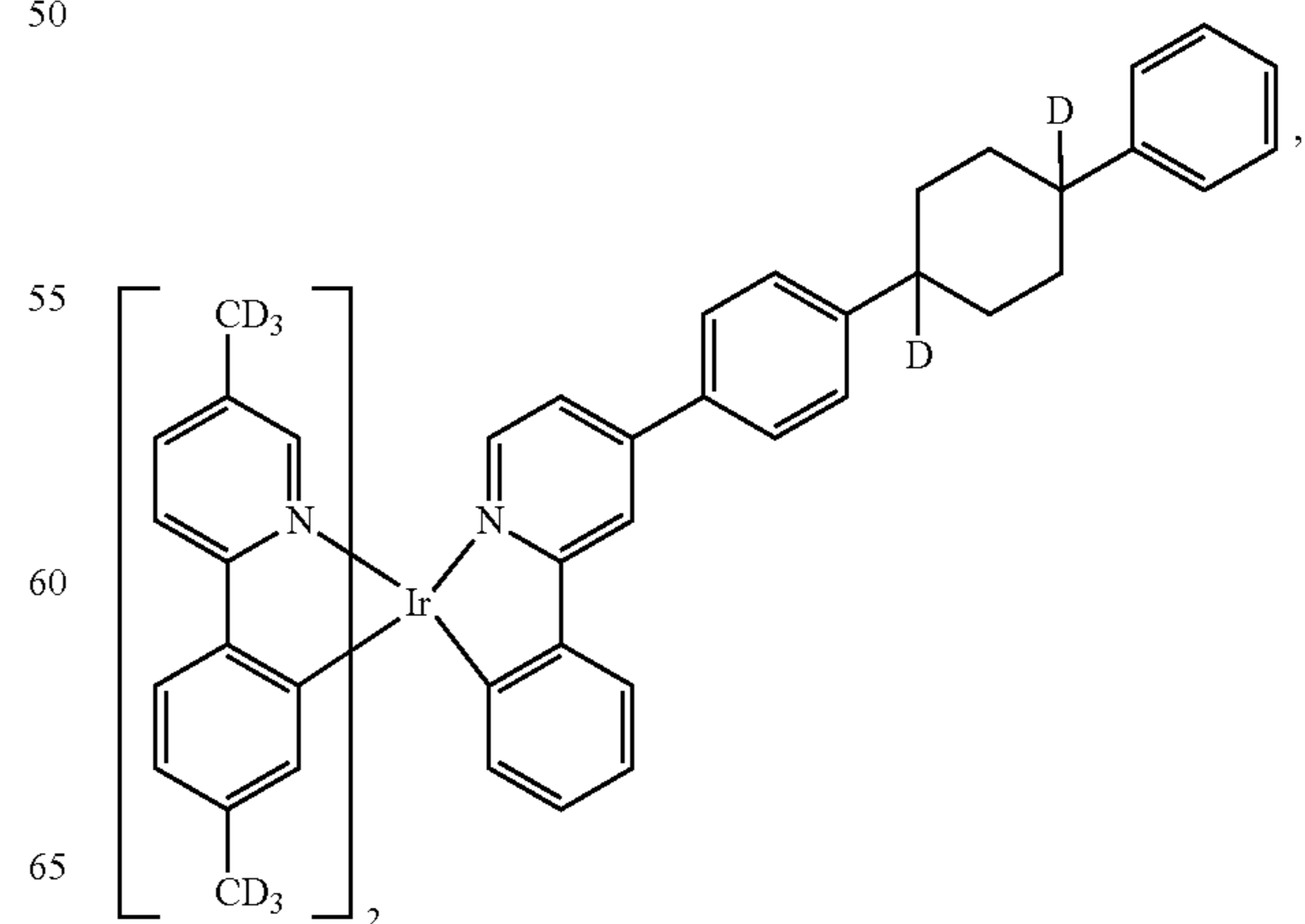
Compound 53
