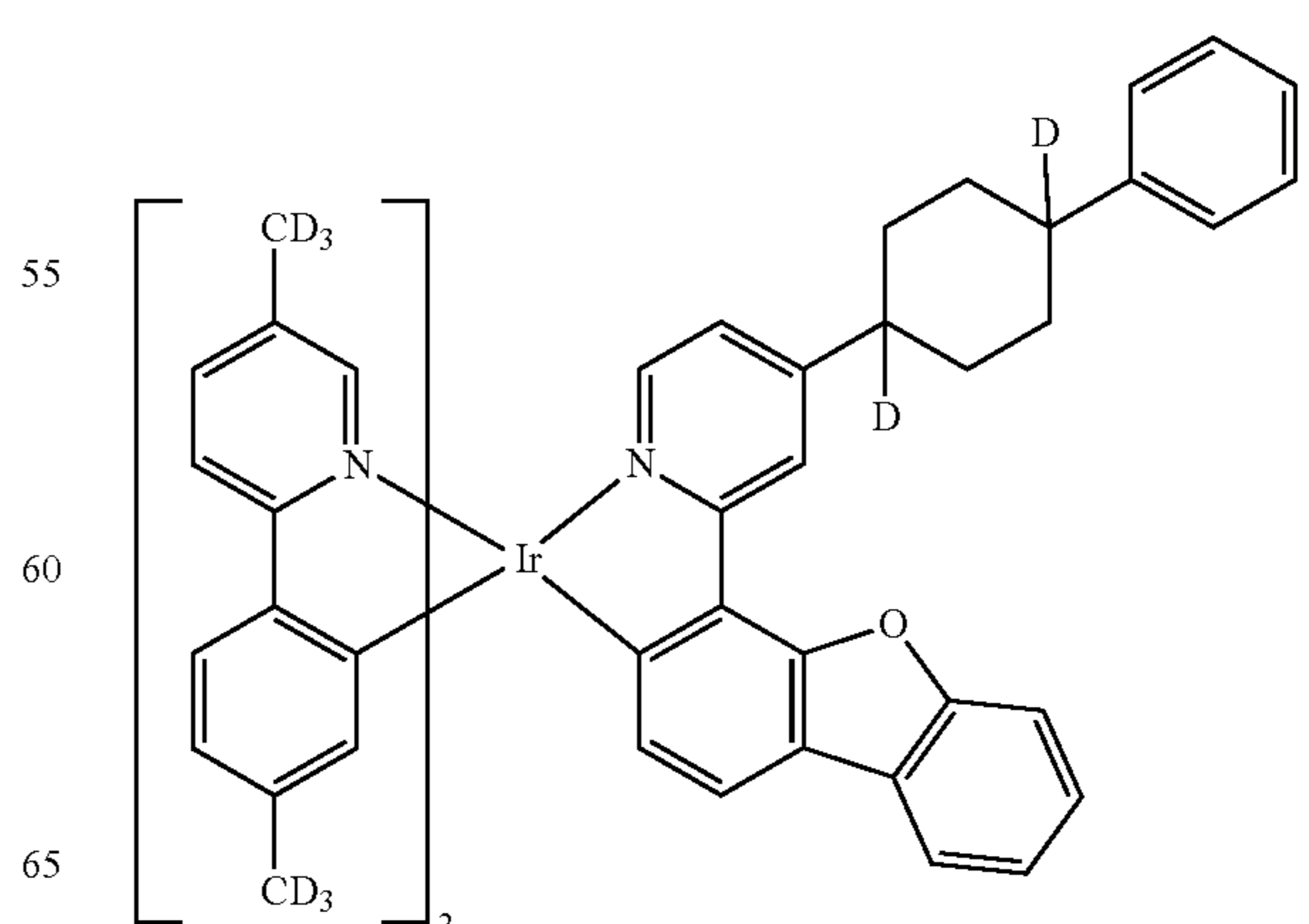
Compound 22
