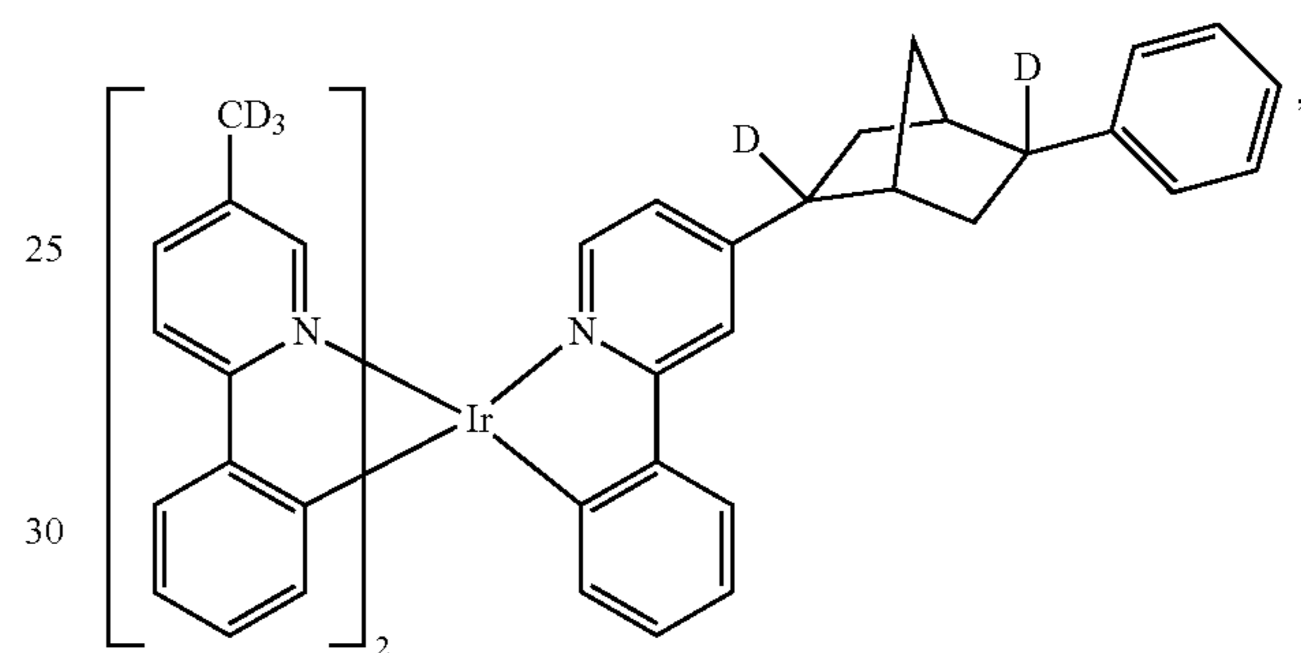
Compound 64
