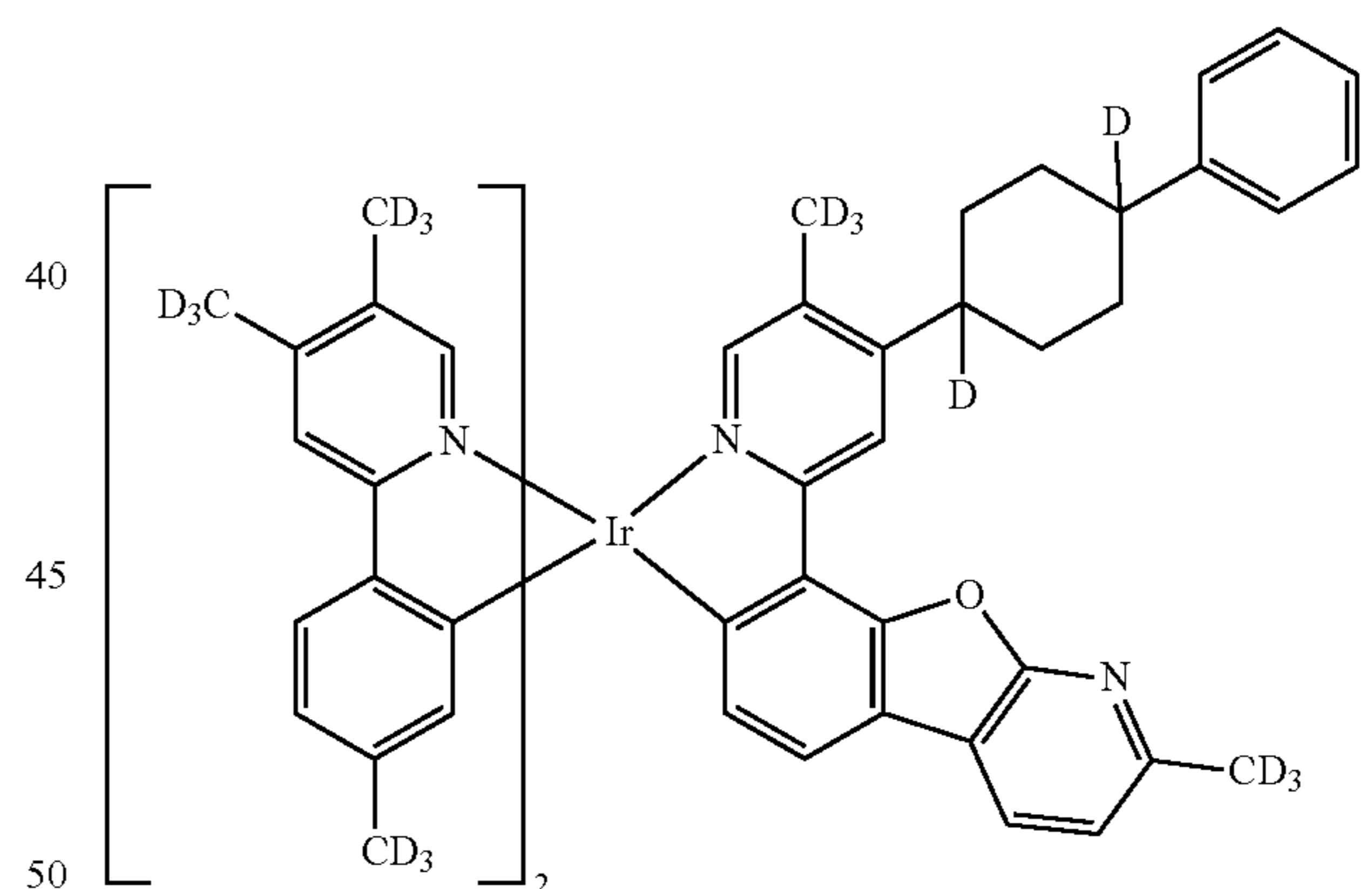
Compound 49
