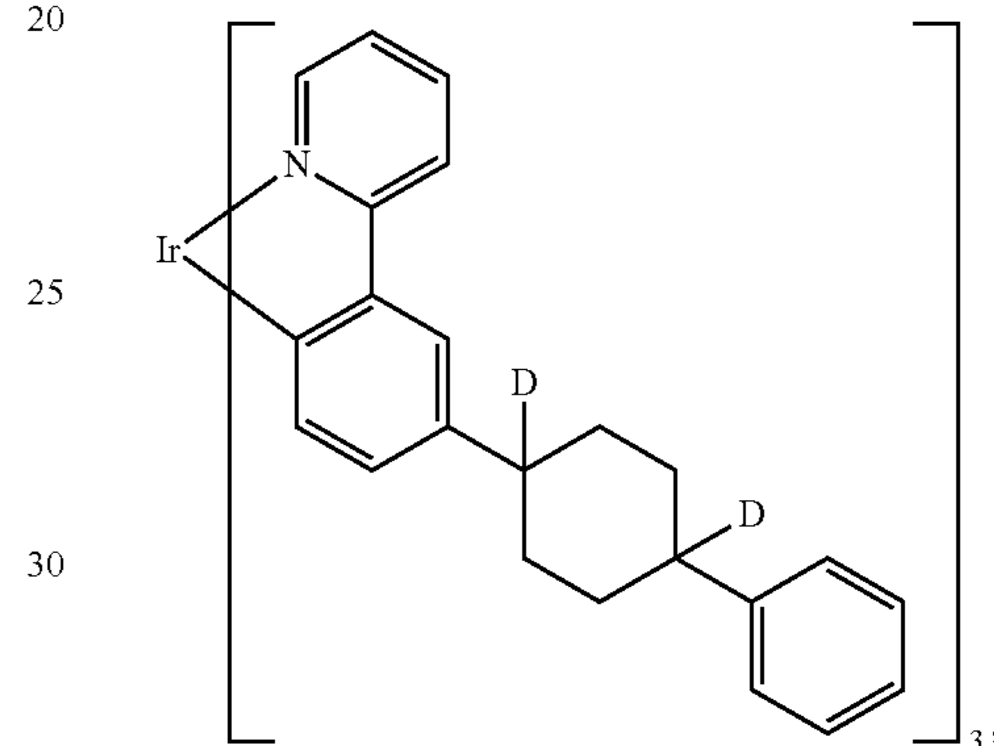
Compound 74
