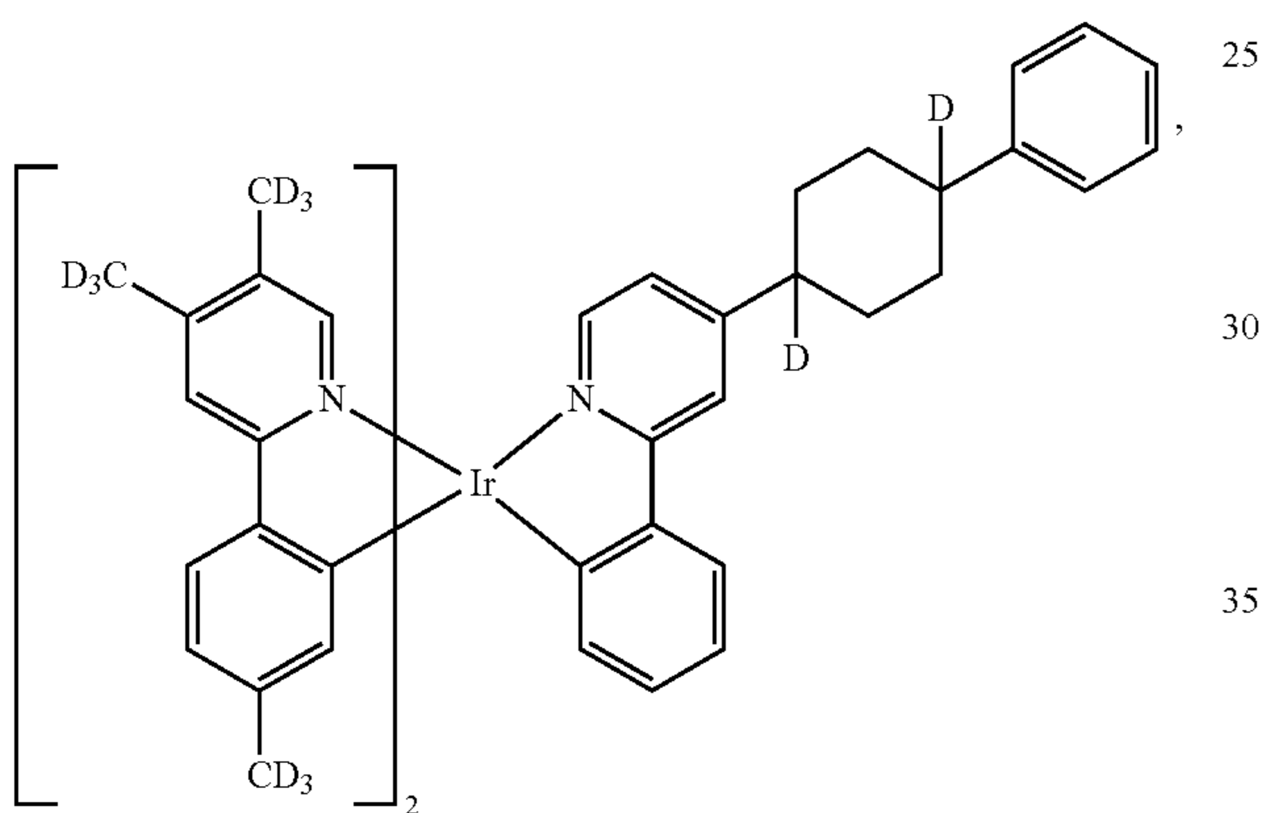
Compound 12
