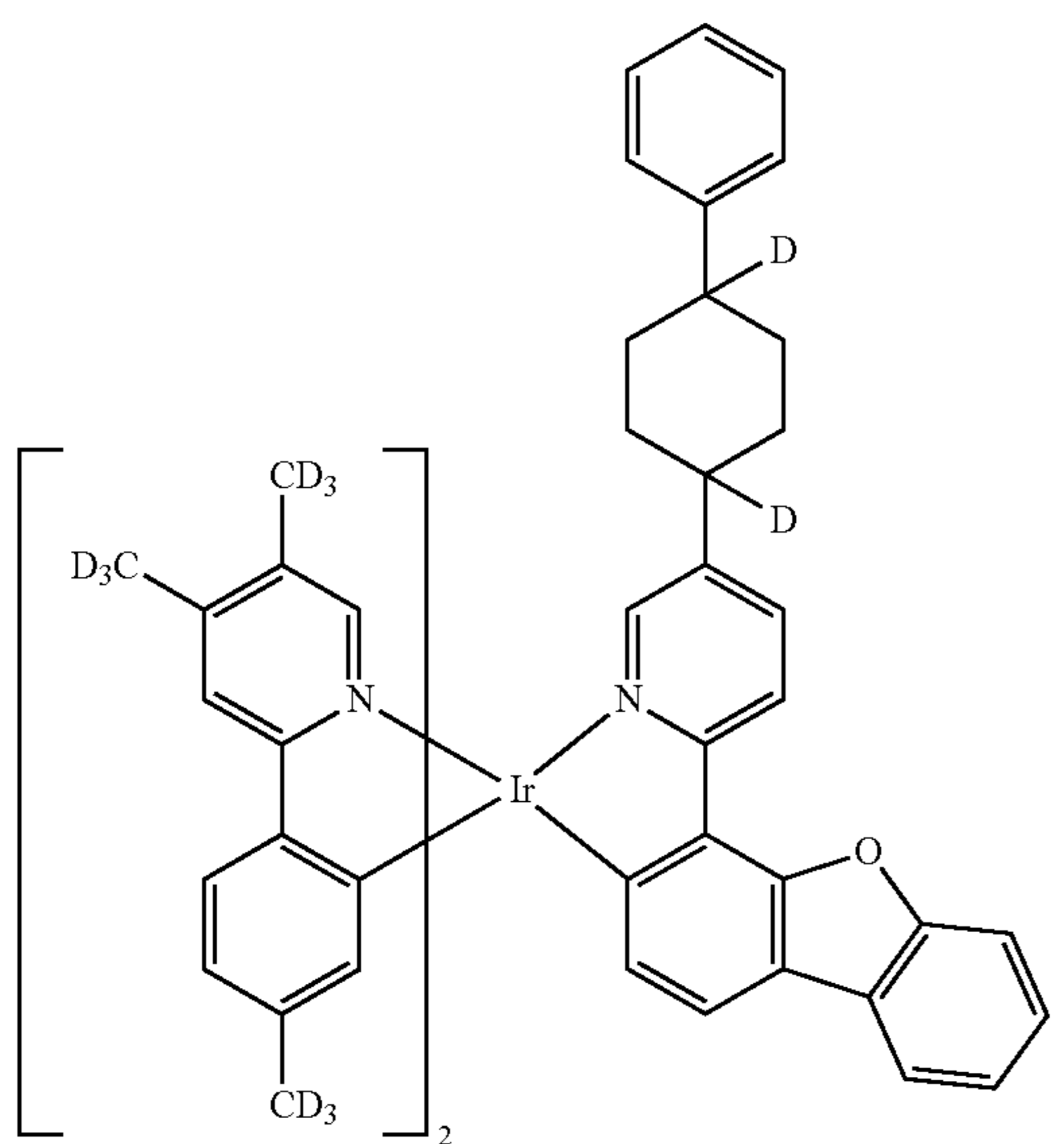
Compound 18
