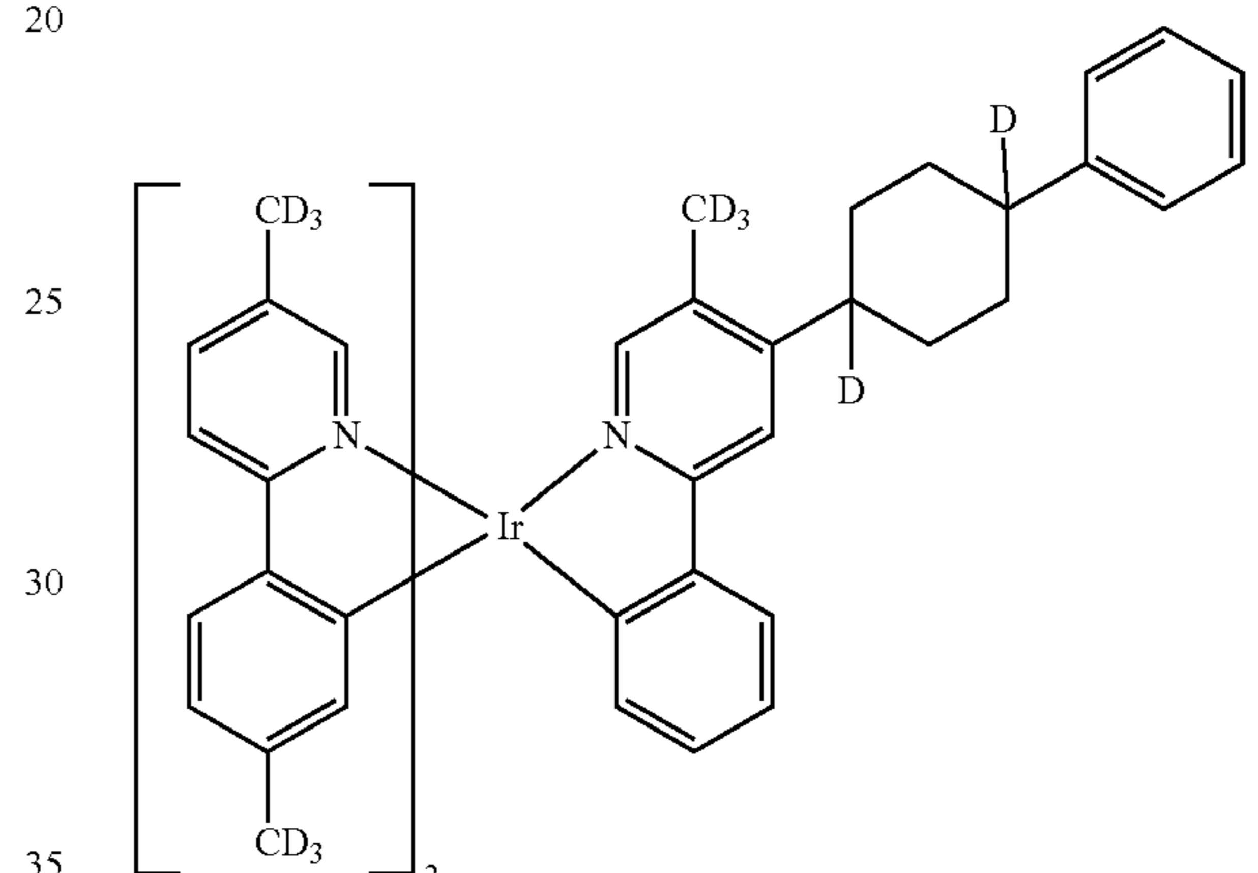
Compound 41
