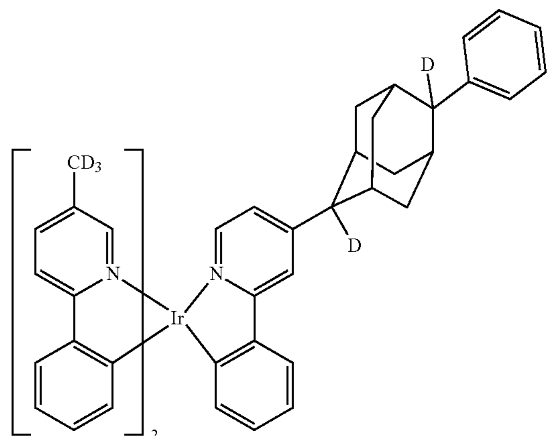
Compound 64
