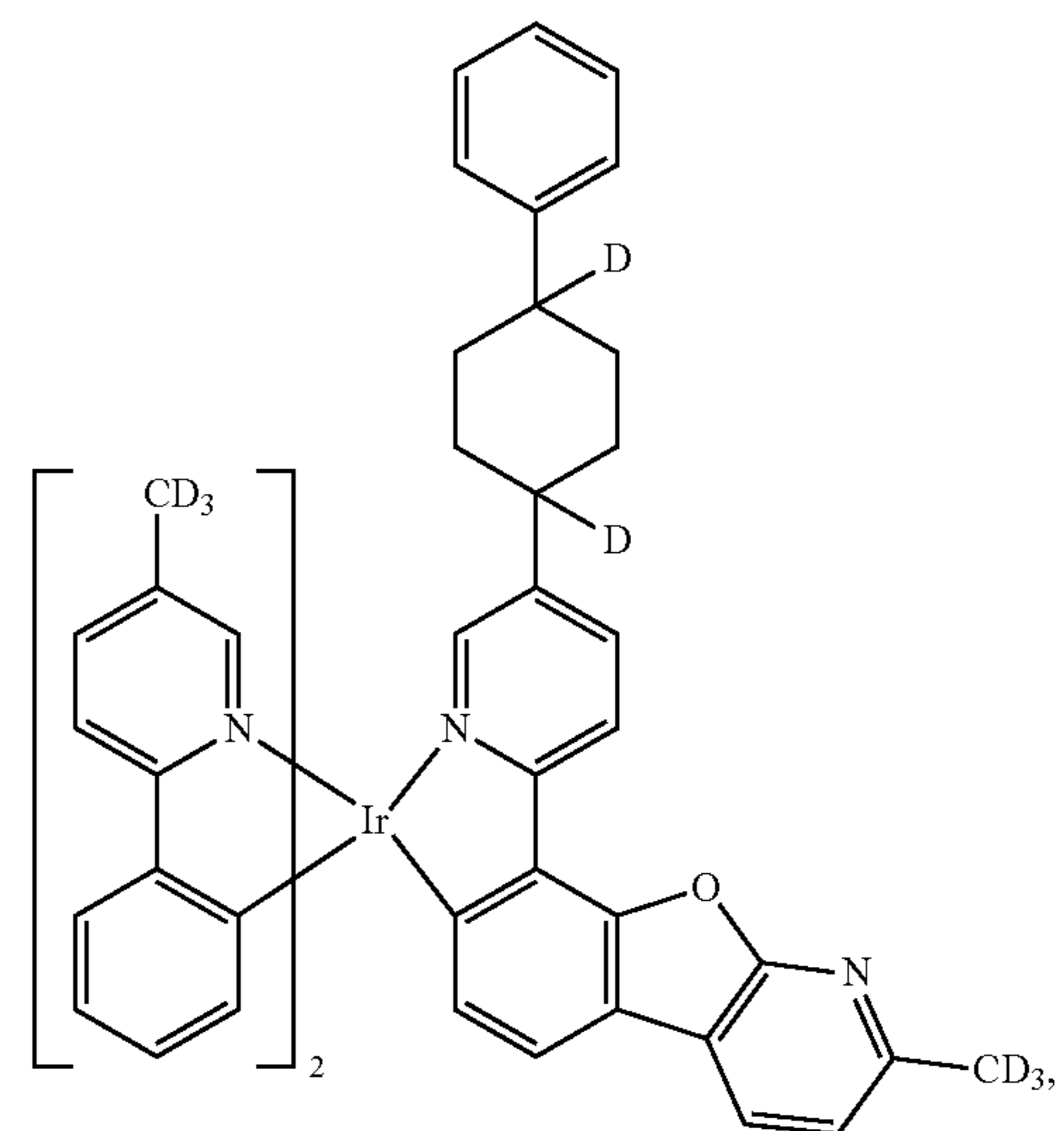
Compound 27
