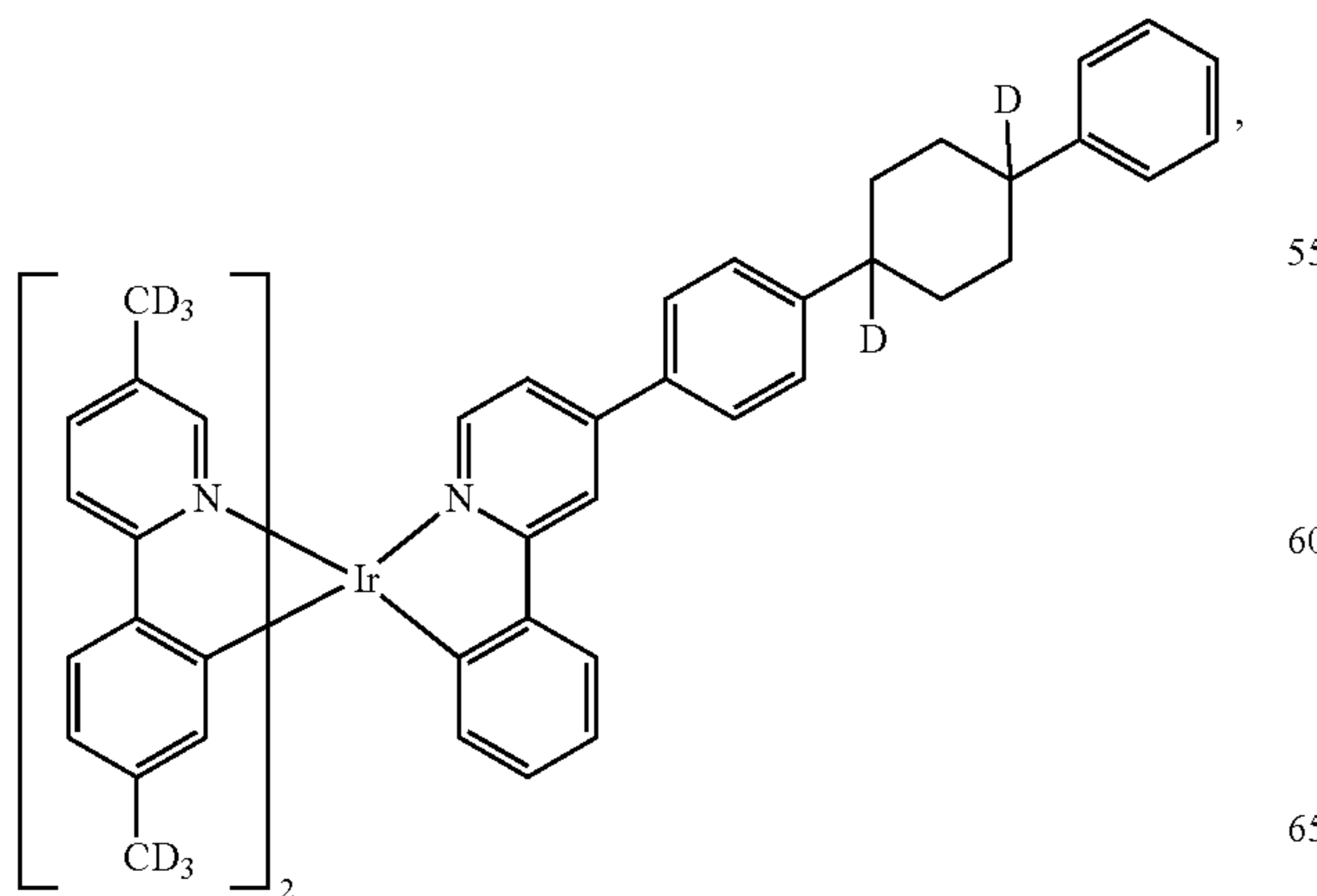
Compound 53
