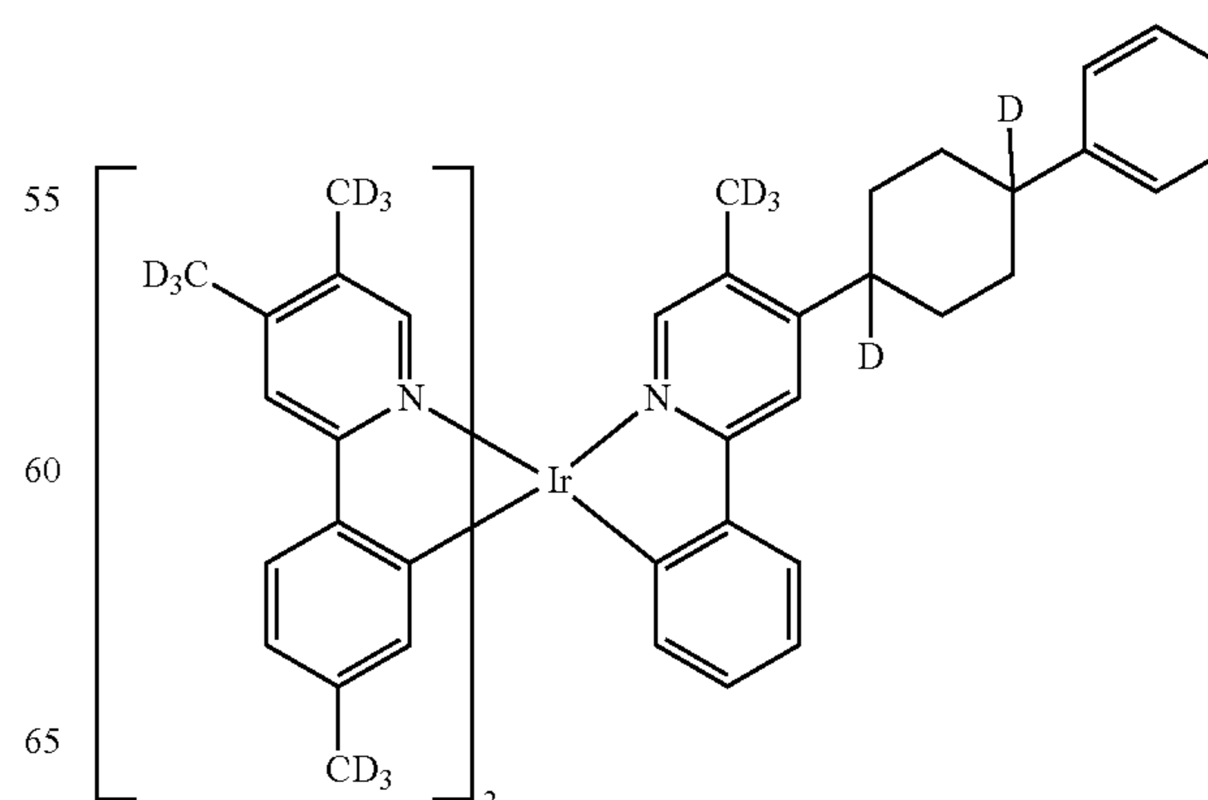
Compound 42
