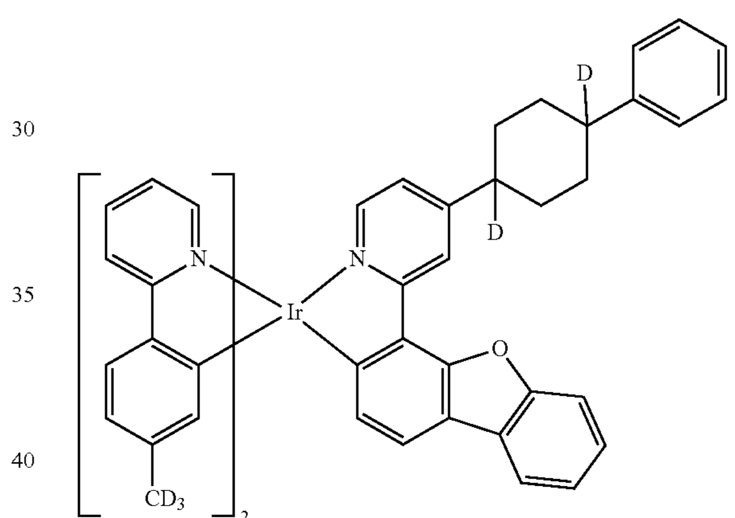
Compound 21
