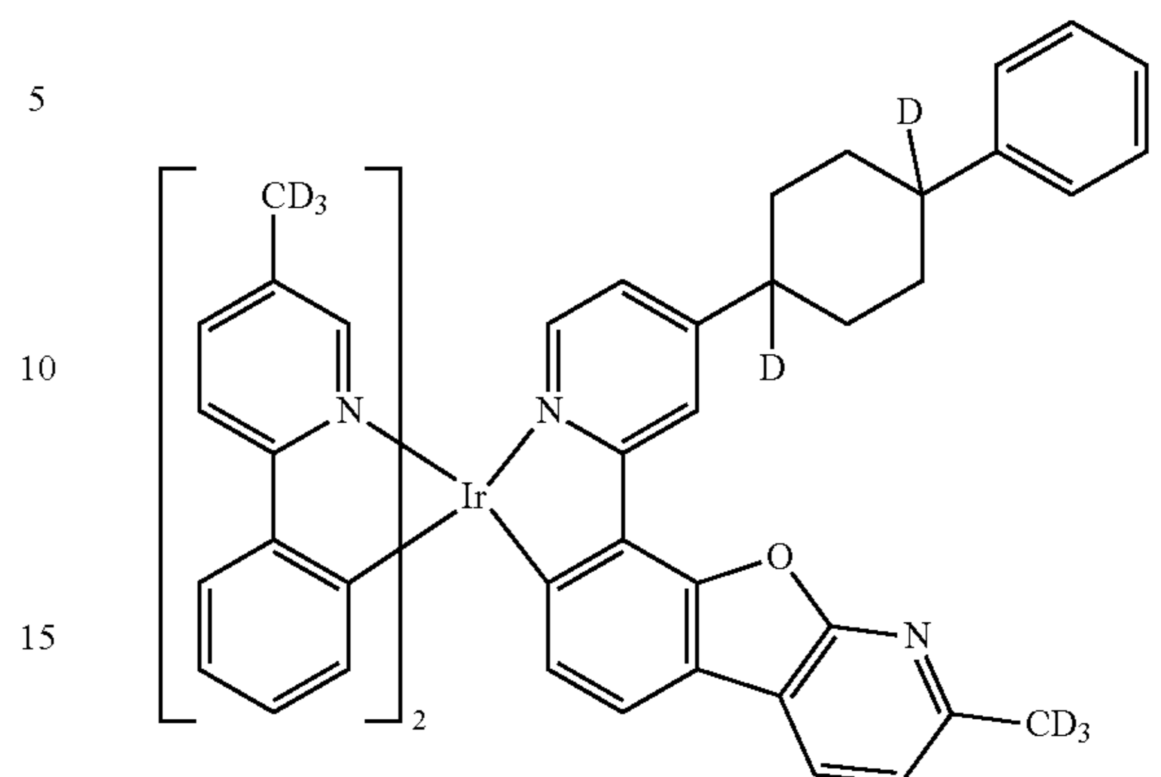
Compound 32
