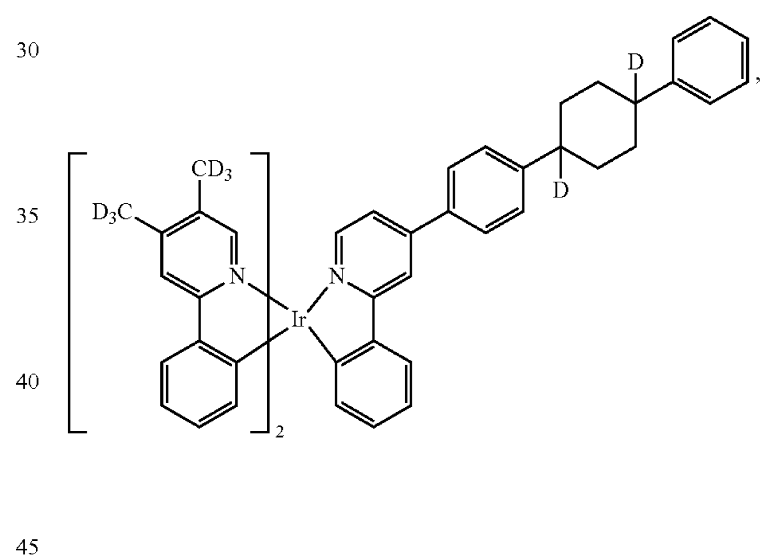
Compound 52
