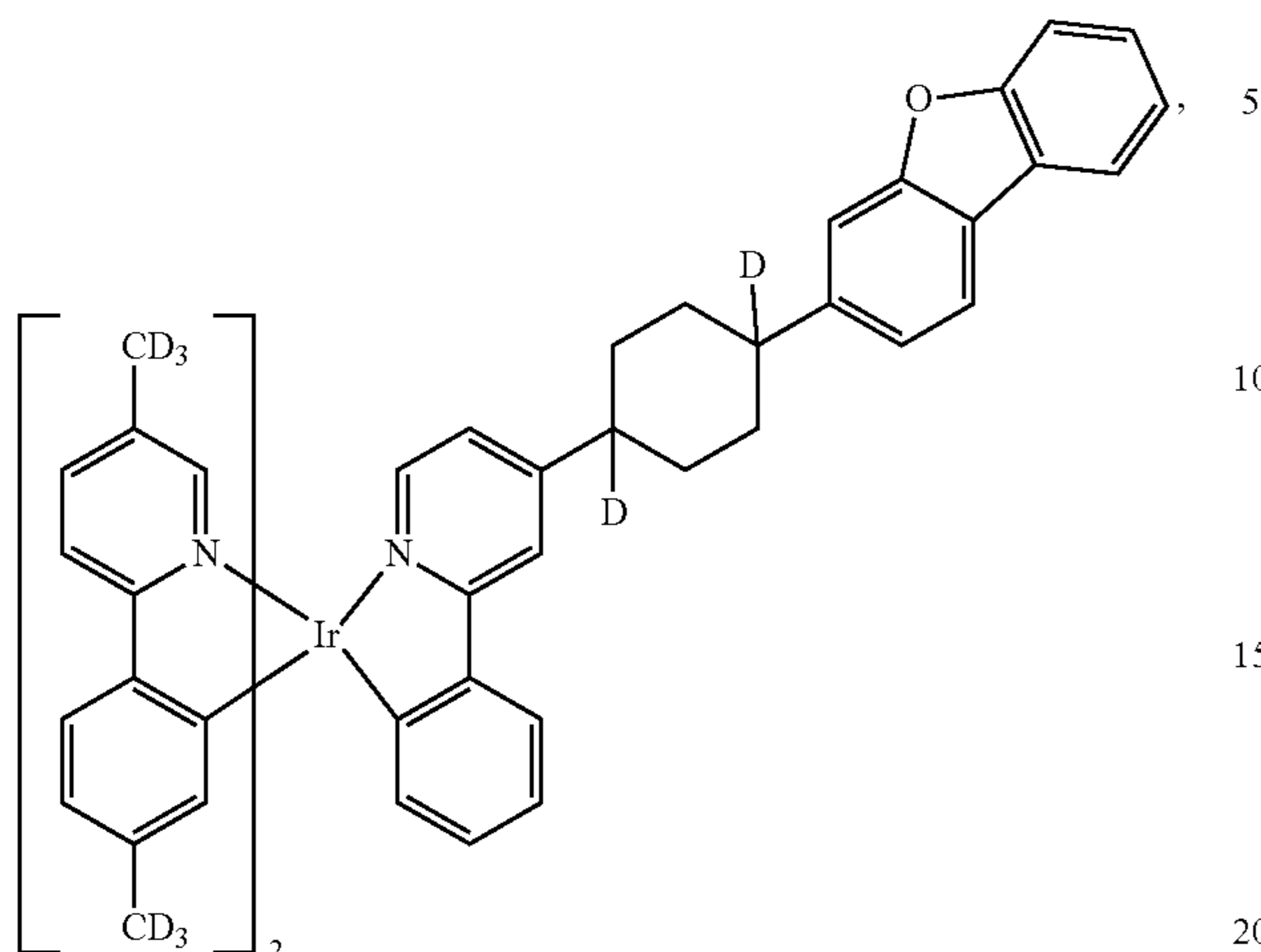
Compound 66
