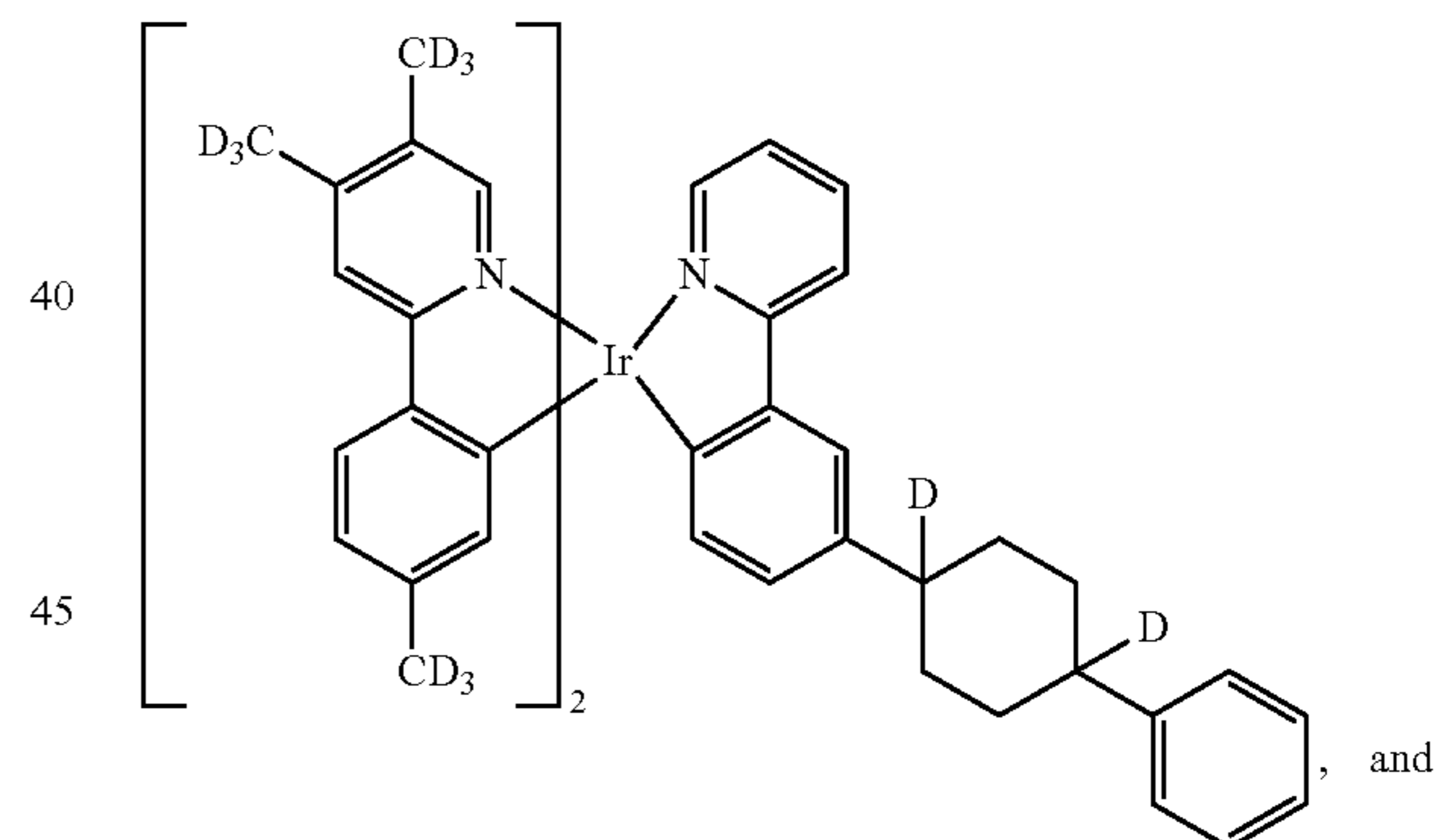
Compound 79
