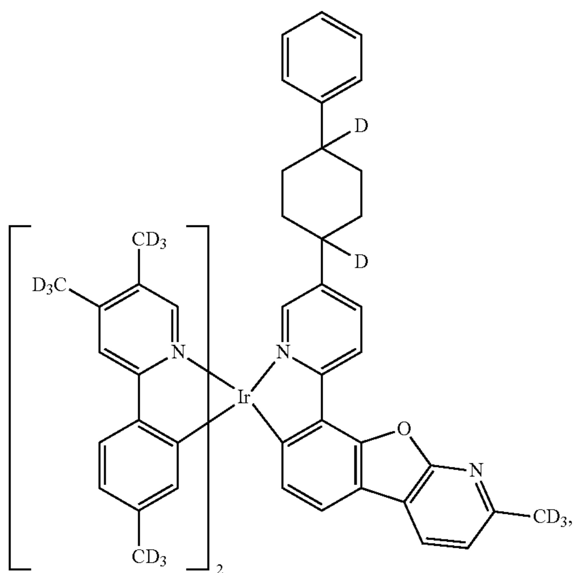
Compound 30
