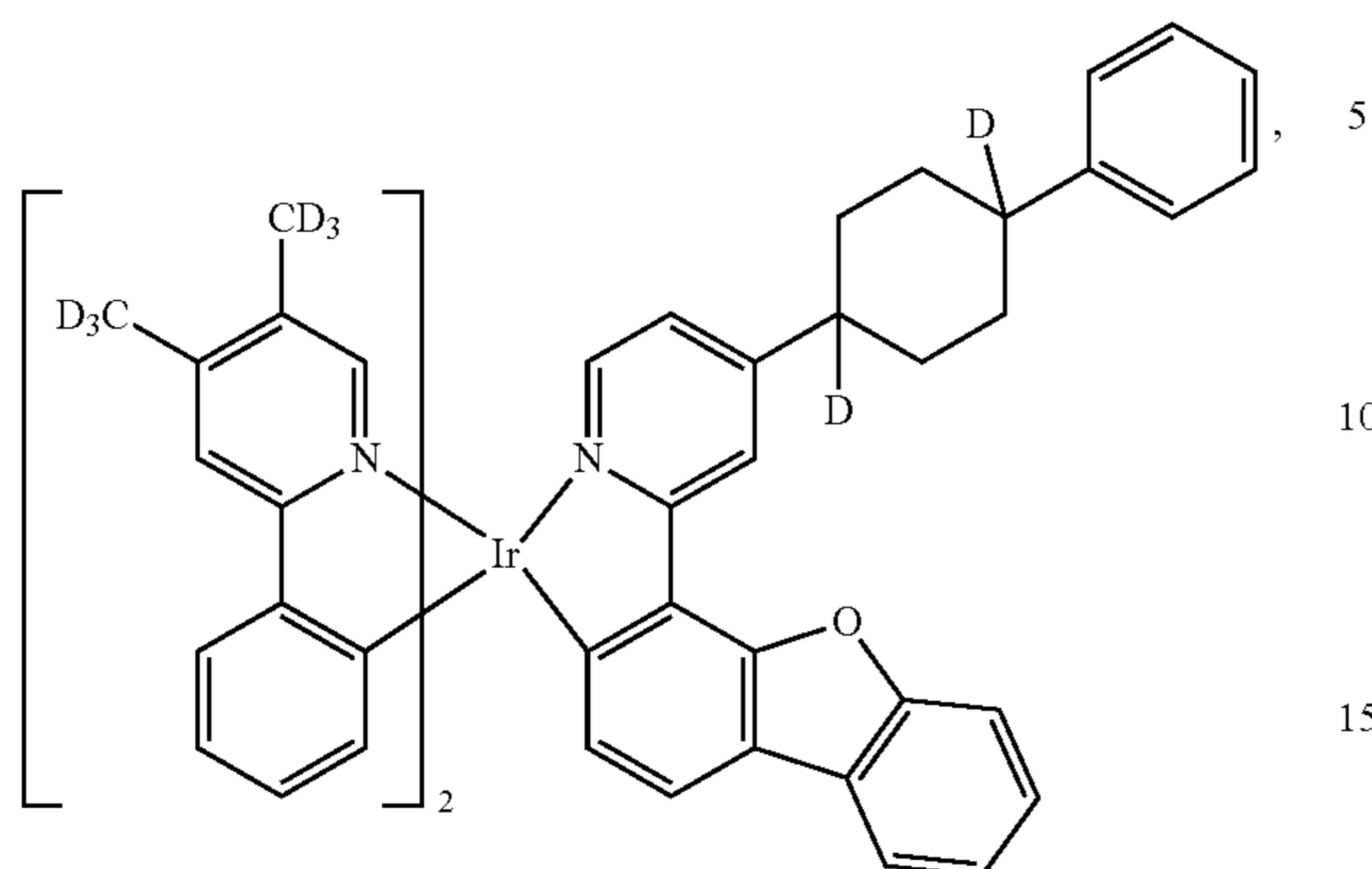
Compound 23
