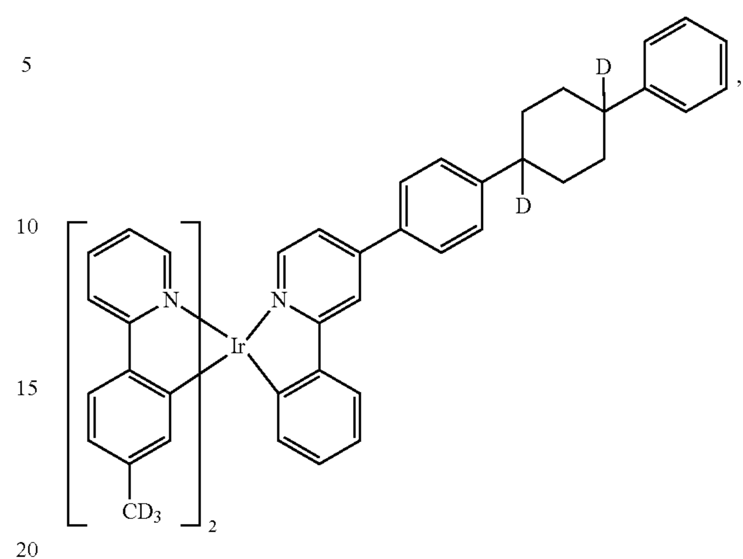
Compound 51
