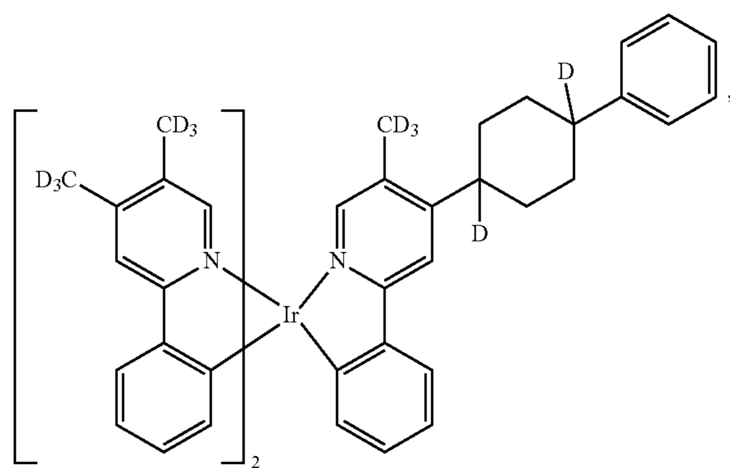
Compound 41
