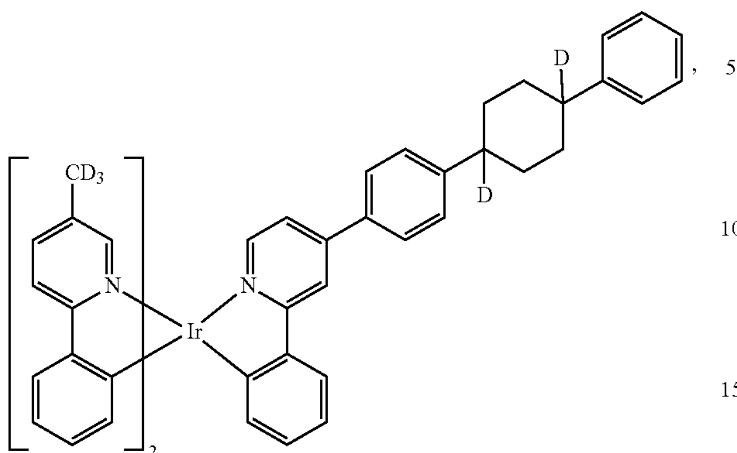
Compound 51
