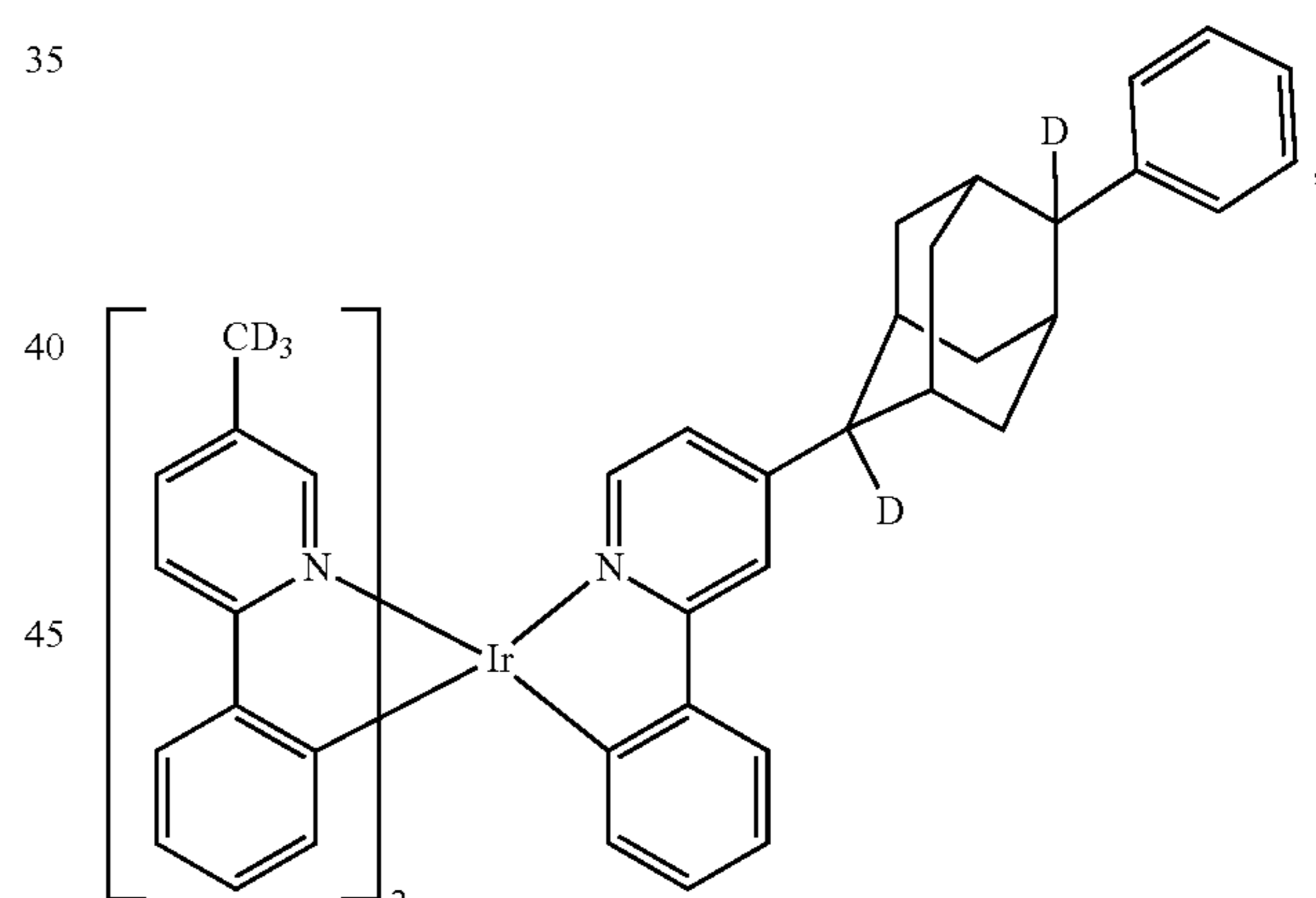
Compound 65
