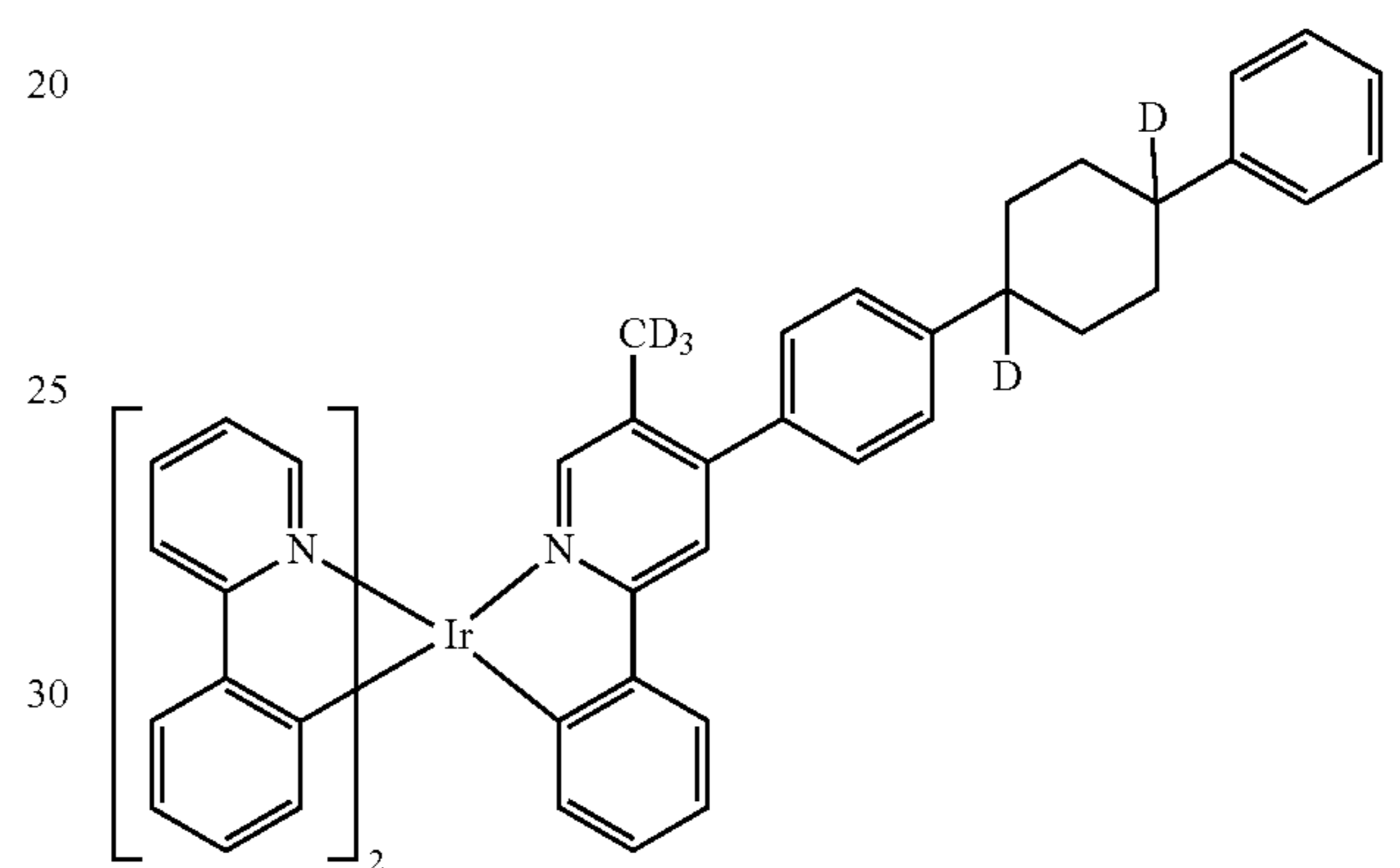
Compound 56
