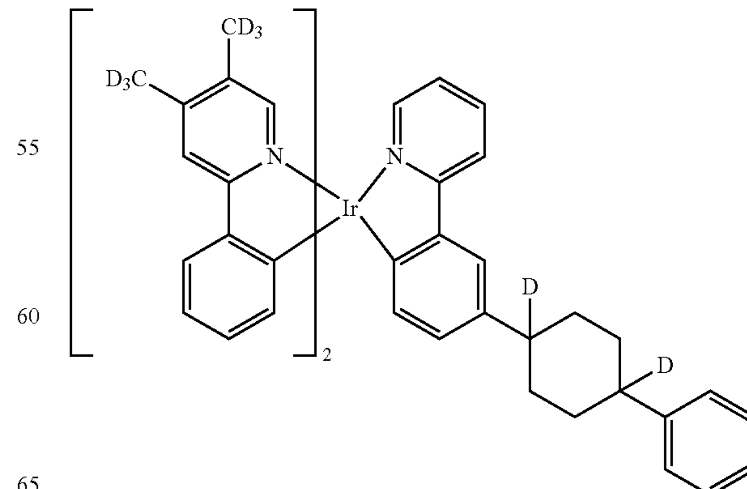
Compound 79
