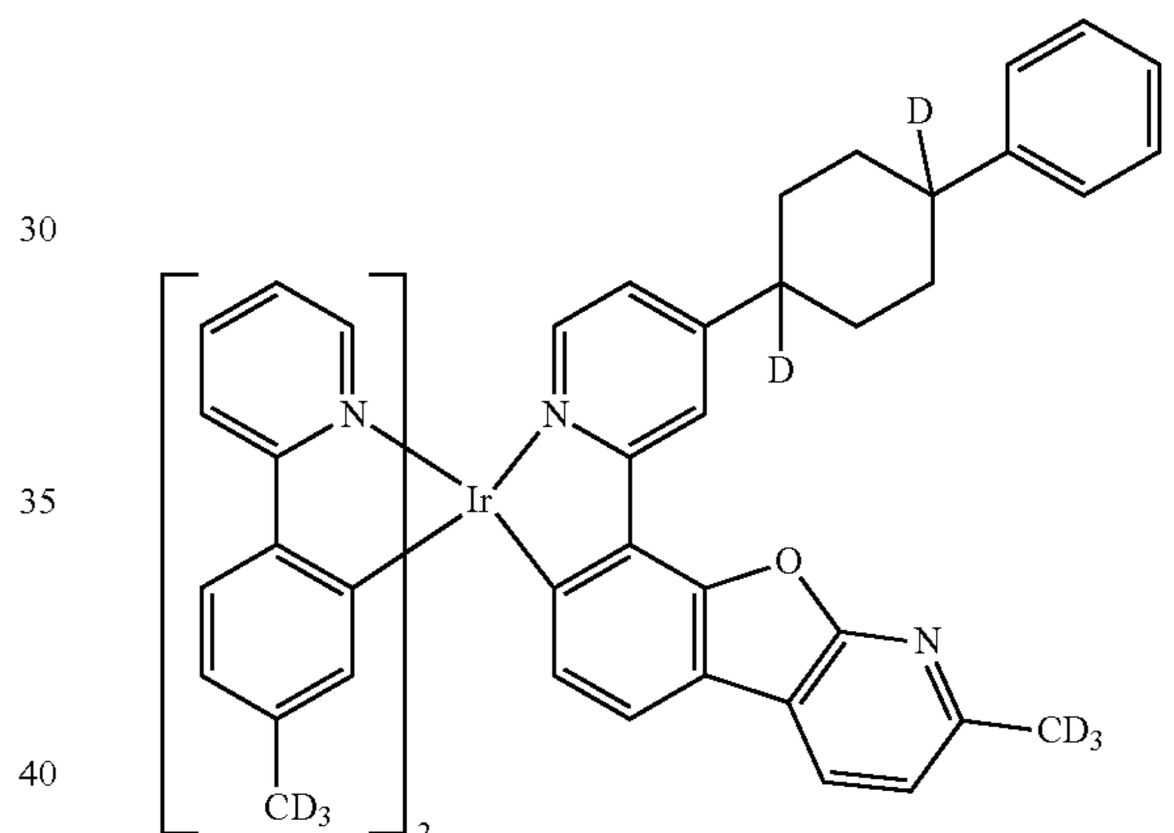
Compound 33
