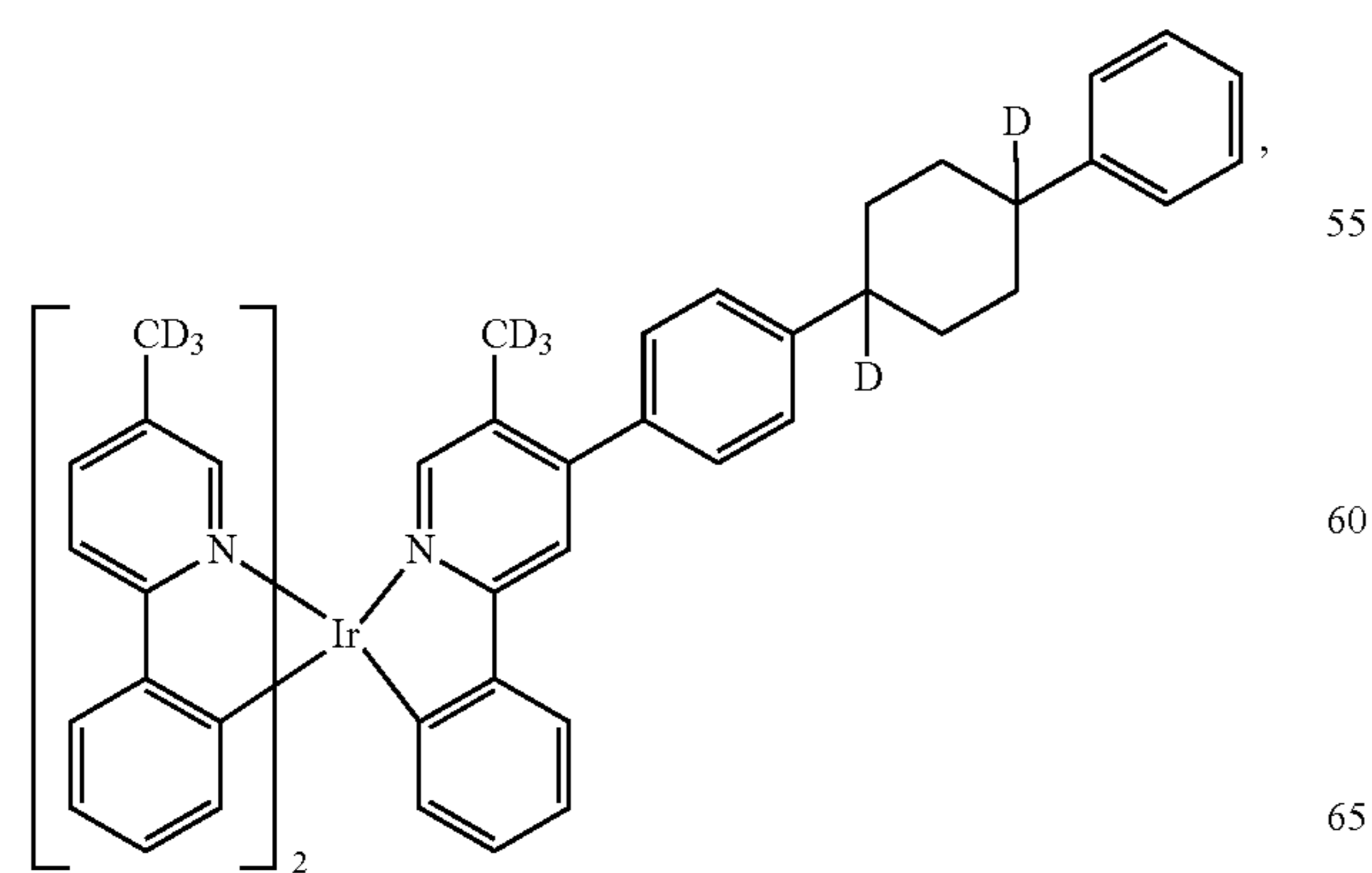
Compound 56
