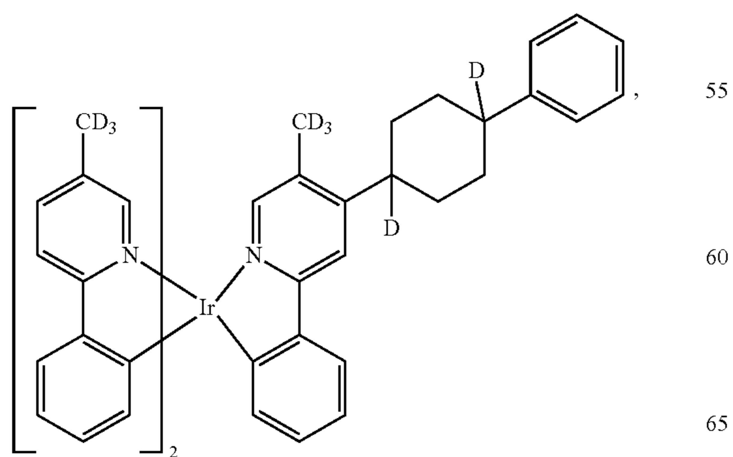
Compound 38
