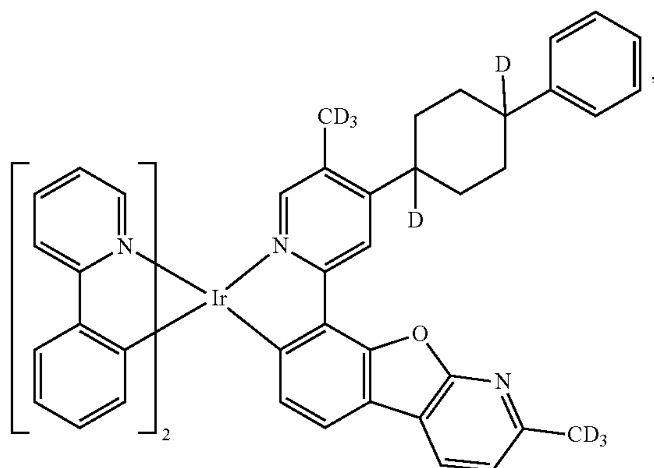
Compound 43
