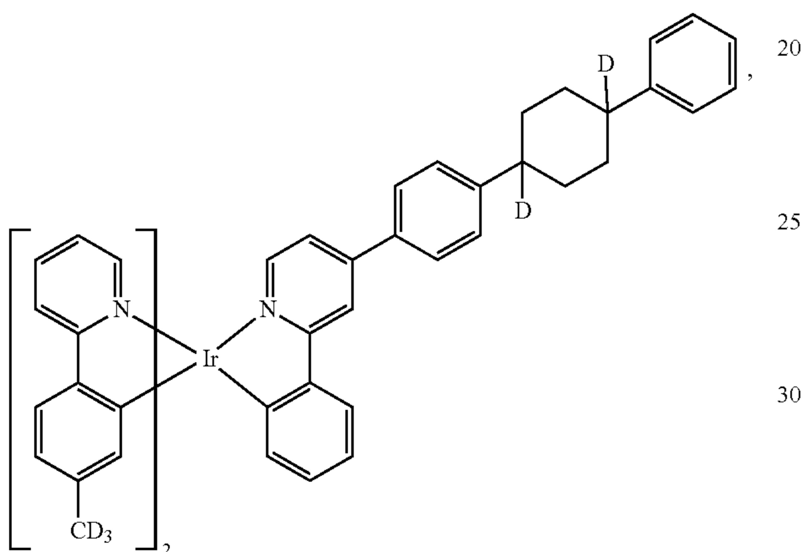
Compound 52
