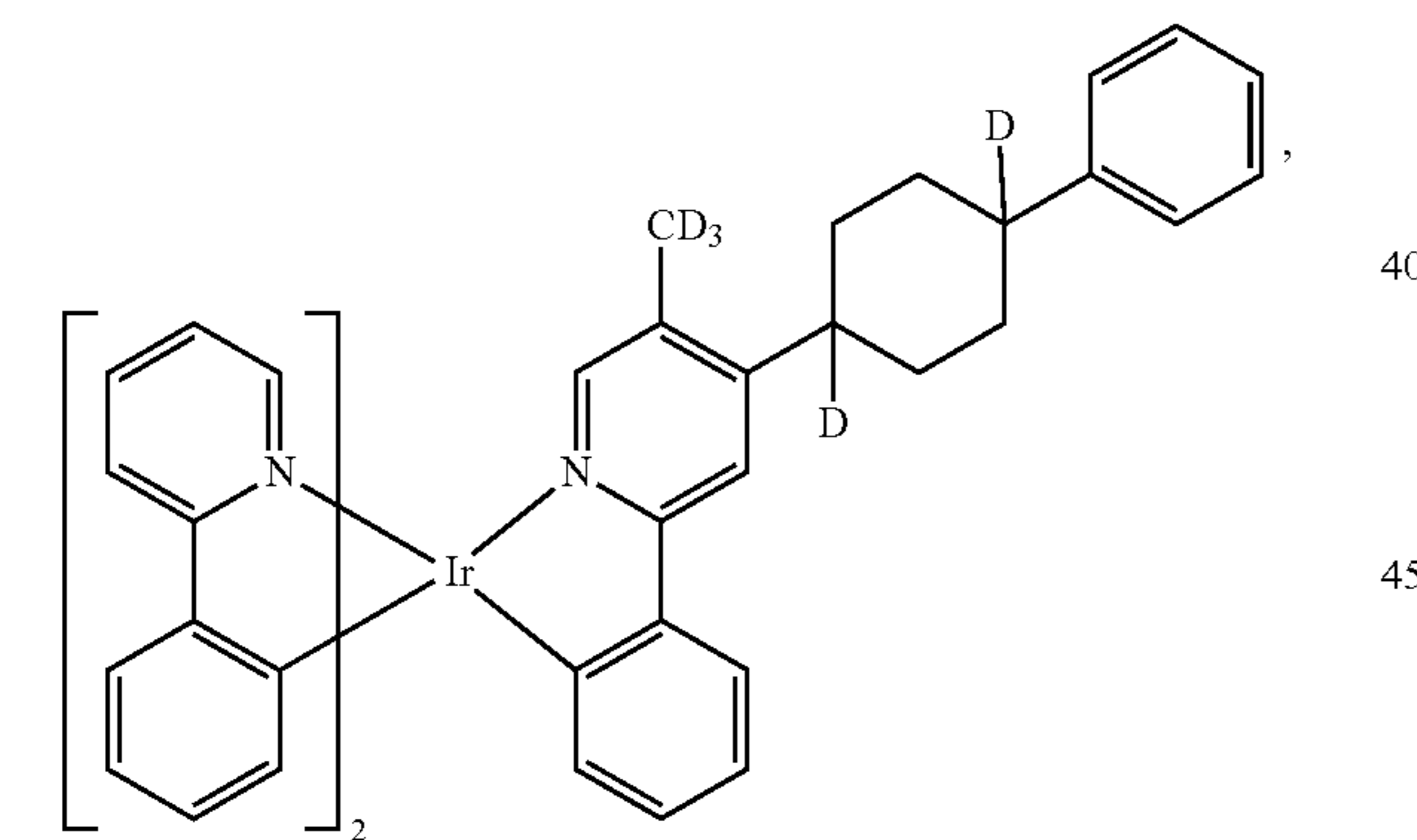
Compound 37
