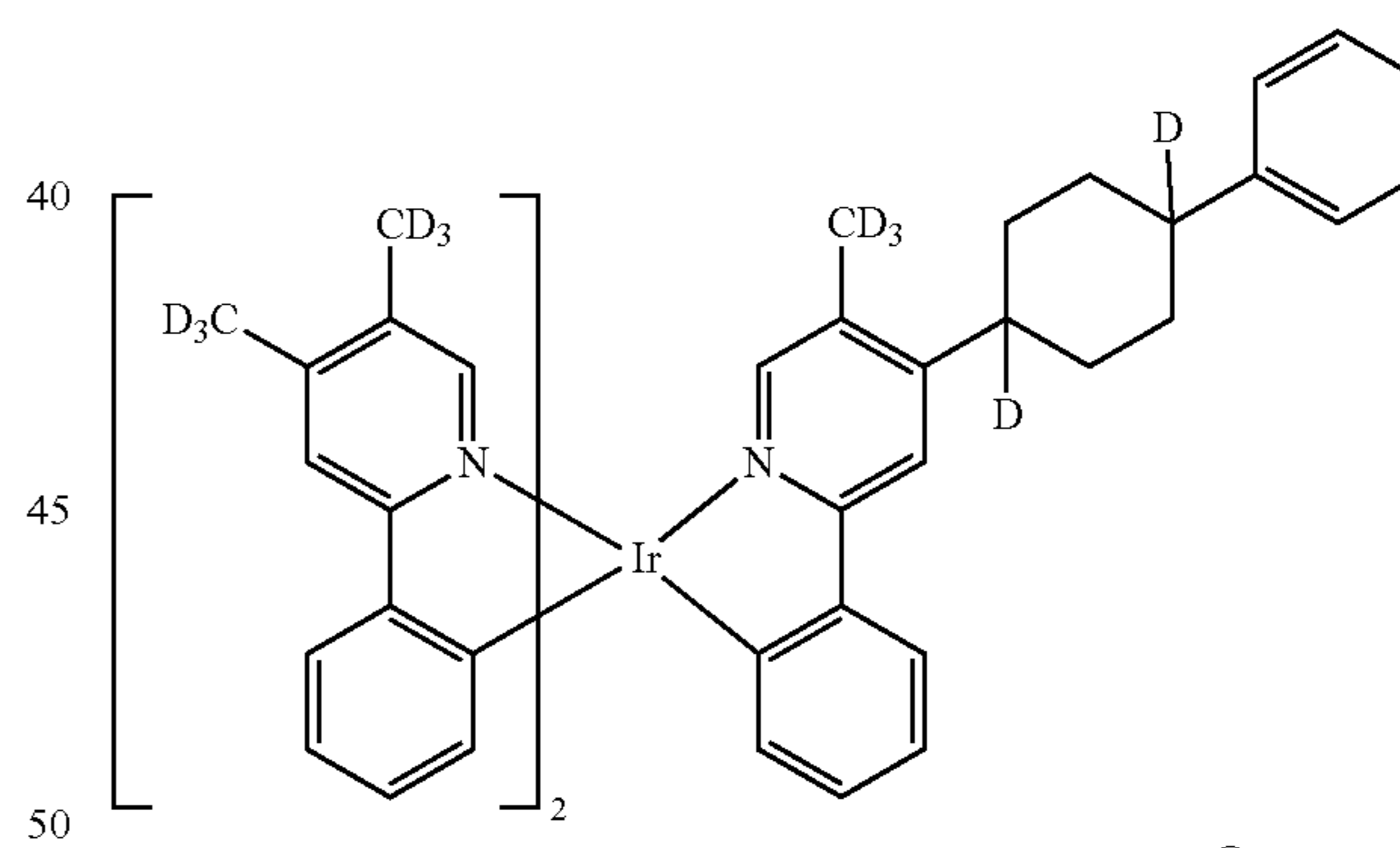
Compound 42
