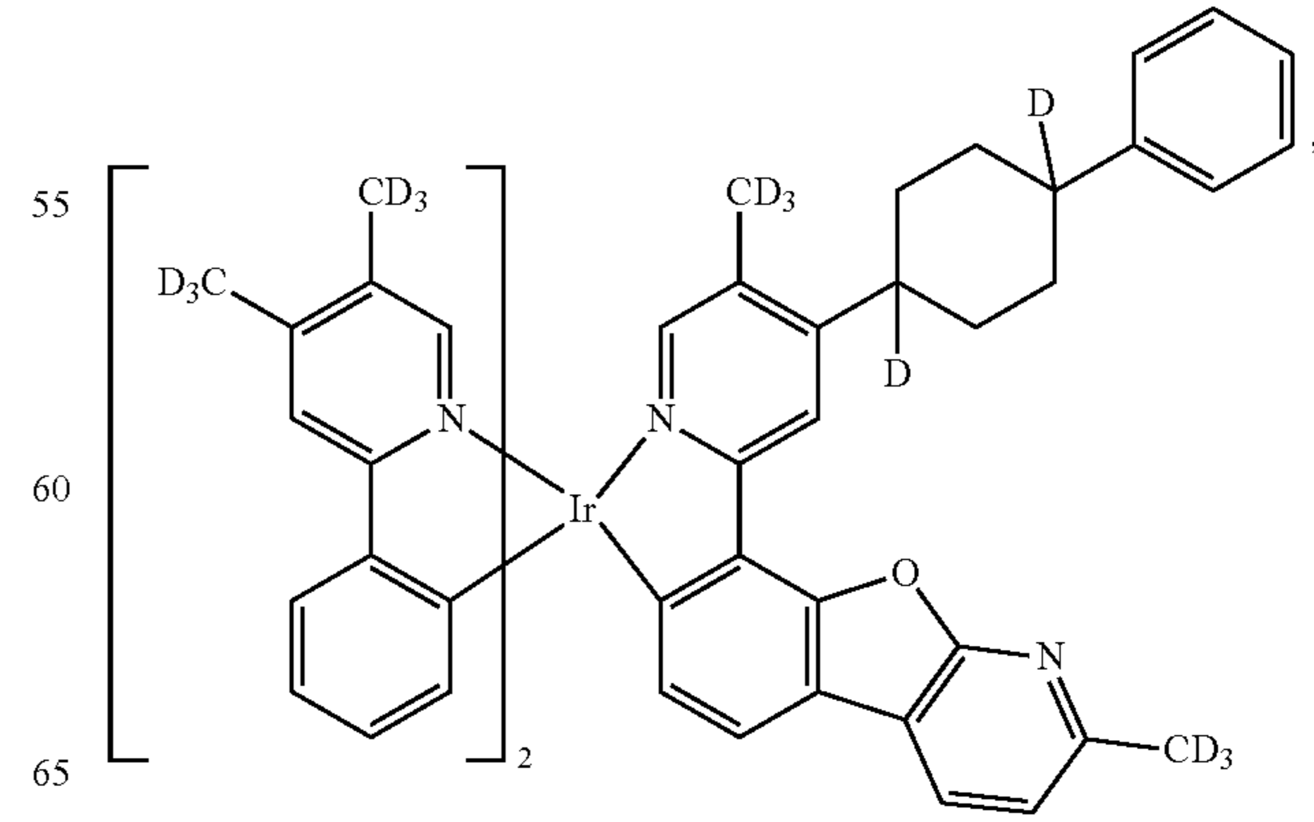
Compound 47
