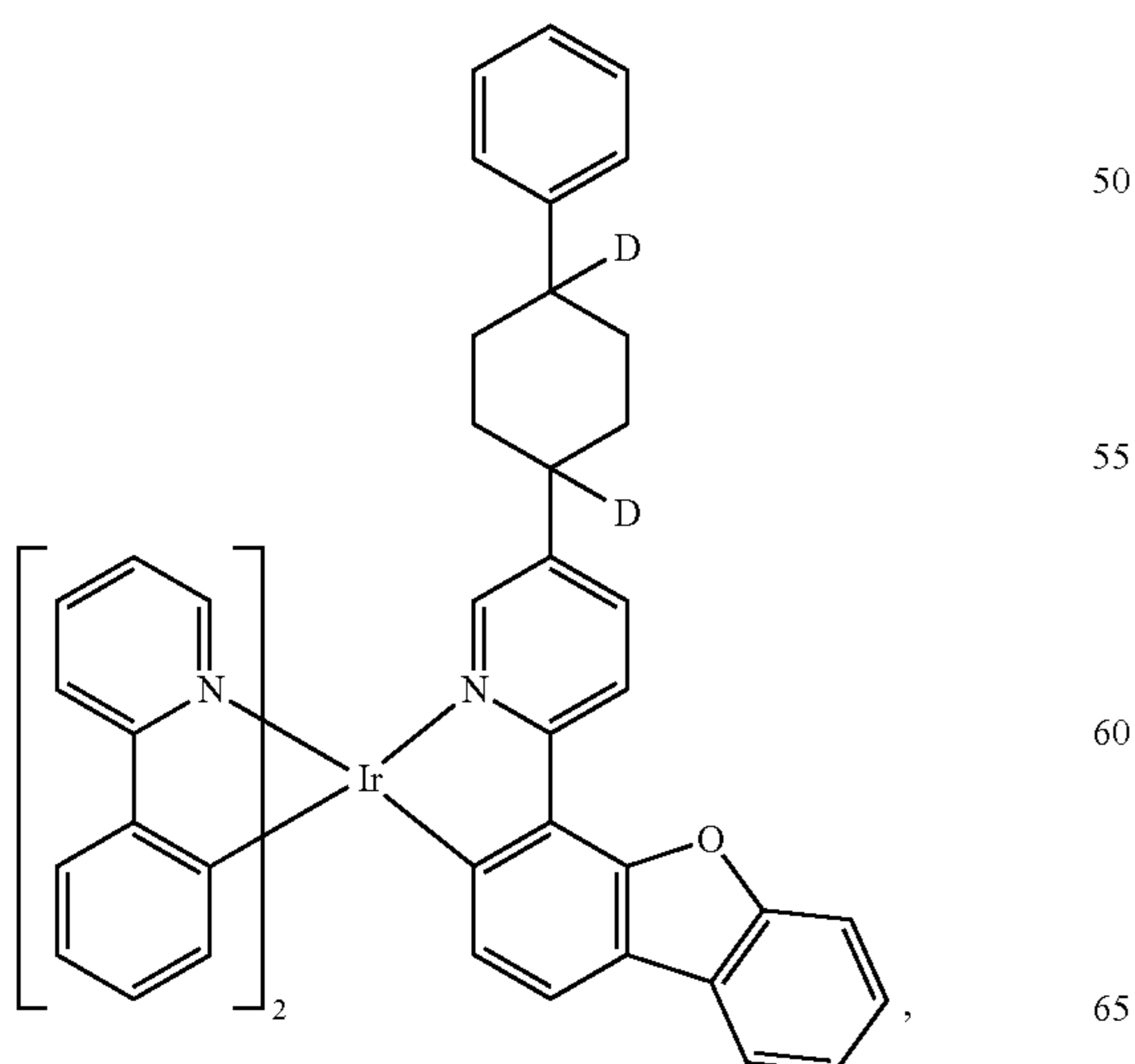
Compound 13
