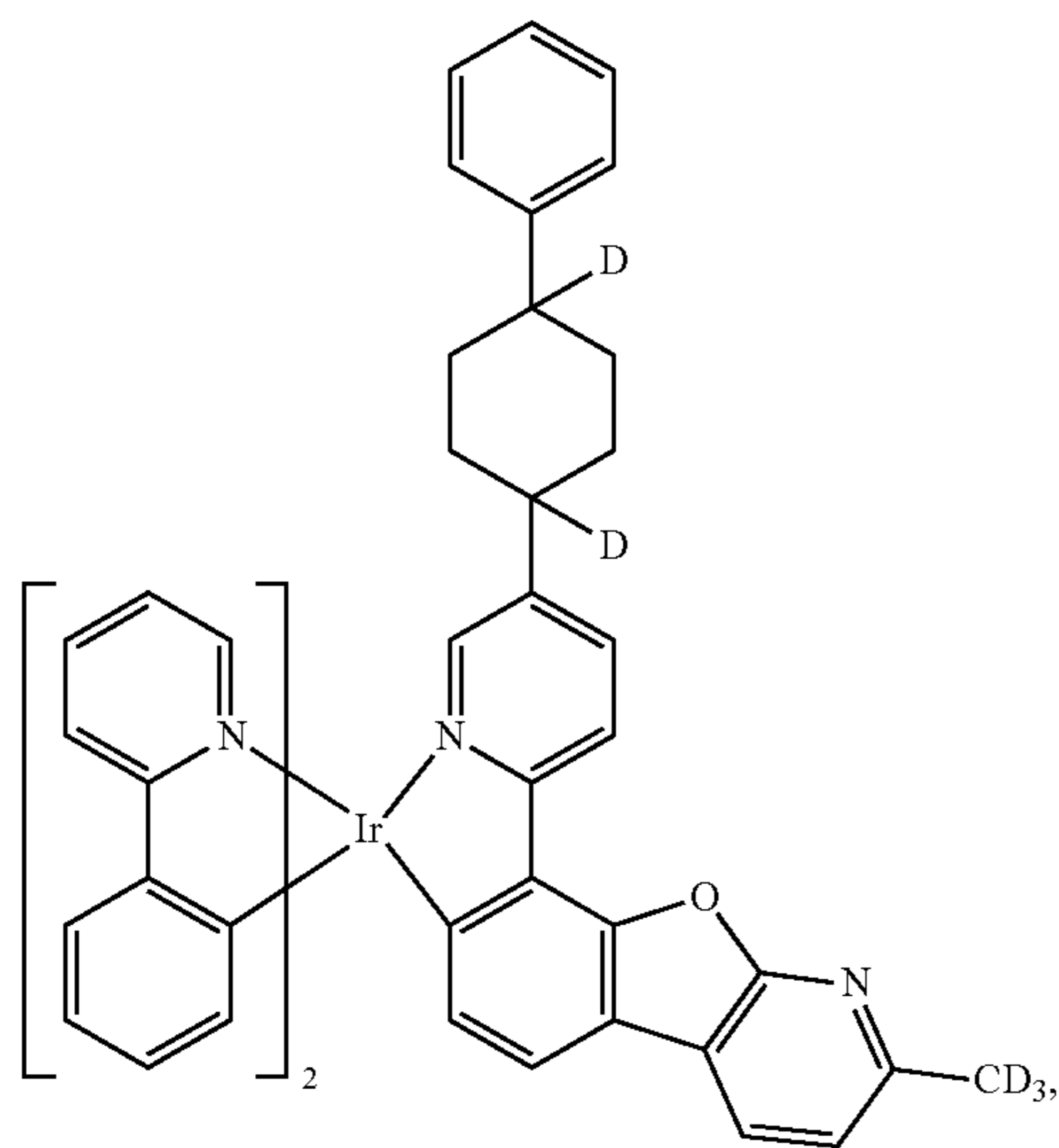
Compound 25
