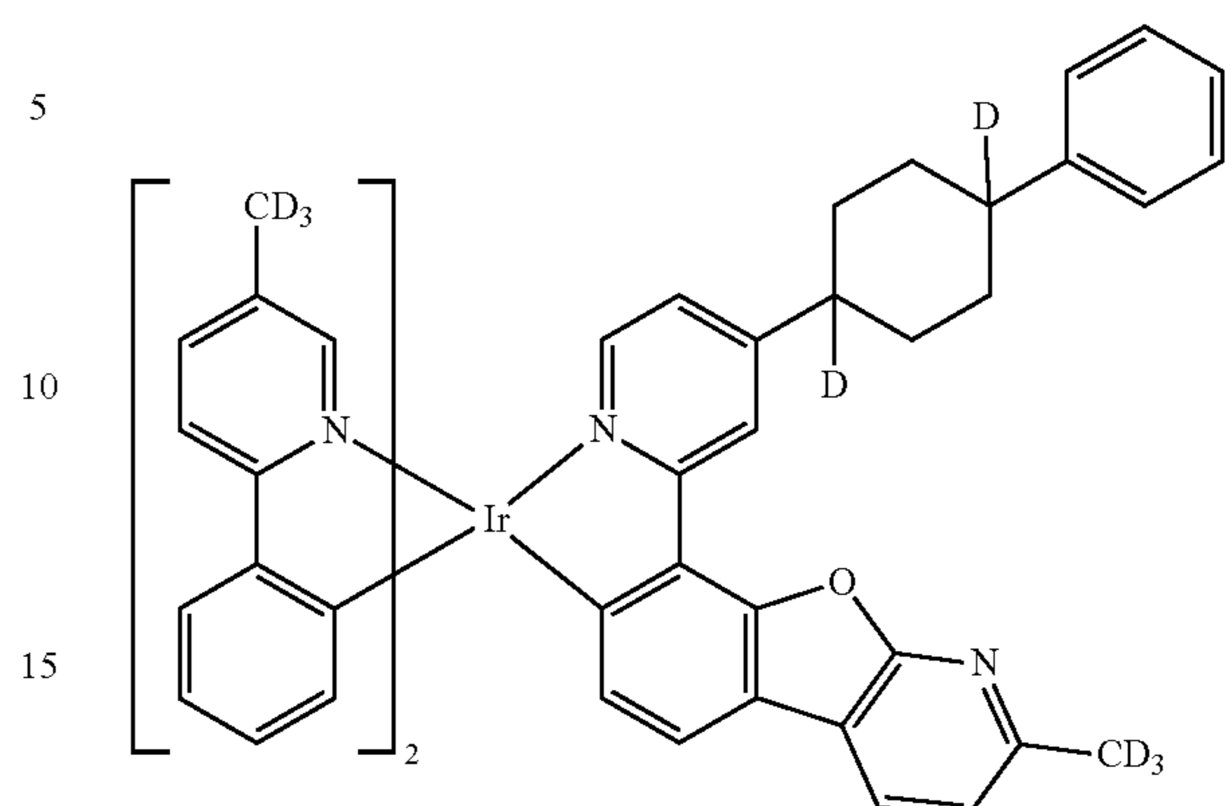
Compound 32
