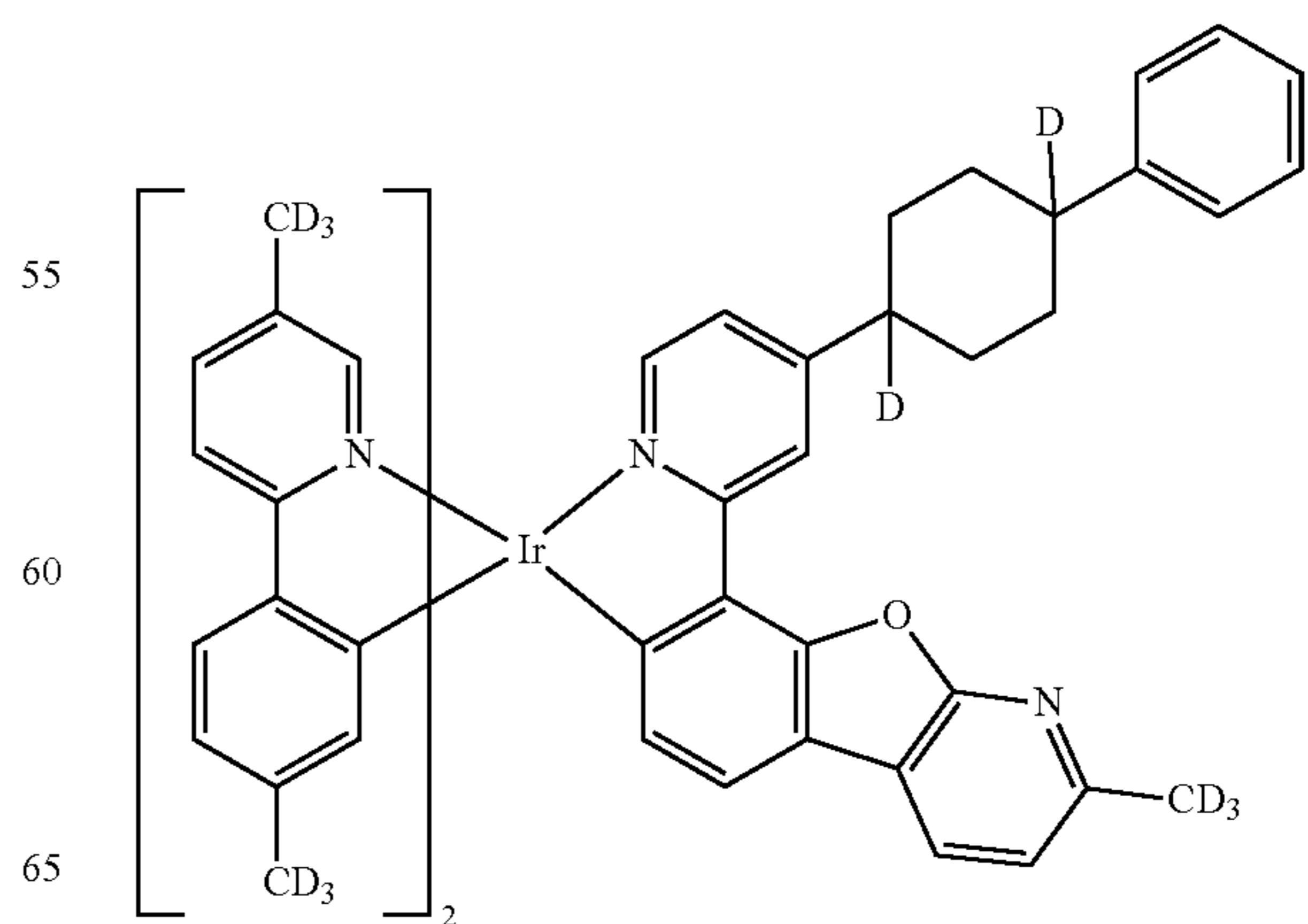
Compound 34
