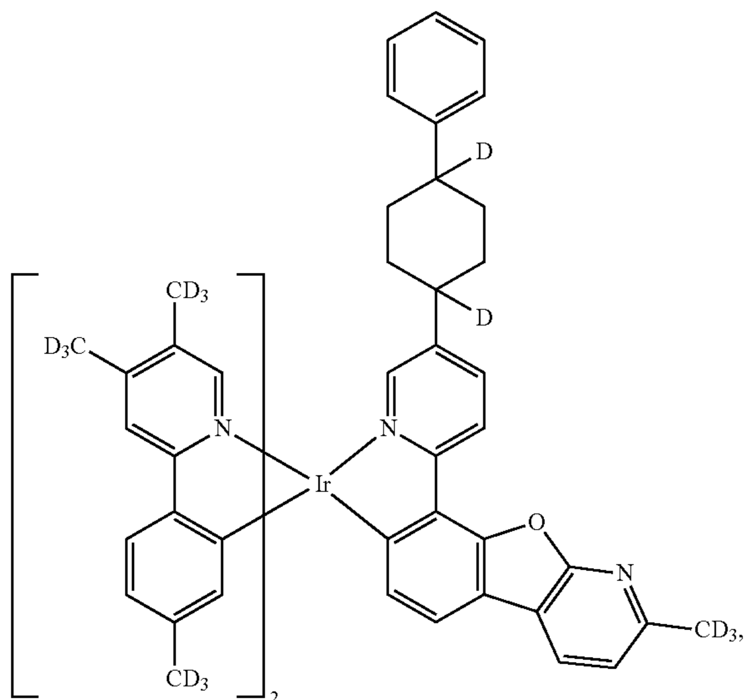
Compound 30
