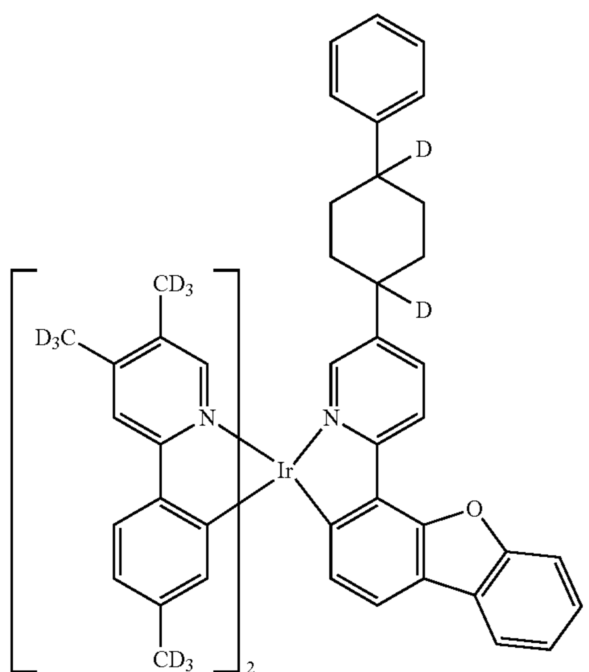
Compound 18
