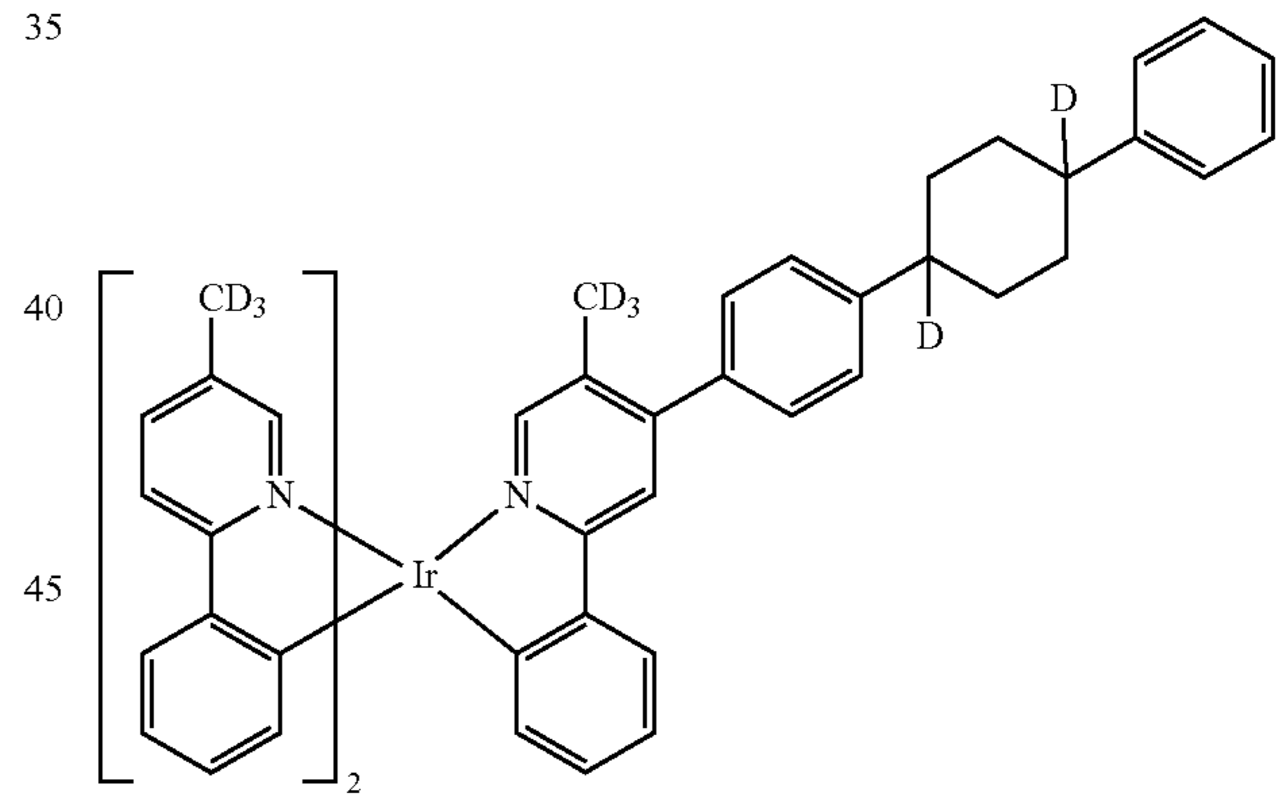
Compound 57
