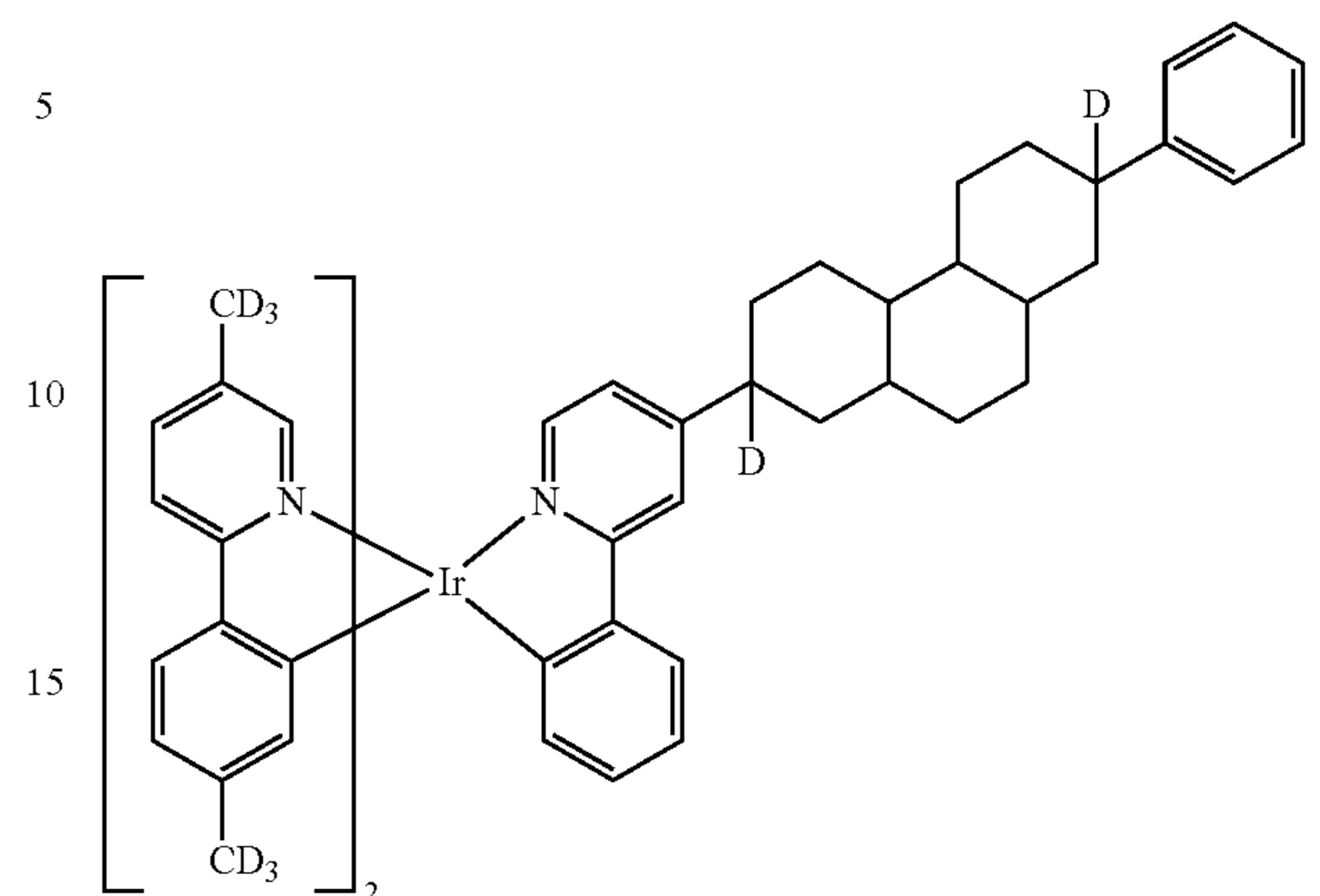
Compound 63
