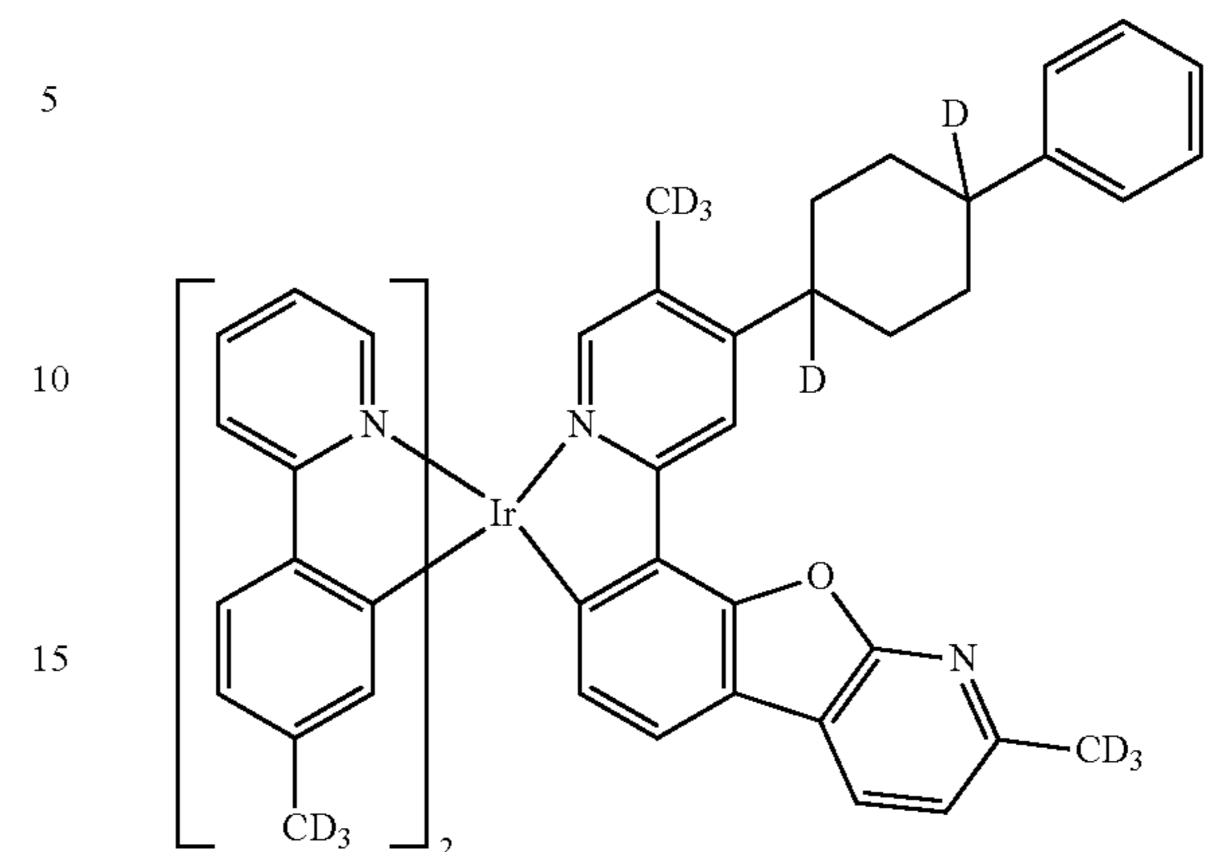
Compound 45
