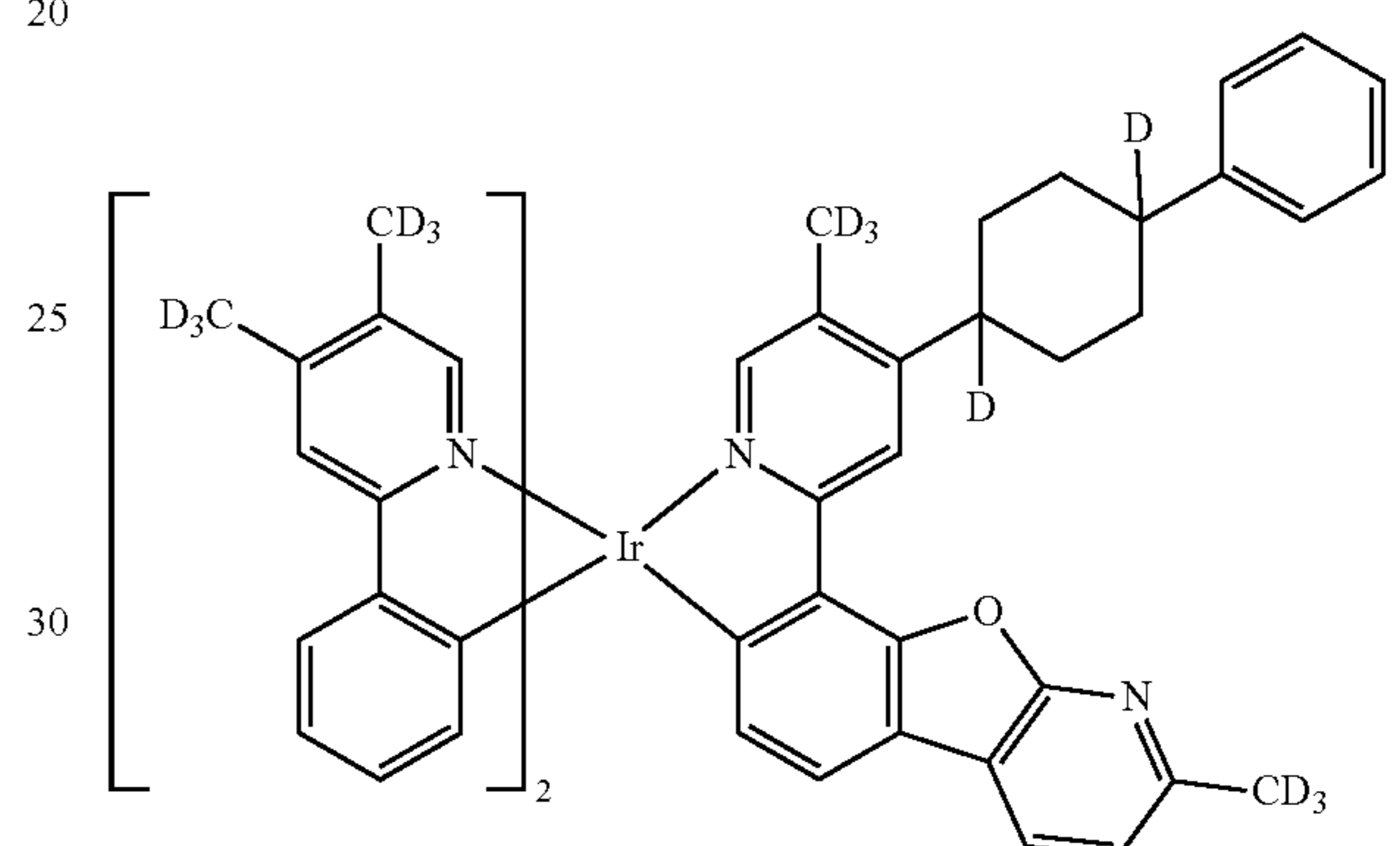
Compound 48
