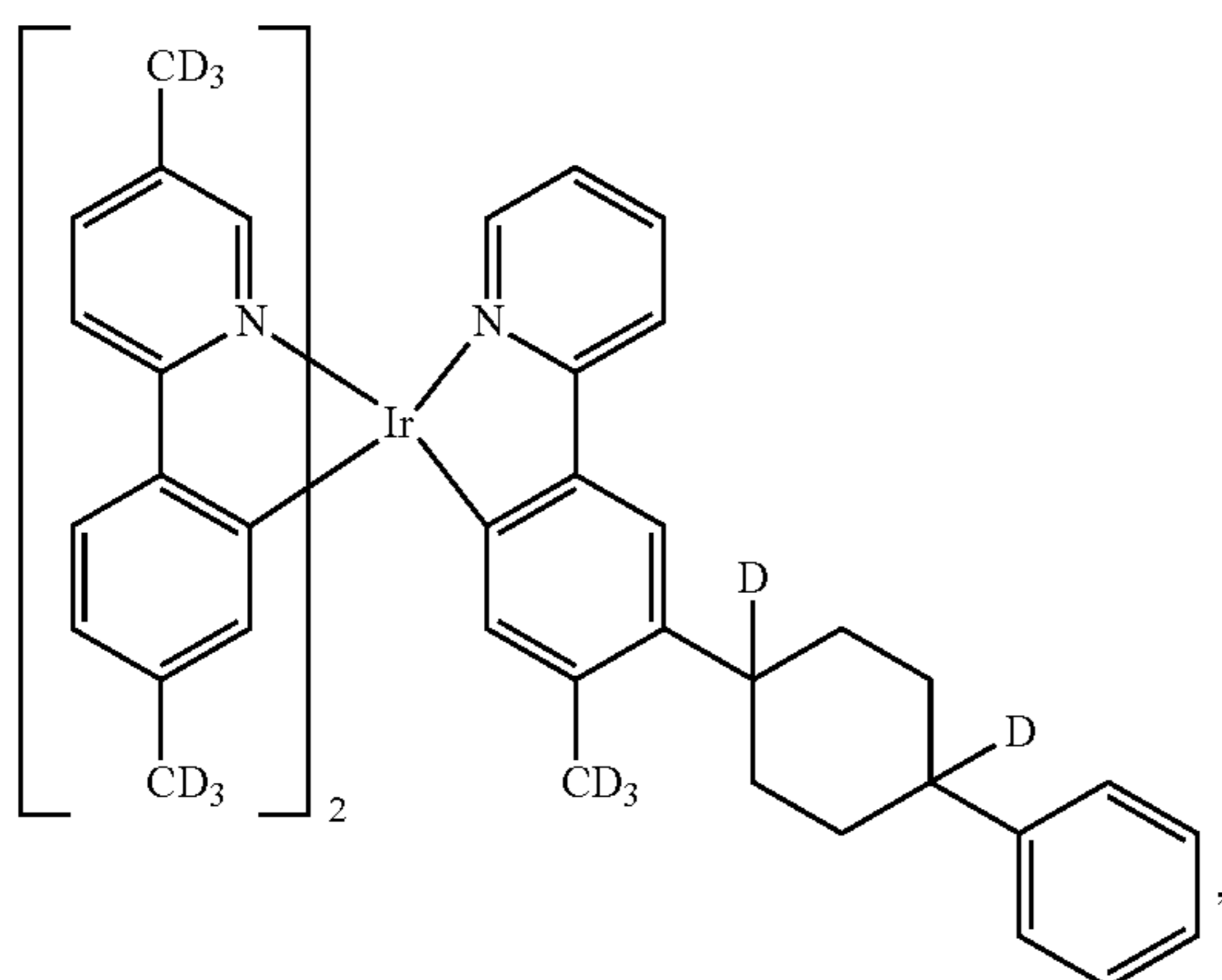
Compound 75
