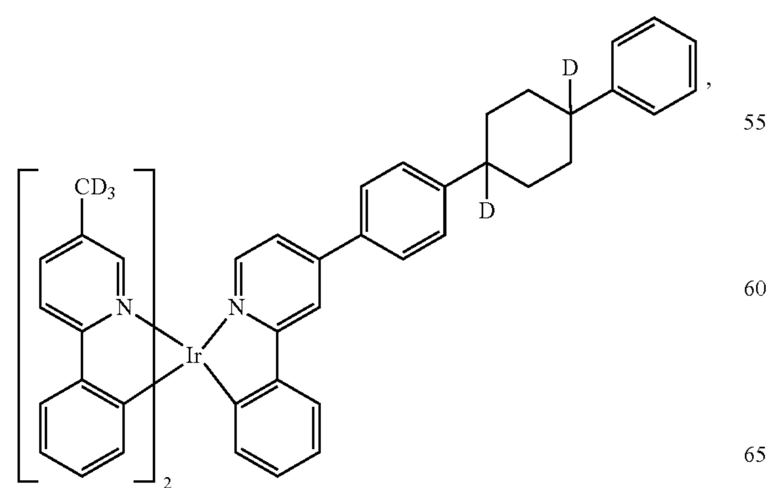
Compound 50
