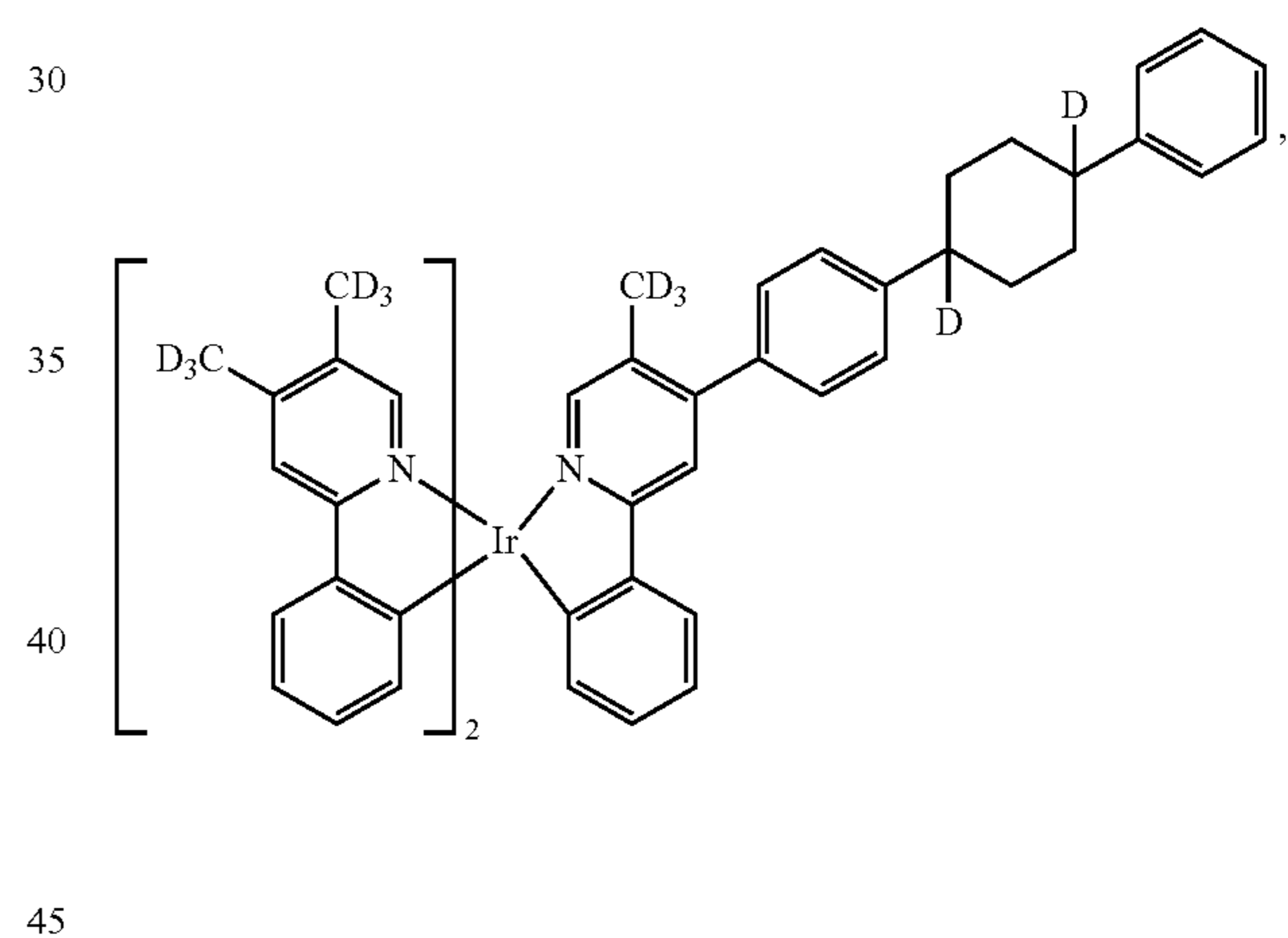
Compound 58
