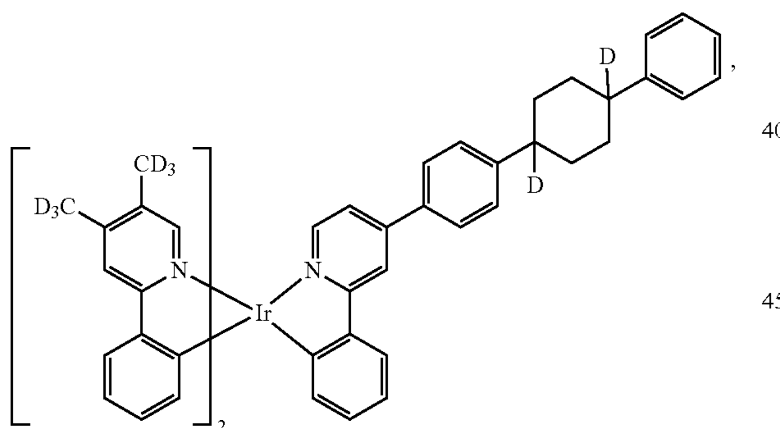
Compound 53
