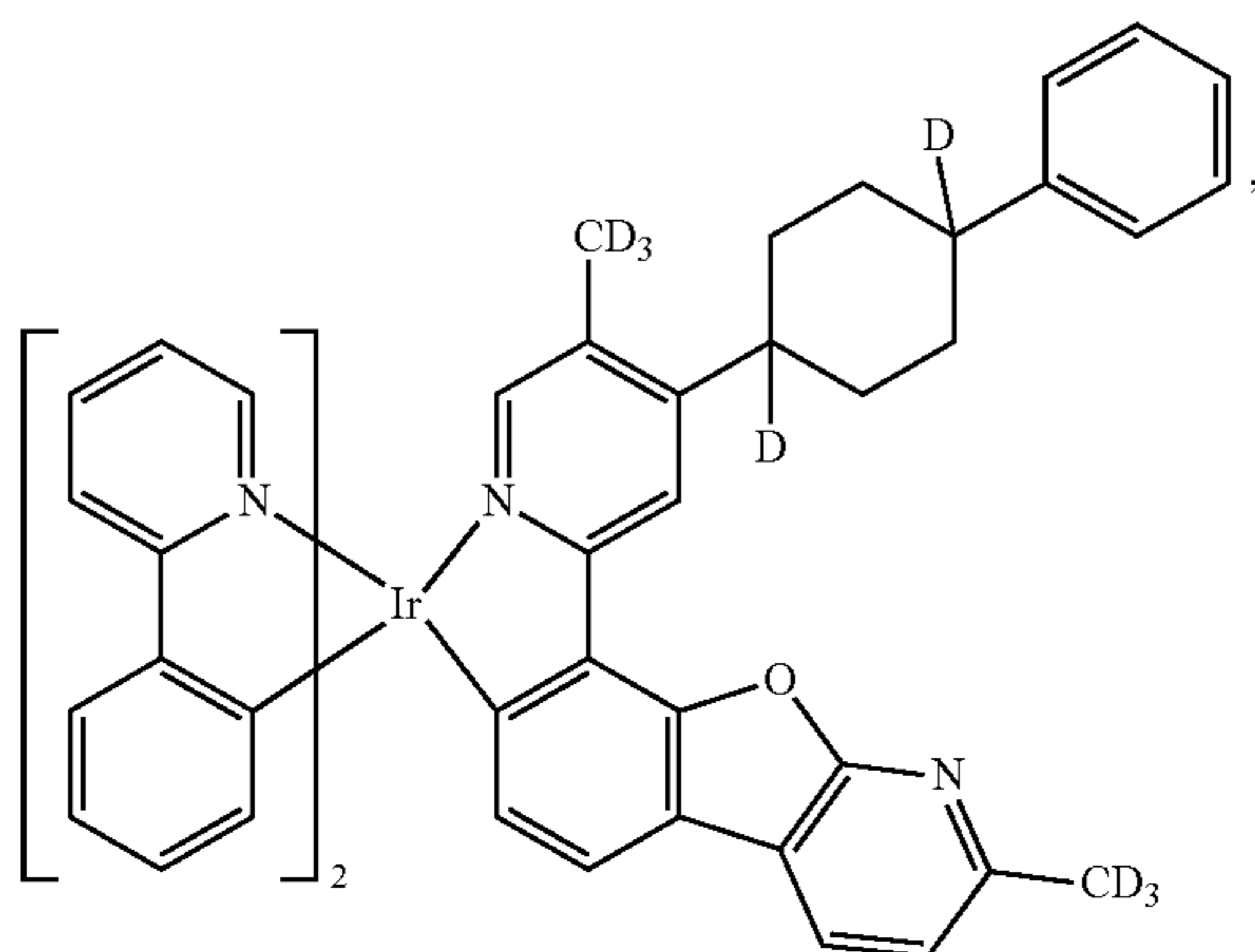
Compound 43
