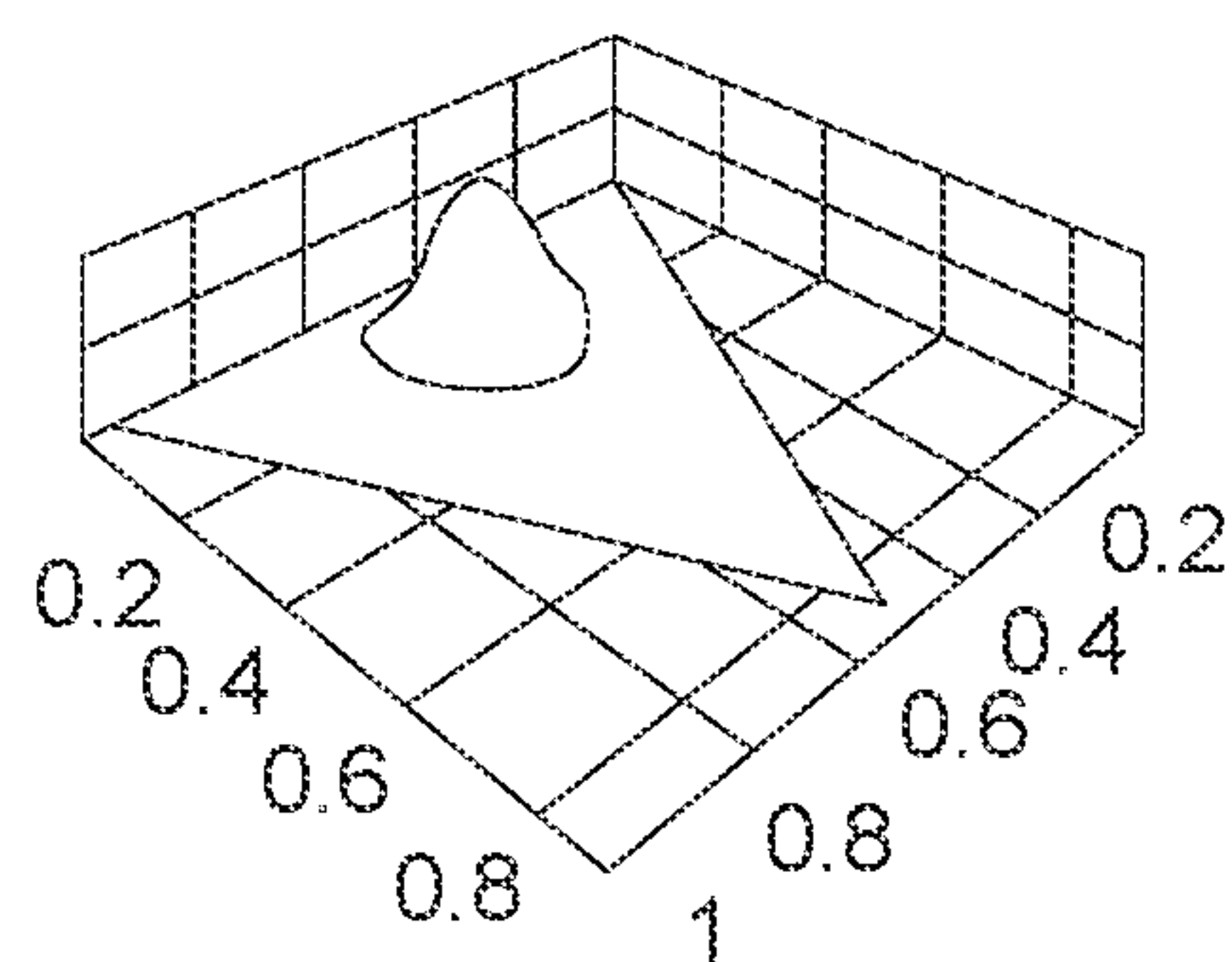
p(y_2|\alpha_2) DISTRIBUTION
