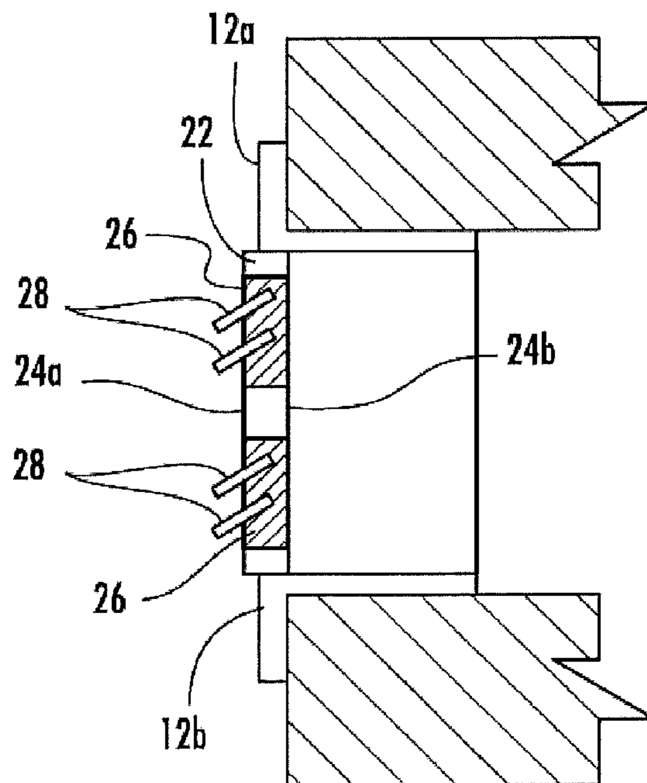
FIG. 2D
