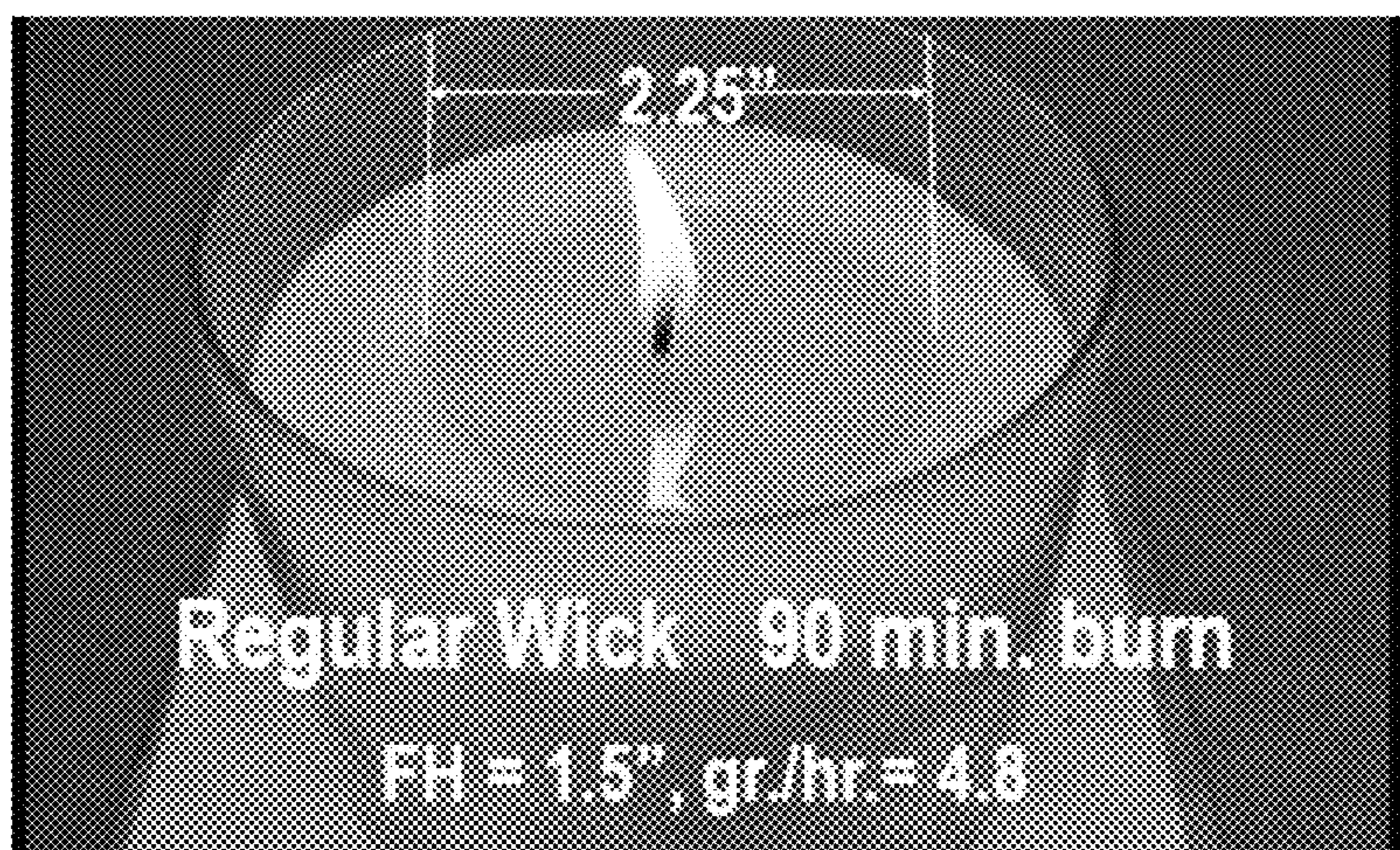
FIG. 6C (Prior Art)
