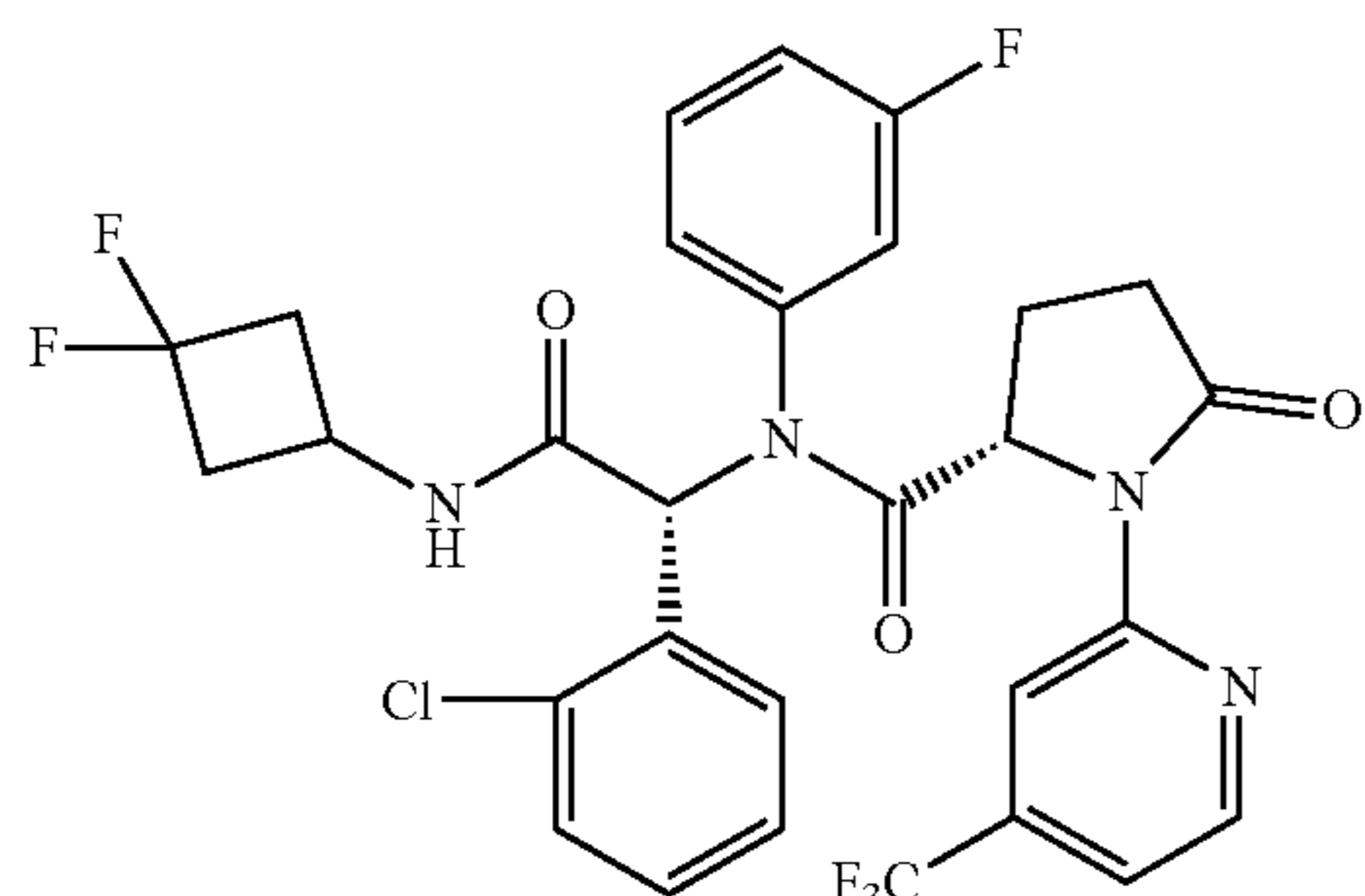
Compound 39
