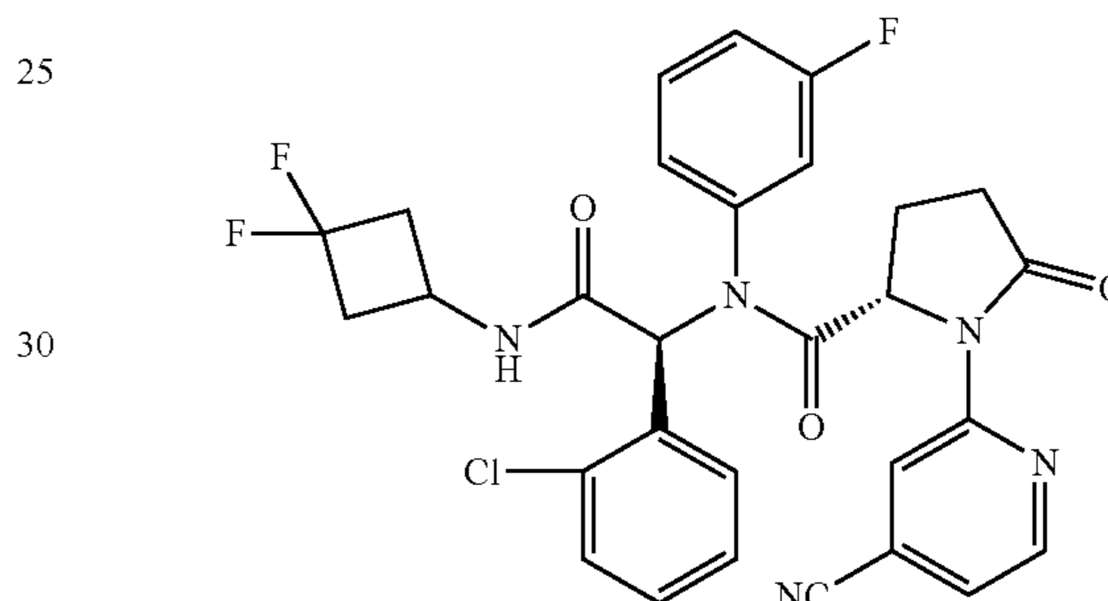
Compound 37
