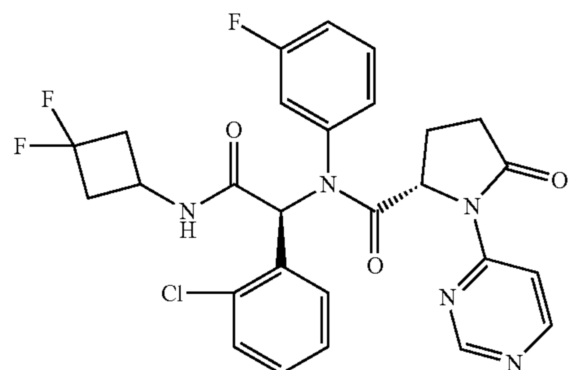
Compound 22 50
