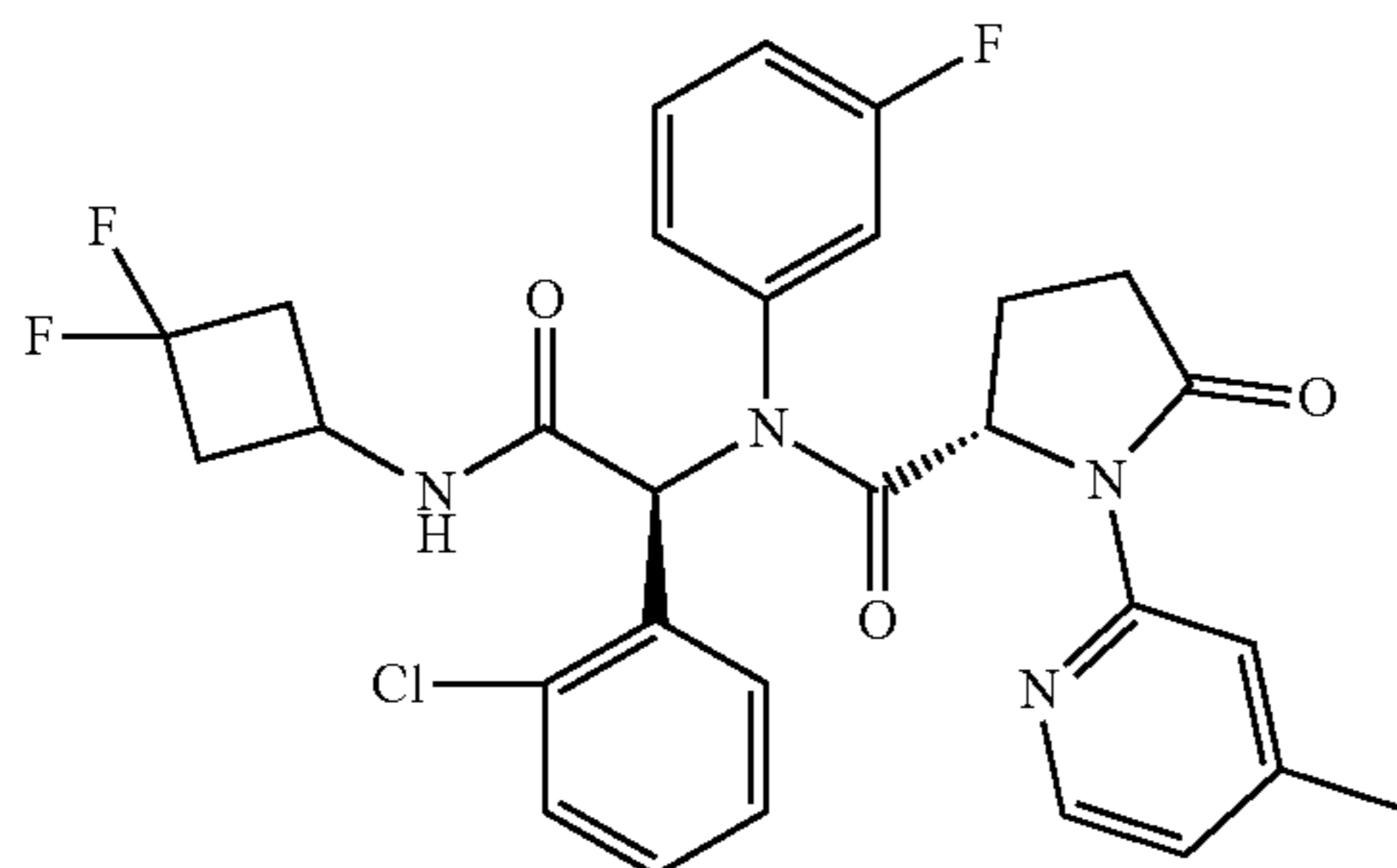
Compound 27
