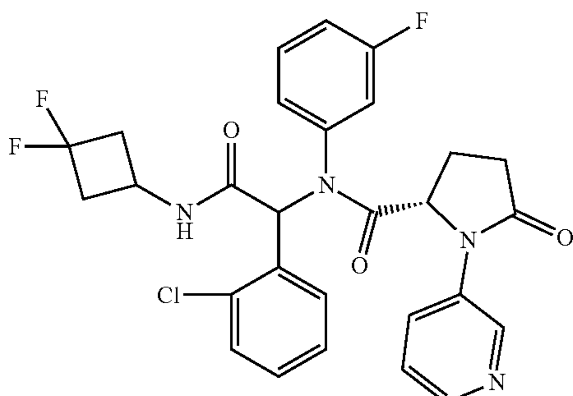
Compound 10
