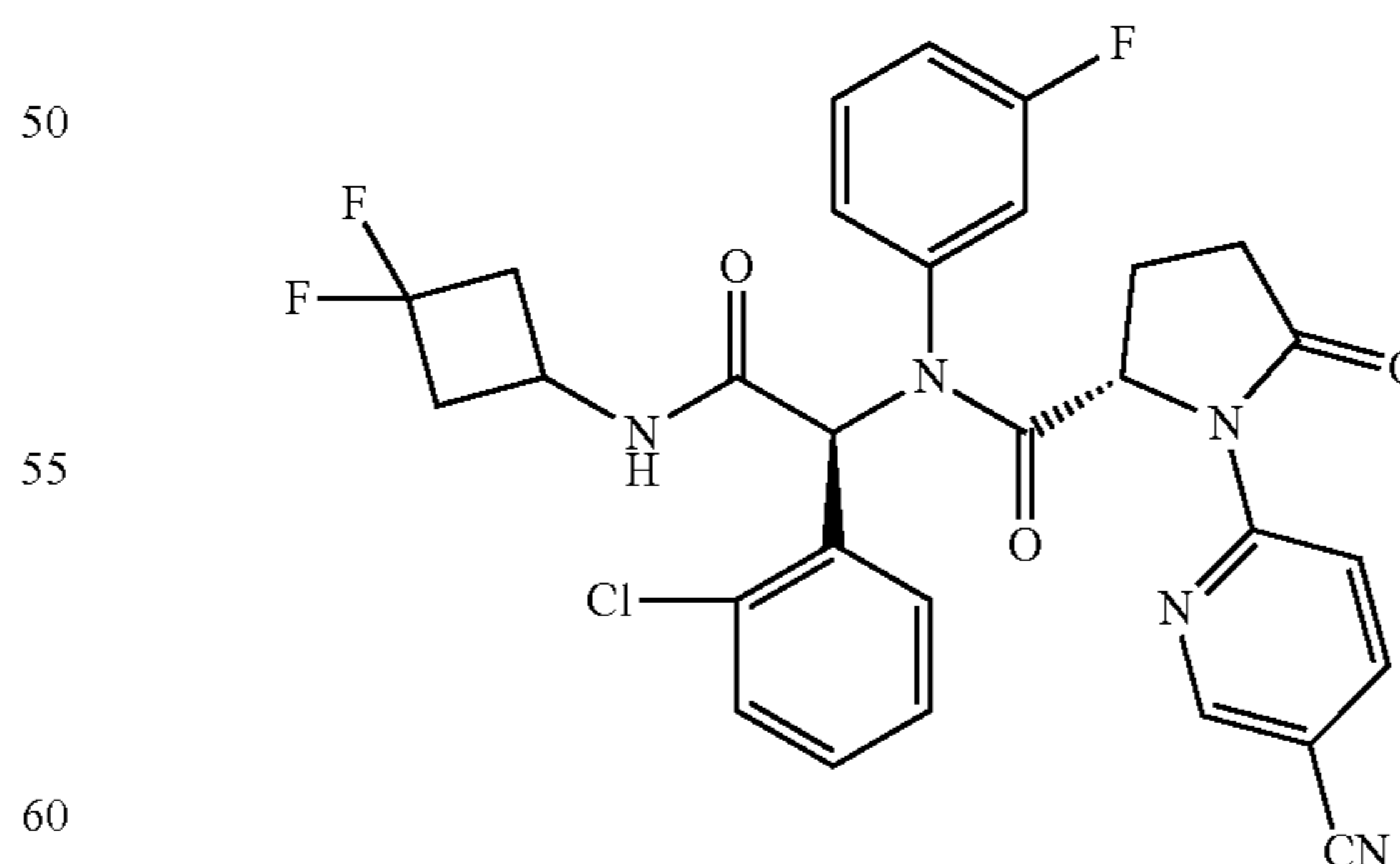
Compound 47
