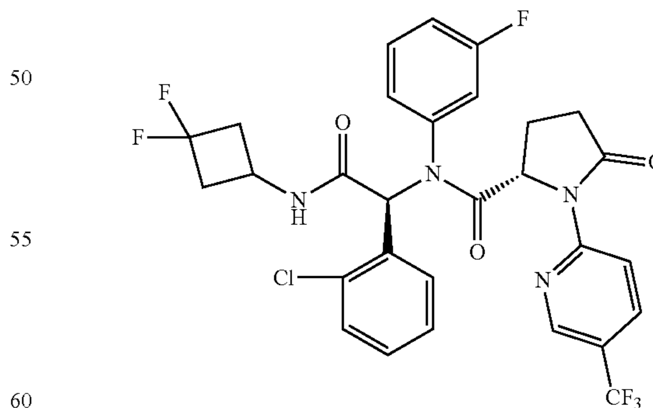
Compound 31
