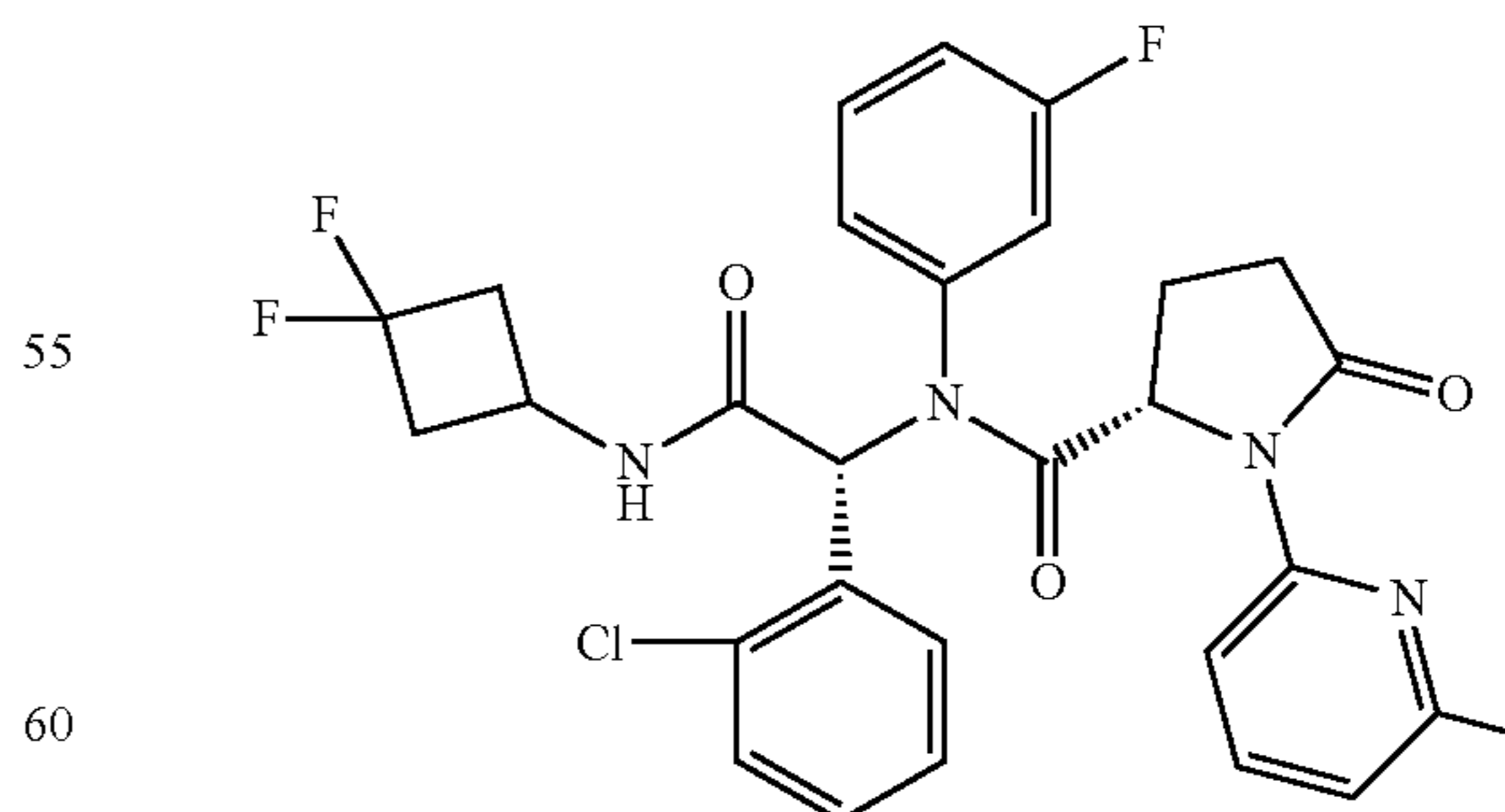
Compound 34
