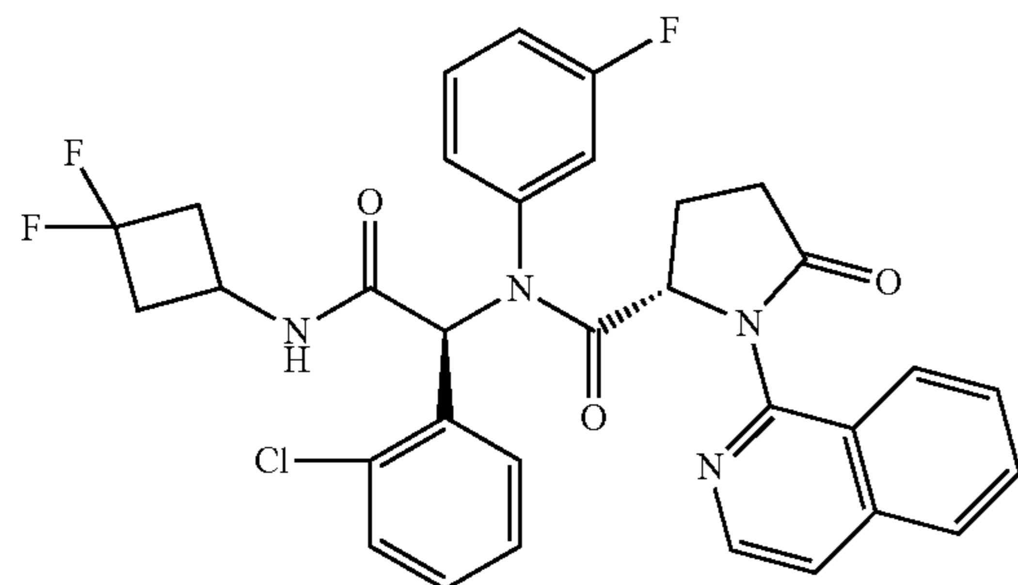
Compound 16
