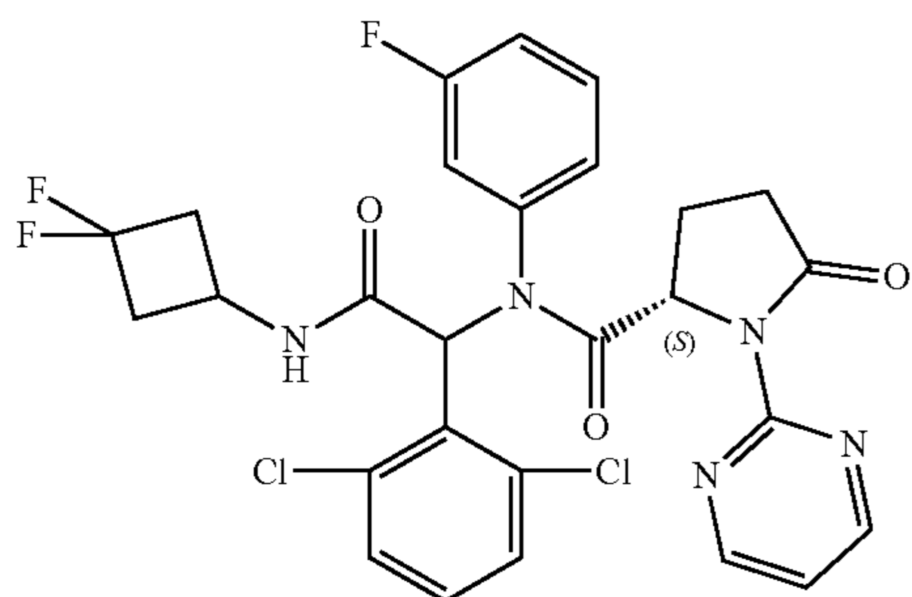
Compound 51
