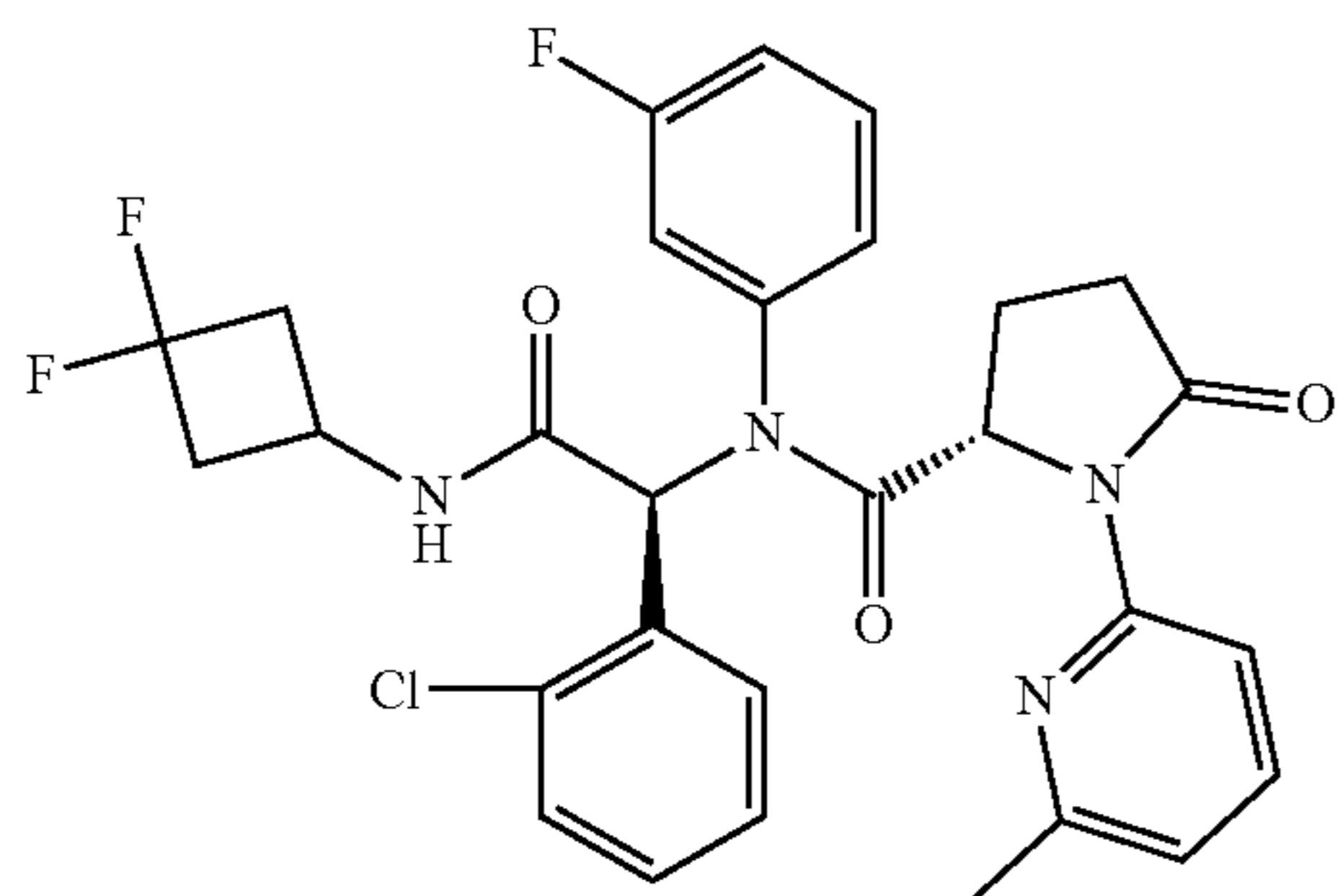
Compound 28
