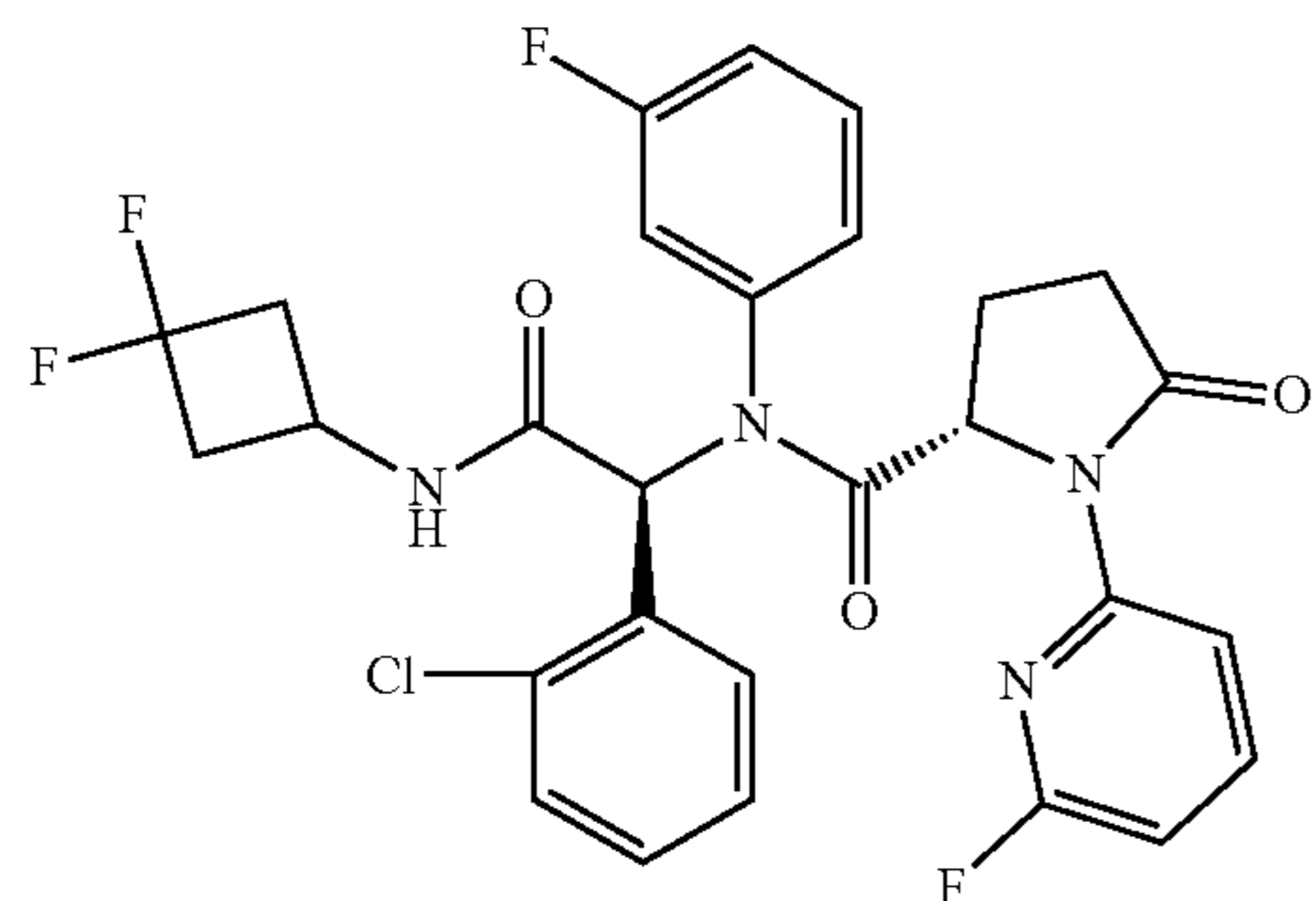
Compound 11
