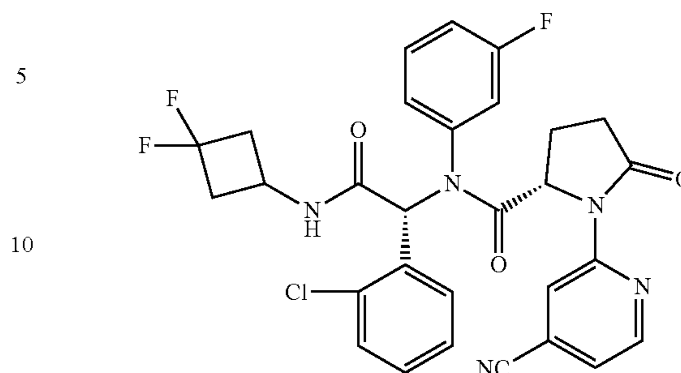
Compound 36
