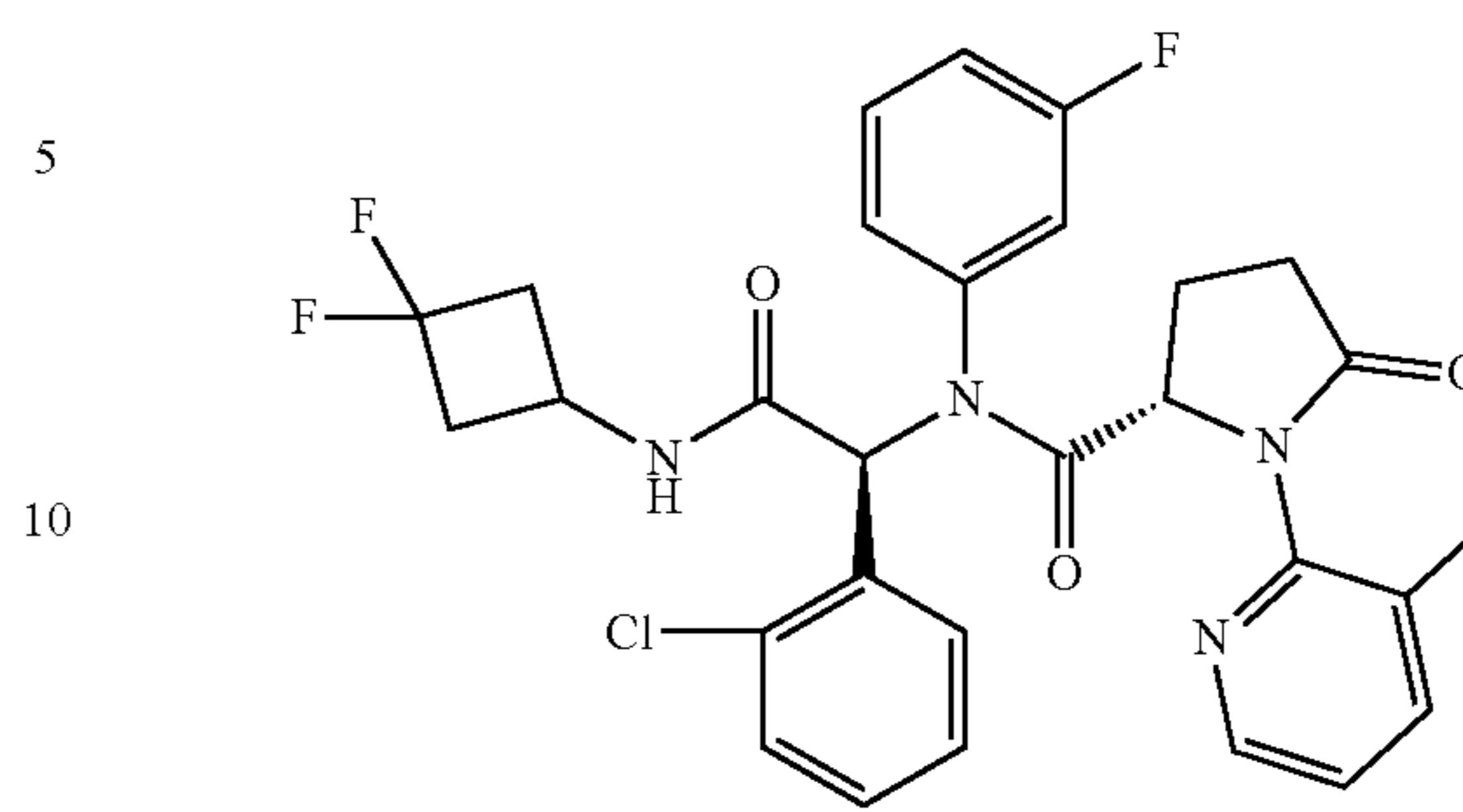
Compound 15
