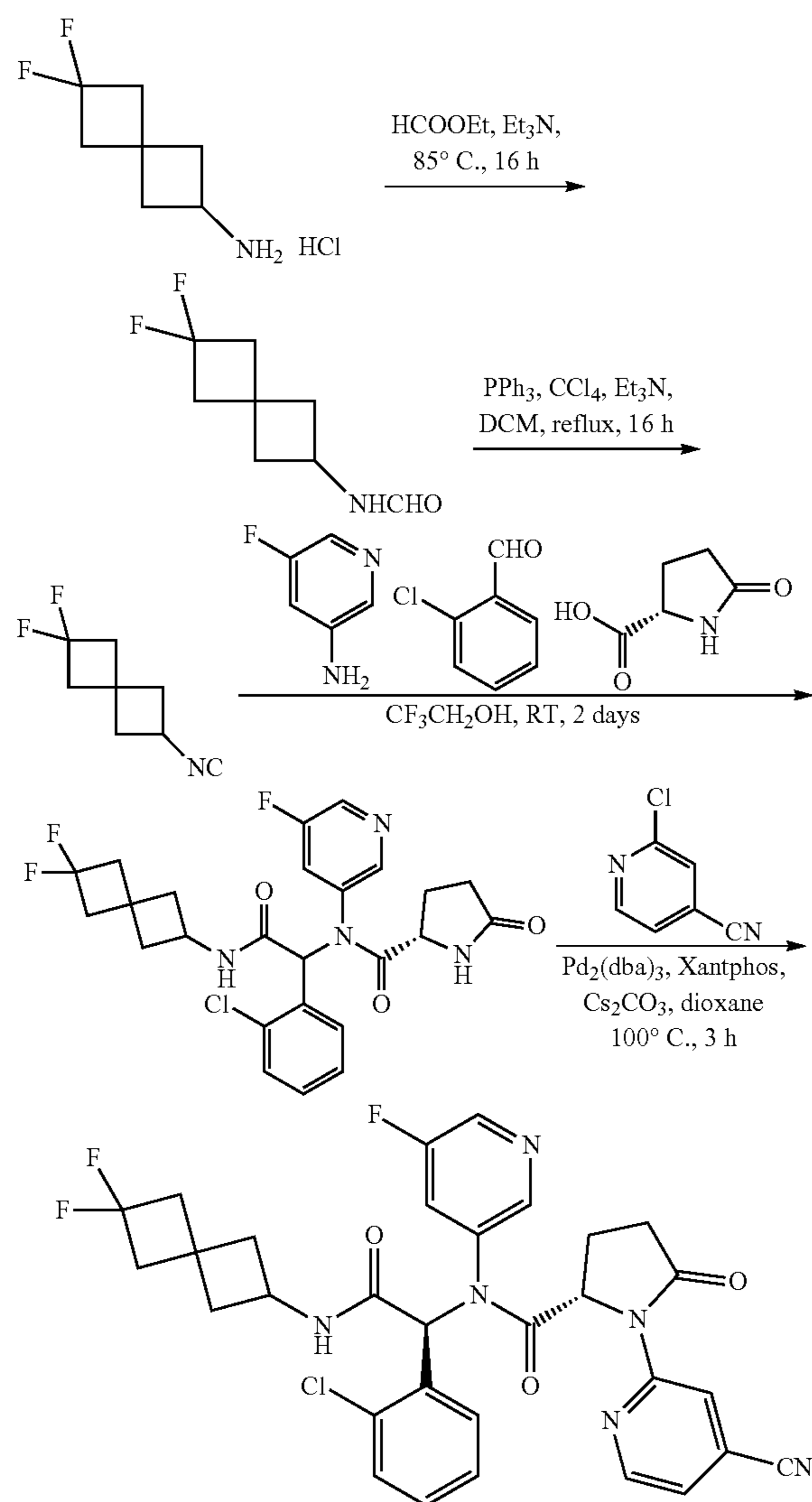
Step A: N-(6,6-difluorospiro[3.3]heptan-2-yl)formamide
