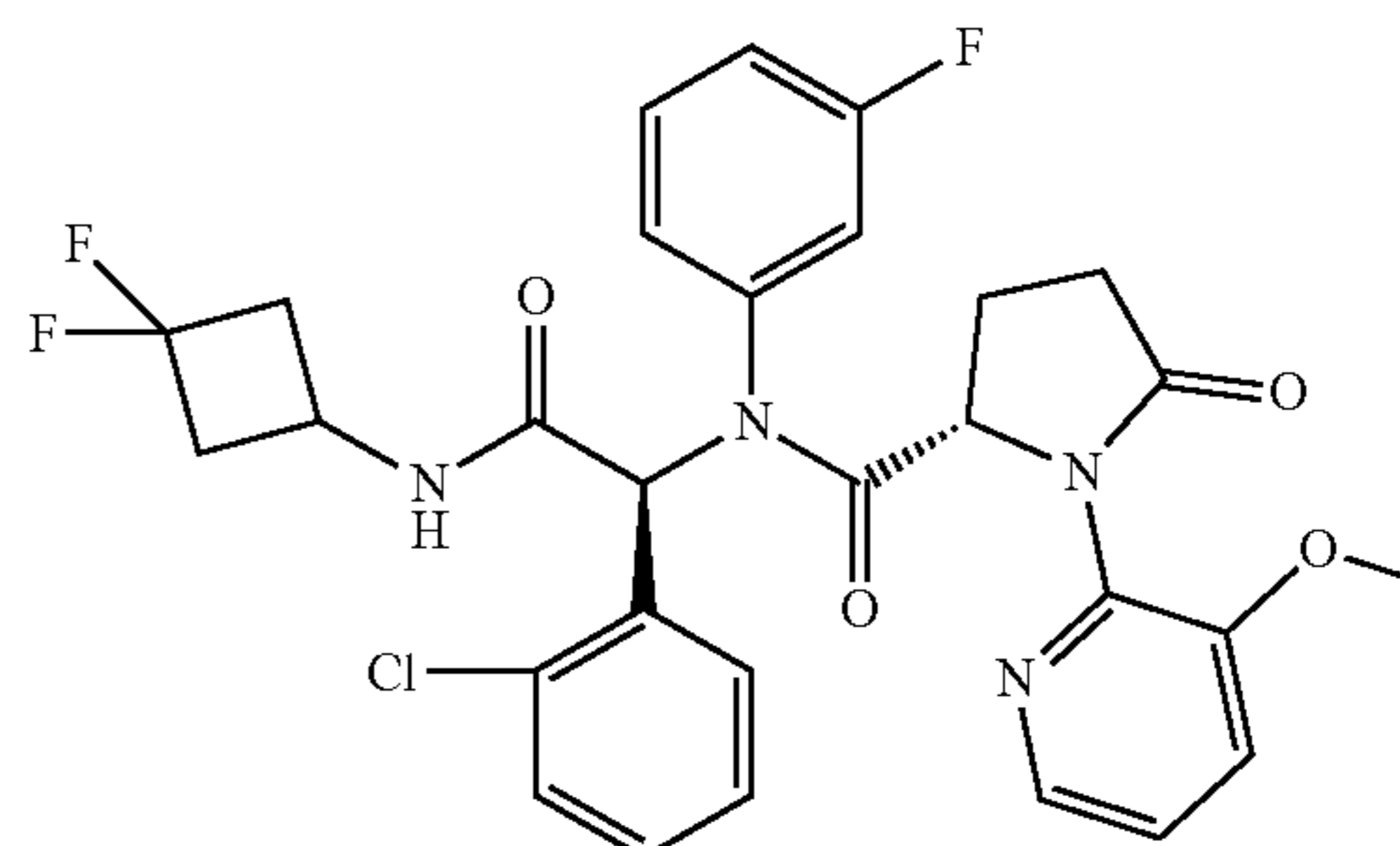
Compound 17
