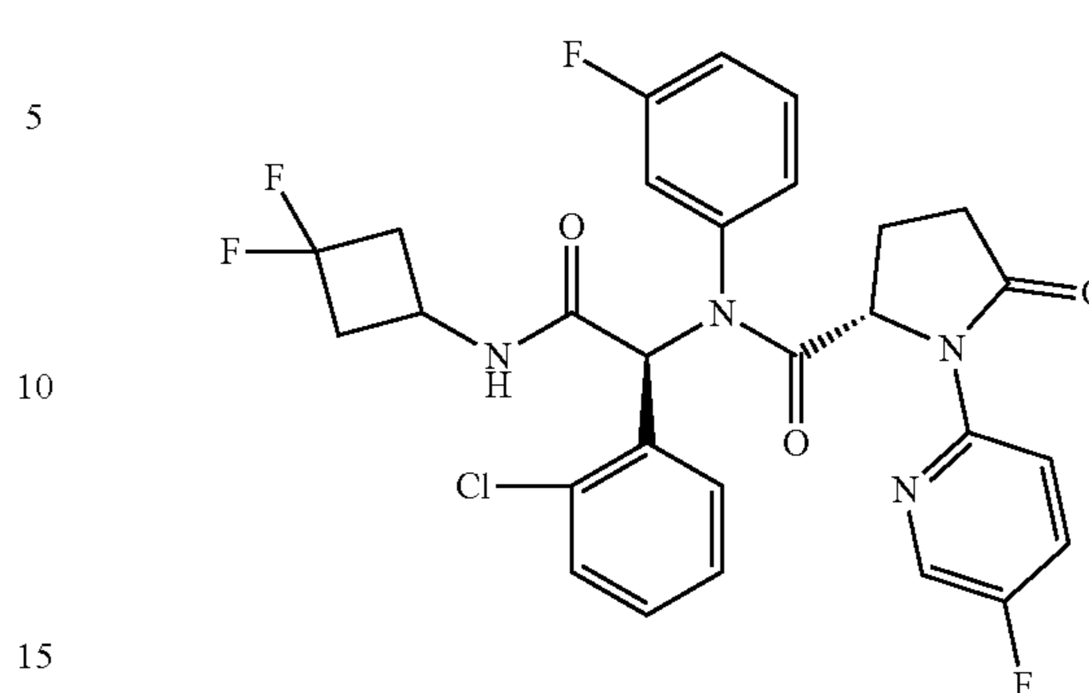
Compound 29
