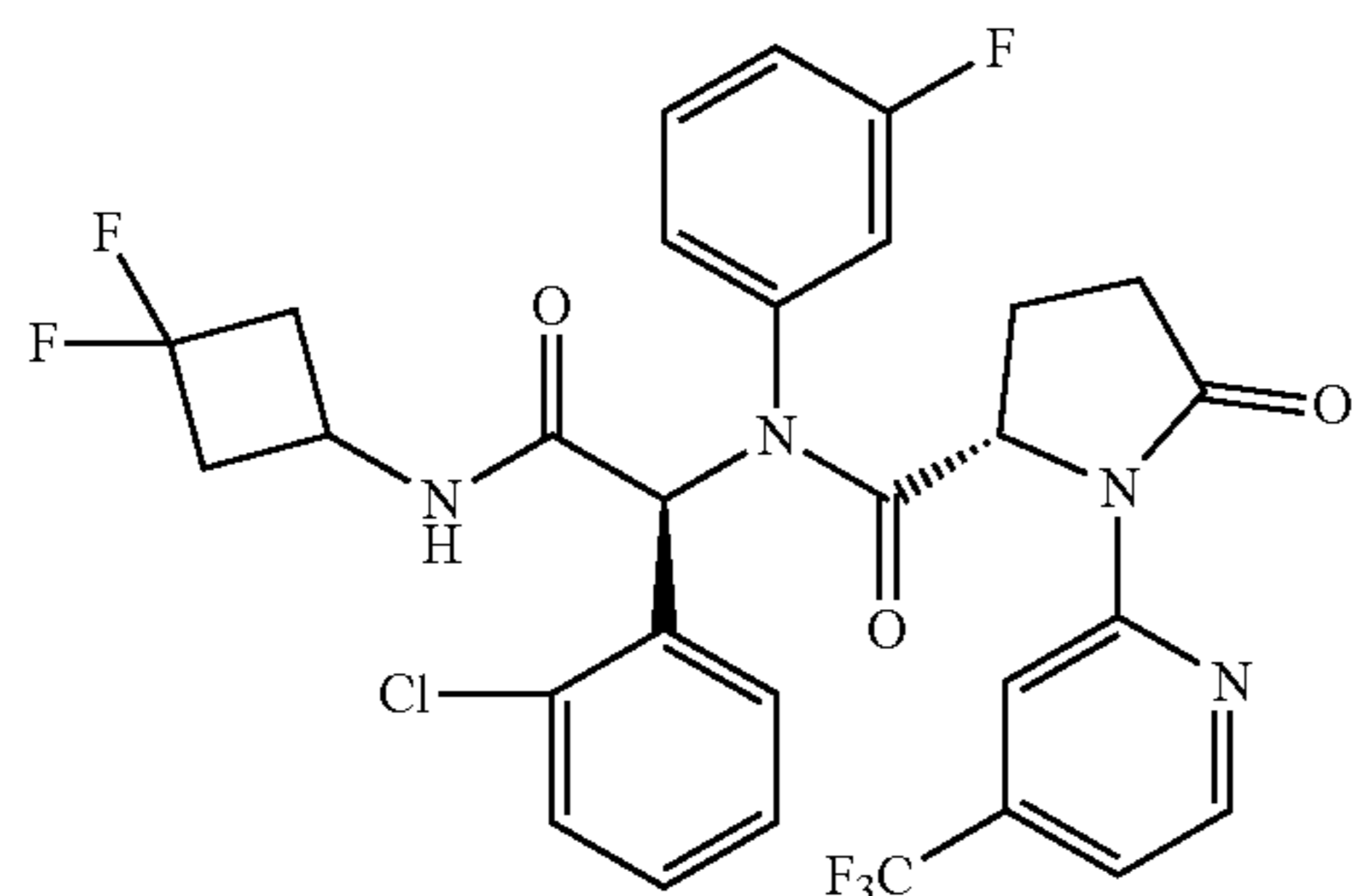
Compound 40
