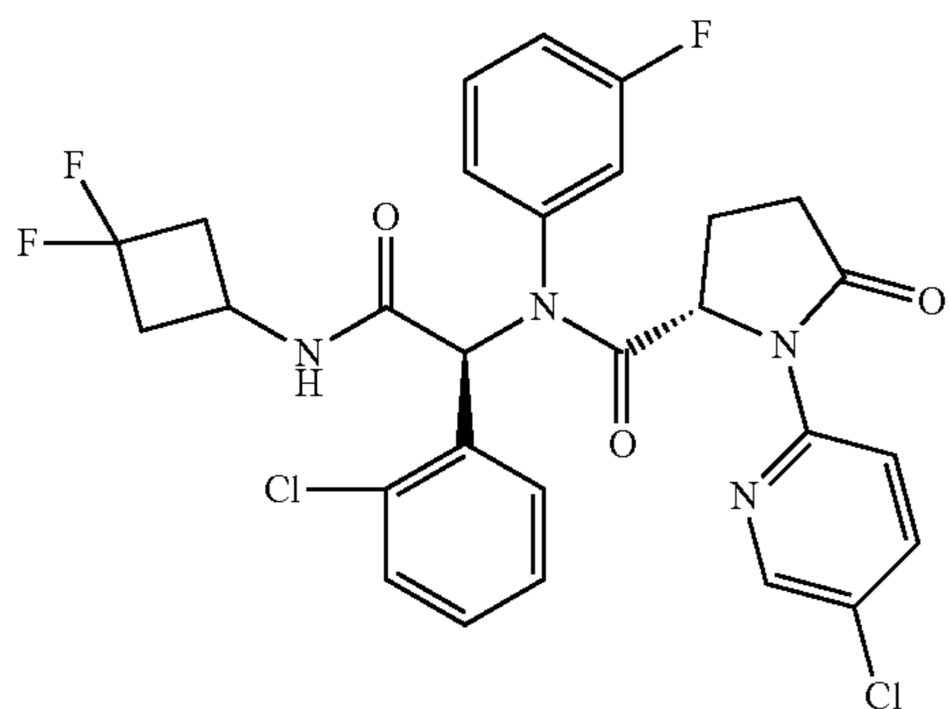
Compound 48
