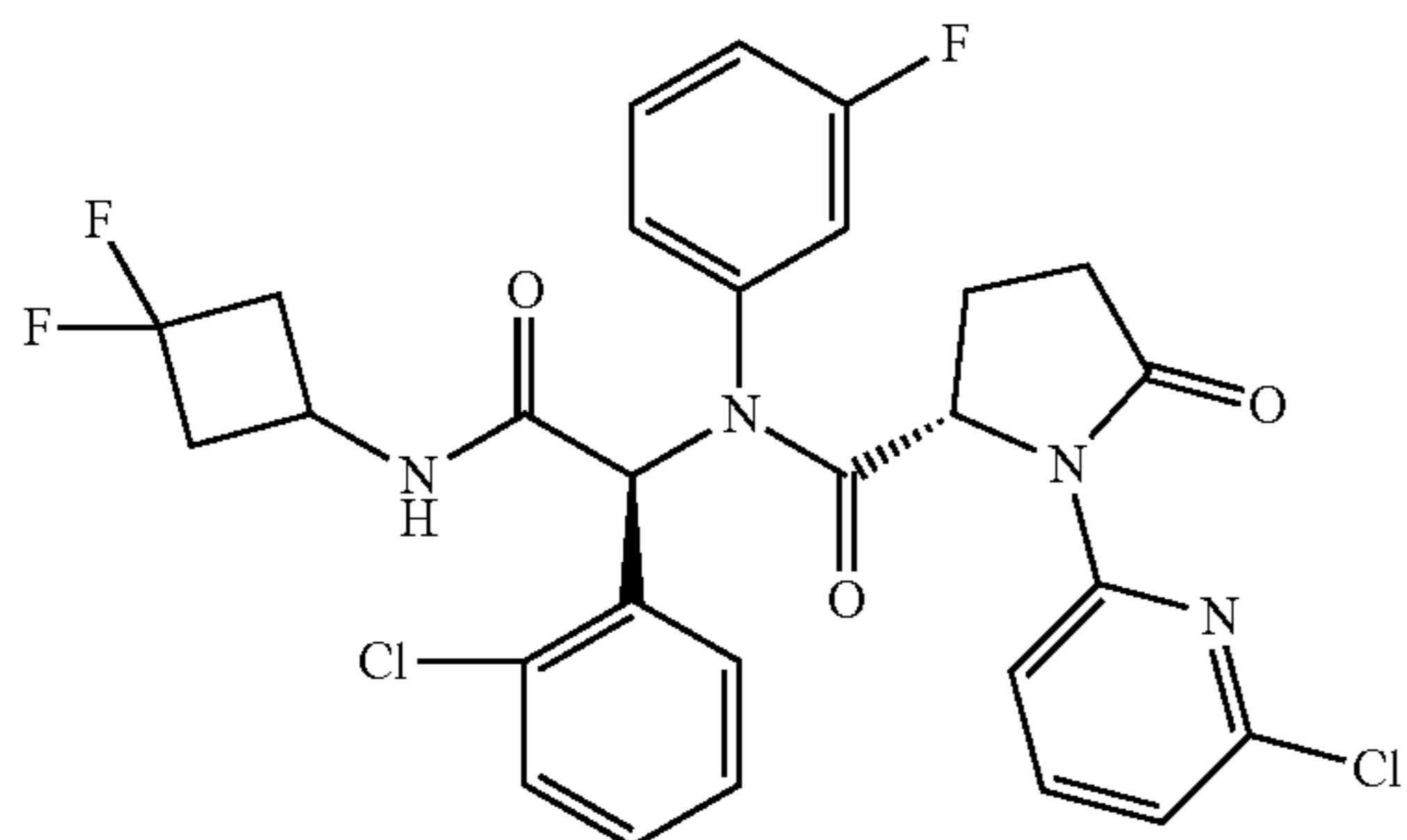
Compound 35
