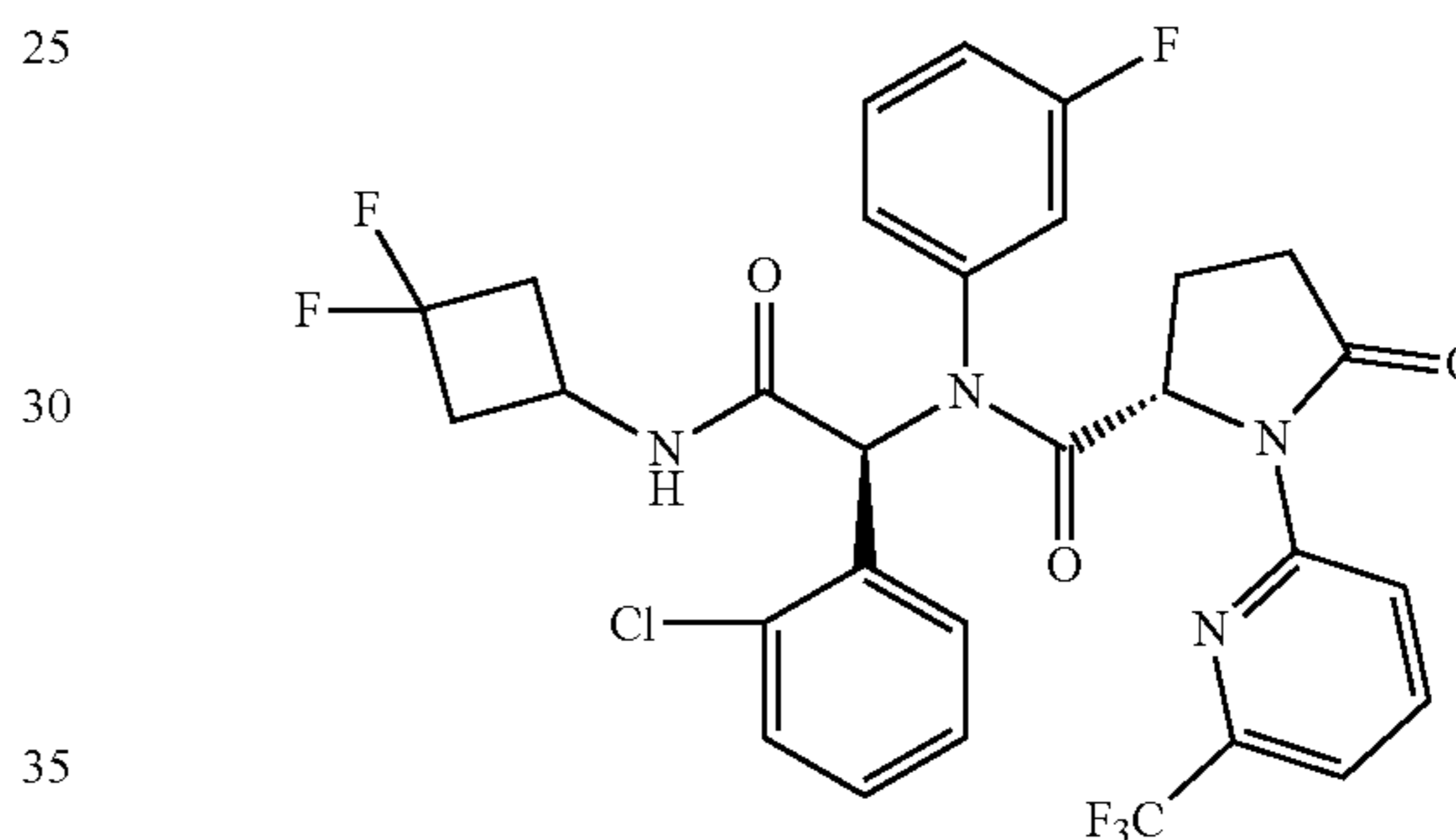
Compound 25
