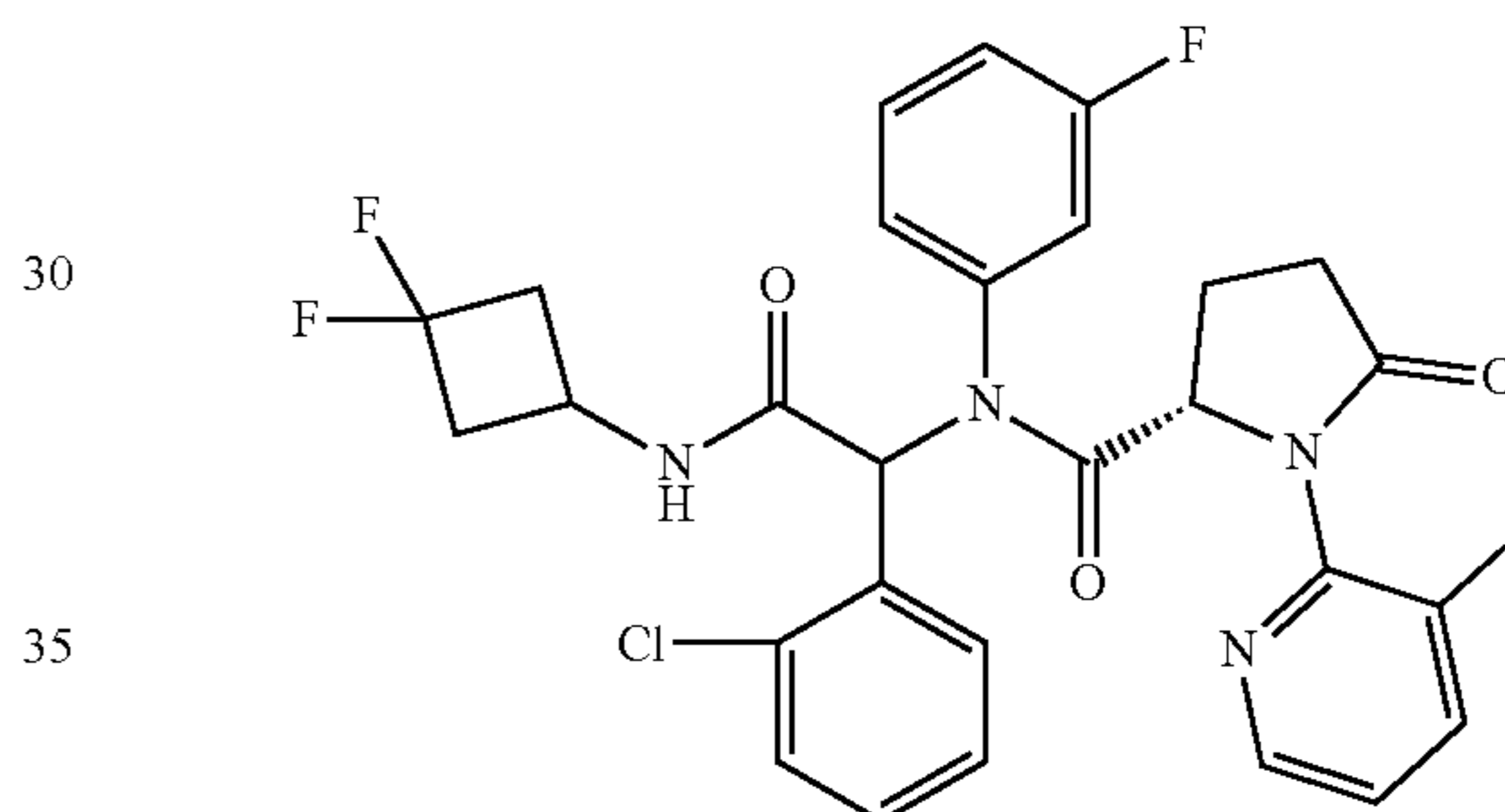
Compound 12
