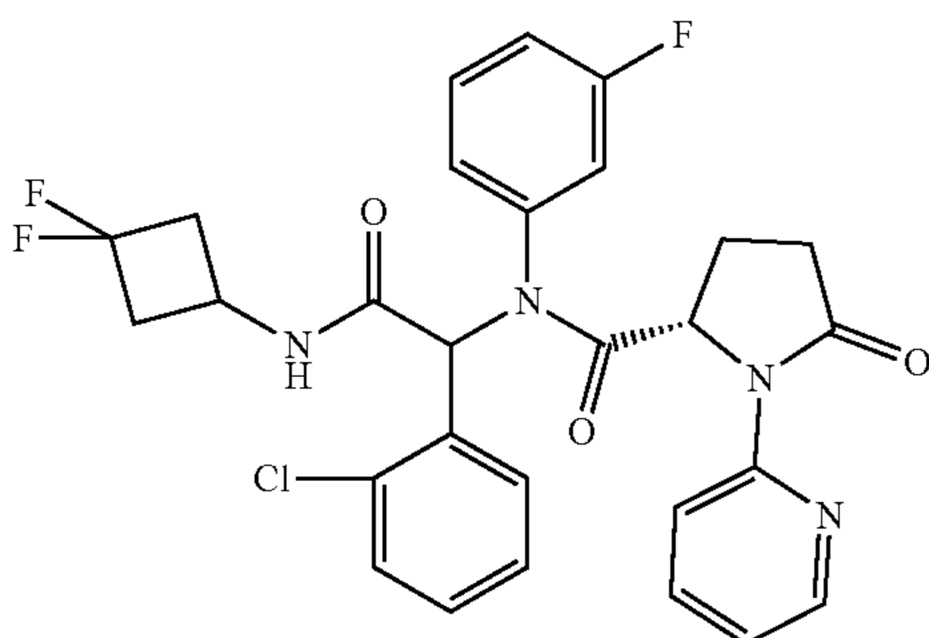
Compound 5
