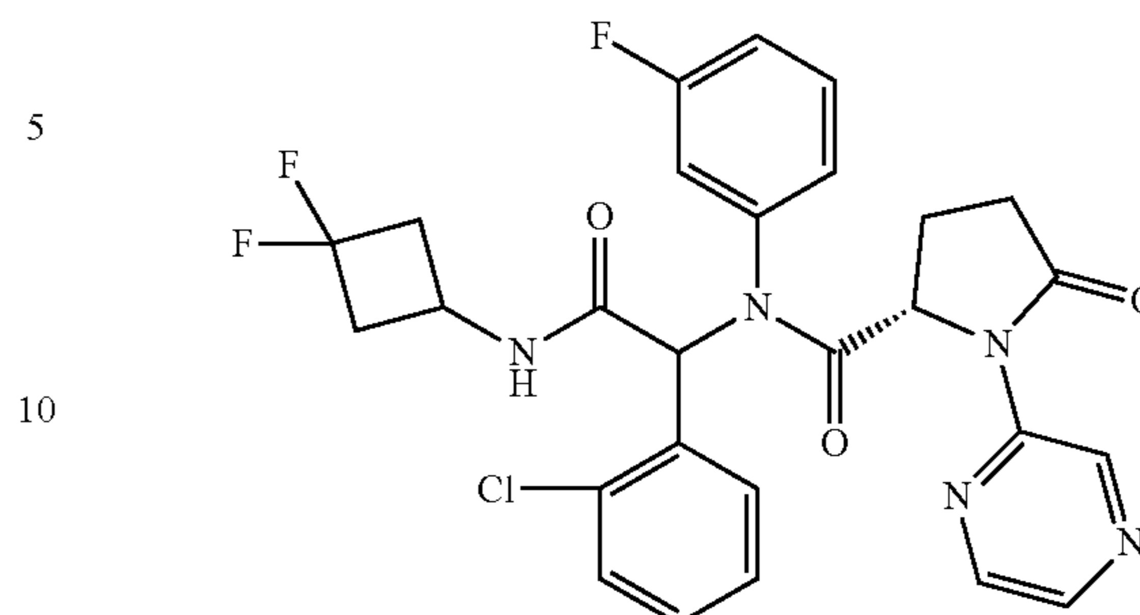
Compound 18
