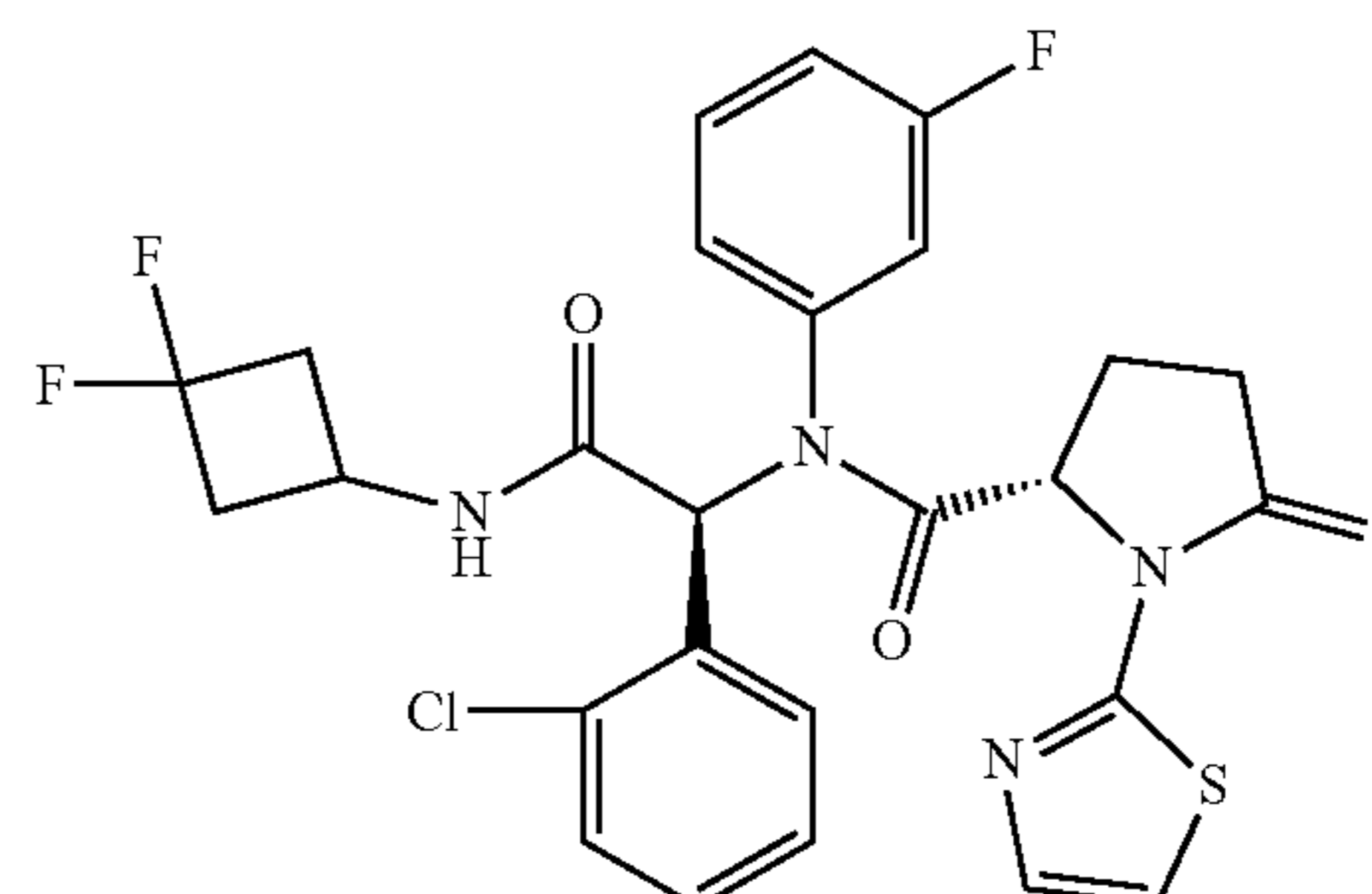
Compound 14
