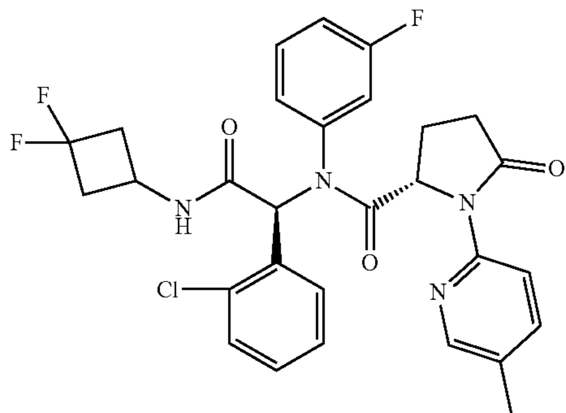
Compound 21
