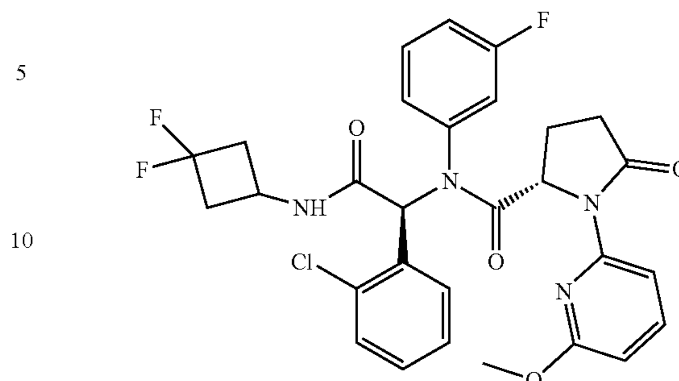
Compound 41
