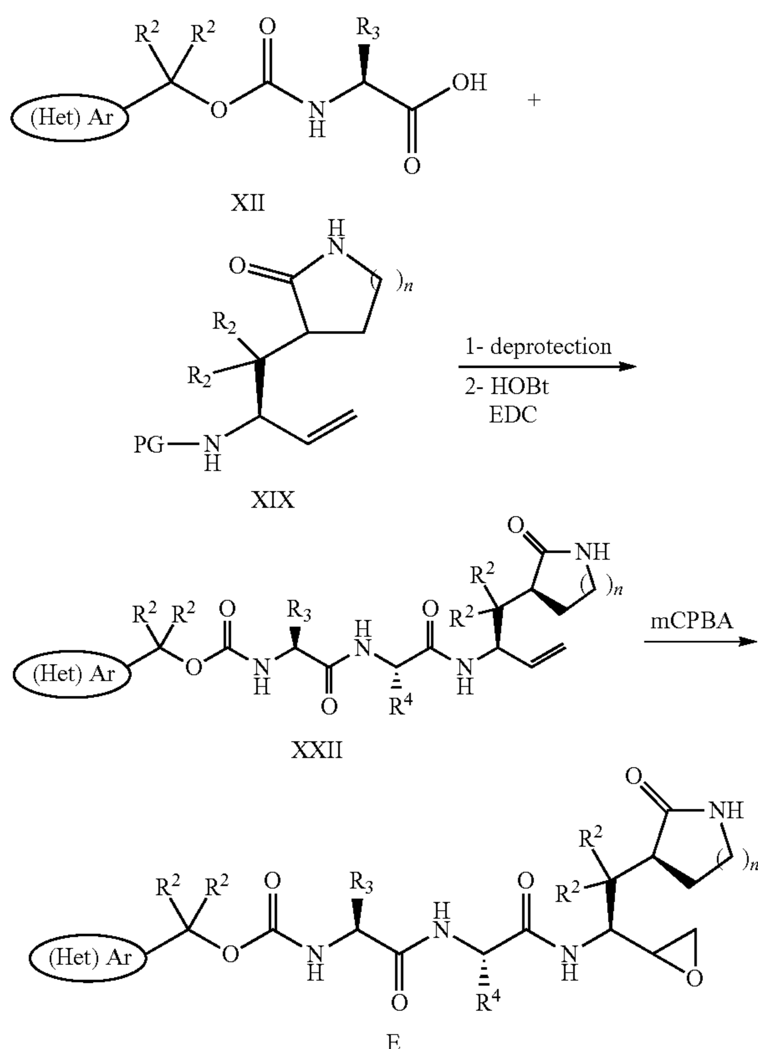
Scheme 3 A synthetic approach to compounds E
