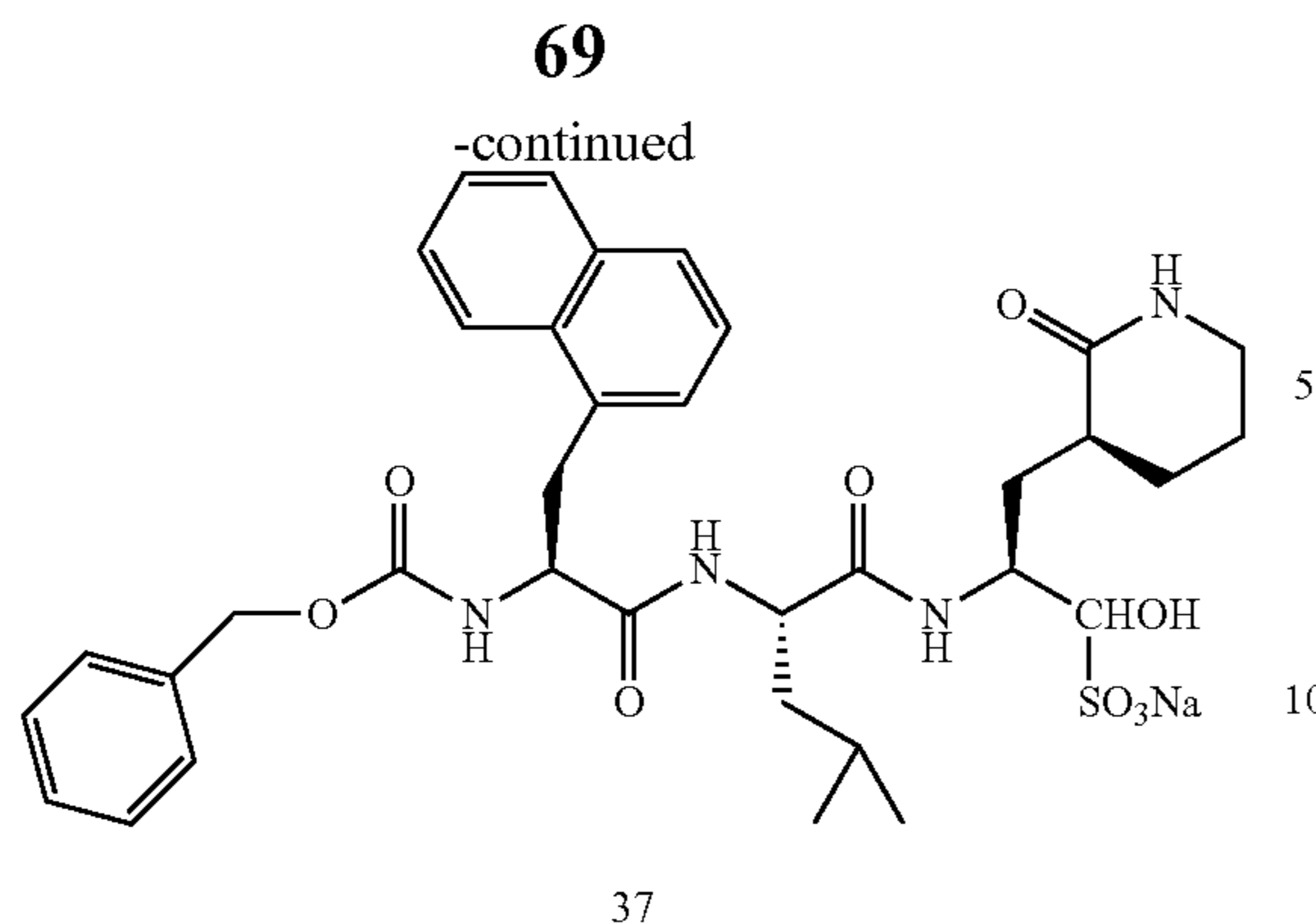
Sodium (5S,8S,11S)-12-hydroxy-8-isobutyl-5-(naphthalen-1-ylmethyl)-3,6,9-trioxo-11-(((S)-2-oxopiperidin-3-yl)methyl)-1-phenyl-2-oxa-4,7,10-triazadodecane-12-sulfonate (37)
