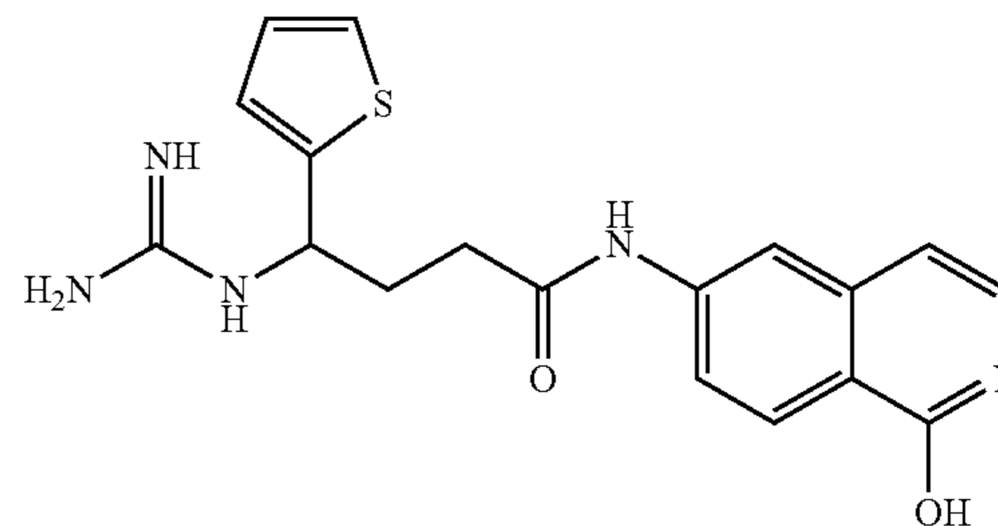
4-guanidino-N-(1-hydroxyisoquinolin-6-yl)-4-(thiophen-2-yl)butanamide
