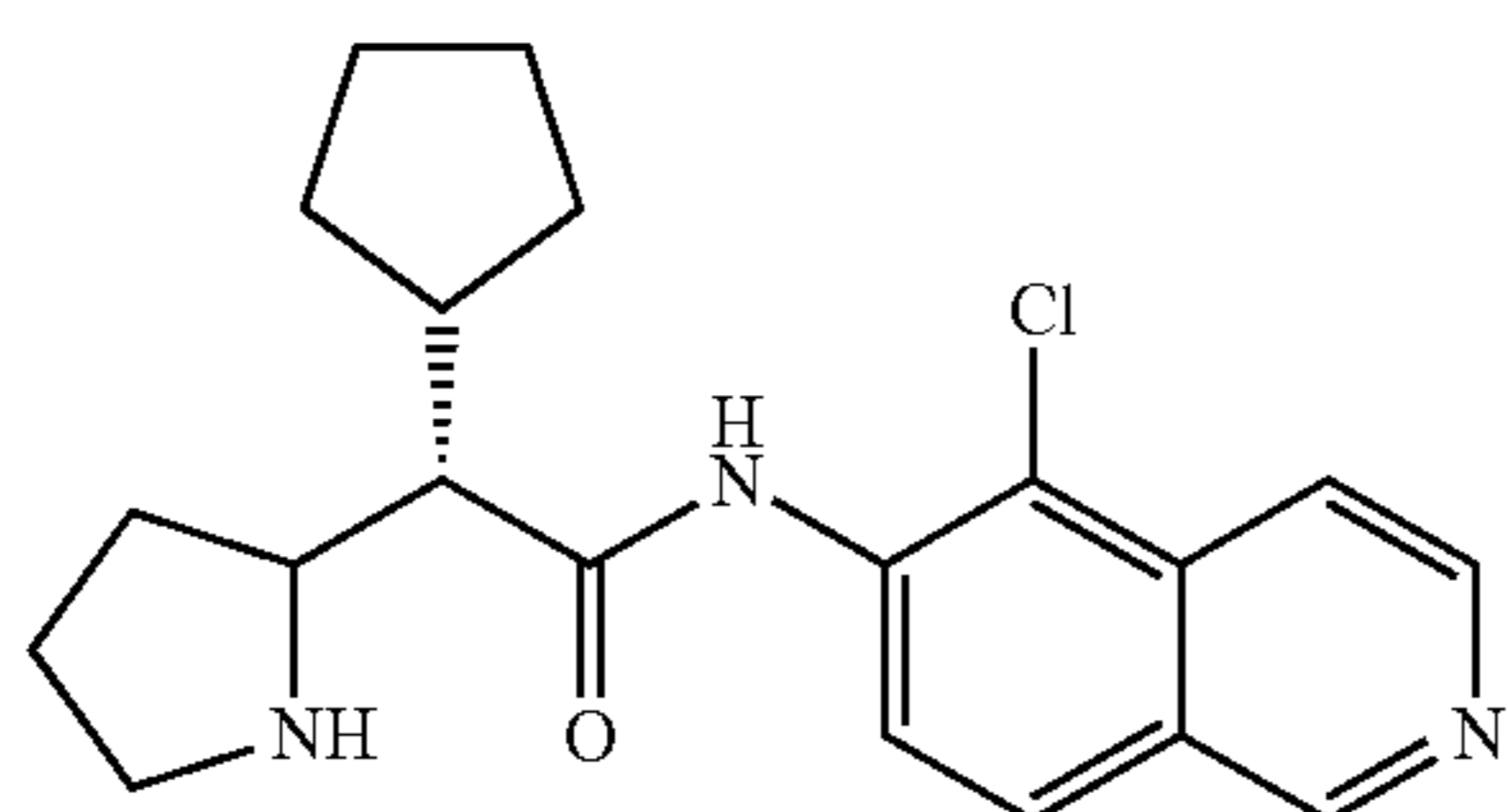
(2S)-N-(5-chloroisoquinolin-6-yl)-2-cyclopentyl-2-(pyrrolidin-2-yl)acetamide
