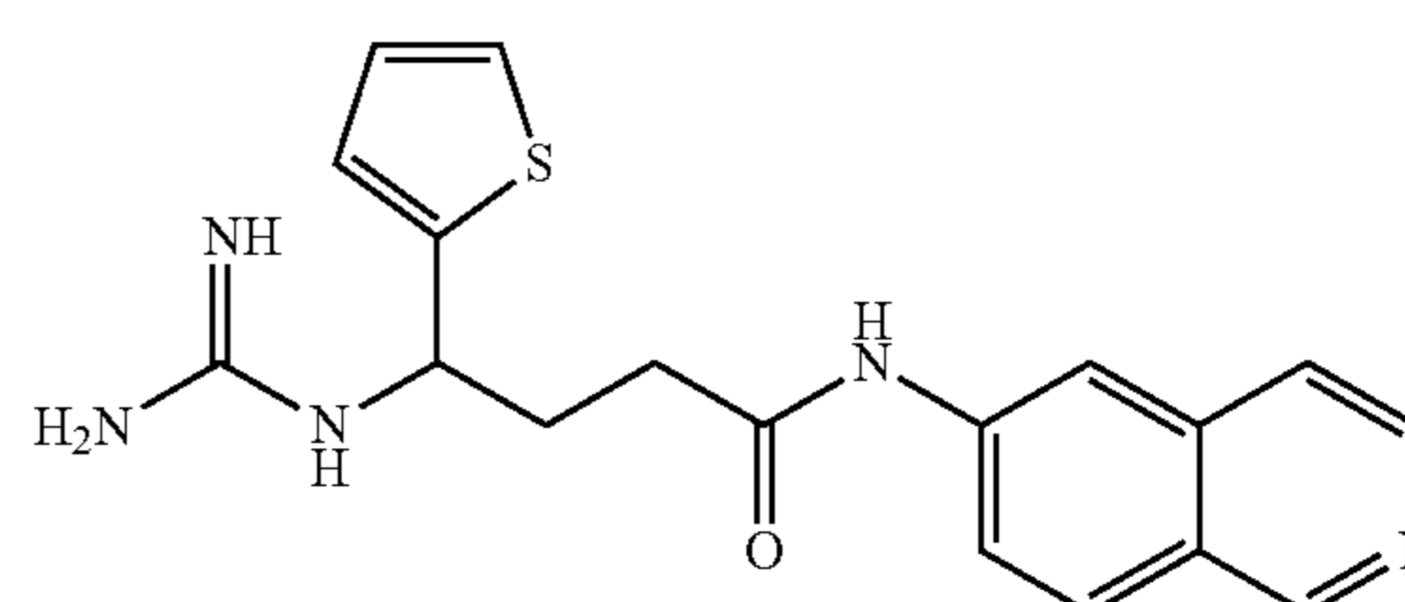
4-guanidino-N-(isoquinolin-6-yl)-4-(thiophen-2-yl)butanamide
