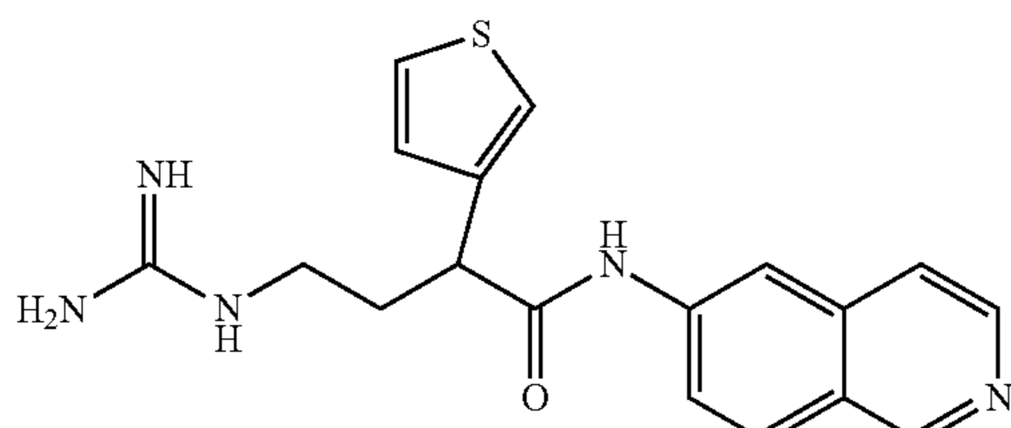
4-guanidino-N-(isoquinolin-6-yl)-2-(thiophen-3-yl)butanamide
