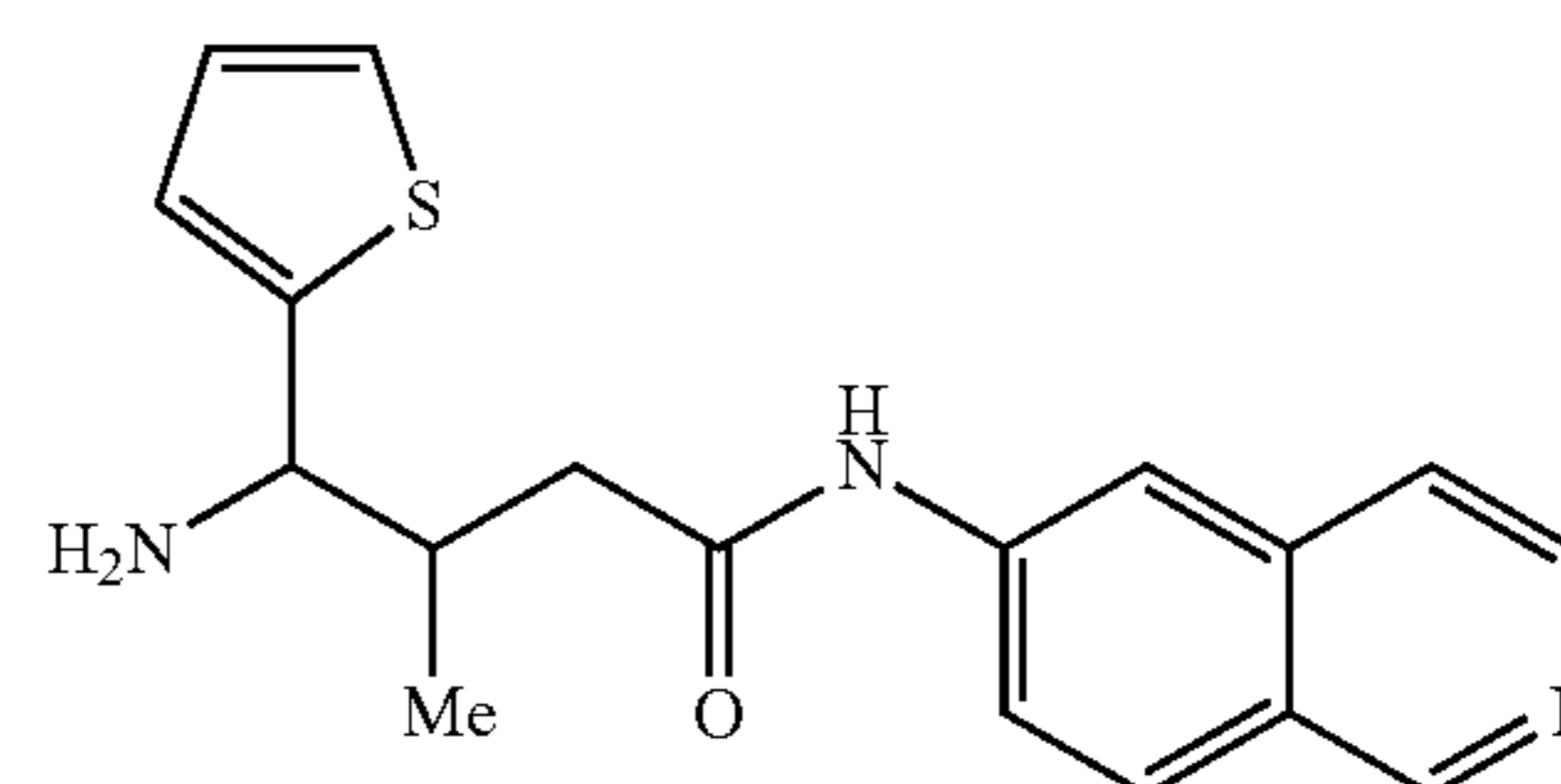
4-amino-N-(isoquinolin-6-yl)-3-methyl-4-(thiophen-2-yl)butanamide
