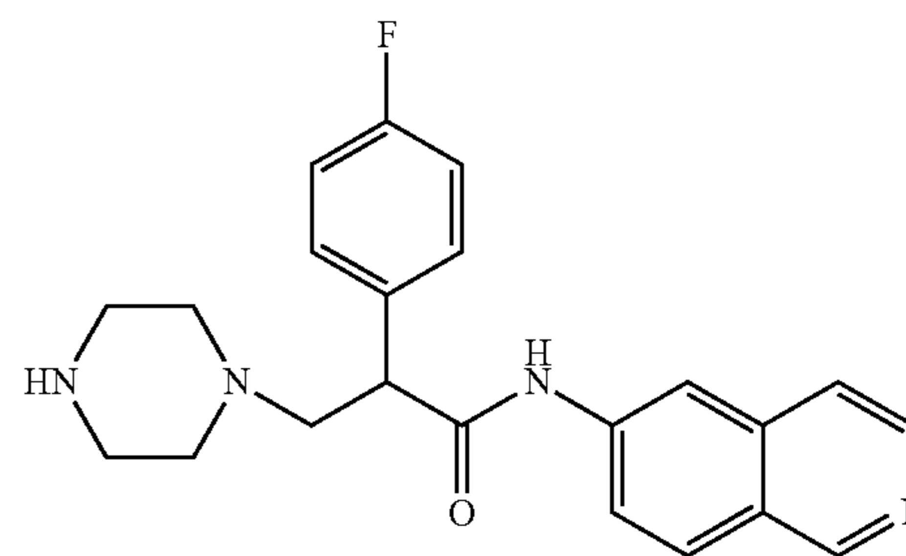
2-(4-fluorophenyl)-N-(isoquinolin-6-yl)-3-(piperazin-1-yl)propanamide
