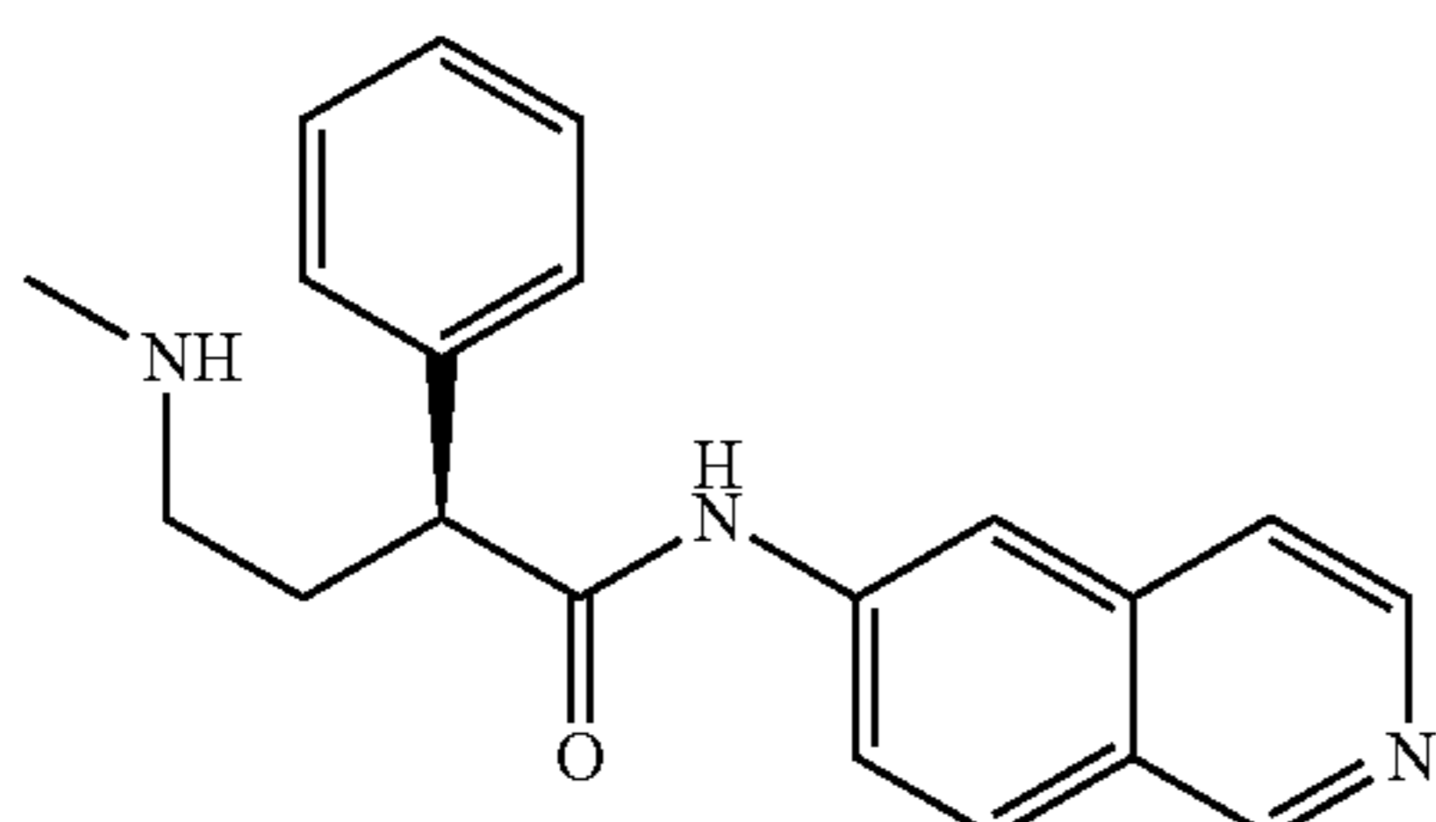
(S)-N-(isoquinolin-6-yl)-4-(methylamino)-2-phenylbutanamide
