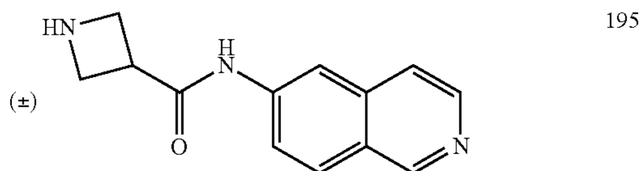
N-(isoquinolin-6-yl)azetidine-3-carboxamide
