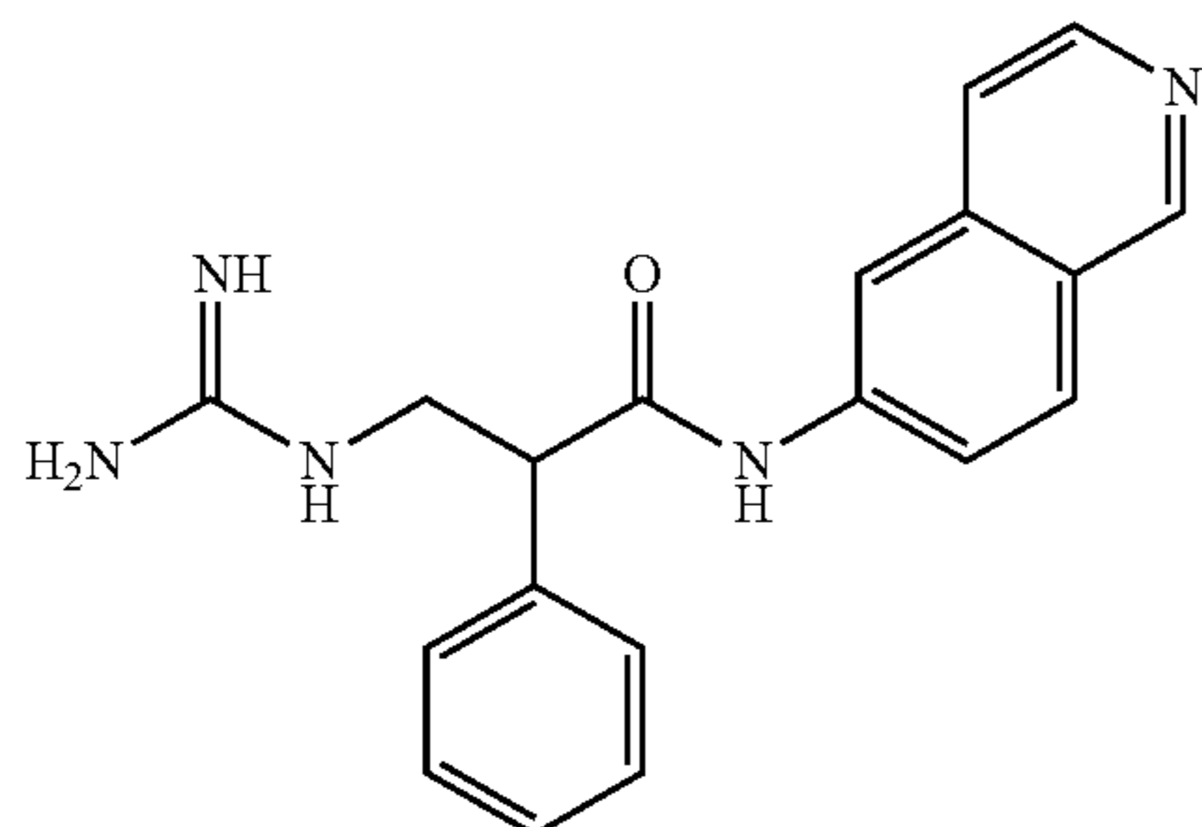
3-guanidino-N-(isoquinolin-6-yl)-2-phenylpropanamide
