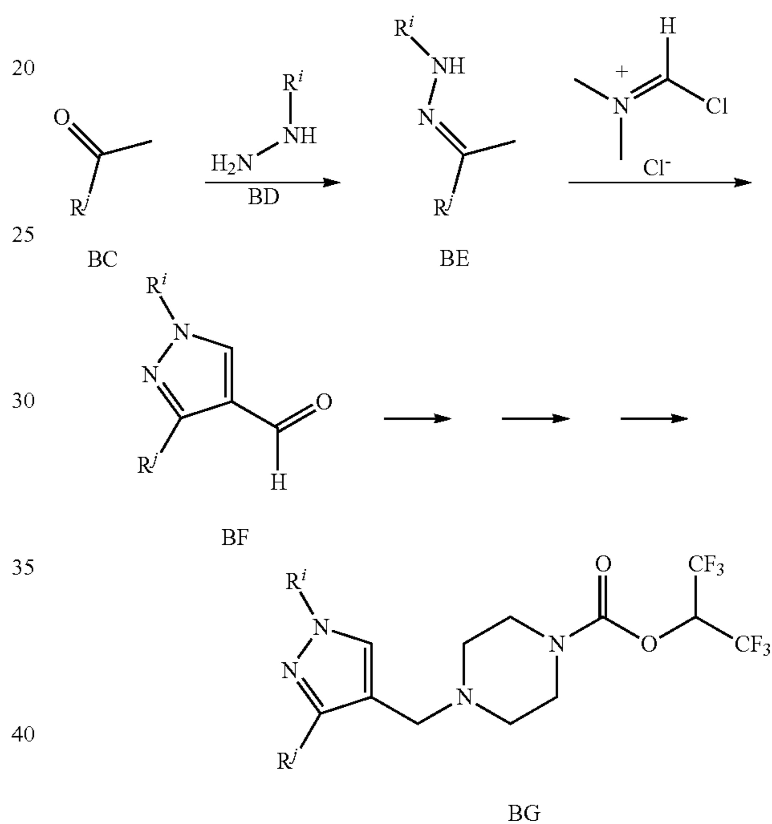
SCHEME 14
