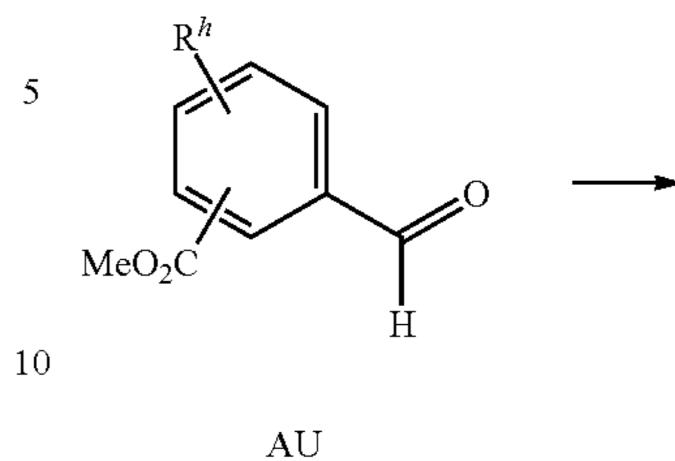
SCHEME 12
