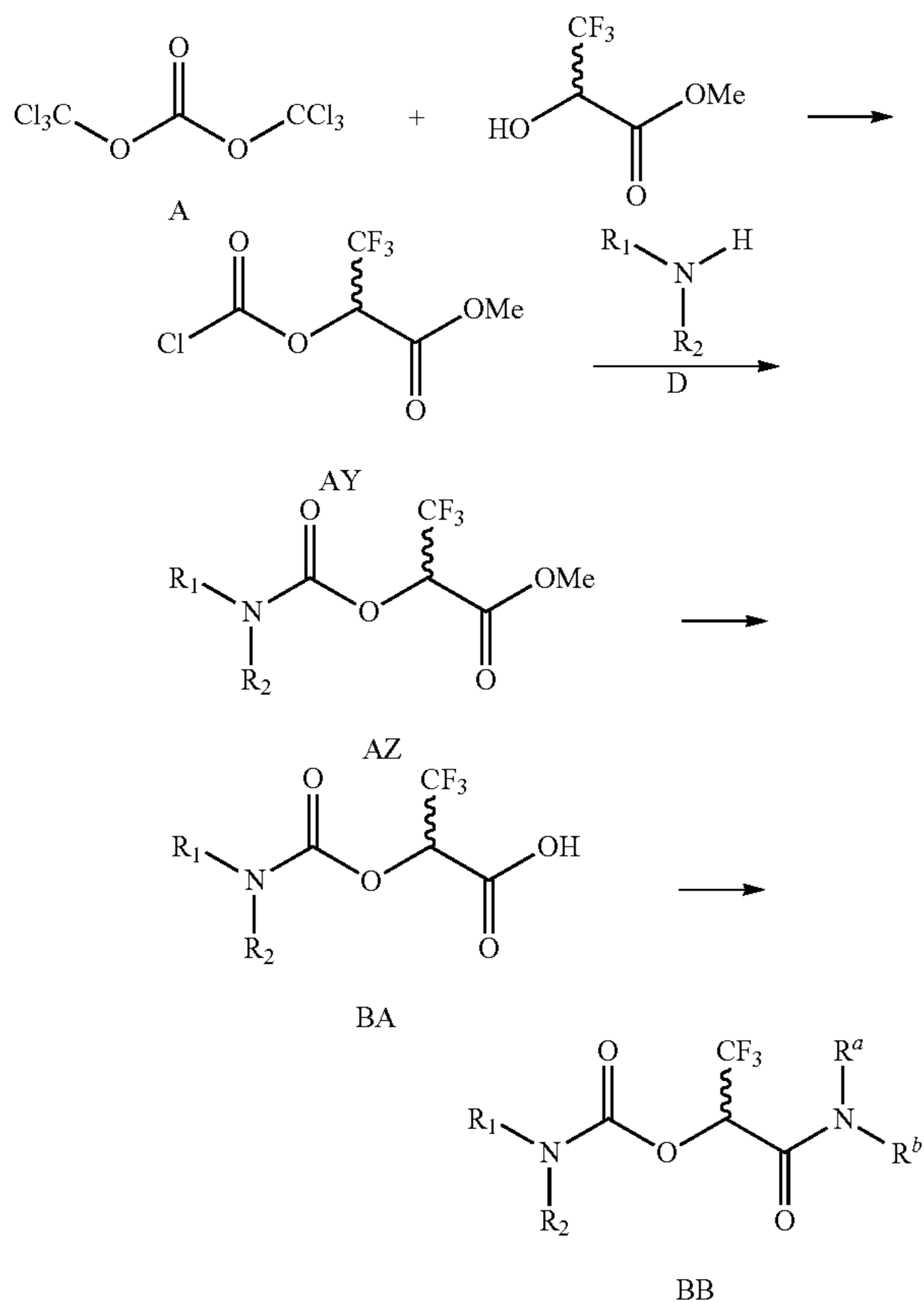
SCHEME 13
