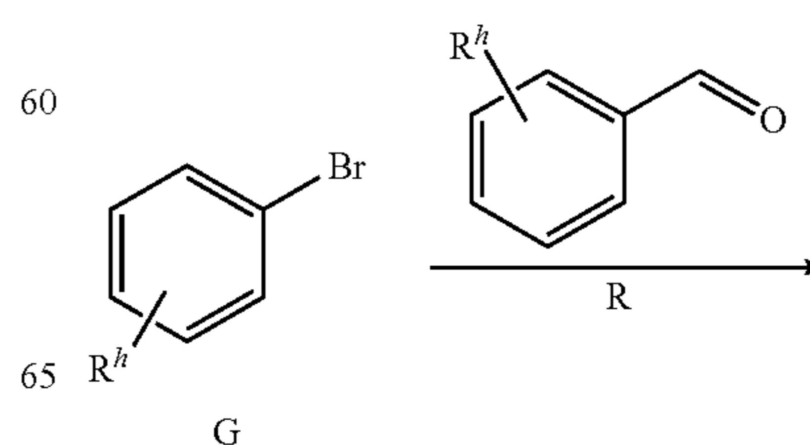
SCHEME 5
