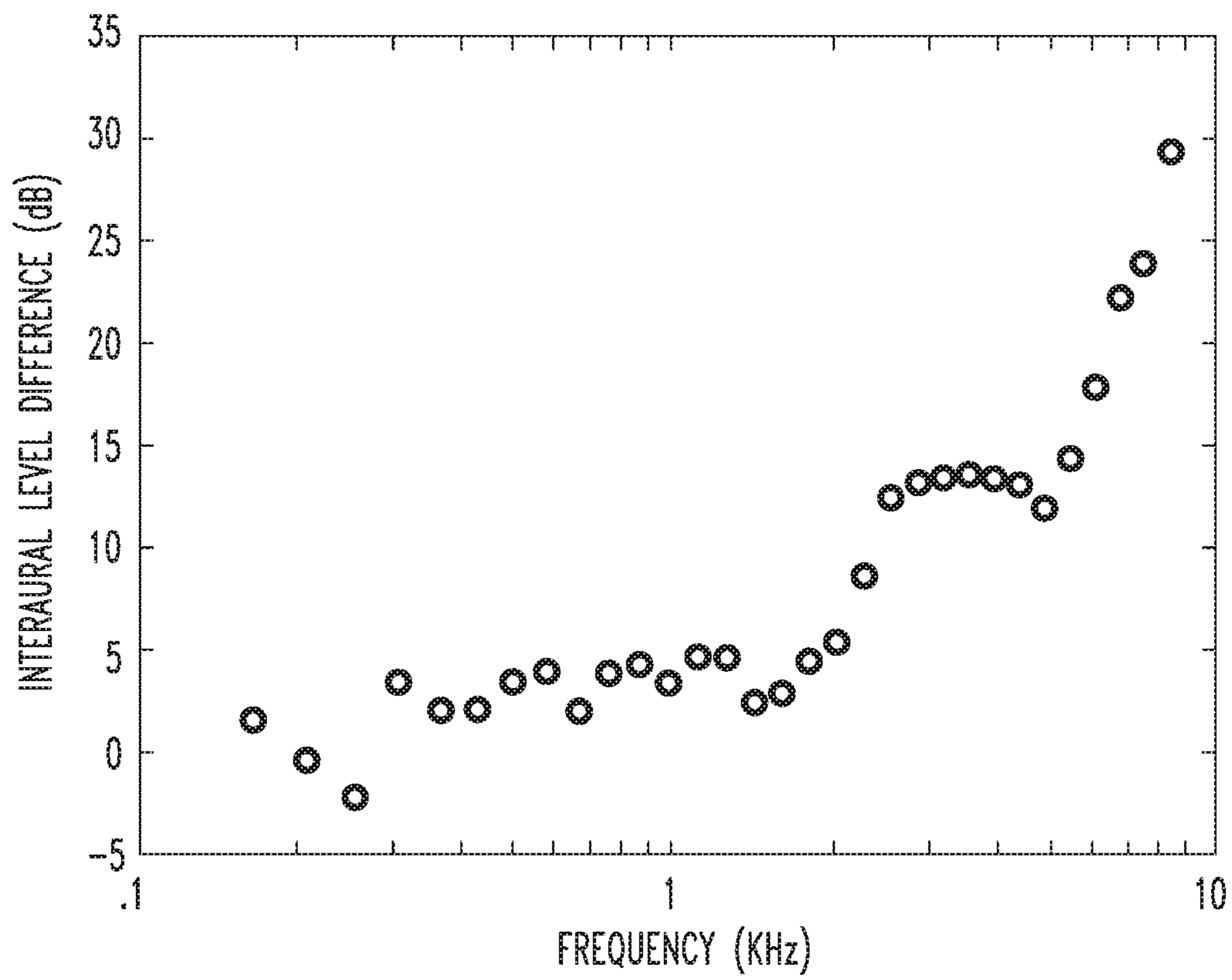
FIG. 1 (PRIOR ART)
