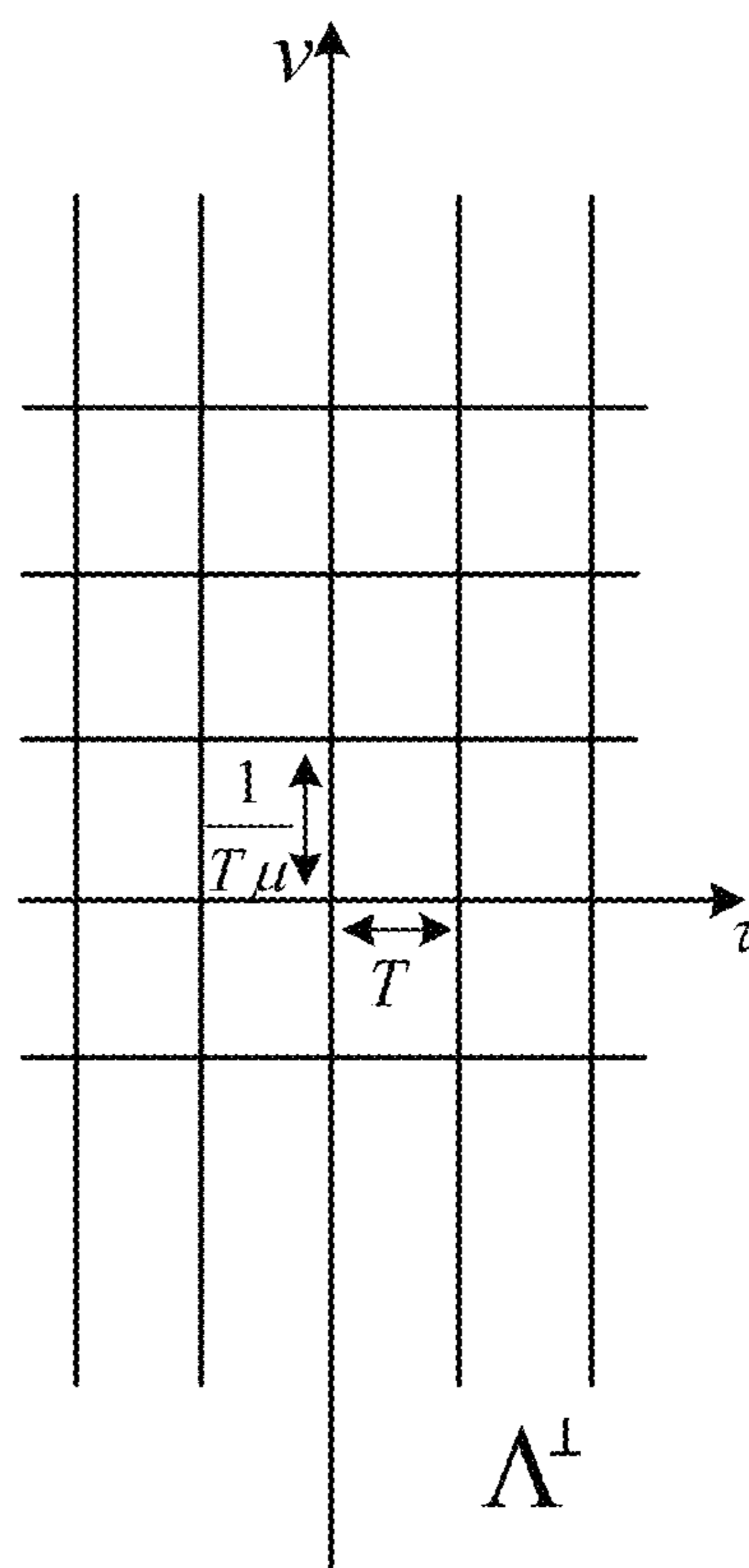
Reciprocal lattice
