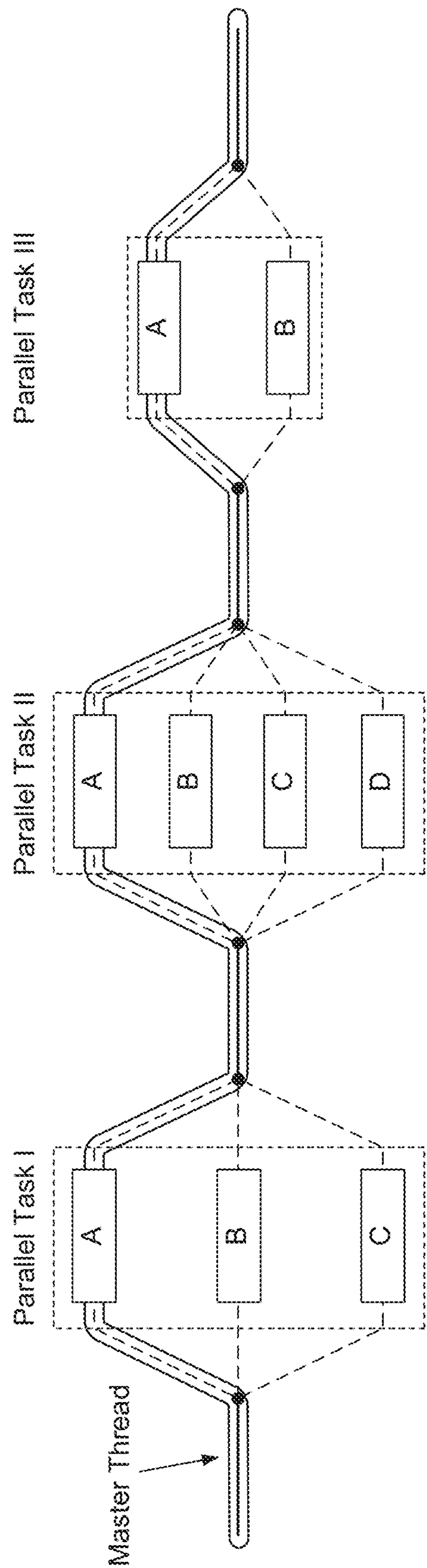
FIG. 1 (Prior Art)
