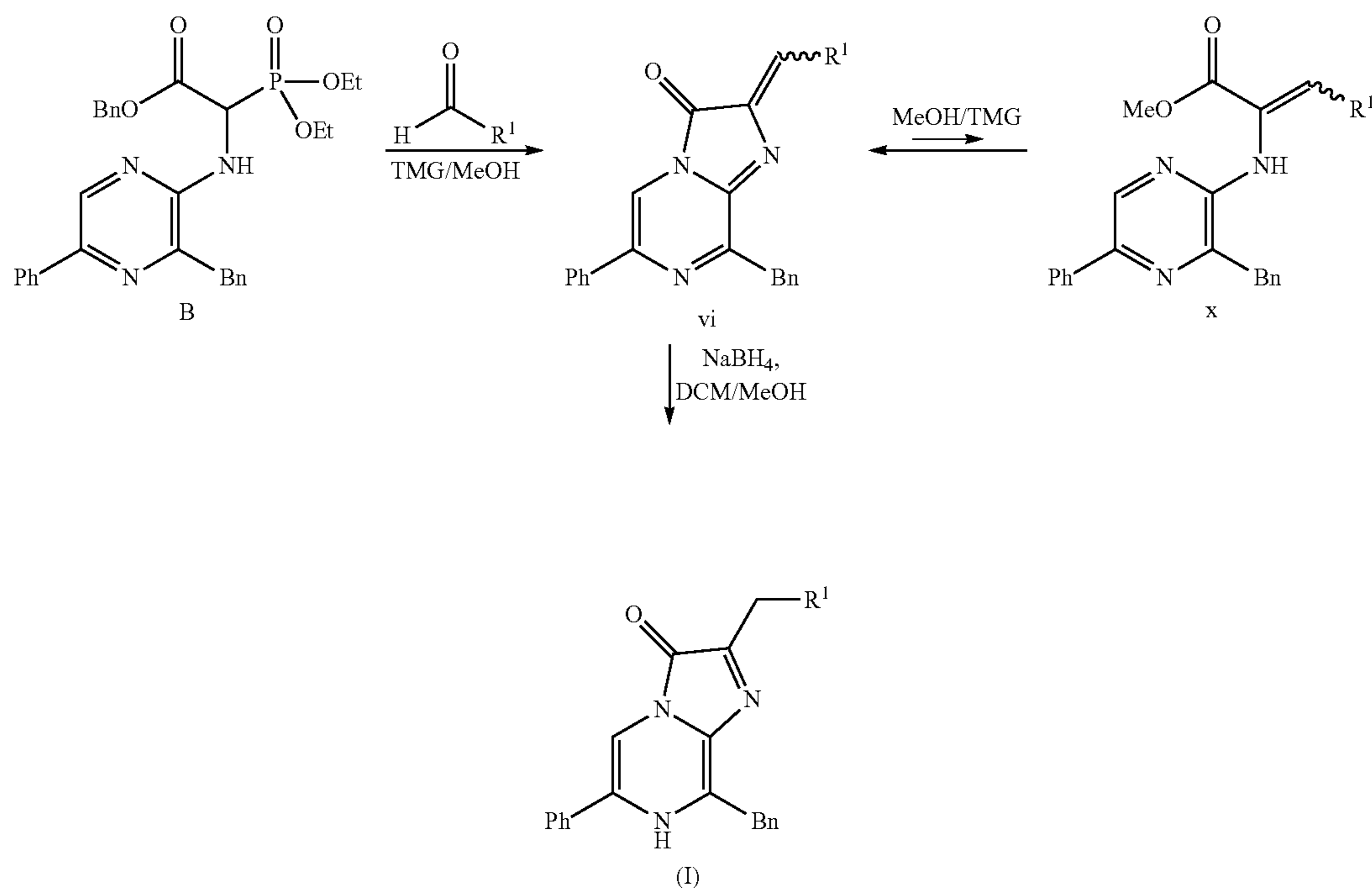
Scheme 6. Modified Method I
