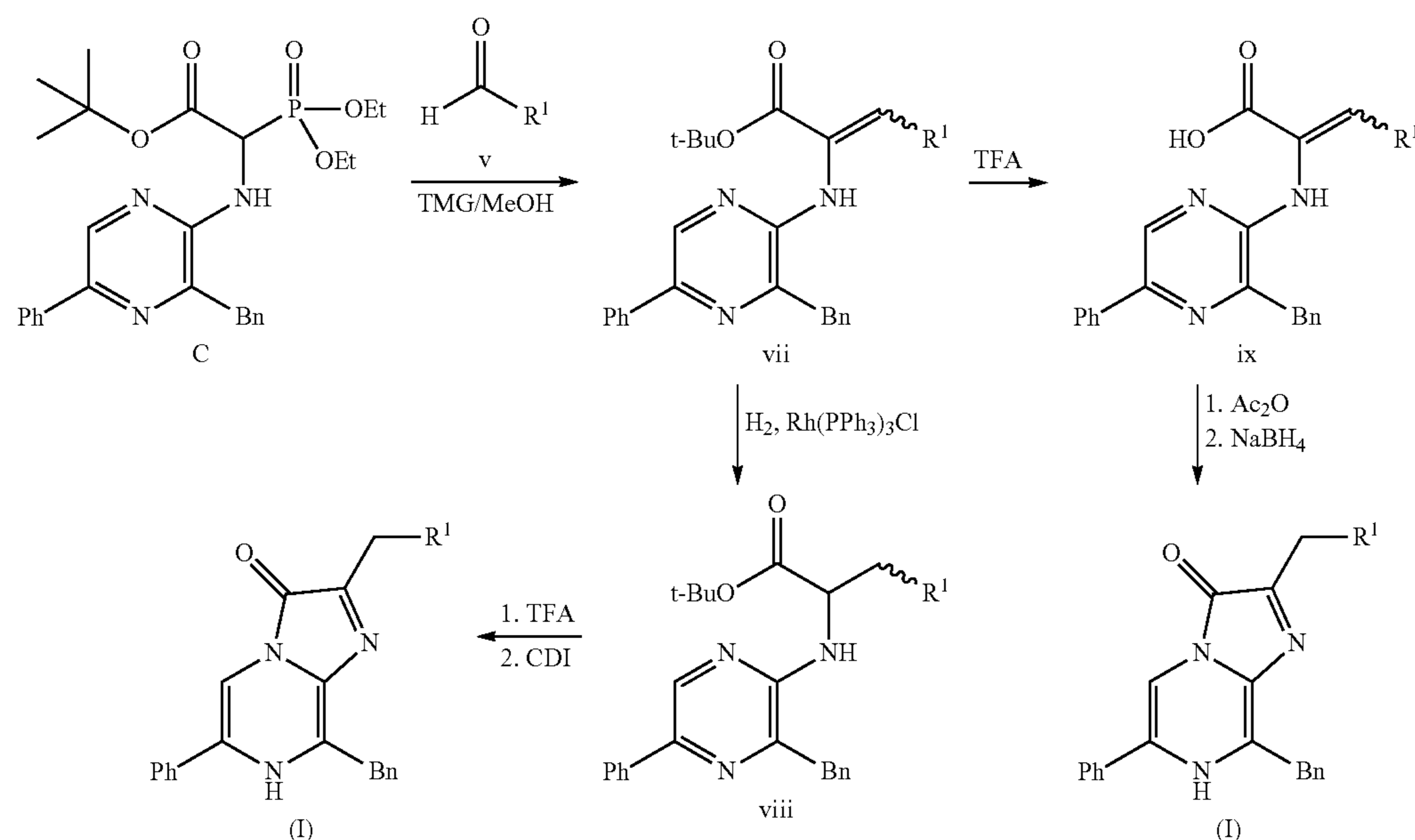
Scheme 3. Synthesis of the compound of formula (I)
