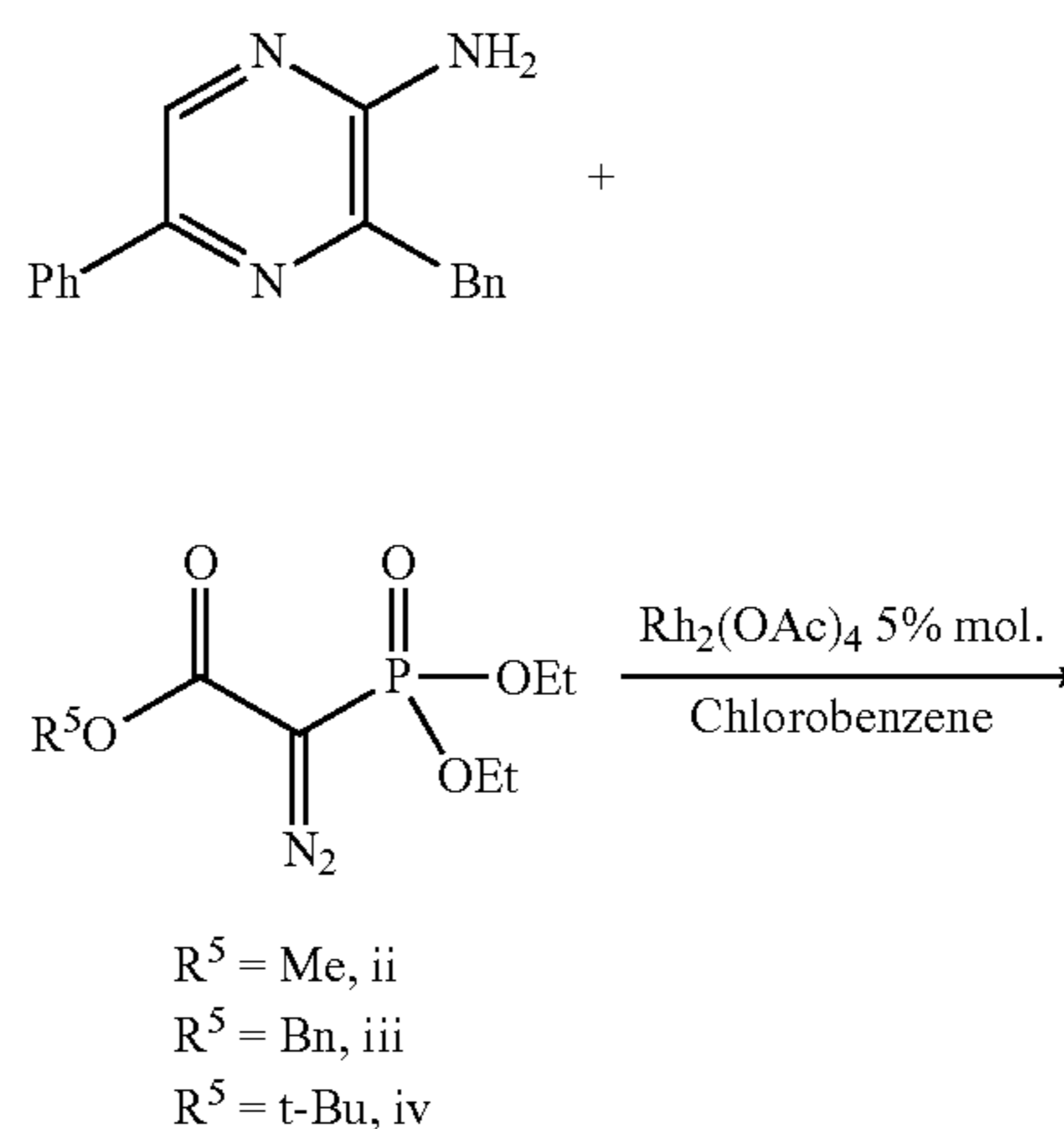
Scheme 4. Synthesis of Intermediates A-C
