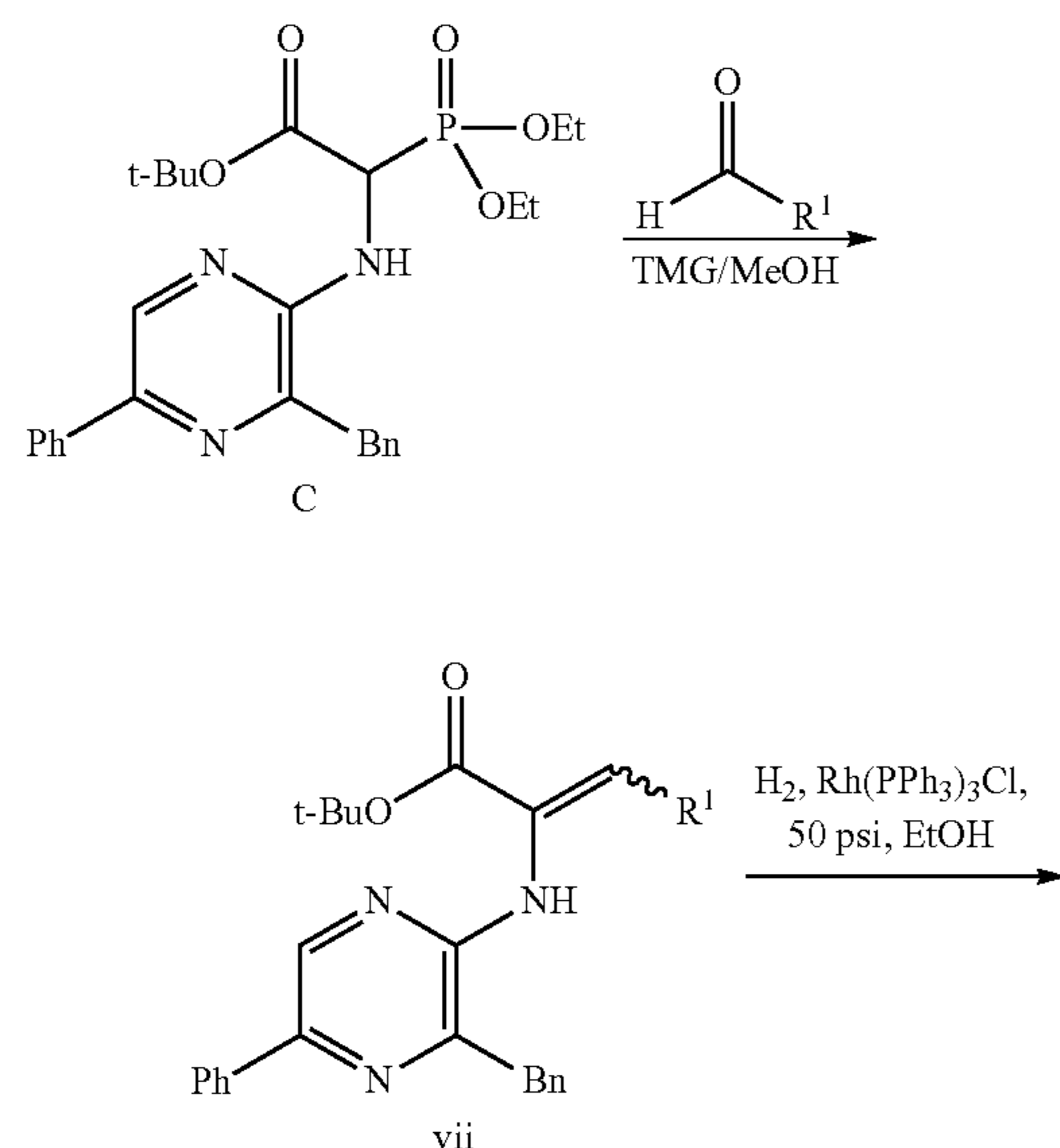
Scheme 8. Method III
