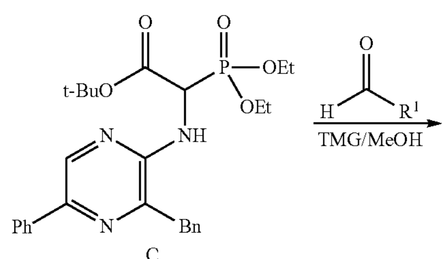
Scheme 7. Method II
