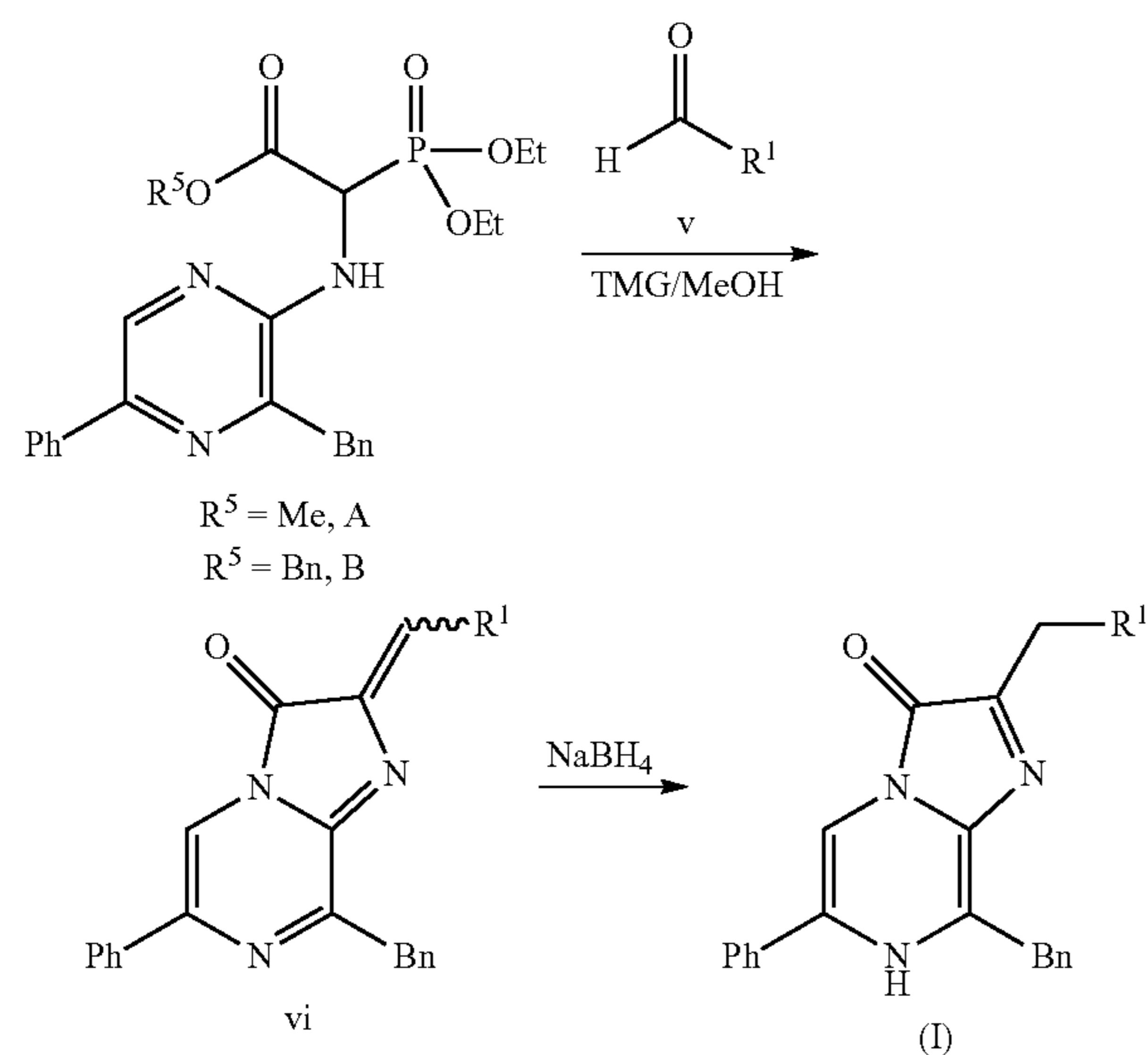
Scheme 2. Synthesis of the compound of formula (I)
