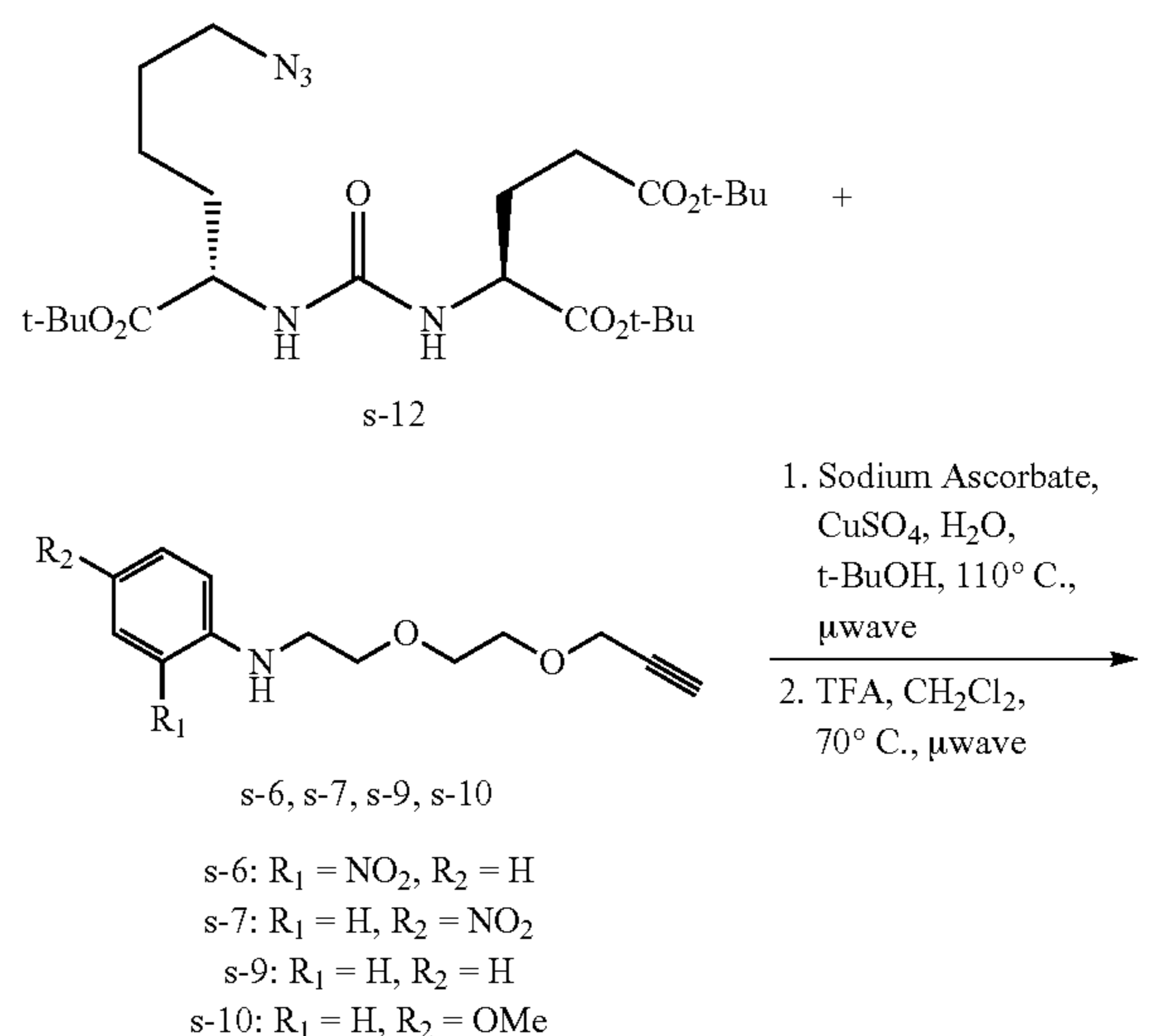
Scheme S-6: General synthesis of 13-16.
