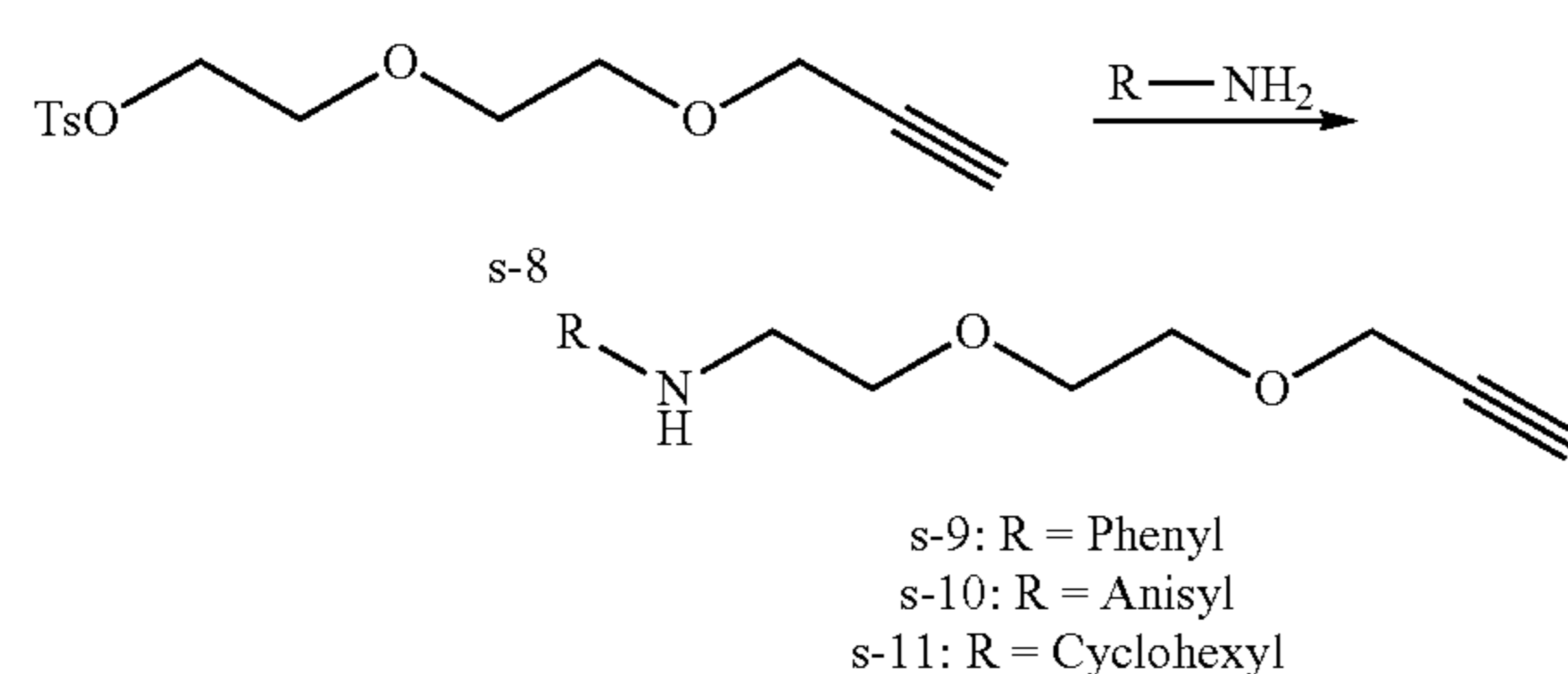
Scheme S-3: General synthesis of (PEG) 2 -alkynes.
