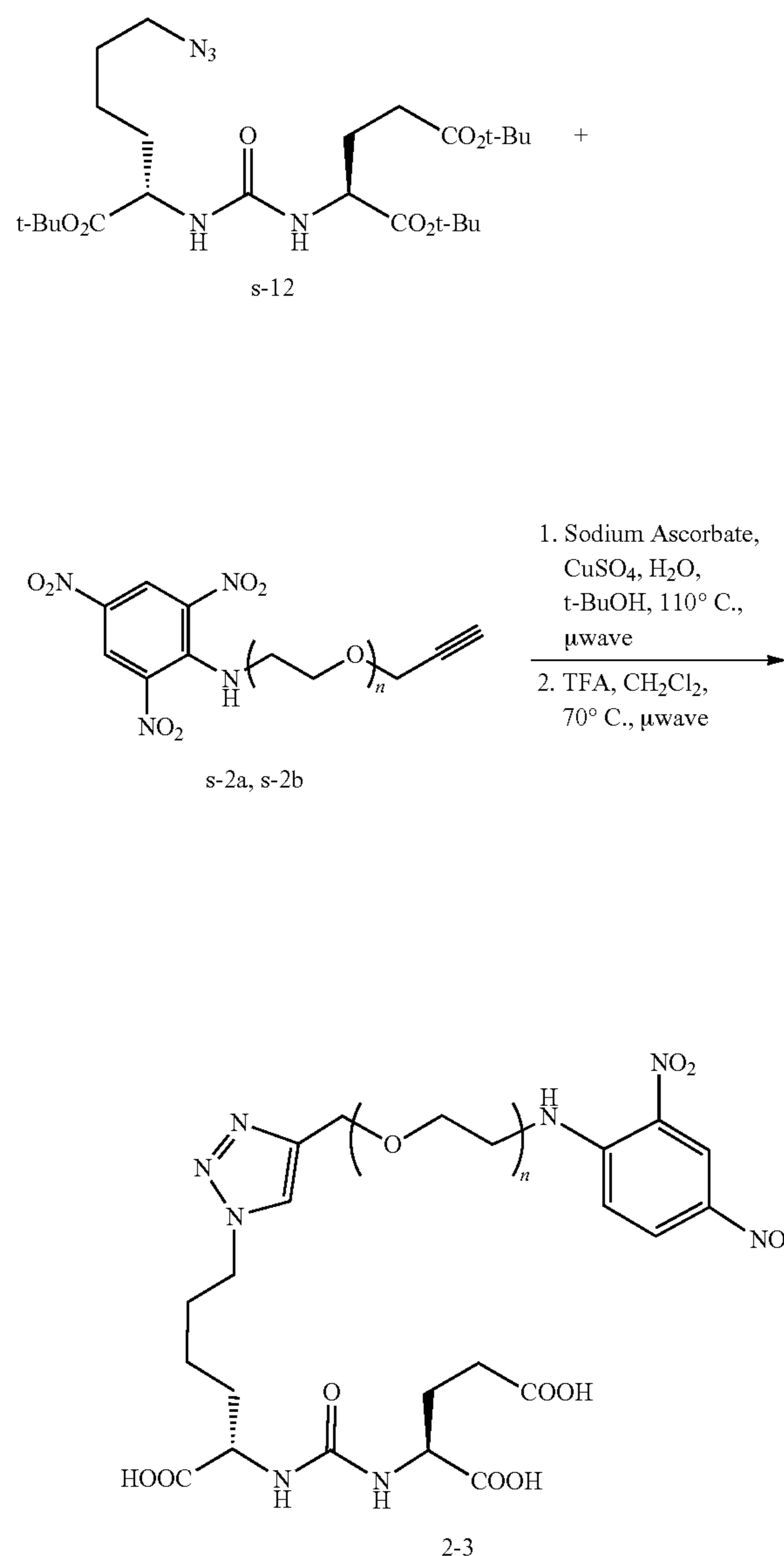
Scheme S-4: General synthesis of 2 and 3. (2, n = 1; 3, n = 2).
