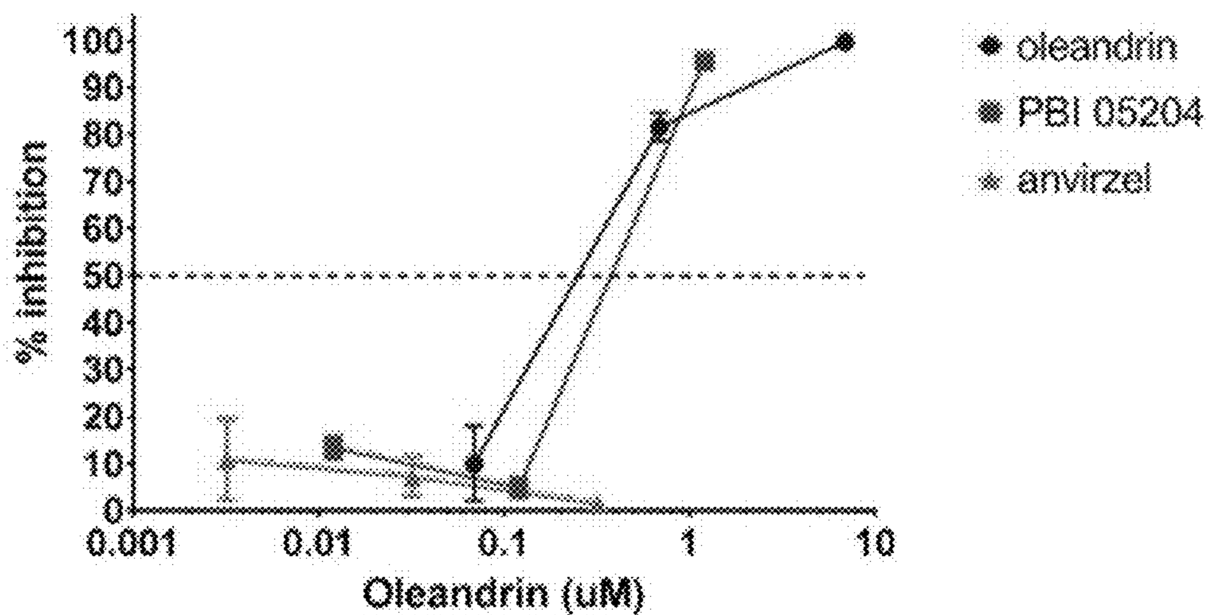
Inhibition of EBOV after passaging
