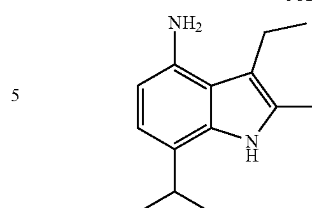
3-ethyl-2-methyl-7-(propan-2-yl)-1H-indol-4-amine
