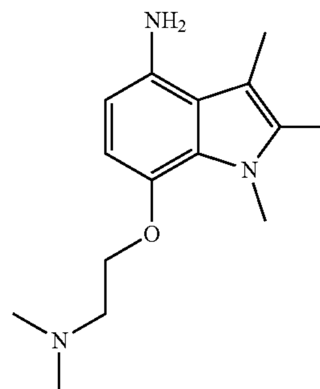
7-[2-(dimethylamino)ethoxy]-1,2,3-trimethyl-1H-indol-4-amine
