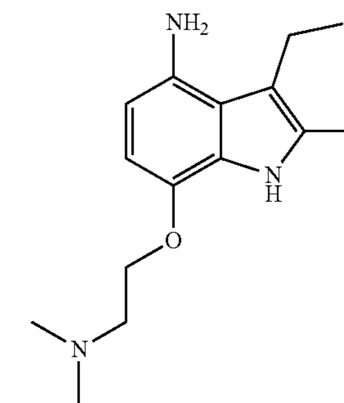
7-[2-(dimethylamino)ethoxy]-3-ethyl-2-methyl-1H-indol-4-amine
