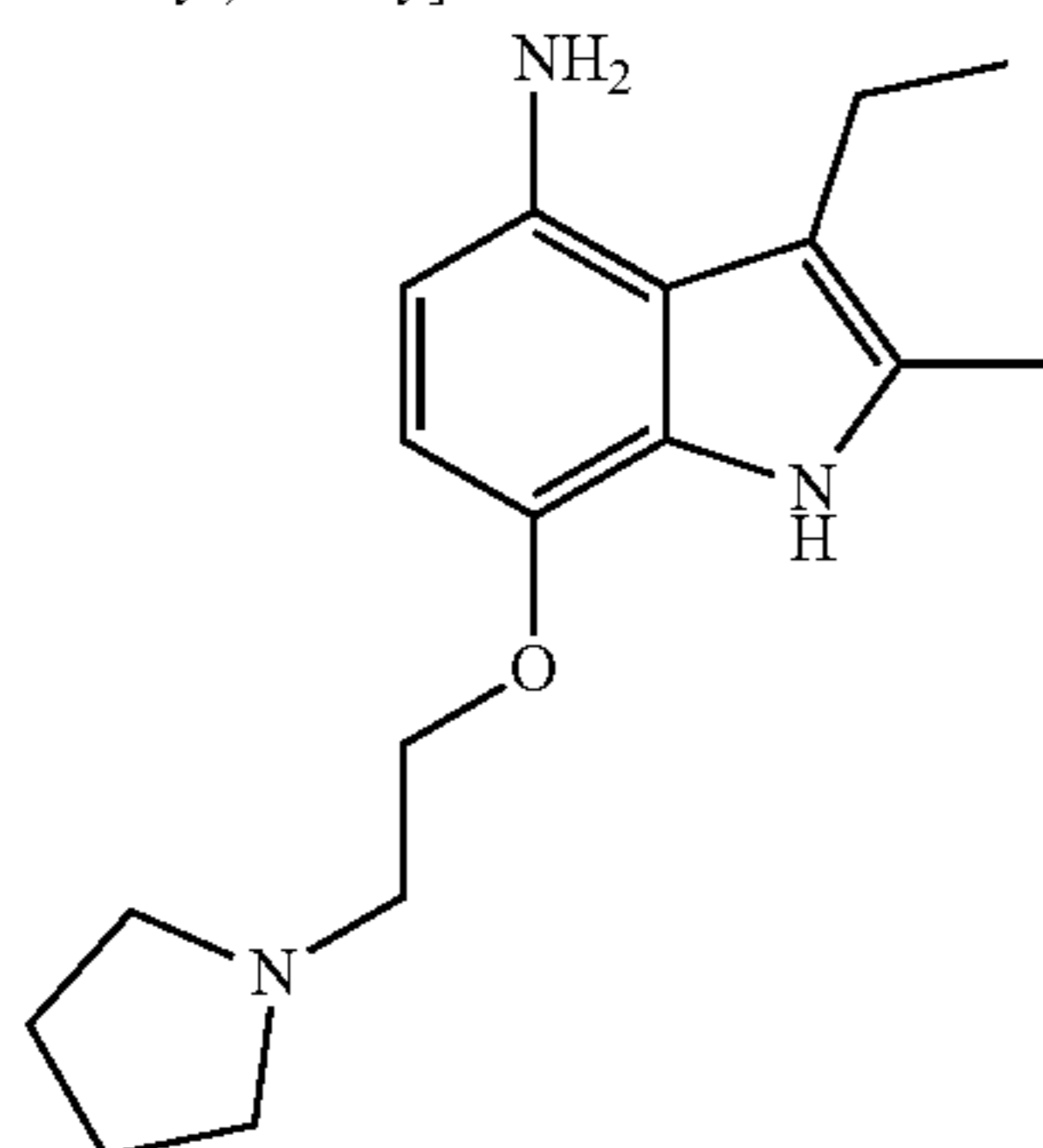
3-ethyl-2-methyl-7-[2-(pyrrolidin-1-yl)ethoxy]-1H-indol-4-amine
