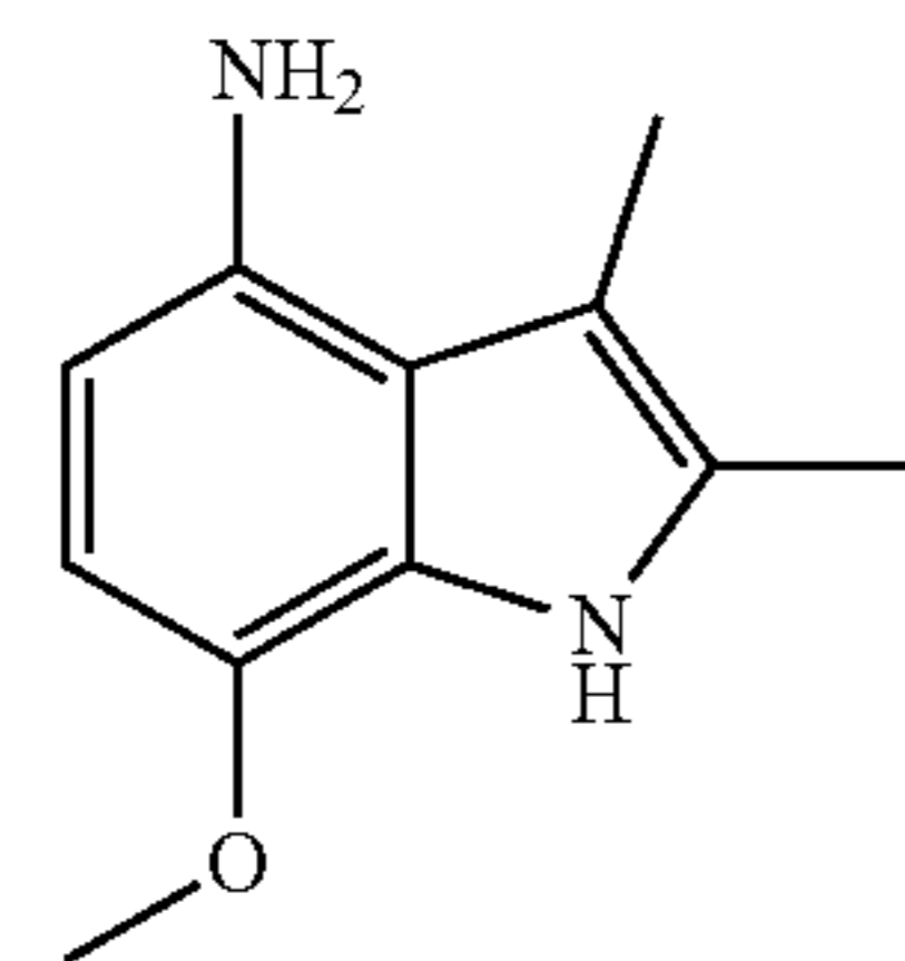
7-methoxy-2,3-dimethyl-1H-indol-4-amine
