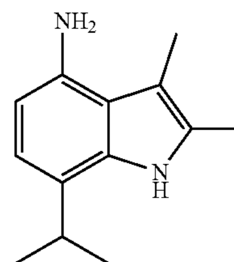
60 2,3-dimethyl-7-(propan-2-yl)-1H-indol-4-amine
