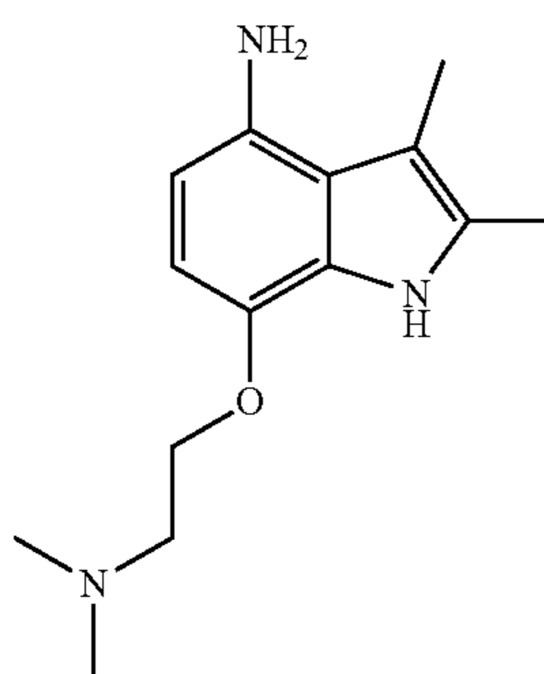
7-[2-(dimethylamino)ethoxy]-2,3-dimethyl-1H-indol-4-amine
