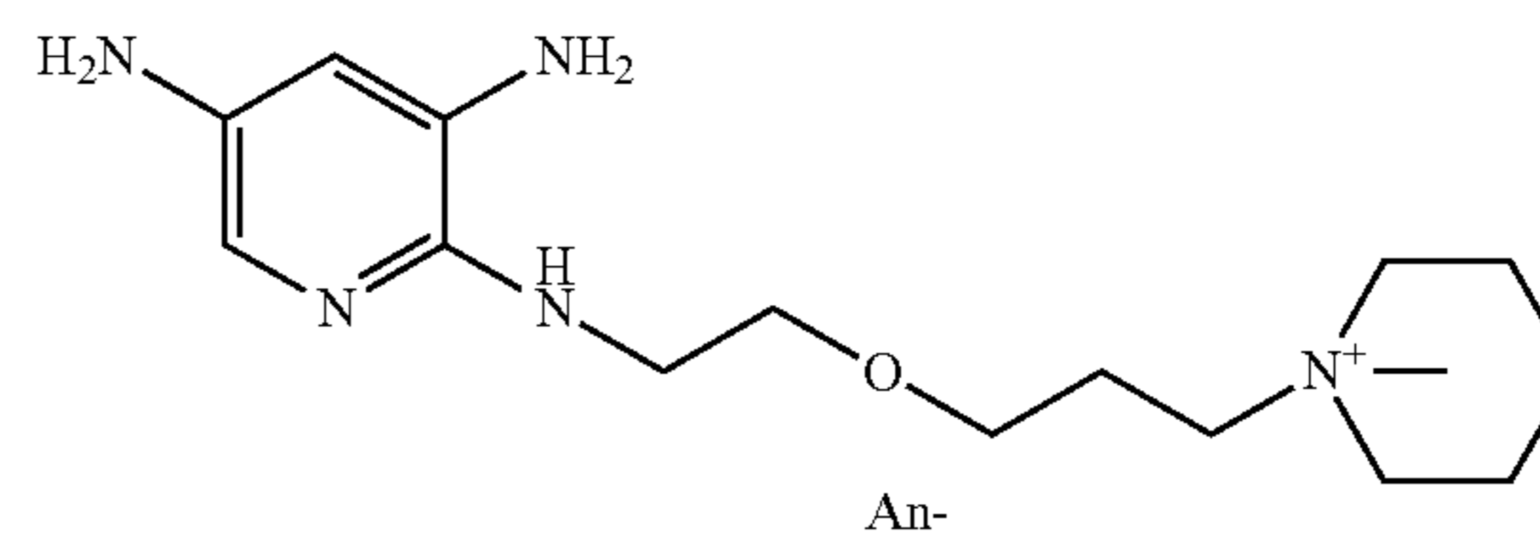
1-(3-((2-[(3,5-diaminopyridin-2-yl)amino]ethoxy)propyl)-1-methylpiperidinium, An -
