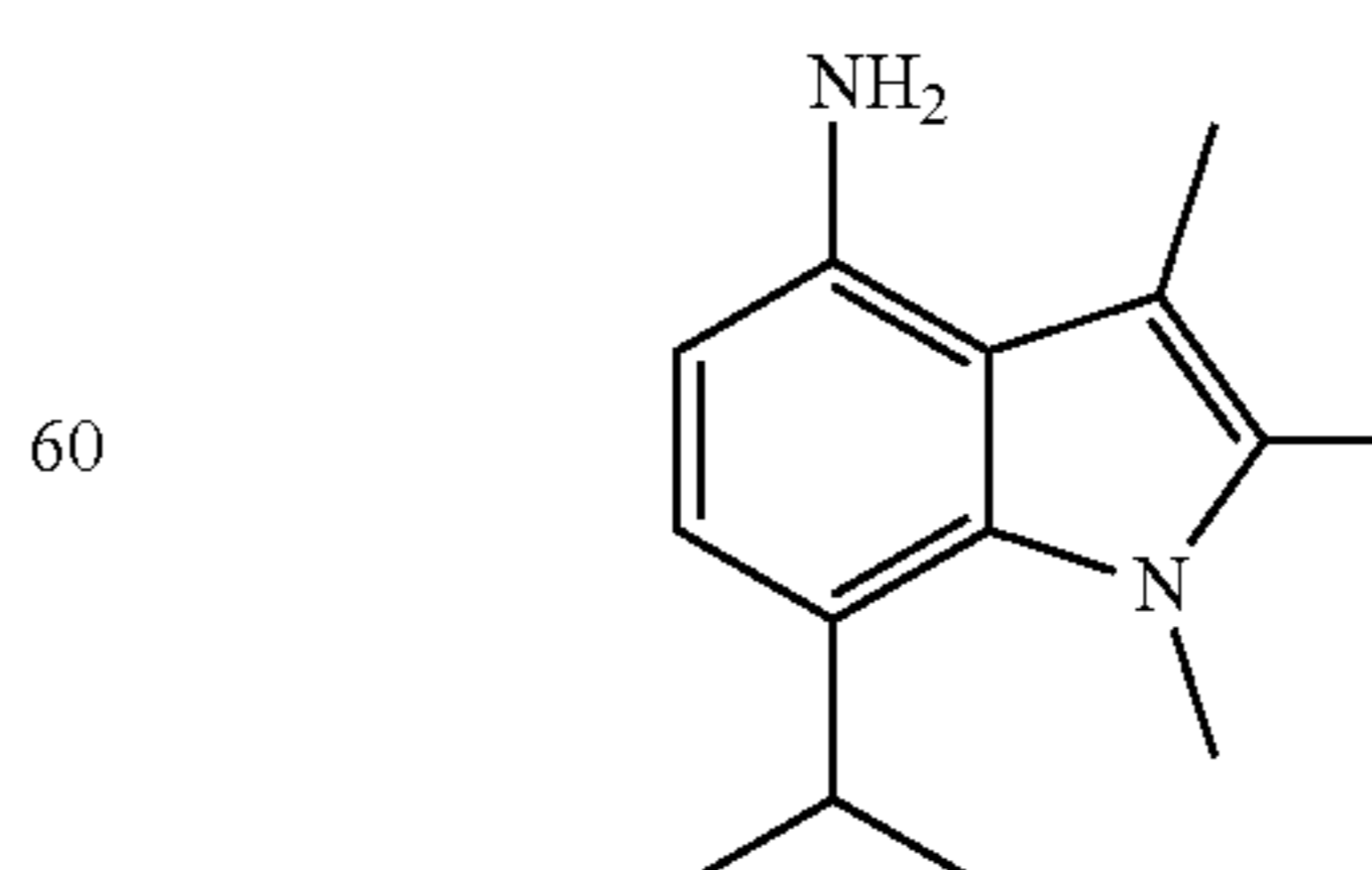
1,2,3-trimethyl-7-(propan-2-yl)-1H-indol-4-amine
