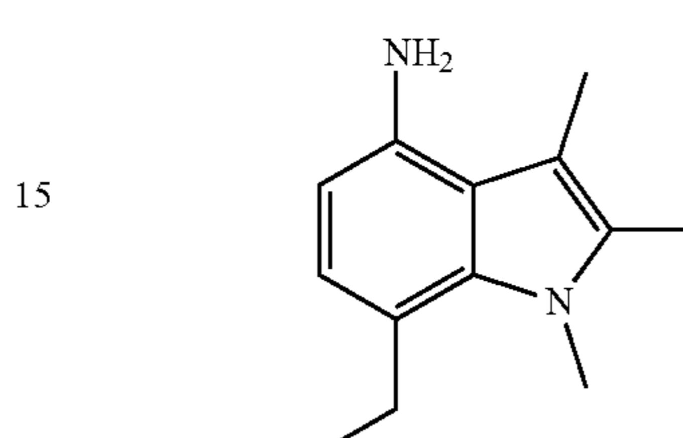
7-ethyl-1,2,3-trimethyl-1H-indol-4-amine
