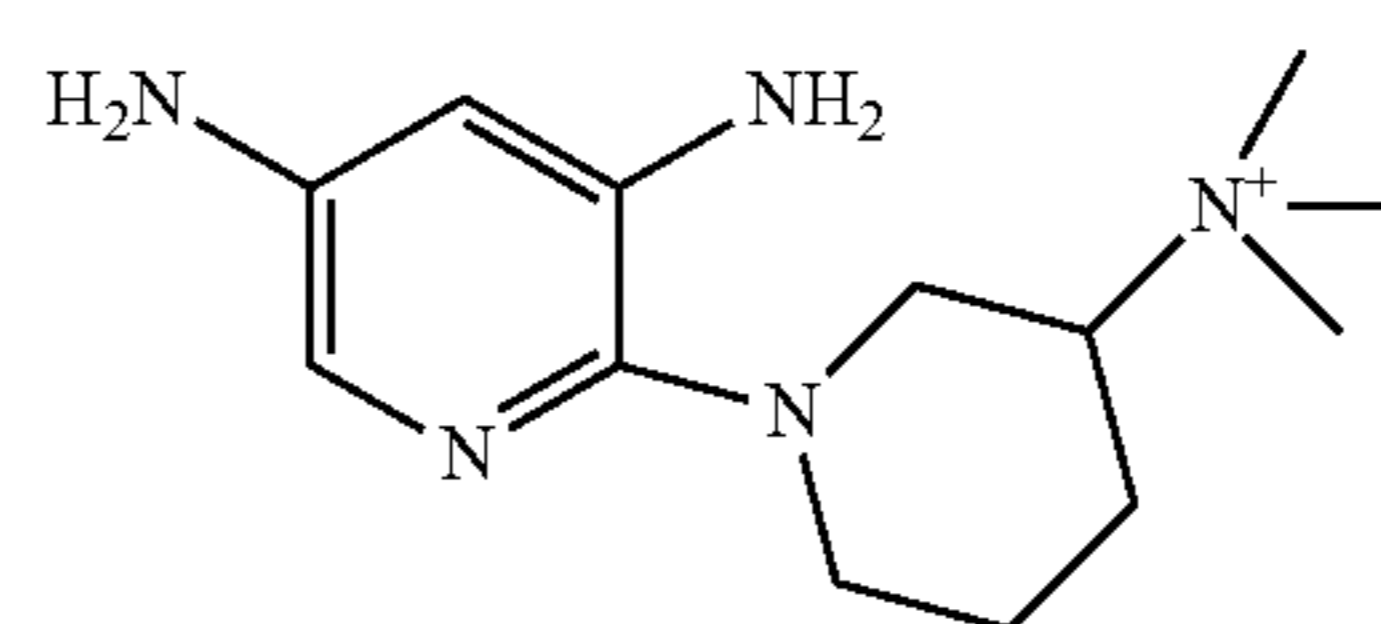
(3,5-diaminopyridin-2-yl)-3-trimethylpiperidinammonium, An -
