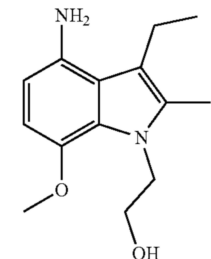
2-(4-amino-3-ethyl-7-methoxy-2-methyl-1H-indol-1-yl)ethanol
