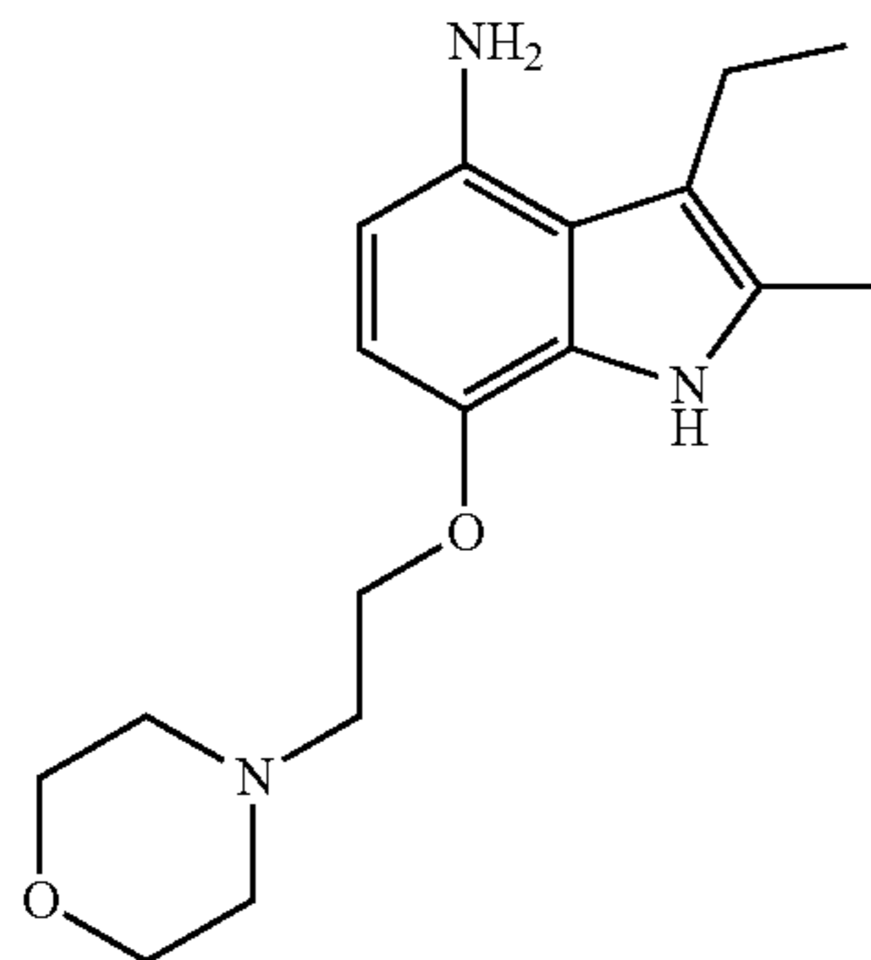
3-ethyl-2-methyl-7-[2-(morpholin-4-yl)ethoxy]-1H-indol-4-amine
