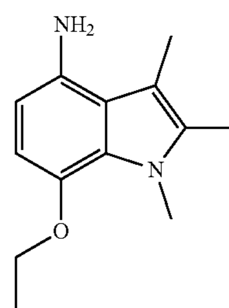
7-ethoxy-1,2,3-trimethyl-1H-indol-4-amine
