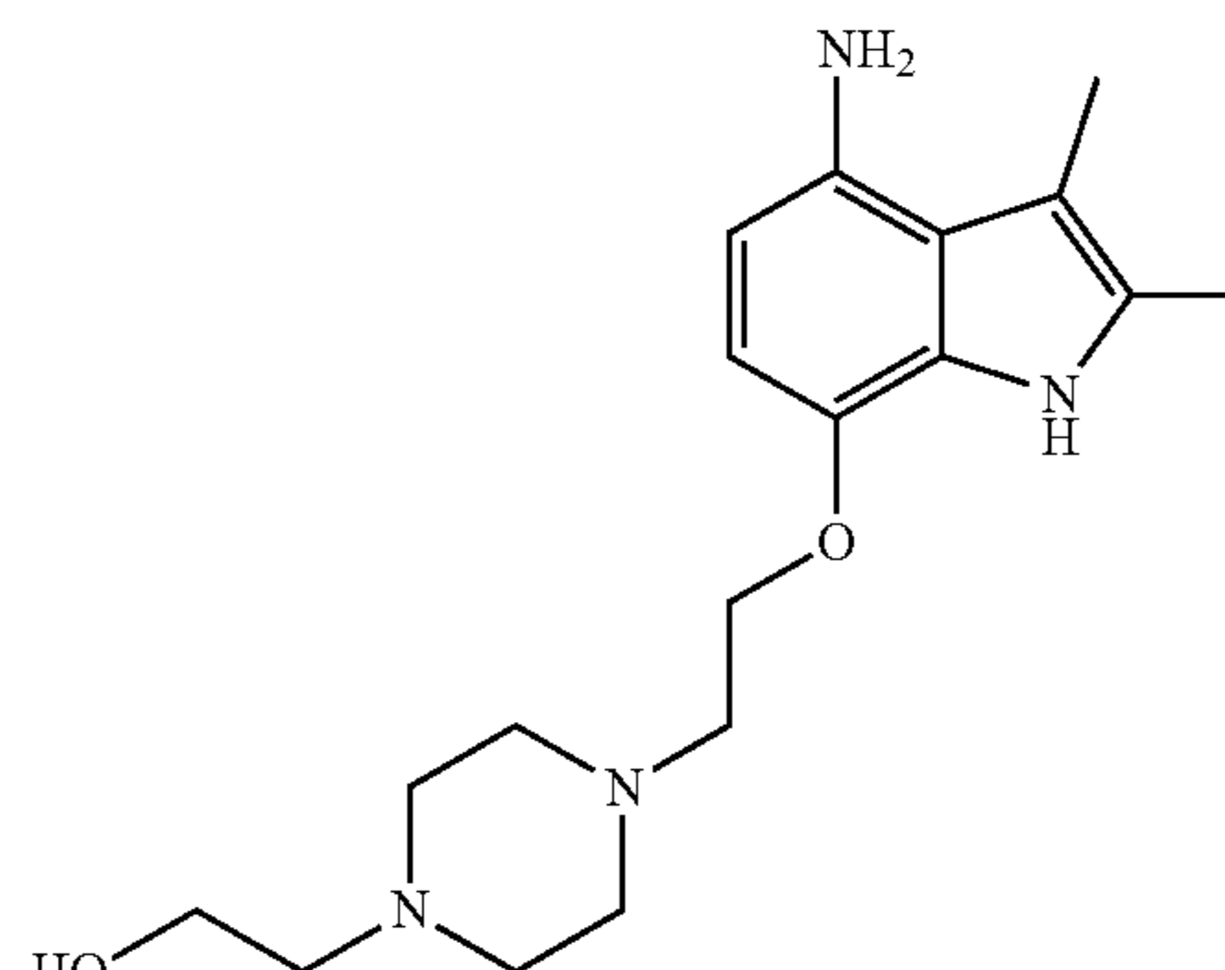
2-(4-{2-[(4-amino-2,3-dimethyl-1H-indol-7-yl)oxy]ethyl}piperazin-1-yl)ethanol
