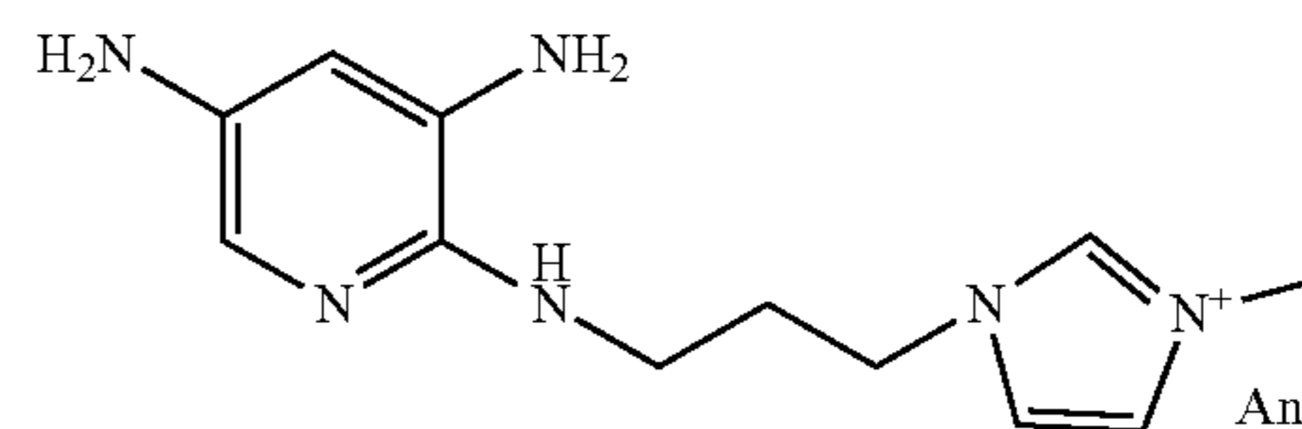
1-(3-[(3,5-diaminopyridin-2-yl)amino]propyl)-3-methyl-1H-imidazol-3-ium, An -
