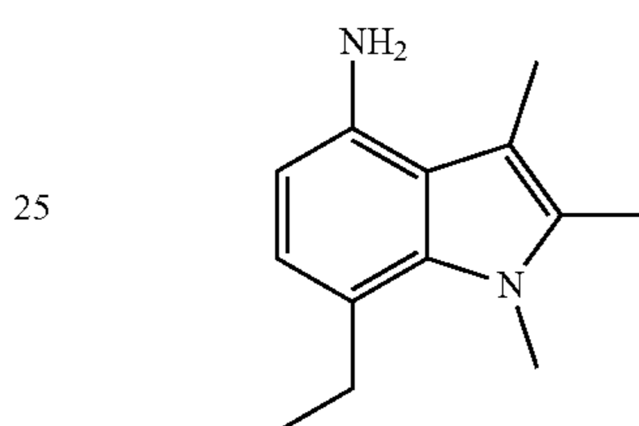
3,7-diethyl-1,2-dimethyl-1H-indol-4-amine
