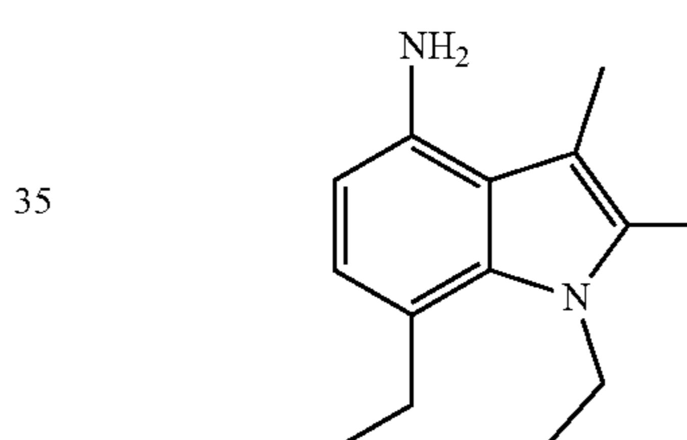
3,7-diethyl-1,2-dimethyl-1H-indol-4-amine
