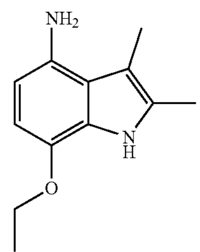
7-ethoxy-2,3-dimethyl-1H-indol-4-amine
