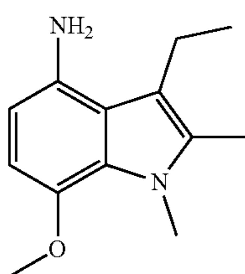
3-ethyl-7-methoxy-1,2-dimethyl-1H-indol-4-amine
