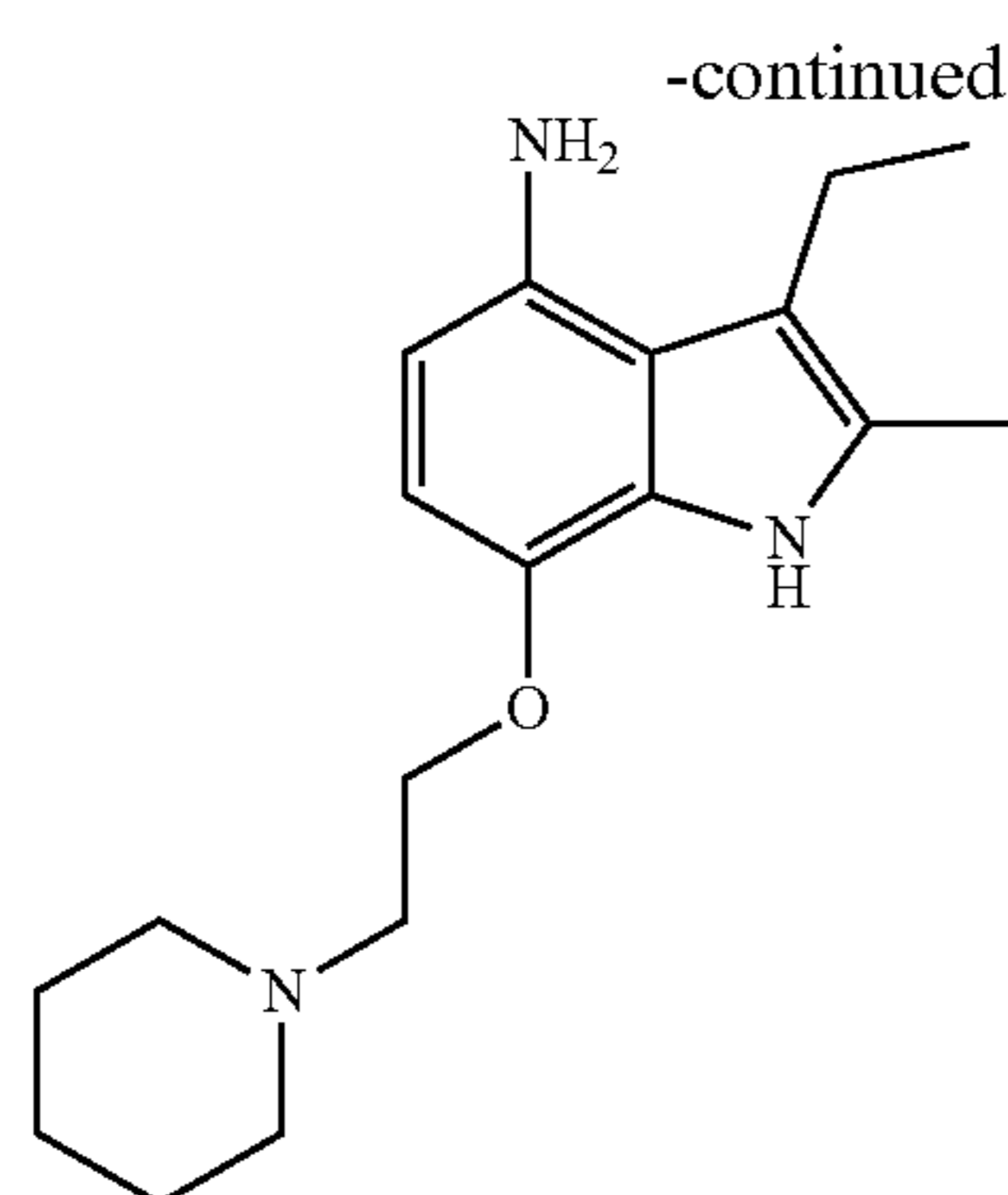
3-ethyl-2-methyl-7-[2-(piperidin-1-yl)ethoxy]-1H-indol-4-amine
