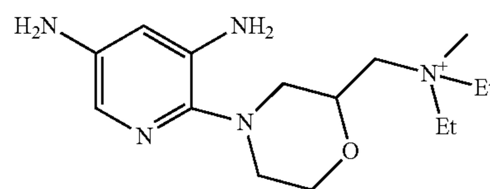
4-(3,5-diaminopyridin-2-yl)-(2-trimethylethan)-morpholin-ammonium, An -
