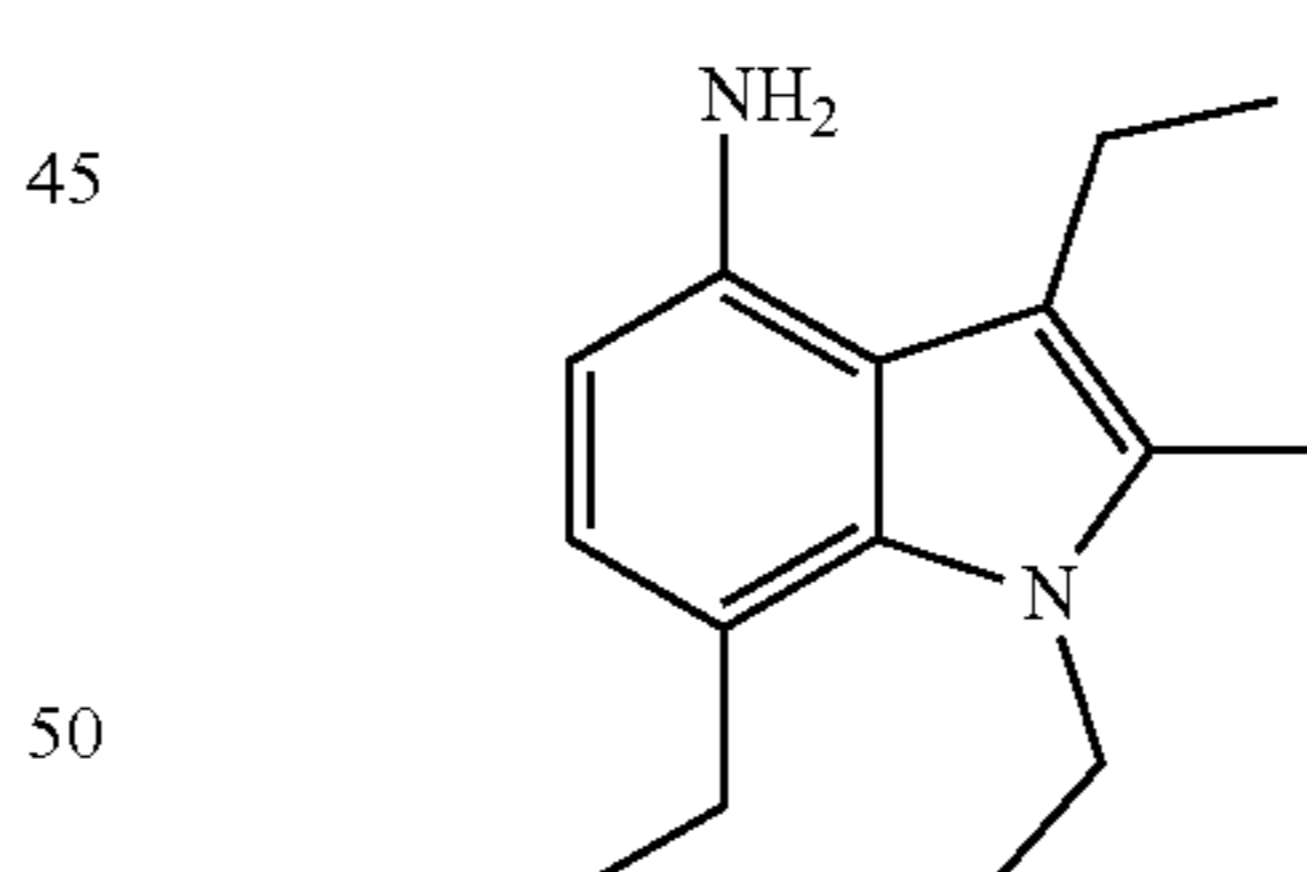
2-(4-amino-7-ethyl-2,3-dimethyl-1H-indol-1-yl)ethanol
