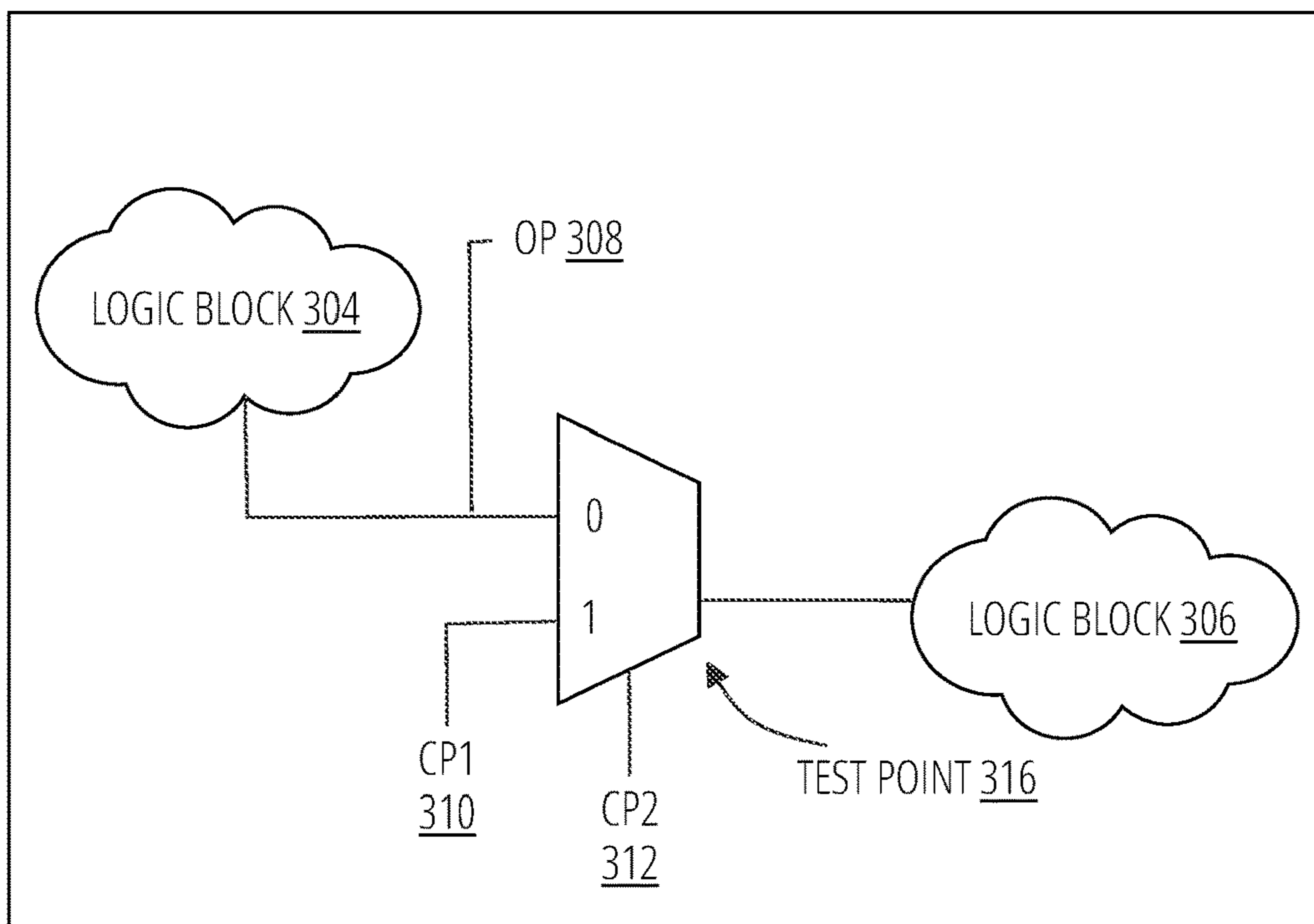
MODIFIED CIRCUIT 302
