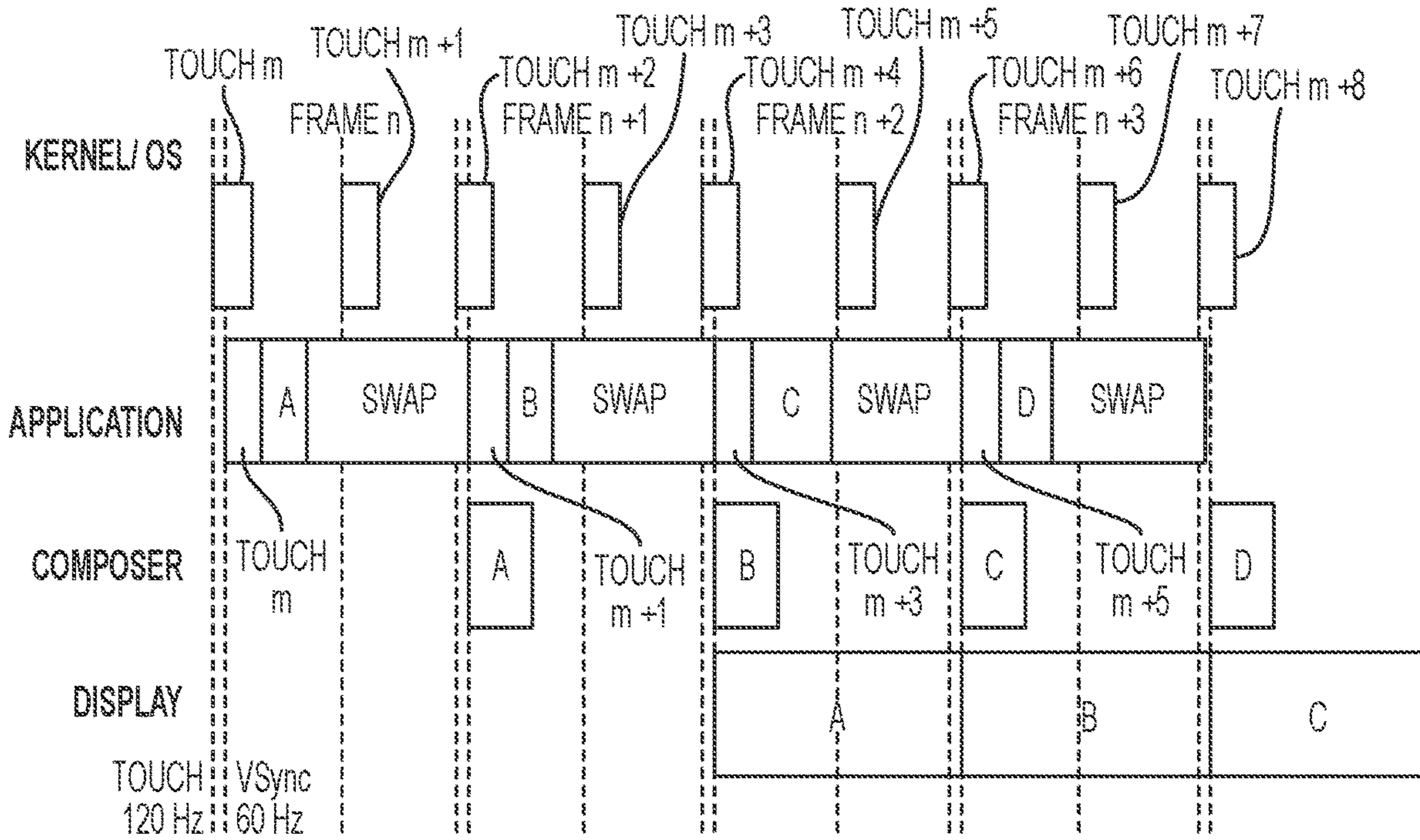
FIG. 2 PRIOR ART
