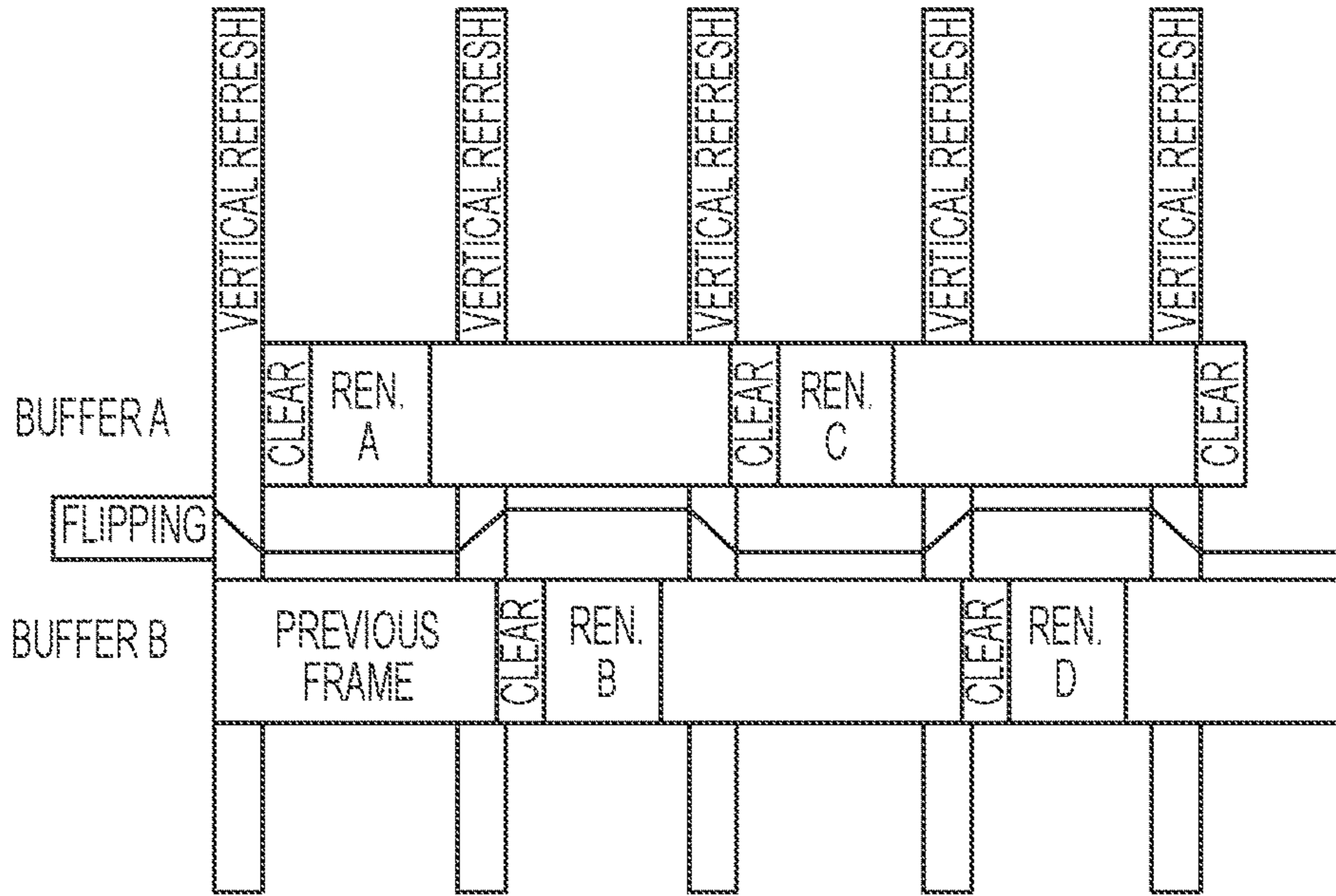
FIG. 1 PRIOR ART
