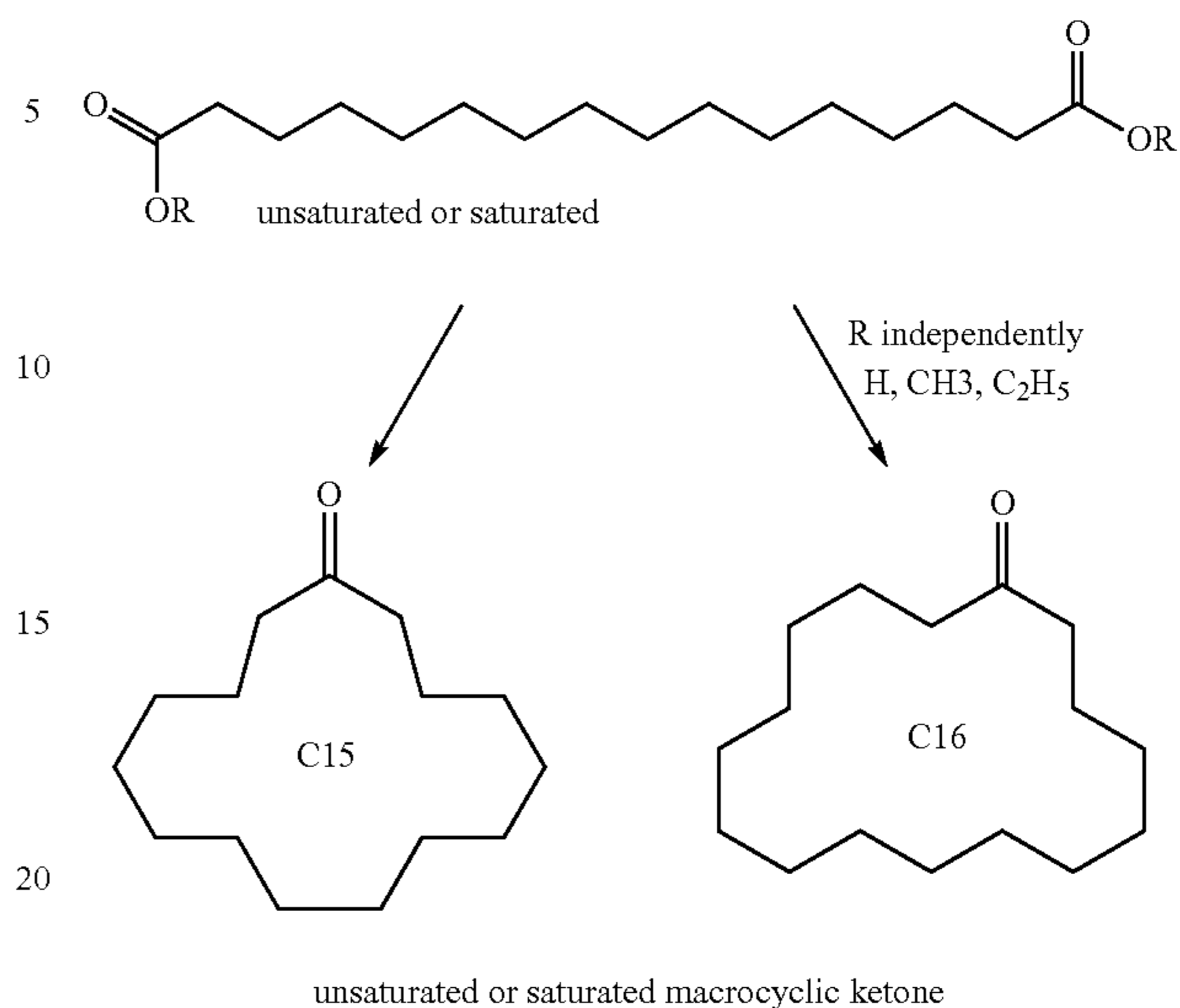
Scheme VII
