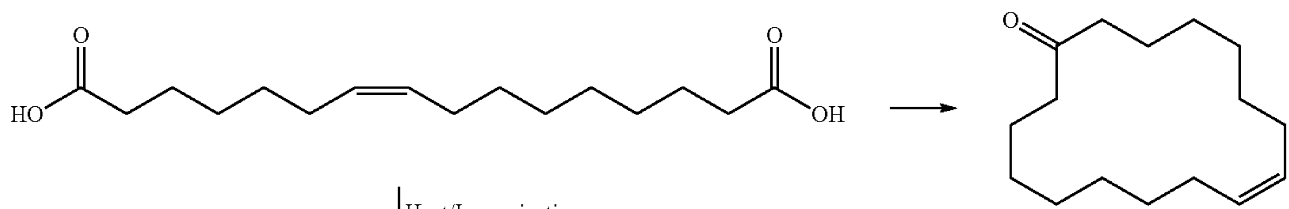
Scheme IX
