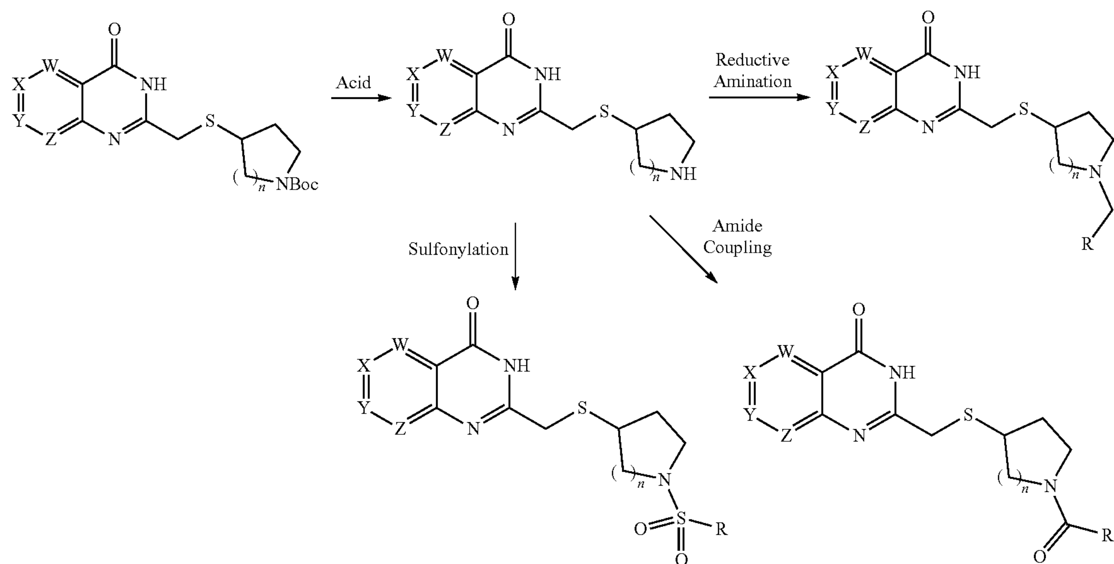
Scheme 12
