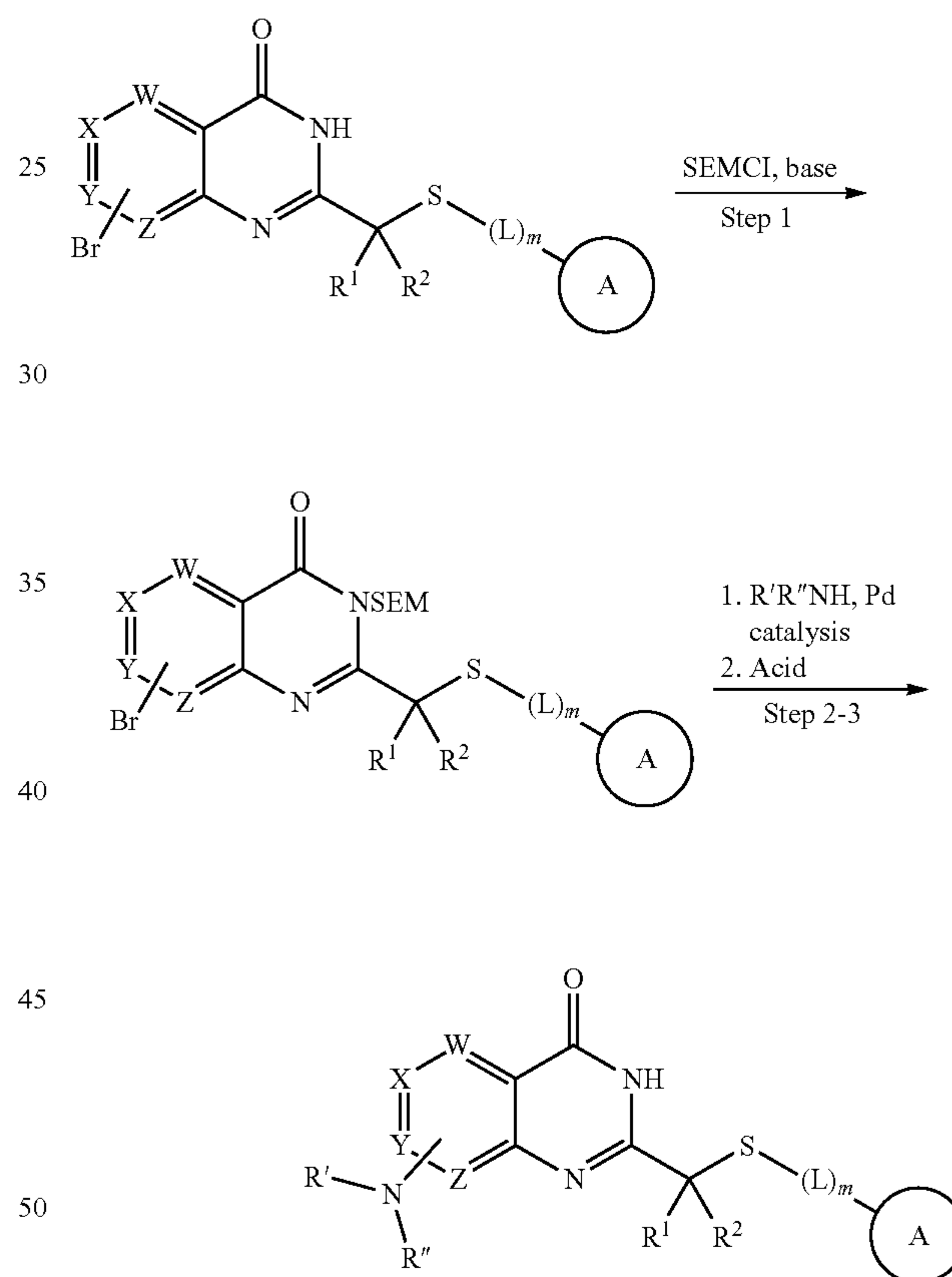
Scheme 6
