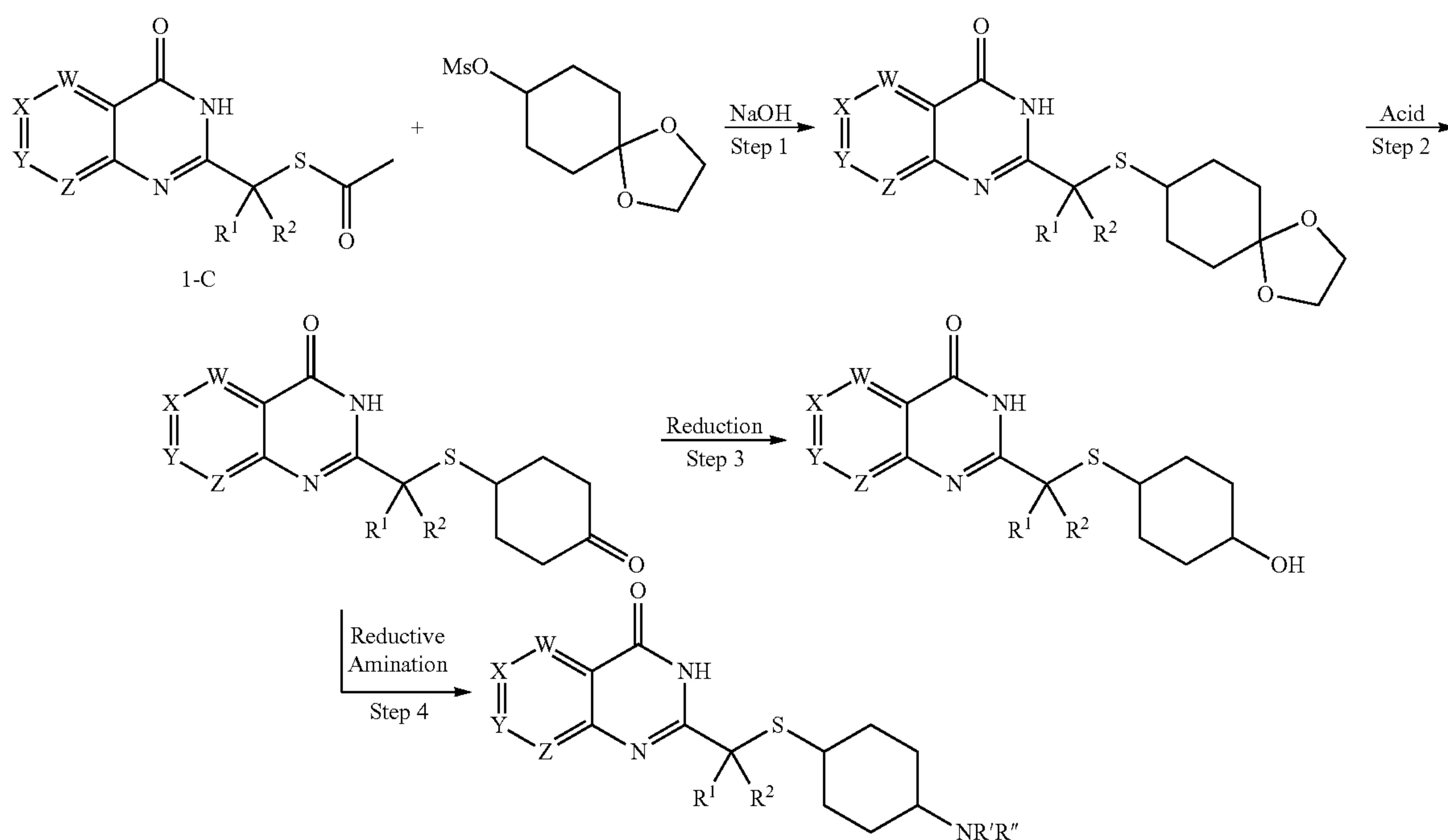
Scheme 13
