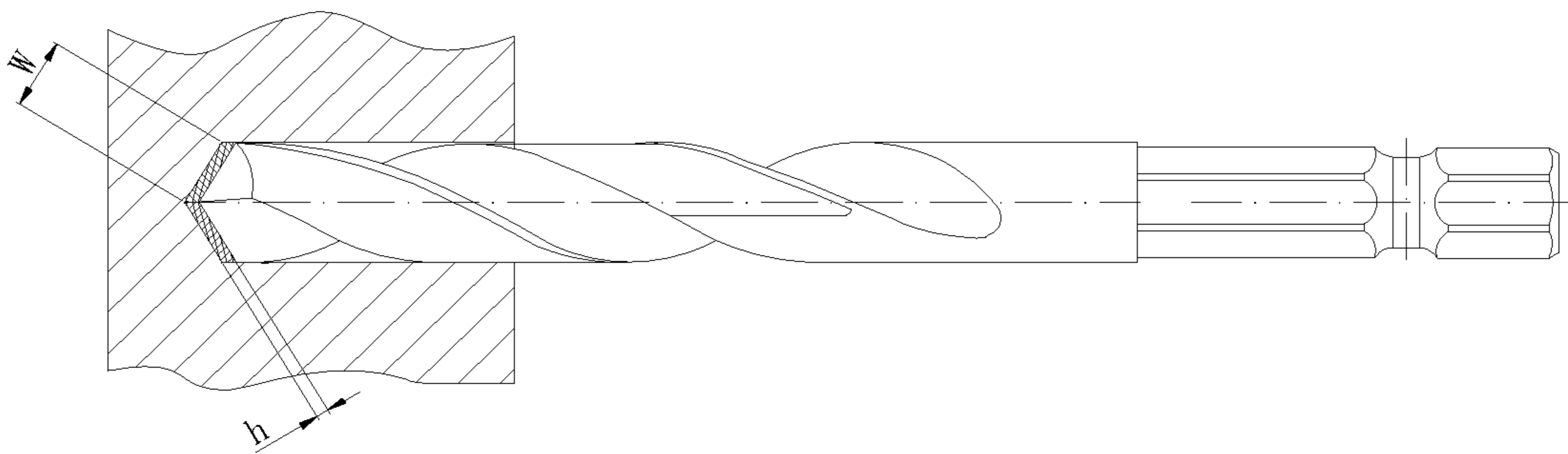
FIG. 2 (Prior Art)
