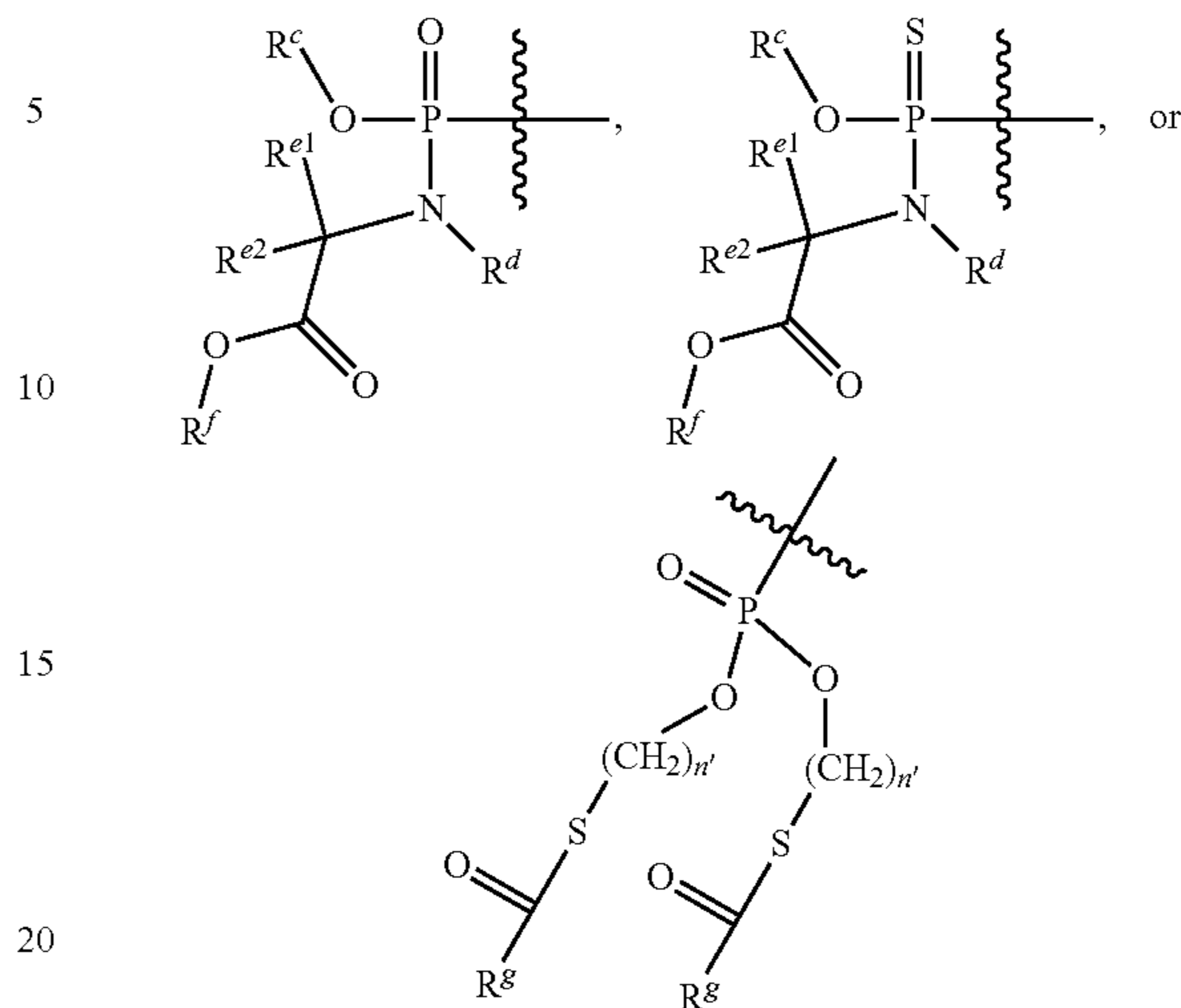
Formula I
