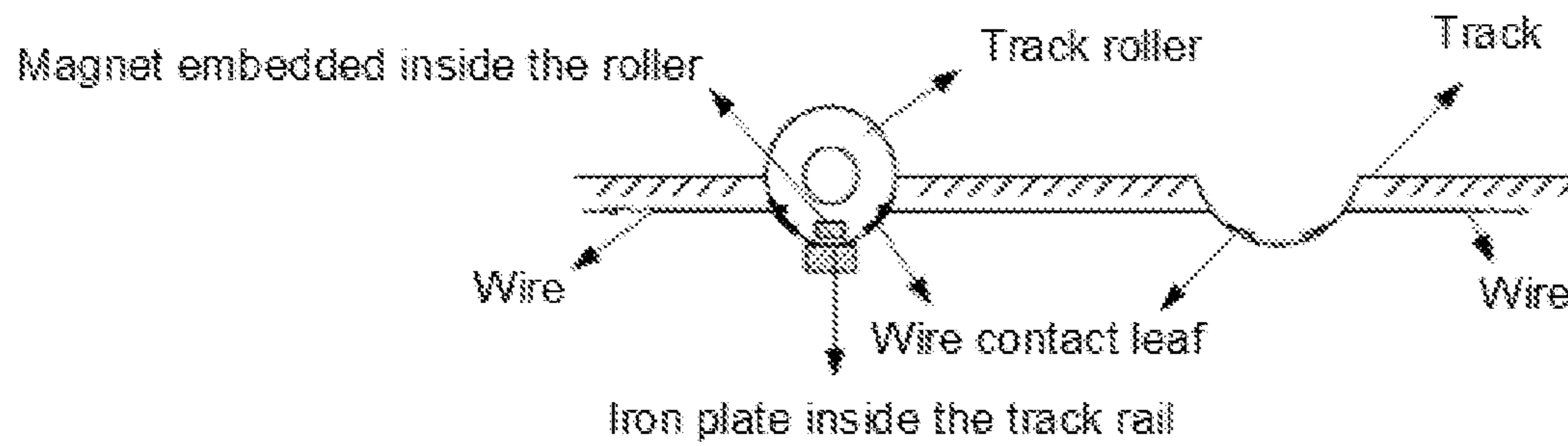
Front view of track roller inside the track rail
