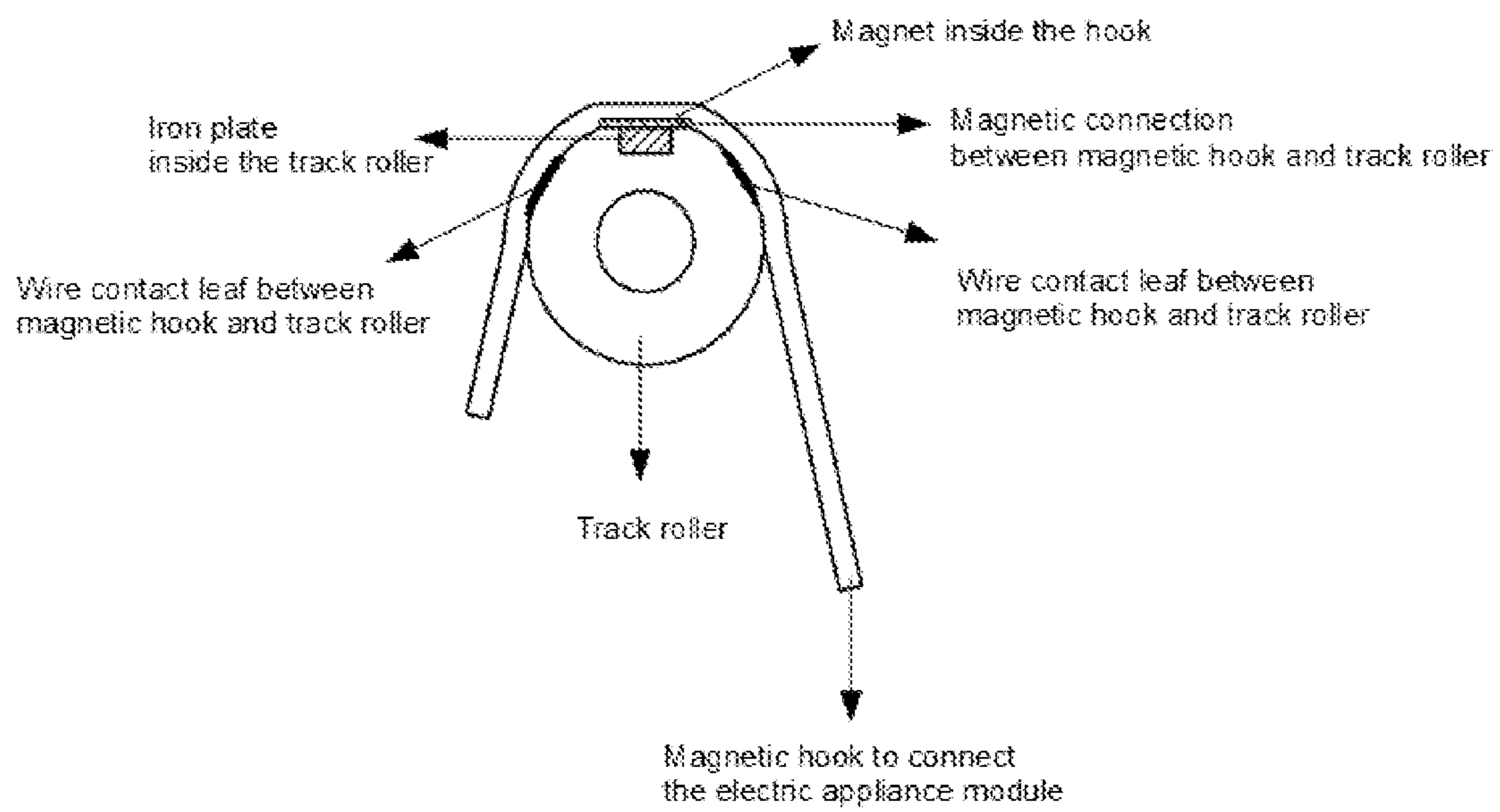
Side view of magnetic hook connecting the track roller
