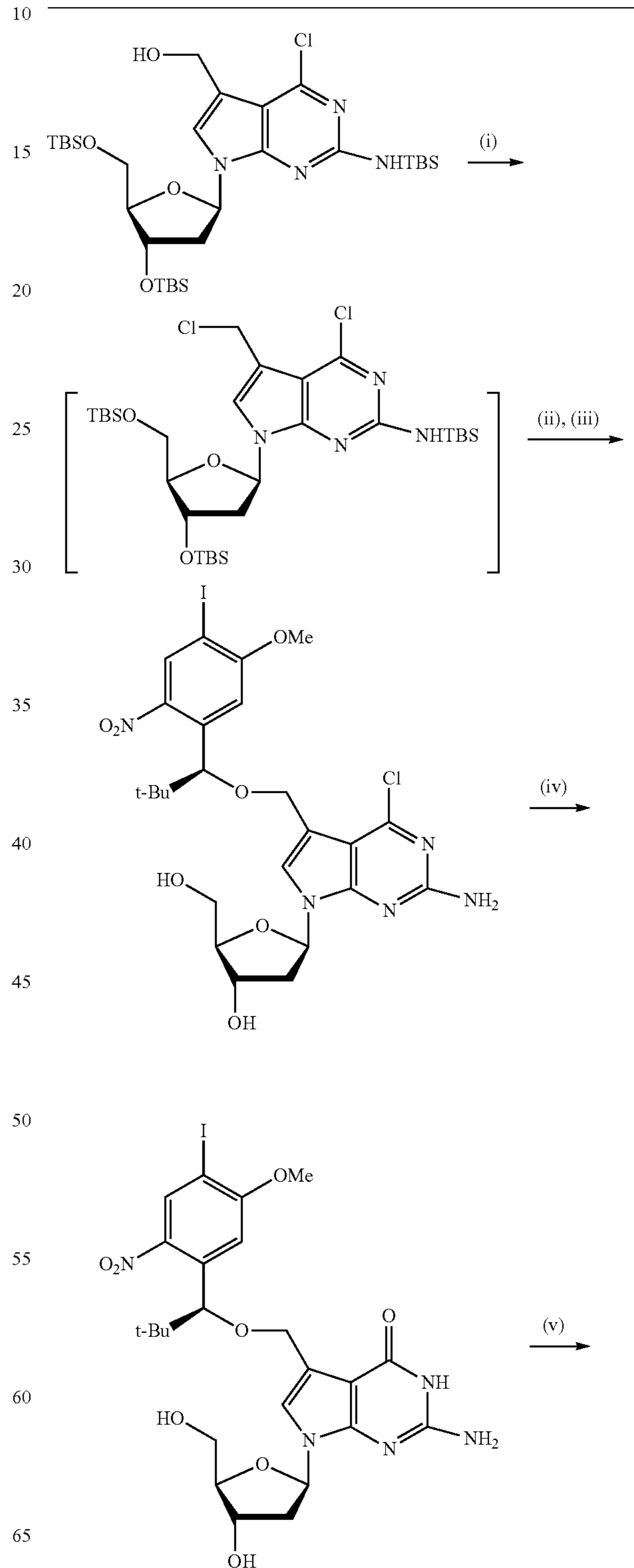
Scheme 4a. Synthesis of dye labeled 7-[(S)-1-(5-methoxy-2-nitrophenyl)-2,2-dimethyl-propyloxy]methyl-7-deaza-2'-deoxyguanosine-5'-triphosphate.
