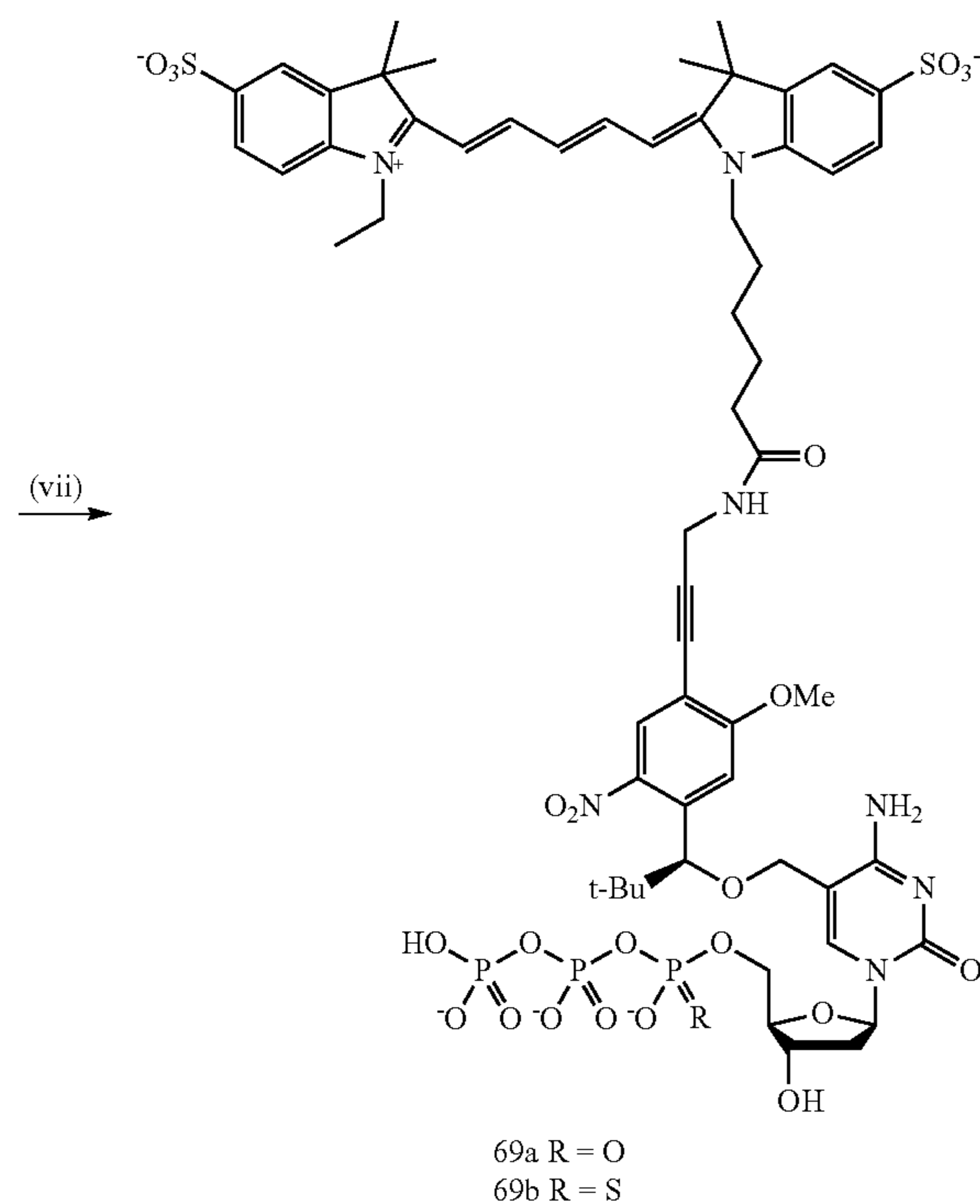
Scheme S28b.
