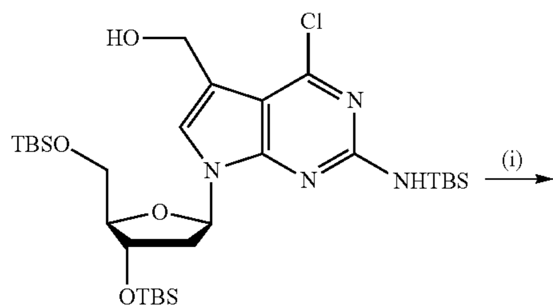
Scheme S16. Synthesis of 7-[1-(5-methoxy-2-nitrophenyl)-2,2-dimethyl-propyloxy]methyl-7-deaza-2'-deoxyguanosine-5'-triphosphate.
