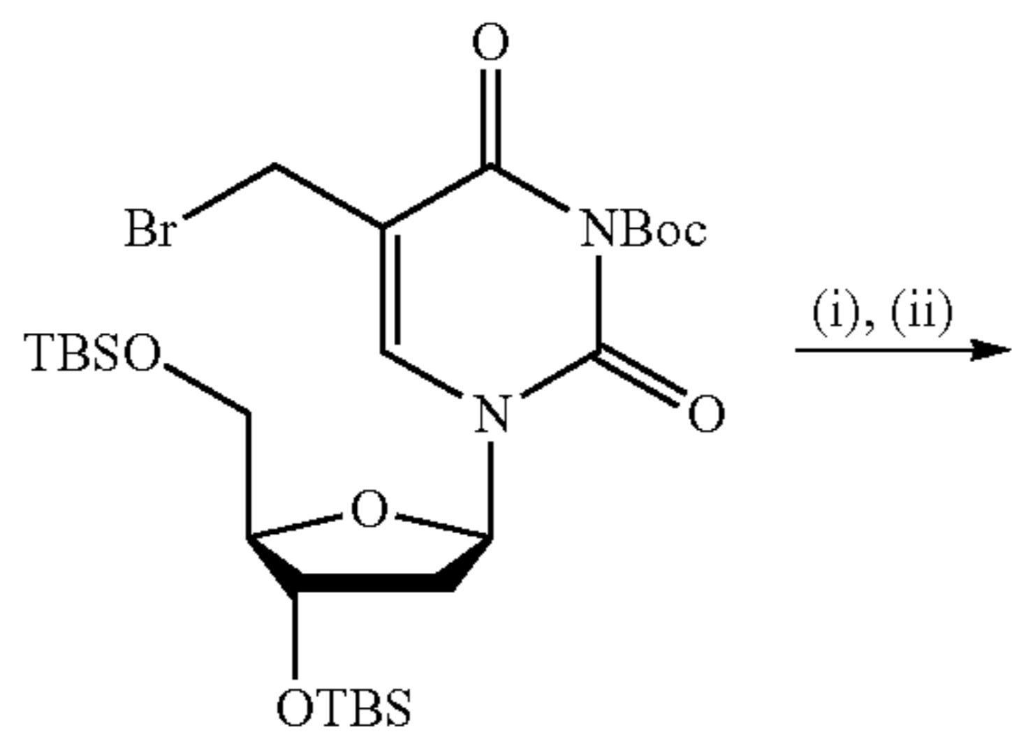
Scheme 3a. Synthesis of dye labeled 5-[(S)-1-(5-methoxy-2-nitrophenyl)-2,2-dimethyl-propyloxy]methyl-2'-deoxyuridine-5'-triphosphate.
