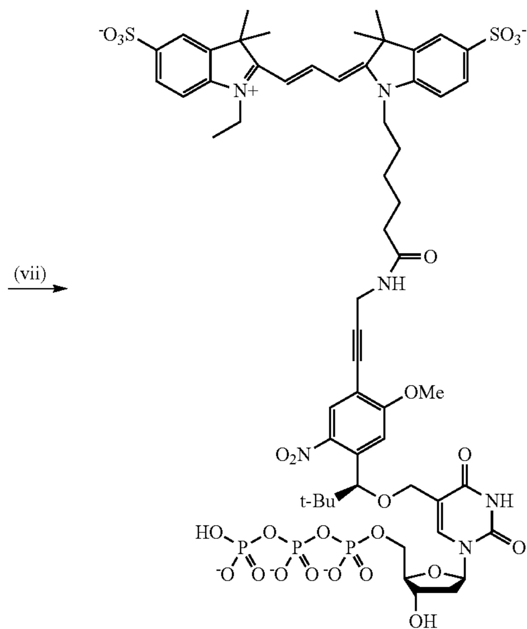
Scheme 3d.
