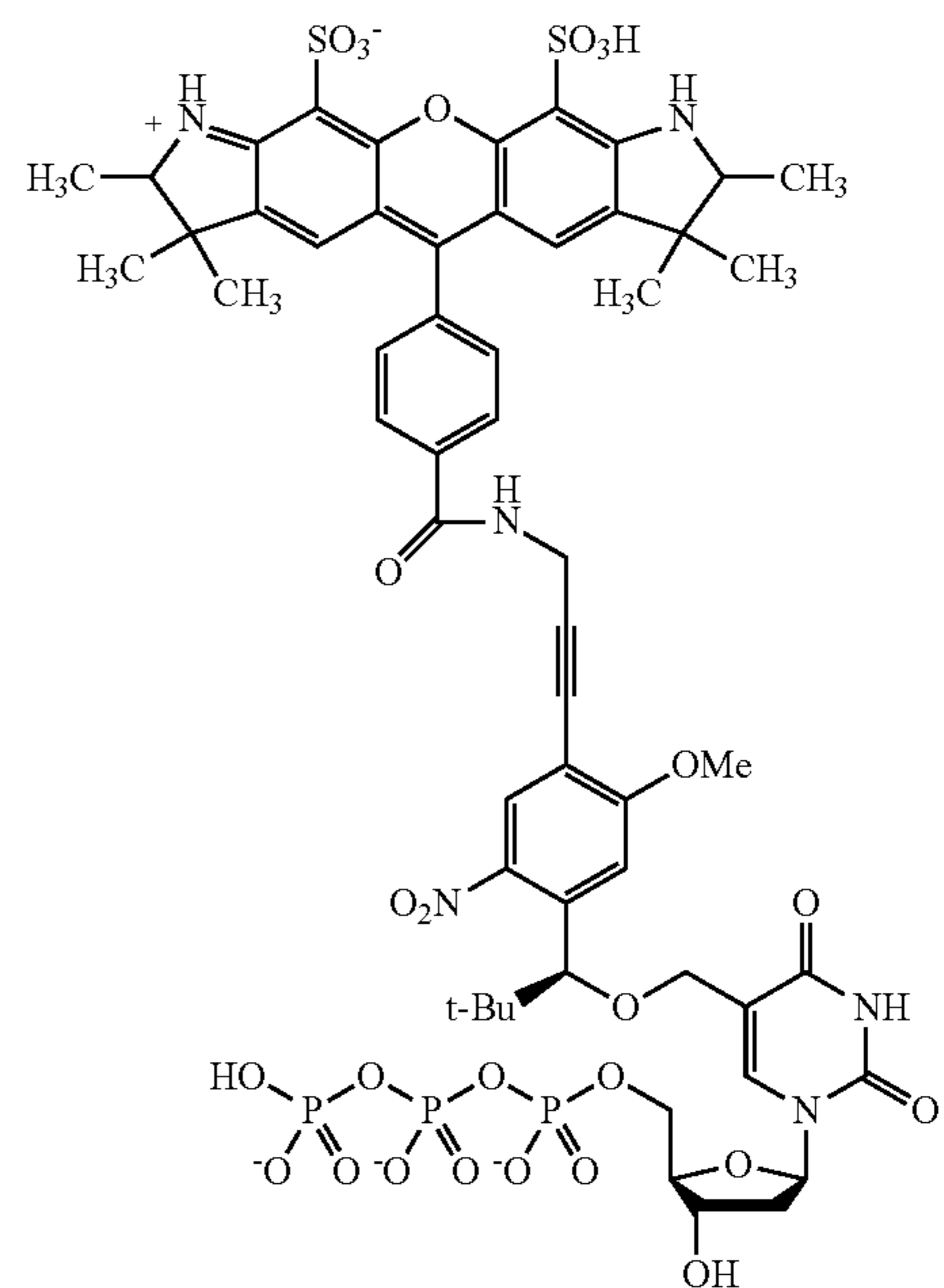
Scheme 3b.
