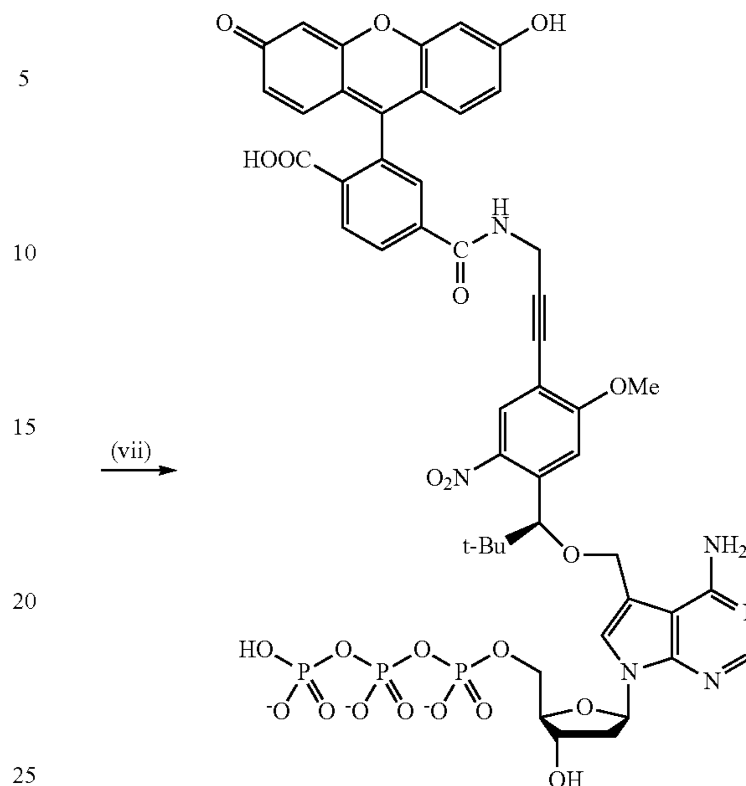
Scheme 2c.
