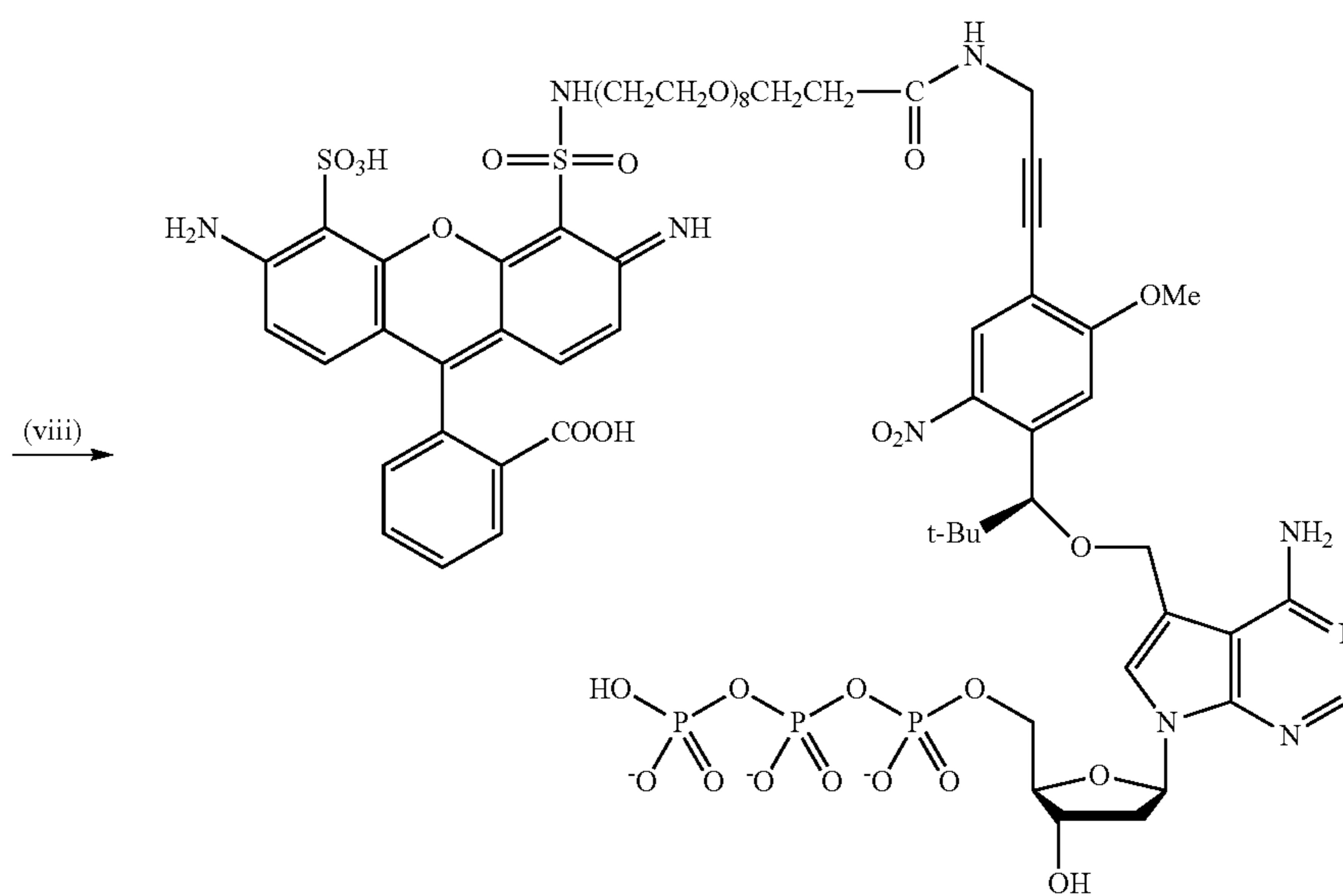
Scheme 2d.
