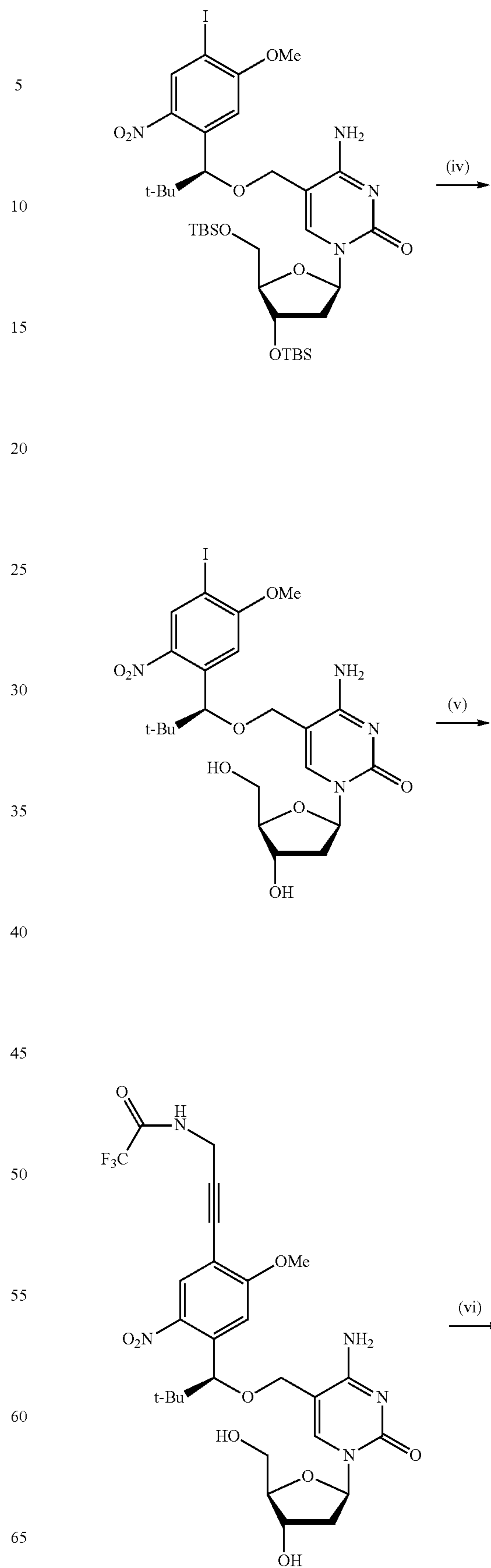
Scheme 5a. Synthesis of dye labeled 5-[(S)-1-(5-methoxy-2-nitrophenyl)-2,2-dimethyl-propyloxy]methyl-2'-deoxycytidine-5'-triphosphate.
