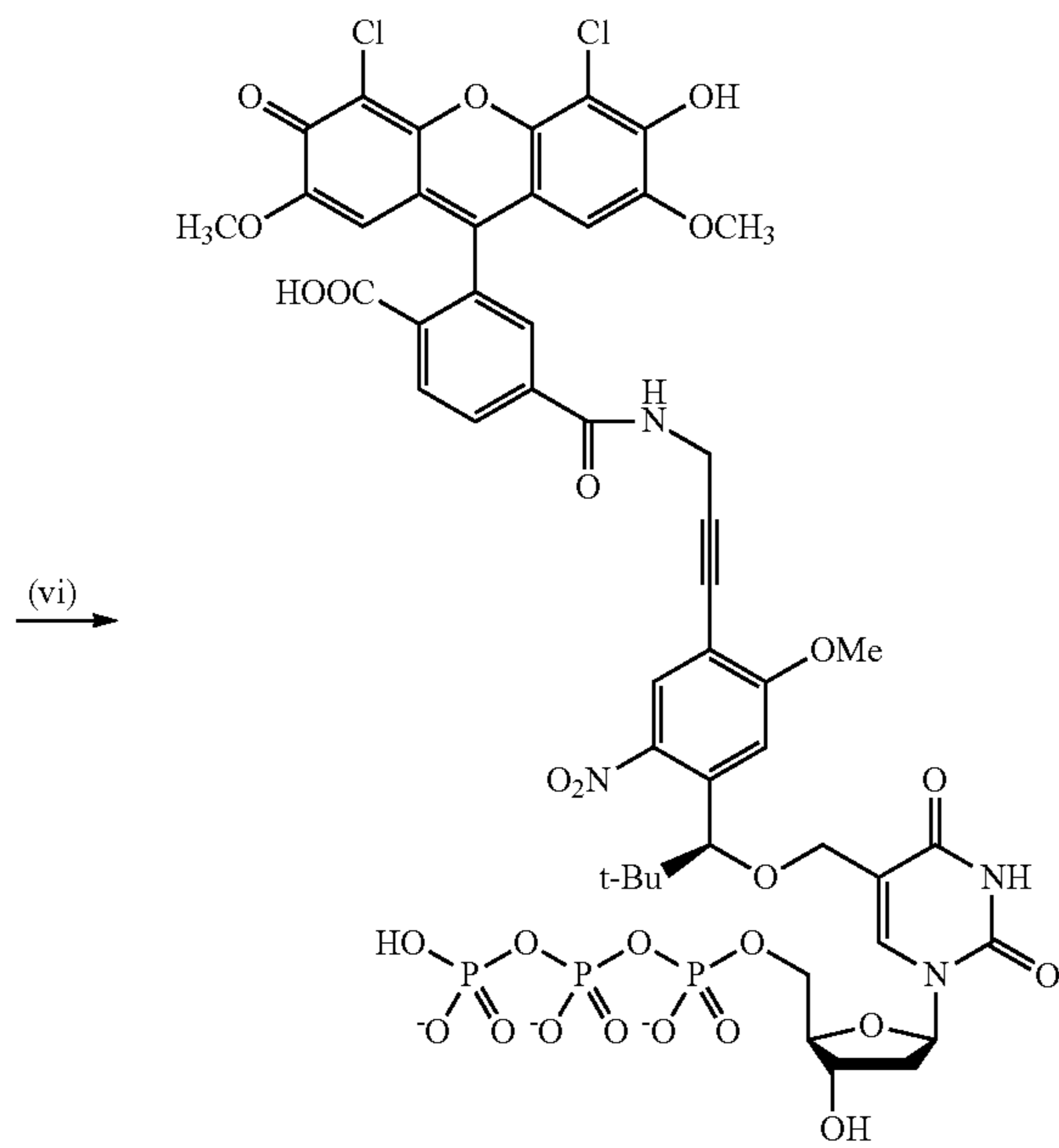
Scheme 3c.
