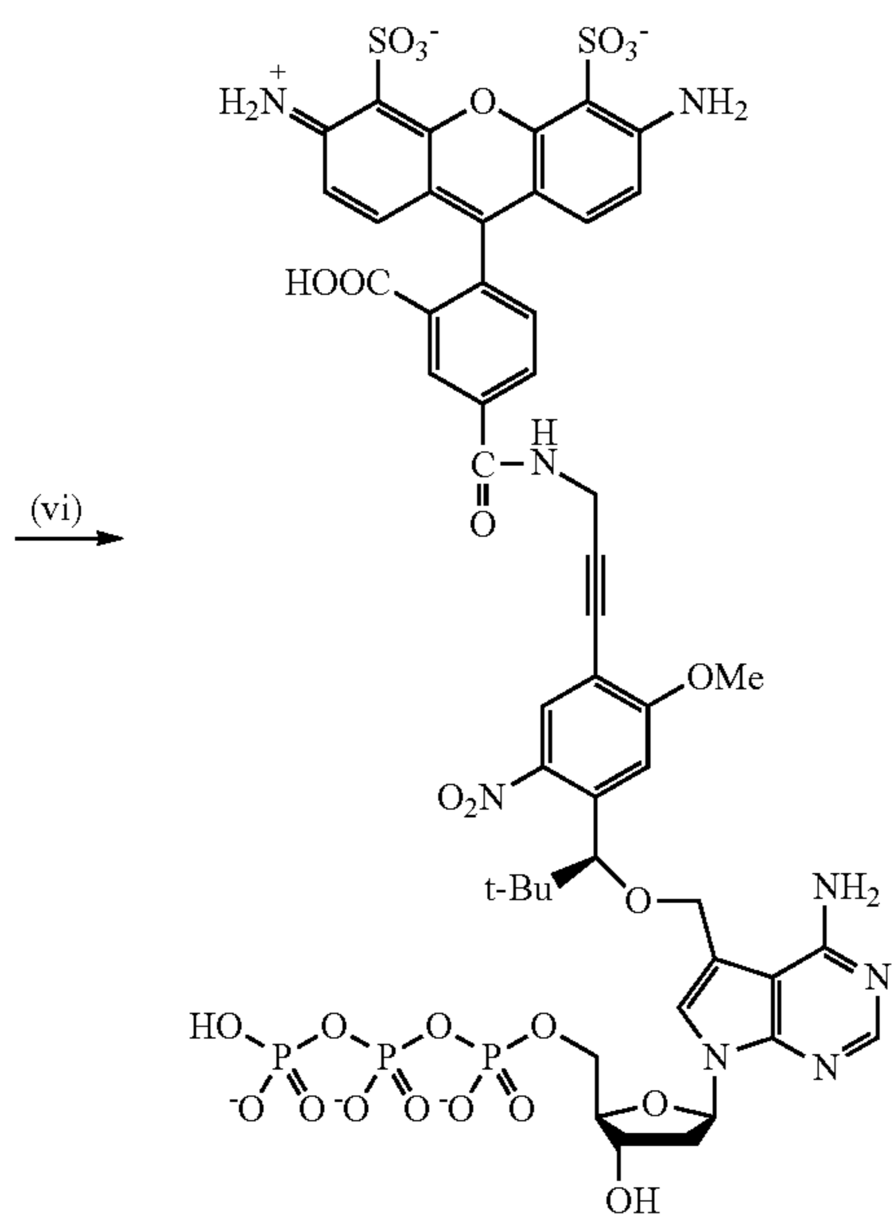
Scheme 2b.
