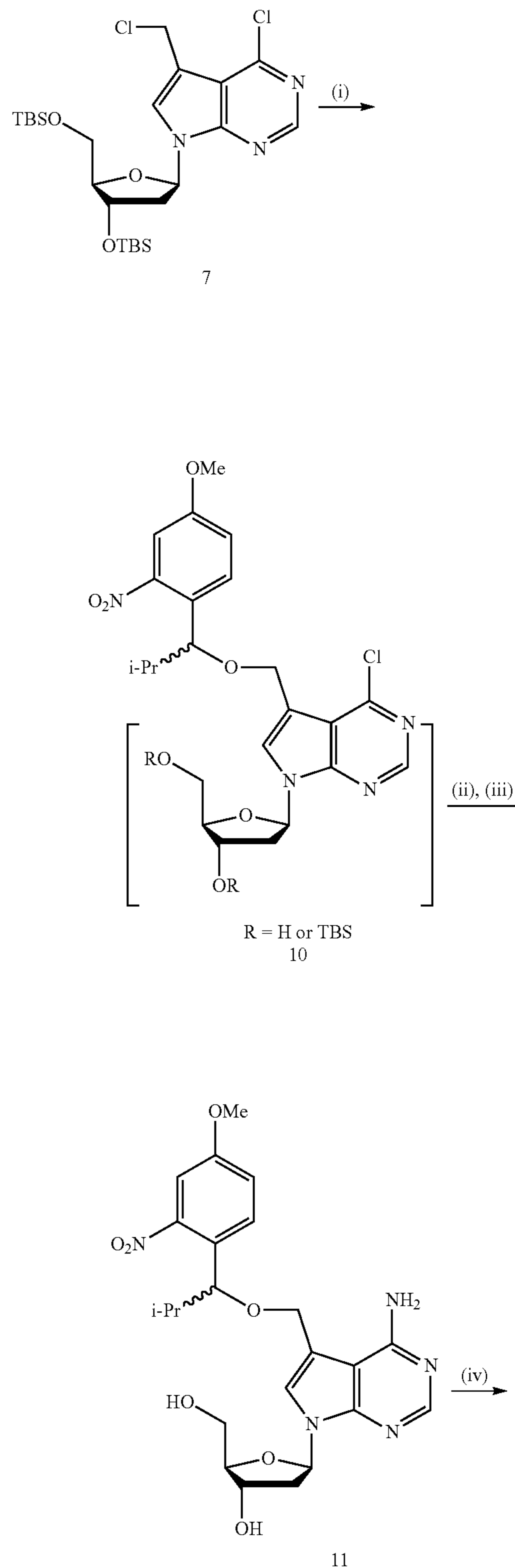
Scheme S8. Synthesis of 7-[1-(4-methoxy-2-nitrophenyl)-2-methyl-propyloxy]methyl-7-deaza-2'-deoxyadenosine-5'-triphosphate.
