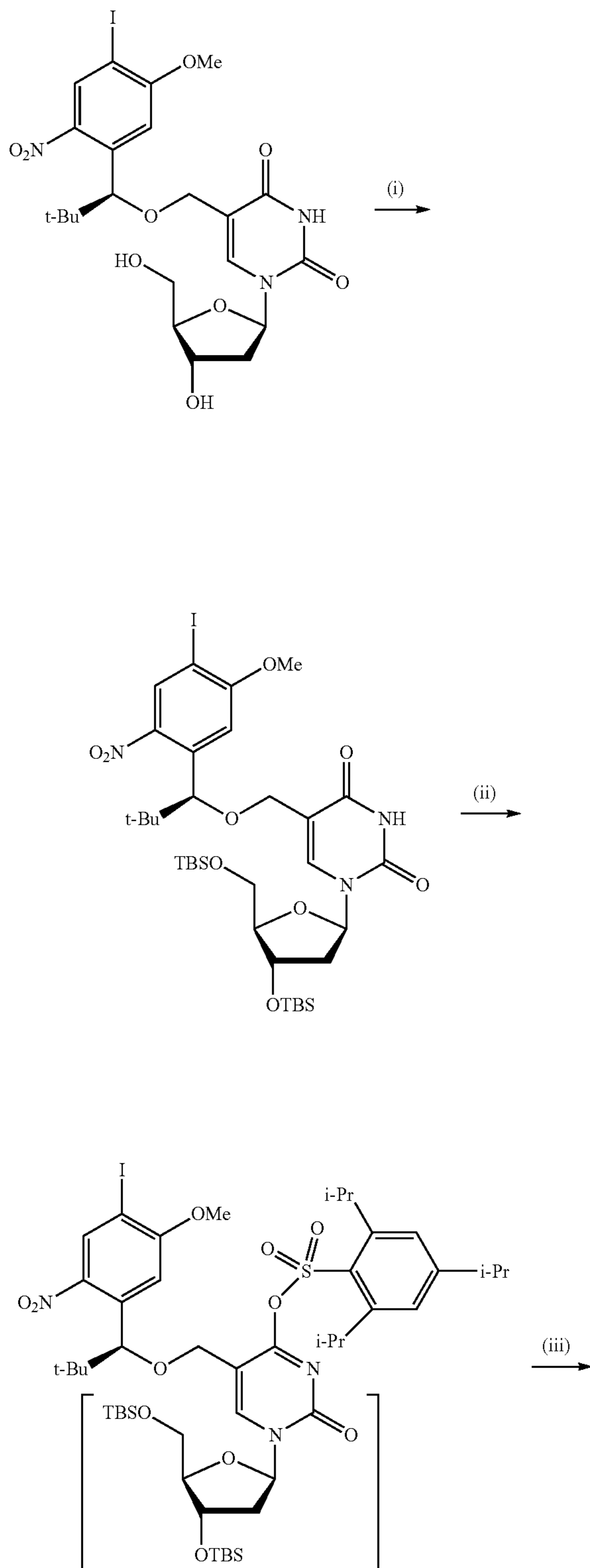
Scheme 5a. Synthesis of dye labeled 5-[(S)-1-(5-methoxy-2-nitrophenyl)-2,2-dimethyl-propyloxy]methyl-2'-deoxycytidine-5'-triphosphate.
