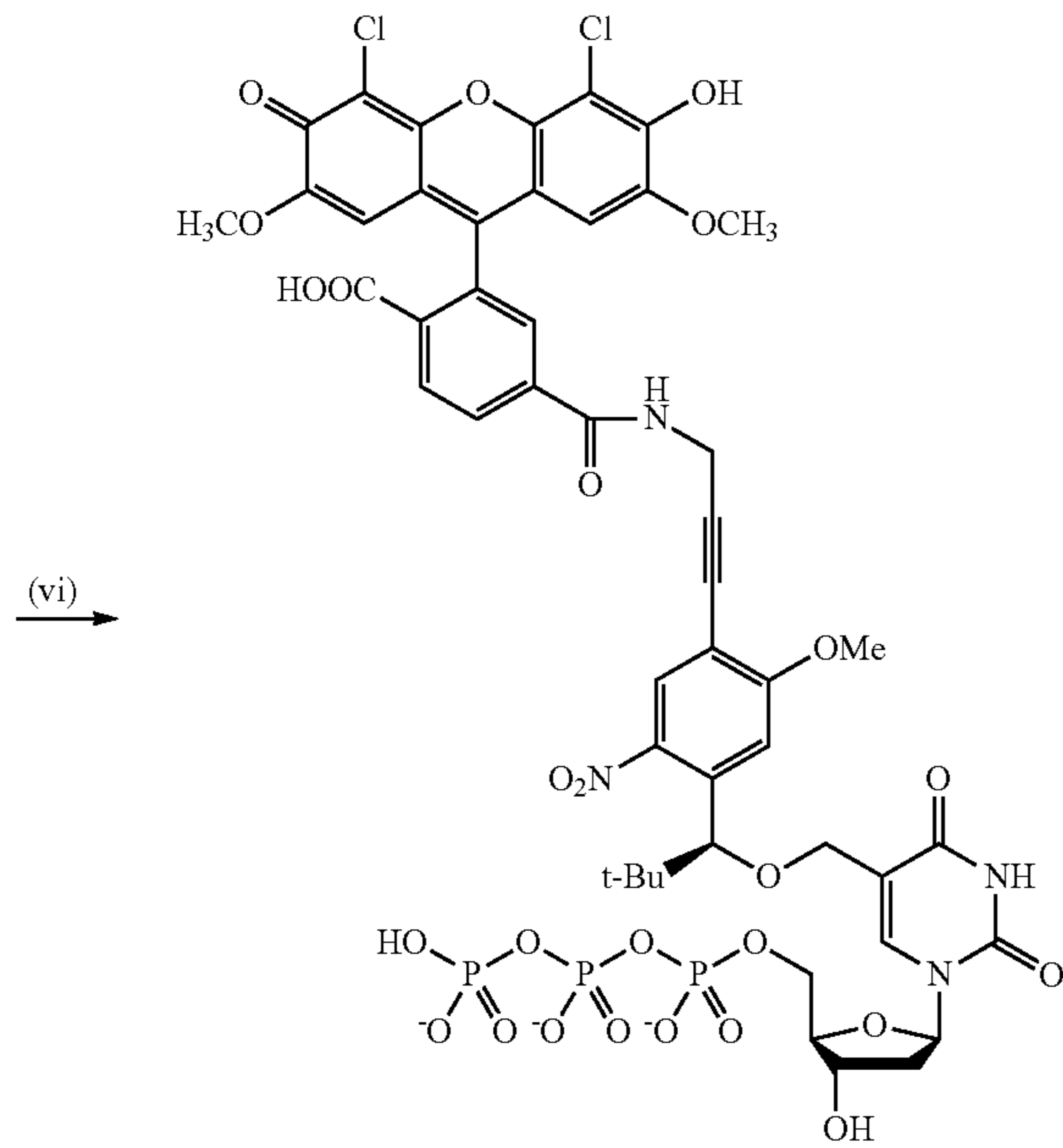
Scheme 3c.
