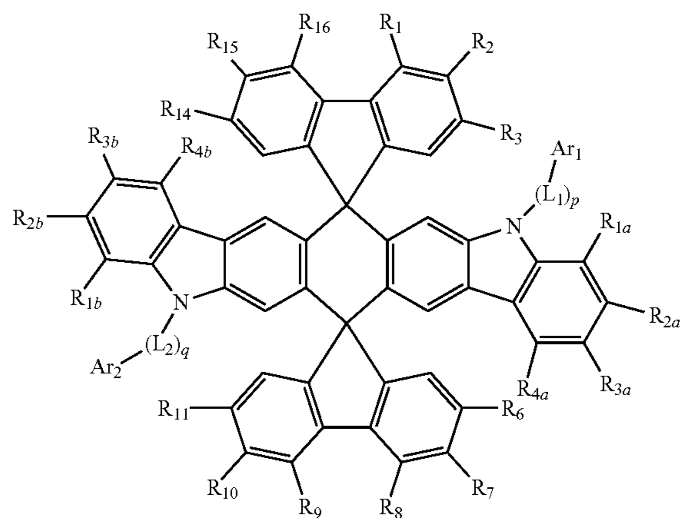
[Chemical Formula 3]
