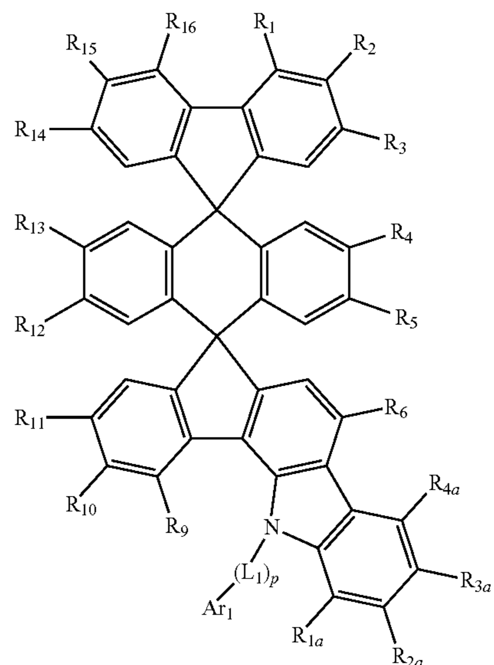
[Chemical Formula 6]
