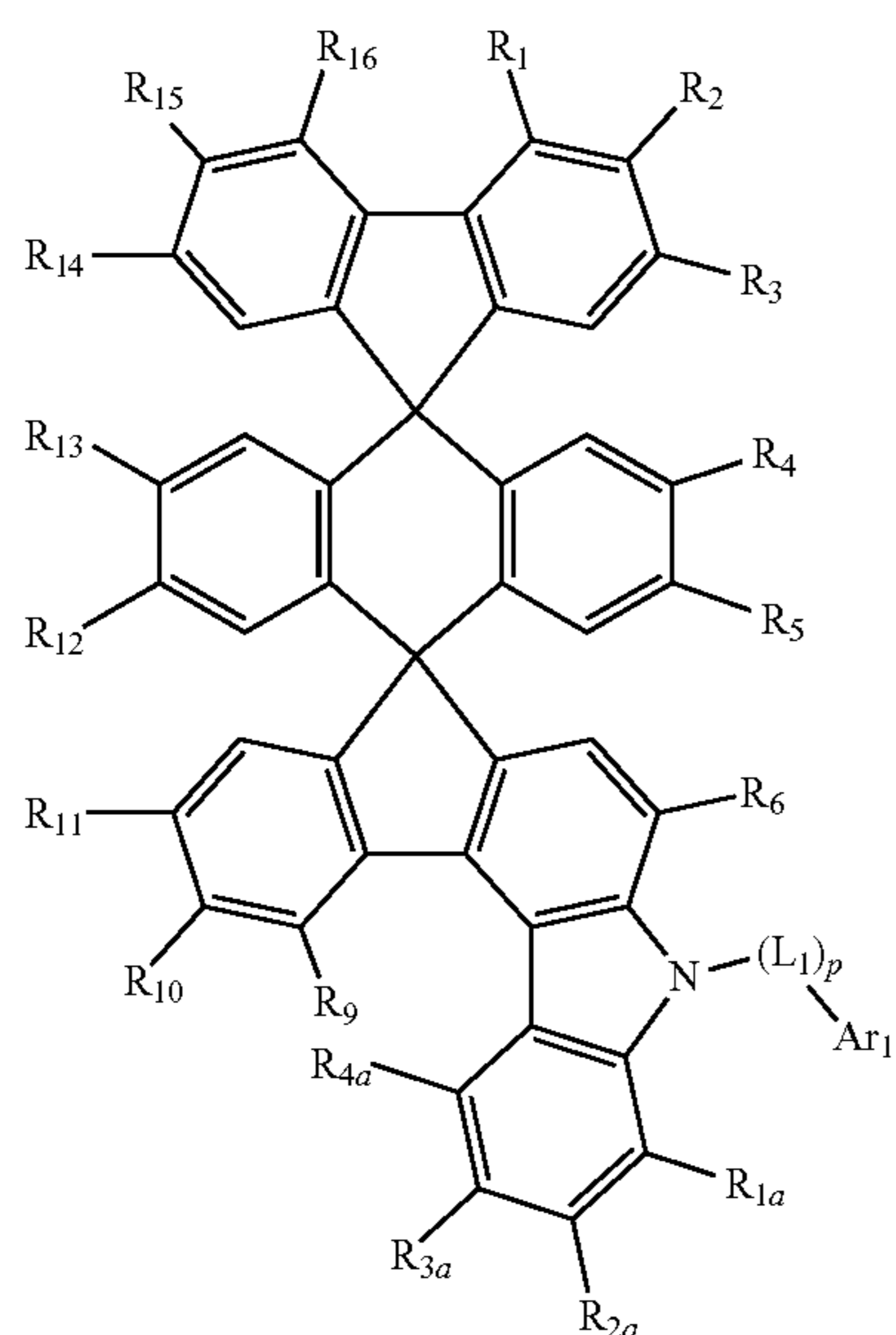
[Chemical Formula 5]
