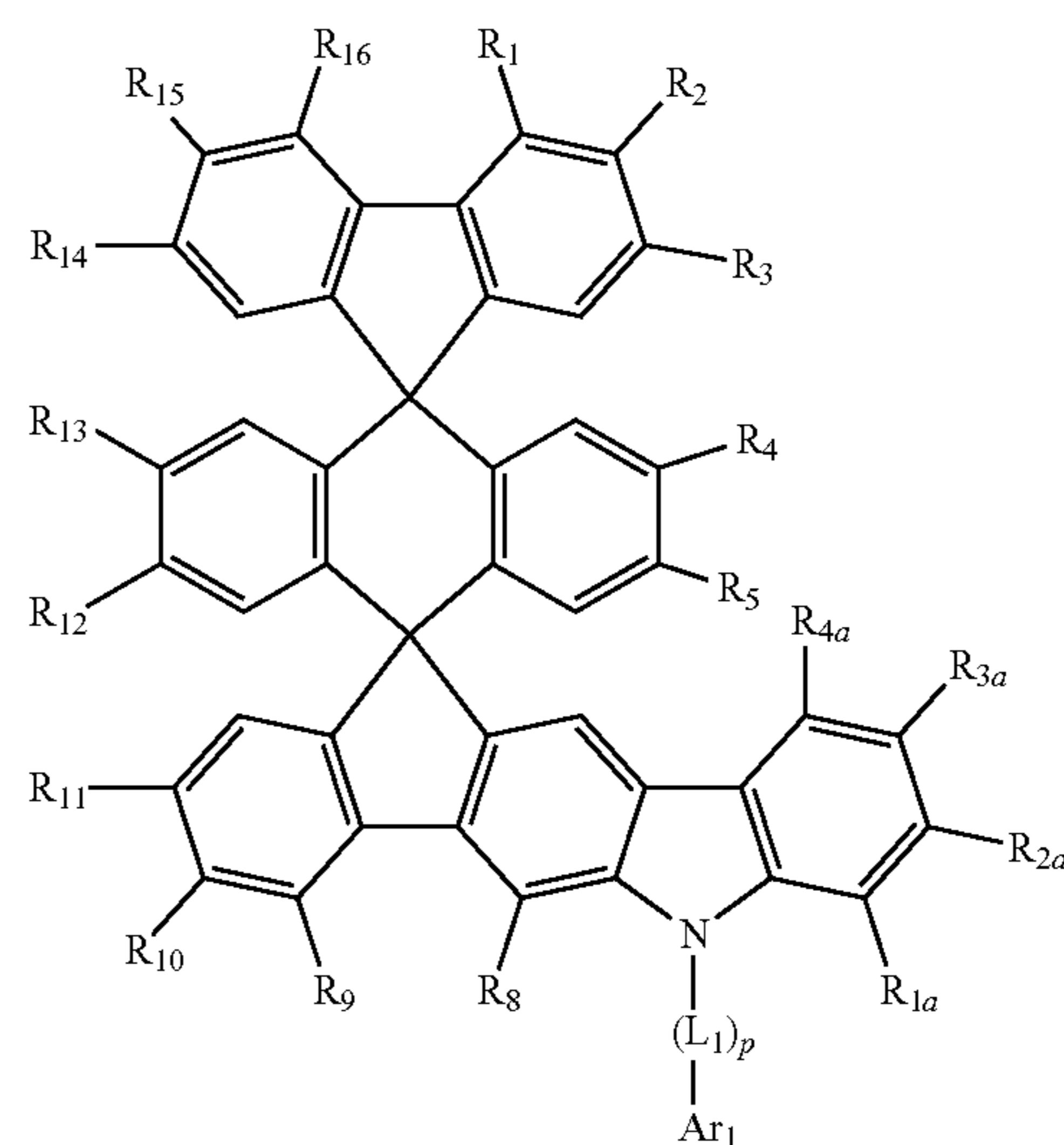
[Chemical Formula 7]
