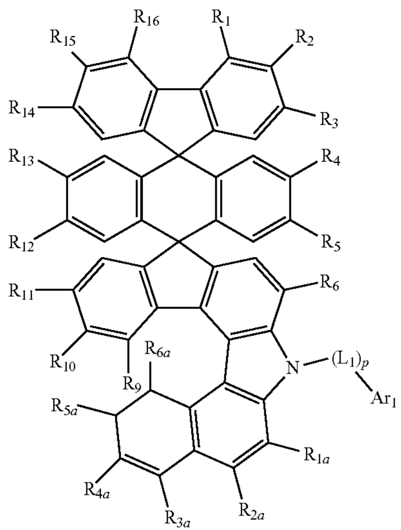
[Chemical Formula 12]
