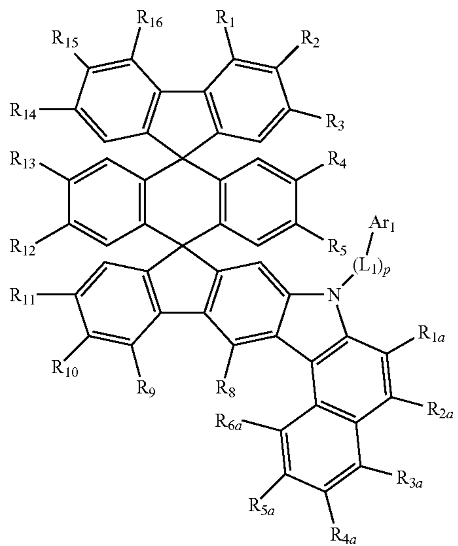
[Chemical Formula 11]
