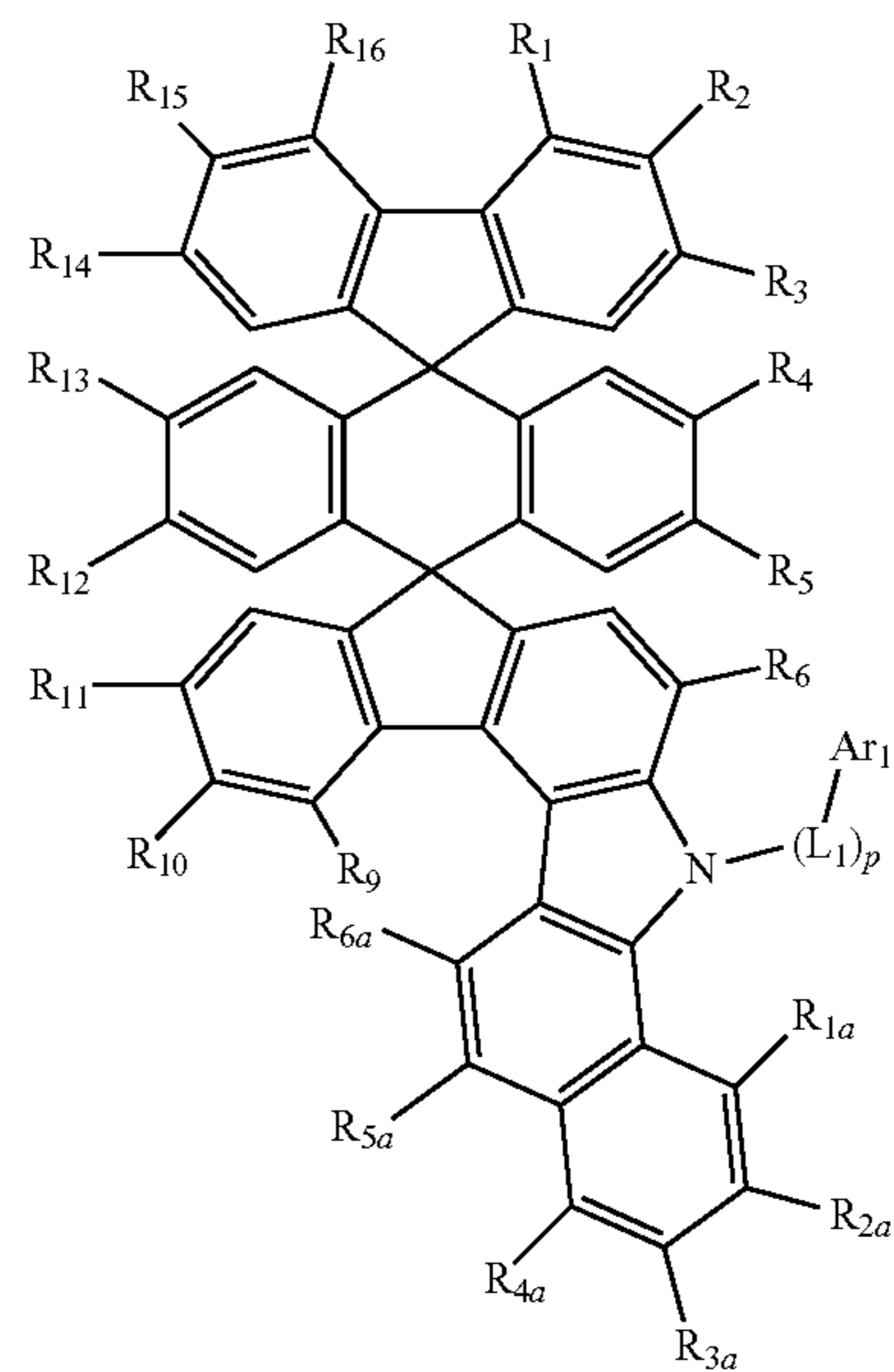
[Chemical Formula 13]
