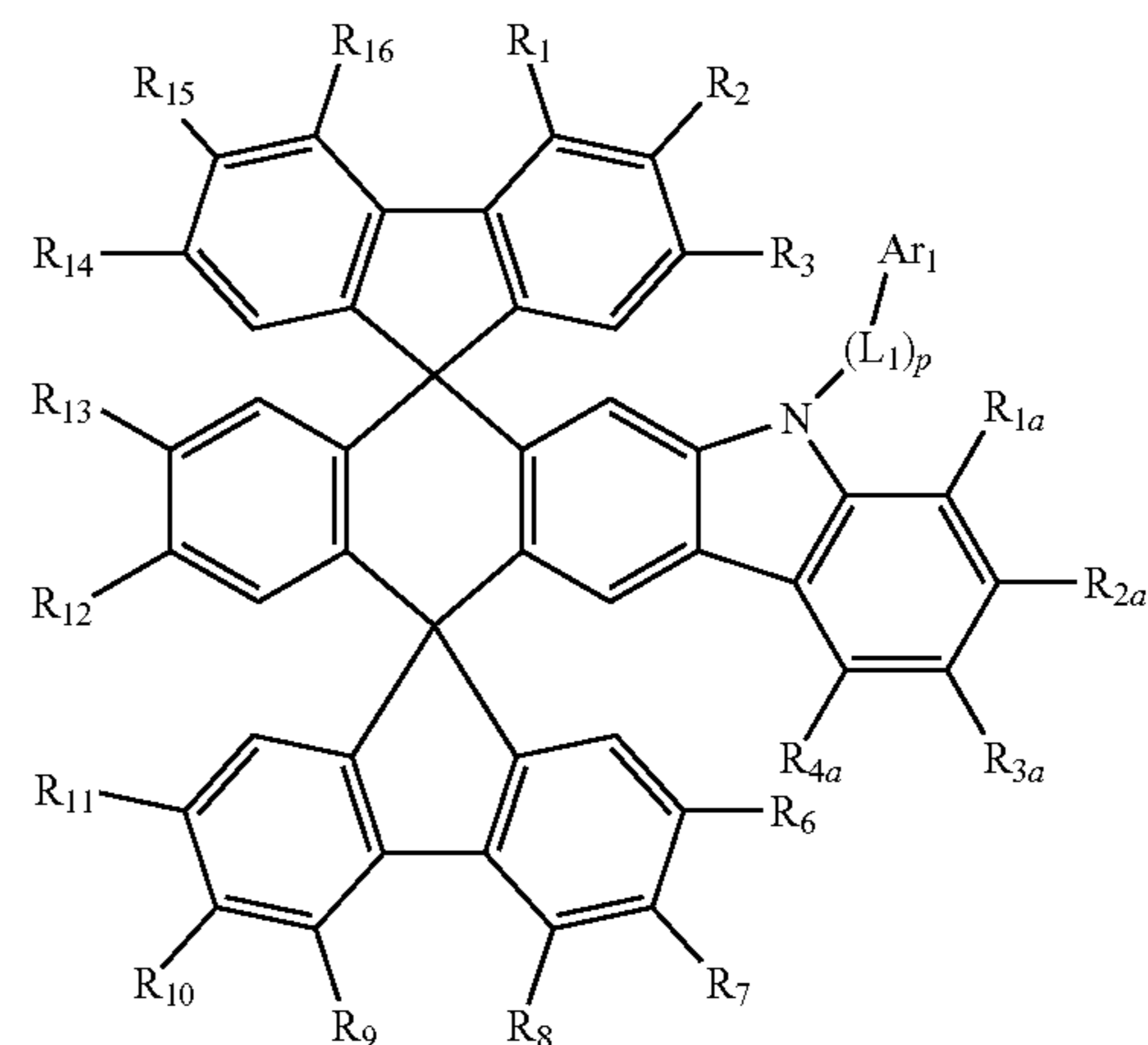
[Chemical Formula 3]
