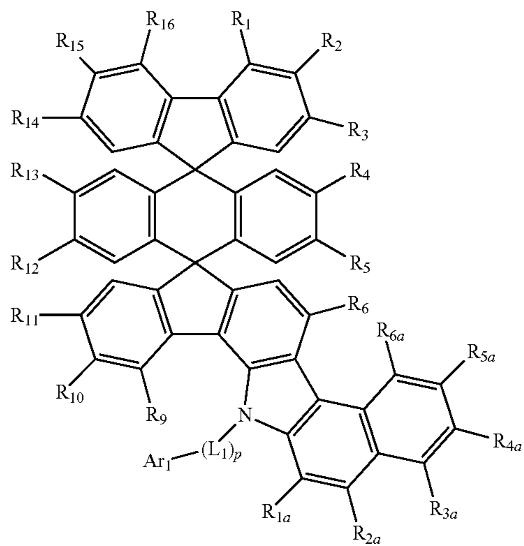
[Chemical Formula 14]
