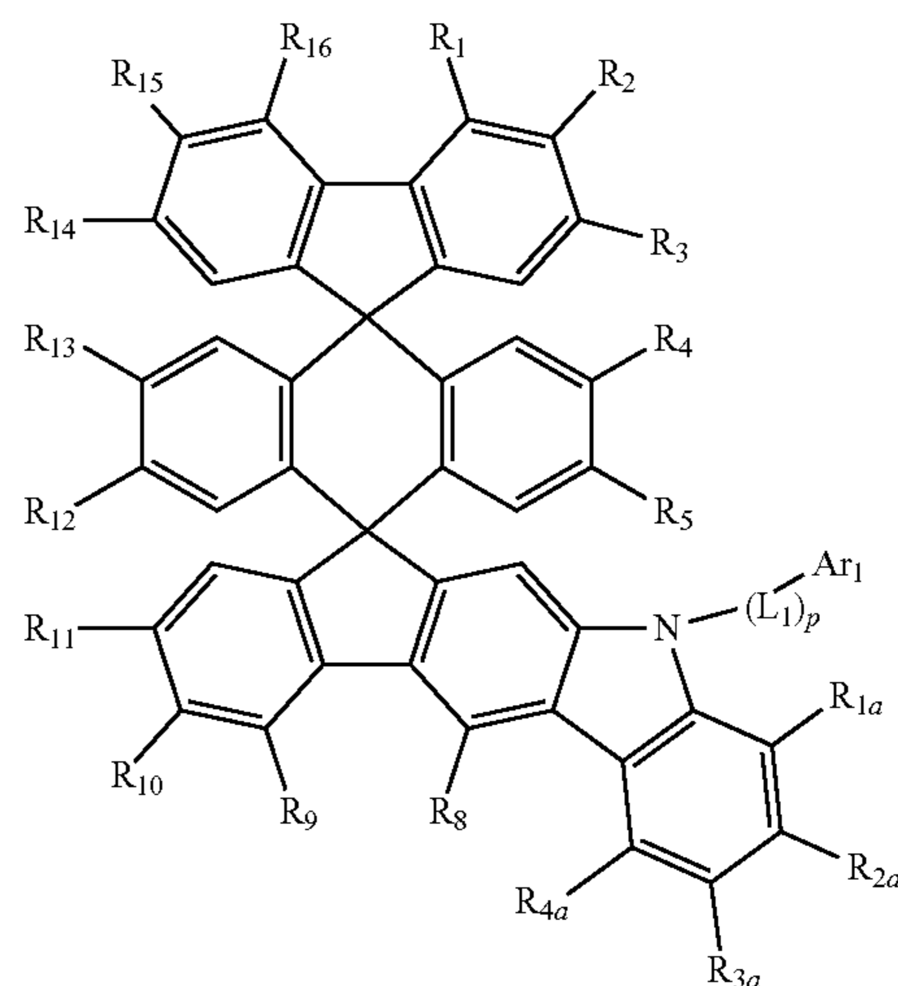
[Chemical Formula 4]
