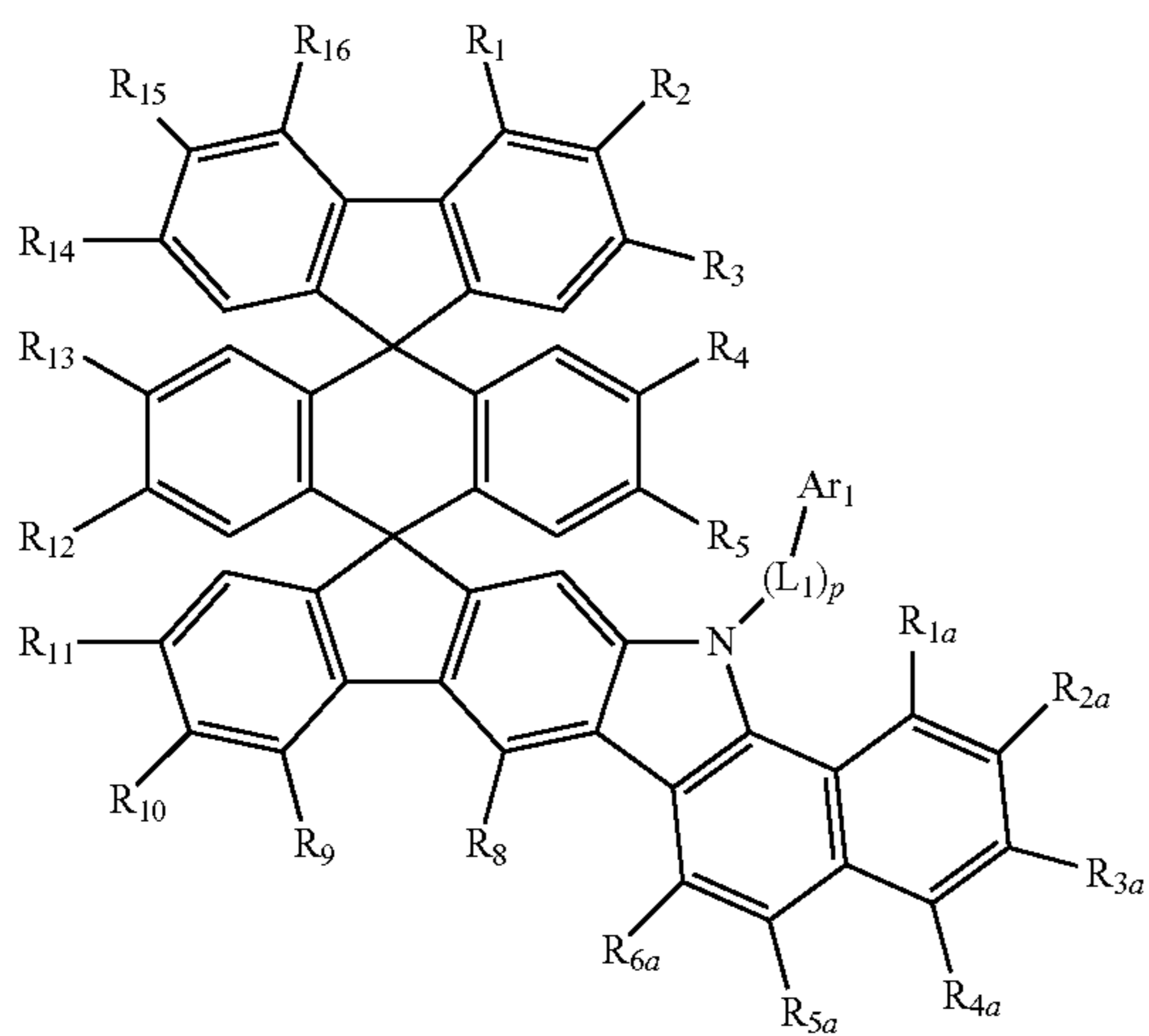
[Chemical Formula 11]
