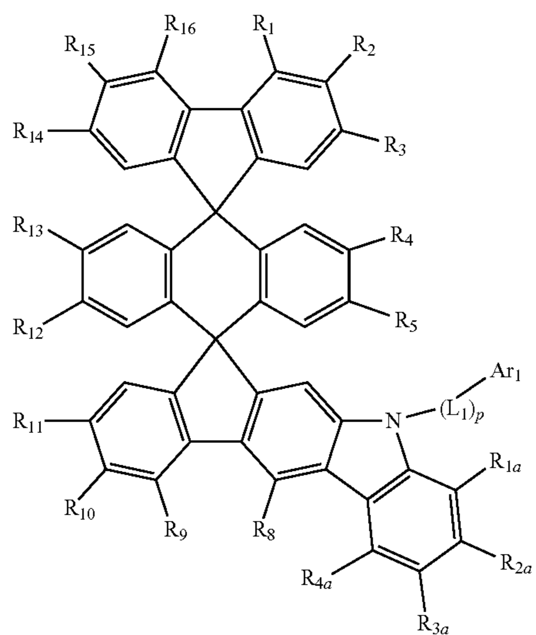
[Chemical Formula 4]
