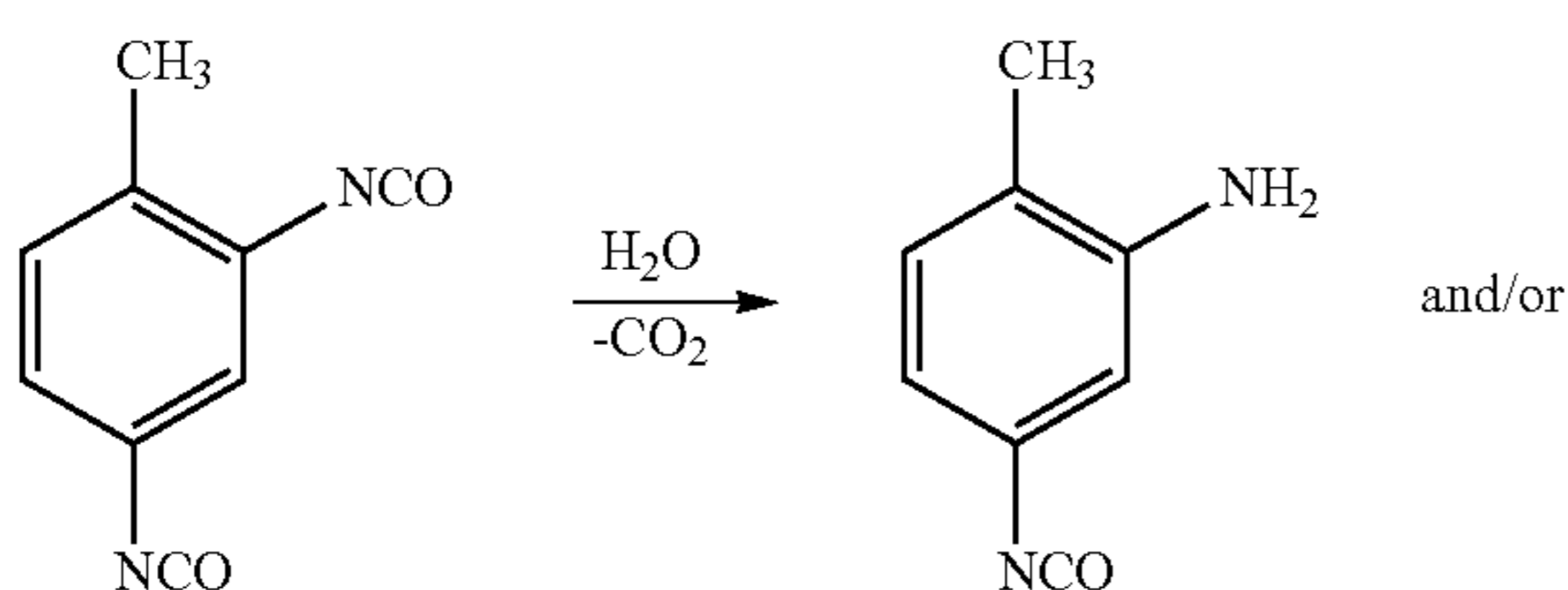
Scheme 1: Effects of water on isocyanate groups of TDI.
