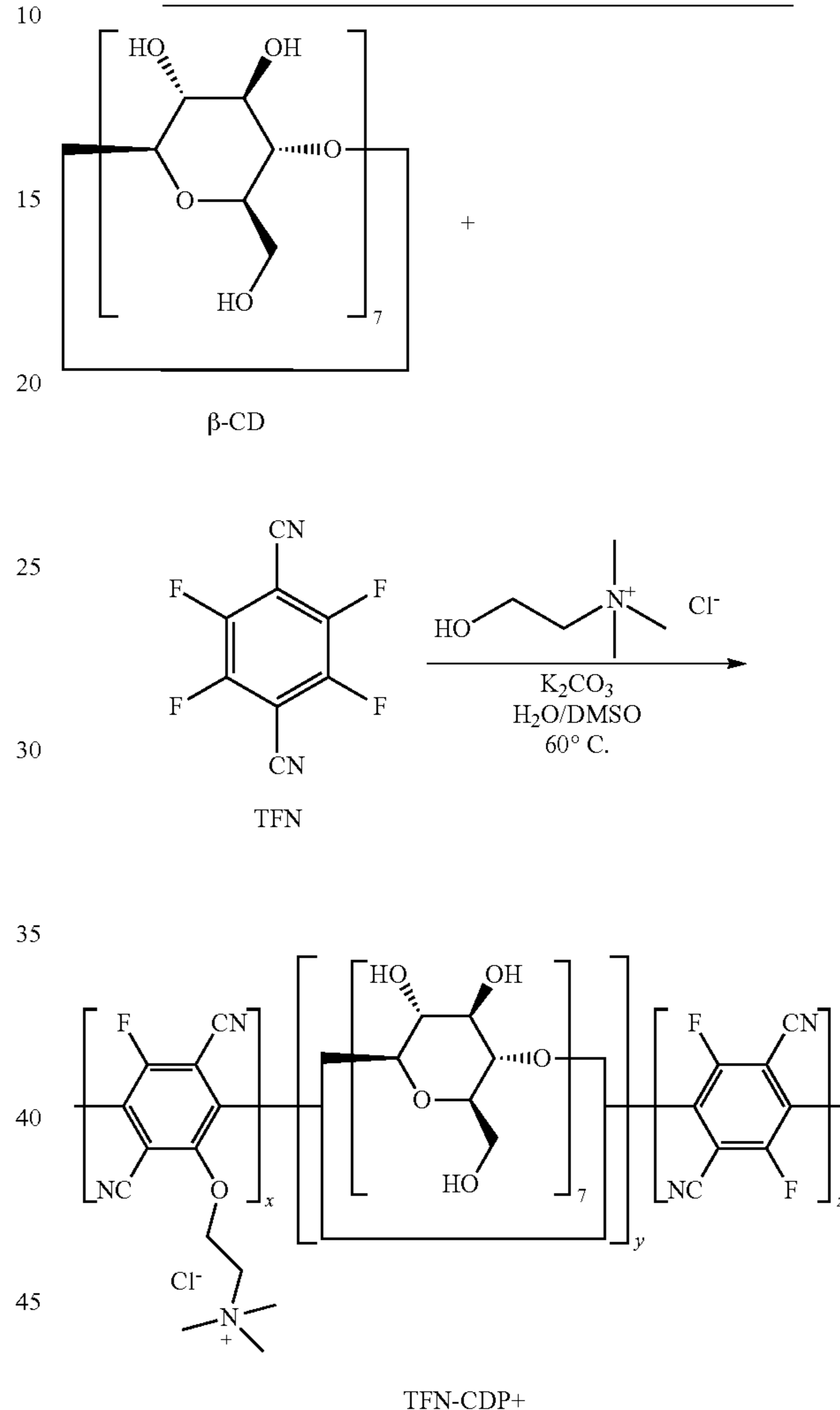
Scheme 2: Synthetic overview for choline chloride-modified β-CD-TFN polymers
