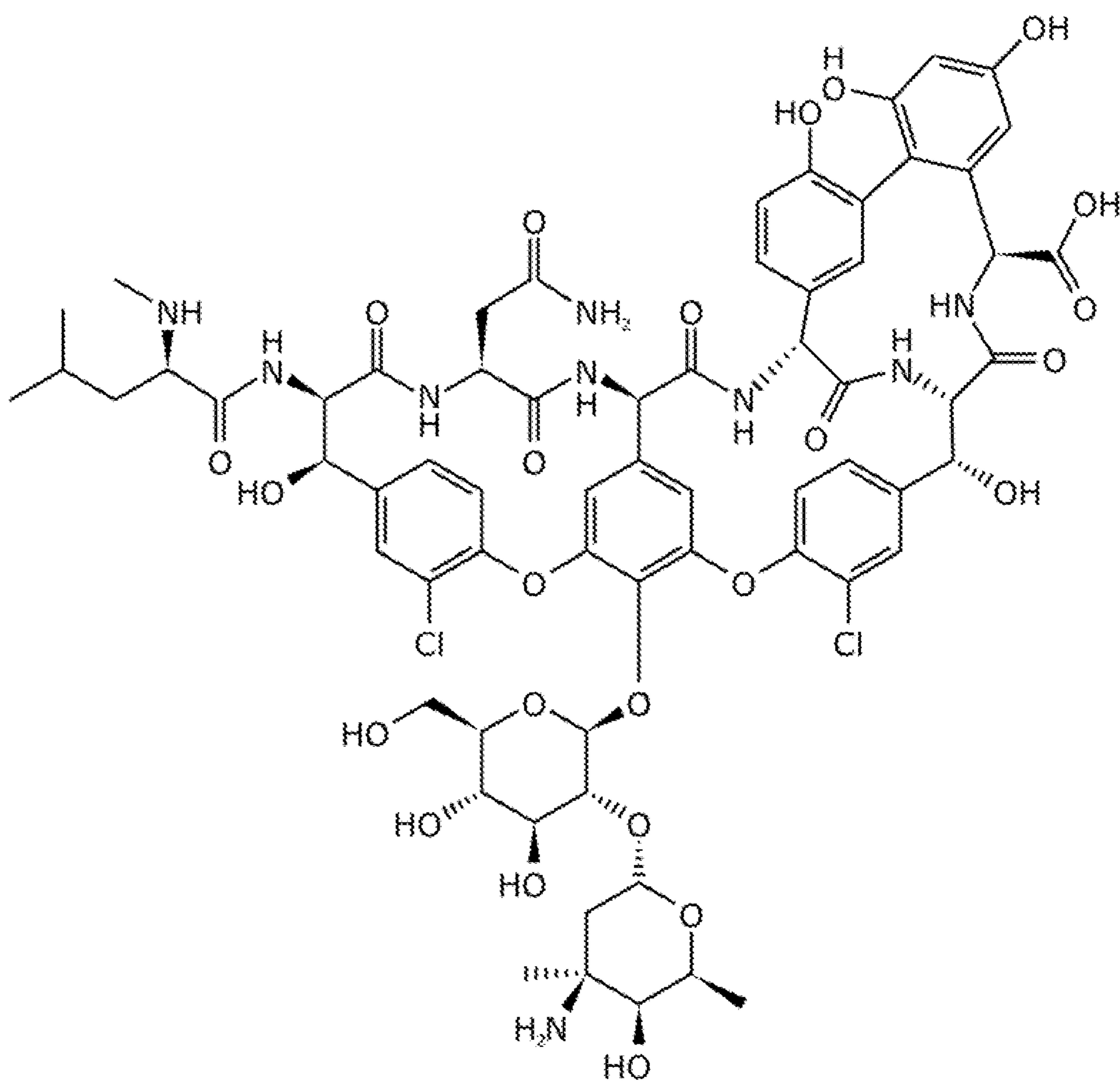
Vancomycin (Formula 1)
