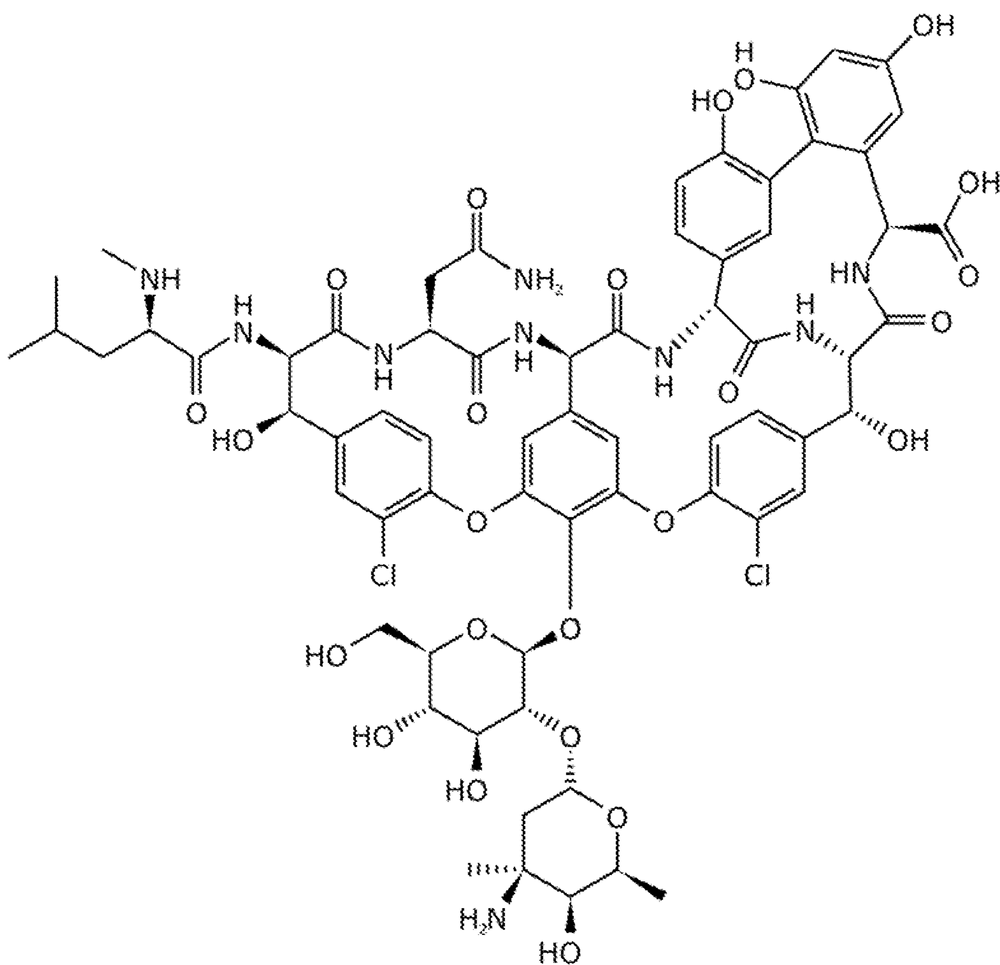
Vancomycin (Formula 1)
