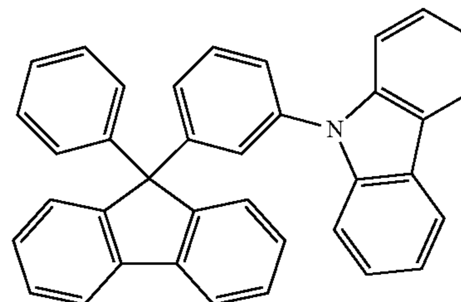
mCzFLP
