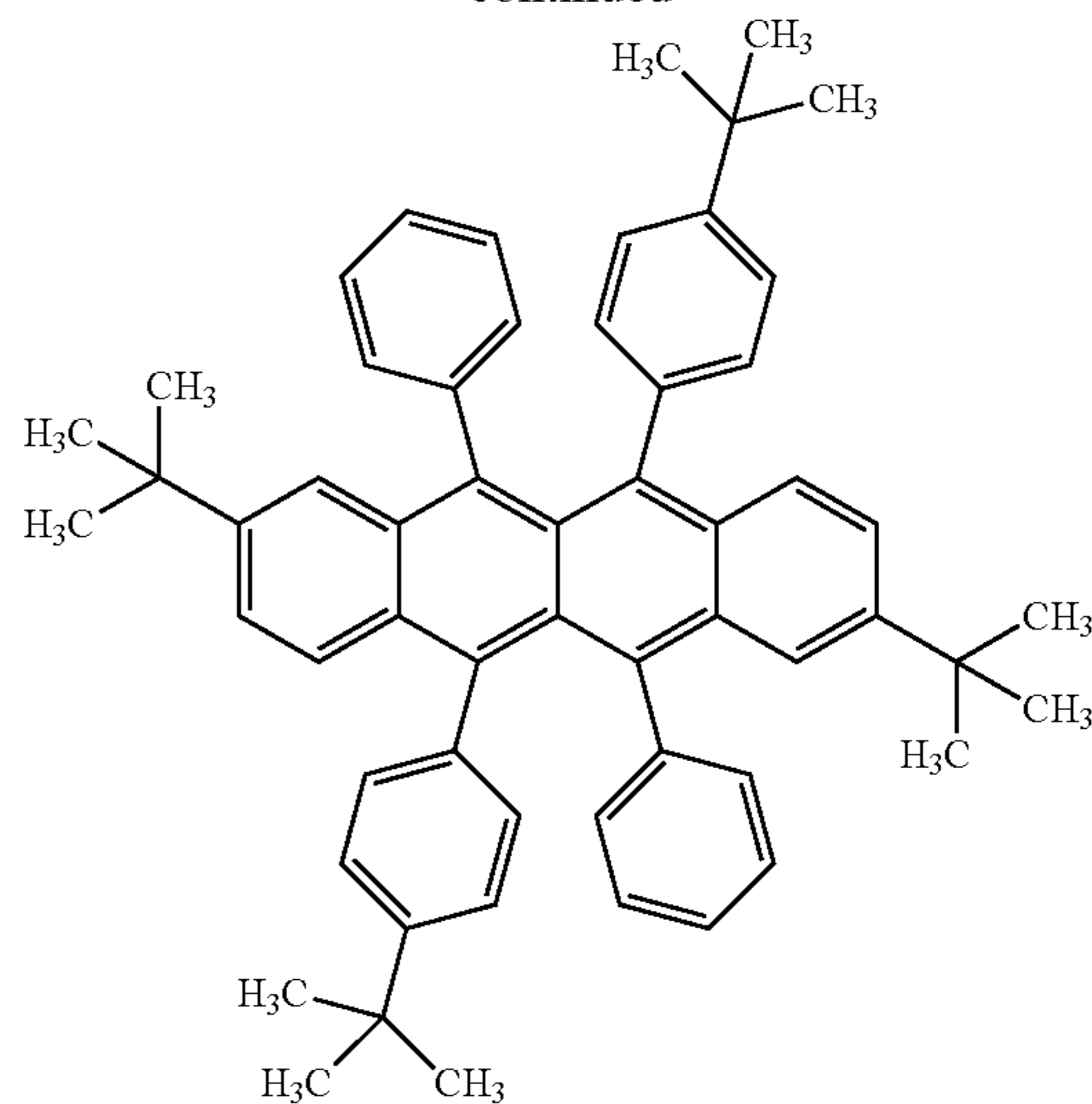
TBRb
