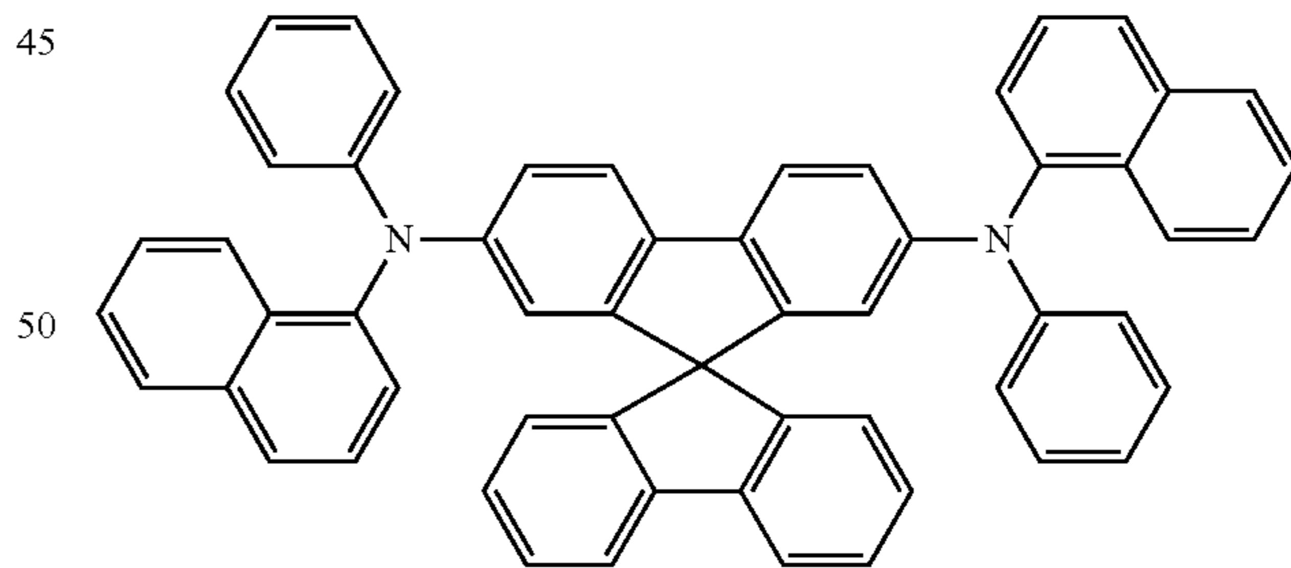
Spiro-NPB
