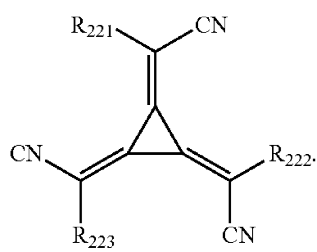
F4-TCNQ
