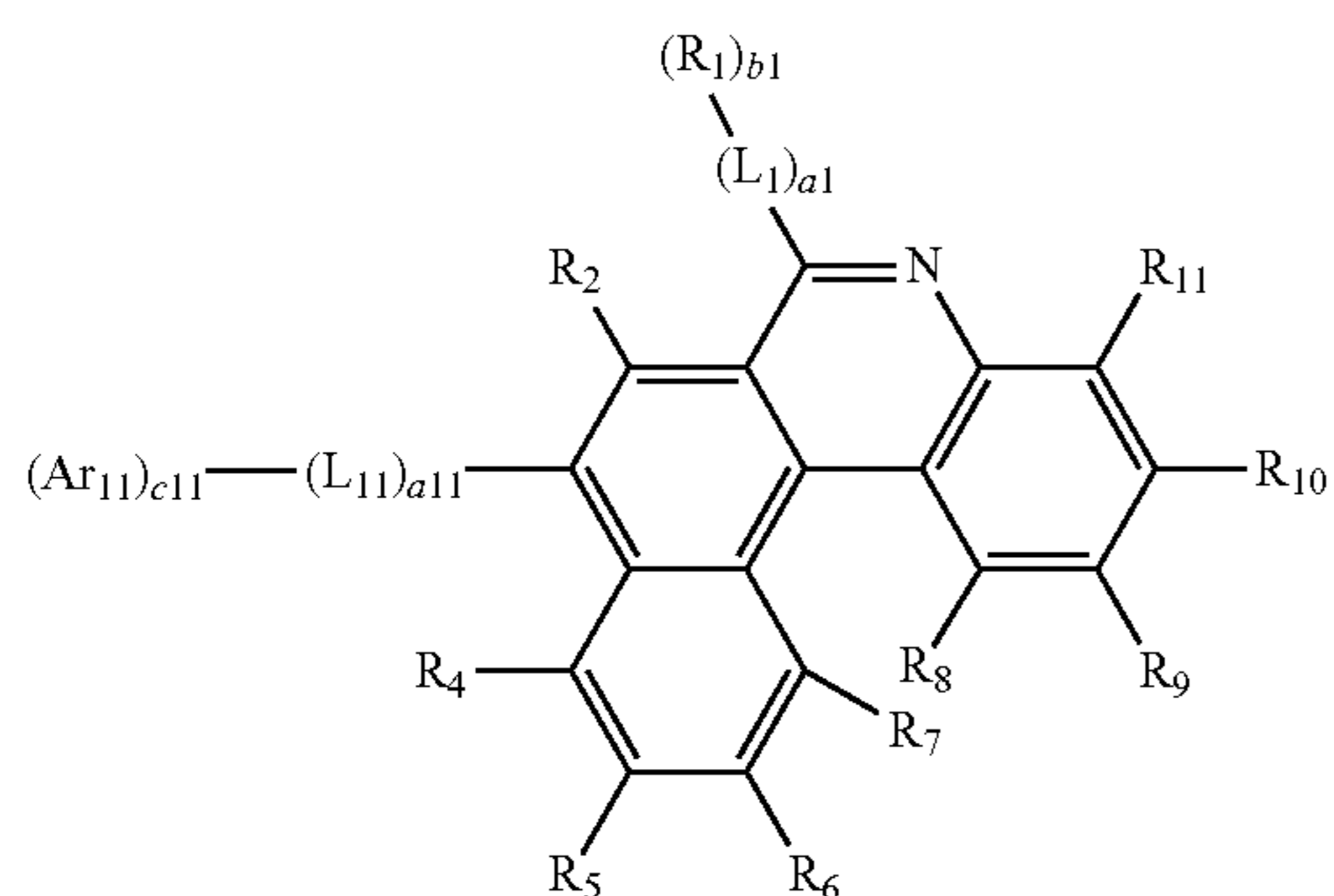
Formula 1-1
