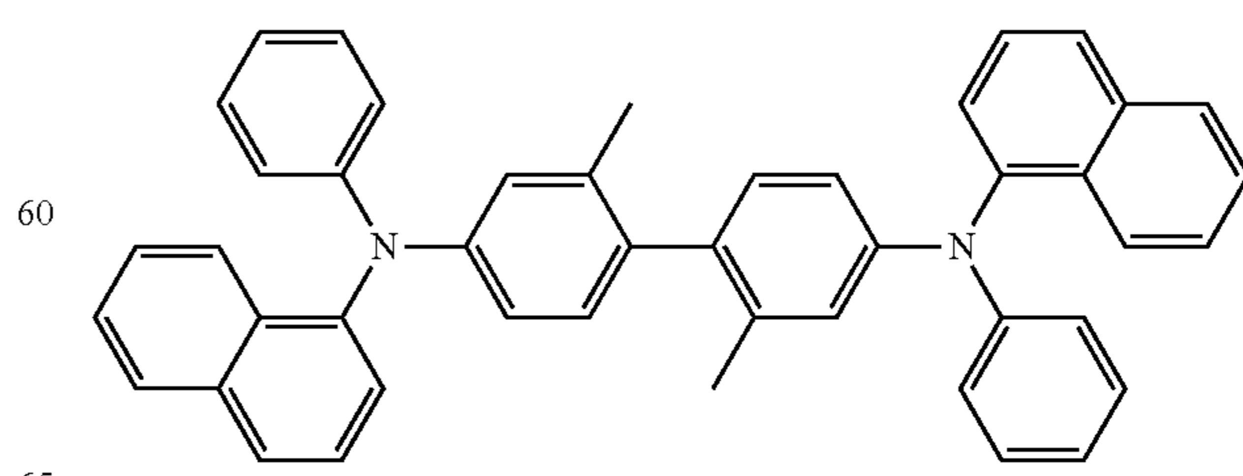
methylated NPB
