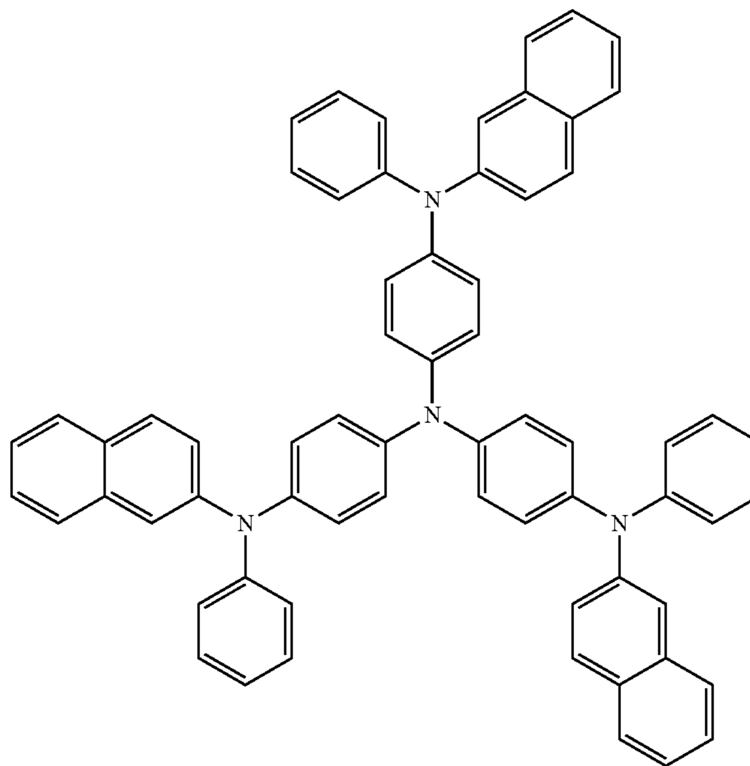
2-TNATA
