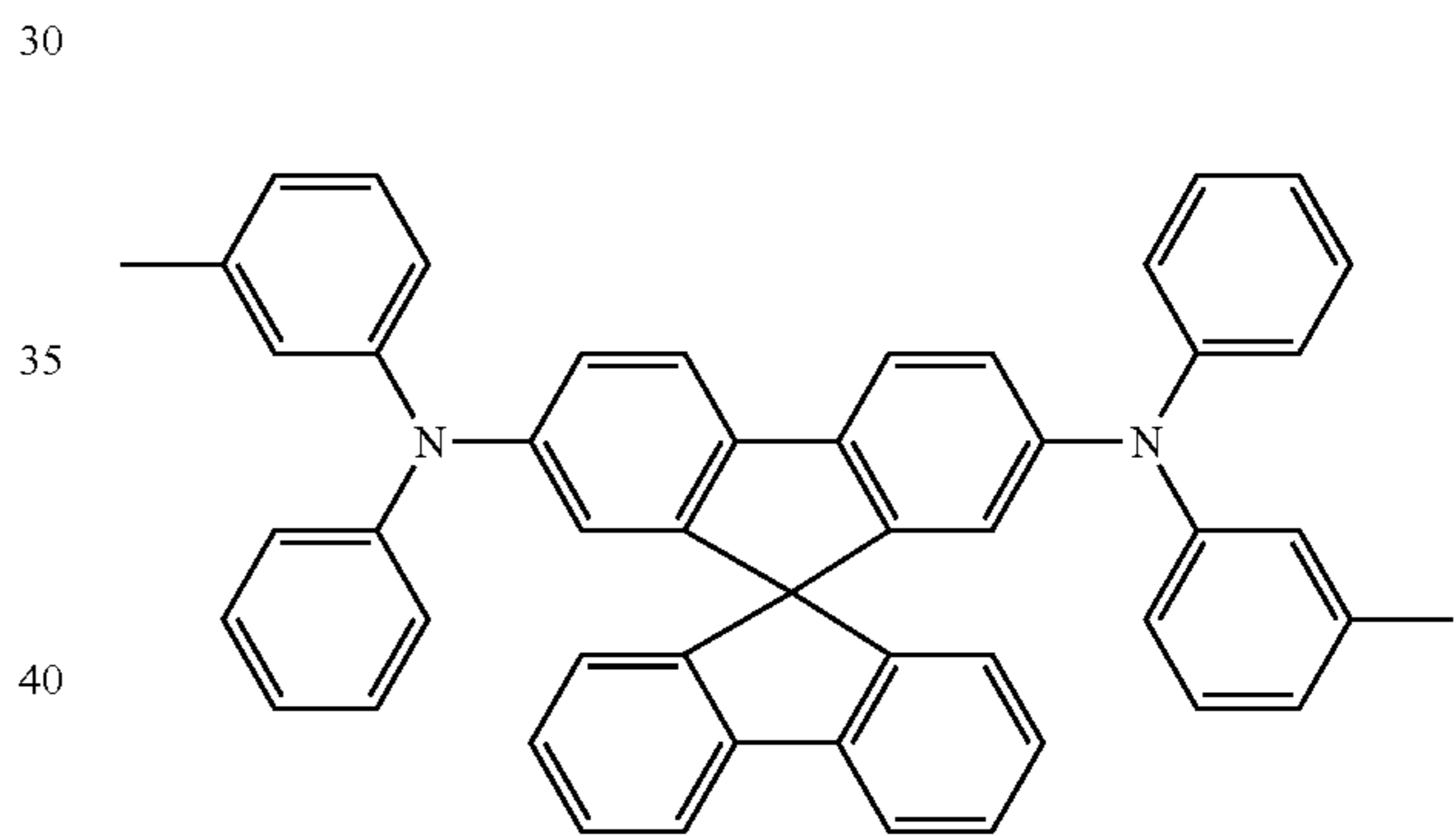
Spiro-TPD
