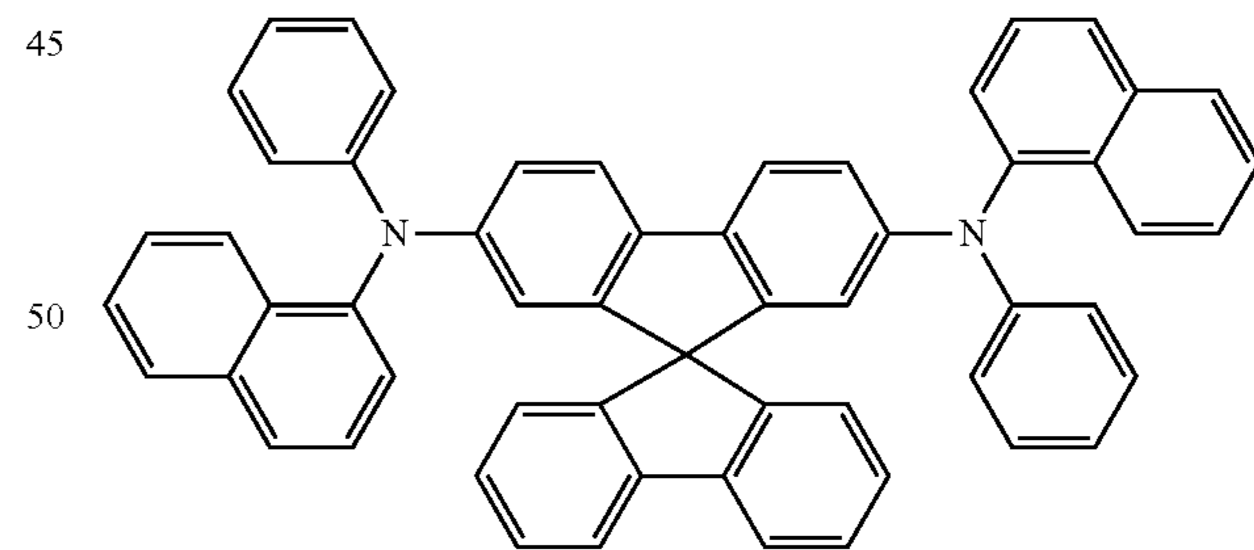
Spiro-NPB
