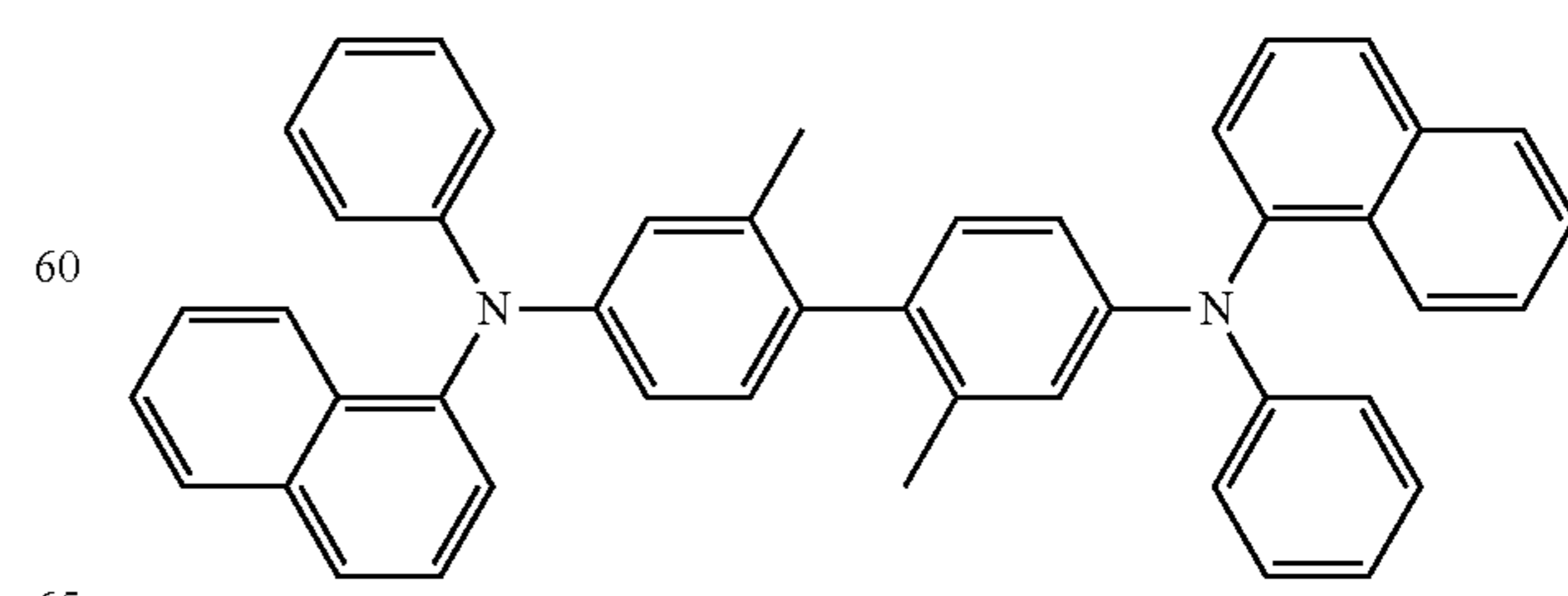
methylated NPB
