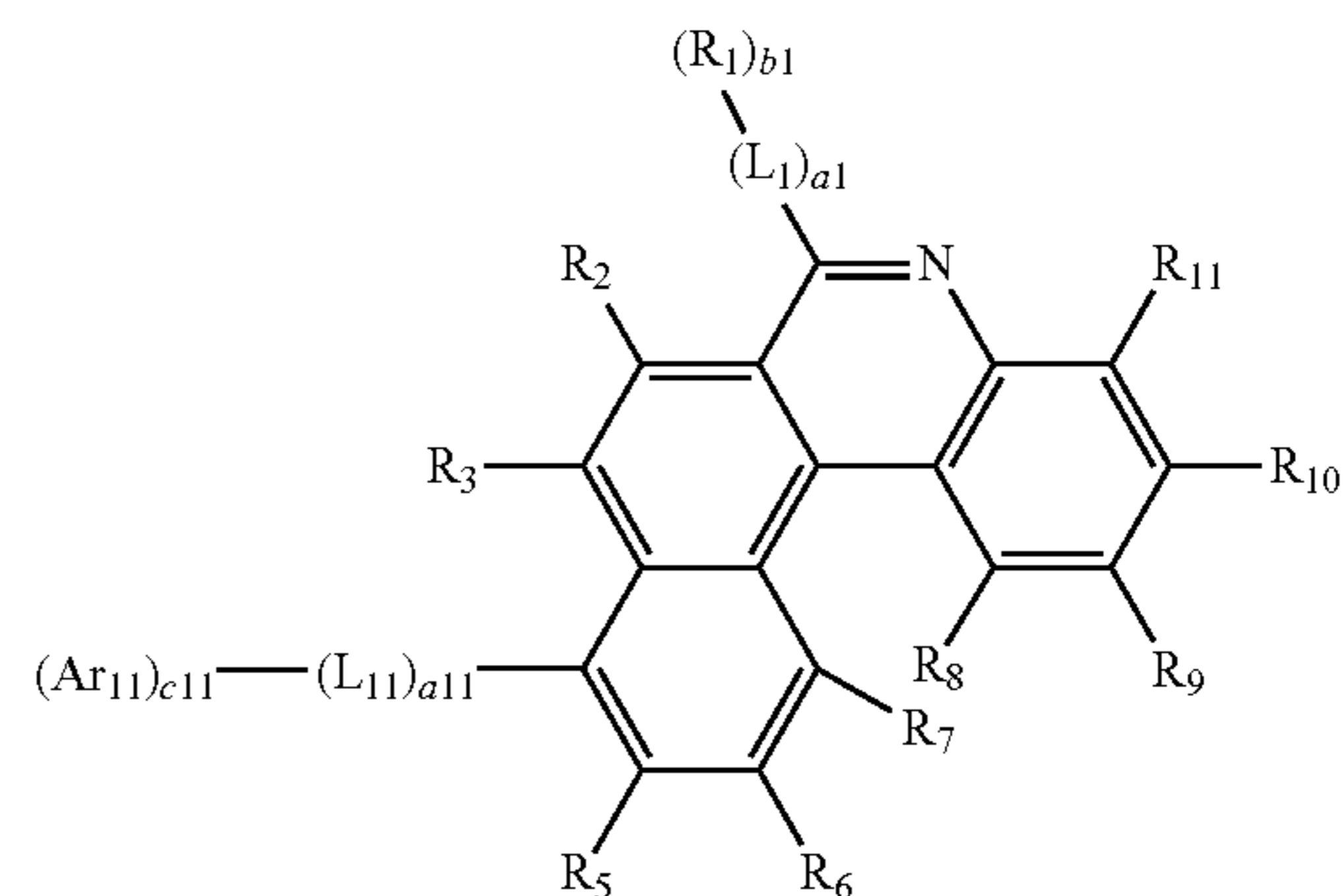
Formula 1-3
