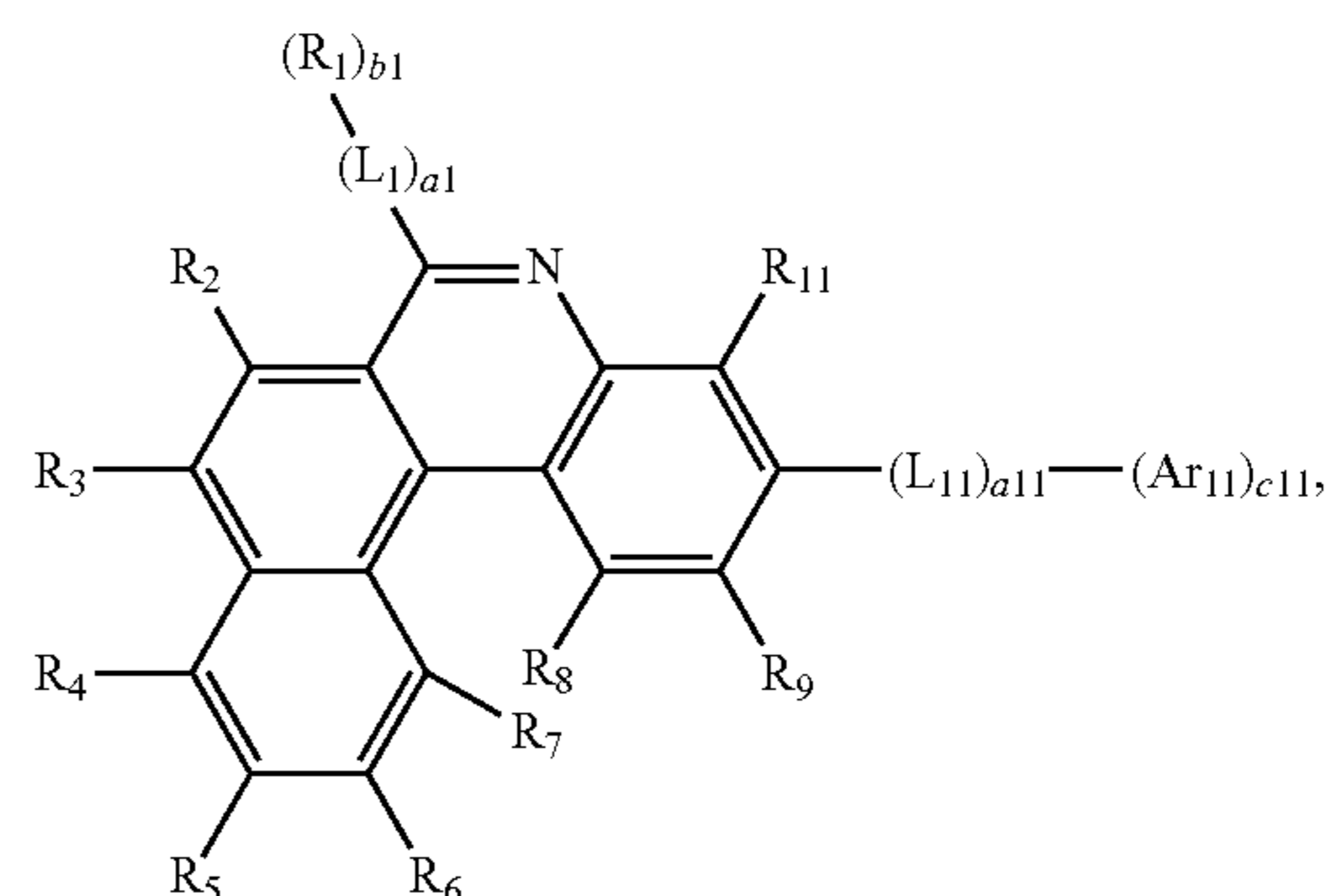
Formula 1-3
