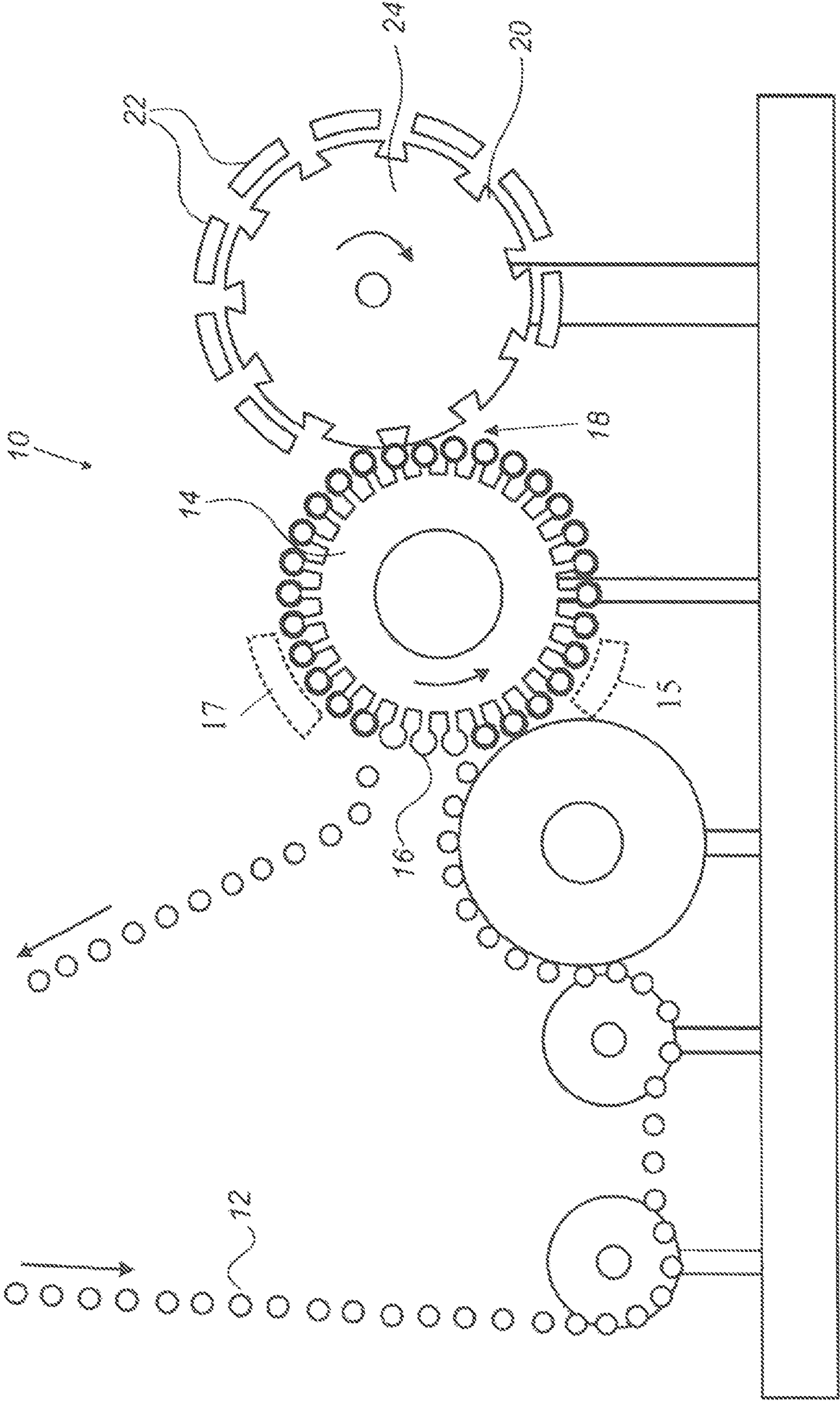
Fig. 1 - Prior Art
