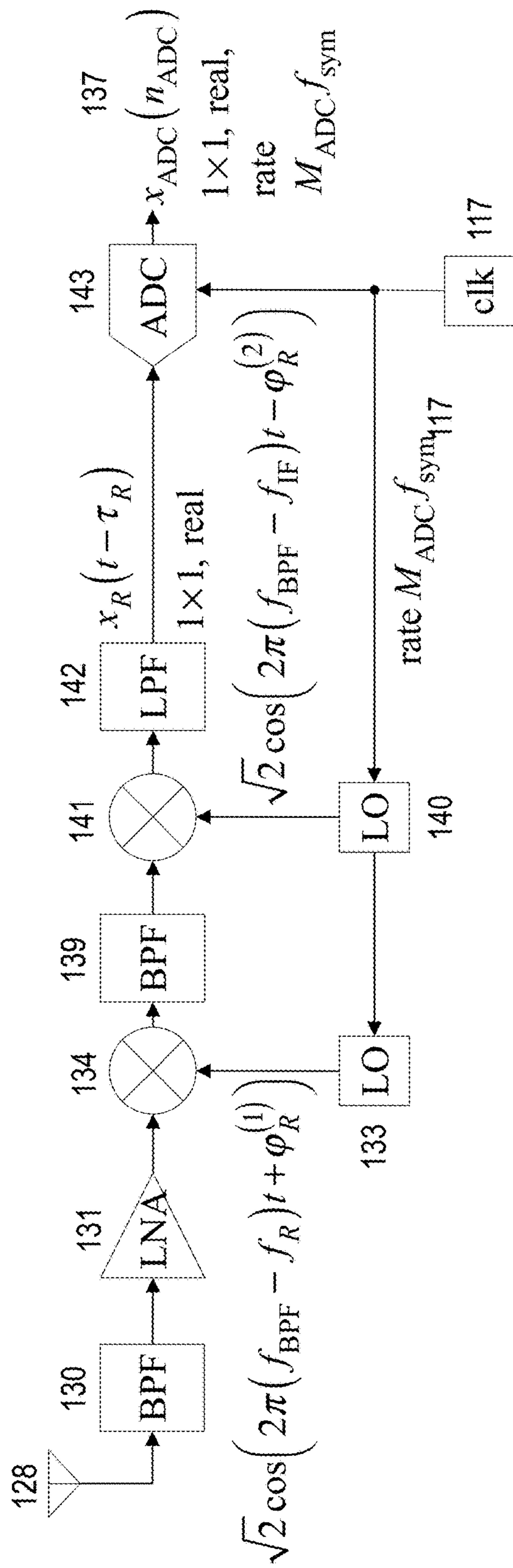
5A: Superhetrodyne Dedicated Receiver Front-End
