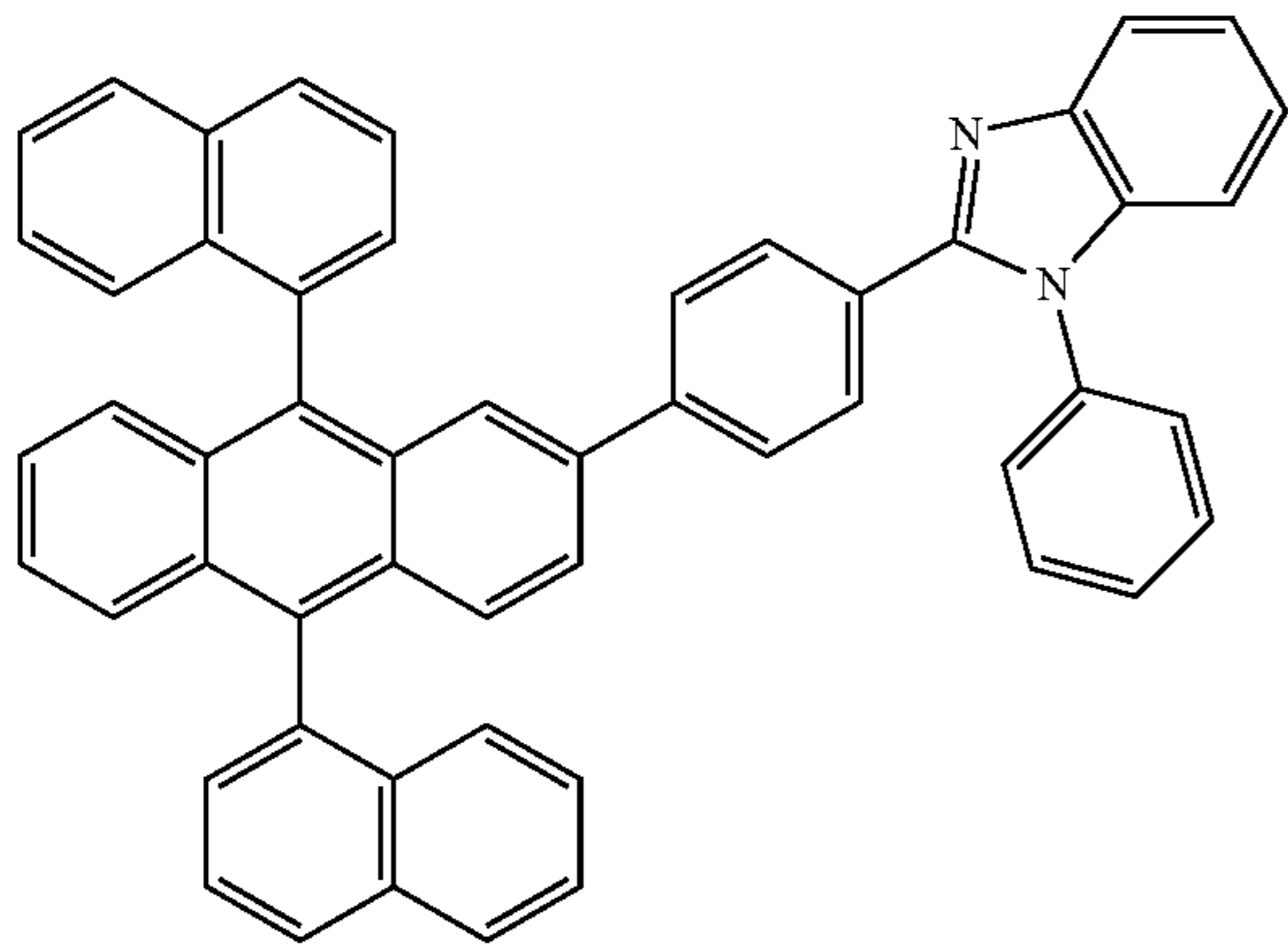
Compound ET6
