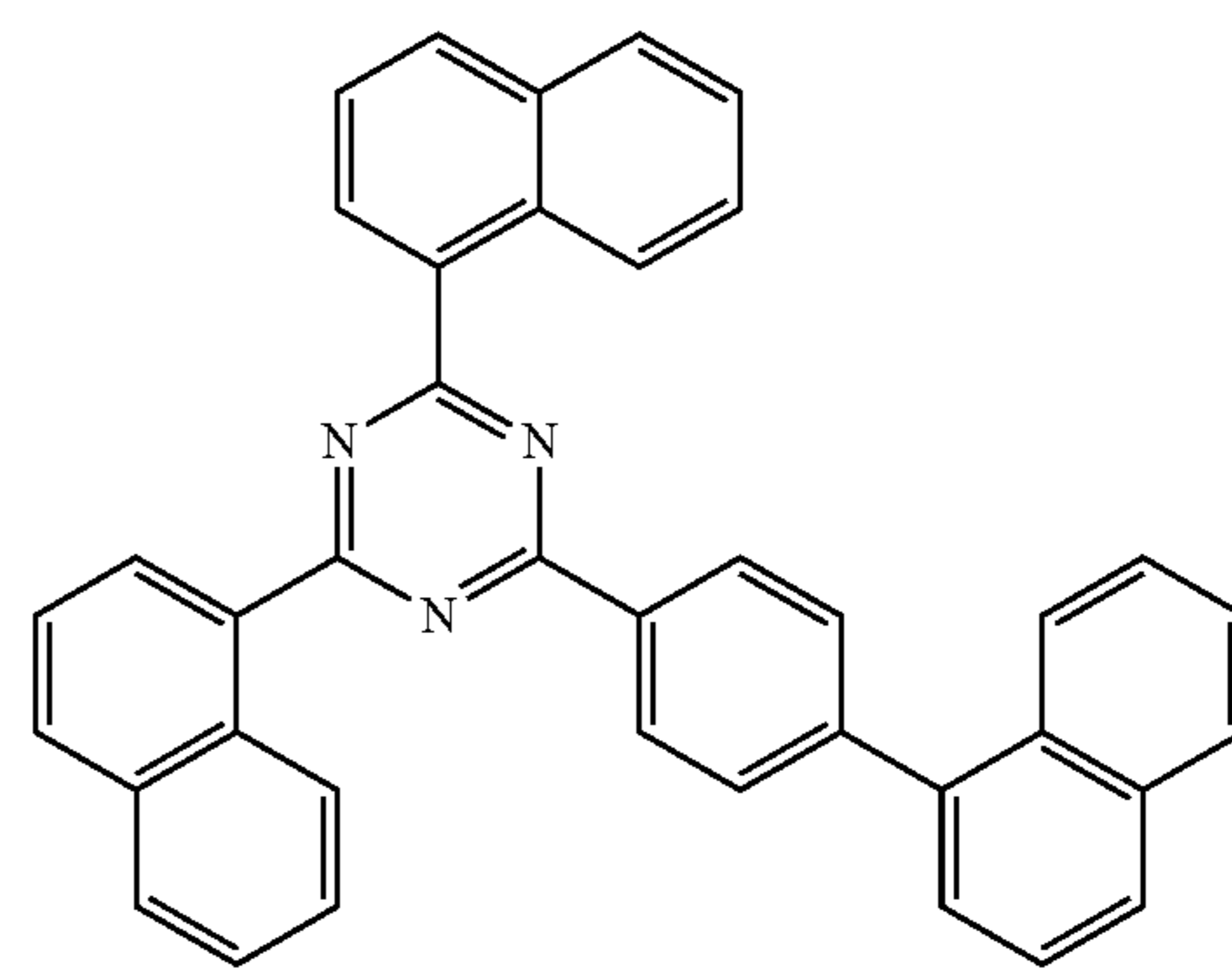
Compound ET15
