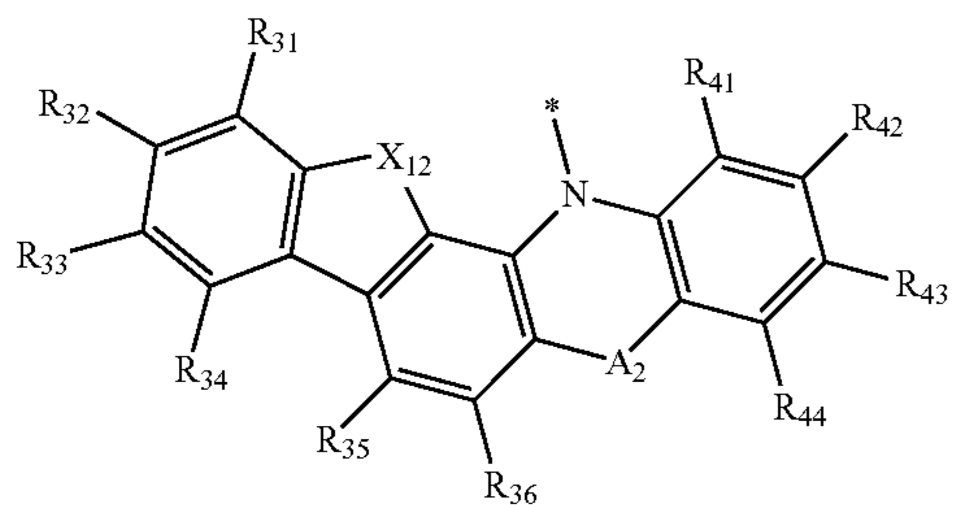
Formula 13-2
