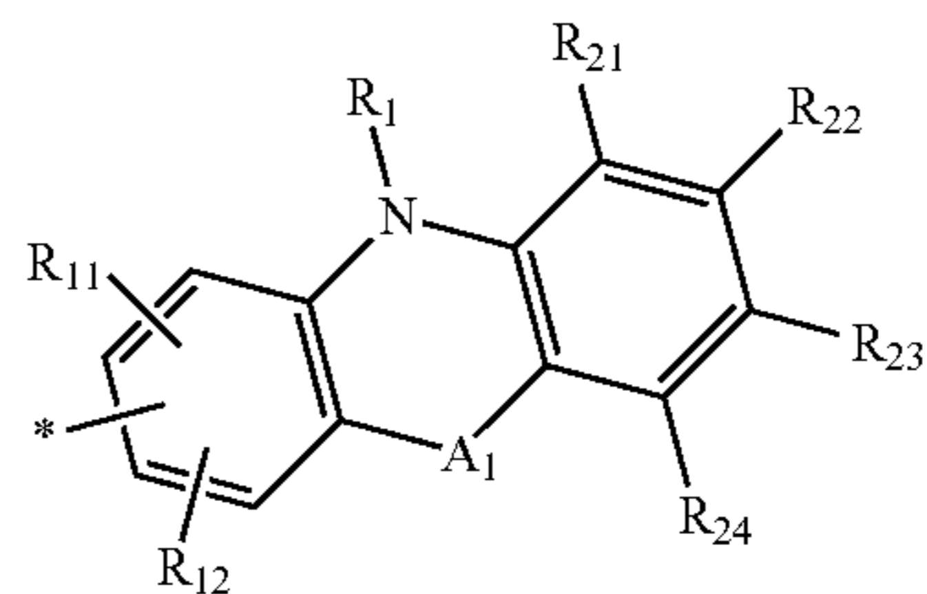
Formula 12-2
