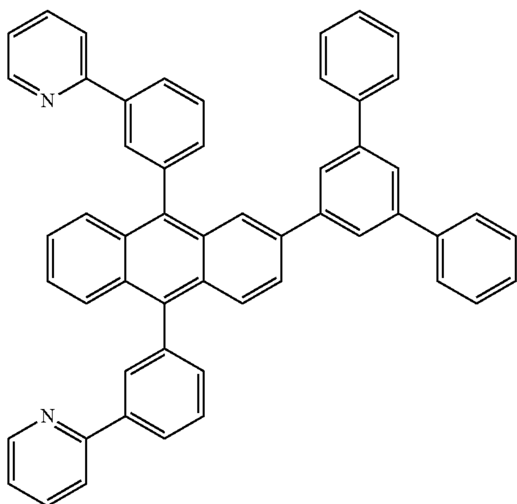
Compound ET8
