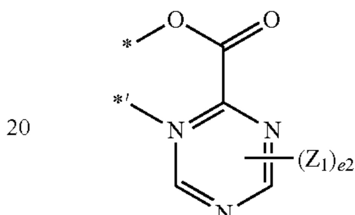
Formula 3-1(104)
