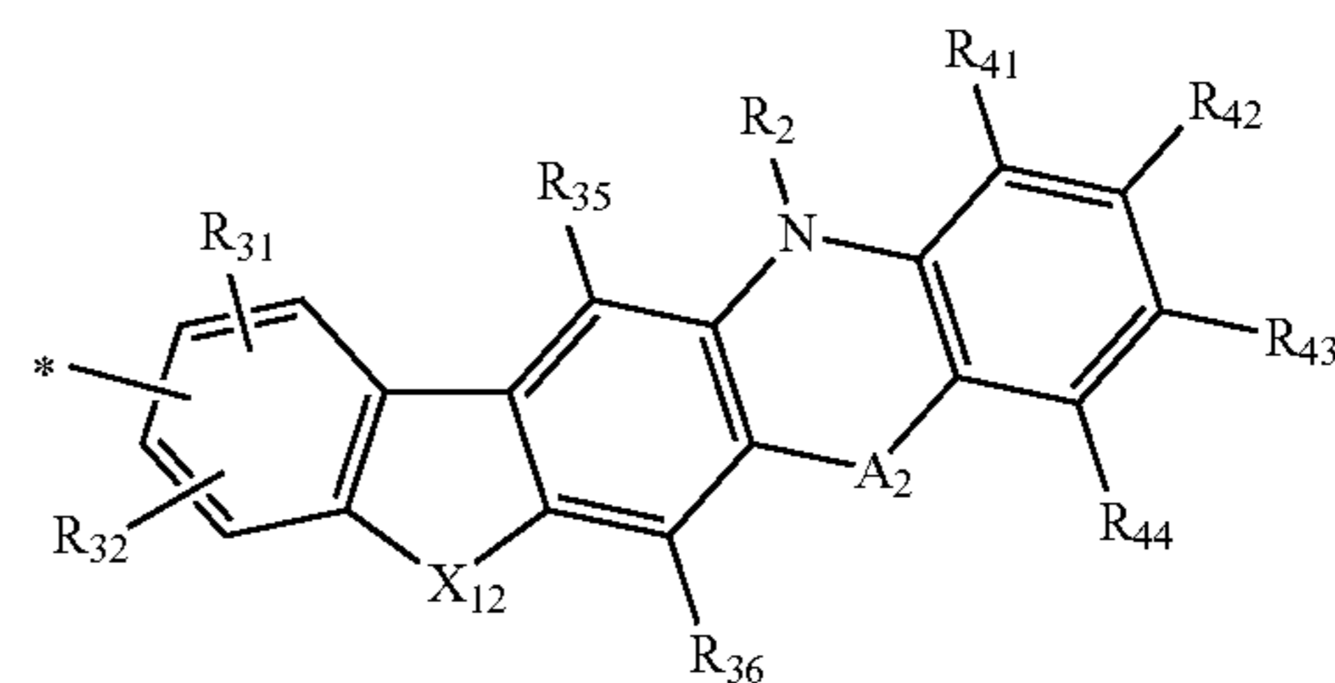
Formula 14-4
