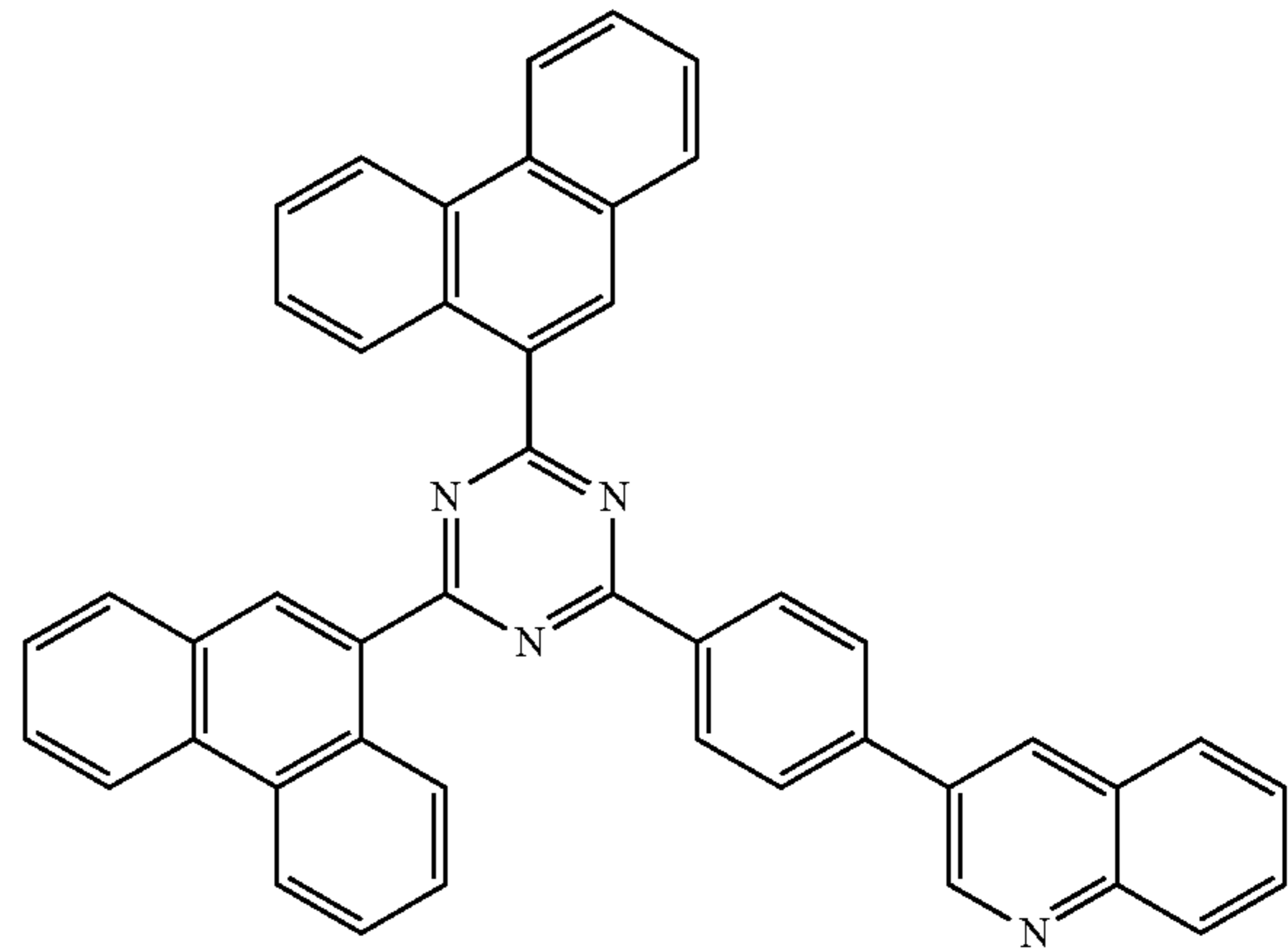
Compound ET14
