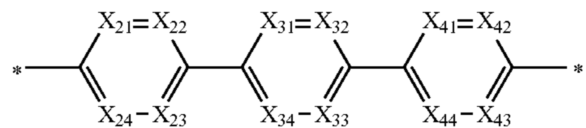
Formula 4-14
