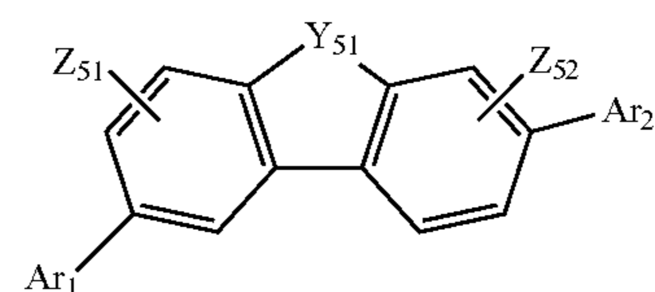
Formula D-1(3)
