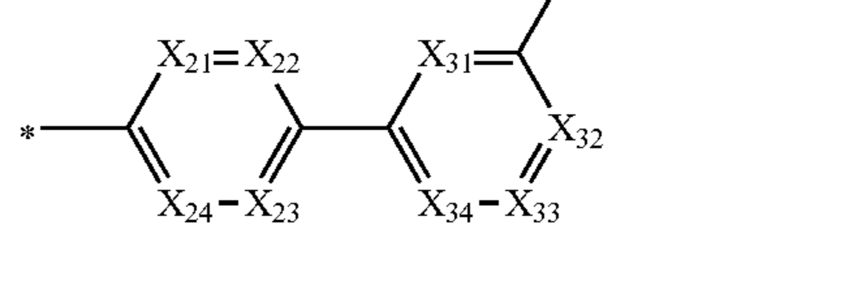
Formula 4-18
