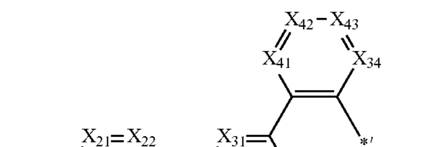
Formula 4-21
