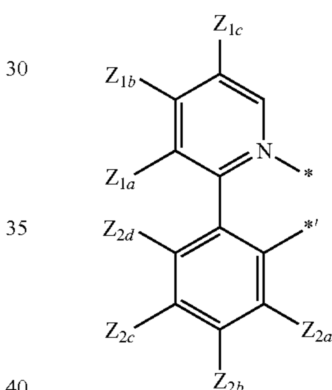
Formula 3-1(50)
