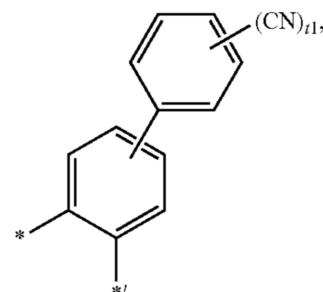
Formula 17-1 10
