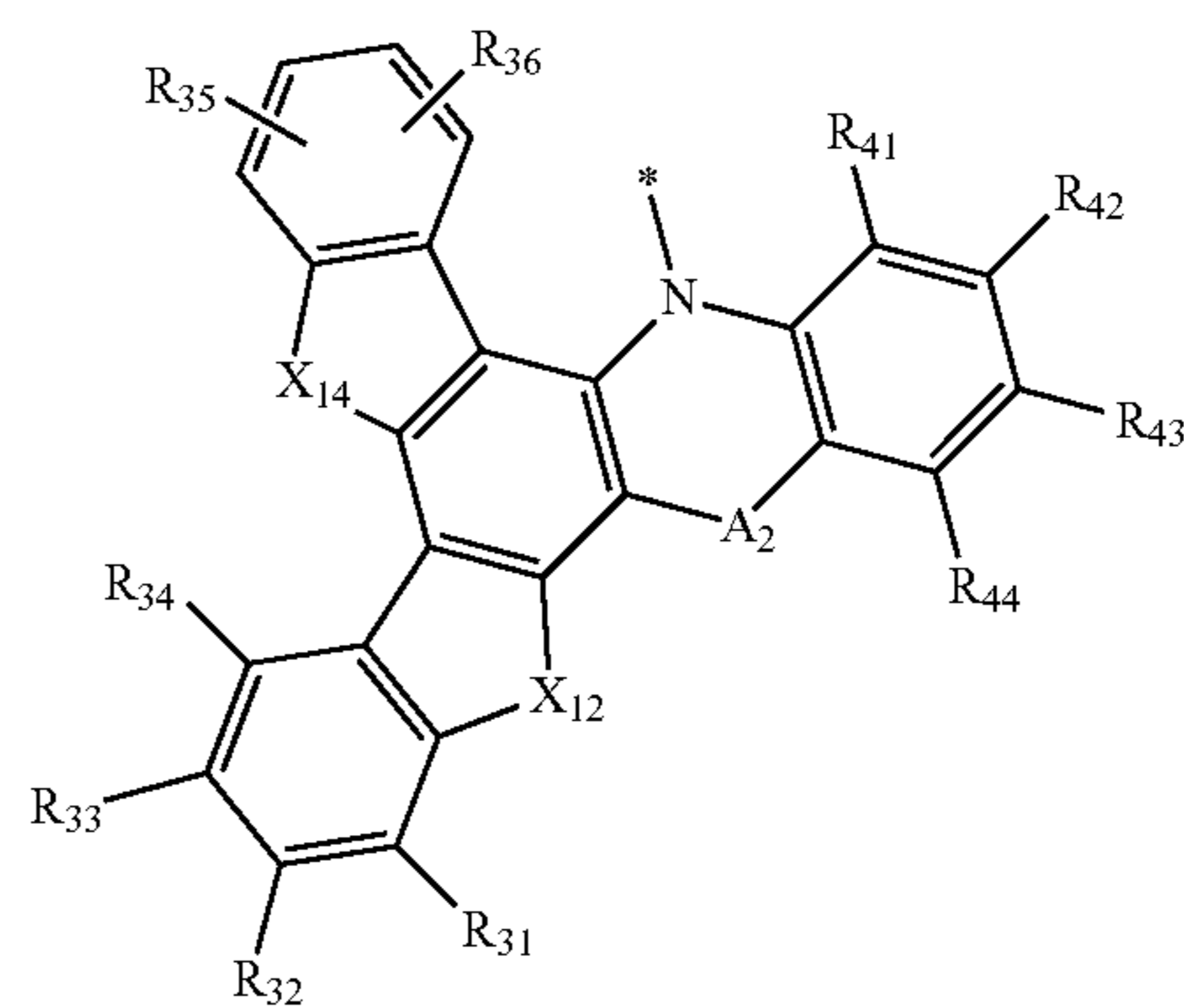
Formula 13-4
