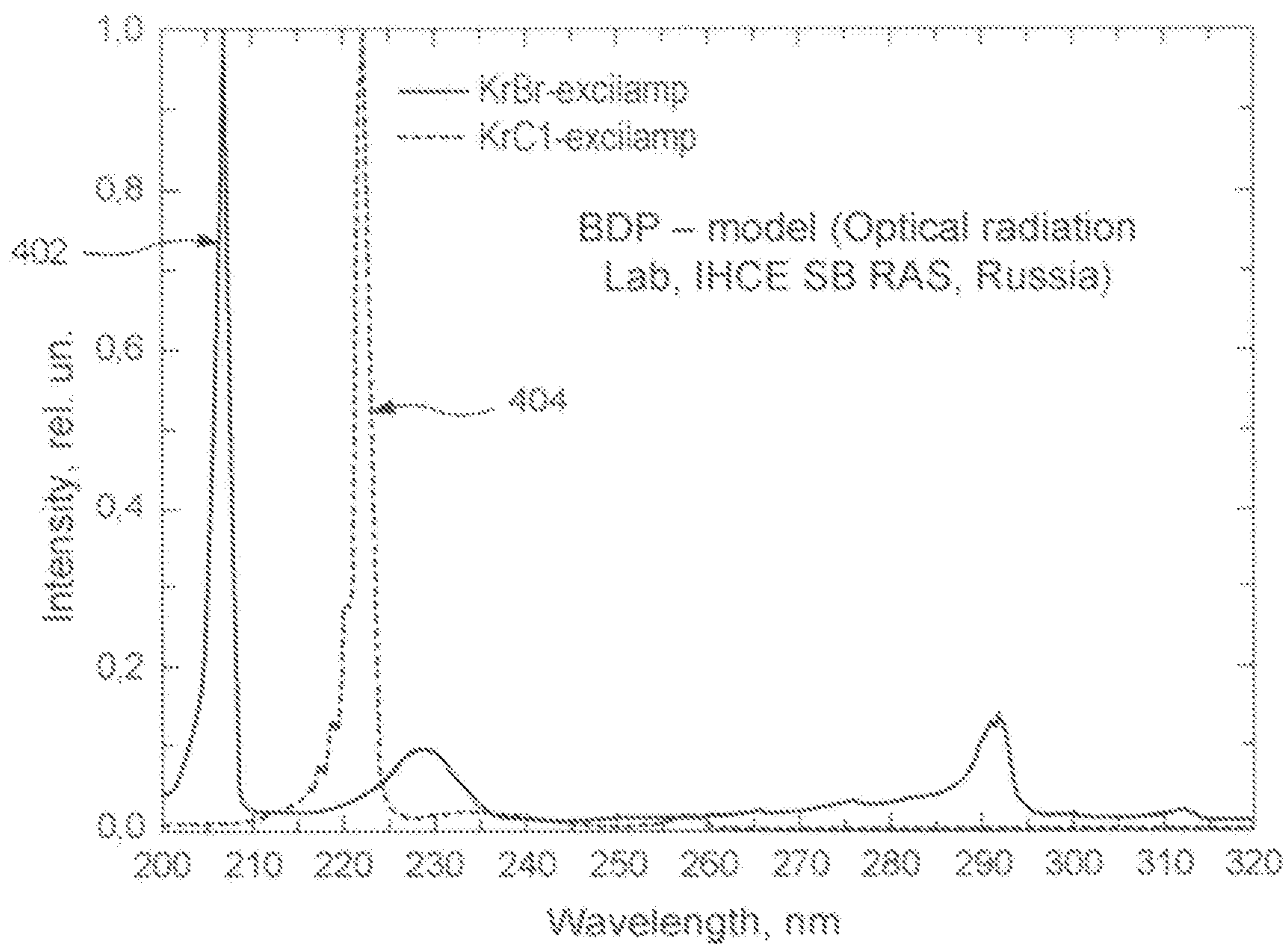
Spectral distribution of KrBr and KrCl excilamps in relative units
