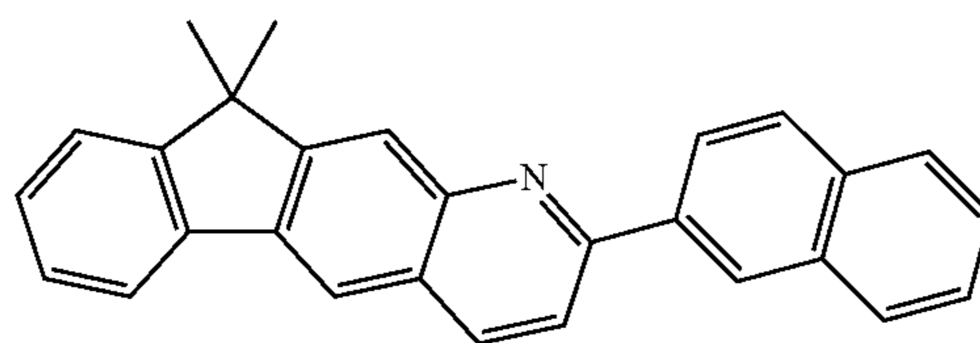
Compound Y
