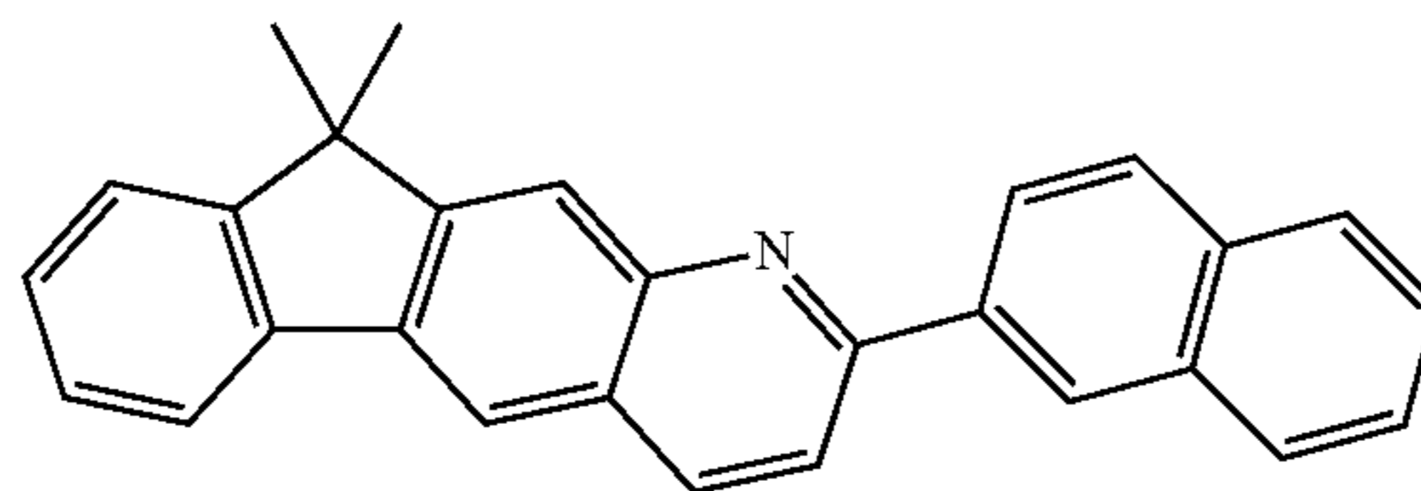
Compound Y
