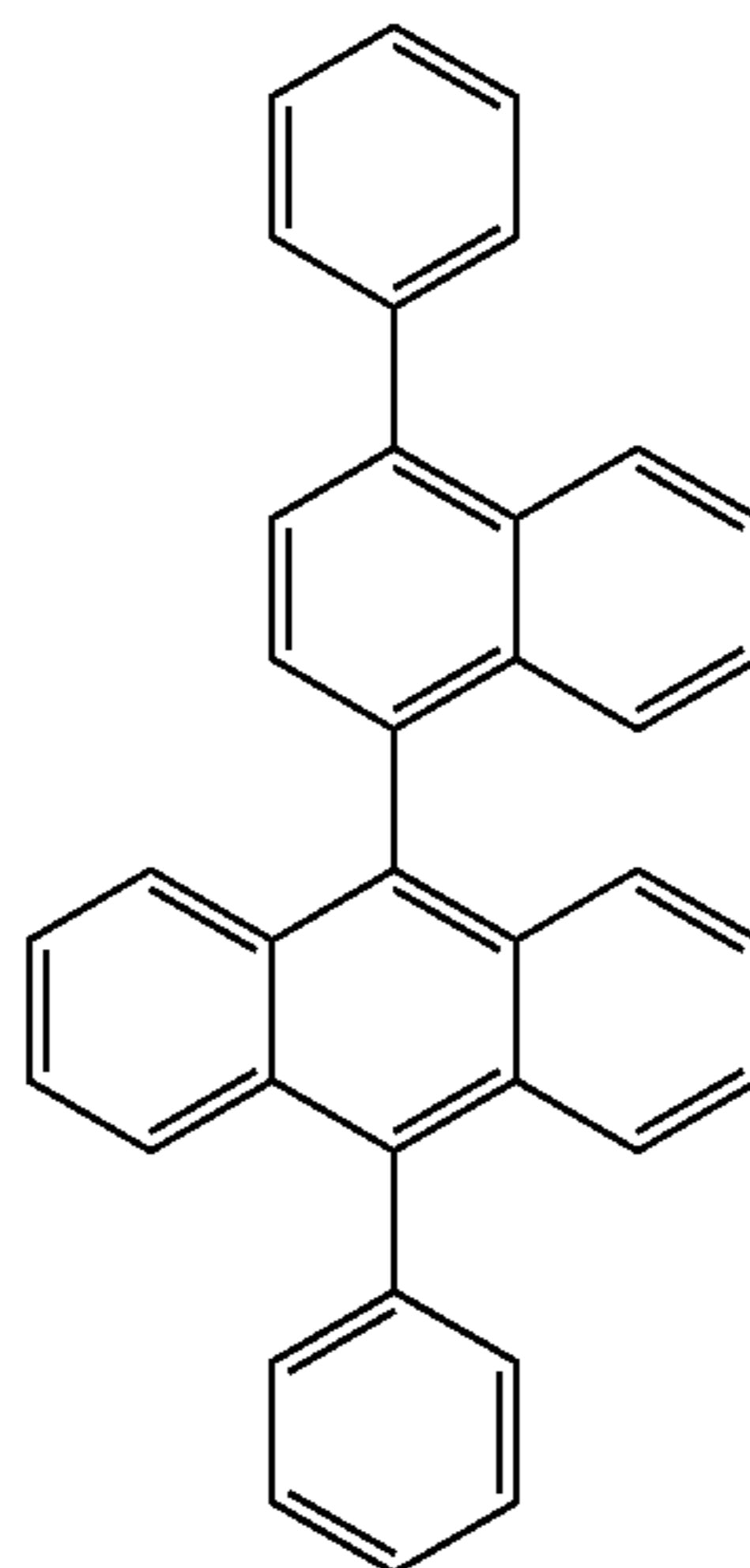
H-15
