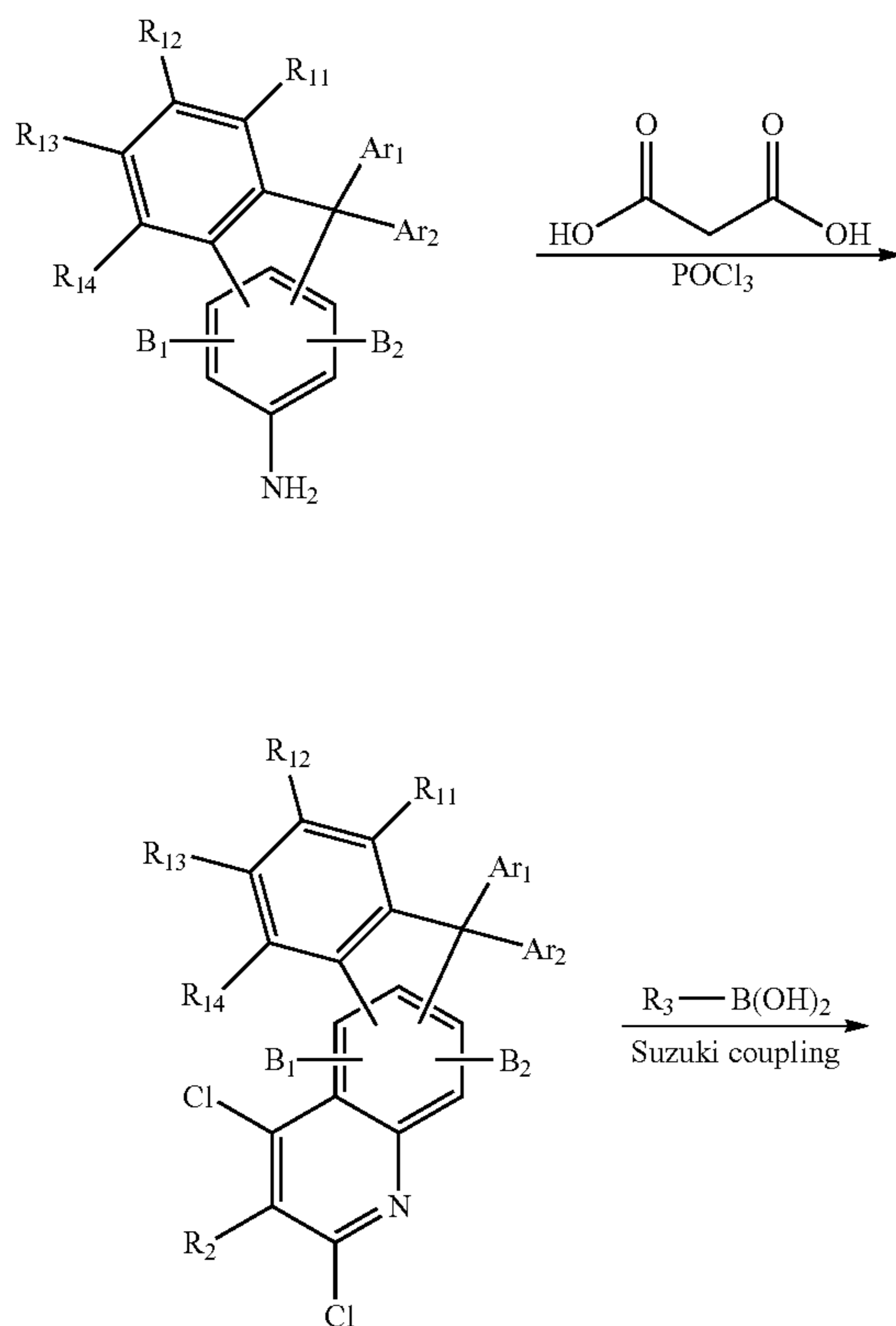
[Reaction Scheme 1]
