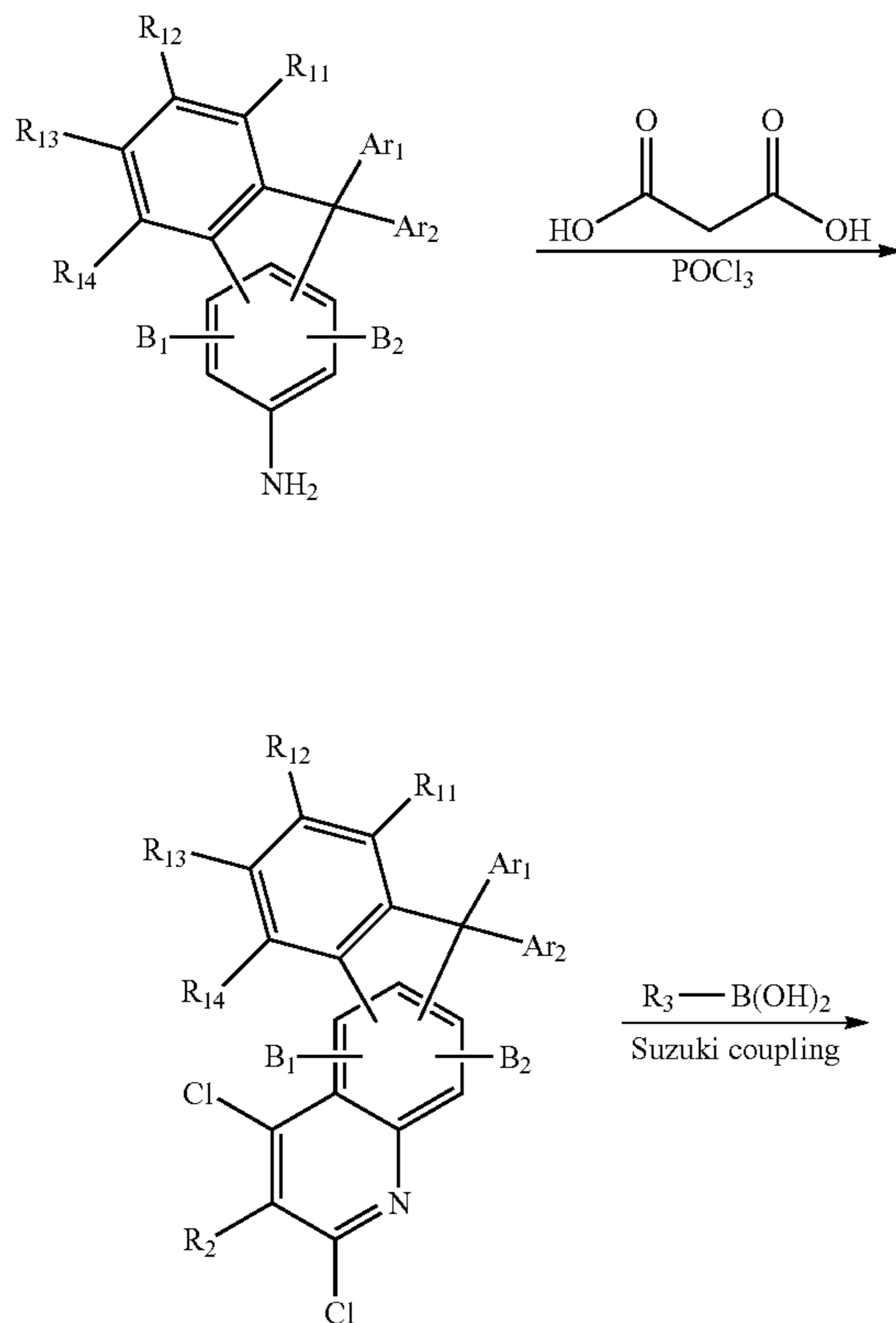
[Reaction Scheme 1]
