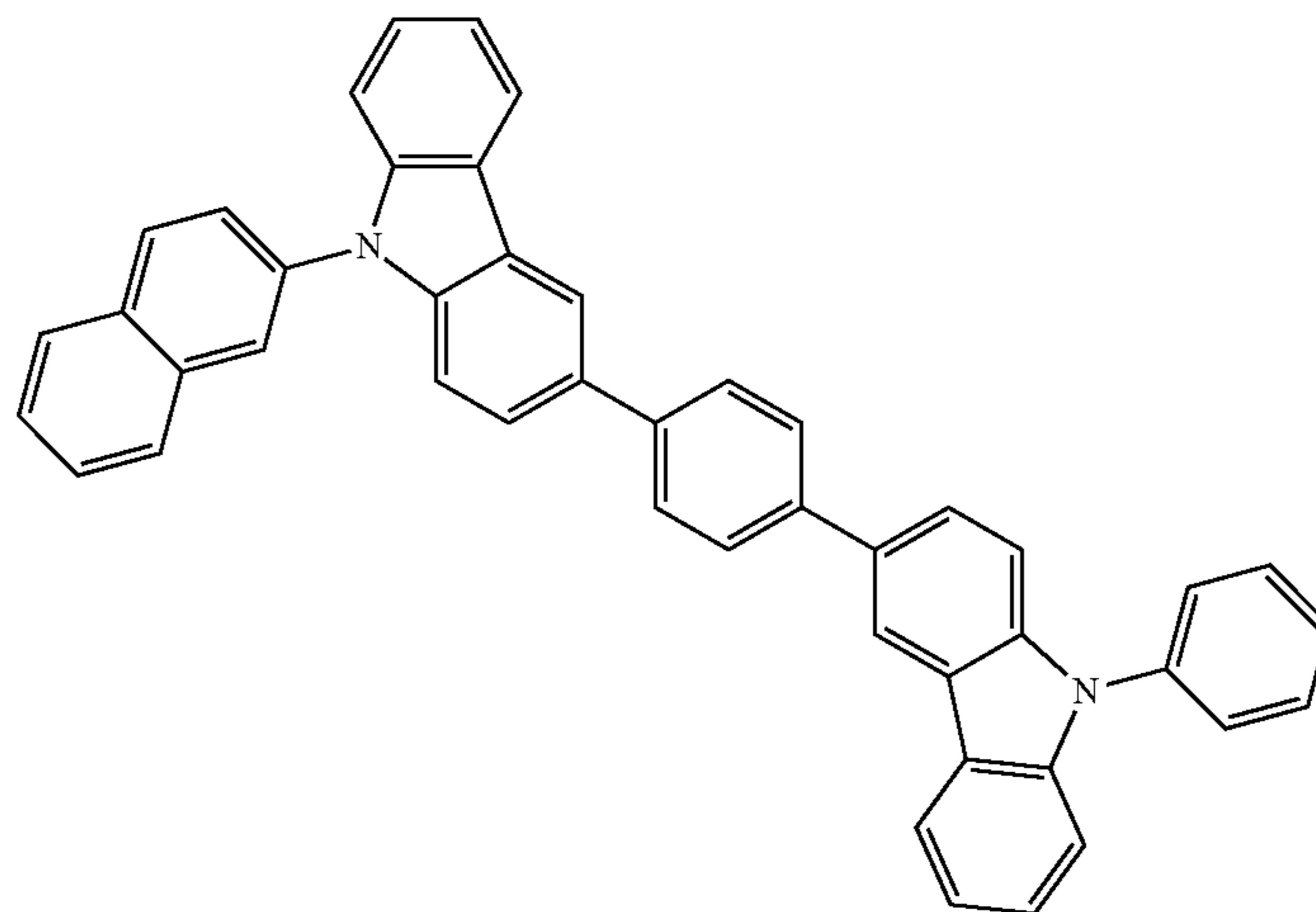
HT-2
